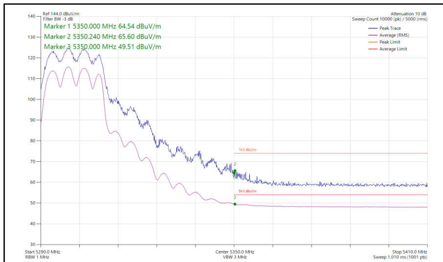
Figure 79 - 802.11n HT20, CDD, Core 0-1 - 5300 MHz Band Edge Frequency 5350 MHz
