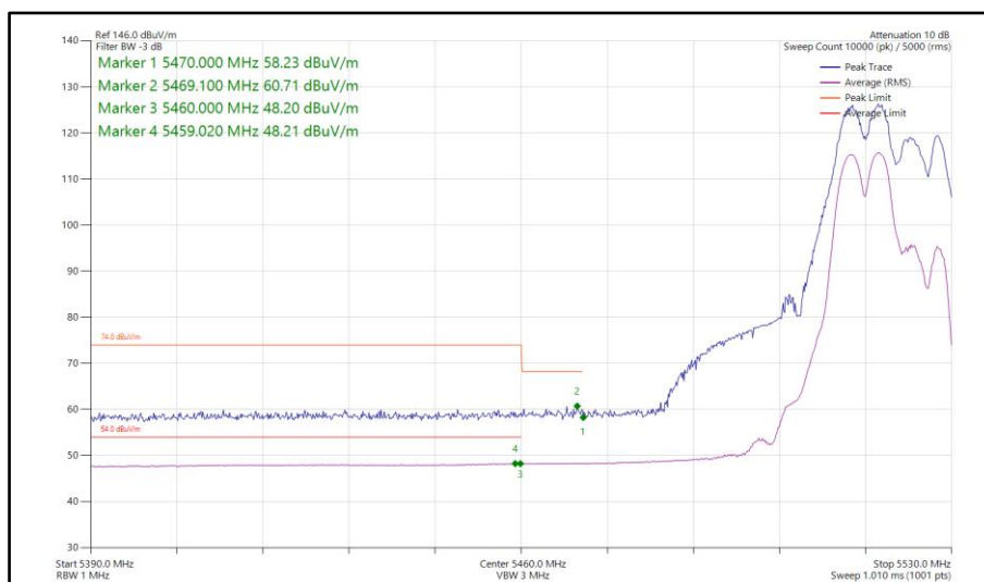
Figure 100 - 802.11be EHT20, CDD, RU 106+26-82, Core 0-1 - 5520 MHz Band Edge Frequency 5460 MHz
