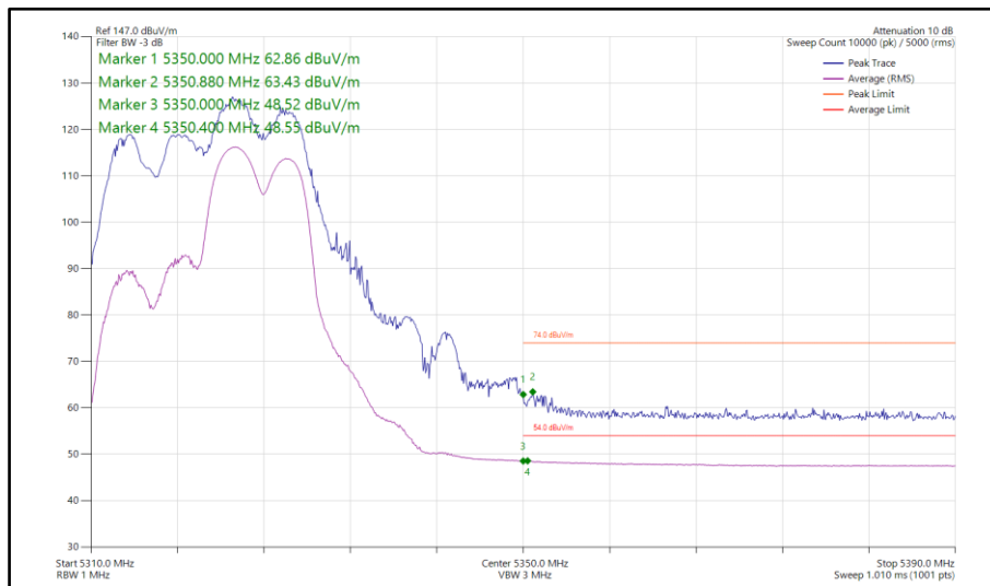
Figure 113 - 802.11ax HE20, RU 106-54, SDM, Core 0-1 - 5320 MHz Band Edge Frequency 5350 MHz
