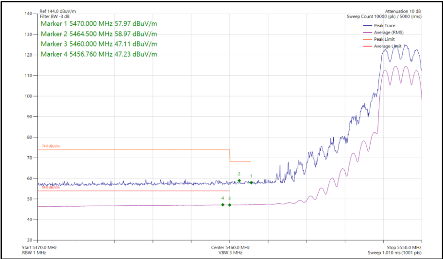
Figure 97 - 802.11ax HE20, SU, CDD, Core 0-1 - 5540 MHz Band Edge Frequency 5460 MHz
