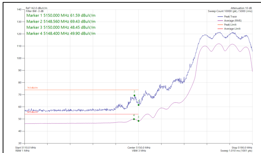
Figure 69 - 802.11n HT20, CDD, Core 0-1 - 5180 MHz Band Edge Frequency 5150 MHz
