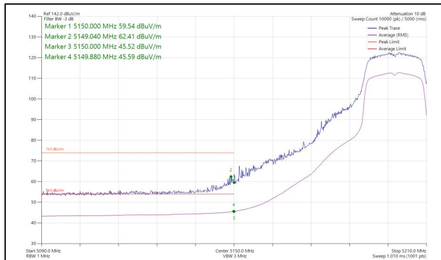
Figure 127 - 802.11ac VHT20, TxBF, Core 0-1 - 5200 MHz Band Edge Frequency 5150 MHz
