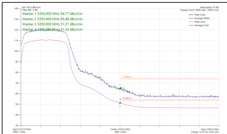
Figure 110 - 802.11n HT20, SDM, Core 0-1 - 5320 MHz Band Edge Frequency 5350 MHz
