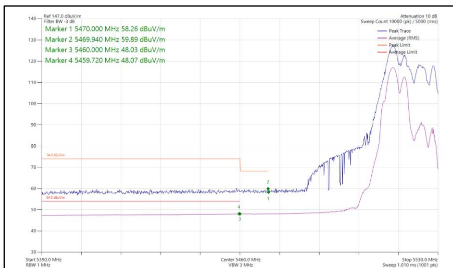
Figure 96 - 802.11ax HE20, RU 106-53, CDD, Core 0-1 - 5520 MHz Band Edge Frequency 5460 MHz
