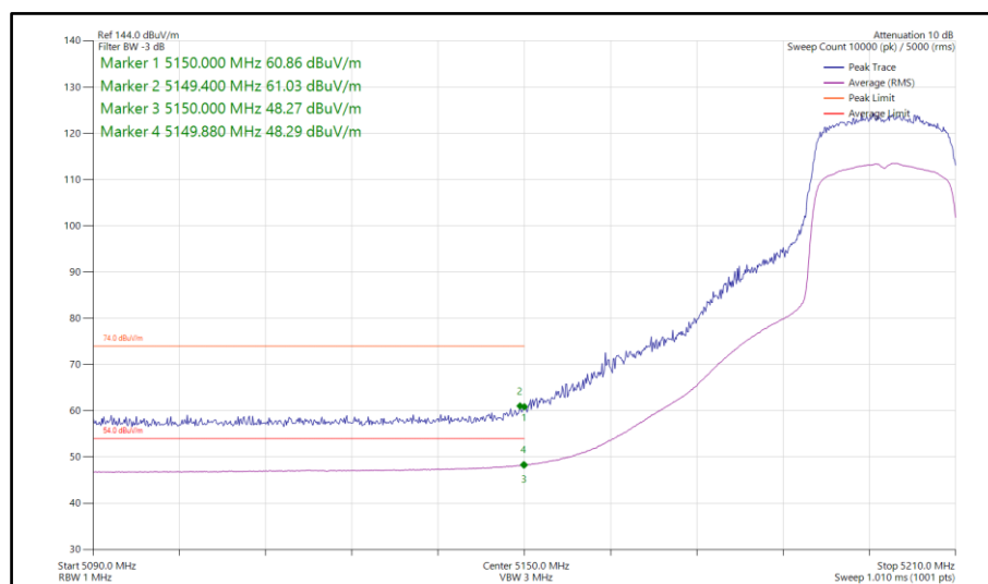
Figure 106 - 802.11ax HE20, SU, SDM, Core 0-1 - 5200 MHz Band Edge Frequency 5150 MHz
