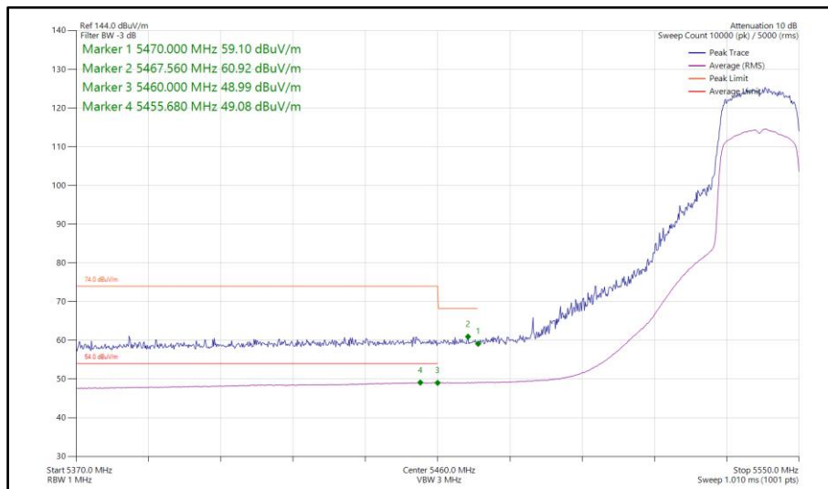
Figure 123 - 802.11ax HE20, SU, SDM, Core 0-1 - 5540 MHz Band Edge Frequency 5460 MHz
