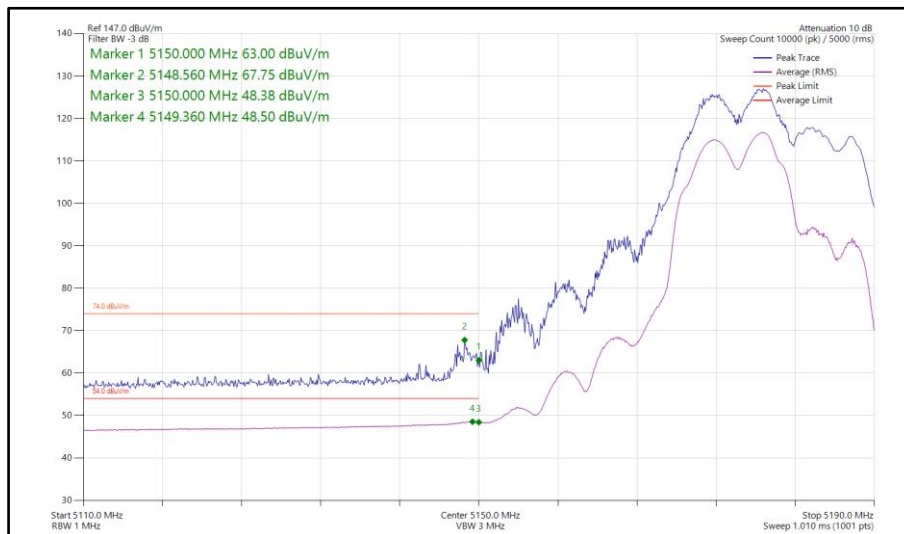
Figure 107 - 802.11be EHT20, RU 106+26-82, SDM, Core 0-1 - 5180 MHz Band Edge Frequency 5150 MHz
