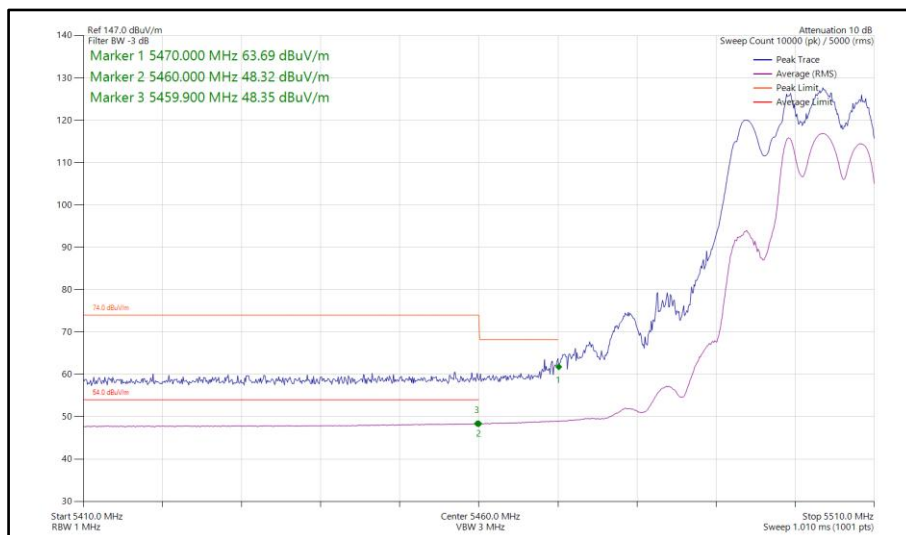
Figure 124 - 802.11be EHT20, RU 106+26-83, SDM, Core 0-1 - 5500 MHz Band Edge Frequency 5460 MHz
