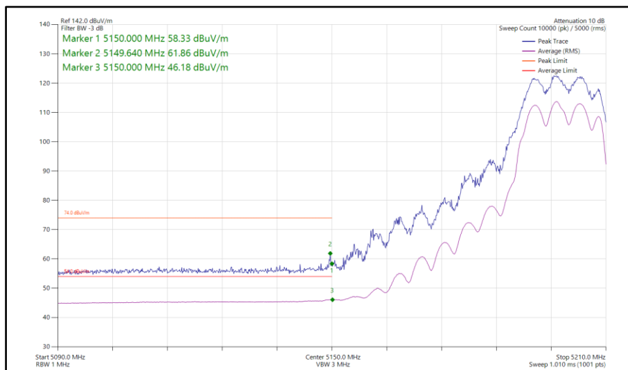
Figure 68 - 802.11a, CDD, Core 0-1 - 5200 MHz Band Edge Frequency 5150 MHz
