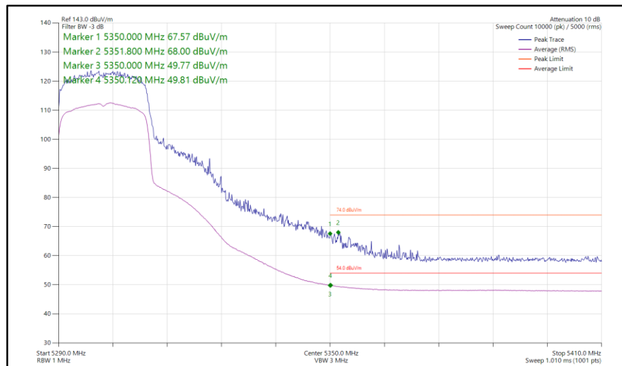
Figure 111 - 802.11ax HE20, SU, SDM, Core 0-1 - 5300 MHz Band Edge Frequency 5350 MHz
