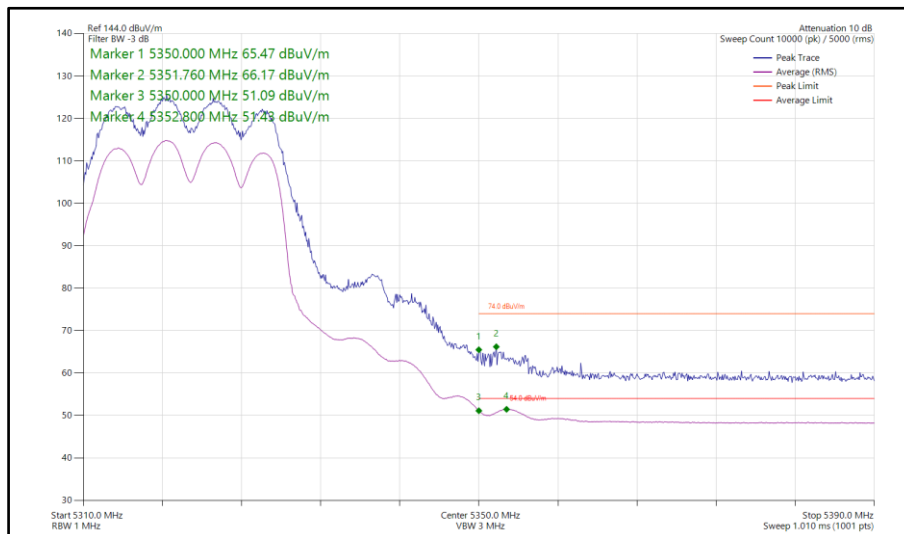
Figure 83 - 802.11ax HE20, SU, CDD, Core 0-1 - 5320 MHz Band Edge Frequency 5350 MHz
