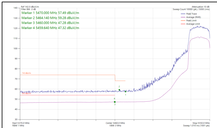
Figure 64 - 802.11ax HE20, SU, SISO, Core 1 - 5540 MHz Band Edge Frequency 5460 MHz
