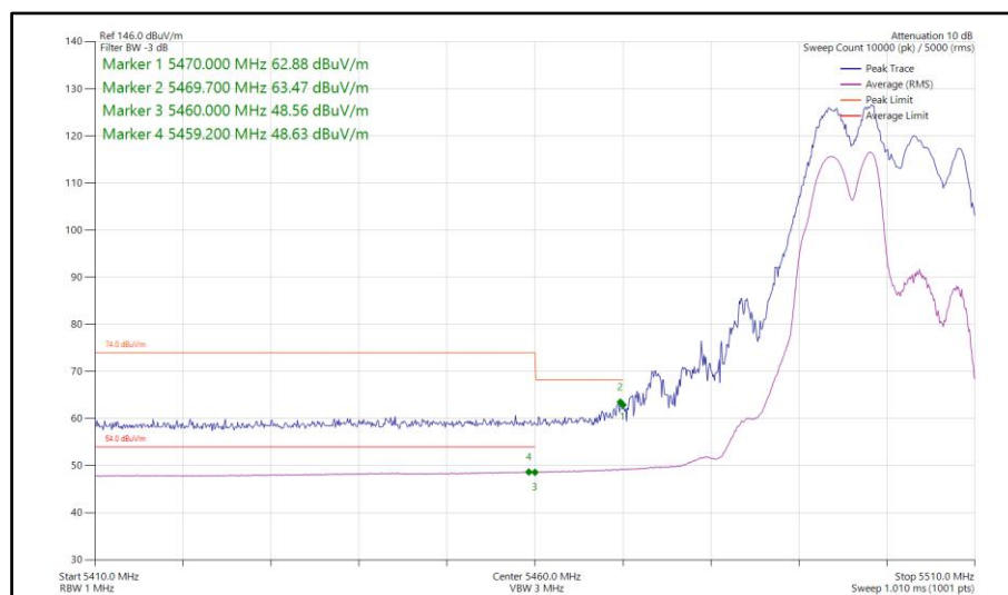
Figure 94 - 802.11ax HE20, RU 106-53, CDD, Core 0-1 - 5500 MHz Band Edge Frequency 5460 MHz
