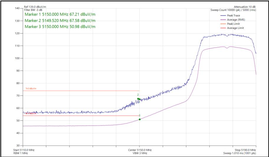
Figure 101 - 802.11n HT20, SDM, Core 0-1 - 5180 MHz Band Edge Frequency 5150 MHz
