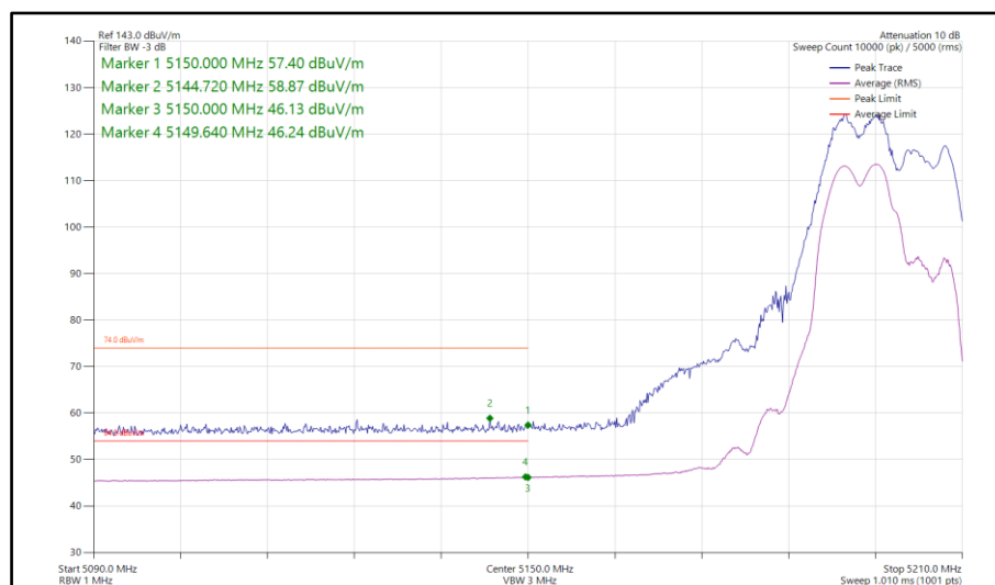
Figure 76 - 802.11be EHT20, RU 106+26-82, CDD, Core 0-1 - 5200 MHz Band Edge Frequency 5150 MHz
