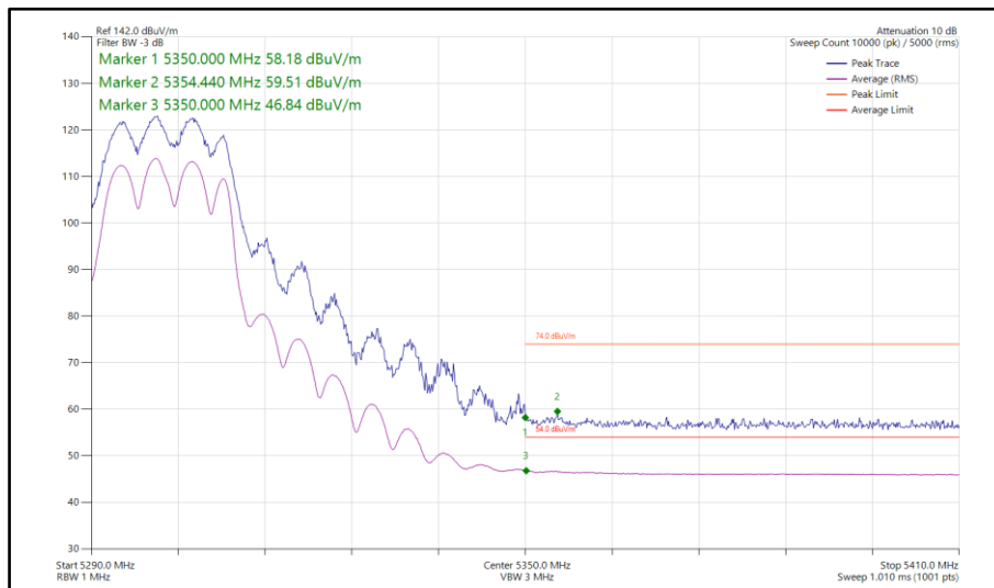
Figure 77 - 802.11a, CDD, Core 0-1 - 5300 MHz Band Edge Frequency 5350 MHz
