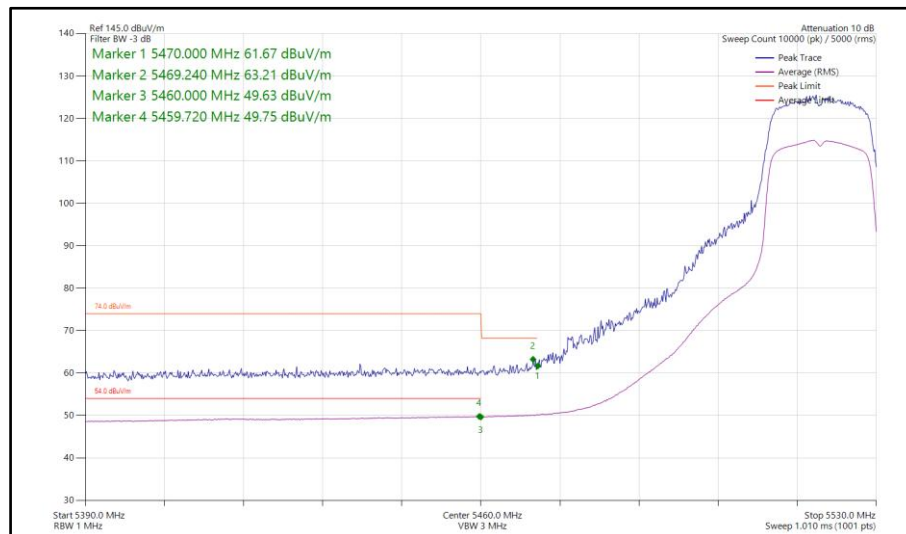
Figure 117 - 802.11n HT20, SDM, Core 0-1 - 5520 MHz Band Edge Frequency 5460 MHz
