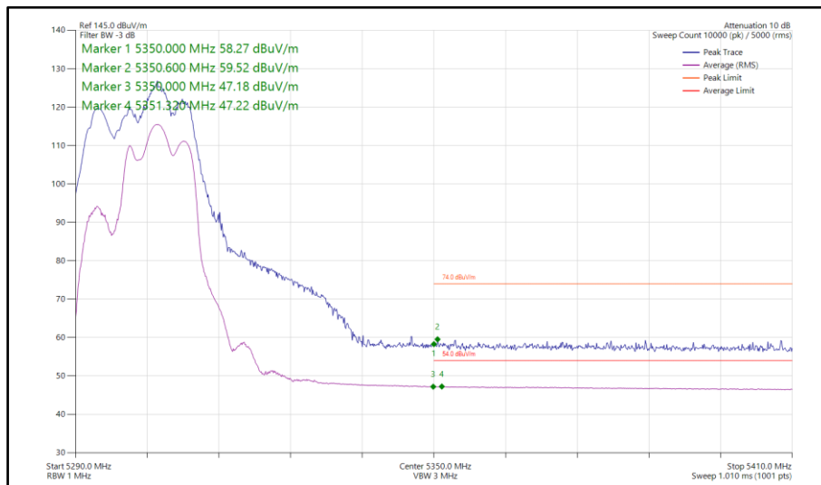
Figure 85 - 802.11be EHT20, RU 106+26-83, CDD, Core 0-1 - 5300 MHz Band Edge Frequency 5350 MHz
