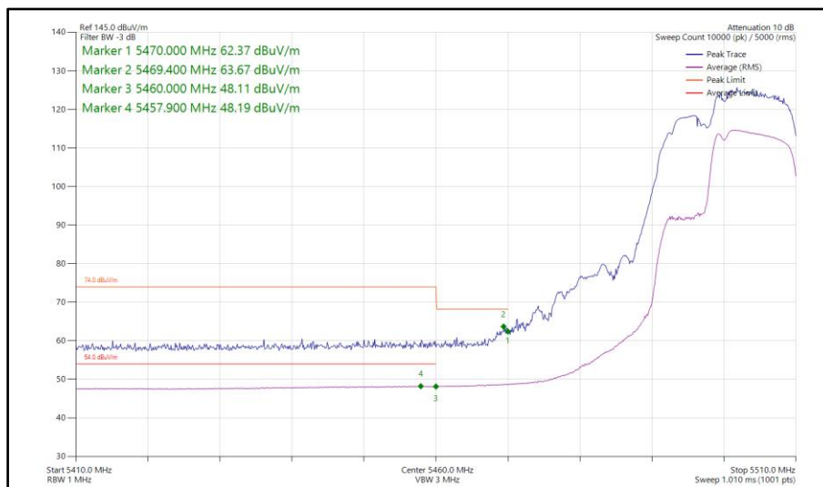
Figure 65 - 802.11be EHT20, RU 106+26-83, SISO, Core 1 - 5500 MHz Band Edge Frequency 5460 MHz
