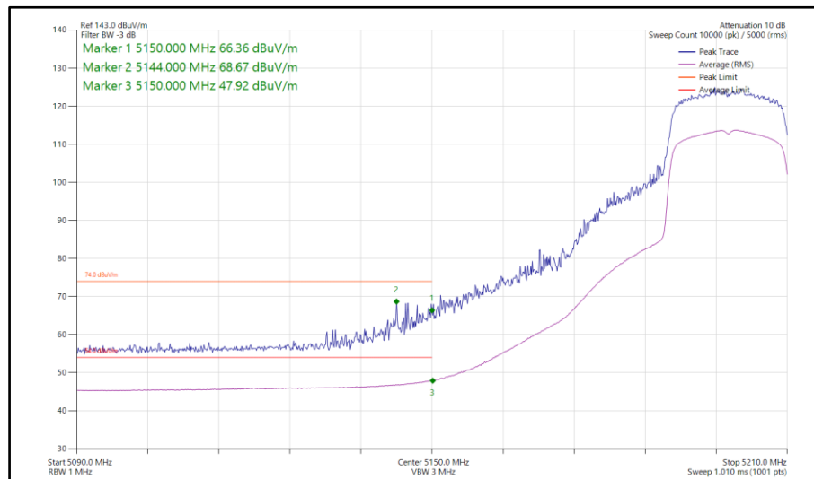
Figure 129 - 802.11ax HE20, SU, TxBF, Core 0-1 - 5200 MHz Band Edge Frequency 5150 MHz
