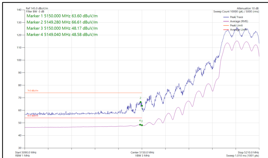
Figure 73 - 802.11ax HE20, SU, CDD, Core 0-1 - 5200 MHz Band Edge Frequency 5150 MHz
