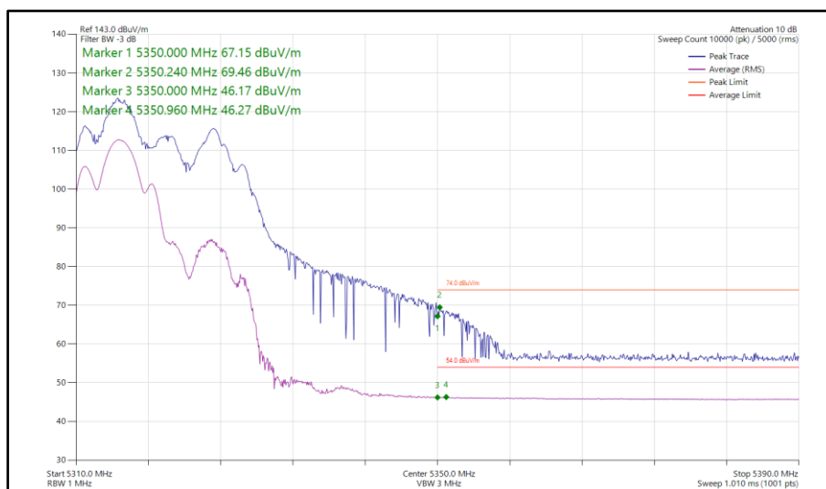
Figure 84 - 802.11ax HE20, RU 106-53, CDD, Core 0-1 - 5320 MHz Band Edge Frequency 5350 MHz
