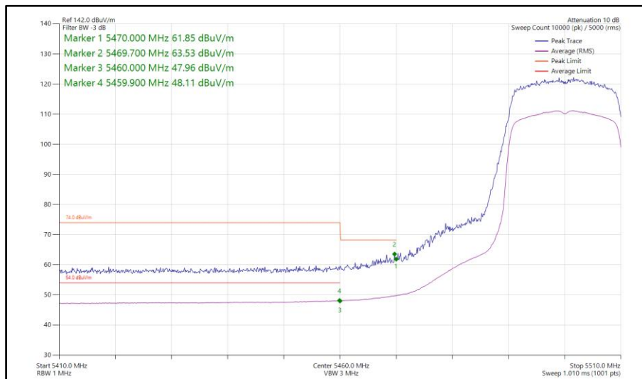
Figure 119 - 802.11ax HE20, SU, SDM, Core 0-1 - 5500 MHz Band Edge Frequency 5460 MHz
