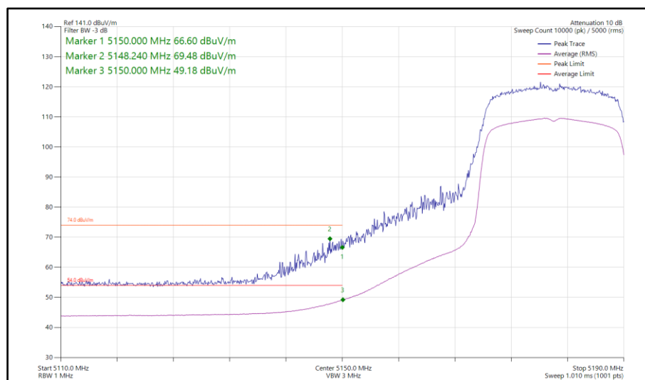
Figure 128 - 802.11ax HE20, SU, TxBF, Core 0-1 - 5180 MHz Band Edge Frequency 5150 MHz
