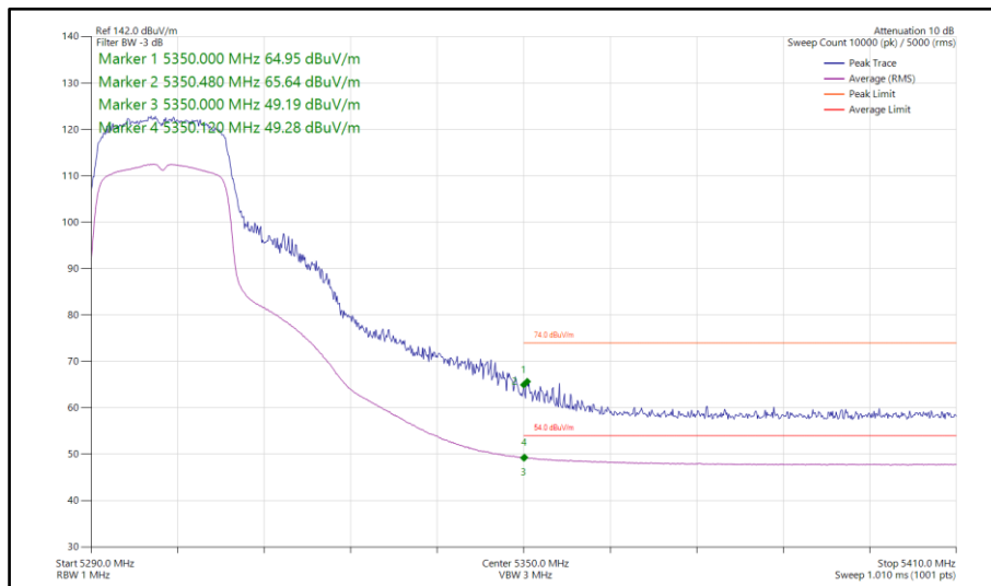
Figure 109 - 802.11n HT20, SDM, Core 0-1 - 5300 MHz Band Edge Frequency 5350 MHz
