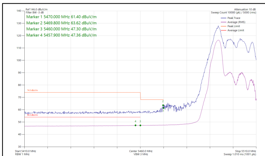
Figure 120 - 802.11ax HE20, RU 52-37, SDM, Core 0-1 - 5500 MHz Band Edge Frequency 5460 MHz
