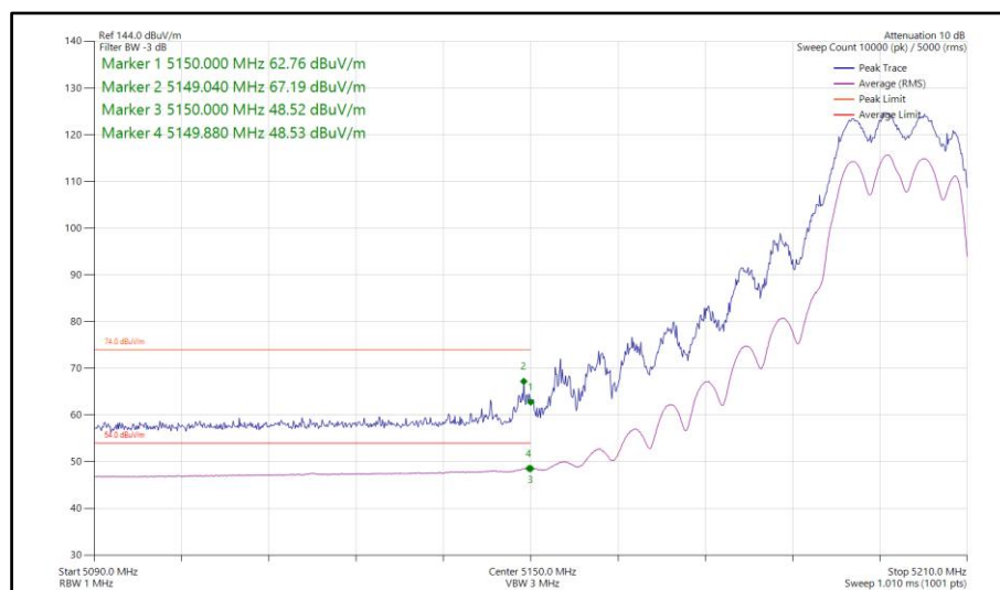
Figure 70 - 802.11n HT20, CDD, Core 0-1 - 5200 MHz Band Edge Frequency 5150 MHz
