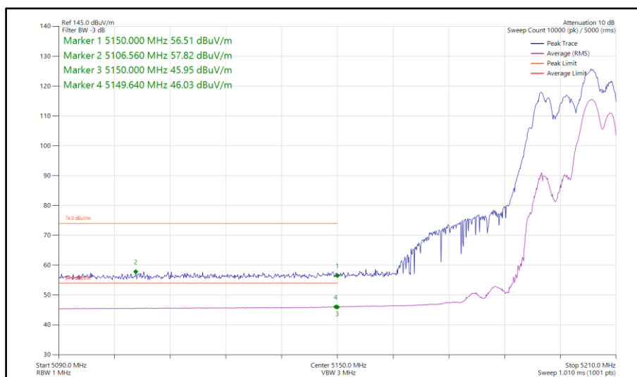
Figure 74 - 802.11ax HE20, RU 106-54, CDD, Core 0-1 - 5200 MHz Band Edge Frequency 5150 MHz
