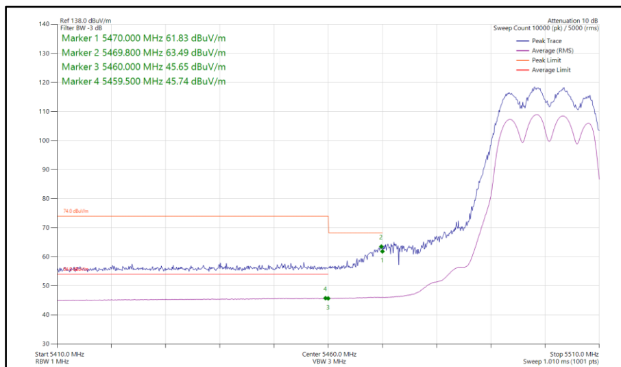
Figure 90 - 802.11n HT20, CDD, Core 0-1 - 5500 MHz Band Edge Frequency 5460 MHz
