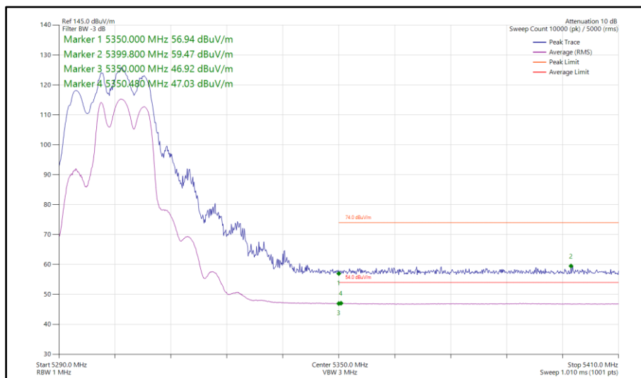
Figure 114 - 802.11be EHT20, RU 106+26-83, SDM, Core 0-1 - 5300 MHz Band Edge Frequency 5350 MHz
