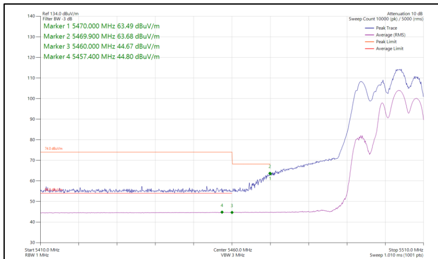
Figure 99 - 802.11be EHT20, RU 106+26-83, CDD, Core 0-1 - 5500 MHz Band Edge Frequency 5460 MHz
