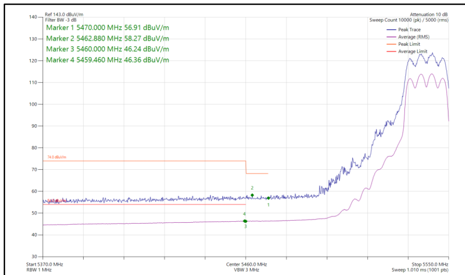
Figure 89 - 802.11a, CDD, Core 0-1 - 5540 MHz Band Edge Frequency 5460 MHz
