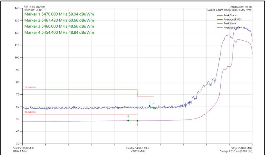
Figure 66 - 802.11be EHT20, RU 106+26-83, SISO, Core 1 - 5520 MHz Band Edge Frequency 5460 MHz
