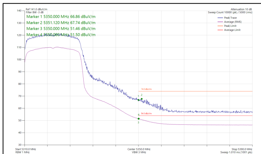
Figure 112 - 802.11ax HE20, SU, SDM, Core 0-1 - 5320 MHz Band Edge Frequency 5350 MHz
