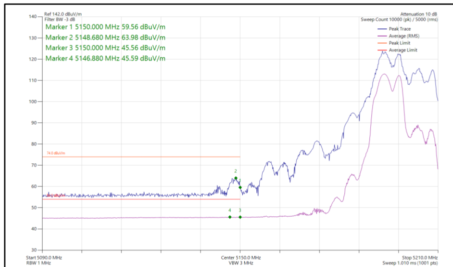
Figure 105 - 802.11ax HE20, RU 106-53, SDM, Core 0-1 - 5200 MHz Band Edge Frequency 5150 MHz
