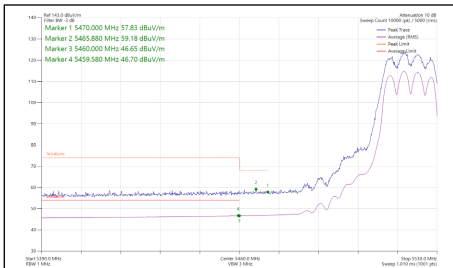
Figure 88 - 802.11a, CDD, Core 0-1 - 5520 MHz Band Edge Frequency 5460 MHz
