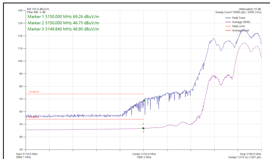
Figure 72 - 802.11ax HE20, RU 106-54, CDD, Core 0-1 - 5180 MHz Band Edge Frequency 5150 MHz
