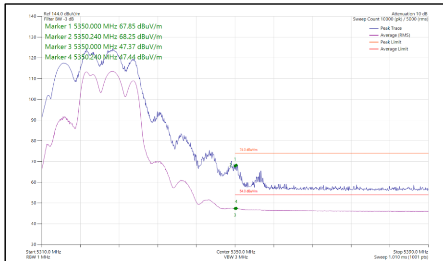
Figure 115 - 802.11be EHT20, RU 106+26-83, SDM, Core 0-1 - 5320 MHz Band Edge Frequency 5350 MHz
