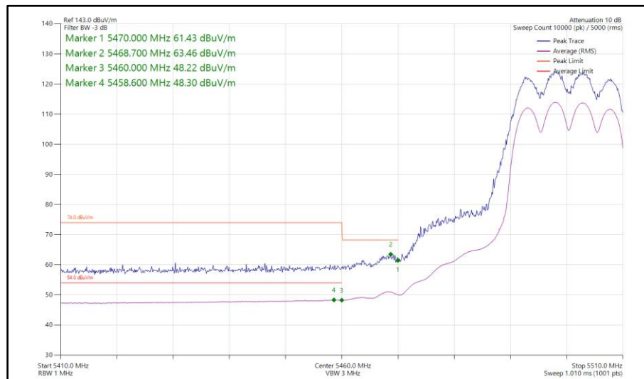
Figure 93 - 802.11ax HE20, SU, CDD, Core 0-1 - 5500 MHz Band Edge Frequency 5460 MHz
