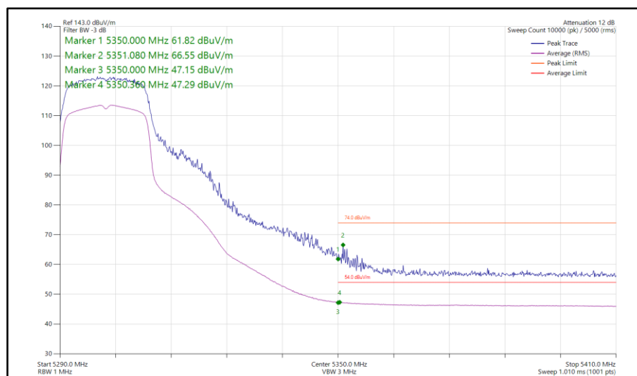
Figure 130 - 802.11ac VHT20, TxBF, Core 0-1 - 5300 MHz Band Edge Frequency 5350 MHz
