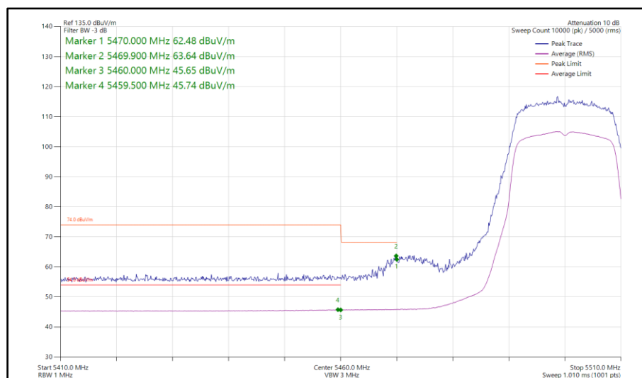
Figure 116 - 802.11n HT20, SDM, Core 0-1 - 5500 MHz Band Edge Frequency 5460 MHz
