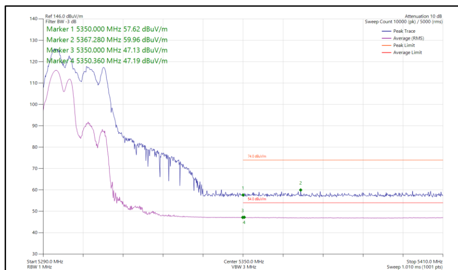
Figure 82 - 802.11ax HE20, RU 106-53, CDD, Core 0-1 - 5300 MHz Band Edge Frequency 5350 MHz
