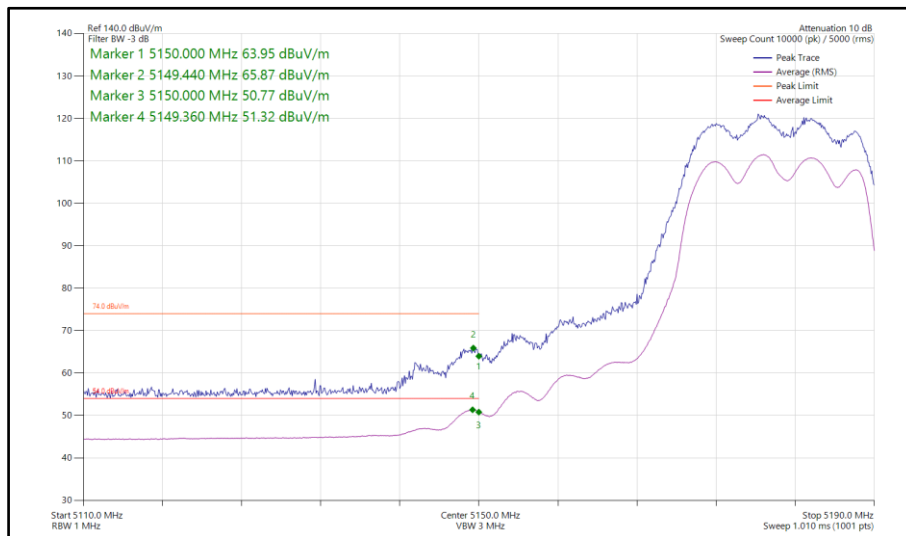
Figure 67 - 802.11a, CDD, Core 0-1 - 5180 MHz Band Edge Frequency 5150 MHz
