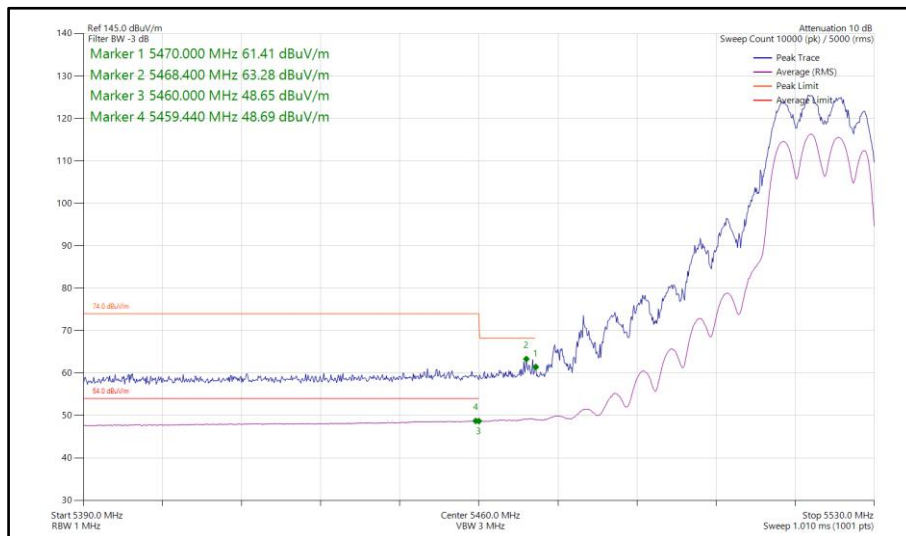
Figure 91 - 802.11n HT20, CDD, Core 0-1 - 5520 MHz Band Edge Frequency 5460 MHz
