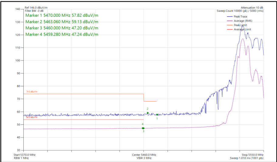
Figure 98 - 802.11ax HE20, RU 106-53, CDD, Core 0-1 - 5540 MHz Band Edge Frequency 5460 MHz
