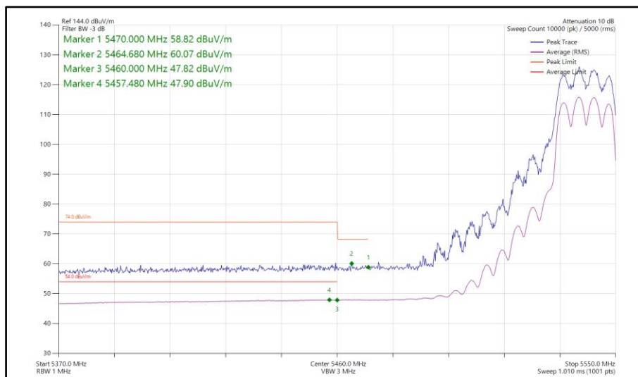
Figure 92 - 802.11n HT20, CDD, Core 0-1 - 5540 MHz Band Edge Frequency 5460 MHz
