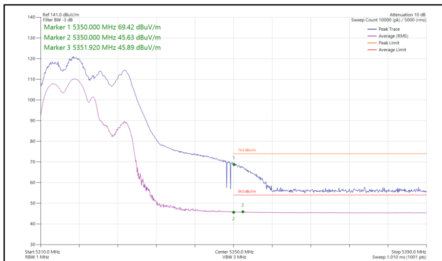
Figure 86 - 802.11be EHT20, RU 106+26-82, CDD, Core 0-1 - 5320 MHz Band Edge Frequency 5350 MHz
