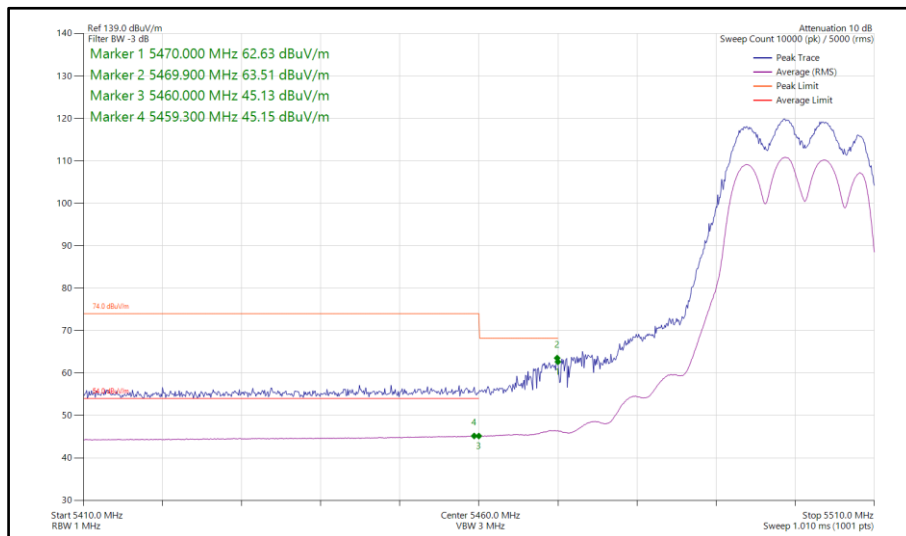
Figure 87 - 802.11a, CDD, Core 0-1 - 5500 MHz Band Edge Frequency 5460 MHz
