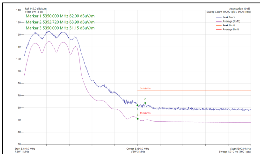
Figure 80 - 802.11n HT20, CDD, Core 0-1 - 5320 MHz Band Edge Frequency 5350 MHz
