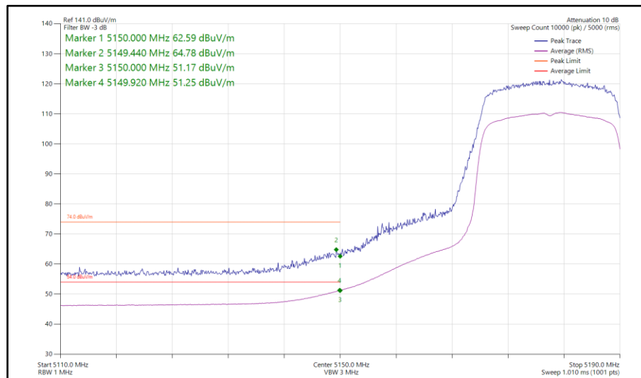
Figure 103 - 802.11ax HE20, SU, SDM, Core 0-1 - 5180 MHz Band Edge Frequency 5150 MHz
