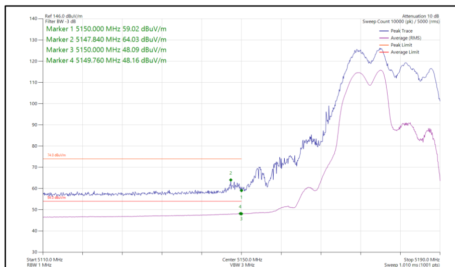
Figure 104 - 802.11ax HE20, RU 106-53, SDM, Core 0-1 - 5180 MHz Band Edge Frequency 5150 MHz
