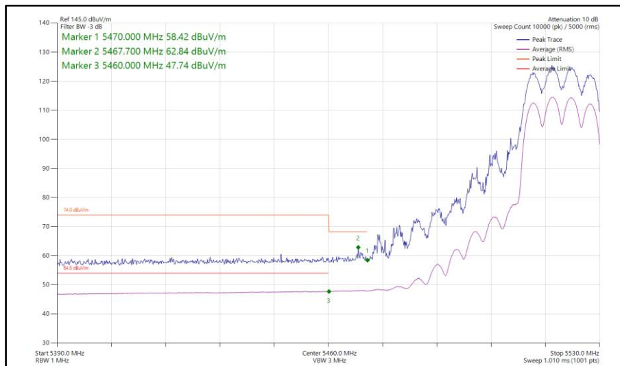
Figure 95 - 802.11ax HE20, SU, CDD, Core 0-1 - 5520 MHz Band Edge Frequency 5460 MHz
