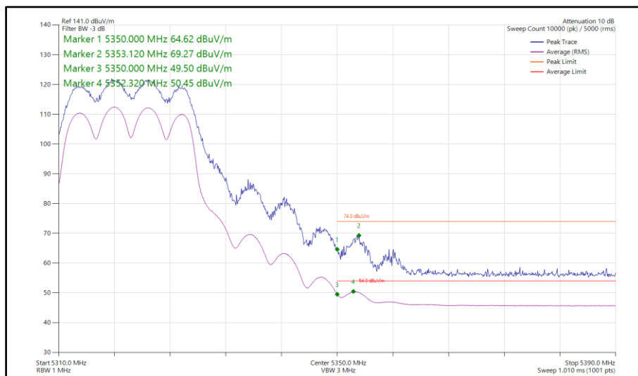
Figure 78 - 802.11a, CDD, Core 0-1 - 5320 MHz Band Edge Frequency 5350 MHz
