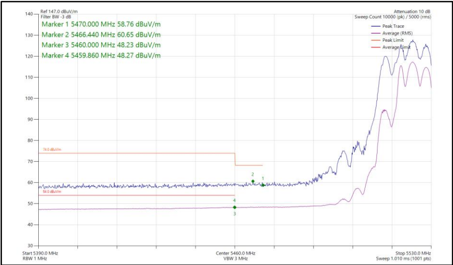
Figure 125 - 802.11be EHT20, RU 106+26-83, SDM, Core 0-1 - 5520 MHz Band Edge Frequency 5460 MHz
