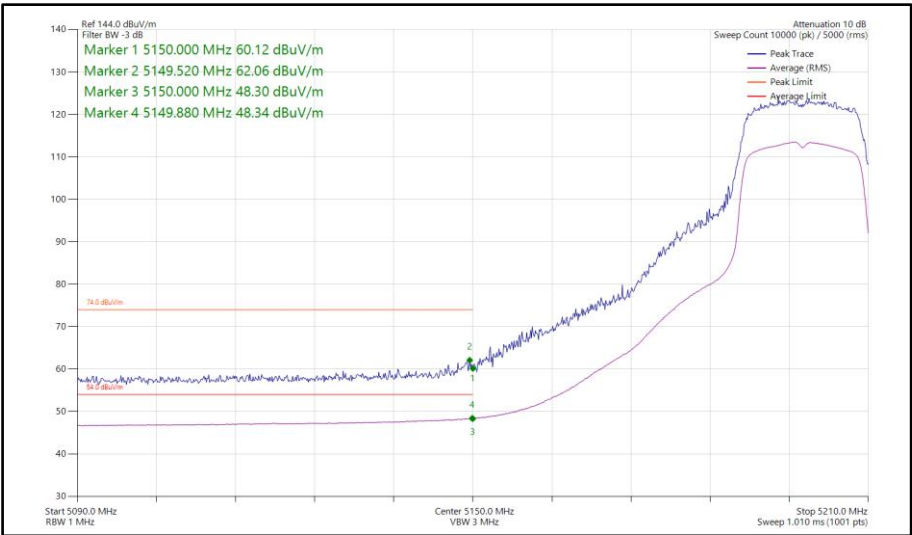
Figure 102 - 802.11n HT20, SDM, Core 0-1 - 5200 MHz Band Edge Frequency 5150 MHz
