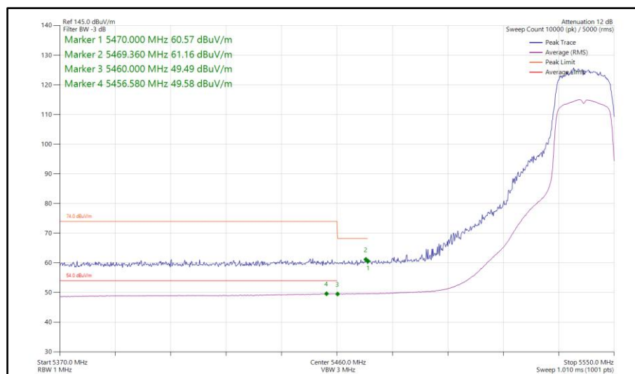
Figure 118 - 802.11n HT20, SDM, Core 0-1 - 5540 MHz Band Edge Frequency 5460 MHz
