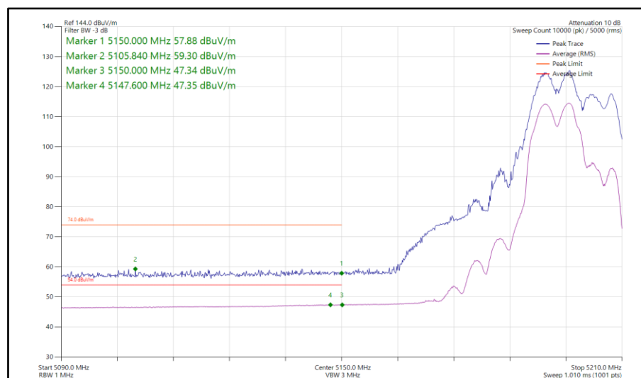
Figure 108 - 802.11be EHT20, RU 106+26-82, SDM, Core 0-1 - 5200 MHz Band Edge Frequency 5150 MHz
