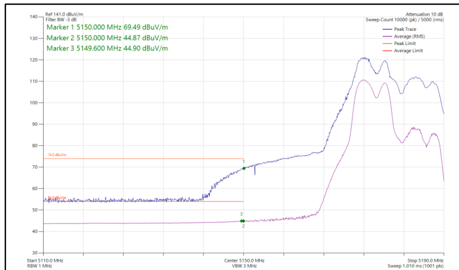
Figure 75 - 802.11be EHT20, RU 52+26-70, CDD, Core 0-1 - 5180 MHz Band Edge Frequency 5150 MHz
