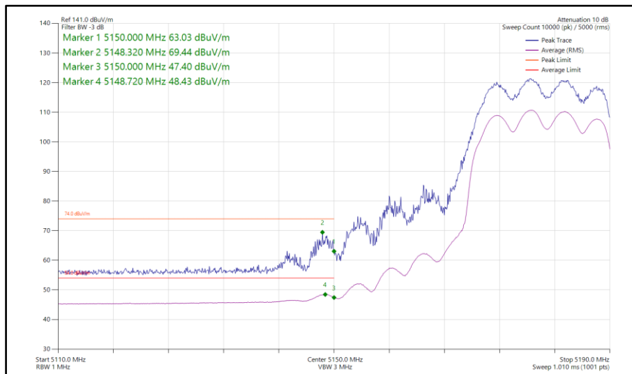
Figure 71 - 802.11ax HE20, SU, CDD, Core 0-1 - 5180 MHz Band Edge Frequency 5150 MHz
