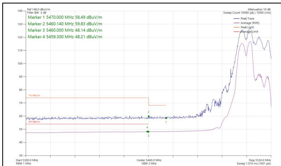
Figure 122 - 802.11ax HE20, RU 106-53, SDM, Core 0-1 - 5520 MHz Band Edge Frequency 5460 MHz
