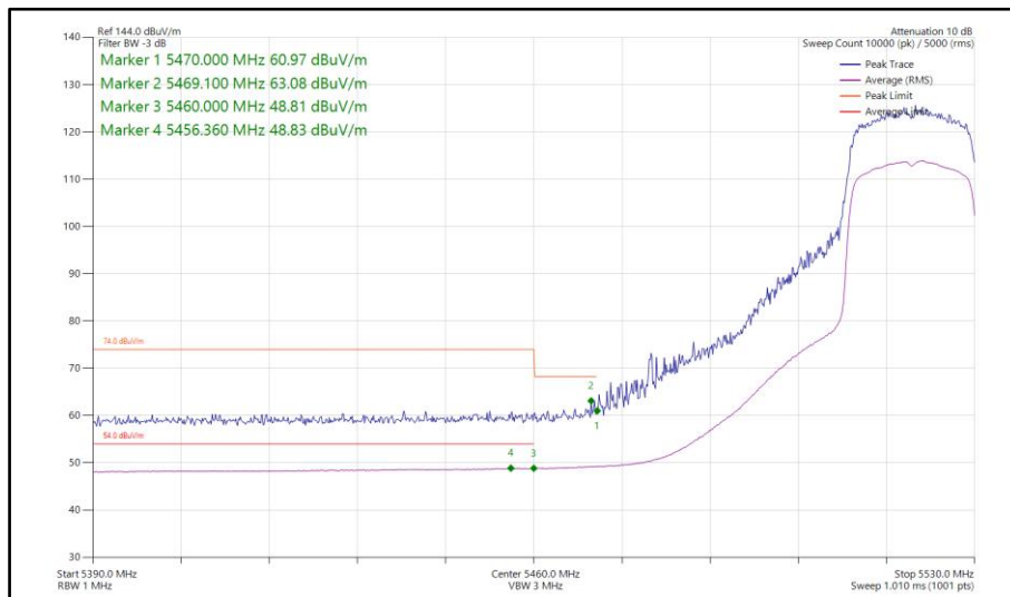
Figure 121 - 802.11ax HE20, SU, SDM, Core 0-1 - 5520 MHz Band Edge Frequency 5460 MHz
