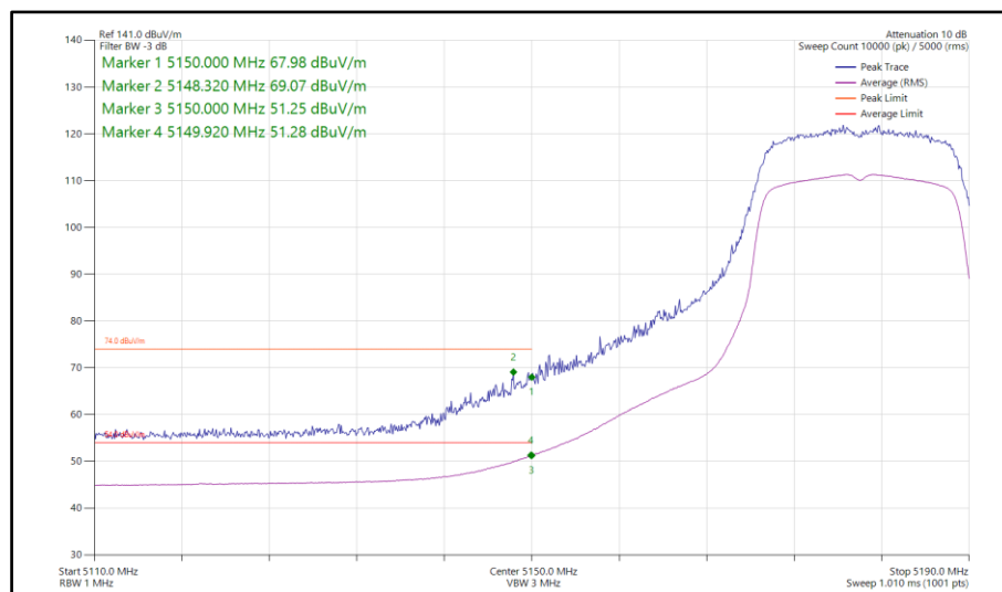
Figure 126 - 802.11ac VHT20, TxBF, Core 0-1 - 5180 MHz Band Edge Frequency 5150 MHz
