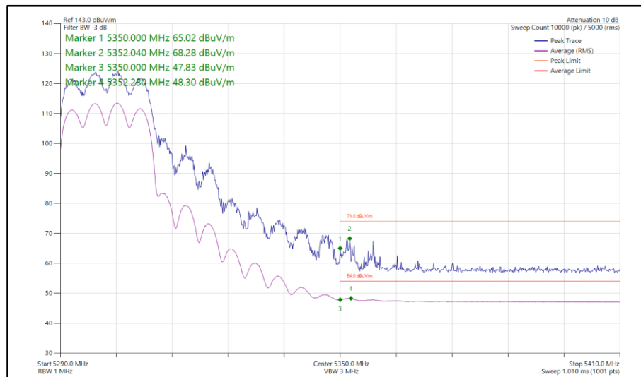
Figure 81 - 802.11ax HE20, SU, CDD, Core 0-1 - 5300 MHz Band Edge Frequency 5350 MHz
