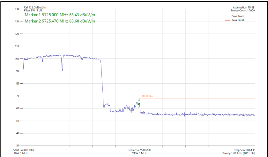
Figure 1165 - 802.11ac VHT160, SISO, Core 0 - 5570 MHz Band Edge Frequency 5725 MHz
