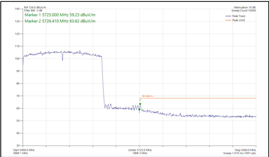
Figure 1194 - 802.11ax HE160, SU, SDM, Core 0-1 - 5570 MHz Band Edge Frequency 5725 MHz
