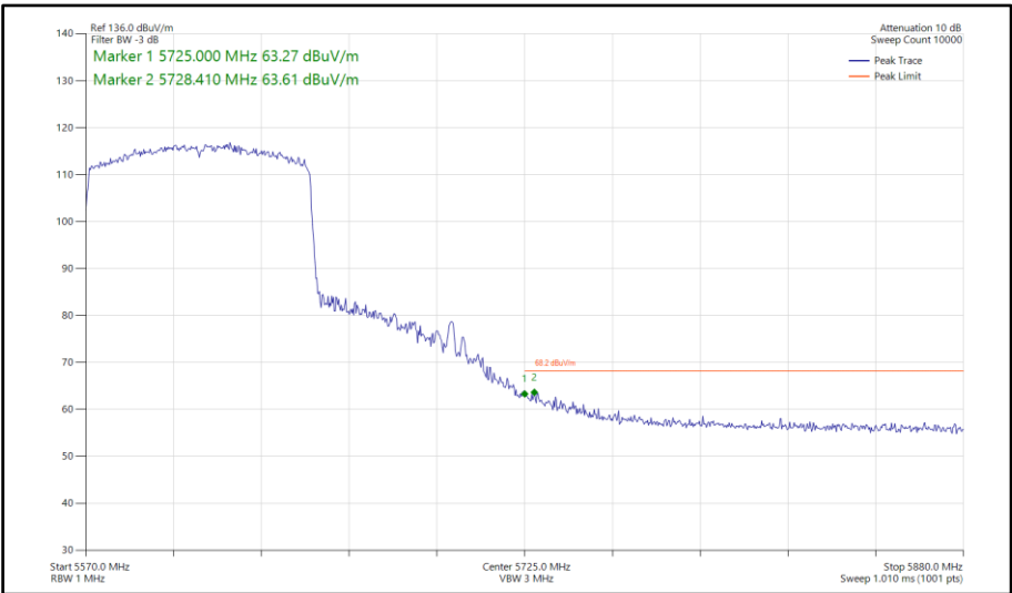
Figure 1136 - 802.11ax HE80, SU, SDM, Core 0-1 - 5610 MHz Band Edge Frequency 5725 MHz
