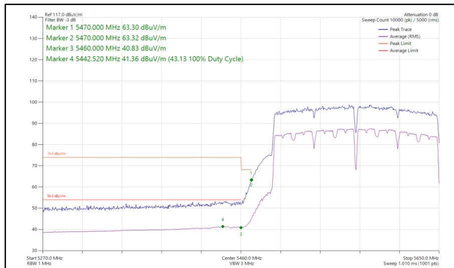
Figure 1159 - 802.11a, SISO, Core 0 - 5570 MHz Band Edge Frequency 5470 MHz
