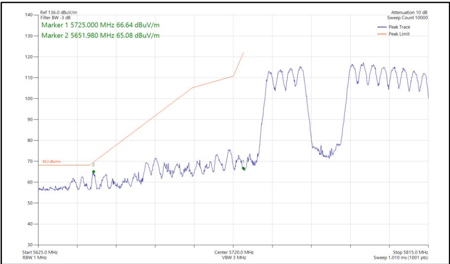
Figure 1134 - 802.11be EHT80, RU 484+242-91, SDM, Core 0-1 - 5775 MHz Band Edge Frequency 5725 MHz
