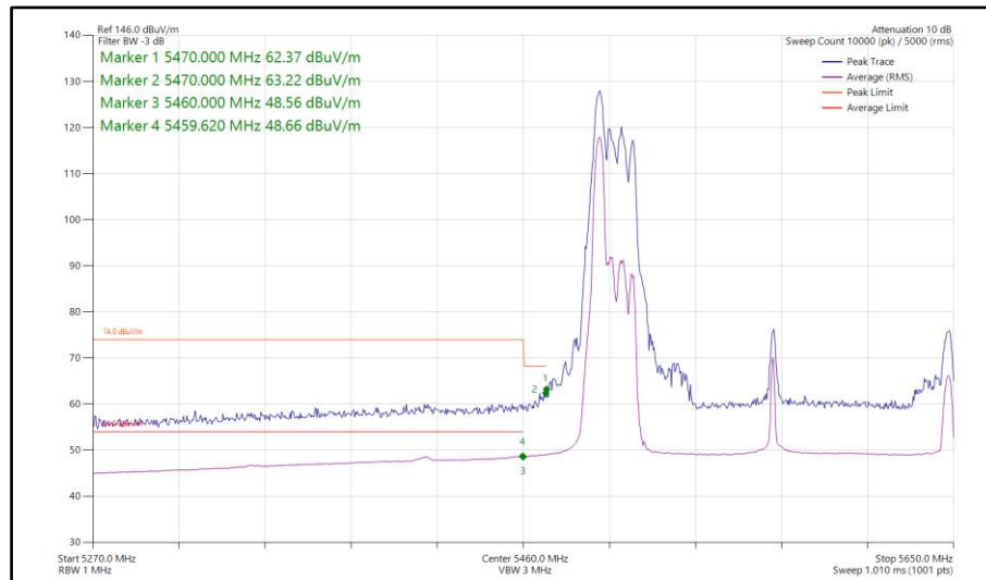
Figure 1191 - 802.11ax HE160, RU 52-37P, SDM, Core 0-1 - 5570 MHz Band Edge Frequency 5470 MHz
