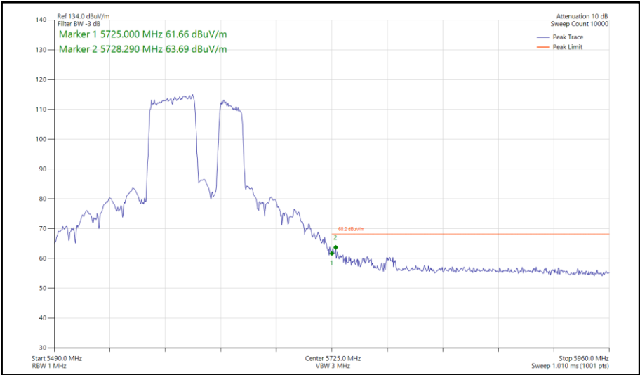
Figure 1168 - 802.11be EHT160, RU 484+242-92S, SISO, Core 0 - 5570 MHz Band Edge Frequency 5725 MHz
