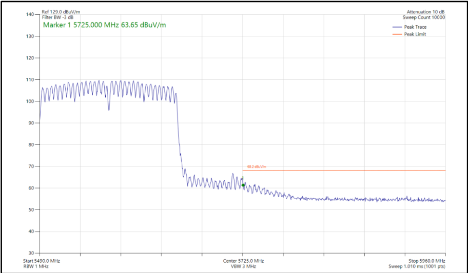
Figure 1185 - 802.11ac VHT160, CDD, Core 0-1 - 5570 MHz Band Edge Frequency 5725 MHz
