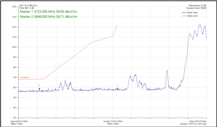
Figure 1133 - 802.11ax HE80, RU 106-60, SDM, Core 0-1 - 5775 MHz Band Edge Frequency 5725 MHz
