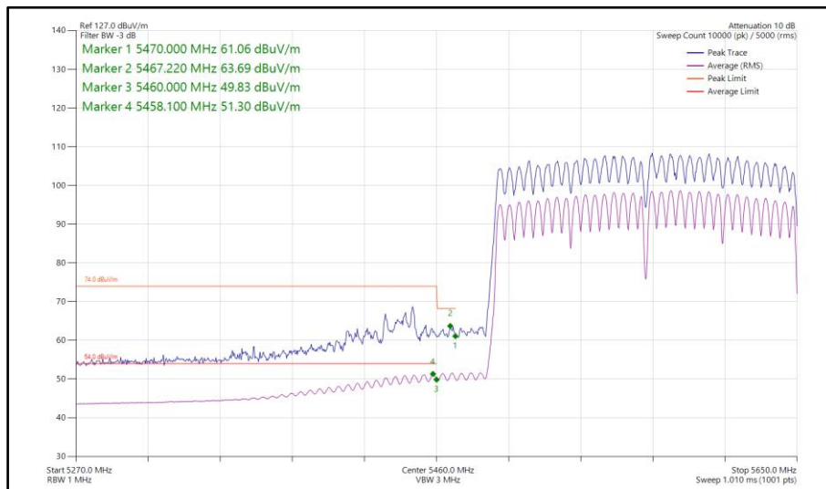
Figure 1180 - 802.11ac VHT160, CDD, Core 0-1 - 5570 MHz Band Edge Frequency 5470 MHz
