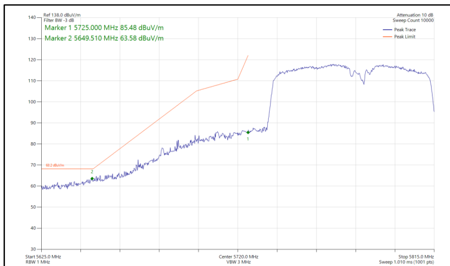
Figure 1151 - 802.11ac VHT80, TxBF, Core 0-1 - 5775 MHz Band Edge Frequency 5725 MHz
