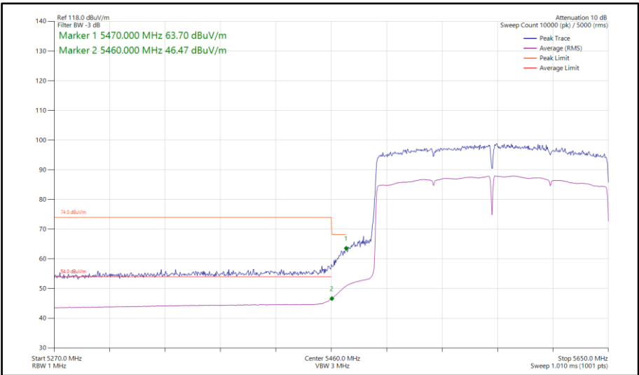
Figure 1171 - 802.11ax HE160, SU, SISO, Core 1 - 5570 MHz Band Edge Frequency 5470 MHz
