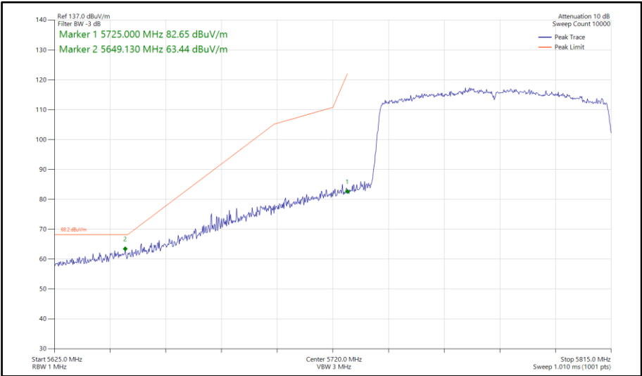
Figure 1152 - 802.11ax HE80, SU, TxBF, Core 0-1 - 5775 MHz Band Edge Frequency 5725 MHz
