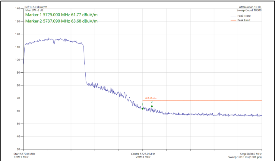
Figure 1135 - 802.11ac VHT80, SDM, Core 0-1 - 5610 MHz Band Edge Frequency 5725 MHz
