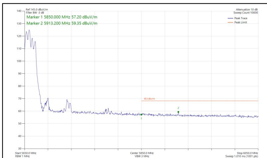
Figure 1142 - 802.11ax HE80, RU 106-53, SDM, Core 0-1 - 5690 MHz Band Edge Frequency 5850 MHz
