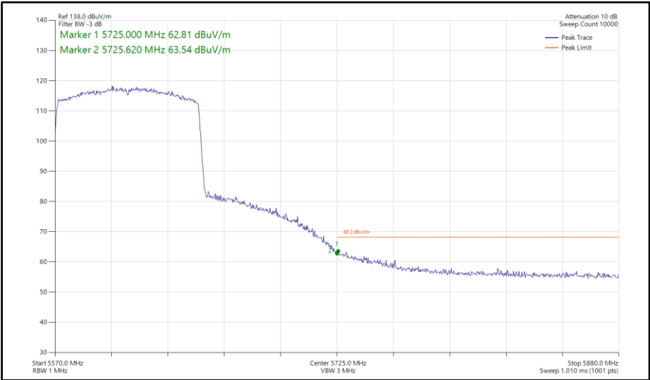
Figure 1154 - 802.11ax HE80, SU, TxBF, Core 0-1 - 5610 MHz Band Edge Frequency 5725 MHz
