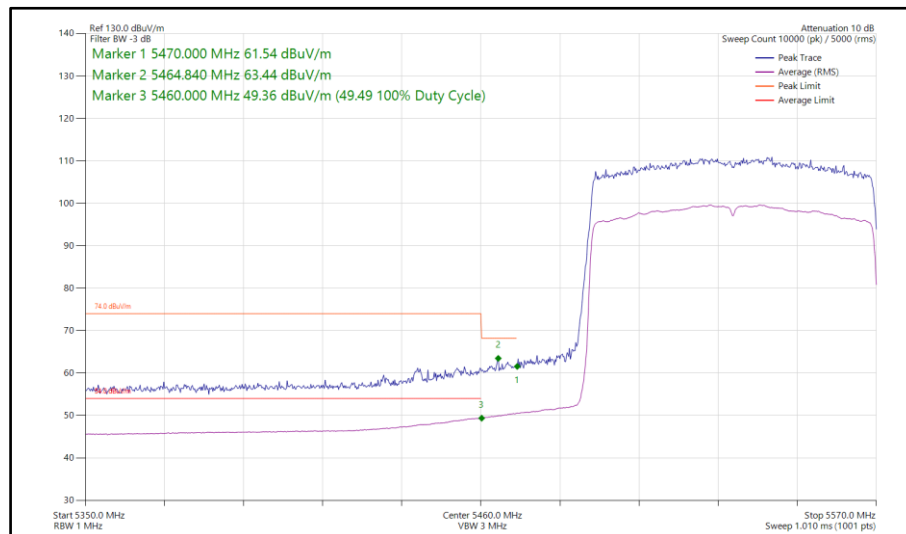
Figure 1125 - 802.11ax HE80, SU, SDM, Core 0-1 - 5530 MHz Band Edge Frequency 5470 MHz
