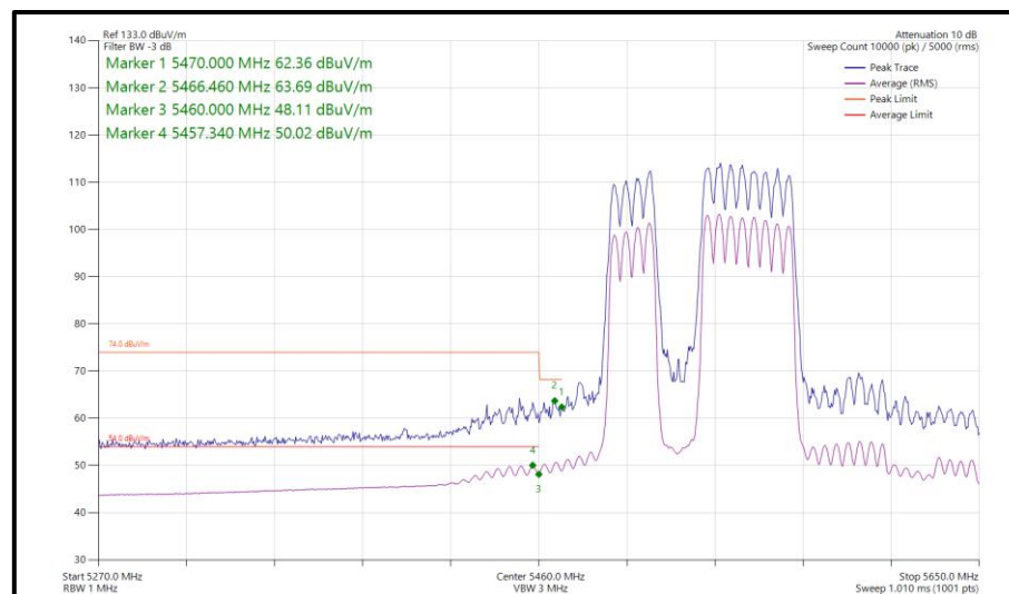
Figure 1192 - 802.11be EHT160, RU 484+242-91P, SDM, Core 0-1 - 5570 MHz Band Edge Frequency 5470 MHz
