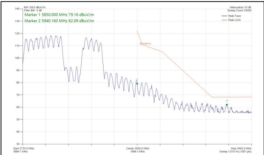
Figure 1146 - 802.11be EHT80, RU 484+242-92, SDM, Core 0-1 - 5775 MHz Band Edge Frequency 5850 MHz
