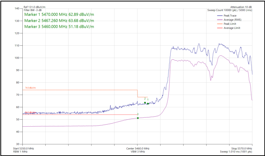
Figure 1147 - 802.11ac VHT80, TxBF, Core 0-1 - 5530 MHz Band Edge Frequency 5470 MHz
