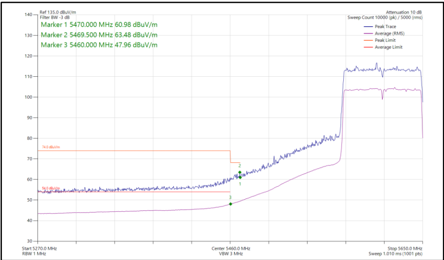
Figure 1124 - 802.11ac VHT80, SDM, Core 0-1 - 5610 MHz Band Edge Frequency 5470 MHz
