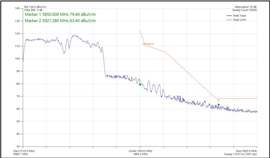
Figure 1156 - 802.11ac VHT80, TxBF, Core 0-1 - 5775 MHz Band Edge Frequency 5850 MHz
