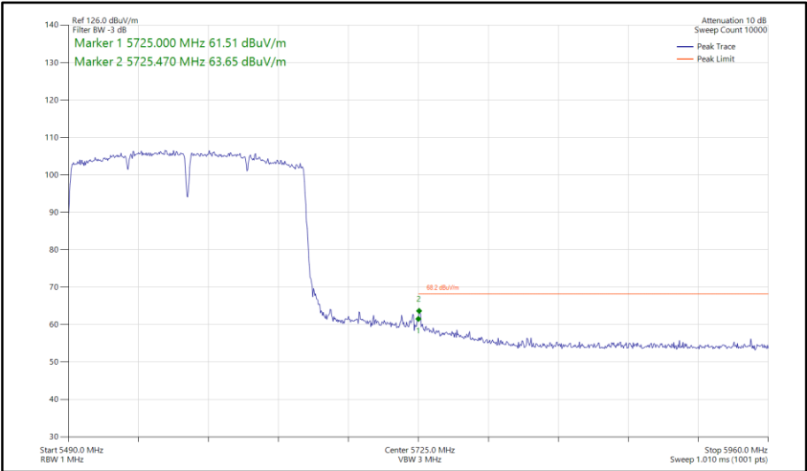
Figure 1175 - 802.11ac VHT160, SISO, Core 1 - 5570 MHz Band Edge Frequency 5725 MHz
