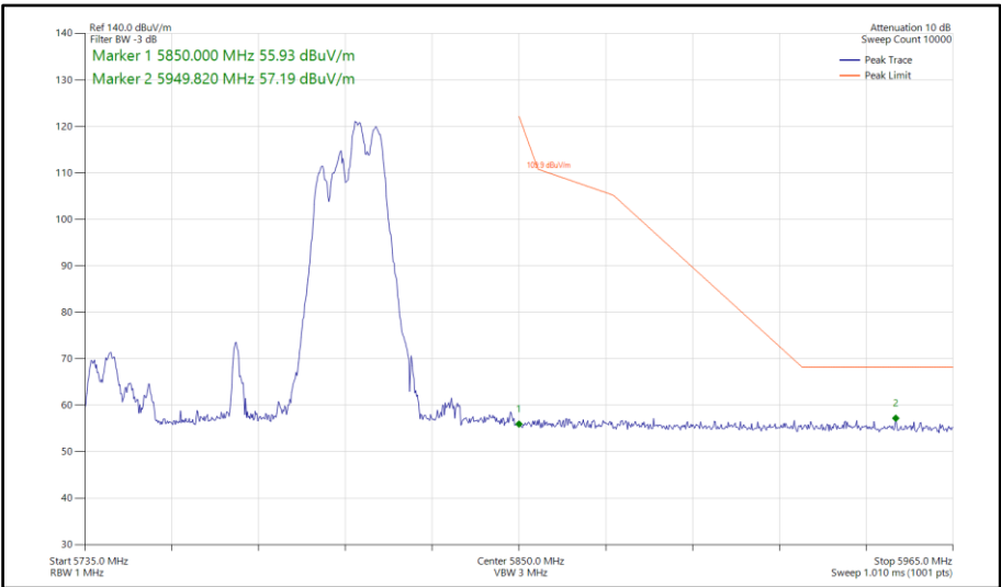
Figure 1144 - 802.11ax HE80, RU 106-60, SDM, Core 0-1 - 5775 MHz Band Edge Frequency 5850 MHz
