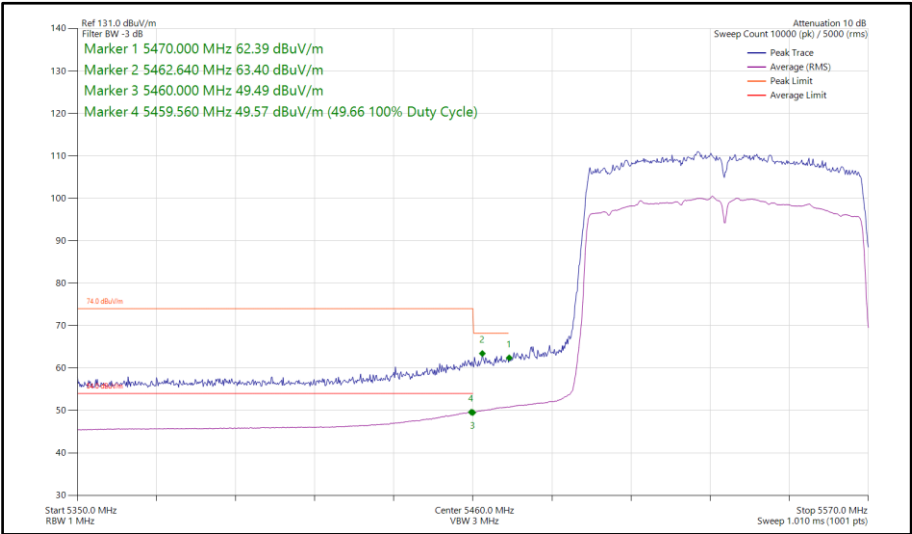
Figure 1123 - 802.11ac VHT80, SDM, Core 0-1 - 5530 MHz Band Edge Frequency 5470 MHz
