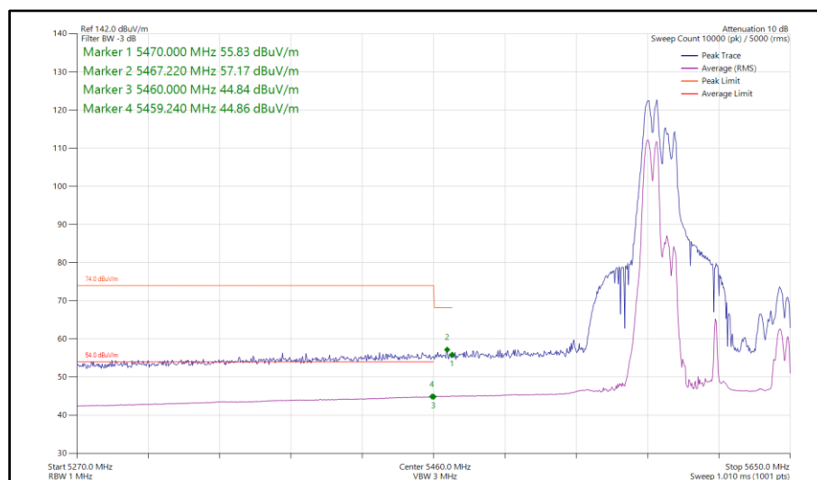
Figure 1128 - 802.11ax HE80, RU 106-53, SDM, Core 0-1 - 5610 MHz Band Edge Frequency 5470 MHz
