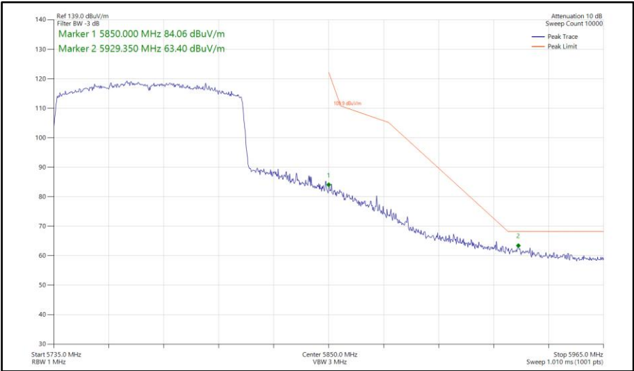
Figure 1143 - 802.11ax HE80, SU, SDM, Core 0-1 - 5775 MHz Band Edge Frequency 5850 MHz
