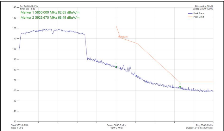
Figure 1140 - 802.11ac VHT80, SDM, Core 0-1 - 5775 MHz Band Edge Frequency 5850 MHz
