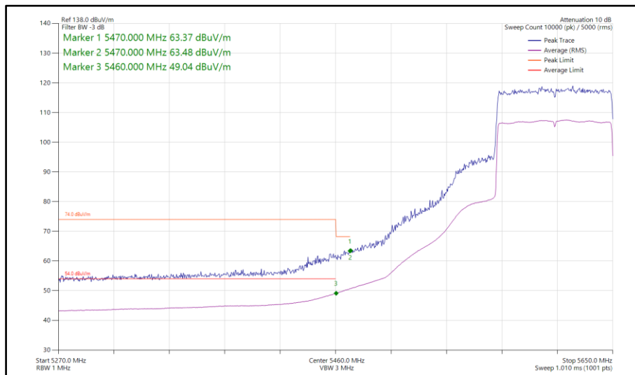
Figure 1150 - 802.11ax HE80, SU, TxBF, Core 0-1 - 5610 MHz Band Edge Frequency 5470 MHz
