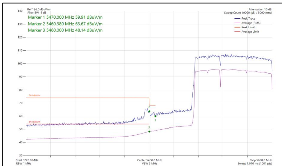
Figure 1163 - 802.11be EHT160, RU 996+484-94P, SISO, Core 0 - 5570 MHz Band Edge Frequency 5470 MHz
