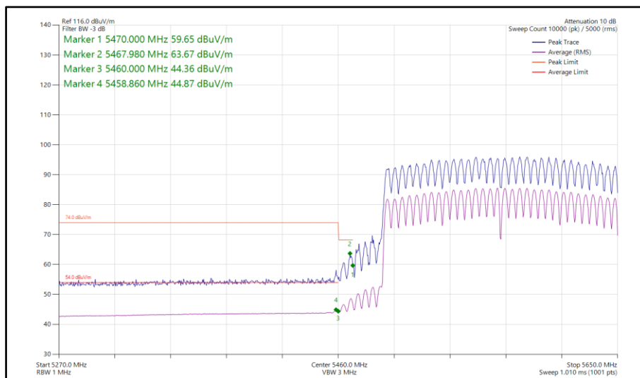
Figure 1181 - 802.11ax HE160, SU, CDD, Core 0-1 - 5570 MHz Band Edge Frequency 5470 MHz
