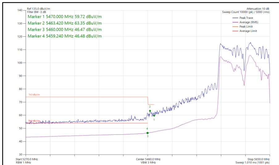
Figure 1148 - 802.11ac VHT80, TxBF, Core 0-1 - 5610 MHz Band Edge Frequency 5470 MHz
