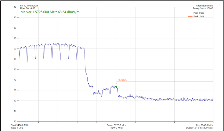
Figure 1164 - 802.11a, SISO, Core 0 - 5570 MHz Band Edge Frequency 5725 MHz
