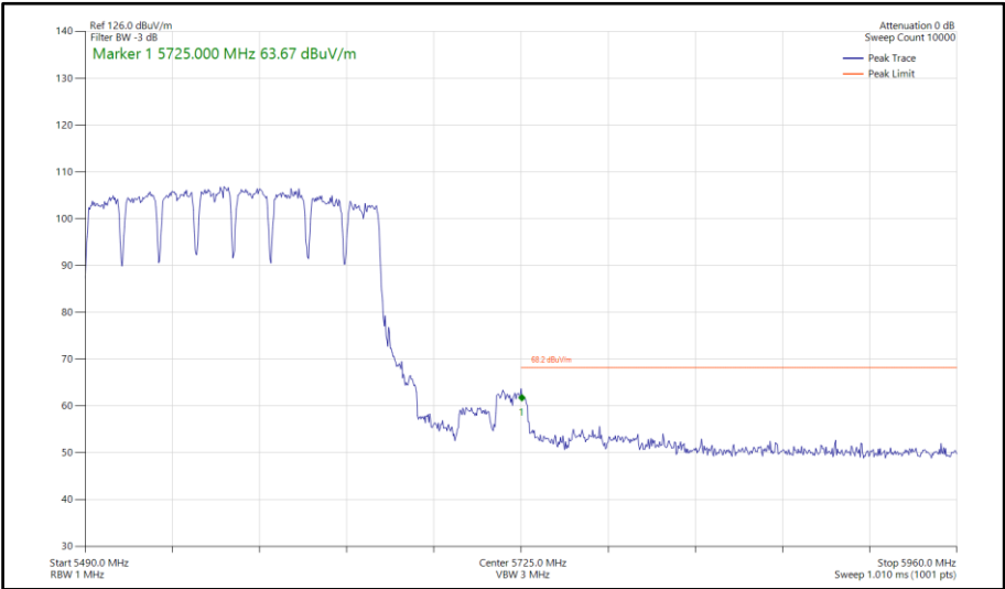
Figure 1174 - 802.11a, SISO, Core 1 - 5570 MHz Band Edge Frequency 5725 MHz
