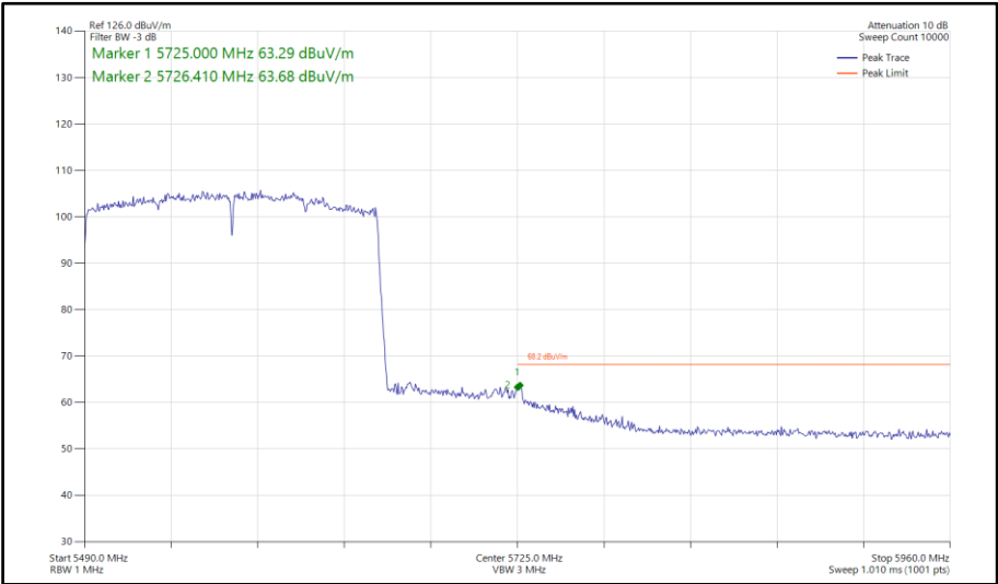
Figure 1166 - 802.11ax HE160, SU, SISO, Core 0 - 5570 MHz Band Edge Frequency 5725 MHz
