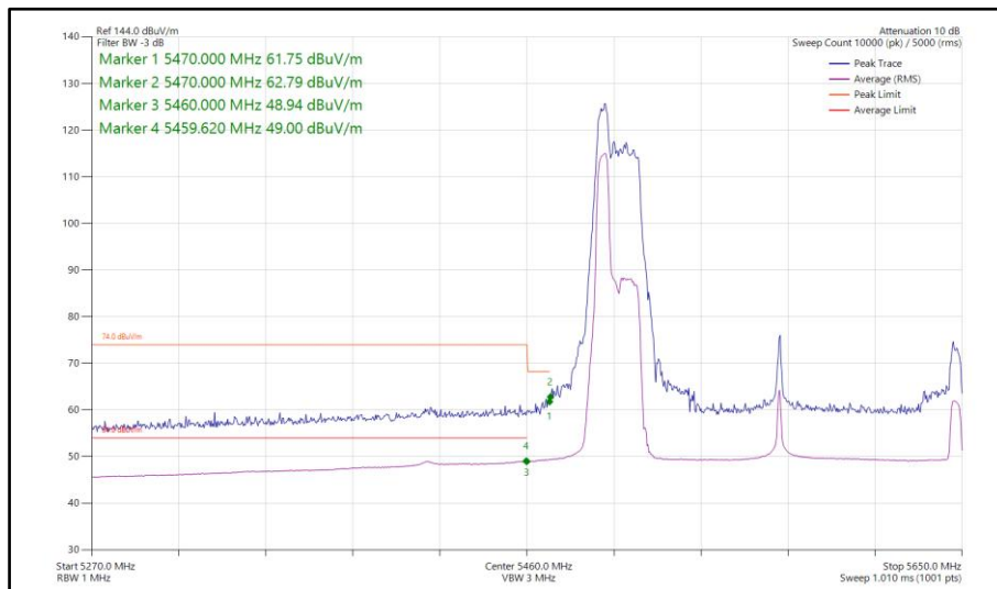
Figure 1162 - 802.11ax HE160, RU 52-37P, SISO, Core 0 - 5570 MHz Band Edge Frequency 5470 MHz
