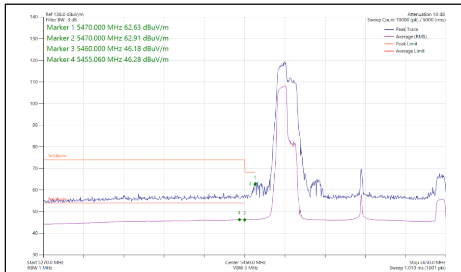
Figure 1172 - 802.11ax HE160, RU 106-53P, SISO, Core 1 - 5570 MHz Band Edge Frequency 5470 MHz
