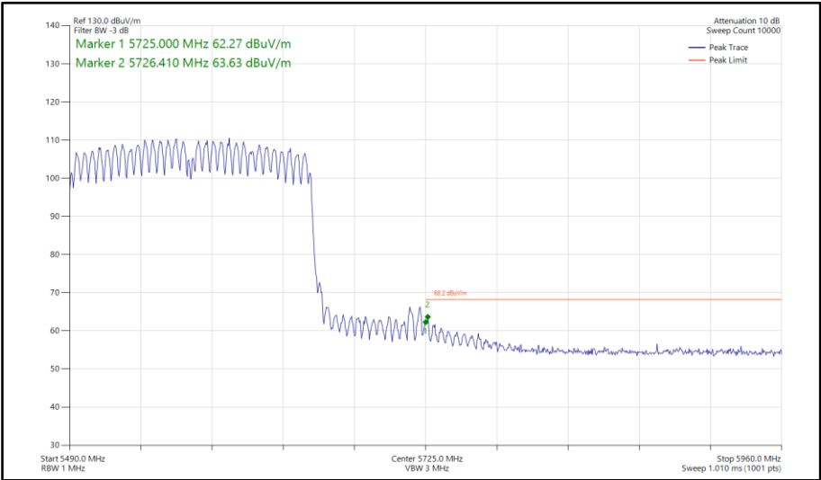
Figure 1186 - 802.11ax HE160, SU, CDD, Core 0-1 - 5570 MHz Band Edge Frequency 5725 MHz
