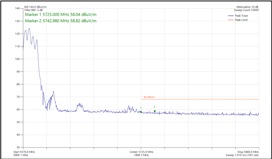
Figure 1137 - 802.11ax HE80, RU 106-53, SDM, Core 0-1 - 5610 MHz Band Edge Frequency 5725 MHz
