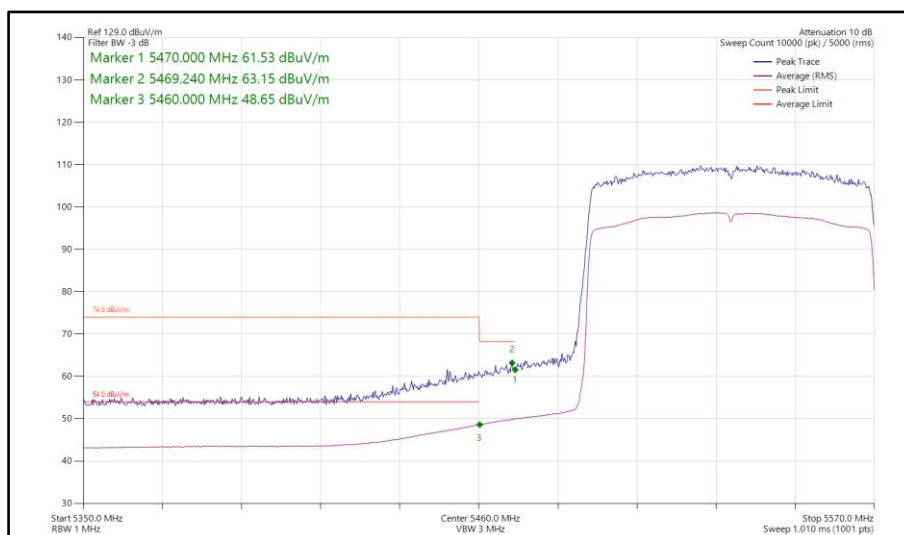
Figure 1149 - 802.11ax HE80, SU, TxBF, Core 0-1 - 5530 MHz Band Edge Frequency 5470 MHz
