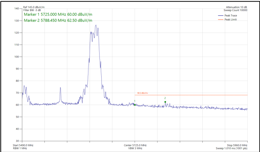
Figure 1187 - 802.11ax HE160, RU 106-60S, CDD, Core 0-1 - 5570 MHz Band Edge Frequency 5725 MHz
