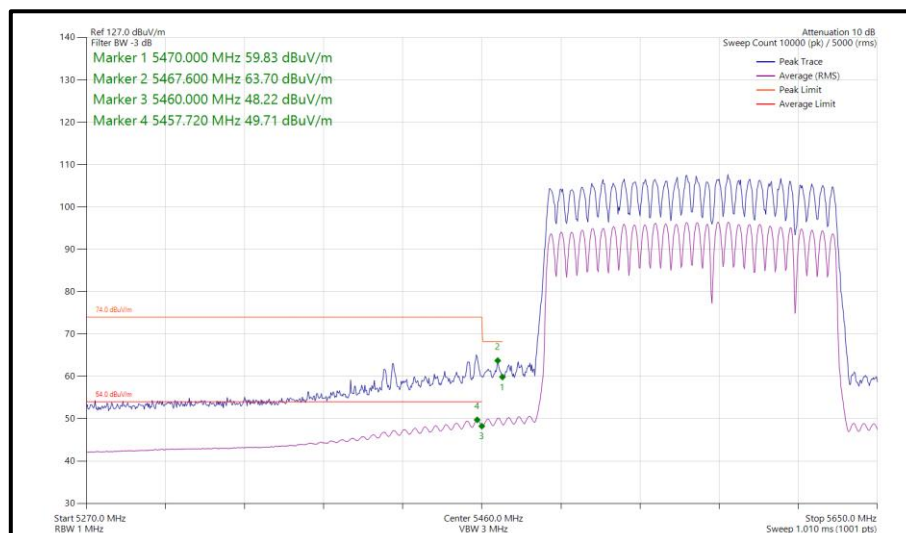
Figure 1183 - 802.11be EHT160, RU 996+484+242-99S, CDD, Core 0-1 - 5570 MHz Band Edge Frequency 5470 MHz
