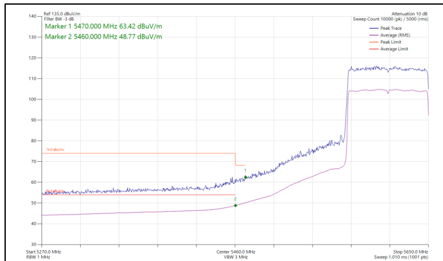
Figure 1127 - 802.11ax HE80, SU, SDM, Core 0-1 - 5610 MHz Band Edge Frequency 5470 MHz
