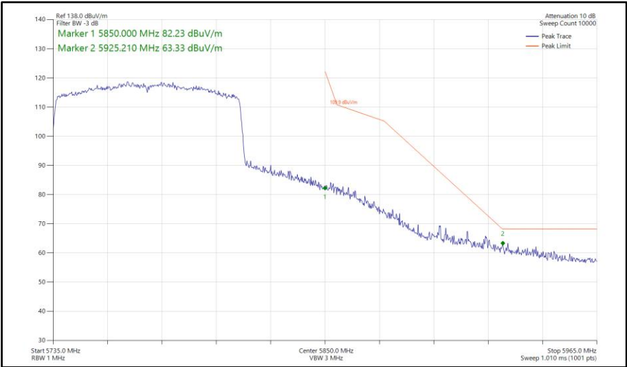
Figure 1158 - 802.11ax HE80, SU, TxBF, Core 0-1 - 5775 MHz Band Edge Frequency 5850 MHz
