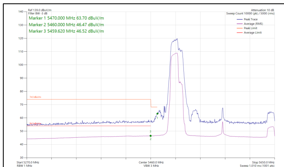
Figure 1173 - 802.11be EHT160, RU 106+26-82P, SISO, Core 1 - 5570 MHz Band Edge Frequency 5470 MHz
