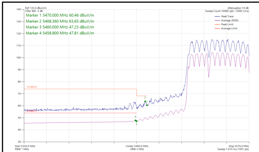
Figure 1129 - 802.11be EHT80, RU 484+242-90, SDM, Core 0-1 - 5530 MHz Band Edge Frequency 5470 MHz
