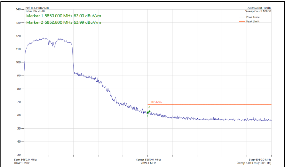
Figure 1155 - 802.11ac VHT80, TxBF, Core 0-1 - 5690 MHz Band Edge Frequency 5850 MHz
