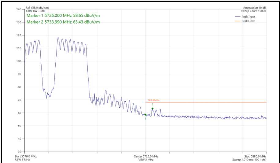
Figure 1138 - 802.11be EHT80, RU 484+242-91, SDM, Core 0-1 - 5610 MHz Band Edge Frequency 5725 MHz
