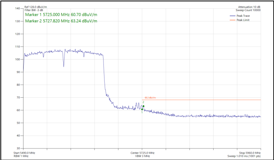
Figure 1193 - 802.11ac VHT160, SDM, Core 0-1 - 5570 MHz Band Edge Frequency 5725 MHz
