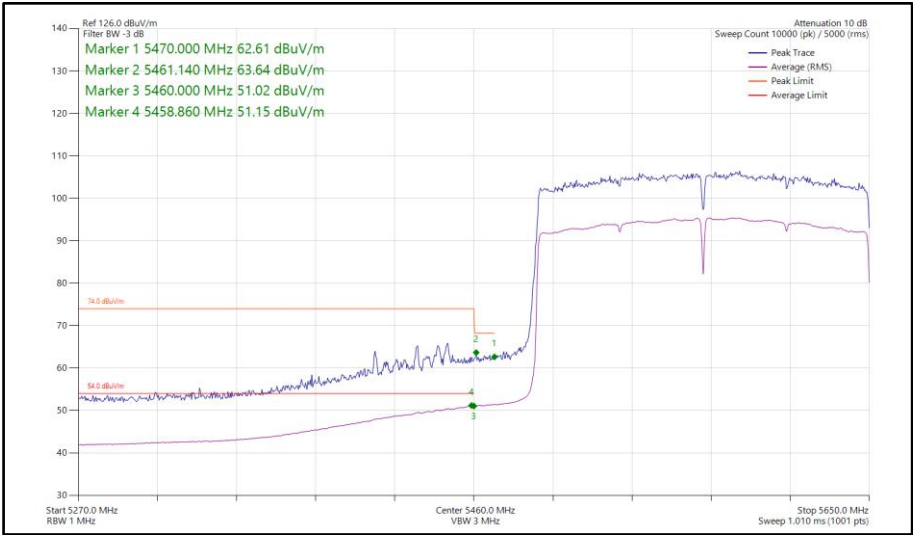
Figure 1189 - 802.11ac VHT160, SDM, Core 0-1 - 5570 MHz Band Edge Frequency 5470 MHz
