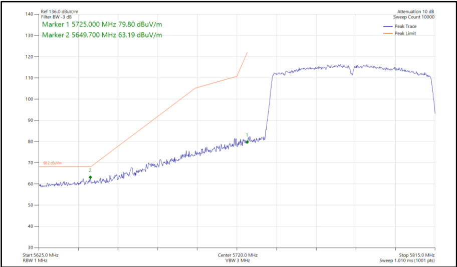
Figure 1131 - 802.11ac VHT80, SDM, Core 0-1 - 5775 MHz Band Edge Frequency 5725 MHz
