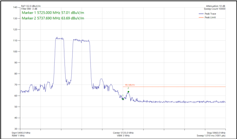
Figure 1178 - 802.11be EHT160, RU 484+242-91S, SISO, Core 1 - 5570 MHz Band Edge Frequency 5725 MHz
