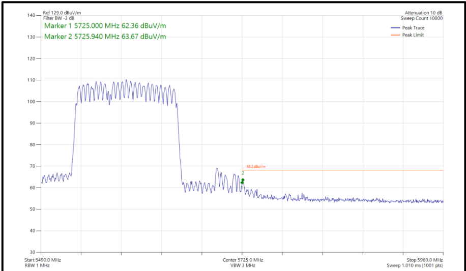
Figure 1196 - 802.11be EHT160, RU 996+484-94P, SDM, Core 0-1 - 5570 MHz Band Edge Frequency 5725 MHz
