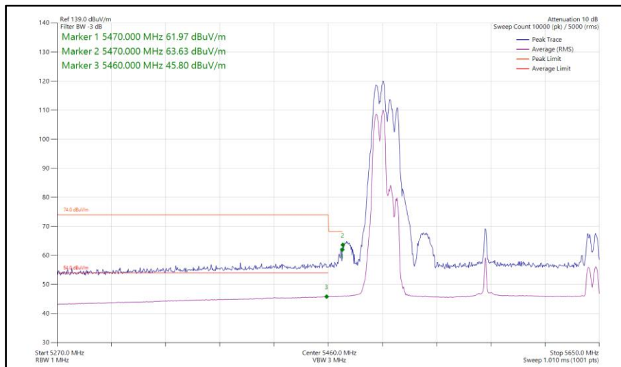
Figure 1182 - 802.11ax HE160, RU 106-53P, CDD, Core 0-1 - 5570 MHz Band Edge Frequency 5470 MHz
