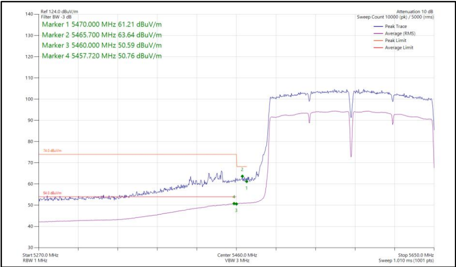
Figure 1160 - 802.11ac VHT160, SISO, Core 0 - 5570 MHz Band Edge Frequency 5470 MHz
