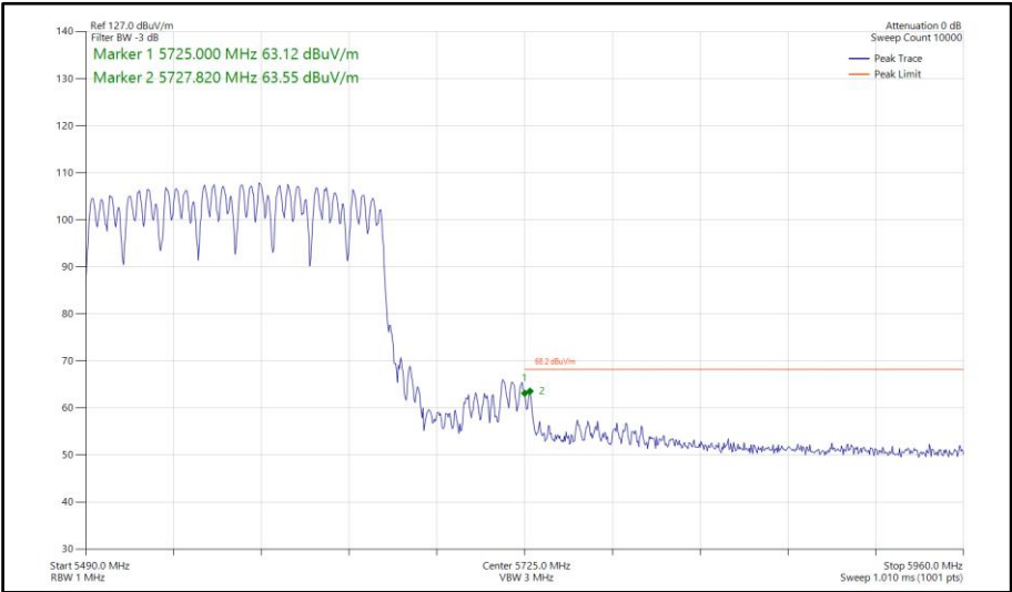
Figure 1184 - 802.11a, CDD, Core 0-1 - 5570 MHz Band Edge Frequency 5725 MHz
