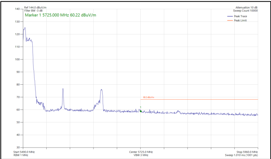
Figure 1167 - 802.11ax HE160, RU 52-37P, SISO, Core 0 - 5570 MHz Band Edge Frequency 5725 MHz
