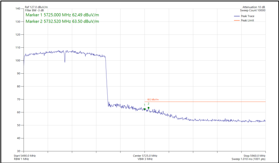
Figure 1176 - 802.11ax HE160, SU, SISO, Core 1 - 5570 MHz Band Edge Frequency 5725 MHz
