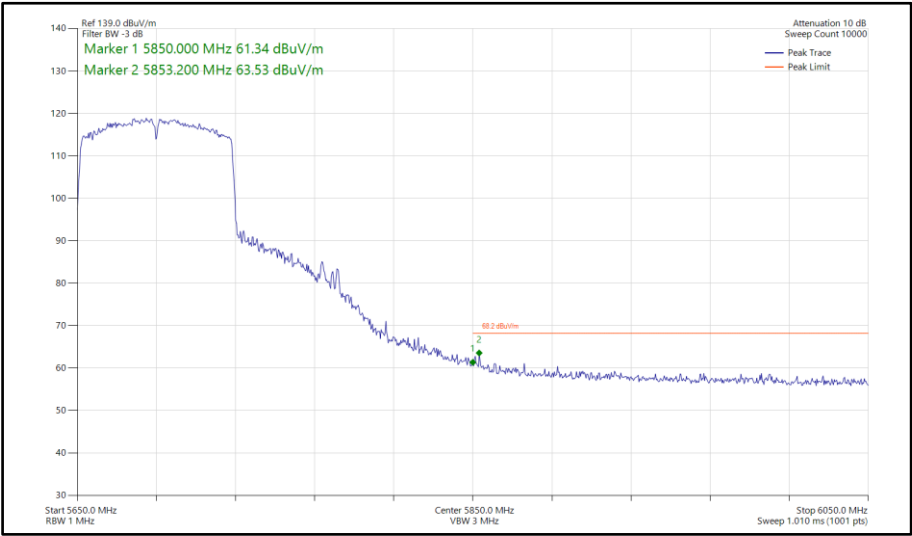
Figure 1139 - 802.11ac VHT80, SDM, Core 0-1 - 5690 MHz Band Edge Frequency 5850 MHz
