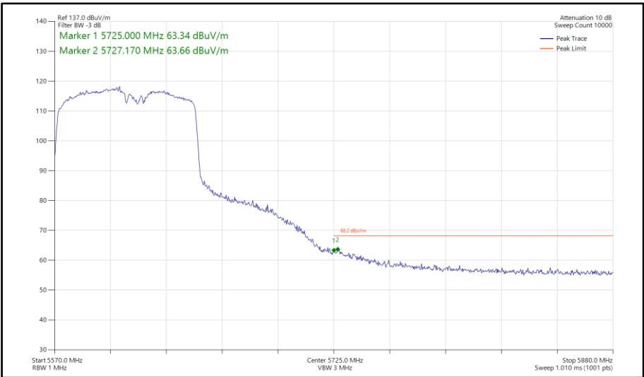
Figure 1153 - 802.11ac VHT80, TxBF, Core 0-1 - 5610 MHz Band Edge Frequency 5725 MHz
