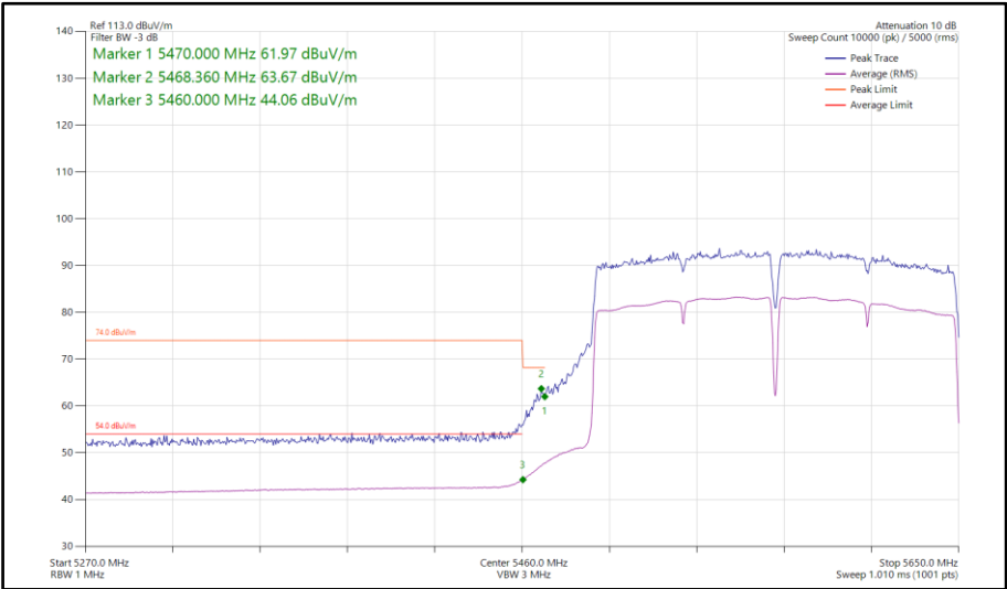
Figure 1170 - 802.11ac VHT160, SISO, Core 1 - 5570 MHz Band Edge Frequency 5470 MHz
