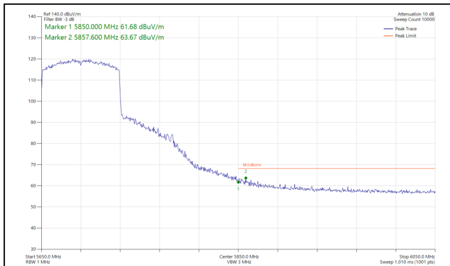
Figure 1141 - 802.11ax HE80, SU, SDM, Core 0-1 - 5690 MHz Band Edge Frequency 5850 MHz
