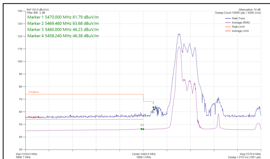
Figure 1126 - 802.11ax HE80, RU 52-37, SDM, Core 0-1 - 5530 MHz Band Edge Frequency 5470 MHz
