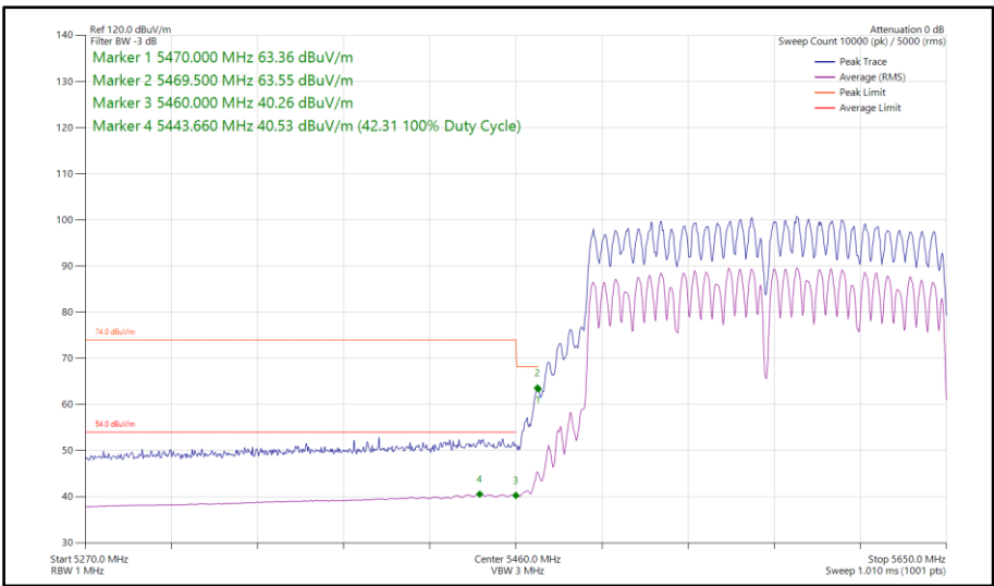
Figure 1179 - 802.11a, CDD, Core 0-1 - 5570 MHz Band Edge Frequency 5470 MHz
