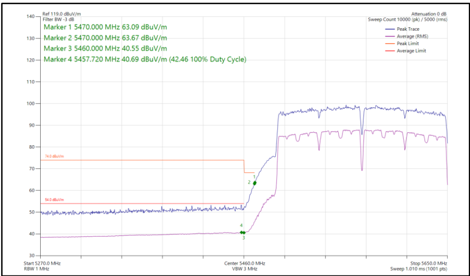
Figure 1169 - 802.11a, SISO, Core 1 - 5570 MHz Band Edge Frequency 5470 MHz
