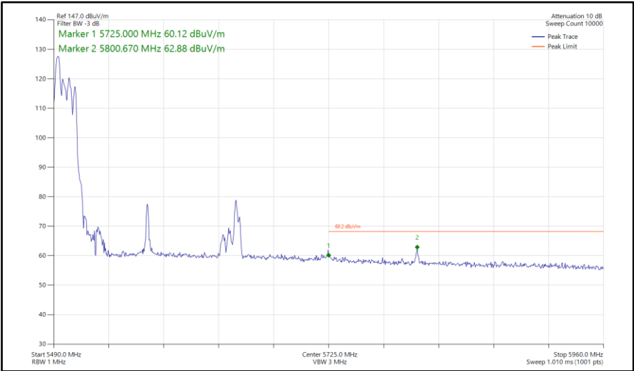
Figure 1195 - 802.11ax HE160, RU 52-37P, SDM, Core 0-1 - 5570 MHz Band Edge Frequency 5725 MHz
