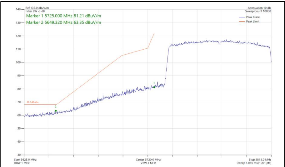
Figure 1132 - 802.11ax HE80, SU, SDM, Core 0-1 - 5775 MHz Band Edge Frequency 5725 MHz
