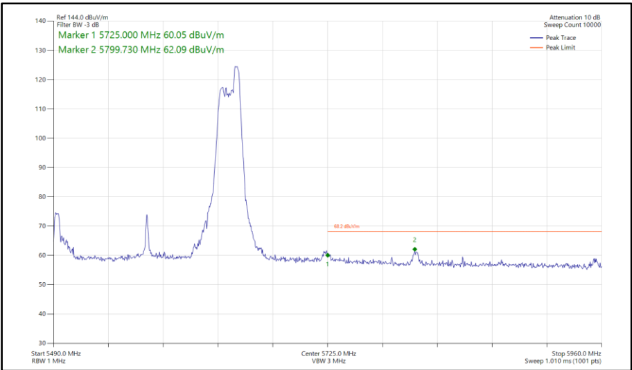
Figure 1177 - 802.11ax HE160, RU 52-52S, SISO, Core 1 - 5570 MHz Band Edge Frequency 5725 MHz
