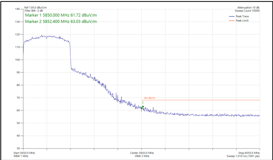
Figure 1157 - 802.11ax HE80, SU, TxBF, Core 0-1 - 5690 MHz Band Edge Frequency 5850 MHz
