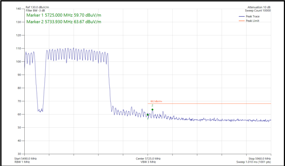
Figure 1188 - 802.11be EHT160, RU996+484+242-97P, CDD, Core 0-1 - 5570 MHz Band Edge Frequency 5725 MHz
