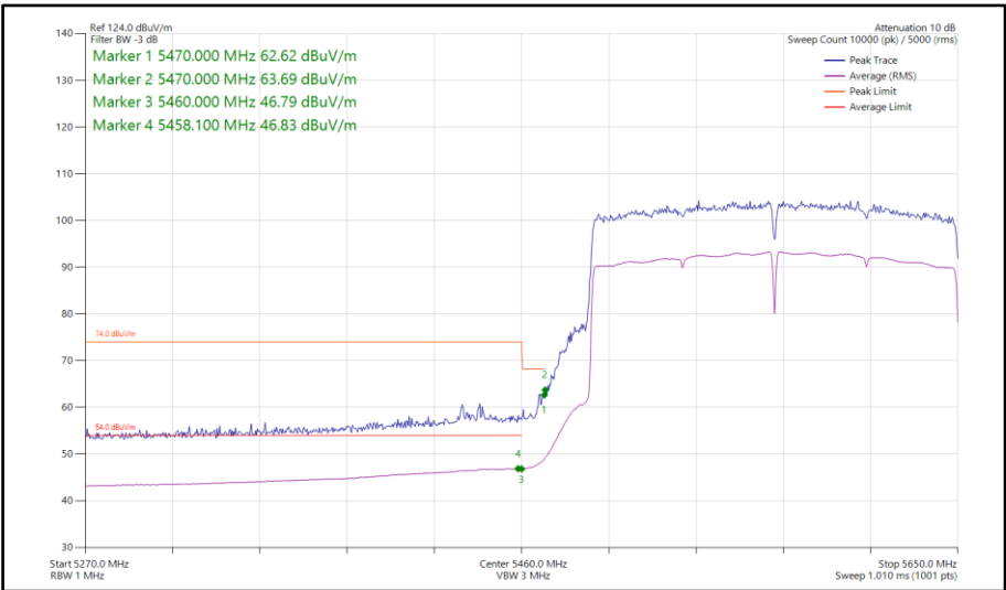
Figure 1161 - 802.11ax HE160, SU, SISO, Core 0 - 5570 MHz Band Edge Frequency 5470 MHz
