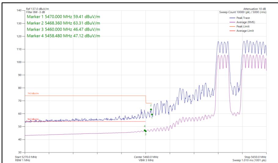
Figure 1130 - 802.11be EHT80, RU 484+242-91, SDM, Core 0-1 - 5610 MHz Band Edge Frequency 5470 MHz
