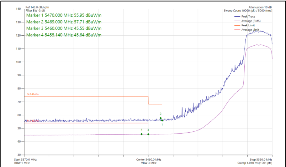
Figure 139 - 802.11ax HE20, SU, TxBF, Core 0-1 - 5540 MHz Band Edge Frequency 5460 MHz
