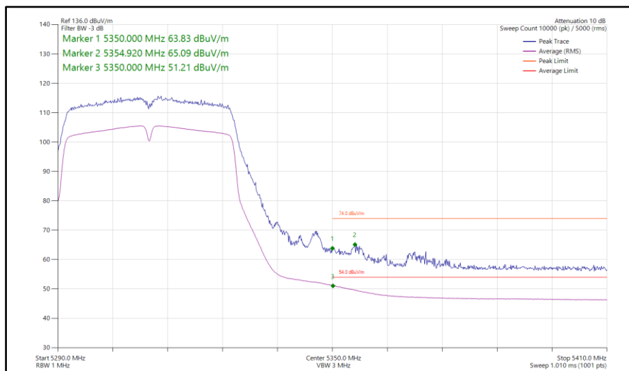
Figure 185 - 802.11n HT40, SISO, Core 1 - 5310 MHz Band Edge Frequency 5350 MHz
