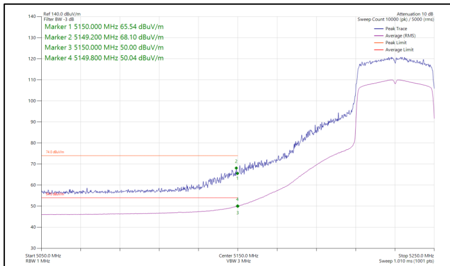
Figure 178 - 802.11ax HE40, SU, SISO, Core 1 - 5230 MHz Band Edge Frequency 5150 MHz
