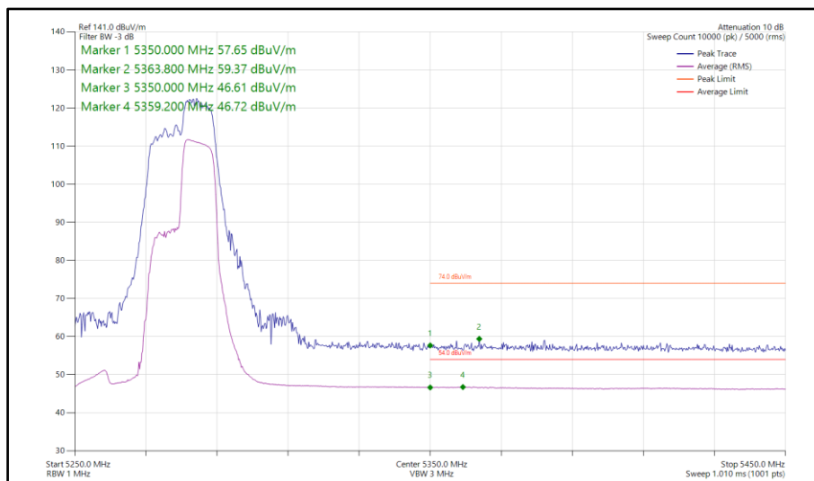
Figure 155 - 802.11ax HE40, RU 106-56, SISO, Core 0 - 5270 MHz Band Edge Frequency 5350 MHz
