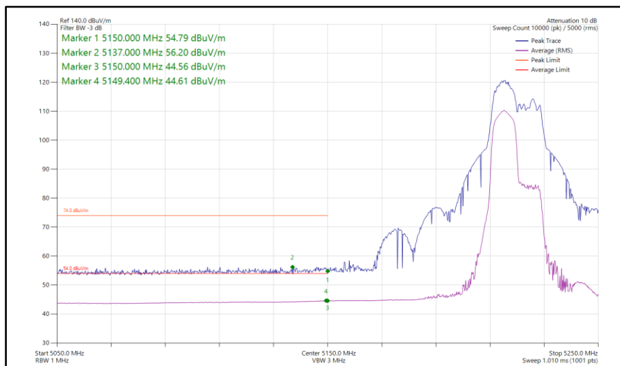
Figure 147 - 802.11ax HE40, RU 106-53, SISO, Core 0 - 5230 MHz Band Edge Frequency 5150 MHz
