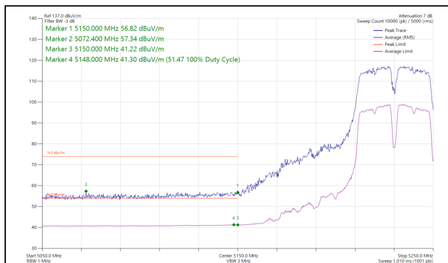
Figure 173 - 802.11a, SISO, Core 1 - 5230 MHz Band Edge Frequency 5150 MHz
