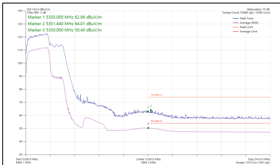
Figure 191 - 802.11be EHT40, RU 106+26-82, SISO, Core 1 - 5310 MHz Band Edge Frequency 5350 MHz
