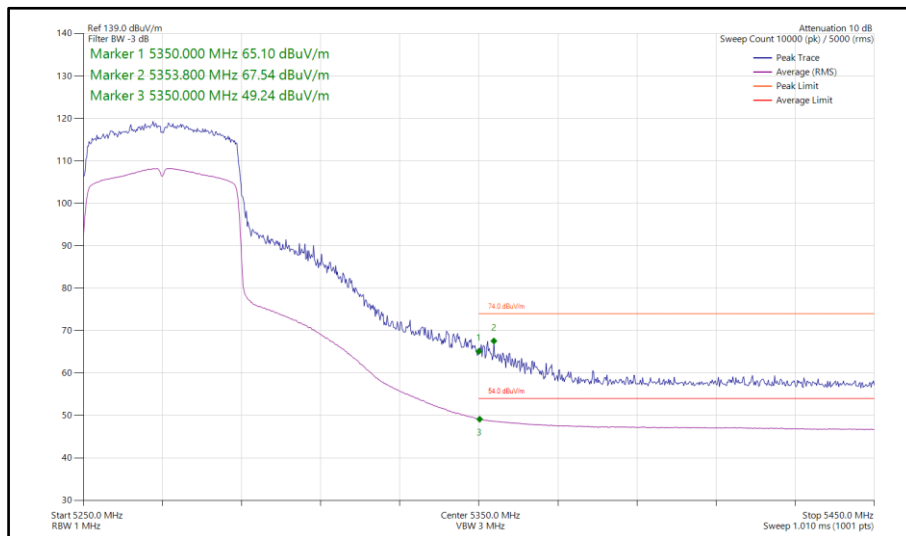
Figure 186 - 802.11ax HE40, SU, SISO, Core 1 - 5270 MHz Band Edge Frequency 5350 MHz
