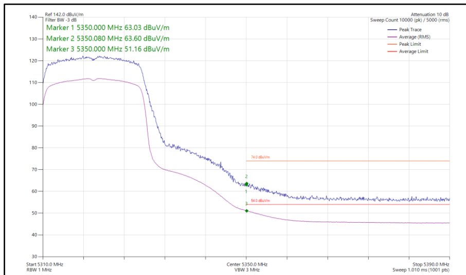
Figure 133 - 802.11ax HE20, SU, TxBF, Core 0-1 - 5320 MHz Band Edge Frequency 5350 MHz
