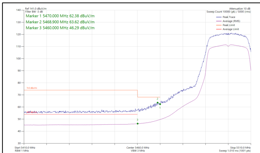
Figure 134 - 802.11ac VHT20, TxBF, Core 0-1 - 5500 MHz Band Edge Frequency 5460 MHz
