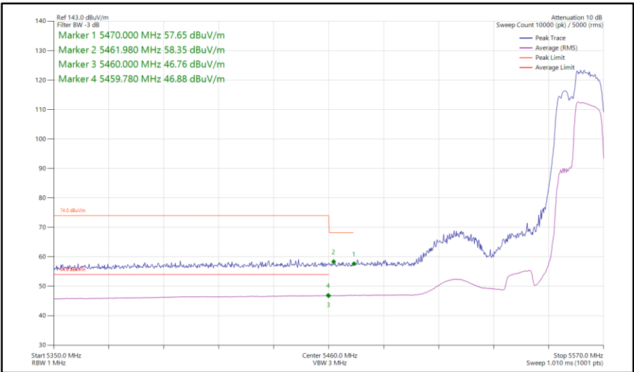
Figure 171 - 802.11be EHT40, RU 106+26-85, SISO, Core 0 - 5550 MHz Band Edge Frequency 5460 MHz
