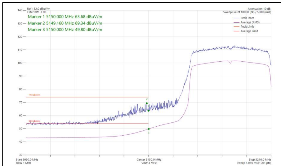
Figure 144 - 802.11ax HE40, SU, SISO, Core 0 - 5190 MHz Band Edge Frequency 5150 MHz
