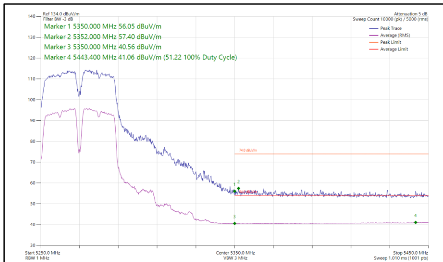
Figure 150 - 802.11a, SISO, Core 0 - 5270 MHz Band Edge Frequency 5350 MHz
