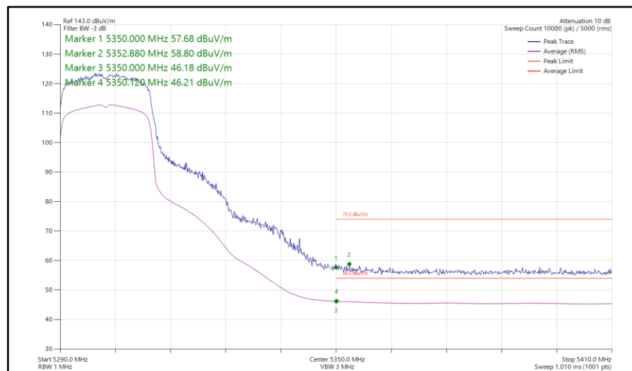
Figure 132 - 802.11ax HE20, SU, TxBF, Core 0-1 - 5300 MHz Band Edge Frequency 5350 MHz
