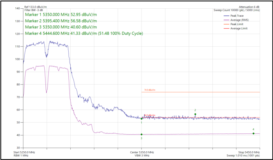
Figure 182 - 802.11a, SISO, Core 1 - 5270 MHz Band Edge Frequency 5350 MHz
