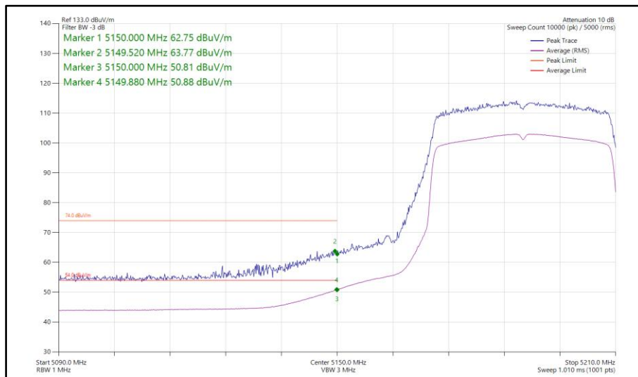
Figure 176 - 802.11ax HE40, SU, SISO, Core 1 - 5190 MHz Band Edge Frequency 5150 MHz
