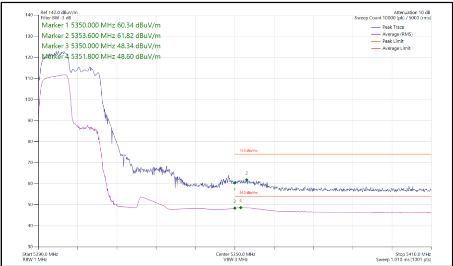
Figure 157 - 802.11ax HE40, RU 106-53, SISO, Core 0 - 5310 MHz Band Edge Frequency 5350 MHz
