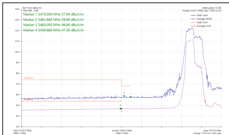
Figure 169 - 802.11ax HE40, RU 106-53, SISO, Core 0 - 5550 MHz Band Edge Frequency 5460 MHz
