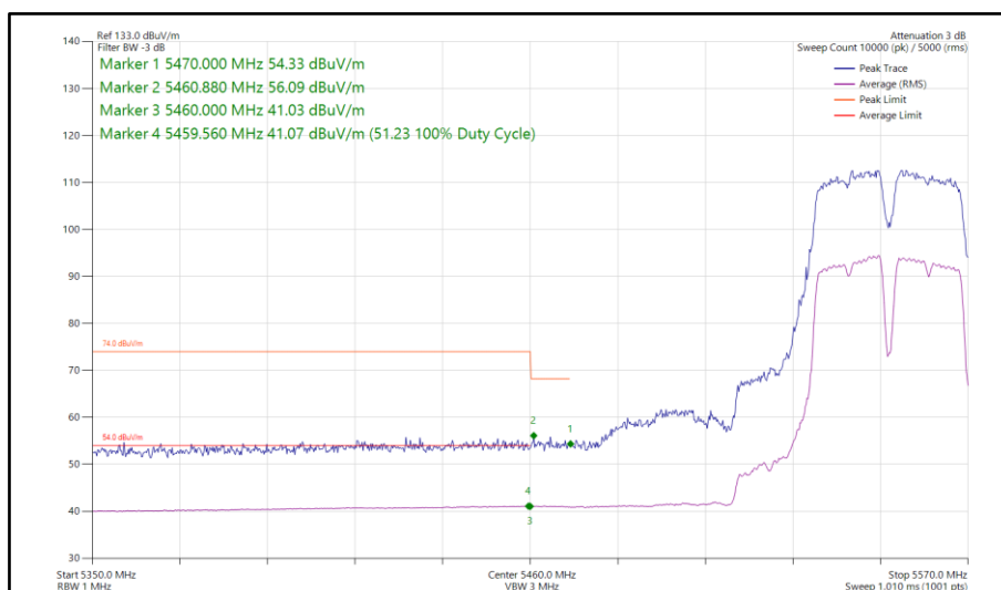
Figure 161 - 802.11a, SISO, Core 0 - 5550 MHz Band Edge Frequency 5460 MHz
