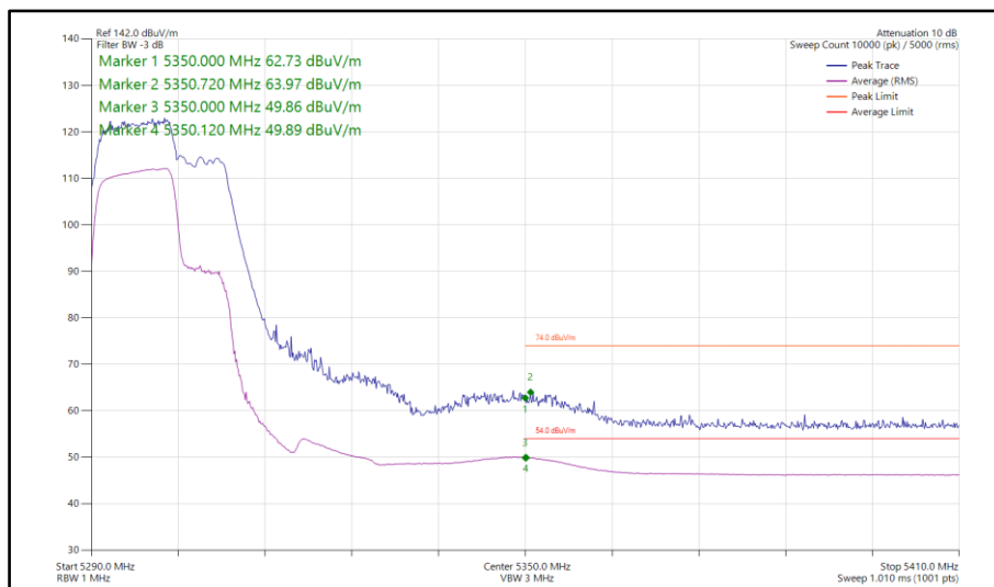
Figure 159 - 802.11be EHT40, RU 106+26-82, SISO, Core 0 - 5310 MHz Band Edge Frequency 5350 MHz
