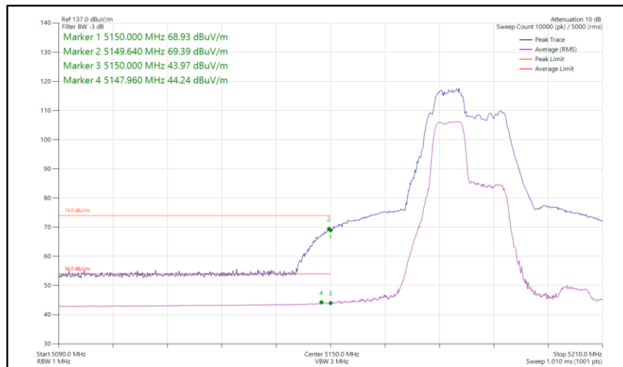
Figure 148 - 802.11be EHT40, RU 52+26-70, SISO, Core 0 - 5190 MHz Band Edge Frequency 5150 MHz
