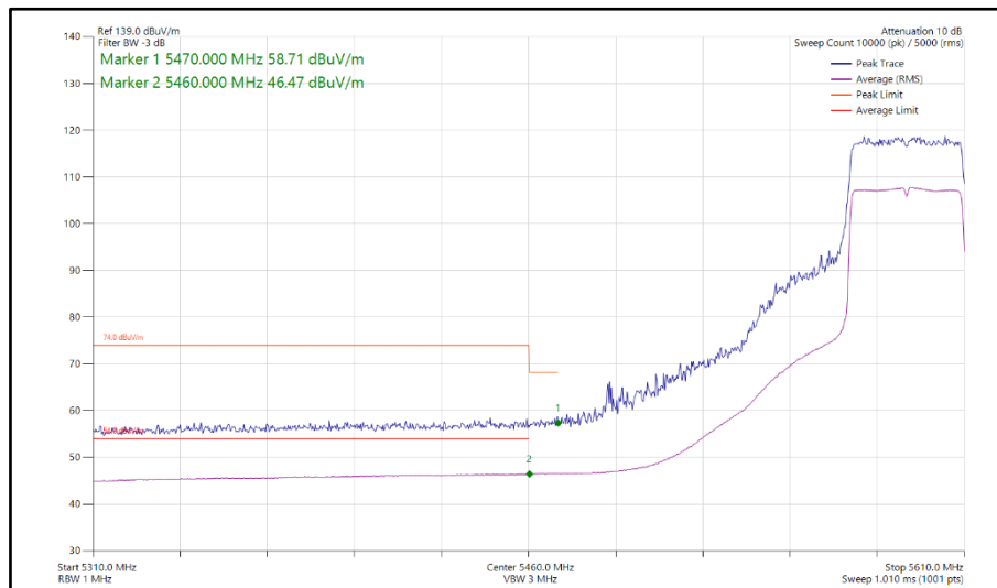
Figure 168 - 802.11ax HE40, SU, SISO, Core 0 - 5590 MHz Band Edge Frequency 5460 MHz
