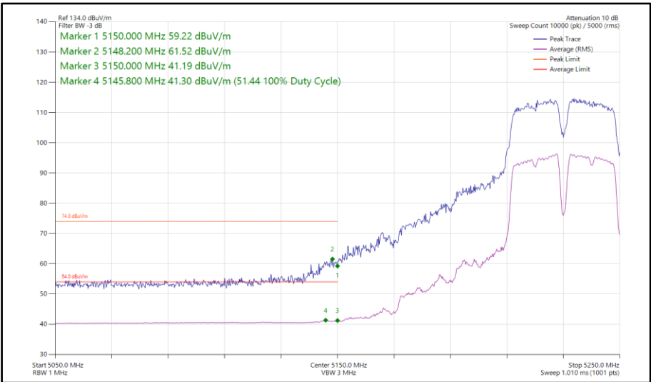
Figure 141 - 802.11a, SISO, Core 0 - 5230 MHz Band Edge Frequency 5150 MHz
