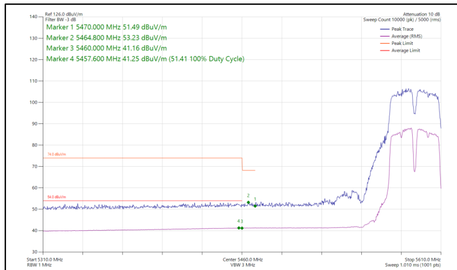
Figure 162 - 802.11a, SISO, Core 0 - 5590 MHz Band Edge Frequency 5460 MHz
