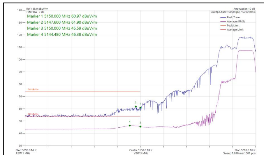
Figure 145 - 802.11ax HE40, RU 106-56, SISO, Core 0 - 5190 MHz Band Edge Frequency 5150 MHz
