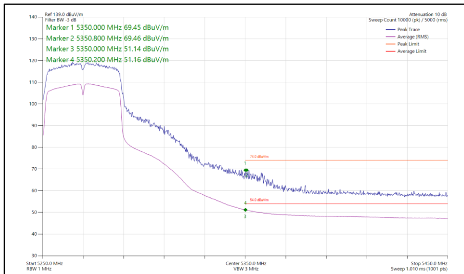
Figure 152 - 802.11n HT40, SISO, Core 0 - 5270 MHz Band Edge Frequency 5350 MHz
