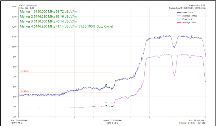
Figure 140 - 802.11a, SISO, Core 0 - 5190 MHz Band Edge Frequency 5150 MHz
