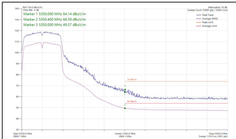
Figure 184 - 802.11n HT40, SISO, Core 1 - 5270 MHz Band Edge Frequency 5350 MHz
