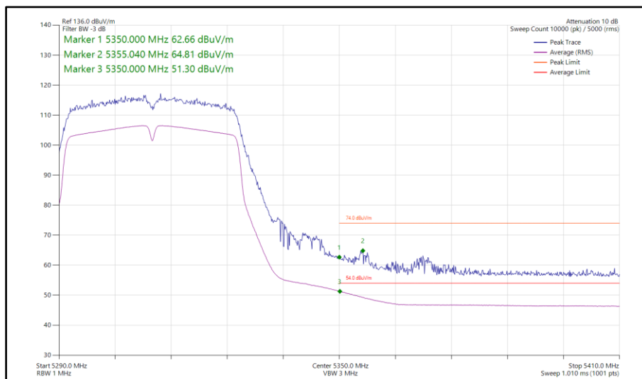
Figure 153 - 802.11n HT40, SISO, Core 0 - 5310 MHz Band Edge Frequency 5350 MHz
