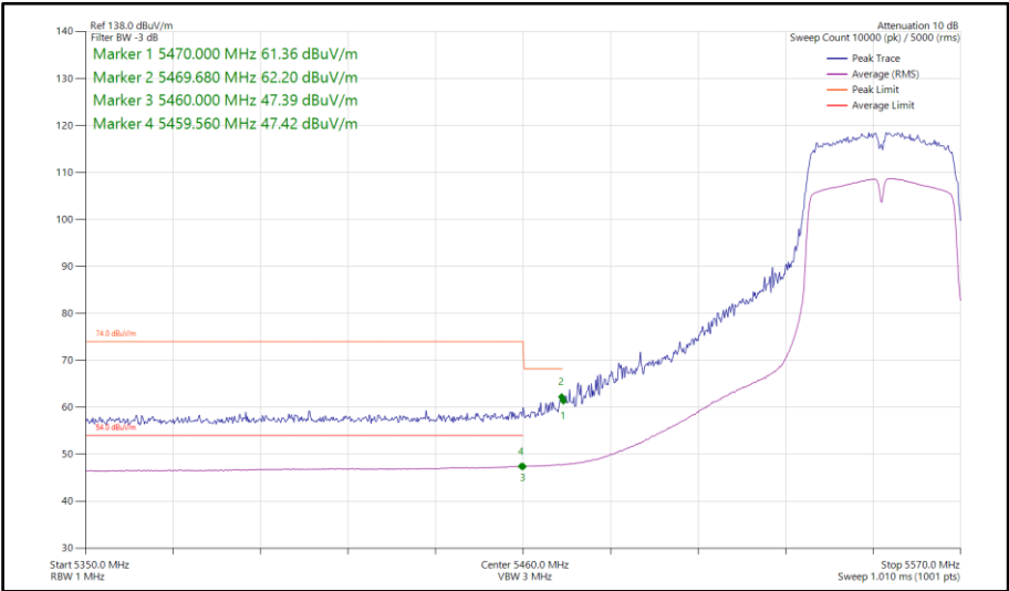
Figure 164 - 802.11n HT40, SISO, Core 0 - 5550 MHz Band Edge Frequency 5460 MHz
