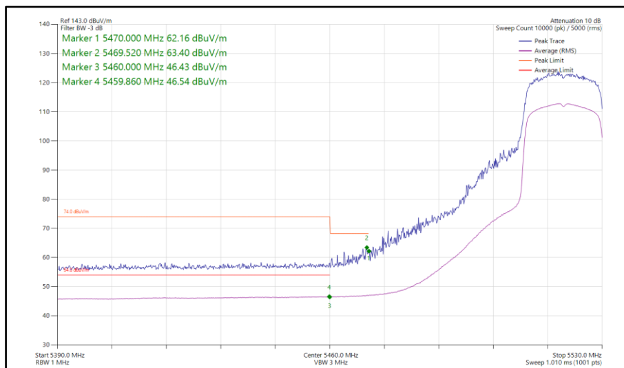
Figure 138 - 802.11ax HE20, SU, TxBF, Core 0-1 - 5520 MHz Band Edge Frequency 5460 MHz
