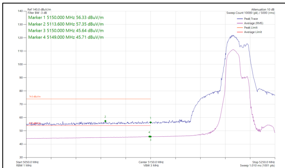
Figure 181 - 802.11be EHT40, RU 106+26-82, SISO, Core 1 - 5230 MHz Band Edge Frequency 5150 MHz
