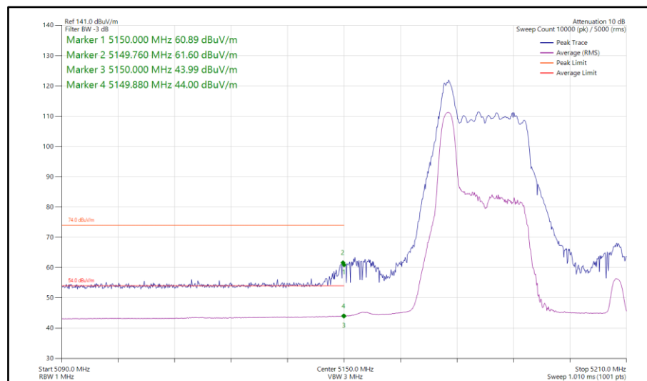
Figure 177 - 802.11ax HE40, RU 26-0, SISO, Core 1 - 5190 MHz Band Edge Frequency 5150 MHz
