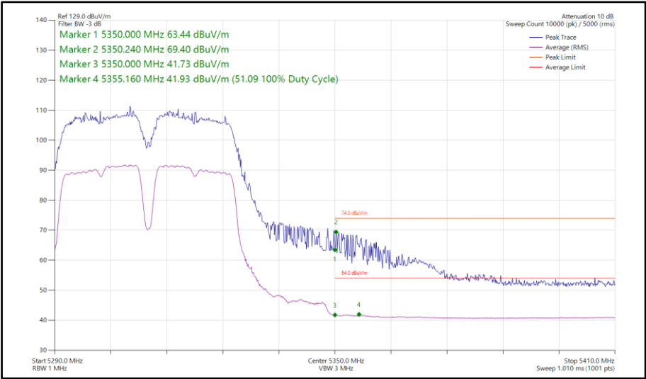
Figure 183 - 802.11a, SISO, Core 1 - 5310 MHz Band Edge Frequency 5350 MHz
