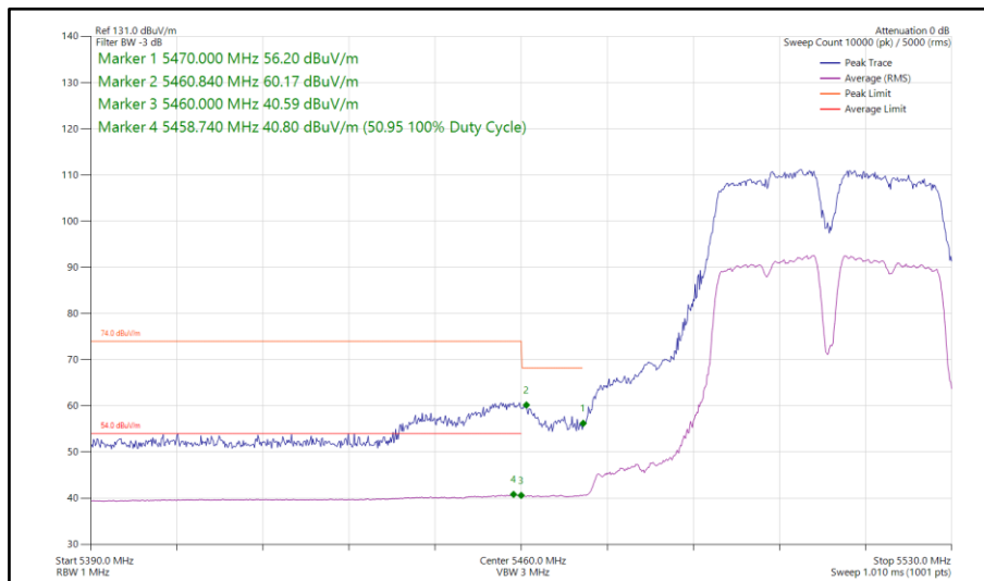
Figure 160 - 802.11a, SISO, Core 0 - 5510 MHz Band Edge Frequency 5460 MHz
