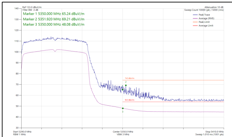
Figure 188 - 802.11ax HE40, SU, SISO, Core 1 - 5310 MHz Band Edge Frequency 5350 MHz
