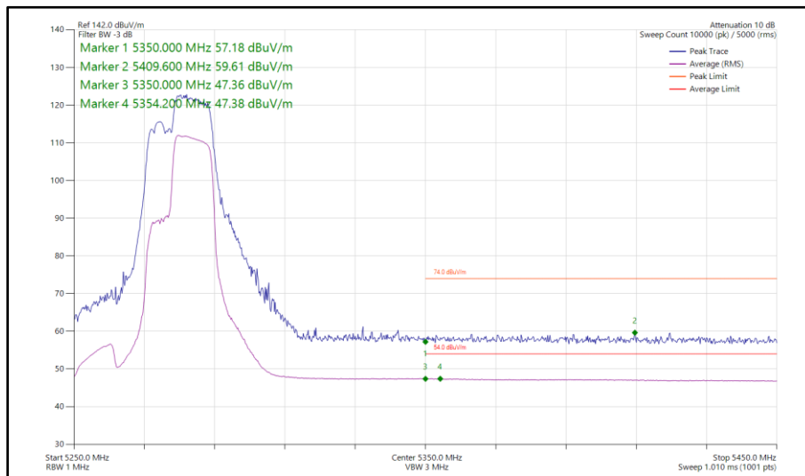
Figure 190 - 802.11be EHT40, RU 106+26-85, SISO, Core 1 - 5270 MHz Band Edge Frequency 5350 MHz
