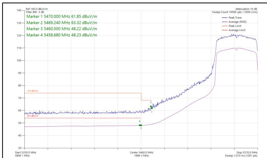
Figure 167 - 802.11ax HE40, SU, SISO, Core 0 - 5550 MHz Band Edge Frequency 5460 MHz
