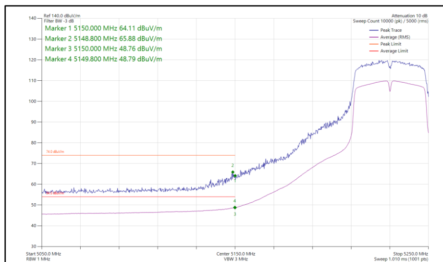
Figure 175 - 802.11n HT40, SISO, Core 1 - 5230 MHz Band Edge Frequency 5150 MHz
