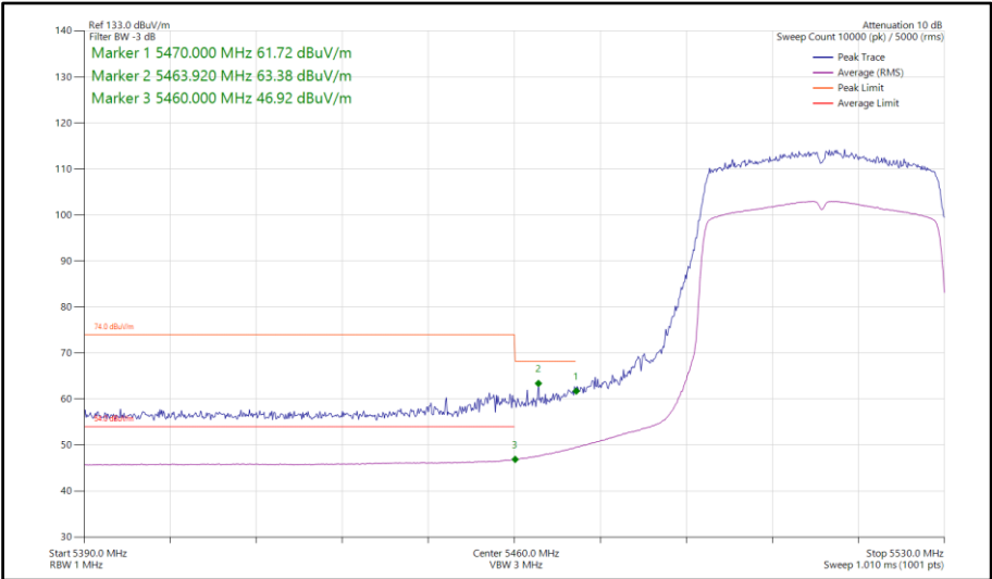
Figure 165 - 802.11ax HE40, SU, SISO, Core 0 - 5510 MHz Band Edge Frequency 5460 MHz
