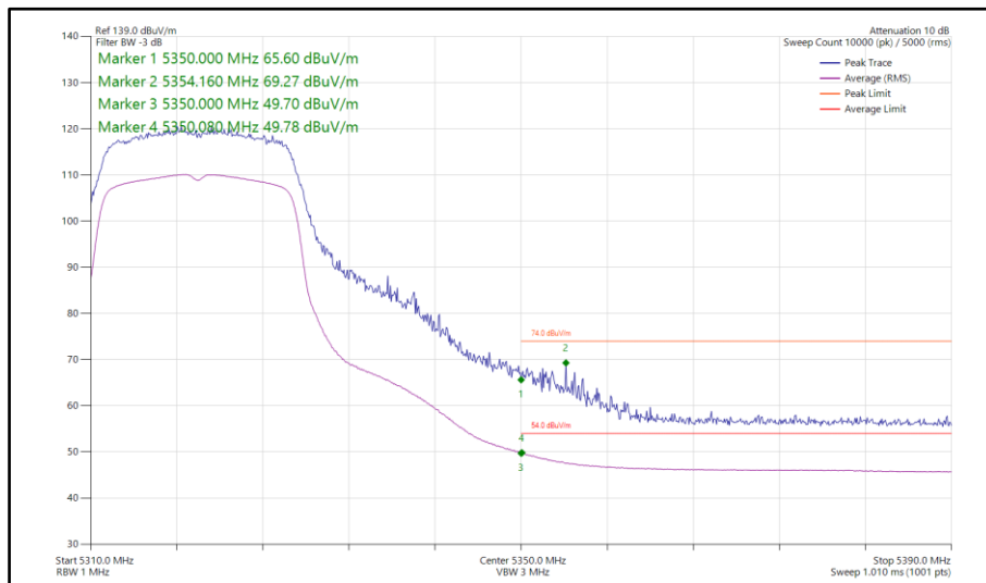
Figure 131 - 802.11ac VHT20, TxBF, Core 0-1 - 5320 MHz Band Edge Frequency 5350 MHz
