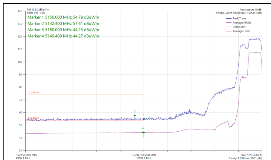
Figure 149 - 802.11be EHT40, RU 106+26-85, SISO, Core 0 - 5230 MHz Band Edge Frequency 5150 MHz
