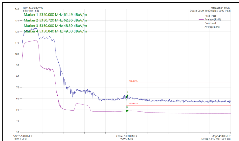
Figure 189 - 802.11ax HE40, RU 106-53, SISO, Core 1 - 5310 MHz Band Edge Frequency 5350 MHz
