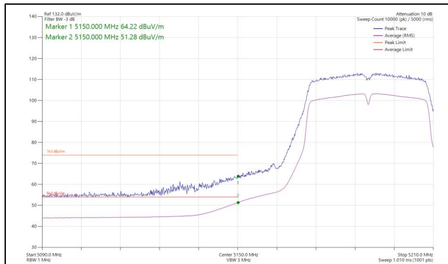
Figure 174 - 802.11n HT40, SISO, Core 1 - 5190 MHz Band Edge Frequency 5150 MHz
