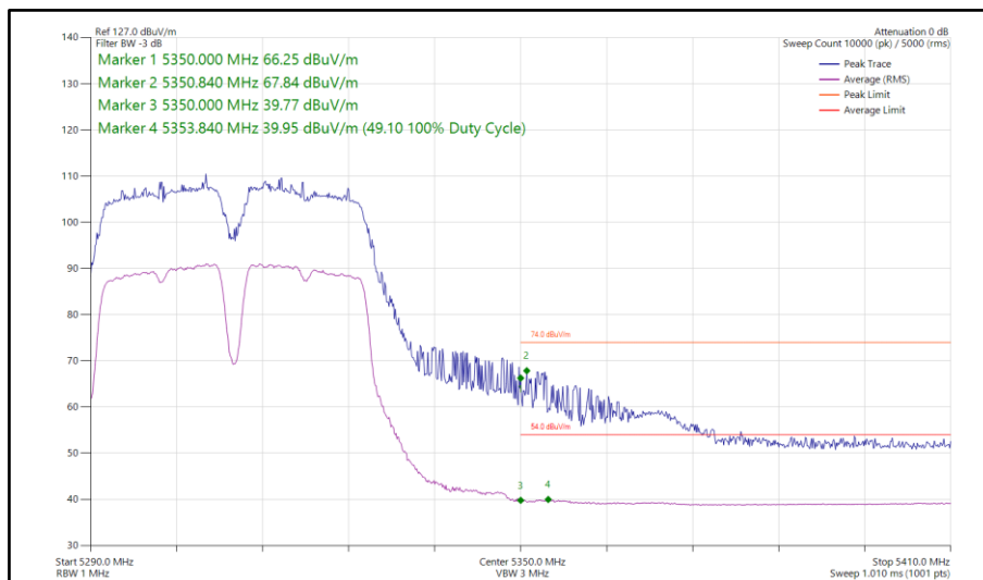
Figure 151 - 802.11a, SISO, Core 0 - 5310 MHz Band Edge Frequency 5350 MHz
