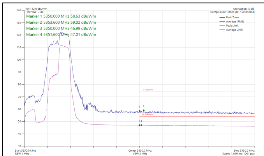
Figure 187 - 802.11ax HE40, RU 106-56, SISO, Core 1 - 5270 MHz Band Edge Frequency 5350 MHz
