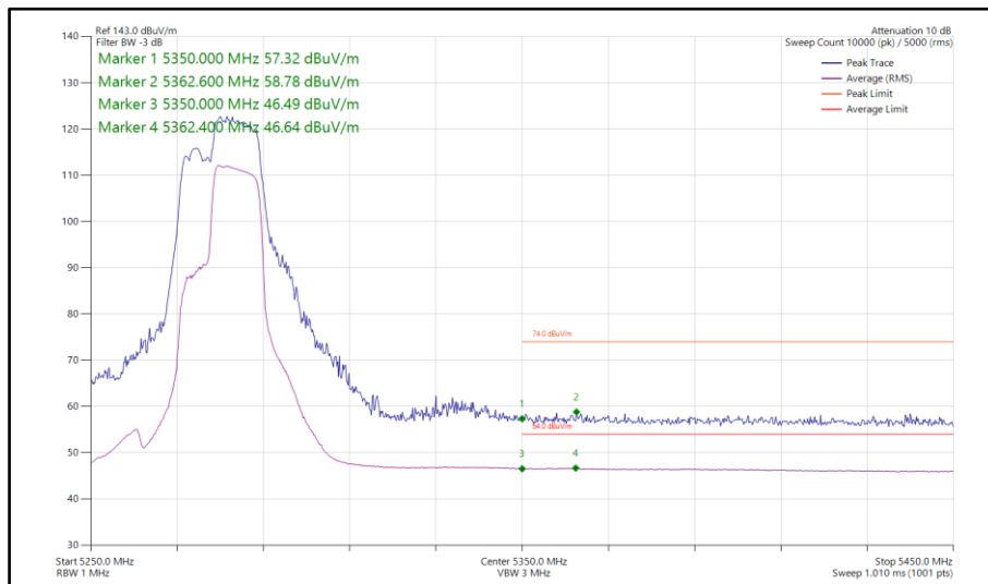
Figure 158 - 802.11be EHT40, RU 106+26-85, SISO, Core 0 - 5270 MHz Band Edge Frequency 5350 MHz
