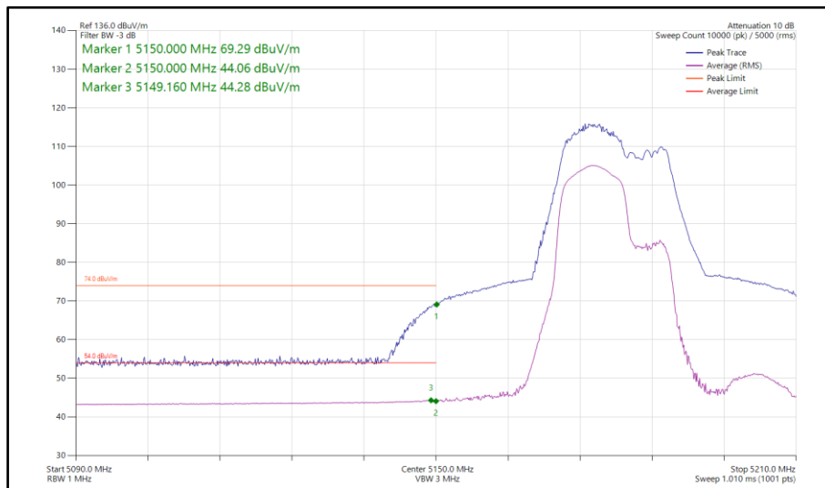
Figure 180 - 802.11be EHT40, RU 106+26-82, SISO, Core 1 - 5190 MHz Band Edge Frequency 5150 MHz
