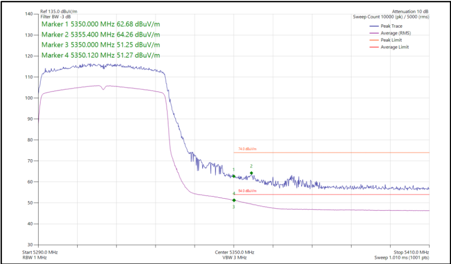
Figure 156 - 802.11ax HE40, SU, SISO, Core 0 - 5310 MHz Band Edge Frequency 5350 MHz
