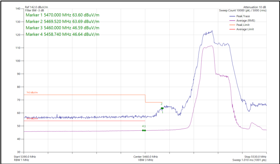
Figure 170 - 802.11be EHT40, RU 52+26-70, SISO, Core 0 - 5510 MHz Band Edge Frequency 5460 MHz
