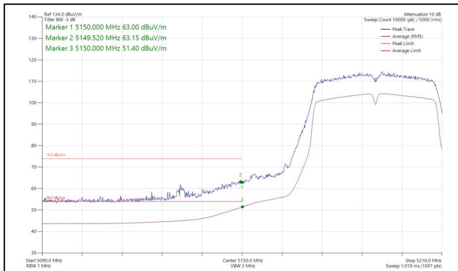
Figure 142 - 802.11n HT40, SISO, Core 0 - 5190 MHz Band Edge Frequency 5150 MHz
