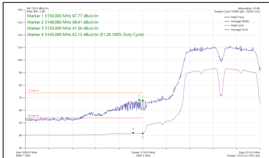
Figure 172 - 802.11a, SISO, Core 1 - 5190 MHz Band Edge Frequency 5150 MHz
