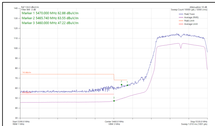
Figure 163 - 802.11n HT40, SISO, Core 0 - 5510 MHz Band Edge Frequency 5460 MHz
