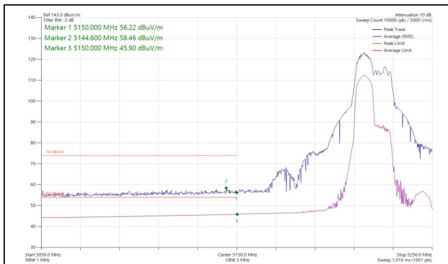
Figure 179 - 802.11ax HE40, RU 106-53, SISO, Core 1 - 5230 MHz Band Edge Frequency 5150 MHz
