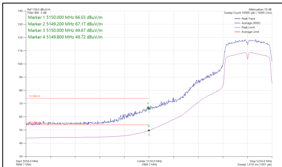
Figure 143 - 802.11n HT40, SISO, Core 0 - 5230 MHz Band Edge Frequency 5150 MHz
