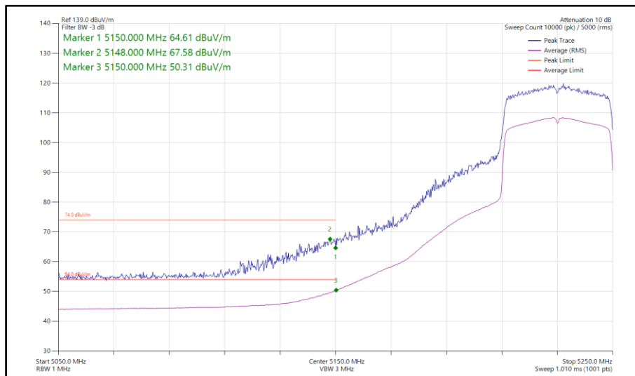
Figure 146 - 802.11ax HE40, SU, SISO, Core 0 - 5230 MHz Band Edge Frequency 5150 MHz
