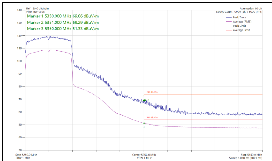
Figure 154 - 802.11ax HE40, SU, SISO, Core 0 - 5270 MHz Band Edge Frequency 5350 MHz
