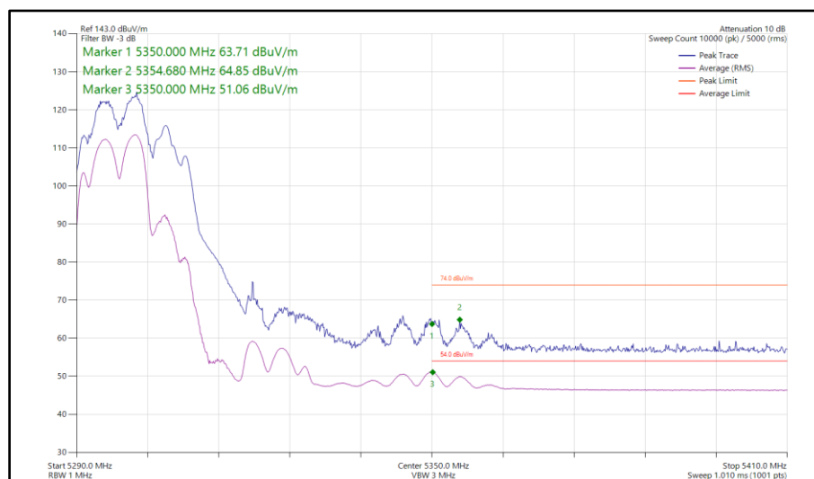
Figure 251 - 802.11be EHT40, RU 106+26-82, SDM, Core 0-1 - 5310 MHz Band Edge Frequency 5350 MHz
