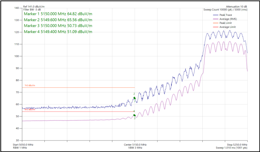
Figure 206 - 802.11n HT40, CDD, Core 0-1 - 5230 MHz Band Edge Frequency 5150 MHz
