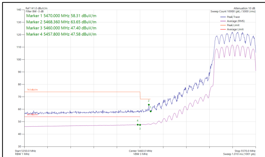
Figure 231 - 802.11ax HE40, SU, CDD, Core 0-1 - 5550 MHz Band Edge Frequency 5460 MHz
