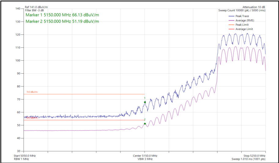
Figure 209 - 802.11ax HE40, SU, CDD, Core 0-1 - 5230 MHz Band Edge Frequency 5150 MHz
