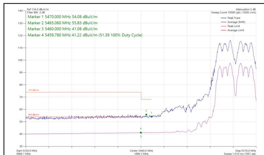
Figure 224 - 802.11a, CDD, Core 0-1 - 5550 MHz Band Edge Frequency 5460 MHz
