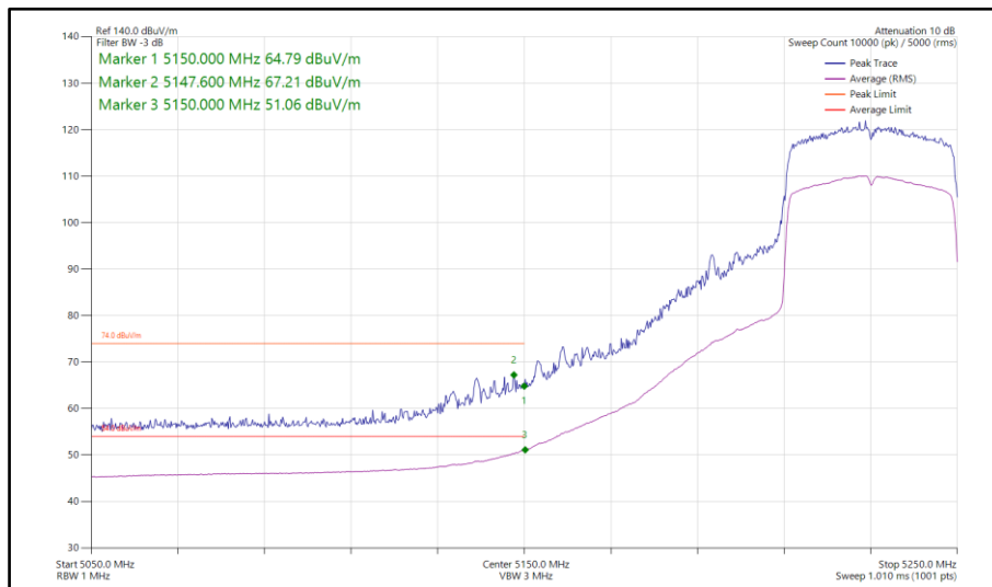
Figure 240 - 802.11ax HE40, SU, SDM, Core 0-1 - 5230 MHz Band Edge Frequency 5150 MHz
