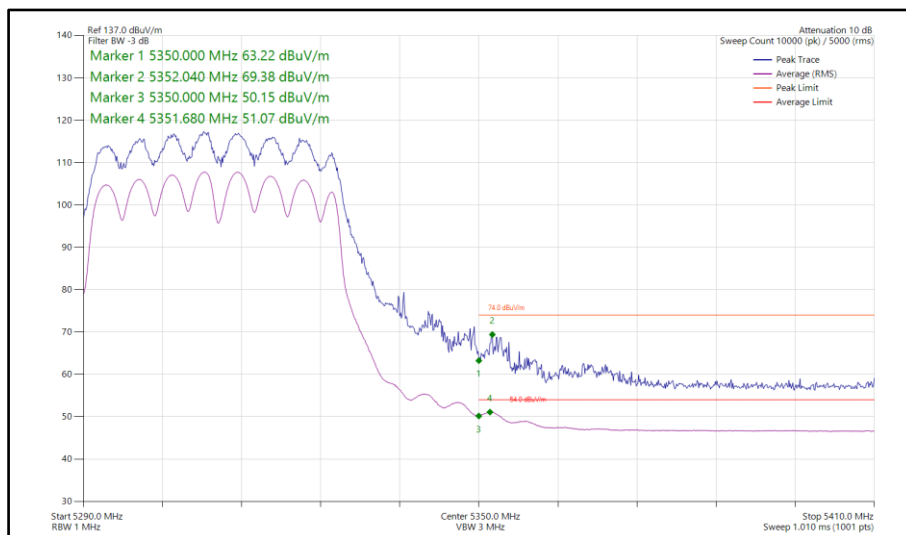
Figure 216 - 802.11n HT40, CDD, Core 0-1 - 5310 MHz Band Edge Frequency 5350 MHz
