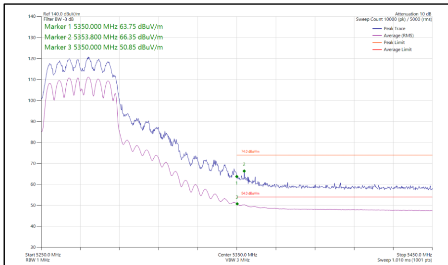
Figure 215 - 802.11n HT40, CDD, Core 0-1 - 5270 MHz Band Edge Frequency 5350 MHz
