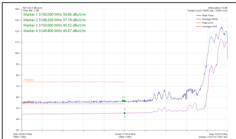
Figure 241 - 802.11ax HE40, RU 106-56, SDM, Core 0-1 - 5230 MHz Band Edge Frequency 5150 MHz
