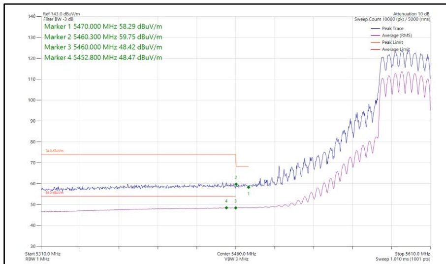
Figure 233 - 802.11ax HE40, SU, CDD, Core 0-1 - 5590 MHz Band Edge Frequency 5460 MHz
