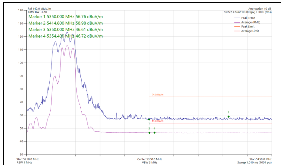
Figure 250 - 802.11be EHT40, RU 106+26-85, SDM, Core 0-1 - 5270 MHz Band Edge Frequency 5350 MHz
