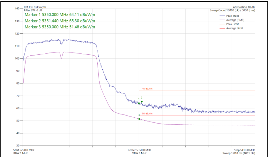
Figure 245 - 802.11n HT40, SDM, Core 0-1 - 5310 MHz Band Edge Frequency 5350 MHz
