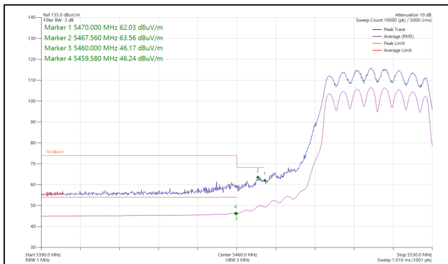
Figure 226 - 802.11n HT40, CDD, Core 0-1 - 5510 MHz Band Edge Frequency 5460 MHz
