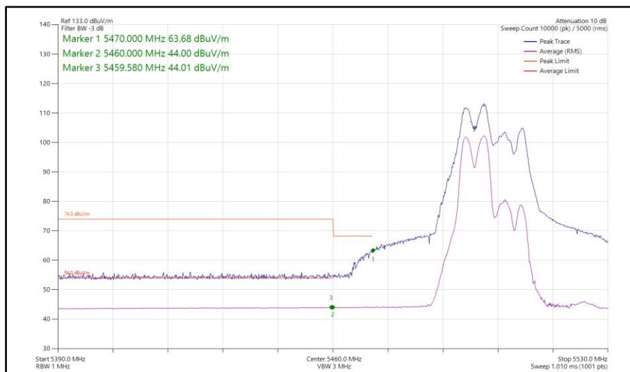
Figure 234 - 802.11be EHT40, RU 52+26-70, CDD, Core 0-1 - 5510 MHz Band Edge Frequency 5460 MHz
