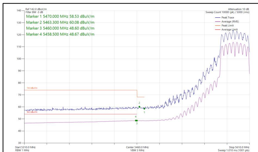
Figure 228 - 802.11n HT40, CDD, Core 0-1 - 5590 MHz Band Edge Frequency 5460 MHz
