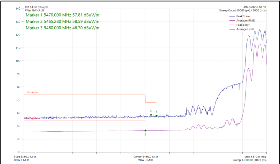
Figure 235 - 802.11be EHT40, RU 106+26-85, CDD, Core 0-1 - 5550 MHz Band Edge Frequency 5460 MHz
