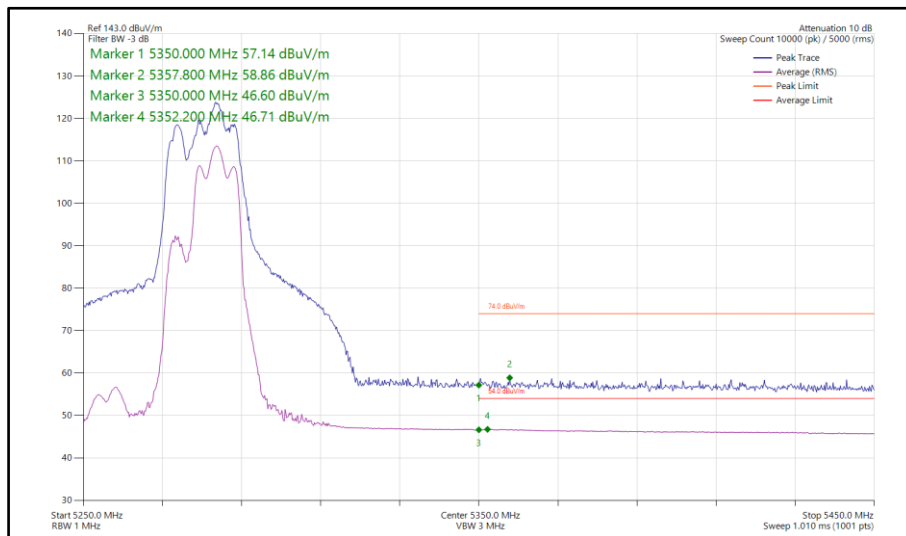
Figure 221 - 802.11be EHT40, RU 106+26-85, CDD, Core 0-1 - 5270 MHz Band Edge Frequency 5350 MHz
