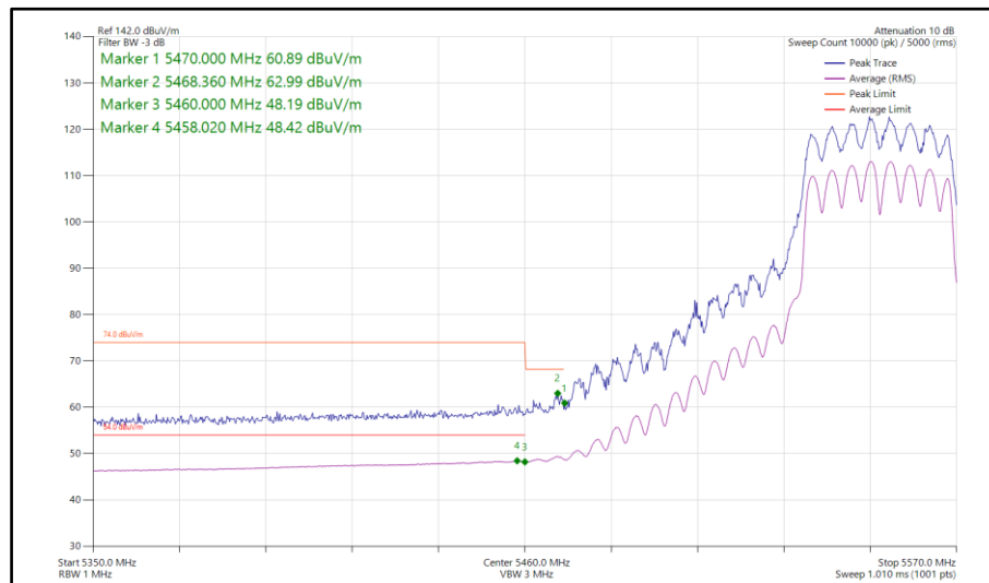
Figure 227 - 802.11n HT40, CDD, Core 0-1 - 5550 MHz Band Edge Frequency 5460 MHz
