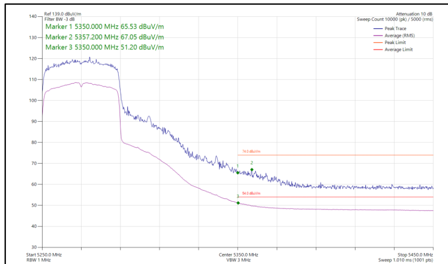
Figure 246 - 802.11ax HE40, SU, SDM, Core 0-1 - 5270 MHz Band Edge Frequency 5350 MHz
