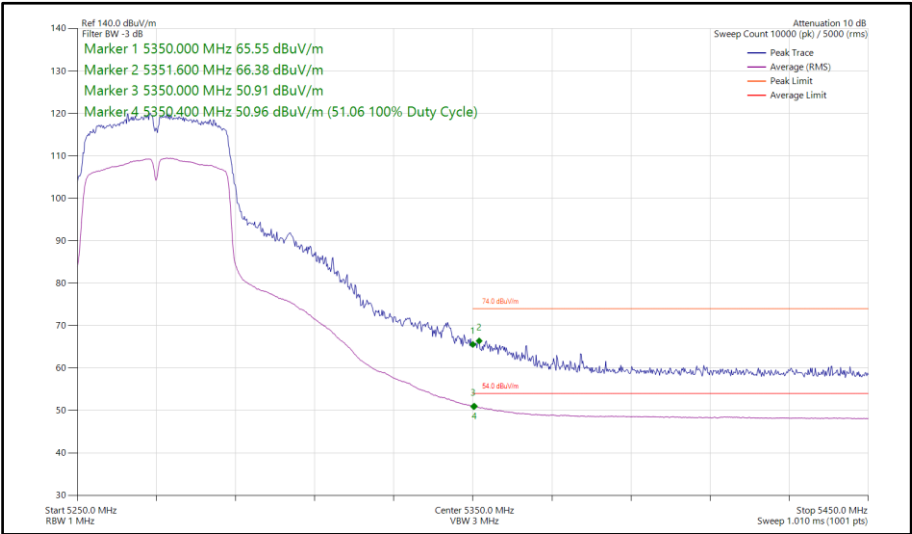
Figure 244 - 802.11n HT40, SDM, Core 0-1 - 5270 MHz Band Edge Frequency 5350 MHz
