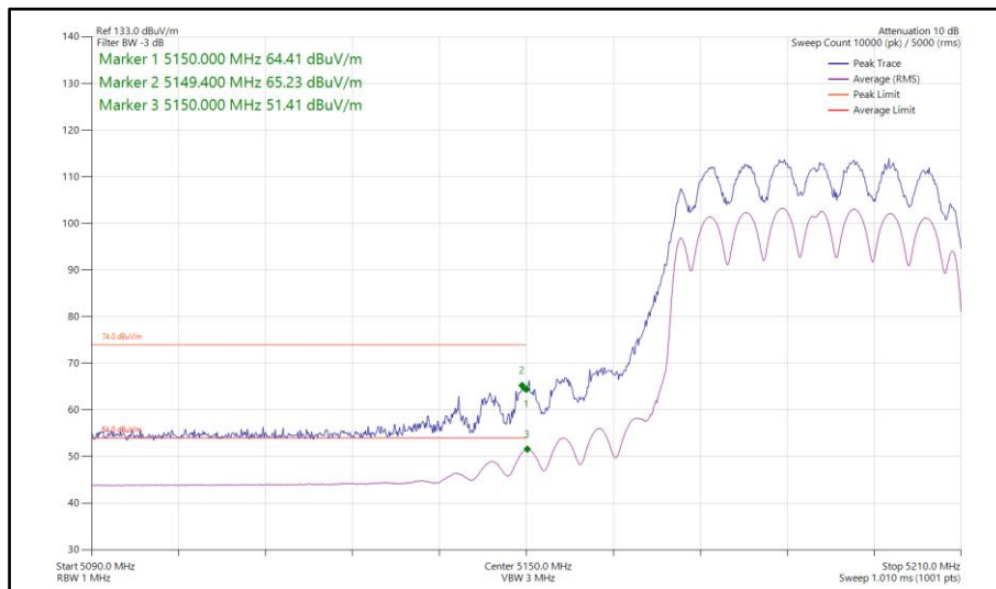
Figure 207 - 802.11ax HE40, SU, CDD, Core 0-1 - 5190 MHz Band Edge Frequency 5150 MHz
