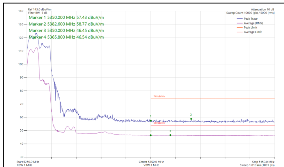
Figure 247 - 802.11ax HE40, RU 106-53, SDM, Core 0-1 - 5270 MHz Band Edge Frequency 5350 MHz
