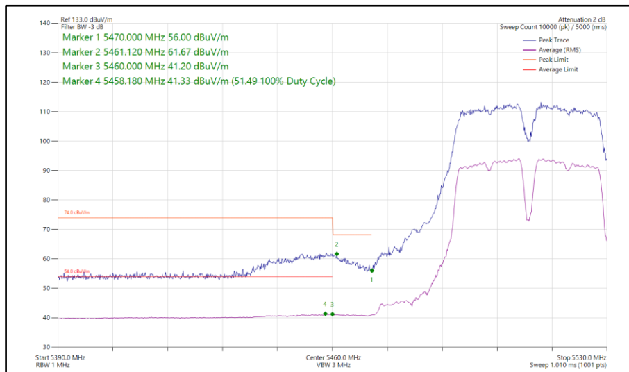
Figure 192 - 802.11a, SISO, Core 1 - 5510 MHz Band Edge Frequency 5460 MHz
