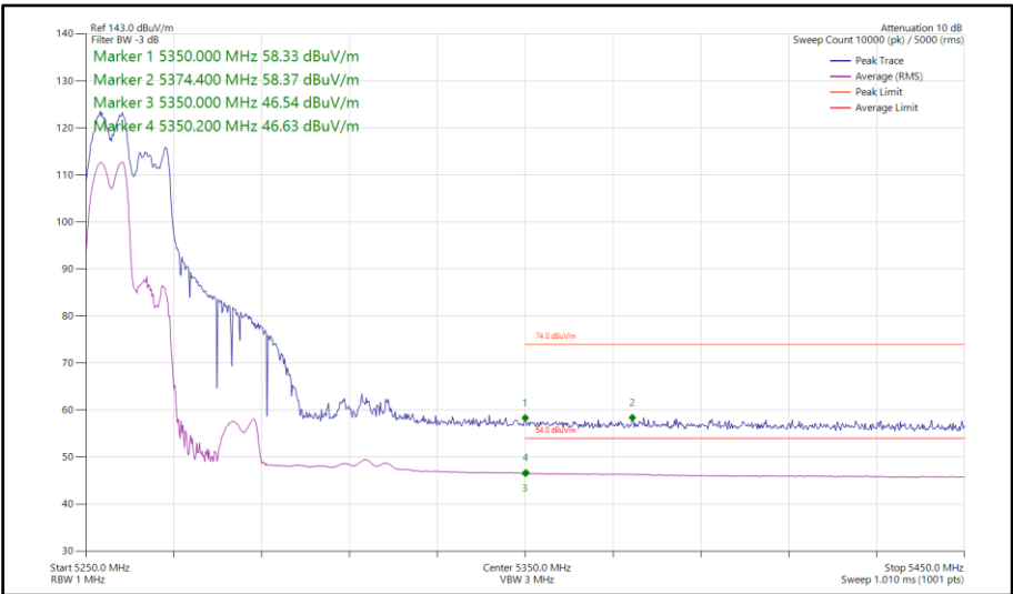
Figure 218 - 802.11ax HE40, RU 106-53, CDD, Core 0-1 - 5270 MHz Band Edge Frequency 5350 MHz
