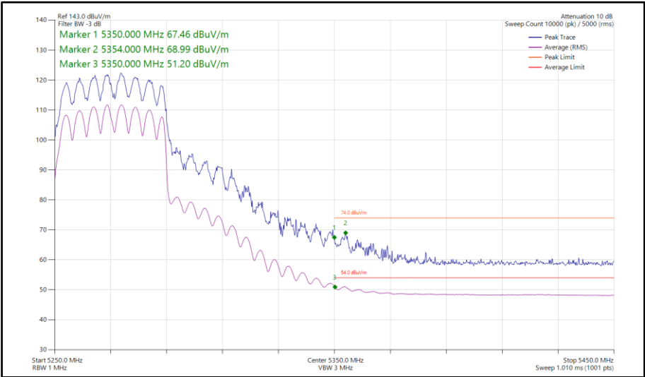
Figure 217 - 802.11ax HE40, SU, CDD, Core 0-1 - 5270 MHz Band Edge Frequency 5350 MHz
