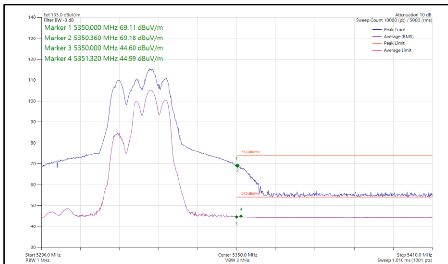
Figure 222 - 802.11be EHT40, RU 106+26-85, CDD, Core 0-1 - 5310 MHz Band Edge Frequency 5350 MHz
