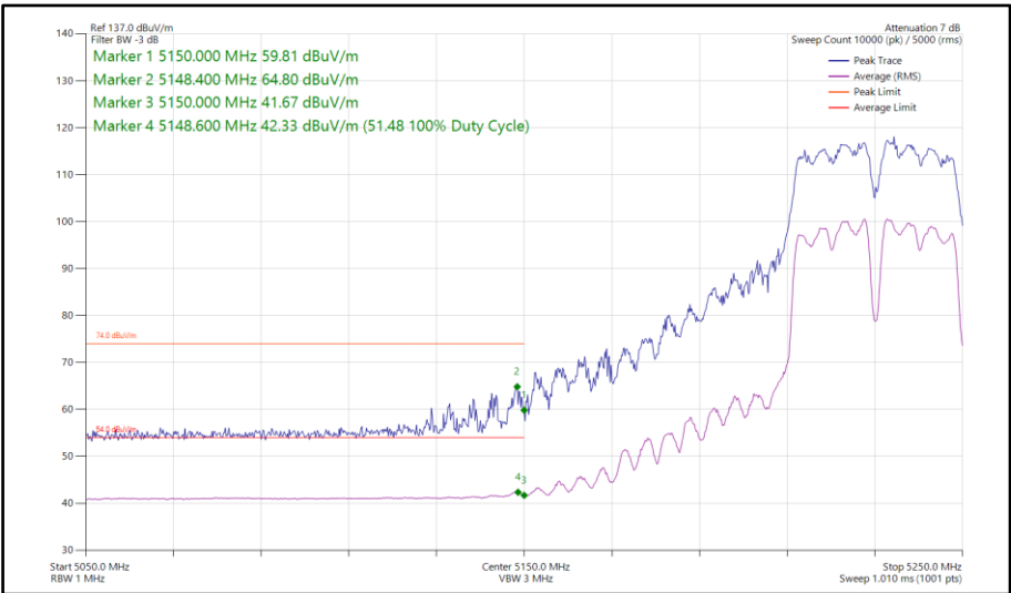
Figure 204 - 802.11a, CDD, Core 0-1 - 5230 MHz Band Edge Frequency 5150 MHz
