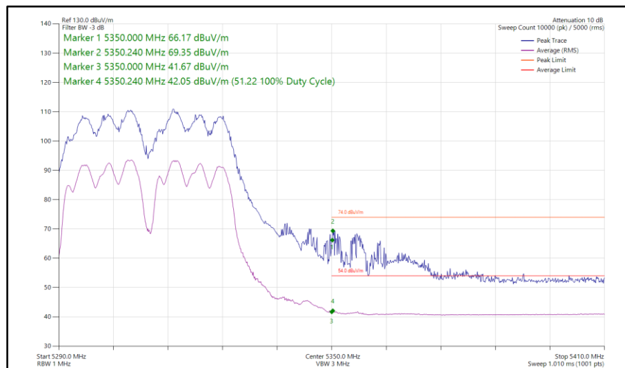
Figure 214 - 802.11a, CDD, Core 0-1 - 5310 MHz Band Edge Frequency 5350 MHz
