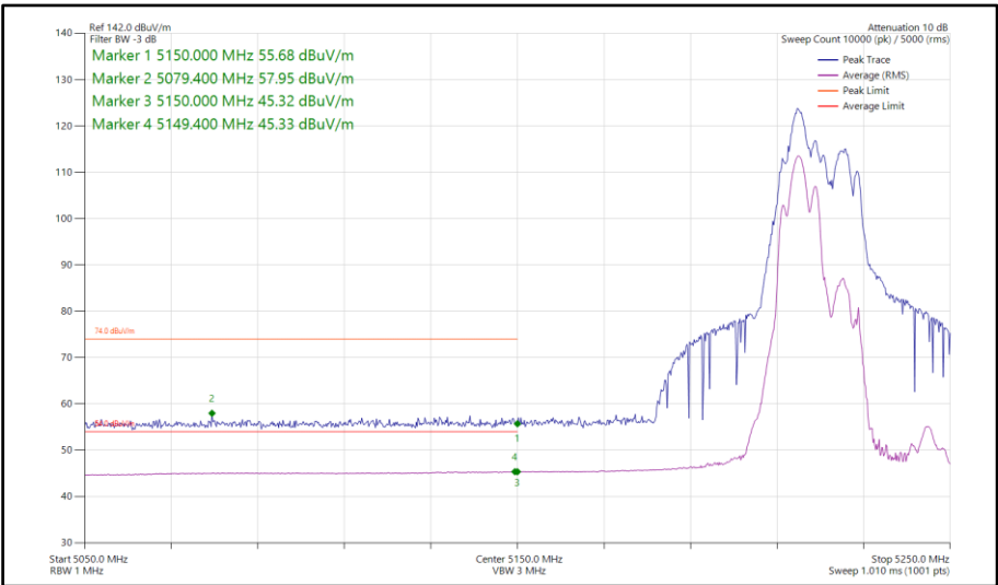
Figure 210 - 802.11ax HE40, RU 106-53, CDD, Core 0-1 - 5230 MHz Band Edge Frequency 5150 MHz
