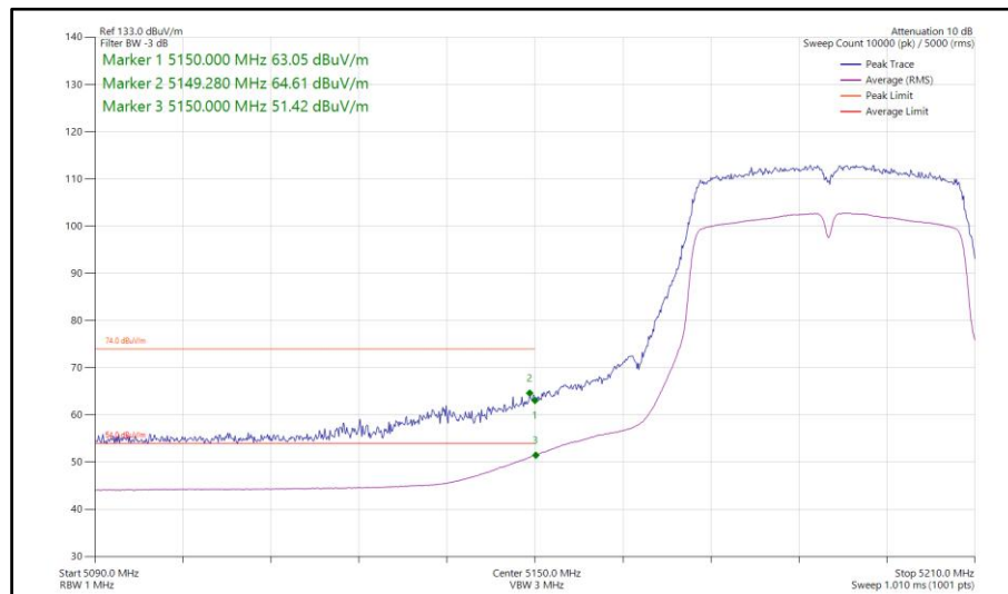
Figure 236 - 802.11n HT40, SDM, Core 0-1 - 5190 MHz Band Edge Frequency 5150 MHz
