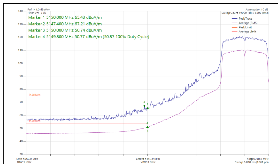
Figure 237 - 802.11n HT40, SDM, Core 0-1 - 5230 MHz Band Edge Frequency 5150 MHz
