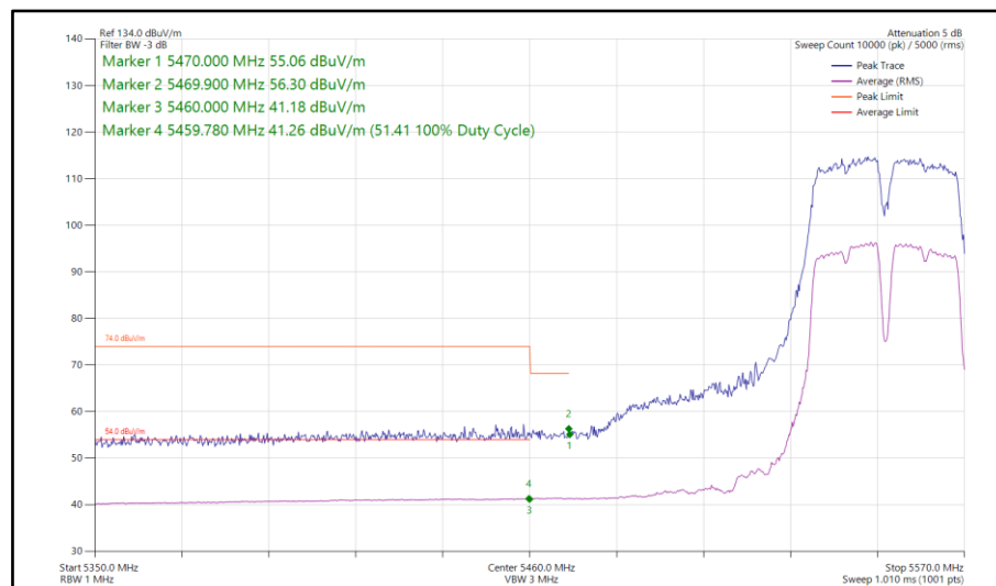
Figure 193 - 802.11a, SISO, Core 1 - 5550 MHz Band Edge Frequency 5460 MHz
