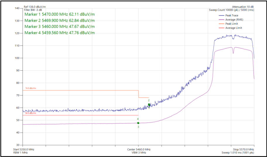
Figure 196 - 802.11n HT40, SISO, Core 1 - 5550 MHz Band Edge Frequency 5460 MHz
