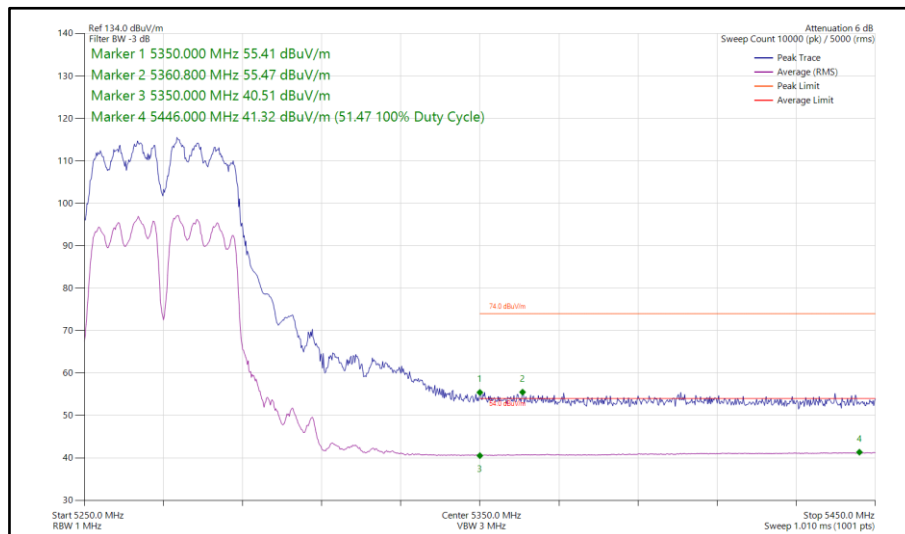
Figure 213 - 802.11a, CDD, Core 0-1 - 5270 MHz Band Edge Frequency 5350 MHz
