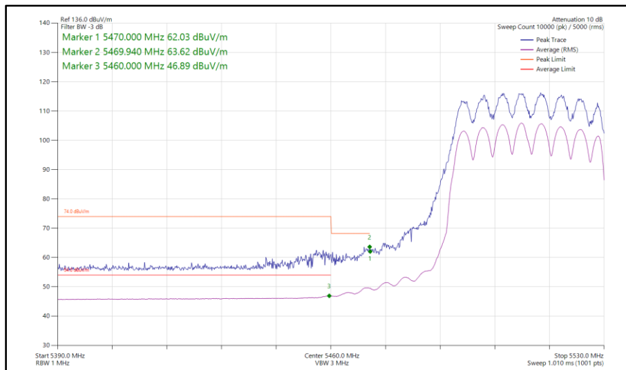
Figure 229 - 802.11ax HE40, SU, CDD, Core 0-1 - 5510 MHz Band Edge Frequency 5460 MHz
