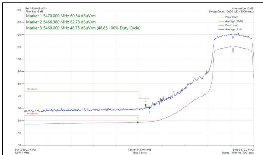
Figure 253 - 802.11n HT40, SDM, Core 0-1 - 5550 MHz Band Edge Frequency 5460 MHz
