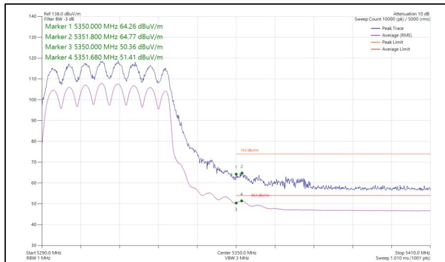
Figure 219 - 802.11ax HE40, SU, CDD, Core 0-1 - 5310 MHz Band Edge Frequency 5350 MHz
