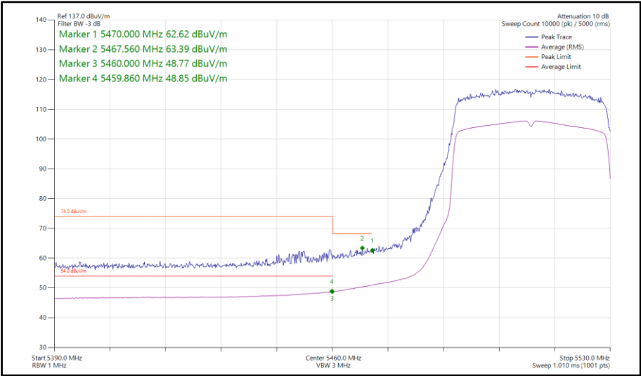
Figure 197 - 802.11ax HE40, SU, SISO, Core 1 - 5510 MHz Band Edge Frequency 5460 MHz
