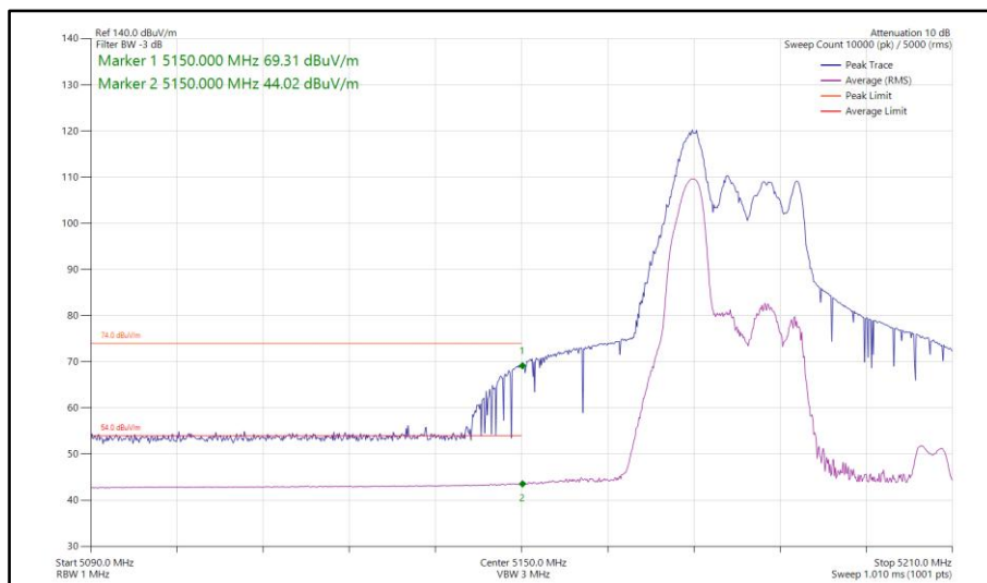
Figure 208 - 802.11ax HE40, RU 52-37, CDD, Core 0-1 - 5190 MHz Band Edge Frequency 5150 MHz
