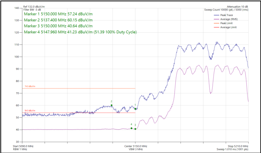
Figure 203 - 802.11a, CDD, Core 0-1 - 5190 MHz Band Edge Frequency 5150 MHz
