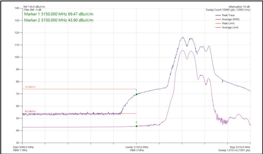
Figure 211 - 802.11be EHT40, RU 106+26-82, CDD, Core 0-1 - 5190 MHz Band Edge Frequency 5150 MHz
