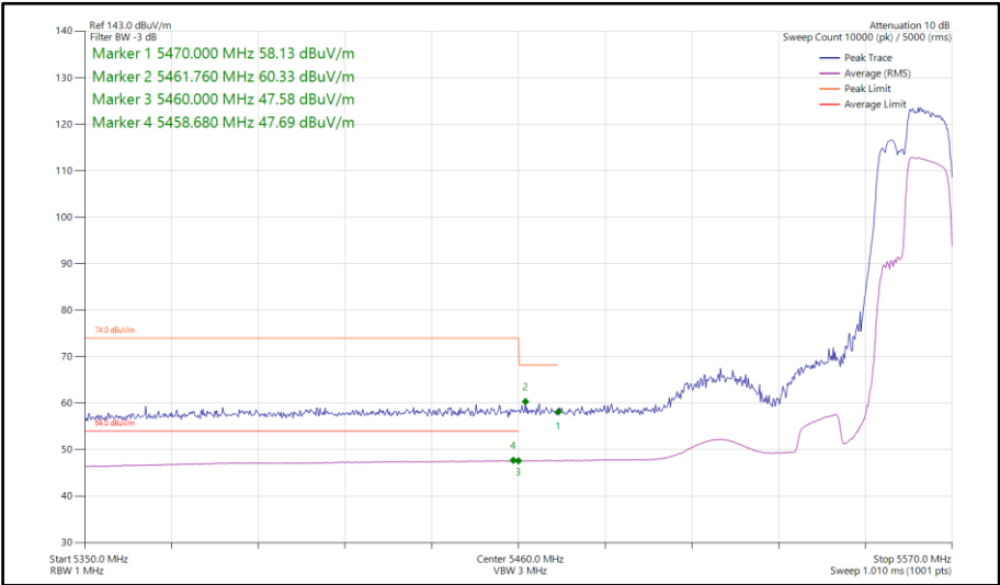
Figure 202 - 802.11be EHT40, RU 106+26-85, SISO, Core 1 - 5550 MHz Band Edge Frequency 5460 MHz
