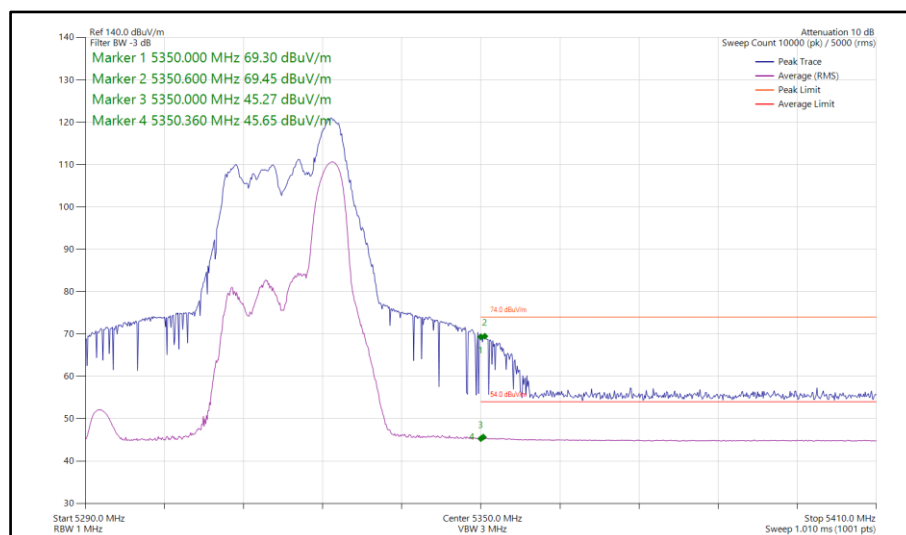
Figure 220 - 802.11ax HE40, RU 52-44, CDD, Core 0-1 - 5310 MHz Band Edge Frequency 5350 MHz
