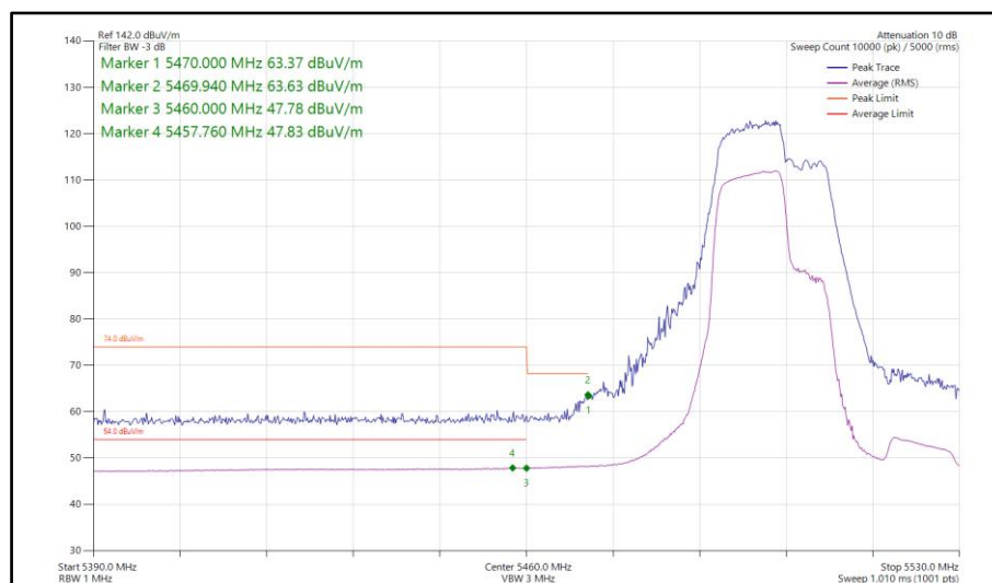
Figure 201 - 802.11be EHT40, RU106+26-82, SISO, Core 1 - 5510 MHz Band Edge Frequency 5460 MHz
