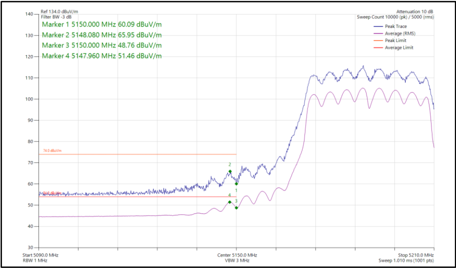
Figure 205 - 802.11n HT40, CDD, Core 0-1 - 5190 MHz Band Edge Frequency 5150 MHz
