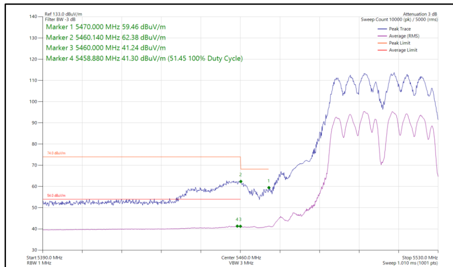
Figure 223 - 802.11a, CDD, Core 0-1 - 5510 MHz Band Edge Frequency 5460 MHz
