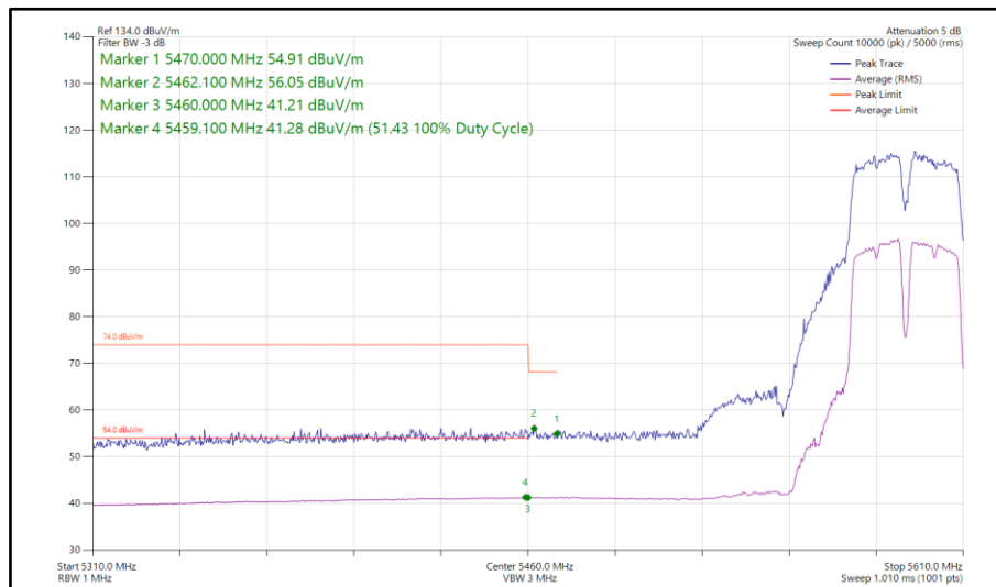
Figure 194 - 802.11a, SISO, Core 1 - 5590 MHz Band Edge Frequency 5460 MHz
