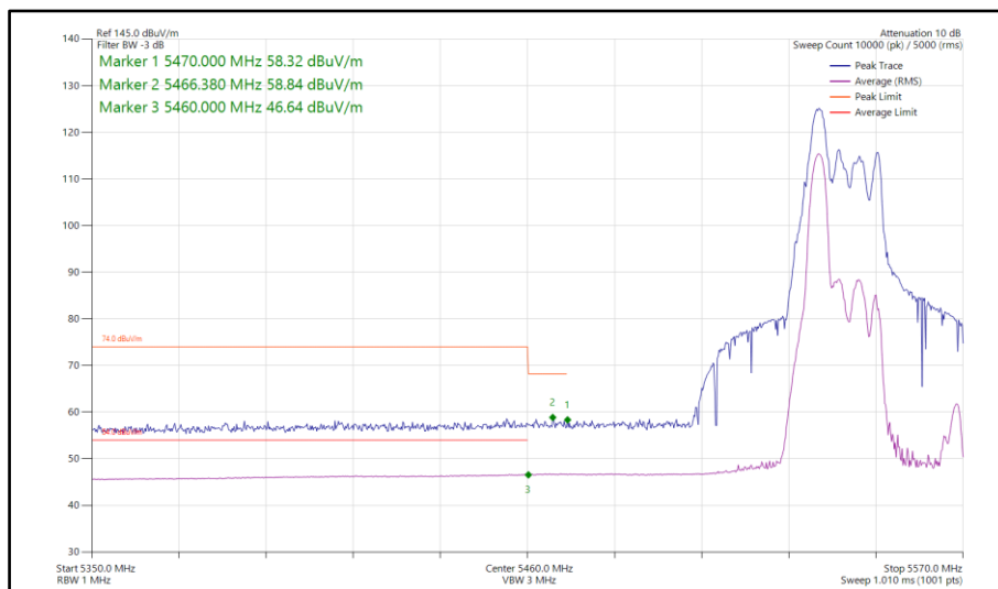
Figure 232 - 802.11ax HE40, RU 52-37, CDD, Core 0-1 - 5550 MHz Band Edge Frequency 5460 MHz
