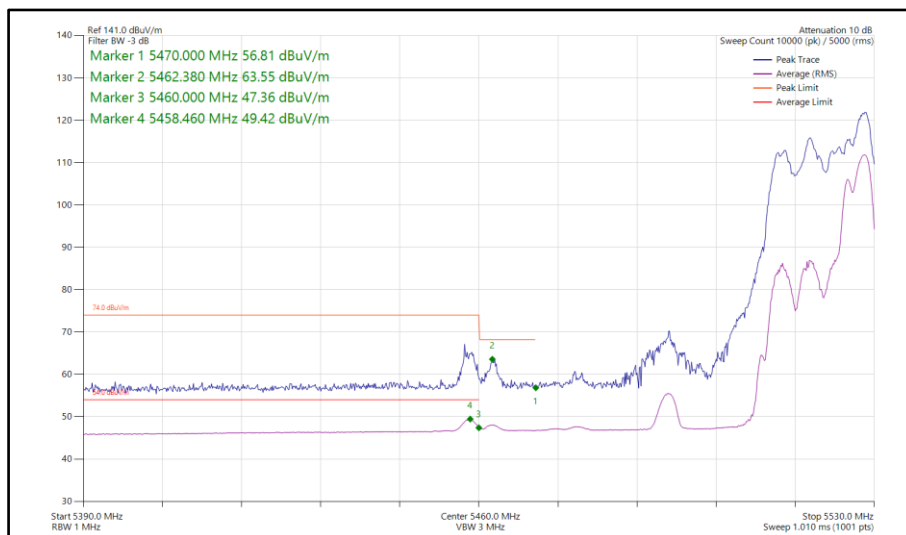
Figure 230 - 802.11ax HE40, RU 52-44, CDD, Core 0-1 - 5510 MHz Band Edge Frequency 5460 MHz
