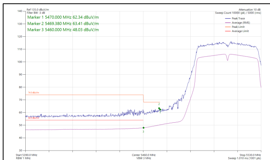
Figure 195 - 802.11n HT40, SISO, Core 1 - 5510 MHz Band Edge Frequency 5460 MHz
