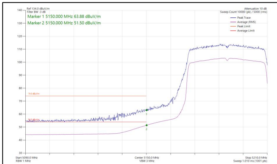
Figure 238 - 802.11ax HE40, SU, SDM, Core 0-1 - 5190 MHz Band Edge Frequency 5150 MHz
