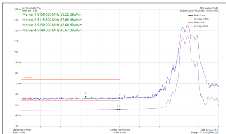
Figure 243 - 802.11be EHT40, RU 106+26-82, SDM, Core 0-1 - 5230 MHz Band Edge Frequency 5150 MHz
