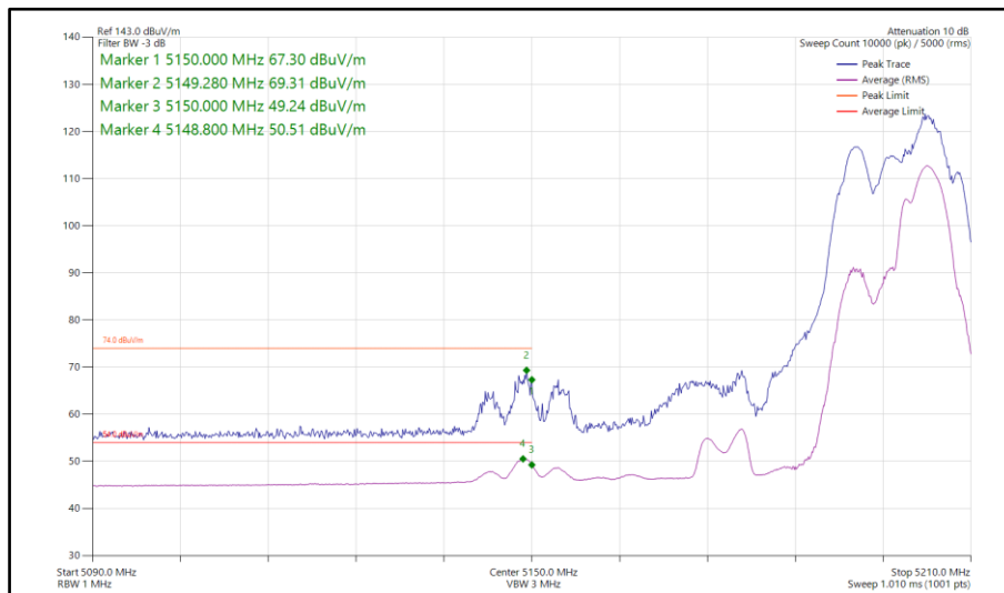
Figure 242 - 802.11be EHT40, RU 52+26-75, SDM, Core 0-1 - 5190 MHz Band Edge Frequency 5150 MHz
