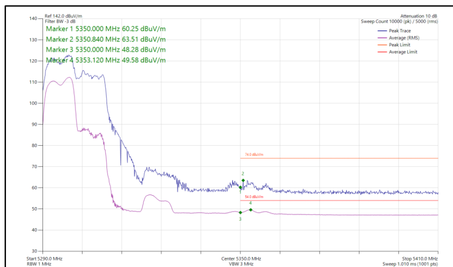
Figure 249 - 802.11ax HE40, RU 106-53, SDM, Core 0-1 - 5310 MHz Band Edge Frequency 5350 MHz
