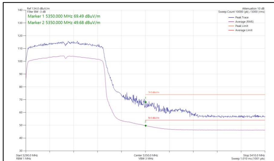
Figure 248 - 802.11ax HE40, SU, SDM, Core 0-1 - 5310 MHz Band Edge Frequency 5350 MHz
