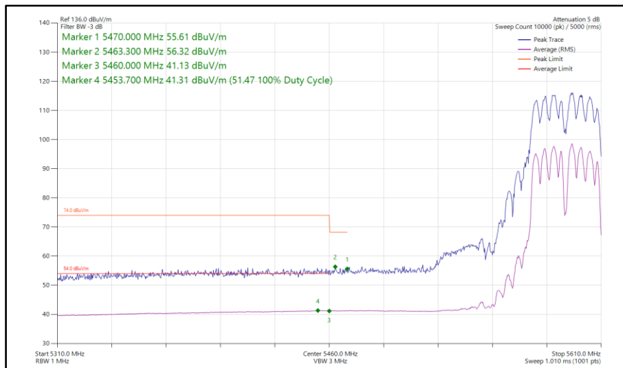
Figure 225 - 802.11a, CDD, Core 0-1 - 5590 MHz Band Edge Frequency 5460 MHz
