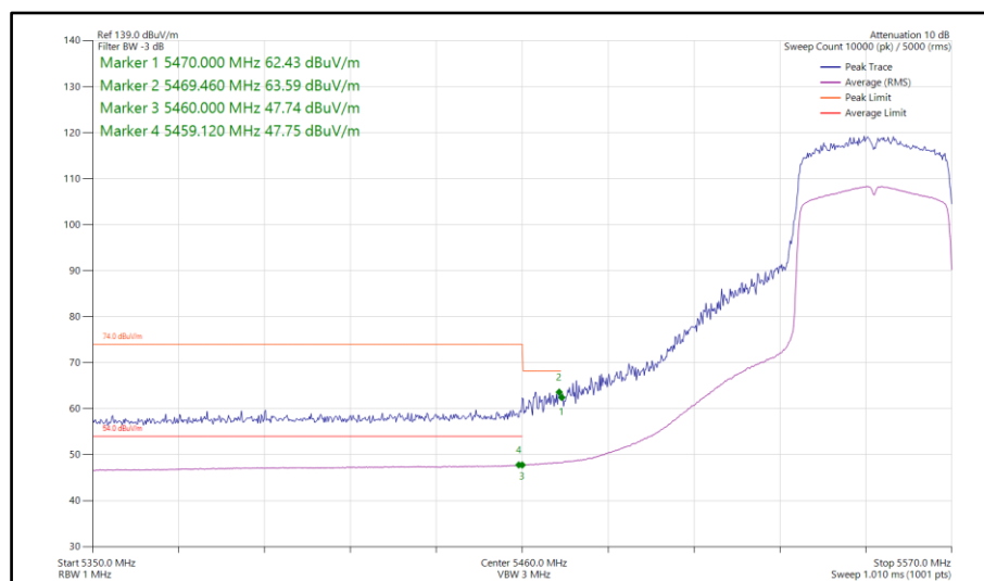
Figure 199 - 802.11ax HE40, SU, SISO, Core 1 - 5550 MHz Band Edge Frequency 5460 MHz
