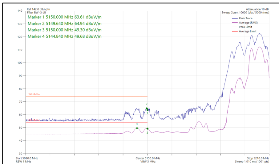
Figure 239 - 802.11ax HE40, RU 106-56, SDM, Core 0-1 - 5190 MHz Band Edge Frequency 5150 MHz
