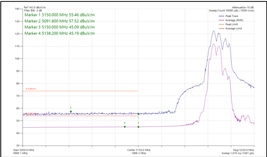
Figure 212 - 802.11be EHT40, RU 106+26-82, CDD, Core 0-1 - 5230 MHz Band Edge Frequency 5150 MHz
