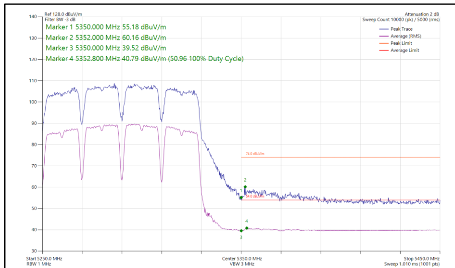
Figure 277 - 802.11a, SISO, Core 0 - 5290 MHz Band Edge Frequency 5350 MHz
