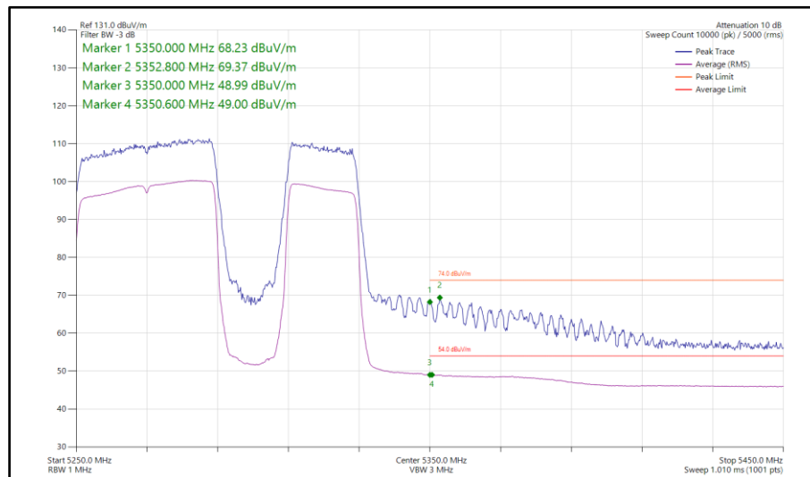
Figure 301 - 802.11be EHT80, RU 484+242-92, SISO, Core 1 - 5290 MHz Band Edge Frequency 5350 MHz
