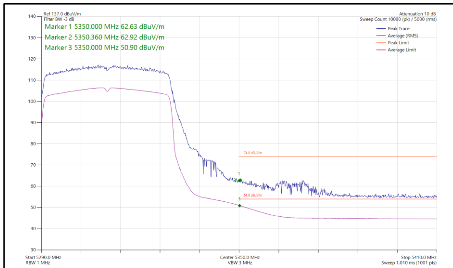
Figure 267 - 802.11ax HE40, SU, TxBF, Core 0-1 - 5310 MHz Band Edge Frequency 5350 MHz
