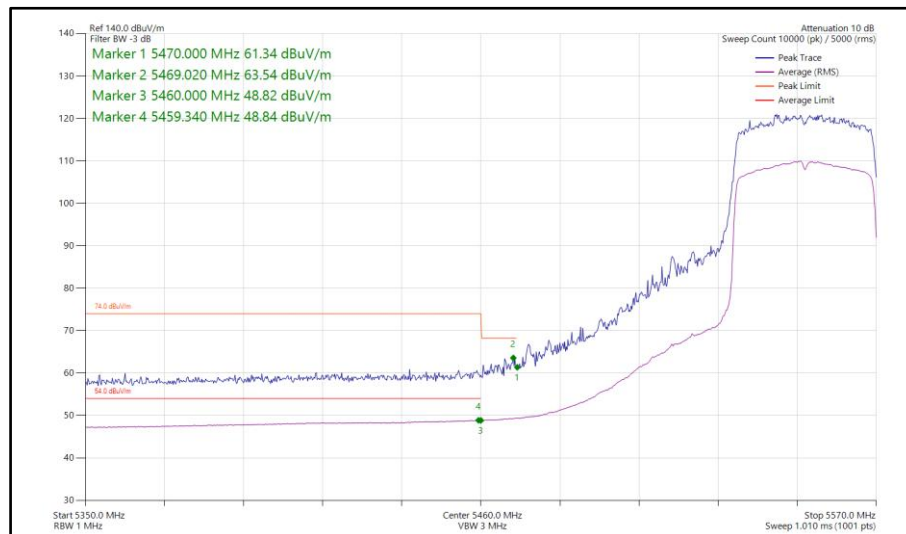
Figure 256 - 802.11ax HE40, SU, SDM, Core 0-1 - 5550 MHz Band Edge Frequency 5460 MHz
