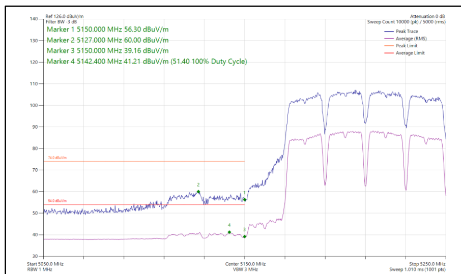
Figure 272 - 802.11a, SISO, Core 0 - 5210 MHz Band Edge Frequency 5150 MHz
