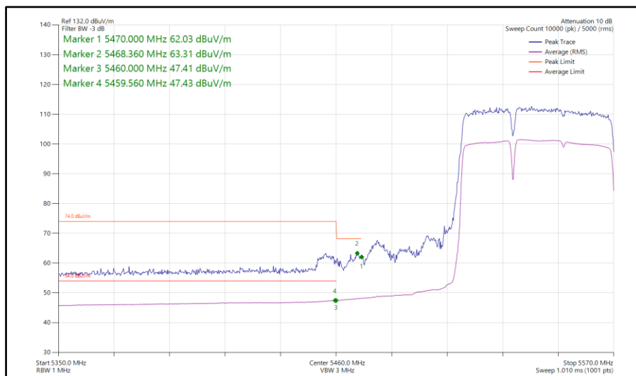
Figure 310 - 802.11be EHT80, RU 484+242-90, SISO, Core 1 - 5530 MHz Band Edge Frequency 5460 MHz
