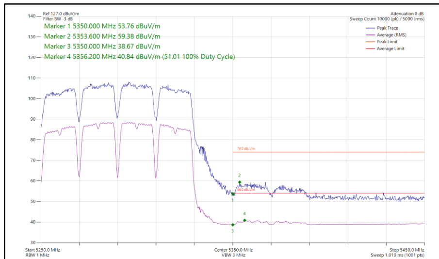
Figure 297 - 802.11a, SISO, Core 1 - 5290 MHz Band Edge Frequency 5350 MHz
