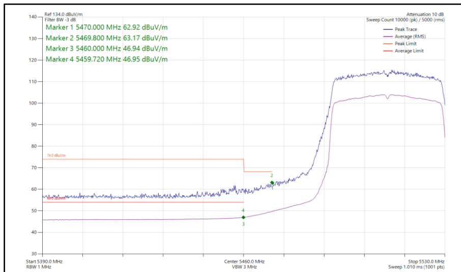
Figure 254 - 802.11ax HE40, SU, SDM, Core 0-1 - 5510 MHz Band Edge Frequency 5460 MHz
