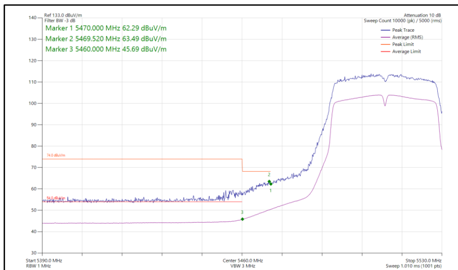
Figure 268 - 802.11ac VHT40, TxBF, Core 0-1 - 5510 MHz Band Edge Frequency 5460 MHz
