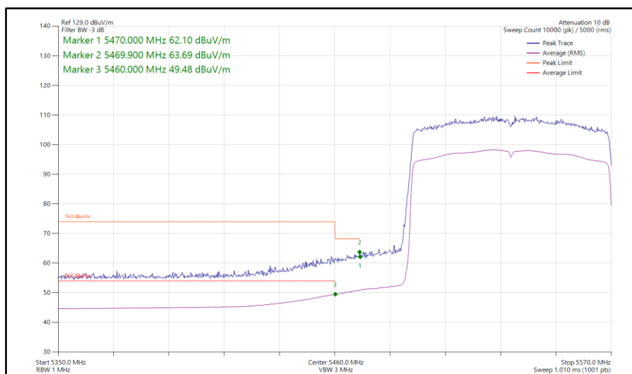
Figure 286 - 802.11ax HE80, SU, SISO, Core 0 - 5530 MHz Band Edge Frequency 5460 MHz
