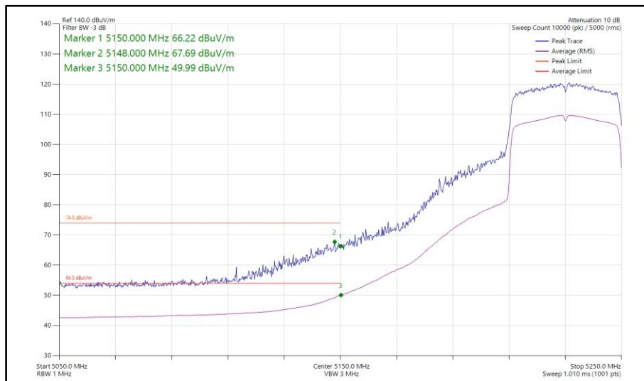
Figure 263 - 802.11ax HE40, SU, TxBF, Core 0-1 - 5230 MHz Band Edge Frequency 5150 MHz
