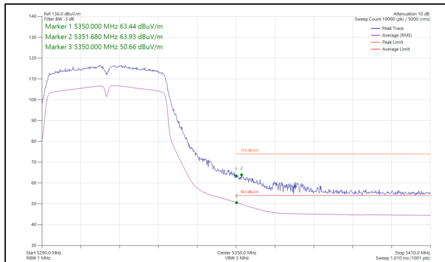
Figure 265 - 802.11ac VHT40, TxBF, Core 0-1 - 5310 MHz Band Edge Frequency 5350 MHz
