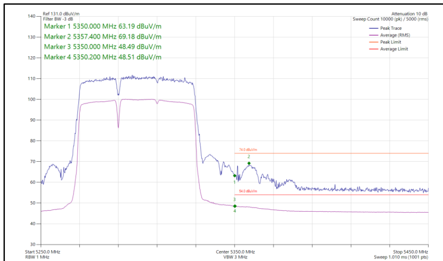
Figure 281 - 802.11be EHT80, RU 484+242-90, SISO, Core 0 - 5290 MHz Band Edge Frequency 5350 MHz
