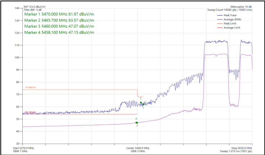
Figure 311 - 802.11be EHT80, RU 484+242-92, SISO, Core 1 - 5610 MHz Band Edge Frequency 5460 MHz
