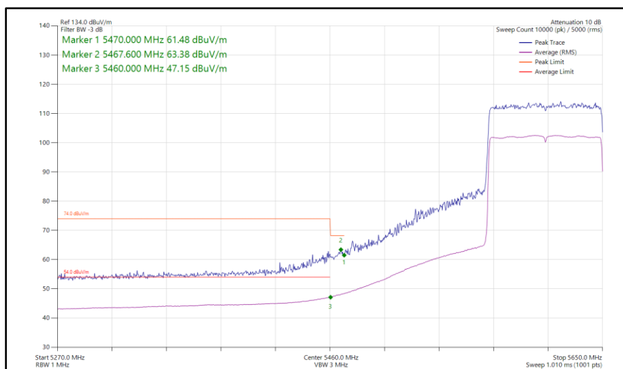
Figure 288 - 802.11ax HE80, SU, SISO, Core 0 - 5610 MHz Band Edge Frequency 5460 MHz
