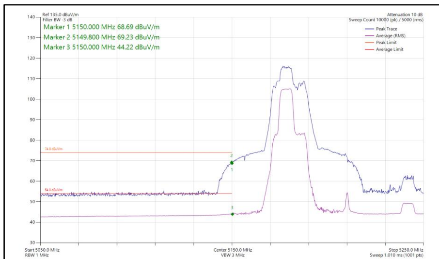
Figure 276 - 802.11be EHT80, RU 52+26-71, SISO, Core 0 - 5210 MHz Band Edge Frequency 5150 MHz
