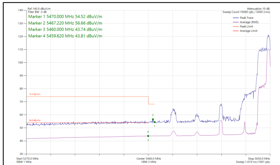
Figure 289 - 802.11ax HE80, RU 52-52, SISO, Core 0 - 5610 MHz Band Edge Frequency 5460 MHz
