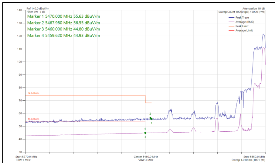
Figure 309 - 802.11ax HE80, RU 52-52, SISO, Core 1 - 5610 MHz Band Edge Frequency 5460 MHz
