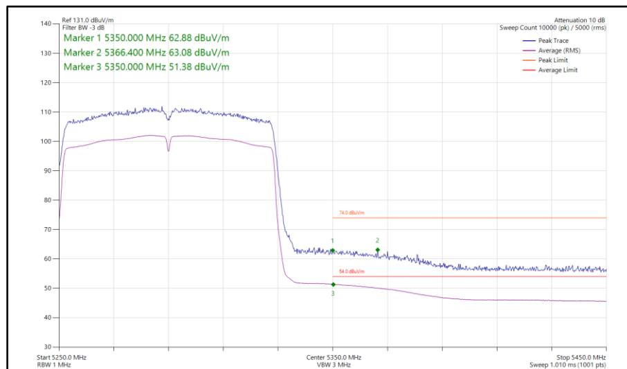
Figure 298 - 802.11ac VHT80, SISO, Core 1 - 5290 MHz Band Edge Frequency 5350 MHz
