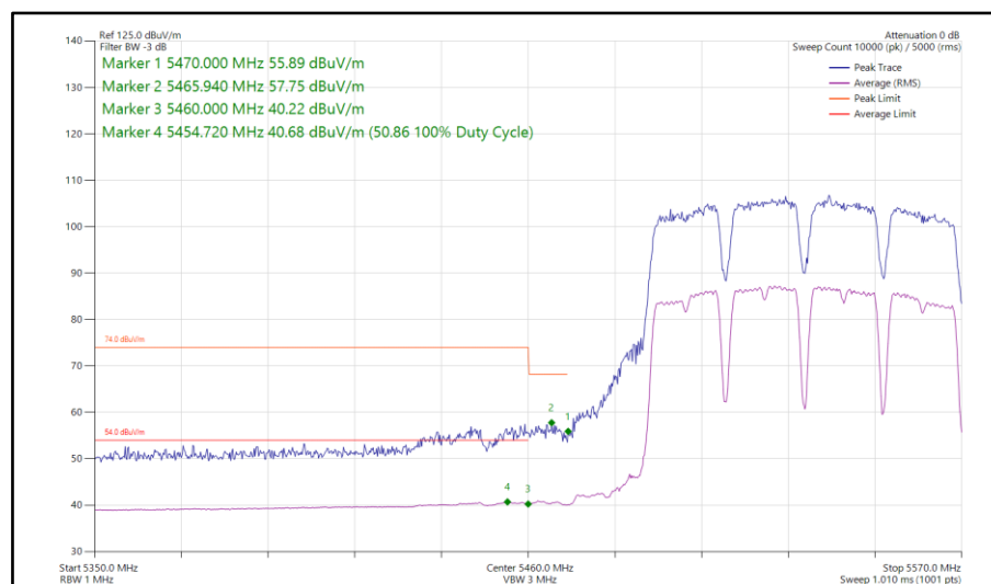
Figure 282 - 802.11a, SISO, Core 0 - 5530 MHz Band Edge Frequency 5460 MHz
