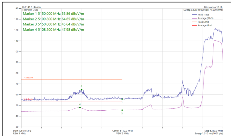
Figure 295 - 802.11ax HE80, RU 106-60, SISO, Core 1 - 5210 MHz Band Edge Frequency 5150 MHz
