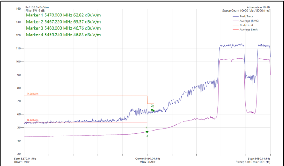
Figure 291 - 802.11be EHT80, RU 484+242-92, SISO, Core 0 - 5610 MHz Band Edge Frequency 5460 MHz
