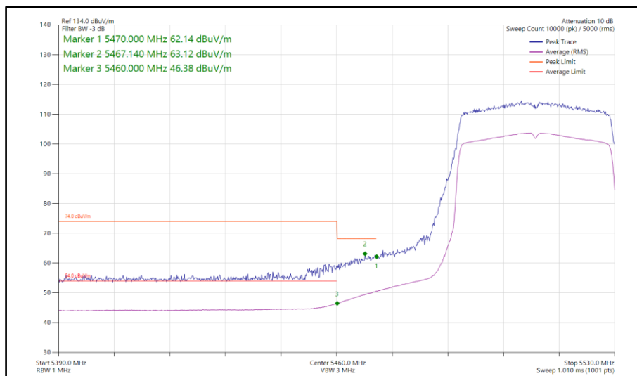
Figure 270 - 802.11ax HE40, SU, TxBF, Core 0-1 - 5510 MHz Band Edge Frequency 5460 MHz
