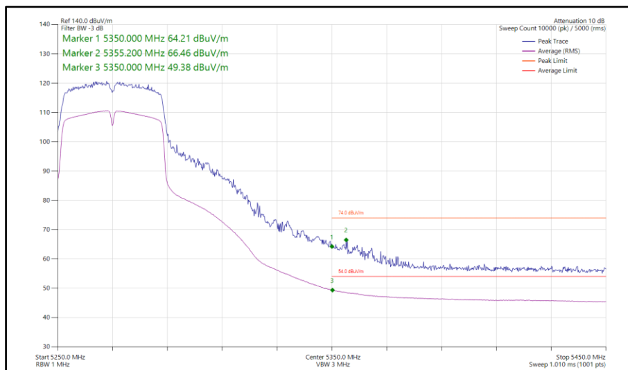
Figure 264 - 802.11ac VHT40, TxBF, Core 0-1 - 5270 MHz Band Edge Frequency 5350 MHz
