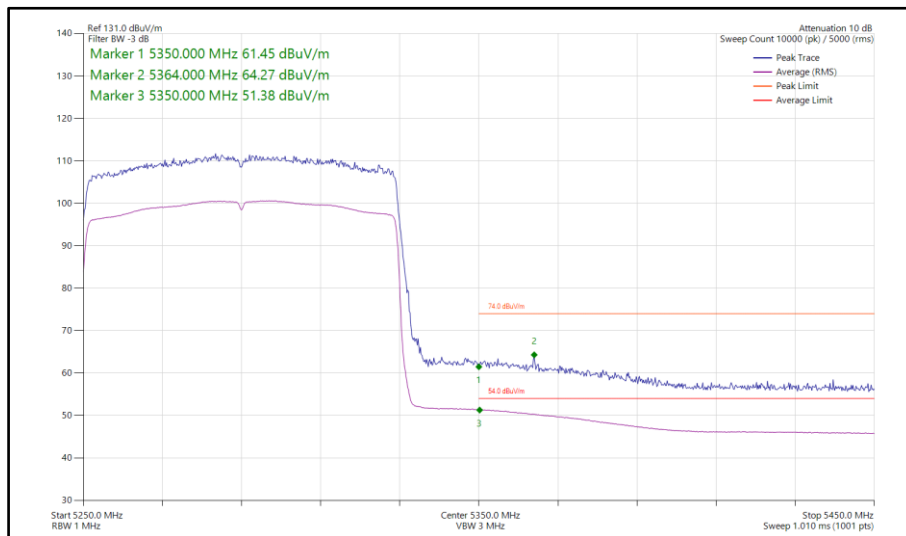
Figure 299 - 802.11ax HE80, SU, SISO, Core 1 - 5290 MHz Band Edge Frequency 5350 MHz
