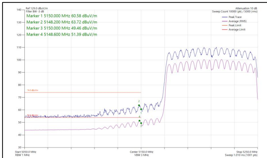
Figure 313 - 802.11ac VHT80, CDD, Core 0-1 - 5210 MHz Band Edge Frequency 5150 MHz
