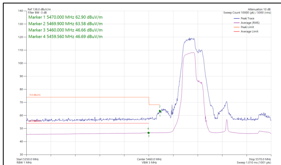
Figure 290 - 802.11be EHT80, RU 106+26-82, SISO, Core 0 - 5530 MHz Band Edge Frequency 5460 MHz
