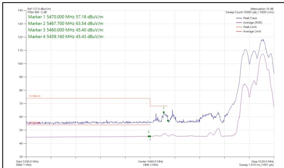
Figure 258 - 802.11be EHT40, RU 52+26-75, SDM, Core 0-1 - 5510 MHz Band Edge Frequency 5460 MHz
