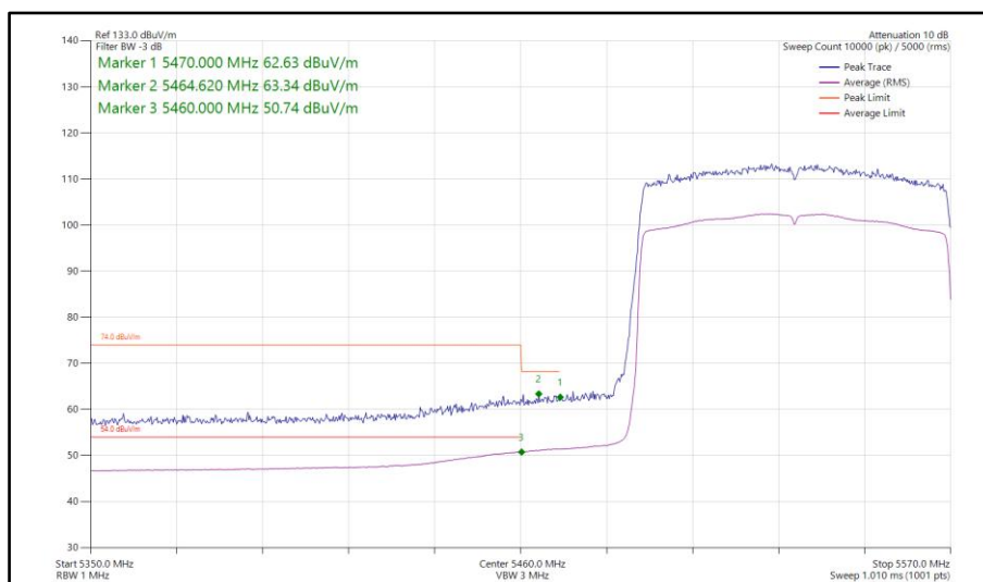
Figure 306 - 802.11ax HE80, SU, SISO, Core 1 - 5530 MHz Band Edge Frequency 5460 MHz
