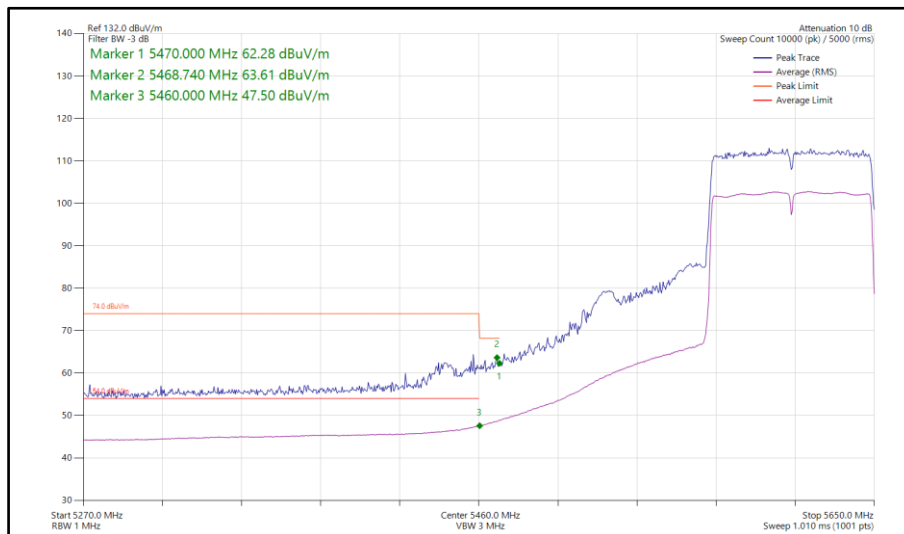
Figure 305 - 802.11ac VHT80, SISO, Core 1 - 5610 MHz Band Edge Frequency 5460 MHz
