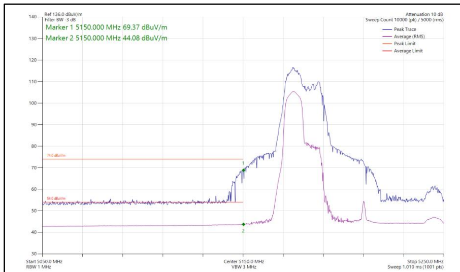
Figure 275 - 802.11ax HE80, RU 106-53, SISO, Core 0 - 5210 MHz Band Edge Frequency 5150 MHz
