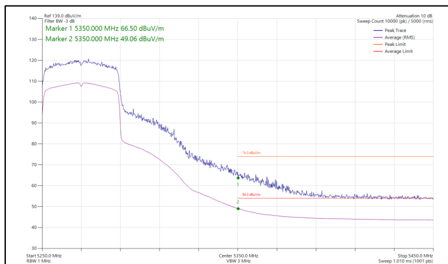
Figure 266 - 802.11ax HE40, SU, TxBF, Core 0-1 - 5270 MHz Band Edge Frequency 5350 MHz
