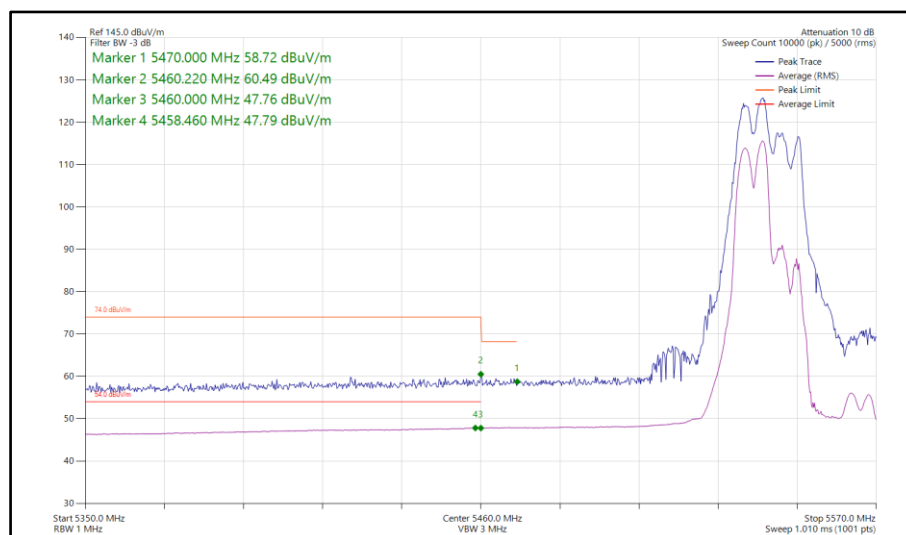
Figure 257 - 802.11ax HE40, RU 106-53, SDM, Core 0-1 - 5550 MHz Band Edge Frequency 5460 MHz
