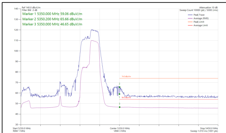
Figure 280 - 802.11ax HE80, RU 106-60, SISO, Core 0 - 5290 MHz Band Edge Frequency 5350 MHz
