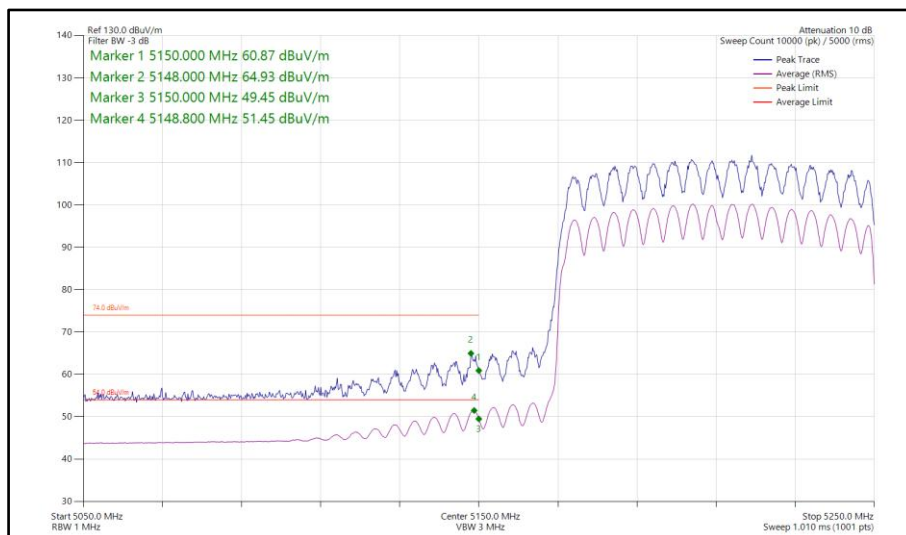
Figure 314 - 802.11ax HE80, SU, CDD, Core 0-1 - 5210 MHz Band Edge Frequency 5150 MHz
