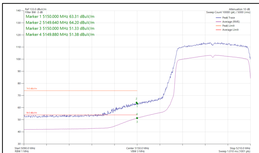
Figure 262 - 802.11ax HE40, SU, TxBF, Core 0-1 - 5190 MHz Band Edge Frequency 5150 MHz
