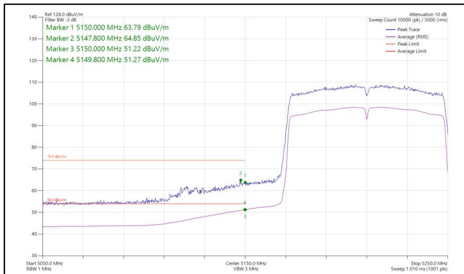
Figure 293 - 802.11ac VHT80, SISO, Core 1 - 5210 MHz Band Edge Frequency 5150 MHz
