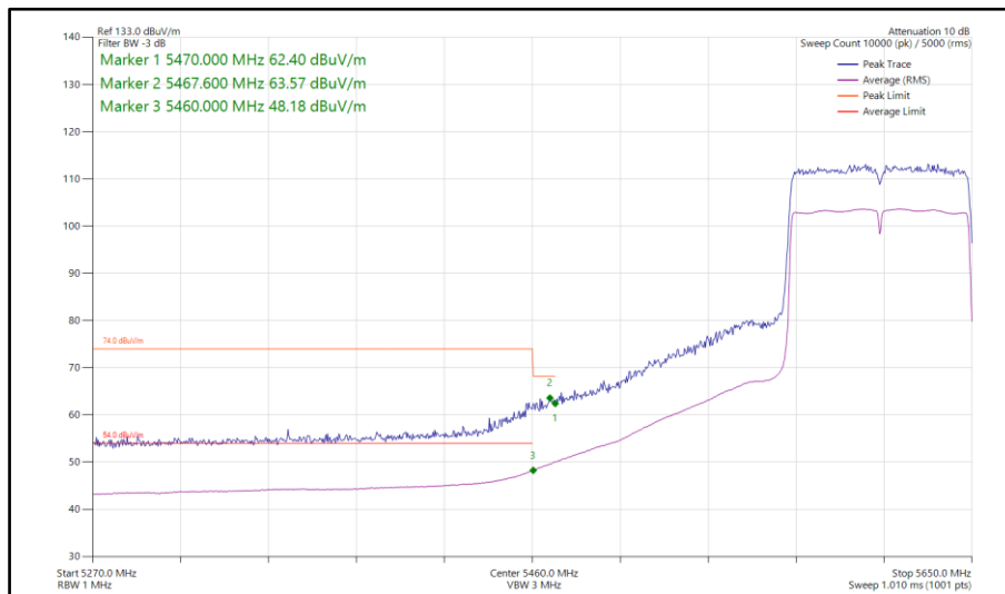
Figure 285 - 802.11ac VHT80, SISO, Core 0 - 5610 MHz Band Edge Frequency 5460 MHz
