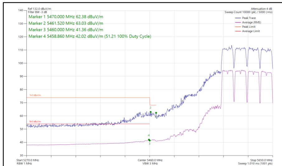
Figure 303 - 802.11a, SISO, Core 1 - 5610 MHz Band Edge Frequency 5460 MHz
