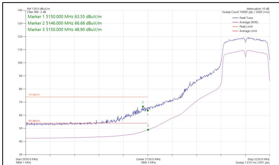
Figure 261 - 802.11ac VHT40, TxBF, Core 0-1 - 5230 MHz Band Edge Frequency 5150 MHz
