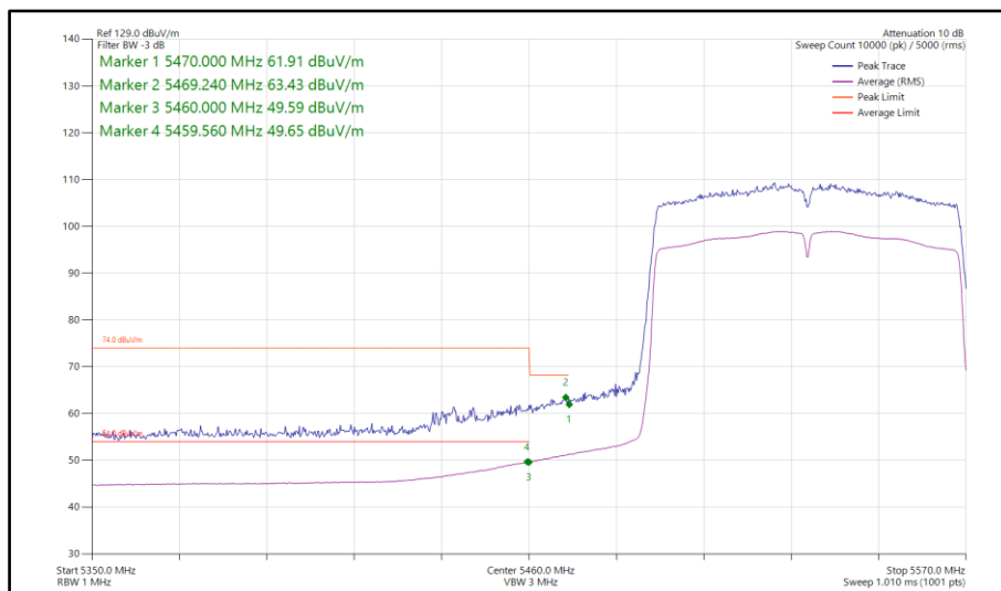
Figure 284 - 802.11ac VHT80, SISO, Core 0 - 5530 MHz Band Edge Frequency 5460 MHz
