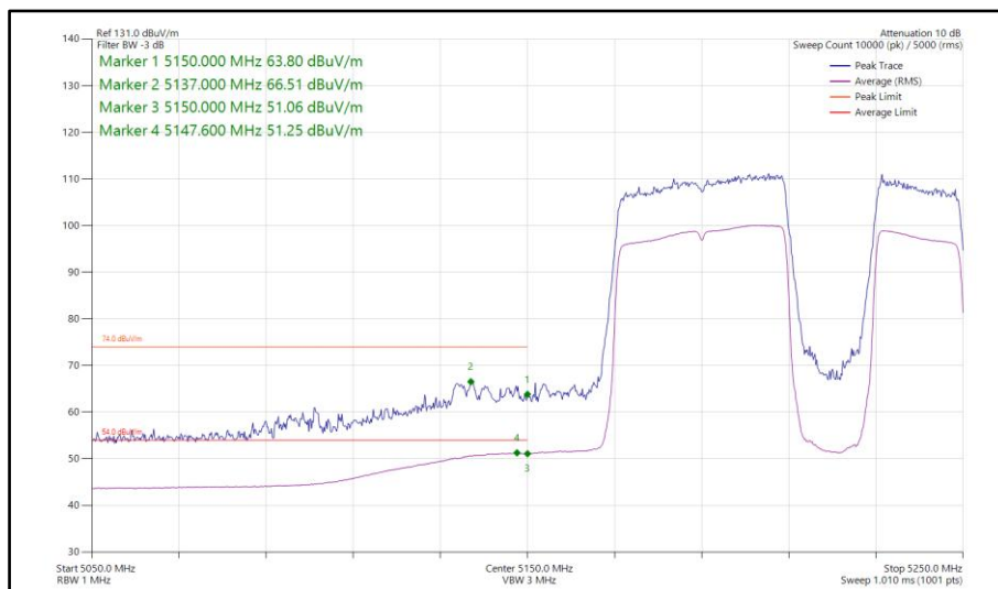
Figure 296 - 802.11be EHT80, RU 484+242-92, SISO, Core 1 - 5210 MHz Band Edge Frequency 5150 MHz
