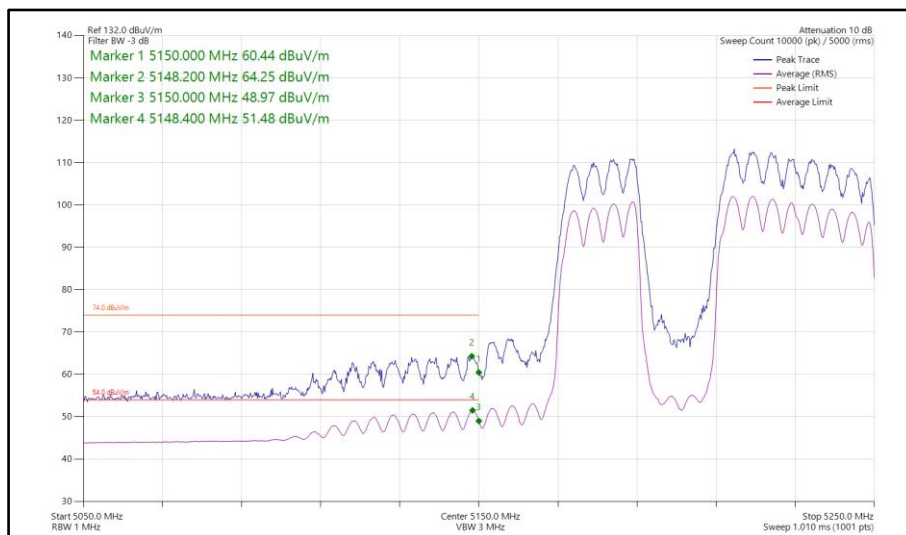
Figure 316 - 802.11be EHT80, RU 484+242-91, CDD, Core 0-1 - 5210 MHz Band Edge Frequency 5150 MHz
