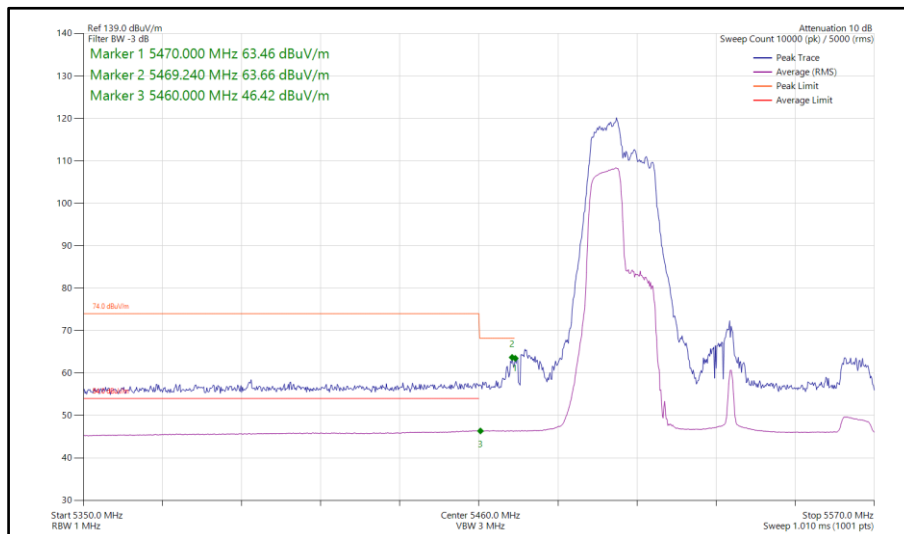
Figure 287 - 802.11ax HE80, RU 106-53, SISO, Core 0 - 5530 MHz Band Edge Frequency 5460 MHz
