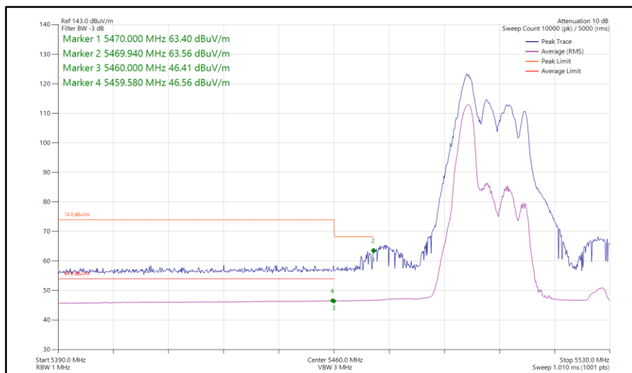
Figure 255 - 802.11ax HE40, RU 52-37, SDM, Core 0-1 - 5510 MHz Band Edge Frequency 5460 MHz
