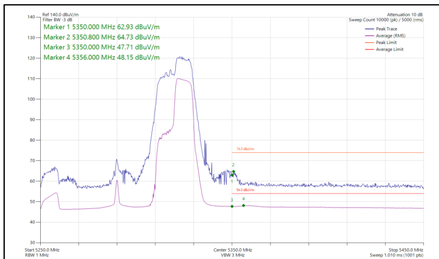
Figure 300 - 802.11ax HE80, RU 106-60, SISO, Core 1 - 5290 MHz Band Edge Frequency 5350 MHz
