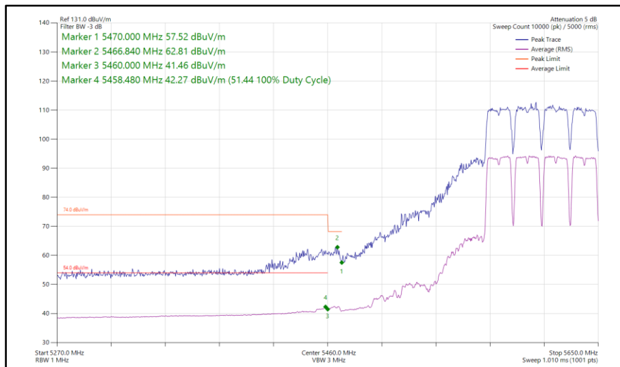
Figure 283 - 802.11a, SISO, Core 0 - 5610 MHz Band Edge Frequency 5460 MHz
