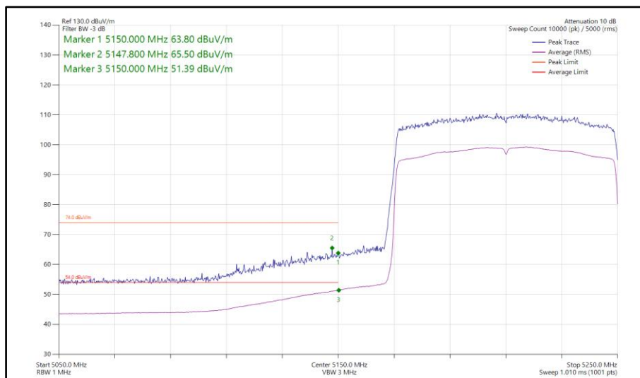
Figure 294 - 802.11ax HE80, SU, SISO, Core 1 - 5210 MHz Band Edge Frequency 5150 MHz
