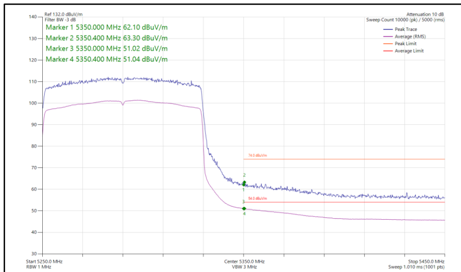
Figure 279 - 802.11ax HE80, SU, SISO, Core 0 - 5290 MHz Band Edge Frequency 5350 MHz
