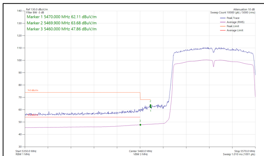
Figure 304 - 802.11ac VHT80, SISO, Core 1 - 5530 MHz Band Edge Frequency 5460 MHz
