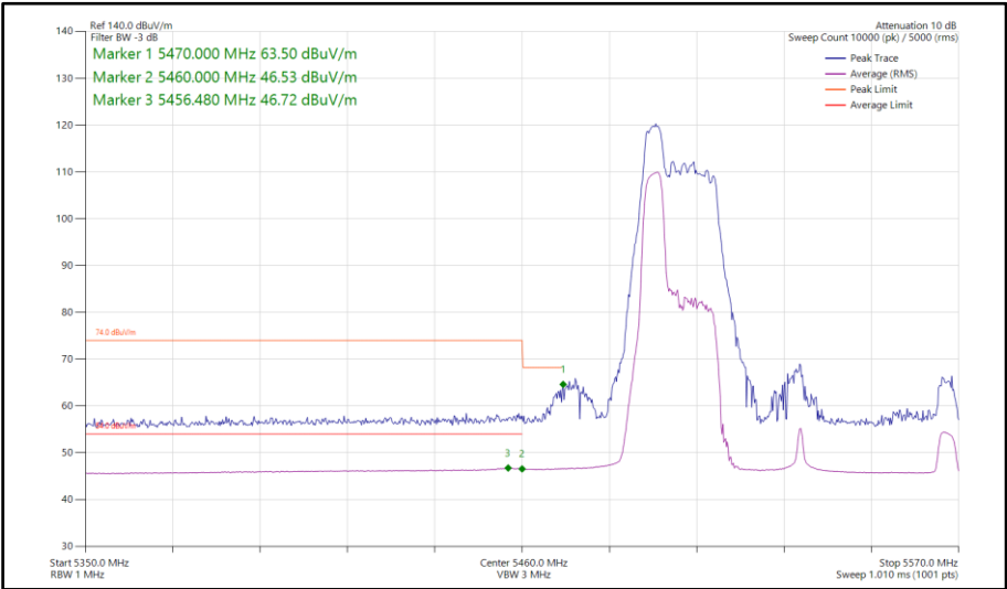
Figure 307 - 802.11ax HE80, RU 52-37, SISO, Core 1 - 5530 MHz Band Edge Frequency 5460 MHz
