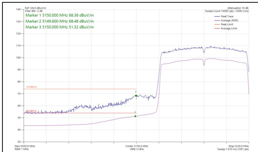
Figure 273 - 802.11ac VHT80, SISO, Core 0 - 5210 MHz Band Edge Frequency 5150 MHz
