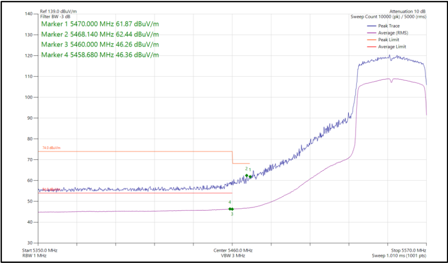
Figure 271 - 802.11ax HE40, SU, TxBF, Core 0-1 - 5550 MHz Band Edge Frequency 5460 MHz
