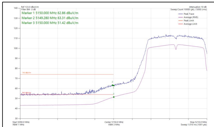
Figure 260 - 802.11ac VHT40, TxBF, Core 0-1 - 5190 MHz Band Edge Frequency 5150 MHz
