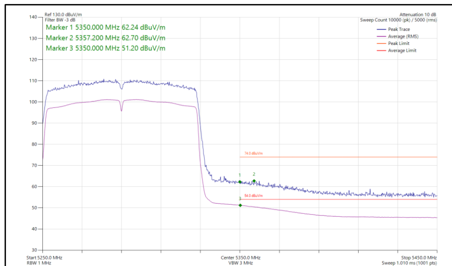
Figure 278 - 802.11ac VHT80, SISO, Core 0 - 5290 MHz Band Edge Frequency 5350 MHz
