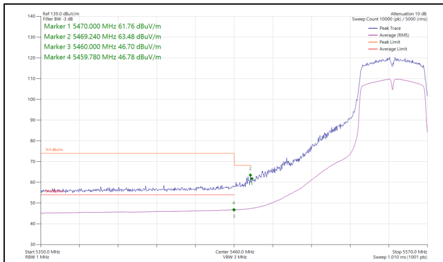
Figure 269 - 802.11ac VHT40, TxBF, Core 0-1 - 5550 MHz Band Edge Frequency 5460 MHz
