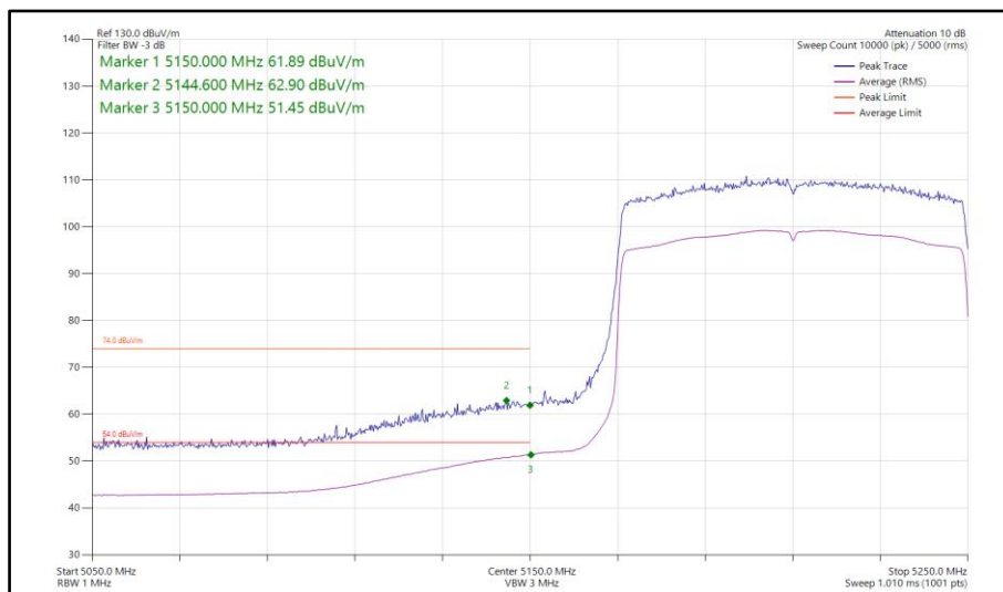
Figure 274 - 802.11ax HE80, SU, SISO, Core 0 - 5210 MHz Band Edge Frequency 5150 MHz
