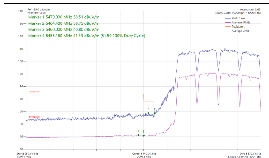
Figure 302 - 802.11a, SISO, Core 1 - 5530 MHz Band Edge Frequency 5460 MHz
