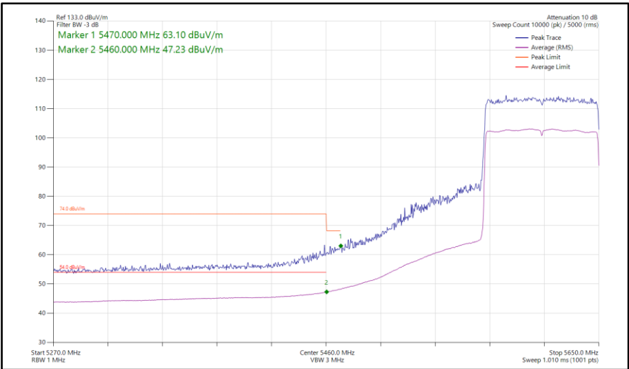
Figure 308 - 802.11ax HE80, SU, SISO, Core 1 - 5610 MHz Band Edge Frequency 5460 MHz
