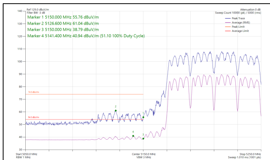
Figure 312 - 802.11a, CDD, Core 0-1 - 5210 MHz Band Edge Frequency 5150 MHz
