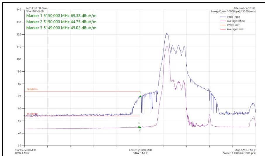
Figure 315 - 802.11ax HE80, RU 52-37, CDD, Core 0-1 - 5210 MHz Band Edge Frequency 5150 MHz
