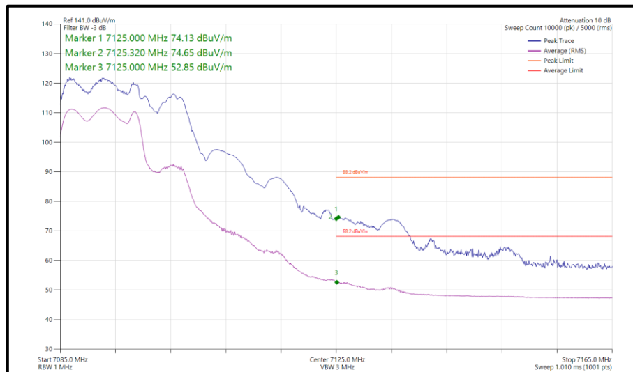
Figure 432 - 802.11be EHT20, RU106+26-82, SDM, Core 0-1 - 7095 MHz Band Edge Frequency 7125 MHz
