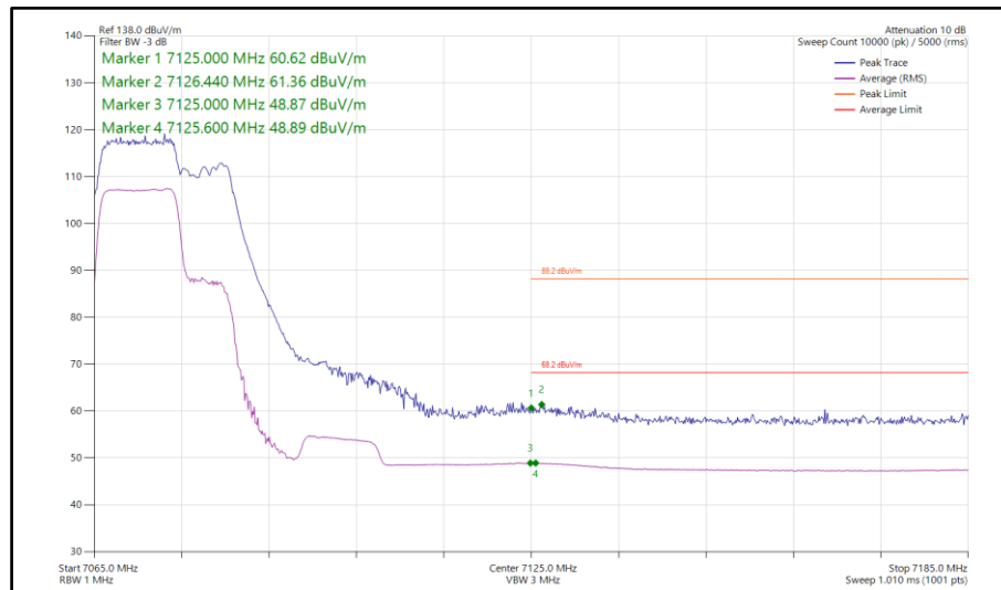
Figure 446 - 802.11be EHT40, RU106+26-82, SISO, Core 0 - 7085 MHz Band Edge Frequency 7125 MHz
