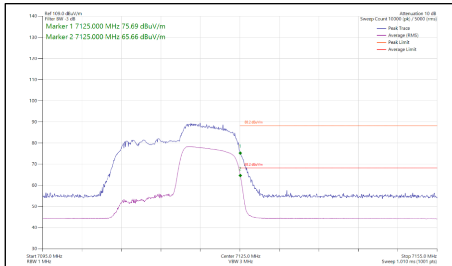
Figure 398 - 802.11ax HE20, RU 106-54, SISO, Core 0 - 7115 MHz Band Edge Frequency 7125 MHz
