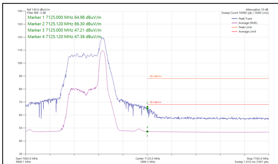
Figure 455 - 802.11ax HE40, RU 26-17, SISO, Core 1 - 7085 MHz Band Edge Frequency 7125 MHz
