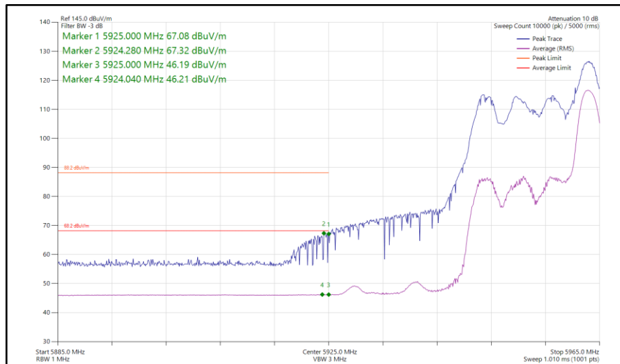
Figure 426 - 802.11ax HE20, RU 26-8, SDM, Core 0-1 - 5955 MHz Band Edge Frequency 5925 MHz
