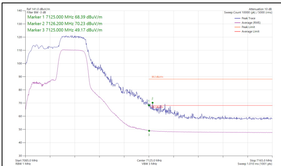
Figure 396 - 802.11ax HE20, RU 106-54, SISO, Core 0 - 7095 MHz Band Edge Frequency 7125 MHz
