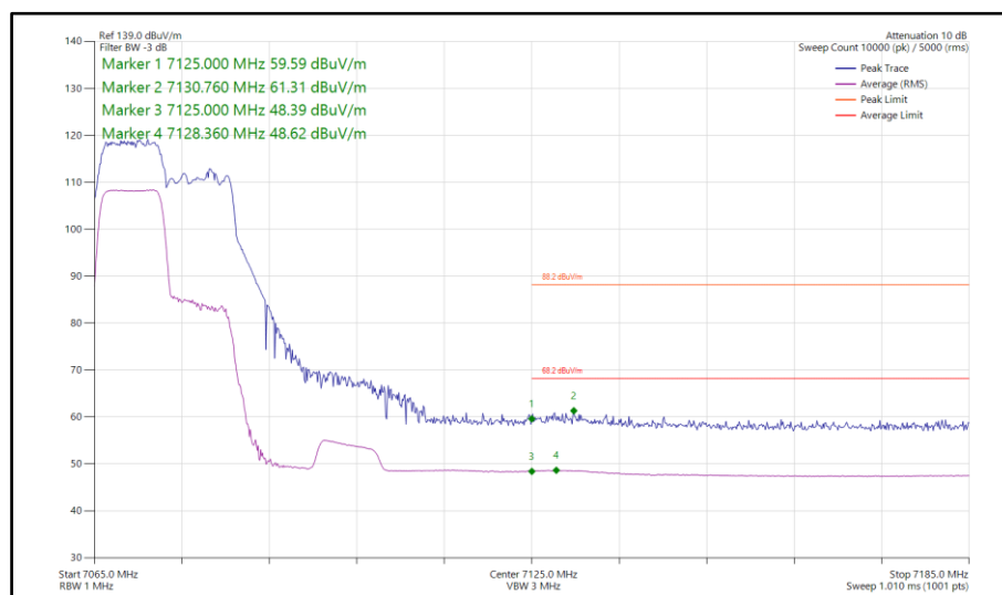
Figure 445 - 802.11ax HE40, RU 106-53, SISO, Core 0 - 7085 MHz Band Edge Frequency 7125 MHz
