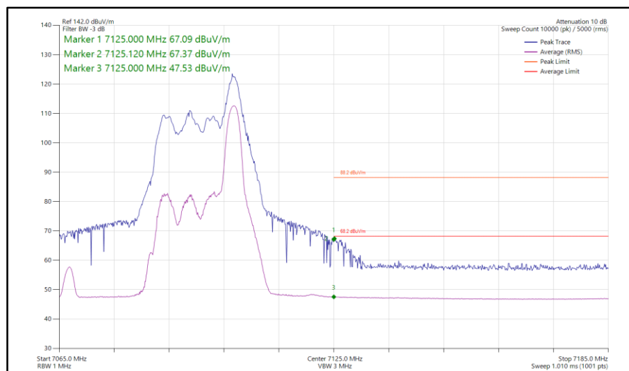
Figure 465 - 802.11ax HE40, RU 26-17, CDD, Core 0-1 - 7085 MHz Band Edge Frequency 7125 MHz
