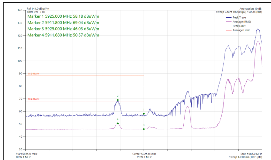
Figure 468 - 802.11ax HE40, RU 26-17, SDM, Core 0-1 - 5965 MHz Band Edge Frequency 5925 MHz
