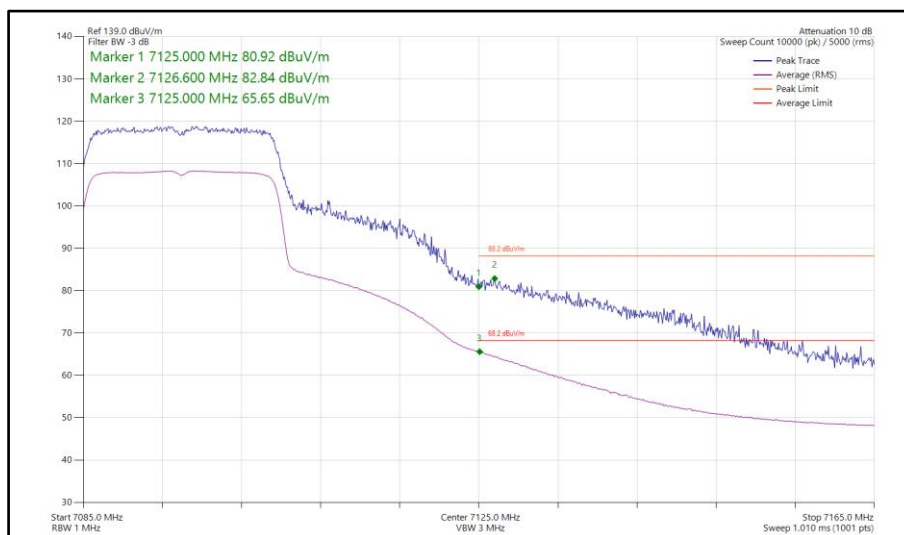
Figure 407 - 802.11ax HE20, SU, SISO, Core 1 - 7095 MHz Band Edge Frequency 7125 MHz
