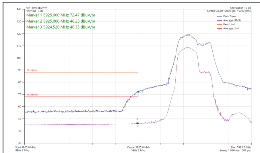
Figure 440 - 802.11be EHT40, RU106+26-82, SISO, Core 0 - 5965 MHz Band Edge Frequency 5925 MHz
