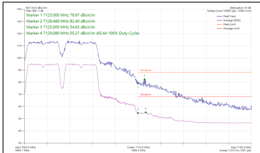
Figure 452 - 802.11a, SISO, Core 1 - 7085 MHz Band Edge Frequency 7125 MHz
