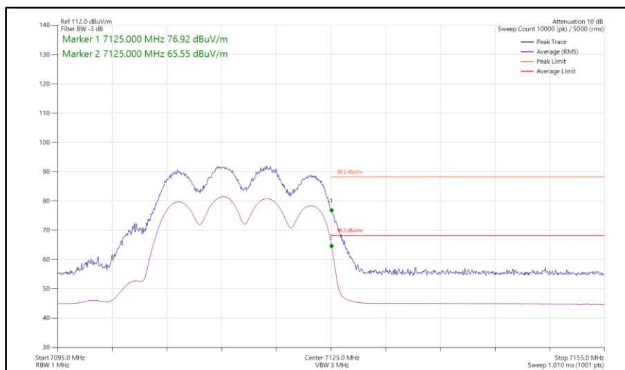
Figure 421 - 802.11ax HE20, SU, CDD, Core 0-1 - 7115 MHz Band Edge Frequency 7125 MHz
