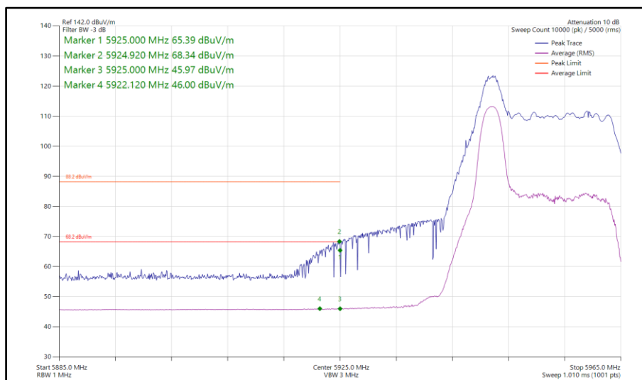
Figure 403 - 802.11ax HE20, RU 26-0, SISO, Core 1 - 5955 MHz Band Edge Frequency 5925 MHz
