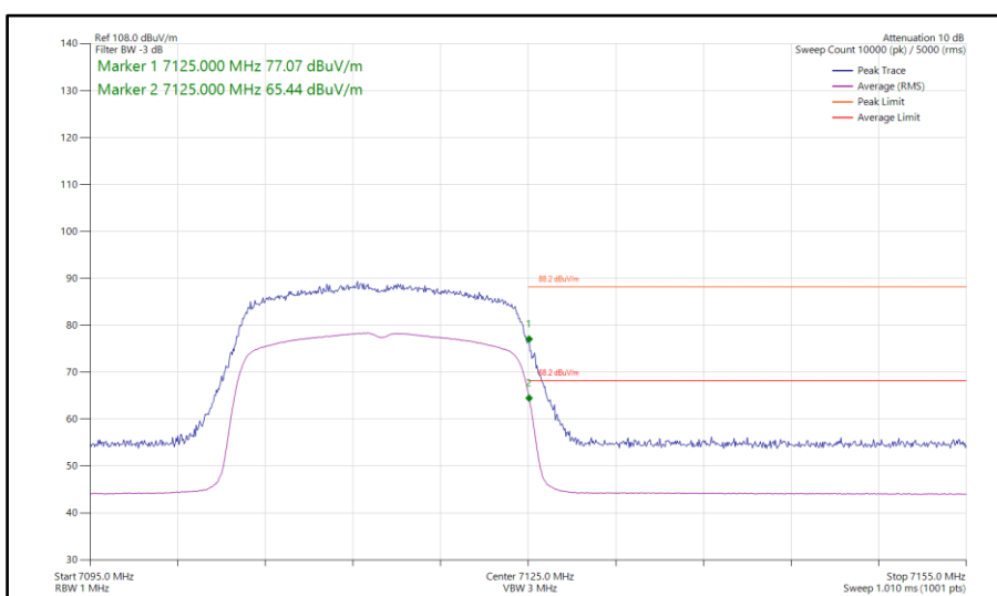
Figure 397 - 802.11ax HE20, SU, SISO, Core 0 - 7115 MHz Band Edge Frequency 7125 MHz
