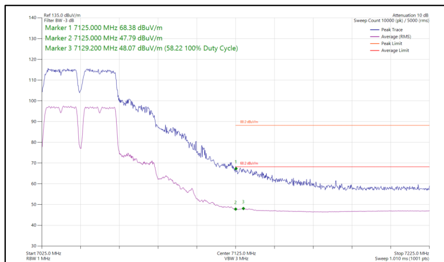
Figure 451 - 802.11a, SISO, Core 1 - 7045 MHz Band Edge Frequency 7125 MHz
