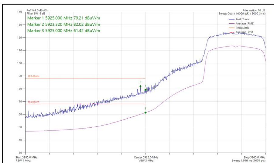
Figure 434 - 802.11ax HE20, SU, TxBF, Core 0-1 - 5955 MHz Band Edge Frequency 5925 MHz
