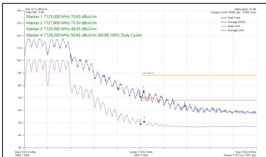
Figure 461 - 802.11a, CDD, Core 0-1 - 7045 MHz Band Edge Frequency 7125 MHz
