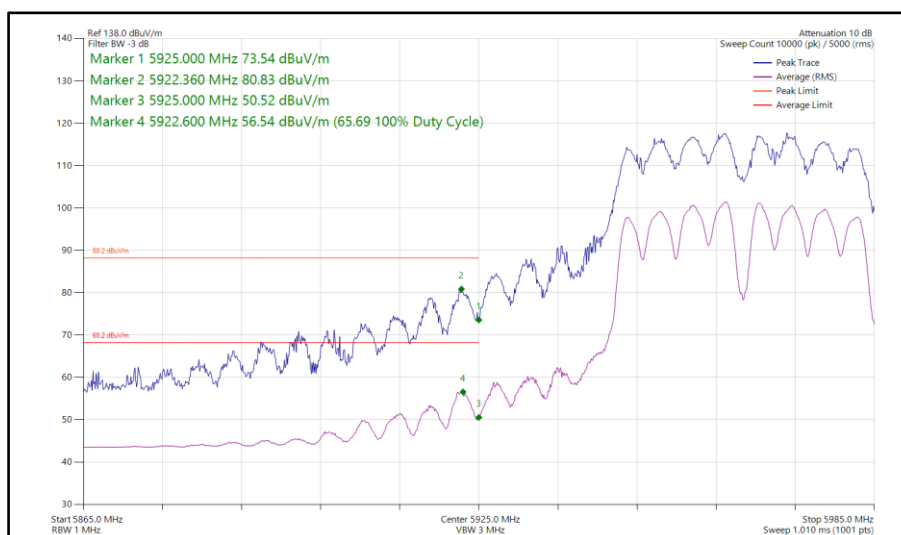
Figure 457 - 802.11a, CDD, Core 0-1 - 5965 MHz Band Edge Frequency 5925 MHz
