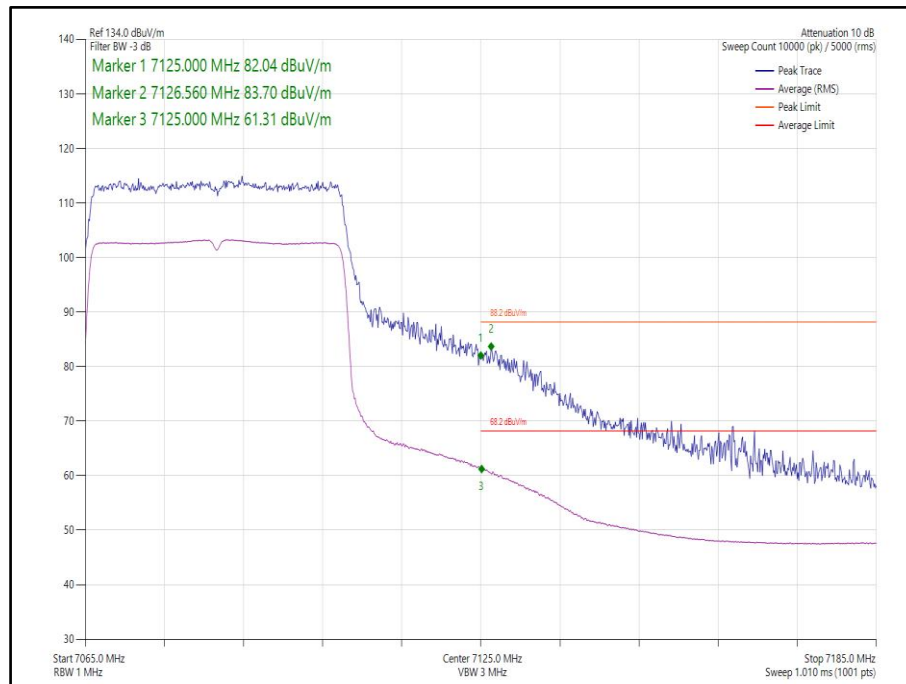
Figure 444 - 802.11ax HE40, SU, SISO, Core 0 - 7085 MHz Band Edge Frequency 7125 MHz
