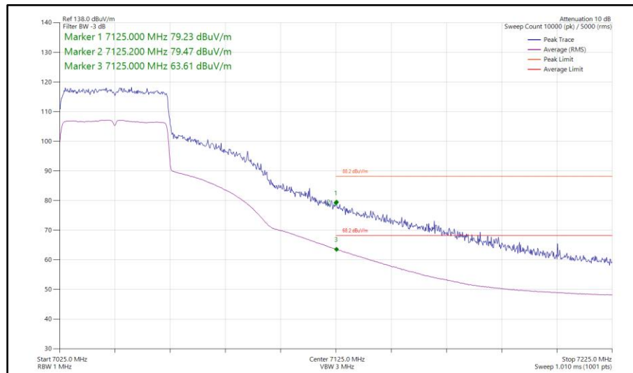
Figure 470 - 802.11ax HE40, SU, SDM, Core 0-1 - 7045 MHz Band Edge Frequency 7125 MHz
