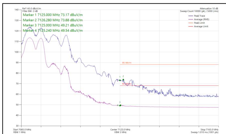
Figure 429 - 802.11ax HE20, RU 106-53, SDM, Core 0-1 - 7095 MHz Band Edge Frequency 7125 MHz
