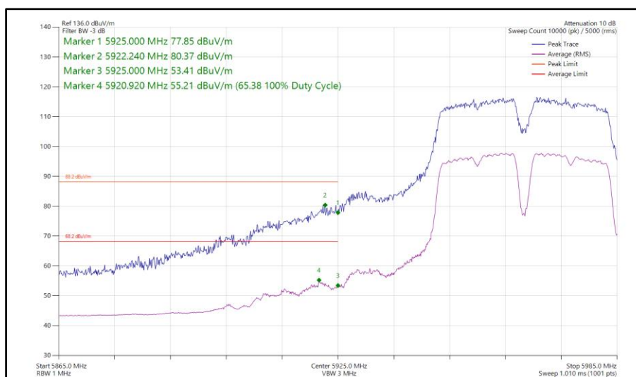
Figure 447 - 802.11a, SISO, Core 1 - 5965 MHz Band Edge Frequency 5925 MHz
