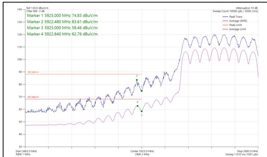
Figure 458 - 802.11ax HE40, SU, CDD, Core 0-1 - 5965 MHz Band Edge Frequency 5925 MHz
