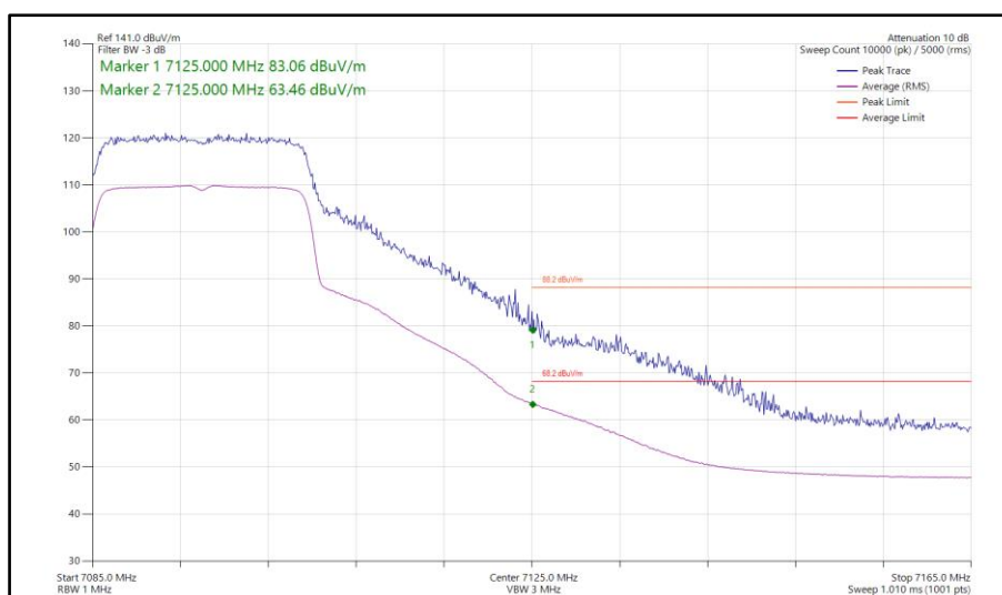
Figure 435 - 802.11ax HE20, SU, TxBF, Core 0-1 - 7095 MHz Band Edge Frequency 7125 MHz
