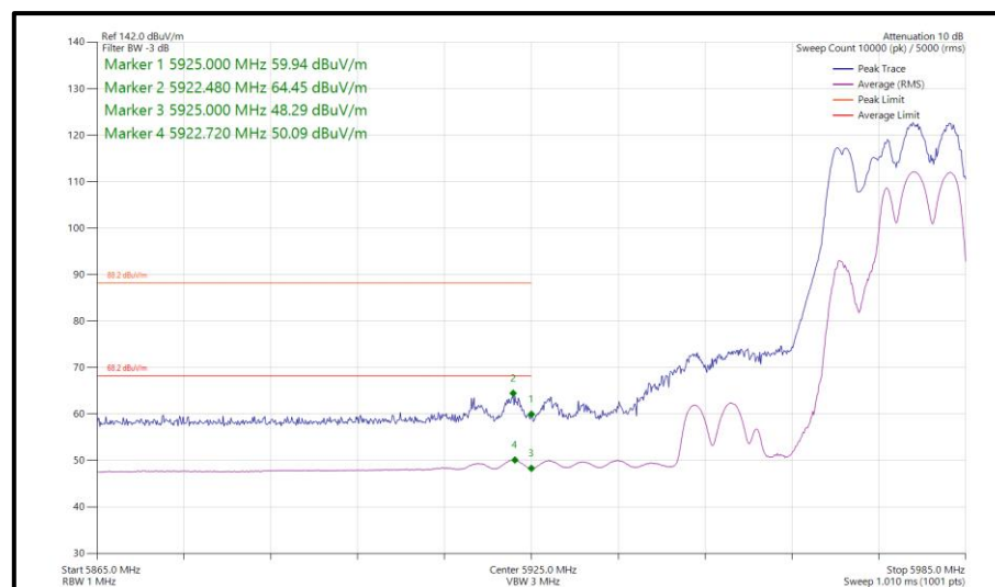
Figure 469 - 802.11be EHT40, RU106+26-85, SDM, Core 0-1 - 5965 MHz Band Edge Frequency 5925 MHz
