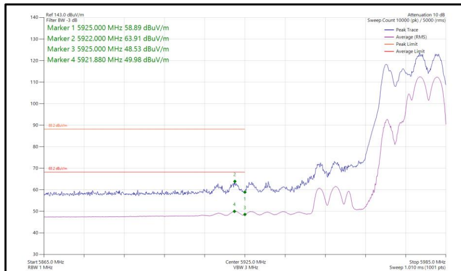
Figure 460 - 802.11be EHT40, RU106+26-85, CDD, Core 0-1 - 5965 MHz Band Edge Frequency 5925 MHz
