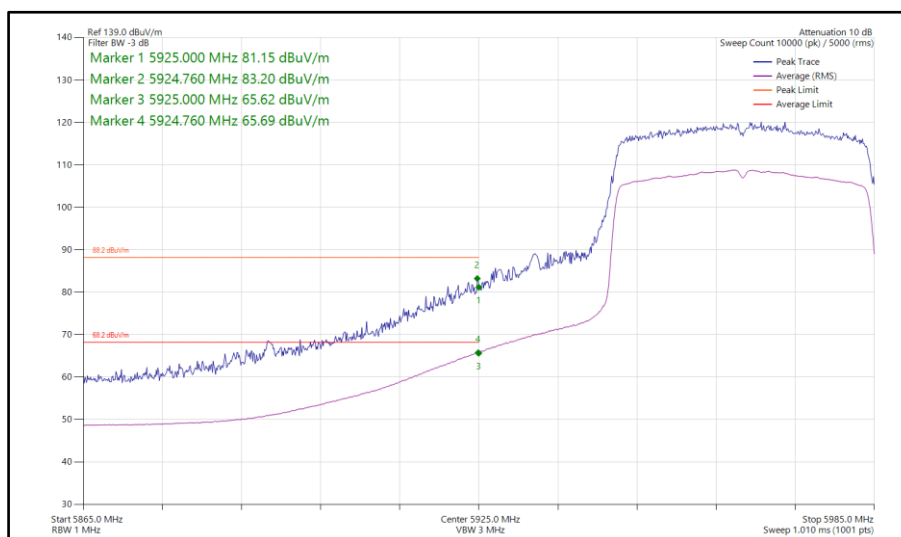
Figure 467 - 802.11ax HE40, SU, SDM, Core 0-1 - 5965 MHz Band Edge Frequency 5925 MHz
