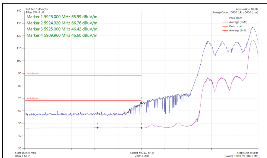
Figure 415 - 802.11ax HE20, RU 26-8, CDD, Core 0-1 - 5955 MHz Band Edge Frequency 5925 MHz
