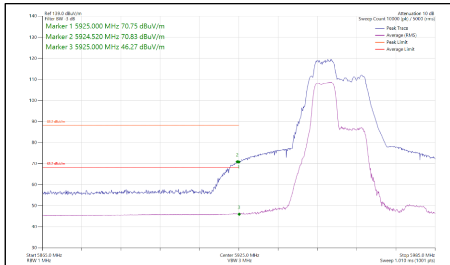
Figure 450 - 802.11be EHT40, RU52+26-70, SISO, Core 1 - 5965 MHz Band Edge Frequency 5925 MHz
