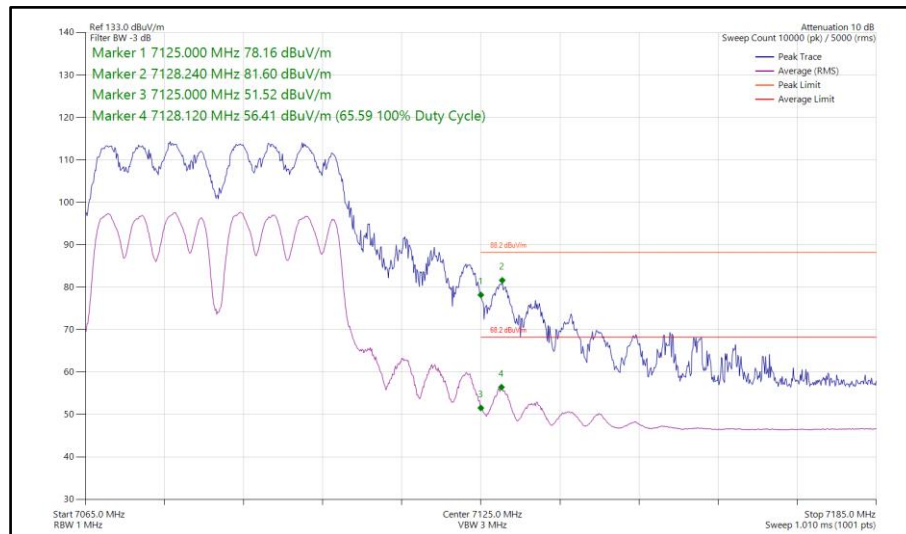
Figure 462 - 802.11a, CDD, Core 0-1 - 7085 MHz Band Edge Frequency 7125 MHz
