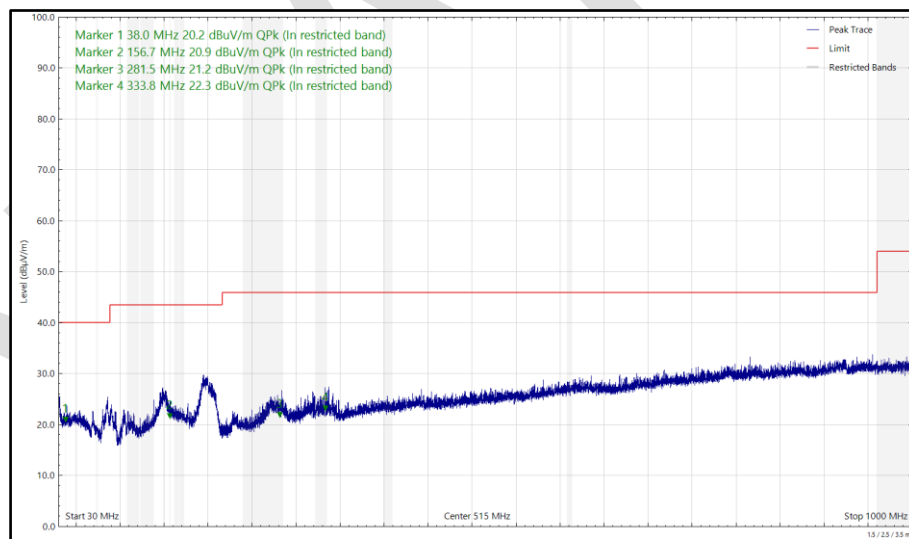
Figure 50 - 6175 MHz (CH45), HE20, SU, CDD, Core 0 + Core 1 and 2440 MHz (CH18), Thread, ePA, Core 1, 30 MHz to 1 GHz, Horizontal (Peak)
