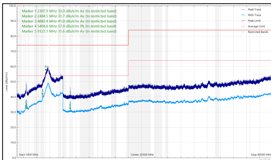
Figure 13 - 5785 MHz (CH157), HT20, CDD, Core 0 + Core 1 and 2441 MHz (CH39), DH5, ePA, Core 0 + Core 1, 1 GHz to 40 GHz, Vertical
