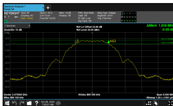
Figure 20 - Core 0 (A) 2475 MHz (CH25) 6 dB Bandwidth
