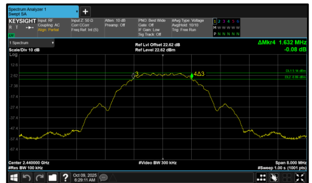
Figure 12 - Core 0 (A) 2440 MHz (CH18) 6 dB Bandwidth
