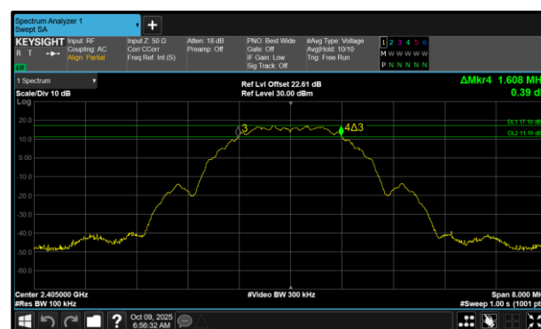
Figure 16 - Core 0 (A) 2405 MHz (CH11) 6 dB Bandwidth
