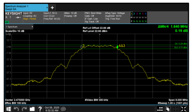
Figure 14 - Core 0 (A) 2475 MHz (CH25) 6 dB Bandwidth
