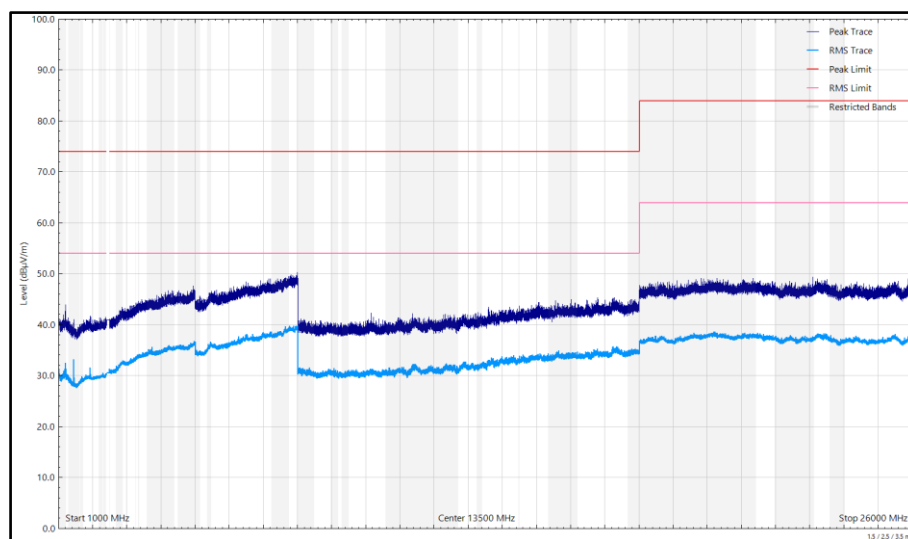
Figure 65 - 2440 MHz (CH18), Thread, iPA, Core 1, 1 GHz to 26 GHz, Horizontal
