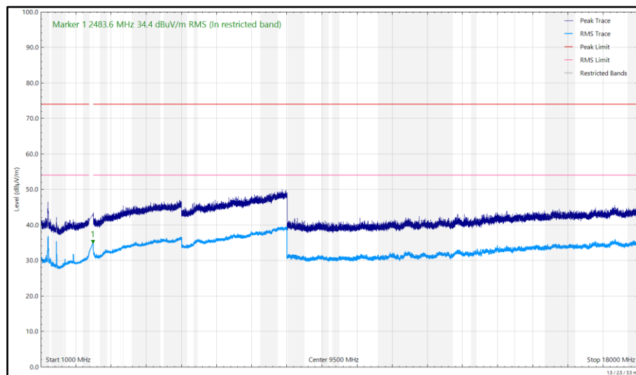
Figure 39 - 2405 MHz (CH11), Thread, ePA, Core 0, 1 GHz to 18 GHz, Vertical
