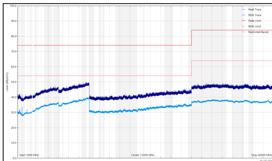
Figure 57 - 2440 MHz (CH18), Thread, iPA, Core 0, 1 GHz to 26 GHz, Horizontal
