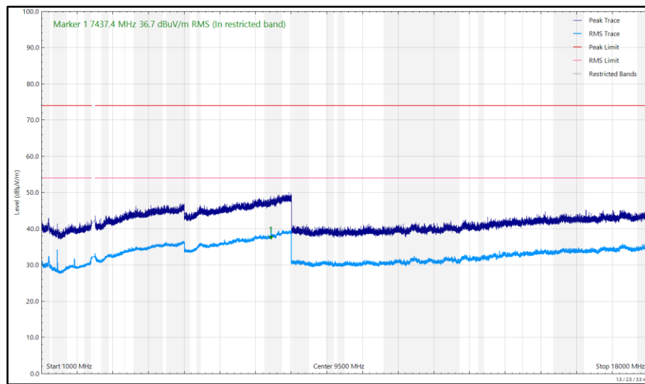
Figure 52 - 2475 MHz (CH25), Thread, ePA, Core 1, 1 GHz to 18 GHz, Horizontal
