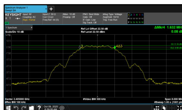
Figure 22 - Core 1 (B) 2405 MHz (CH11) 6 dB Bandwidth
