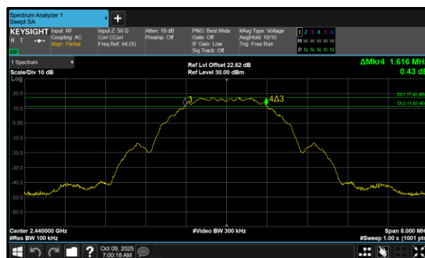
Figure 18 - Core 0 (A) 2440 MHz (CH18) 6 dB Bandwidth
