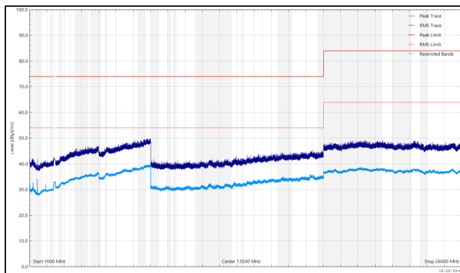
Figure 41 - 2440 MHz (CH18), Thread, ePA, Core 0, 1 GHz to 26 GHz, Horizontal
