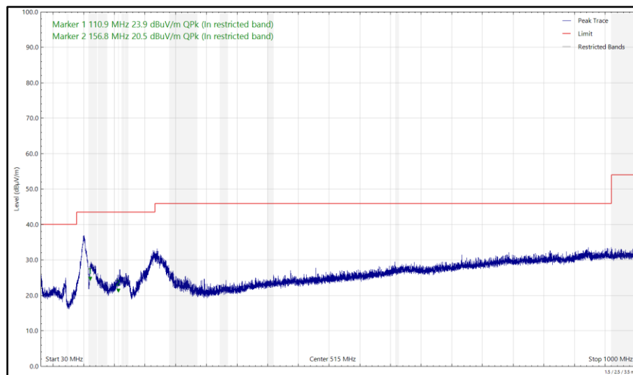
Figure 56 - 2440 MHz (CH18), Thread, iPA, Core 0, 30 MHz to 1 GHz, Horizontal (Peak)
