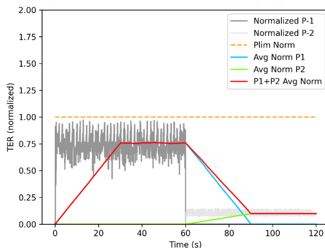
Figure 6-1 Technology Switch Normalized Time-averaged conducted TX power
