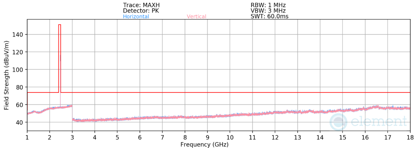
Plot 7-48. Radiated Spurious Emissions 1-18GHz Antenna WF7b (802.15.4 ePA – Ch. 25)
