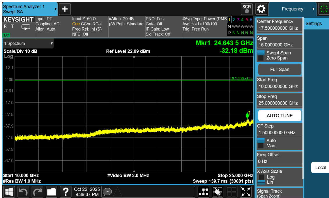
Plot 7-32. Conducted Spurious Antenna WF8 (802.15.4, ePA – Ch. 18)
