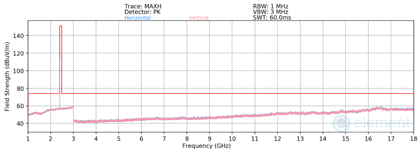
Plot 7-45. Radiated Spurious Emissions 1-18GHz Antenna WF7b (802.15.4 ePA – Ch. 11)
