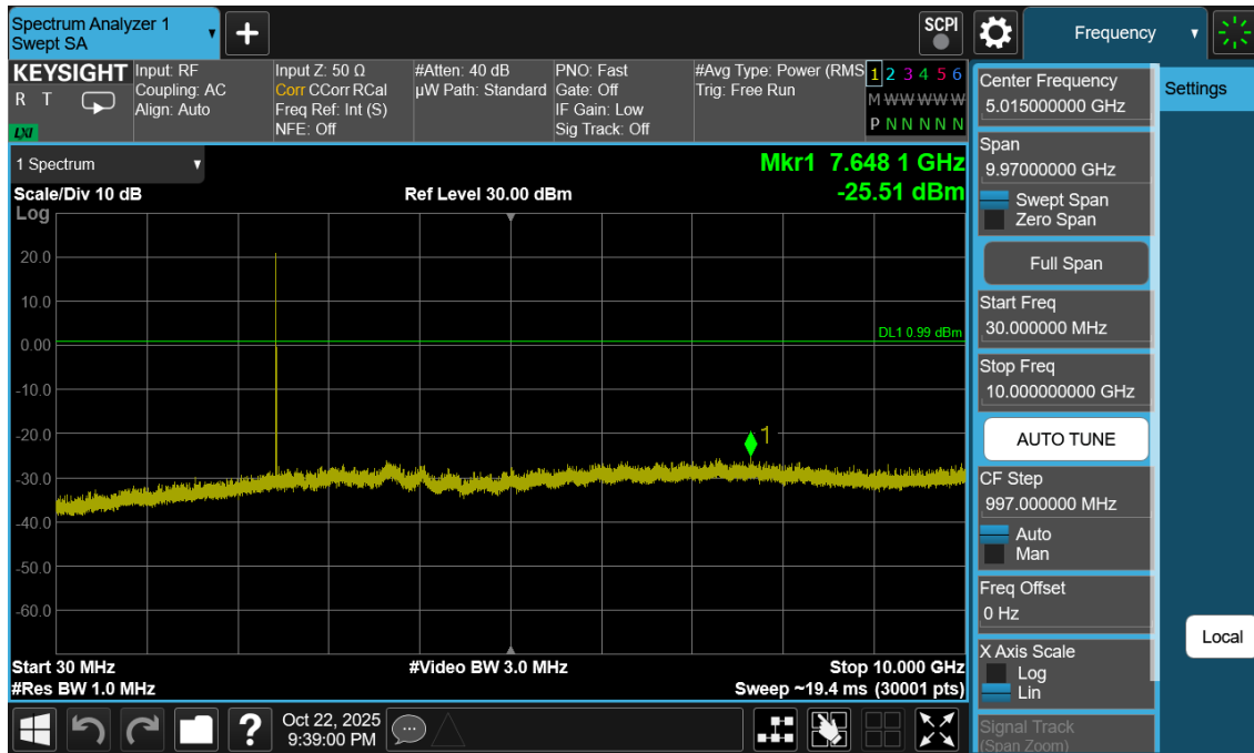
Plot 7-31. Conducted Spurious Antenna WF8 (802.15.4, ePA – Ch. 18)
