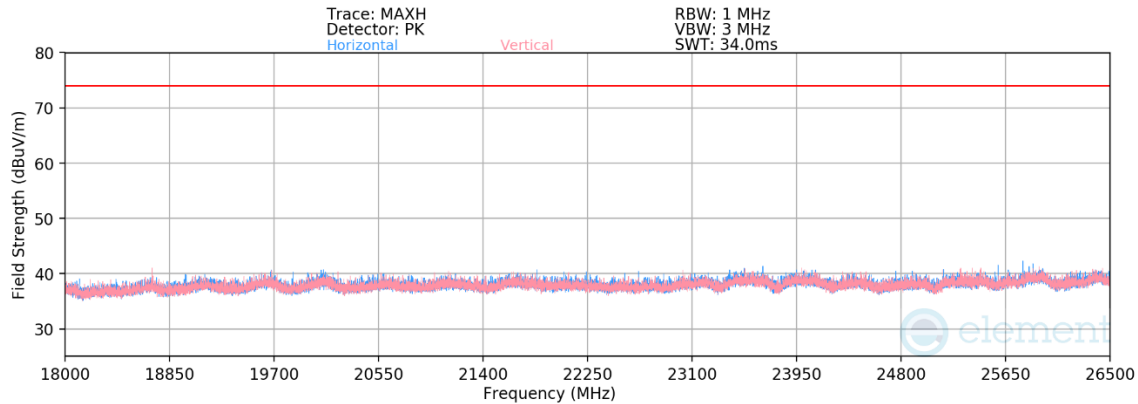
Plot 7-47. Radiated Spurious Emissions Above 18GHz Antenna WF7b (802.15.4 ePA – Ch. 18)
