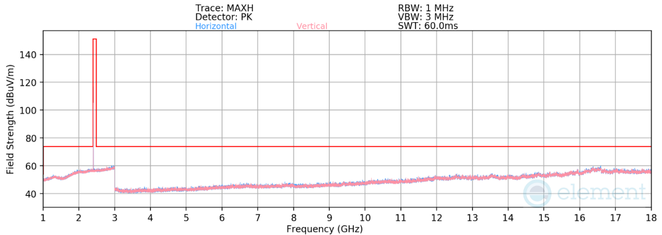
Plot 7-41. Radiated Spurious Emissions 1-18GHz Antenna WF8 (802.15.4 ePA – Ch. 11)
