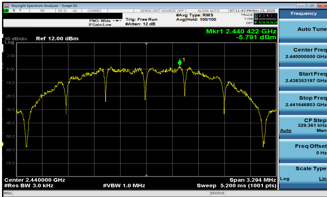
Plot 7-23. Power Spectral Density Antenna WF7b (802.15.4, iPA – Ch. 18)
