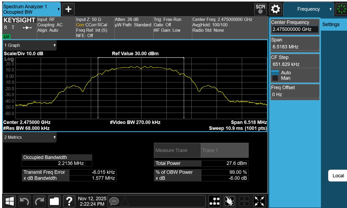
Plot 7-3. 99% OBW Antenna WF8 (802.15.4, Ch. 25)
