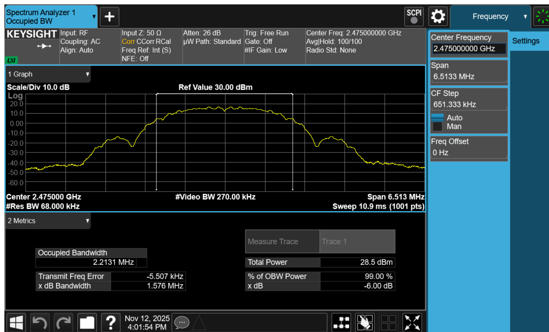
Plot 7-6. 99% OBW Antenna WF7b(802.15.4, Ch. 25)
