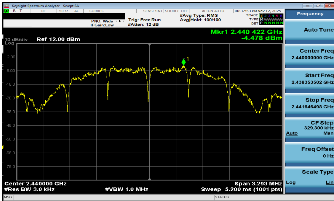
Plot 7-17. Power Spectral Density Antenna WF8 (802.15.4, iPA – Ch. 18)
