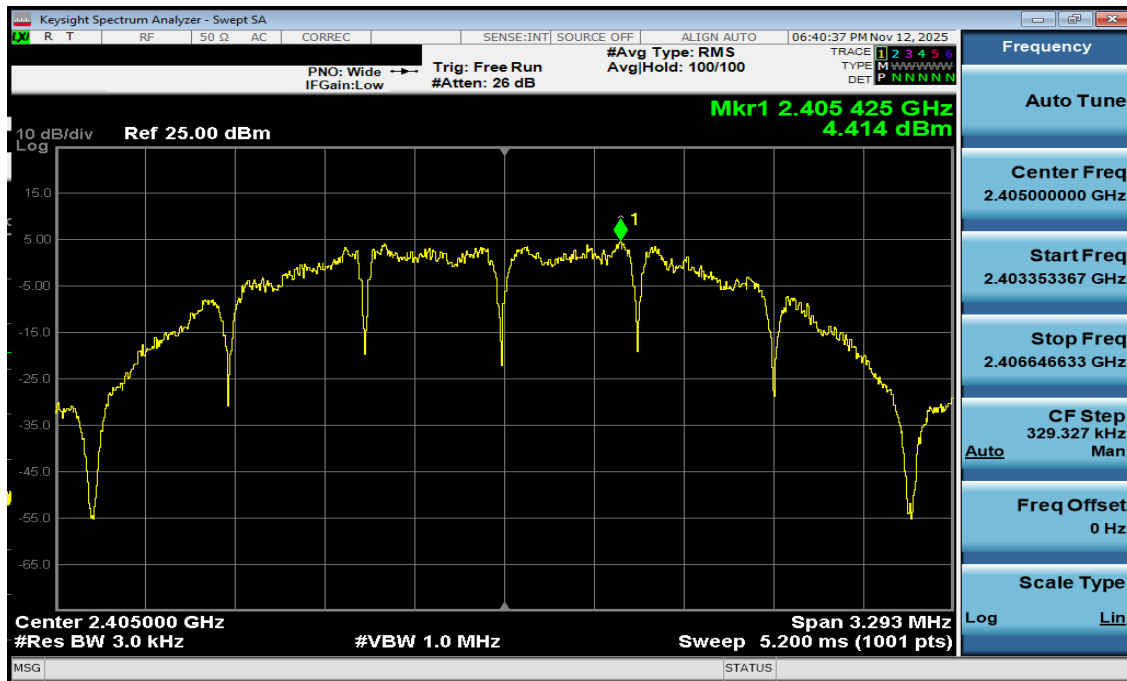
Plot 7-19. Power Spectral Density Antenna WF7b (802.15.4, ePA – Ch. 11)
