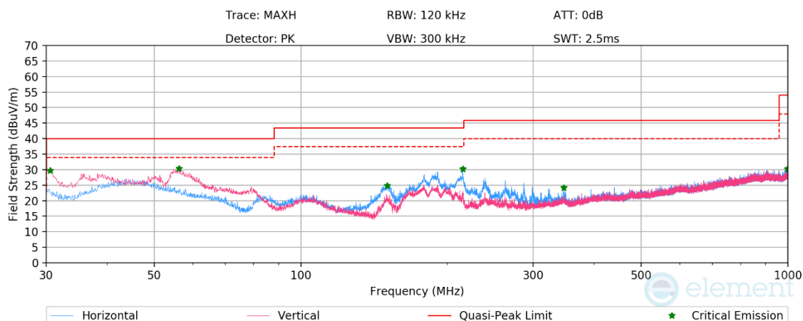
Plot 7-53. Radiated Spurious Emissions 30MHz-1GHz Antenna WF8 (ePA - Ch.18, with AC/DC Adapter)
