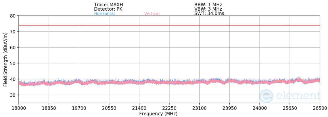
Plot 7-43. Radiated Spurious Emissions Above 18GHz Antenna WF8 (802.15.4 ePA – Ch. 18)
