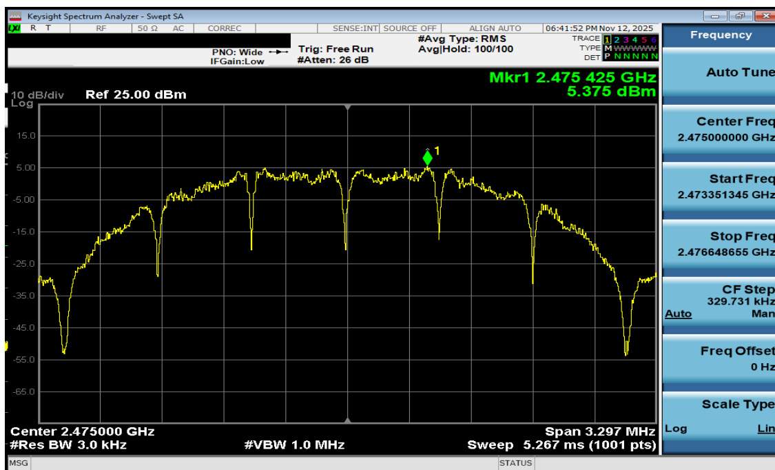
Plot 7-21. Power Spectral Density Antenna WF7b (802.15.4, ePA – Ch. 25)
