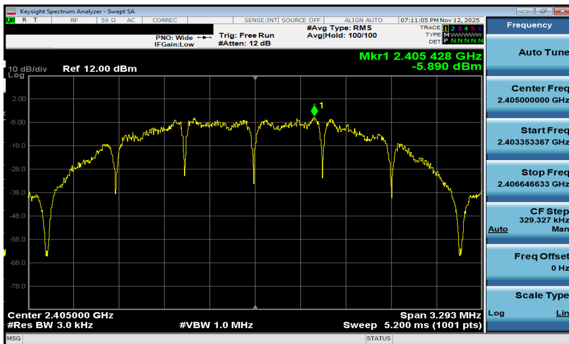
Plot 7-22. Power Spectral Density Antenna WF7b (802.15.4, iPA – Ch. 11)
