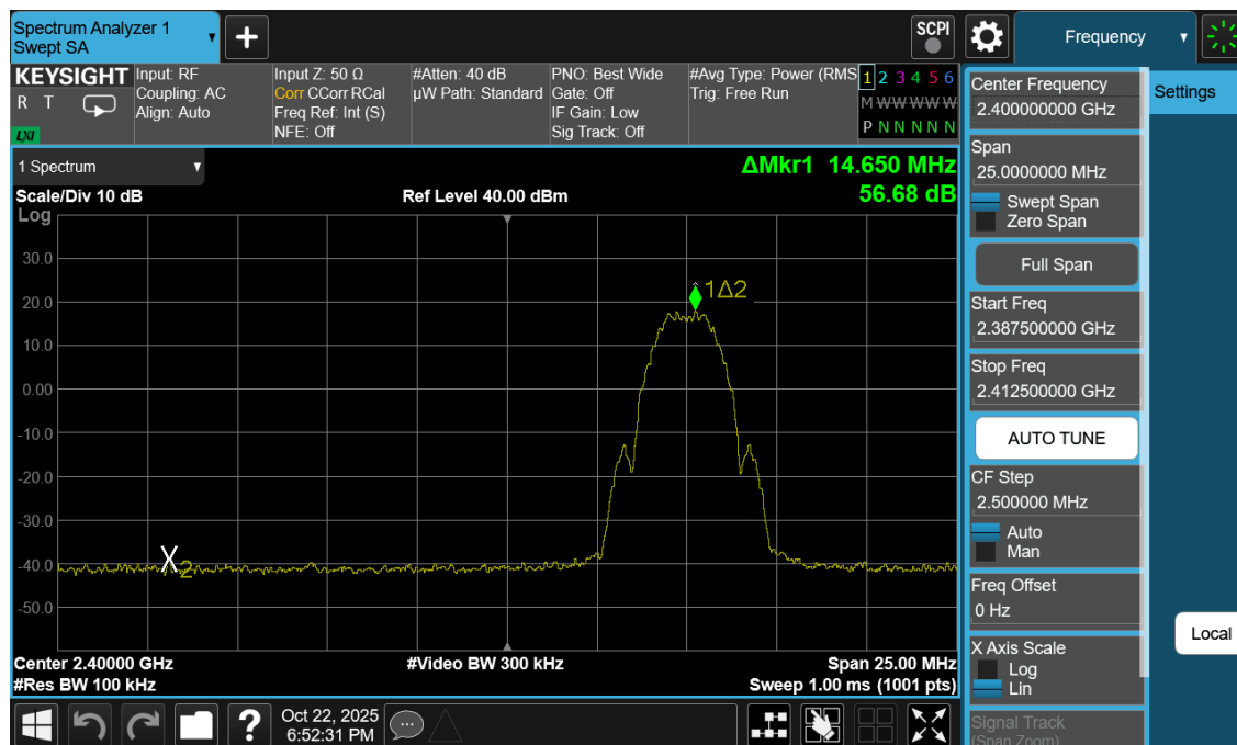
Plot 7-27. Band Edge Antenna WF7b (802.15.4, ePA – Ch. 11)
