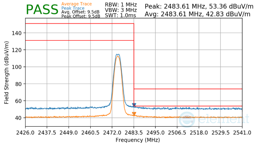
Plot 7-52. Radiated Restricted Upper Band Edge Measurement Antenna WF7b
