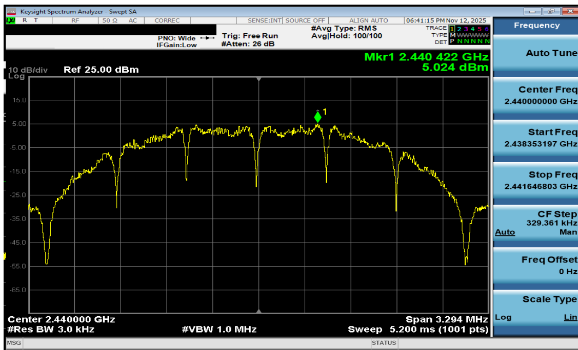
Plot 7-20. Power Spectral Density Antenna WF7b (802.15.4, ePA – Ch. 18)
