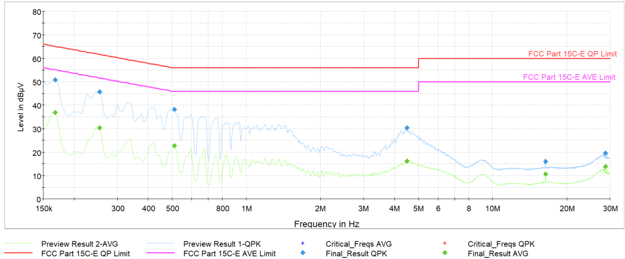
Plot 7-54. AC Line Conducted Emission with 802.15.4 Antenna WF8 (L1, Ch.18 - ePA, with AC/DC Adapter)
