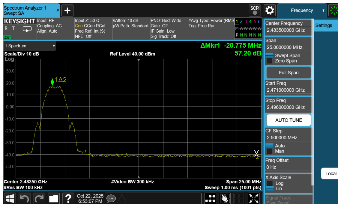
Plot 7-28. Band Edge Antenna WF7b (802.15.4, ePA – Ch. 25)
