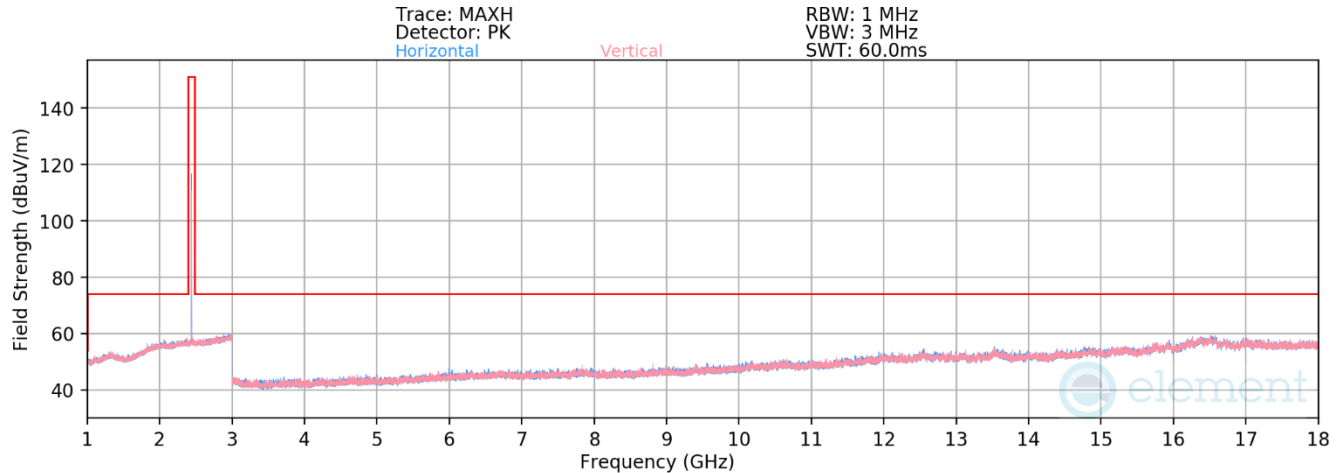
Plot 7-46. Radiated Spurious Emissions 1-18GHz Antenna WF7b (802.15.4 ePA – Ch. 18)
