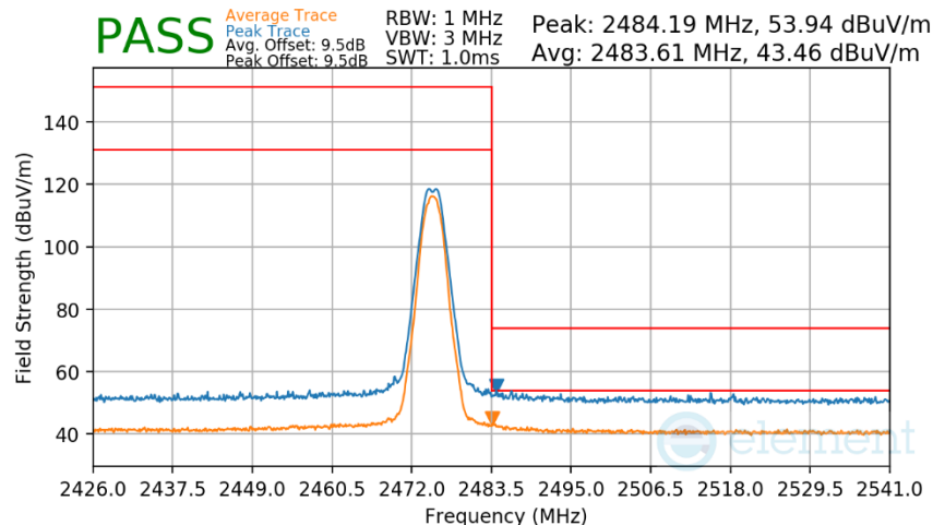
Plot 7-50. Radiated Restricted Upper Band Edge Measurement Antenna WF8
