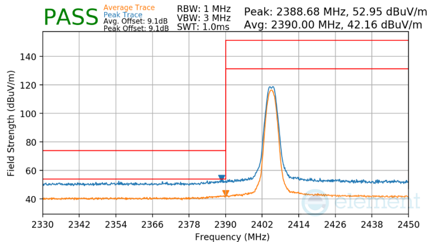
Plot 7-49. Radiated Restricted Lower Band Edge Measurement Antenna WF8
