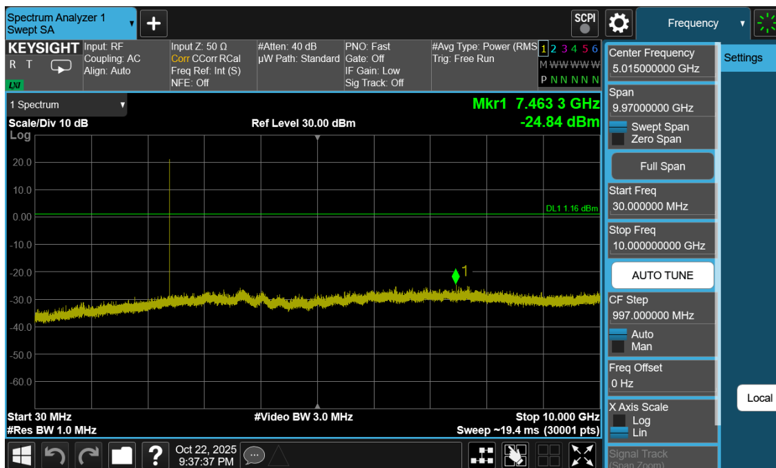
Plot 7-29. Conducted Spurious Antenna WF8 (802.15.4, ePA – Ch. 11)
