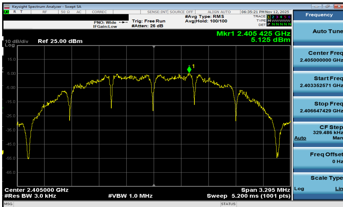
Plot 7-13. Power Spectral Density Antenna WF8 (802.15.4, ePA - Ch. 11)
