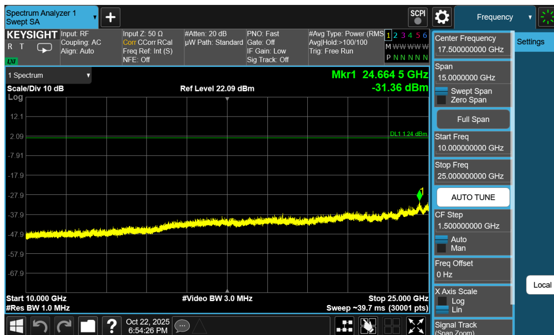
Plot 7-36. Conducted Spurious Antenna WF7b (802.15.4, ePA – Ch. 11)
