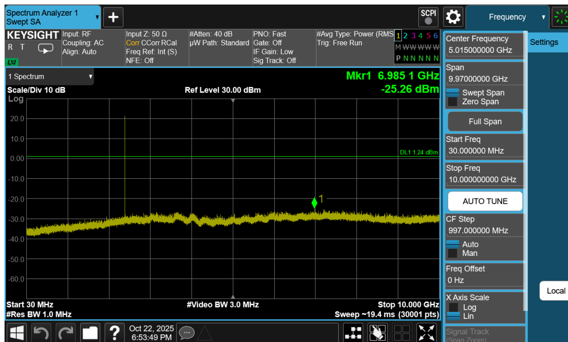
Plot 7-35. Conducted Spurious Antenna WF7b (802.15.4, ePA – Ch. 11)
