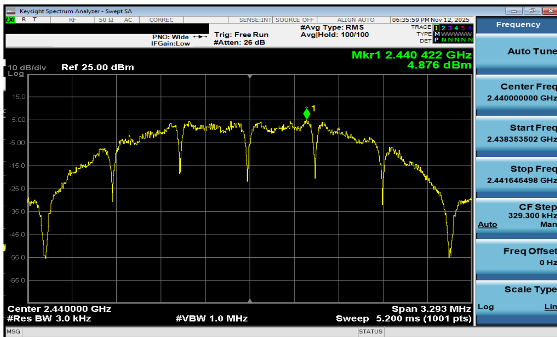
Plot 7-14. Power Spectral Density Antenna WF8 (802.15.4, ePA - Ch. 18)
