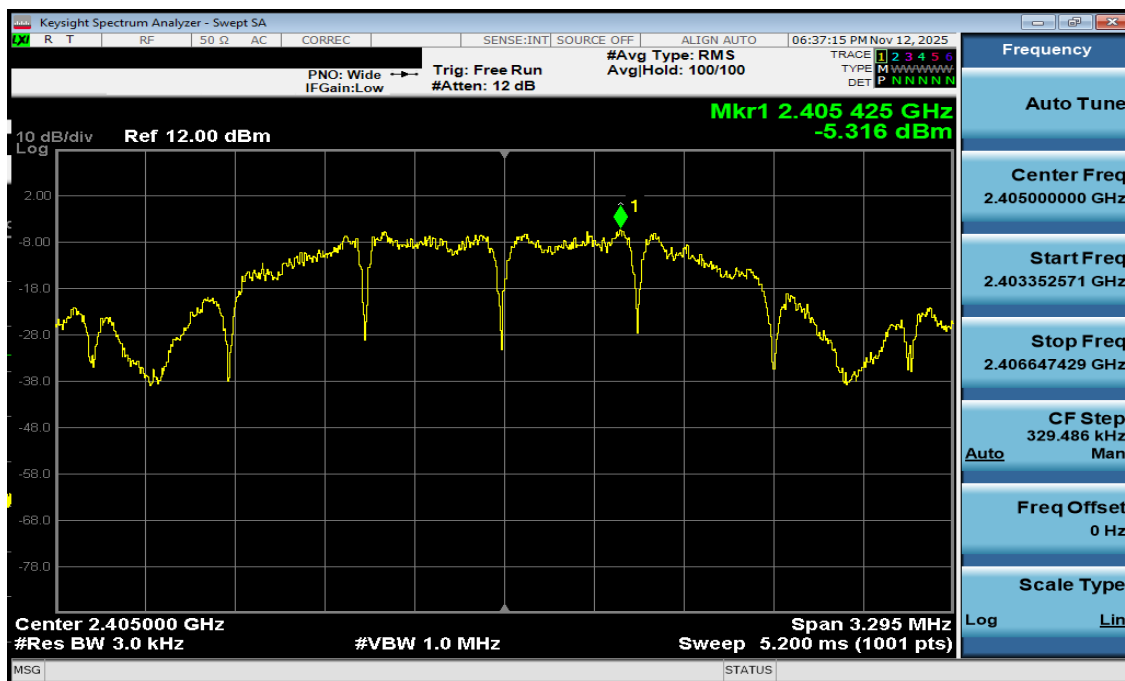
Plot 7-16. Power Spectral Density Antenna WF8 (802.15.4, iPA – Ch. 11)
