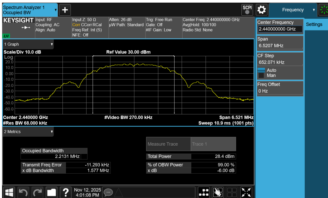
Plot 7-5. 99% OBW Antenna WF7b (802.15.4, Ch. 18)
