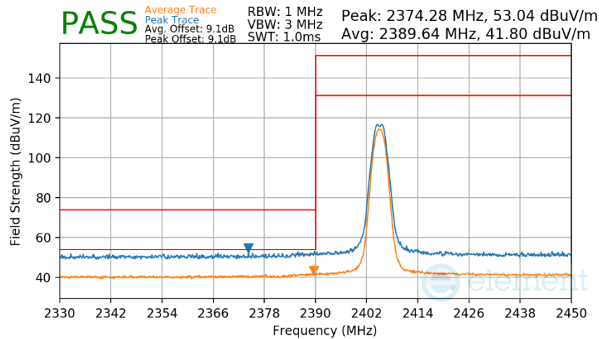
Plot 7-51. Radiated Restricted Lower Band Edge Measurement Antenna WF7b
