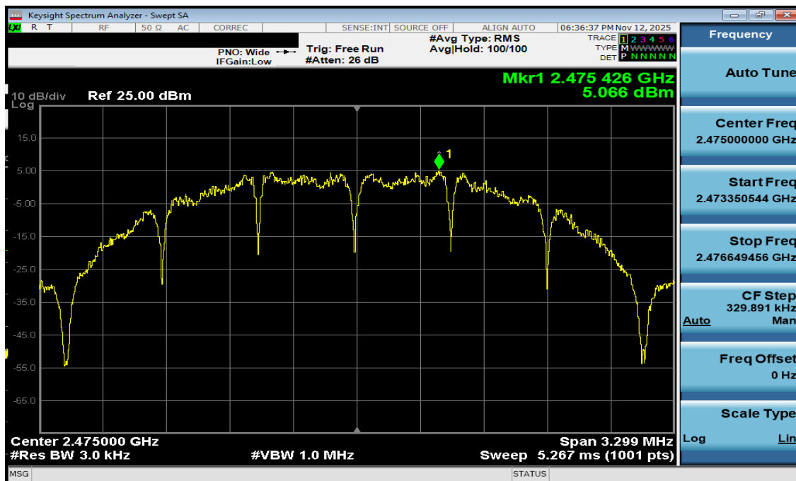
Plot 7-15. Power Spectral Density Antenna WF8 (802.15.4, ePA – Ch. 25)
