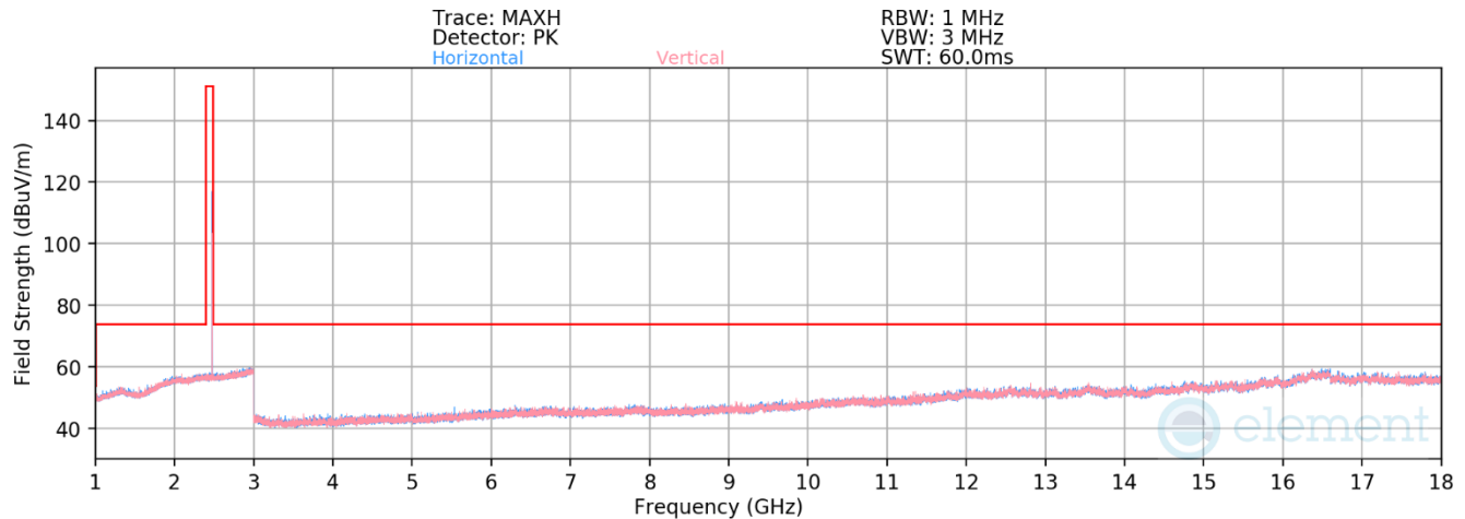
Plot 7-44. Radiated Spurious Emissions 1-18GHz Antenna WF8 (802.15.4 ePA – Ch. 25)
