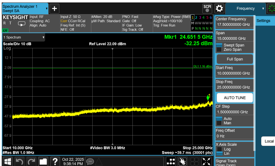
Plot 7-30. Conducted Spurious Antenna WF8 (802.15.4, ePA – Ch. 11)
