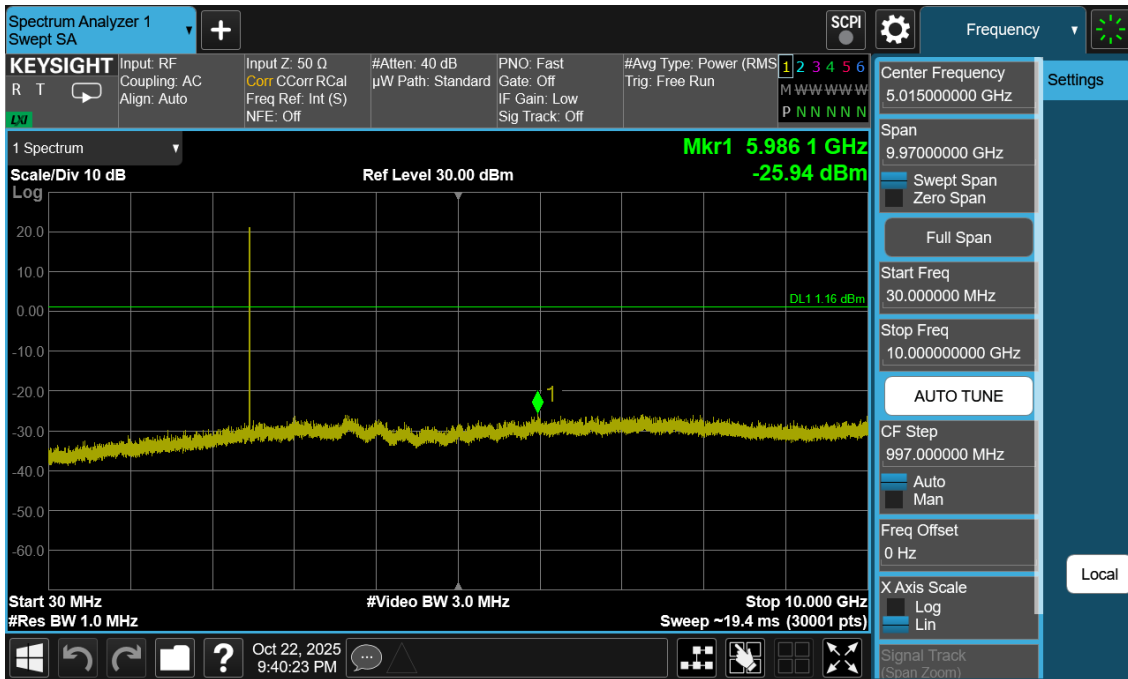
Plot 7-33. Conducted Spurious Antenna WF8 (802.15.4, ePA – Ch. 25)
