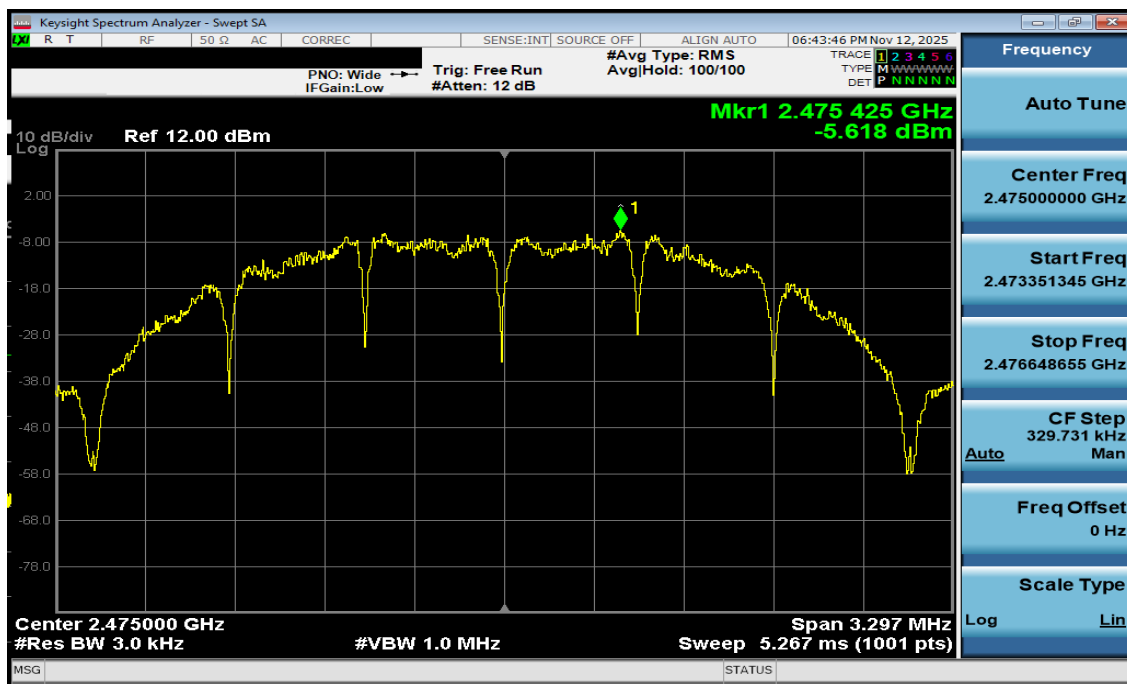
Plot 7-24. Power Spectral Density Antenna WF7b (802.15.4, iPA – Ch. 25)
