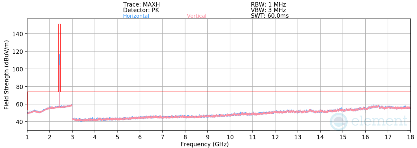
Plot 7-42. Radiated Spurious Emissions 1-18GHz Antenna WF8 (802.15.4 ePA – Ch. 18)
