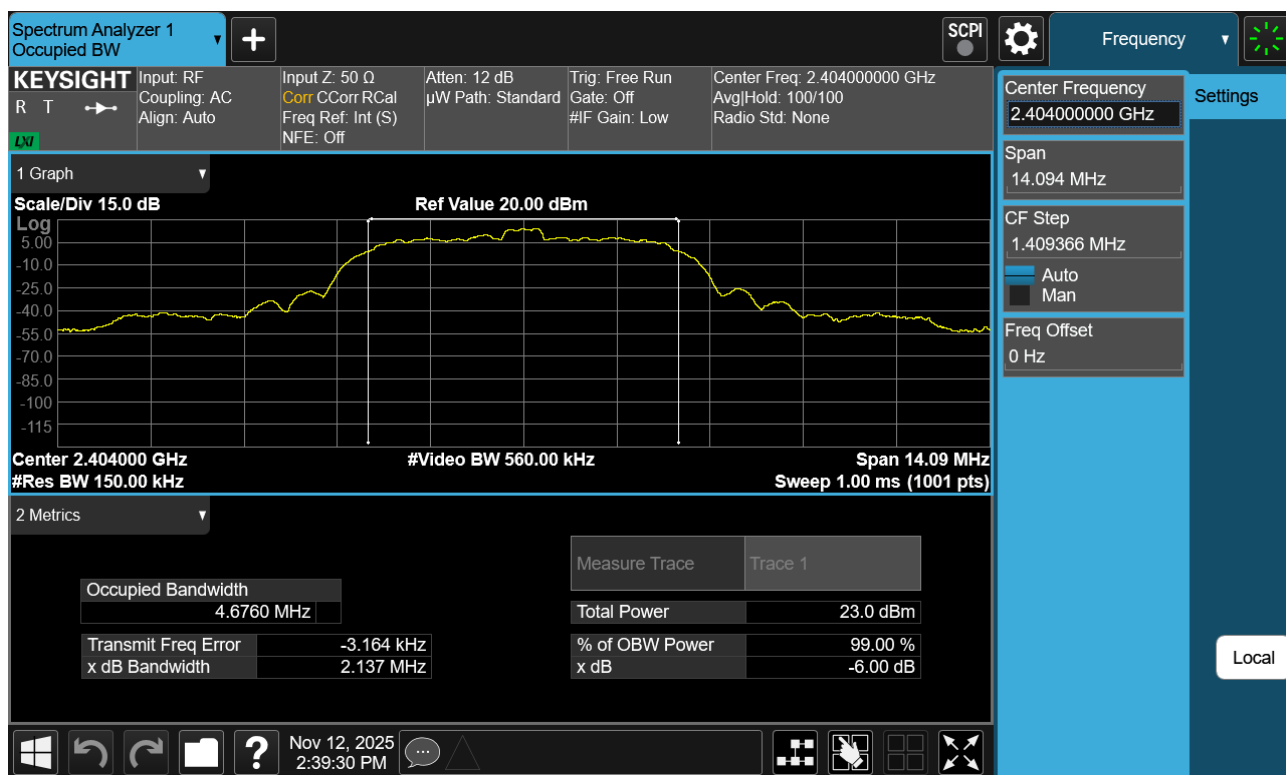
Plot 7-22. 99% OBW Plot Antenna WF7b (Bluetooth (HDR8), 8Mbps, ePA – Ch. 1)
