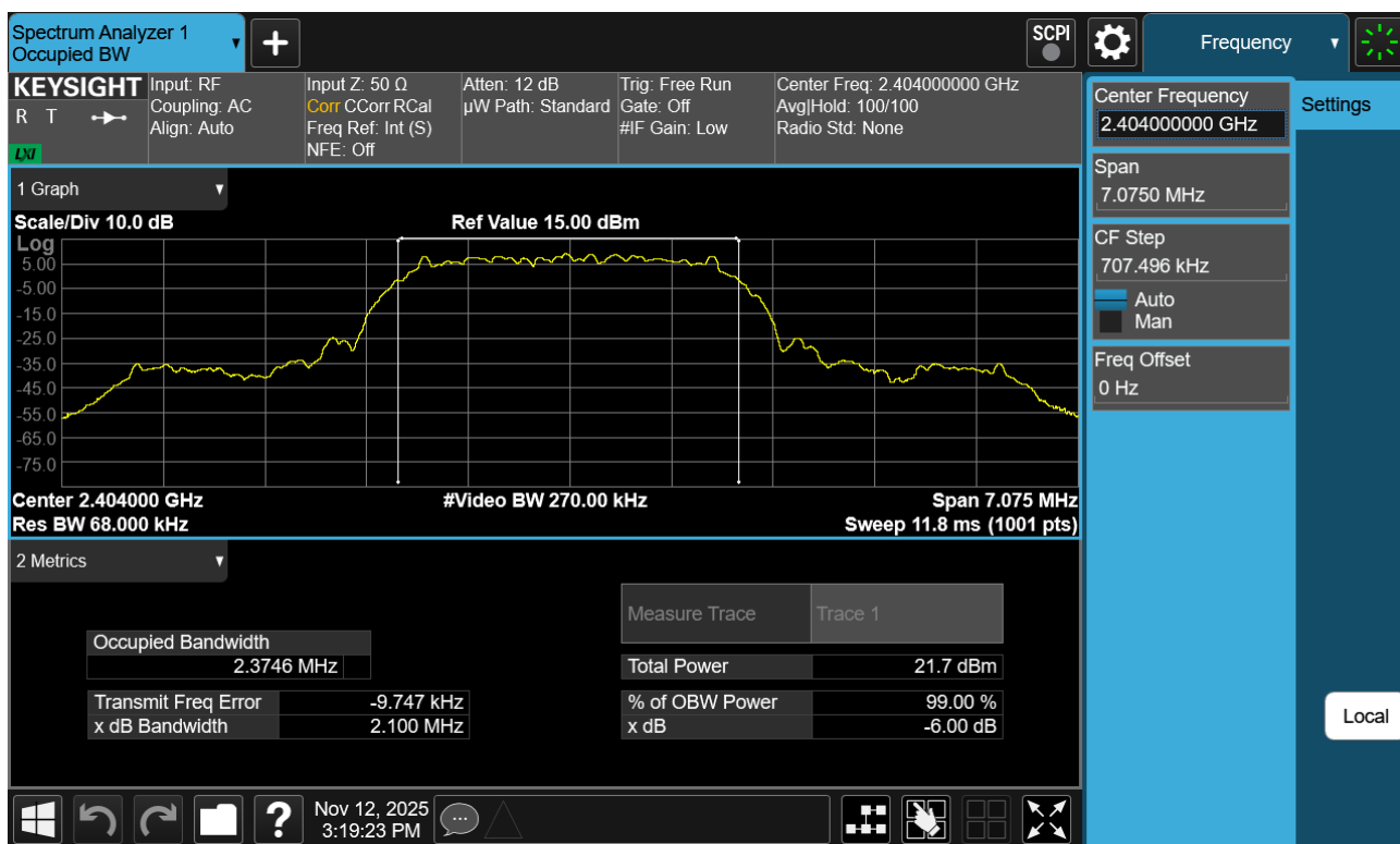
Plot 7-34. 99% OBW Plot Antenna WF7b (Bluetooth (HDT2), 2Mbps, ePA – Ch. 1)
