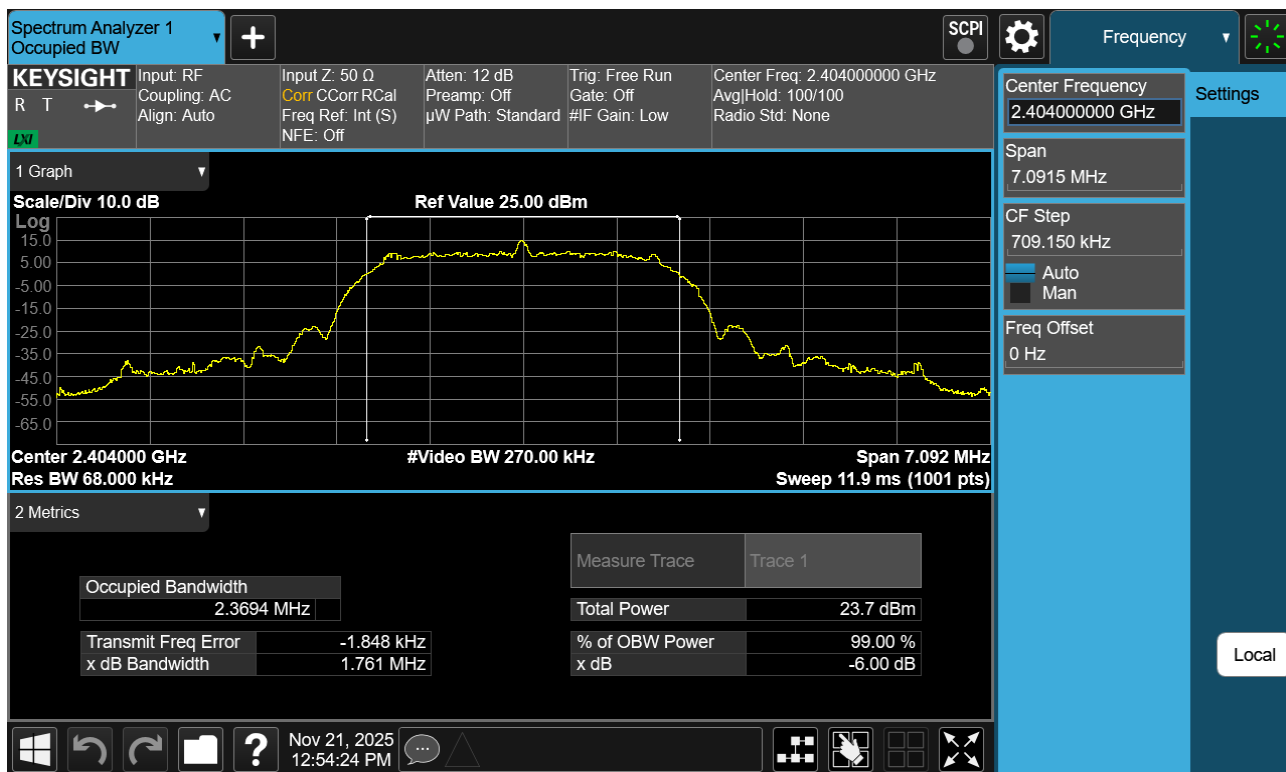
Plot 7-7. 99% OBW Plot Antenna WF8 (Bluetooth (HDRPS2), 2Mbps, ePA – Ch. 1)
