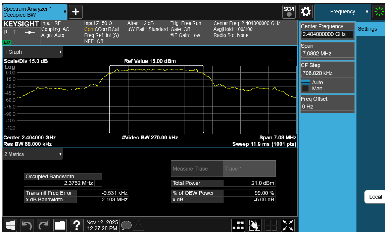
Plot 7-16. 99% OBW Plot Antenna WF8 (Bluetooth (HDT2), 2Mbps, ePA – Ch. 1)
