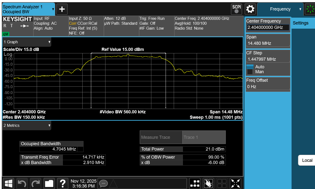
Plot 7-31. 99% OBW Plot Antenna WF7b (Bluetooth (HDRPM16), 16Mbps, ePA – Ch. 1)
