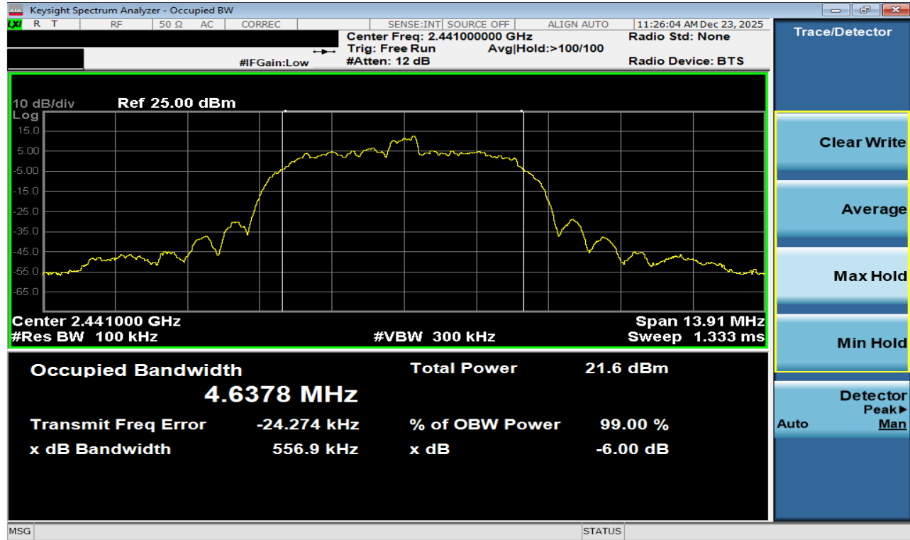
Plot 7-41. 6dB BW Plot Antenna WF8 (Bluetooth (HDR8), 8Mbps, ePA – Ch. 38)
