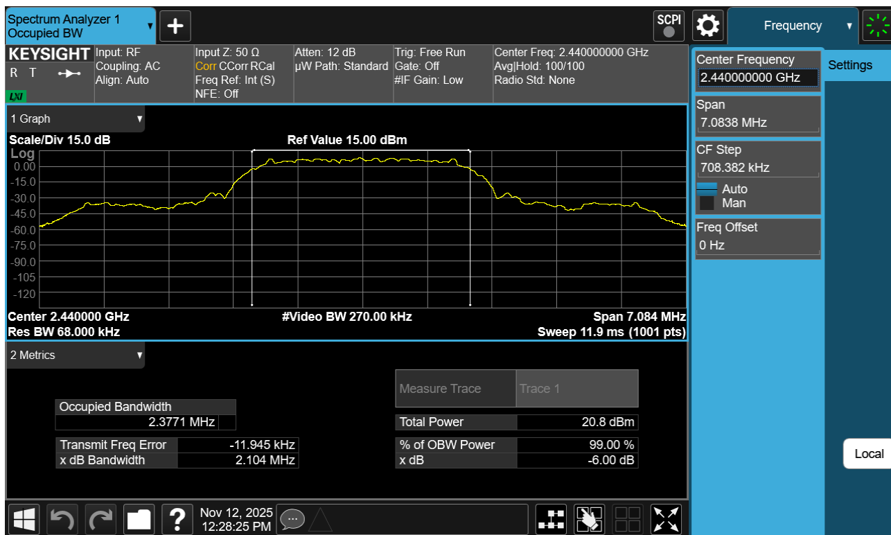
Plot 7-17. 99% OBW Plot Antenna WF8 (Bluetooth (HDT2), 2Mbps, ePA – Ch. 37)
