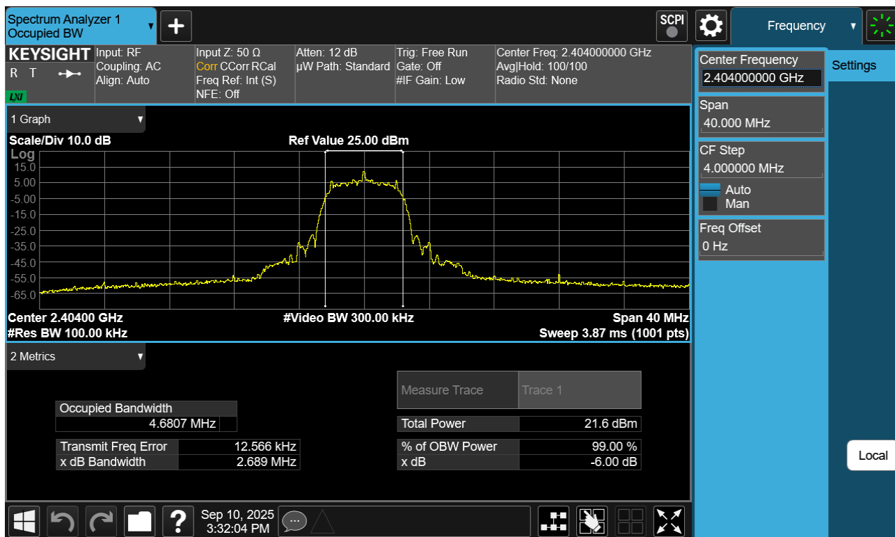
Plot 7-49. 6dB BW Plot Antenna WF8 (Bluetooth (HDRPM16), 16Mbps, ePA – Ch. 1)
