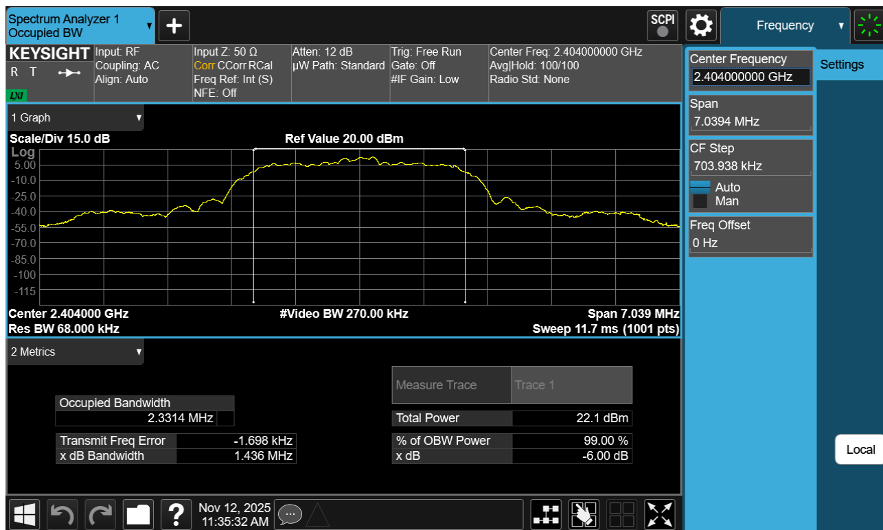
Plot 7-1. 99% OBW Plot Antenna WF8 (Bluetooth (HDR4), 4Mbps, ePA – Ch. 1)
