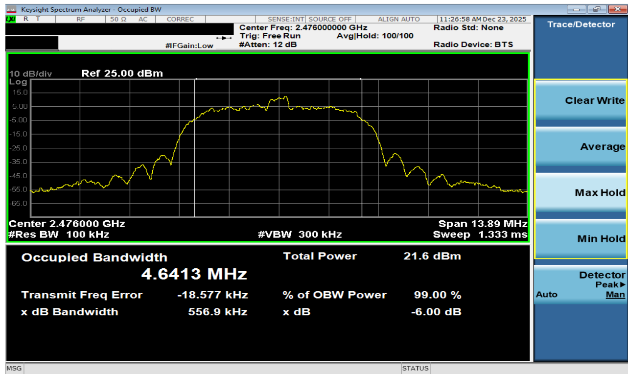
Plot 7-42. 6dB BW Plot Antenna WF8 (Bluetooth (HDR8), 8Mbps, ePA – Ch. 73)
