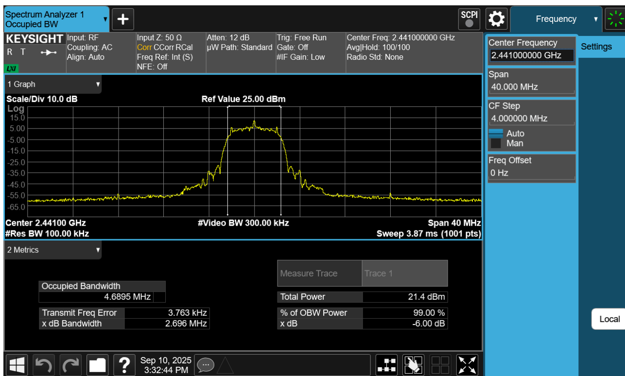
Plot 7-50. 6dB BW Plot Antenna WF8 (Bluetooth (HDRPM16), 16Mbps, ePA – Ch. 38)
