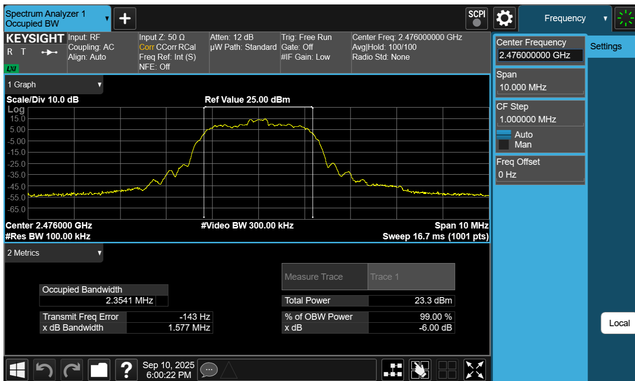
Plot 7-57. 6dB BW Plot Antenna WF7b (Bluetooth (HDR4), 4Mbps, ePA – Ch. 73)
