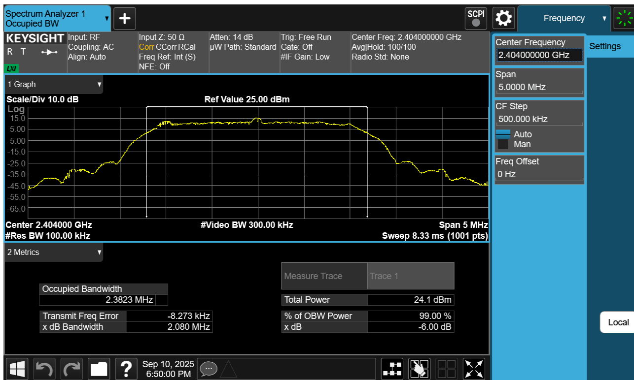
Plot 7-61. 6dB BW Plot Antenna WF7b (Bluetooth (HDRPS2), 2Mbps, ePA – Ch. 1)
