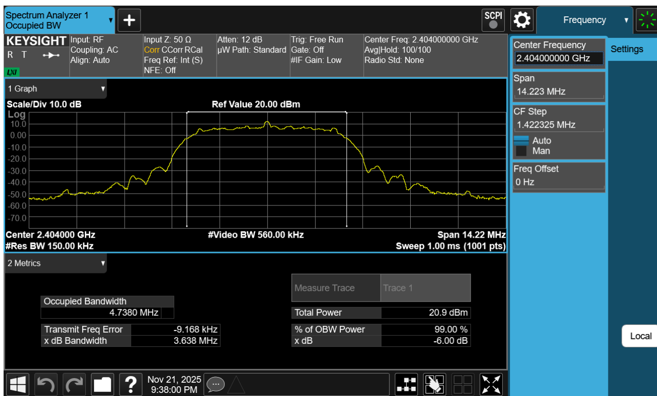
Plot 7-10. 99% OBW Plot Antenna WF8 (Bluetooth (XHDRPM6), 6Mbps, ePA – Ch. 1)
