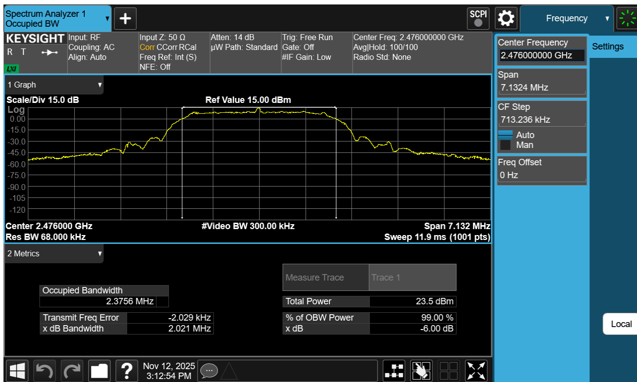
Plot 7-27. 99% OBW Plot Antenna WF7b (Bluetooth (HDRPS2), 2Mbps, ePA – Ch. 73)
