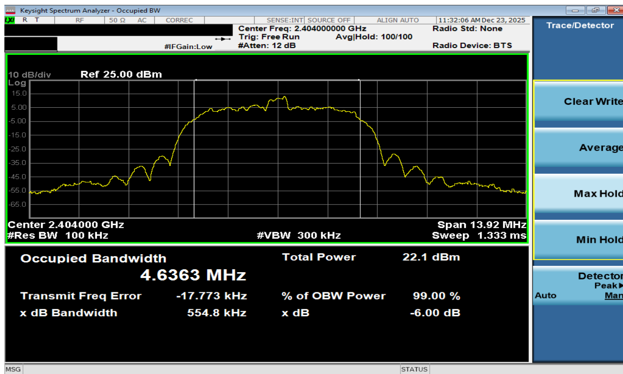
Plot 7-58. 6dB BW Plot Antenna WF7b (Bluetooth (HDR8), 8Mbps, ePA – Ch. 1)
