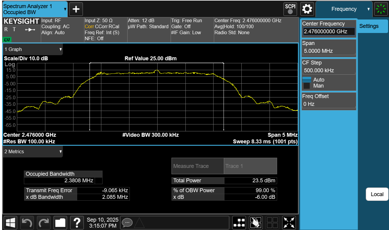
Plot 7-45. 6dB BW Plot Antenna WF8 (Bluetooth (HDRPS2), 2Mbps, ePA – Ch. 73)
