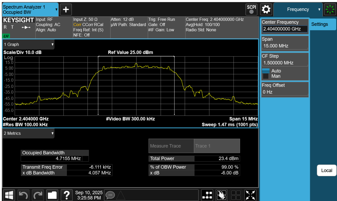
Plot 7-46. 6dB BW Plot Antenna WF8 (Bluetooth (XHDRPM6), 6Mbps, ePA – Ch. 1)
