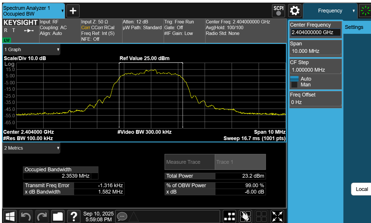
Plot 7-55. 6dB BW Plot Antenna WF7b (Bluetooth (HDR4), 4Mbps, ePA – Ch. 1)
