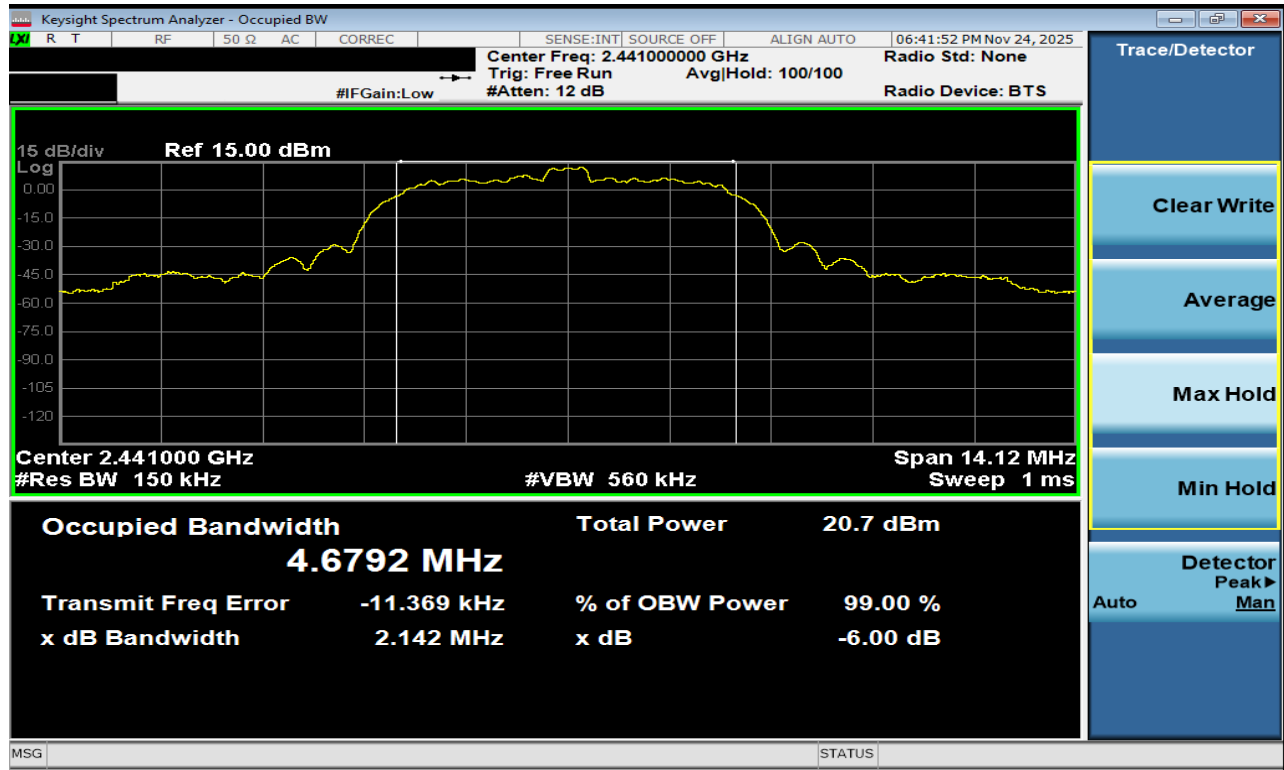
Plot 7-5. 99% OBW Plot Antenna WF8 (Bluetooth (HDR8), 8Mbps, ePA – Ch. 38)
