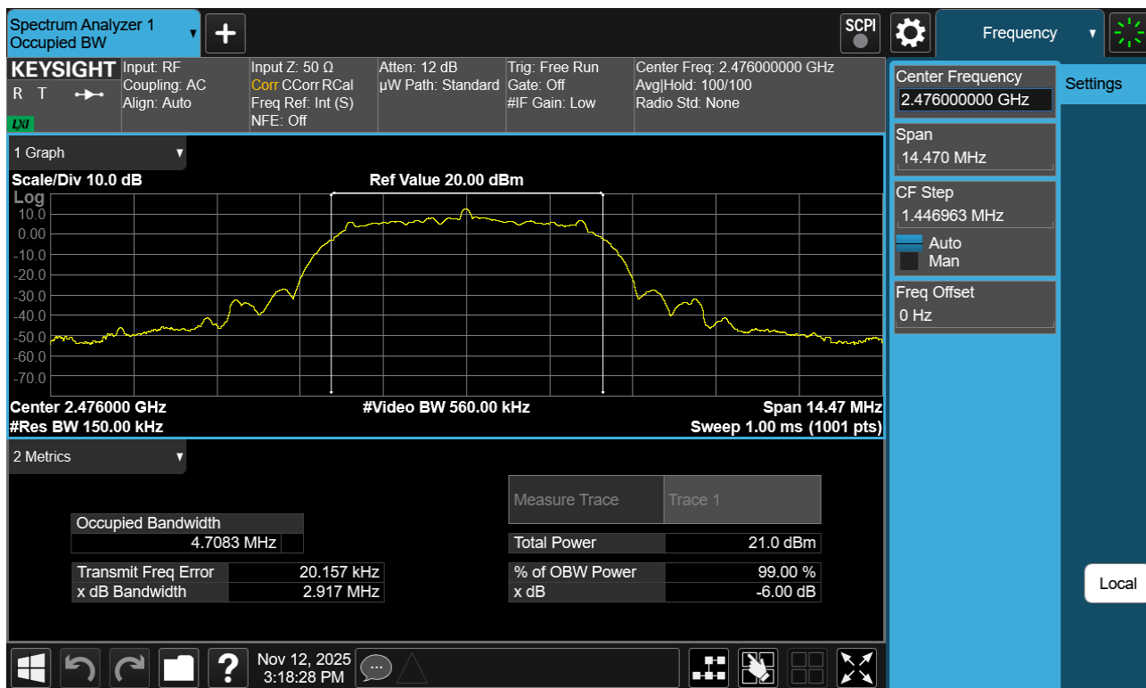
Plot 7-33. 99% OBW Plot Antenna WF7b (Bluetooth (HDRPM16), 16Mbps, ePA – Ch. 73)
