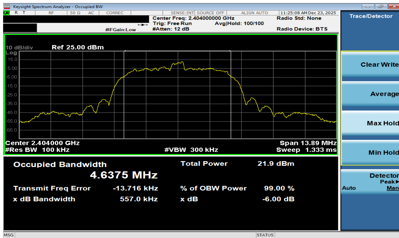
Plot 7-40. 6dB BW Plot Antenna WF8 (Bluetooth (HDR8), 8Mbps, ePA – Ch. 1)
