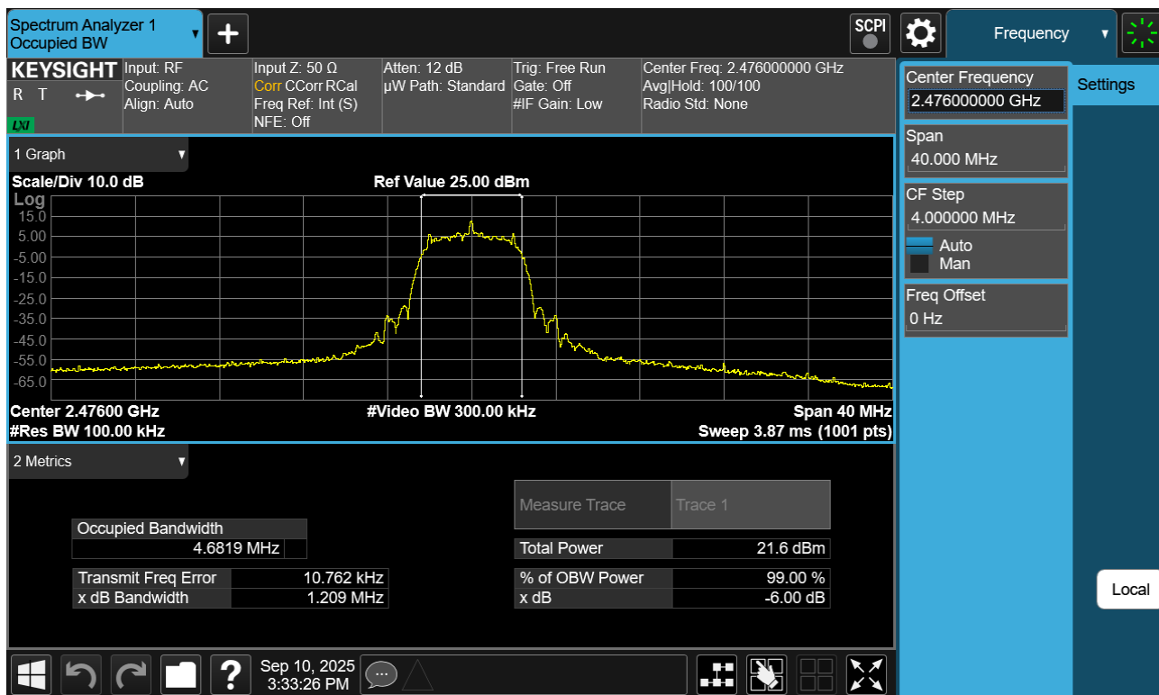
Plot 7-51. 6dB BW Plot Antenna WF8 (Bluetooth (HDRPM16), 16Mbps, ePA – Ch. 73)
