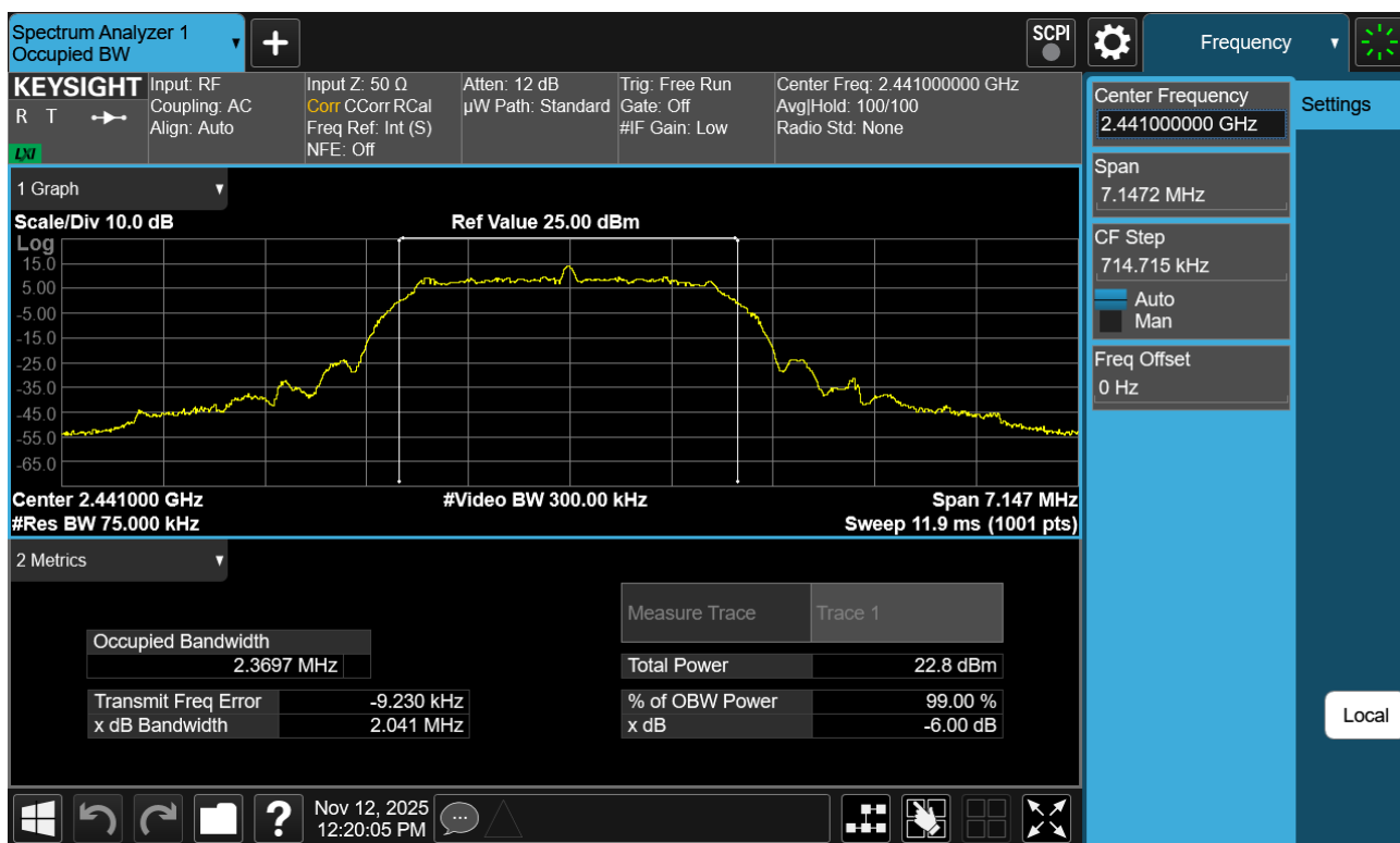
Plot 7-8. 99% OBW Plot Antenna WF8 (Bluetooth (HDRPS2), 2Mbps, ePA – Ch. 38)
