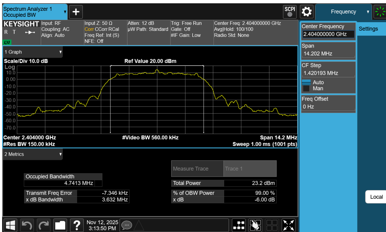
Plot 7-28. 99% OBW Plot Antenna WF7b (Bluetooth (XHDRPM6), 6Mbps, ePA – Ch. 1)
