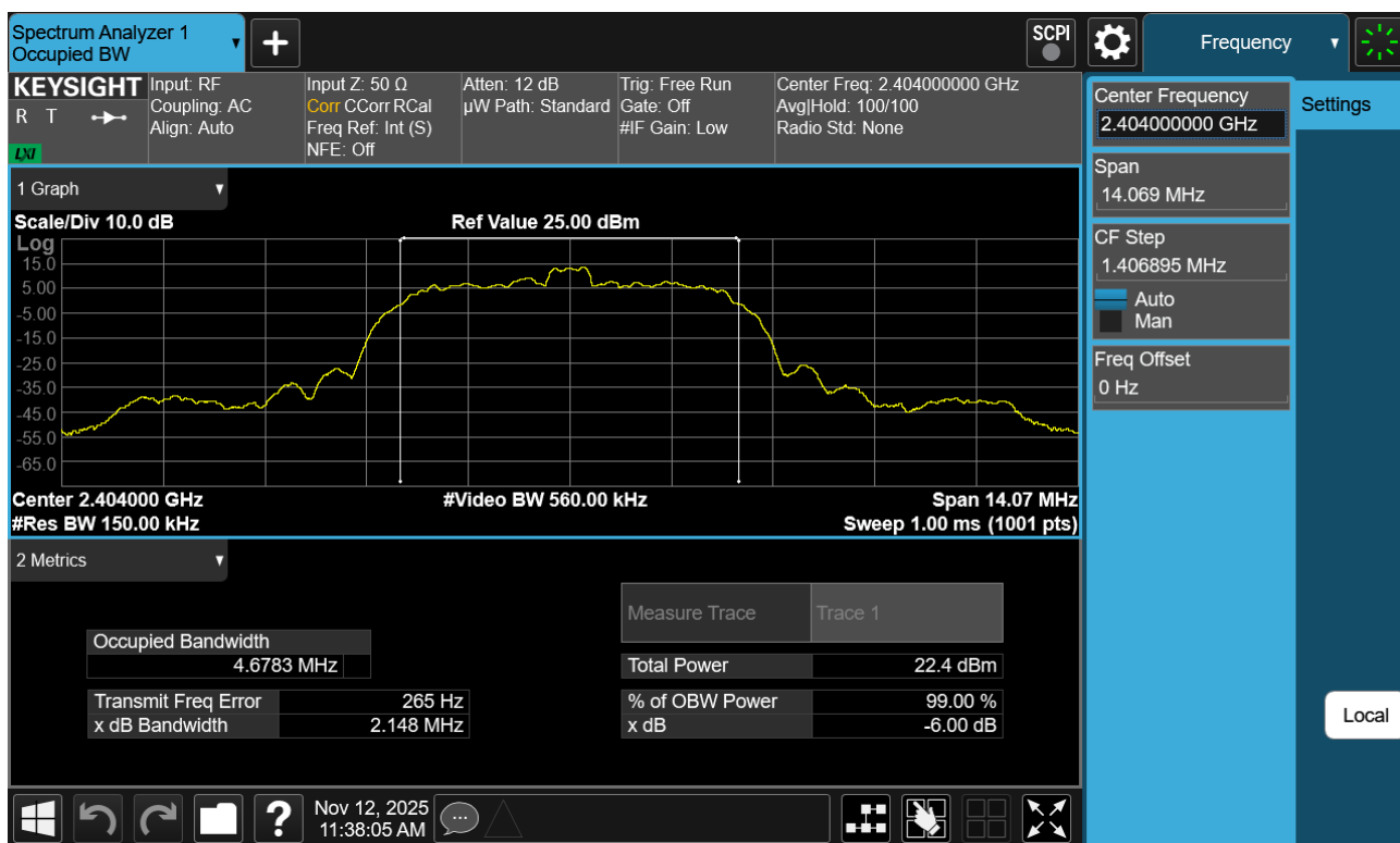
Plot 7-4. 99% OBW Plot Antenna WF8 (Bluetooth (HDR8), 8Mbps, ePA – Ch. 1)
