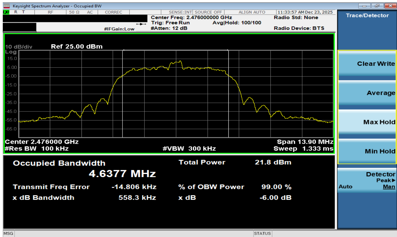
Plot 7-60. 6dB BW Plot Antenna WF7b (Bluetooth (HDR8), 8Mbps, ePA – Ch. 73)
