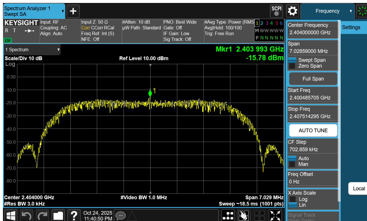
Plot 7-136. Power Spectral Density Plot Antenna WF7b (Bluetooth (HDRPM16), 16Mbps, iPA – Ch. 1)
