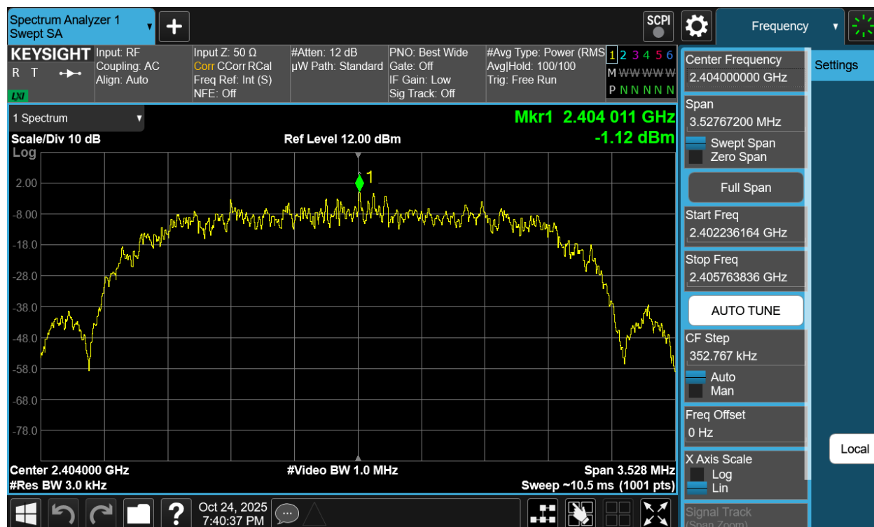
Plot 7-145. Power Spectral Density Plot Tx BF Antenna WF8 (Bluetooth (HDR4), 4Mbps, ePA – Ch. 1)
