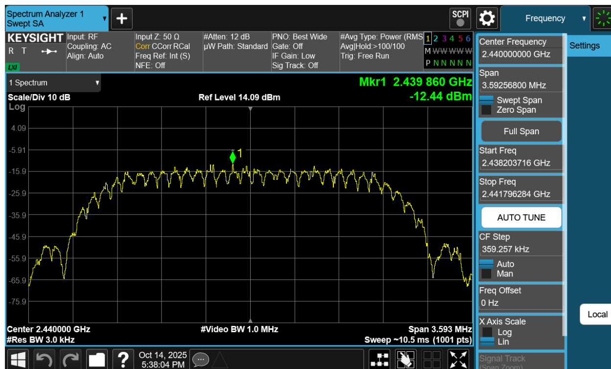
Plot 7-143. Power Spectral Density Plot Antenna WF7b (Bluetooth (HDT2), 2Mbps, iPA – Ch. 37)
