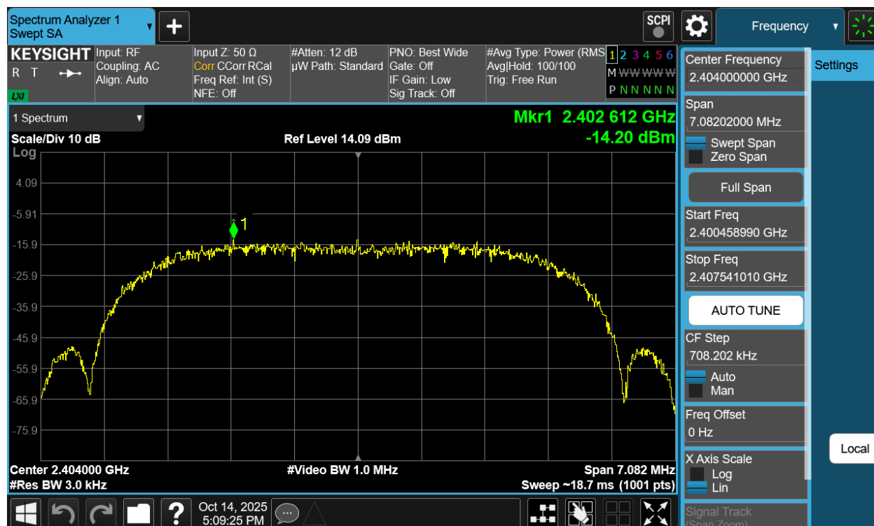
Plot 7-130. Power Spectral Density Plot Antenna WF7b (Bluetooth (XHDRPM6), 6Mbps, iPA – Ch. 1)
