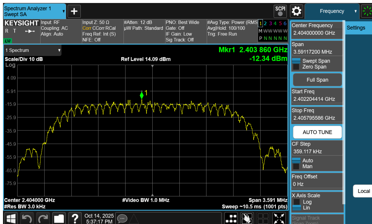
Plot 7-142. Power Spectral Density Plot Antenna WF7b (Bluetooth (HDT2), 2Mbps, iPA – Ch. 1)
