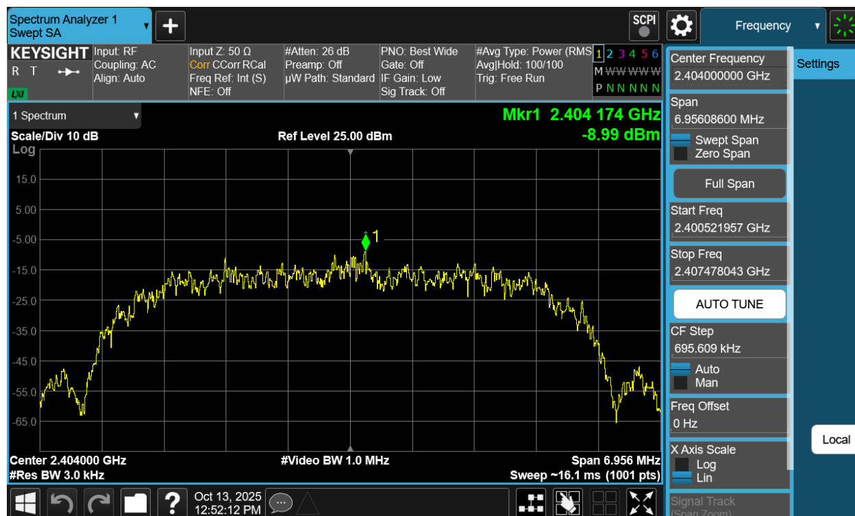
Plot 7-163. Power Spectral Density Plot Tx BF Antenna WF8 (Bluetooth (HDR8), 8Mbps, iPA – Ch. 1)
