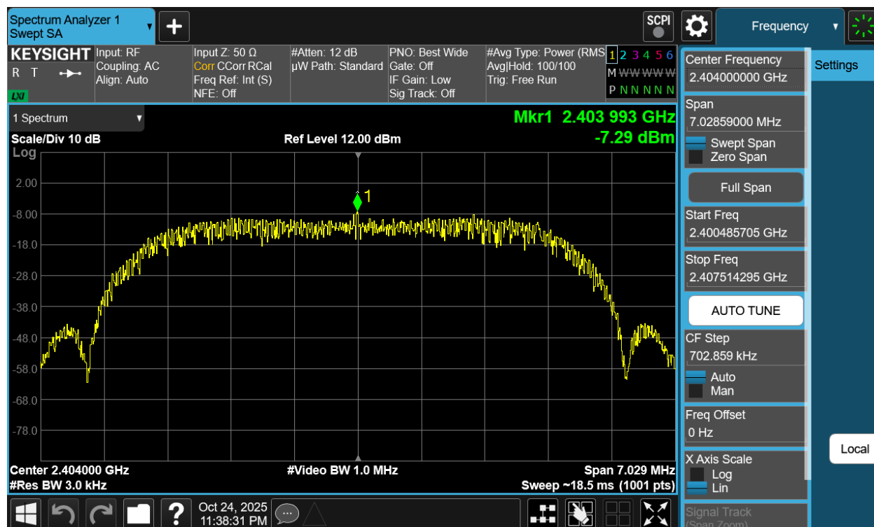
Plot 7-133. Power Spectral Density Plot Antenna WF7b (Bluetooth (HDRPM16), 16Mbps, ePA – Ch. 1)
