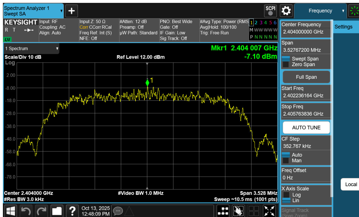
Plot 7-151. Power Spectral Density Plot Tx BF Antenna WF8 (Bluetooth (HDR4), 4Mbps, iPA – Ch. 1)
