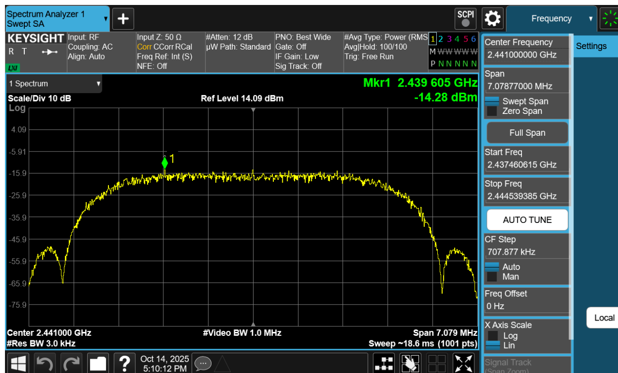
Plot 7-131. Power Spectral Density Plot Antenna WF7b (Bluetooth (XHDRPM6), 6Mbps, iPA – Ch. 38)
