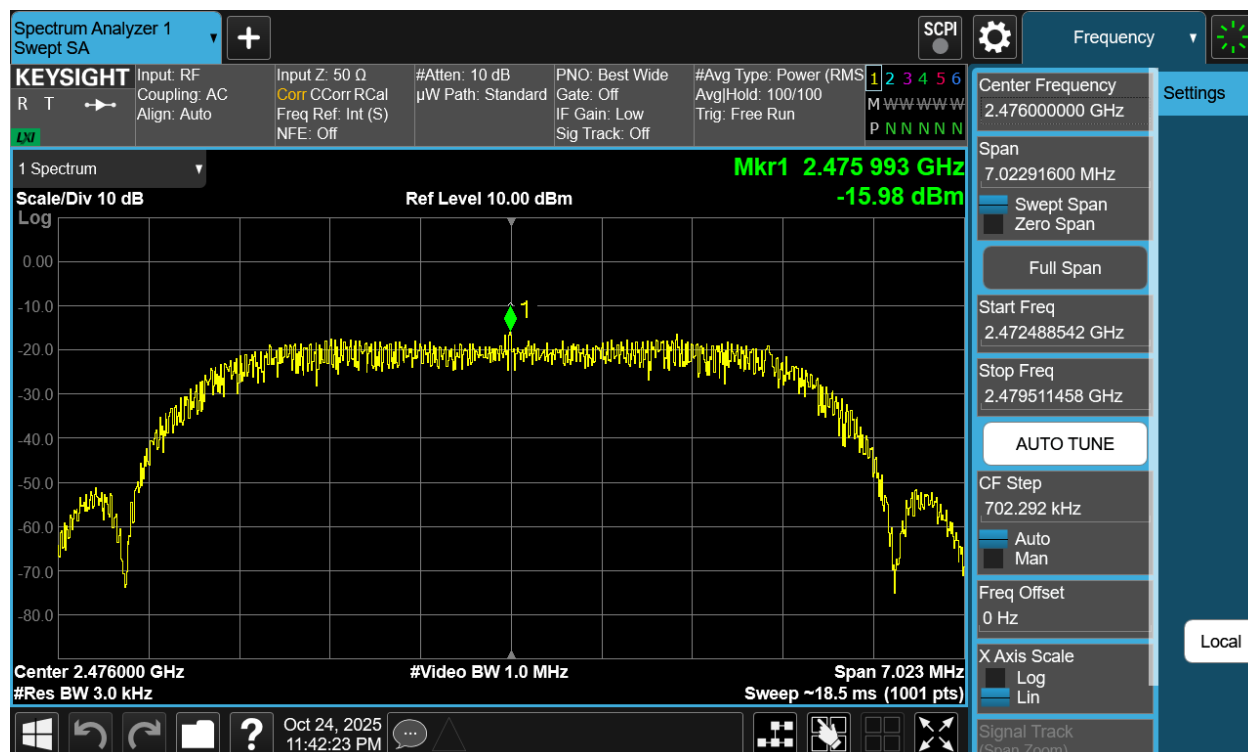
Plot 7-138. Power Spectral Density Plot Antenna WF7b (Bluetooth (HDRPM16), 16Mbps, iPA – Ch. 73)
