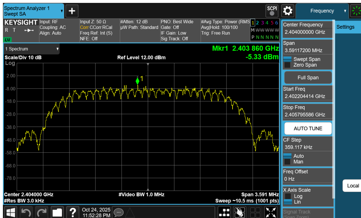
Plot 7-139. Power Spectral Density Plot Antenna WF7b (Bluetooth (HDT2), 2Mbps, ePA – Ch. 1)
