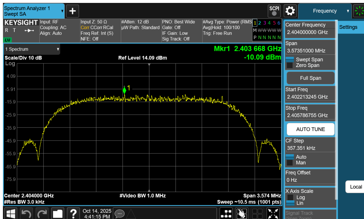
Plot 7-124. Power Spectral Density Plot Antenna WF7b (Bluetooth (HDRPS2), 2Mbps, iPA – Ch. 1)
