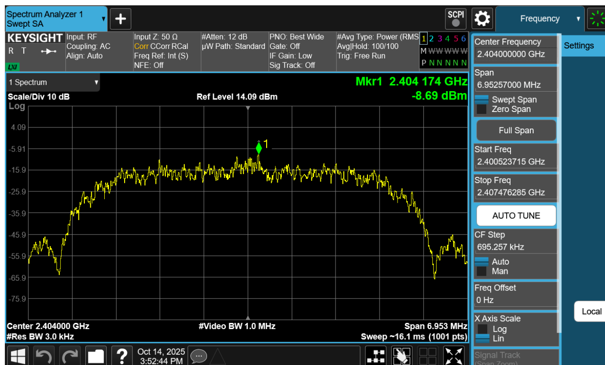
Plot 7-164. Power Spectral Density Plot Tx BF Antenna WF7b (Bluetooth (HDR8), 8Mbps, iPA – Ch. 1)
