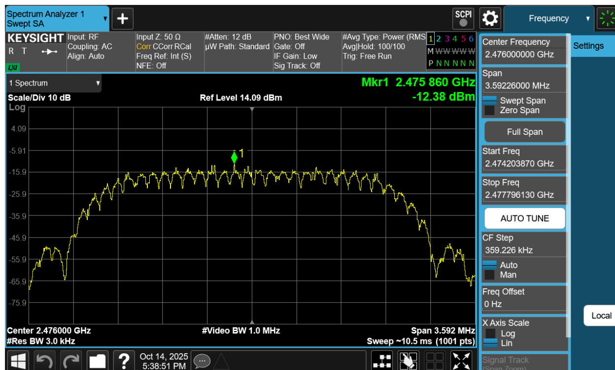
Plot 7-144. Power Spectral Density Plot Antenna WF7b (Bluetooth (HDT2), 2Mbps, iPA – Ch. 73)
