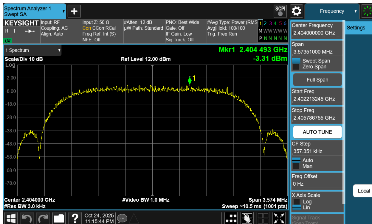
Plot 7-121. Power Spectral Density Plot Antenna WF7b (Bluetooth (HDRPS2), 2Mbps, ePA – Ch. 1)
