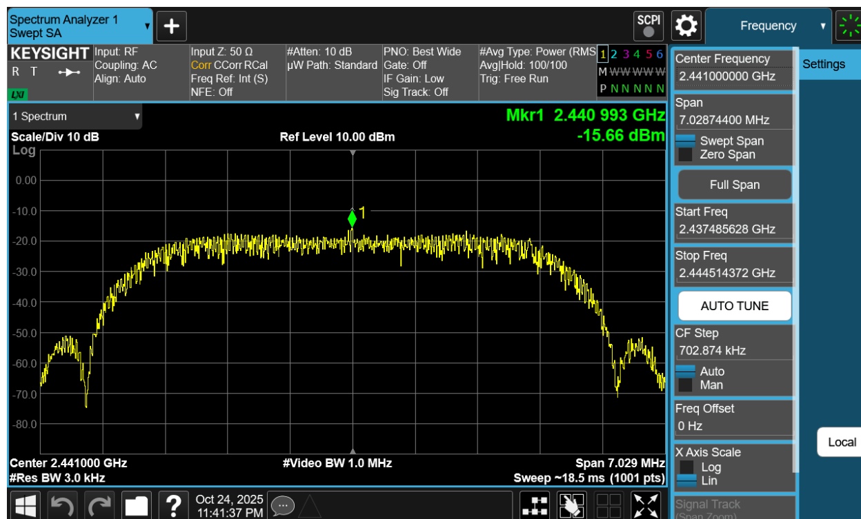
Plot 7-137. Power Spectral Density Plot Antenna WF7b (Bluetooth (HDRPM16), 16Mbps, iPA – Ch. 38)
