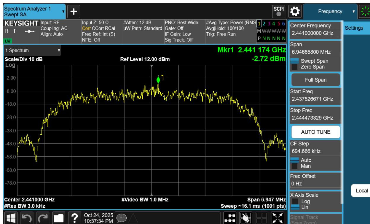
Plot 7-160. Power Spectral Density Plot Tx BF Antenna WF7b (Bluetooth (HDR8), 8Mbps, ePA – Ch. 38)
