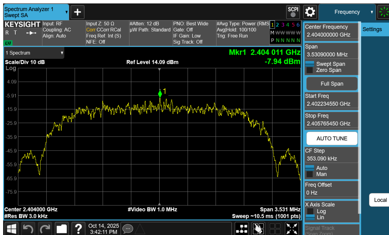
Plot 7-152. Power Spectral Density Plot Tx BF Antenna WF7b (Bluetooth (HDR4), 4Mbps, iPA – Ch. 1)
