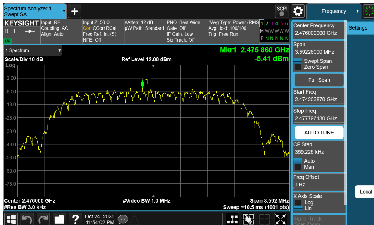
Plot 7-141. Power Spectral Density Plot Antenna WF7b (Bluetooth (HDT2), 2Mbps, ePA – Ch. 73)
