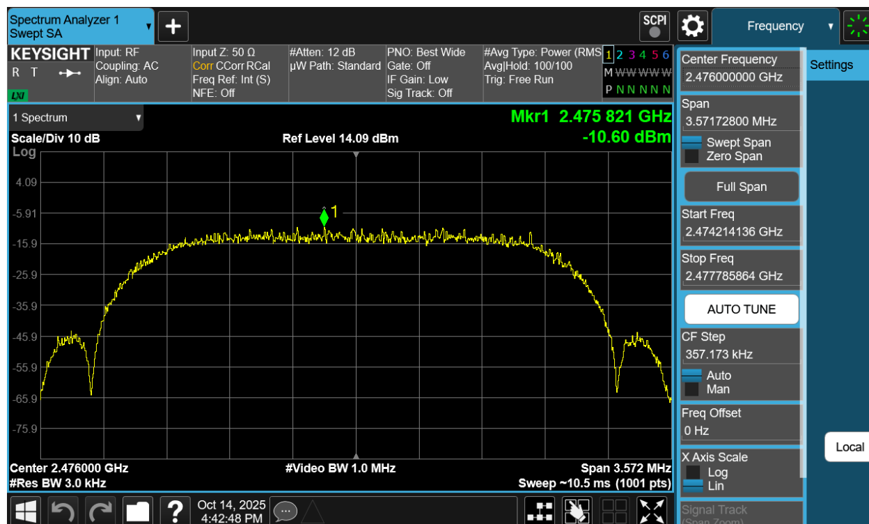
Plot 7-126. Power Spectral Density Plot Antenna WF7b (Bluetooth (HDRPS2), 2Mbps, iPA – Ch. 73)
