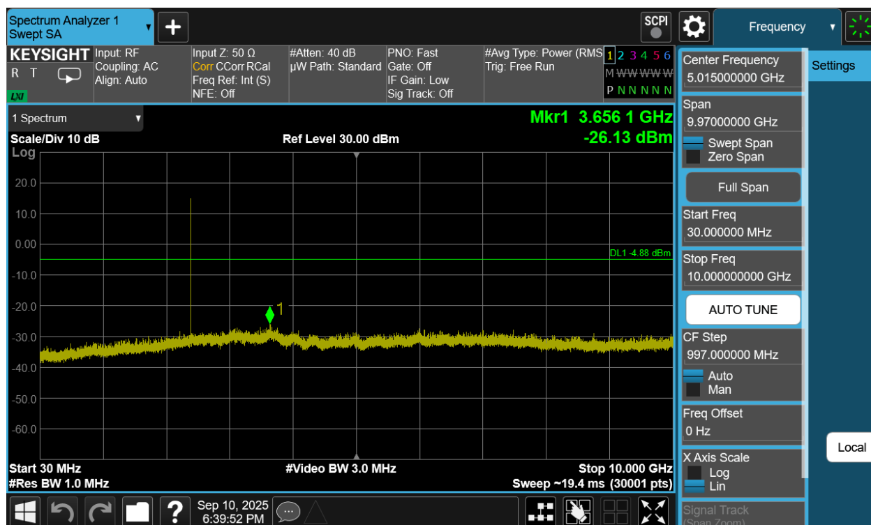
Plot 7-271. Conducted Spurious Plot Antenna WF7b (Bluetooth (HDR4), 4 Mbps, ePA – Ch. 1)
