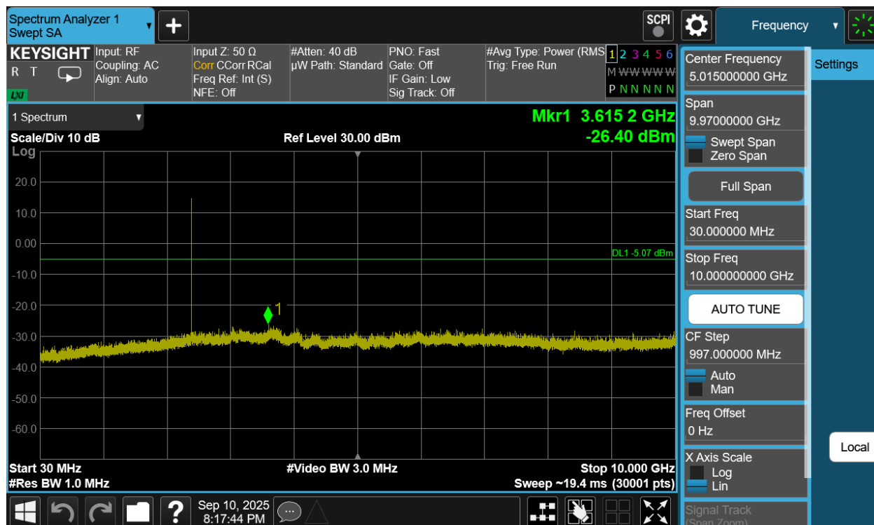
Plot 7-283. Conducted Spurious Plot Antenna WF7b (Bluetooth (XHDRPM6), 6Mbps, ePA – Ch. 1)
