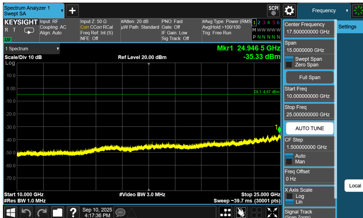
Plot 7-252. Conducted Spurious Plot Antenna WF8 (Bluetooth (HDRPS2), 8Mbps, ePA – Ch. 73)
