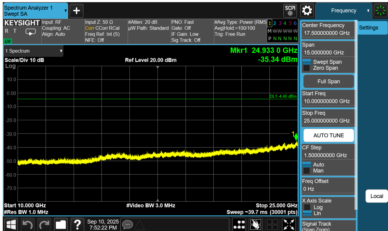
Plot 7-280. Conducted Spurious Plot Antenna WF7b (Bluetooth (HDRPS2), 8Mbps, ePA – Ch. 38)
