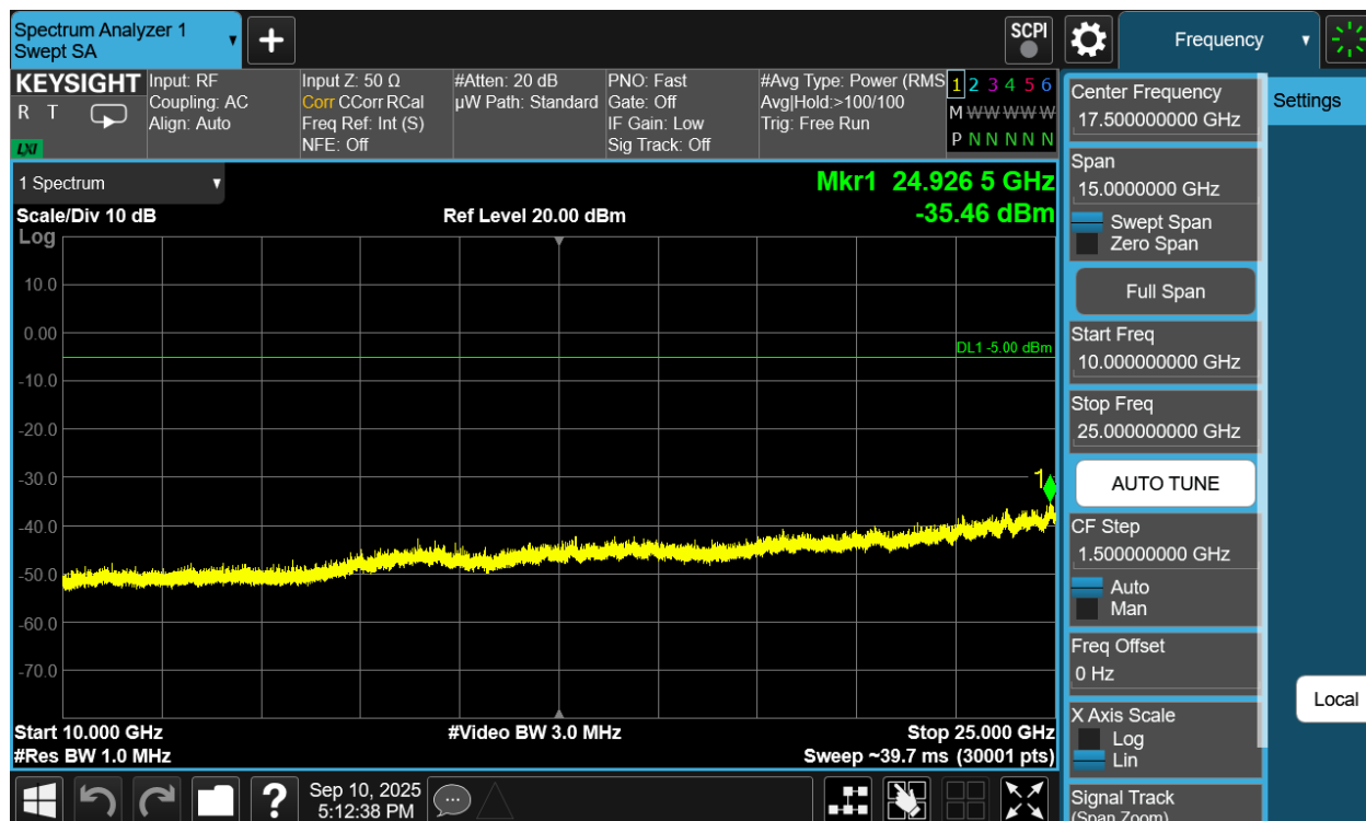
Plot 7-270. Conducted Spurious Plot Antenna WF8 (Bluetooth (HDT2), 2Mbps, ePA – Ch. 73)
