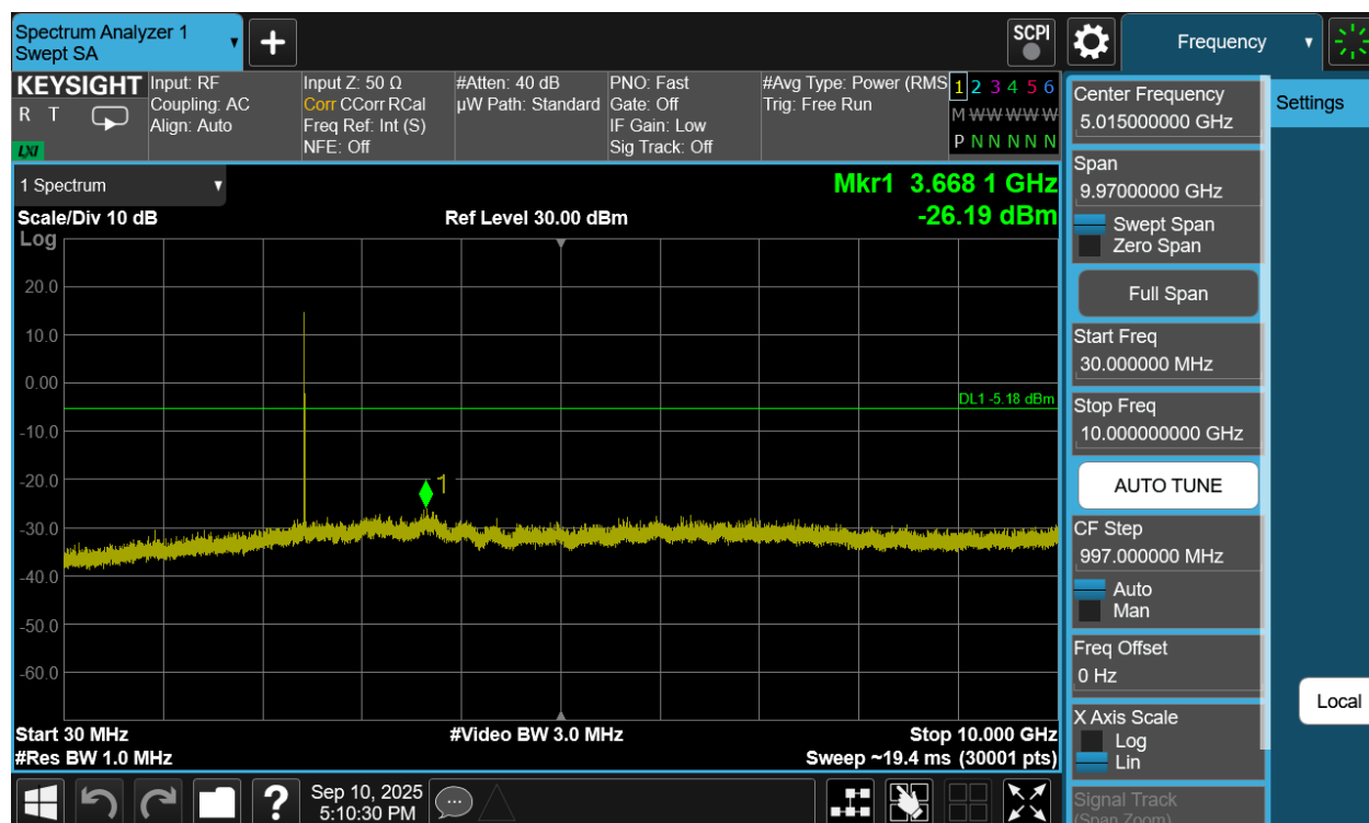
Plot 7-267. Conducted Spurious Plot Antenna WF8 (Bluetooth (HDT2), 2Mbps, ePA – Ch. 37)
