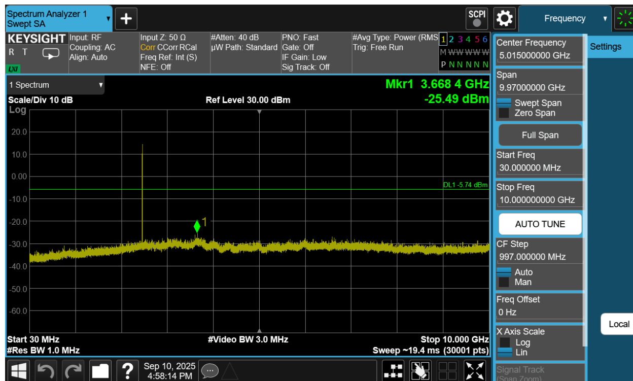
Plot 7-263. Conducted Spurious Plot Antenna WF8 (Bluetooth (HDRPM16), 16Mbps, ePA – Ch. 73)
