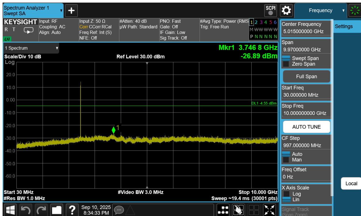
Plot 7-293. Conducted Spurious Plot Antenna WF7b (Bluetooth (HDRPM16), 16Mbps, ePA – Ch. 73)
