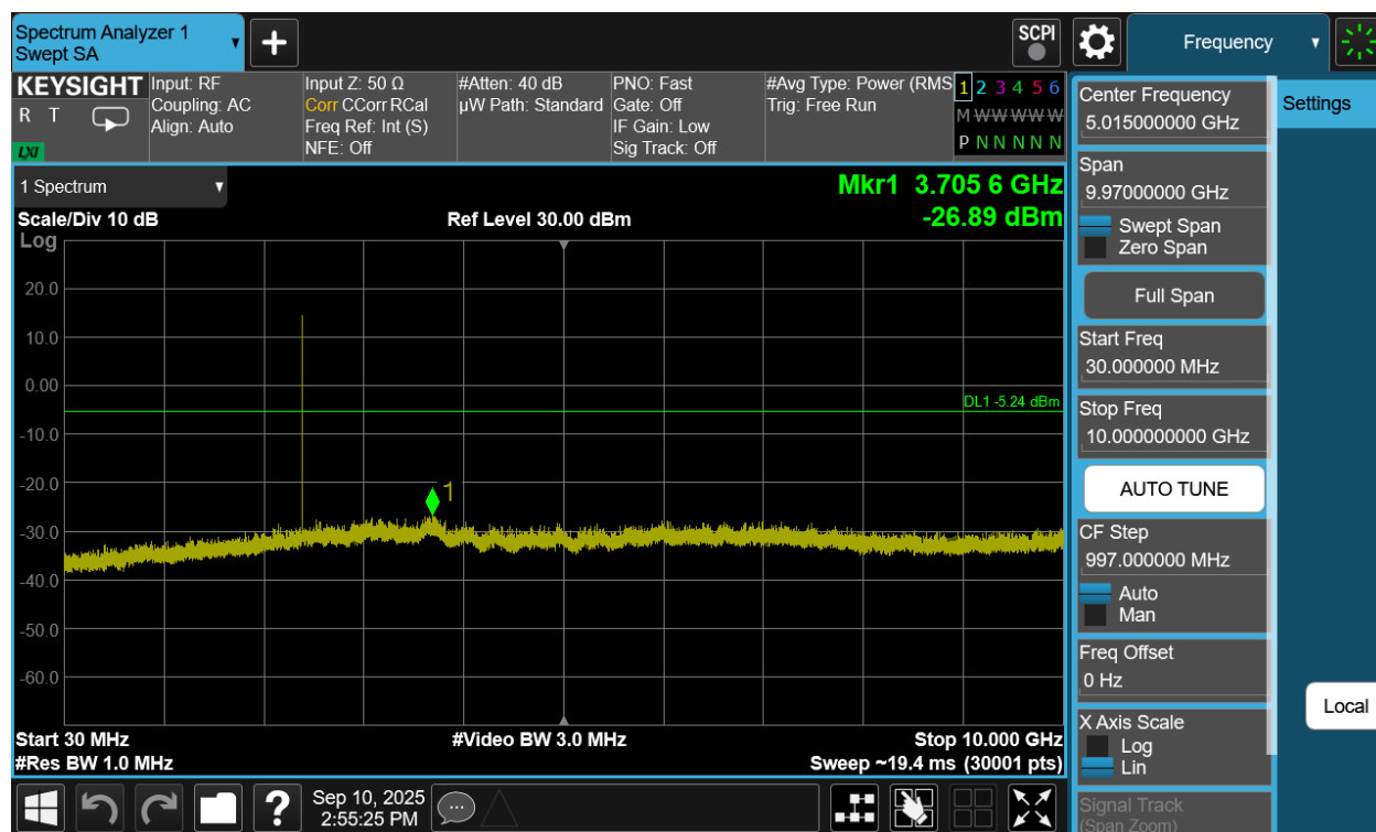
Plot 7-241. Conducted Spurious Plot Antenna WF8 (Bluetooth (HDR4), 4 Mbps, ePA – Ch. 1)
