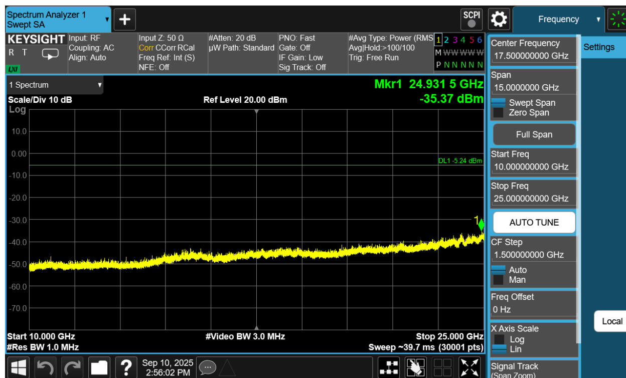
Plot 7-242. Conducted Spurious Plot Antenna WF8 (Bluetooth (HDR4), 4 Mbps, ePA – Ch. 1)
