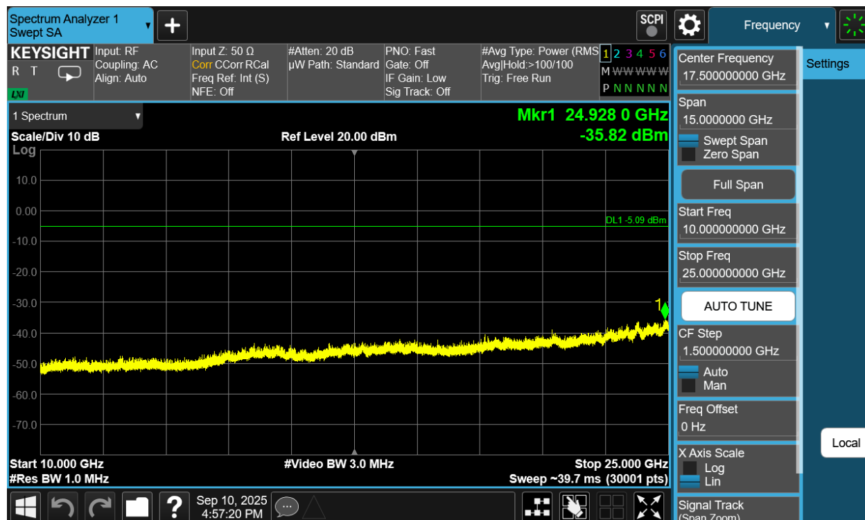
Plot 7-262. Conducted Spurious Plot Antenna WF8 (Bluetooth (HDRPM16), 16Mbps, ePA – Ch. 38)
