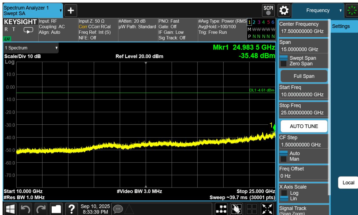
Plot 7-292. Conducted Spurious Plot Antenna WF7b (Bluetooth (HDRPM16), 16Mbps, ePA – Ch. 38)
