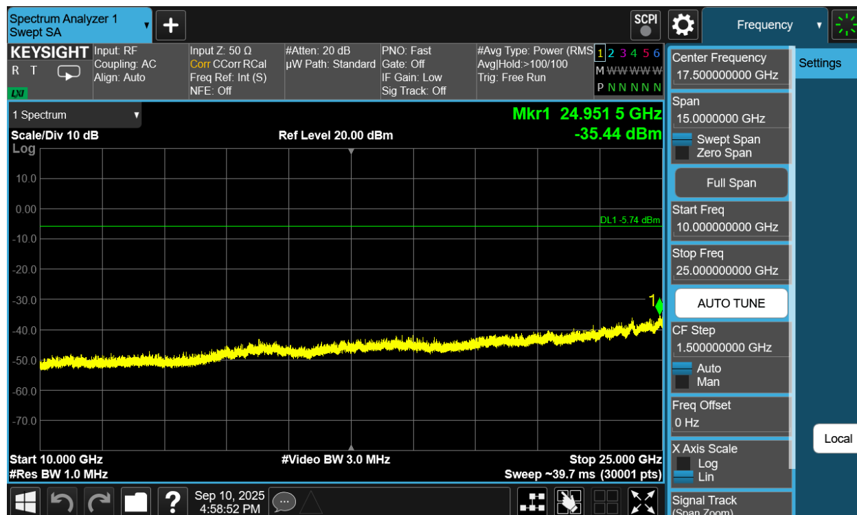
Plot 7-264. Conducted Spurious Plot Antenna WF8 (Bluetooth (HDRPM16), 16Mbps, ePA – Ch. 73)
