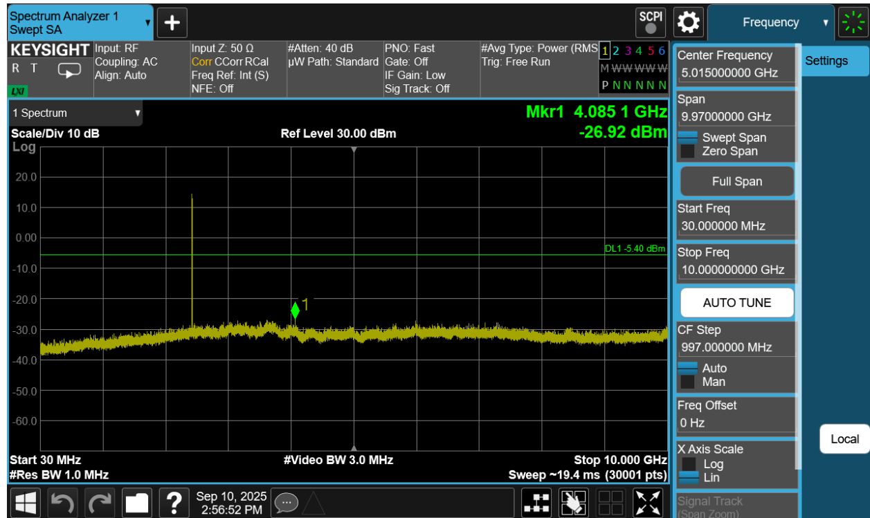
Plot 7-243. Conducted Spurious Plot Antenna WF8 (Bluetooth (HDR4), 4 Mbps, ePA – Ch. 38)
