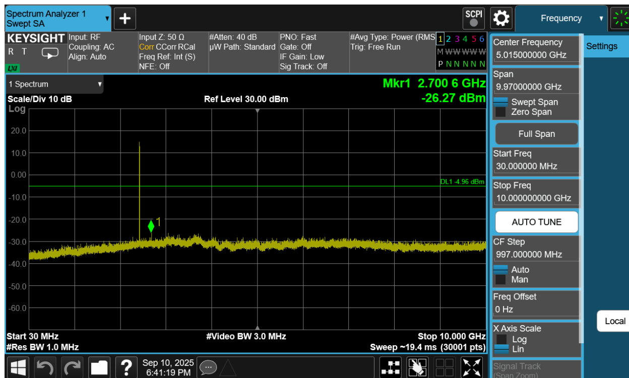
Plot 7-273. Conducted Spurious Plot Antenna WF7b (Bluetooth (HDR4), 4 Mbps, ePA – Ch. 38)
