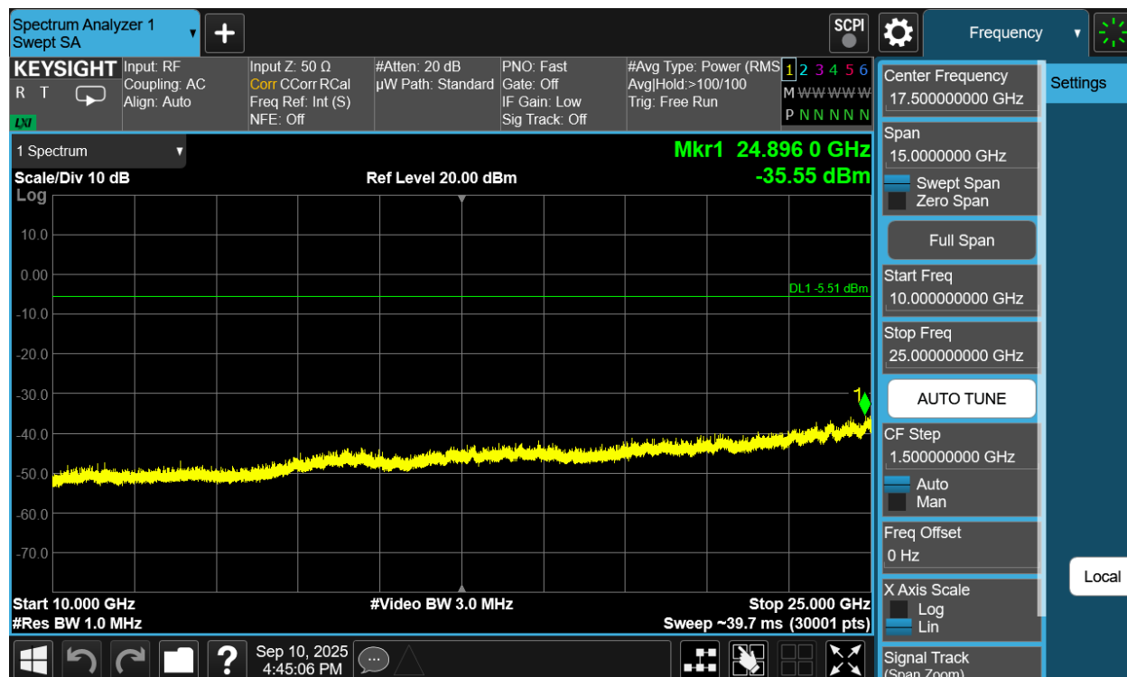
Plot 7-258. Conducted Spurious Plot Antenna WF8 (Bluetooth (XHDRPM6), 6Mbps, ePA – Ch. 73)
