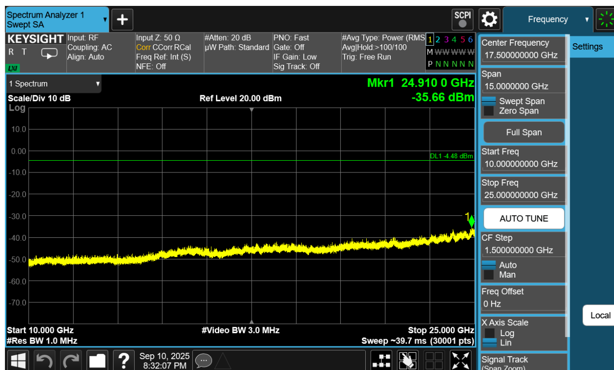
Plot 7-290. Conducted Spurious Plot Antenna WF7b (Bluetooth (HDRPM16), 16Mbps, ePA – Ch. 1)
