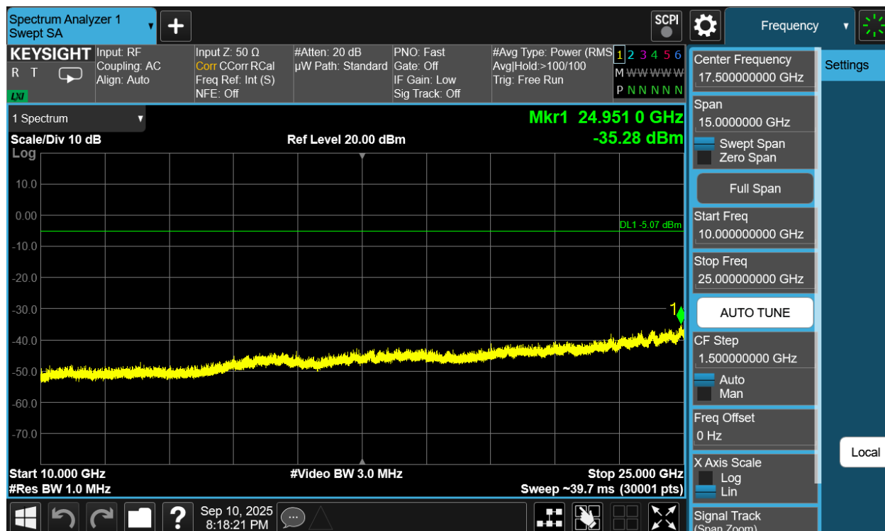
Plot 7-284. Conducted Spurious Plot Antenna WF7b (Bluetooth (XHDRPM6), 6Mbps, ePA – Ch. 1)
