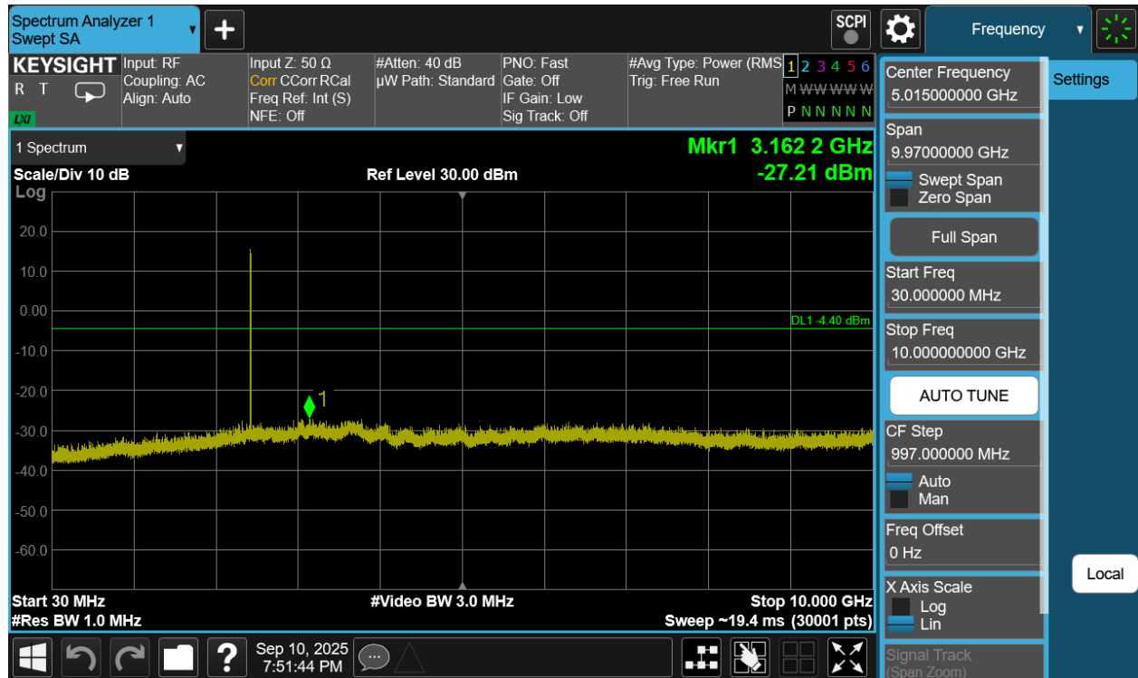
Plot 7-279. Conducted Spurious Plot Antenna WF7b (Bluetooth (HDRPS2), 8Mbps, ePA – Ch. 38)
