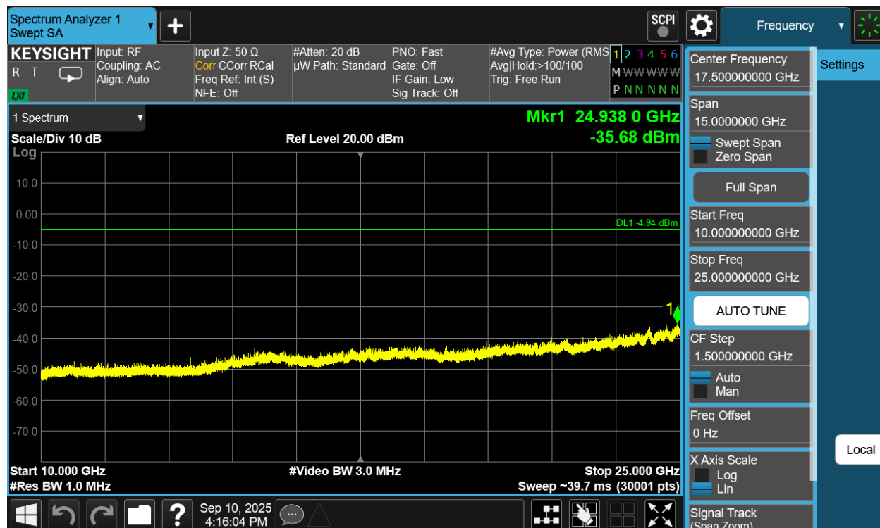
Plot 7-250. Conducted Spurious Plot Antenna WF8 (Bluetooth (HDRPS2), 8Mbps, ePA – Ch. 38)
