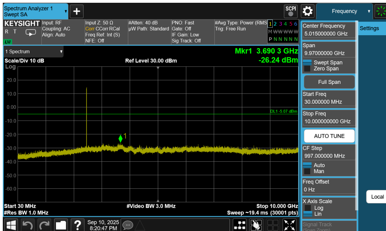
Plot 7-287. Conducted Spurious Plot Antenna WF7b (Bluetooth (XHDRPM6), 6Mbps, ePA – Ch. 73)
