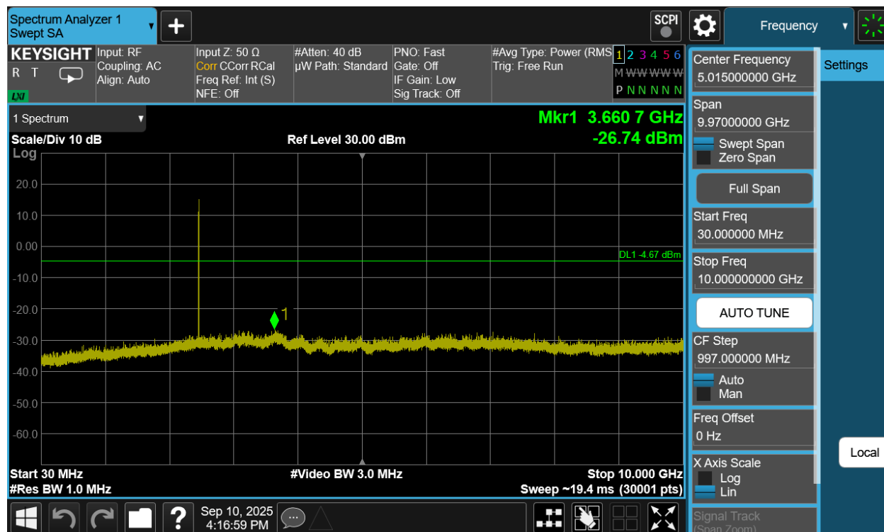
Plot 7-251. Conducted Spurious Plot Antenna WF8 (Bluetooth (HDRPS2), 8Mbps, ePA – Ch. 73)
