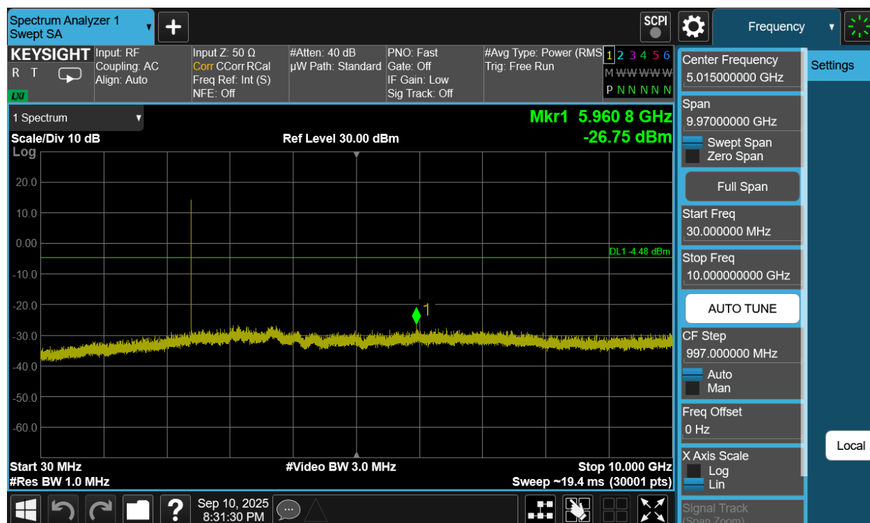
Plot 7-289. Conducted Spurious Plot Antenna WF7b (Bluetooth (HDRPM16), 16Mbps, ePA – Ch. 1)
