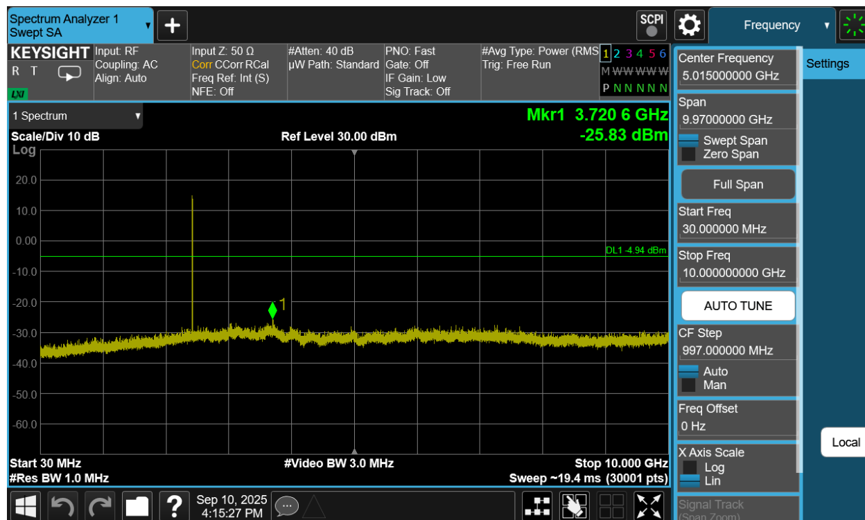
Plot 7-249. Conducted Spurious Plot Antenna WF8 (Bluetooth (HDRPS2), 8Mbps, ePA – Ch. 38)
