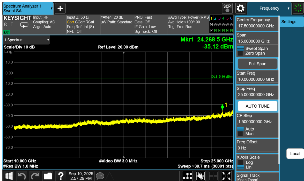
Plot 7-244. Conducted Spurious Plot Antenna WF8 (Bluetooth (HDR4), 4 Mbps, ePA – Ch. 38)
