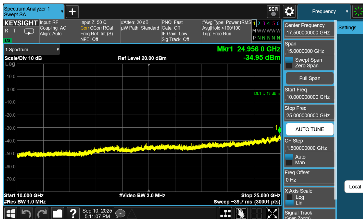
Plot 7-268. Conducted Spurious Plot Antenna WF8 (Bluetooth (HDT2), 2Mbps, ePA – Ch. 37)
