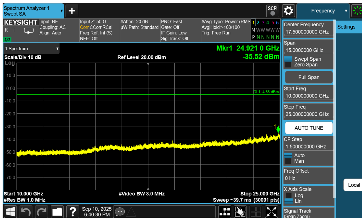
Plot 7-272. Conducted Spurious Plot Antenna WF7b (Bluetooth (HDR4), 4 Mbps, ePA – Ch. 1)
