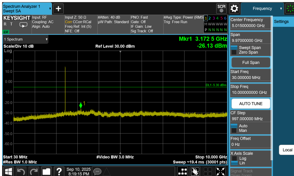
Plot 7-285. Conducted Spurious Plot Antenna WF7b (Bluetooth (XHDRPM6), 6Mbps, ePA – Ch. 38)
