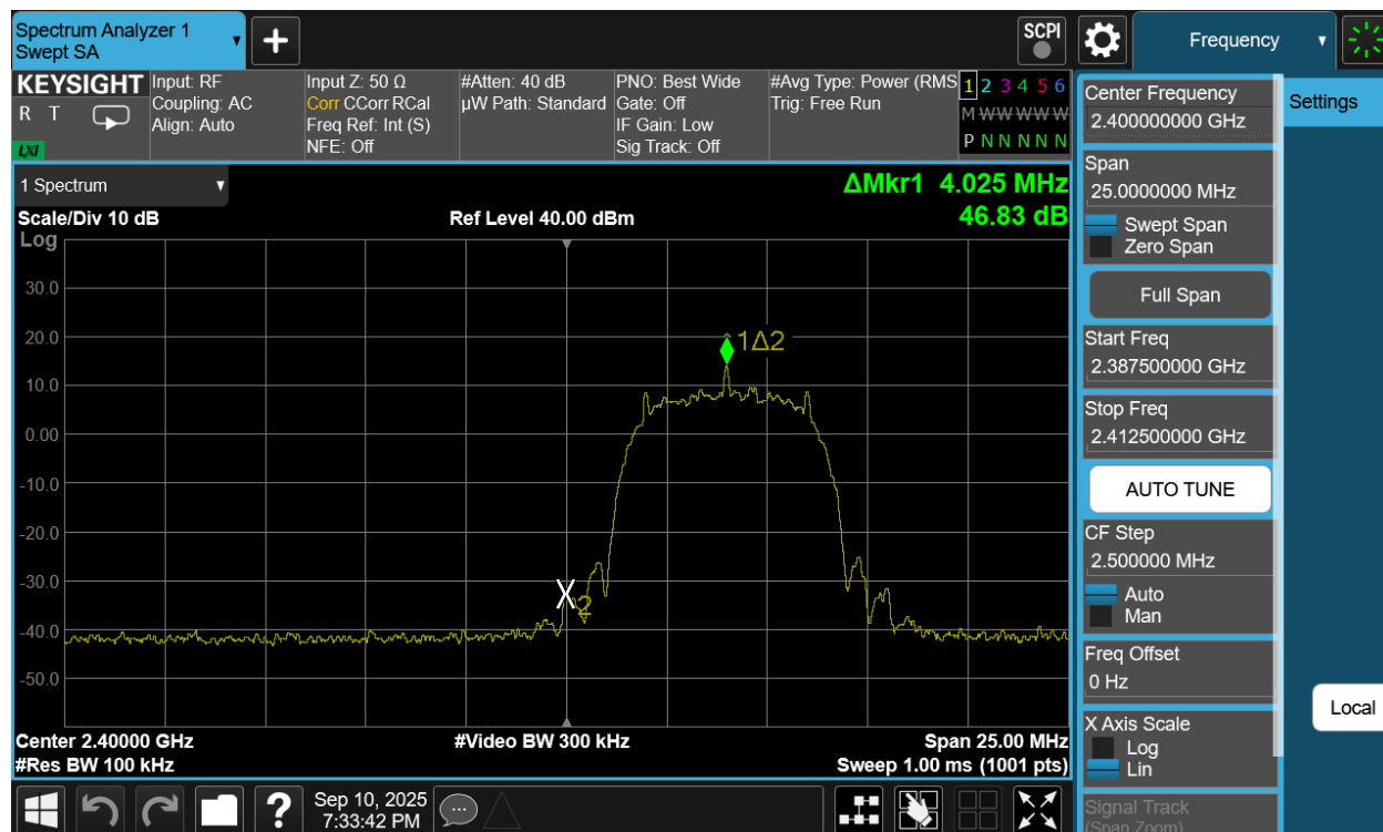
Plot 7-235. Band Edge Plot Antenna WF7b (Bluetooth (XHDRPM6), 6Mbps, ePA – Ch. 1)
