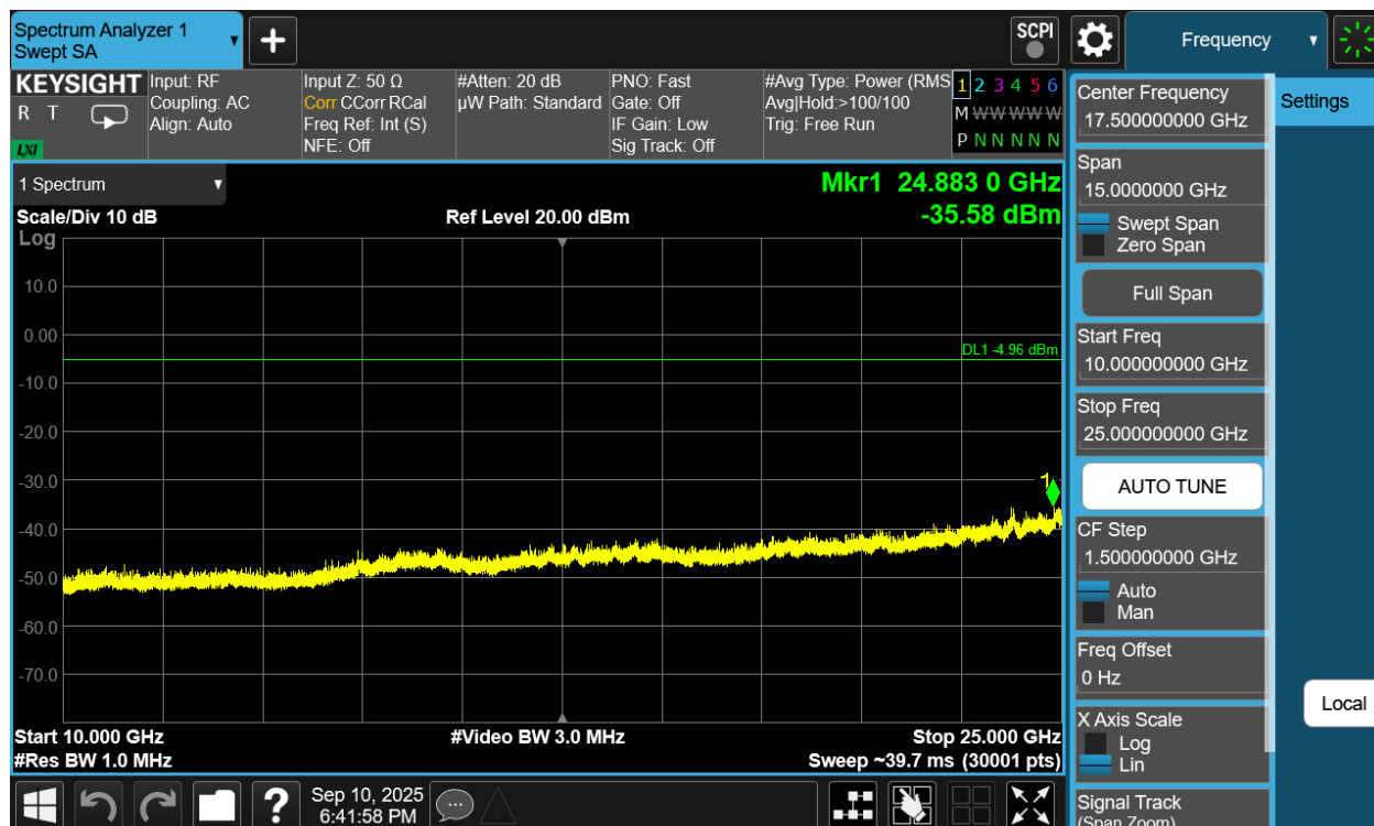
Plot 7-274. Conducted Spurious Plot Antenna WF7b (Bluetooth (HDR4), 4 Mbps, ePA – Ch. 38)
