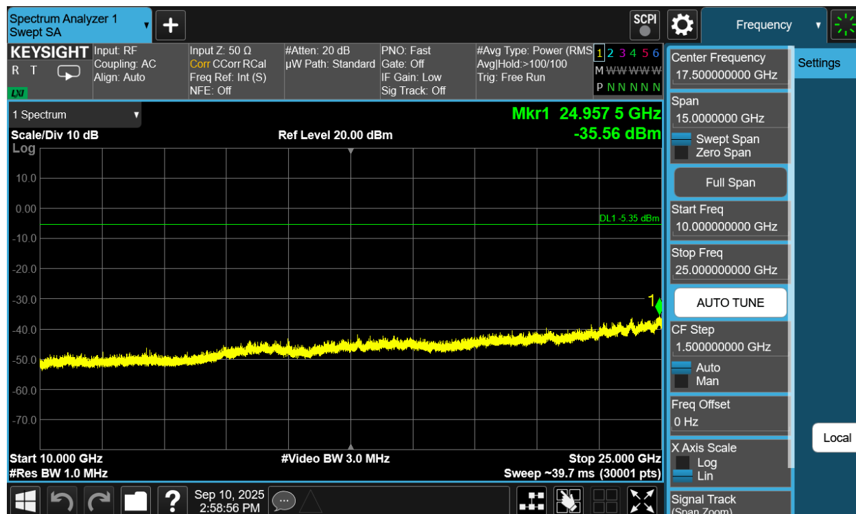
Plot 7-246. Conducted Spurious Plot Antenna WF8 (Bluetooth (HDR4), 4 Mbps, ePA – Ch. 73)
