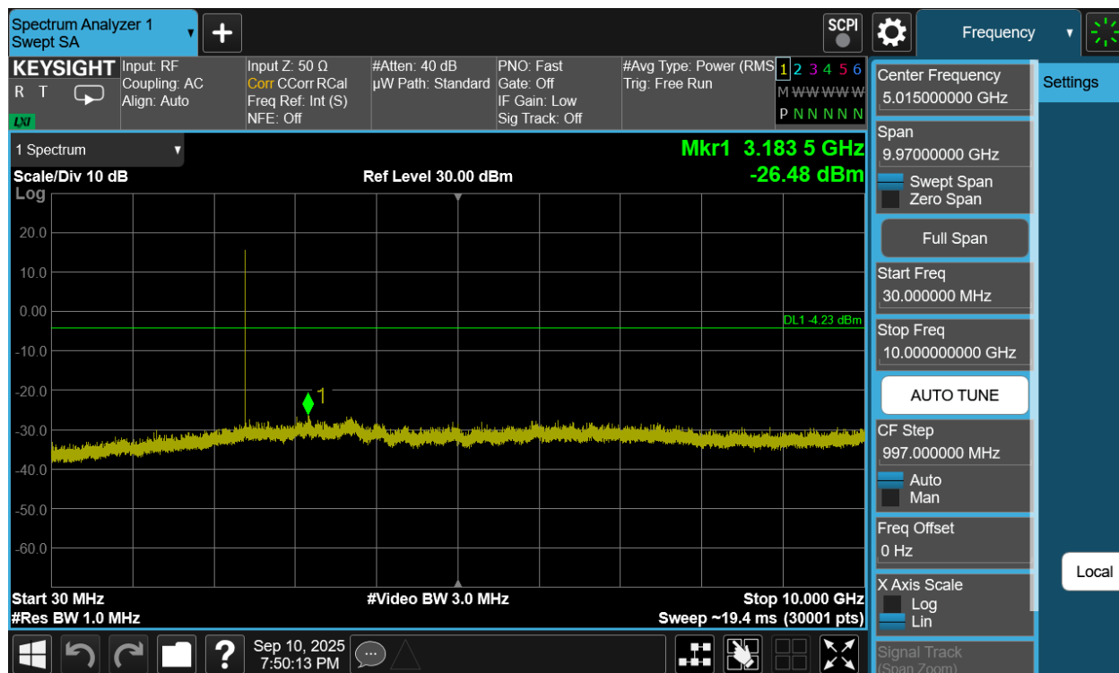
Plot 7-277. Conducted Spurious Plot Antenna WF7b (Bluetooth (HDRPS2), 8Mbps, ePA – Ch. 1)
