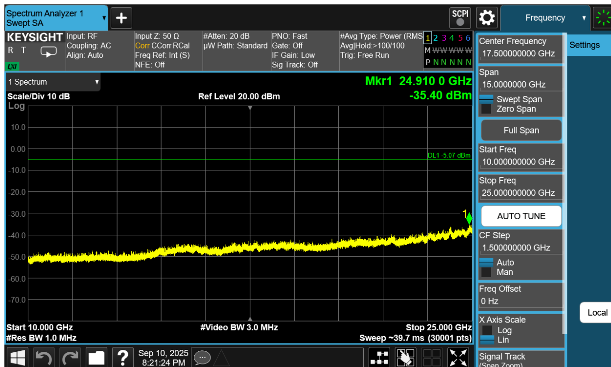
Plot 7-288. Conducted Spurious Plot Antenna WF7b (Bluetooth (XHDRPM6), 6Mbps, ePA – Ch. 73)
