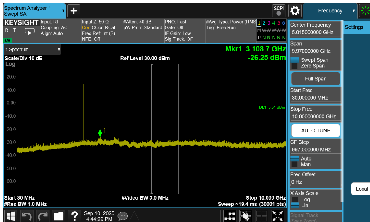
Plot 7-257. Conducted Spurious Plot Antenna WF8 (Bluetooth (XHDRPM6), 6Mbps, ePA – Ch. 73)
