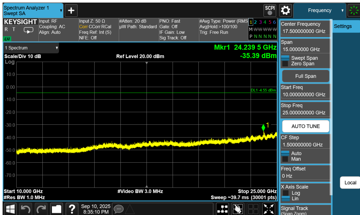
Plot 7-294. Conducted Spurious Plot Antenna WF7b (Bluetooth (HDRPM16), 16Mbps, ePA – Ch. 73)
