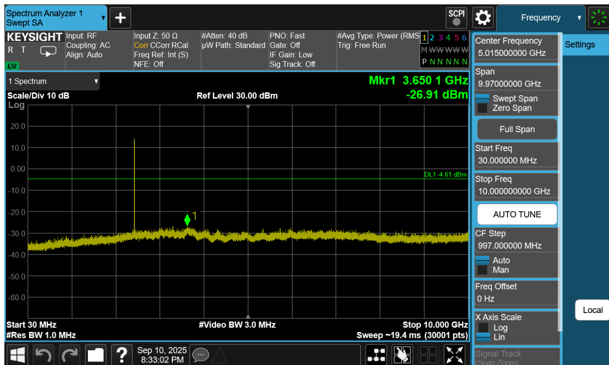
Plot 7-291. Conducted Spurious Plot Antenna WF7b (Bluetooth (HDRPM16), 16Mbps, ePA – Ch. 38)
