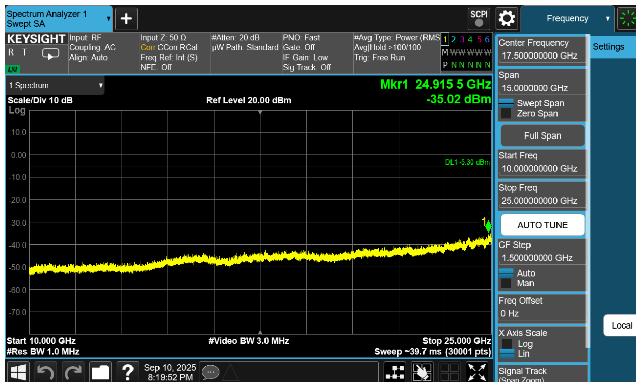
Plot 7-286. Conducted Spurious Plot Antenna WF7b (Bluetooth (XHDRPM6), 6Mbps, ePA – Ch. 38)
