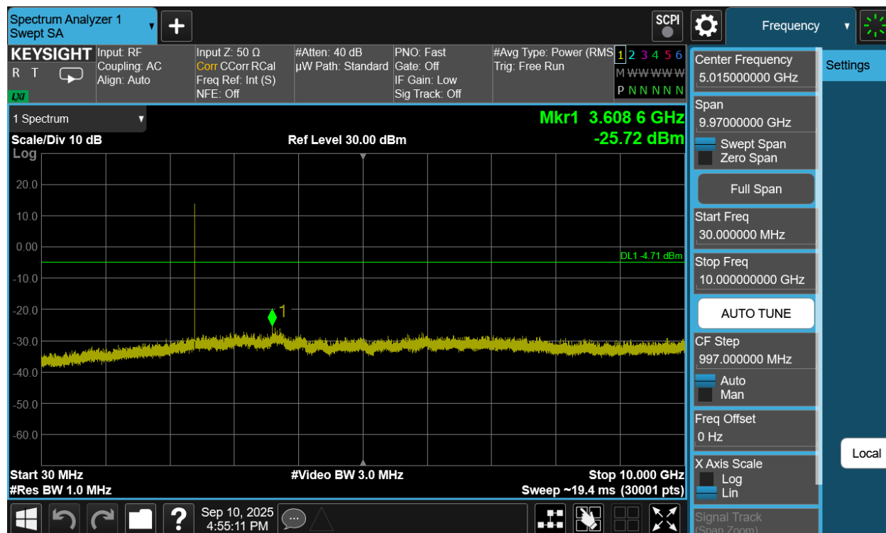
Plot 7-259. Conducted Spurious Plot Antenna WF8 (Bluetooth (HDRPM16), 16Mbps, ePA – Ch. 1)
