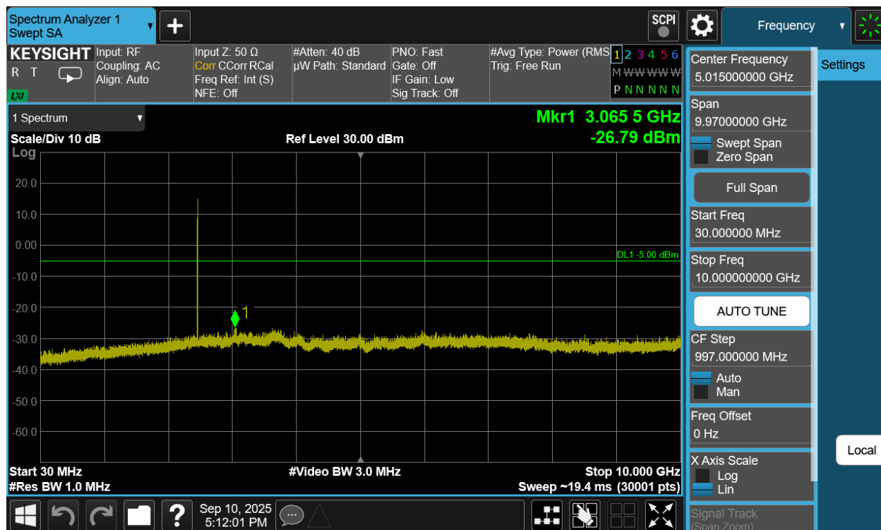
Plot 7-269. Conducted Spurious Plot Antenna WF8 (Bluetooth (HDT2), 2Mbps, ePA – Ch. 73)
