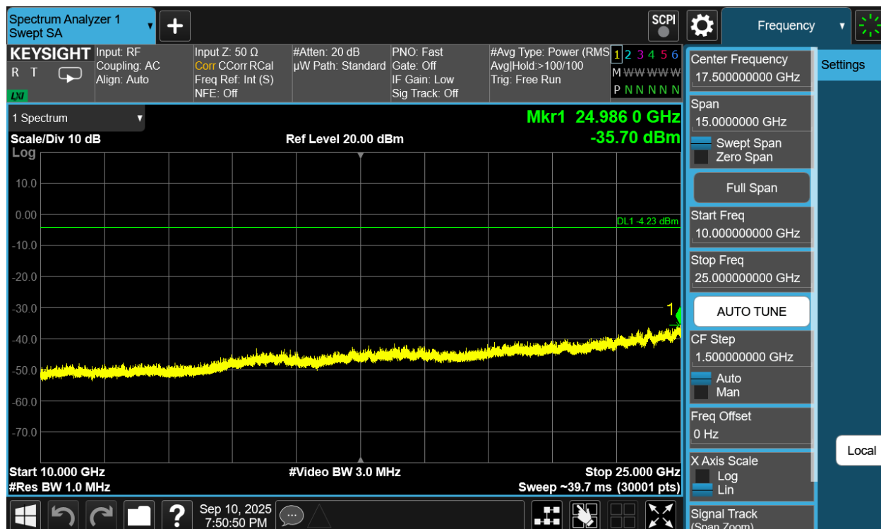
Plot 7-278. Conducted Spurious Plot Antenna WF7b (Bluetooth (HDRPS2), 8Mbps, ePA – Ch. 1)
