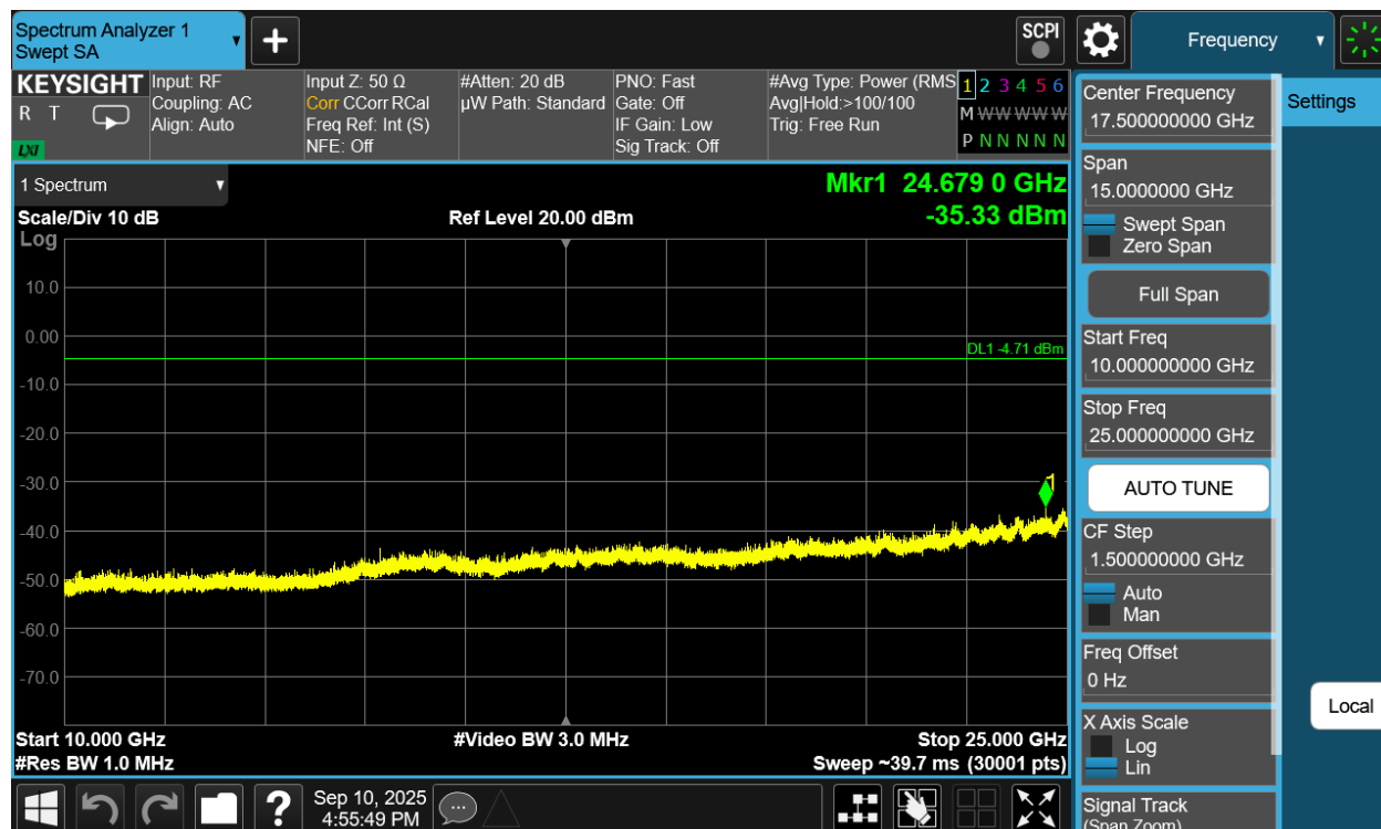
Plot 7-260. Conducted Spurious Plot Antenna WF8 (Bluetooth (HDRPM16), 16Mbps, ePA – Ch. 1)
