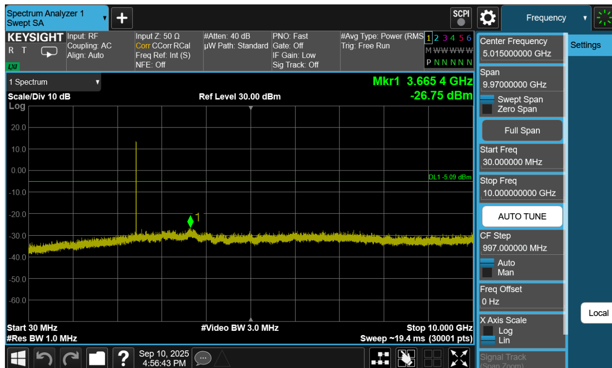
Plot 7-261. Conducted Spurious Plot Antenna WF8 (Bluetooth (HDRPM16), 16Mbps, ePA – Ch. 38)
