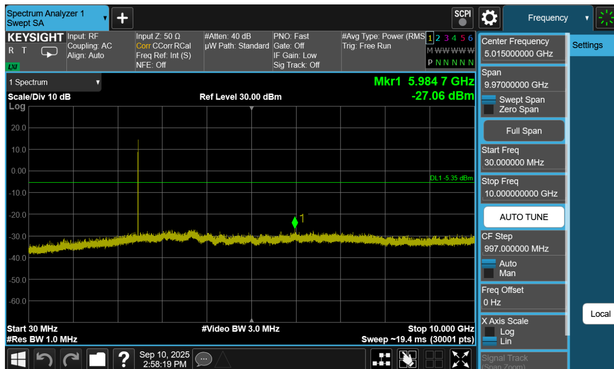
Plot 7-245. Conducted Spurious Plot Antenna WF8 (Bluetooth (HDR4), 4 Mbps, ePA – Ch. 73)
