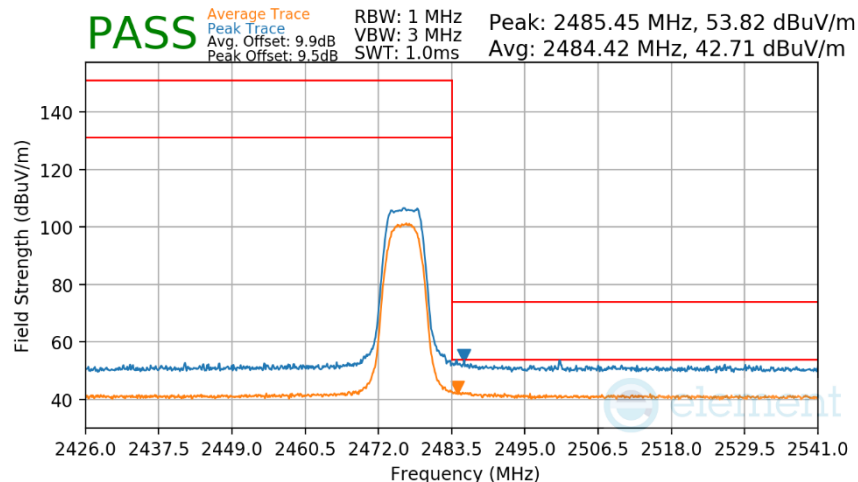
Plot 7-326. Radiated Restricted Upper Band Edge Measurement Antenna WF7b
