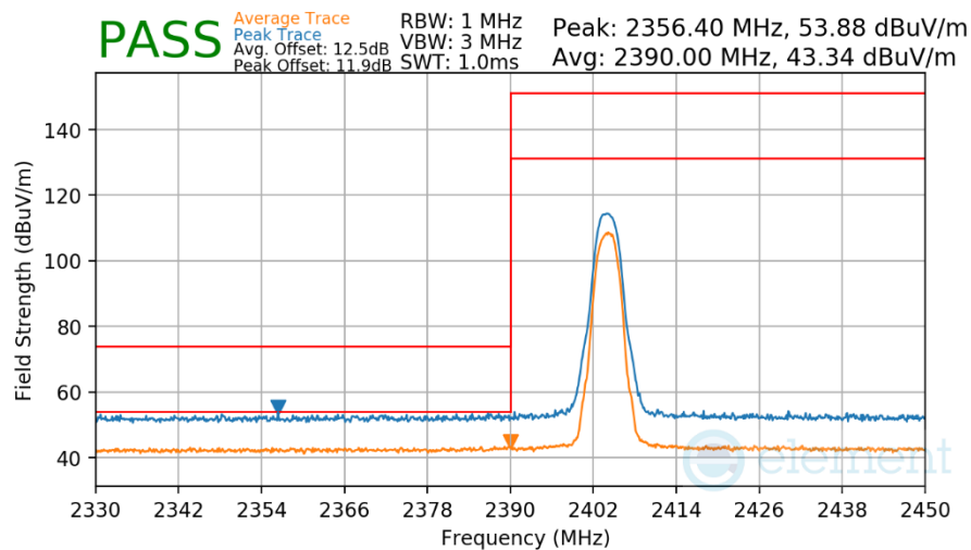
Plot 7-310. Radiated Restricted Lower Band Edge Measurement Antenna WF8
