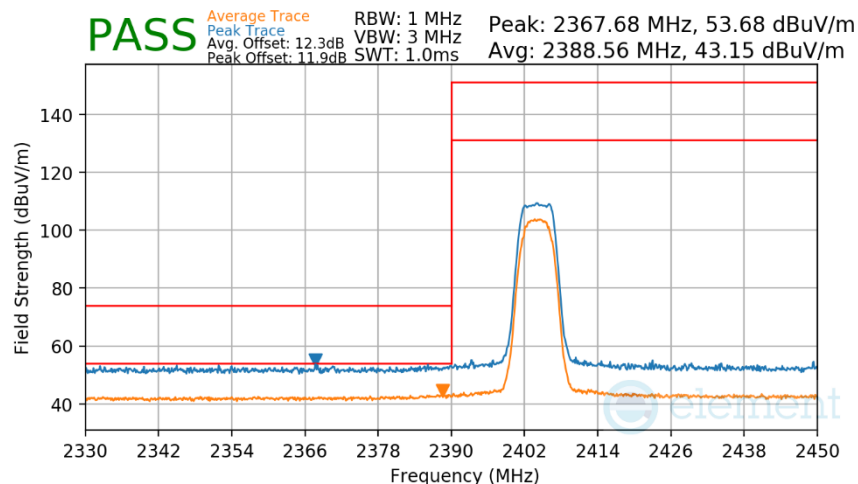
Plot 7-320. Radiated Restricted Lower Band Edge Measurement Antenna WF7b
