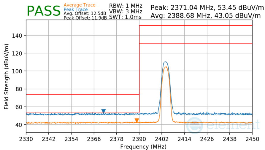
Plot 7-322. Radiated Restricted Lower Band Edge Measurement Antenna WF7b
