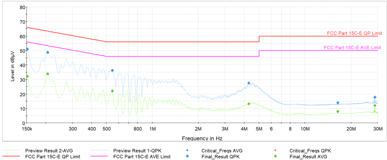
Plot 7-343. AC Line Conducted Plot with Bluetooth HDR Tx BF (N, HDR4 ePA - Ch.38 with AC/DC Adapter)
