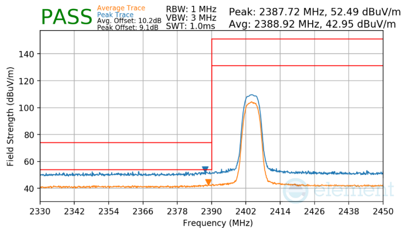
Plot 7-318. Radiated Restricted Lower Band Edge Measurement Antenna WF7b
