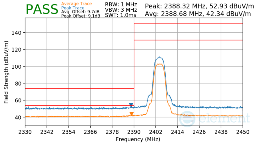
Plot 7-309. Radiated Restricted Lower Band Edge Measurement Antenna WF8
