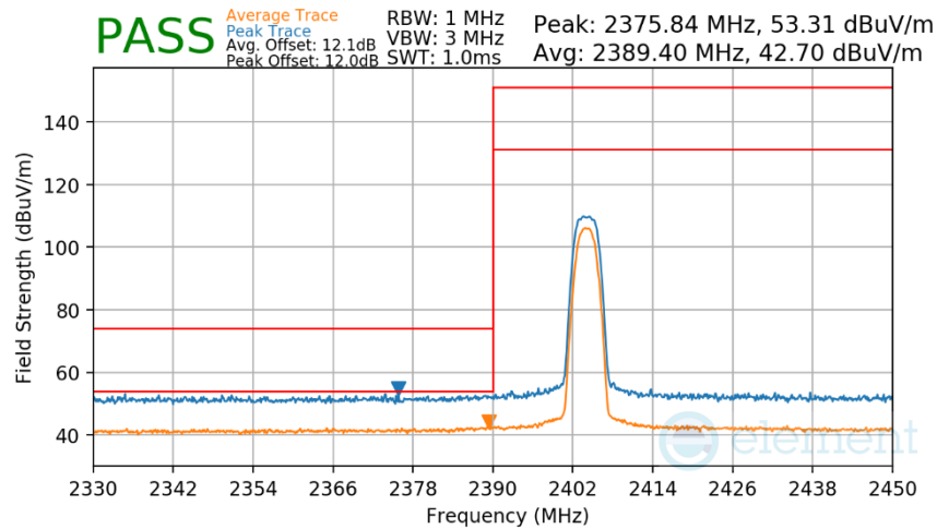
Plot 7-319. Radiated Restricted Lower Band Edge Measurement Antenna WF7b
