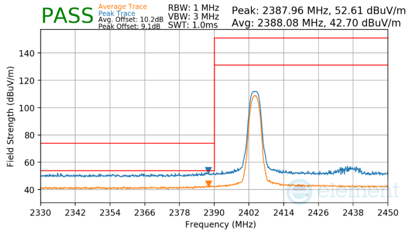
Plot 7-305. Radiated Restricted Lower Band Edge Measurement Antenna WF8
