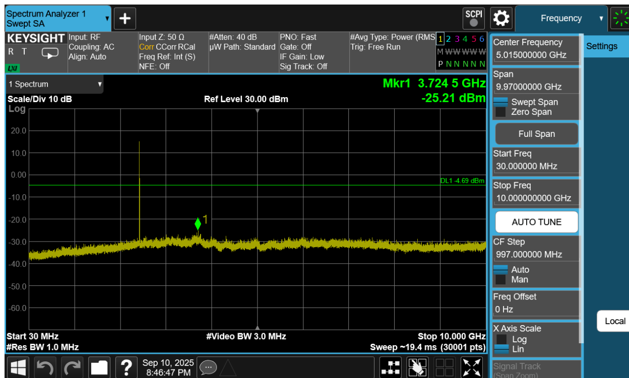
Plot 7-297. Conducted Spurious Plot Antenna WF7b (Bluetooth (HDT2), 2Mbps, ePA – Ch. 37)
