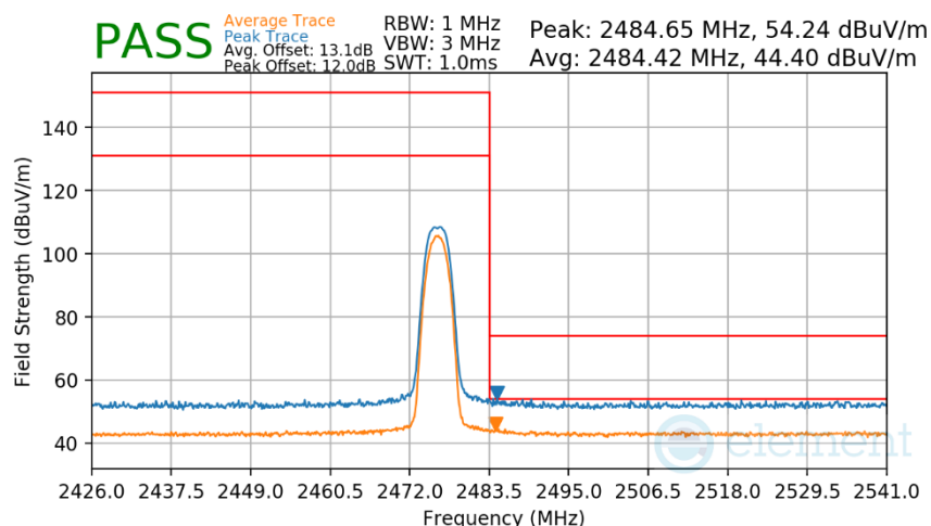
Plot 7-323. Radiated Restricted Upper Band Edge Measurement Antenna WF7b
