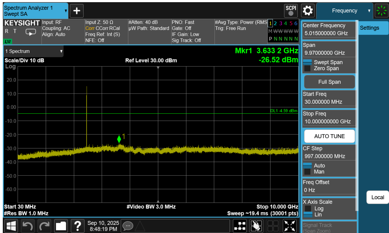
Plot 7-299. Conducted Spurious Plot Antenna WF7b (Bluetooth (HDT2), 2Mbps, ePA – Ch. 73)
