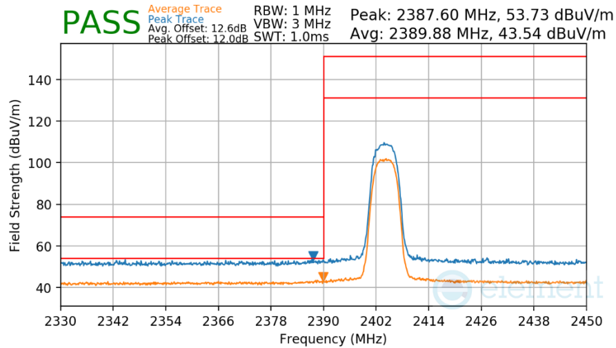
Plot 7-321. Radiated Restricted Lower Band Edge Measurement Antenna WF7b
