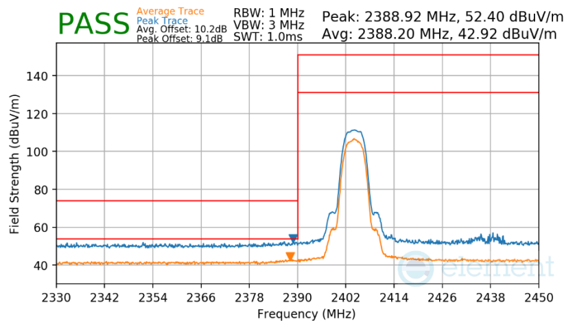
Plot 7-306. Radiated Restricted Lower Band Edge Measurement Antenna WF8
