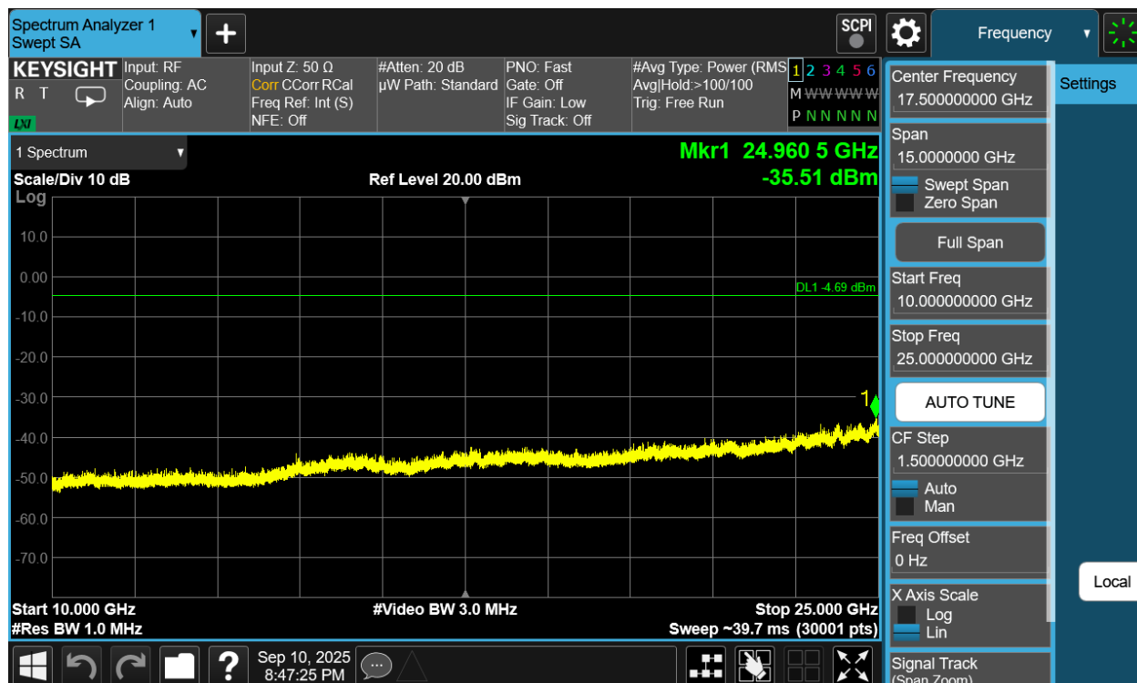
Plot 7-298. Conducted Spurious Plot Antenna WF7b (Bluetooth (HDT2), 2Mbps, ePA – Ch. 37)
