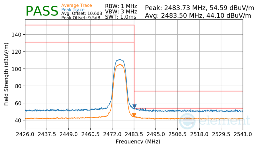
Plot 7-312. Radiated Restricted Upper Band Edge Measurement Antenna WF8
