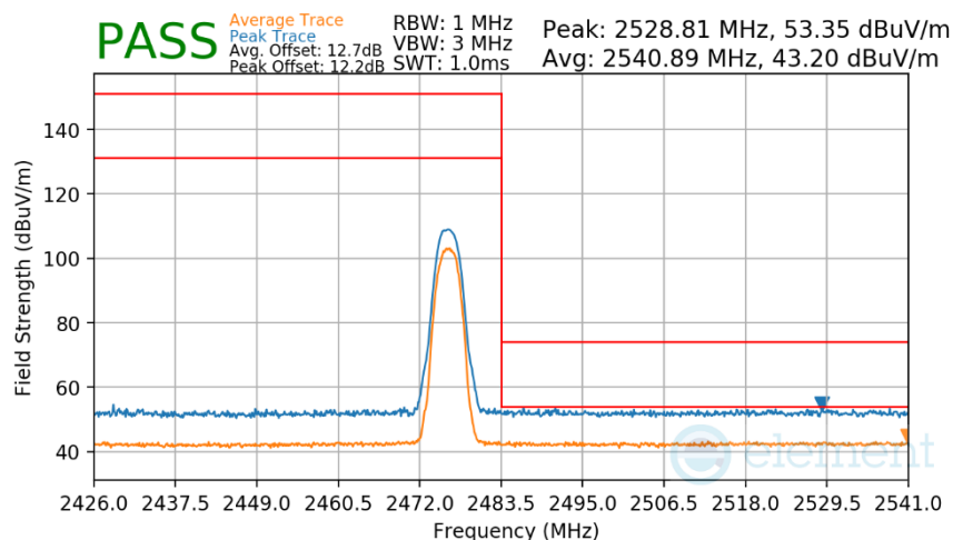
Plot 7-328. Radiated Restricted Upper Band Edge Measurement Antenna WF7b
