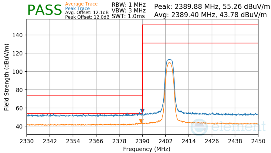
Plot 7-307. Radiated Restricted Lower Band Edge Measurement Antenna WF8
