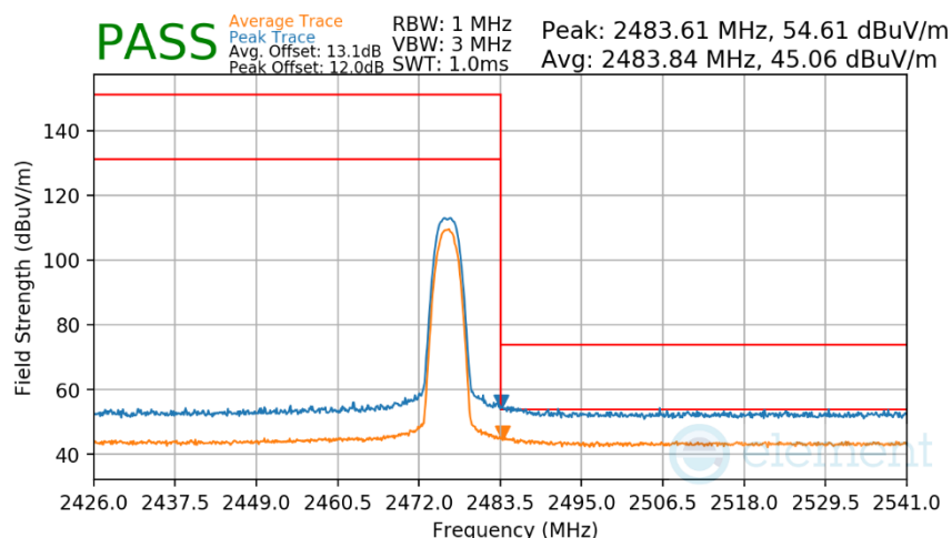
Plot 7-311. Radiated Restricted Upper Band Edge Measurement Antenna WF8
