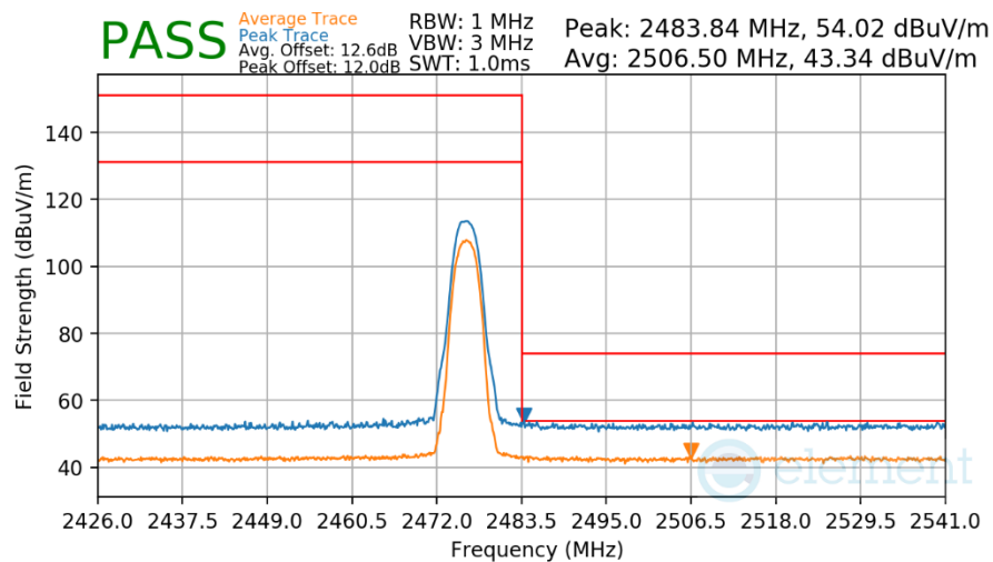
Plot 7-316. Radiated Restricted Upper Band Edge Measurement Antenna WF8
