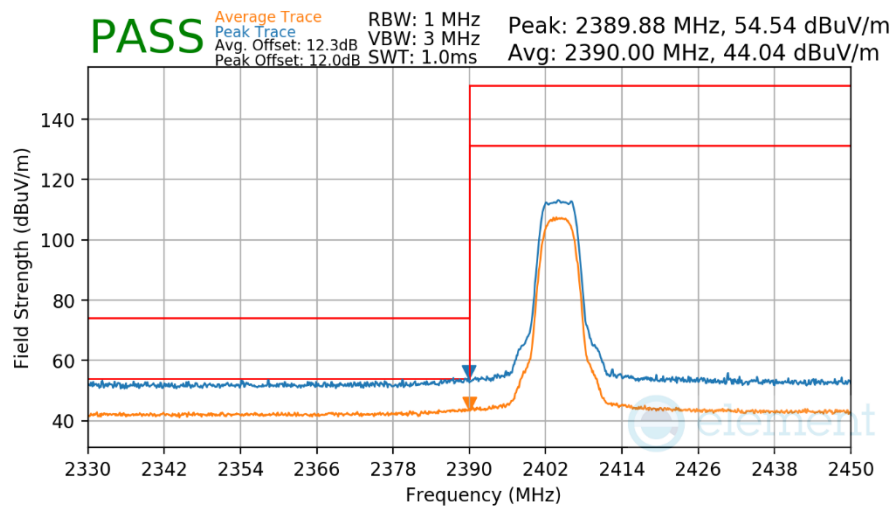
Plot 7-308. Radiated Restricted Lower Band Edge Measurement Antenna WF8
