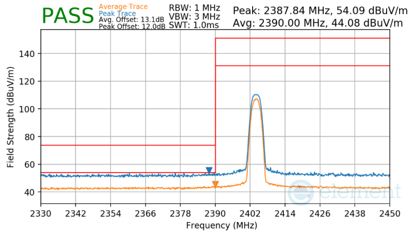
Plot 7-317. Radiated Restricted Lower Band Edge Measurement Antenna WF7b
