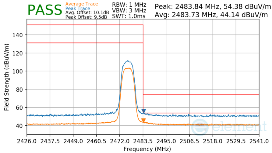
Plot 7-315. Radiated Restricted Upper Band Edge Measurement Antenna WF8
