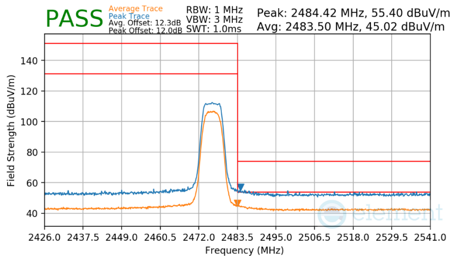
Plot 7-314. Radiated Restricted Upper Band Edge Measurement Antenna WF8
