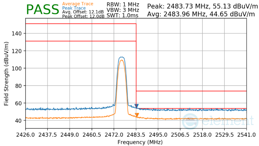
Plot 7-313. Radiated Restricted Upper Band Edge Measurement Antenna WF8
