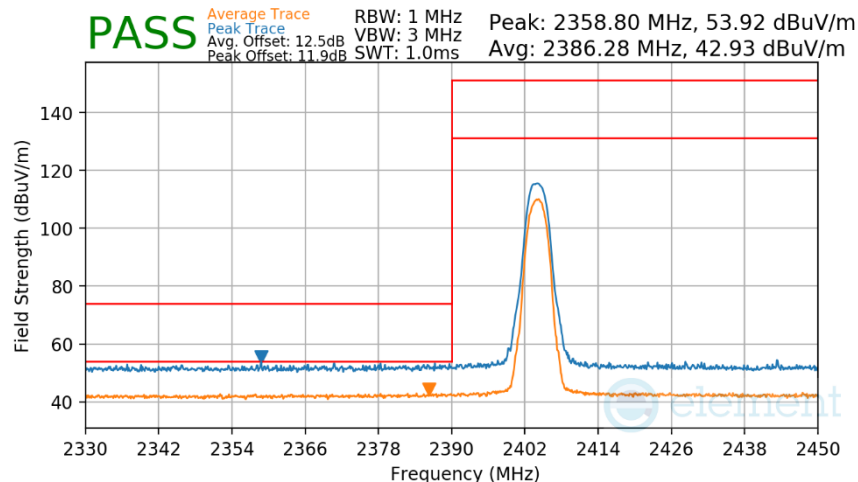
Plot 7-334. Radiated Restricted Lower Band Edge Measurement TxBF
