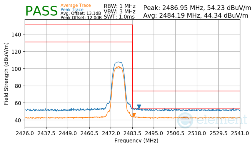
Plot 7-324. Radiated Restricted Upper Band Edge Measurement Antenna WF7b
