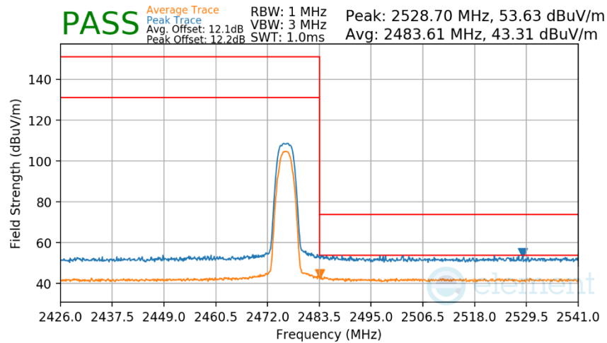
Plot 7-325. Radiated Restricted Upper Band Edge Measurement Antenna WF7b
