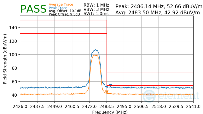
Plot 7-327. Radiated Restricted Upper Band Edge Measurement Antenna WF7b
