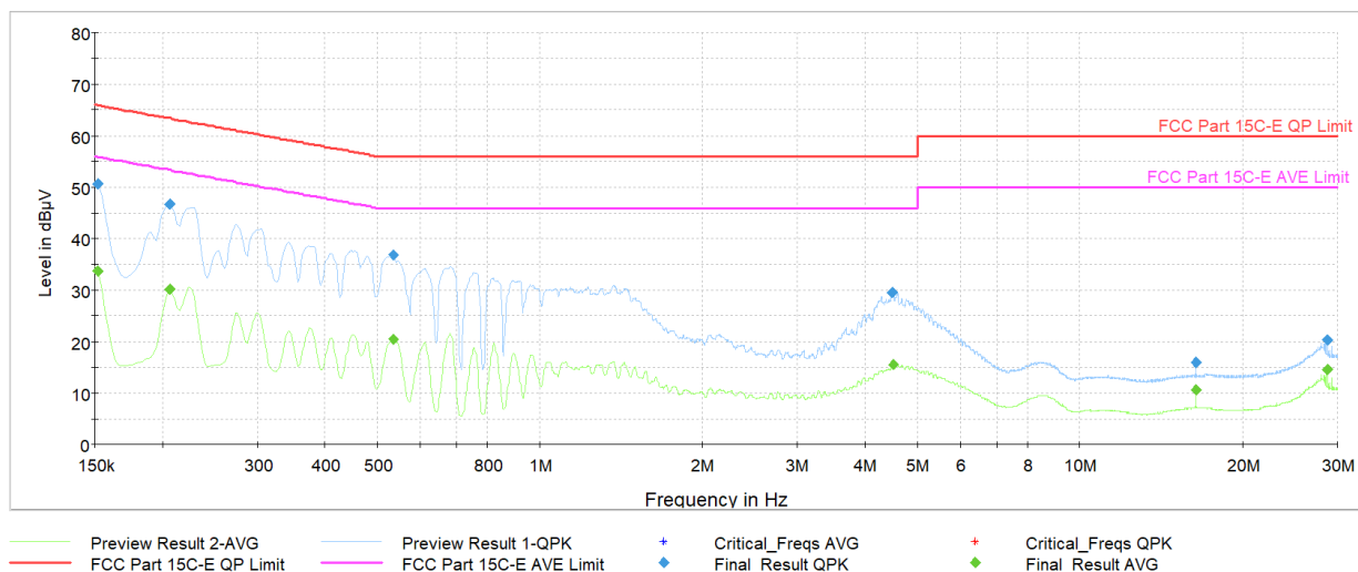
Plot 7-342. AC Line Conducted Plot with Bluetooth HDR TxBF (L1, HDR4 ePA - Ch.38 with AC/DC Adapter)
