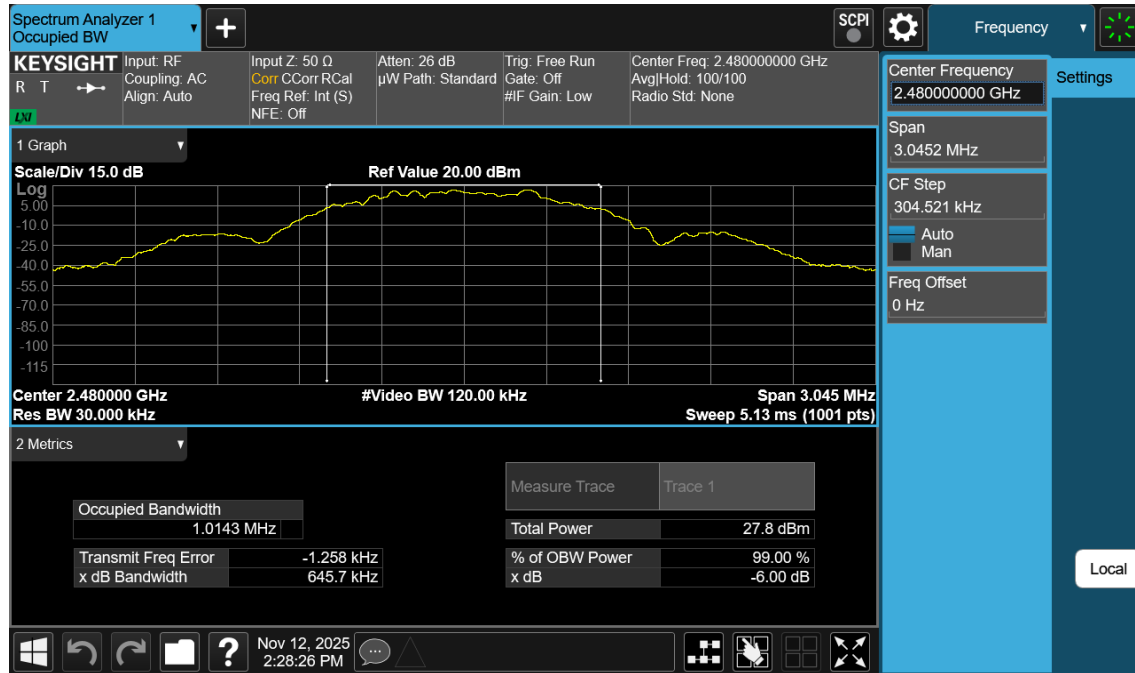
Plot 7-21. 99% OBW Plot Antenna WF7b (Bluetooth (LE), 1Mbps, ePA – Ch. 39)
