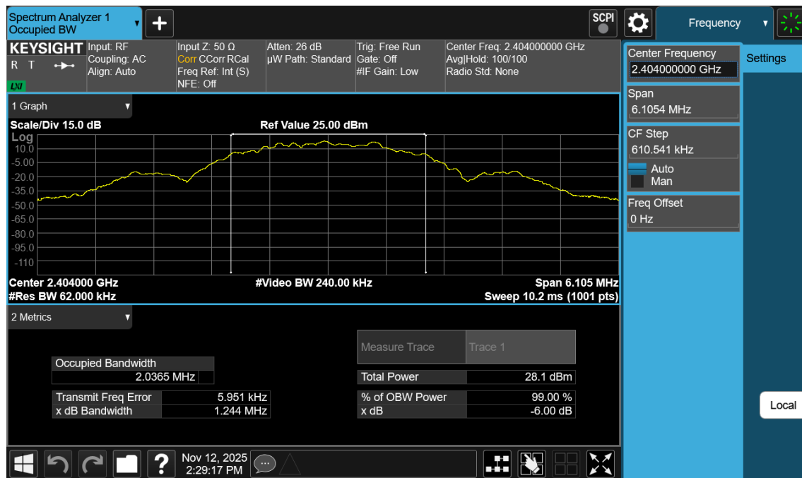
Plot 7-22. 99% OBW Plot Antenna WF7b (Bluetooth (LE), 2Mbps, ePA – Ch. 1)
