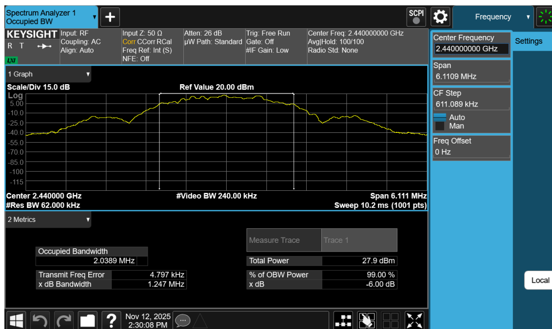
Plot 7-23. 99% OBW Plot Antenna WF7b (Bluetooth (LE), 2Mbps, ePA – Ch. 19)
