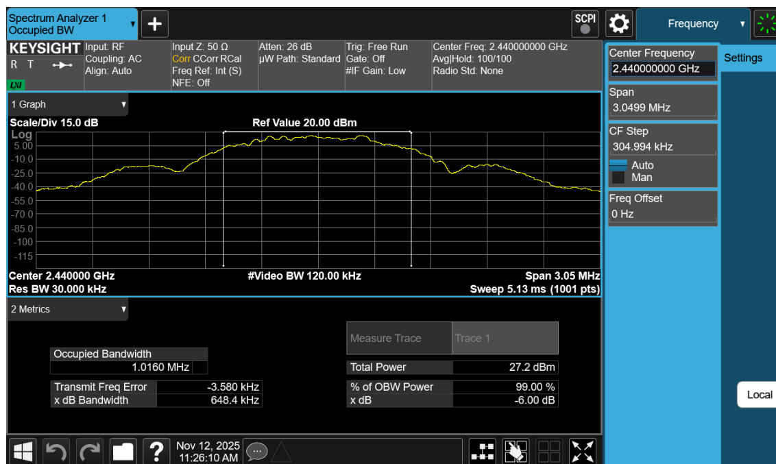
Plot 7-8. 99% OBW Plot Antenna WF8 (Bluetooth (LE), 1Mbps, ePA – Ch. 19)
