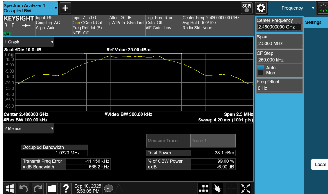
Plot 7-45. 6dB BW Plot Antenna WF7b (Bluetooth (LE), 1Mbps, ePA – Ch. 39)
