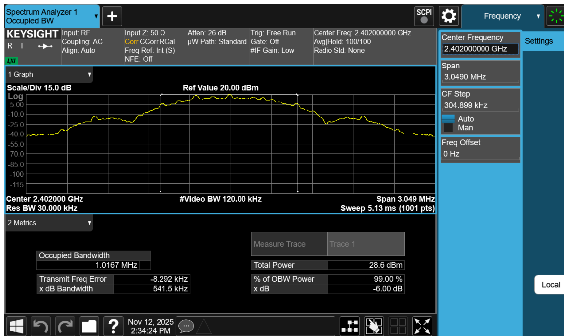
Plot 7-16. 99% OBW Plot Antenna WF7b (Bluetooth (LE), 500kbps, ePA – Ch. 0)
