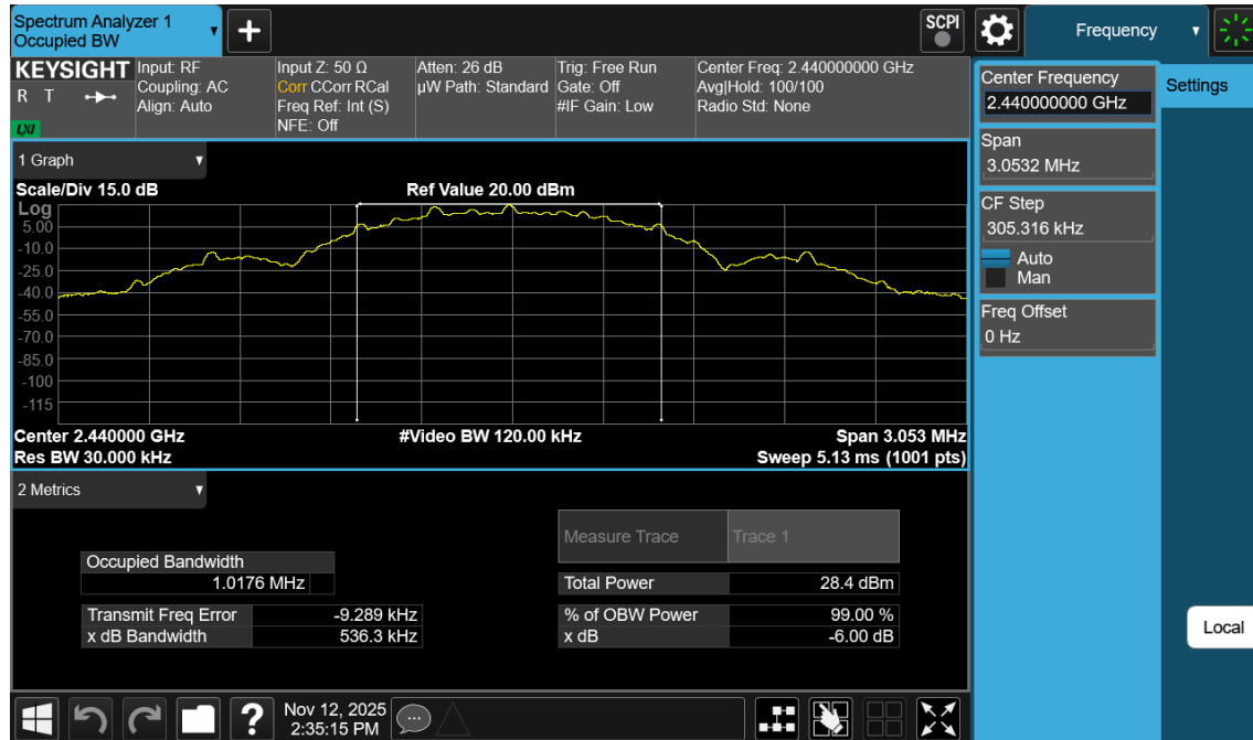
Plot 7-17.99% OBW Plot Antenna WF7b (Bluetooth (LE), 500kbps, ePA – Ch. 19)
