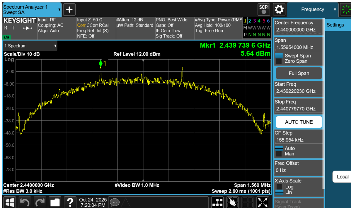
Plot 7-56. Power Spectral Density Plot Antenna WF8 (Bluetooth (LE), 500kbps, ePA – Ch. 19)
