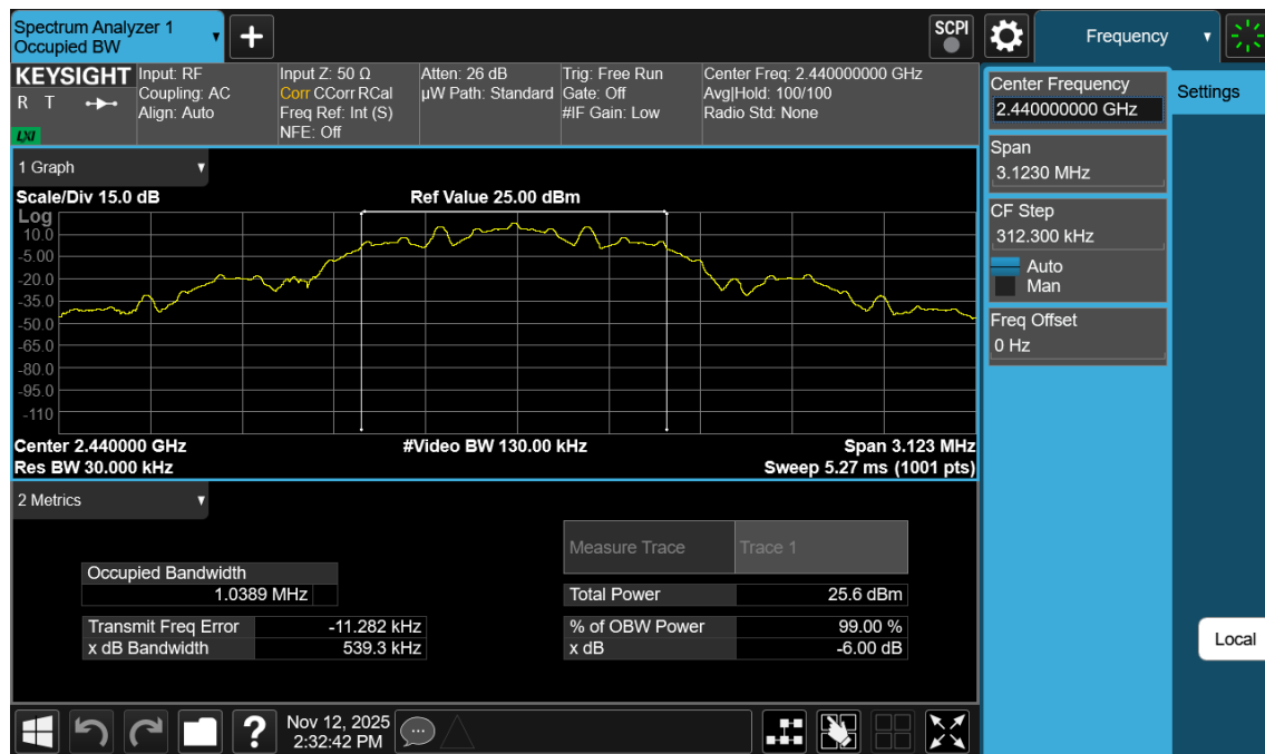
Plot 7-14.99% OBW Plot Antenna WF7b (Bluetooth (LE), 125kbps, ePA – Ch. 19)
