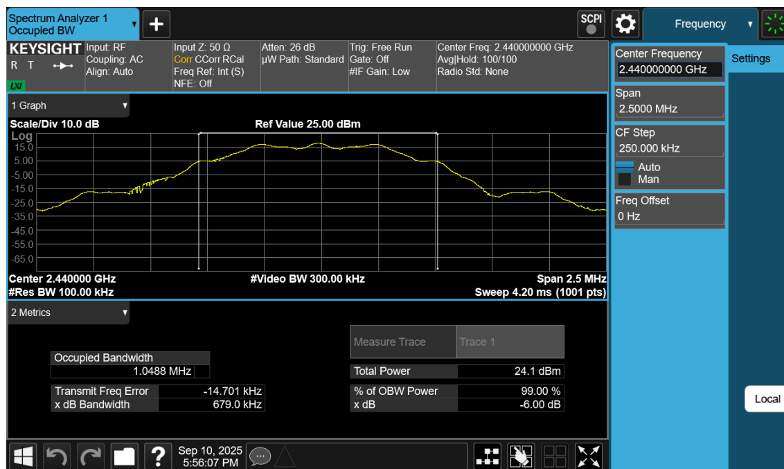
Plot 7-38. 6dB BW Plot Antenna WF7b (Bluetooth (LE), 125kbps, ePA – Ch. 19)
