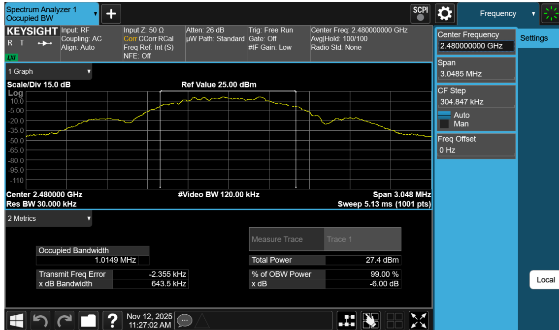
Plot 7-9. 99% OBW Plot Antenna WF8 (Bluetooth (LE), 1Mbps, ePA – Ch. 39)
