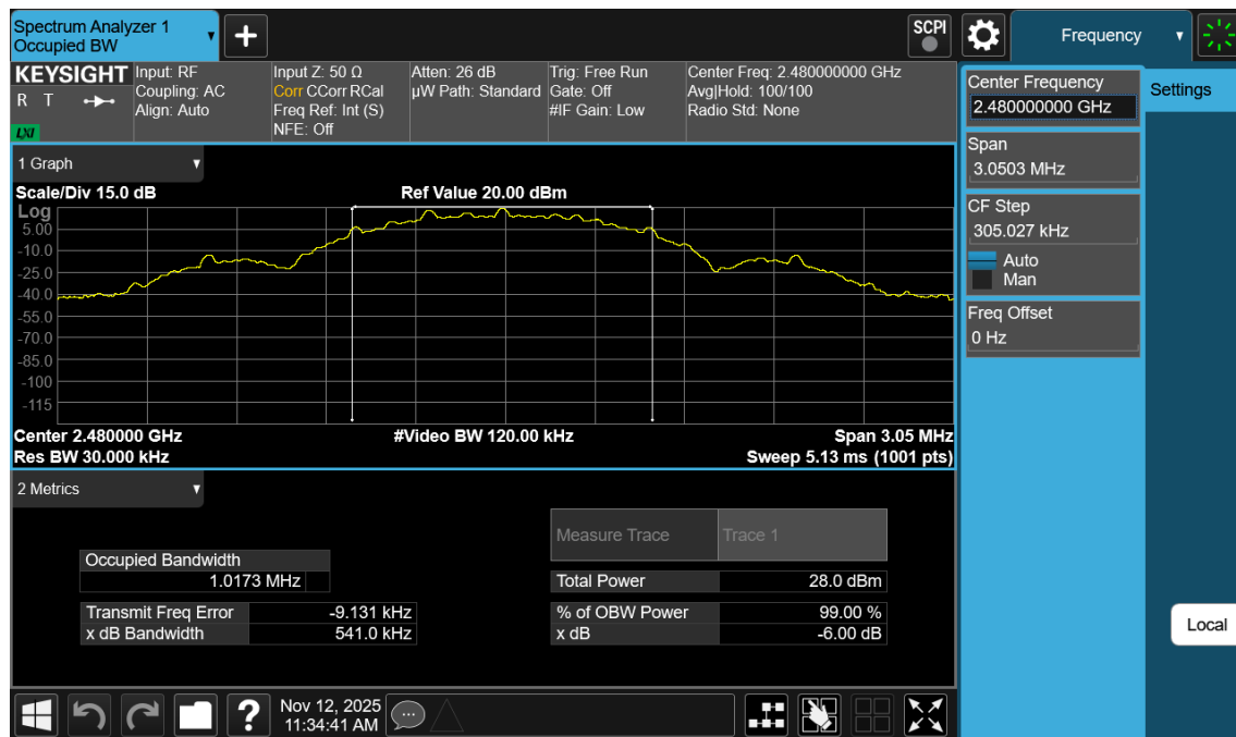
Plot 7-6. 99% OBW Plot Antenna WF8 (Bluetooth (LE), 500kbps, ePA – Ch. 39)
