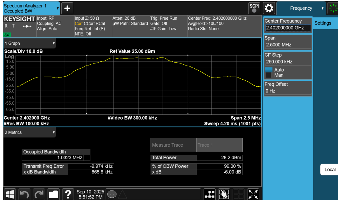
Plot 7-43. 6dB BW Plot Antenna WF7b (Bluetooth (LE), 1Mbps, ePA – Ch. 0)
