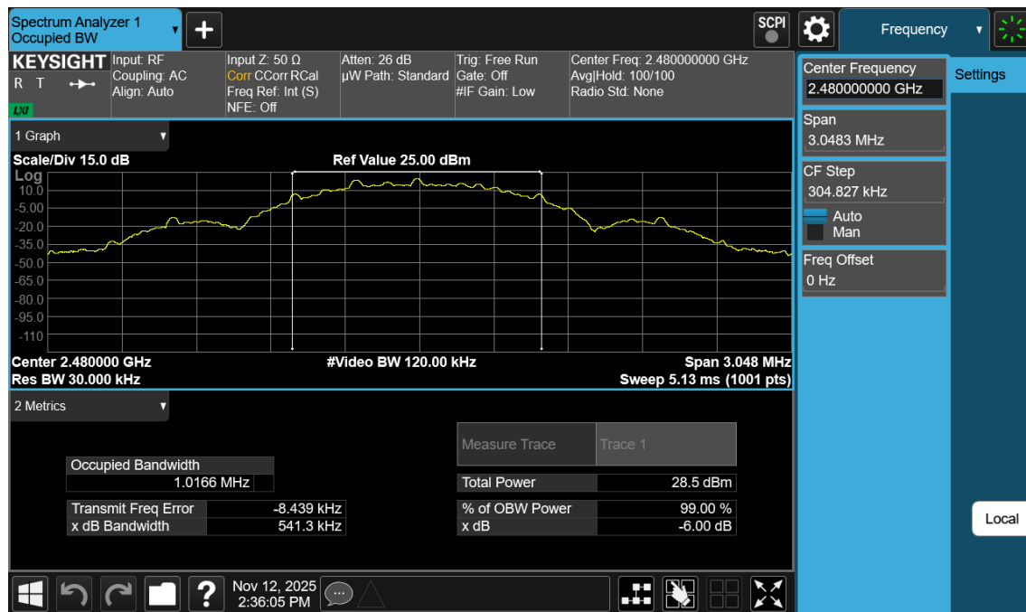
Plot 7-18. 99% OBW Plot Antenna WF7b (Bluetooth (LE), 500kbps, ePA – Ch. 39)
