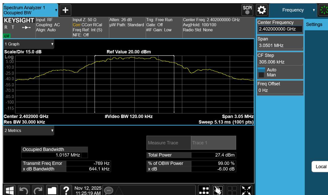
Plot 7-7. 99% OBW Plot Antenna WF8 (Bluetooth (LE), 1Mbps, ePA – Ch. 0)
