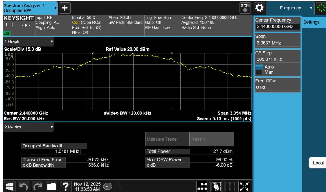
Plot 7-5.99% OBW Plot Antenna WF8 (Bluetooth (LE), 500kbps, ePA – Ch. 19)
