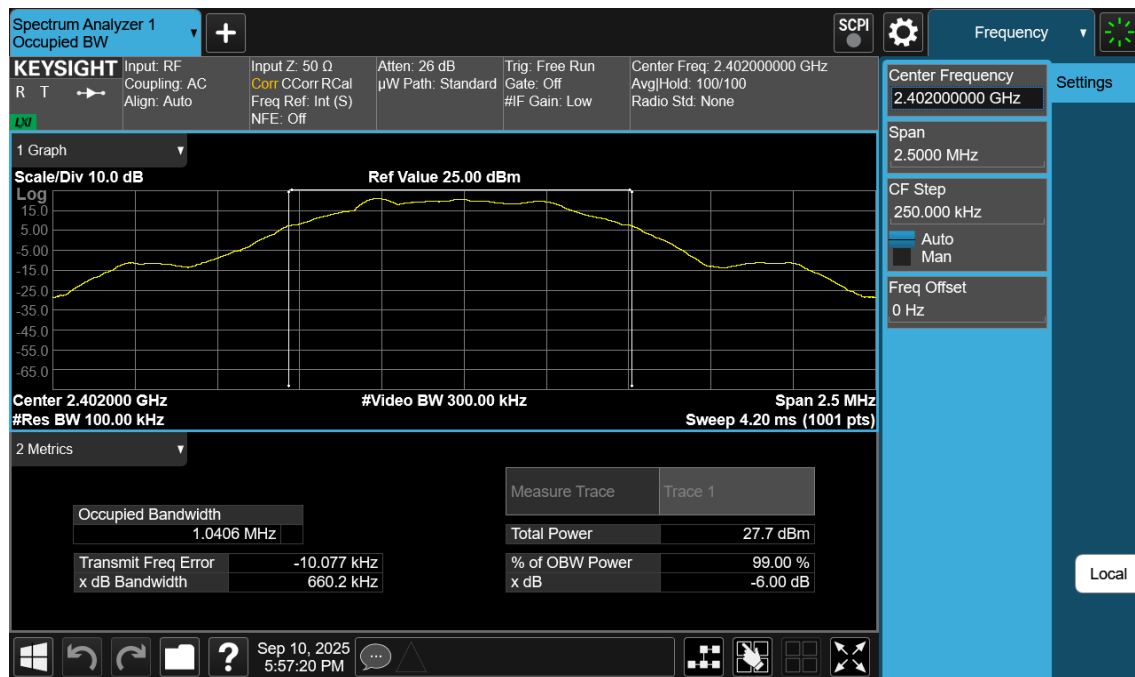
Plot 7-40. 6dB BW Plot Antenna WF7b (Bluetooth (LE), 500kbps, ePA – Ch. 0)
