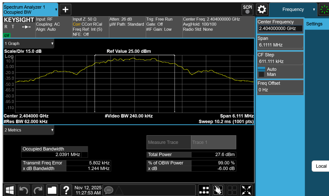
Plot 7-10. 99% OBW Plot Antenna WF8 (Bluetooth (LE), 2Mbps, ePA – Ch. 1)
