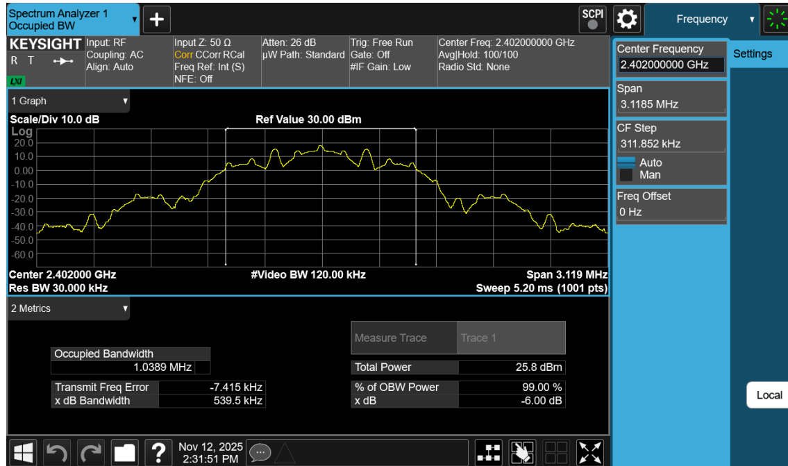
Plot 7-13. 99% OBW Plot Antenna WF7b (Bluetooth (LE), 125kbps, ePA – Ch. 0)
