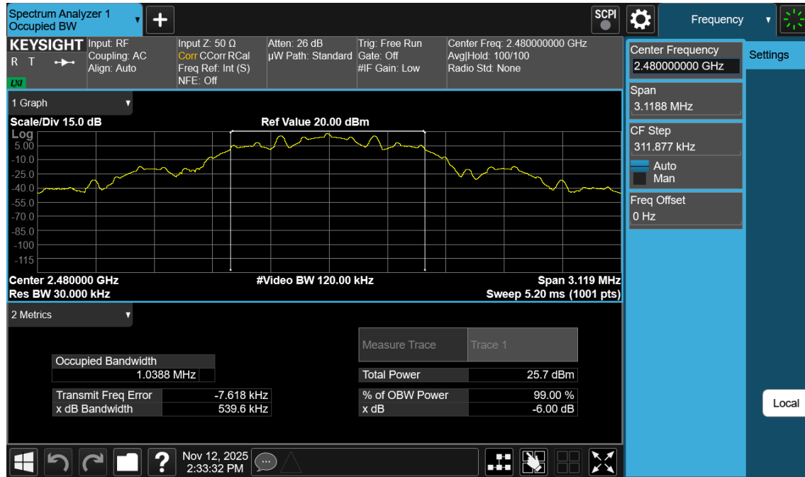
Plot 7-15. 99% OBW Plot Antenna WF7b (Bluetooth (LE), 125kbps, ePA – Ch. 39)
