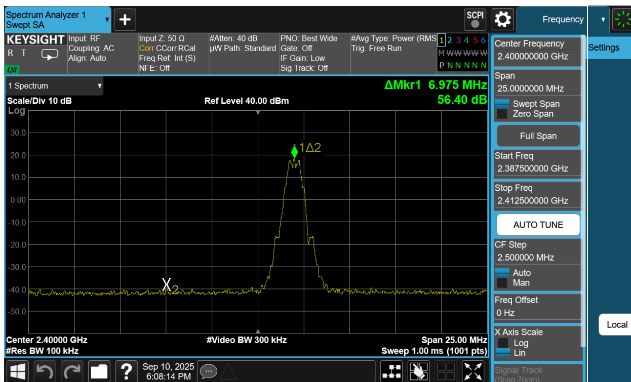
Plot 7-153. Band Edge Plot Antenna WF7b (Bluetooth (LE), 125kbps, ePA – Ch.0)
