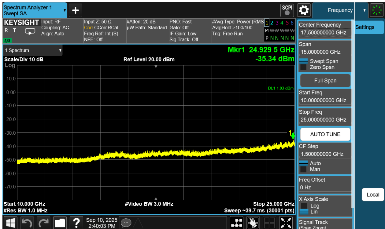
Plot 7-164. Conducted Spurious Plot Antenna WF8 (Bluetooth (LE), 1Mbps, ePA – Ch. 19)
