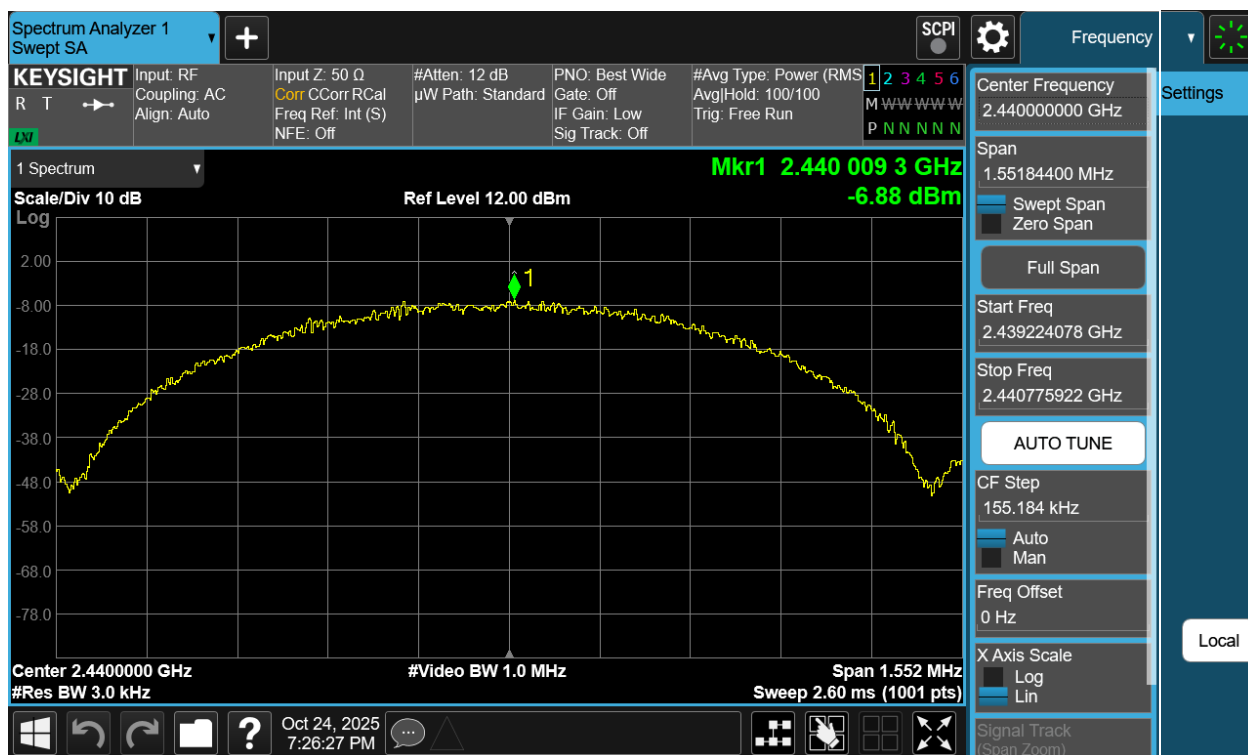
Plot 7-129. Power Spectral Density Plot Antenna WF8 (Bluetooth (LE), 1Mbps, iPA – Ch. 19)
