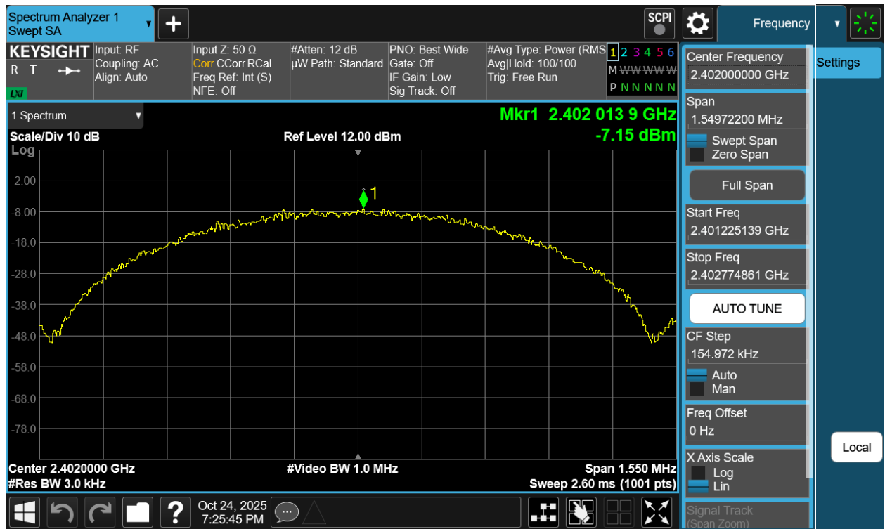
Plot 7-127. Power Spectral Density Plot Antenna WF8 (Bluetooth (LE), 1Mbps, iPA – Ch. 0)
