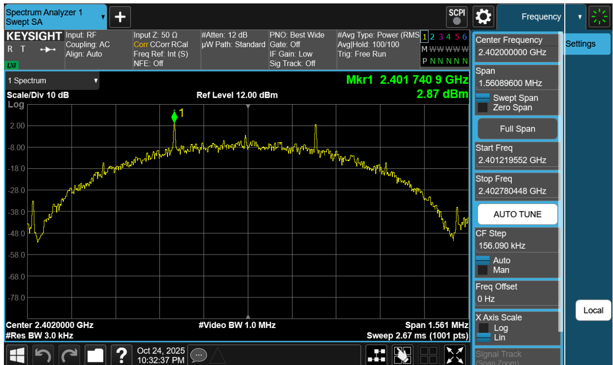
Plot 7-116. Power Spectral Density Plot Antenna WF7b (Bluetooth (LE), 500kbps, iPA – Ch. 0)
