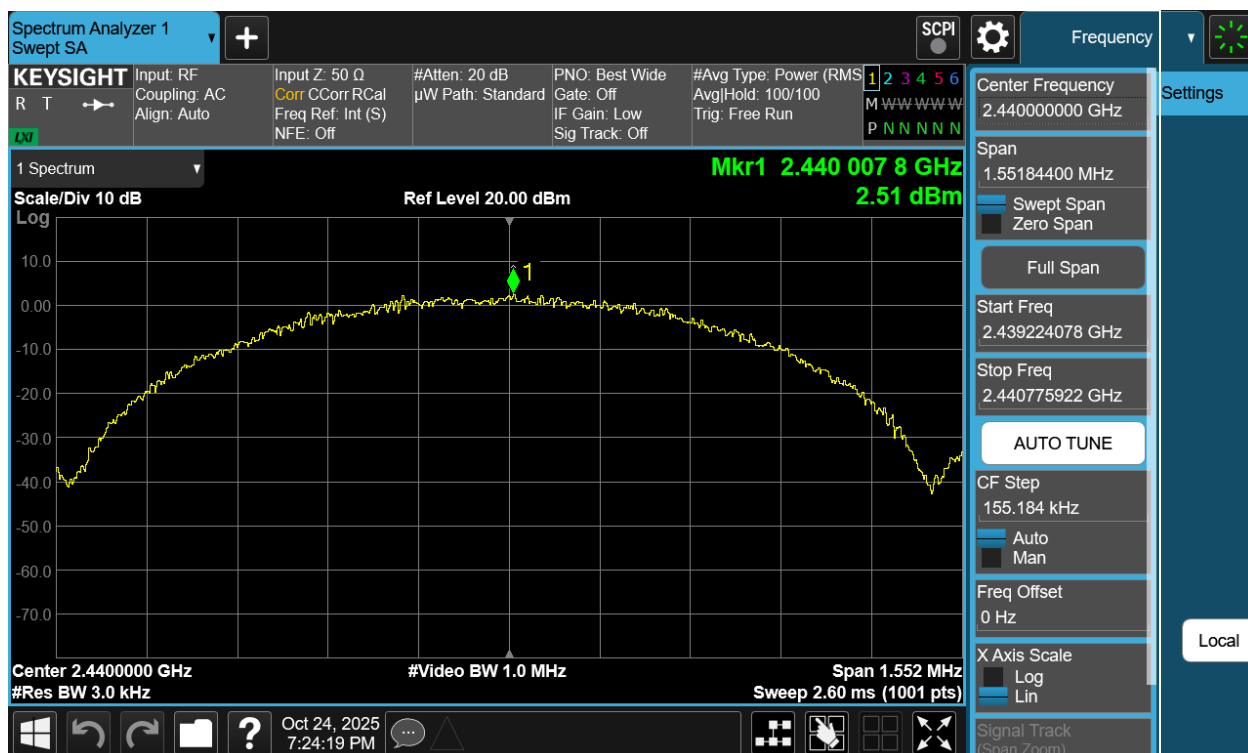
Plot 7-123. Power Spectral Density Plot Antenna WF8 (Bluetooth (LE), 1Mbps, ePA – Ch. 19)
