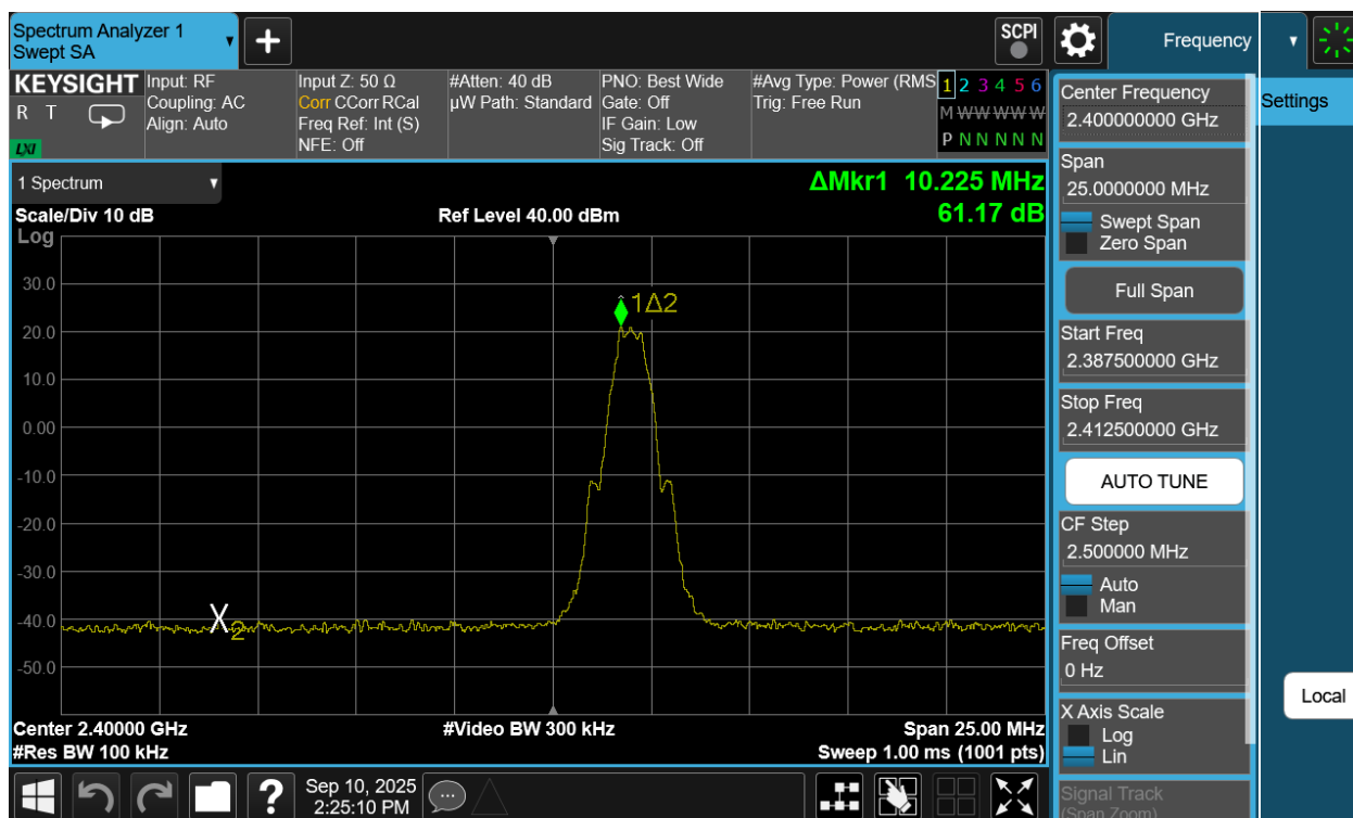
Plot 7-147. Band Edge Plot Antenna WF8 (Bluetooth (LE), 500kbps, ePA – Ch.0)
