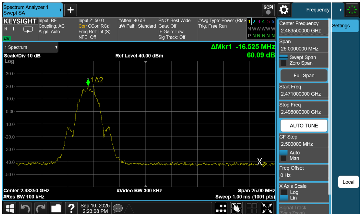
Plot 7-152. Band Edge Plot Antenna WF8 (Bluetooth (LE), 2Mbps, ePA – Ch. 38)
