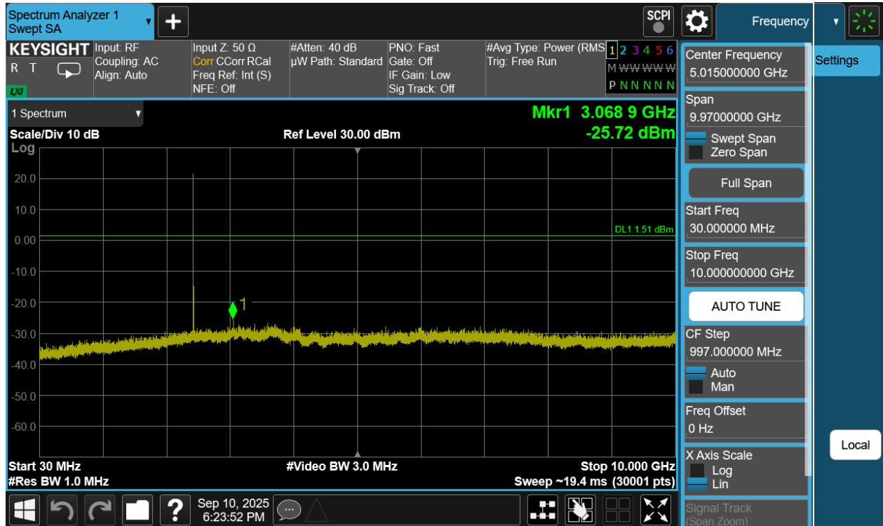
Plot 7-169. Conducted Spurious Plot Antenna WF7b (Bluetooth (LE), 1Mbps, ePA – Ch. 19)
