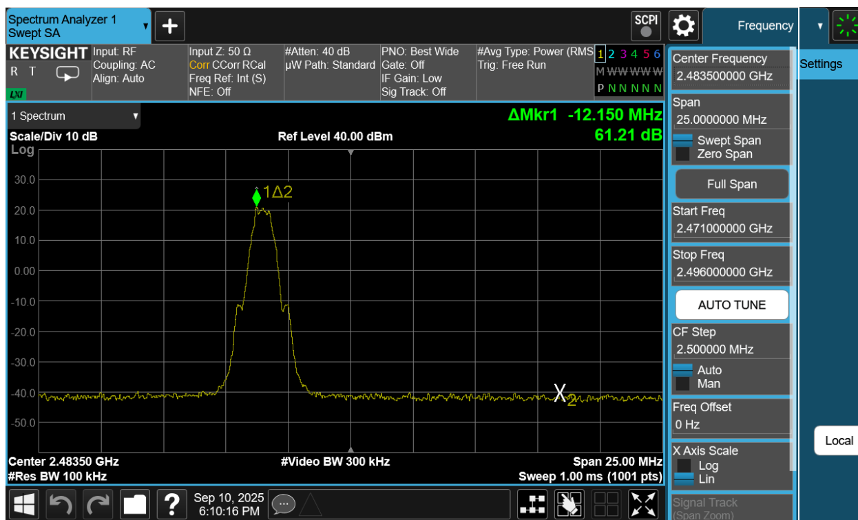
Plot 7-156. Band Edge Plot Antenna WF7b (Bluetooth (LE), 500kbps, ePA – Ch. 39)
