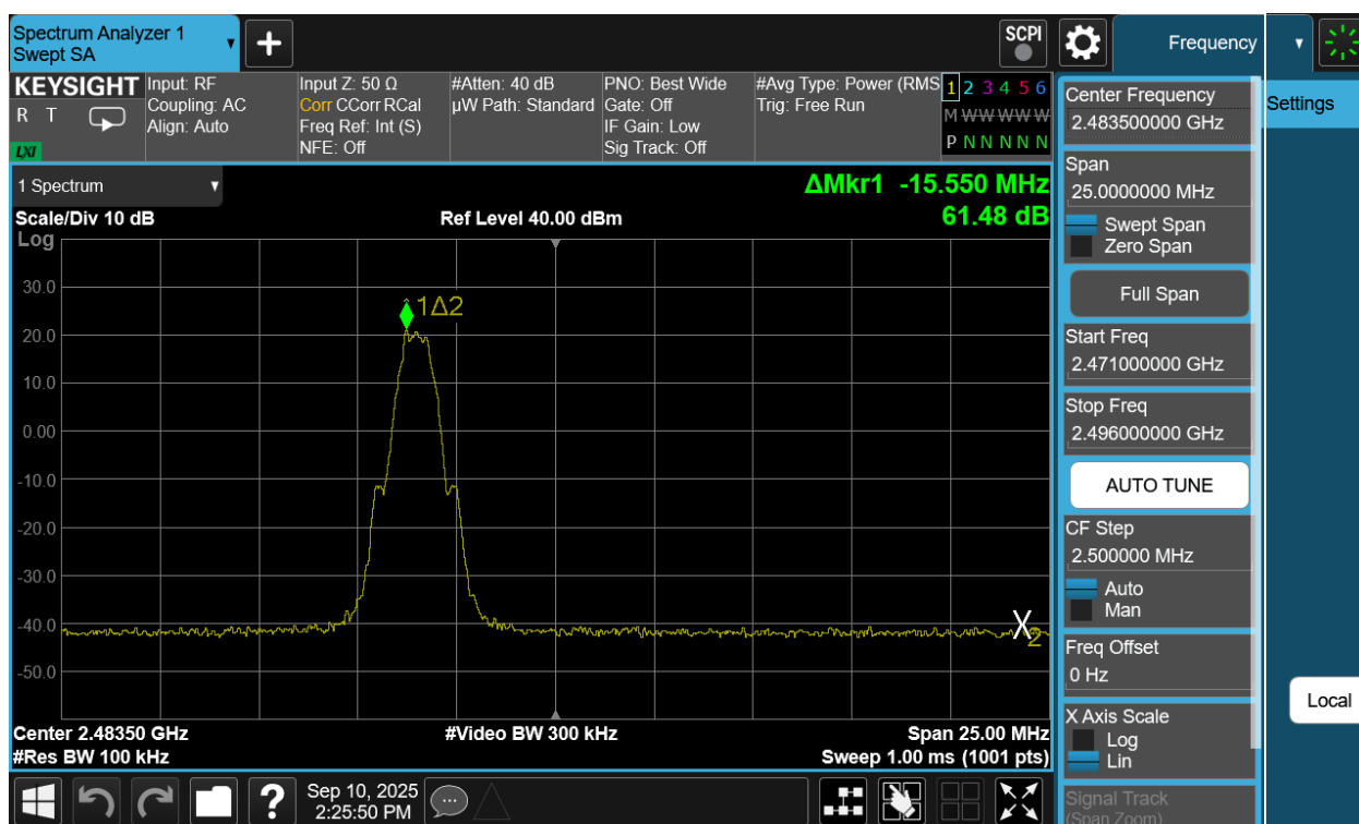
Plot 7-148. Band Edge Plot Antenna WF8 (Bluetooth (LE), 500kbps, ePA – Ch. 39)
