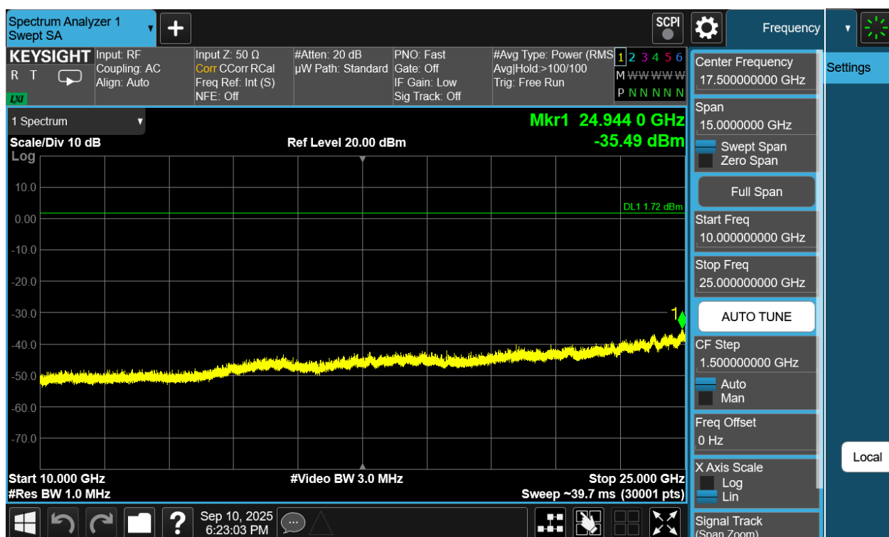
Plot 7-168. Conducted Spurious Plot Antenna WF7b (Bluetooth (LE), 1Mbps, ePA – Ch. 0)
