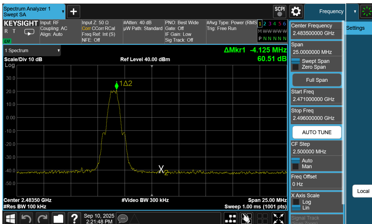
Plot 7-150. Band Edge Plot Antenna WF8 (Bluetooth (LE), 1Mbps, ePA – Ch. 39)
