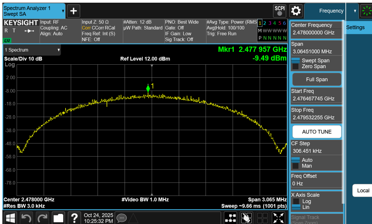
Plot 7-144. Power Spectral Density Plot Antenna WF7b (Bluetooth (LE), 2Mbps, iPA – Ch. 38)
