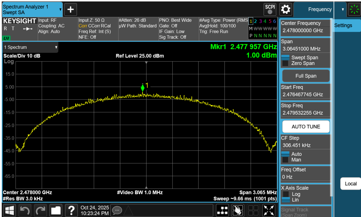
Plot 7-138. Power Spectral Density Plot Antenna WF7b (Bluetooth (LE), 2Mbps, ePA – Ch. 38)
