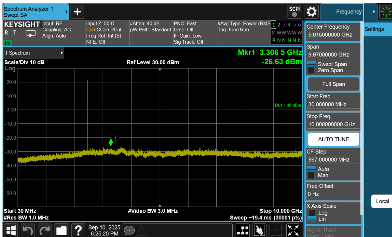
Plot 7-171. Conducted Spurious Plot Antenna WF7b (Bluetooth (LE), 1Mbps, ePA – Ch. 39)
