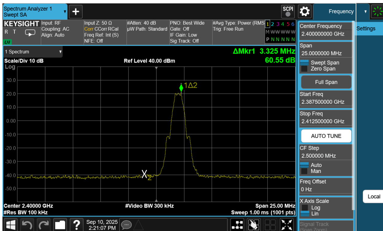
Plot 7-149. Band Edge Plot Antenna WF8 (Bluetooth (LE), 1Mbps, ePA – Ch.0)
