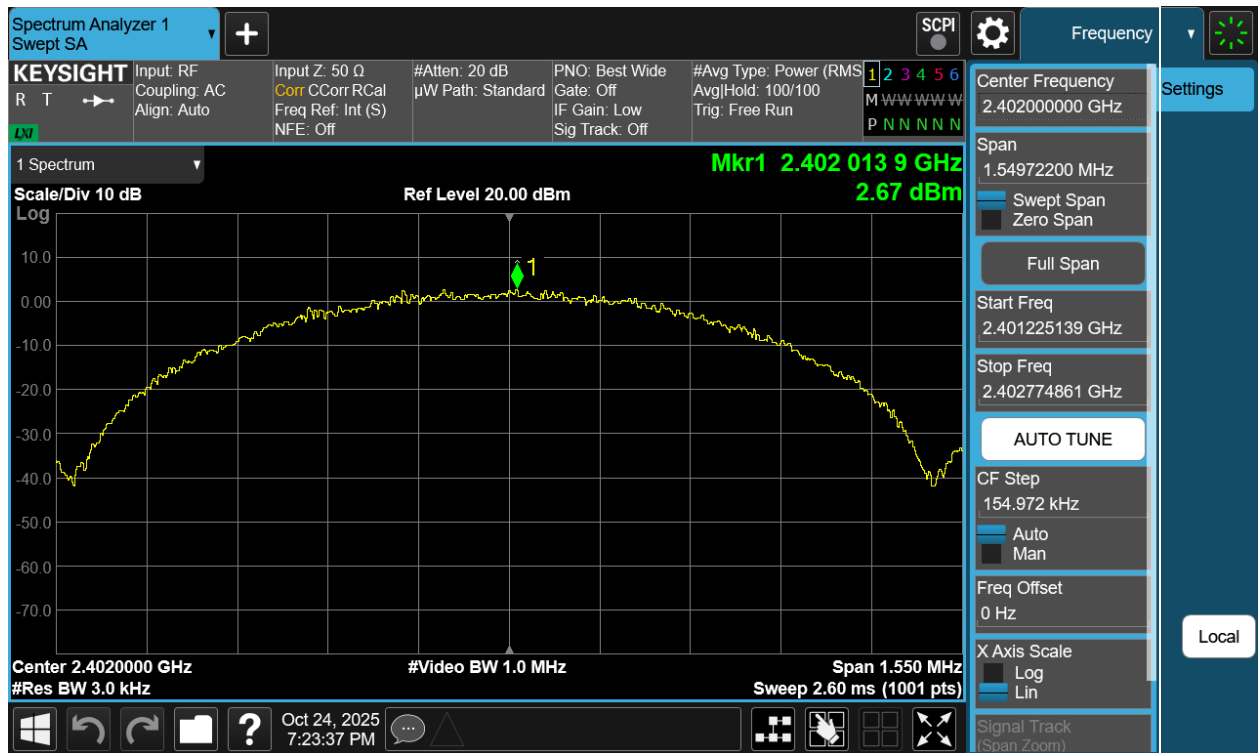
Plot 7-121. Power Spectral Density Plot Antenna WF8 (Bluetooth (LE), 1Mbps, ePA – Ch. 0)
