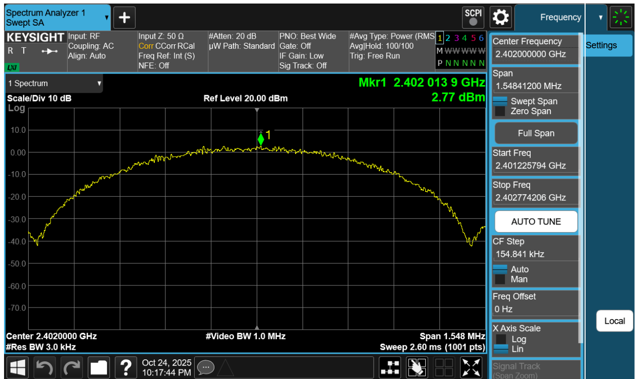
Plot 7-122. Power Spectral Density Plot Antenna WF7b (Bluetooth (LE), 1Mbps, ePA – Ch. 0)
