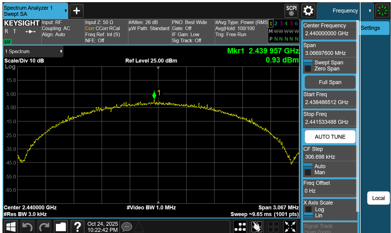
Plot 7-136. Power Spectral Density Plot Antenna WF7b (Bluetooth (LE), 2Mbps, ePA – Ch. 19)
