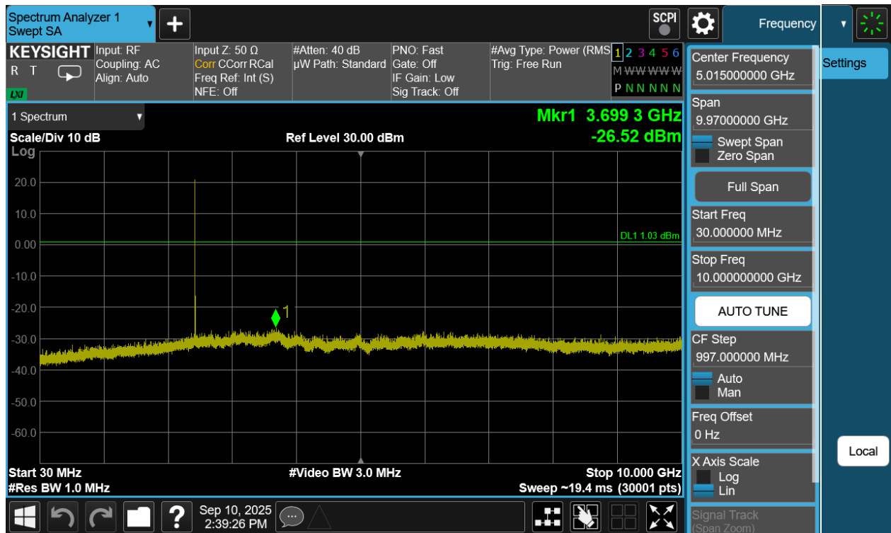
Plot 7-163. Conducted Spurious Plot Antenna WF8 (Bluetooth (LE), 1Mbps, ePA – Ch. 19)
