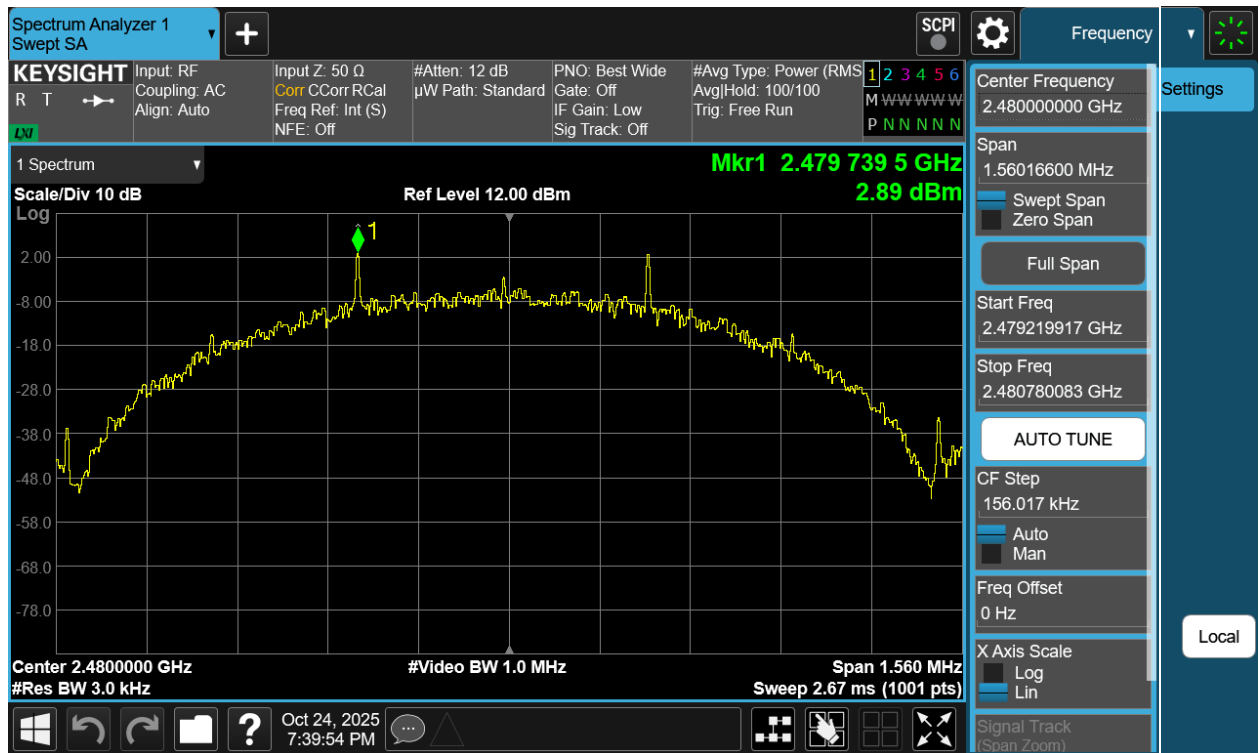
Plot 7-119. Power Spectral Density Plot Antenna WF8 (Bluetooth (LE), 500kbps, iPA – Ch. 39)
