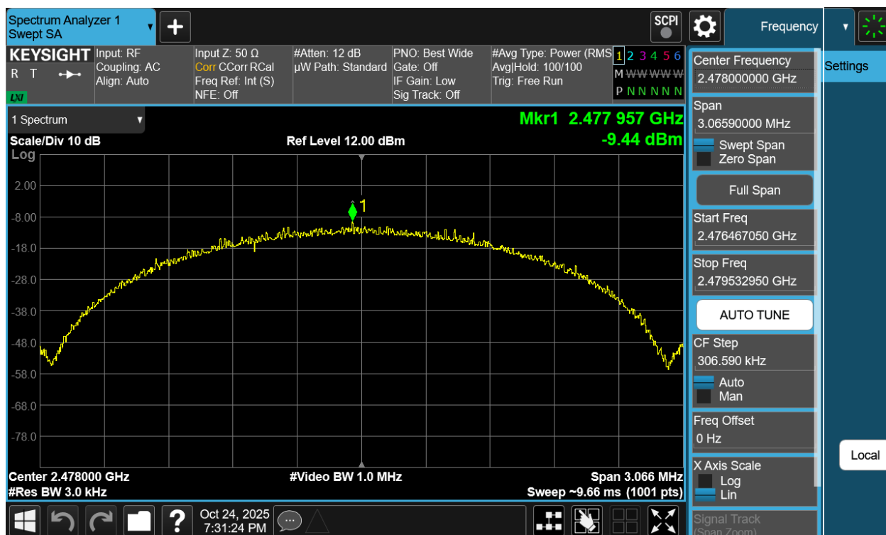
Plot 7-143. Power Spectral Density Plot Antenna WF8 (Bluetooth (LE), 2Mbps, iPA – Ch. 38)
