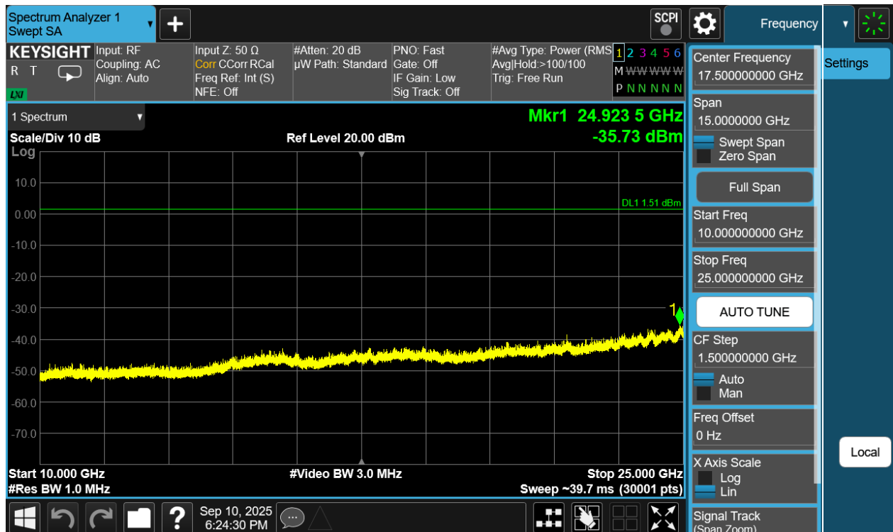
Plot 7-170. Conducted Spurious Plot Antenna WF7b (Bluetooth (LE), 1Mbps, ePA – Ch. 19)
