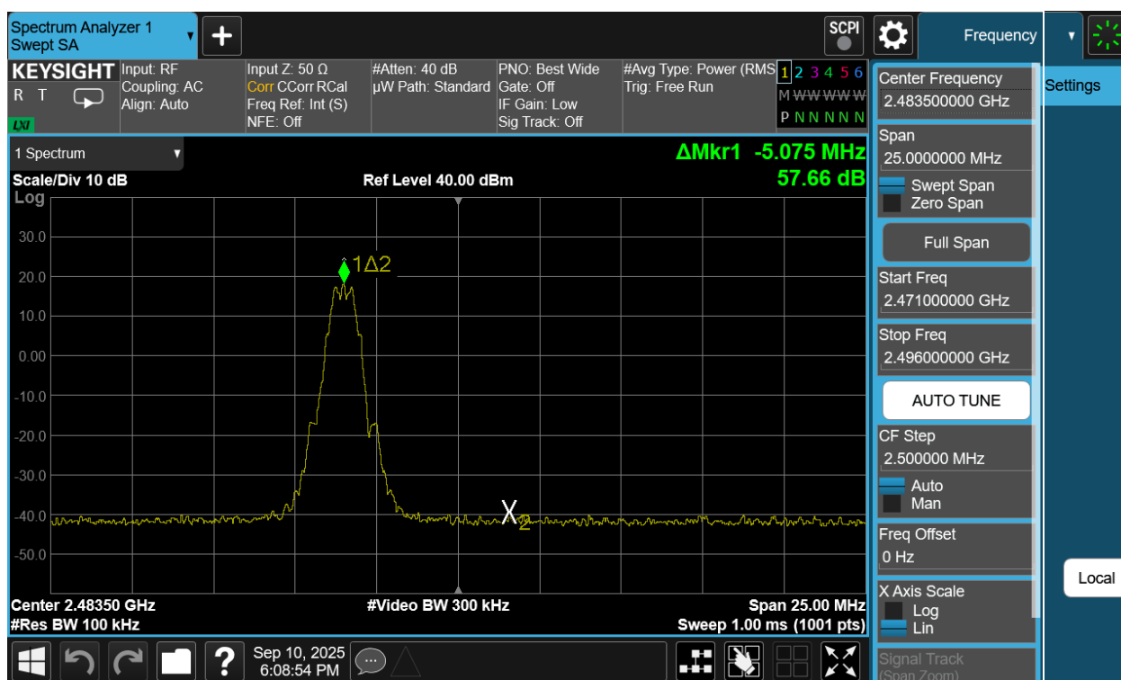
Plot 7-154. Band Edge Plot Antenna WF7b (Bluetooth (LE), 125kbps, ePA – Ch. 39)
