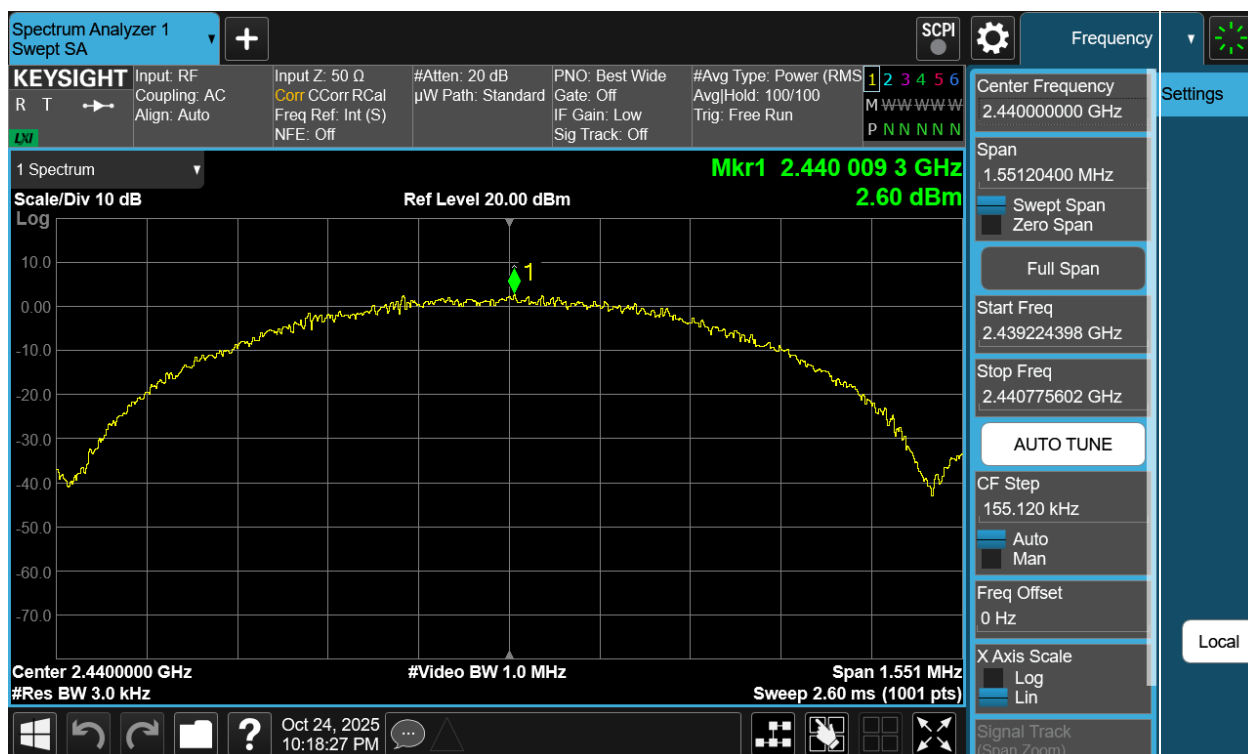
Plot 7-124. Power Spectral Density Plot Antenna WF7b (Bluetooth (LE), 1Mbps, ePA – Ch. 19)
