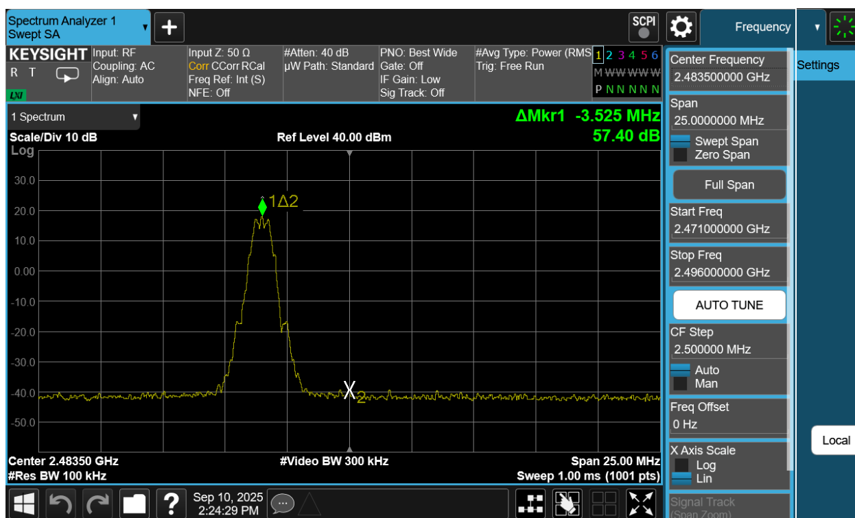
Plot 7-146. Band Edge Plot Antenna WF8 (Bluetooth (LE), 125kbps, ePA – Ch. 39)
