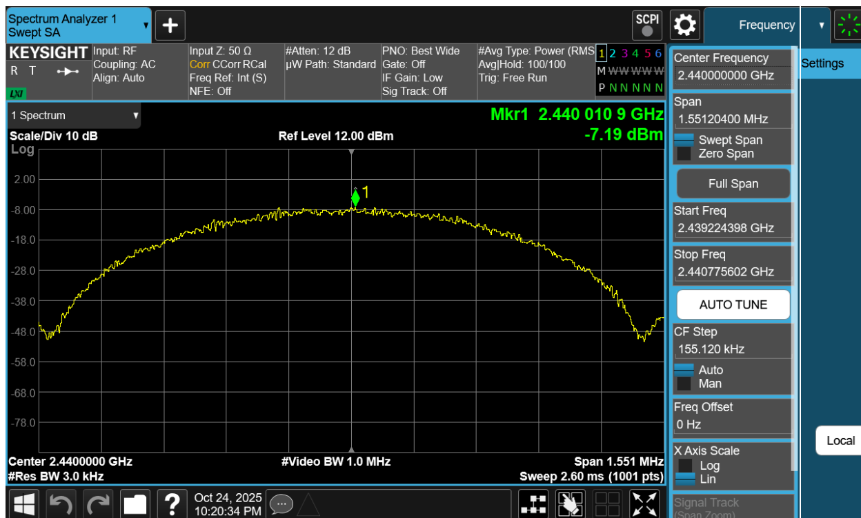
Plot 7-130. Power Spectral Density Plot Antenna WF7b (Bluetooth (LE), 1Mbps, iPA – Ch. 19)
