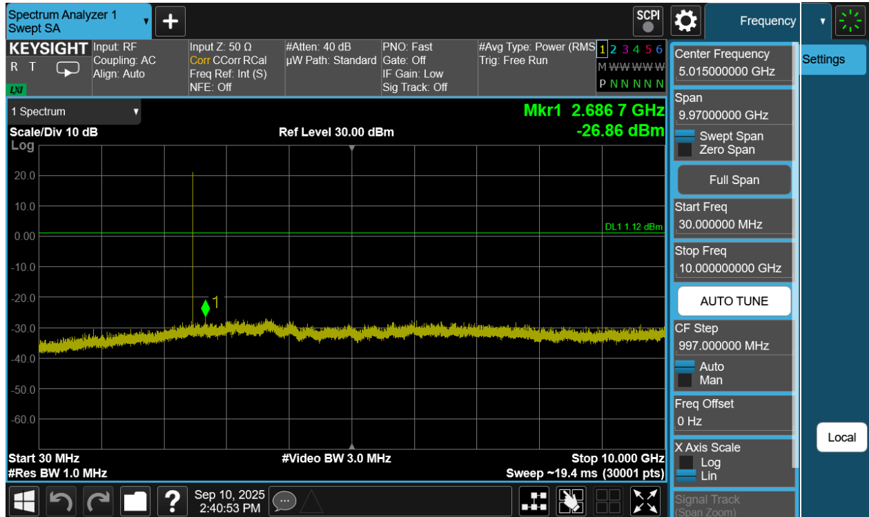
Plot 7-165. Conducted Spurious Plot Antenna WF8 (Bluetooth (LE), 1Mbps, ePA – Ch. 39)
