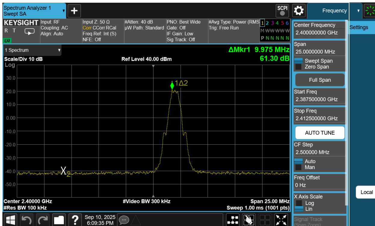
Plot 7-155. Band Edge Plot Antenna WF7b (Bluetooth (LE), 500kbps, ePA – Ch.0)
