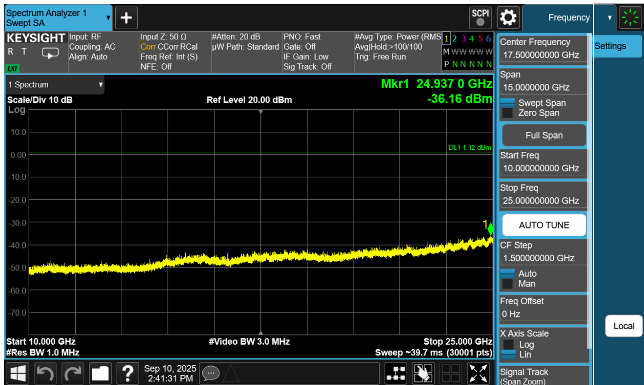
Plot 7-166. Conducted Spurious Plot Antenna WF8 (Bluetooth (LE), 1Mbps, ePA – Ch. 39)
