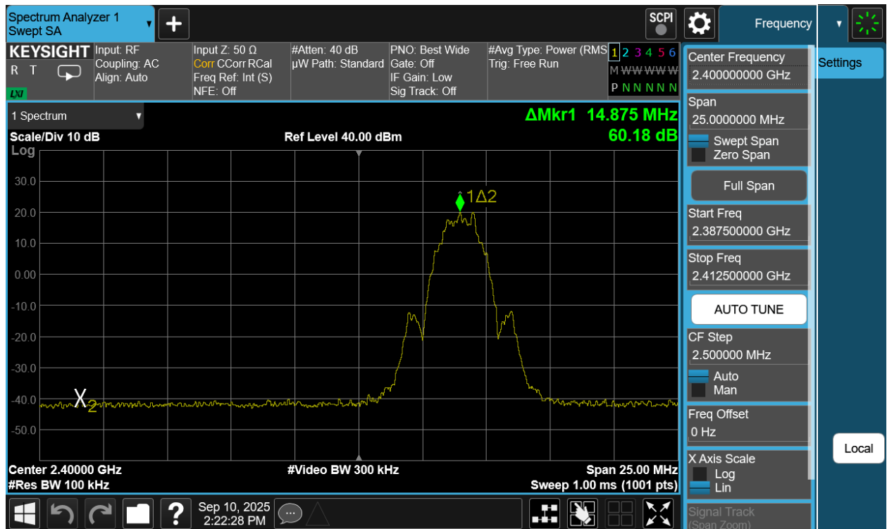
Plot 7-151. Band Edge Plot Antenna WF8 (Bluetooth (LE), 2Mbps, ePA – Ch. 1)
