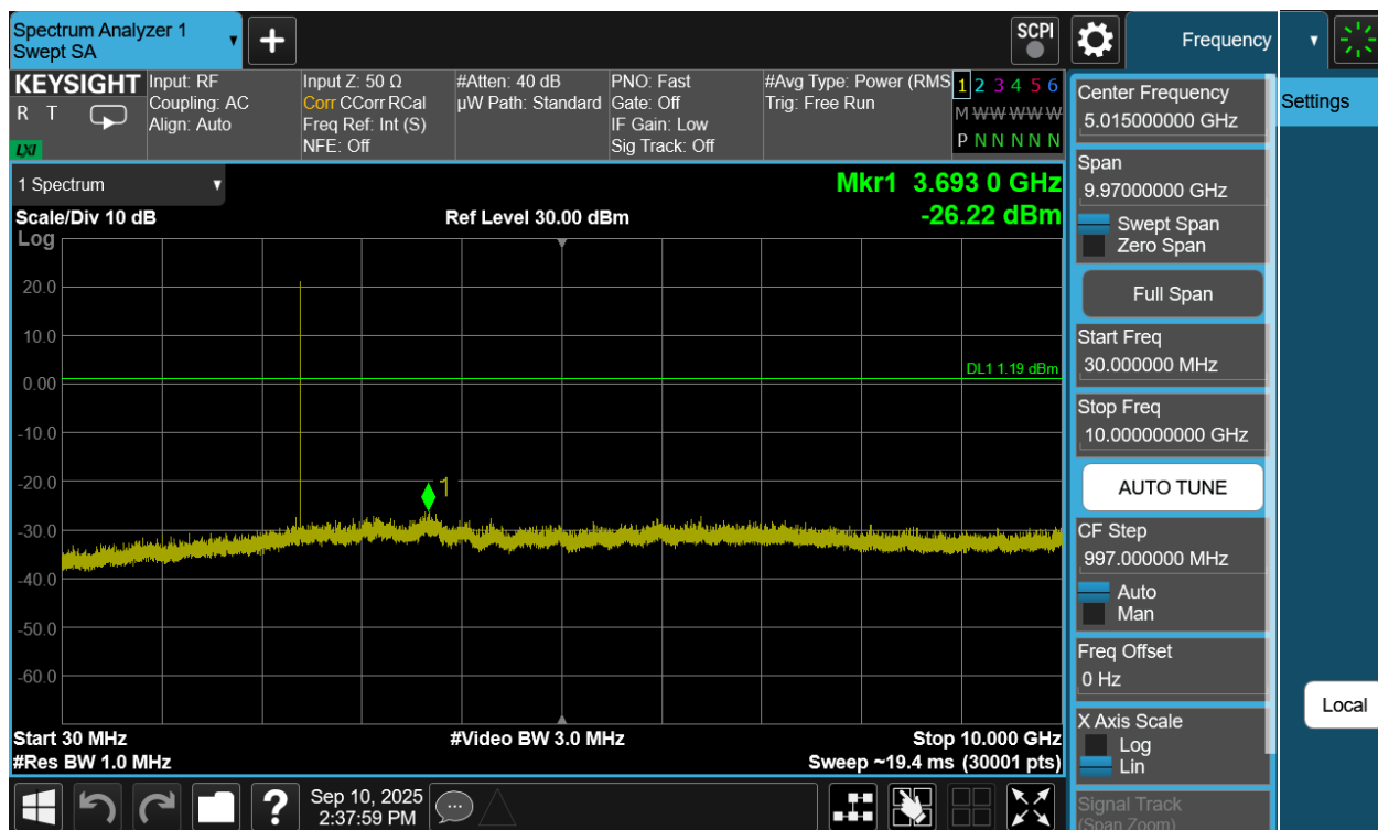
Plot 7-161. Conducted Spurious Plot Antenna WF8 (Bluetooth (LE), 1Mbps, ePA - Ch. 0)
