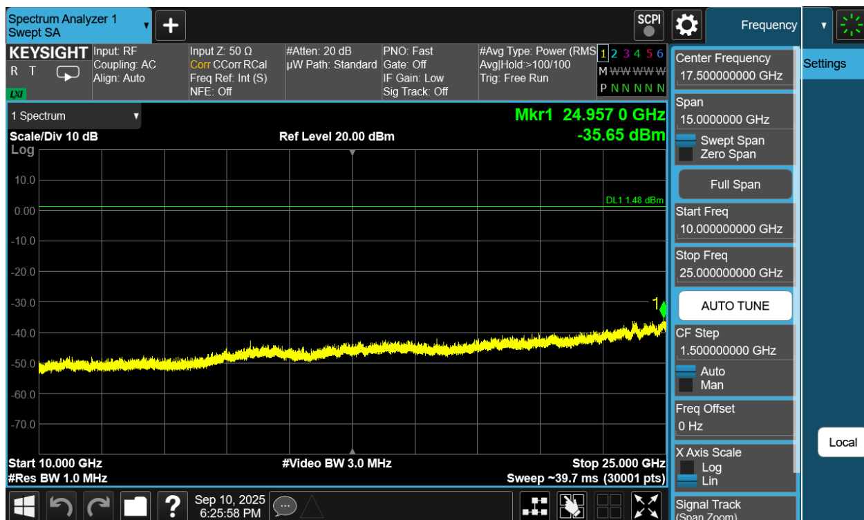
Plot 7-172. Conducted Spurious Plot Antenna WF7b (Bluetooth (LE), 1Mbps, ePA – Ch. 39)
