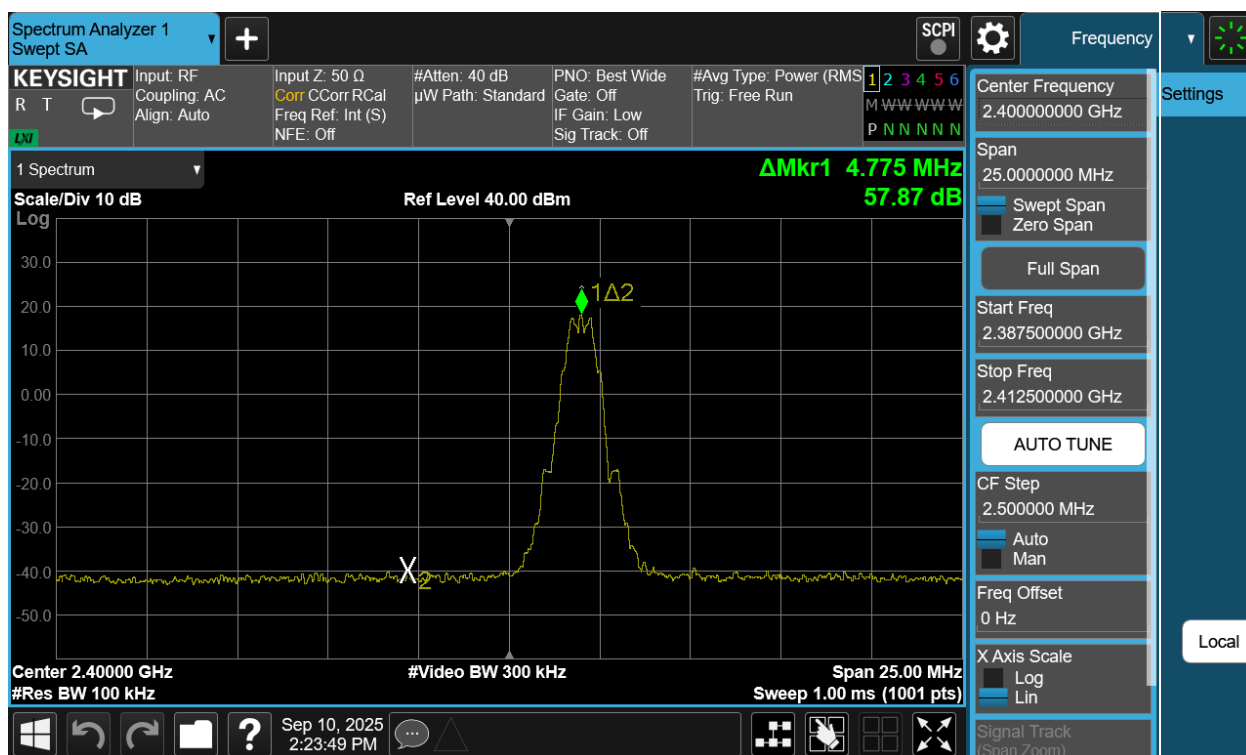
Plot 7-145. Band Edge Plot Antenna WF8 (Bluetooth (LE), 125kbps, ePA – Ch.0)
