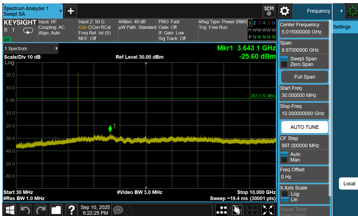
Plot 7-167. Conducted Spurious Plot Antenna WF7b (Bluetooth (LE), 1Mbps, ePA – Ch. 0)
