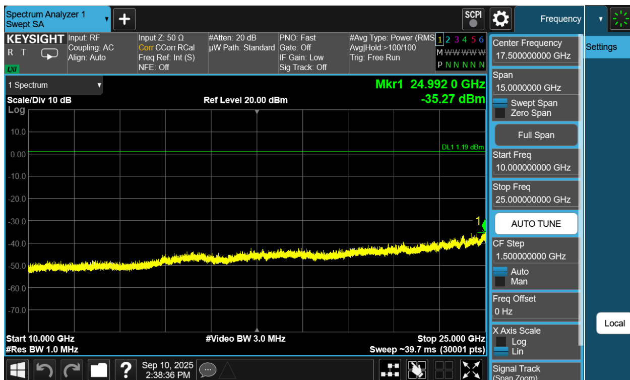
Plot 7-162. Conducted Spurious Plot Antenna WF8 (Bluetooth (LE), 1Mbps, ePA - Ch. 0)
