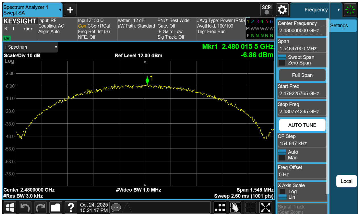
Plot 7-132. Power Spectral Density Plot Antenna WF7b (Bluetooth (LE), 1Mbps, iPA – Ch. 39)
