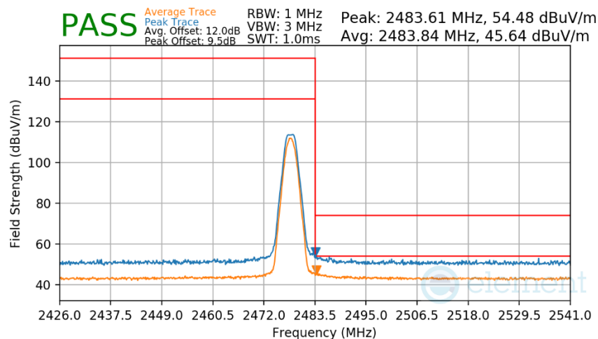
Plot 7-184. Radiated Restricted Upper Band Edge Measurement Antenna WF7b (Average & Peak)
