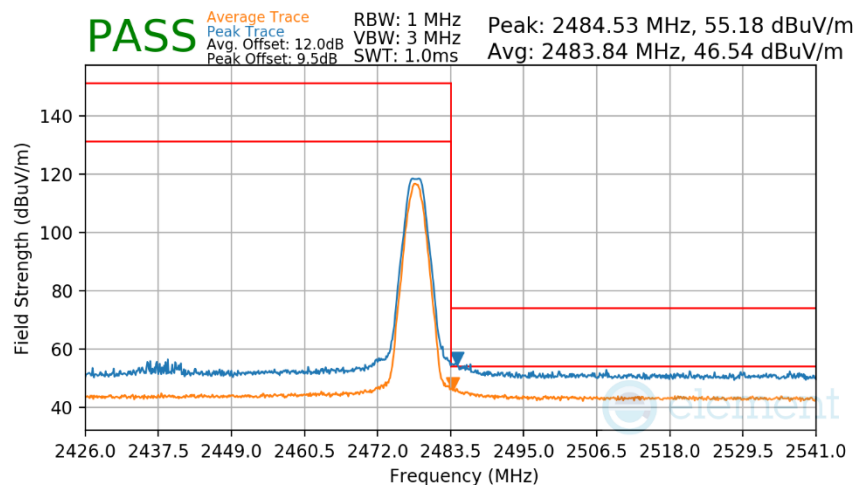
Plot 7-180. Radiated Restricted Upper Band Edge Measurement Antenna WF8 (Average & Peak)
