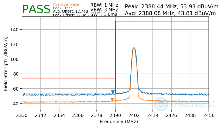
Plot 7-181. Radiated Restricted Lower Band Edge Measurement Antenna WF7b (Average & Peak)
