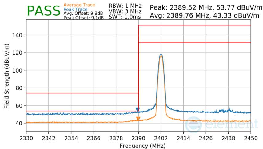
Plot 7-177. Radiated Restricted Lower Band Edge Measurement Antenna WF8 (Average & Peak)
