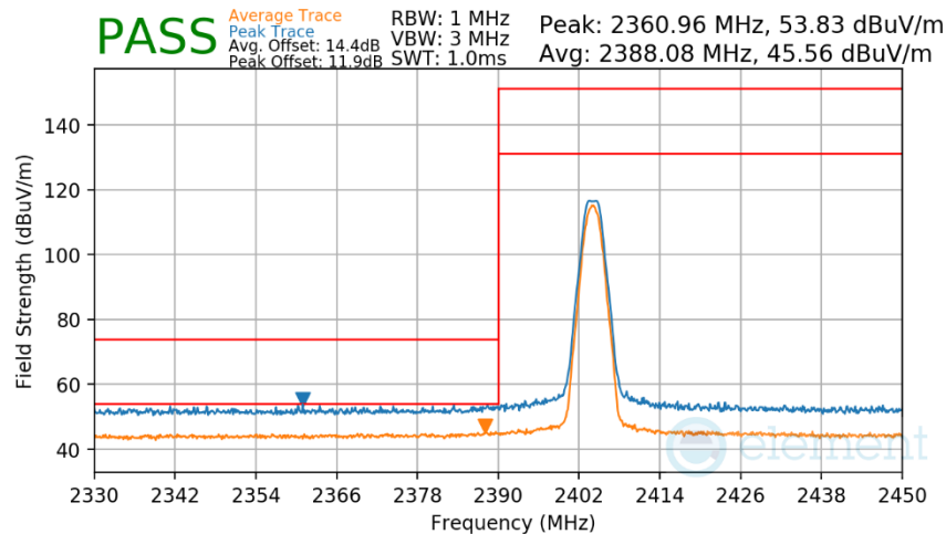
Plot 7-183. Radiated Restricted Lower Band Edge Measurement Antenna WF7b (Average & Peak)
