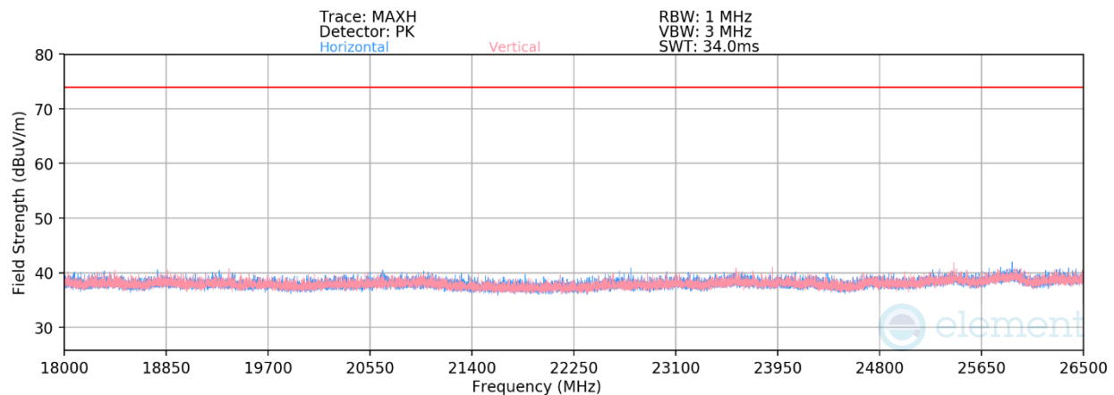
Plot 7-175. Radiated Spurious Emissions Above 18GHz TxBF (1Mbps ePA – Ch. 19)
