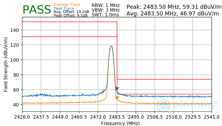
Plot 7-178. Radiated Restricted Upper Band Edge Measurement Antenna WF8 (Average & Peak)
