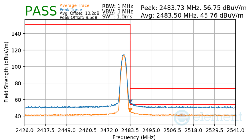
Plot 7-182. Radiated Restricted Upper Band Edge Measurement Antenna WF7b (Average & Peak)
