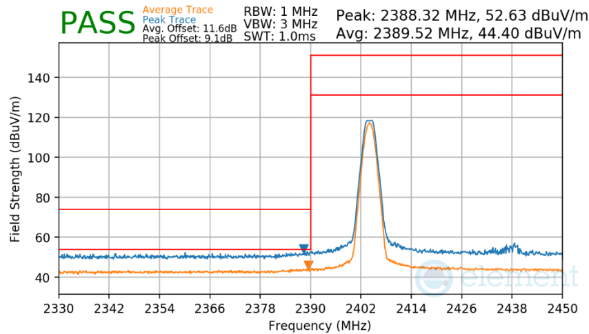
Plot 7-179. Radiated Restricted Lower Band Edge Measurement Antenna WF8 (Average & Peak)
