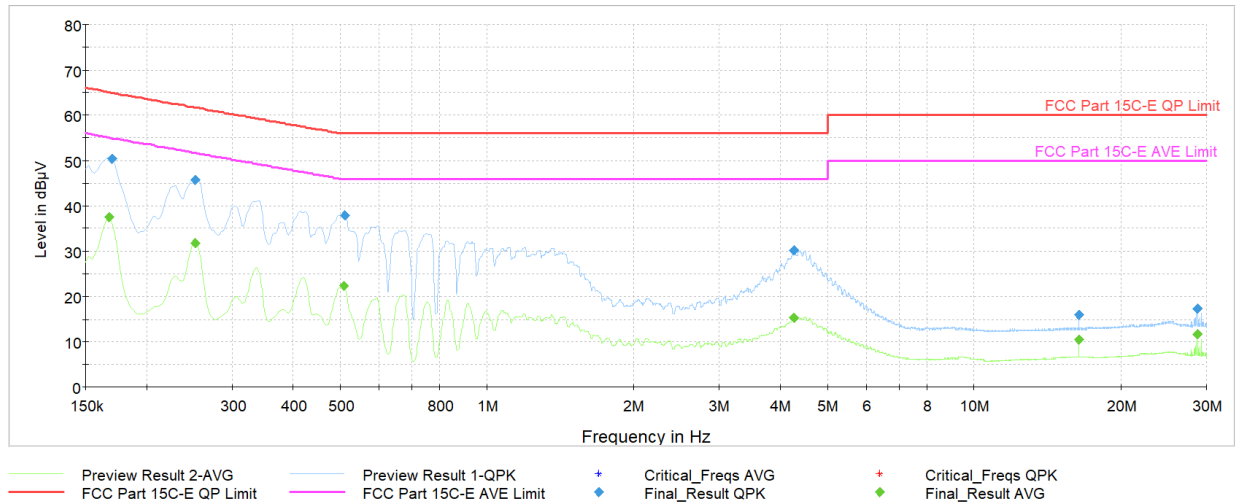
Plot 7-190. AC Line Conducted Plot with Bluetooth LE Tx BF (L1, 1Mbps ePA – Ch.19 with AC/DC Adapter)
