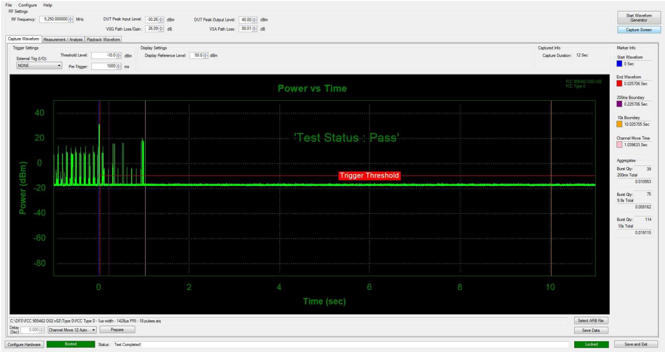
Figure 9-12. 5250MHz - Channel Move/ Closing Transmission Time - Mode 1 (160 MHz)
