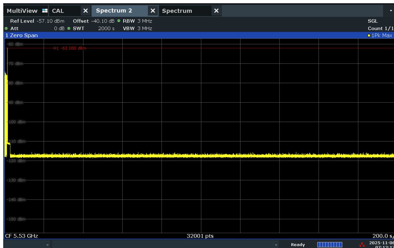
Figure 9-16. 5530MHz - Non-Occupancy Period (30 Minutes) - Mode 1 (80MHz)
