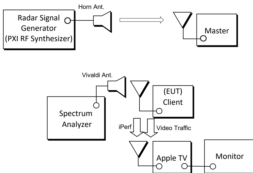
Figure 8-3. Test Setup (Mode 3)
