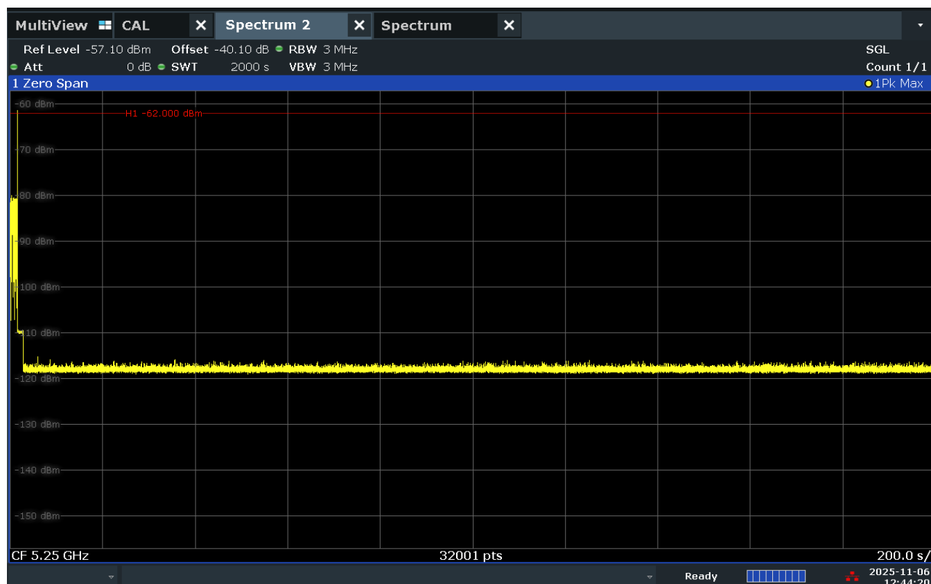
Figure 9-17. 5250MHz - Non-Occupancy Period (30 Minutes) - Mode 1 (160MHz)
