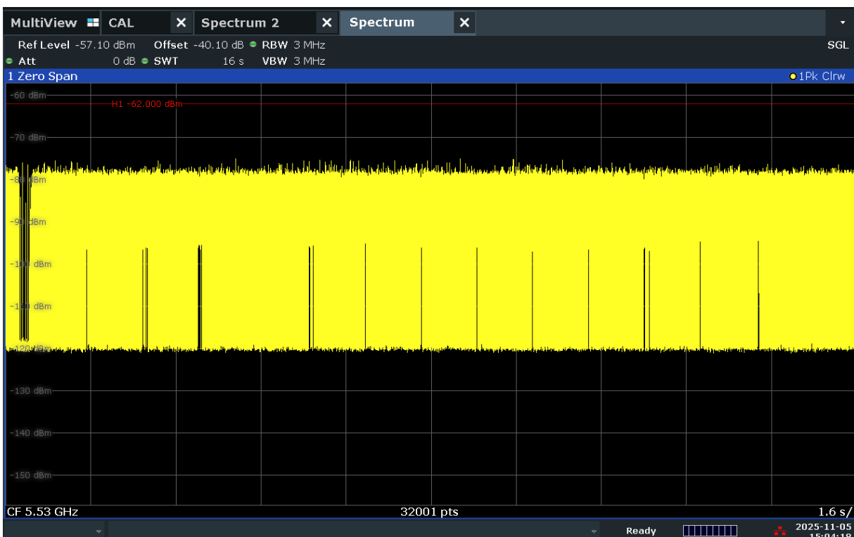
Figure 9-1. 5530MHz - Channel Loading - Mode 1 (80MHz)
