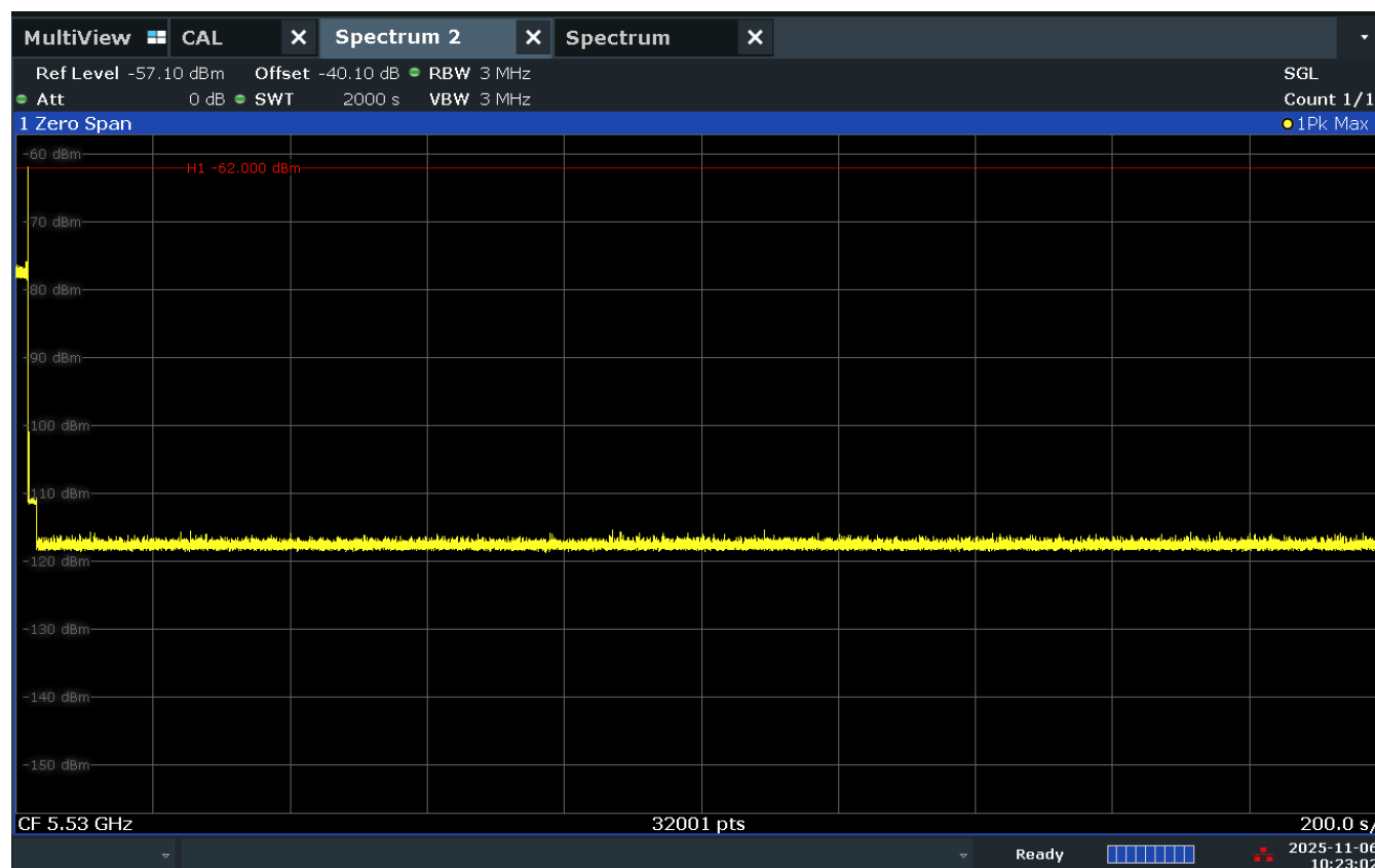
Figure 9-19. 5530MHz - Non-Occupancy Period (30 Minutes) - Mode 3 (80MHz)
