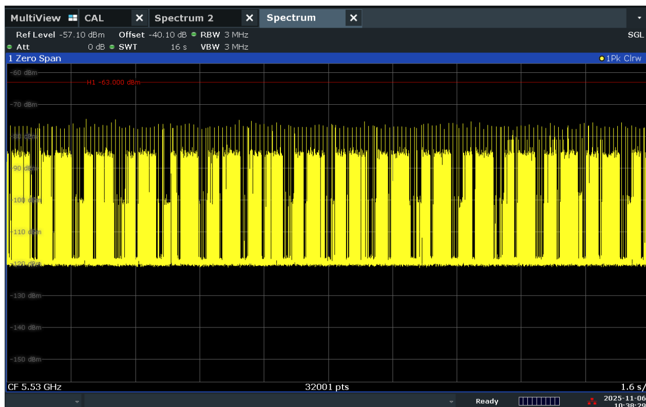
Figure 9-9. 5530 MHz - Channel Loading - Mode 4 (80MHz)
