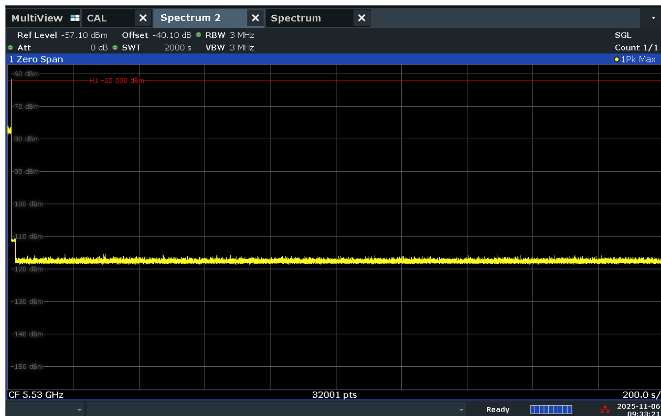
Figure 9-18. 5530MHz - Non-Occupancy Period (30 Minutes) - Mode 2 (80MHz)
