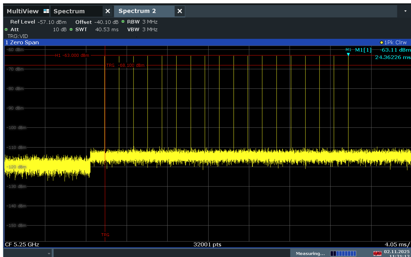
Figure 7-4. 5250MHz – Radar Pulse Type 0 (160MHz)
