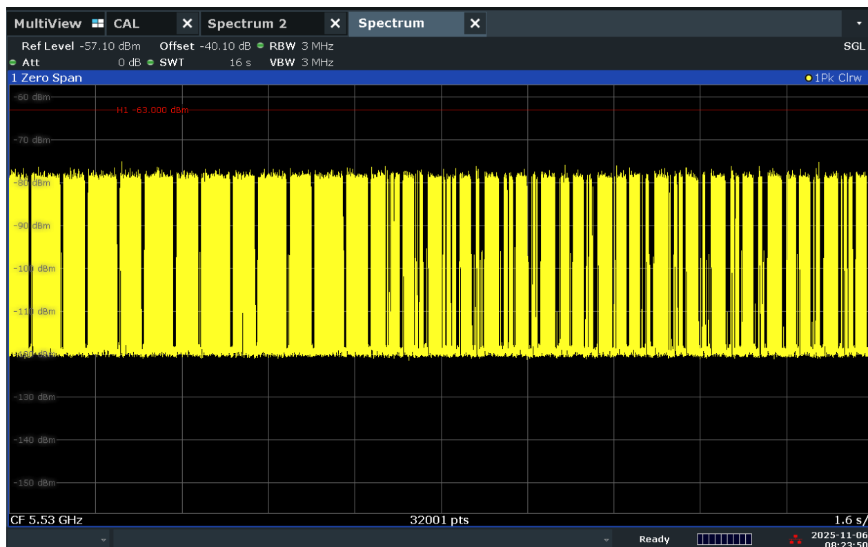
Figure 9-5. 5530MHz - Channel Loading - Mode 2 (80MHz)
