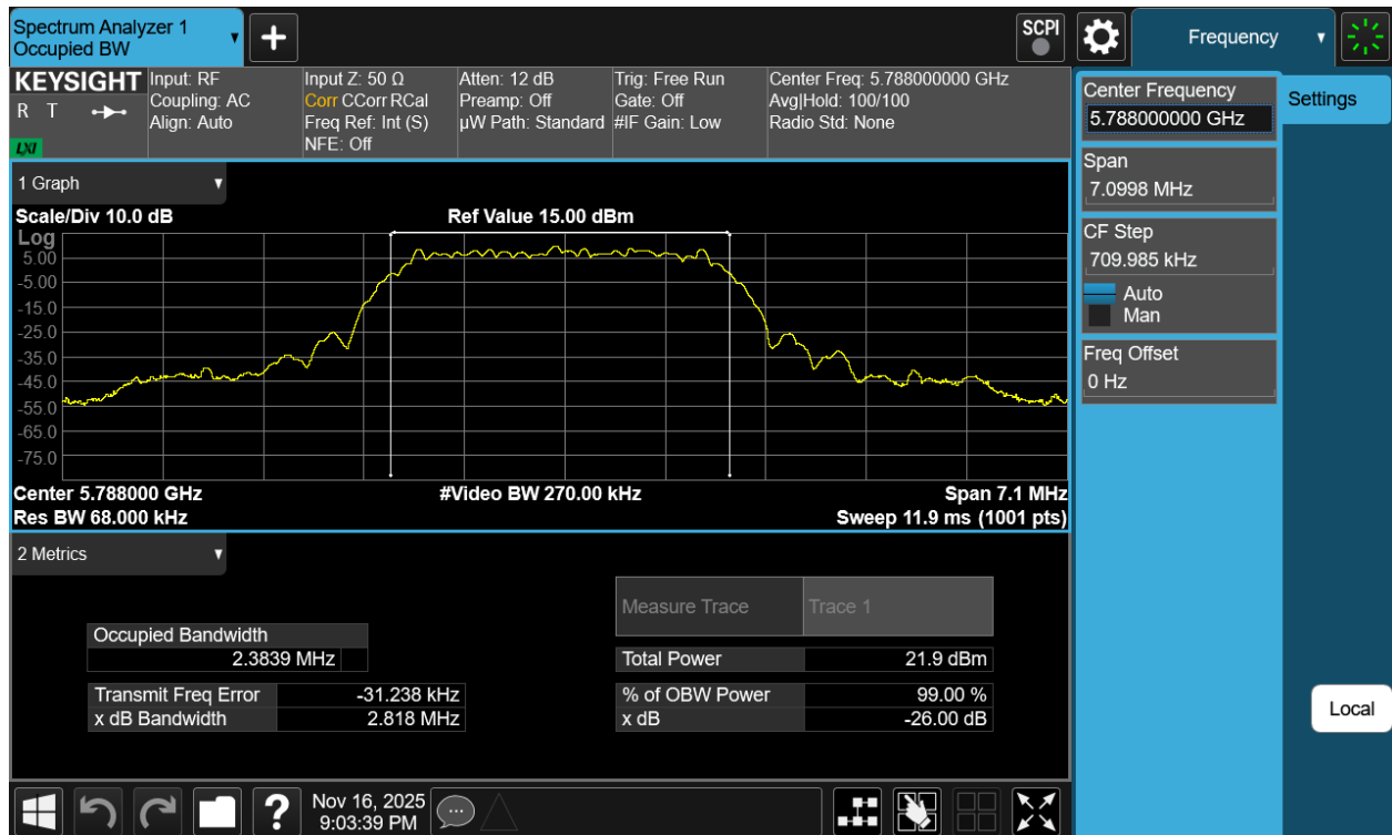
Plot 7-51. 99% OBW Antenna WF7a (NB UNII HDT4, ePA- 5788MHz)
