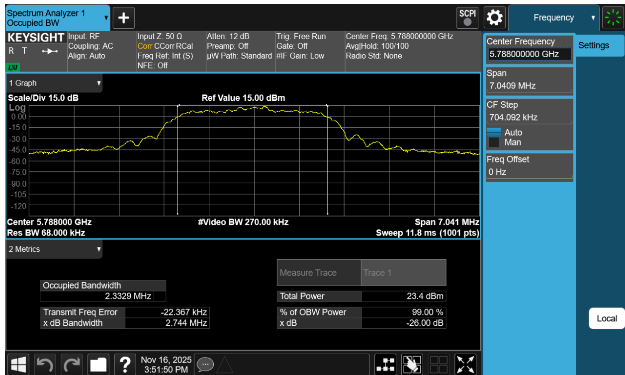
Plot 7-43. 99% OBW Antenna WF7a (NB UNII HDR4, ePA – 5788MHz)
