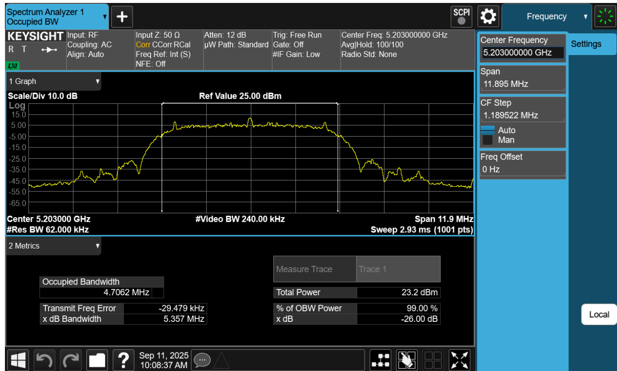
Plot 7-33. 26dB BW Antenna WF7a (NB UNII XHDRPM6, ePA- 5203MHz)
