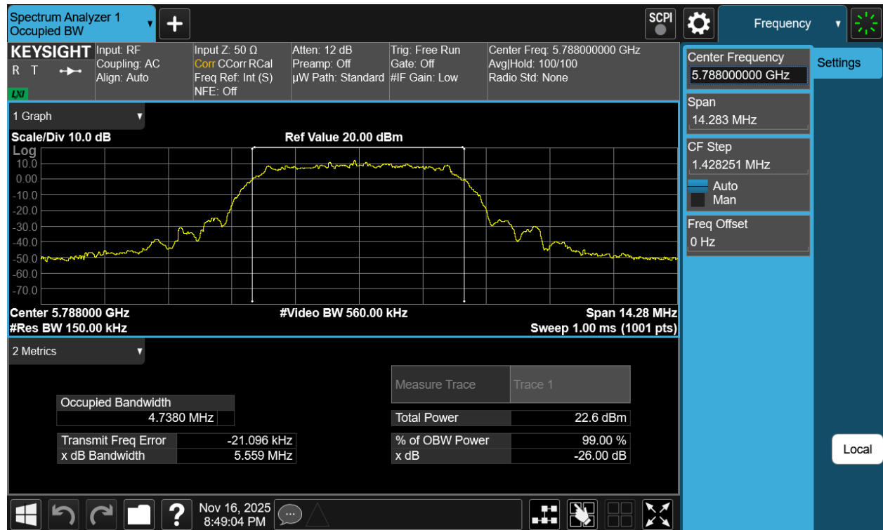
Plot 7-46. 99% OBW Antenna WF7a (NB UNII XHDRPM6, ePA – 5788MHz)
