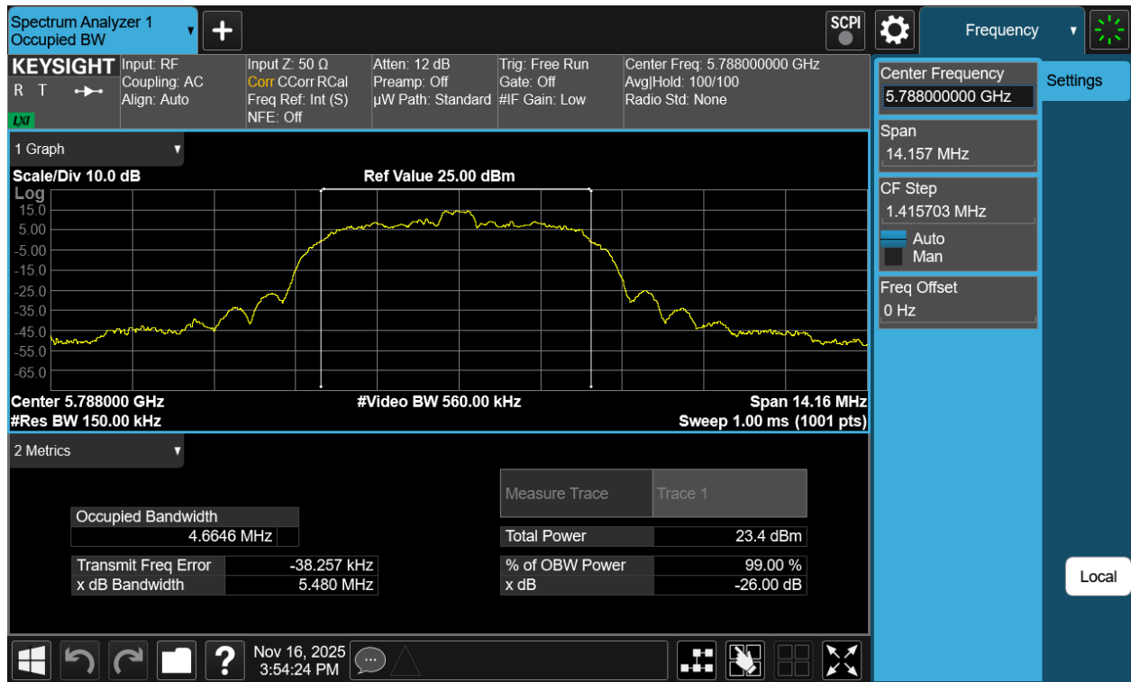
Plot 7-44. 99% OBW Antenna WF7a (NB UNII HDR8, ePA - 5788MHz)
