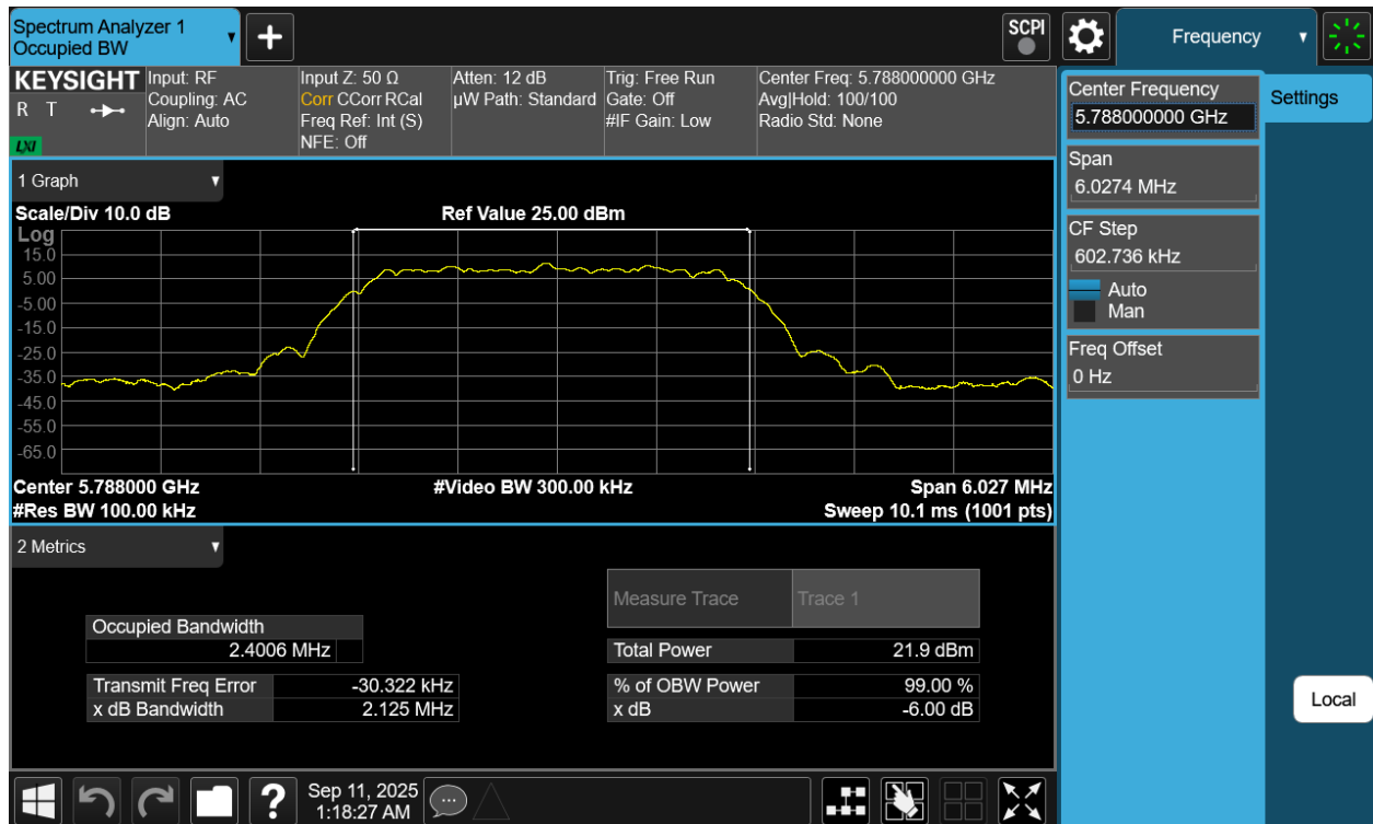
Plot 7-64. 6dB BW Antenna WF8 (NB UNII HDT4, ePA- 5788MHz)
