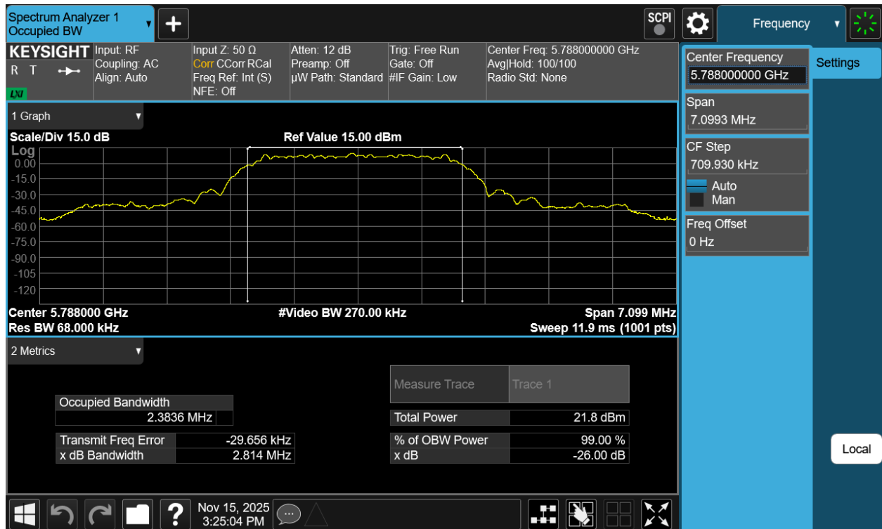
Plot 7-25. 99% OBW Antenna WF8 (NB UNII HDT4, ePA- 5788MHz)
