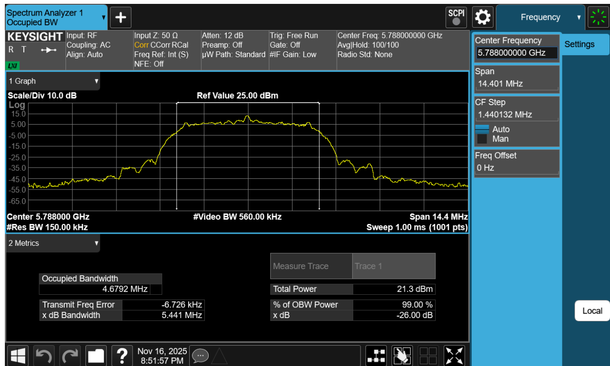
Plot 7-47. 99% OBW Antenna WF7a (NB UNII HDRPM16, ePA – 5788MHz)
