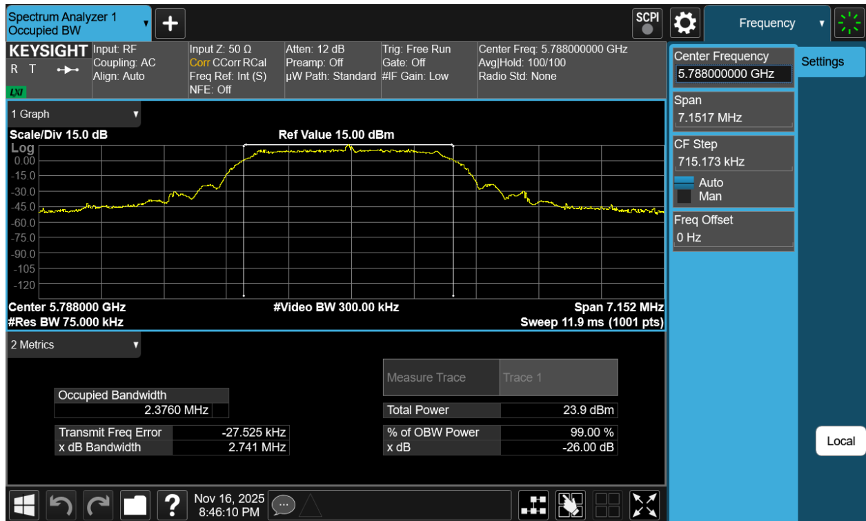
Plot 7-45. 99% OBW Antenna WF7a (NB UNII HDRPS2, ePA - 5788MHz)
