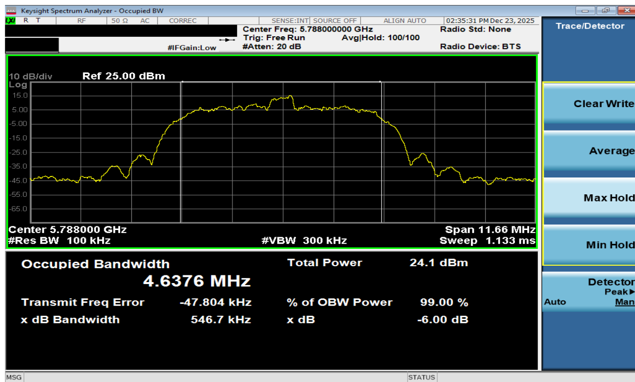
Plot 7-57. 6dB BW Antenna WF8 (NB UNII HDR8, ePA – 5788MHz)
