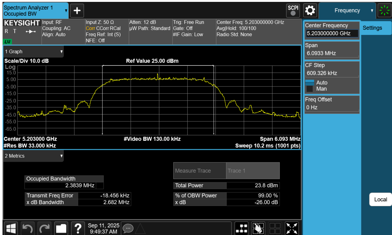
Plot 7-32. 26dB BW Antenna WF7a (NB UNII HDRPS2, ePA- 5203MHz)
