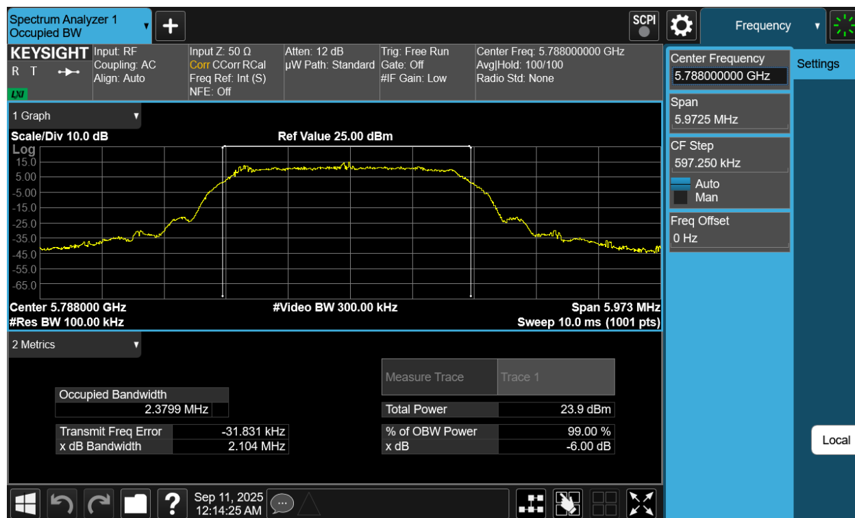
Plot 7-58. 6dB BW Antenna WF8 (NB UNII HDRPS2, ePA – 5788MHz)
