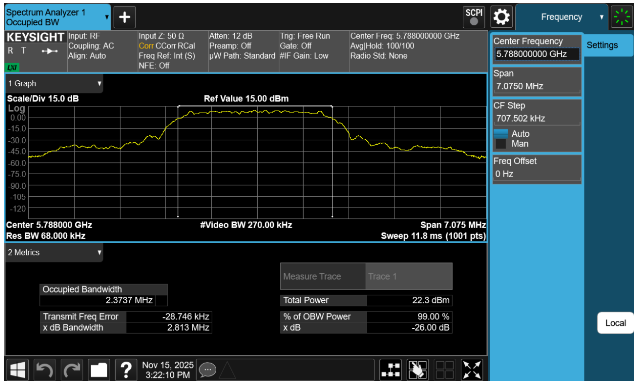
Plot 7-24. 99% OBW Antenna WF8 (NB UNII HDT2, ePA- 5788MHz)
