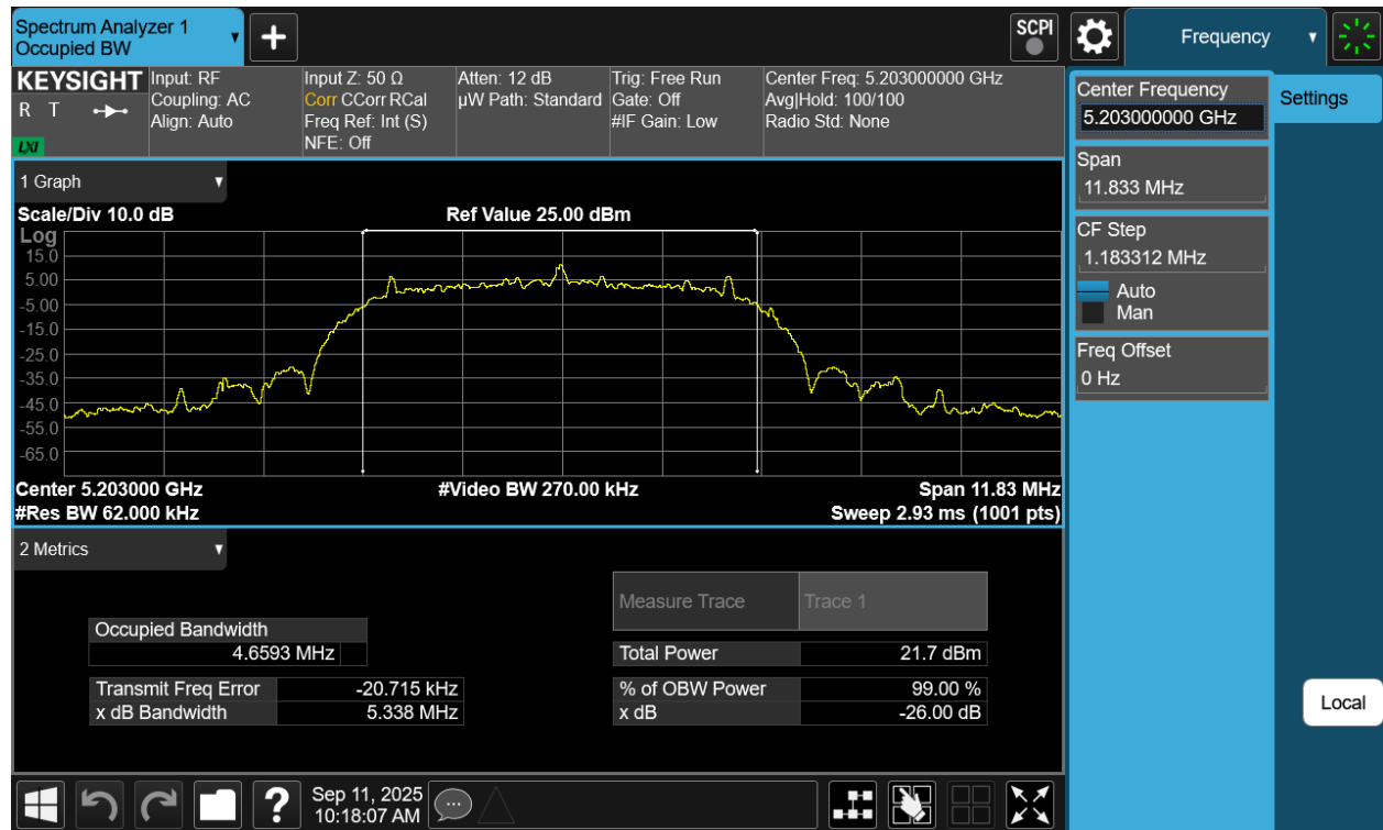
Plot 7-34. 26dB BW Antenna WF7a (NB UNII HDRPM16, ePA- 5203MHz)
