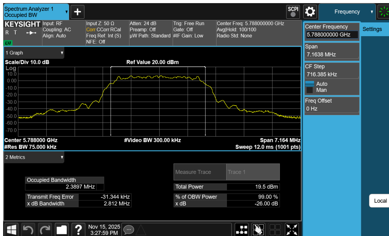
Plot 7-26. 99% OBW Antenna WF8 (NB UNII HDT6, ePA– 5788MHz)
