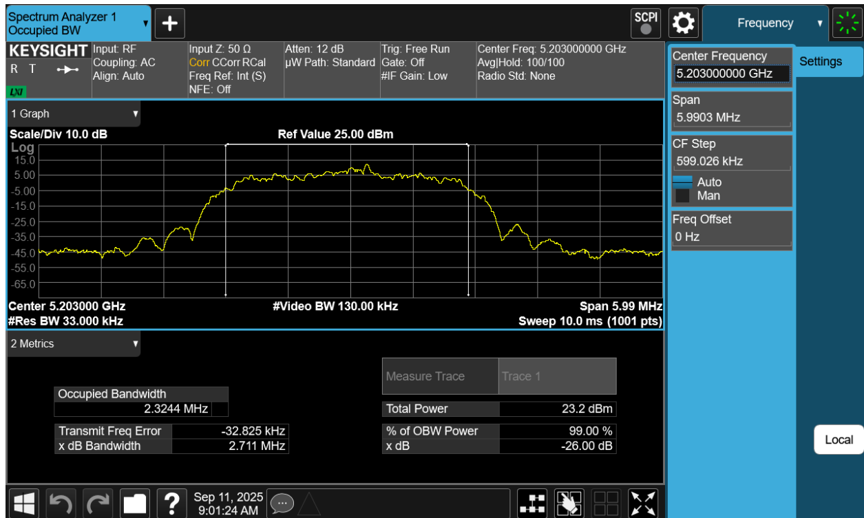
Plot 7-30. 26dB BW Antenna WF7a (NB UNII HDR4, ePA- 5203MHz)
