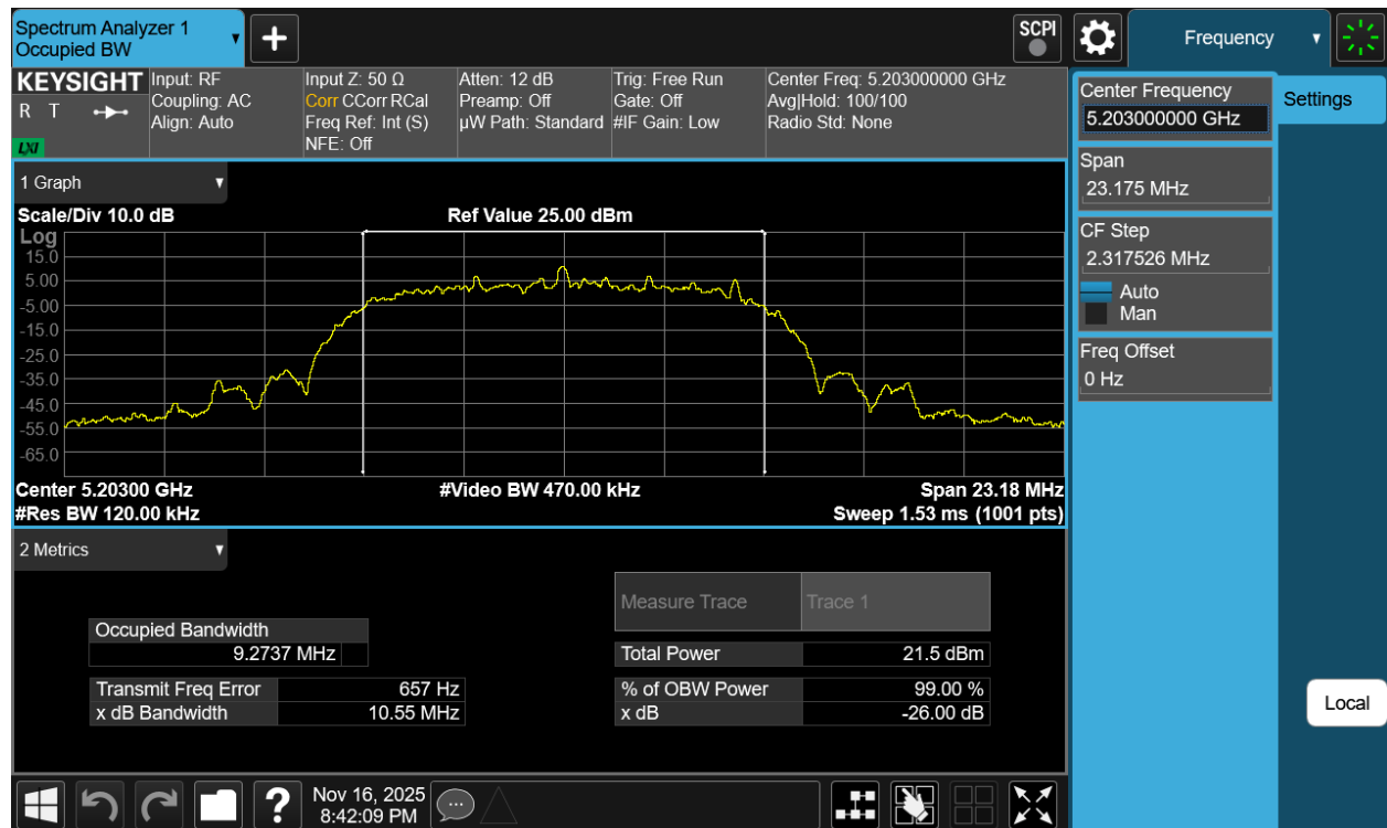
Plot 7-36. 26dB BW Antenna WF7a (NB UNII HDRPL32, ePA- 5203MHz)
