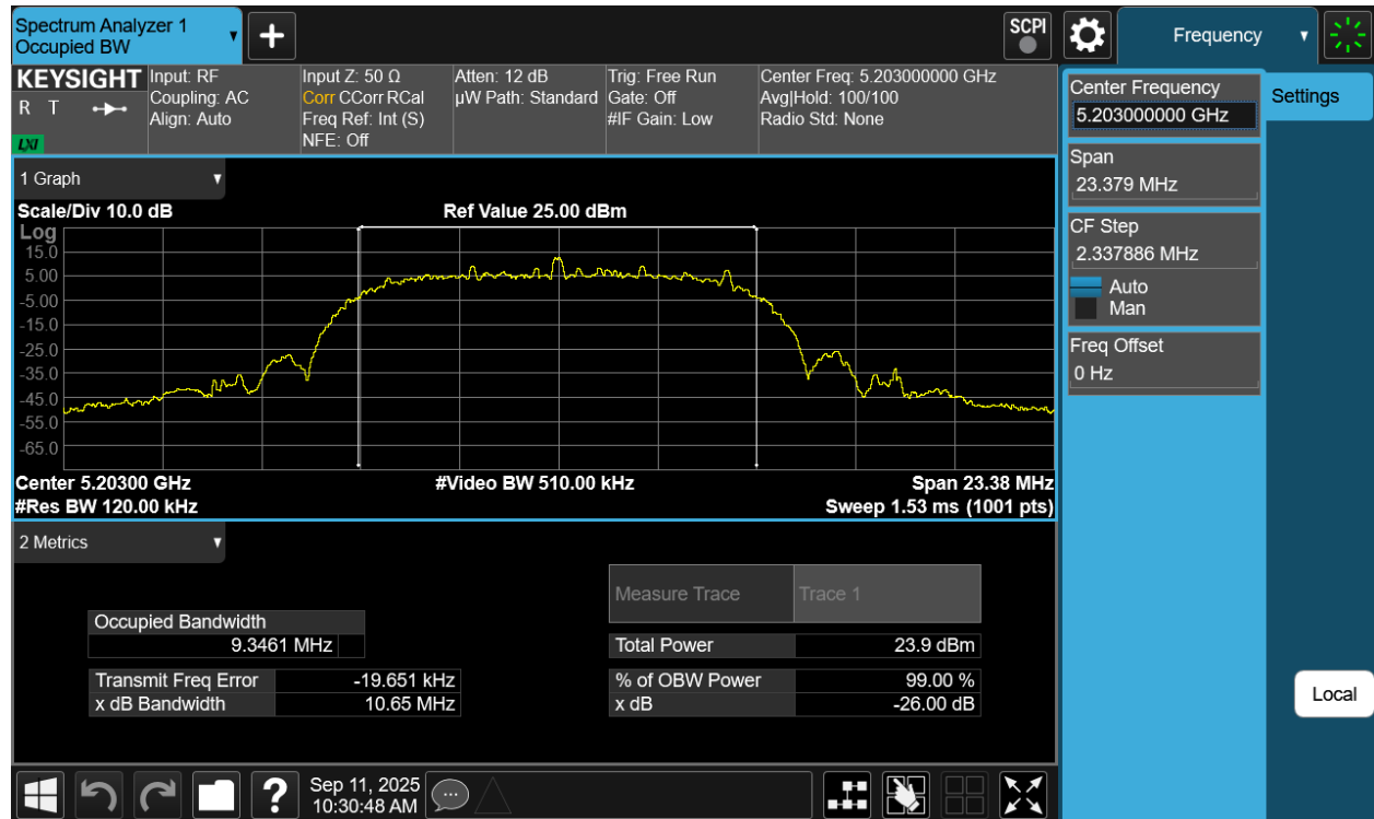
Plot 7-35. 26dB BW Antenna WF7a (NB UNII HDRPL12, ePA- 5203MHz)
