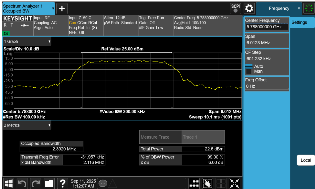
Plot 7-63. 6dB BW Antenna WF8 (NB UNII HDT2, ePA- 5788MHz)
