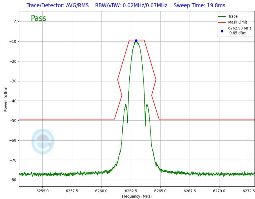
Plot 7-134. In-Band Emission Antenna WF8 (NB UNII LE1M, iPA – 6263MHz)
