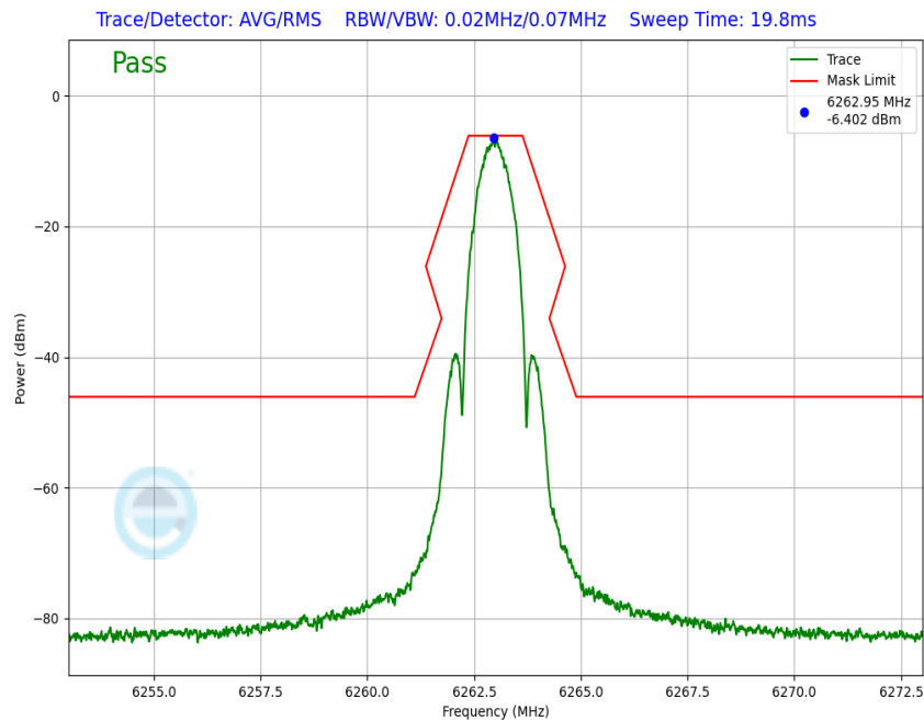
Plot 7-160. In-Band Emission Antenna WF7a (NB UNII LE1M, iPA – 6263MHz)
