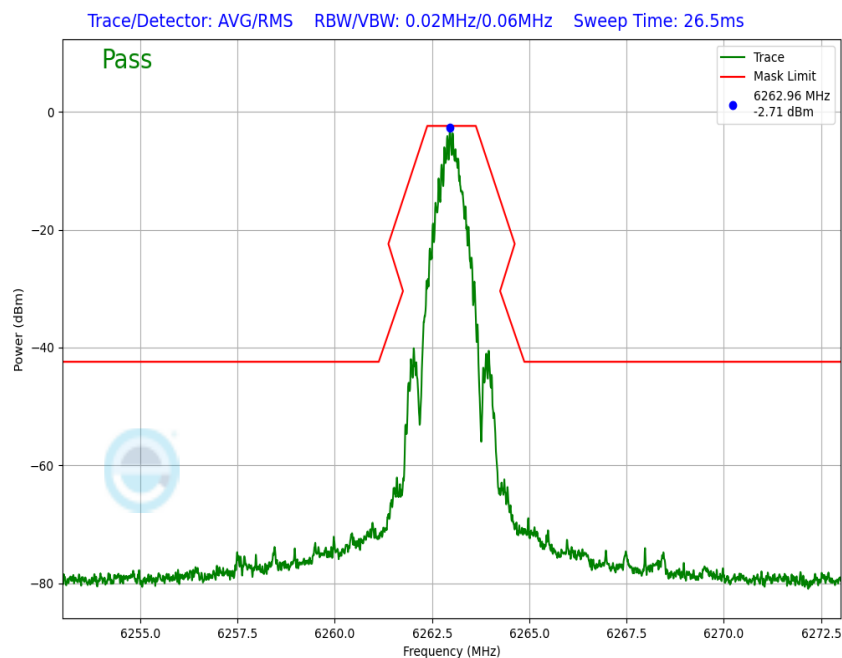
Plot 7-157. In-Band Emission Antenna WF7a (NB UNII BDR, ePA – 6263MHz)
