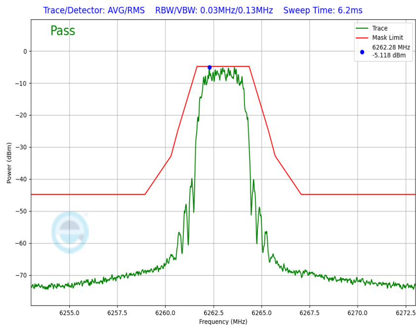
Plot 7-163. In-Band Emission Antenna WF7a (NB UNII HDR4, ePA – 6263MHz)
