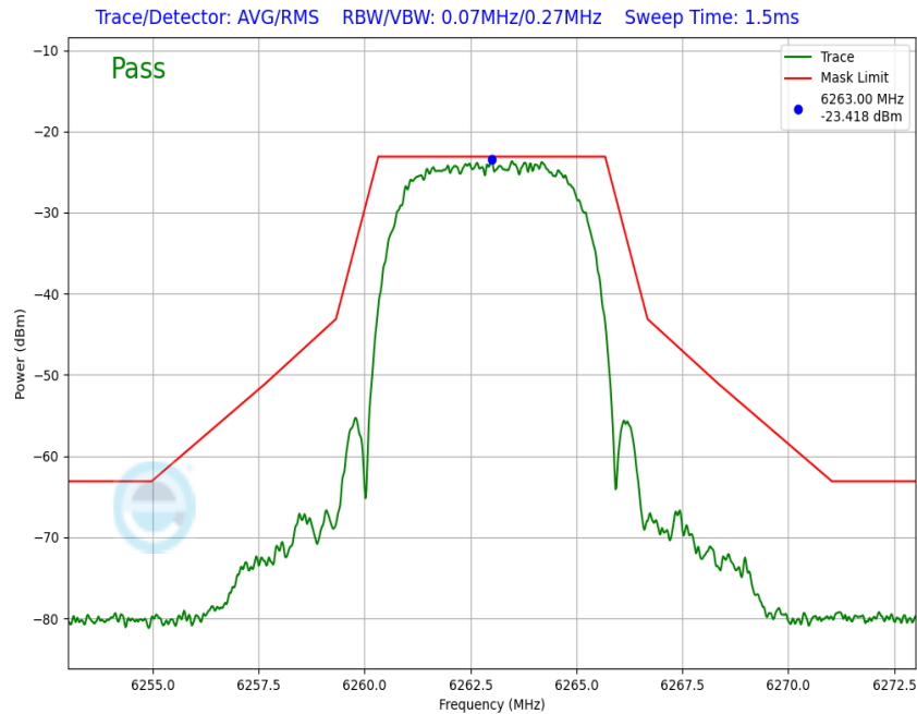
Plot 7-144. In-Band Emission Antenna WF8 (NB UNII XHDRPM6, iPA – 6263MHz)
