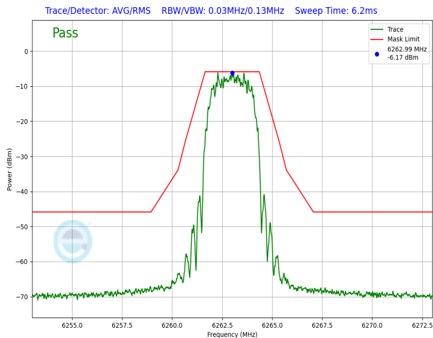
Plot 7-137. In-Band Emission Antenna WF8 (NB UNII HDR4, ePA – 6263MHz)
