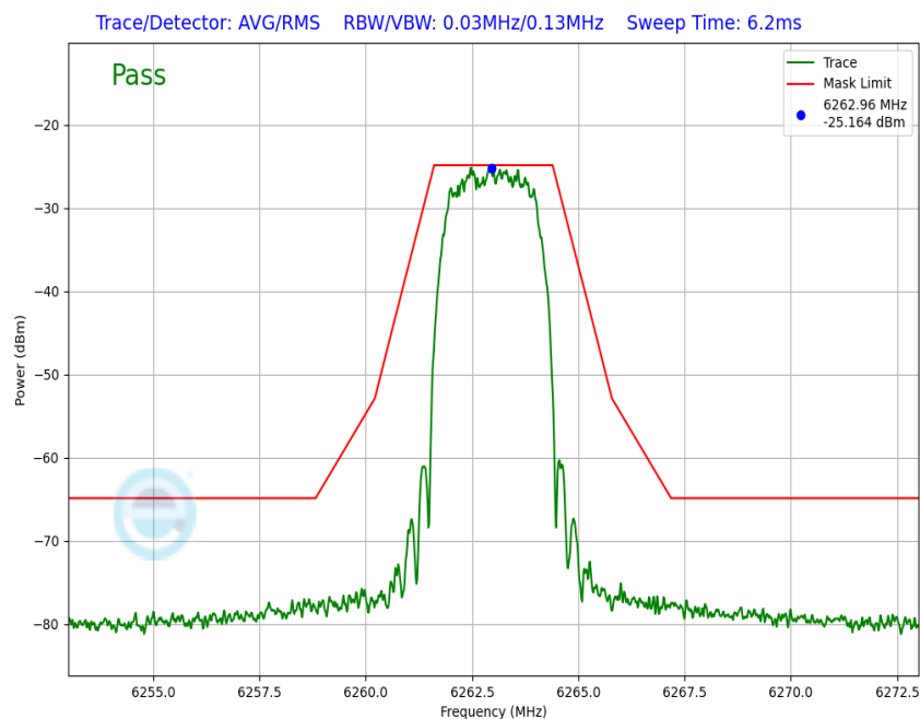
Plot 7-155. In-Band Emission Antenna WF8 (NB UNII HDT6, ePA – 6263MHz)
