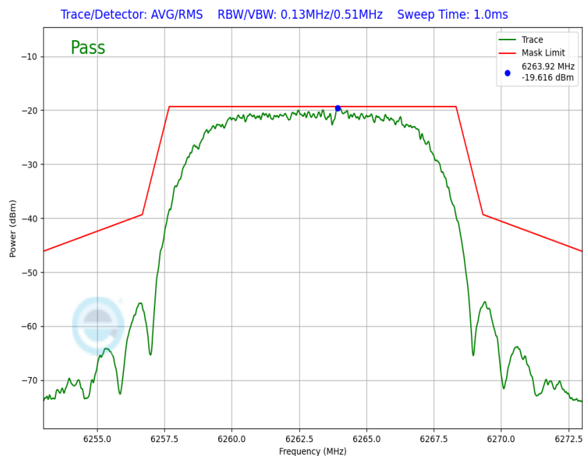
Plot 7-147. In-Band Emission Antenna WF8 (NB UNII HDRPL12, ePA – 6263MHz)
