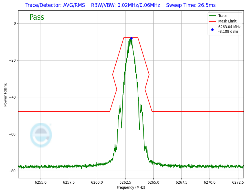
Plot 7-132. In-Band Emission Antenna WF8 (NB UNII BDR, iPA – 6263MHz)
