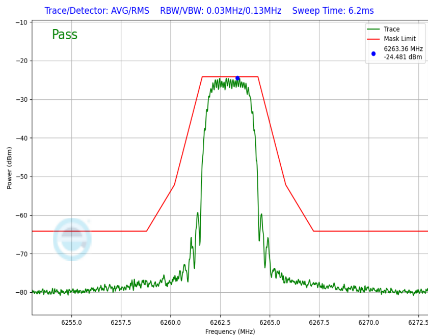
Plot 7-153. In-Band Emission Antenna WF8 (NB UNII HDT4, ePA – 6263MHz)
