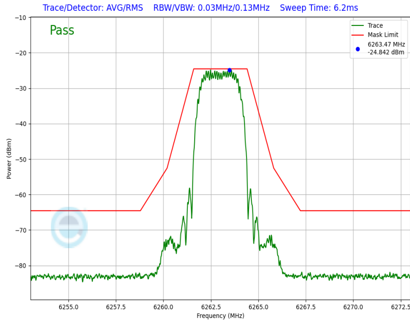
Plot 7-154. In-Band Emission Antenna WF8 (NB UNII HDT4, iPA – 6263MHz)
