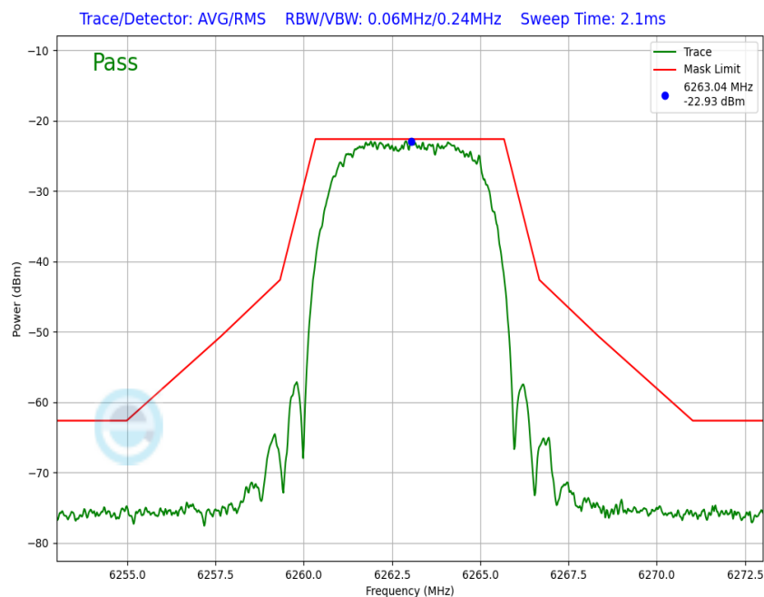
Plot 7-171. In-Band Emission Antenna WF7a (NB UNII HDRPM16, ePA – 6263MHz)
