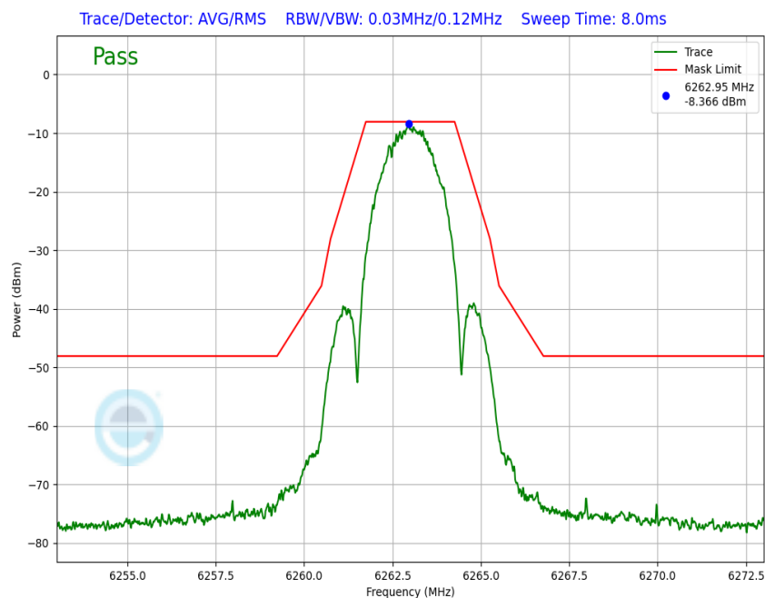
Plot 7-135. In-Band Emission Antenna WF8 (NB UNII LE2M, ePA – 6263MHz)
