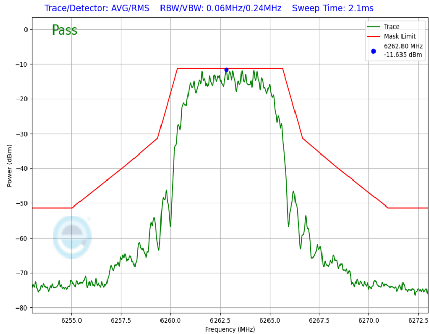
Plot 7-166. In-Band Emission Antenna WF7a (NB UNII HDR8, iPA – 6263MHz)
