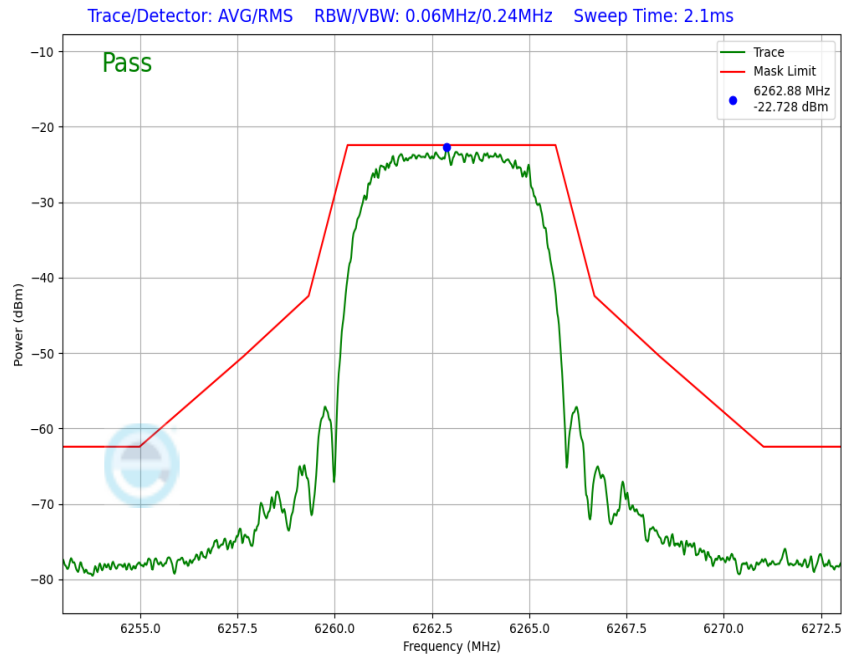
Plot 7-172. In-Band Emission Antenna WF7a (NB UNII HDRPM16, iPA – 6263MHz)
