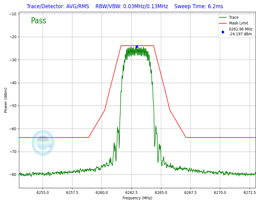
Plot 7-151. In-Band Emission Antenna WF8 (NB UNII HDT2, ePA – 6263MHz)
