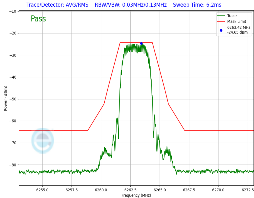
Plot 7-152. In-Band Emission Antenna WF8 (NB UNII HDT2, iPA – 6263MHz)
