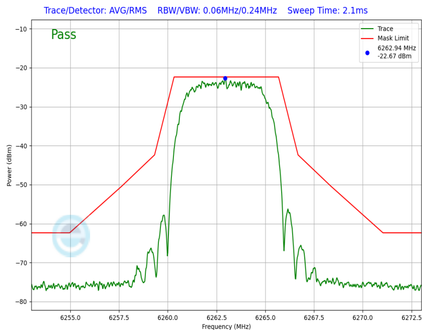
Plot 7-169. In-Band Emission Antenna WF7a (NB UNII XHDRPM6, ePA – 6263MHz)
