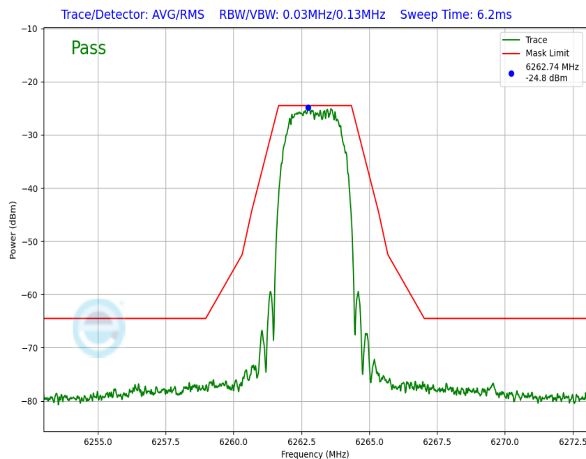
Plot 7-167. In-Band Emission Antenna WF7a (NB UNII HDRPS2, ePA – 6263MHz)
