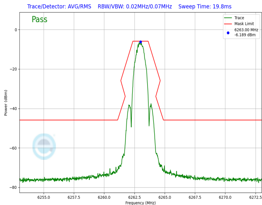
Plot 7-133. In-Band Emission Antenna WF8 (NB UNII LE1M, ePA – 6263MHz)
