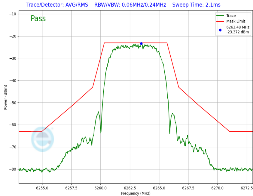
Plot 7-170. In-Band Emission Antenna WF7a (NB UNII XHDRPM6, iPA – 6263MHz)
