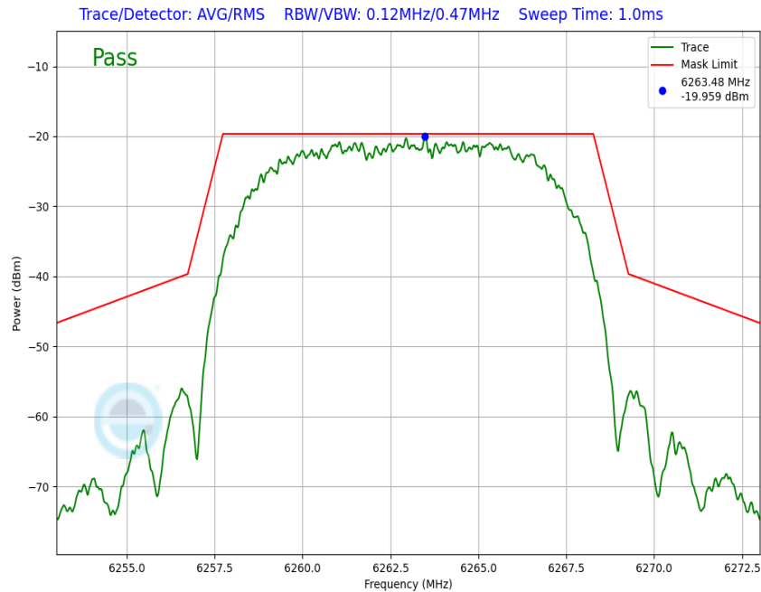
Plot 7-150. In-Band Emission Antenna WF8 (NB UNII HDRPL32, iPA – 6263MHz)
