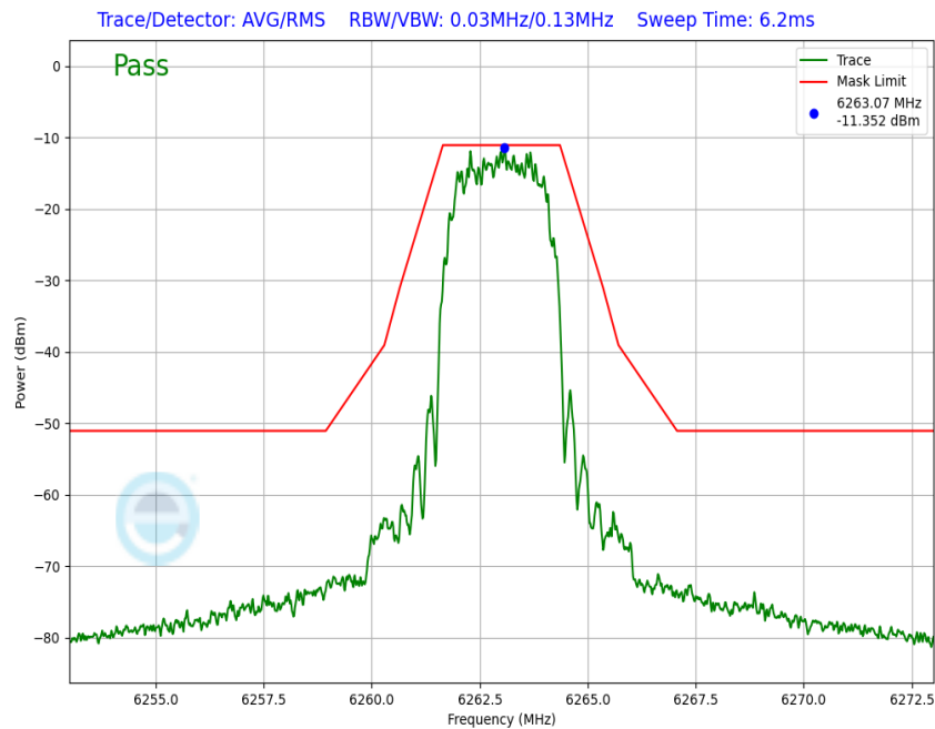
Plot 7-164. In-Band Emission Antenna WF7a (NB UNII HDR4, iPA – 6263MHz)
