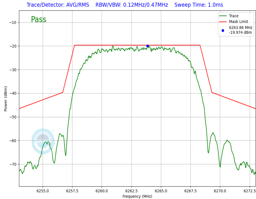
Plot 7-174. In-Band Emission Antenna WF7a (NB UNII HDRPL12, iPA – 6263MHz)
