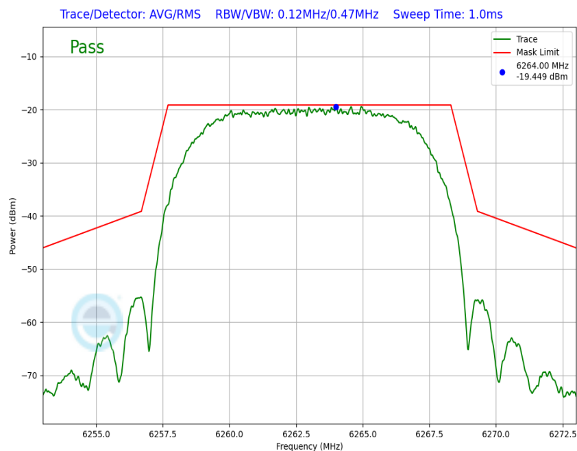
Plot 7-173. In-Band Emission Antenna WF7a (NB UNII HDRPL12, ePA – 6263MHz)
