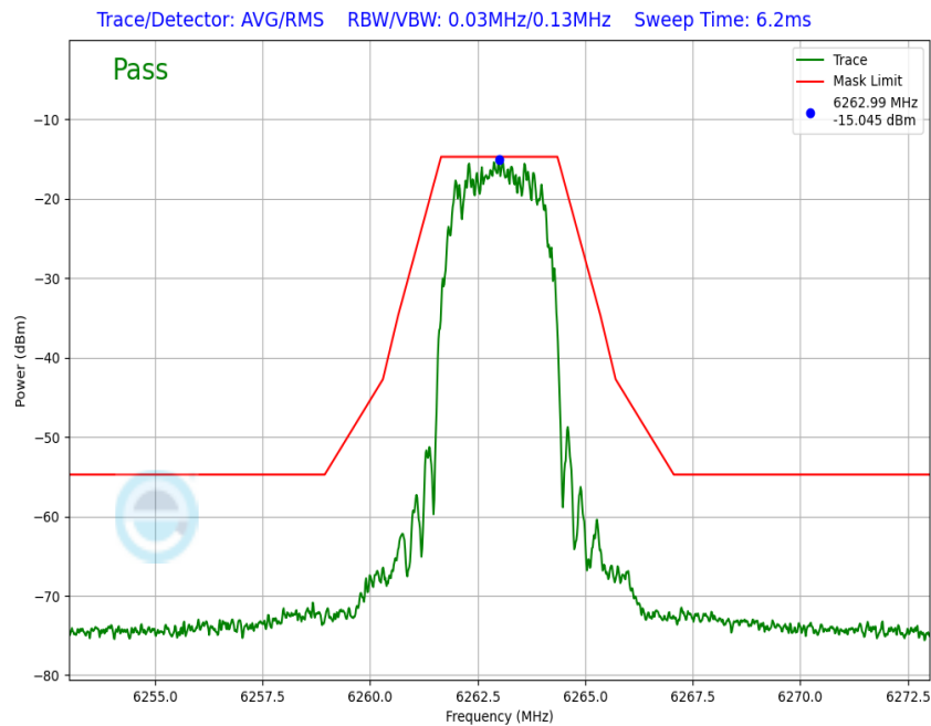
Plot 7-138. In-Band Emission Antenna WF8 (NB UNII HDR4, iPA – 6263MHz)
