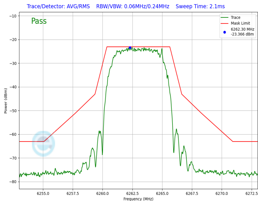
Plot 7-145. In-Band Emission Antenna WF8 (NB UNII HDRPM16, ePA – 6263MHz)
