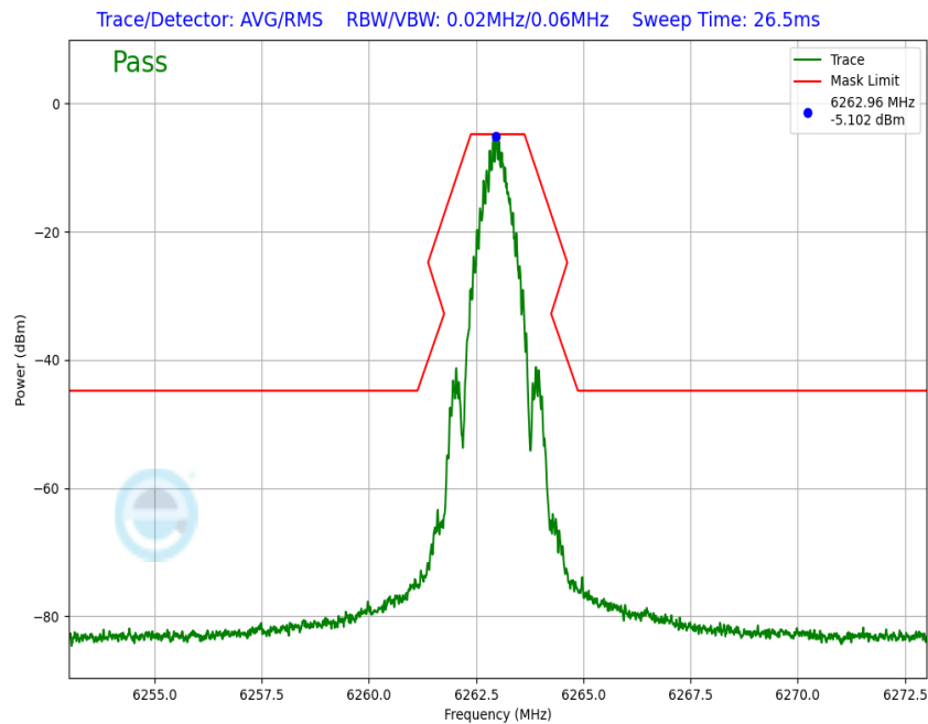
Plot 7-158. In-Band Emission Antenna WF7a (NB UNII BDR, iPA – 6263MHz)
