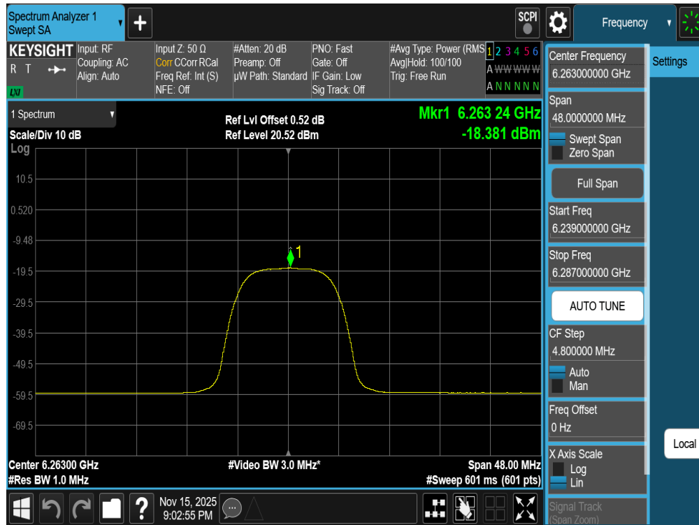
Plot 7-115. PSD TxBF Antenna WF8 (NB UNII HDRPL32, ePA – 6263MHz)
