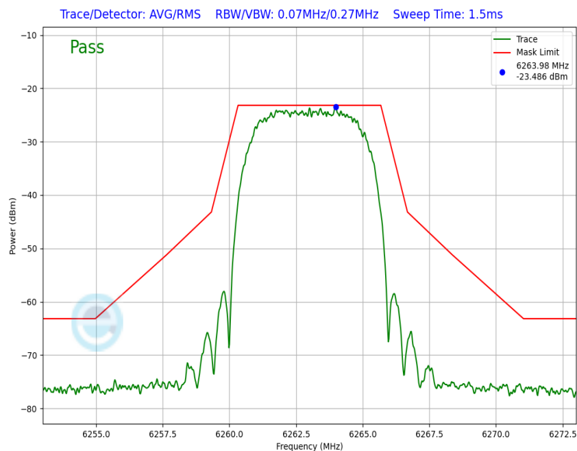
Plot 7-143. In-Band Emission Antenna WF8 (NB UNII XHDRPM6, ePA – 6263MHz)
