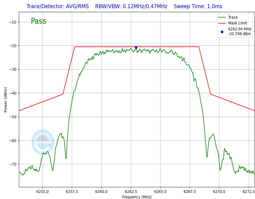
Plot 7-149. In-Band Emission Antenna WF8 (NB UNII HDRPL32, ePA – 6263MHz)
