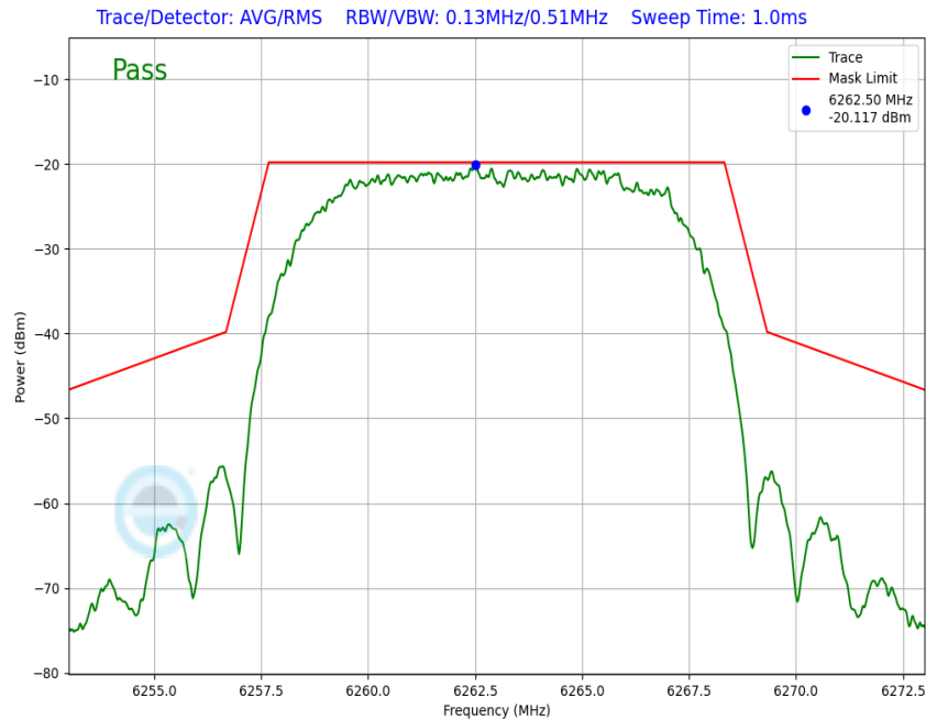
Plot 7-148. In-Band Emission Antenna WF8 (NB UNII HDRPL12, iPA – 6263MHz)
