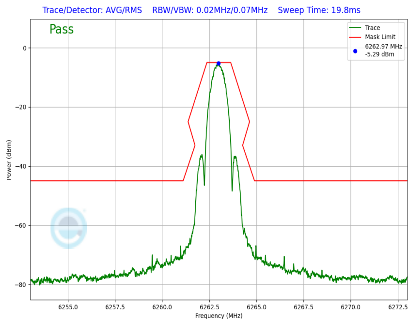
Plot 7-159. In-Band Emission Antenna WF7a (NB UNII LE1M, ePA – 6263MHz)
