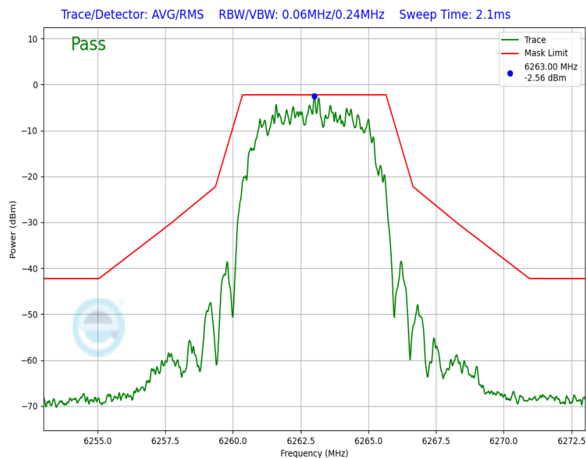
Plot 7-139. In-Band Emission Antenna WF8 (NB UNII HDR8, ePA – 6263MHz)
