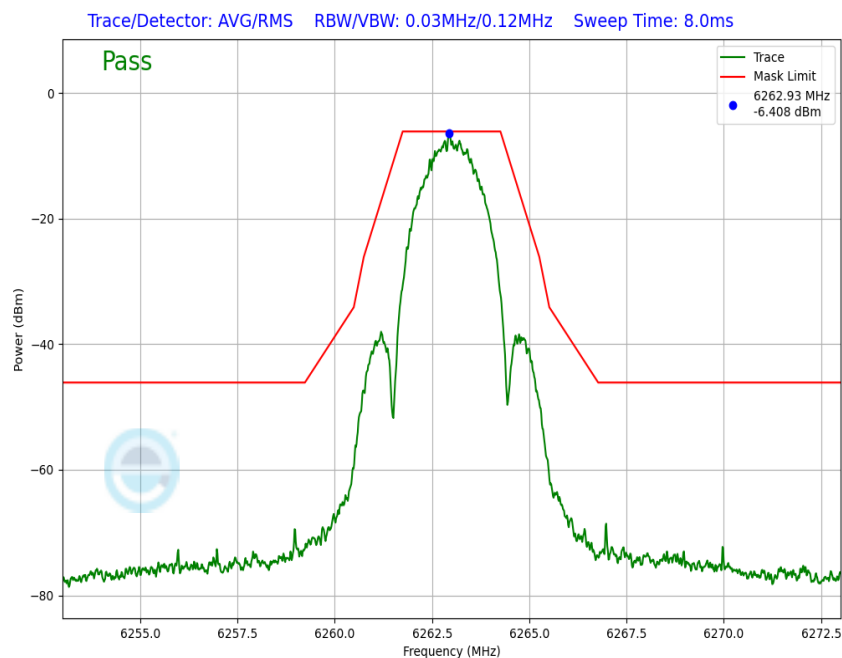
Plot 7-161. In-Band Emission Antenna WF7a (NB UNII LE2M, ePA – 6263MHz)
