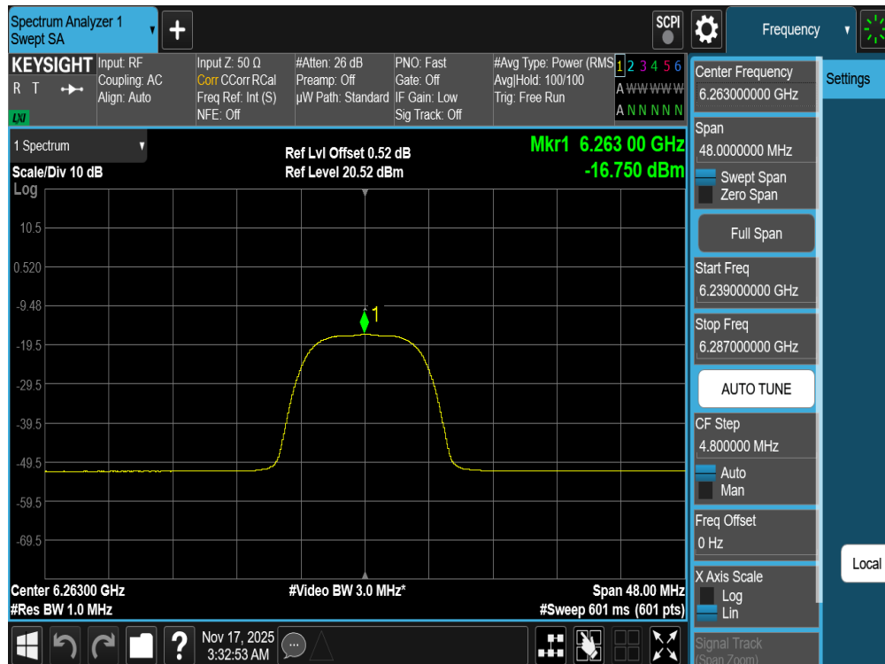
Plot 7-116. PSD TxBF Antenna WF7a (NB UNII HDRPL32, ePA – 6263MHz)
