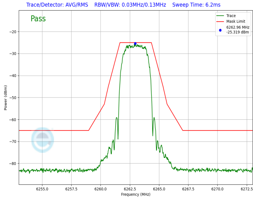
Plot 7-142. In-Band Emission Antenna WF8 (NB UNII HDRPS2, iPA – 6263MHz)
