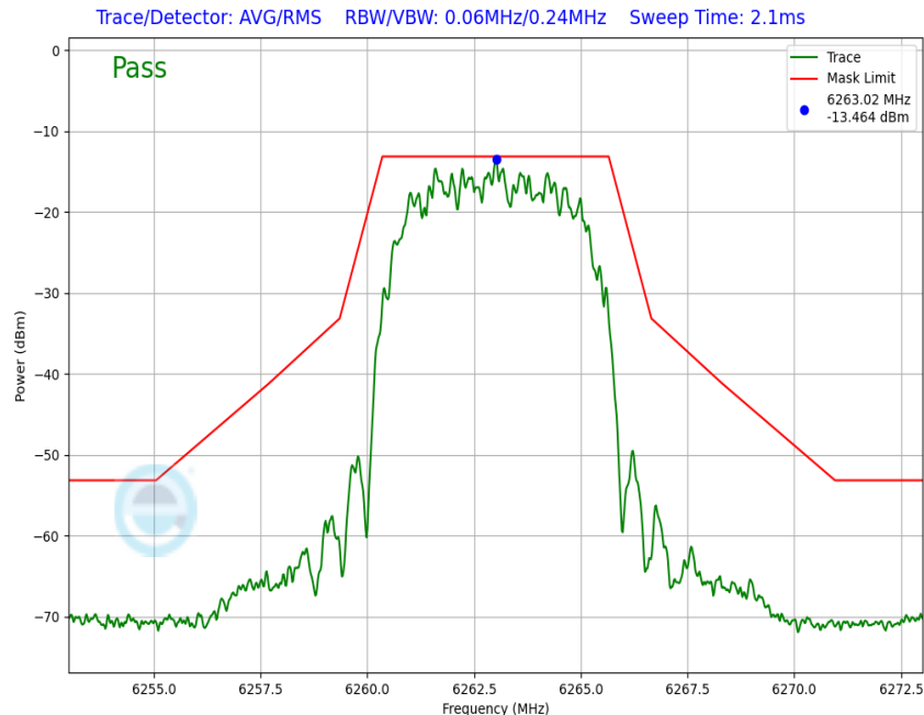
Plot 7-140. In-Band Emission Antenna WF8 (NB UNII HDR8, iPA – 6263MHz)
