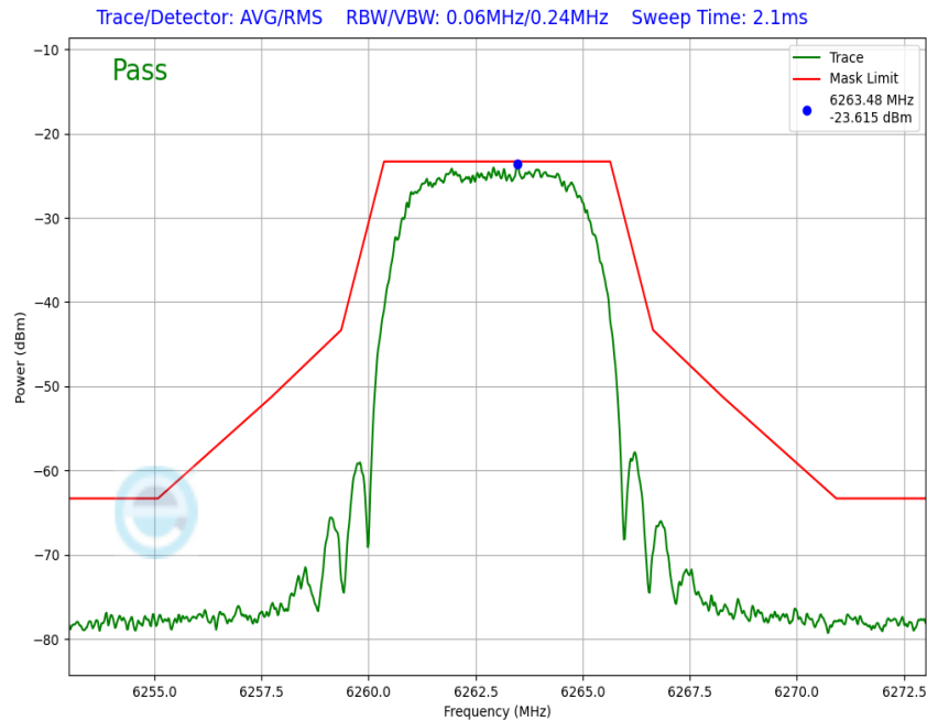
Plot 7-146. In-Band Emission Antenna WF8 (NB UNII HDRPM16, iPA – 6263MHz)
