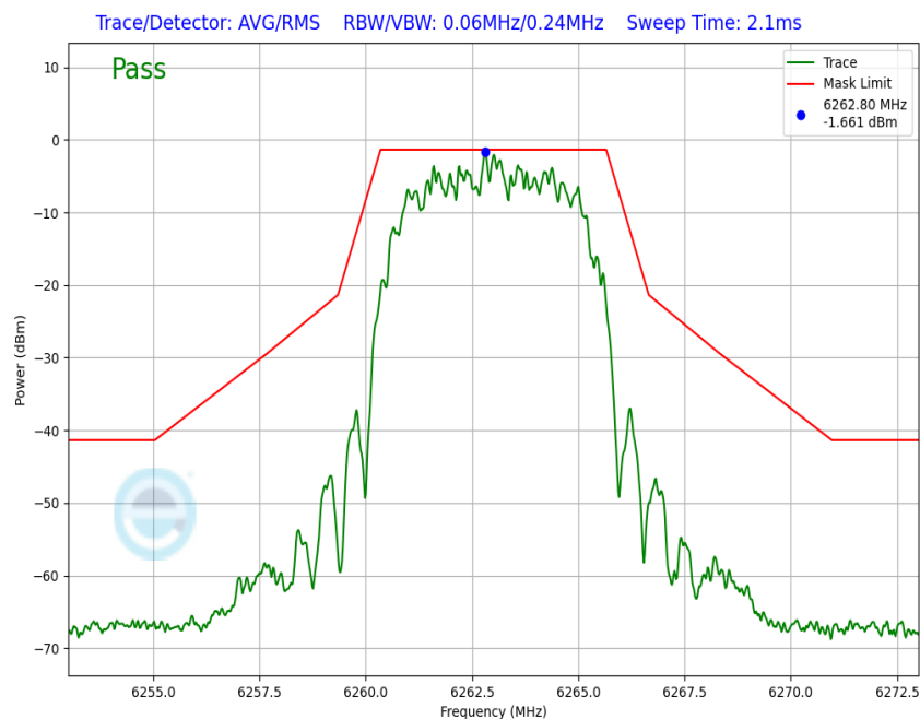
Plot 7-165. In-Band Emission Antenna WF7a (NB UNII HDR8, ePA – 6263MHz)
