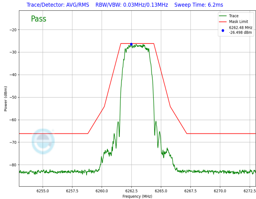
Plot 7-156. In-Band Emission Antenna WF8 (NB UNII HDT6, iPA – 6263MHz)
