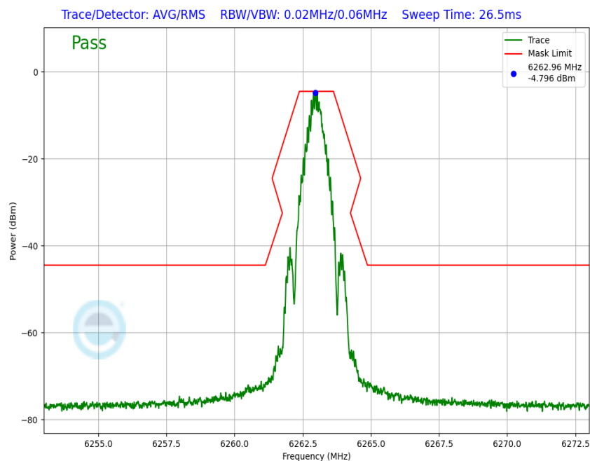
Plot 7-131. In-Band Emission Antenna WF8 (NB UNII BDR, ePA – 6263MHz)
