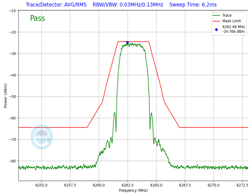
Plot 7-168. In-Band Emission Antenna WF7a (NB UNII HDRPS2, iPA – 6263MHz)
