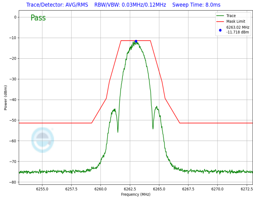
Plot 7-136. In-Band Emission Antenna WF8 (NB UNII LE2M, iPA – 6263MHz)
