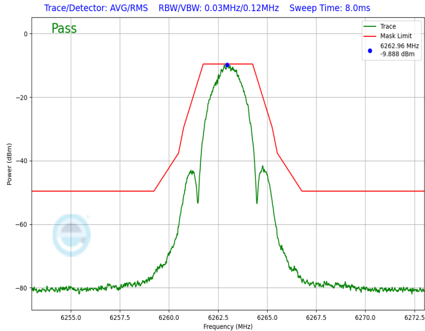
Plot 7-162. In-Band Emission Antenna WF7a (NB UNII LE2M, iPA – 6263MHz)
