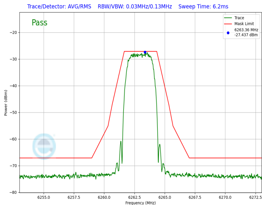
Plot 7-141. In-Band Emission Antenna WF8 (NB UNII HDRPS2, ePA – 6263MHz)
