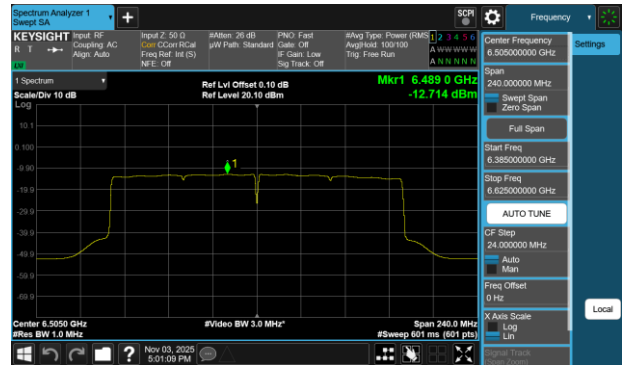
Plot 7-56 PSD Antenna WF7a (160MHz BW 802.11be(SU) - Ch.111)
