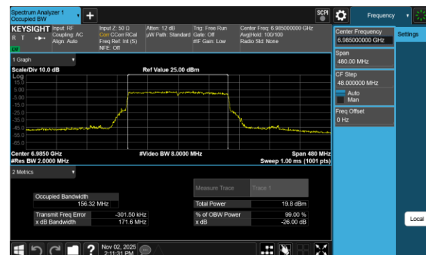
Plot 7-16 26dB BW & 99% OBW Antenna WF8 (160MHz BW 802.11be(SU) - Ch.207)
