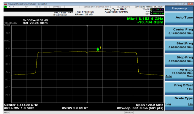
Plot 7-71 PSD CDD Antenna WF7a (80MHz BW 802.11be(SU) - Ch.39)
