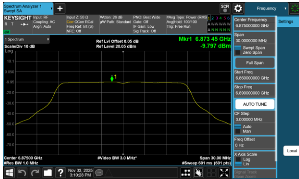
Plot 7-57 PSD Antenna WF7a (20MHz BW 802.11a - Ch.185)
