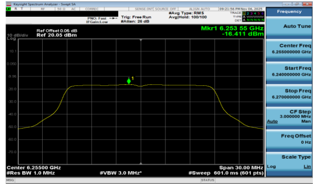
Plot 7-69 PSD CDD Antenna WF7a (20MHz BW 802.11a - Ch.61)
