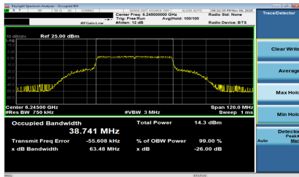
Plot 7-18 26dB BW & 99% OBW Antenna WF7a (40MHz BW 802.11be(SU) - Ch.59)
