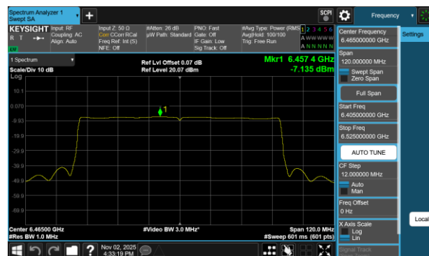
Plot 7-39 PSD Antenna WF8 (80MHz BW 802.11be(SU) - Ch.103)
