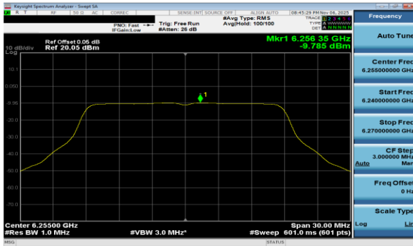
Plot 7-49 PSD Antenna WF7a (20MHz BW 802.11a - Ch.61)
