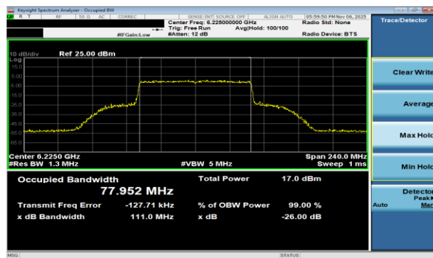
Plot 7-3 26dB BW & 99% OBW Antenna WF8 (80MHz BW 802.11be(SU) - Ch.55)
