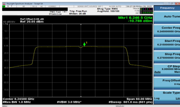
Plot 7-34 PSD Antenna WF8 (40MHz BW 802.11be(SU) - Ch.59)
