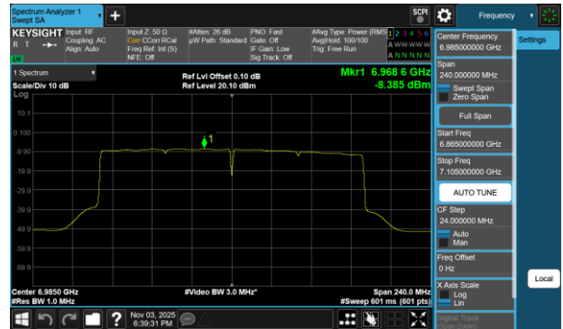
Plot 7-64 PSD Antenna WF7a (160MHz BW 802.11be(SU) - Ch.207)
