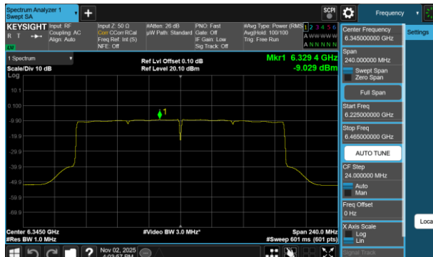
Plot 7-36 PSD Antenna WF8 (160MHz BW 802.11be(SU) - Ch.79)
