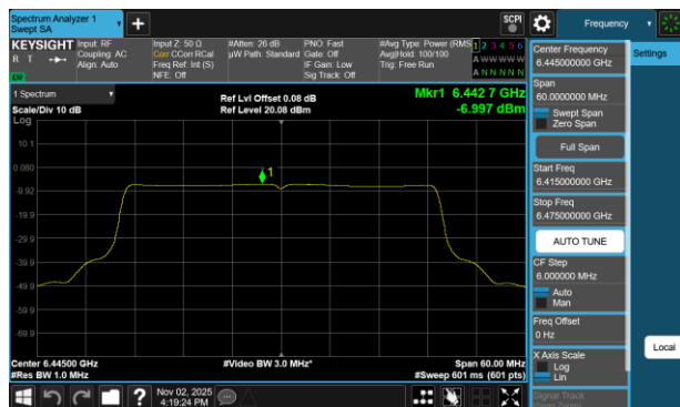
Plot 7-38 PSD Antenna WF8 (40MHz BW 802.11be(SU) - Ch.99)
