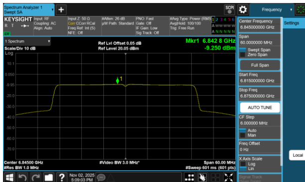
Plot 7-42 PSD Antenna WF8 (40MHz BW 802.11be(SU) - Ch.179)
