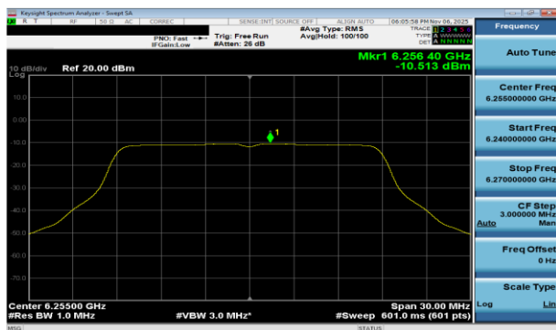
Plot 7-33 PSD Antenna WF8 (20MHz BW 802.11a - Ch.61)
