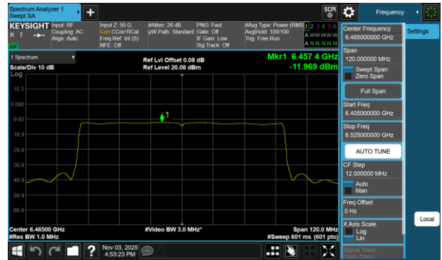
Plot 7-55 PSD Antenna WF7a (80MHz BW 802.11be(SU) - Ch.103)
