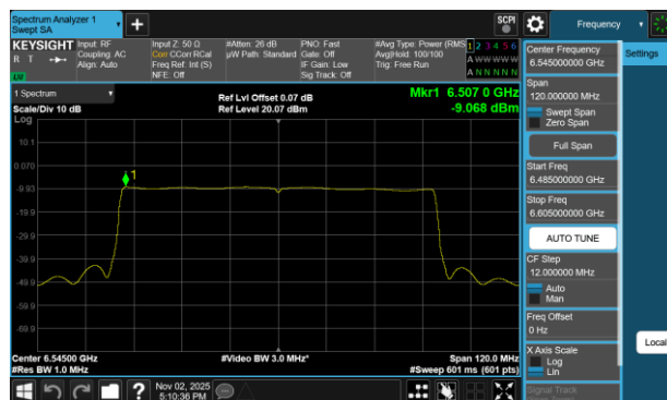
Plot 7-43 PSD Antenna WF8 (80MHz BW 802.11be(SU) - Ch.119)
