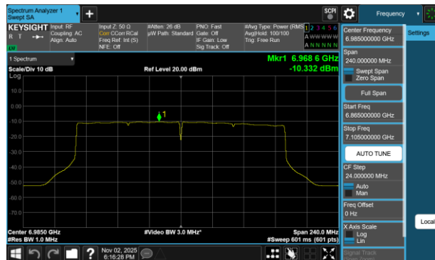
Plot 7-48 PSD Antenna WF8 (160MHz BW 802.11be(SU) - Ch.207)
