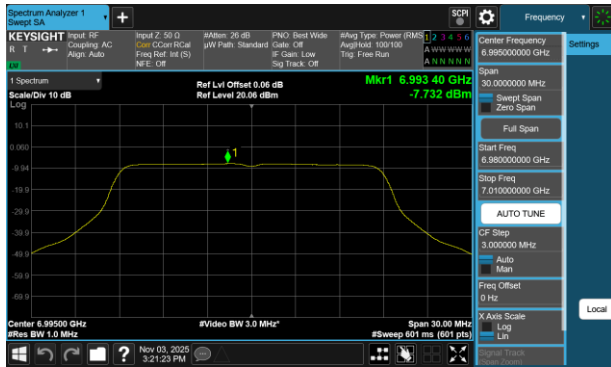
Plot 7-61 PSD Antenna WF7a (20MHz BW 802.11a - Ch.209)
