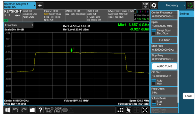
Plot 7-59 PSD Antenna WF7a (80MHz BW 802.11be(SU) - Ch.183)
