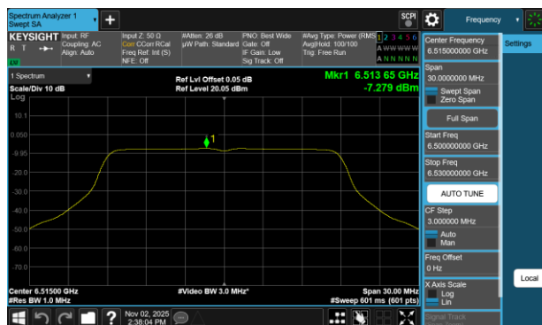
Plot 7-37 PSD Antenna WF8 (20MHz BW 802.11a - Ch.113)
