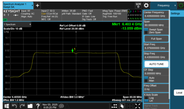
Plot 7-70 PSD CDD Antenna WF7a (40MHz BW 802.11be(SU) - Ch.91)
