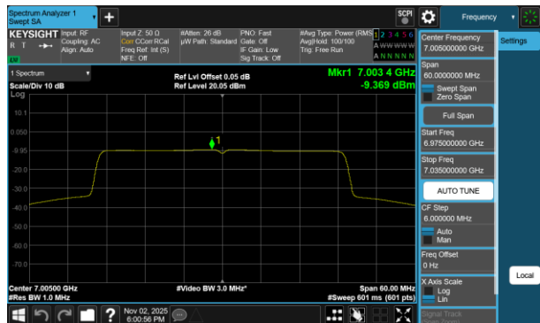
Plot 7-46 PSD Antenna WF8 (40MHz BW 802.11be(SU) - Ch.211)
