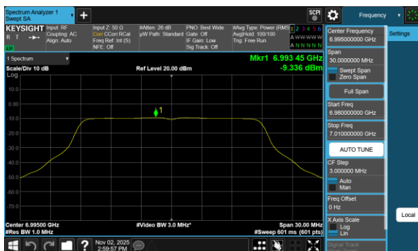
Plot 7-45 PSD Antenna WF8 (20MHz BW 802.11a - Ch.209)
