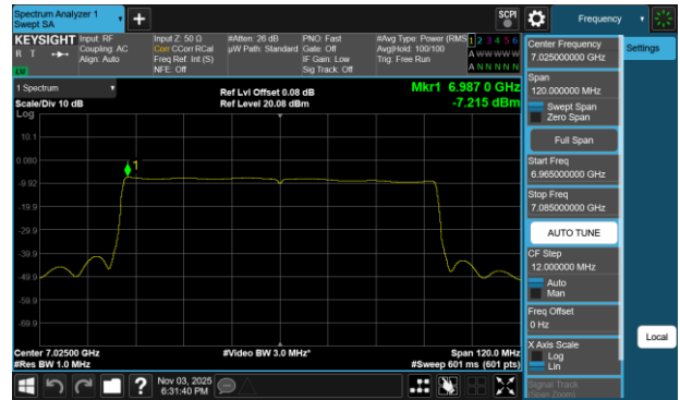
Plot 7-63 PSD Antenna WF7a (80MHz BW 802.11be(SU) - Ch.215)
