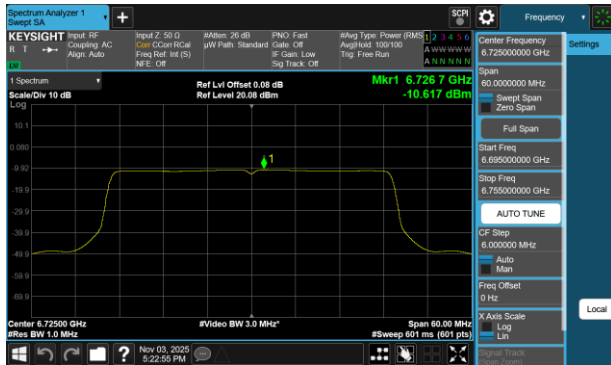
Plot 7-58 PSD Antenna WF7a (40MHz BW 802.11be(SU) - Ch.155)
