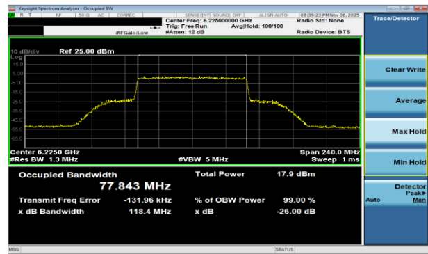
Plot 7-19 26dB BW & 99% OBW Antenna WF7a (80MHz BW 802.11be(SU) - Ch.55)
