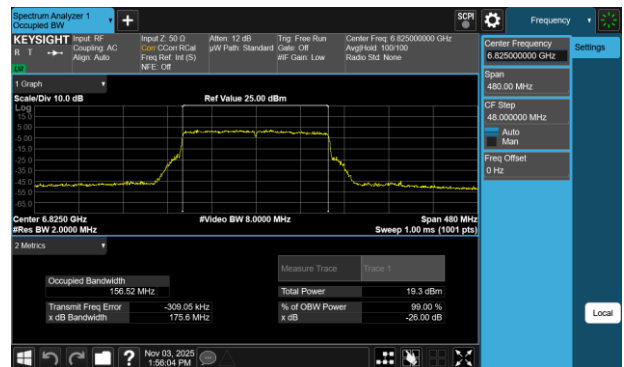
Plot 7-28 26dB BW & 99% OBW Antenna WF7a (160MHz BW 802.11be(SU) - Ch.175)
