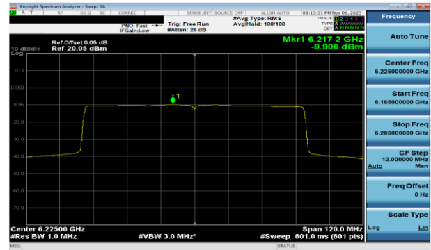
Plot 7-51 PSD Antenna WF7a (80MHz BW 802.11be(SU) - Ch.55)
