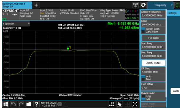
Plot 7-53 PSD Antenna WF7a (20MHz BW 802.11be(SU) - Ch.97)
