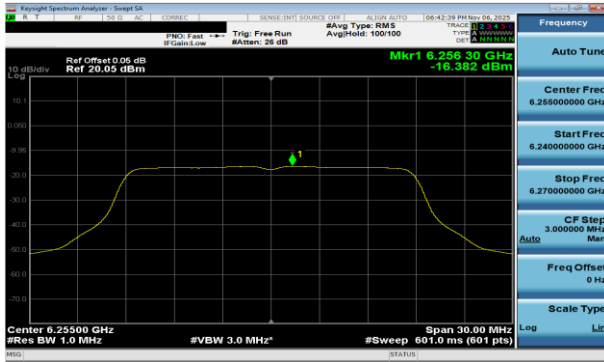
Plot 7-65 PSD CDD Antenna WF8 (20MHz BW 802.11a - Ch.61)
