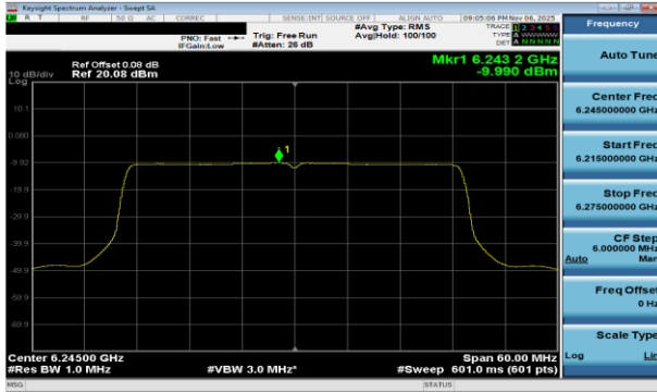
Plot 7-50 PSD Antenna WF7a (40MHz BW 802.11be(SU) - Ch.59)
