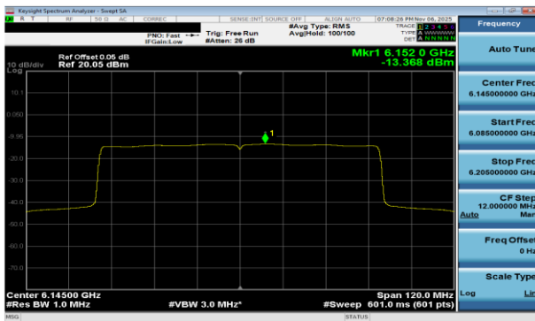
Plot 7-67 PSD CDD Antenna WF8 (80MHz BW 802.11be(SU) - Ch.39)
