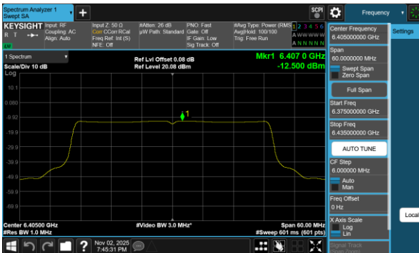
Plot 7-66 PSD CDD Antenna WF8 (40MHz BW 802.11be(SU) - Ch.91)
