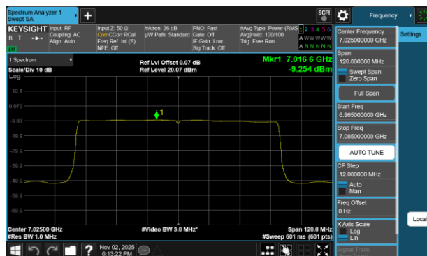
Plot 7-47 PSD Antenna WF8 (80MHz BW 802.11be(SU) - Ch.215)
