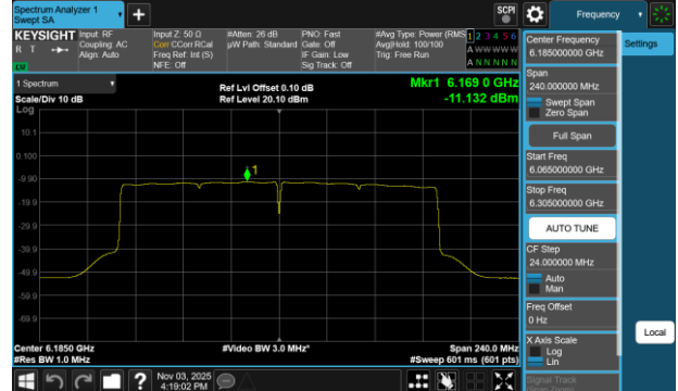
Plot 7-52 PSD Antenna WF7a (160MHz BW 802.11be(SU) - Ch.47)
