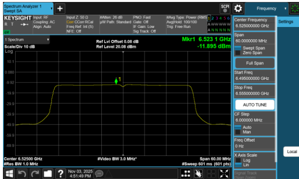
Plot 7-54 PSD Antenna WF7a (40MHz BW 802.11be(SU) - Ch.115)
