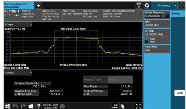
Plot 7-32 26dB BW & 99% OBW Antenna WF7a (160MHz BW 802.11be(SU) - Ch.207)
