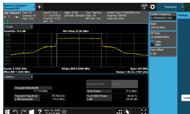
Plot 7-11 26dB BW & 99% OBW Antenna WF8 (80MHz BW 802.11be(SU) - Ch.151)
