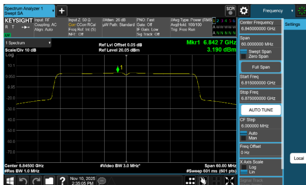
Plot 7-66 PSD Antenna WF8 (40MHz BW 802.11be(SU) - Ch.179)
