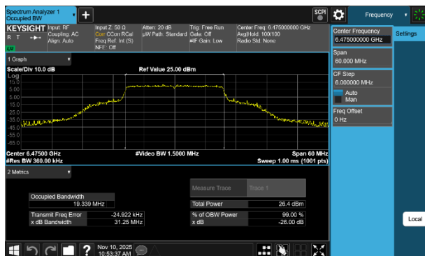
Plot 7-5 26dB BW & 99% OBW Antenna WF8 (20MHz BW 802.11be(SU) - Ch.105)
