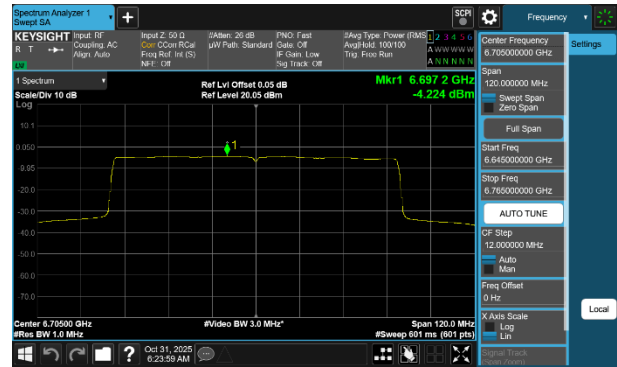
Plot 7-79 PSD Antenna WF8 (80MHz BW 802.11be(SU) - Ch.151)
