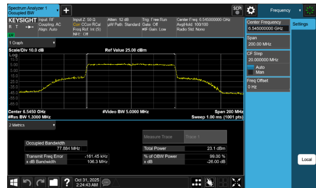
Plot 7-23 26dB BW & 99% OBW Antenna WF8 (80MHz BW 802.11be(SU) - Ch.119)
