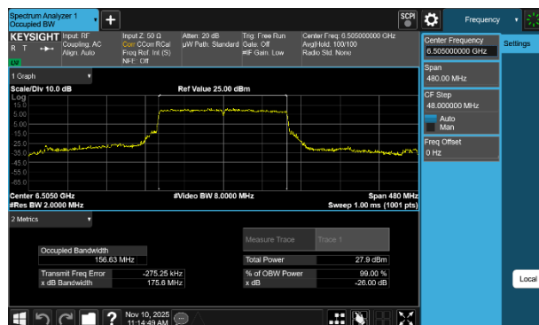
Plot 7-8 26dB BW & 99% OBW Antenna WF8 (160MHz BW 802.11be(SU) - Ch.111)
