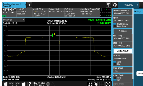
Plot 7-68 PSD Antenna WF8 (160MHz BW 802.11be(SU) - Ch.143)
