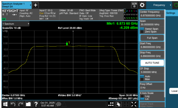
Plot 7-77 PSD Antenna WF8 (20MHz BW 802.11be(SU) - Ch.185)
