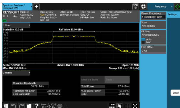
Plot 7-2 26dB BW & 99% OBW Antenna WF8 (40MHz BW 802.11be(SU) - Ch.3)
