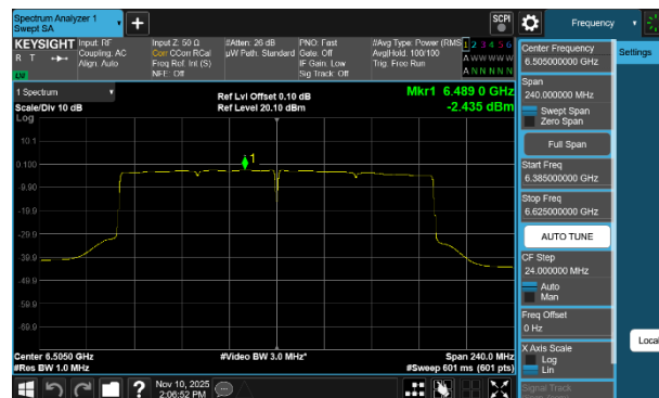
Plot 7-64 PSD Antenna WF8 (160MHz BW 802.11be(SU) - Ch.111)
