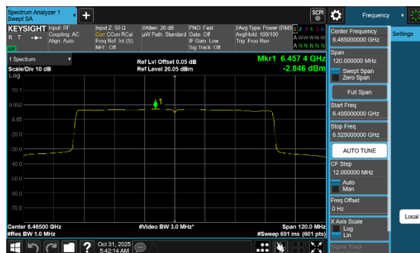
Plot 7-75 PSD Antenna WF8 (80MHz BW 802.11be(SU) - Ch.103)
