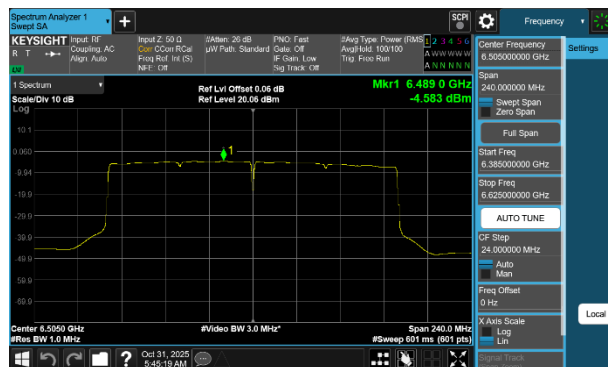
Plot 7-76 PSD Antenna WF8 (160MHz BW 802.11be(SU) - Ch.111)
