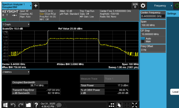
Plot 7-46 26dB BW & 99% OBW Antenna WF7a (40MHz BW 802.11be(SU) - Ch.99)
