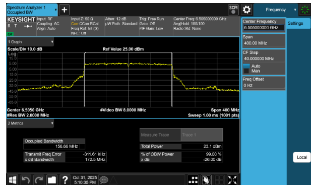
Plot 7-48 26dB BW & 99% OBW Antenna WF7a (160MHz BW 802.11be(SU) - Ch.111)
