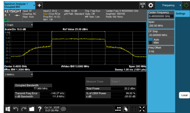
Plot 7-47 26dB BW & 99% OBW Antenna WF7a (80MHz BW 802.11be(SU) - Ch.103)
