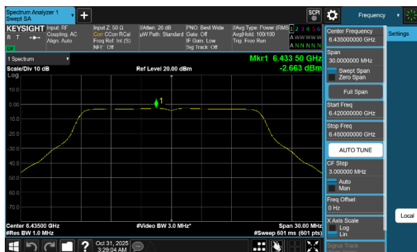
Plot 7-73 PSD Antenna WF8 (20MHz BW 802.11a - Ch.97)
