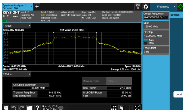
Plot 7-6 26dB BW & 99% OBW Antenna WF8 (40MHz BW 802.11be(SU) - Ch.107)
