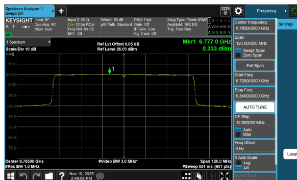
Plot 7-67 PSD Antenna WF8 (80MHz BW 802.11be(SU) - Ch.167)
