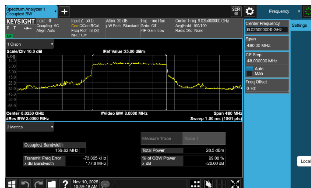
Plot 7-4 26dB BW & 99% OBW Antenna WF8 (160MHz BW 802.11be(SU) - Ch.15)
