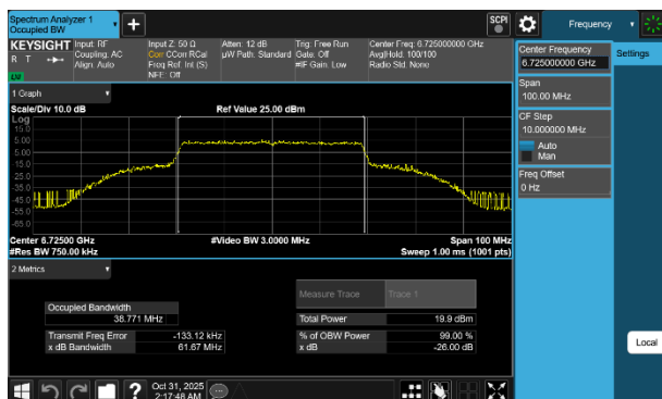
Plot 7-22 26dB BW & 99% OBW Antenna WF8 (40MHz BW 802.11be(SU) - Ch.155)
