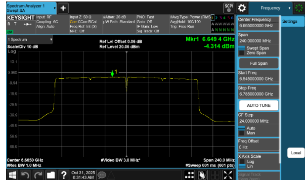
Plot 7-80 PSD Antenna WF8 (160MHz BW 802.11be(SU) - Ch.143)
