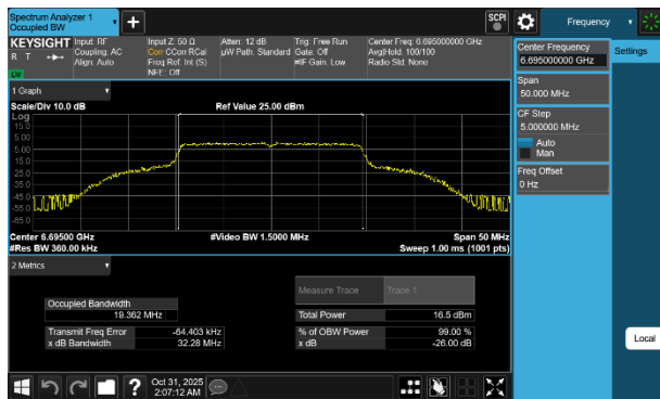
Plot 7-21 26dB BW & 99% OBW Antenna WF8 (20MHz BW 802.11be(SU) - Ch.149)
