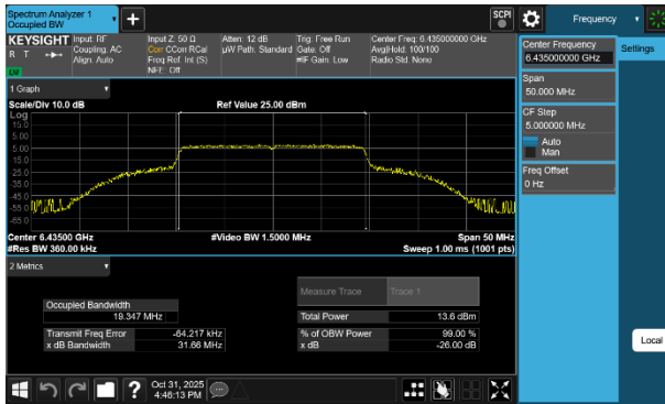
Plot 7-45 26dB BW & 99% OBW Antenna WF7a (20MHz BW 802.11be(SU) - Ch.97)
