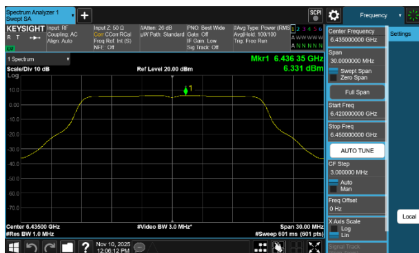
Plot 7-61 PSD Antenna WF8 (20MHz BW 802.11a - Ch.97)
