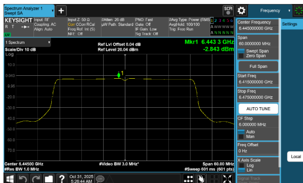
Plot 7-74 PSD Antenna WF8 (40MHz BW 802.11be(SU) - Ch.99)
