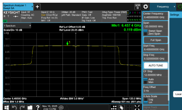
Plot 7-63 PSD Antenna WF8 (80MHz BW 802.11be(SU) - Ch.103)
