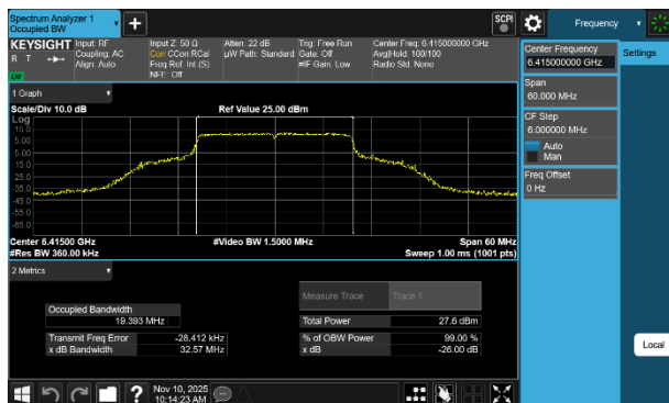
Plot 7-1 26dB BW & 99% OBW Antenna WF8 (20MHz BW 802.11be(SU) - Ch.93)
