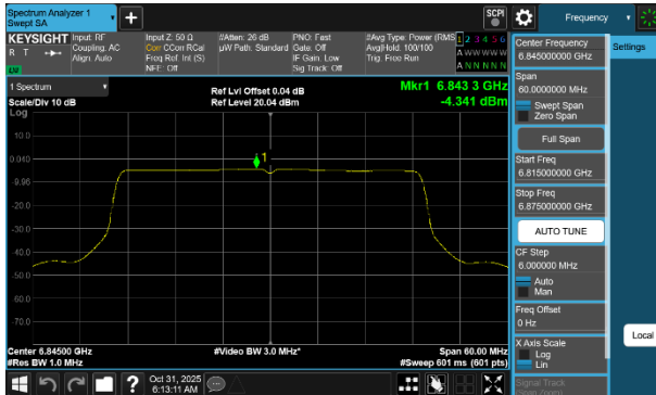
Plot 7-78 PSD Antenna WF8 (40MHz BW 802.11be(SU) - Ch.179)
