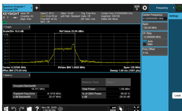
Plot 7-57 26dB BW & 99% OBW Antenna WF7a (40MHz BW 802.11be(RU) RU26 Index8 - Ch.115)
