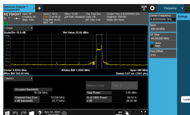
Plot 7-26 26dB BW & 99% OBW Antenna WF8 (160MHz BW 802.11be(RU) RU26 Index36 - Ch.175)
