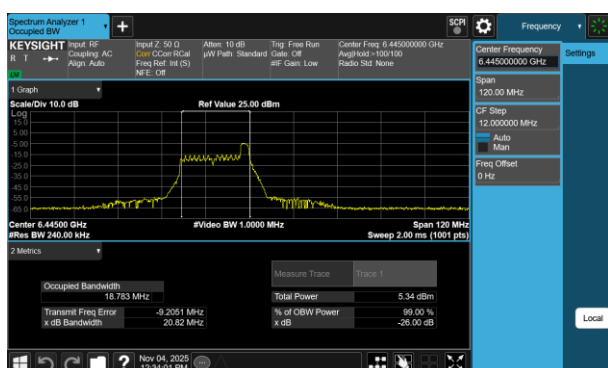
Plot 7-13 26dB BW & 99% OBW Antenna WF8 (40MHz BW 802.11be(RU) RU26 Index8 - Ch.99)
