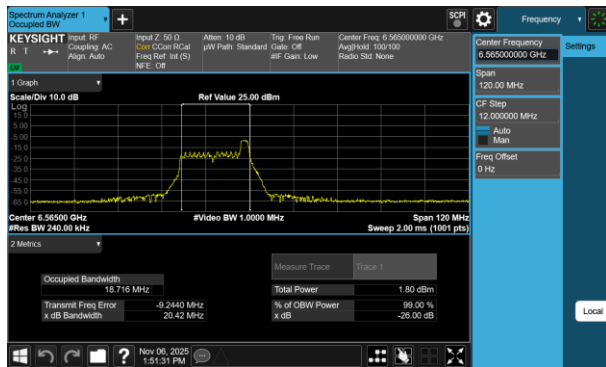
Plot 7-68 26dB BW & 99% OBW Antenna WF7a (40MHz BW 802.11be(RU) RU26 Index8 - Ch.123)
