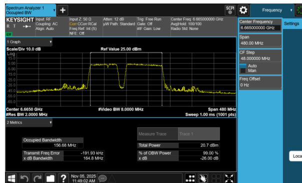
Plot 7-29 26dB BW & 99% OBW Antenna WF8 (160MHz BW 802.11be(RU) RU996+484+242 Index99 - Ch.143)
