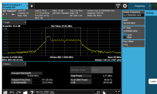
Plot 7-1 26dB BW & 99% OBW Antenna WF8 (20MHz BW 802.11be(RU) RU26 Index0 - Ch.93)
