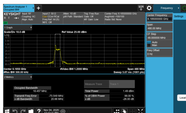
Plot 7-4 26dB BW & 99% OBW Antenna WF8 (160MHz BW 802.11be(RU) RU26 Index0 - Ch.47)
