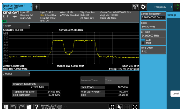
Plot 7-28 26dB BW & 99% OBW Antenna WF8 (80MHz BW 802.11be(RU) RU484+242 Index91 - Ch.183)
