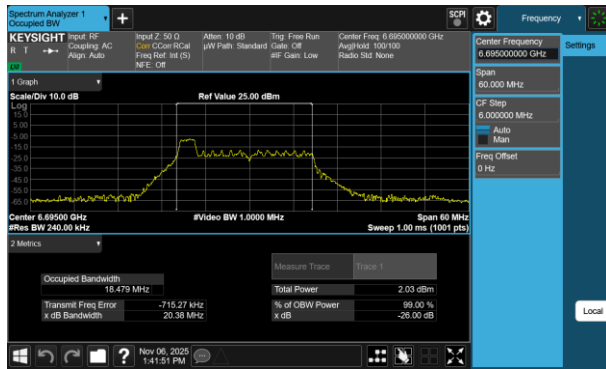
Plot 7-67 26dB BW & 99% OBW Antenna WF7a (20MHz BW 802.11be(RU) RU26 Index0 - Ch.149)
