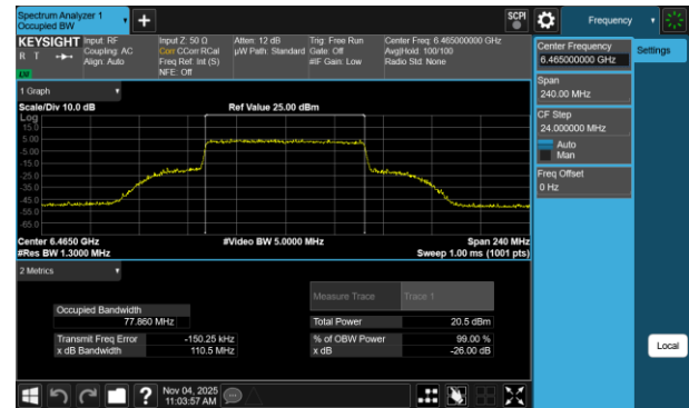
Plot 7-21 26dB BW & 99% OBW Antenna WF8 (80MHz BW 802.11be(RU) RU996 Index67 - Ch.103)
