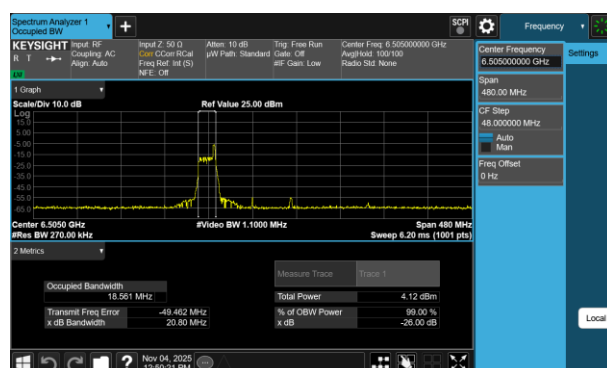
Plot 7-15 26dB BW & 99% OBW Antenna WF8 (160MHz BW 802.11be(RU) RU26 Index17 - Ch.111)
