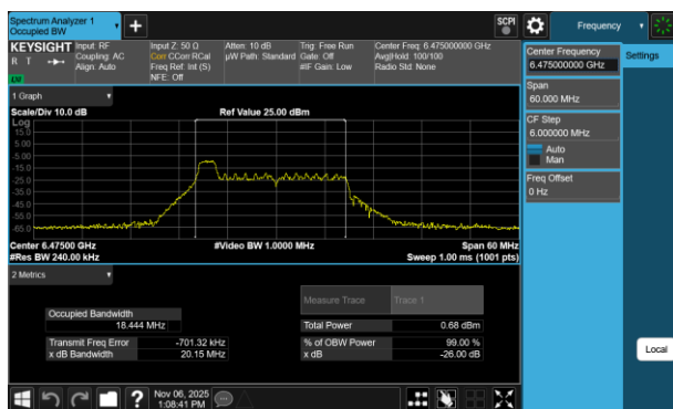
Plot 7-56 26dB BW & 99% OBW Antenna WF7a (20MHz BW 802.11be(RU) RU26 Index0 - Ch.105)
