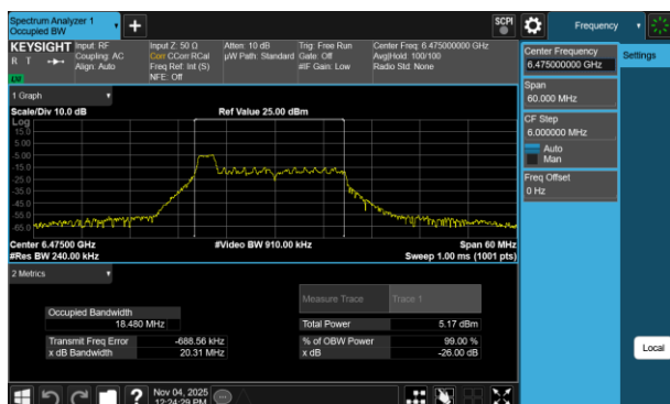
Plot 7-12 26dB BW & 99% OBW Antenna WF8 (20MHz BW 802.11be(RU) RU26 Index0 - Ch.105)
