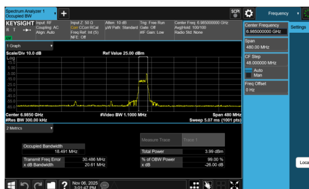
Plot 7-81 26dB BW & 99% OBW Antenna WF7a (160MHz BW 802.11be(RU) RU26 Index17 - Ch.207)
