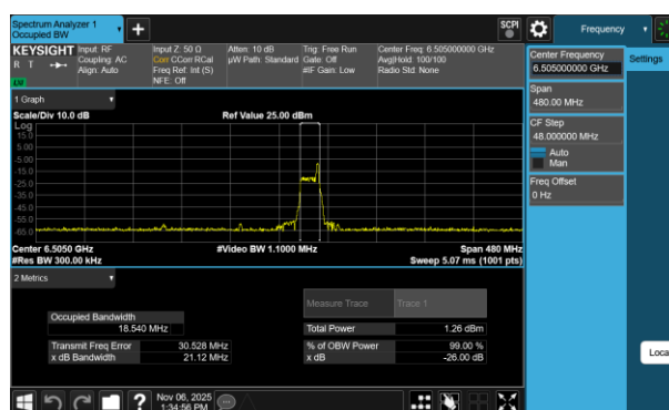
Plot 7-59 26dB BW & 99% OBW Antenna WF7a (160MHz BW 802.11be(RU) RU26 Index17 - Ch.111)
