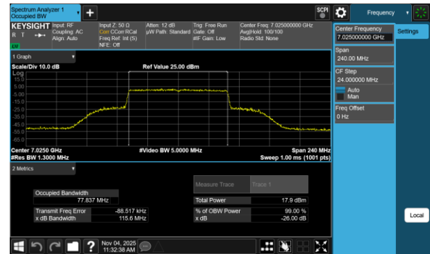
Plot 7-43 26dB BW & 99% OBW Antenna WF8 (80MHz BW 802.11be(RU) RU996 Index67 - Ch.215)
