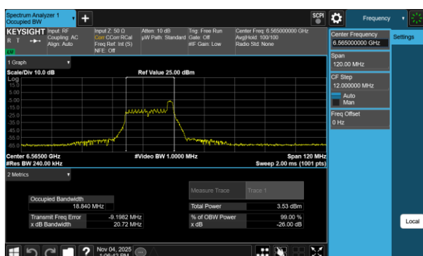
Plot 7-24 26dB BW & 99% OBW Antenna WF8 (40MHz BW 802.11be(RU) RU26 Index8 - Ch.123)
