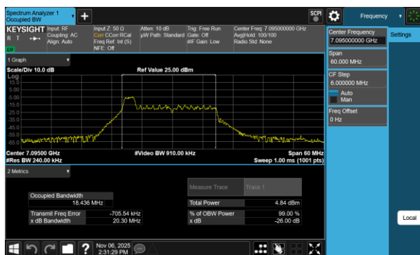
Plot 7-78 26dB BW & 99% OBW Antenna WF7a (20MHz BW 802.11be(RU) RU26 Index0 - Ch.229)
