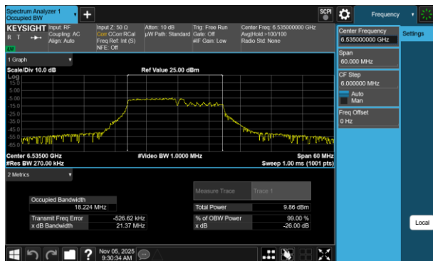
Plot 7-27 26dB BW & 99% OBW Antenna WF8 (20MHz BW 802.11be(RU) RU106+26 Index82 - Ch.117)
