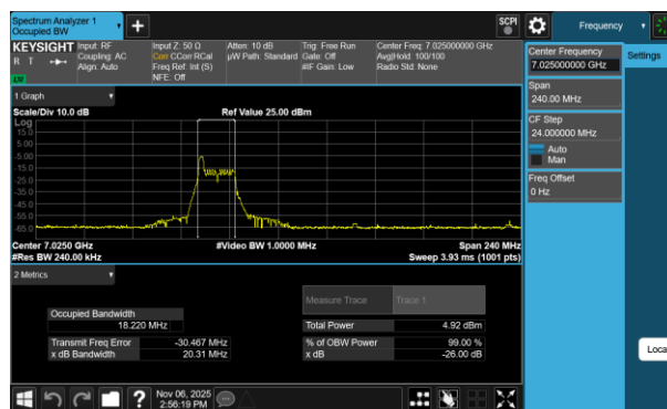
Plot 7-80 26dB BW & 99% OBW Antenna WF7a (80MHz BW 802.11be(RU) RU26 Index0 - Ch.215)
