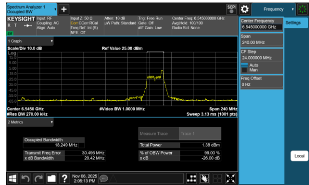
Plot 7-69 26dB BW & 99% OBW Antenna WF7a (80MHz BW 802.11be(RU) RU26 Index36 - Ch.119)
