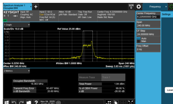
Plot 7-3 26dB BW & 99% OBW Antenna WF8 (80MHz BW 802.11be(RU) RU26 Index36 - Ch.55)
