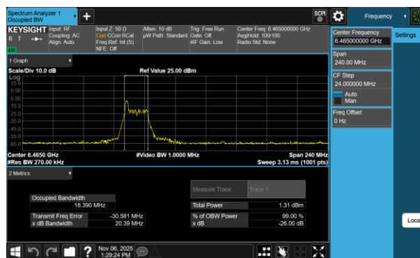
Plot 7-58 26dB BW & 99% OBW Antenna WF7a (80Mhz BW 802.11be(RU) RU26 Index0 - Ch.103)
