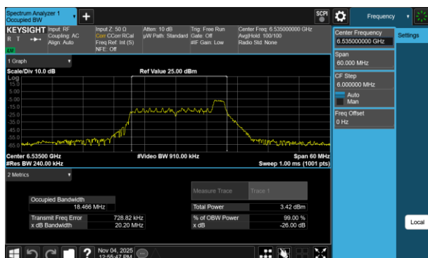
Plot 7-23 26dB BW & 99% OBW Antenna WF8 (20MHz BW 802.11be(RU) RU26 Index8 - Ch.117)
