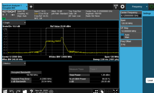
Plot 7-2 26dB BW & 99% OBW Antenna WF8 (40MHz BW 802.11be(RU) RU26 Index8 - Ch.35)
