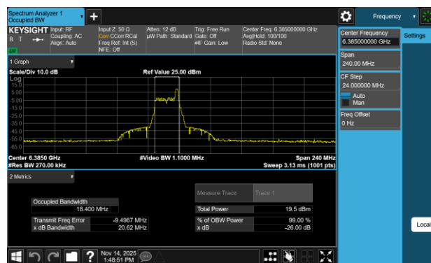
Plot 7-3 26dB BW & 99% OBW Antenna WF8 (80MHz BW 802.11be(RU) RU26 Index17 - Ch.87)
