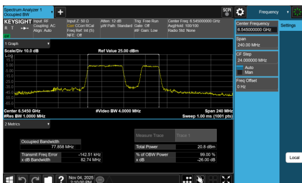
Plot 7-61 26dB BW & 99% OBW Antenna WF8 (80MHz BW 802.11be(RU) RU484+242 Index92 - Ch.119)
