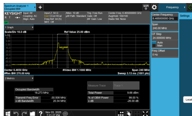
Plot 7-47 26dB BW & 99% OBW Antenna WF8 (80MHz BW 802.11be(RU) RU26 Index0 - Ch.103)
