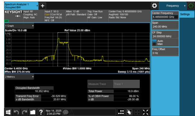
Plot 7-14 26dB BW & 99% OBW Antenna WF8 (80MHz BW 802.11be(RU) RU26 Index0 - Ch.103)
