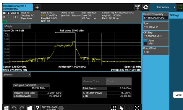
Plot 7-46 26dB BW & 99% OBW Antenna WF8 (40MHz BW 802.11be(RU) RU26 Index8 - Ch.107)
