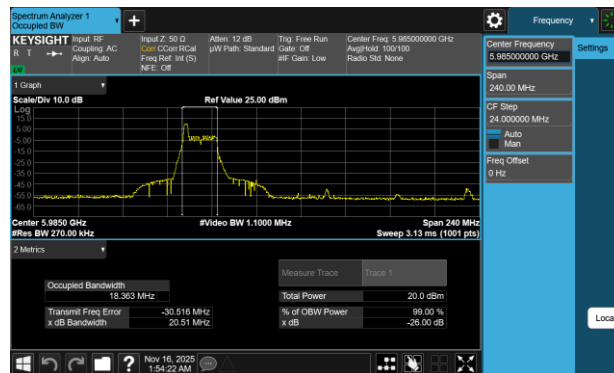
Plot 7-80 26dB BW & 99% OBW Antenna WF7a (80MHz BW 802.11be(RU) RU26 Index0 - Ch.7)
