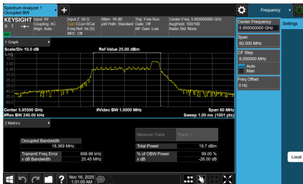
Plot 7-78 26dB BW & 99% OBW Antenna WF7a (20MHz BW 802.11be(RU) RU26 Index8 - Ch.1)
