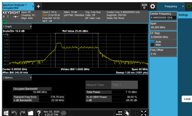
Plot 7-67 26dB BW & 99% OBW Antenna WF8 (20MHz BW 802.11be(RU) RU26 Index0 - Ch.209)
