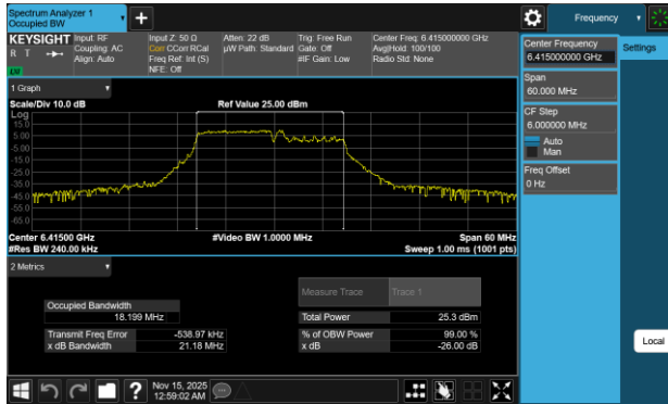
Plot 7-5 26dB BW & 99% OBW Antenna WF8 (20MHz BW 802.11be(RU) RU106+26 Index82 - Ch.93)
