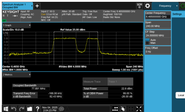
Plot 7-50 26dB BW & 99% OBW Antenna WF8 (80MHz BW 802.11be(RU) RU484+242 Index92 - Ch.103)
