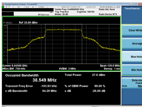
Plot 7-20 26dB BW & 99% OBW Antenna WF8 (40MHz BW 802.11be(RU) RU484 Index65 - Ch.99)
