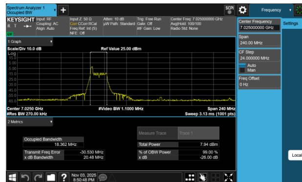
Plot 7-69 26dB BW & 99% OBW Antenna WF8 (80MHz BW 802.11be(RU) RU26 Index0 - Ch.215)
