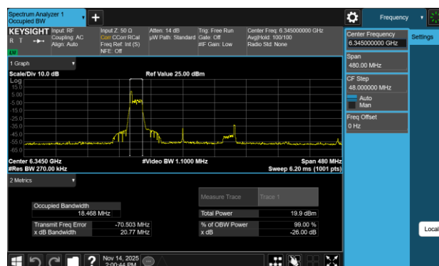
Plot 7-4 26dB BW & 99% OBW Antenna WF8 (160MHz BW 802.11be(RU) RU26 Index0 - Ch.79)
