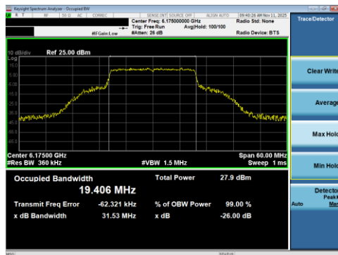
Plot 7-8 26dB BW & 99% OBW Antenna WF8 (20MHz BW 802.11be(RU) RU242 Index61 - Ch.45)
