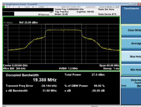
Plot 7-30 26dB BW & 99% OBW Antenna WF8 (20MHz BW 802.11be(RU) RU242 Index61 - Ch.181)
