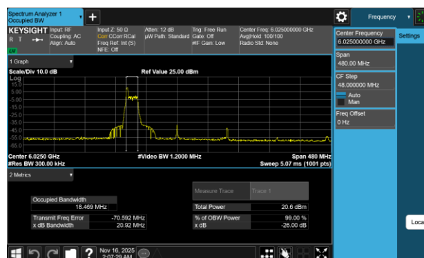
Plot 7-81 26dB BW & 99% OBW Antenna WF7a (160MHz BW 802.11be(RU) RU26 Index0 - Ch.15)
