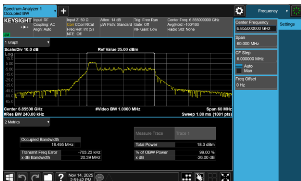
Plot 7-23 26dB BW & 99% OBW Antenna WF8 (20MHz BW 802.11be(RU) RU26 Index0 - Ch.181)
