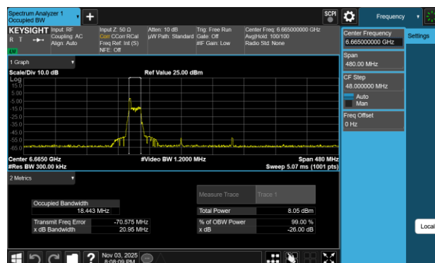
Plot 7-59 26dB BW & 99% OBW Antenna WF8 (160MHz BW 802.11be(RU) RU26 Index0 - Ch.143)
