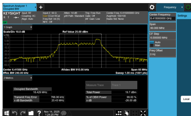
Plot 7-1 26dB BW & 99% OBW Antenna WF8 (20MHz BW 802.11be(RU) RU26 Index8 - Ch.93)
