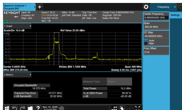
Plot 7-26 26dB BW & 99% OBW Antenna WF8 (160MHz BW 802.11be(RU) RU26 Index0 - Ch.143)
