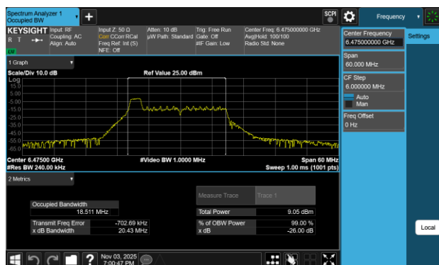
Plot 7-45 26dB BW & 99% OBW Antenna WF8 (20MHz BW 802.11be(RU) RU26 Index0 - Ch.105)
