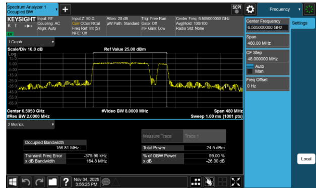
Plot 7-51 26dB BW & 99% OBW Antenna WF8 (160MHz BW 802.11be(RU) RU996+484+242 Index98 - Ch.111)
