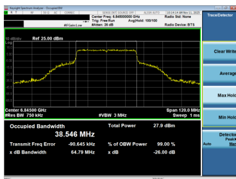
Plot 7-31 26dB BW & 99% OBW Antenna WF8 (40MHz BW 802.11be(RU) RU484 Index65 - Ch.179)
