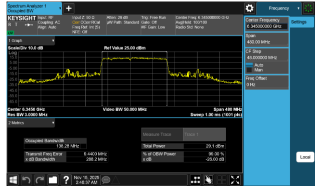
Plot 7-7 26dB BW & 99% OBW Antenna WF8 (160MHz BW 802.11be(RU) RU996+484+242 Index96 - Ch.79)
