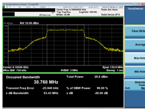
Plot 7-9 26dB BW & 99% OBW Antenna WF8 (40MHz BW 802.11be(RU) RU484 Index65 - Ch.43)
