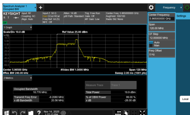
Plot 7-2 26dB BW & 99% OBW Antenna WF8 (40MHz BW 802.11be(RU) RU26 Index8 - Ch.3)
