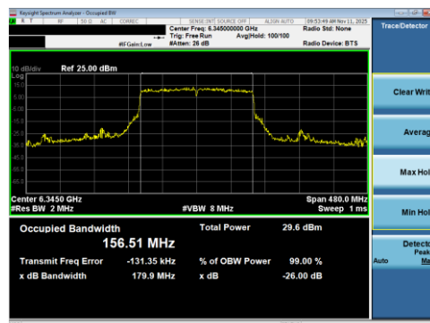
Plot 7-11 26dB BW & 99% OBW Antenna WF8 (160MHz BW 802.11be(RU) RU996X2 Index68 - Ch.79)
