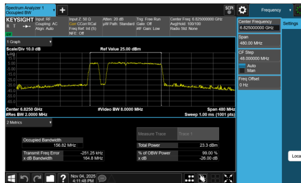
Plot 7-62 26dB BW & 99% OBW Antenna WF8 (160MHz BW 802.11be(RU) RU996+484+242 Index97 - Ch.175)
