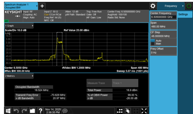
Plot 7-15 26dB BW & 99% OBW Antenna WF8 (160MHz BW 802.11be(RU) RU26 Index0 - Ch.111)
