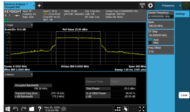
Plot 7-55 26dB BW & 99% OBW Antenna WF8 (160MHz BW 802.11be(RU) RU996X2 Index68 - Ch.111)
