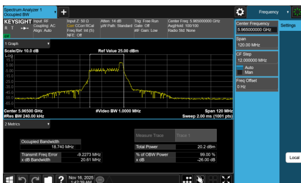
Plot 7-79 26dB BW & 99% OBW Antenna WF7a (40MHz BW 802.11be(RU) RU26 Index8 - Ch.3)
