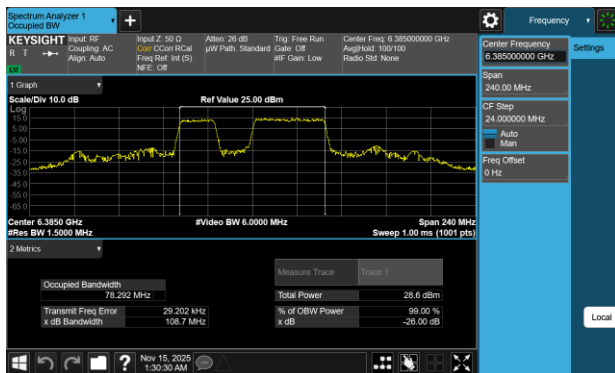
Plot 7-6 26dB BW & 99% OBW Antenna WF8 (80MHz BW 802.11be(RU) RU484+242 Index91 - Ch.87)
