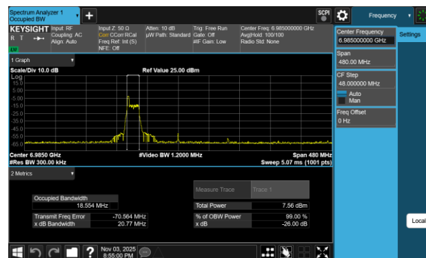
Plot 7-70 26dB BW & 99% OBW Antenna WF8 (160MHz BW 802.11be(RU) RU26 Index0 - Ch.207)
