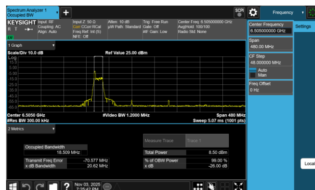
Plot 7-48 26dB BW & 99% OBW Antenna WF8 (160MHz BW 802.11be(RU) RU26 Index0 - Ch.111)
