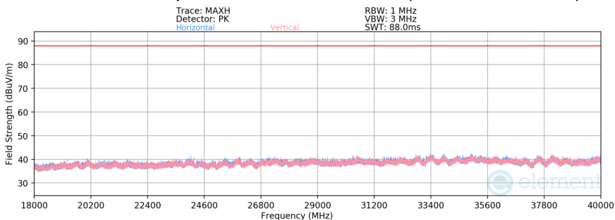
Plot 7-502. Radiated Spurious Emissions 18-40GHz SDM (802.11be – Ch. 149 – RU26)
