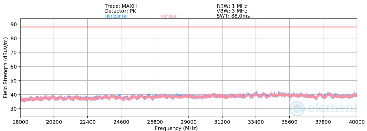
Plot 7-506. Radiated Spurious Emissions 18-40GHz SDM (802.11be – Ch. 209 – RU26)
