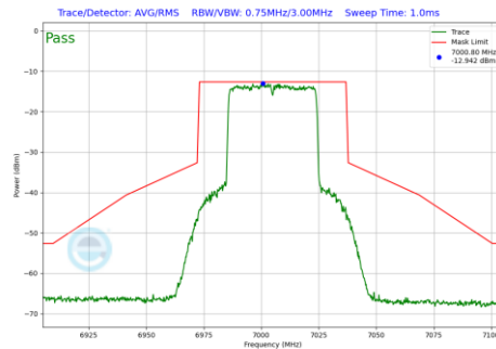
Plot 7-422 In-Band Emission Plot SDM Antenna WF8 (40MHz BW 802.11be(RU) RU484 Index65 (UNII Band 8) - Ch.211)
