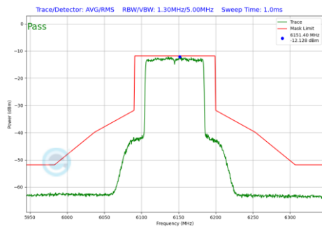
Plot 7-411 In-Band Emission Plot SDM Antenna WF8 (80MHz BW 802.11be(RU) RU996 Index67 (UNII Band 5) - Ch.39)
