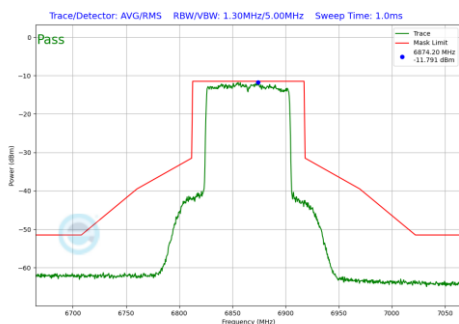
Plot 7-435 In-Band Emission Plot SDM Antenna WF7a (80MHz BW 802.11be(RU) RU996 Index67 (UNII Band 7) - Ch.183)
