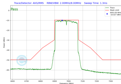
Plot 7-424 In-Band Emission Plot SDM Antenna WF8 (160MHz BW 802.11be(RU) RU996X2 Index68 (UNII Band 8) - Ch.207)
