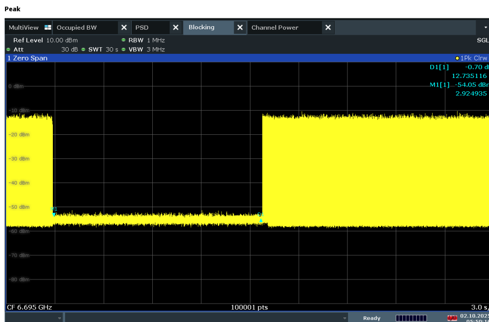
Plot 7-481. Contention Based Protocol Timing Plot – UNII 7 – 20MHz Channel 149
