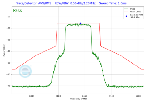
Plot 7-425 In-Band Emission Plot SDM Antenna WF7a (20MHz BW 802.11be(RU) RU242 Index61 (UNII Band 5) - Ch.33)
