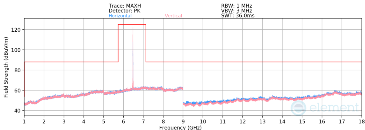
Plot 7-497. Radiated Spurious Emissions above 1GHz SDM (802.11be – Ch. 105 – RU26)
