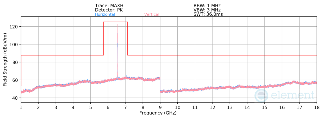
Plot 7-500. Radiated Spurious Emissions above 1GHz SDM (802.11be – Ch. 117 – RU26)
