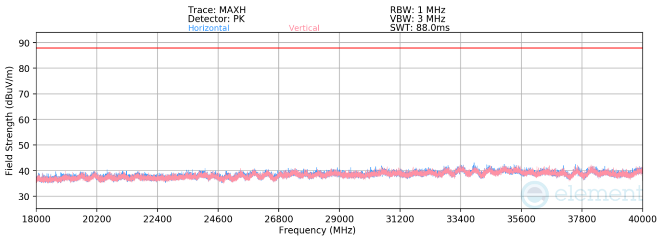
Plot 7-510. Radiated Spurious Emissions 18-40GHz SDM (802.11be – Ch. 61 – RU242)
