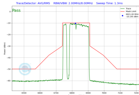
Plot 7-405 In-Band Emission Plot SDM Antenna WF7a (160MHz BW 802.11be(RU) RU996+484+242 Index97 (UNII Band 7) - Ch.175)
