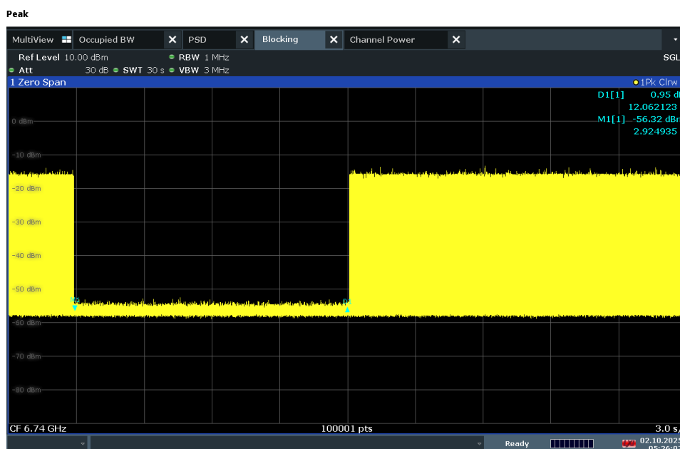
Plot 7-482. Contention Based Protocol Timing Plot – UNII 7 – 160MHz Channel 143 – Low
