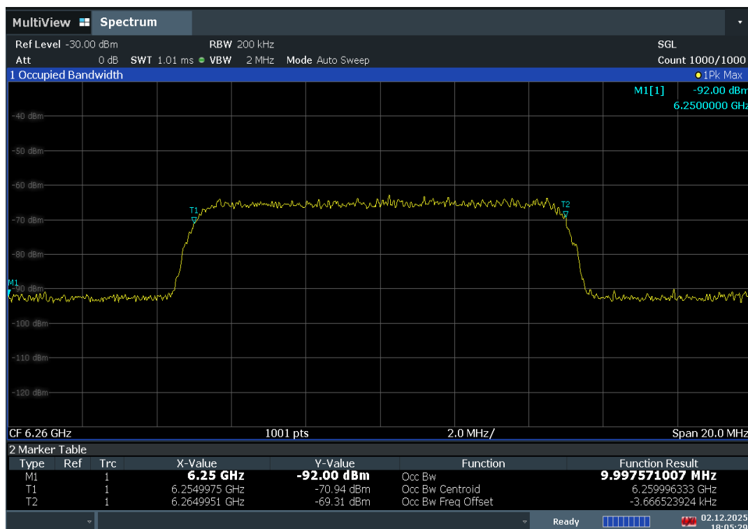
Plot 7-444. AWGN Signal – UNII 5 – 160MHz - High
