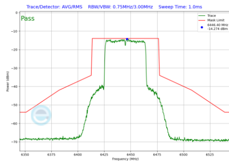
Plot 7-430 In-Band Emission Plot SDM Antenna WF7a (40MHz BW 802.11be(RU) RU484 Index65 (UNII Band 6) - Ch.99)
