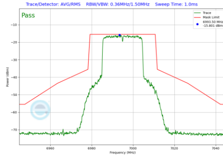
Plot 7-421 In-Band Emission Plot SDM Antenna WF8 (20MHz BW 802.11be(RU) RU242 Index61 (UNII Band 8) - Ch.209)
