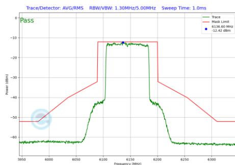
Plot 7-427 In-Band Emission Plot SDM Antenna WF7a (80MHz BW 802.11be(RU) RU996 Index67 (UNII Band 5) - Ch.39)
