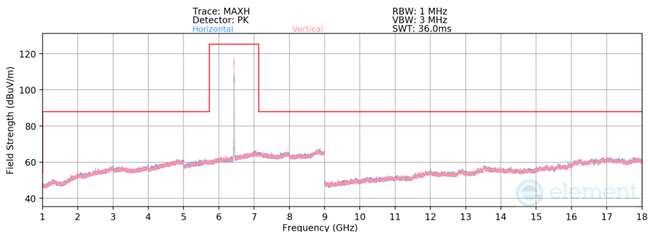
Plot 7-512. Radiated Spurious Emissions 1-18GHz SDM (802.11be – Ch. 97 – RU242)
