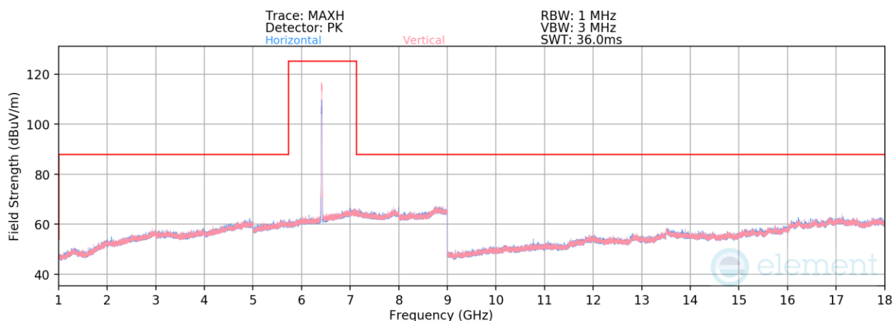
Plot 7-511. Radiated Spurious Emissions 1-18GHz SDM (802.11be – Ch. 93 – RU242)
