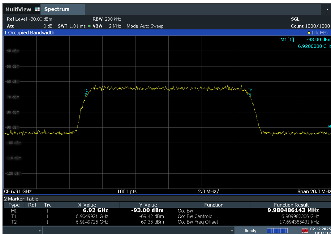
Plot 7-454. AWGN Signal – UNII 8 – 160MHz - Low
