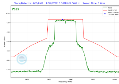
Plot 7-413 In-Band Emission Plot SDM Antenna WF8 (20MHz BW 802.11be(RU) RU242 Index61 (UNII Band 6) - Ch.97)
