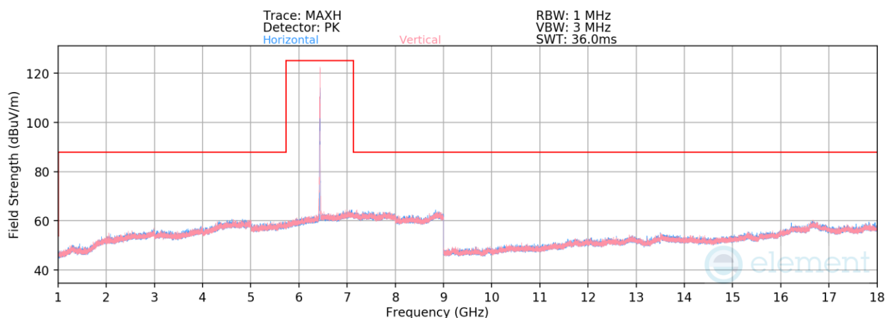
Plot 7-496. Radiated Spurious Emissions above 1GHz SDM (802.11be – Ch. 97 – RU26)
