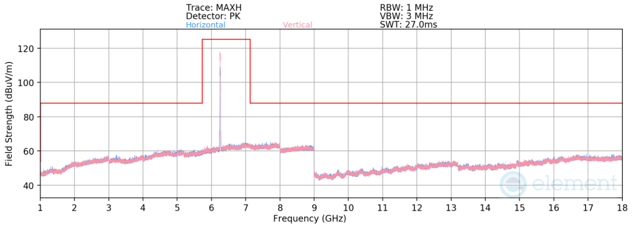
Plot 7-509. Radiated Spurious Emissions 1-18GHz SDM (802.11be – Ch. 61 – RU242)
