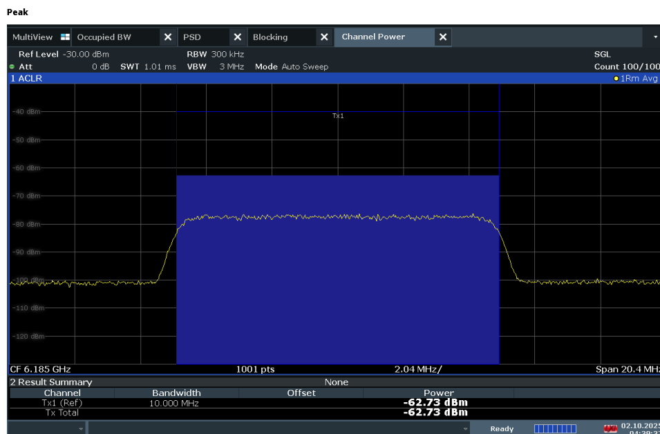
Plot 7-459. Channel Power – UNII 5 – 160MHz – Mid
