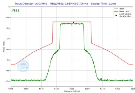
Plot 7-410 In-Band Emission Plot SDM Antenna WF8 (40MHz BW 802.11be(RU) RU484 Index65 (UNII Band 5) - Ch.35)
