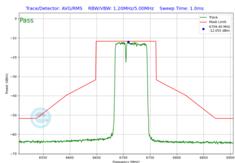
Plot 7-404 In-Band Emission Plot SDM Antenna WF7a (80MHz BW 802.11be(RU) RU484+242 Index90 (UNII Band 7) - Ch.151)
