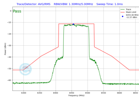
Plot 7-415 In-Band Emission Plot SDM Antenna WF8 (80MHz BW 802.11be(RU) RU996 Index67 (UNII Band 6) - Ch.103)
