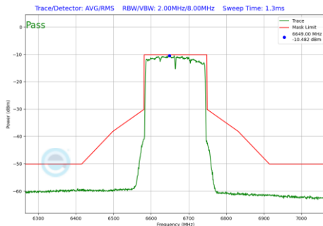
Plot 7-420 In-Band Emission Plot SDM Antenna WF8 (160MHz BW 802.11be(RU) RU996X2 Index68 (UNII Band 7) - Ch.143)
