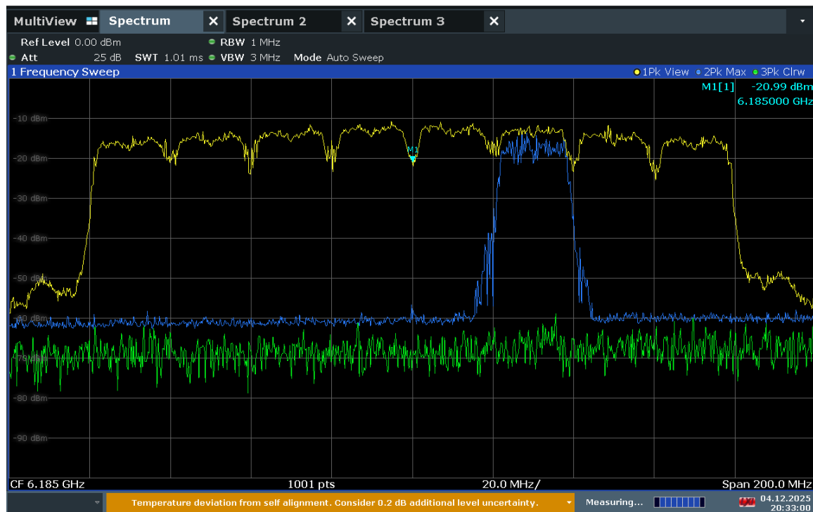
Plot 7-490. 160MHz Bandwidth, AWGN Signal Injected – 6185MHz
