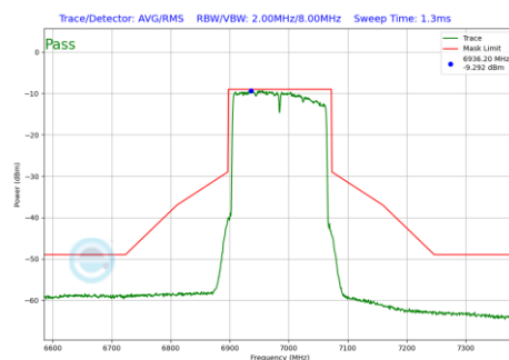
Plot 7-440 In-Band Emission Plot SDM Antenna WF7a (160MHz BW 802.11be(RU) RU996X2 Index68 (UNII Band 8) - Ch.207)
