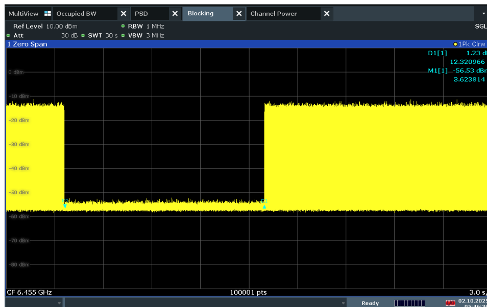
Plot 7-477. Contention Based Protocol Timing Plot – UNII 6 – 20MHz Channel 101
