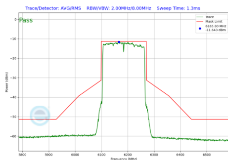
Plot 7-428 In-Band Emission Plot SDM Antenna WF7a (160MHz BW 802.11be(RU) RU996X2 Index68 (UNII Band 5) - Ch.47)
