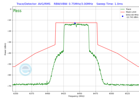
Plot 7-414 In-Band Emission Plot SDM Antenna WF8 (40MHz BW 802.11be(RU) RU484 Index65 (UNII Band 6) - Ch.99)
