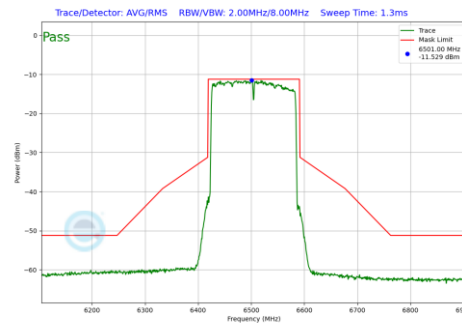
Plot 7-416 In-Band Emission Plot SDM Antenna WF8 (160MHz BW 802.11be(RU) RU996X2 Index68 (UNII Band 6) - Ch.111)
