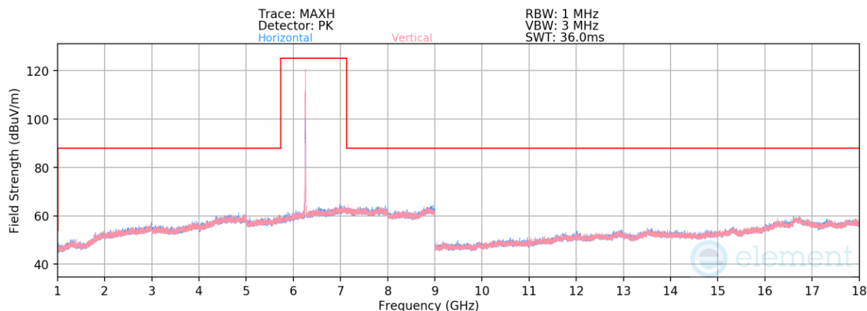
Plot 7-493. Radiated Spurious Emissions above 1GHz SDM (802.11be – Ch. 61 – RU26)
