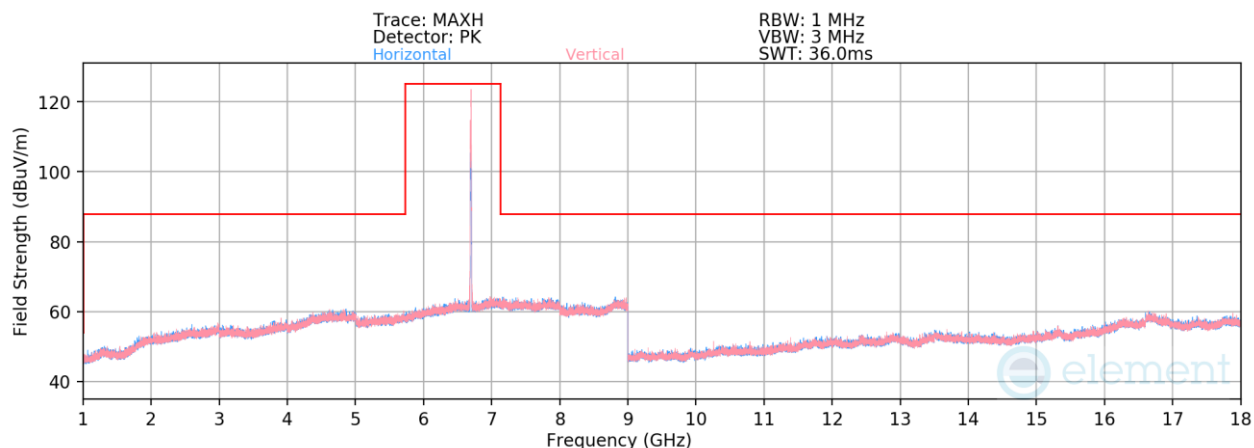
Plot 7-501. Radiated Spurious Emissions above 1GHz SDM (802.11be – Ch. 149 – RU26)
