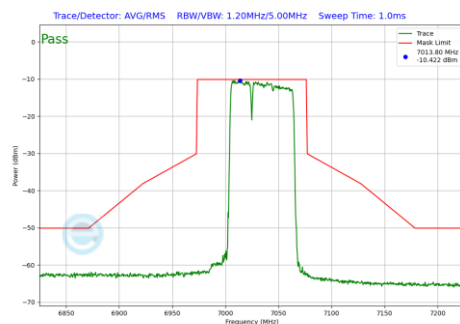
Plot 7-407 In-Band Emission Plot SDM Antenna WF7a (80MHz BW 802.11be(RU) RU484+242 Index90 (UNII Band 8) - Ch.215)
