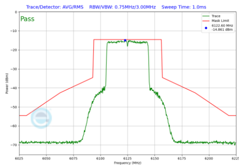
Plot 7-426 In-Band Emission Plot SDM Antenna WF7a (40MHz BW 802.11be(RU) RU484 Index65 (UNII Band 5) - Ch.35)
