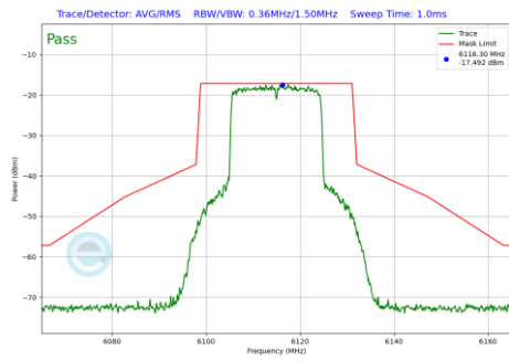
Plot 7-409 In-Band Emission Plot SDM Antenna WF8 (20MHz BW 802.11be(RU) RU242 Index61 (UNII Band 5) - Ch.33)
