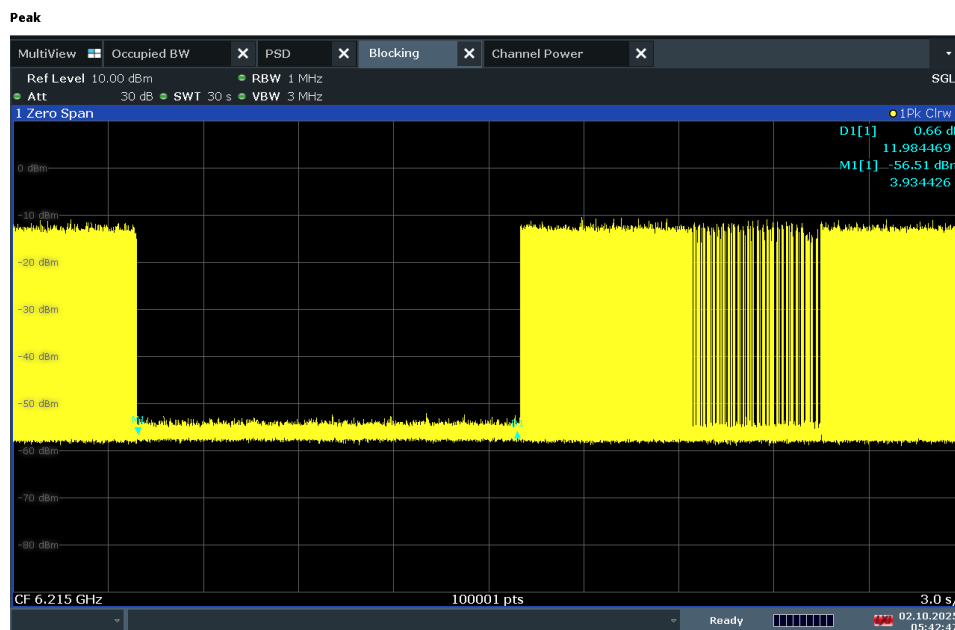
Plot 7-473. Contention Based Protocol Timing Plot – UNII 5 – 20MHz Channel 53
