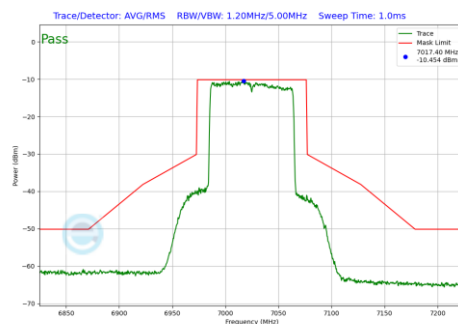
Plot 7-439 In-Band Emission Plot SDM Antenna WF7a (80MHz BW 802.11be(RU) RU996 Index67 (UNII Band 8) - Ch.215)
