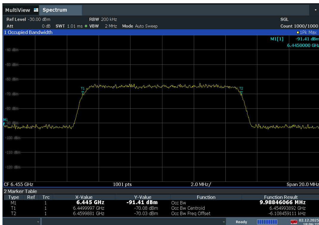
Plot 7-445. AWGN Signal – UNII 6 – 20MHz
