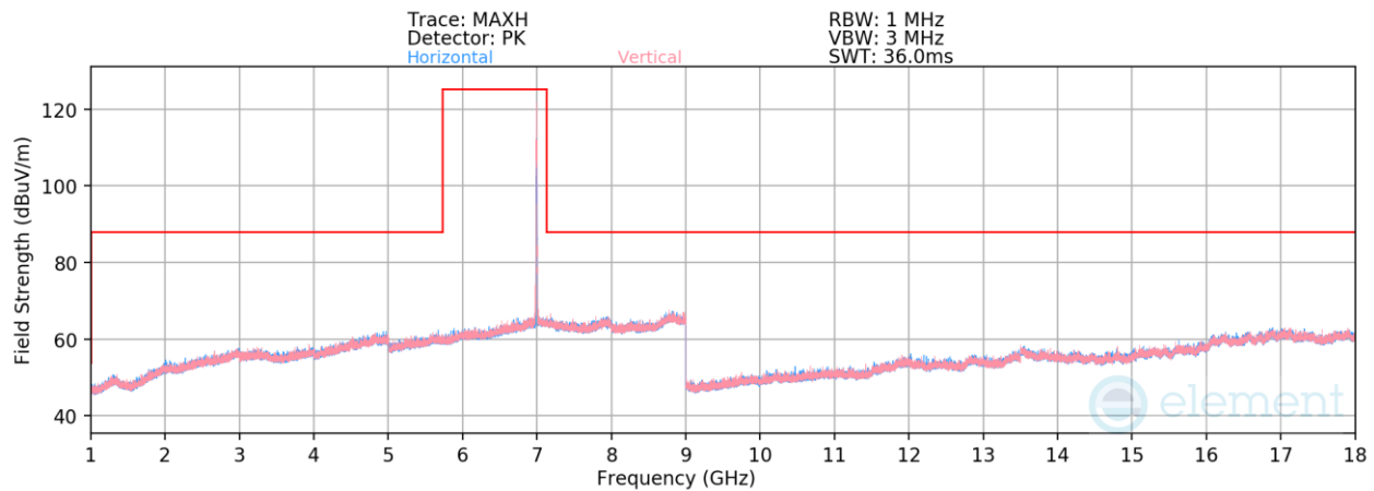
Plot 7-505. Radiated Spurious Emissions above 1GHz SDM (802.11be – Ch. 209 – RU26)
