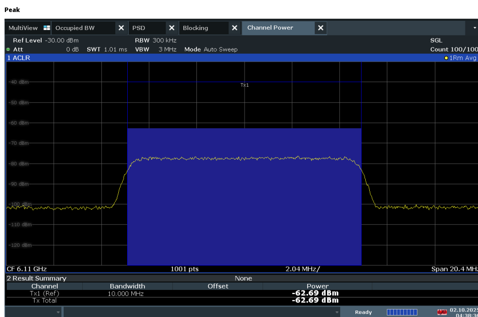
Plot 7-458. Channel Power – UNII 5 – 160MHz - Low
