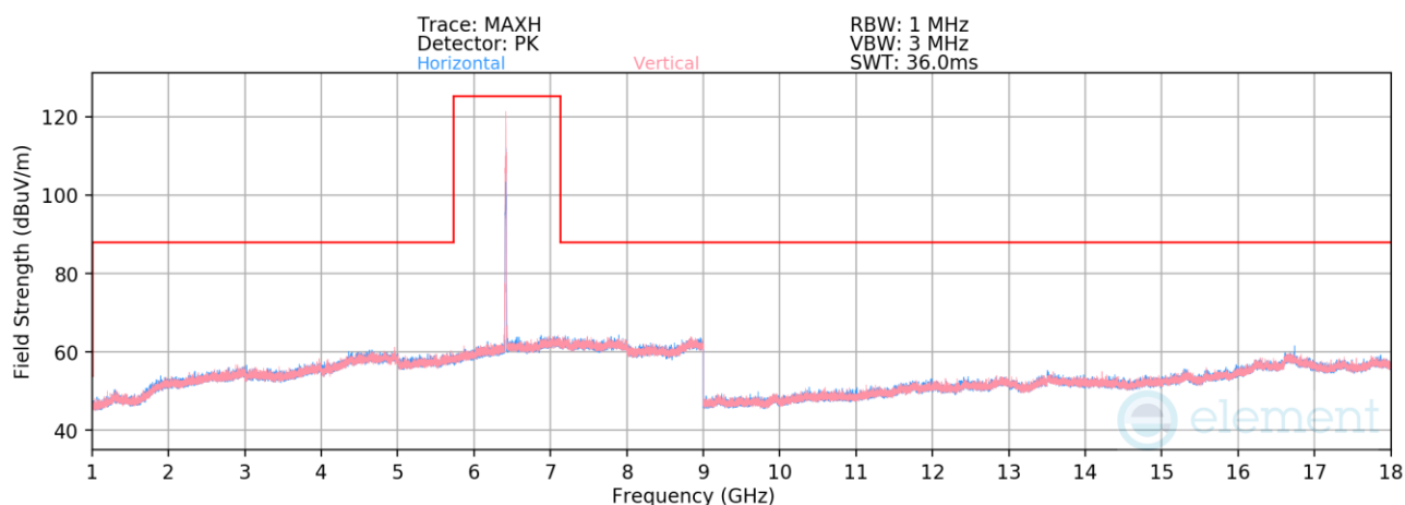
Plot 7-495. Radiated Spurious Emissions above 1GHz SDM (802.11be – Ch. 93 – RU26)
