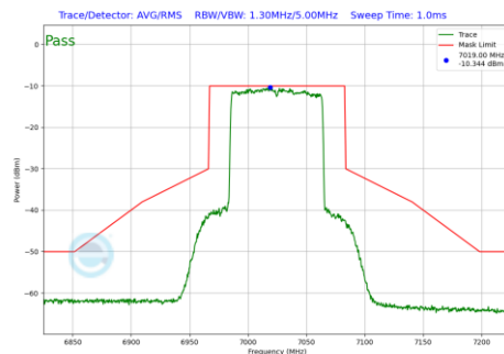
Plot 7-423 In-Band Emission Plot SDM Antenna WF8 (80MHz BW 802.11be(RU) RU996 Index67 (UNII Band 8) - Ch.215)
