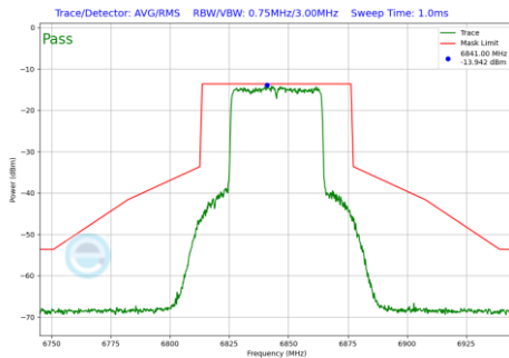
Plot 7-418 In-Band Emission Plot SDM Antenna WF8 (40MHz BW 802.11be(RU) RU484 Index65 (UNII Band 7) - Ch.179)
