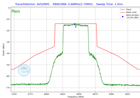
Plot 7-434 In-Band Emission Plot SDM Antenna WF7a (40MHz BW 802.11be(RU) RU484 Index65 (UNII Band 7) - Ch.179)
