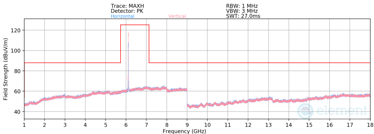
Plot 7-508. Radiated Spurious Emissions 1-18GHz SDM (802.11be – Ch. 33 – RU242)
