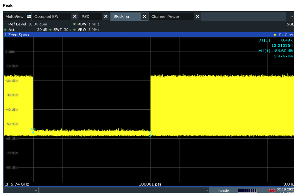
Plot 7-484. Contention Based Protocol Timing Plot – UNII 7 – 160MHz Channel 143 – High
