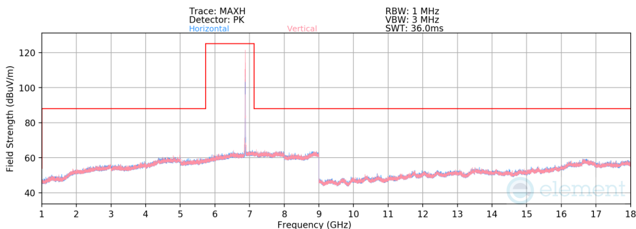
Plot 7-503. Radiated Spurious Emissions above 1GHz SDM (802.11be – Ch. 185 – RU26)
