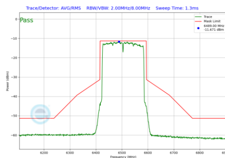
Plot 7-432 In-Band Emission Plot SDM Antenna WF7a (160MHz BW 802.11be(RU) RU996X2 Index68 (UNII Band 6) - Ch.111)
