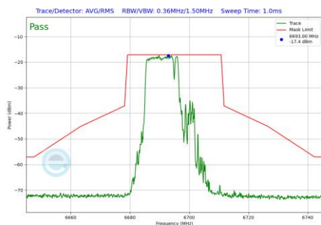
Plot 7-403 In-Band Emission Plot SDM Antenna WF7a (20MHz BW 802.11be(RU) RU106+26 Index82 (UNII Band 7) - Ch.149)
