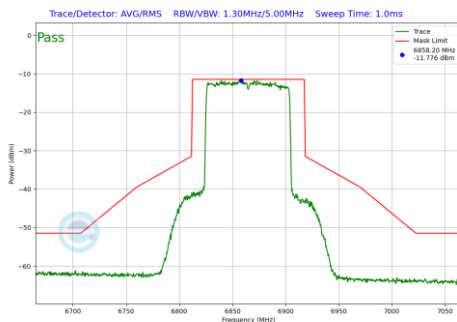
Plot 7-419 In-Band Emission Plot SDM Antenna WF8 (80MHz BW 802.11be(RU) RU996 Index67 (UNII Band 7) - Ch.183)
