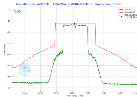
Plot 7-438 In-Band Emission Plot SDM Antenna WF7a (40MHz BW 802.11be(RU) RU484 Index65 (UNII Band 8) - Ch.211)
