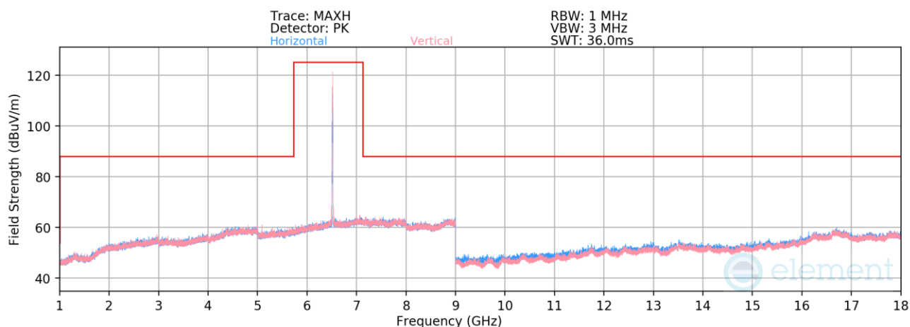
Plot 7-499. Radiated Spurious Emissions above 1GHz SDM (802.11be – Ch. 113 – RU26)
