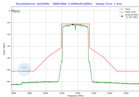
Plot 7-412 In-Band Emission Plot SDM Antenna WF8 (160MHz BW 802.11be(RU) RU996X2 Index68 (UNII Band 5) - Ch.47)
