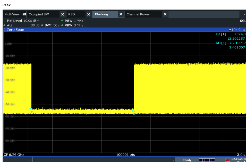
Plot 7-476. Contention Based Protocol Timing Plot – UNII 5 – 160MHz Channel 47 – High
