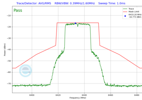
Plot 7-429 In-Band Emission Plot SDM Antenna WF7a (20MHz BW 802.11be(RU) RU242 Index61 (UNII Band 6) - Ch.97)
