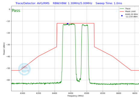
Plot 7-401 In-Band Emission Plot SDM Antenna WF7a (80MHz BW 802.11be(RU) RU484+242 Index92 (UNII Band 6) - Ch.103)
