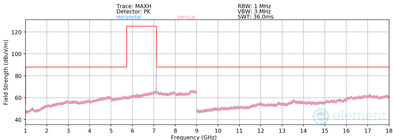
Plot 7-507. Radiated Spurious Emissions above 1GHz SDM (802.11be – Ch. 229 – RU26)
