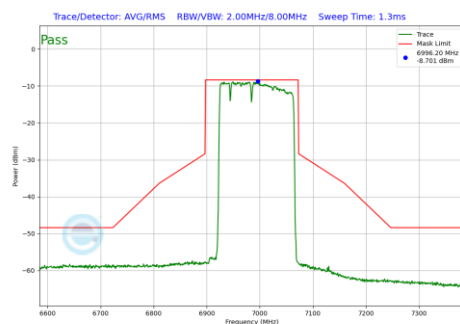
Plot 7-408 In-Band Emission Plot SDM Antenna WF7a (160MHz BW 802.11be(RU) RU996+484+242 Index96 (UNII Band 8) - Ch.207)
