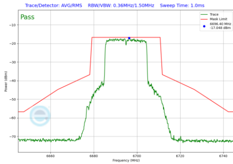
Plot 7-433 In-Band Emission Plot SDM Antenna WF7a (20MHz BW 802.11be(RU) RU242 Index61 (UNII Band 7) - Ch.149)
