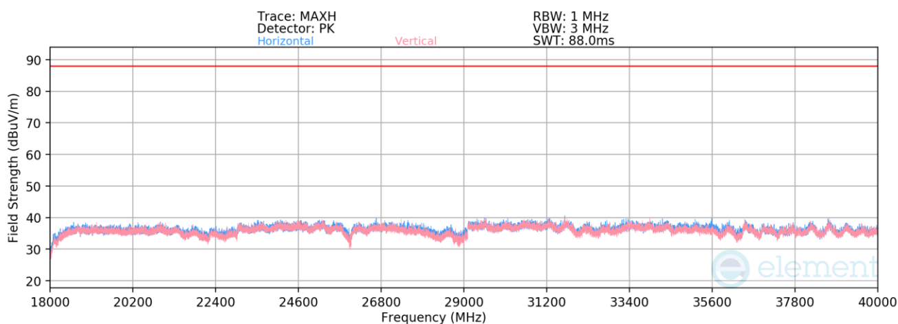
Plot 7-498. Radiated Spurious Emissions 18-40GHz SDM (802.11be – Ch. 105 – RU26)
