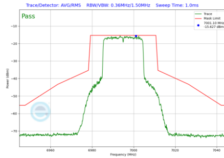
Plot 7-437 In-Band Emission Plot SDM Antenna WF7a (20MHz BW 802.11be(RU) RU242 Index61 (UNII Band 8) - Ch.209)
