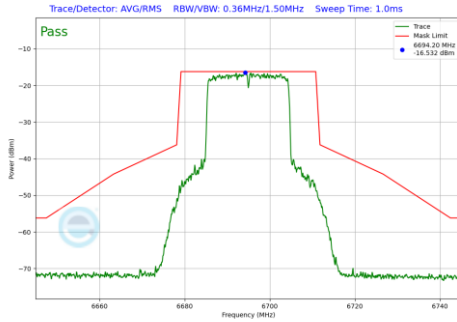
Plot 7-417 In-Band Emission Plot SDM Antenna WF8 (20MHz BW 802.11be(RU) RU242 Index61 (UNII Band 7) - Ch.149)
