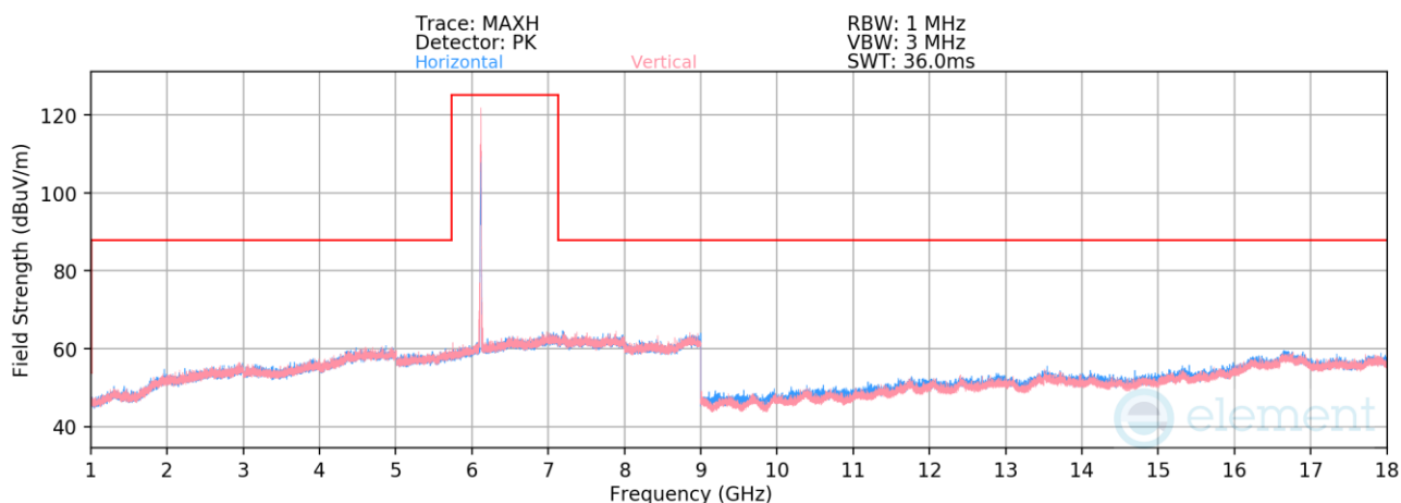
Plot 7-492. Radiated Spurious Emissions above 1GHz SDM (802.11be – Ch. 33 – RU26)
