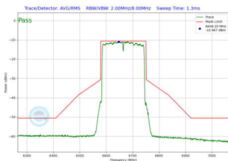
Plot 7-436 In-Band Emission Plot SDM Antenna WF7a (160MHz BW 802.11be(RU) RU996X2 Index68 (UNII Band 7) - Ch.143)
