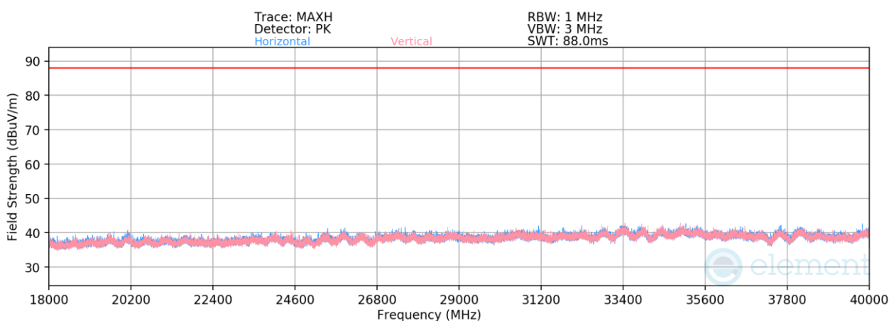
Plot 7-494. Radiated Spurious Emissions 18-40GHz SDM (802.11be – Ch. 61 – RU26)
