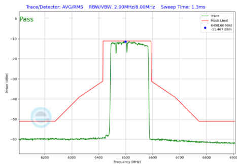
Plot 7-402 In-Band Emission Plot SDM Antenna WF7a (160MHz BW 802.11be(RU) RU996+484+242 Index96 (UNII Band 6) - Ch.111)
