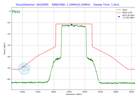
Plot 7-431 In-Band Emission Plot SDM Antenna WF7a (80MHz BW 802.11be(RU) RU996 Index67 (UNII Band 6) - Ch.103)
