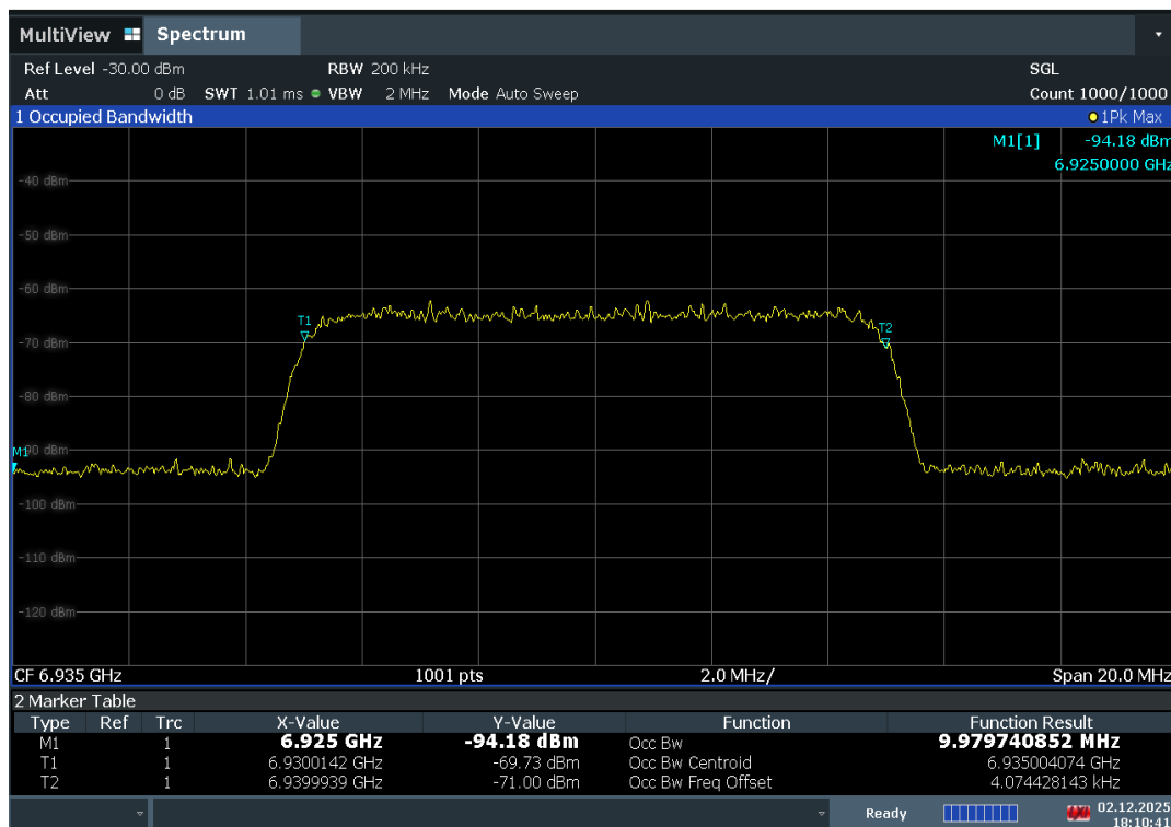
Plot 7-453. AWGN Signal – UNII 8 – 20MHz
