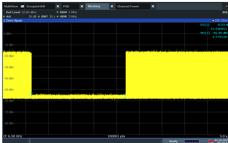
Plot 7-478. Contention Based Protocol Timing Plot – UNII 6 – 160MHz Channel 111 – Low
