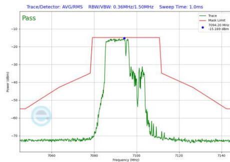
Plot 7-406 In-Band Emission Plot SDM Antenna WF7a (20MHz BW 802.11be(RU) RU106+26 Index82 (UNII Band 8) - Ch.229)
