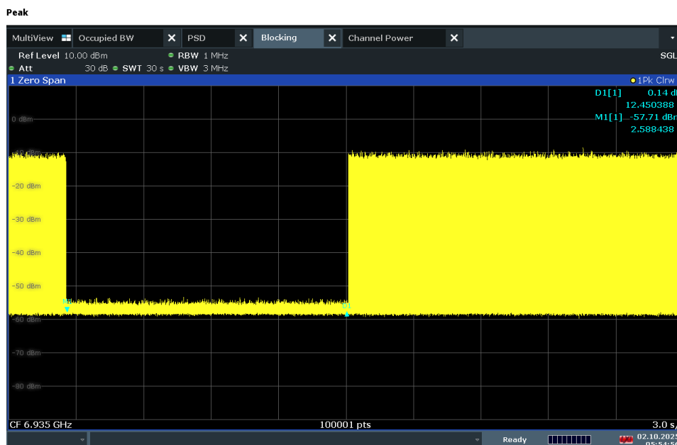
Plot 7-485. Contention Based Protocol Timing Plot – UNII 8 – 20MHz Channel 197
