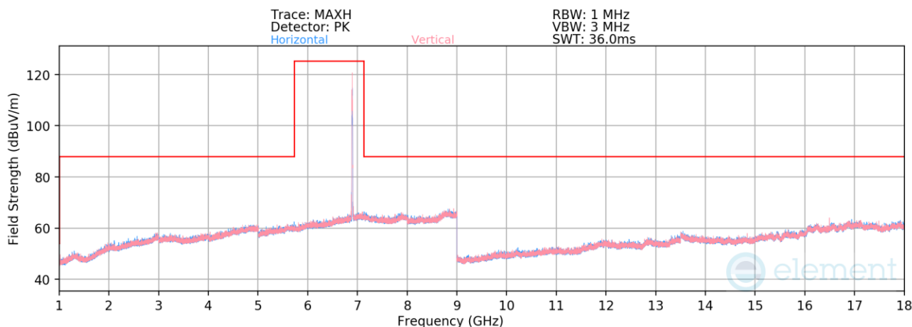
Plot 7-504. Radiated Spurious Emissions above 1GHz SDM (802.11be – Ch. 189 – RU26)
