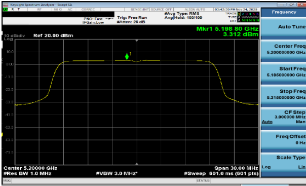
Plot 7-151 PSD CDD Antenna WF8 (20MHz BW 802.11be(RU) RU242 Index61 - Ch.40)
