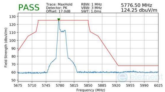
Plot 7-208. Antenna WF8 (Peak, RU26, Index 0, Ch.157, MCS11)
