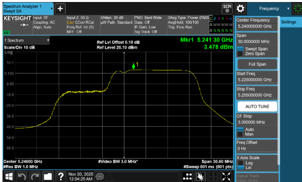
Plot 7-145 PSD CDD Antenna WF8 (20MHz BW 802.11be(RU) RU106+26 Index83 - Ch.48)
