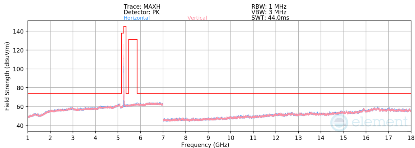
Plot 7-163. Radiated Spurious Emissions above 1GHz CDD (11be Ch.52 — RU52)
