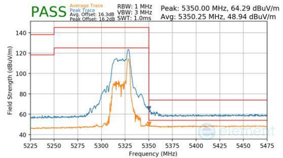
Plot 7-194. Antenna WF8 (Peak & Average, RU26, Index 8, Ch.64, MCS11)
