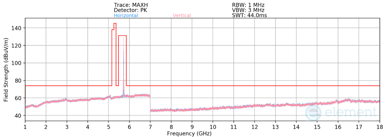
Plot 7-170. Radiated Spurious Emissions above 1GHz CDD (11be Ch.144 — RU52)
