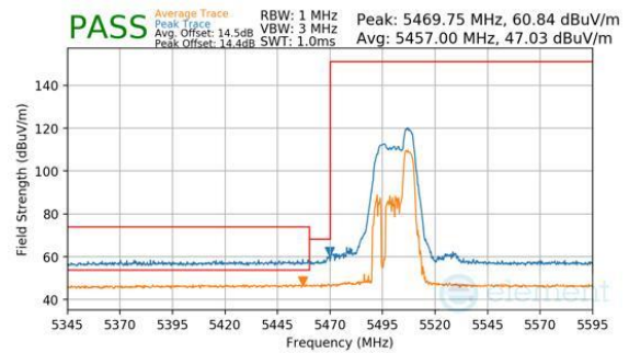
Plot 7-217. Antenna WF8 (Peak & Average, RU52, Index 40, Ch.100, MCS11)
