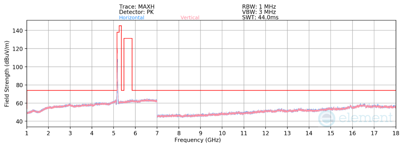
Plot 7-175. Radiated Spurious Emissions above 1GHz CDD (11be – Ch.36 – RU242)
