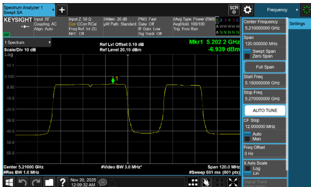
Plot 7-146 PSD CDD Antenna WF8 (80MHz BW 802.11be(RU) RU484+242 Index92 - Ch.42)
