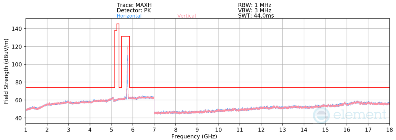
Plot 7-187. Radiated Spurious Emissions above 1GHz CDD (11be – Ch.149 – RU242)
