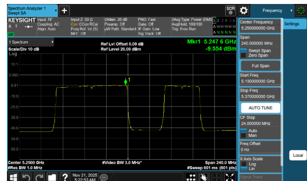
Plot 7-150 PSD CDD Antenna WF7a (160MHz BW 802.11be(RU) RU996+484 Index94 - Ch.50)
