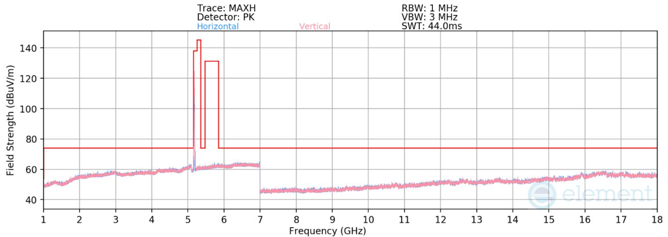
Plot 7-159. Radiated Spurious Emissions above 1GHz CDD (11be Ch.36 — RU26)
