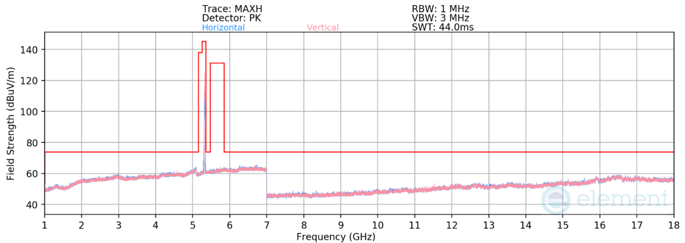
Plot 7-166. Radiated Spurious Emissions above 1GHz CDD (11be Ch.64 — RU52)
