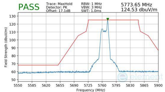
Plot 7-207. Antenna WF8 (Peak, RU26, Index 8, Ch.153, MCS11)
