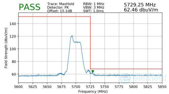
Plot 7-218. Antenna WF8 (Peak, RU52, Index 37, Ch.140, MCS11)
