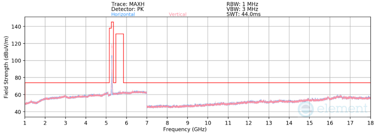
Plot 7-180. Radiated Spurious Emissions above 1GHz CDD (11be - Ch.56 - RU242)
