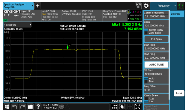
Plot 7-157 PSD CDD Antenna WF7a (80MHz BW 802.11be(RU) RU996 Index67 - Ch.42)
