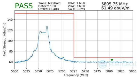
Plot 7-199. Antenna WF8 (Peak, RU26, Index 8, Ch.132, MCS11)
