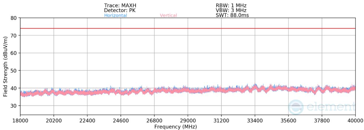
Plot 7-181. Radiated Spurious Emissions 18 GHz - 40GHz CDD (11be Ch.56 - RU242)
