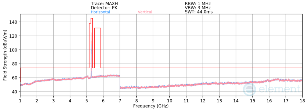
Plot 7-164. Radiated Spurious Emissions above 1GHz CDD (11be Ch.56 — RU52)
