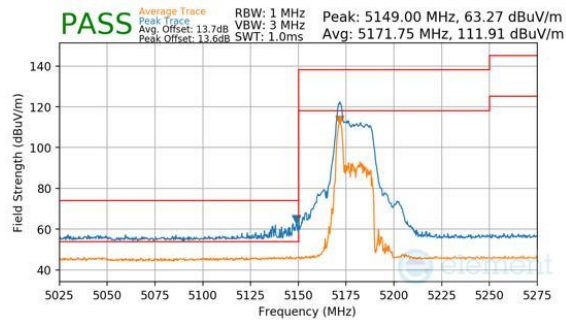
Plot 7-191. Antenna WF8 (Peak & Average, RU26, Index 0, Ch.36, MCS11)
