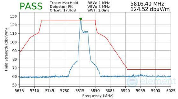
Plot 7-212. Antenna WF8 (Peak, RU26, Index 0, Ch.165, MCS11)
