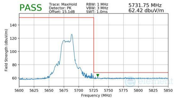
Plot 7-201. Antenna WF8 (Peak, RU26, Index 8, Ch.136, MCS11)
