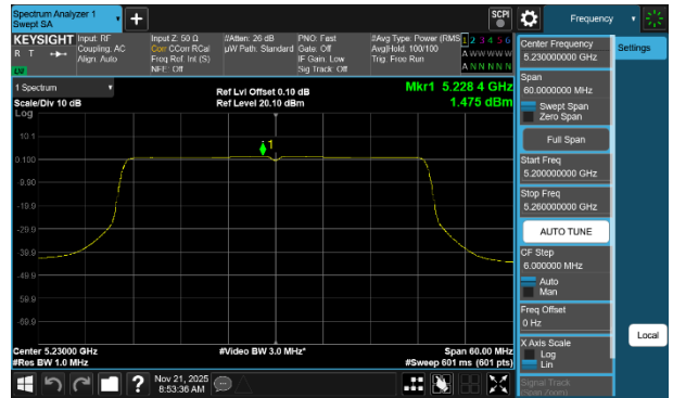
Plot 7-156 PSD CDD Antenna WF7a (40MHz BW 802.11be(RU) RU484 Index65 - Ch.46)
