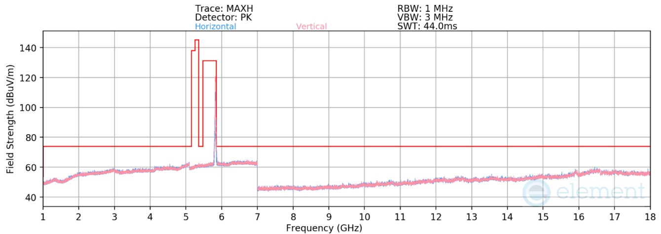
Plot 7-190. Radiated Spurious Emissions above 1GHz CDD (11be – Ch.165 – RU242)
