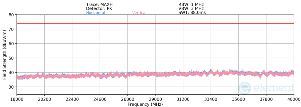
Plot 7-189. Radiated Spurious Emissions 18 GHz - 40GHz CDD (11be Ch.157 - RU242)
