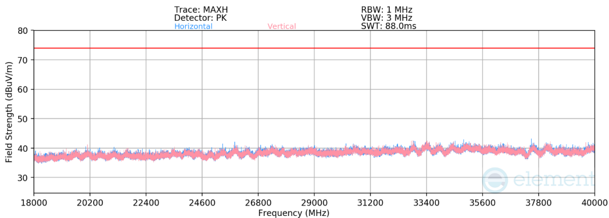
Plot 7-169. Radiated Spurious Emissions 18 GHz - 40GHz CDD (11be Ch.116 — RU52)
