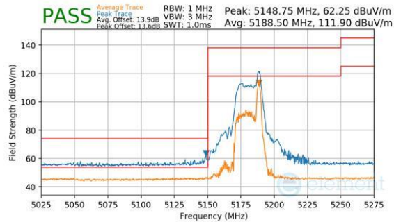
Plot 7-192. Antenna WF8 (Peak & Average, RU26, Index 8, Ch.36, MCS11)
