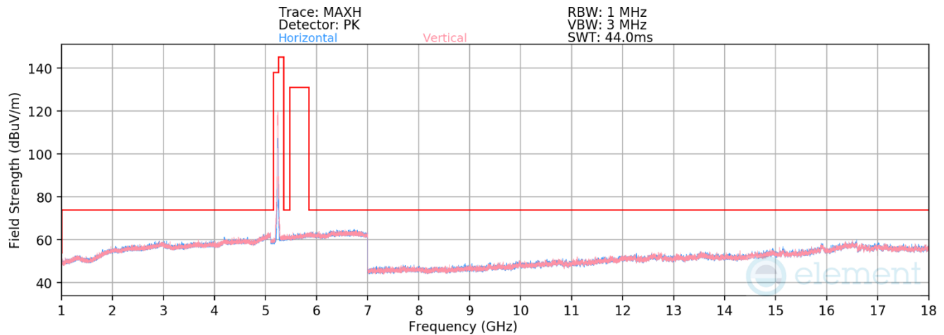
Plot 7-178. Radiated Spurious Emissions above 1GHz CDD (11be – Ch.48 – RU242)
