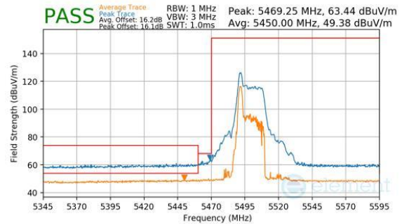
Plot 7-195. Antenna WF8 (Peak & Average, RU26, Index 0, Ch.100, MCS11)
