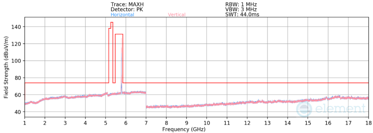
Plot 7-172. Radiated Spurious Emissions above 1GHz CDD (11be Ch.157 — RU26)
