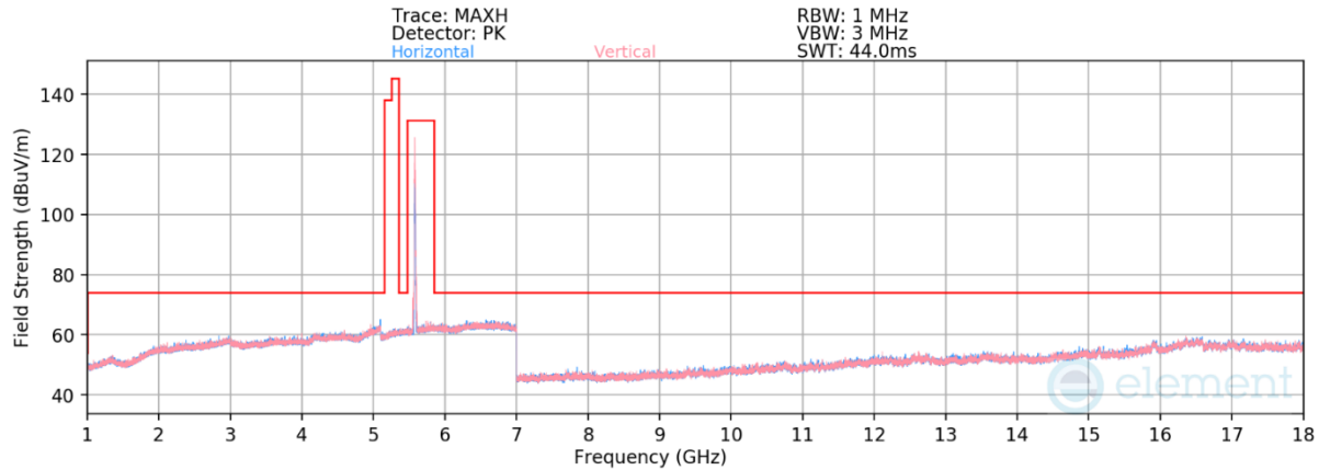
Plot 7-168. Radiated Spurious Emissions above 1GHz CDD (11be Ch.116 — RU52)
