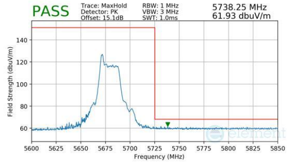
Plot 7-200. Antenna WF8 (Peak, RU26, Index 0, Ch.136, MCS11)
