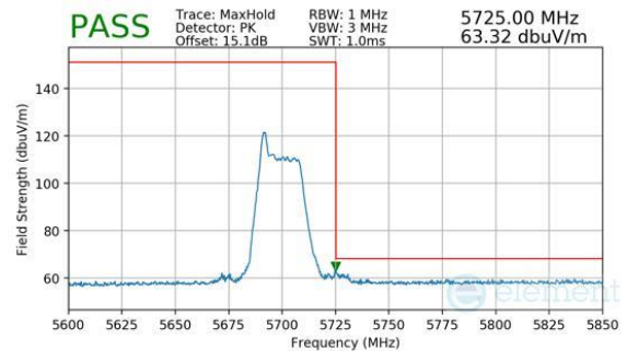
Plot 7-202. Antenna WF8 (Peak, RU26, Index 0, Ch.140, MCS11)
