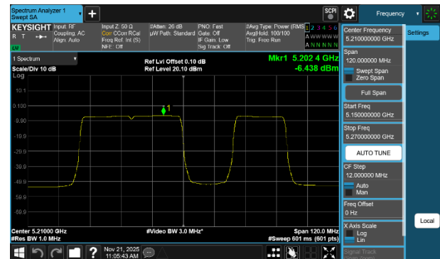
Plot 7-149 PSD CDD Antenna WF7a (80MHz BW 802.11be(RU) RU484+242 Index92 - Ch.42)
