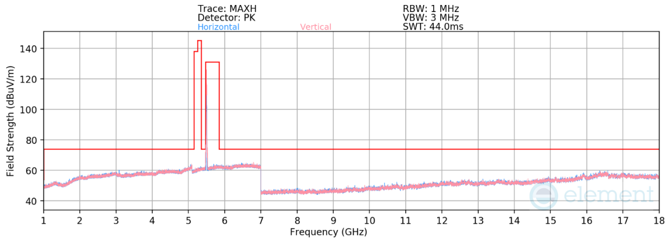
Plot 7-167. Radiated Spurious Emissions above 1GHz CDD (11be Ch.100 — RU52)
