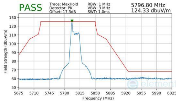
Plot 7-210. Antenna WF8 (Peak, RU26, Index 0, Ch.161, MCS11)
