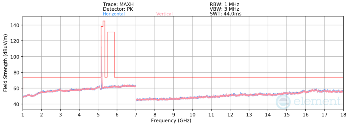
Plot 7-160. Radiated Spurious Emissions above 1GHz CDD (11be Ch.40 — RU26)
