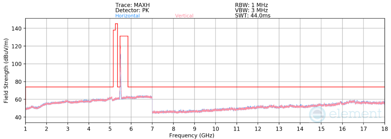
Plot 7-183. Radiated Spurious Emissions above 1GHz CDD (11be – Ch.100 – RU242)
