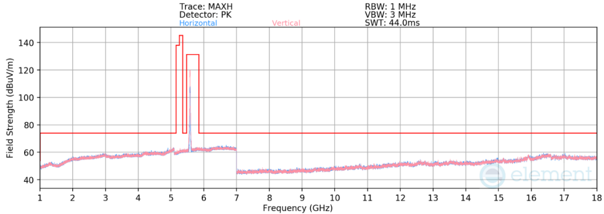
Plot 7-184. Radiated Spurious Emissions above 1GHz CDD (11be - Ch.116 - RU242)
