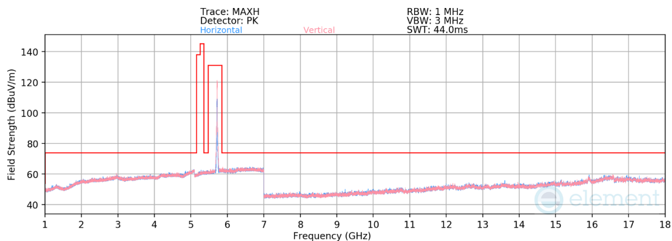
Plot 7-186. Radiated Spurious Emissions above 1GHz CDD (11be – Ch.144 – RU242)
