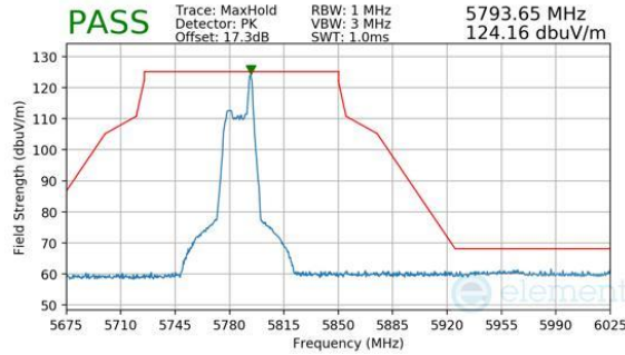
Plot 7-209. Antenna WF8 (Peak, RU26, Index 8, Ch.157, MCS11)
