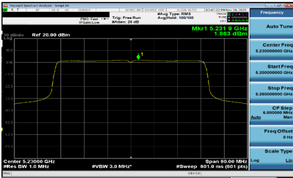
Plot 7-152 PSD CDD Antenna WF8 (40MHz BW 802.11be(RU) RU484 Index65 - Ch.46)
