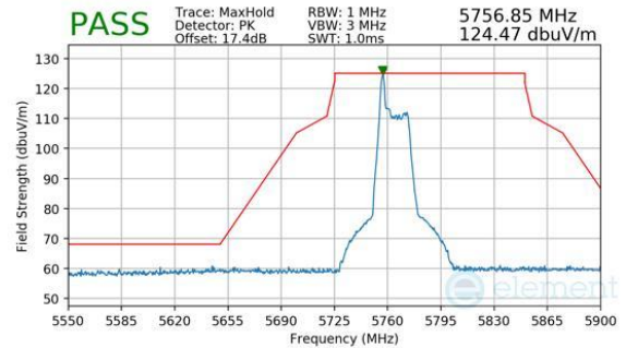
Plot 7-206. Antenna WF8 (Peak, RU26, Index 0, Ch.153, MCS11)
