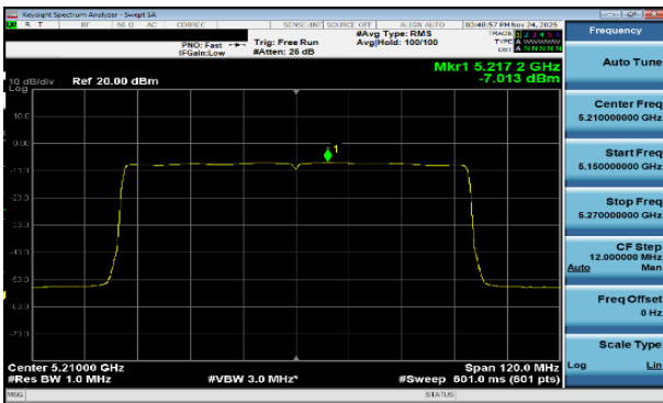
Plot 7-153 PSD CDD Antenna WF8 (80MHz BW 802.11be(RU) RU996 Index67 - Ch.42)
