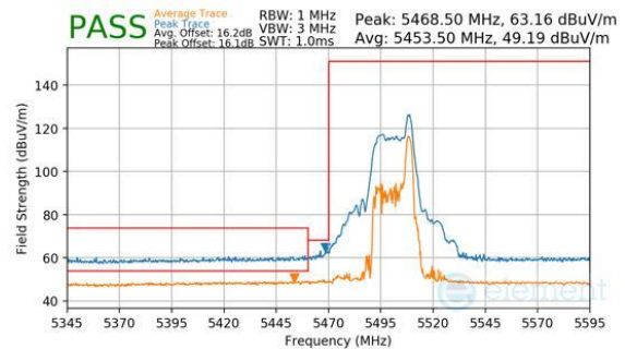
Plot 7-196. Antenna WF8 (Peak & Average, RU26, Index 8, Ch.100, MCS11)
