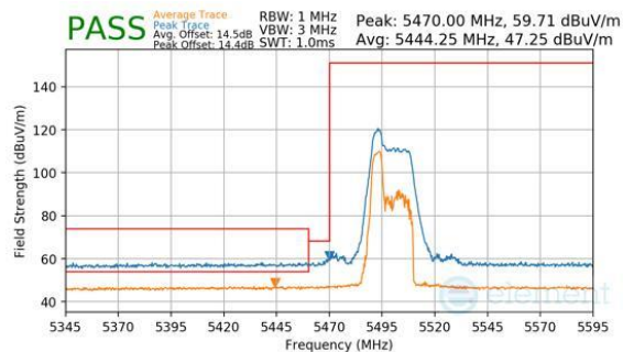
Plot 7-216. Antenna WF8 (Peak & Average, RU52, Index 37, Ch.100, MCS11)
