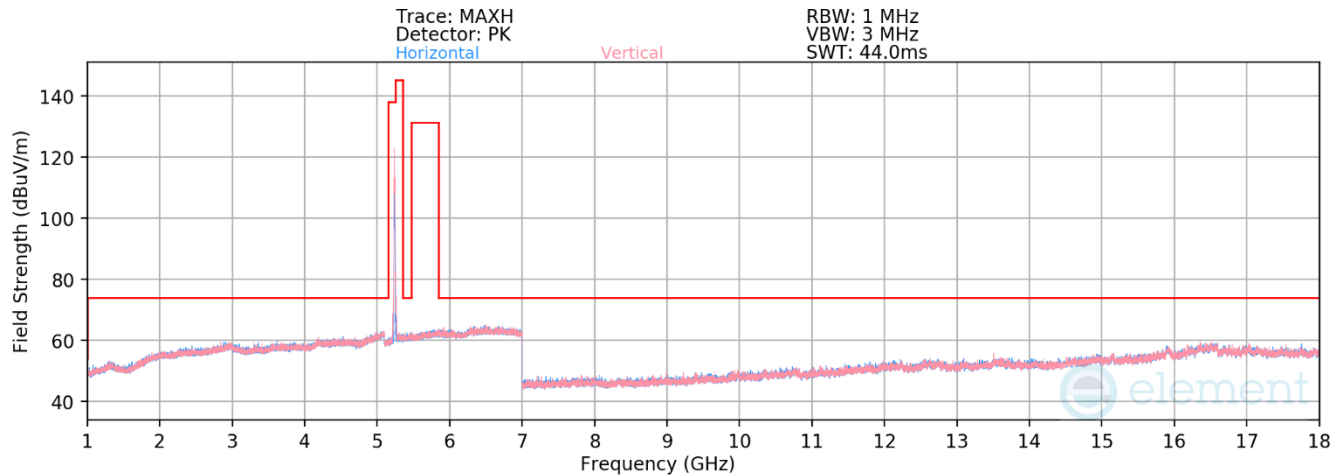
Plot 7-162. Radiated Spurious Emissions above 1GHz CDD (11be Ch.48 — RU26)
