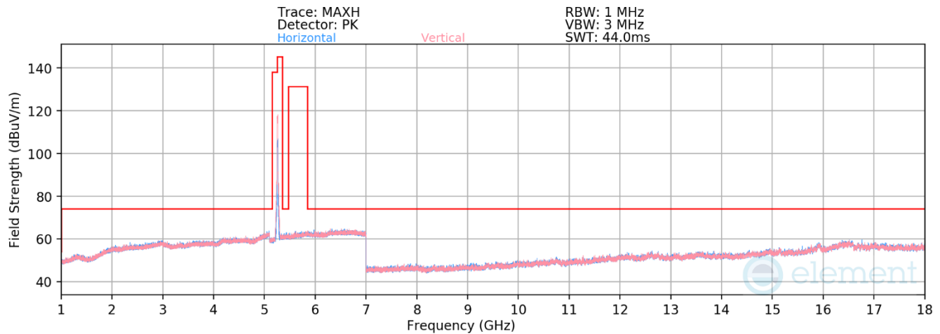
Plot 7-179. Radiated Spurious Emissions above 1GHz CDD (11be – Ch.52 – RU242)
