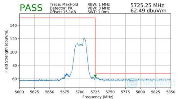
Plot 7-219. Antenna WF8 (Peak, RU52, Index 40, Ch.140, MCS11)
