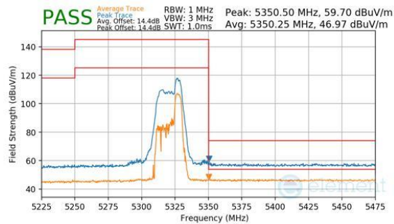
Plot 7-215. Antenna WF8 (Peak & Average, RU52, Index 40, Ch.64, MCS11)
