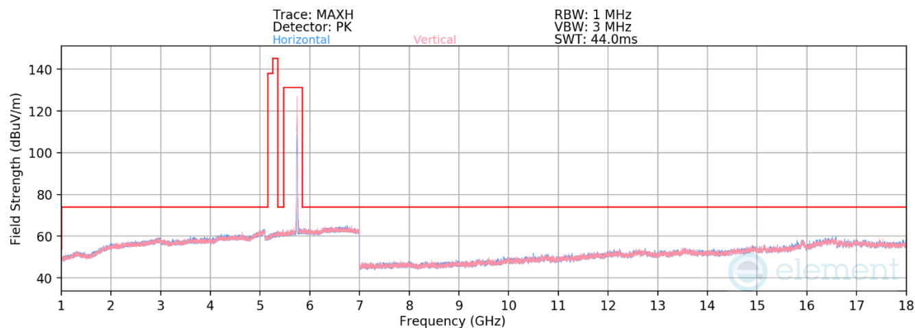
Plot 7-171. Radiated Spurious Emissions above 1GHz CDD (11be Ch.149 — RU26)
