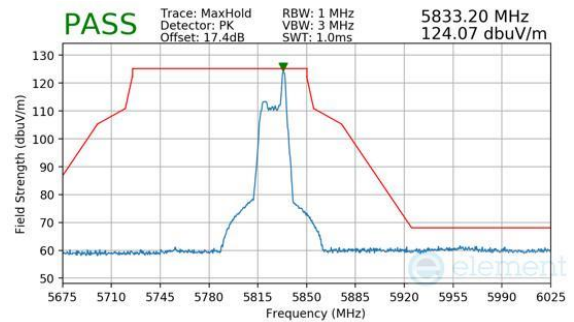
Plot 7-213. Antenna WF8 (Peak, RU26, Index 8, Ch.165, MCS11)
