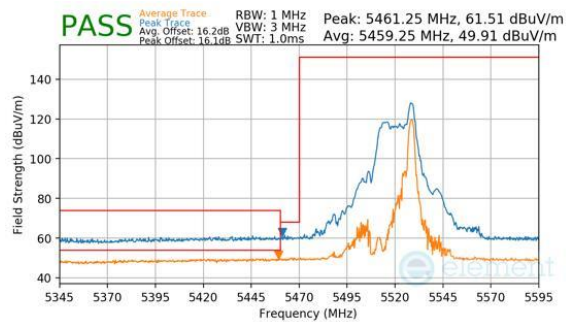
Plot 7-198. Antenna WF8 (Peak & Average, RU26, Index 8, Ch.104, MCS11)
