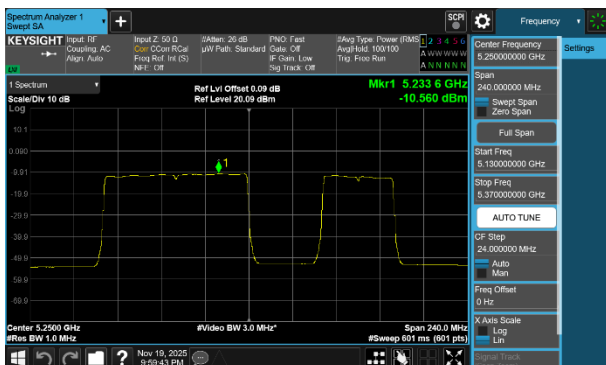
Plot 7-147 PSD CDD Antenna WF8 (160MHz BW 802.11be(RU) RU996+484 Index94 - Ch.50)
