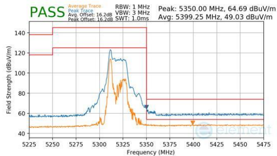
Plot 7-193. Antenna WF8 (Peak & Average, RU26, Index 0, Ch.64, MCS11)
