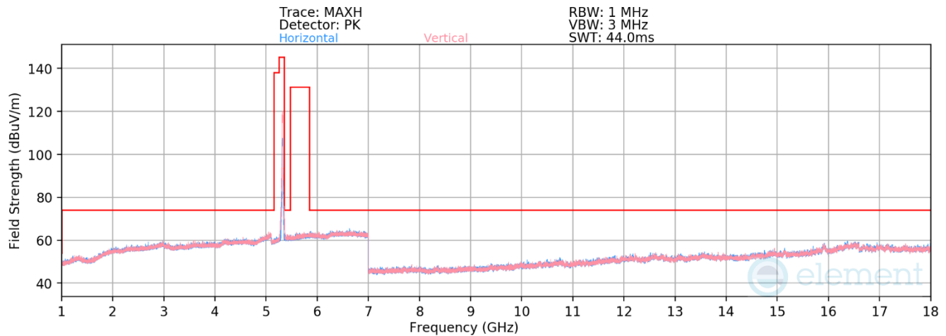
Plot 7-182. Radiated Spurious Emissions above 1GHz CDD (11be – Ch.64 – RU242)
