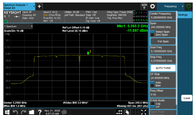
Plot 7-158 PSD CDD Antenna WF7a (160MHz BW 802.11be(RU) RU996X2 Index68 - Ch.50)
