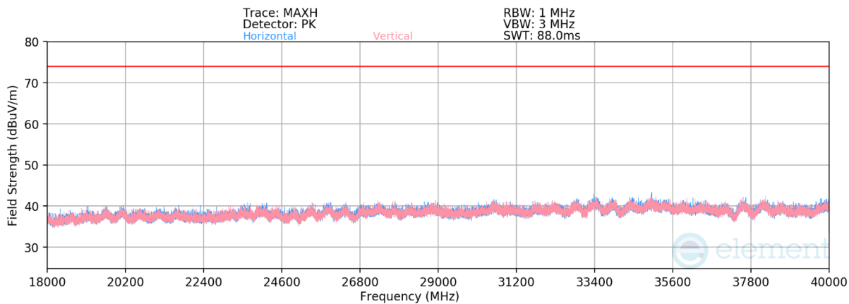
Plot 7-185. Radiated Spurious Emissions 18 GHz - 40GHz CDD (11be Ch.116 - RU242)
