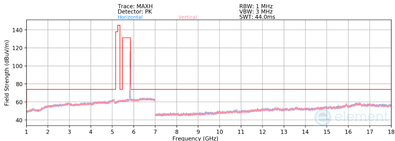
Plot 7-174. Radiated Spurious Emissions above 1GHz CDD (11be Ch.165 — RU26)
