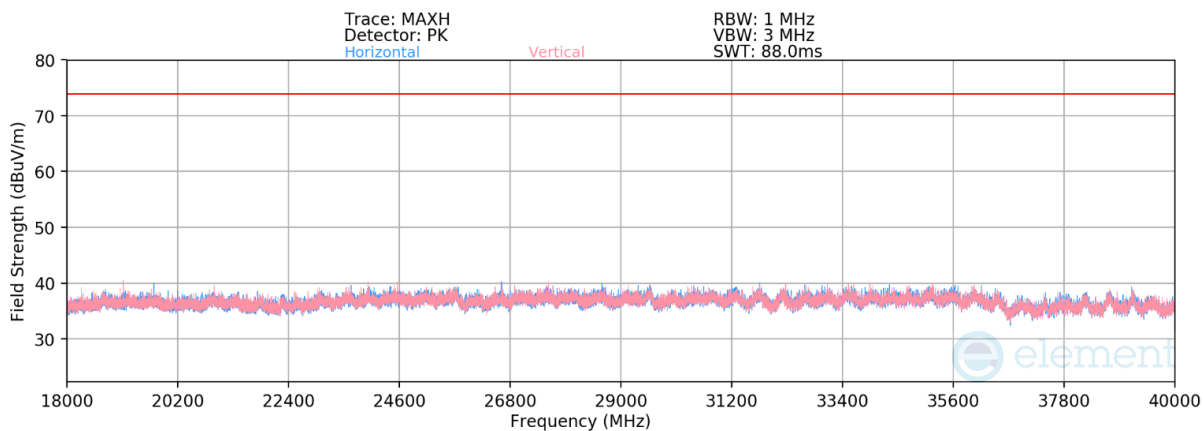
Plot 7-165. Radiated Spurious Emissions 18 GHz - 40GHz CDD (11be Ch.56 — RU52)
