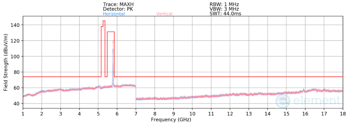
Plot 7-188. Radiated Spurious Emissions above 1GHz CDD (11be - Ch.157 - RU242)
