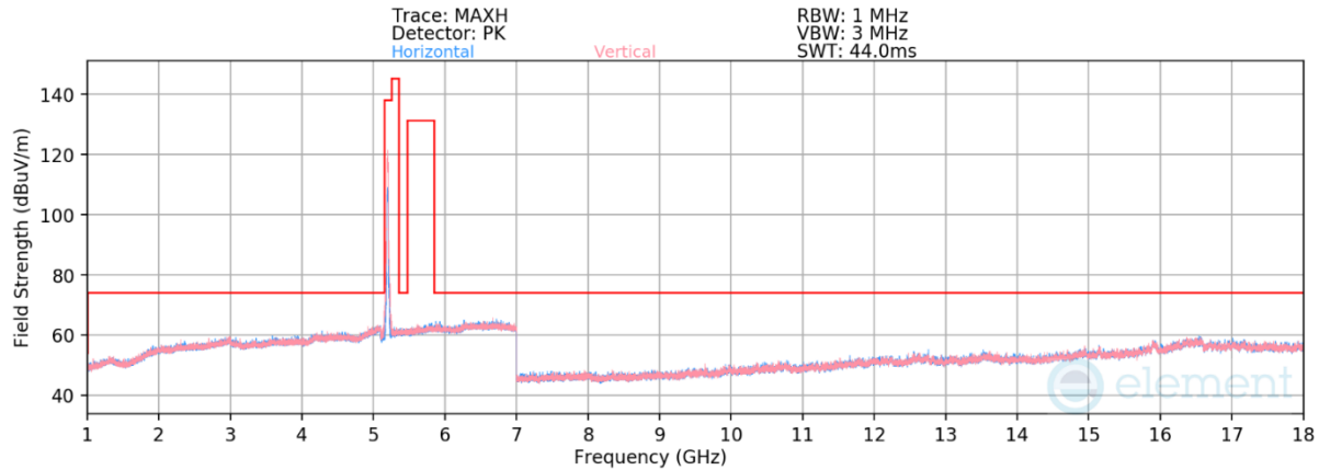
Plot 7-176. Radiated Spurious Emissions above 1GHz CDD (11be - Ch.40 - RU242)
