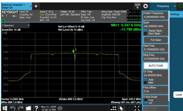
Plot 7-154 PSD CDD Antenna WF8 (160MHz BW 802.11be(RU) RU996X2 Index68 - Ch.50)
