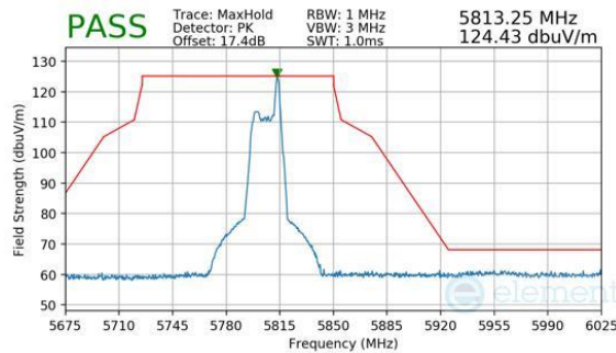
Plot 7-211. Antenna WF8 (Peak, RU26, Index 8, Ch.161, MCS11)
