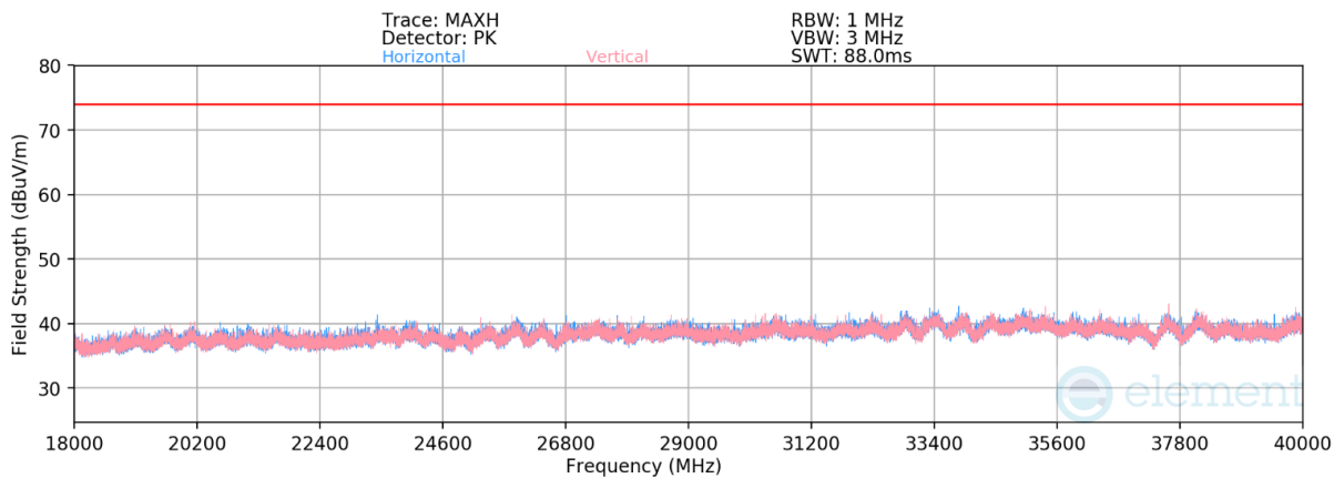
Plot 7-173. Radiated Spurious Emissions 18 GHz - 40GHz CDD (11be Ch.157 — RU26)
