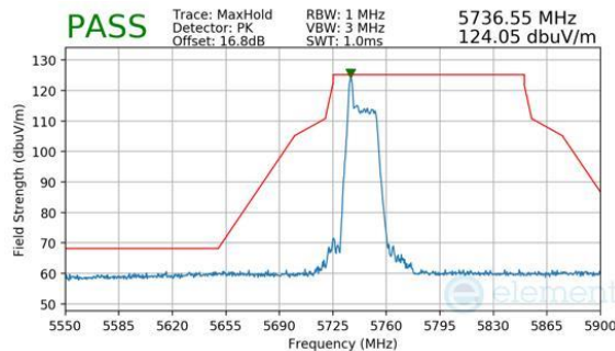
Plot 7-204. Antenna WF8 (Peak, RU26, Index 0, Ch.149, MCS11)
