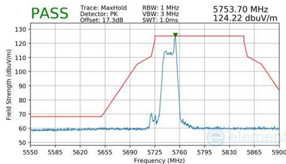
Plot 7-205. Antenna WF8 (Peak, RU26, Index 8, Ch.149, MCS11)
