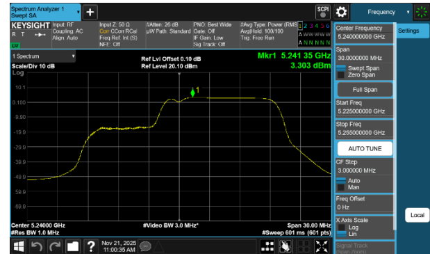
Plot 7-148 PSD CDD Antenna WF7a (20MHz BW 802.11be(RU) RU106+26 Index83 - Ch.48)
