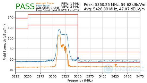
Plot 7-214. Antenna WF8 (Peak & Average, RU52, Index 37, Ch.64, MCS11)
