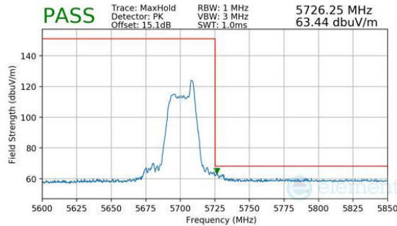
Plot 7-203. Antenna WF8 (Peak, RU26, Index 8, Ch.140, MCS11)
