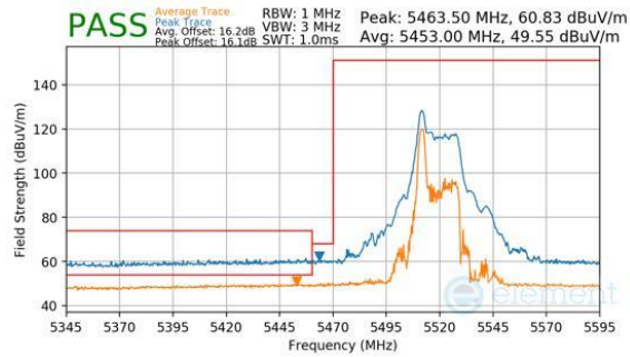
Plot 7-197. Antenna WF8 (Peak & Average, RU26, Index 0, Ch.104, MCS11)
