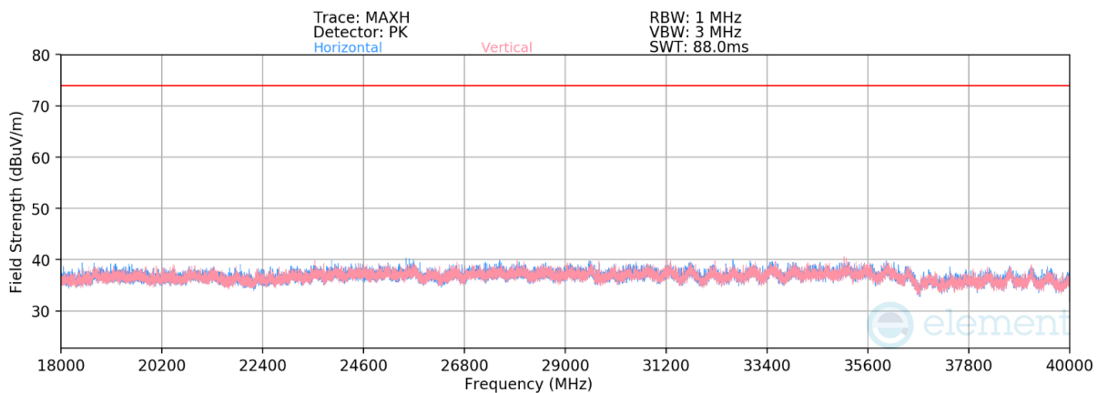
Plot 7-161. Radiated Spurious Emissions 18 GHz - 40GHz CDD (11be Ch.40 — RU26)
