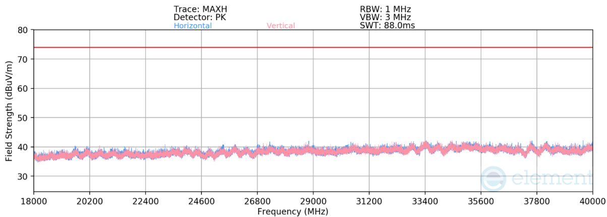
Plot 7-177. Radiated Spurious Emissions 18 GHz - 40GHz CDD (11be Ch.40 - RU242)
