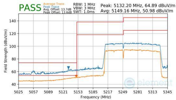
Plot 7-361. Antenna WF8 (Peak & Average, RU996+484, Index 94 (L), Ch.50, MCS11)
