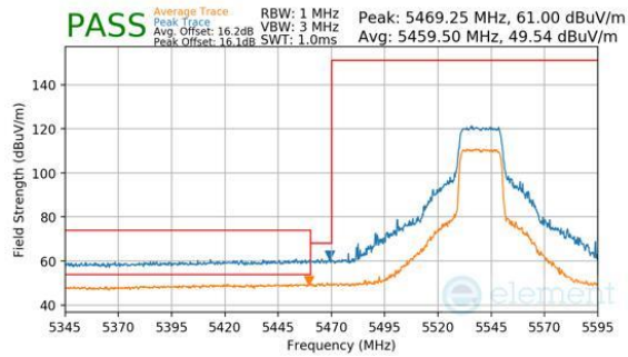
Plot 7-248. Antenna WF8 (Peak & Average, RU242, Index 61, Ch.108, MCS11)
