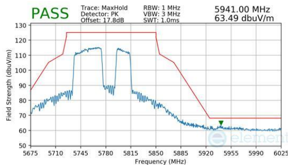
Plot 7-335. Antenna WF8 (Peak, RU484+242, Index 92, Ch.155, MCS11)
