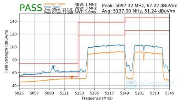
Plot 7-378. Antenna WF8 (Peak & Average, RU996+484+242, Index 96 (H), Ch.50, MCS11)
