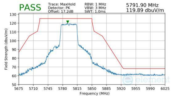
Plot 7-288. Antenna WF8 (Peak, RU484, Index 65, Ch.159, MCS11)
