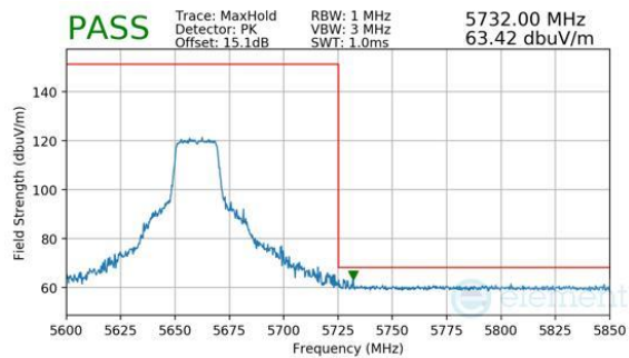
Plot 7-249. Antenna WF8 (Peak, RU242, Index 61, Ch.132, MCS11)
