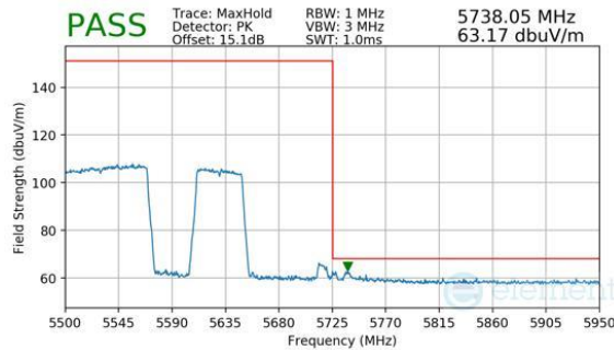
Plot 7-374. Antenna WF8 (Peak, RU996+484, Index 94 (H), Ch.114, MCS11)
