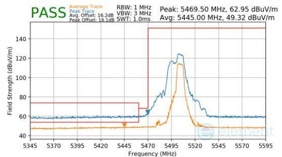
Plot 7-225. Antenna WF8 (Peak & Average, RU52+26, Index 72, Ch.100, MCS11)
