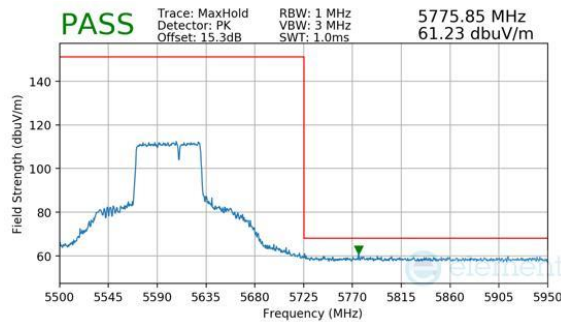
Plot 7-328. Antenna WF8 (Peak, RU484+242, Index 93, Ch.122, MCS11)
