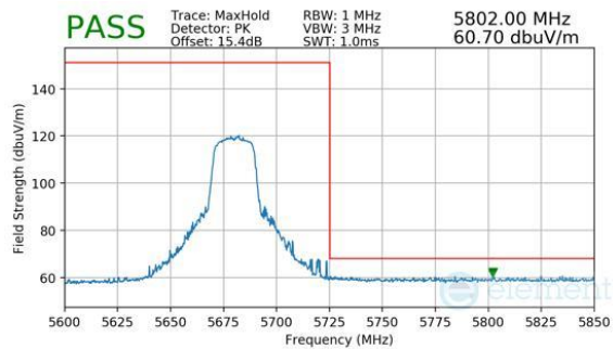
Plot 7-250. Antenna WF8 (Peak, RU242, Index 61, Ch.136, MCS11)
