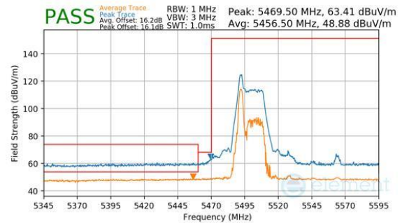
Plot 7-259. Antenna WF8 (Peak & Average, RU26, Index 0, Ch.102, MCS11)
