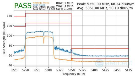
Plot 7-316. Antenna WF8 (Peak & Average, RU484+242, Index 93, Ch.58, MCS11)
