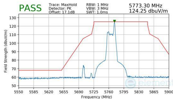
Plot 7-268. Antenna WF8 (Peak, RU26, Index 17, Ch.151, MCS11)
