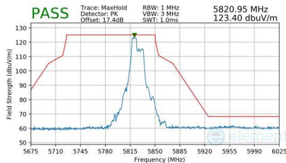
Plot 7-240. Antenna WF8 (Peak, RU52+26, Index 70, Ch.165, MCS11)
