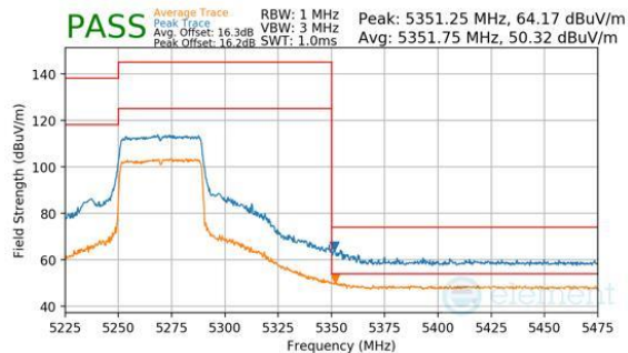
Plot 7-280. Antenna WF8 (Peak & Average, RU484, Index 65, Ch.54, MCS11)
