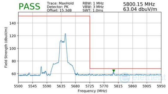
Plot 7-298. Antenna WF8 (Peak, RU26, Index 36, Ch.122, MCS11)
