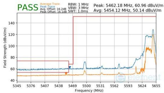
Plot 7-296. Antenna WF8 (Peak & Average, RU26, Index 36, Ch.122, MCS11)
