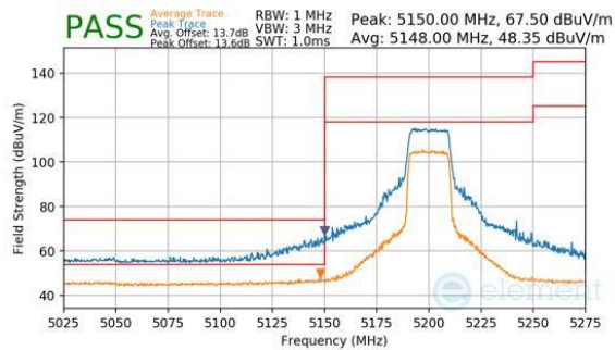
Plot 7-243. Antenna WF8 (Peak & Average, RU242, Index 61, Ch.40, MCS11)
