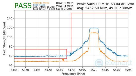
Plot 7-247. Antenna WF8 (Peak & Average, RU242, Index 61, Ch.104, MCS11)
