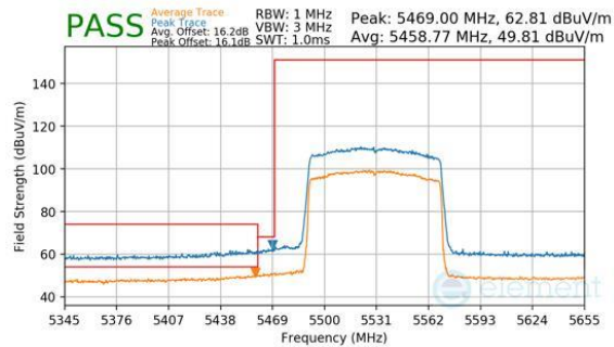
Plot 7-339. Antenna WF8 (Peak & Average, RU996, Index 67, Ch.106, MCS11)
