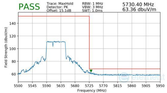
Plot 7-325. Antenna WF8 (Peak, RU484+242, Index 90, Ch.122, MCS11)
