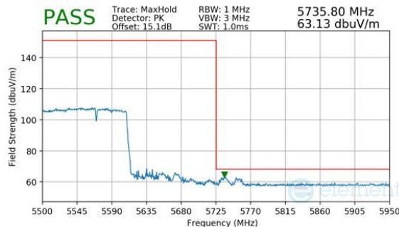
Plot 7-375. Antenna WF8 (Peak, RU996+484, Index 95 (H), Ch.114, MCS11)
