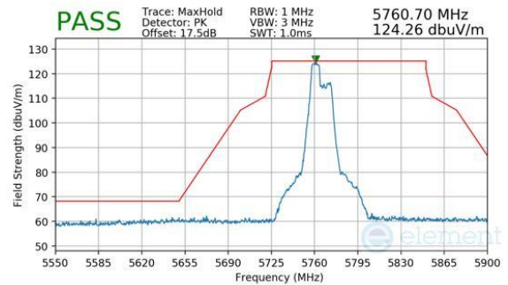
Plot 7-236. Antenna WF8 (Peak, RU52+26, Index 70, Ch.153, MCS11)
