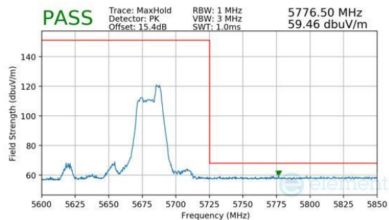
Plot 7-277. Antenna WF8 (Peak, RU52, Index 44, Ch.134, MCS11)
