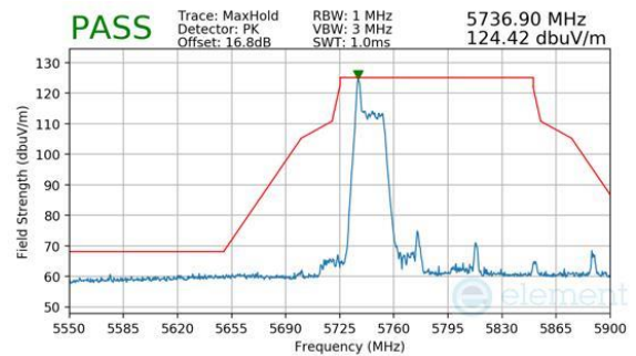
Plot 7-299. Antenna WF8 (Peak, RU26, Index 0, Ch.155, MCS11)
