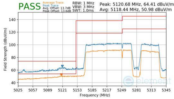
Plot 7-379. Antenna WF8 (Peak & Average, RU996+484+242, Index 97 (H), Ch.50, MCS11)
