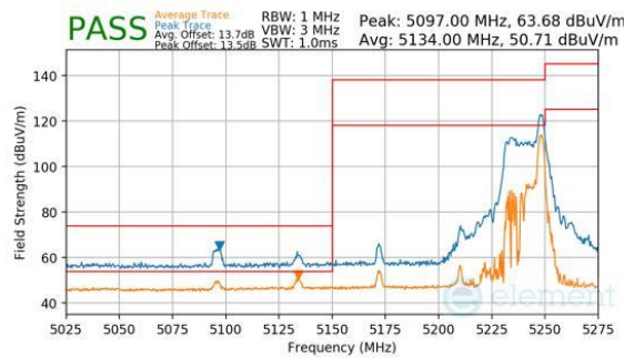
Plot 7-290. Antenna WF8 (Peak & Average, RU26, Index 36, Ch.42, MCS11)
