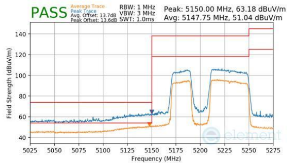
Plot 7-310. Antenna WF8 (Peak & Average, RU484+242, Index 91, Ch.42, MCS11)
