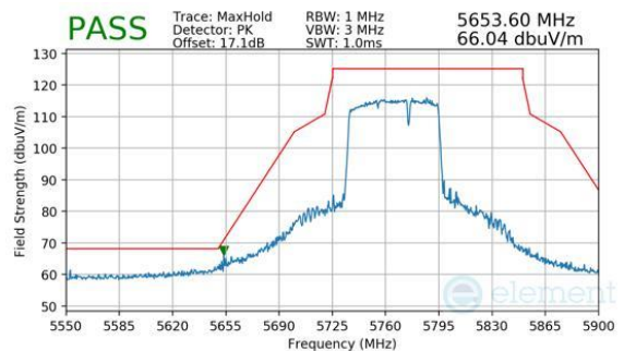
Plot 7-332. Antenna WF8 (Peak, RU484+242, Index 93, Ch.155, MCS11)
