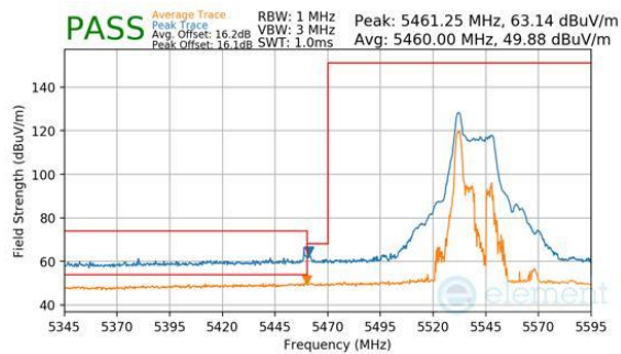
Plot 7-261. Antenna WF8 (Peak & Average, RU26, Index 0, Ch.110, MCS11)
