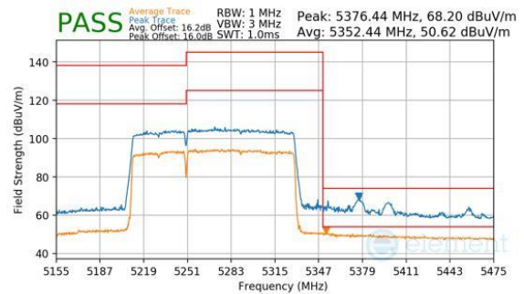
Plot 7-365. Antenna WF8 (Peak & Average, RU996+484, Index 94 (L), Ch.50, MCS11)
