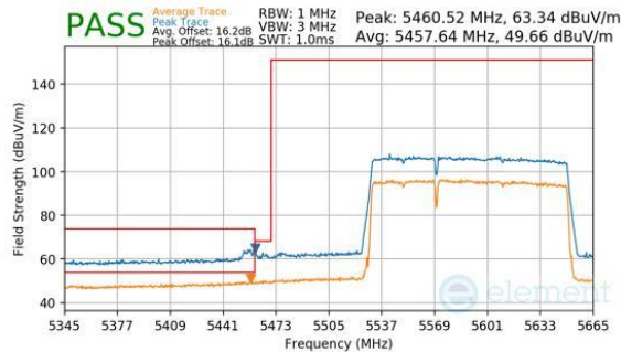
Plot 7-369. Antenna WF8 (Peak & Average, RU996+484, Index 94 (L), Ch.114, MCS11)
