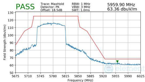
Plot 7-343. Antenna WF8 (Peak, RU996, Index 67, Ch.155, MCS11)
