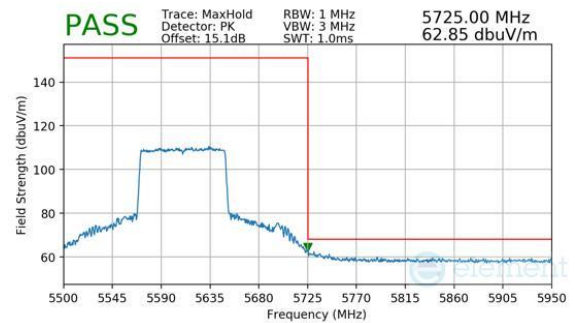
Plot 7-341. Antenna WF8 (Peak, RU996, Index 67, Ch.122, MCS11)
