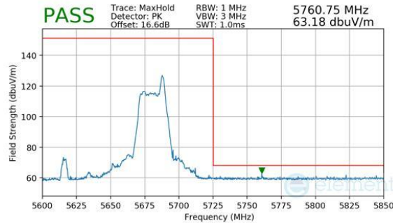
Plot 7-266. Antenna WF8 (Peak, RU26, Index 17, Ch.134, MCS11)
