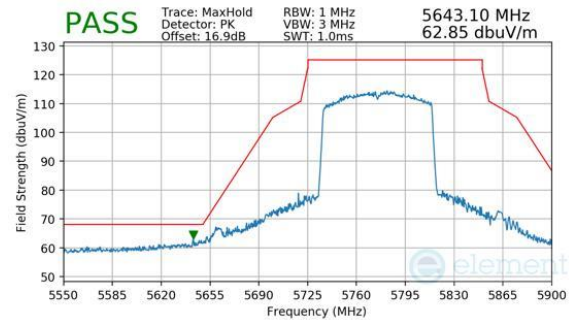
Plot 7-342. Antenna WF8 (Peak, RU996, Index 67, Ch.155, MCS11)
