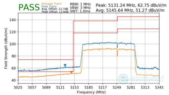
Plot 7-364. Antenna WF8 (Peak & Average, RU996+484, Index 95 (H), Ch.50, MCS11)
