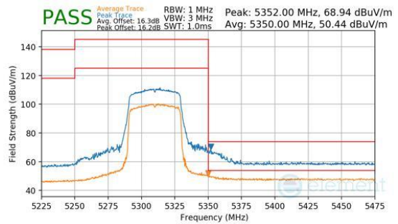
Plot 7-281. Antenna WF8 (Peak & Average, RU484, Index 65, Ch.62, MCS11)
