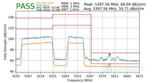
Plot 7-366. Antenna WF8 (Peak & Average, RU996+484, Index 94 (H), Ch.50, MCS11)
