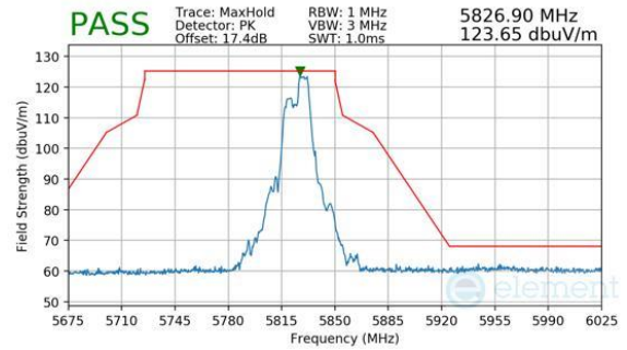
Plot 7-241. Antenna WF8 (Peak, RU52+26, Index 72, Ch.165, MCS11)
