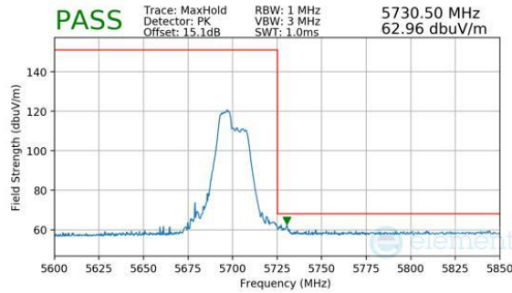
Plot 7-232. Antenna WF8 (Peak, RU52+26, Index 70, Ch.140, MCS11)
