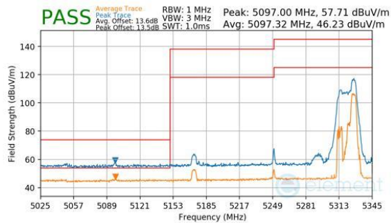
Plot 7-354. Antenna WF8 (Peak & Average, RU52, Index 52 (H), Ch.50, MCS11)
