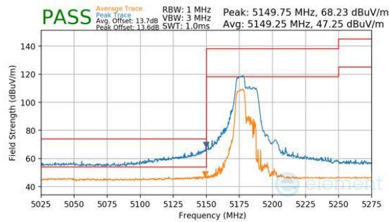
Plot 7-220. Antenna WF8 (Peak & Average, RU52+26, Index 70, Ch.36, MCS11)
