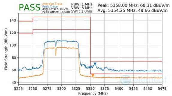
Plot 7-313. Antenna WF8 (Peak & Average, RU484+242, Index 90, Ch.58, MCS11)
