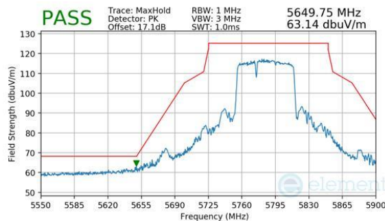
Plot 7-329. Antenna WF8 (Peak, RU484+242, Index 90, Ch.155, MCS11)
