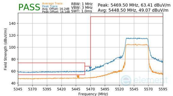
Plot 7-283. Antenna WF8 (Peak & Average, RU484, Index 65, Ch.110, MCS11)
