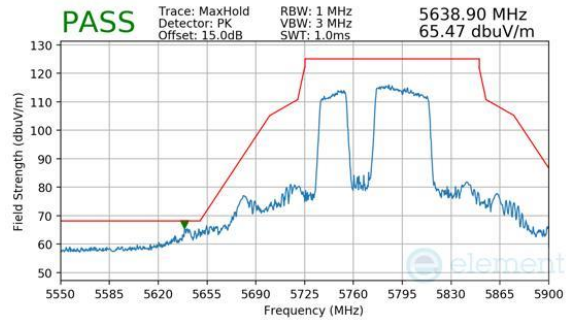
Plot 7-330. Antenna WF8 (Peak, RU484+242, Index 91, Ch.155, MCS11)
