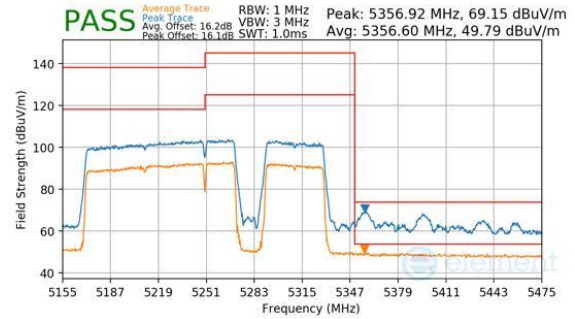
Plot 7-388. Antenna WF8 (Peak & Average, RU996+484+242, Index 97 (H), Ch.50, MCS11)
