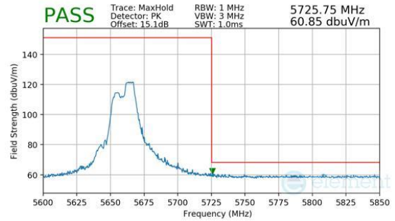
Plot 7-229. Antenna WF8 (Peak, RU52+26, Index 72, Ch.132, MCS11)
