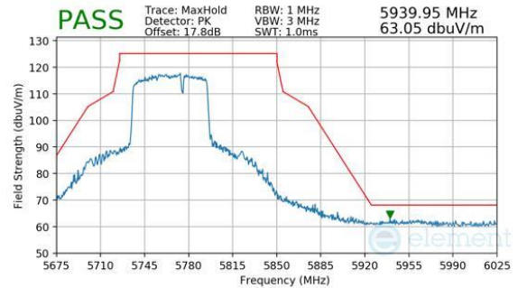
Plot 7-336. Antenna WF8 (Peak, RU484+242, Index 93, Ch.155, MCS11)
