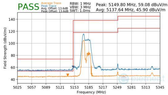
Plot 7-352. Antenna WF8 (Peak & Average, RU52, Index 37 (L), Ch.50, MCS11)
