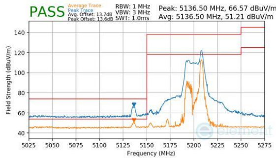
Plot 7-255. Antenna WF8 (Peak & Average, RU26, Index 17, Ch.38, MCS11)
