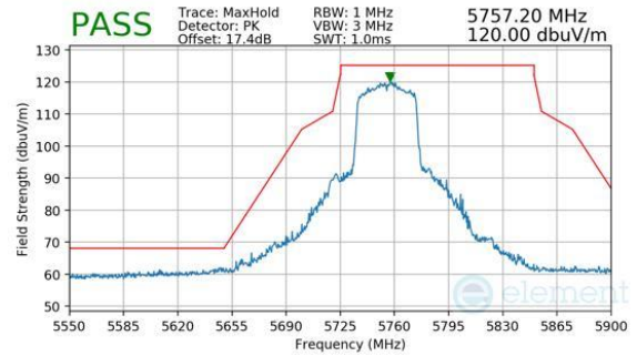
Plot 7-287. Antenna WF8 (Peak, RU484, Index 65, Ch.151, MCS11)
