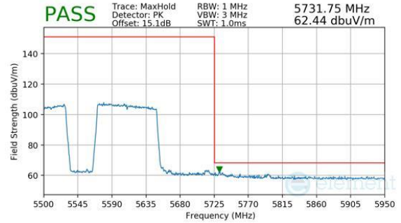
Plot 7-376. Antenna WF8 (Peak, RU996+484, Index 95 (L), Ch.114, MCS11)
