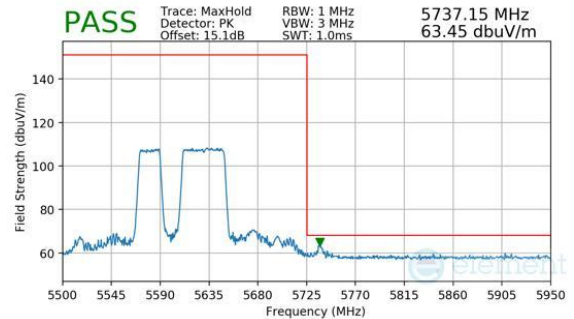
Plot 7-326. Antenna WF8 (Peak, RU484+242, Index 91, Ch.122, MCS11)
