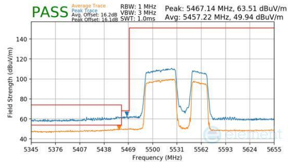
Plot 7-319. Antenna WF8 (Peak & Average, RU484+242, Index 92, Ch.106, MCS11)
