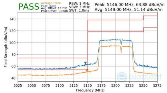
Plot 7-312. Antenna WF8 (Peak & Average, RU484+242, Index 93, Ch.42, MCS11)
