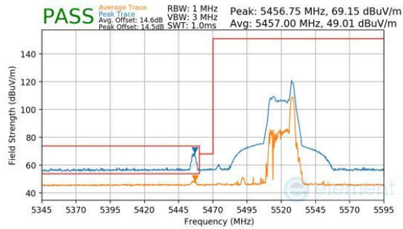
Plot 7-260. Antenna WF8 (Peak & Average, RU26, Index 17, Ch.102, MCS11)
