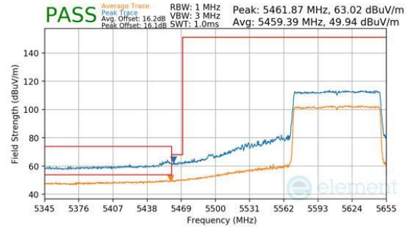
Plot 7-340. Antenna WF8 (Peak & Average, RU996, Index 67, Ch.122, MCS11)
