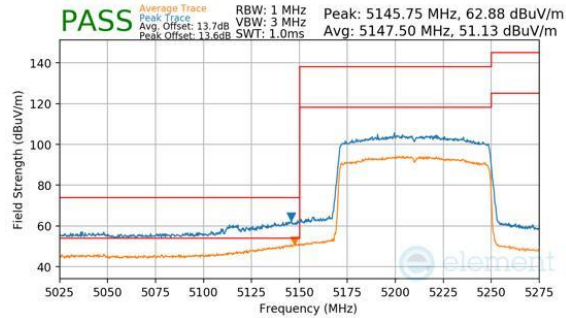
Plot 7-337. Antenna WF8 (Peak & Average, RU996, Index 67, Ch.42, MCS11)
