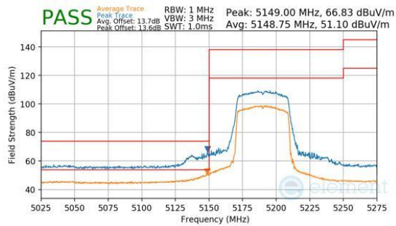
Plot 7-278. Antenna WF8 (Peak & Average, RU484, Index 65, Ch.38, MCS11)
