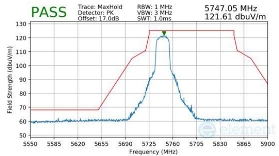
Plot 7-252. Antenna WF8 (Peak, RU242, Index 61, Ch.149, MCS11)
