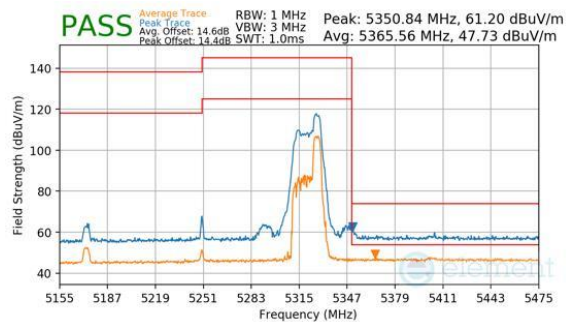
Plot 7-356. Antenna WF8 (Peak & Average, RU52, Index 52 (H), Ch.50, MCS11)
