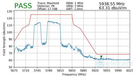
Plot 7-334. Antenna WF8 (Peak, RU484+242, Index 91, Ch.155, MCS11)
