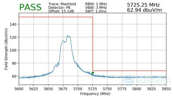
Plot 7-231. Antenna WF8 (Peak, RU52+26, Index 72, Ch.136, MCS11)
