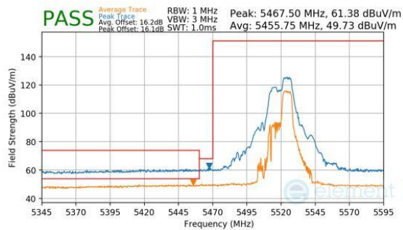
Plot 7-227. Antenna WF8 (Peak & Average, RU52+26, Index 72, Ch.104, MCS11)
