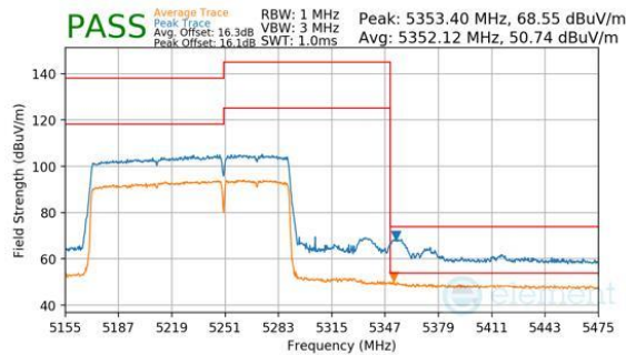
Plot 7-368. Antenna WF8 (Peak & Average, RU996+484, Index 95 (H), Ch.50, MCS11)
