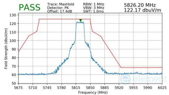
Plot 7-253. Antenna WF8 (Peak, RU242, Index 61, Ch.165, MCS11)
