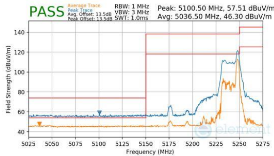
Plot 7-256. Antenna WF8 (Peak & Average, RU26, Index 17, Ch.46, MCS11)
