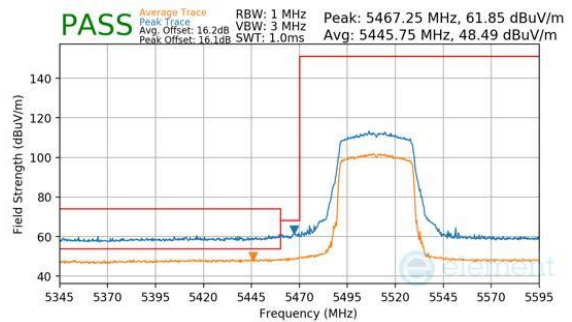
Plot 7-282. Antenna WF8 (Peak & Average, RU484, Index 65, Ch.102, MCS11)
