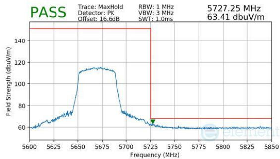
Plot 7-286. Antenna WF8 (Peak, RU484, Index 65, Ch.134, MCS11)
