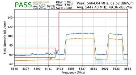
Plot 7-370. Antenna WF8 (Peak & Average, RU996+484, Index 94 (H), Ch.114, MCS11)
