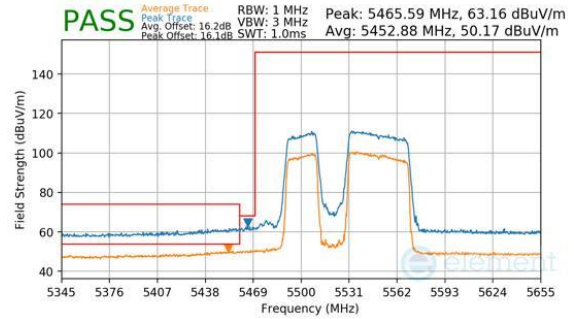
Plot 7-318. Antenna WF8 (Peak & Average, RU484+242, Index 91, Ch.106, MCS11)
