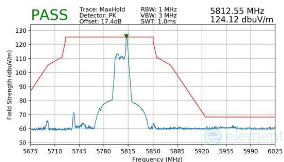
Plot 7-302. Antenna WF8 (Peak, RU26, Index 36, Ch.155, MCS11)
