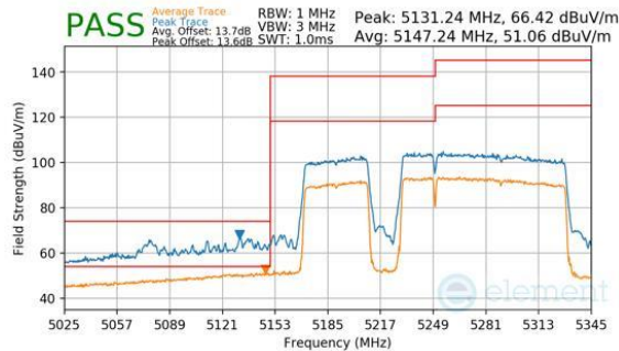
Plot 7-381. Antenna WF8 (Peak & Average, RU996+484+242, Index 98 (L), Ch.50, MCS11)
