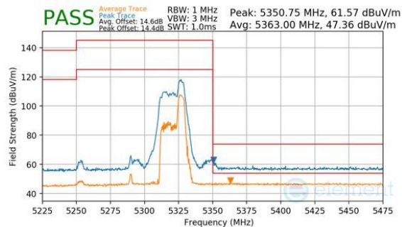
Plot 7-304. Antenna WF8 (Peak & Average, RU52, Index 52, Ch.58, MCS11)
