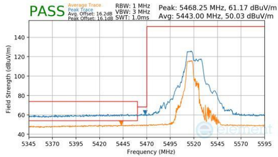
Plot 7-226. Antenna WF8 (Peak & Average, RU52+26, Index 70, Ch.104, MCS11)
