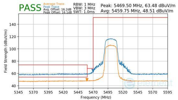
Plot 7-246. Antenna WF8 (Peak & Average, RU242, Index 61, Ch.100, MCS11)
