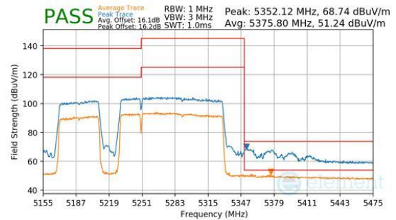
Plot 7-389. Antenna WF8 (Peak & Average, RU996+484+242, Index 98 (L), Ch.50, MCS11)
