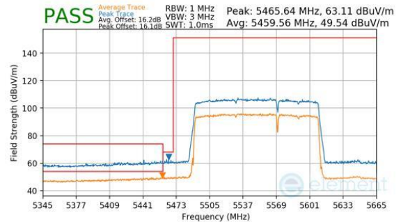
Plot 7-372. Antenna WF8 (Peak & Average, RU996+484, Index 95 (H), Ch.114, MCS11)
