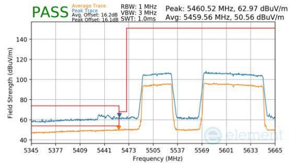
Plot 7-371. Antenna WF8 (Peak & Average, RU996+484, Index 95 (L), Ch.114, MCS11)
