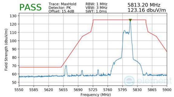
Plot 7-300. Antenna WF8 (Peak, RU26, Index 36, Ch.155, MCS11)
