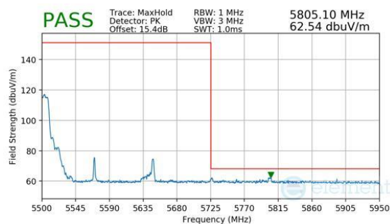
Plot 7-350. Antenna WF8 (Peak, RU26, Index 0 (L), Ch.114, MCS11)
