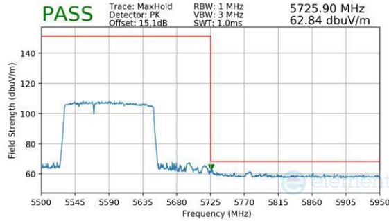
Plot 7-373. Antenna WF8 (Peak, RU996+484, Index 94 (L), Ch.114, MCS11)
