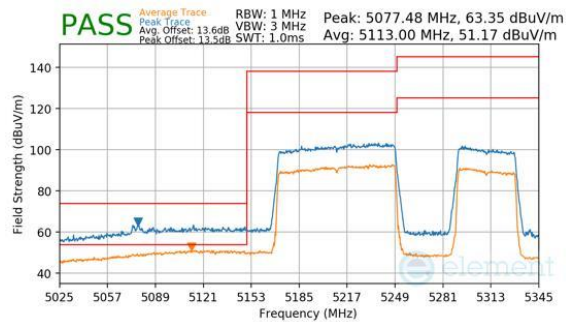
Plot 7-362. Antenna WF8 (Peak & Average, RU996+484, Index 94 (H), Ch.50, MCS11)
