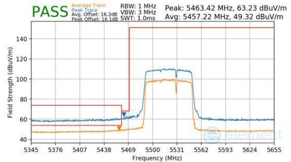
Plot 7-320. Antenna WF8 (Peak & Average, RU484+242, Index 93, Ch.106, MCS11)
