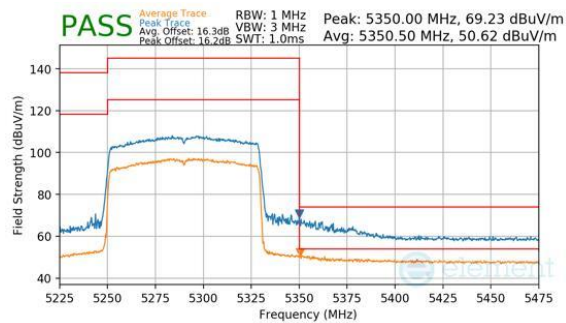
Plot 7-338. Antenna WF8 (Peak & Average, RU996, Index 67, Ch.58, MCS11)
