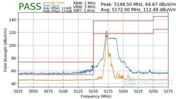
Plot 7-254. Antenna WF8 (Peak & Average, RU26, Index 0, Ch.38, MCS11)
