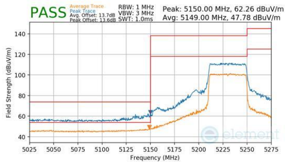
Plot 7-279. Antenna WF8 (Peak & Average, RU484, Index 65, Ch.46, MCS11)
