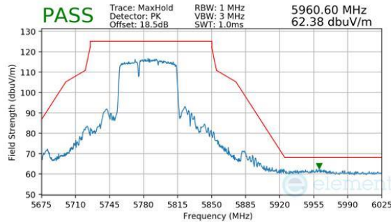
Plot 7-333. Antenna WF8 (Peak, RU484+242, Index 90, Ch.155, MCS11)
