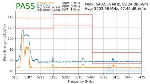
Plot 7-355. Antenna WF8 (Peak & Average, RU52, Index 37 (L), Ch.50, MCS11)
