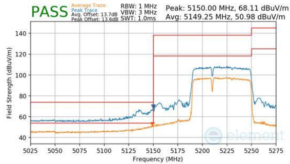
Plot 7-309. Antenna WF8 (Peak & Average, RU484+242, Index 90, Ch.42, MCS11)
