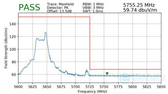
Plot 7-264. Antenna WF8 (Peak, RU26, Index 17, Ch.126, MCS11)
