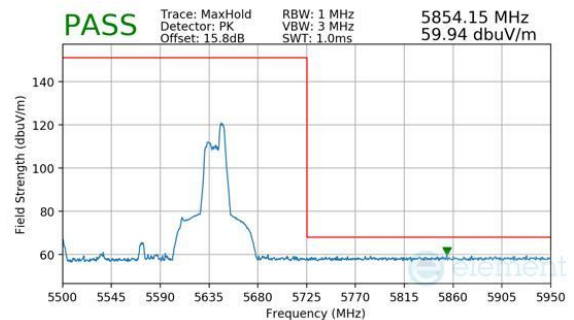
Plot 7-308. Antenna WF8 (Peak, RU52, Index 52, Ch.122, MCS11)
