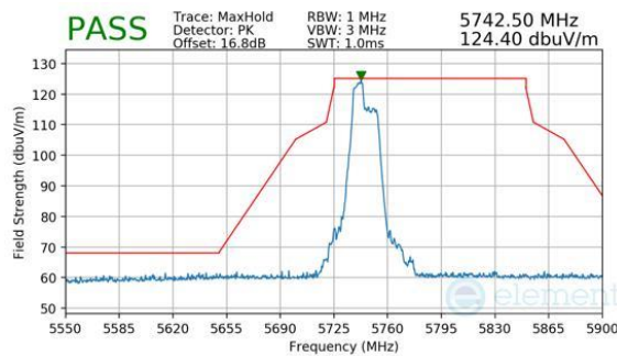
Plot 7-234. Antenna WF8 (Peak, RU52+26, Index 70, Ch.149, MCS11)
