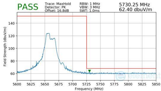
Plot 7-228. Antenna WF8 (Peak, RU52+26, Index 70, Ch.132, MCS11)
