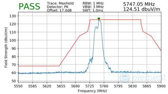
Plot 7-235. Antenna WF8 (Peak, RU52+26, Index 72, Ch.149, MCS11)
