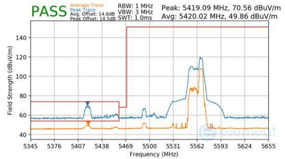
Plot 7-306. Antenna WF8 (Peak & Average, RU52, Index 52, Ch.106, MCS11)
