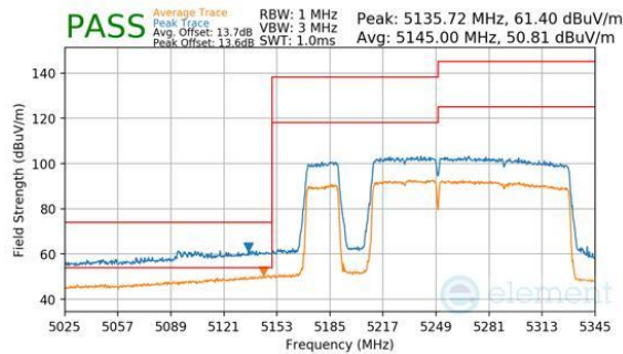
Plot 7-380. Antenna WF8 (Peak & Average, RU996+484+242, Index 97 (L), Ch.50, MCS11)
