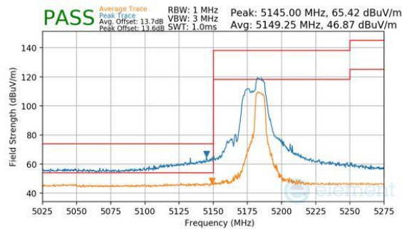
Plot 7-221. Antenna WF8 (Peak & Average, RU52+26, Index 72, Ch.36, MCS11)
