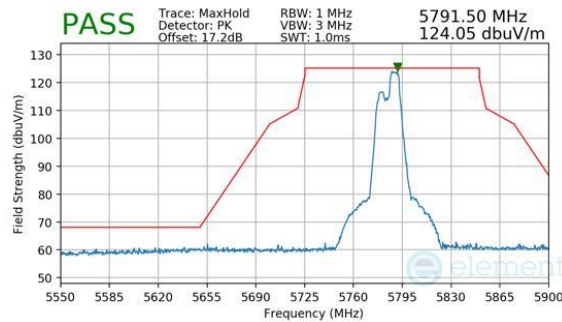
Plot 7-239. Antenna WF8 (Peak, RU52+26, Index 72, Ch.157, MCS11)
