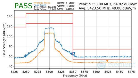
Plot 7-244. Antenna WF8 (Peak & Average, RU242, Index 61, Ch.60, MCS11)
