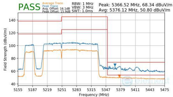
Plot 7-387. Antenna WF8 (Peak & Average, RU996+484+242, Index 97 (L), Ch.50, MCS11)
