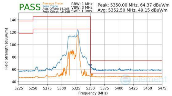
Plot 7-258. Antenna WF8 (Peak & Average, RU26, Index 17, Ch.62, MCS11)
