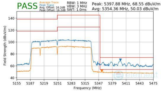
Plot 7-385. Antenna WF8 (Peak & Average, RU996+484+242, Index 96 (L), Ch.50, MCS11)
