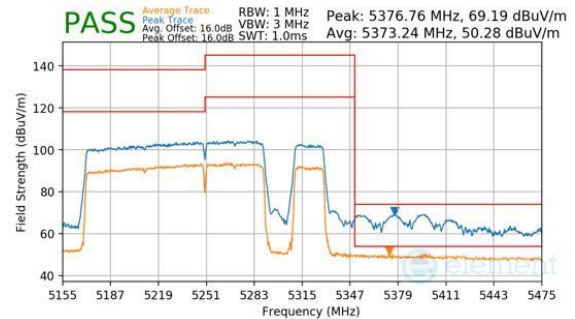
Plot 7-390. Antenna WF8 (Peak & Average, RU996+484+242, Index 98 (H), Ch.50, MCS11)
