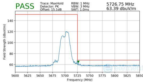
Plot 7-233. Antenna WF8 (Peak, RU52+26, Index 72, Ch.140, MCS11)
