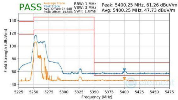
Plot 7-303. Antenna WF8 (Peak & Average, RU52, Index 37, Ch.58, MCS11)
