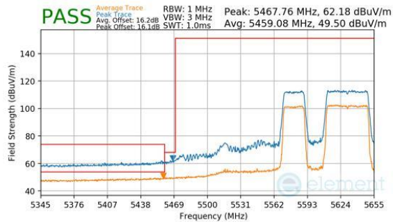
Plot 7-322. Antenna WF8 (Peak & Average, RU484+242, Index 91, Ch.122, MCS11)
