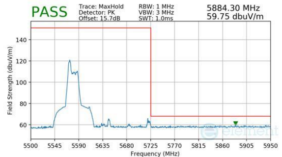
Plot 7-307. Antenna WF8 (Peak, RU52, Index 37, Ch.122, MCS11)
