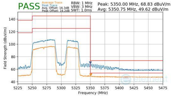
Plot 7-315. Antenna WF8 (Peak & Average, RU484+242, Index 92, Ch.58, MCS11)
