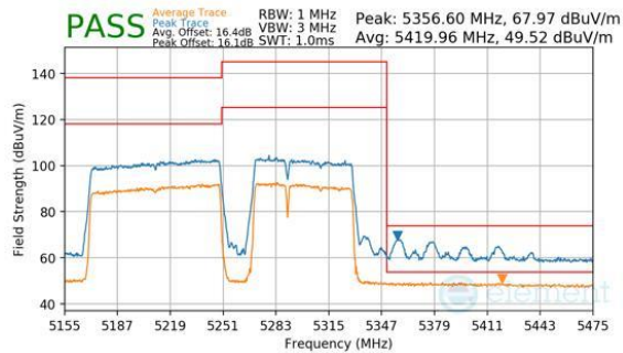
Plot 7-386. Antenna WF8 (Peak & Average, RU996+484+242, Index 96 (H), Ch.50, MCS11)
