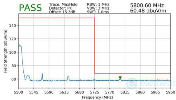
Plot 7-359. Antenna WF8 (Peak, RU52, Index 37 (L), Ch.114, MCS11)
