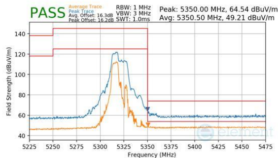
Plot 7-222. Antenna WF8 (Peak & Average, RU52+26, Index 70, Ch.64, MCS11)
