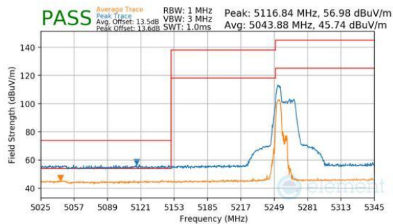
Plot 7-353. Antenna WF8 (Peak & Average, RU52, Index 37, Ch.50, MCS11)
