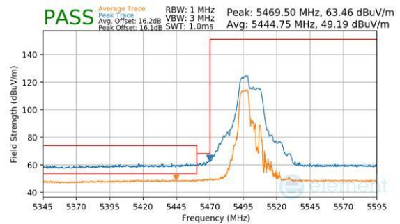
Plot 7-224. Antenna WF8 (Peak & Average, RU52+26, Index 70, Ch.100, MCS11)
