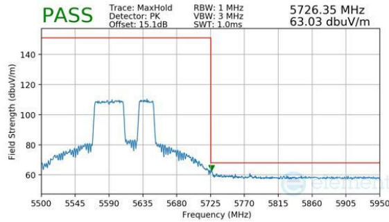
Plot 7-327. Antenna WF8 (Peak, RU484+242, Index 92, Ch.122, MCS11)
