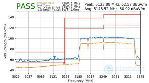
Plot 7-377. Antenna WF8 (Peak & Average, RU996+484+242, Index 96 (L), Ch.50, MCS11)
