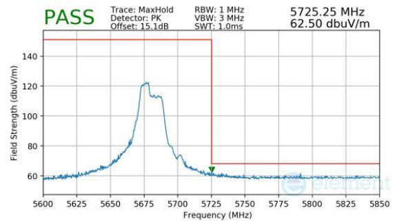
Plot 7-230. Antenna WF8 (Peak, RU52+26, Index 70, Ch.136, MCS11)
