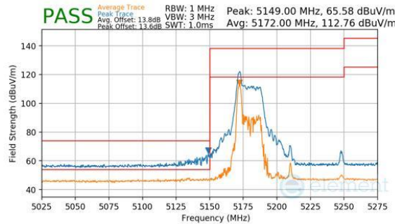
Plot 7-289. Antenna WF8 (Peak & Average, RU26, Index 0, Ch.42, MCS11)
