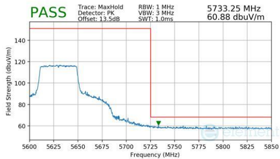
Plot 7-285. Antenna WF8 (Peak, RU484, Index 65, Ch.126, MCS11)
