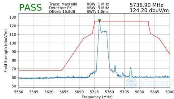
Plot 7-267. Antenna WF8 (Peak, RU26, Index 0, Ch.151, MCS11)
