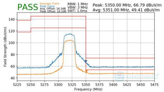
Plot 7-245. Antenna WF8 (Peak & Average, RU242, Index 61, Ch.64, MCS11)
