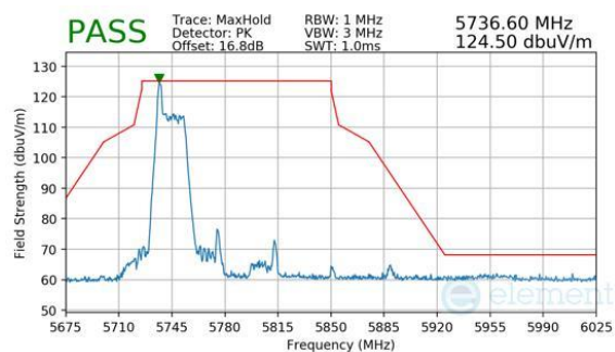
Plot 7-301. Antenna WF8 (Peak, RU26, Index 0, Ch.155, MCS11)
