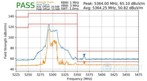
Plot 7-257. Antenna WF8 (Peak & Average, RU26, Index 0, Ch.62, MCS11)
