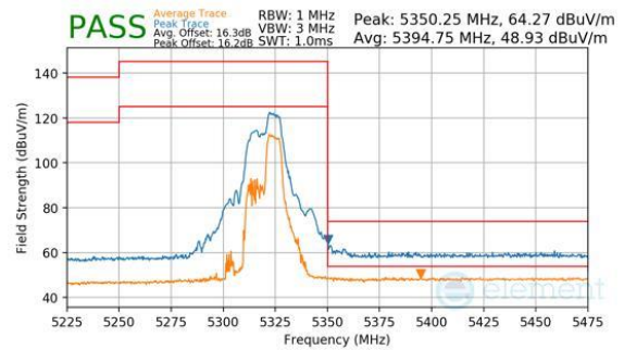
Plot 7-223. Antenna WF8 (Peak & Average, RU52+26, Index 72, Ch.64, MCS11)
