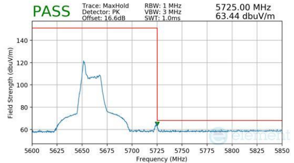
Plot 7-265. Antenna WF8 (Peak, RU26, Index 0, Ch.134, MCS11)
