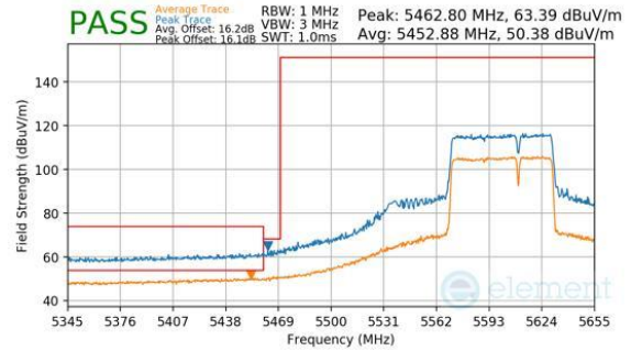
Plot 7-324. Antenna WF8 (Peak & Average, RU484+242, Index 93, Ch.122, MCS11)
