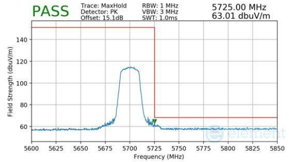
Plot 7-251. Antenna WF8 (Peak, RU242, Index 61, Ch.140, MCS11)
