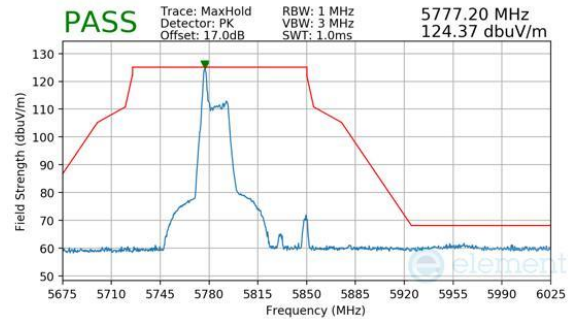
Plot 7-269. Antenna WF8 (Peak, RU26, Index 0, Ch.159, MCS11)
