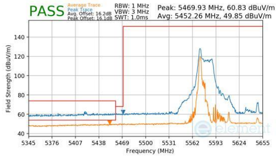
Plot 7-295. Antenna WF8 (Peak & Average, RU26, Index 0, Ch.122, MCS11)
