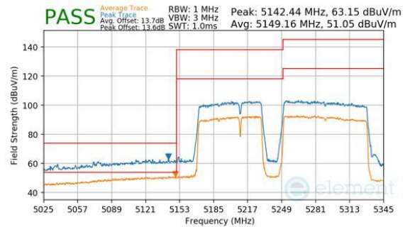
Plot 7-383. Antenna WF8 (Peak & Average, RU996+484+242, Index 99 (L), Ch.50, MCS11)
