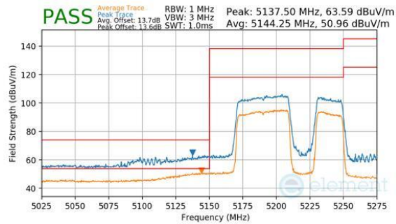
Plot 7-311. Antenna WF8 (Peak & Average, RU484+242, Index 92, Ch.42, MCS11)
