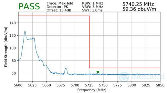
Plot 7-263. Antenna WF8 (Peak, RU26, Index 0, Ch.126, MCS11)
