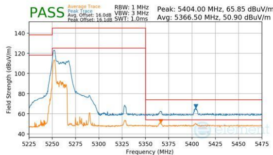
Plot 7-291. Antenna WF8 (Peak & Average, RU26, Index 0, Ch.58, MCS11)
