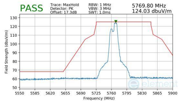
Plot 7-237. Antenna WF8 (Peak, RU52+26, Index 72, Ch.153, MCS11)
