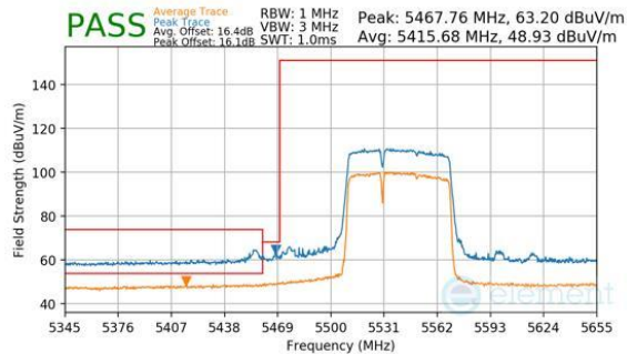
Plot 7-317. Antenna WF8 (Peak & Average, RU484+242, Index 90, Ch.106, MCS11)
