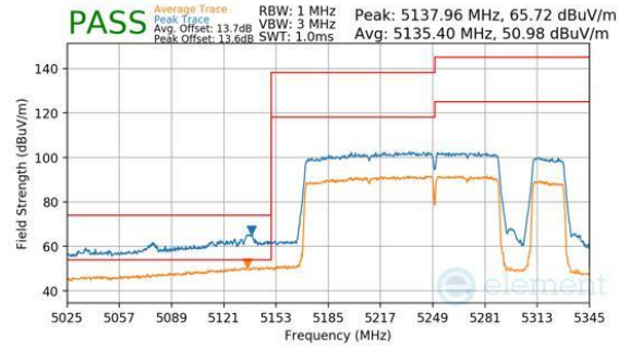
Plot 7-382. Antenna WF8 (Peak & Average, RU996+484+242, Index 98 (H), Ch.50, MCS11)
