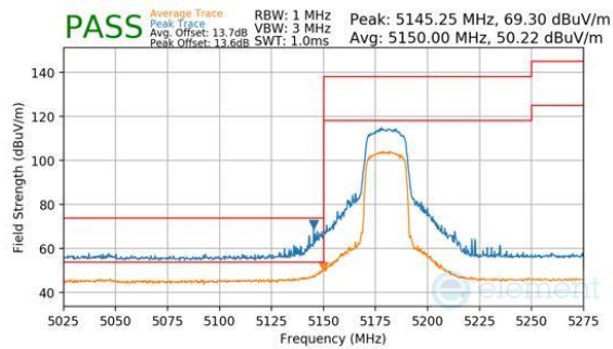
Plot 7-242. Antenna WF8 (Peak & Average, RU242, Index 61, Ch.36, MCS11)
