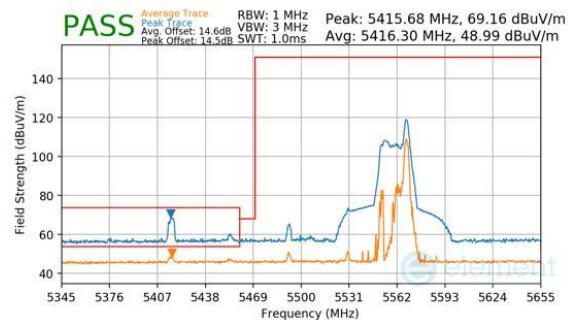
Plot 7-294. Antenna WF8 (Peak & Average, RU26, Index 36, Ch.106, MCS11)
