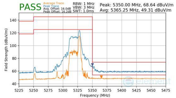
Plot 7-292. Antenna WF8 (Peak & Average, RU26, Index 36, Ch.58, MCS11)
