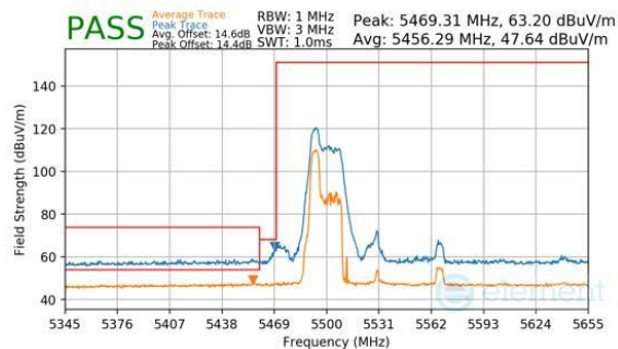
Plot 7-305. Antenna WF8 (Peak & Average, RU52, Index 37, Ch.106, MCS11)
