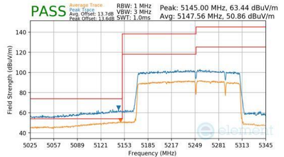
Plot 7-384. Antenna WF8 (Peak & Average, RU996+484+242, Index 99 (H), Ch.50, MCS11)
