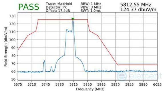
Plot 7-270. Antenna WF8 (Peak, RU26, Index 17, Ch.159, MCS11)
