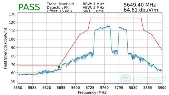
Plot 7-331. Antenna WF8 (Peak, RU484+242, Index 92, Ch.155, MCS11)
