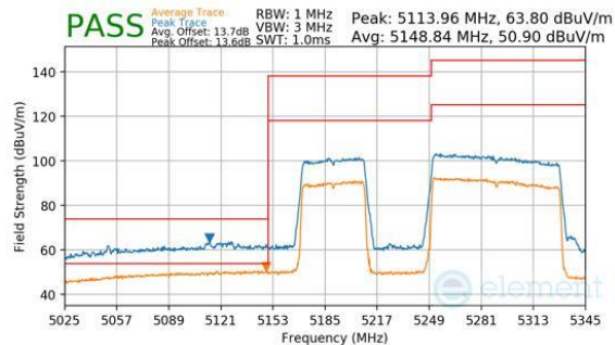
Plot 7-363. Antenna WF8 (Peak & Average, RU996+484, Index 95 (L), Ch.50, MCS11)
