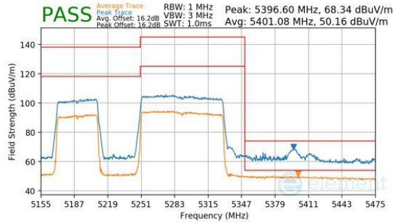
Plot 7-367. Antenna WF8 (Peak & Average, RU996+484, Index 95 (L), Ch.50, MCS11)
