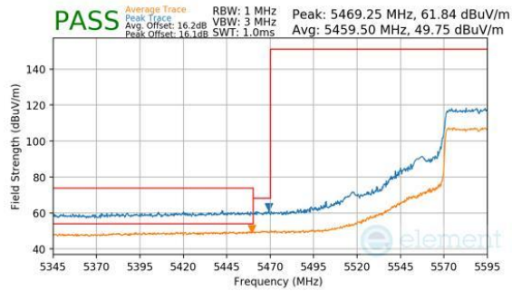
Plot 7-284. Antenna WF8 (Peak & Average, RU484, Index 65, Ch.118, MCS11)
