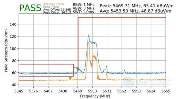
Plot 7-293. Antenna WF8 (Peak & Average, RU26, Index 0, Ch.106, MCS11)
