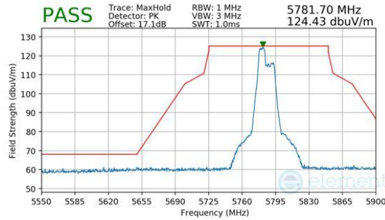
Plot 7-238. Antenna WF8 (Peak, RU52+26, Index 70, Ch.157, MCS11)
