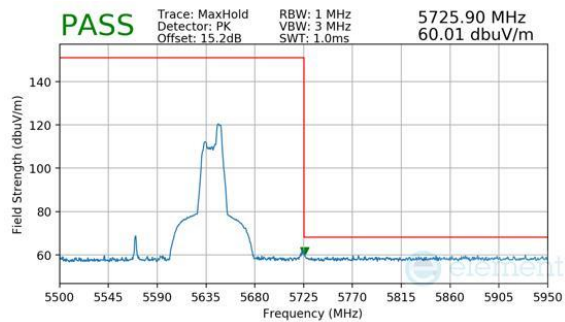
Plot 7-360. Antenna WF8 (Peak, RU52, Index 52 (H), Ch.114, MCS11)
