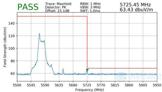
Plot 7-297. Antenna WF8 (Peak, RU26, Index 0, Ch.122, MCS11)
