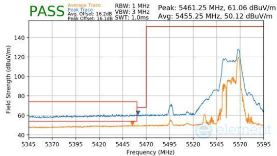
Plot 7-262. Antenna WF8 (Peak & Average, RU26, Index 17, Ch.110, MCS11)
