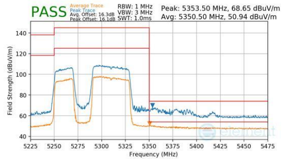
Plot 7-314. Antenna WF8 (Peak & Average, RU484+242, Index 91, Ch.58, MCS11)
