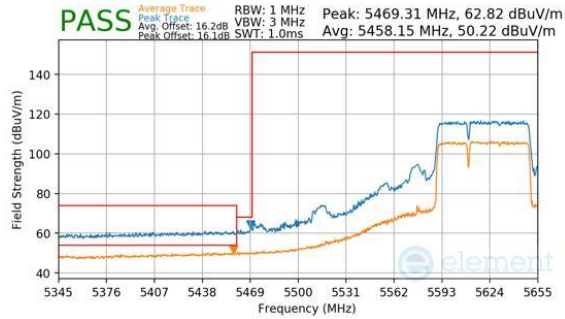
Plot 7-321. Antenna WF8 (Peak & Average, RU484+242, Index 90, Ch.122, MCS11)
