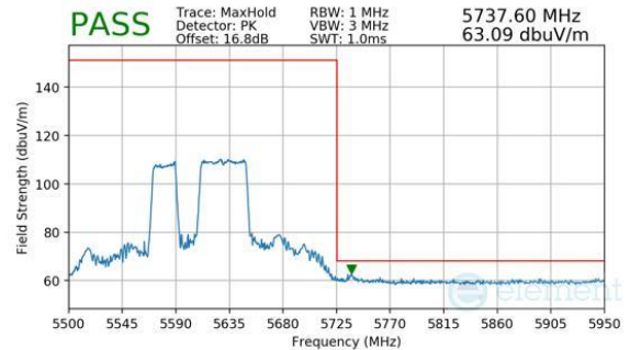
Plot 7-536. Antenna WF7a (Peak, RU484+242, Index 91, Ch.122, MCS11)
