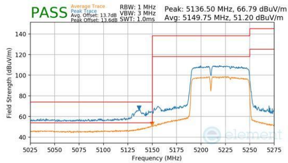
Plot 7-519. Antenna WF7a (Peak & Average, RU484+242, Index 90, Ch.42, MCS11)
