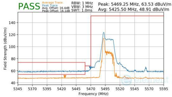
Plot 7-468. Antenna WF7a (Peak & Average, RU26, Index 0, Ch.102, MCS11)
