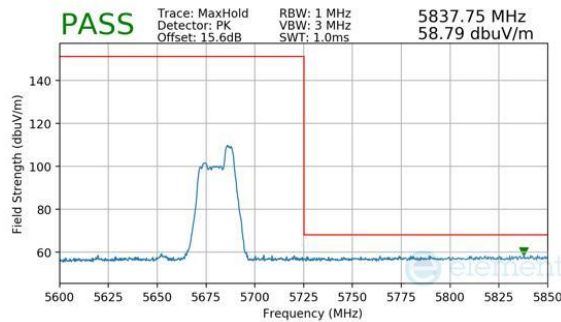
Plot 7-487. Antenna WF7a (Peak, RU52, Index 44, Ch.134, MCS11)
