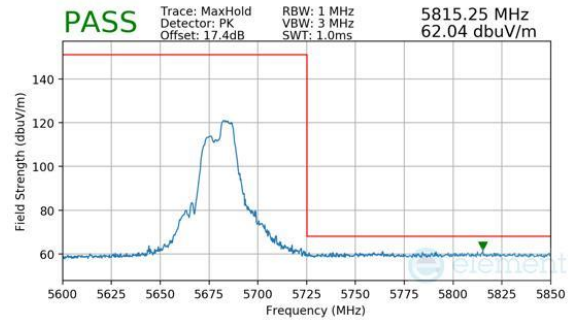
Plot 7-444. Antenna WF7a (Peak, RU52+26, Index 72, Ch.136, MCS11)
