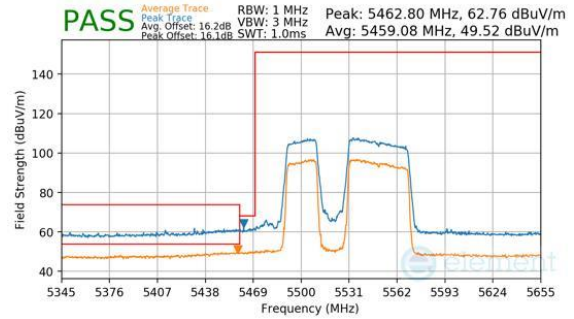
Plot 7-528. Antenna WF7a (Peak & Average, RU484+242, Index 91, Ch.106, MCS11)
