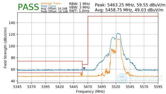
Plot 7-442. Antenna WF7a (Peak & Average, RU52+26, Index 72, Ch.104, MCS11)
