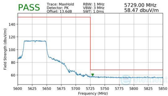
Plot 7-495. Antenna WF7a (Peak, RU484, Index 65, Ch.126, MCS11)
