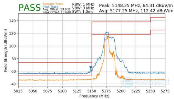
Plot 7-435. Antenna WF7a (Peak & Average, RU52+26, Index 70, Ch.36, MCS11)
