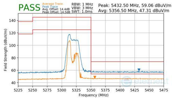
Plot 7-429. Antenna WF7a (Peak & Average, RU52, Index 37, Ch.64, MCS11)
