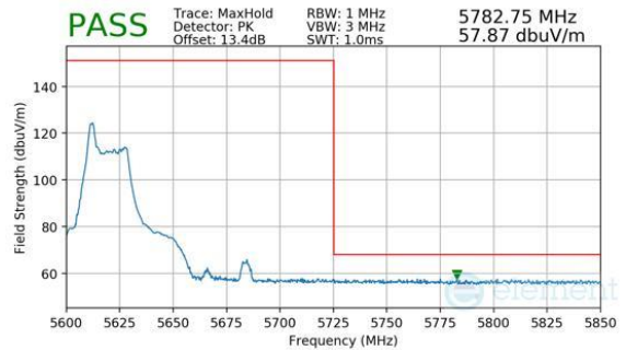
Plot 7-472. Antenna WF7a (Peak, RU26, Index 0, Ch.126, MCS11)
