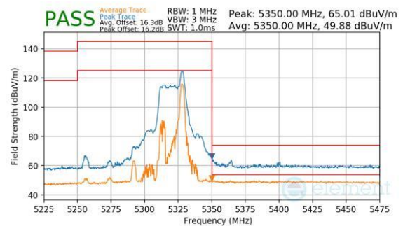
Plot 7-467. Antenna WF7a (Peak & Average, RU26, Index 17, Ch.62, MCS11)
