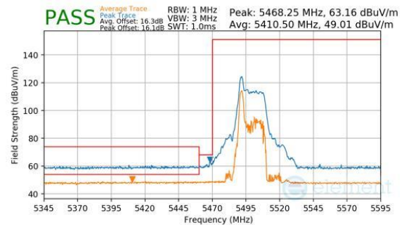
Plot 7-417. Antenna WF7a (Peak & Average, RU26, Index 0, Ch.100, MCS11)
