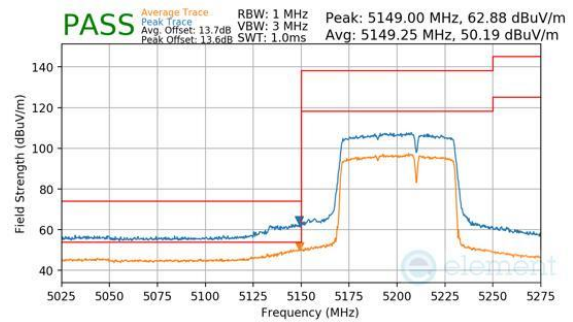
Plot 7-522. Antenna WF7a (Peak & Average, RU484+242, Index 93, Ch.42, MCS11)
