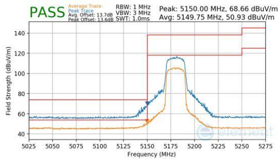
Plot 7-451. Antenna WF7a (Peak & Average, RU242, Index 61, Ch.36, MCS11)
