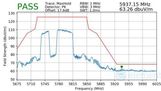
Plot 7-544. Antenna WF7a (Peak, RU484+242, Index 91, Ch.155, MCS11)
