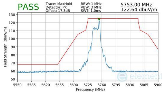
Plot 7-426. Antenna WF7a (Peak, RU26, Index 8, Ch.149, MCS11)
