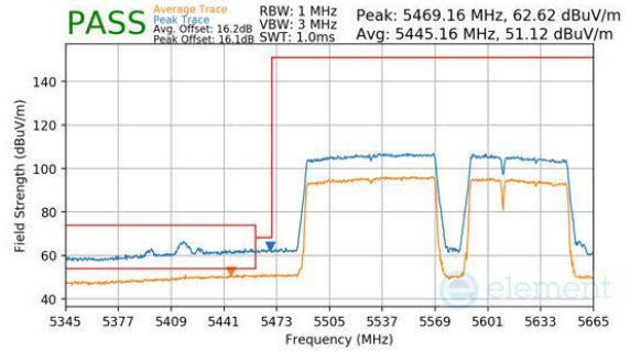
Plot 7-394. Antenna WF8 (Peak & Average, RU996+484+242, Index 96 (H), Ch.114, MCS11)
