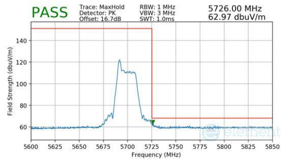
Plot 7-423. Antenna WF7a (Peak, RU26, Index 0, Ch.140, MCS11)
