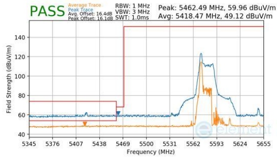
Plot 7-505. Antenna WF7a (Peak & Average, RU26, Index 0, Ch.122, MCS11)
