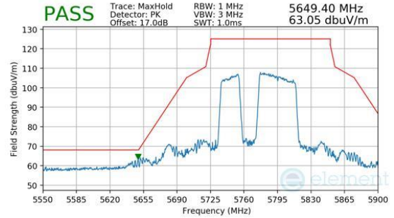
Plot 7-540. Antenna WF7a (Peak, RU484+242, Index 91, Ch.155, MCS11)
