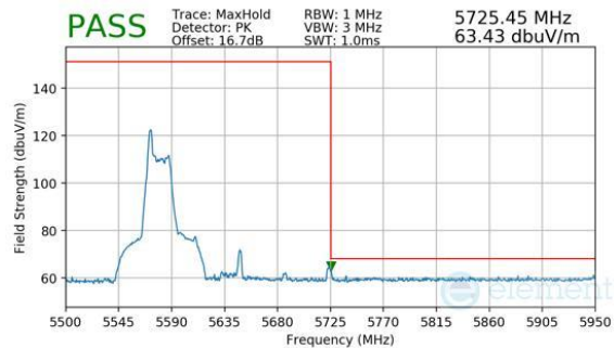
Plot 7-507. Antenna WF7a (Peak, RU26, Index 0, Ch.122, MCS11)
