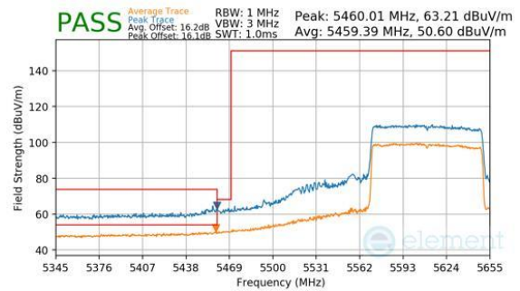
Plot 7-550. Antenna WF7a (Peak & Average, RU996, Index 67, Ch.122, MCS11)
