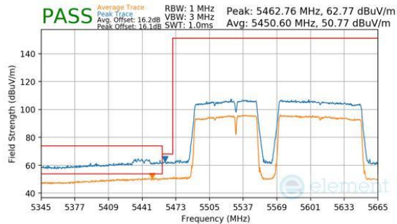
Plot 7-399. Antenna WF8 (Peak & Average, RU996+484+242, Index 99 (L), Ch.114, MCS11)
