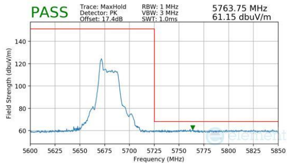
Plot 7-421. Antenna WF7a (Peak, RU26, Index 0, Ch.136, MCS11)
