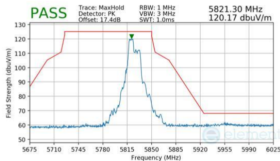
Plot 7-449. Antenna WF7a (Peak, RU52+26, Index 70, Ch.165, MCS11)
