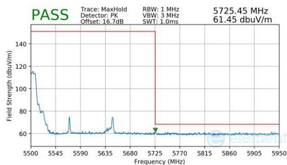
Plot 7-560. Antenna WF7a (Peak, RU26, Index 0 (L), Ch.114, MCS11)
