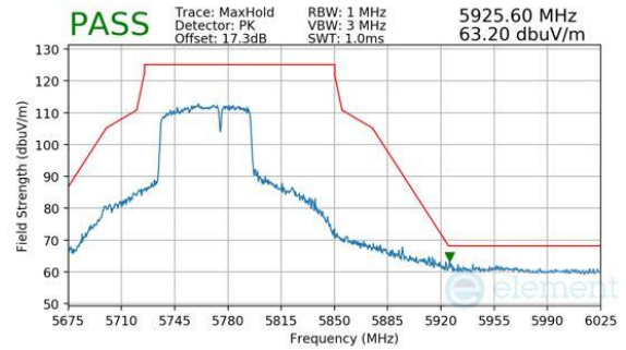
Plot 7-546. Antenna WF7a (Peak, RU484+242, Index 93, Ch.155, MCS11)
