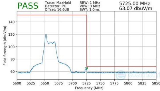
Plot 7-474. Antenna WF7a (Peak, RU26, Index 0, Ch.134, MCS11)
