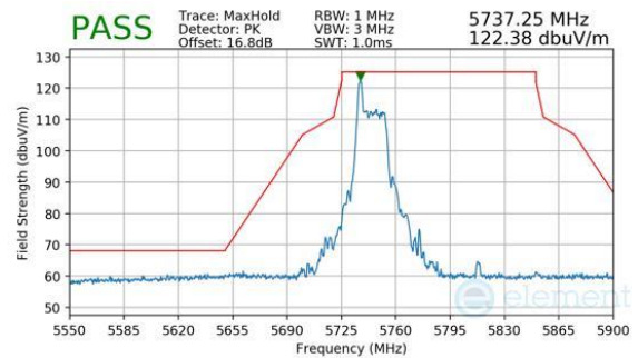
Plot 7-509. Antenna WF7a (Peak, RU26, Index 0, Ch.155, MCS11)
