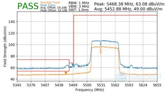
Plot 7-527. Antenna WF7a (Peak & Average, RU484+242, Index 90, Ch.106, MCS11)
