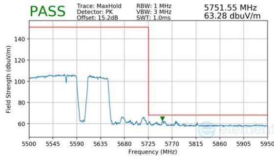
Plot 7-404. Antenna WF8 (Peak, RU996+484+242, Index 97 (H), Ch.114, MCS11)
