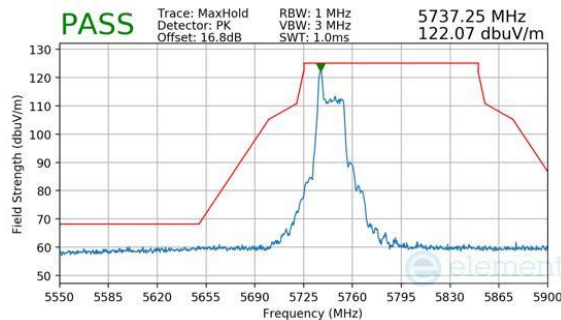
Plot 7-476. Antenna WF7a (Peak, RU26, Index 0, Ch.151, MCS11)
