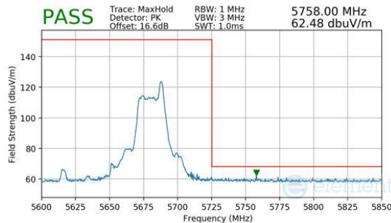
Plot 7-475. Antenna WF7a (Peak, RU26, Index 17, Ch.134, MCS11)
