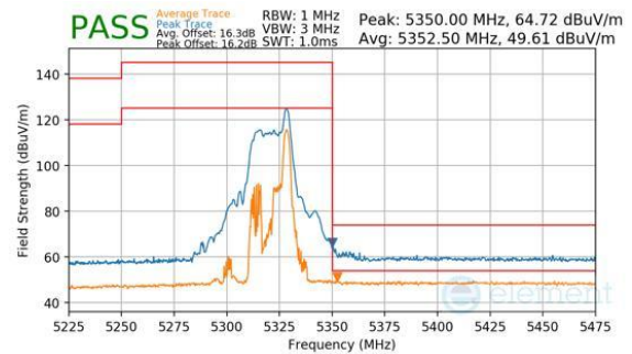
Plot 7-416. Antenna WF7a (Peak & Average, RU26, Index 8, Ch.64, MCS11)
