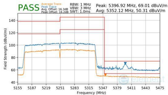
Plot 7-410. Antenna WF8 (Peak & Average, RU996X2, Index 68, Ch.50, MCS11)
