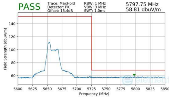
Plot 7-486. Antenna WF7a (Peak, RU52, Index 37, Ch.134, MCS11)
