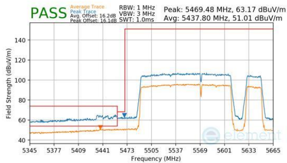
Plot 7-398. Antenna WF8 (Peak & Average, RU996+484+242, Index 98 (H), Ch.114, MCS11)
