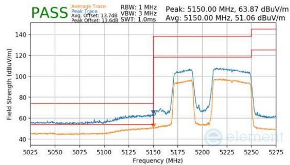
Plot 7-520. Antenna WF7a (Peak & Average, RU484+242, Index 91, Ch.42, MCS11)
