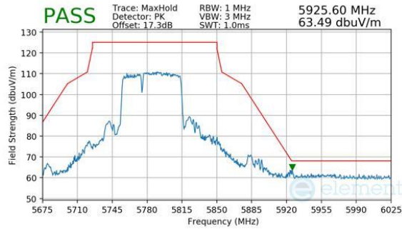
Plot 7-543. Antenna WF7a (Peak, RU484+242, Index 90, Ch.155, MCS11)
