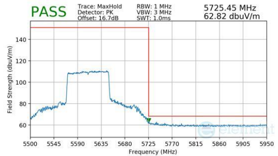
Plot 7-551. Antenna WF7a (Peak, RU996, Index 67, Ch.122, MCS11)
