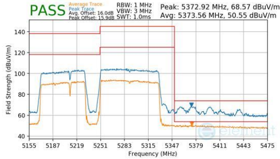
Plot 7-391. Antenna WF8 (Peak & Average, RU996+484+242, Index 99 (L), Ch.50, MCS11)
