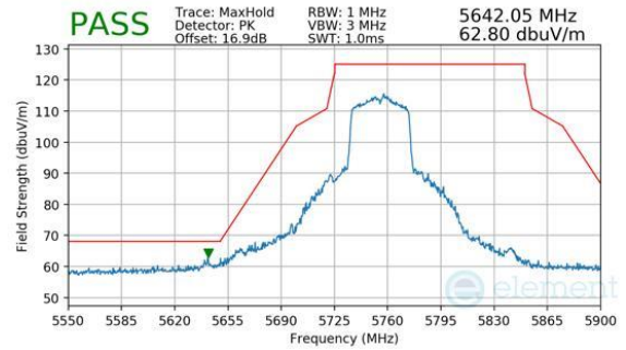
Plot 7-497. Antenna WF7a (Peak, RU484, Index 65, Ch.151, MCS11)
