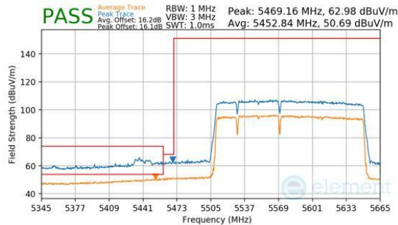
Plot 7-393. Antenna WF8 (Peak & Average, RU996+484+242, Index 96 (L), Ch.114, MCS11)
