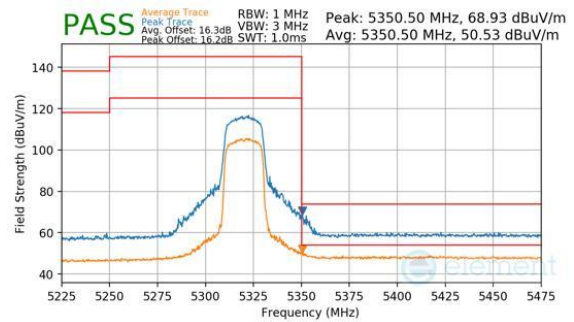
Plot 7-454. Antenna WF7a (Peak & Average, RU242, Index 61, Ch.64, MCS11)
