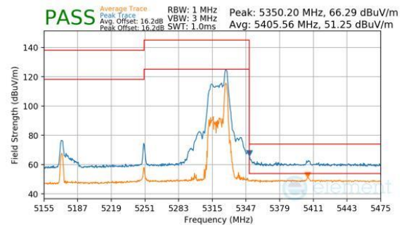
Plot 7-557. Antenna WF7a (Peak & Average, RU26, Index 36, Ch.50, MCS11)
