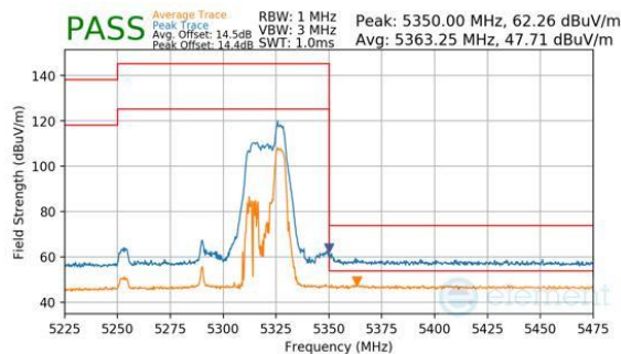
Plot 7-514. Antenna WF7a (Peak & Average, RU52, Index 52, Ch.58, MCS11)
