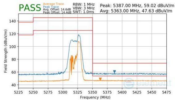
Plot 7-430. Antenna WF7a (Peak & Average, RU52, Index 40, Ch.64, MCS11)
