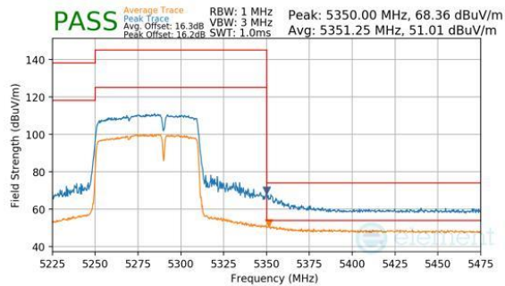
Plot 7-526. Antenna WF7a (Peak & Average, RU484+242, Index 93, Ch.58, MCS11)
