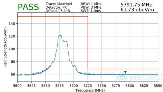
Plot 7-443. Antenna WF7a (Peak, RU52+26, Index 70, Ch.136, MCS11)
