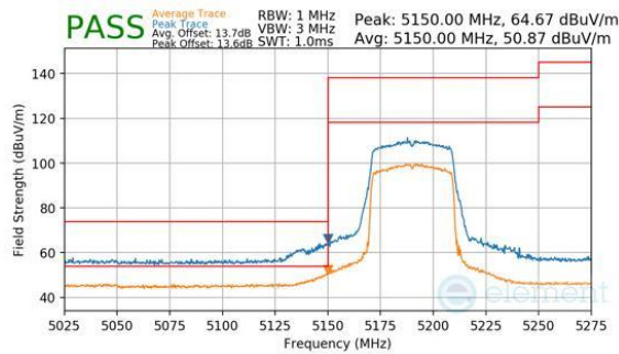
Plot 7-488. Antenna WF7a (Peak & Average, RU484, Index 65, Ch.38, MCS11)
