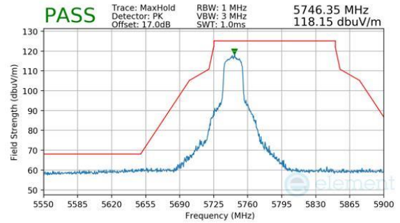
Plot 7-460. Antenna WF7a (Peak, RU242, Index 61, Ch.149, MCS11)
