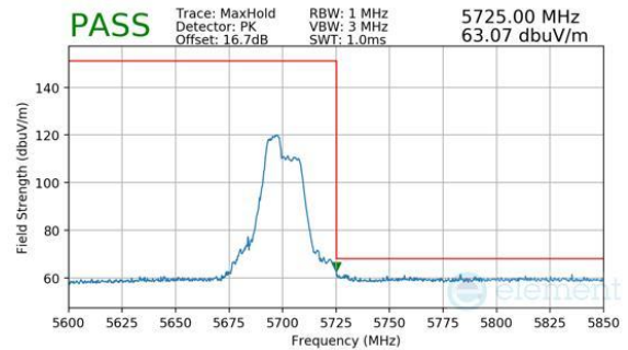
Plot 7-445. Antenna WF7a (Peak, RU52+26, Index 70, Ch.140, MCS11)
