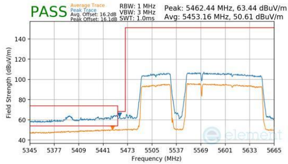
Plot 7-397. Antenna WF8 (Peak & Average, RU996+484+242, Index 98 (L), Ch.114, MCS11)
