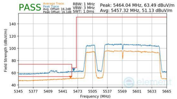
Plot 7-395. Antenna WF8 (Peak & Average, RU996+484+242, Index 97 (L), Ch.114, MCS11)
