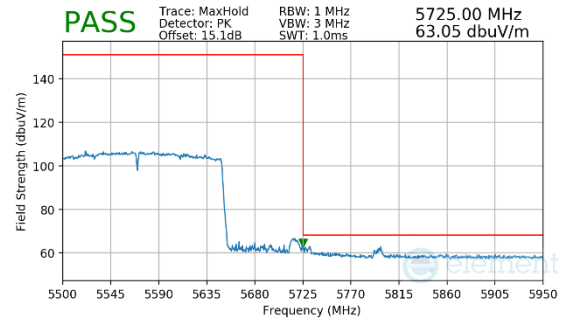
Plot 7-412. Antenna WF8 (Peak & Average, RU996X2, Index 68, Ch.114, MCS11)
