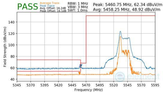
Plot 7-470. Antenna WF7a (Peak & Average, RU26, Index 0, Ch.110, MCS11)
