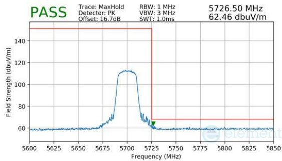
Plot 7-459. Antenna WF7a (Peak, RU242, Index 61, Ch.140, MCS11)
