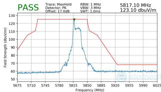
Plot 7-427. Antenna WF7a (Peak, RU26, Index 0, Ch.165, MCS11)
