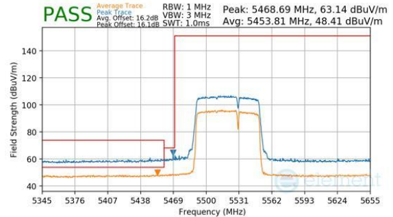
Plot 7-530. Antenna WF7a (Peak & Average, RU484+242, Index 93, Ch.106, MCS11)
