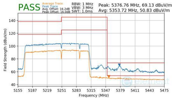
Plot 7-392. Antenna WF8 (Peak & Average, RU996+484+242, Index 99 (H), Ch.50, MCS11)
