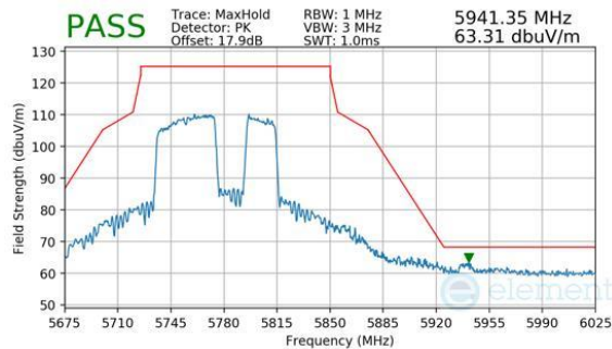
Plot 7-545. Antenna WF7a (Peak, RU484+242, Index 92, Ch.155, MCS11)
