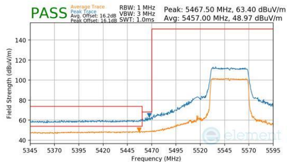
Plot 7-493. Antenna WF7a (Peak & Average, RU484, Index 65, Ch.110, MCS11)
