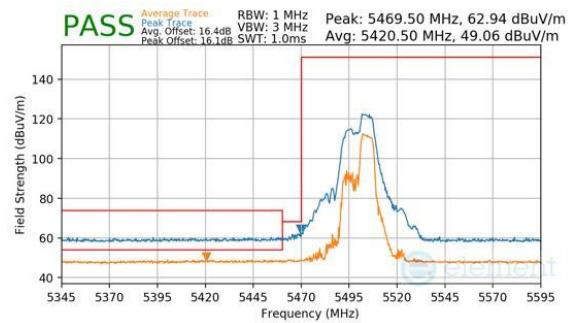
Plot 7-440. Antenna WF7a (Peak & Average, RU52+26, Index 72, Ch.100, MCS11)
