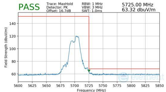
Plot 7-446. Antenna WF7a (Peak, RU52+26, Index 72, Ch.140, MCS11)
