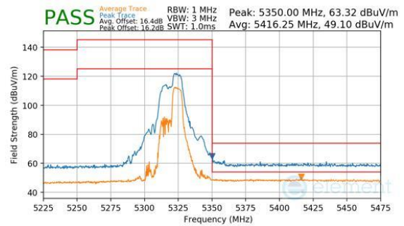
Plot 7-438. Antenna WF7a (Peak & Average, RU52+26, Index 72, Ch.64, MCS11)
