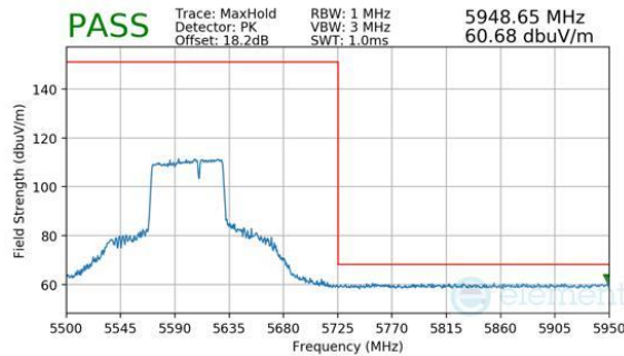
Plot 7-538. Antenna WF7a (Peak, RU484+242, Index 93, Ch.122, MCS11)
