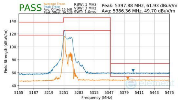
Plot 7-556. Antenna WF7a (Peak & Average, RU26, Index 0, Ch.50, MCS11)
