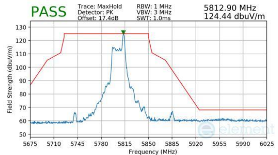
Plot 7-479. Antenna WF7a (Peak, RU26, Index 17, Ch.159, MCS11)
