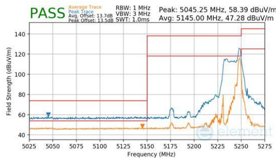
Plot 7-464. Antenna WF7a (Peak & Average, RU26, Index 17, Ch.46, MCS11)
