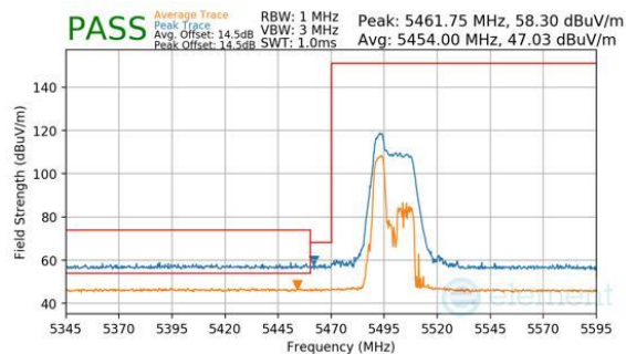
Plot 7-431. Antenna WF7a (Peak & Average, RU52, Index 37, Ch.100, MCS11)
