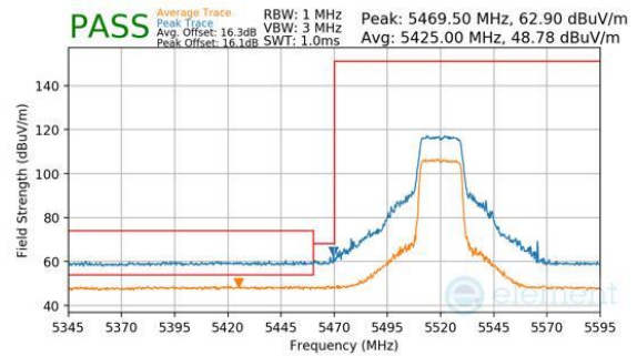
Plot 7-456. Antenna WF7a (Peak & Average, RU242, Index 61, Ch.104, MCS11)
