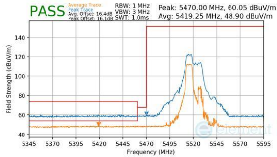
Plot 7-441. Antenna WF7a (Peak & Average, RU52+26, Index 70, Ch.104, MCS11)
