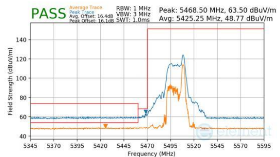
Plot 7-418. Antenna WF7a (Peak & Average, RU26, Index 8, Ch.100, MCS11)
