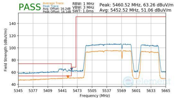
Plot 7-396. Antenna WF8 (Peak & Average, RU996+484+242, Index 97 (H), Ch.114, MCS11)
