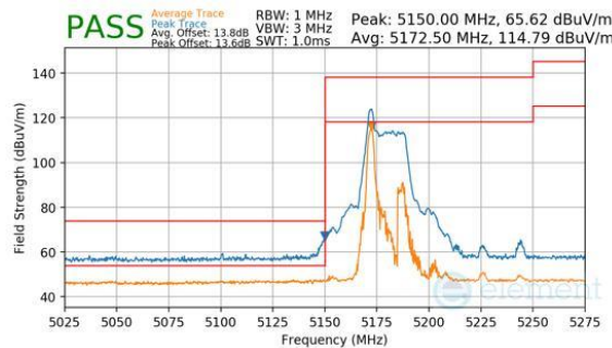
Plot 7-462. Antenna WF7a (Peak & Average, RU26, Index 0, Ch.38, MCS11)
