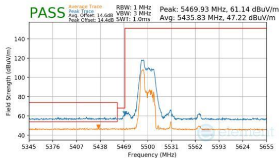
Plot 7-515. Antenna WF7a (Peak & Average, RU52, Index 37, Ch.106, MCS11)
