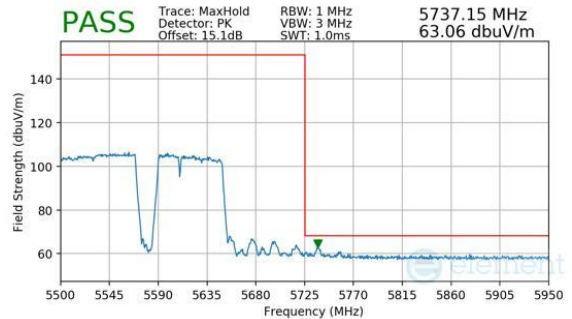
Plot 7-402. Antenna WF8 (Peak, RU996+484+242, Index 96 (H), Ch.114, MCS11)
