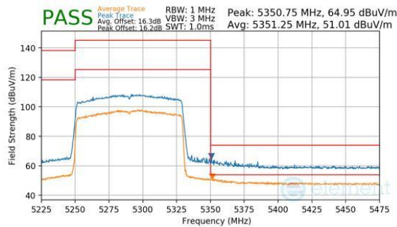
Plot 7-548. Antenna WF7a (Peak & Average, RU996, Index 67, Ch.58, MCS11)
