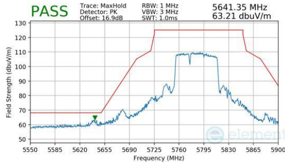
Plot 7-539. Antenna WF7a (Peak, RU484+242, Index 90, Ch.155, MCS11)
