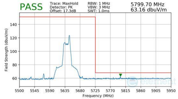
Plot 7-508. Antenna WF7a (Peak, RU26, Index 36, Ch.122, MCS11)
