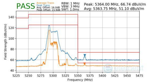
Plot 7-466. Antenna WF7a (Peak & Average, RU26, Index 0, Ch.62, MCS11)
