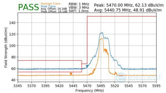
Plot 7-439. Antenna WF7a (Peak & Average, RU52+26, Index 70, Ch.100, MCS11)
