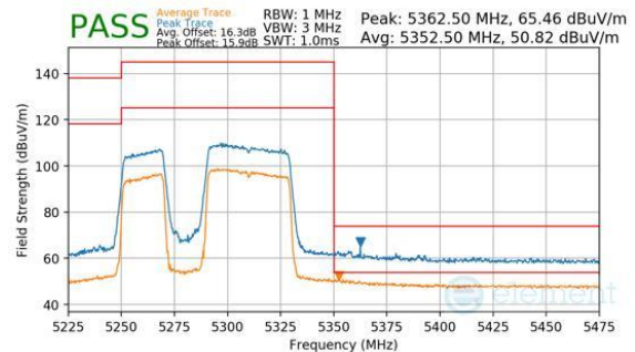
Plot 7-524. Antenna WF7a (Peak & Average, RU484+242, Index 91, Ch.58, MCS11)
