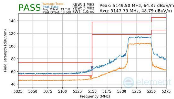
Plot 7-489. Antenna WF7a (Peak & Average, RU484, Index 65, Ch.46, MCS11)
