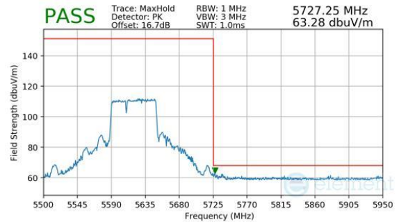
Plot 7-535. Antenna WF7a (Peak, RU484+242, Index 90, Ch.122, MCS11)
