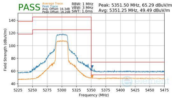
Plot 7-453. Antenna WF7a (Peak & Average, RU242, Index 61, Ch.60, MCS11)
