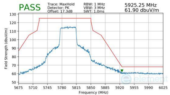
Plot 7-498. Antenna WF7a (Peak, RU484, Index 65, Ch.159, MCS11)
