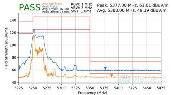
Plot 7-465. Antenna WF7a (Peak & Average, RU26, Index 0, Ch.54, MCS11)
