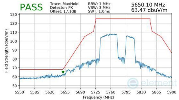
Plot 7-541. Antenna WF7a (Peak, RU484+242, Index 92, Ch.155, MCS11)
