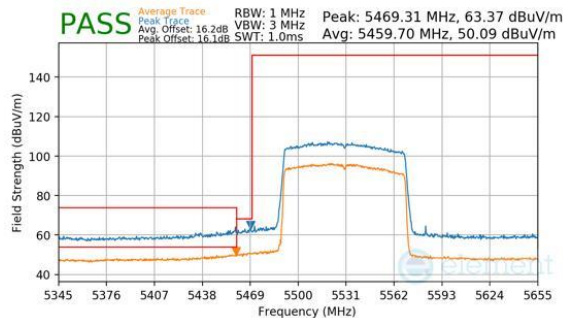
Plot 7-549. Antenna WF7a (Peak & Average, RU996, Index 67, Ch.106, MCS11)
