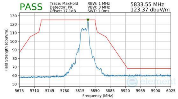
Plot 7-428. Antenna WF7a (Peak, RU26, Index 8, Ch.165, MCS11)
