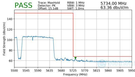
Plot 7-403. Antenna WF8 (Peak, RU996+484+242, Index 97 (L), Ch.114, MCS11)
