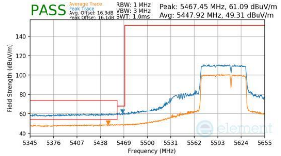
Plot 7-534. Antenna WF7a (Peak & Average, RU484+242, Index 93, Ch.122, MCS11)
