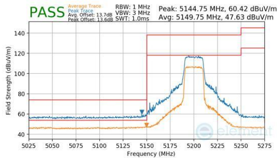
Plot 7-452. Antenna WF7a (Peak & Average, RU242, Index 61, Ch.40, MCS11)
