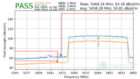
Plot 7-411. Antenna WF8 (Peak & Average, RU996X2, Index 68, Ch.114, MCS11)
