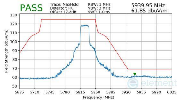
Plot 7-461. Antenna WF7a (Peak, RU242, Index 61, Ch.165, MCS11)
