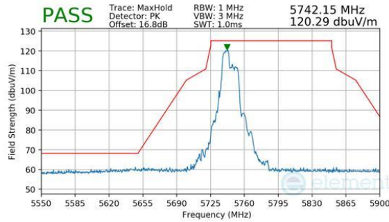
Plot 7-447. Antenna WF7a (Peak, RU52+26, Index 70, Ch.149, MCS11)
