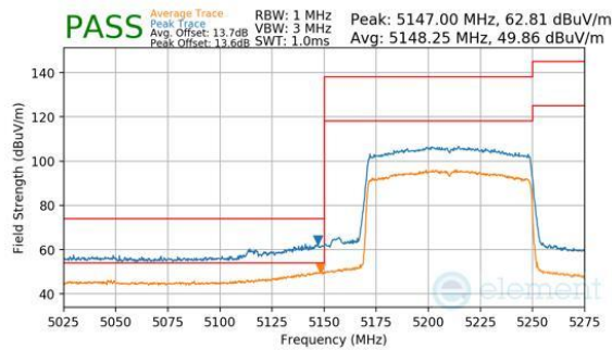
Plot 7-547. Antenna WF7a (Peak & Average, RU996, Index 67, Ch.42, MCS11)
