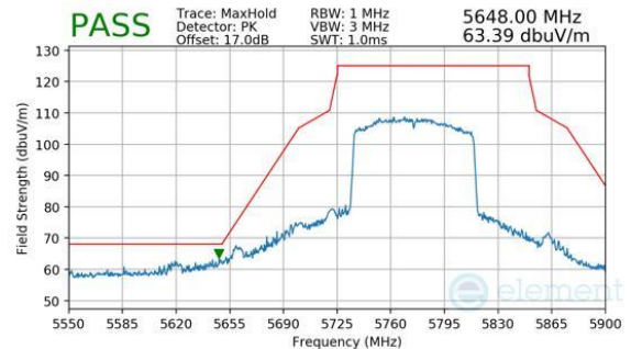
Plot 7-552. Antenna WF7a (Peak, RU996, Index 67, Ch.155, MCS11)
