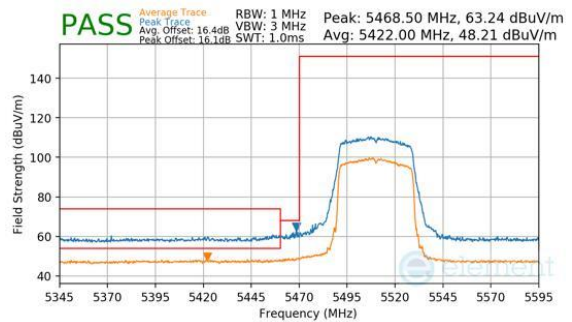
Plot 7-492. Antenna WF7a (Peak & Average, RU484, Index 65, Ch.102, MCS11)
