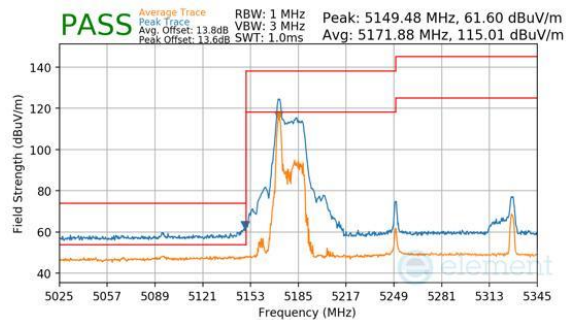
Plot 7-554. Antenna WF7a (Peak & Average, RU26, Index 0, Ch.50, MCS11)
