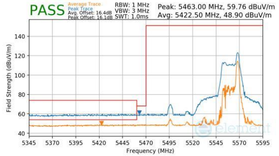
Plot 7-471. Antenna WF7a (Peak & Average, RU26, Index 17, Ch.110, MCS11)
