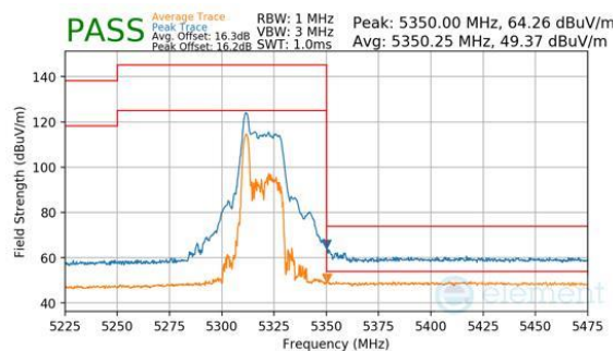
Plot 7-415. Antenna WF7a (Peak & Average, RU26, Index 0, Ch.64, MCS11)
