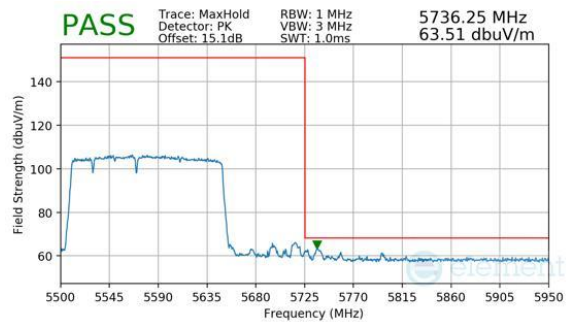
Plot 7-401. Antenna WF8 (Peak, RU996+484+242, Index 96 (L), Ch.114, MCS11)
