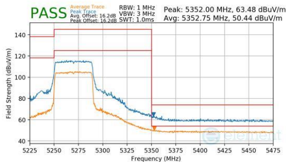
Plot 7-490. Antenna WF7a (Peak & Average, RU484, Index 65, Ch.54, MCS11)
