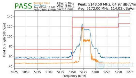
Plot 7-413. Antenna WF7a (Peak & Average, RU26, Index 0, Ch.36, MCS11)
