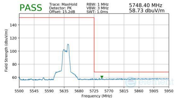
Plot 7-518. Antenna WF7a (Peak, RU52, Index 52, Ch.122, MCS11)
