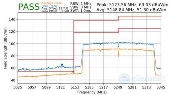
Plot 7-409. Antenna WF8 (Peak & Average, RU996X2, Index 68, Ch.50, MCS11)
