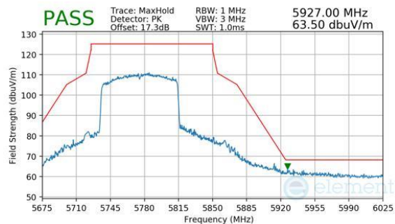
Plot 7-553. Antenna WF7a (Peak, RU996, Index 67, Ch.155, MCS11)
