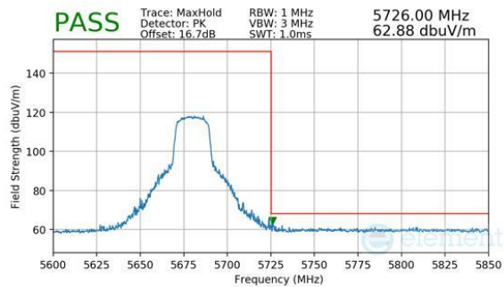
Plot 7-458. Antenna WF7a (Peak, RU242, Index 61, Ch.136, MCS11)
