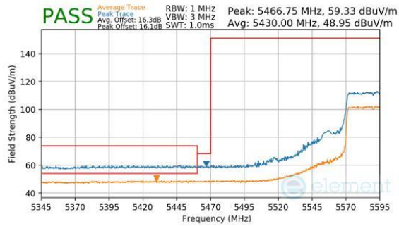
Plot 7-494. Antenna WF7a (Peak & Average, RU484, Index 65, Ch.118, MCS11)
