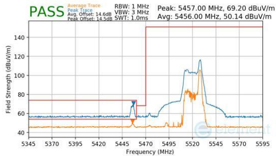
Plot 7-469. Antenna WF7a (Peak & Average, RU26, Index 17, Ch.102, MCS11)
