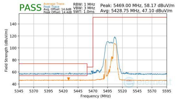
Plot 7-432. Antenna WF7a (Peak & Average, RU52, Index 40, Ch.100, MCS11)
