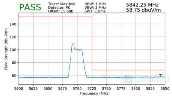
Plot 7-433. Antenna WF7a (Peak, RU52, Index 37, Ch.140, MCS11)
