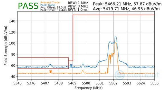
Plot 7-516. Antenna WF7a (Peak & Average, RU52, Index 52, Ch.106, MCS11)
