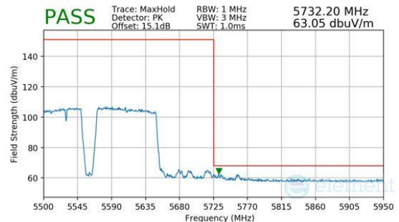
Plot 7-408. Antenna WF8 (Peak, RU996+484+242, Index 99 (L), Ch.114, MCS11)
