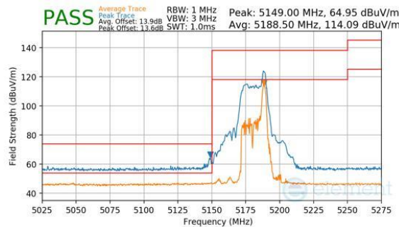
Plot 7-414. Antenna WF7a (Peak & Average, RU26, Index 8, Ch.36, MCS11)
