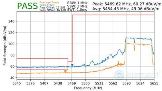
Plot 7-531. Antenna WF7a (Peak & Average, RU484+242, Index 90, Ch.122, MCS11)
