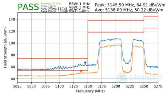
Plot 7-521. Antenna WF7a (Peak & Average, RU484+242, Index 92, Ch.42, MCS11)
