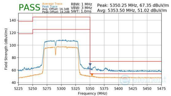
Plot 7-523. Antenna WF7a (Peak & Average, RU484+242, Index 90, Ch.58, MCS11)
