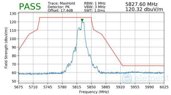
Plot 7-450. Antenna WF7a (Peak, RU52+26, Index 72, Ch.165, MCS11)
