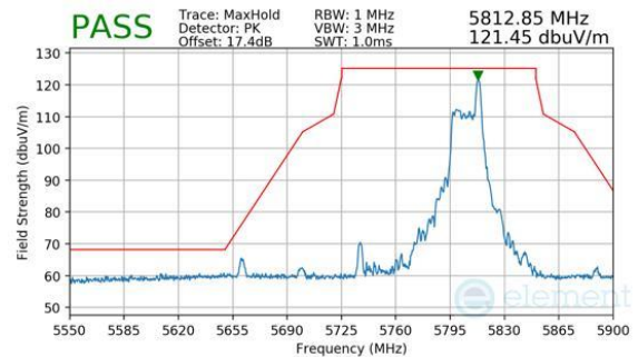
Plot 7-510. Antenna WF7a (Peak, RU26, Index 36, Ch.155, MCS11)
