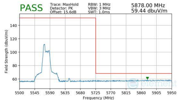
Plot 7-517. Antenna WF7a (Peak, RU52, Index 37, Ch.122, MCS11)
