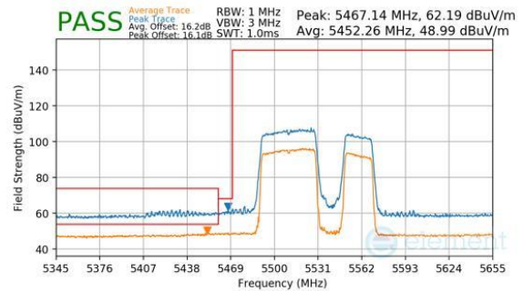
Plot 7-529. Antenna WF7a (Peak & Average, RU484+242, Index 92, Ch.106, MCS11)
