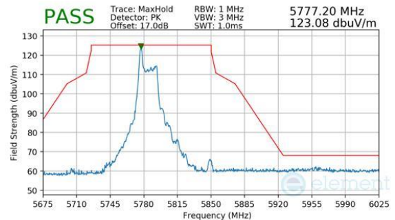
Plot 7-478. Antenna WF7a (Peak, RU26, Index 0, Ch.159, MCS11)
