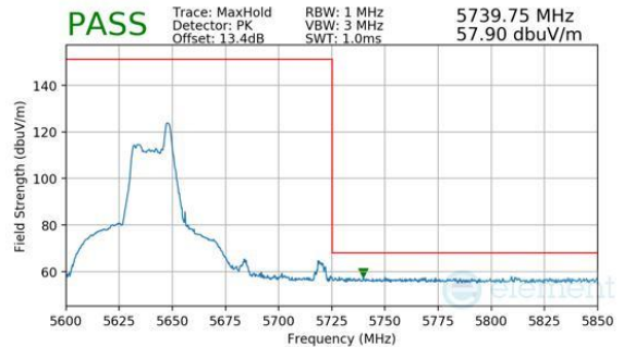
Plot 7-473. Antenna WF7a (Peak, RU26, Index 17, Ch.126, MCS11)
