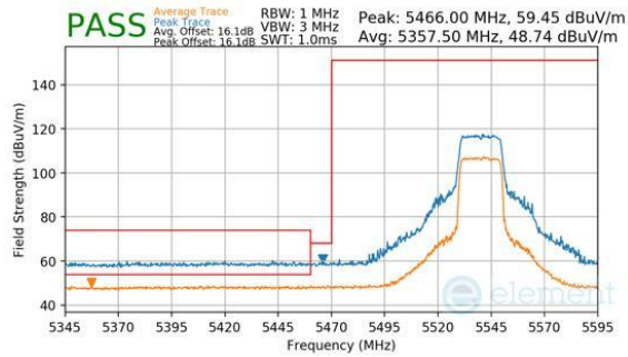
Plot 7-457. Antenna WF7a (Peak & Average, RU242, Index 61, Ch.108, MCS11)
