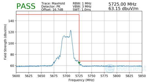
Plot 7-424. Antenna WF7a (Peak, RU26, Index 8, Ch.140, MCS11)
