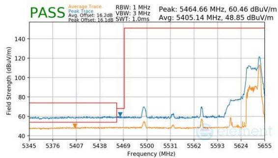
Plot 7-506. Antenna WF7a (Peak & Average, RU26, Index 36, Ch.122, MCS11)
