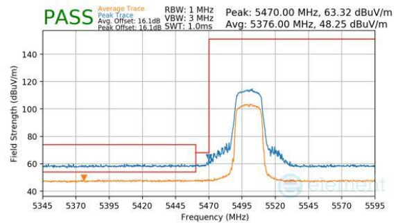
Plot 7-455. Antenna WF7a (Peak & Average, RU242, Index 61, Ch.100, MCS11)
