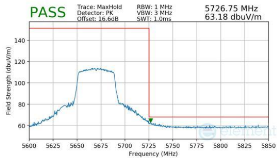
Plot 7-496. Antenna WF7a (Peak, RU484, Index 65, Ch.134, MCS11)
