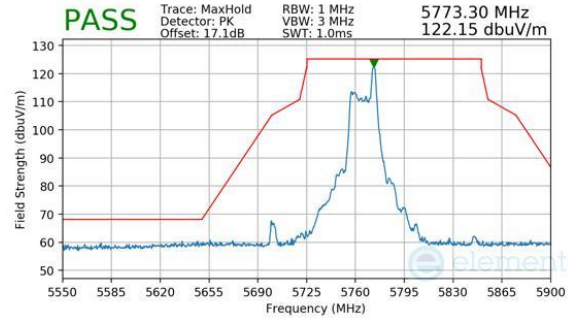
Plot 7-477. Antenna WF7a (Peak, RU26, Index 17, Ch.151, MCS11)
