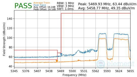
Plot 7-532. Antenna WF7a (Peak & Average, RU484+242, Index 91, Ch.122, MCS11)
