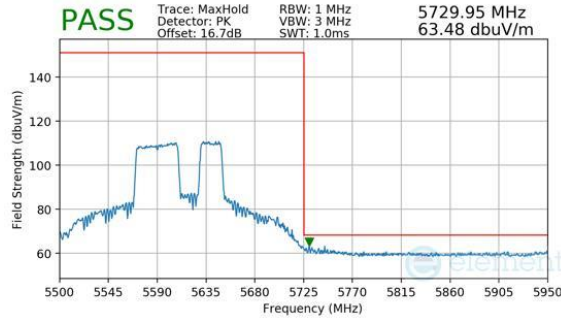
Plot 7-537. Antenna WF7a (Peak, RU484+242, Index 92, Ch.122, MCS11)
