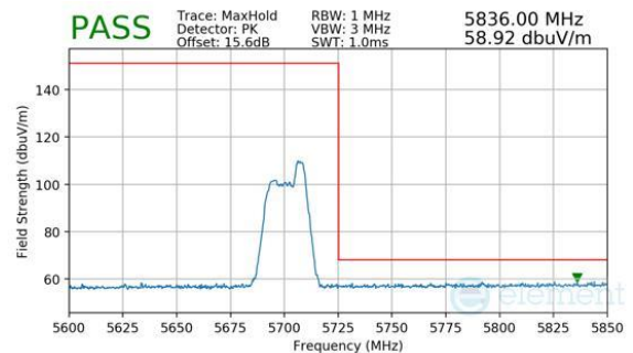
Plot 7-434. Antenna WF7a (Peak, RU52, Index 40, Ch.140, MCS11)
