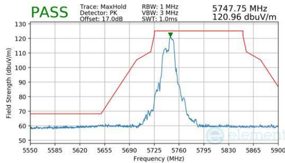
Plot 7-448. Antenna WF7a (Peak, RU52+26, Index 72, Ch.149, MCS11)
