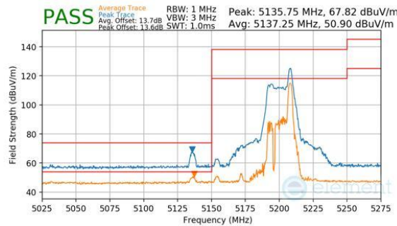
Plot 7-463. Antenna WF7a (Peak & Average, RU26, Index 17, Ch.38, MCS11)
