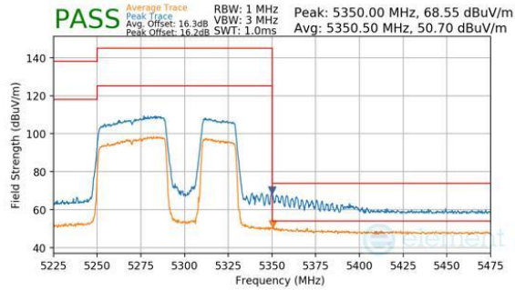
Plot 7-525. Antenna WF7a (Peak & Average, RU484+242, Index 92, Ch.58, MCS11)
