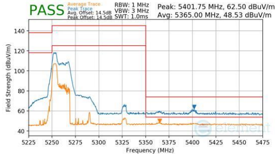
Plot 7-513. Antenna WF7a (Peak & Average, RU52, Index 37, Ch.58, MCS11)
