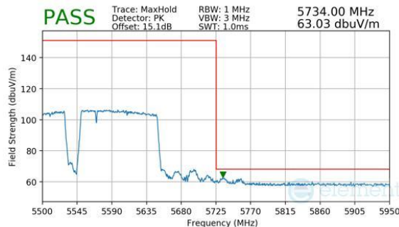
Plot 7-405. Antenna WF8 (Peak, RU996+484+242, Index 98 (L), Ch.114, MCS11)
