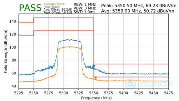
Plot 7-491. Antenna WF7a (Peak & Average, RU484, Index 65, Ch.62, MCS11)
