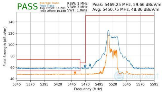
Plot 7-419. Antenna WF7a (Peak & Average, RU26, Index 0, Ch.104, MCS11)
