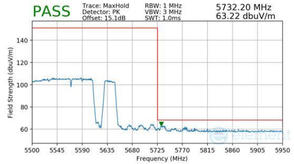
Plot 7-406. Antenna WF8 (Peak, RU996+484+242, Index 98 (H), Ch.114, MCS11)
