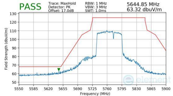
Plot 7-542. Antenna WF7a (Peak, RU484+242, Index 93, Ch.155, MCS11)
