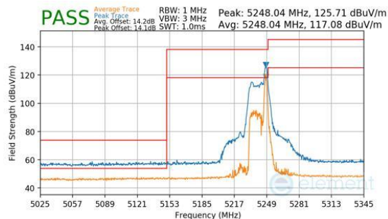
Plot 7-555. Antenna WF7a (Peak & Average, RU26, Index 36, Ch.50, MCS11)
