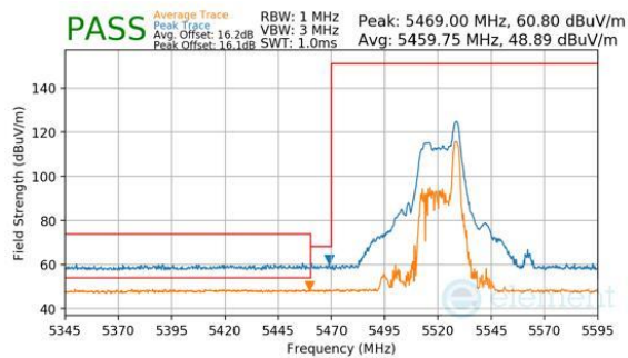
Plot 7-420. Antenna WF7a (Peak & Average, RU26, Index 8, Ch.104, MCS11)
