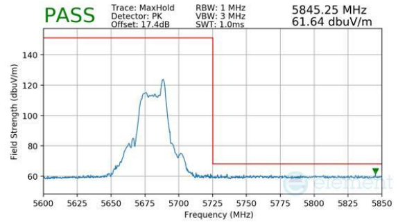
Plot 7-422. Antenna WF7a (Peak, RU26, Index 8, Ch.136, MCS11)
