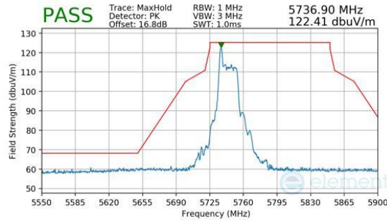
Plot 7-425. Antenna WF7a (Peak, RU26, Index 0, Ch.149, MCS11)
