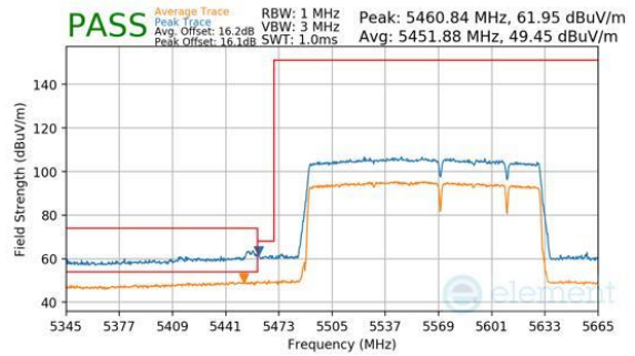
Plot 7-400. Antenna WF8 (Peak & Average, RU996+484+242, Index 99 (H), Ch.114, MCS11)
