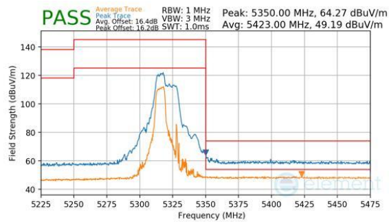
Plot 7-437. Antenna WF7a (Peak & Average, RU52+26, Index 70, Ch.64, MCS11)
