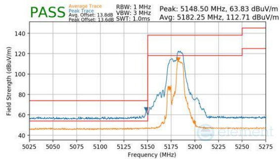
Plot 7-436. Antenna WF7a (Peak & Average, RU52+26, Index 72, Ch.36, MCS11)
