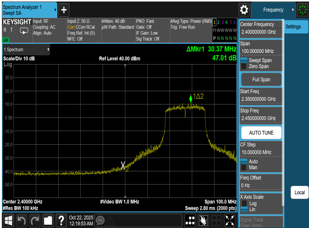
Plot 7-90. Band Edge Plot Antenna WF7b (802.11g – Ch. 4)
