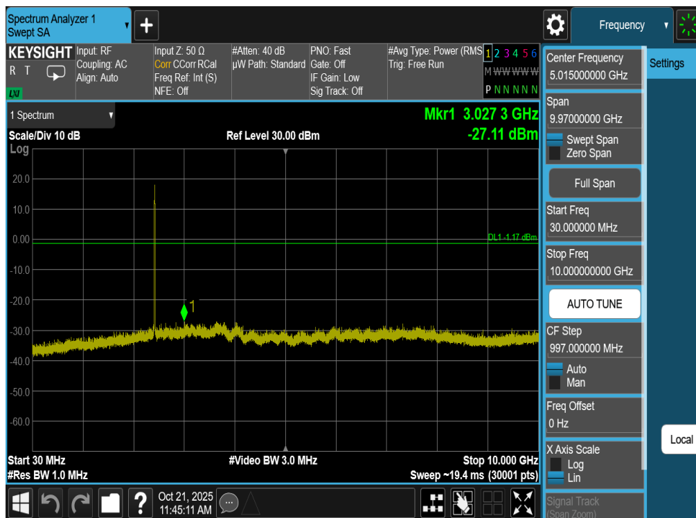
Plot 7-125. Conducted Spurious Plot Antenna WF8 (802.11b – Ch. 6)
