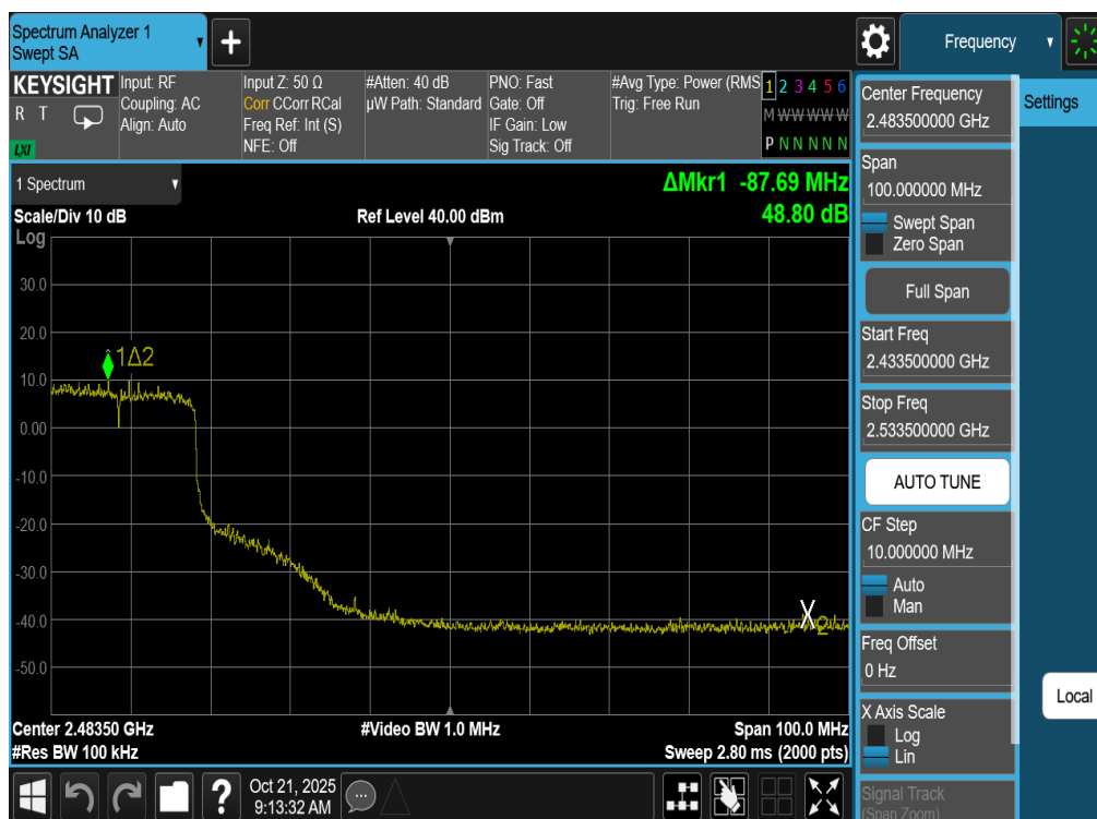
Plot 7-74. Band Edge Plot Antenna WF8 (802.11be (SU - 2.4GHz) – Ch. 7)
