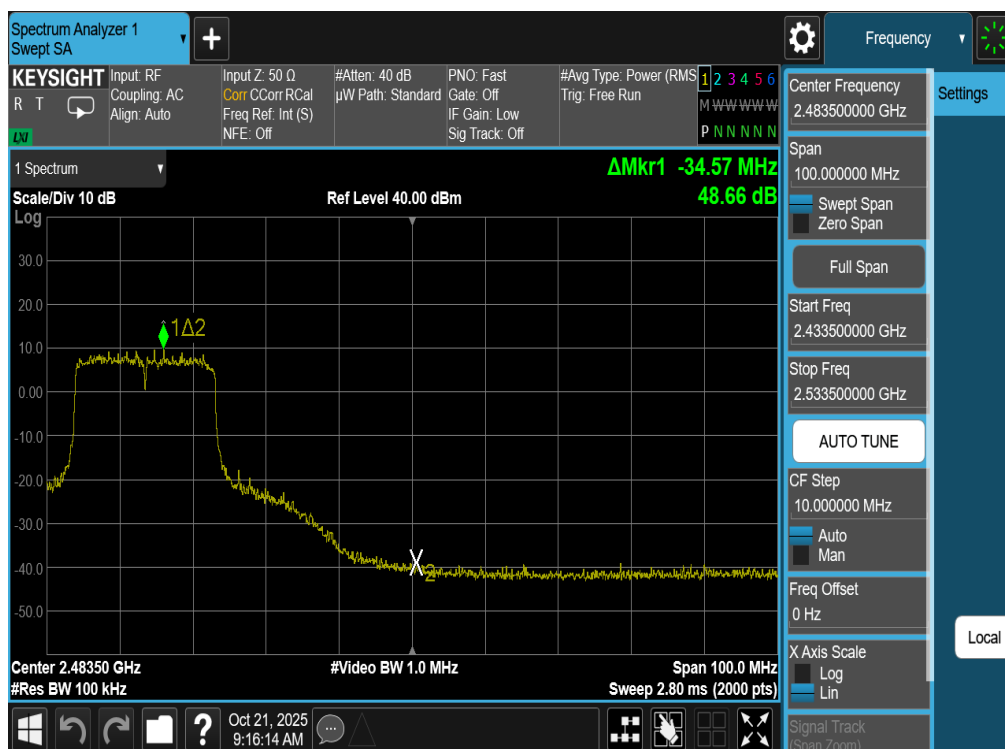
Plot 7-75. Band Edge Plot Antenna WF8 (802.11be (SU - 2.4GHz) – Ch. 8)
