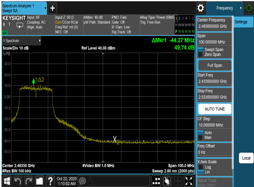
Plot 7-105. Band Edge Plot Antenna WF7b (802.11n (2.4GHz) – Ch. 8)
