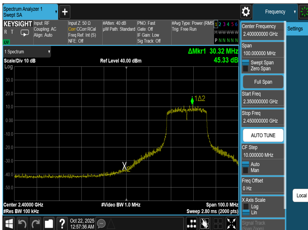
Plot 7-102. Band Edge Plot Antenna WF7b (802.11n (2.4GHz) – Ch. 4)
