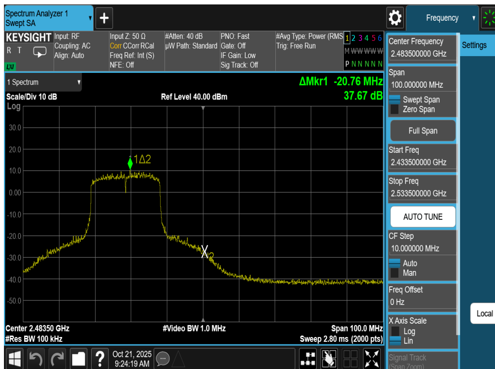
Plot 7-78. Band Edge Plot Antenna WF8 (802.11be (SU - 2.4GHz) – Ch. 11)
