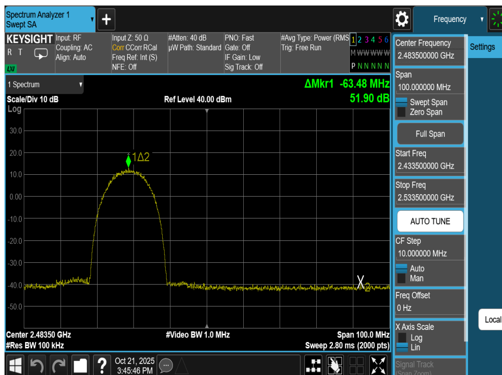
Plot 7-84. Band Edge Plot Antenna WF7b (802.11b – Ch. 11)
