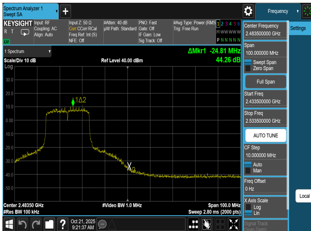
Plot 7-77. Band Edge Plot Antenna WF8 (802.11be (SU - 2.4GHz) – Ch. 10)
