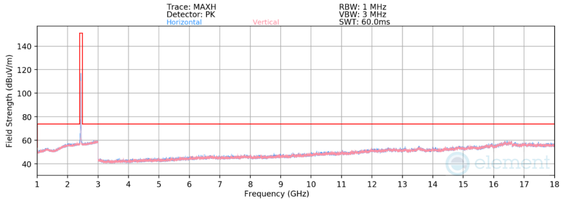
Plot 7-136. Radiated Spurious Emissions above 1GHz CDD (802.11b – Ch. 6)
