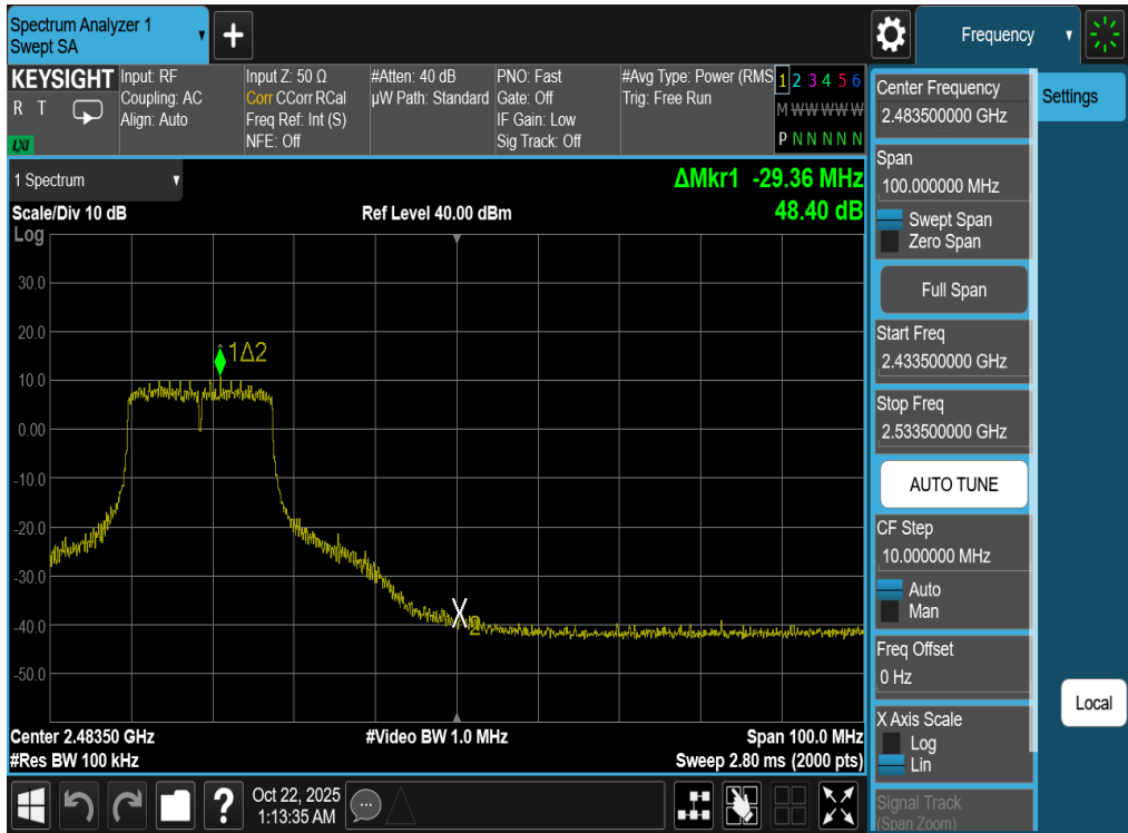
Plot 7-106. Band Edge Plot Antenna WF7b (802.11n (2.4GHz) – Ch. 9)
