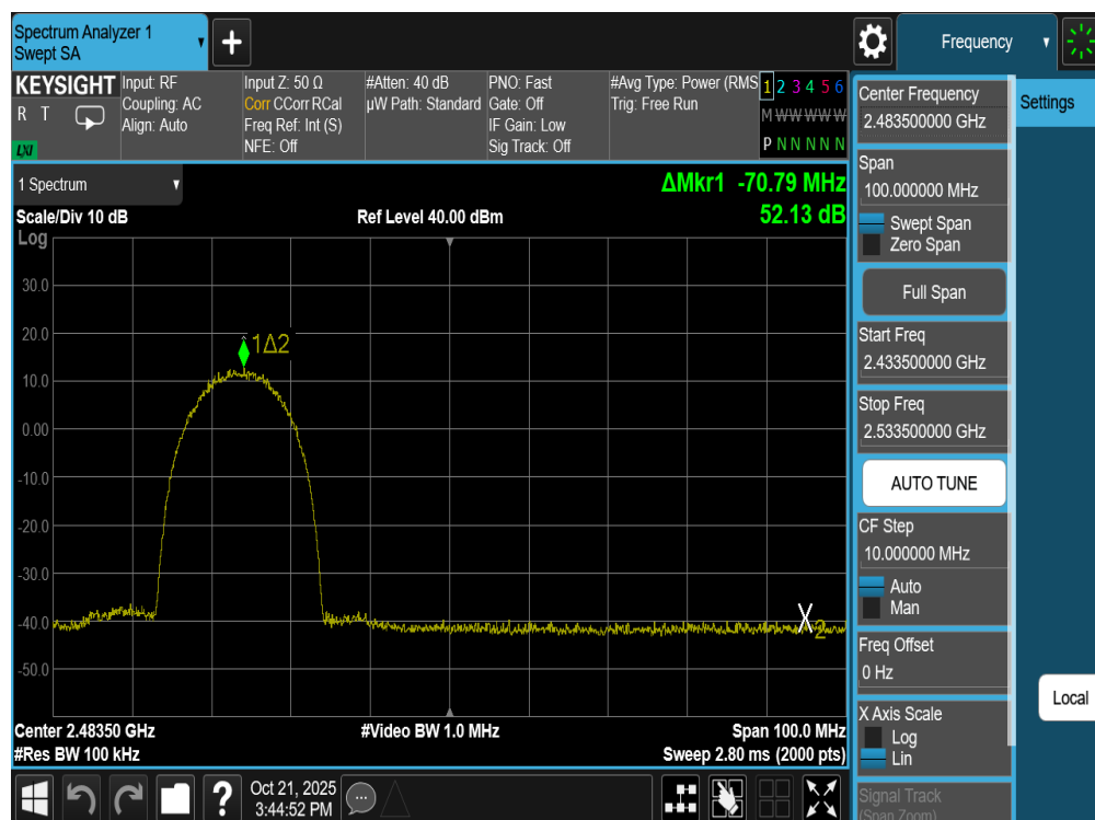
Plot 7-83. Band Edge Plot Antenna WF8 (802.11b – Ch. 10)
