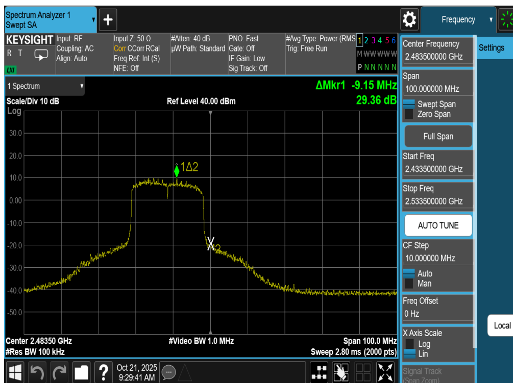
Plot 7-80. Band Edge Plot Antenna WF8 (802.11be (SU - 2.4GHz) – Ch. 13)
