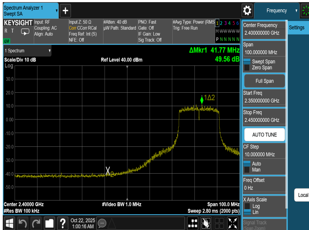
Plot 7-103. Band Edge Plot Antenna WF7b (802.11n (2.4GHz) – Ch. 5)
