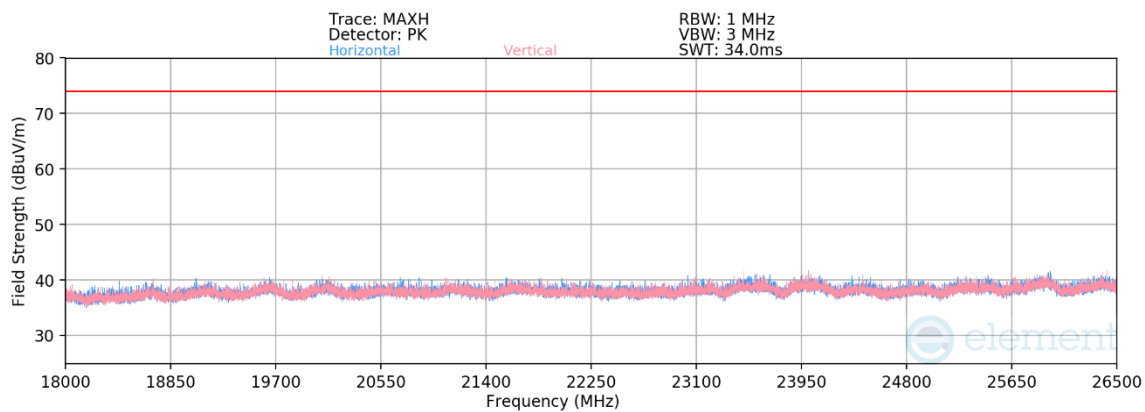
Plot 7-137. Radiated Spurious Emissions above 18GHz CDD (802.11b – Ch.6)
