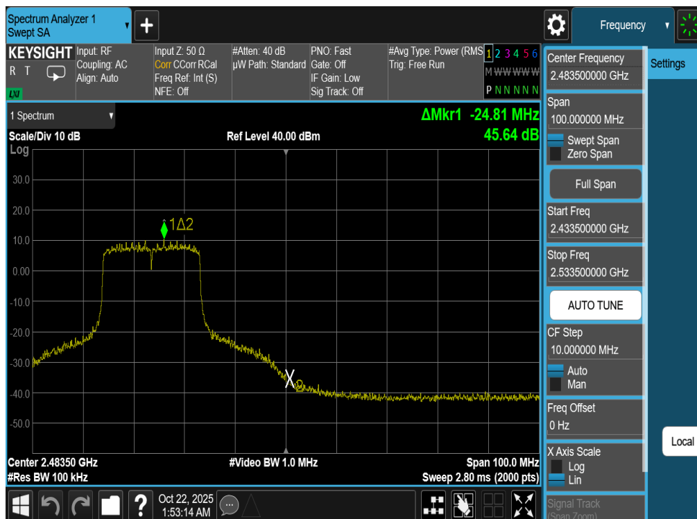
Plot 7-119. Band Edge Plot Antenna WF7b (802.11be (SU - 2.4GHz) – Ch. 10)
