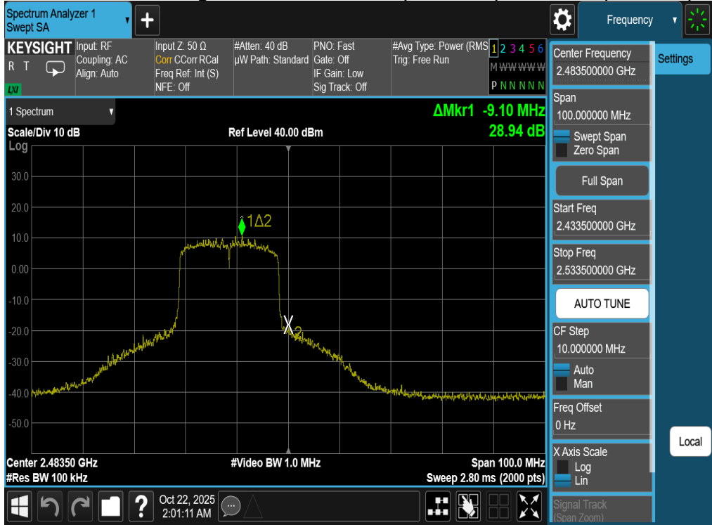
Plot 7-122. Band Edge Plot Antenna WF7b (802.11be (SU - 2.4GHz) – Ch. 13)
