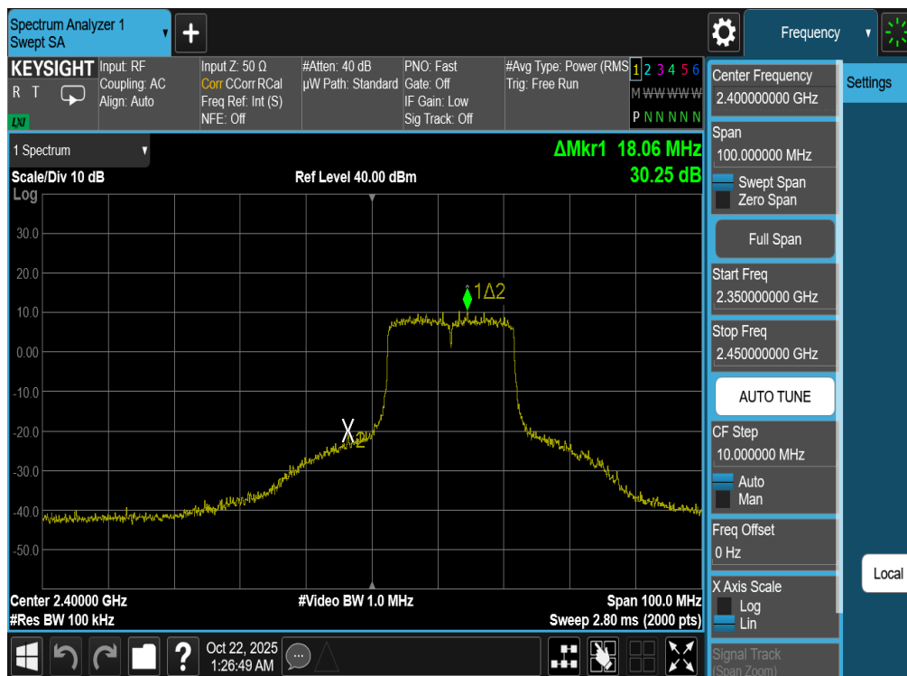
Plot 7-111. Band Edge Plot Antenna WF7b (802.11be (SU - 2.4GHz) – Ch. 1)
