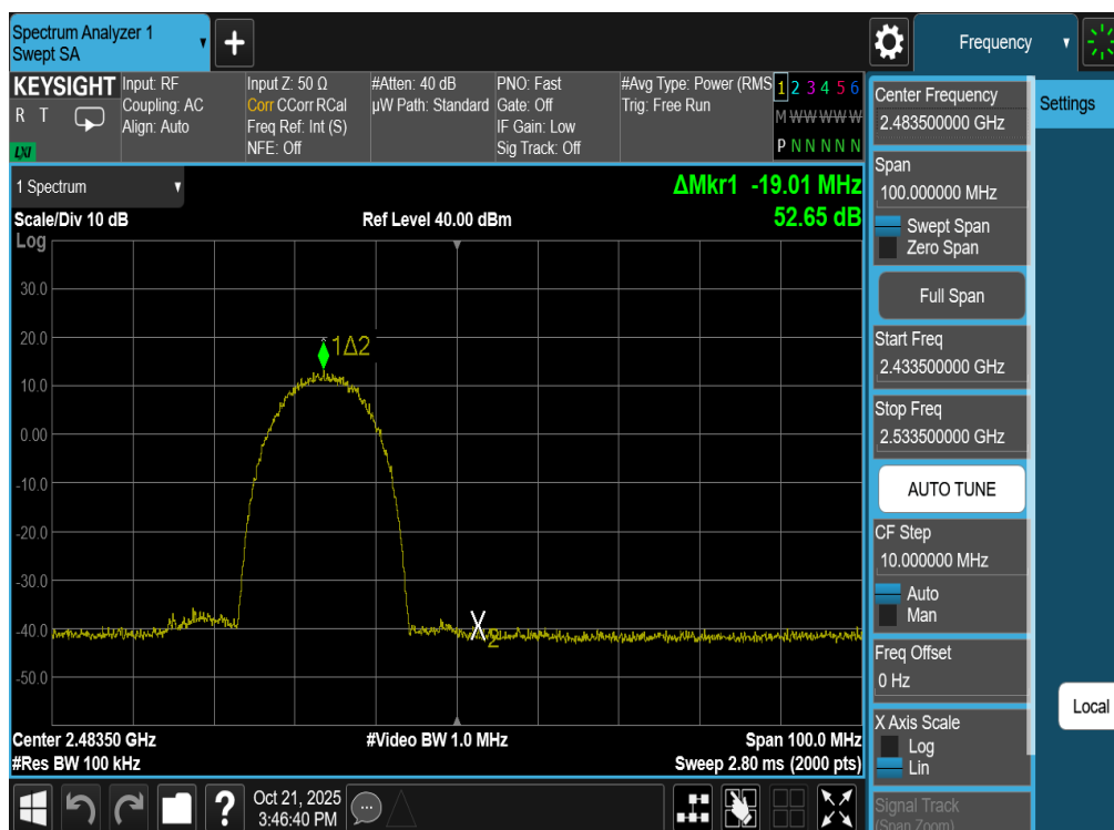
Plot 7-85. Band Edge Plot Antenna WF7b (802.11b – Ch. 12)
