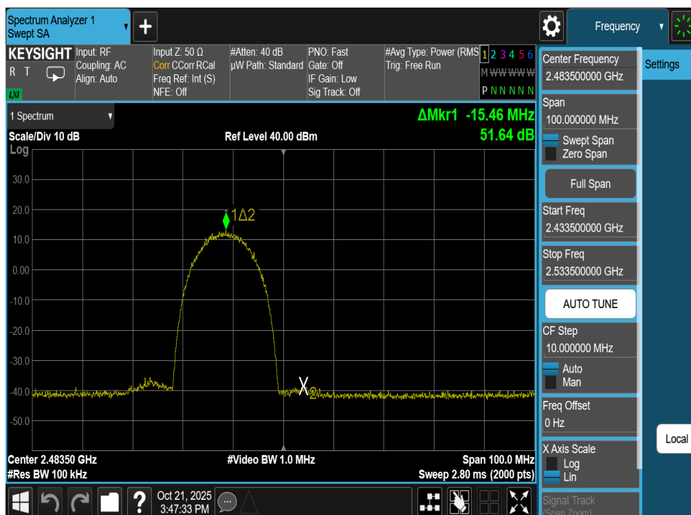
Plot 7-86. Band Edge Plot Antenna WF7b (802.11b – Ch. 13)
