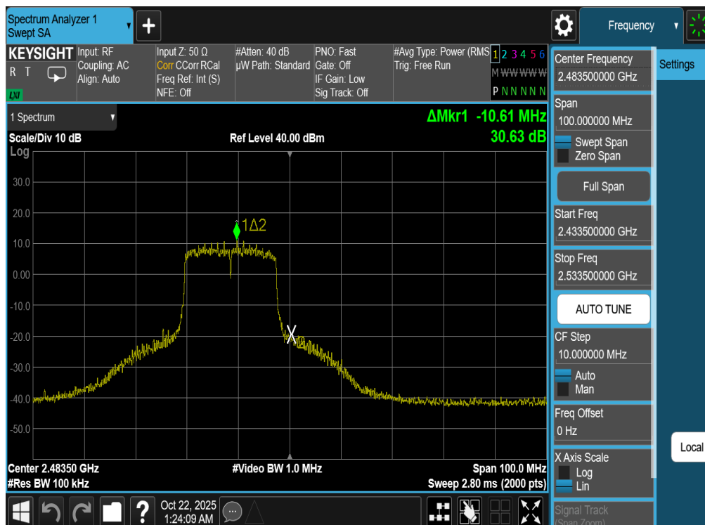
Plot 7-110. Band Edge Plot Antenna WF7b (802.11n (2.4GHz) – Ch. 13)
