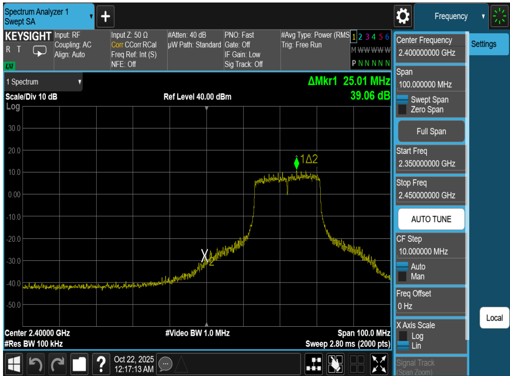
Plot 7-89. Band Edge Plot Antenna WF7b (802.11g – Ch. 3)
