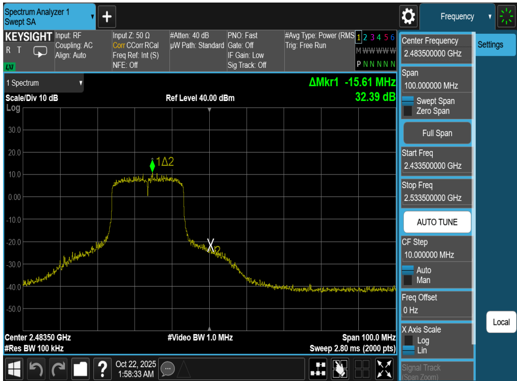
Plot 7-121. Band Edge Plot Antenna WF7b (802.11be (SU - 2.4GHz) – Ch. 12)
