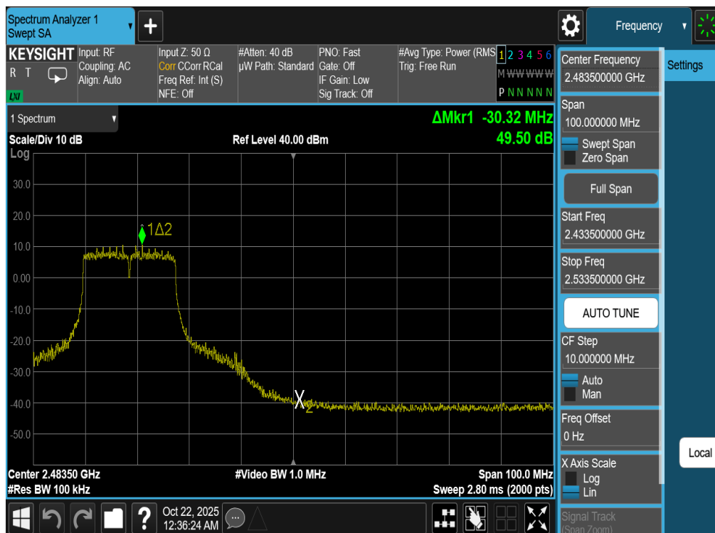
Plot 7-94. Band Edge Plot Antenna WF7b (802.11g – Ch. 9)
