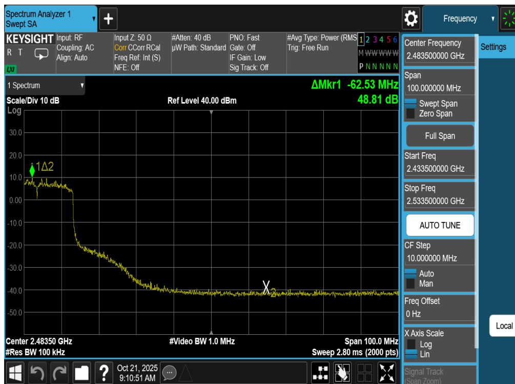
Plot 7-73. Band Edge Plot Antenna WF8 (802.11be (SU - 2.4GHz) – Ch. 6)
