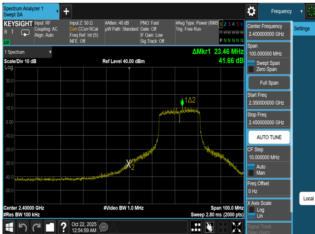
Plot 7-101. Band Edge Plot Antenna WF7b (802.11n (2.4GHz) – Ch. 3)
