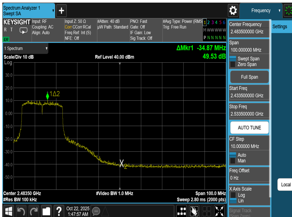
Plot 7-117. Band Edge Plot Antenna WF7b (802.11be (SU - 2.4GHz) – Ch. 8)
