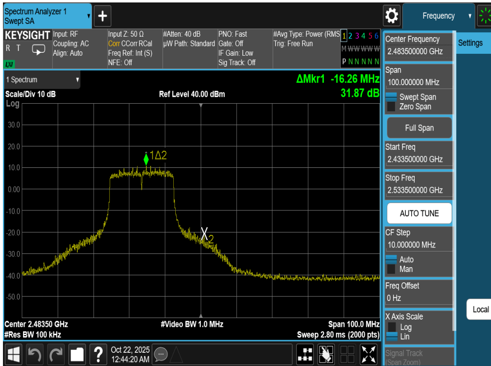
Plot 7-97. Band Edge Plot Antenna WF7b (802.11g – Ch. 12)
