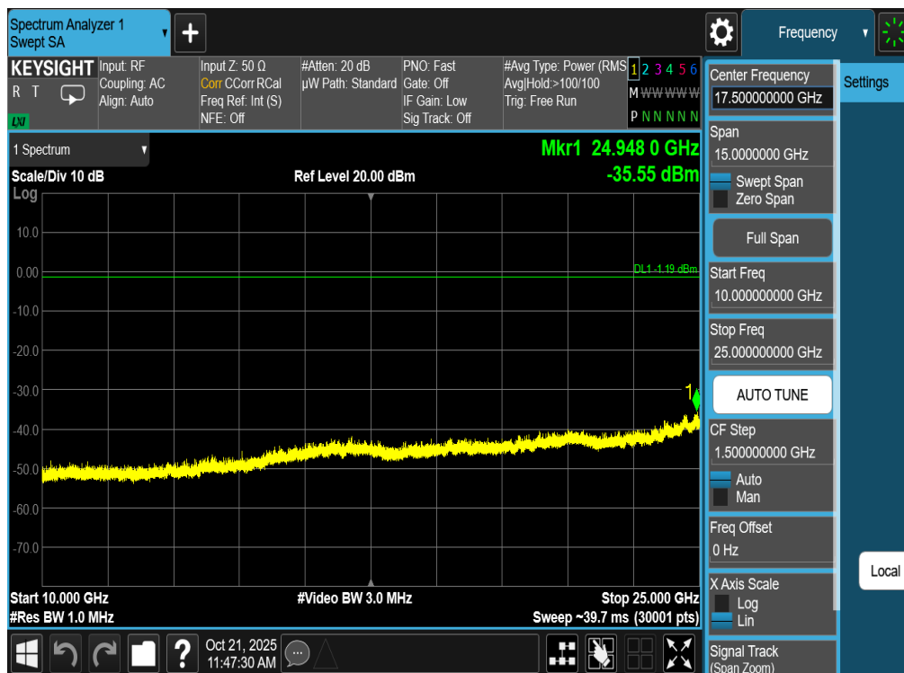
Plot 7-128. Conducted Spurious Plot Antenna WF8 (802.11b – Ch. 11)
