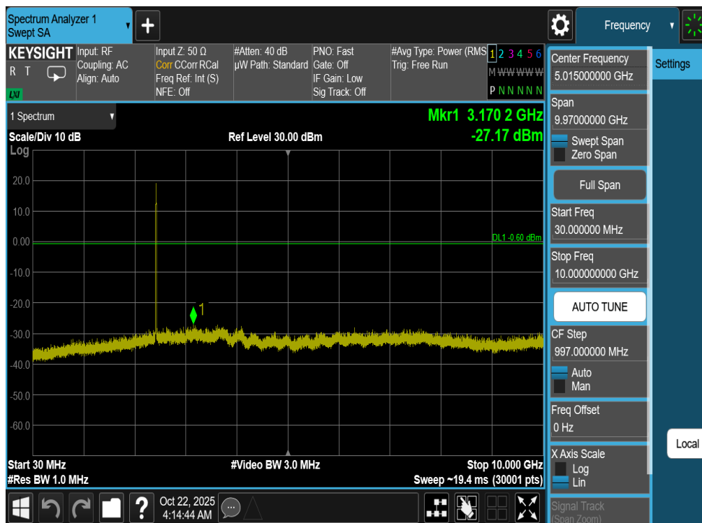
Plot 7-131. Conducted Spurious Plot Antenna WF7b (802.11b – Ch. 6)
