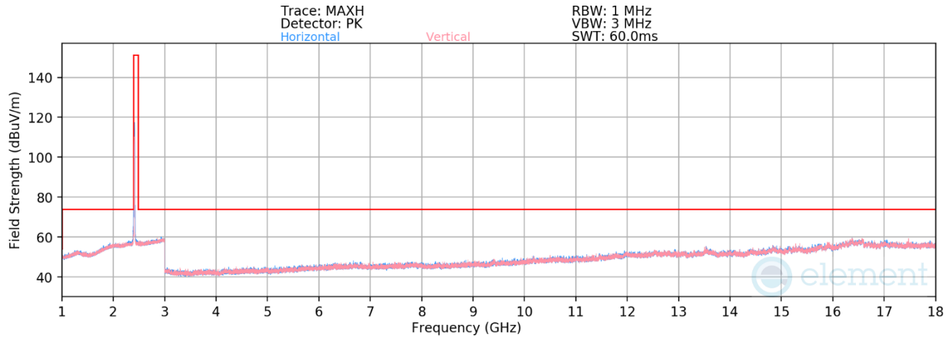
Plot 7-135. Radiated Spurious Emissions above 1GHz CDD (802.11b – Ch. 1)
