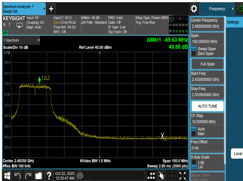
Plot 7-93. Band Edge Plot Antenna WF7b (802.11g – Ch. 8)
