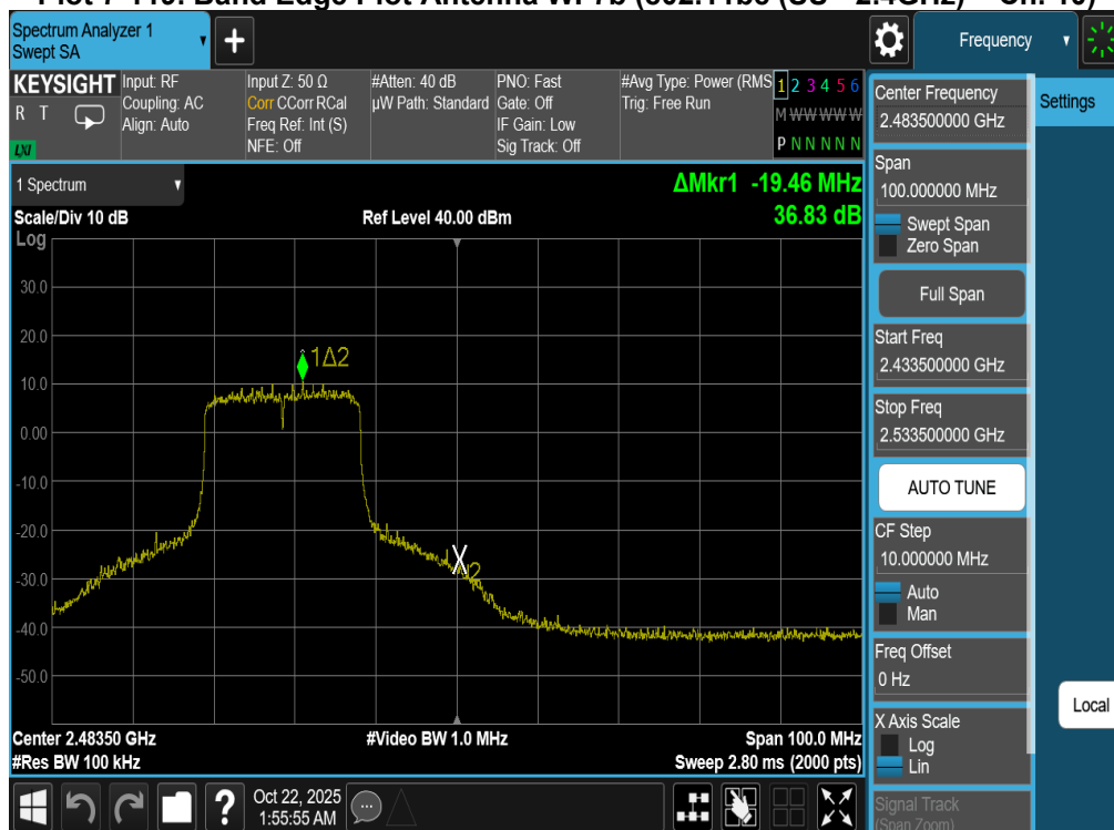
Plot 7-120. Band Edge Plot Antenna WF7b (802.11be (SU - 2.4GHz) – Ch. 11)
