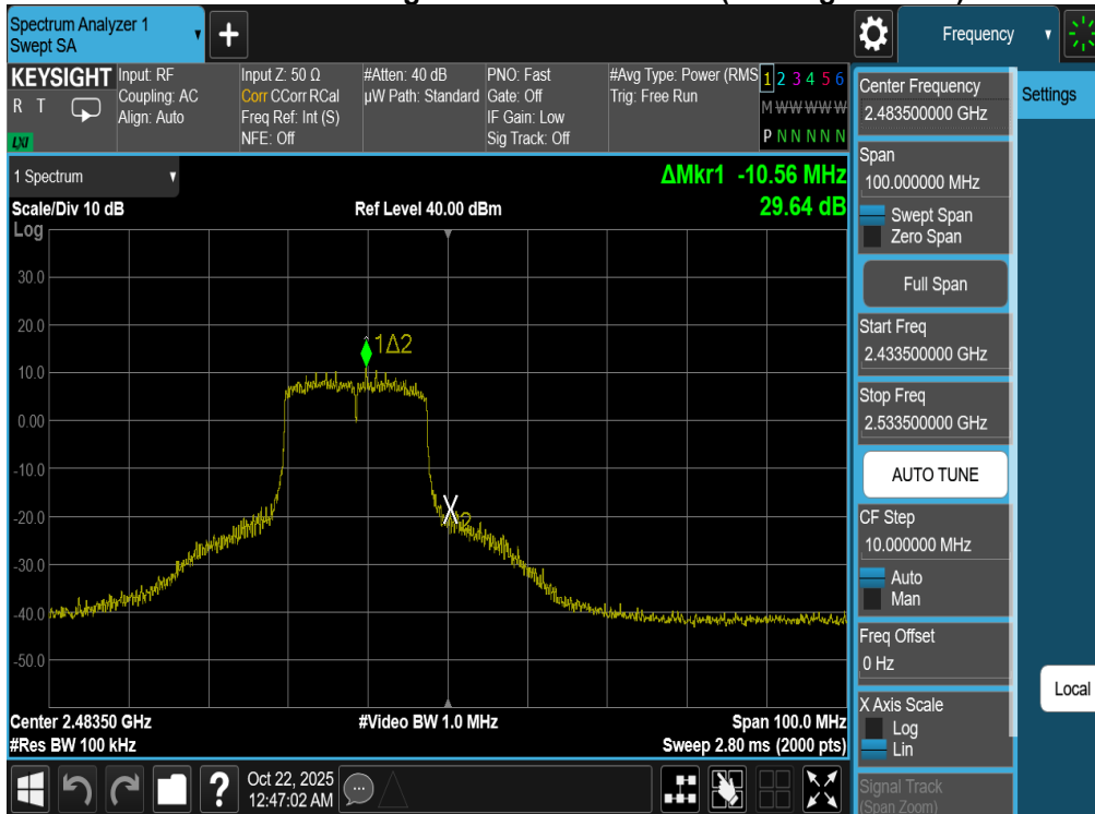
Plot 7-98. Band Edge Plot Antenna WF7b (802.11g – Ch. 13)
