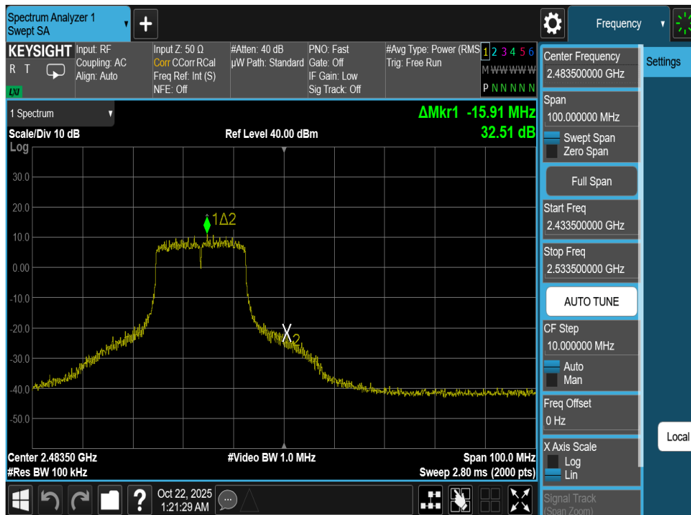
Plot 7-109. Band Edge Plot Antenna WF7b (802.11n (2.4GHz) – Ch. 12)
