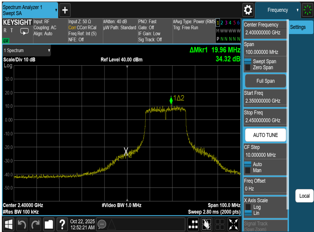
Plot 7-100. Band Edge Plot Antenna WF7b (802.11n (2.4GHz) – Ch. 2)
