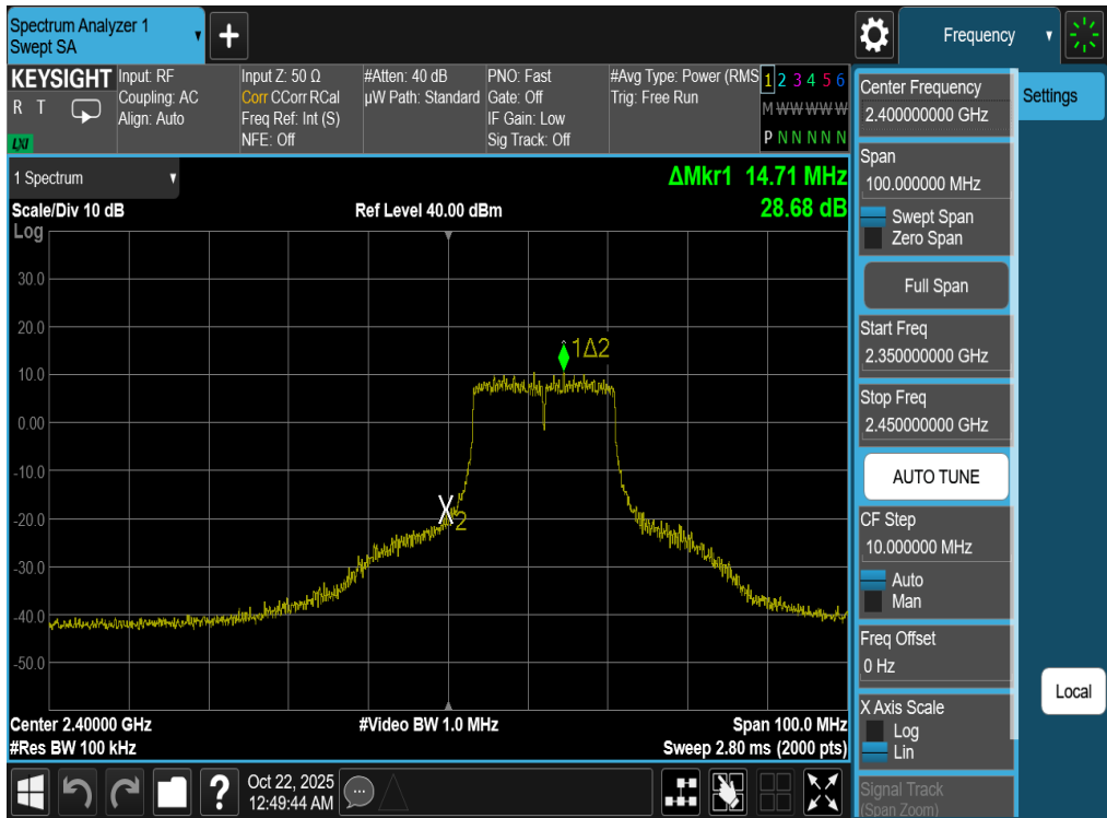
Plot 7-99. Band Edge Plot Antenna WF7b (802.11n (2.4GHz) – Ch. 1)
