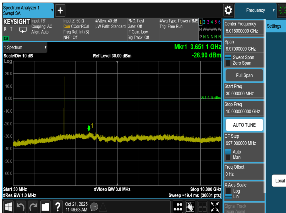
Plot 7-127. Conducted Spurious Plot Antenna WF8 (802.11b – Ch. 11)
