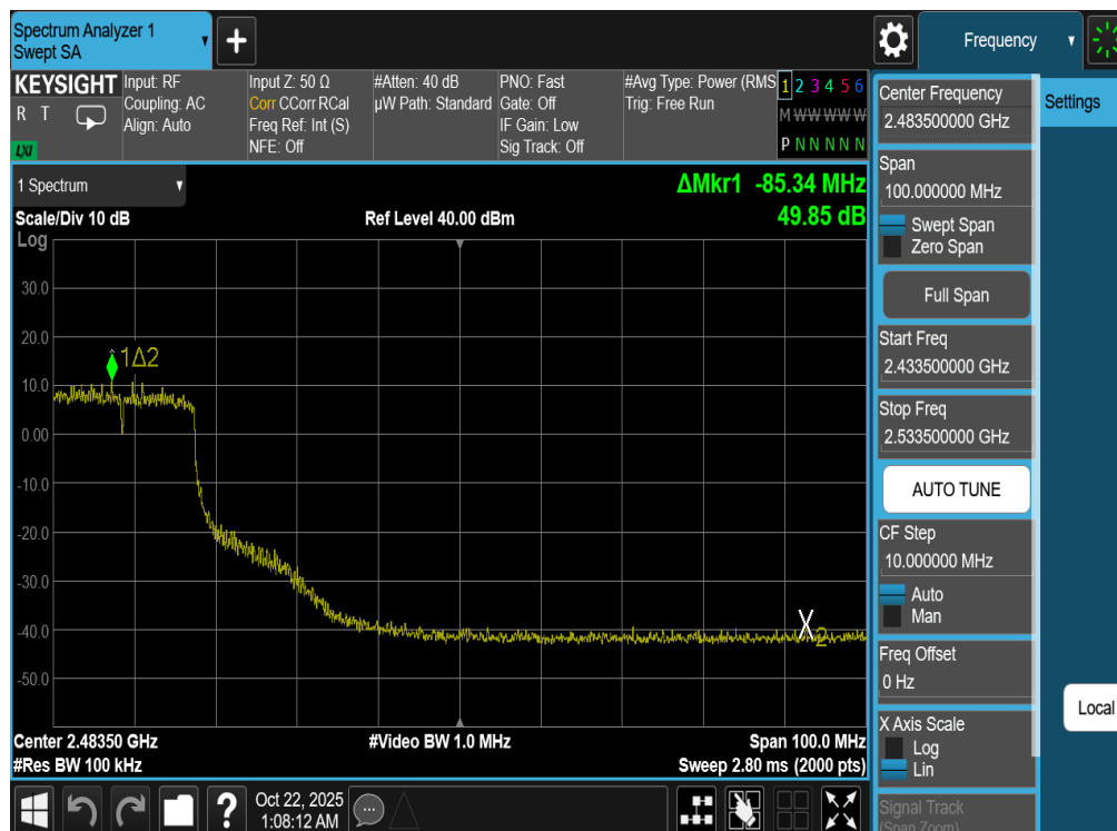
Plot 7-104. Band Edge Plot Antenna WF7b (802.11n (2.4GHz) – Ch. 7)
