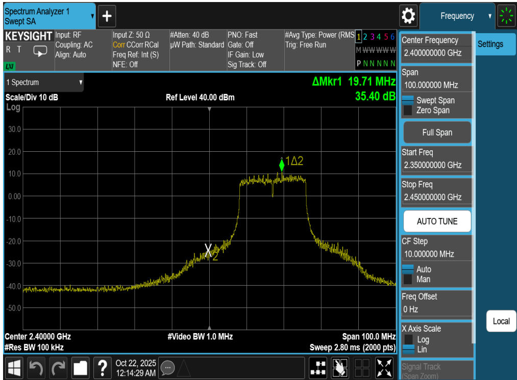
Plot 7-88. Band Edge Plot Antenna WF7b (802.11g – Ch. 2)
