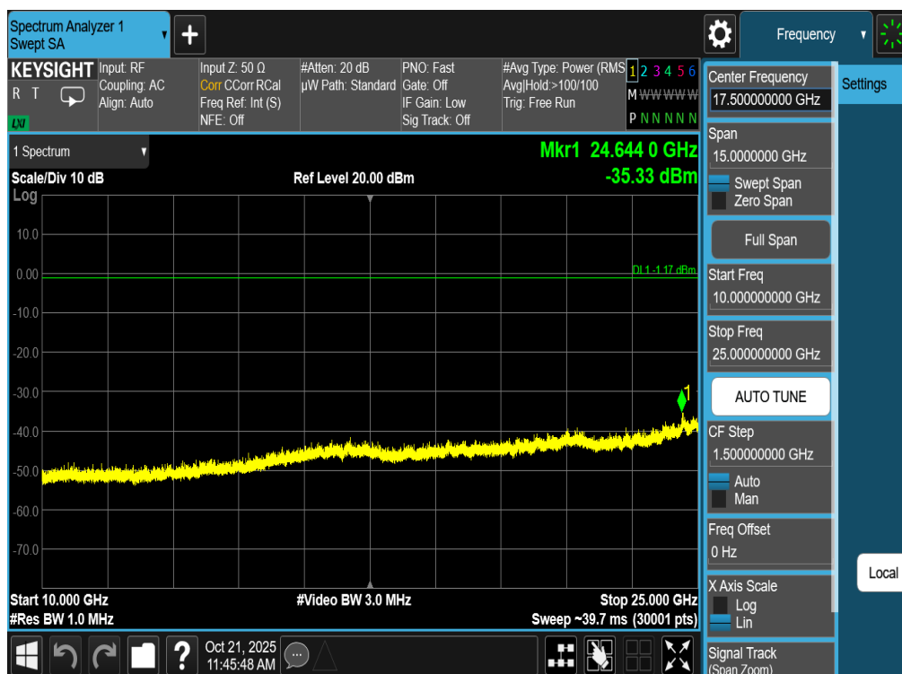
Plot 7-126. Conducted Spurious Plot Antenna WF8 (802.11b – Ch. 6)
