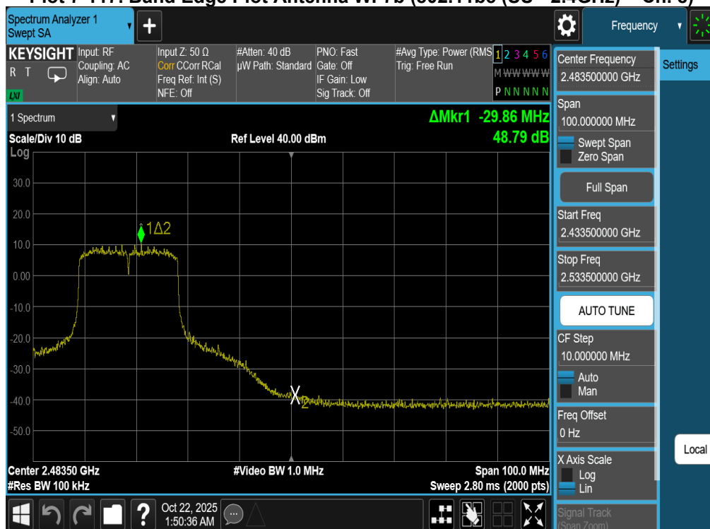
Plot 7-118. Band Edge Plot Antenna WF7b (802.11be (SU - 2.4GHz) – Ch. 9)
