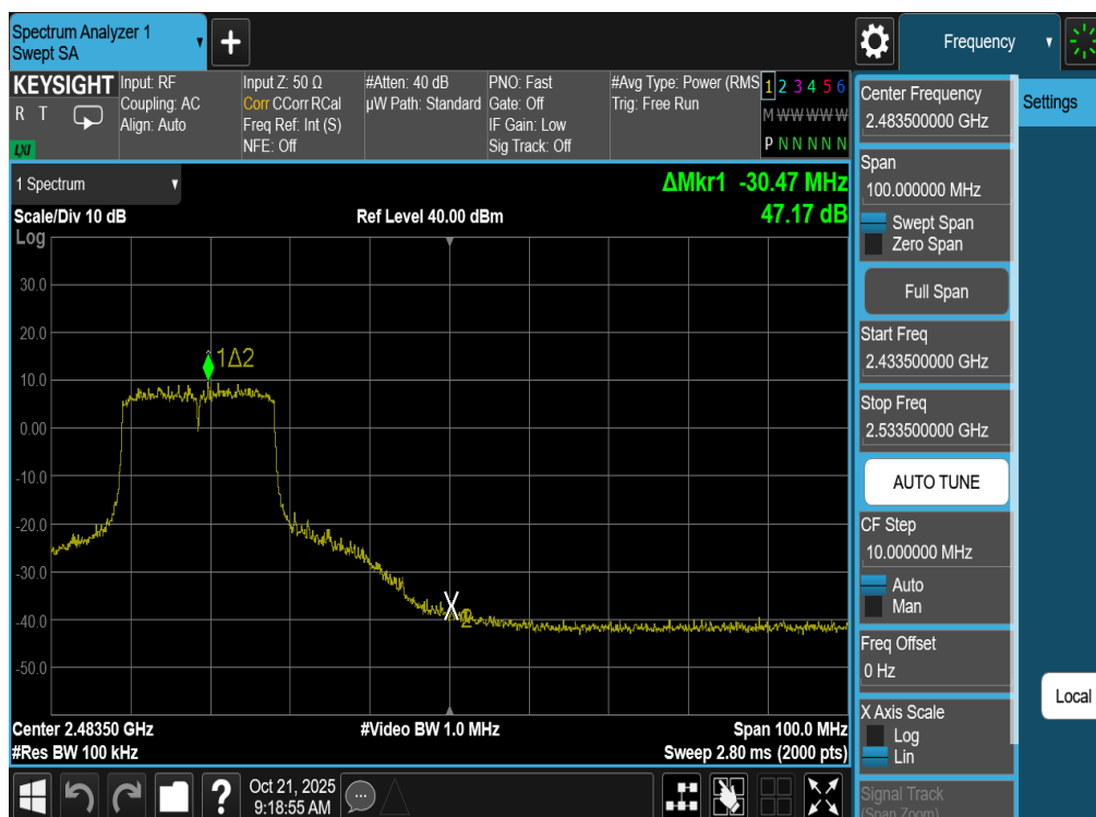
Plot 7-76. Band Edge Plot Antenna WF8 (802.11be (SU - 2.4GHz) – Ch. 9)
