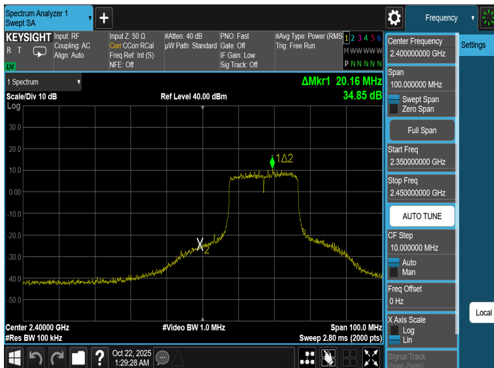
Plot 7-112. Band Edge Plot Antenna WF7b (802.11be (SU - 2.4GHz) – Ch. 2)
