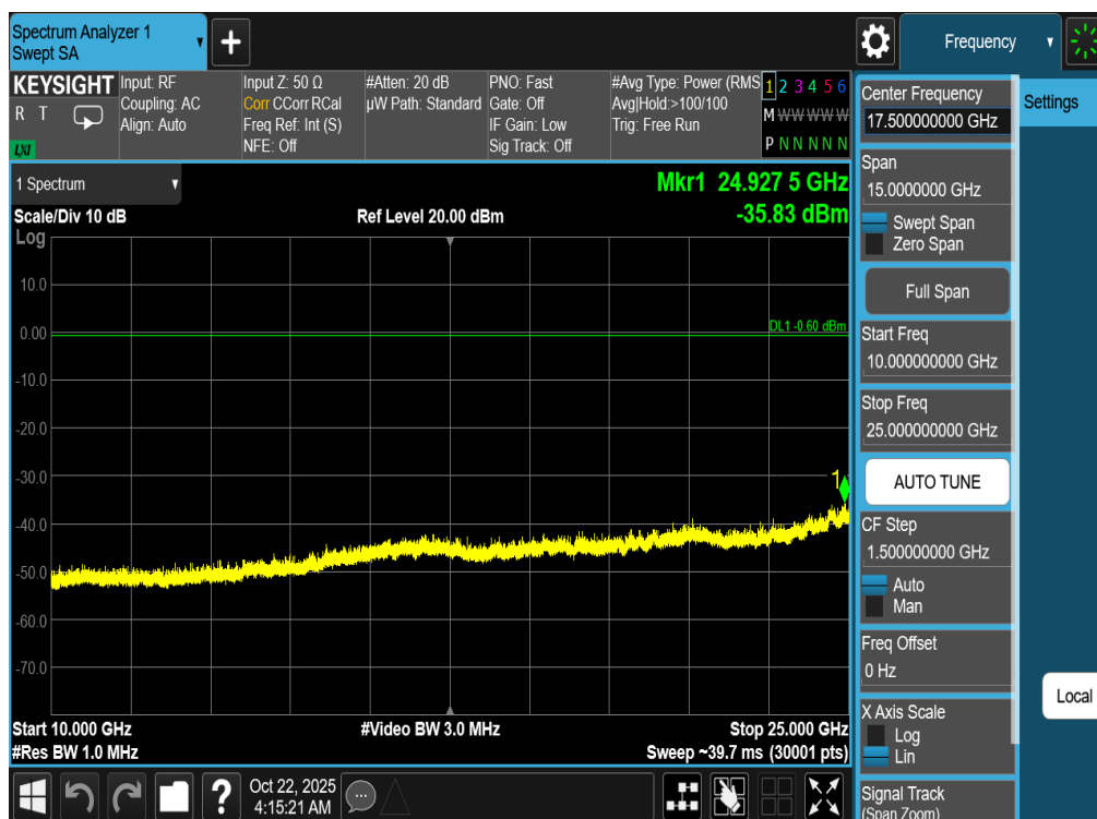
Plot 7-132. Conducted Spurious Plot Antenna WF7b (802.11b – Ch. 6)
