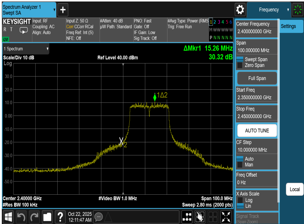
Plot 7-87. Band Edge Plot Antenna WF7b (802.11g – Ch. 1)
