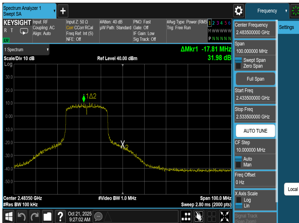
Plot 7-79. Band Edge Plot Antenna WF8 (802.11be (SU - 2.4GHz) – Ch. 12)
