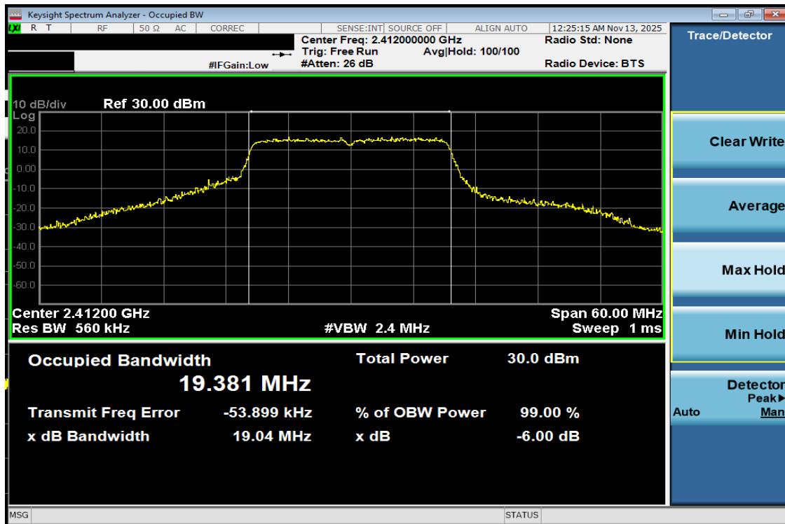
Plot 7-2 99% OBW Antenna WF8 (20MHz BW 802.11be(RU) RU242 Index61 - Ch.1)
