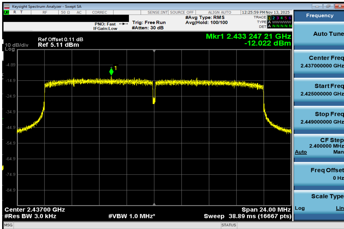
Plot 7-22 PSD Antenna WF7b (20MHz BW 802.11be(RU) RU242 Index61 - Ch.6)
