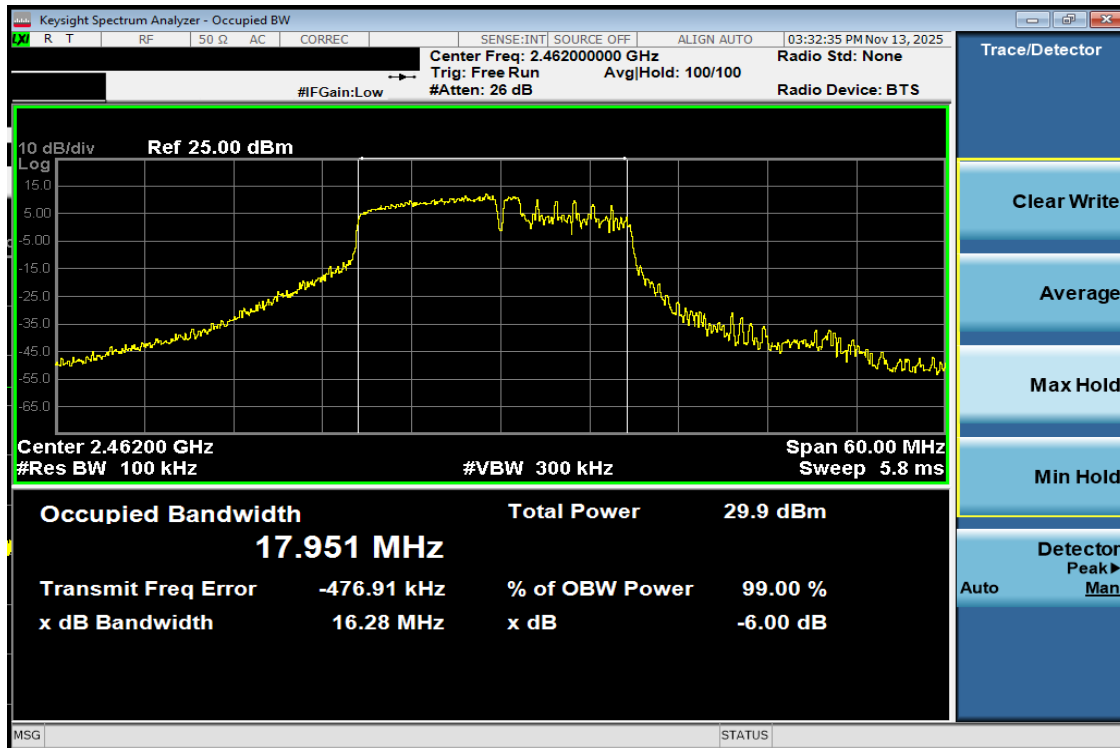
Plot 7-12 6dB OBW Antenna WF8 (20MHz BW 802.11be(RU) RU106+26 Index82 - Ch.11)
