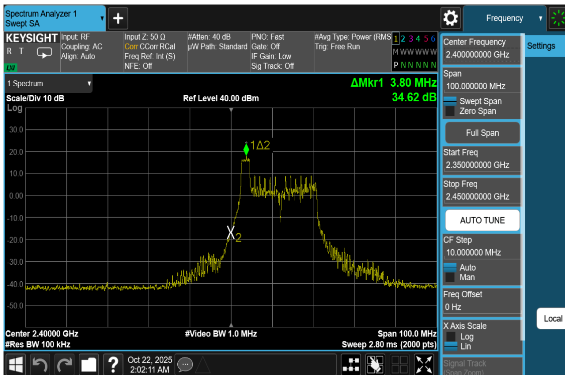
Plot 7-50. Band Edge Antenna WF7b (802.11be OFDMA – RU26 Index 0 – Ch. 1)
