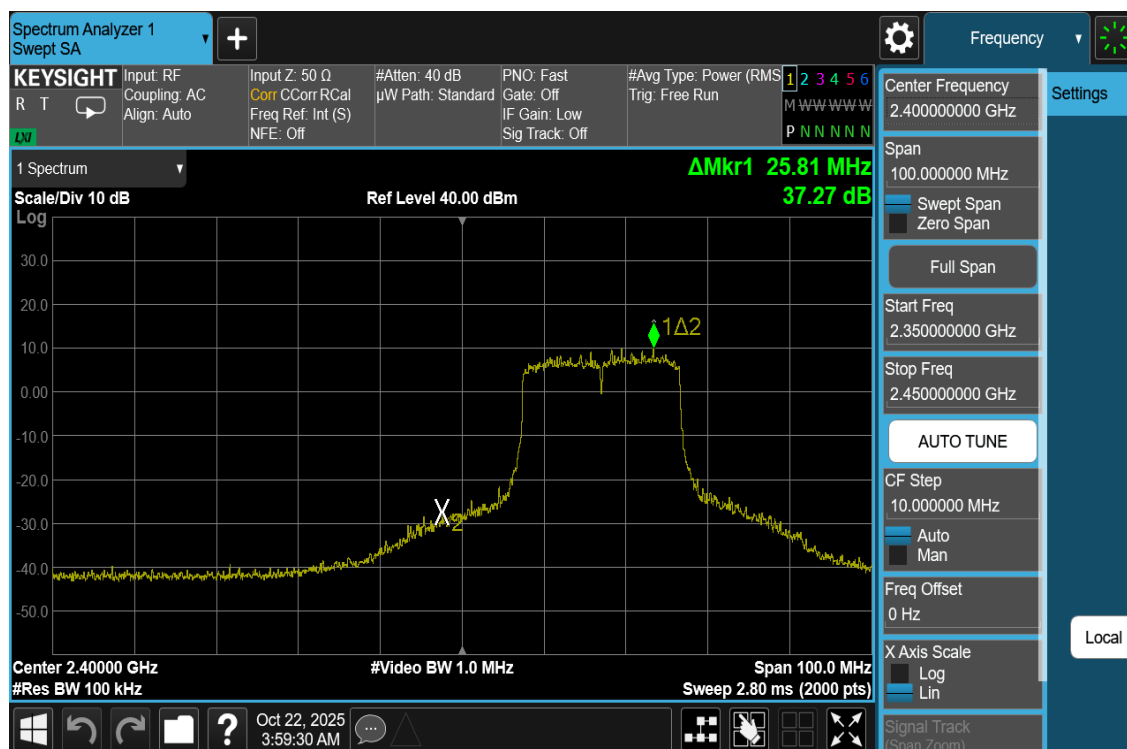
Plot 7-54. Band Edge Antenna WF7b (802.11be OFDMA - RU242 - Ch. 2)
