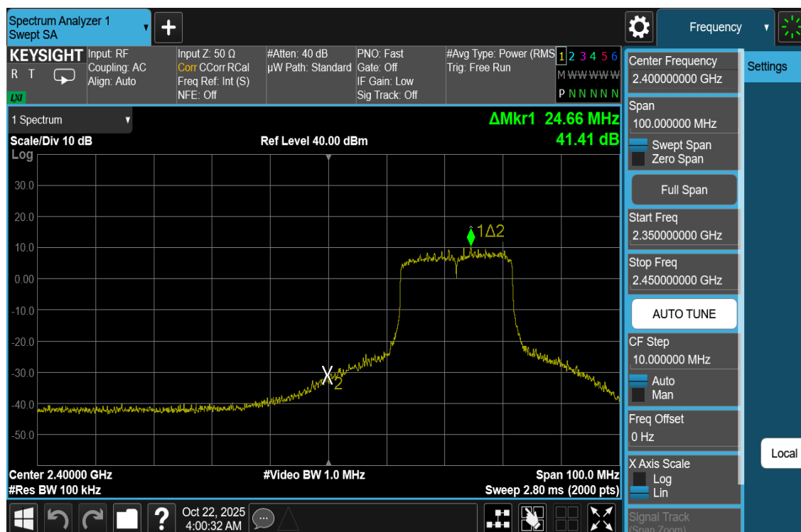
Plot 7-55. Band Edge Antenna WF7b (802.11be OFDMA - RU242 - Ch. 3)
