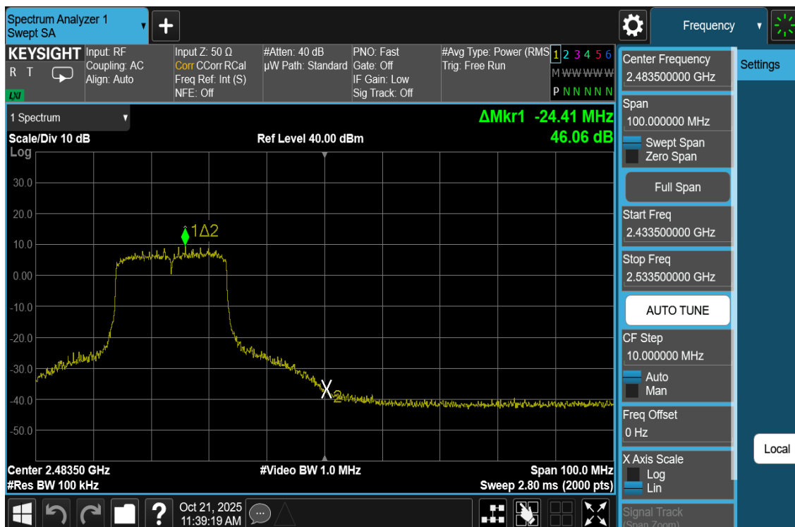
Plot 7-46. Band Edge Antenna WF8 (802.11be OFDMA – RU242 – Ch. 10)
