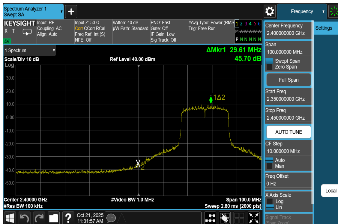
Plot 7-39. Band Edge Antenna WF8 (802.11be OFDMA – RU242 – Ch. 4)
