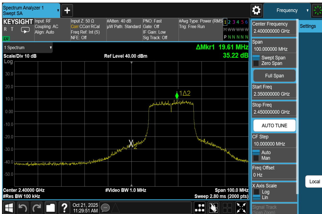
Plot 7-37. Band Edge Antenna WF8 (802.11be OFDMA – RU242 – Ch. 2)
