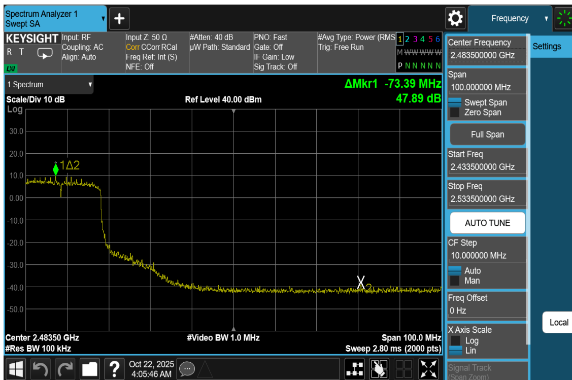
Plot 7-58. Band Edge Antenna WF7b (802.11be OFDMA – RU242 – Ch. 7)
