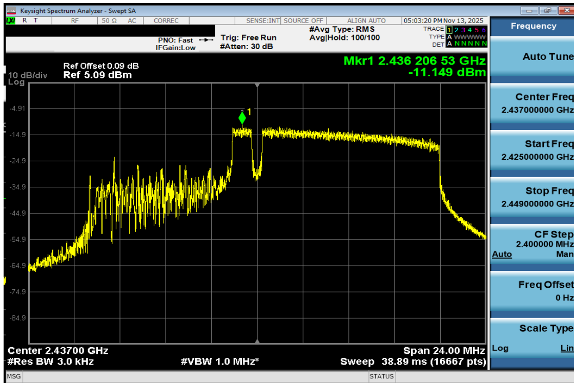
Plot 7-24 PSD Antenna WF7b (20MHz BW 802.11be(RU) RU106+26 Index83 - Ch.6)
