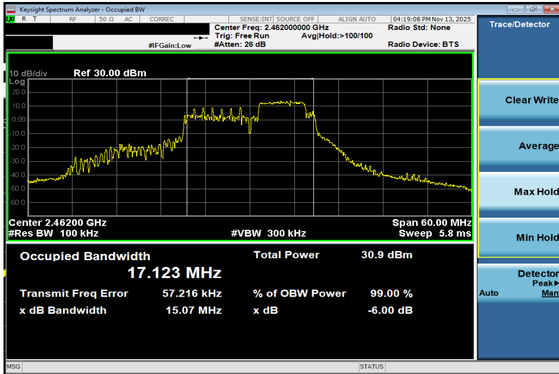
Plot 7-15 6dB OBW Antenna WF7b (20MHz BW 802.11be(RU) RU52+26 Index72 - Ch.11)
