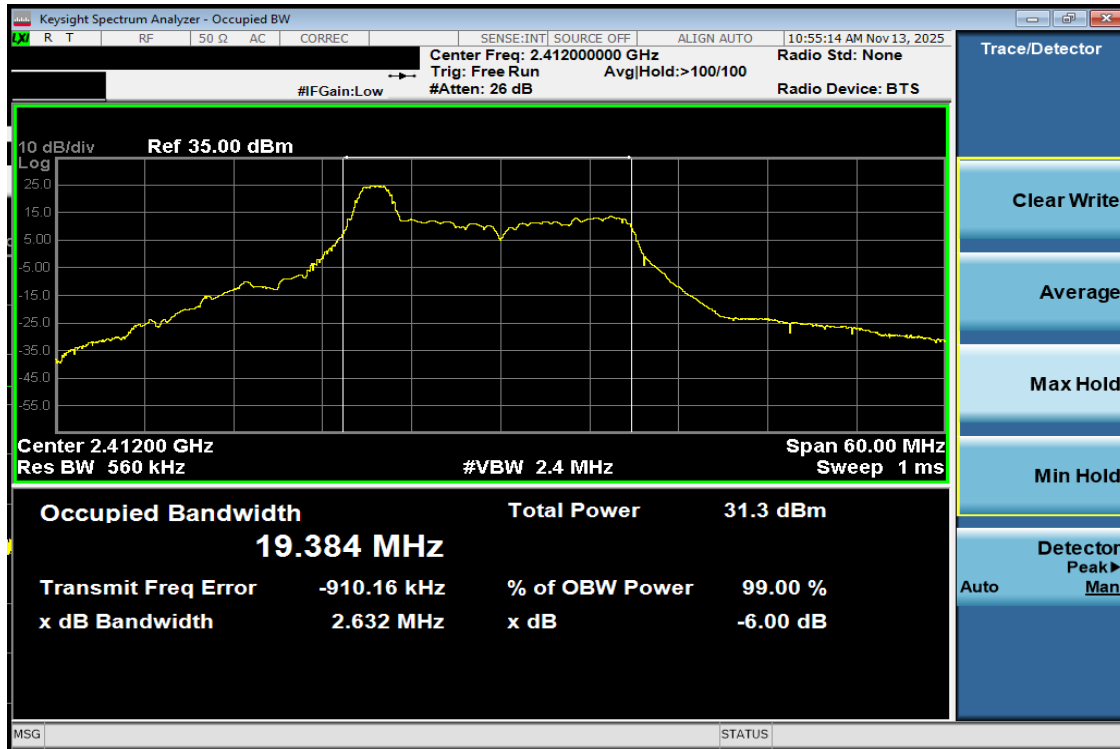
Plot 7-5 99% OBW Antenna WF7b (20MHz BW 802.11be(RU) RU26 Index0 - Ch.1)
