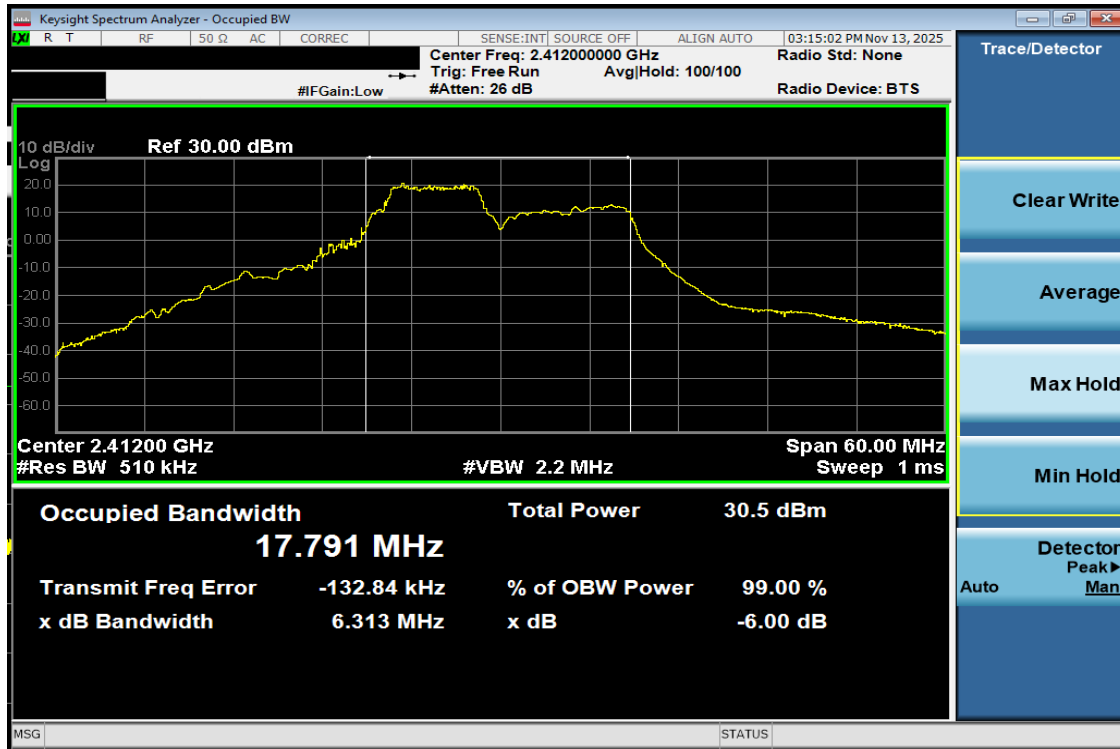
Plot 7-3 99% OBW Antenna WF8 (20MHz BW 802.11be(RU) RU52+26 Index70 - Ch.1)
