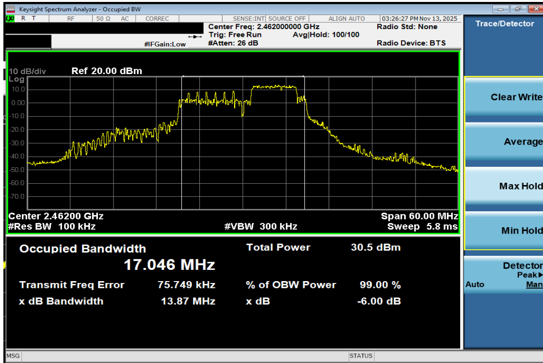
Plot 7-11 6dB OBW Antenna WF8 (20MHz BW 802.11be(RU) RU52+26 Index72 - Ch.11)
