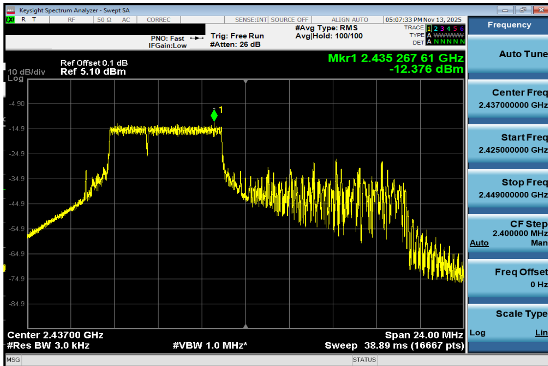
Plot 7-30 PSD CDD Antenna WF7b (20MHz BW 802.11be(RU) RU52+26 Index70 - Ch.6)
