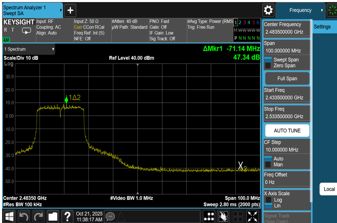
Plot 7-45. Band Edge Antenna WF8 (802.11be OFDMA – RU242 – Ch. 9)
