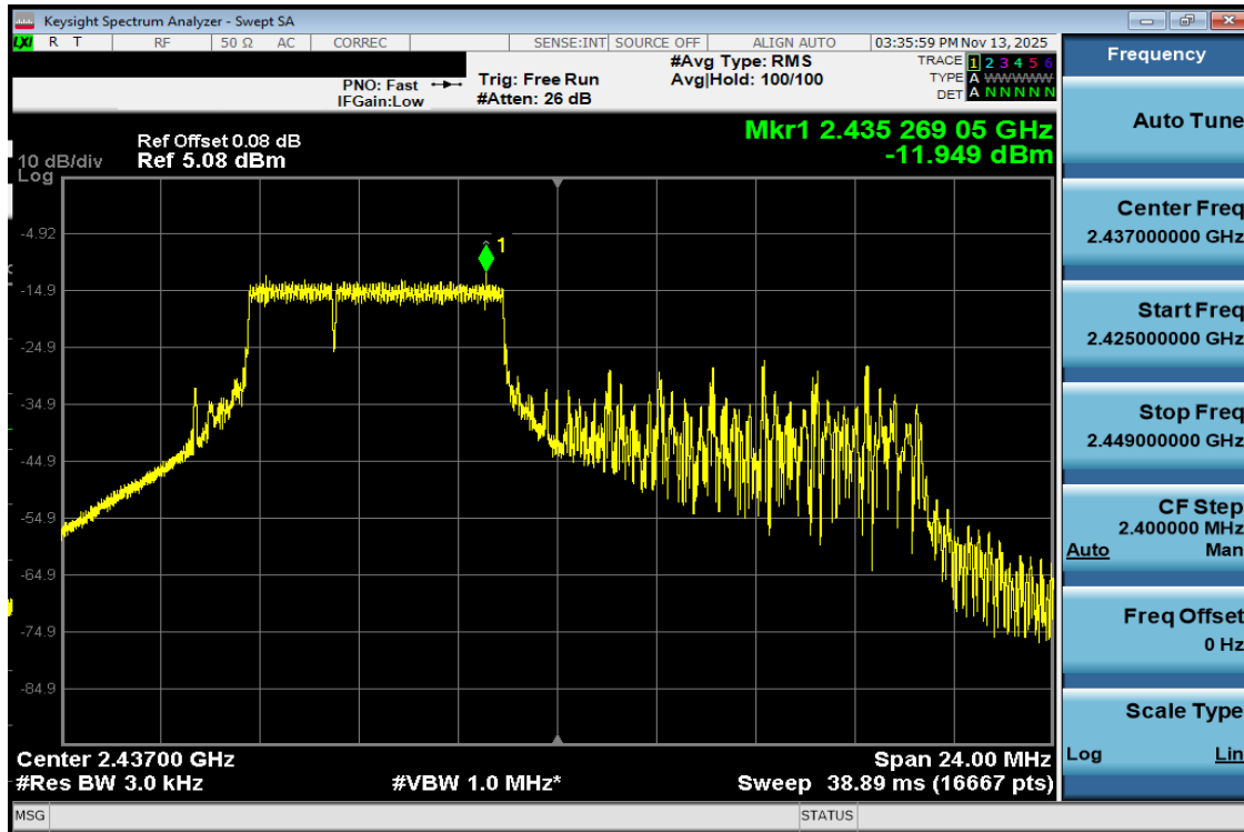
Plot 7-19 PSD Antenna WF8 (20MHz BW 802.11be(RU) RU52+26 Index70 - Ch.6)
