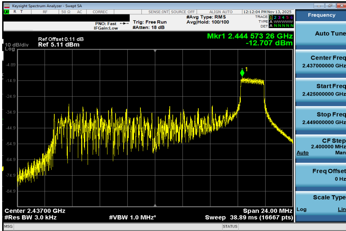
Plot 7-21 PSD Antenna WF7b (20MHz BW 802.11be(RU) RU26 Index8 - Ch.6)
