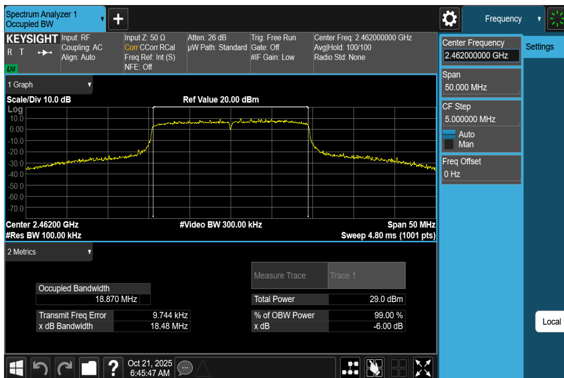
Plot 7-10 6dB OBW Antenna WF8 (20MHz BW 802.11be(RU) RU242 Index61 - Ch.11)
