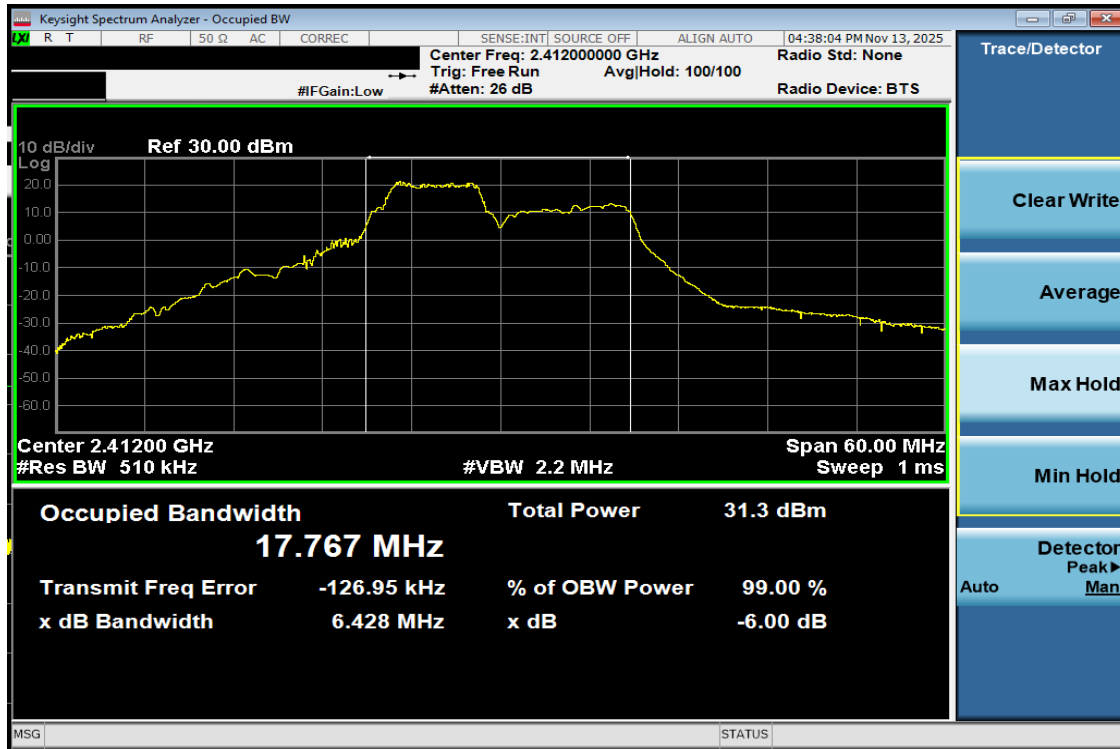
Plot 7-7 99% OBW Antenna WF7b (20MHz BW 802.11be(RU) RU52+26 Index70 - Ch.1)
