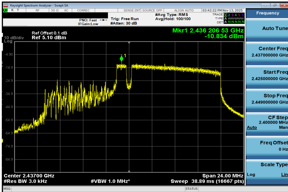
Plot 7-20 PSD Antenna WF8 (20MHz BW 802.11be(RU) RU106+26 Index83 - Ch.6)
