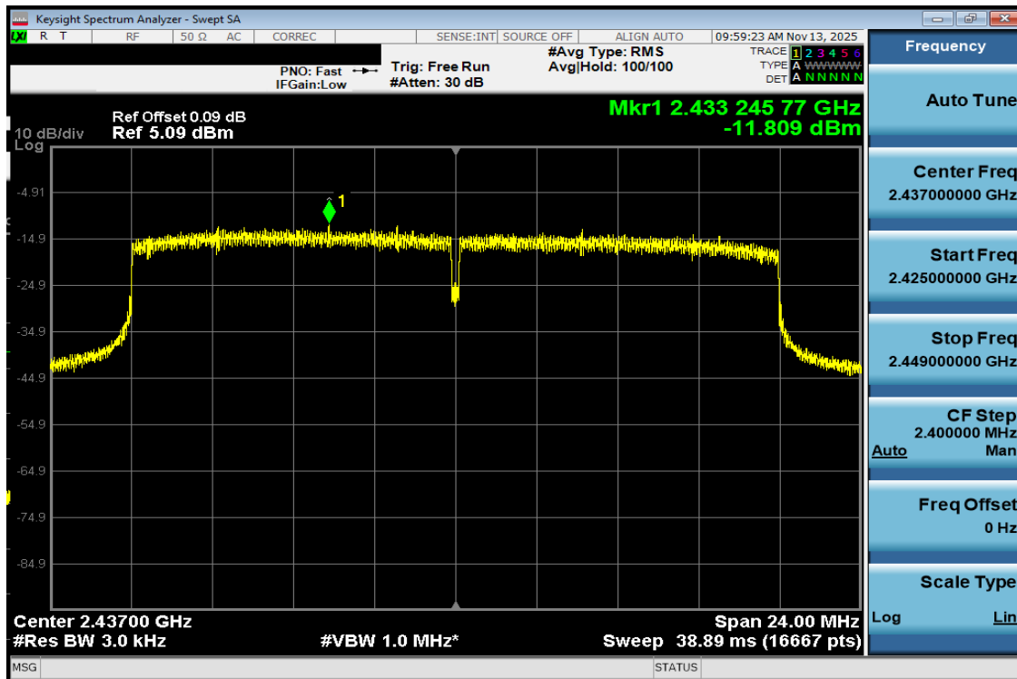
Plot 7-18 PSD Antenna WF8 (20MHz BW 802.11be(RU) RU242 Index61 - Ch.6)
