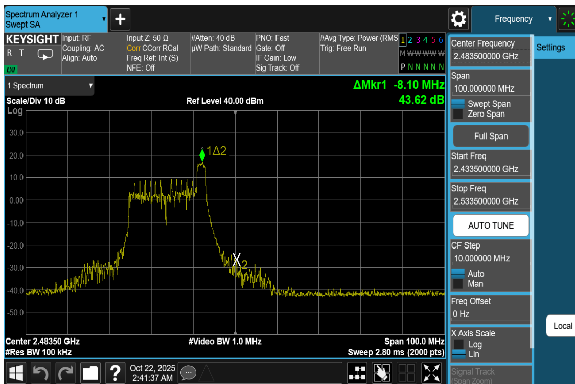
Plot 7-51. Band Edge Antenna WF7b (802.11be OFDMA – RU26 Index 8 – Ch. 12)
