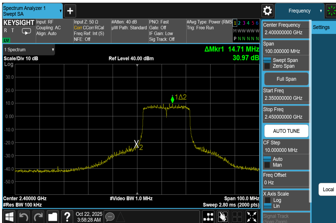
Plot 7-53. Band Edge Antenna WF7b (802.11be OFDMA – RU242 – Ch. 1)
