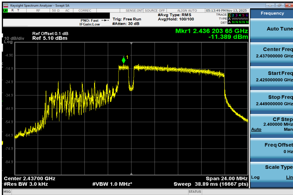
Plot 7-32 PSD CDD Antenna WF7b (20MHz BW 802.11be(RU) RU106+26 Index83 - Ch.6)
