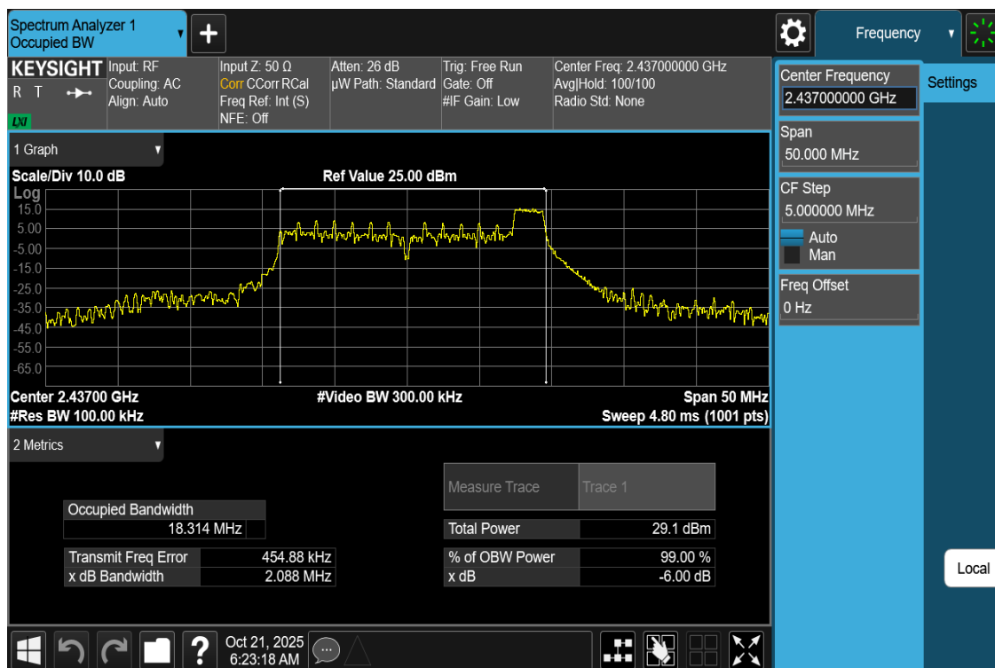
Plot 7-9 6dB OBW Antenna WF8 (20MHz BW 802.11be(RU) RU26 Index8 - Ch.6)
