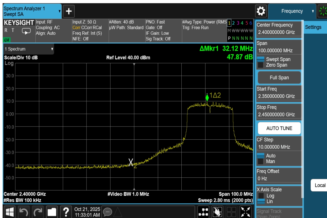
Plot 7-40. Band Edge Antenna WF8 (802.11be OFDMA – RU242 – Ch. 5)
