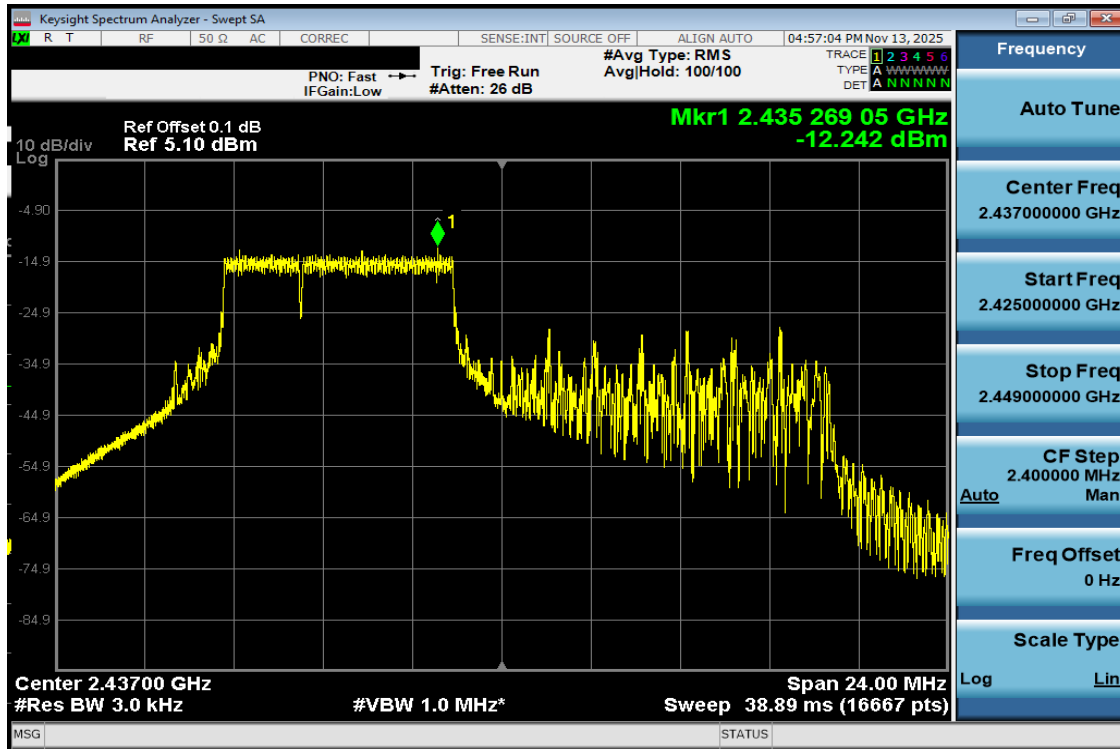
Plot 7-23 PSD Antenna WF7b (20MHz BW 802.11be(RU) RU52+26 Index70 - Ch.6)
