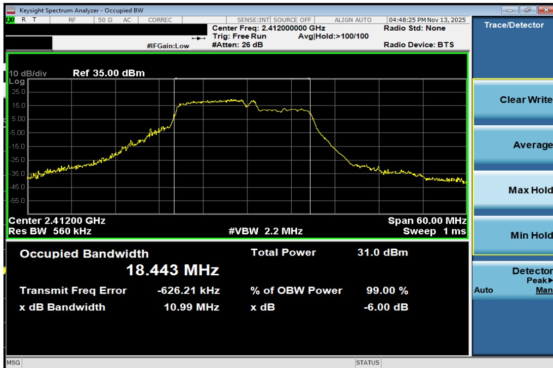
Plot 7-8 99% OBW Antenna WF7b (20MHz BW 802.11be(RU) RU106+26 Index82 - Ch.1)
