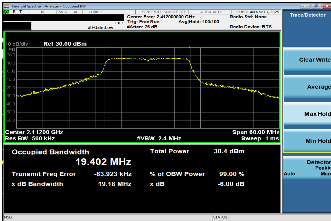
Plot 7-6 99% OBW Antenna WF7b (20MHz BW 802.11be(RU) RU242 Index61 - Ch.1)
