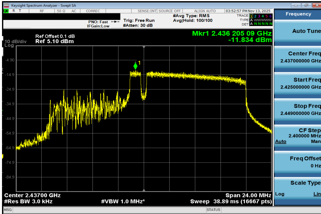
Plot 7-31 PSD CDD Antenna WF8 (20MHz BW 802.11be(RU) RU106+26 Index83 - Ch.6)
