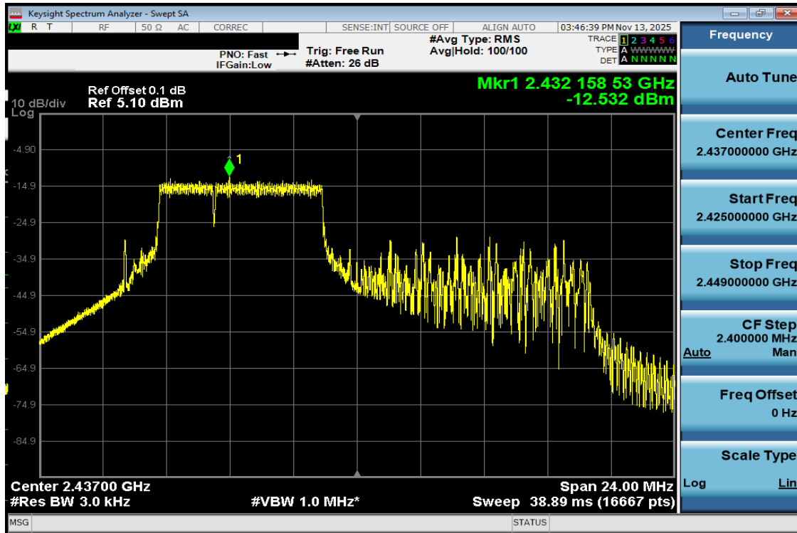
Plot 7-29 PSD CDD Antenna WF8 (20MHz BW 802.11be(RU) RU52+26 Index70 - Ch.6)
