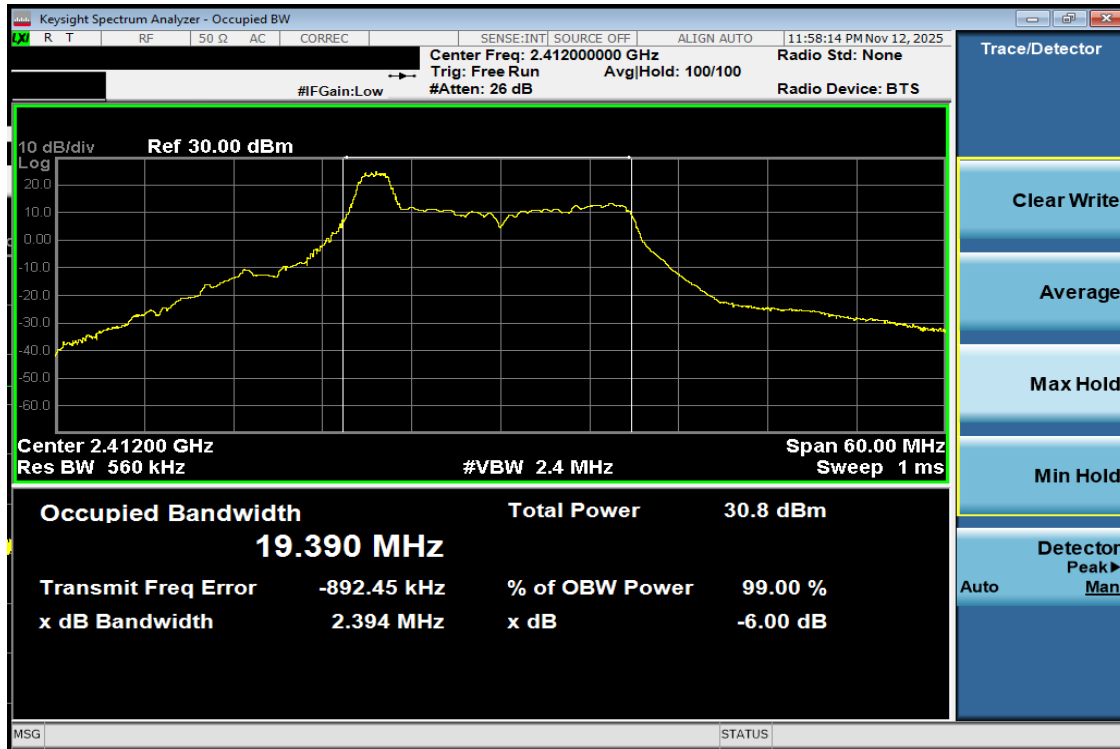
Plot 7-1 99% OBW Antenna WF8 (20MHz BW 802.11be(RU) RU26 Index0 - Ch.1)
