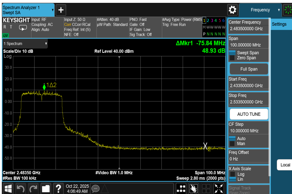
Plot 7-59. Band Edge Antenna WF7b (802.11be OFDMA – RU242 – Ch. 8)
