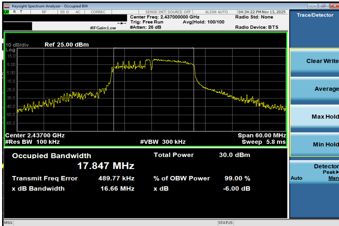
Plot 7-16 6dB OBW Antenna WF7b (20MHz BW 802.11be(RU) RU106+26 Index83 - Ch.6)
