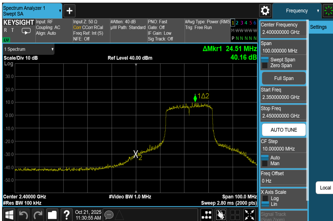
Plot 7-38. Band Edge Antenna WF8 (802.11be OFDMA – RU242 – Ch. 3)
