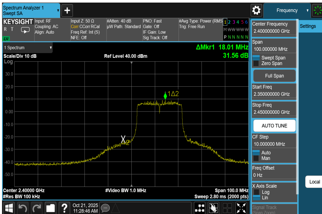
Plot 7-36. Band Edge Antenna WF8 (802.11be OFDMA – RU242 – Ch. 1)
