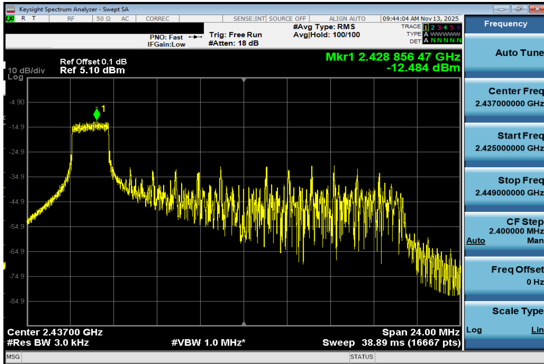
Plot 7-17 PSD Antenna WF8 (20MHz BW 802.11be(RU) RU26 Index0 - Ch.6)
