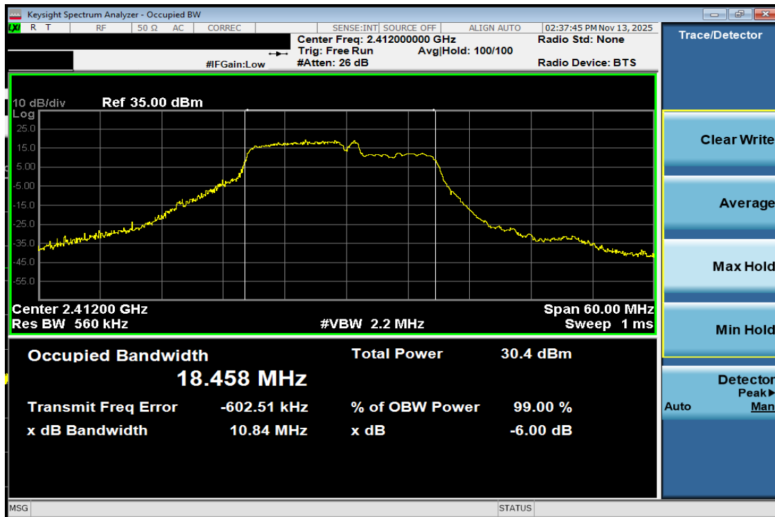
Plot 7-4 99% OBW Antenna WF8 (20MHz BW 802.11be(RU) RU106+26 Index82 - Ch.1)
