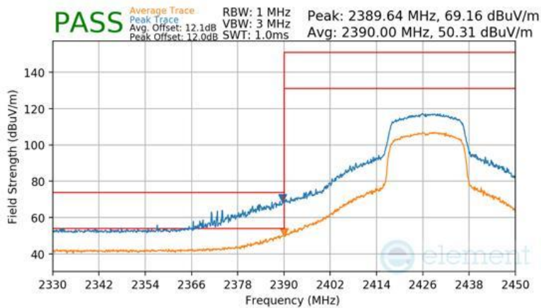
Plot 7-117 Radiated Restricted Lower Band Edge Measurement Antenna WF8 (Peak & Average – RU242)
