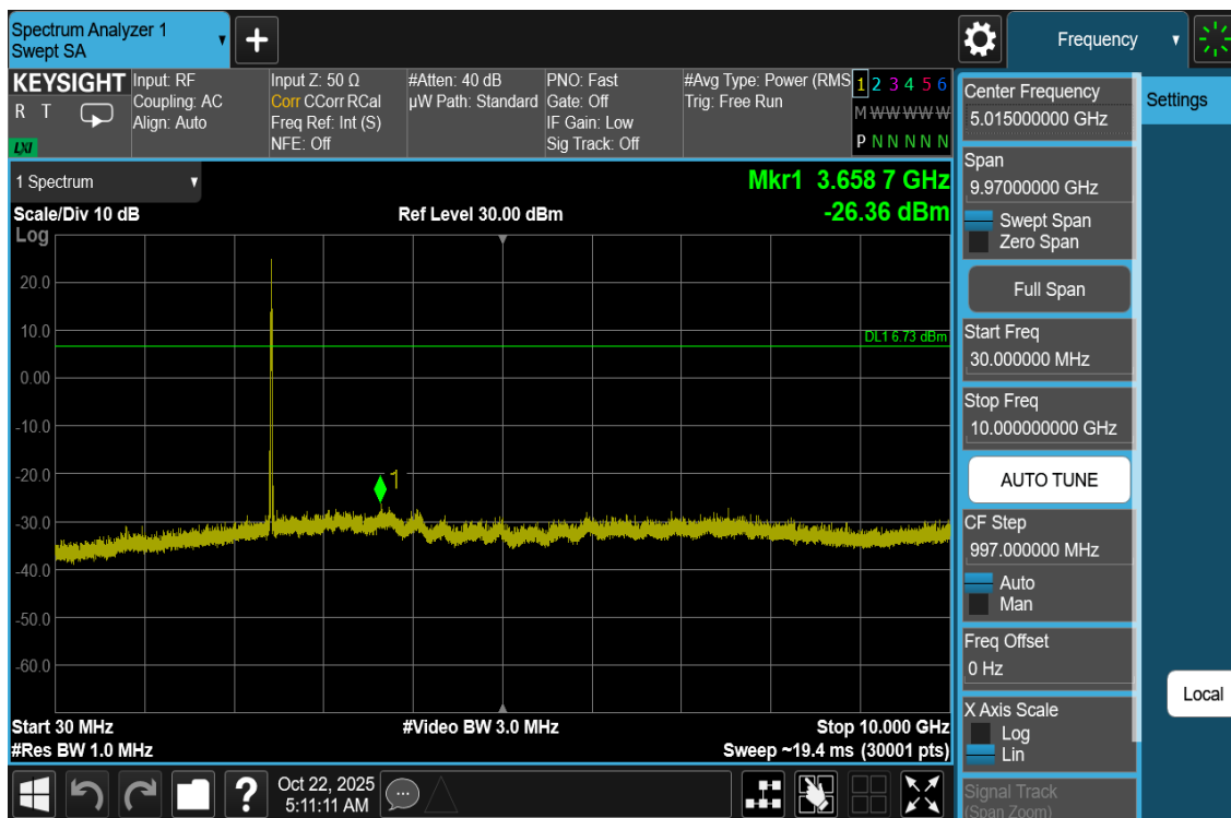
Plot 7-79. Conducted Spurious Plot Antenna WF7b (802.11be OFDMA – RU26 – Ch. 6)
