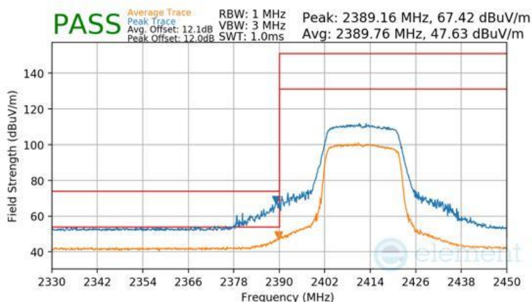
Plot 7-114 Radiated Restricted Lower Band Edge Measurement Antenna WF8 (Peak & Average – RU242)
