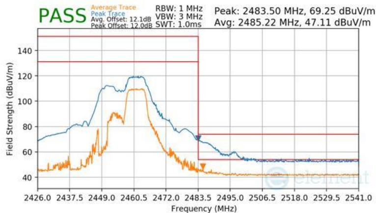
Plot 7-107 Radiated Restricted Upper Band Edge Measurement Antenna WF8 (Peak & Average – RU52+26)
