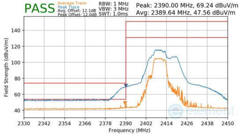
Plot 7-100 Radiated Restricted Lower Band Edge Measurement Antenna WF8 (Peak & Average – RU52+26)
