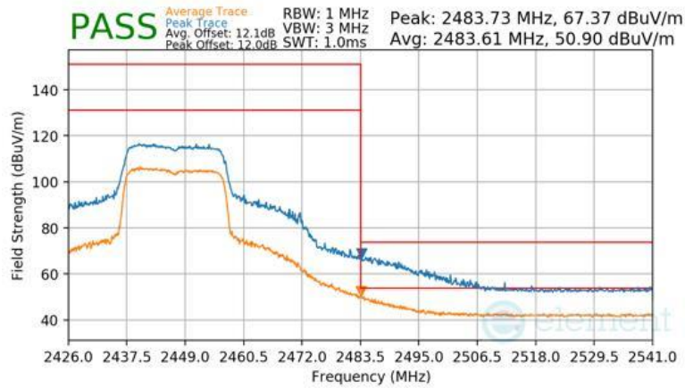
Plot 7-122 Radiated Restricted Upper Band Edge Measurement Antenna WF8 (Peak & Average – RU242)
