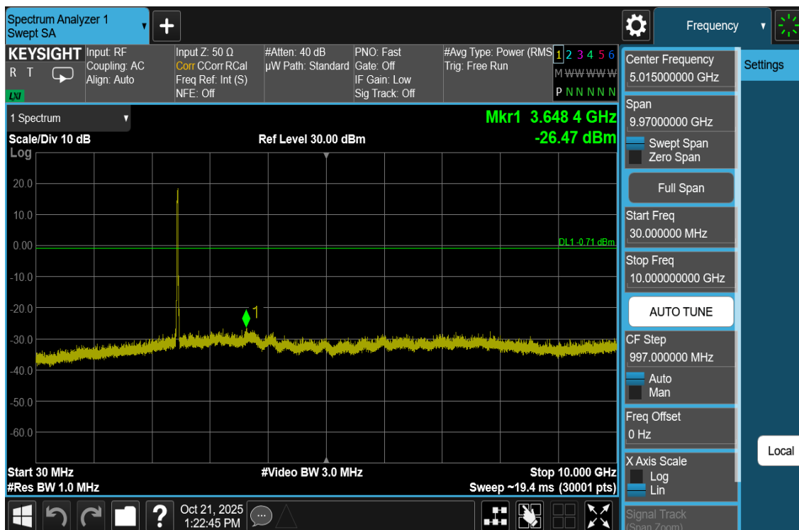
Plot 7-75. Conducted Spurious Plot Antenna WF8 (802.11be OFDMA – RU242 – Ch. 11)
