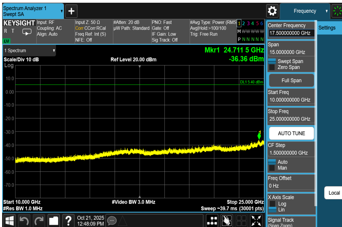
Plot 7-70. Conducted Spurious Plot Antenna WF8 (802.11be OFDMA – RU26 – Ch. 11)
