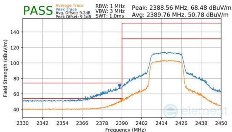
Plot 7-115 Radiated Restricted Lower Band Edge Measurement Antenna WF8 (Peak & Average – RU242)
