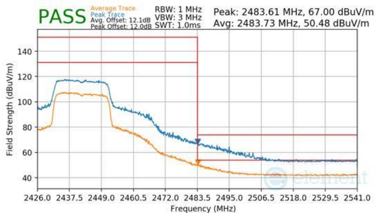
Plot 7-121 Radiated Restricted Upper Band Edge Measurement Antenna WF8 (Peak & Average – RU242)
