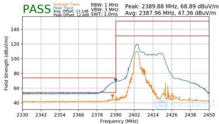
Plot 7-128 Radiated Restricted Lower Band Edge Measurement Antenna WF7b (Peak & Average – RU26)
