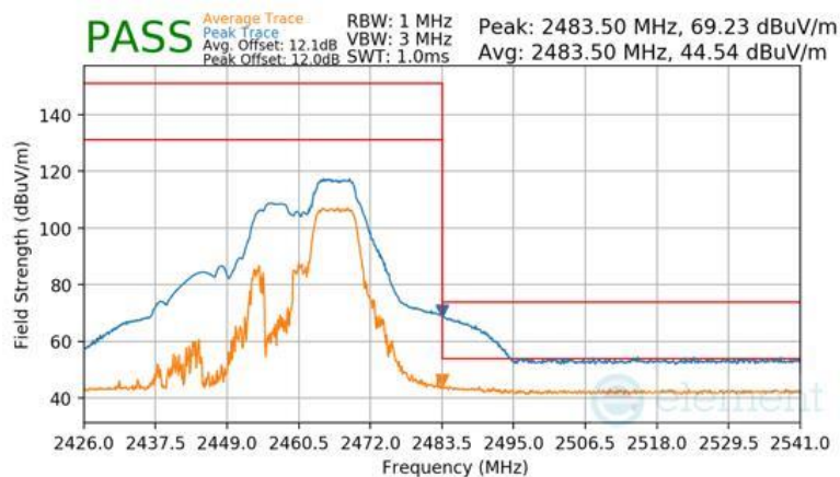
Plot 7-109 Radiated Restricted Upper Band Edge Measurement Antenna WF8 (Peak & Average – RU52+26)
