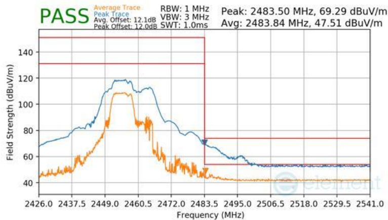
Plot 7-106 Radiated Restricted Upper Band Edge Measurement Antenna WF8 (Peak & Average – RU52+26)
