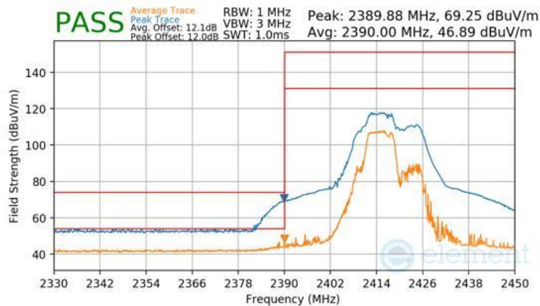
Plot 7-102 Radiated Restricted Lower Band Edge Measurement Antenna WF8 (Peak & Average – RU52+26)
