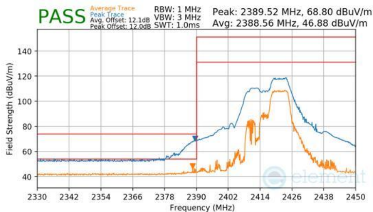
Plot 7-103 Radiated Restricted Lower Band Edge Measurement Antenna WF8 (Peak & Average – RU52+26)
