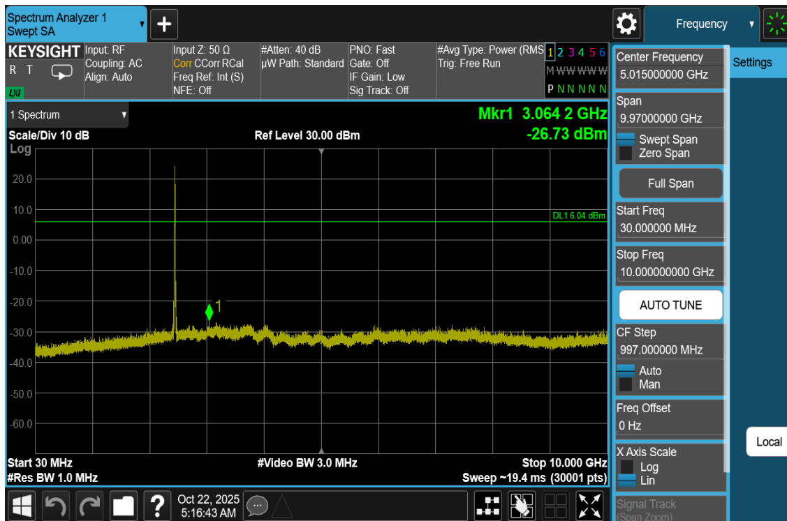
Plot 7-81. Conducted Spurious Plot Antenna WF7b (802.11be OFDMA – RU26 – Ch. 11)
