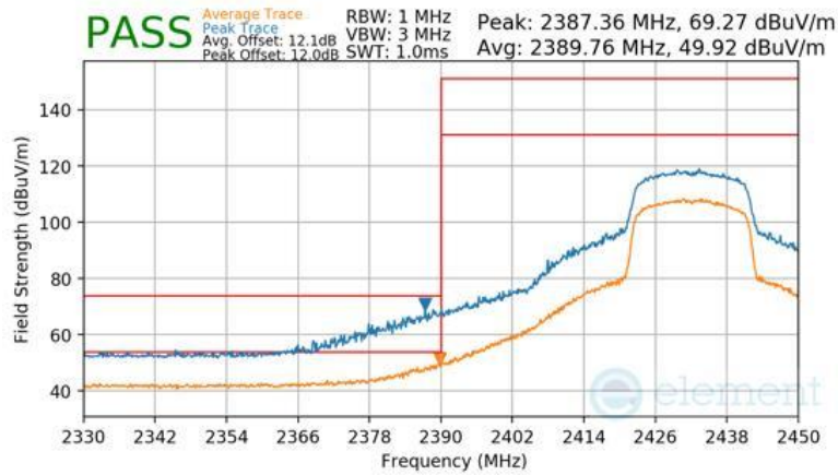
Plot 7-118 Radiated Restricted Lower Band Edge Measurement Antenna WF8 (Peak & Average – RU242)
