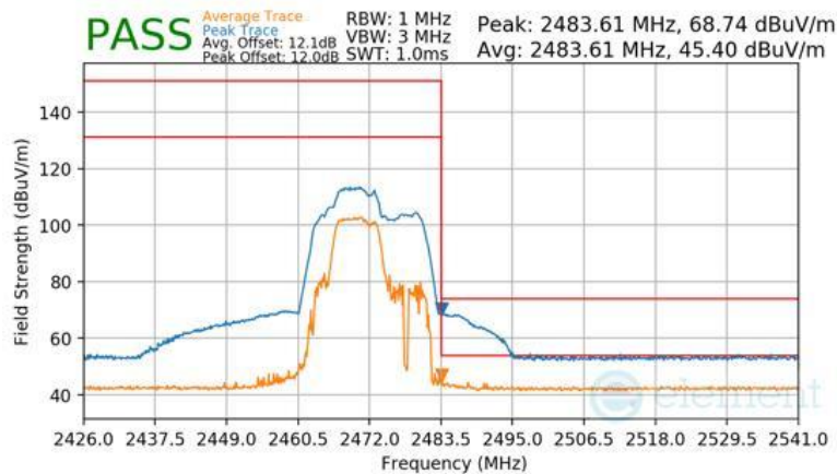
Plot 7-112 Radiated Restricted Upper Band Edge Measurement Antenna WF8 (Peak & Average – RU52+26)
