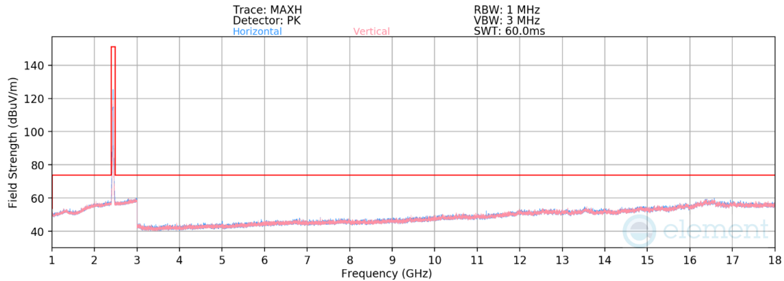
Plot 7-90. Radiated Spurious Emissions above 1GHz CDD (802.11be OFDMA – RU26 – Ch. 6)
