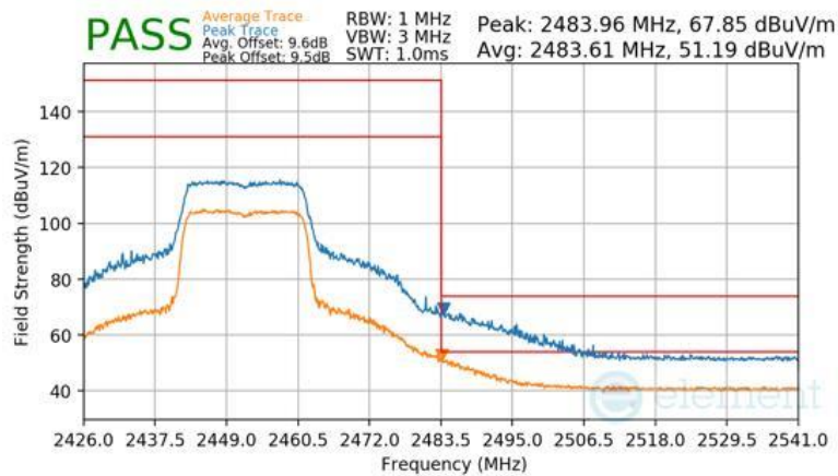
Plot 7-123 Radiated Restricted Upper Band Edge Measurement Antenna WF8 (Peak & Average – RU242)
