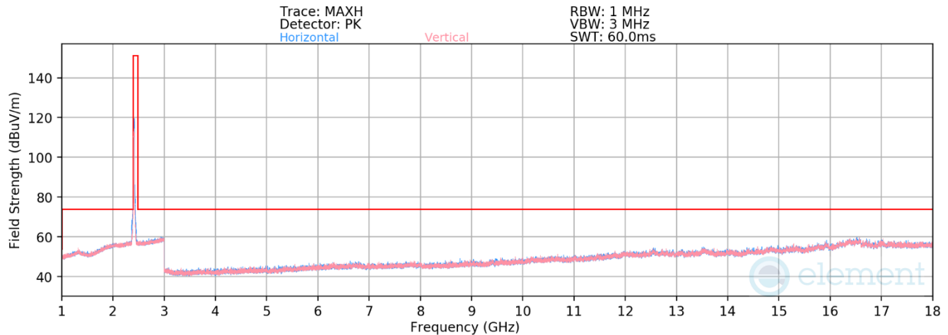
Plot 7-93. Radiated Spurious Emissions above 1GHz CDD (802.11be OFDMA – RU242 – Ch. 1)
