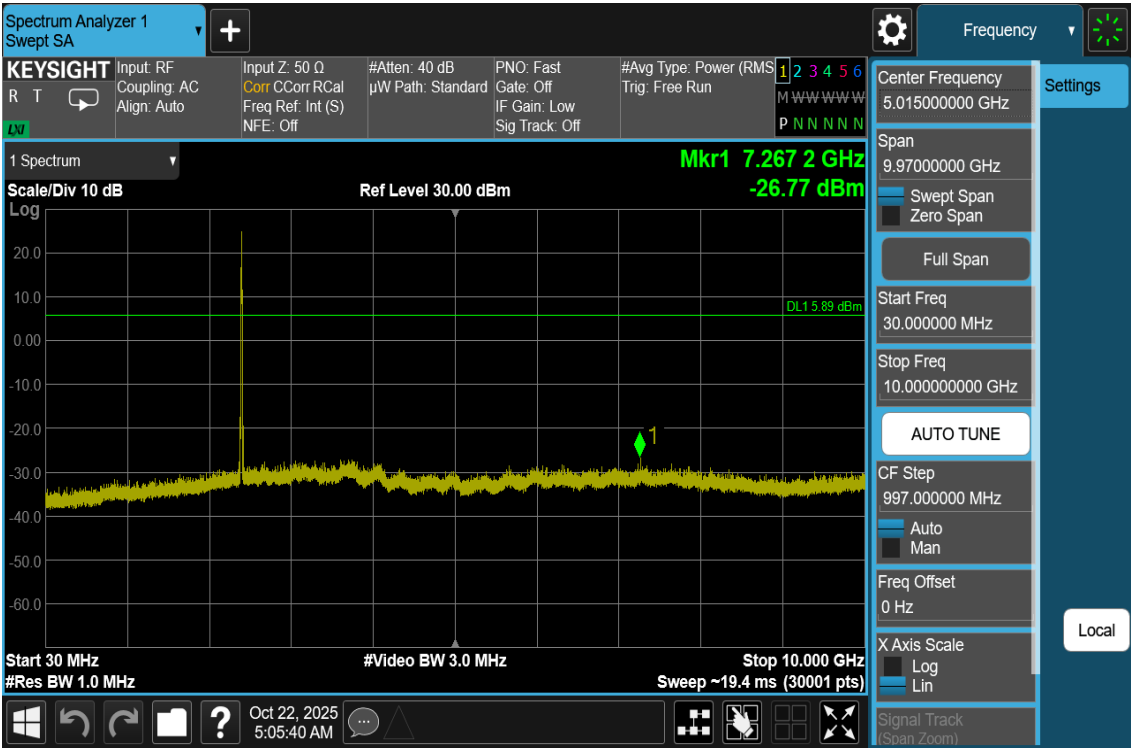
Plot 7-77. Conducted Spurious Plot Antenna WF7b (802.11be OFDMA – RU26 – Ch. 1)
