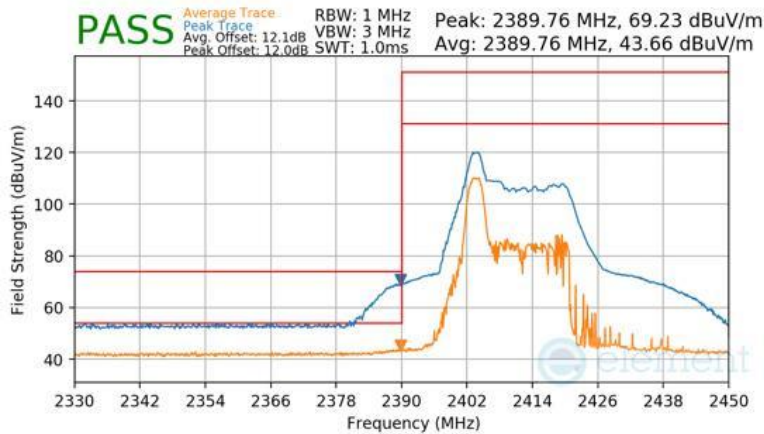
Plot 7-97 Radiated Restricted Lower Band Edge Measurement Antenna WF8 (Peak & Average – RU26)
