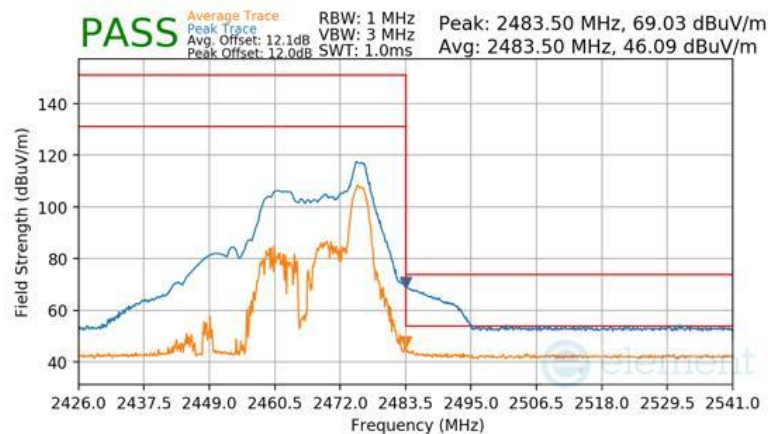
Plot 7-129 Radiated Restricted Upper Band Edge Measurement Antenna WF7b (Peak & Average – RU26)
