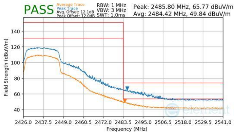
Plot 7-120 Radiated Restricted Upper Band Edge Measurement Antenna WF8 (Peak & Average – RU242)
