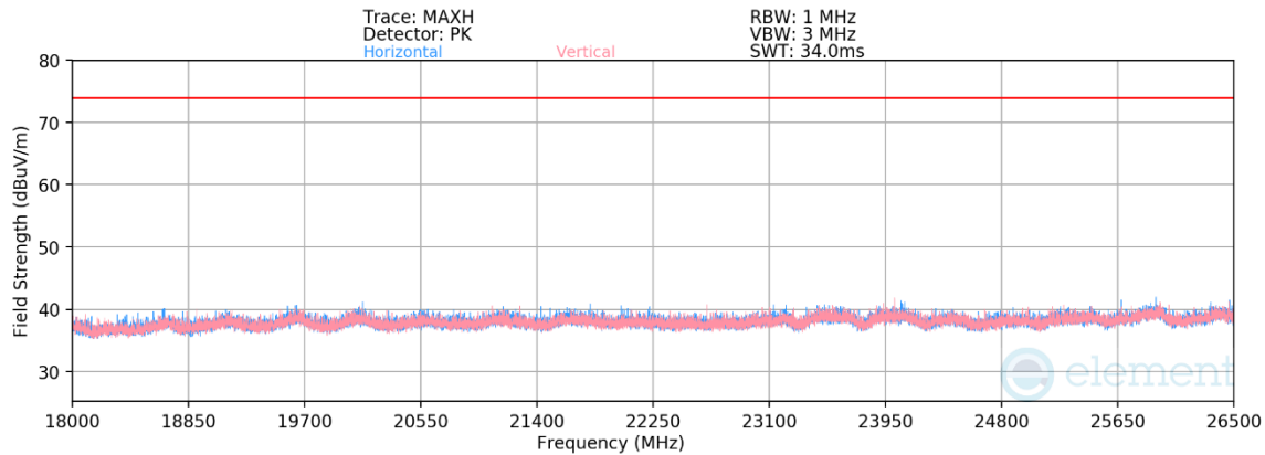
Plot 7-95. Radiated Spurious Emissions above 18GHz CDD (802.11be OFDMA – RU242 – Ch. 6)
