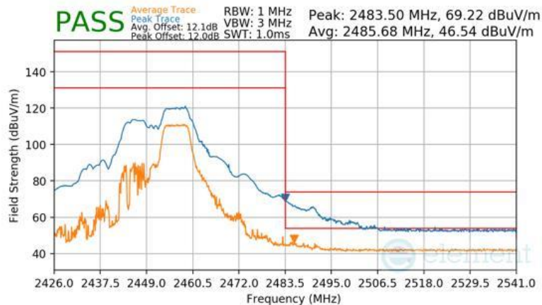
Plot 7-105 Radiated Restricted Upper Band Edge Measurement Antenna WF8 (Peak & Average – RU52+26)
