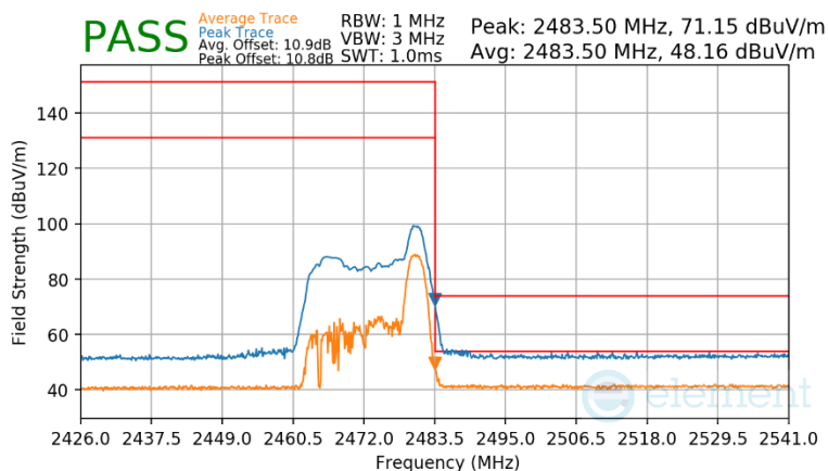
Plot 7-99 Radiated Restricted Upper Band Edge Measurement Antenna WF8 (Peak & Average – RU26)
