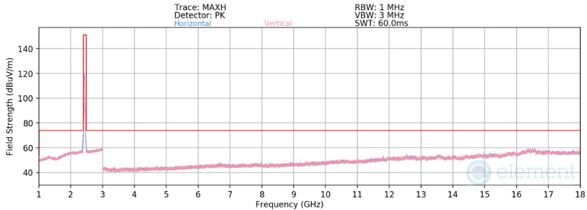
Plot 7-94. Radiated Spurious Emissions above 1GHz CDD (802.11be OFDMA – RU242 – Ch. 6)
