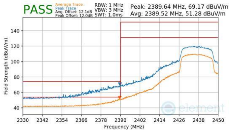
Plot 7-119 Radiated Restricted Lower Band Edge Measurement Antenna WF8 (Peak & Average – RU242)
