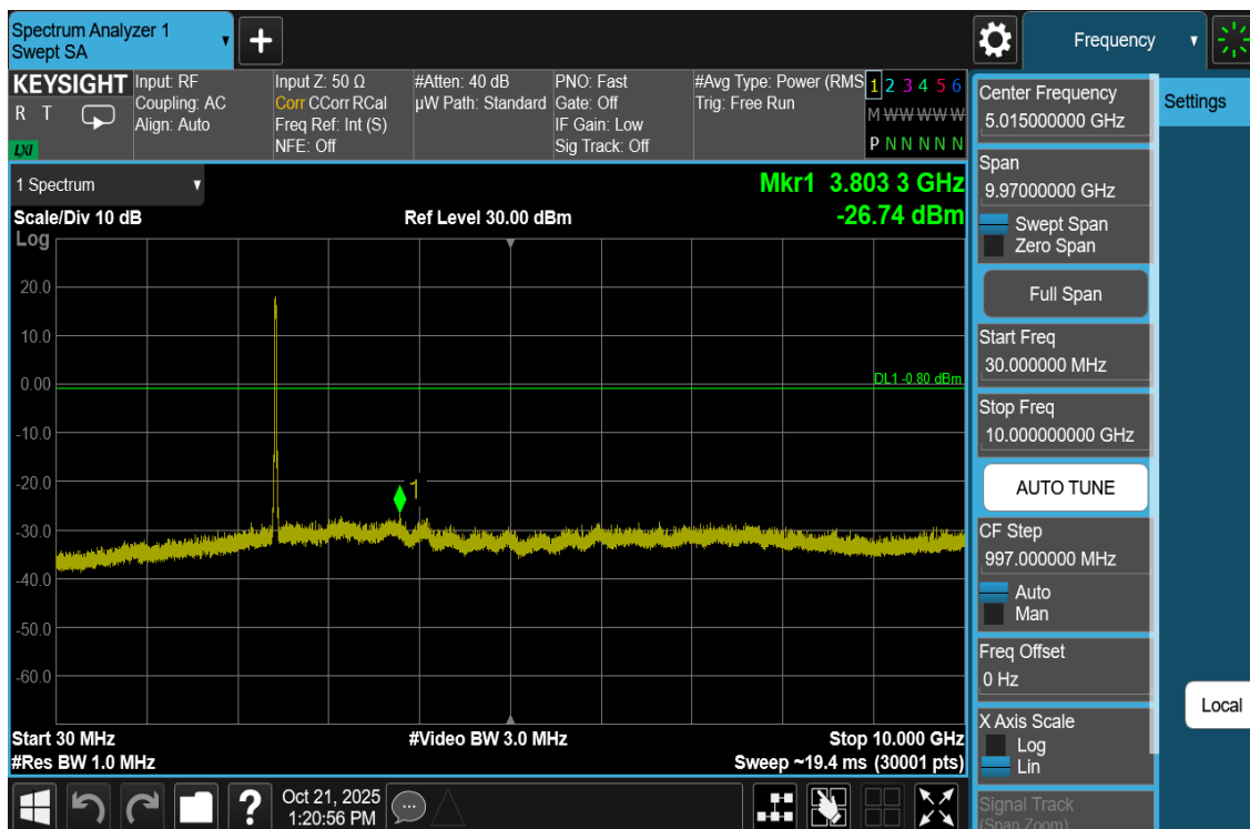
Plot 7-73. Conducted Spurious Plot Antenna WF8 (802.11be OFDMA – RU242 – Ch. 6)
