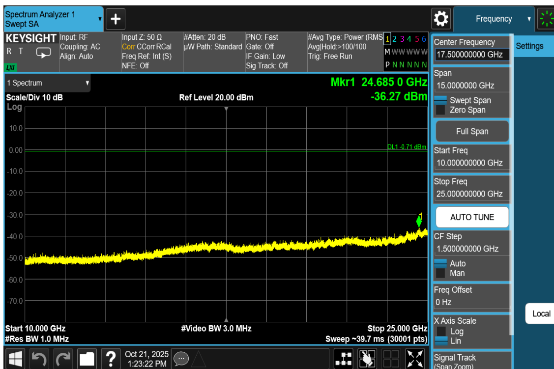
Plot 7-76. Conducted Spurious Plot Antenna WF8 (802.11be OFDMA – RU242 – Ch. 11)
