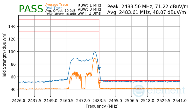
Plot 7-130 Radiated Restricted Upper Band Edge Measurement Antenna WF7b (Peak & Average – RU26)
