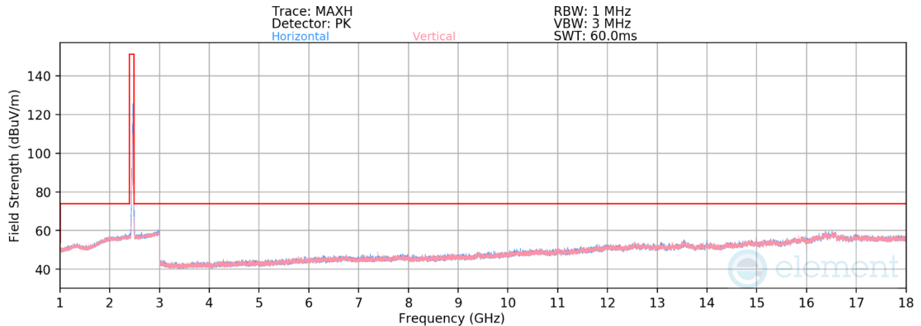
Plot 7-92. Radiated Spurious Emissions above 1GHz CDD (802.11be OFDMA – RU26 – Ch. 11)
