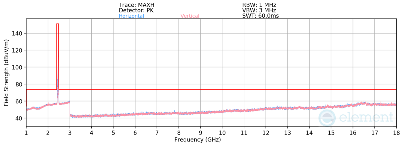
Plot 7-96. Radiated Spurious Emissions above 1GHz CDD (802.11be OFDMA – RU242 – Ch. 11)
