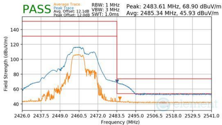
Plot 7-108 Radiated Restricted Upper Band Edge Measurement Antenna WF8 (Peak & Average – RU52+26)
