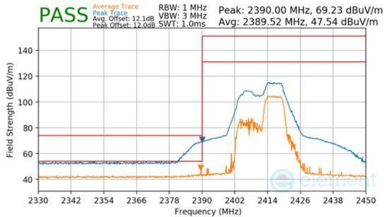
Plot 7-101 Radiated Restricted Lower Band Edge Measurement Antenna WF8 (Peak & Average – RU52+26)
