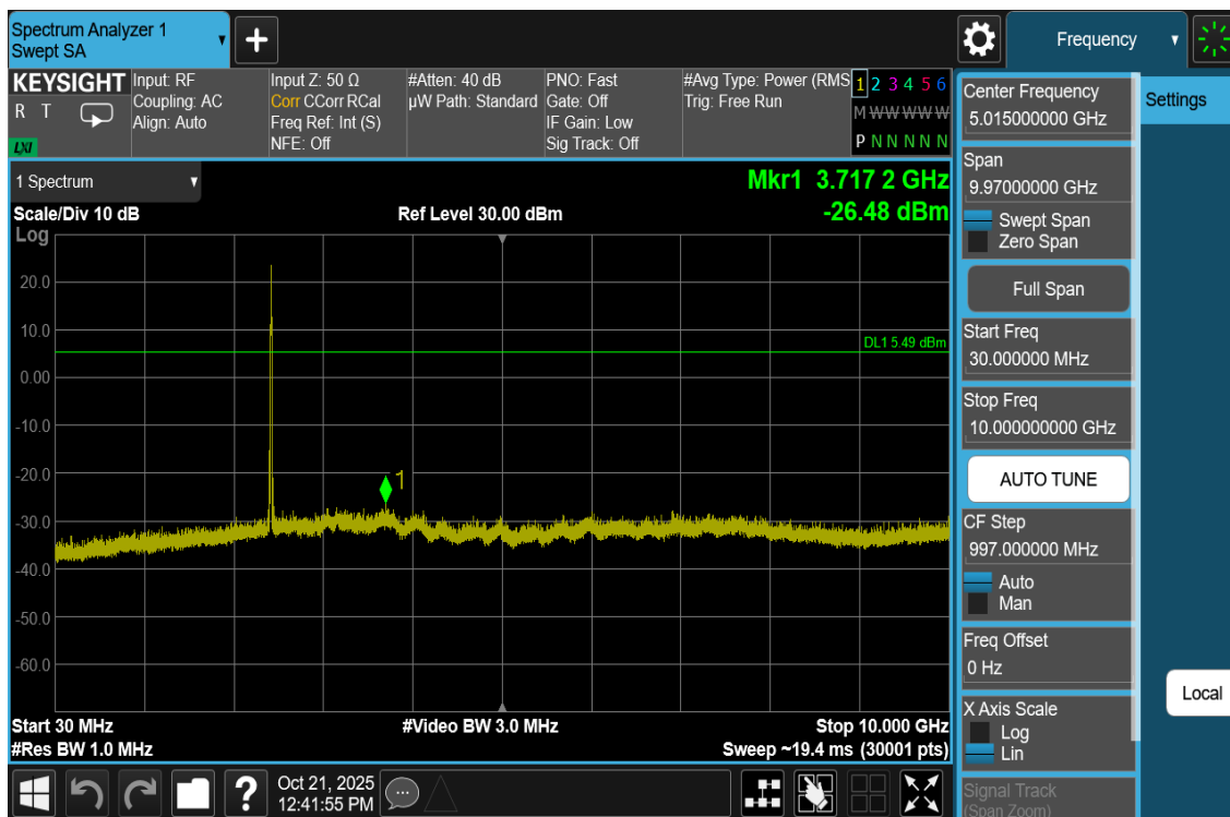
Plot 7-67. Conducted Spurious Plot Antenna WF8 (802.11be OFDMA – RU26 – Ch. 6)
