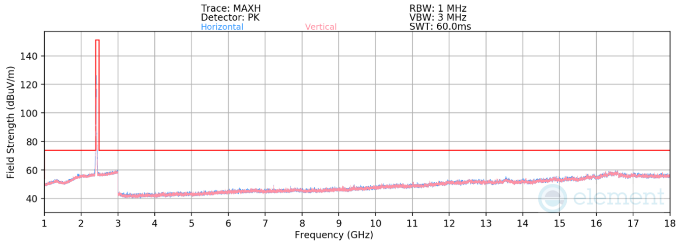
Plot 7-89. Radiated Spurious Emissions above 1GHz CDD (802.11be OFDMA – RU26 – Ch. 1)
