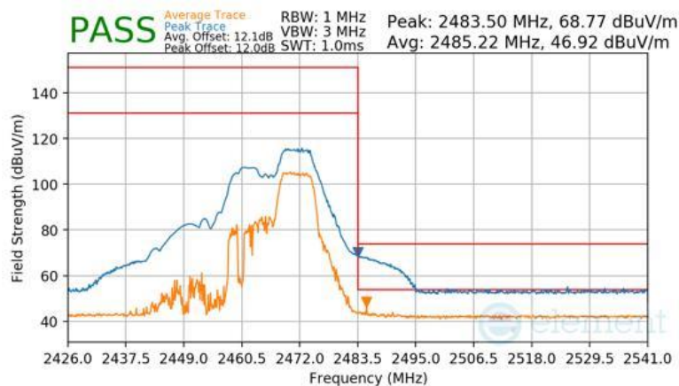
Plot 7-111 Radiated Restricted Upper Band Edge Measurement Antenna WF8 (Peak & Average – RU52+26)
