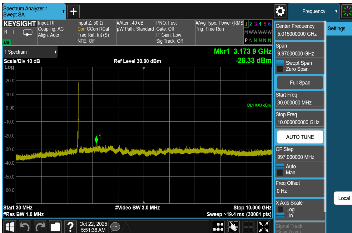
Plot 7-87. Conducted Spurious Plot Antenna WF7b (802.11be OFDMA – RU242 – Ch. 11)
