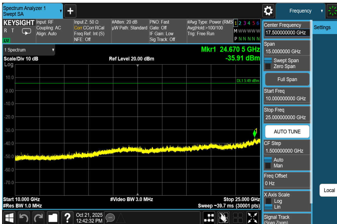
Plot 7-68. Conducted Spurious Plot Antenna WF8 (802.11be OFDMA – RU26 – Ch. 6)
