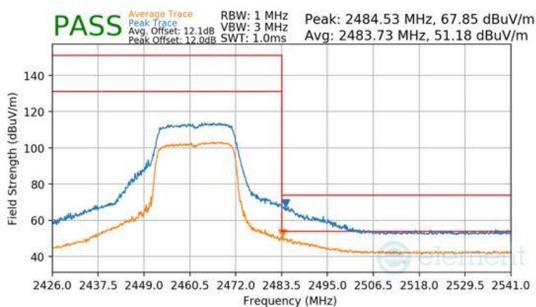
Plot 7-125 Radiated Restricted Upper Band Edge Measurement Antenna WF8 (Peak & Average – RU242)
