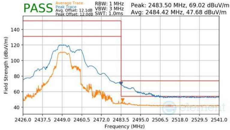
Plot 7-104 Radiated Restricted Upper Band Edge Measurement Antenna WF8 (Peak & Average – RU52+26)
