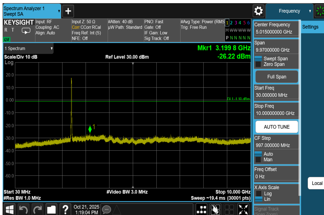
Plot 7-71. Conducted Spurious Plot Antenna WF8 (802.11be OFDMA – RU242 – Ch. 1)
