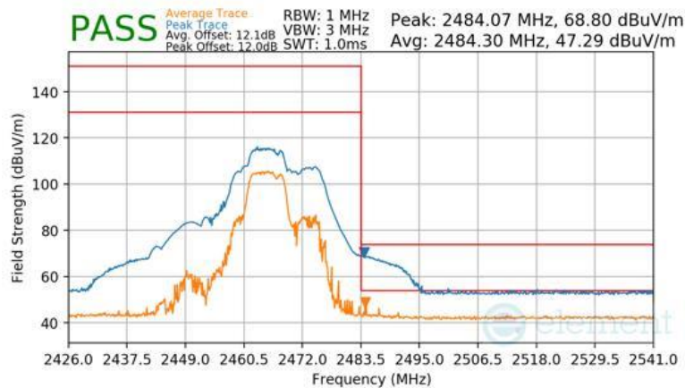
Plot 7-110 Radiated Restricted Upper Band Edge Measurement Antenna WF8 (Peak & Average – RU52+26)
