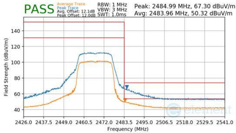
Plot 7-126 Radiated Restricted Upper Band Edge Measurement Antenna WF8 (Peak & Average – RU242)
