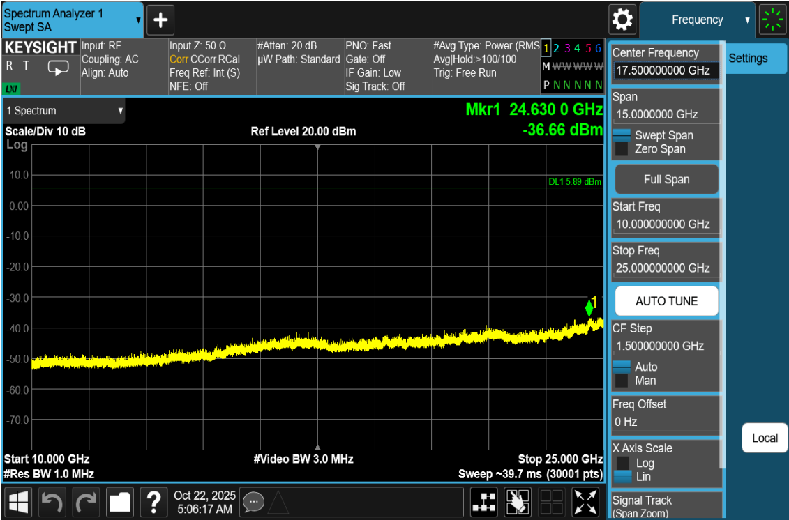
Plot 7-78. Conducted Spurious Plot Antenna WF7b (802.11be OFDMA – RU26 – Ch. 1)
