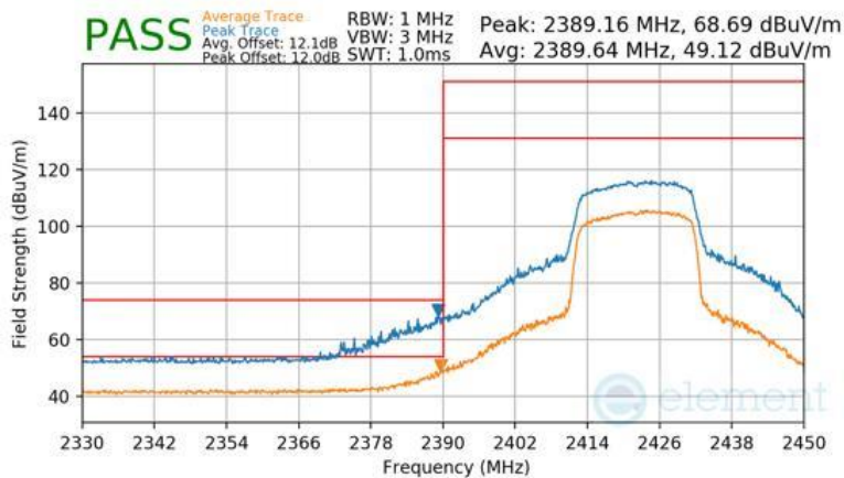
Plot 7-116 Radiated Restricted Lower Band Edge Measurement Antenna WF8 (Peak & Average – RU242)
