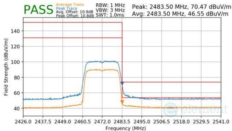
Plot 7-127 Radiated Restricted Upper Band Edge Measurement Antenna WF8 (Peak & Average – RU242)
