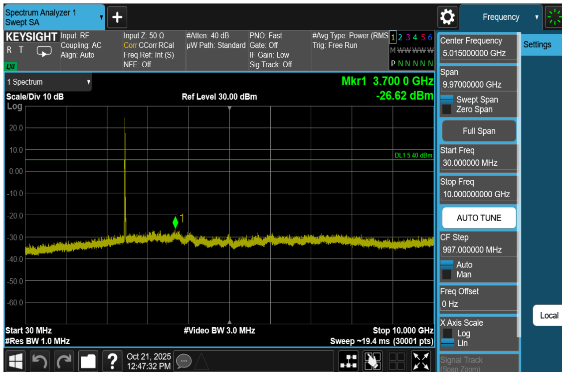
Plot 7-69. Conducted Spurious Plot Antenna WF8 (802.11be OFDMA – RU26 – Ch. 11)
