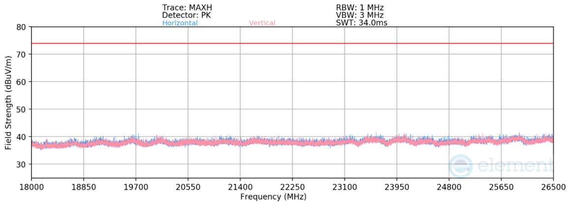
Plot 7-91. Radiated Spurious Emissions above 18GHz CDD (802.11be OFDMA – RU26 – Ch. 6)
