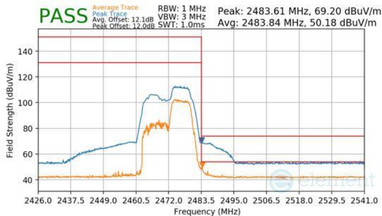
Plot 7-113 Radiated Restricted Upper Band Edge Measurement Antenna WF8 (Peak & Average – RU52+26)
