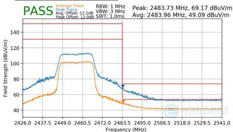
Plot 7-124 Radiated Restricted Upper Band Edge Measurement Antenna WF8 (Peak & Average – RU242)
