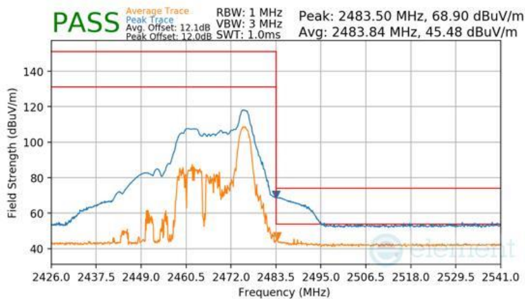
Plot 7-98 Radiated Restricted Upper Band Edge Measurement Antenna WF8 (Peak & Average – RU26)
