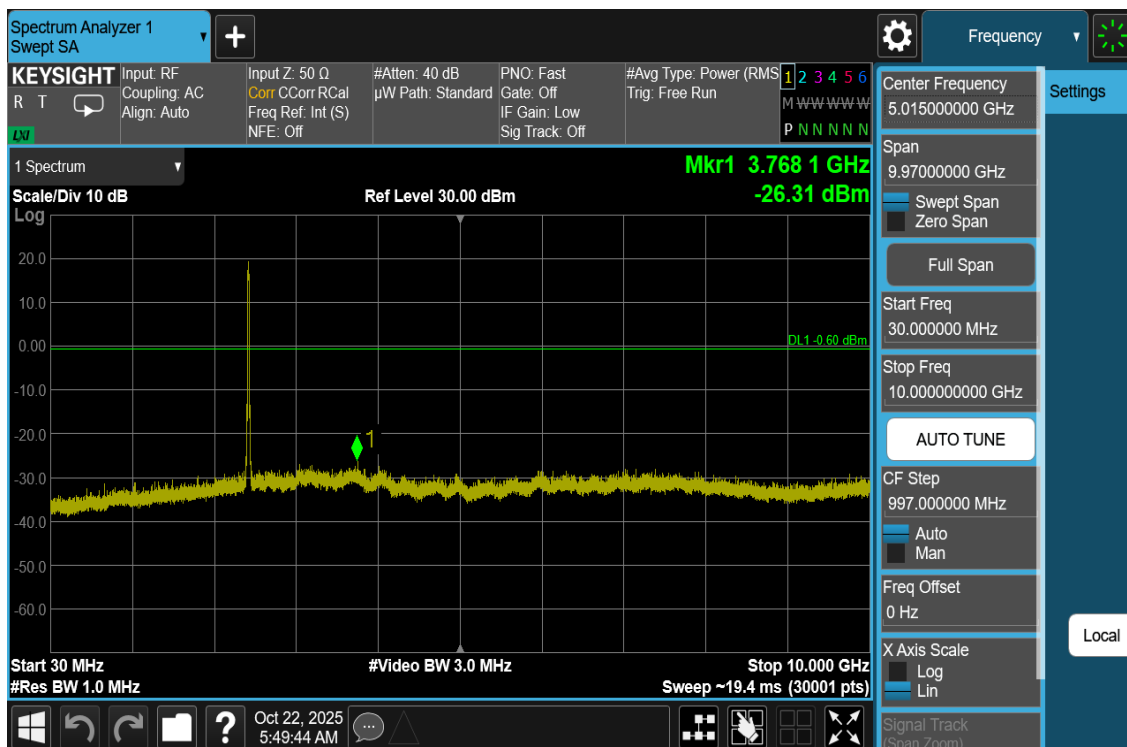
Plot 7-85. Conducted Spurious Plot Antenna WF7b (802.11be OFDMA – RU242 – Ch. 6)
