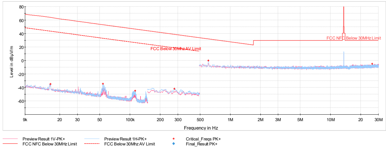
Plot 7-2. Radiated Spurious Plot 9kHz – 30MHz (Charging Rate 2.6C, with Laptop)
