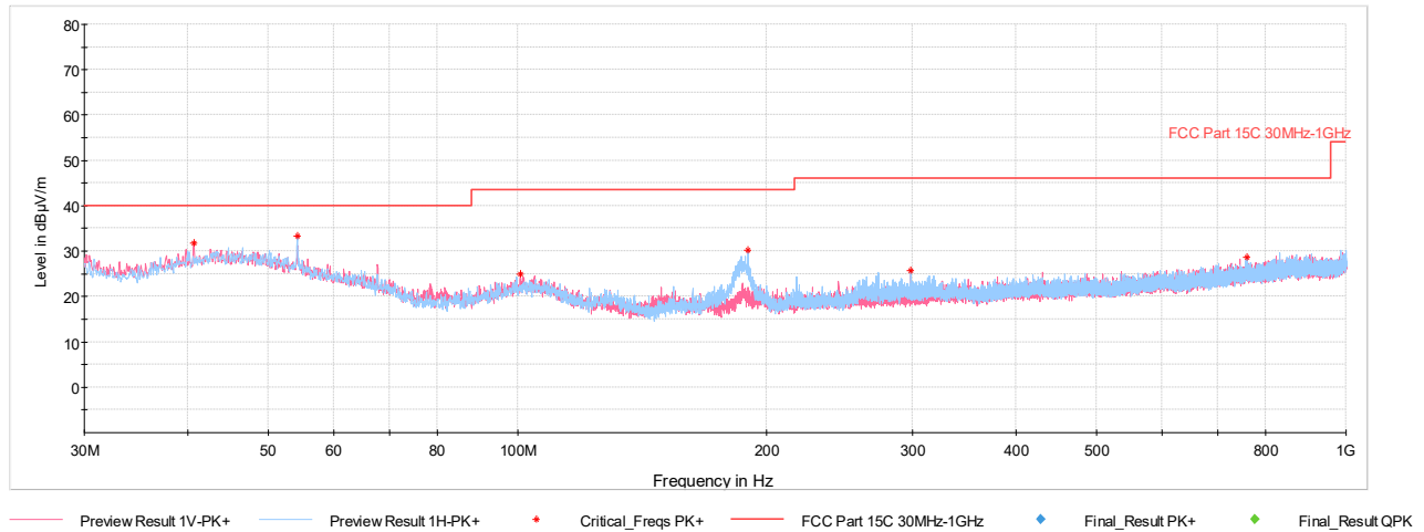
Plot 7-3. Radiated Spurious Emissions 30MHz – 1GHz (Charging Rate 2.6C, with Laptop)
