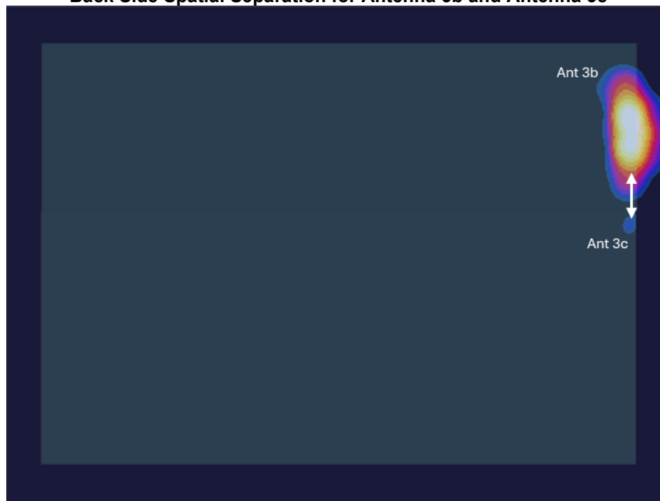
Figure F-19 Back Side Spatial Separation for Antenna 3b and Antenna 3c
