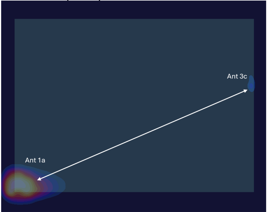
Figure F-5 Back Side Spatial Separation for Antenna 1a and Antenna 3c
