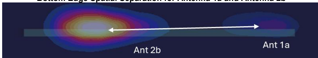
Figure F-36 Bottom Edge Spatial Separation for Antenna 1a and Antenna 2b
