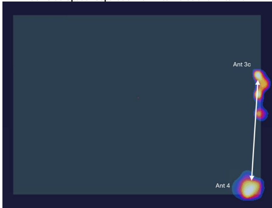
Figure F-20 Back Side Spatial Separation for Antenna 3c and Antenna 4
