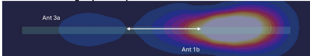
Figure F-40 Bottom Edge Spatial Separation for Antenna 1b and Antenna 3a
