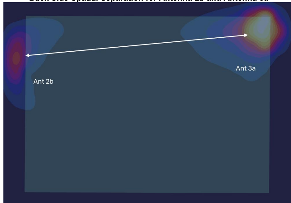
Figure F-15 Back Side Spatial Separation for Antenna 2b and Antenna 3a
