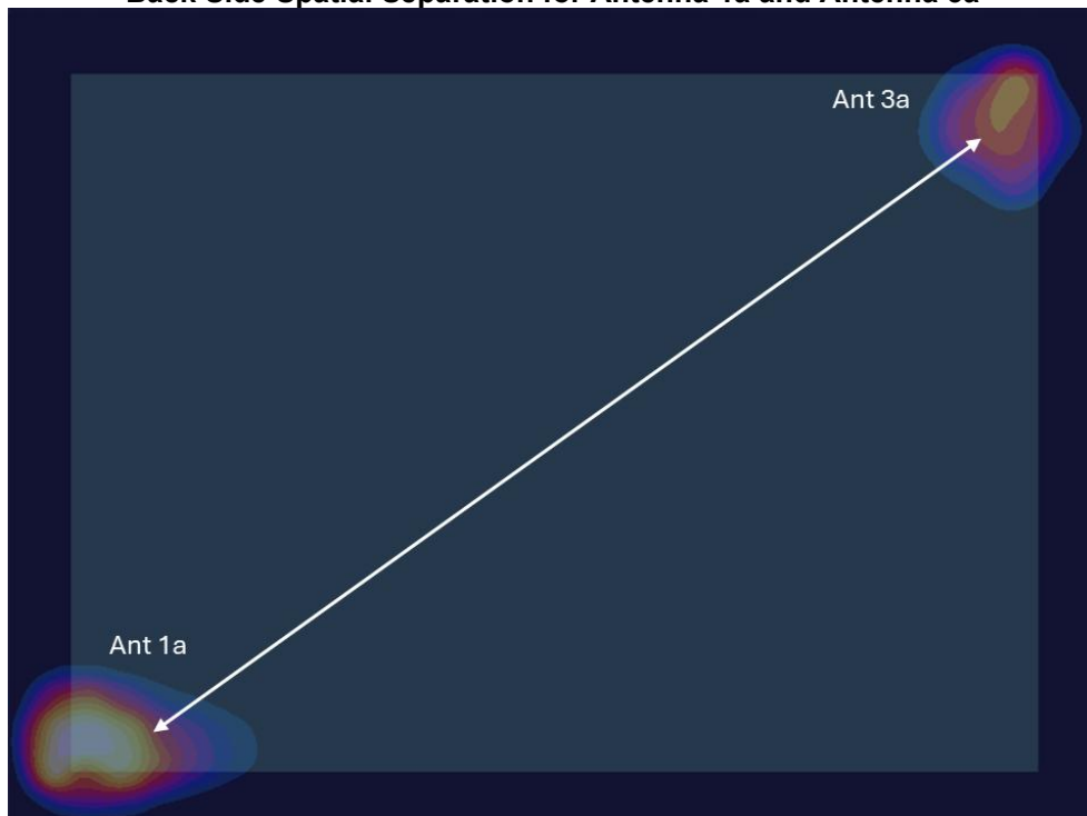
Figure F-3 Back Side Spatial Separation for Antenna 1a and Antenna 3a
