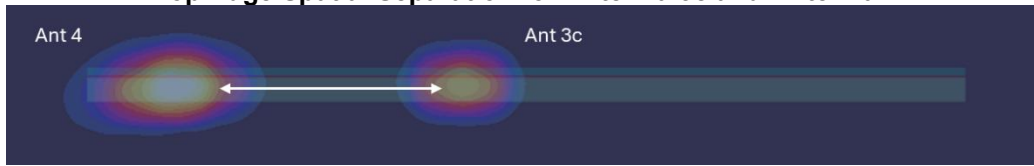
Figure F-34 Top Edge Spatial Separation for Antenna 3c and Antenna 4
