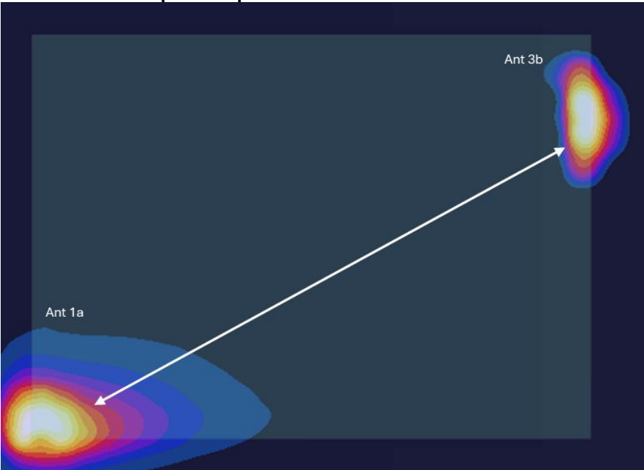
Figure F-4 Back Side Spatial Separation for Antenna 1a and Antenna 3b
