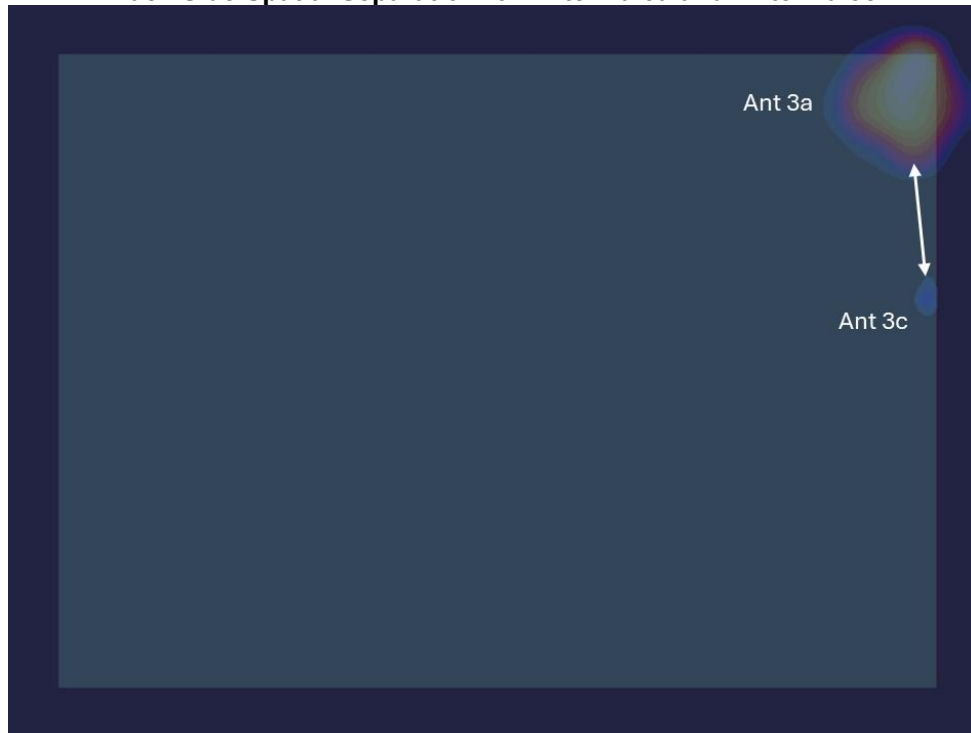
Figure F-17 Back Side Spatial Separation for Antenna 3a and Antenna 3c
