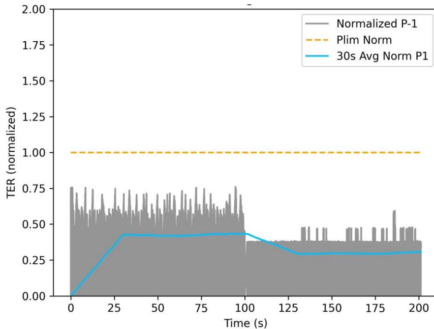
Figure 6-3 Device State Switch Normalized Time-averaged conducted TX power
