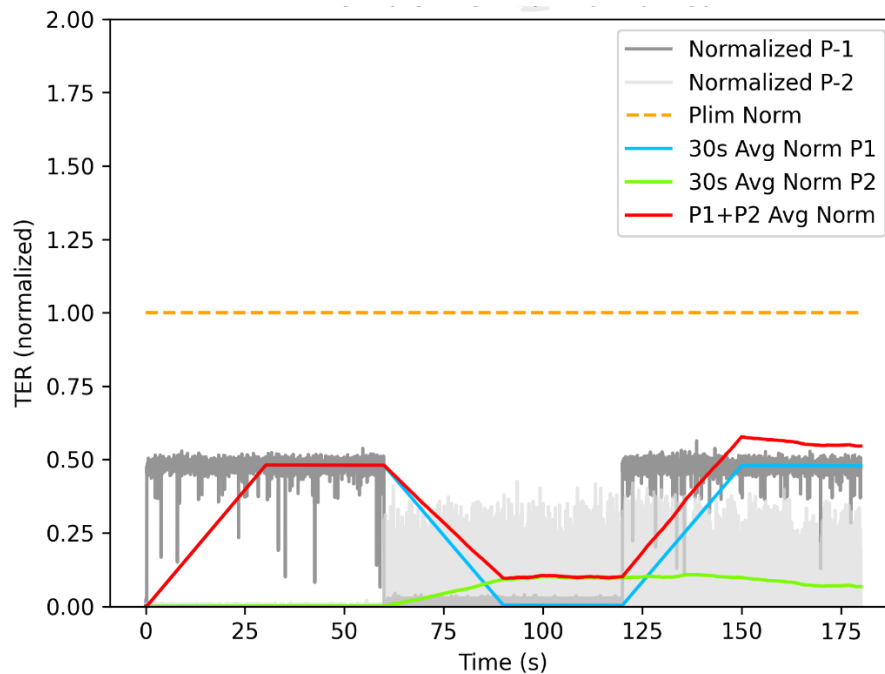
Figure 6-1 Technology Switch Normalized Time-averaged conducted TX power
