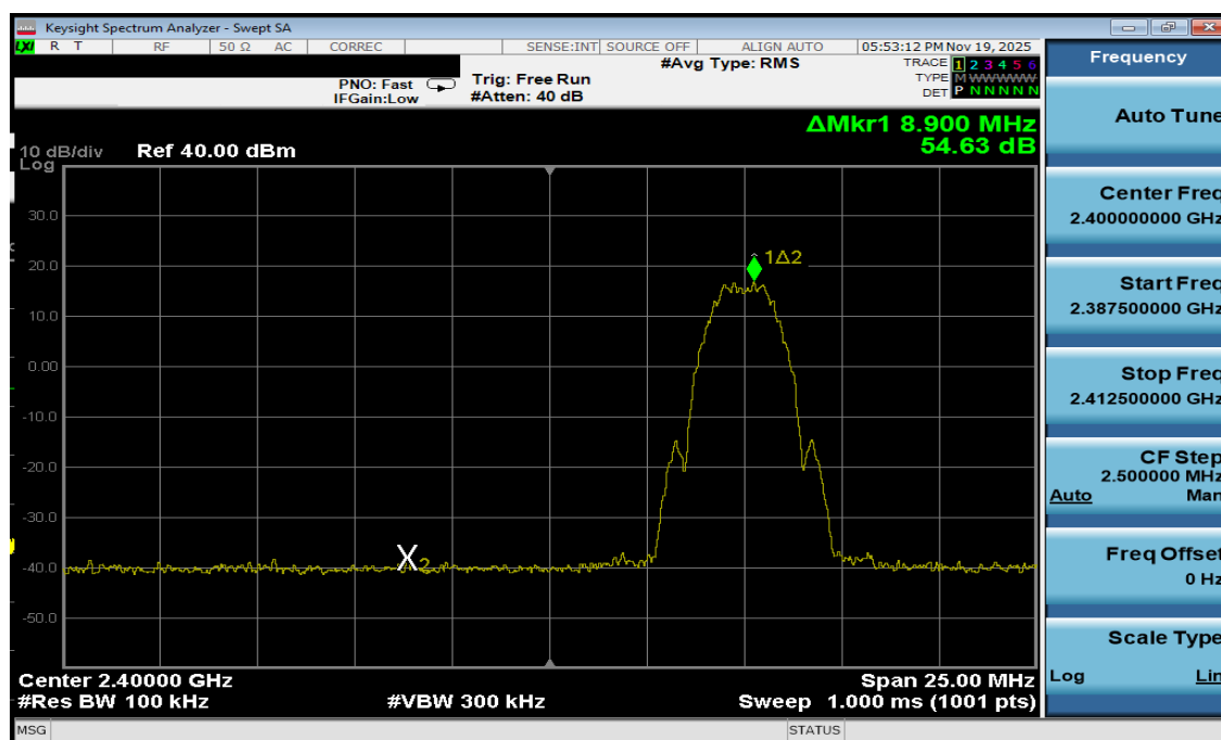
Plot 7-25. Band Edge Antenna 3a (802.15.4, ePA – Ch. 11)
