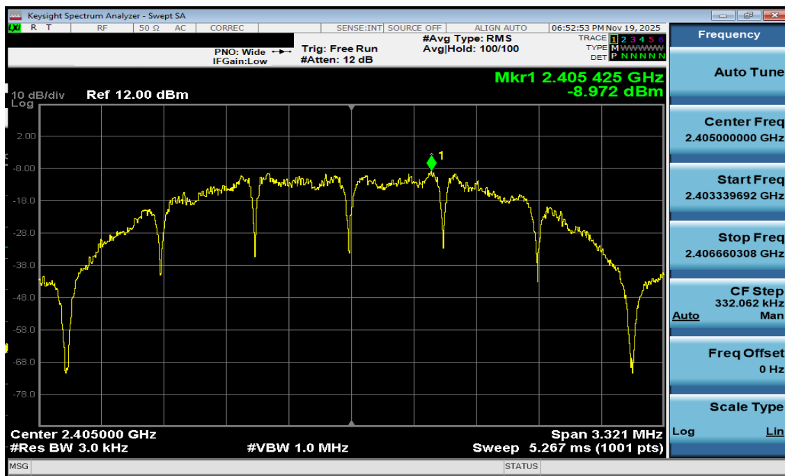
Plot 7-22. Power Spectral Density Antenna 1a (802.15.4, iPA – Ch. 11)
