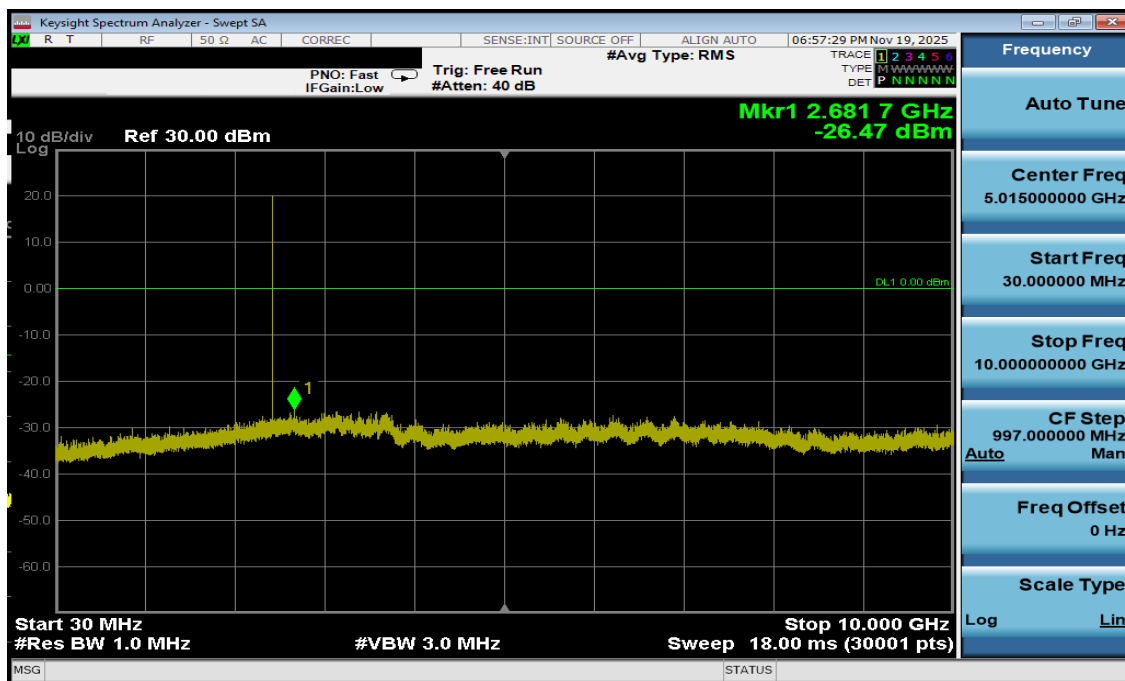
Plot 7-37. Conducted Spurious Antenna 1a (802.15.4, ePA – Ch. 18)
