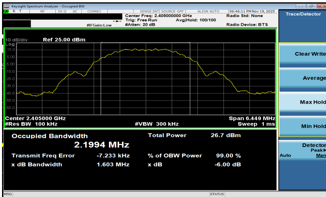
Plot 7-10. 6dB BW Antenna 1a (802.15.4, Ch. 11)
