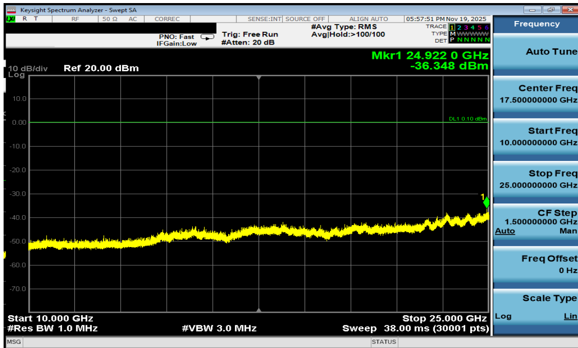
Plot 7-34. Conducted Spurious Antenna 3a (802.15.4, ePA – Ch. 25)
