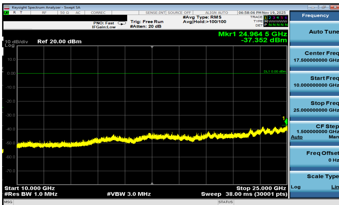
Plot 7-38. Conducted Spurious Antenna 1a (802.15.4, ePA – Ch. 18)
