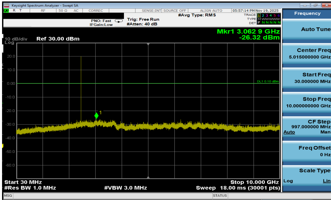
Plot 7-33. Conducted Spurious Antenna 3a (802.15.4, ePA – Ch. 25)
