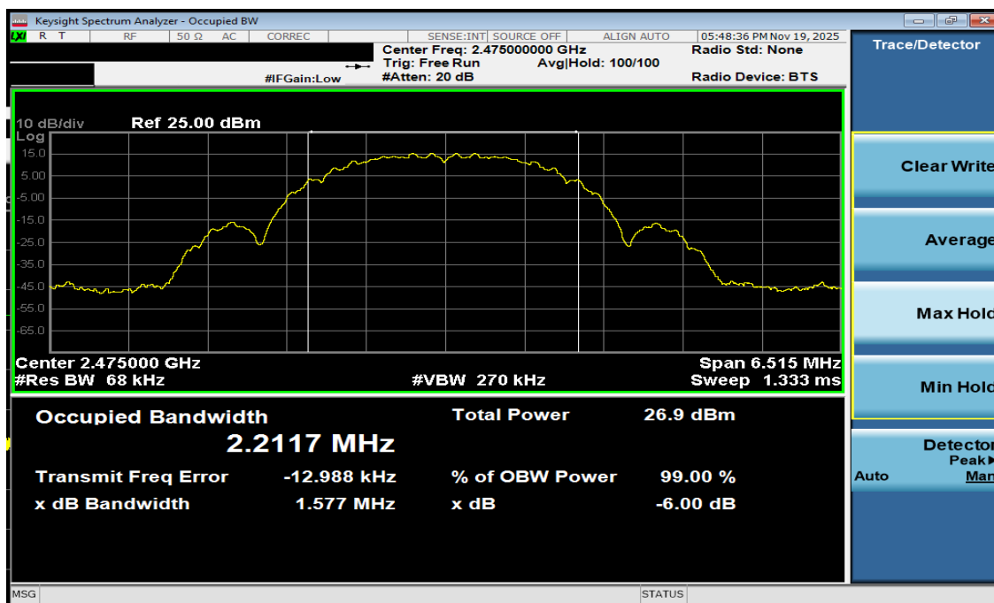
Plot 7-3. 99% OBW Antenna 3a (802.15.4, Ch. 25)
