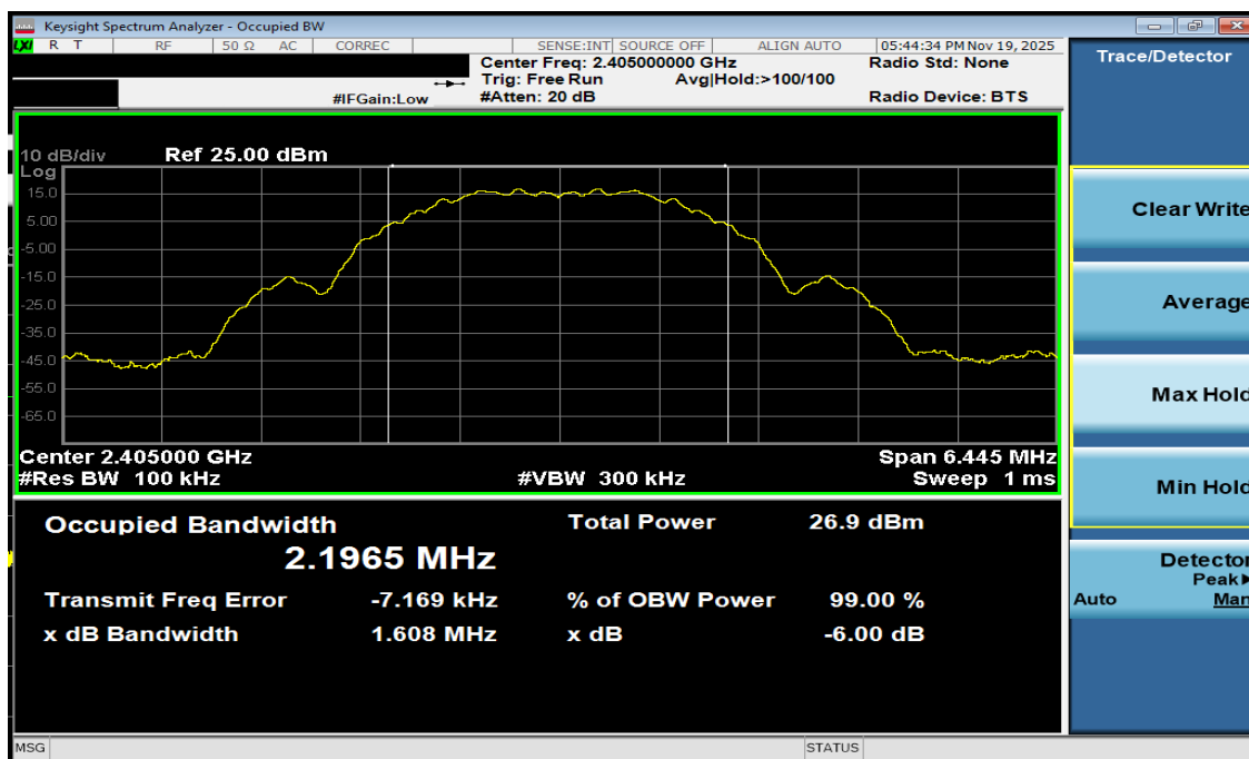
Plot 7-7. 6dB BW Antenna 3a (802.15.4, Ch. 11)
