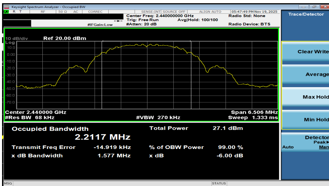
Plot 7-2. 99% OBW Antenna 3a (802.15.4, Ch. 18)
