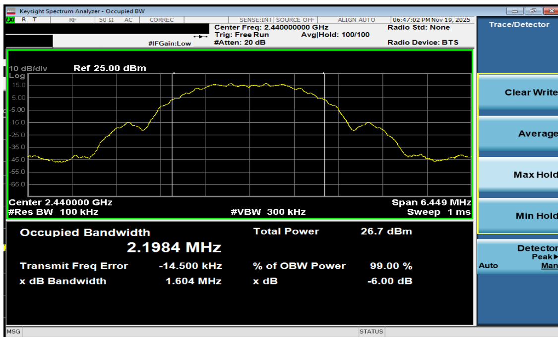
Plot 7-11. 6dB BW Antenna 1a (802.15.4, Ch. 18)
