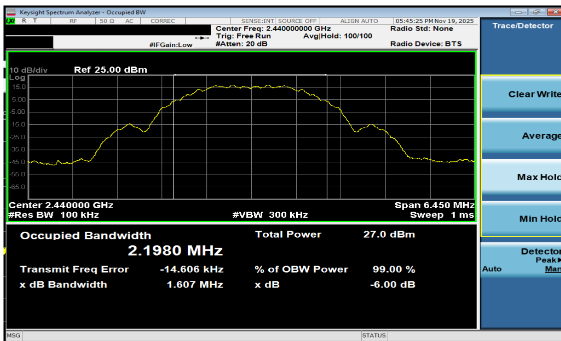
Plot 7-8. 6dB BW Antenna 3a (802.15.4, Ch. 18)
