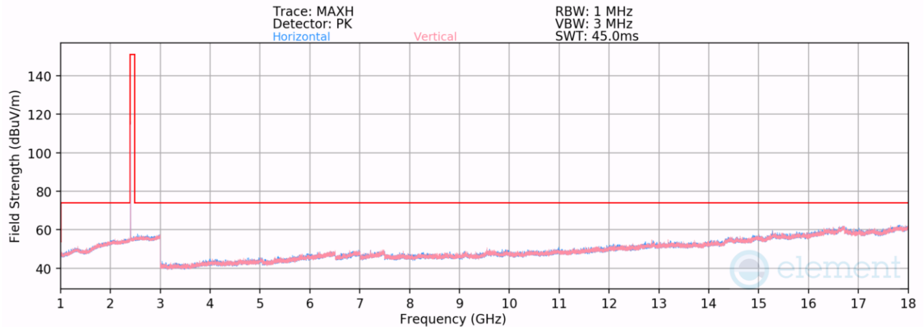
Plot 7-41. Radiated Spurious Emissions 1-18GHz Antenna 3a (802.15.4 ePA – Ch. 11)
