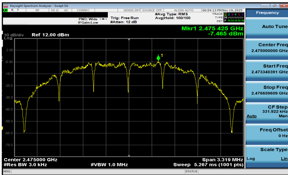
Plot 7-24. Power Spectral Density Antenna 1a (802.15.4, iPA – Ch. 25)
