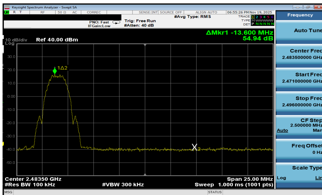
Plot 7-28. Band Edge Antenna 1a (802.15.4, ePA – Ch. 25)
