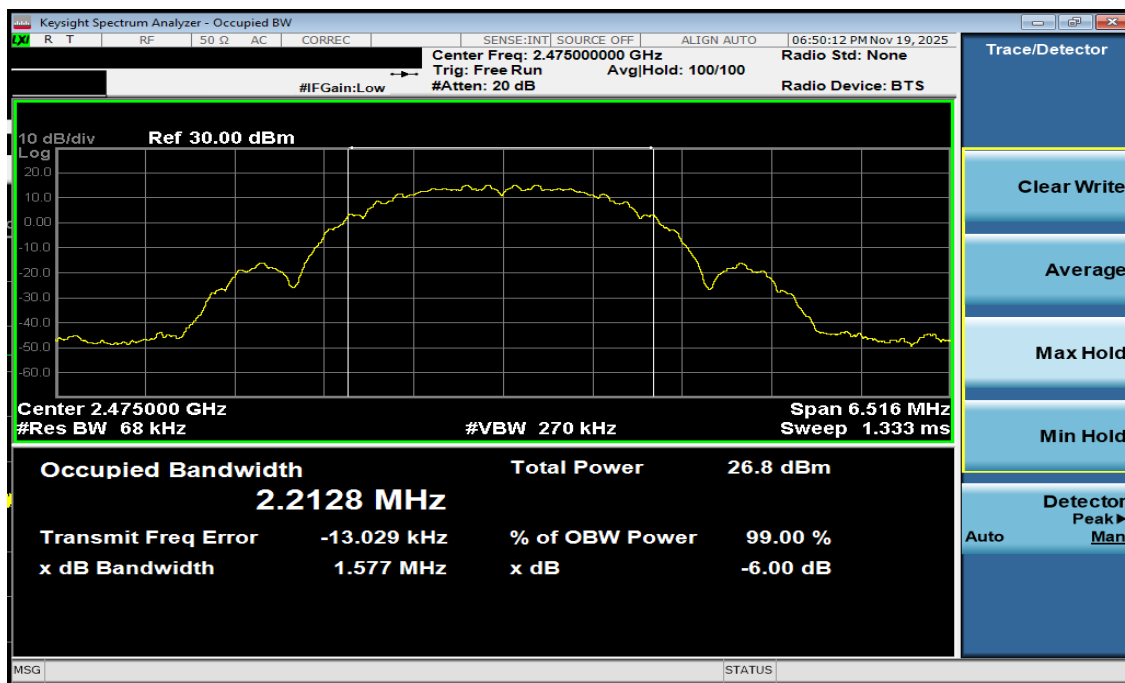
Plot 7-6. 99% OBW Antenna 1a(802.15.4, Ch. 25)
