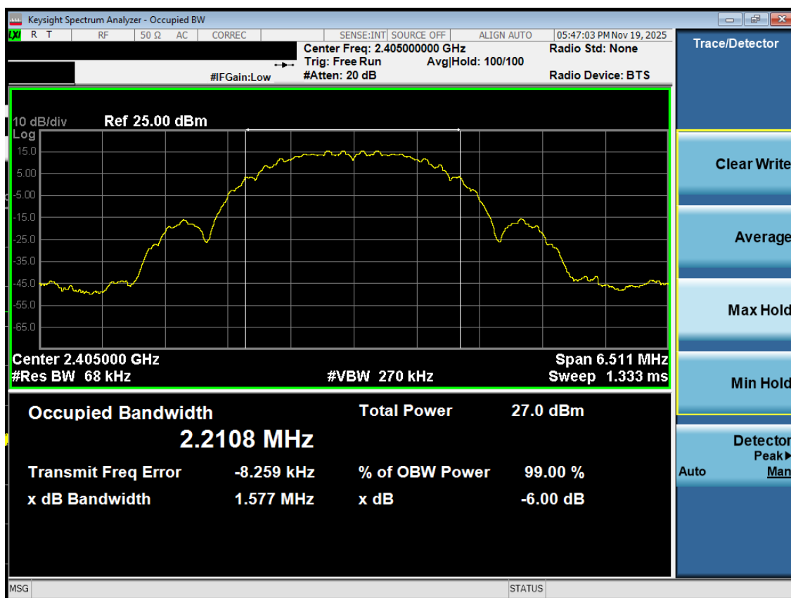
Plot 7-1. 99% OBW Antenna 3a (802.15.4, Ch. 11)
