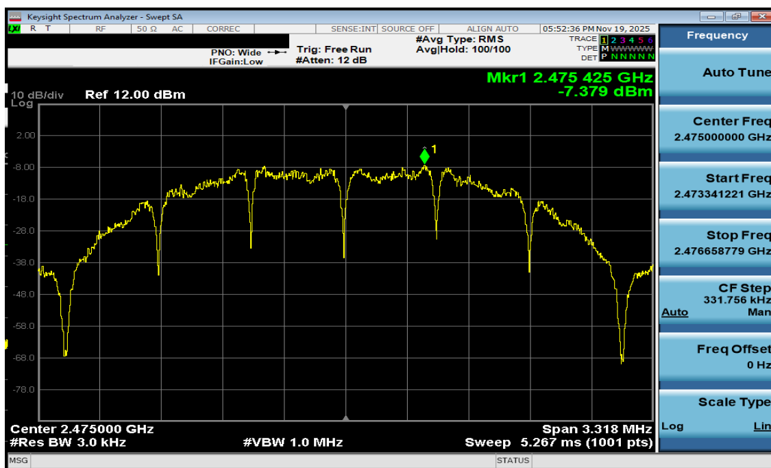
Plot 7-18. Power Spectral Density Antenna 3a (802.15.4, iPA – Ch. 25)
