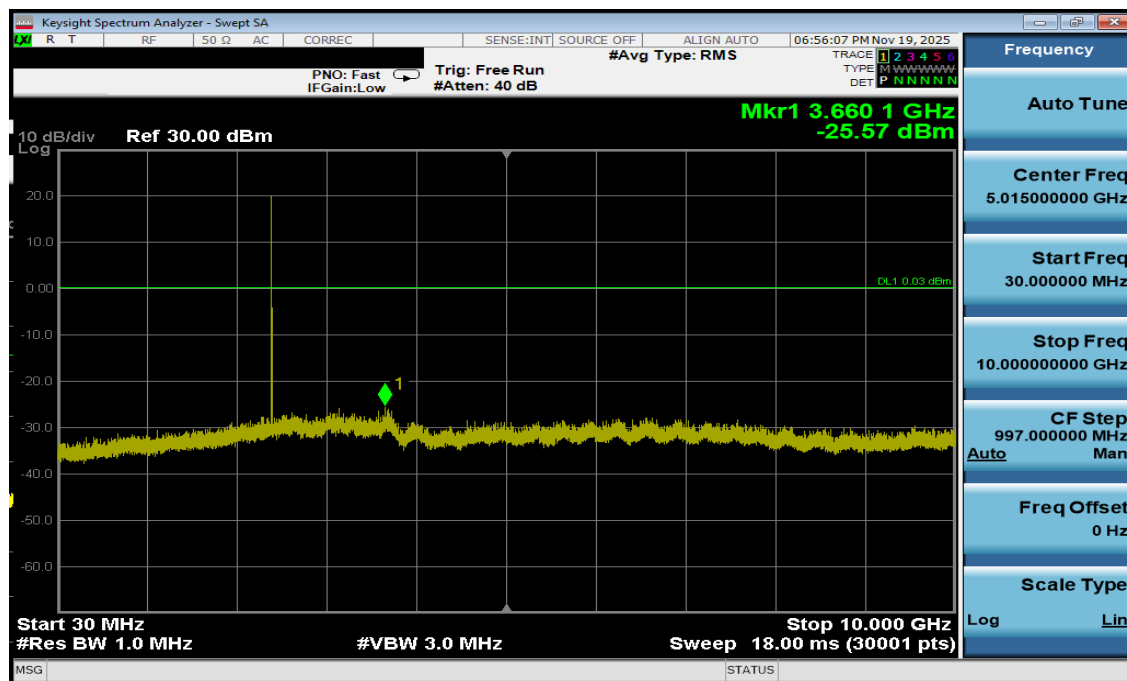
Plot 7-35. Conducted Spurious Antenna 1a (802.15.4, ePA – Ch. 11)
