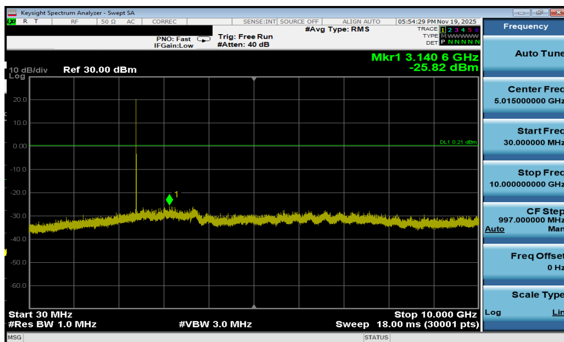
Plot 7-29. Conducted Spurious Antenna 3a (802.15.4, ePA – Ch. 11)
