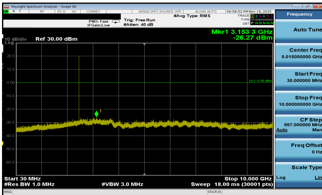
Plot 7-39. Conducted Spurious Antenna 1a (802.15.4, ePA – Ch. 25)
