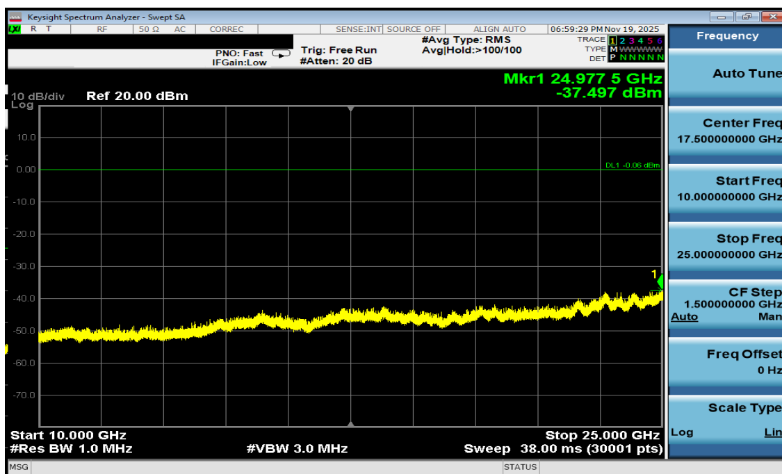
Plot 7-40. Conducted Spurious Antenna 1a (802.15.4, ePA – Ch. 25)
