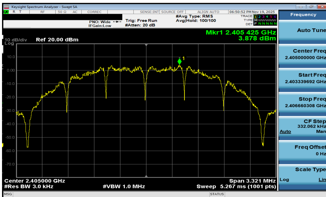
Plot 7-19. Power Spectral Density Antenna 1a (802.15.4, ePA - Ch. 11)
