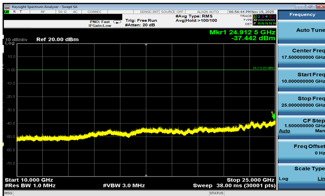
Plot 7-36. Conducted Spurious Antenna 1a (802.15.4, ePA – Ch. 11)
