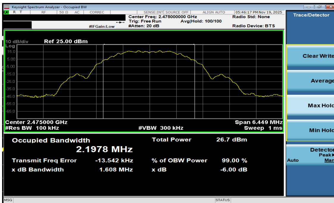
Plot 7-9. 6dB BW Antenna 3a (802.15.4, Ch. 25)
