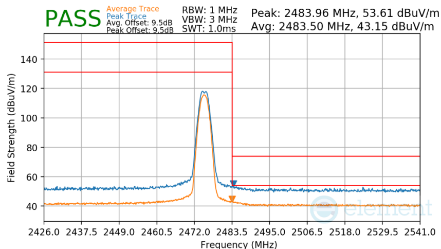
Plot 7-50. Radiated Restricted Upper Band Edge Measurement Antenna 3a
