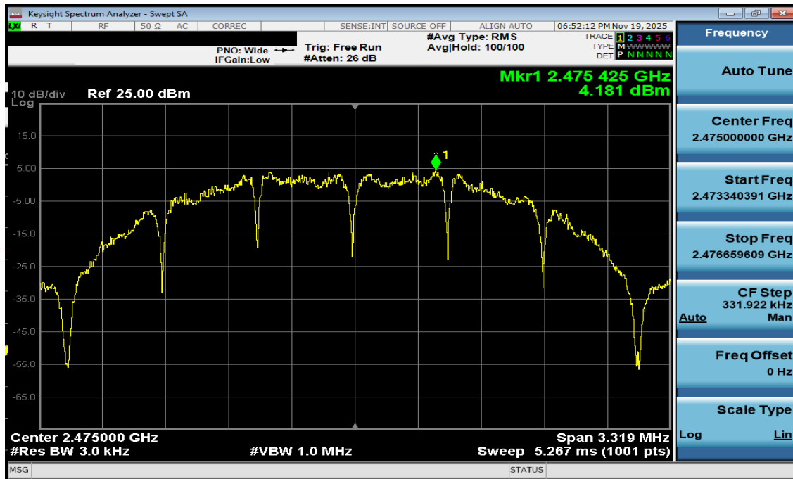
Plot 7-21. Power Spectral Density Antenna 1a (802.15.4, ePA – Ch. 25)
