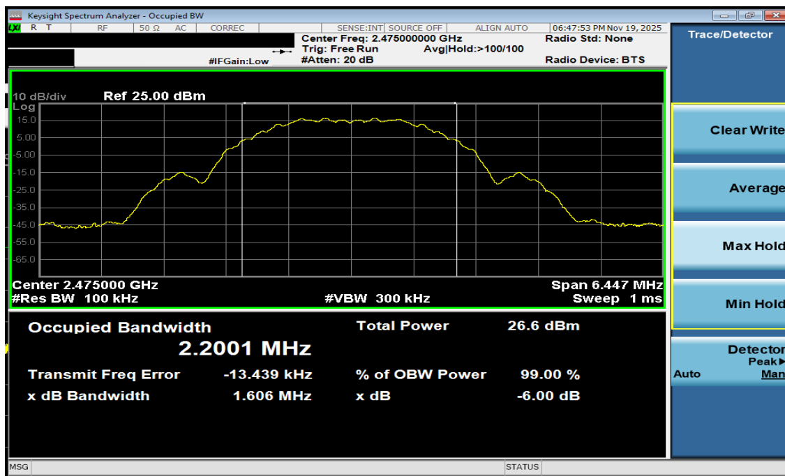
Plot 7-12. 6dB BW Antenna 1a(802.15.4, Ch. 25)
