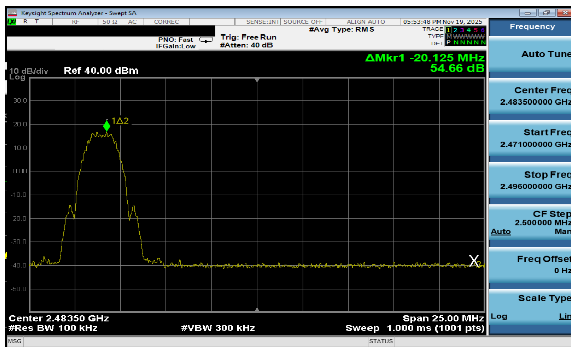
Plot 7-26. Band Edge Antenna 3a (802.15.4, ePA – Ch. 25)
