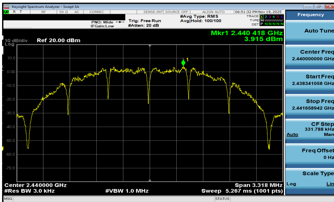
Plot 7-20. Power Spectral Density Antenna 1a (802.15.4, ePA - Ch. 18)
