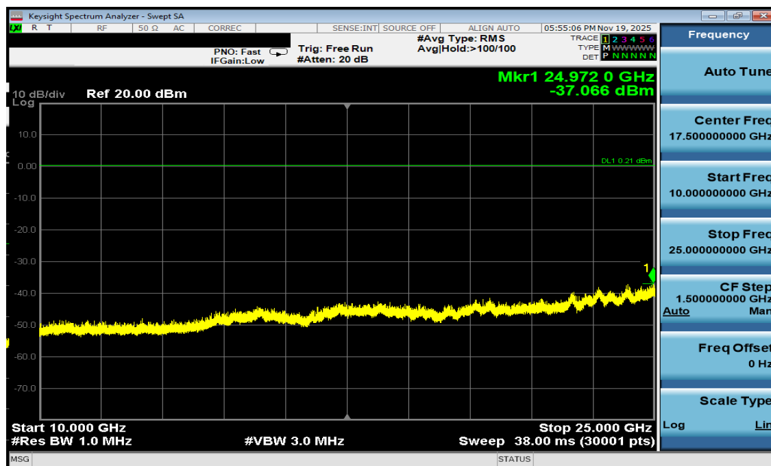
Plot 7-30. Conducted Spurious Antenna 3a (802.15.4, ePA – Ch. 11)
