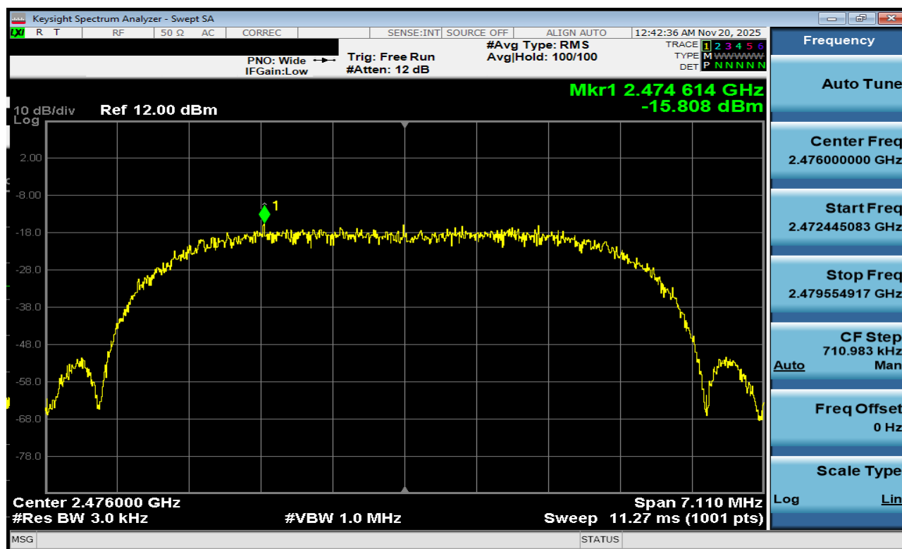
Plot 7-192. Power Spectral Density Plot Tx BF Antenna 1a (Bluetooth (XHDRPM6), 6Mbps, iPA – Ch. 73)
