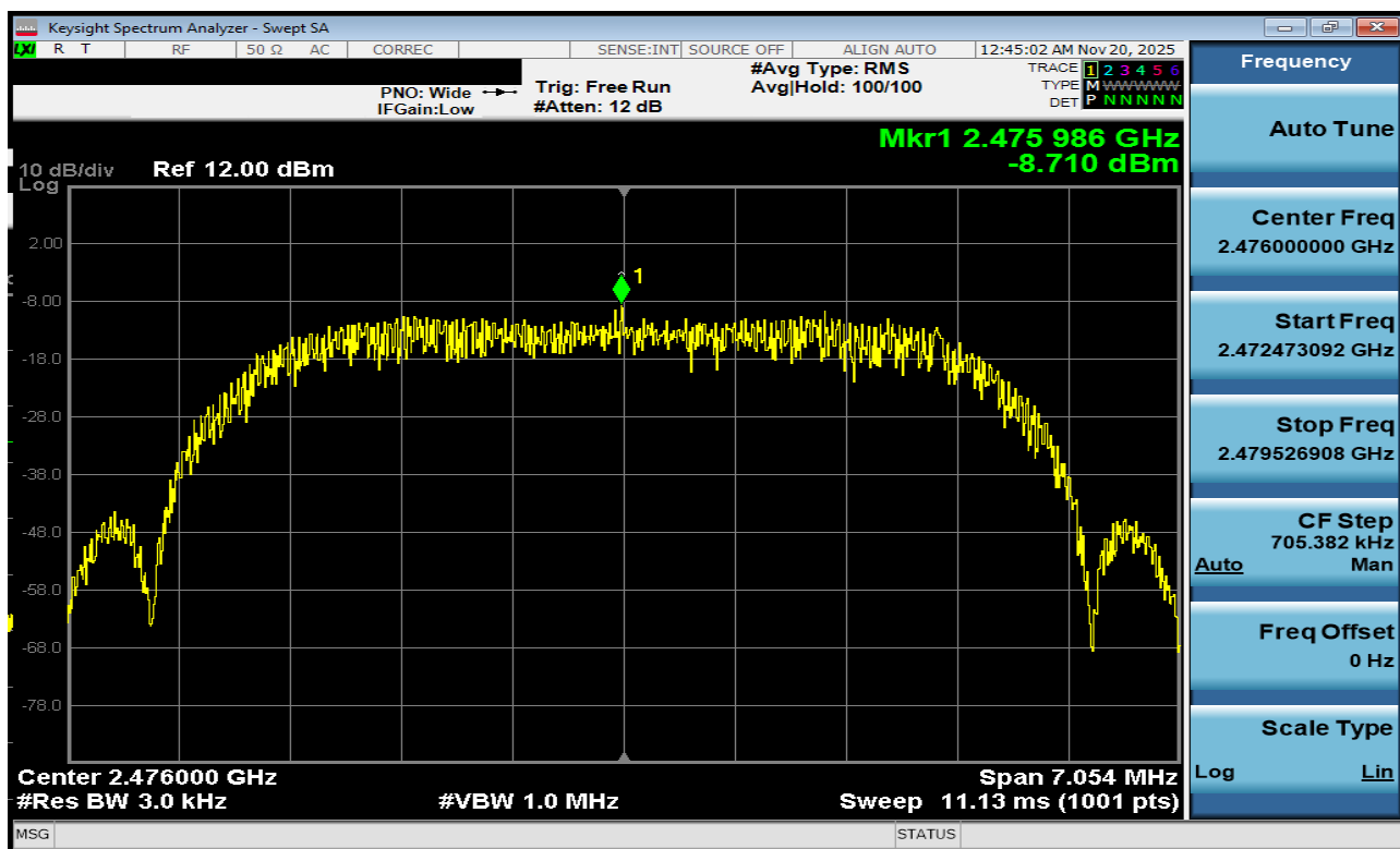
Plot 7-198. Power Spectral Density Plot Tx BF Antenna 1a (Bluetooth (HDRPM16), 16Mbps, ePA – Ch. 73)
