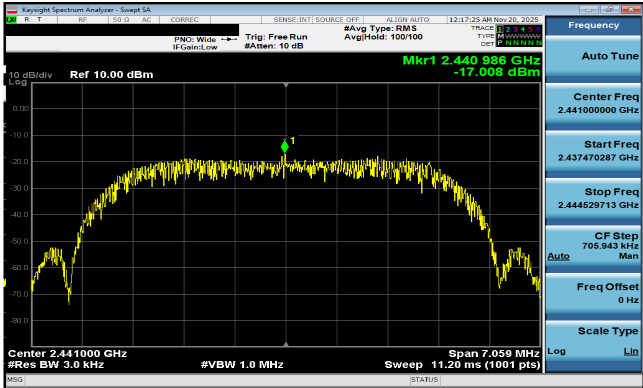
Plot 7-137. Power Spectral Density Plot Antenna 1a (Bluetooth (HDRPM16), 16Mbps, iPA – Ch. 38)
