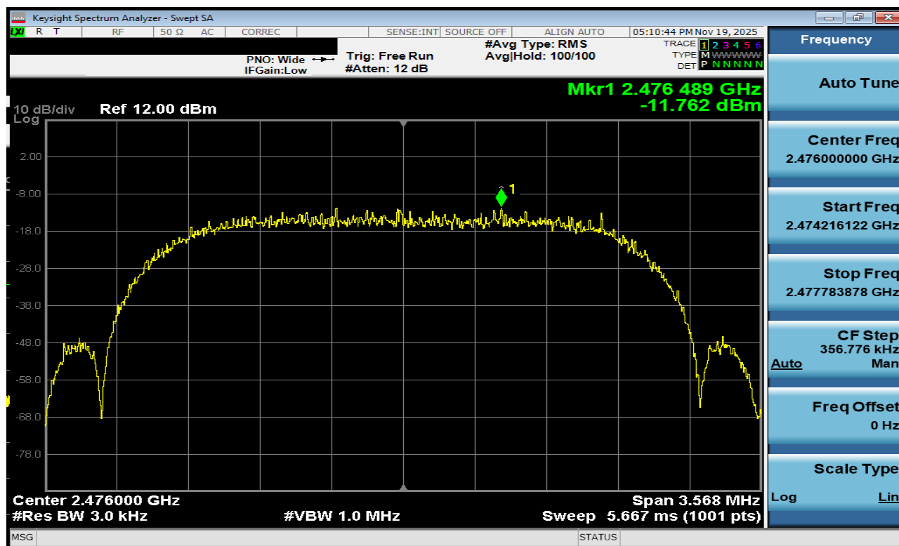
Plot 7-179. Power Spectral Density Plot TxBF Antenna 3a (Bluetooth (HDRPS2), 2Mbps, iPA – Ch. 73)
