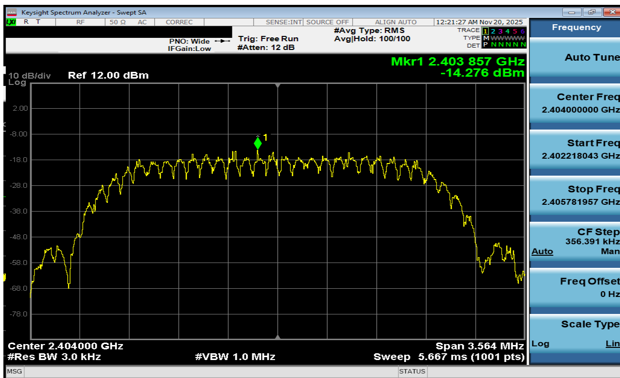
Plot 7-142. Power Spectral Density Plot Antenna 1a (Bluetooth (HDT2), 2Mbps, iPA – Ch. 1)
