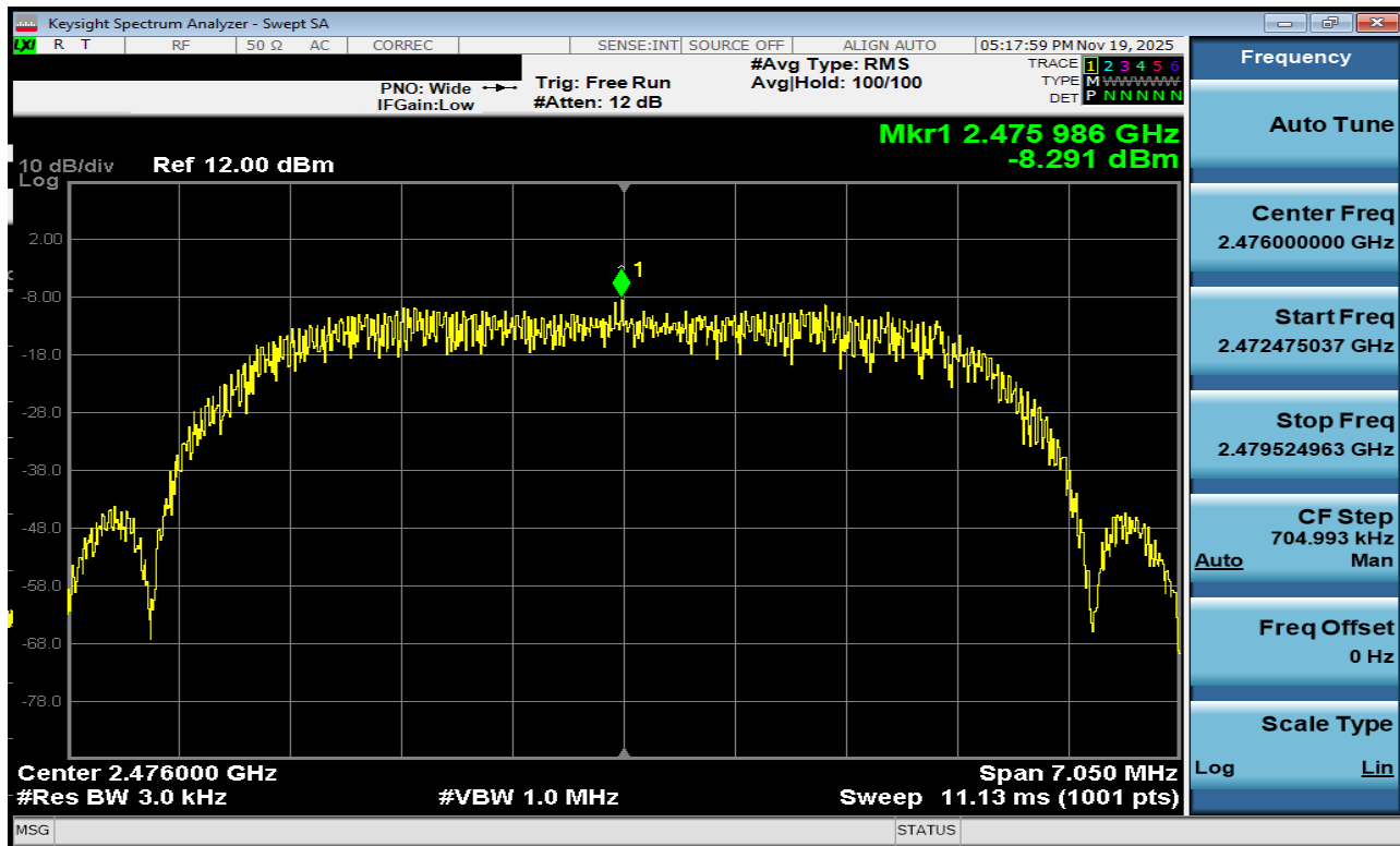
Plot 7-197. Power Spectral Density Plot Tx BF Antenna 3a (Bluetooth (HDRPM16), 16Mbps, ePA – Ch. 73)
