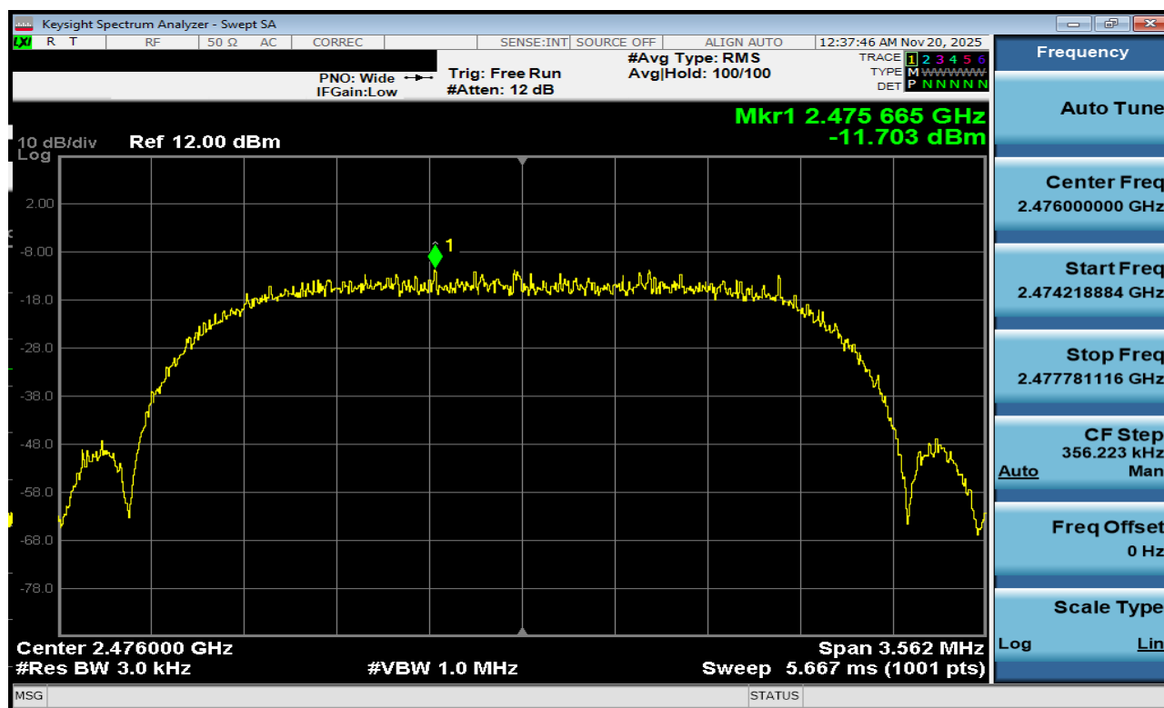
Plot 7-180. Power Spectral Density Plot TxBF Antenna 1a (Bluetooth (HDRPS2), 2Mbps, iPA – Ch. 73)
