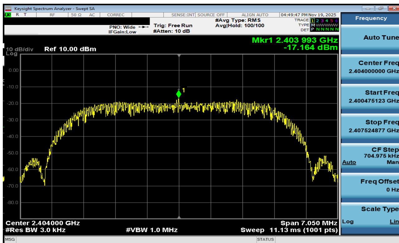
Plot 7-100. Power Spectral Density Plot Antenna 3a (Bluetooth (HDRPM16), 16Mbps, iPA – Ch. 1)
