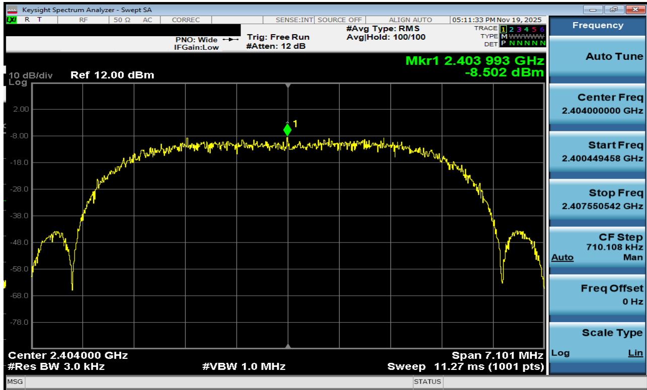
Plot 7-181. Power Spectral Density Plot Tx BF Antenna 3a (Bluetooth (XHDRPM6), 6Mbps, ePA – Ch. 1)
