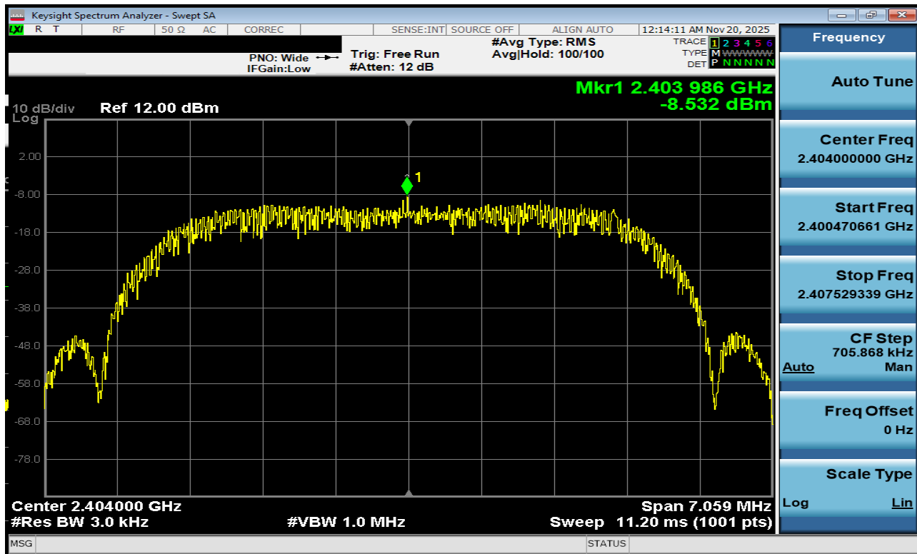
Plot 7-133. Power Spectral Density Plot Antenna 1a (Bluetooth (HDRPM16), 16Mbps, ePA – Ch. 1)
