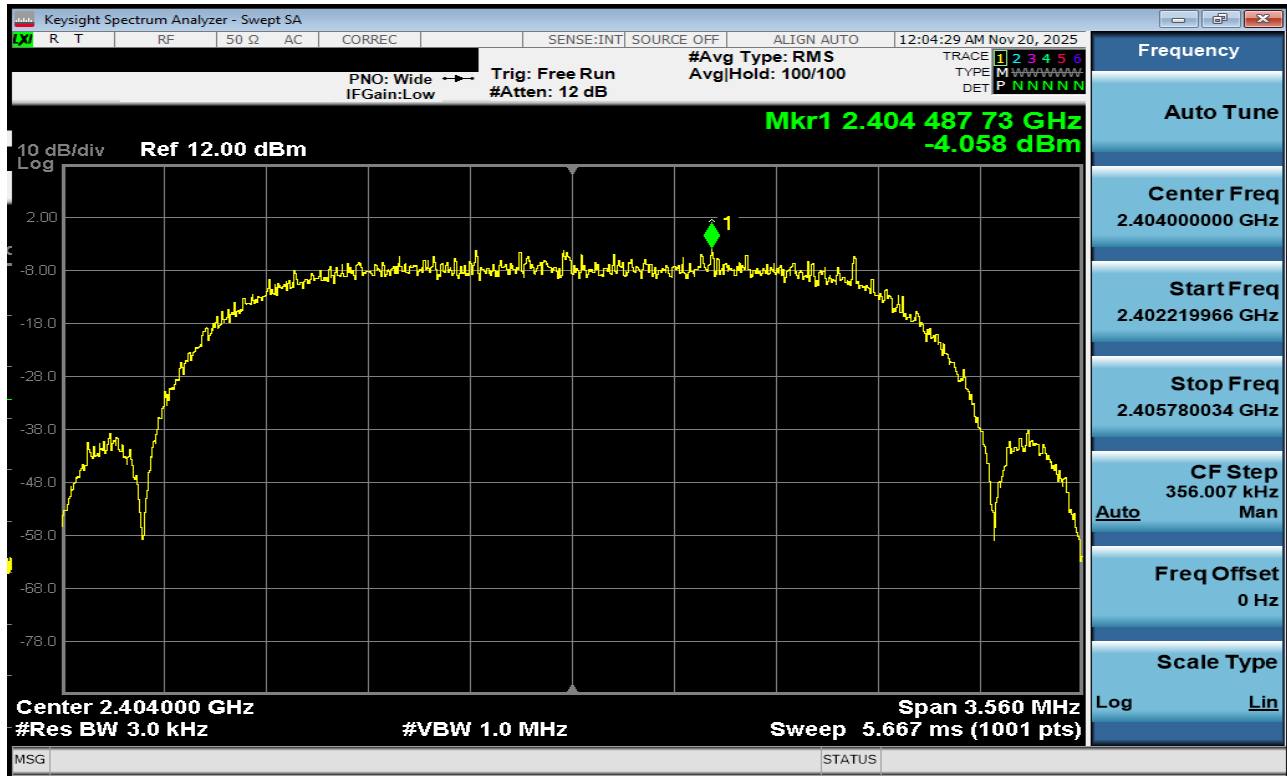
Plot 7-121. Power Spectral Density Plot Antenna 1a (Bluetooth (HDRPS2), 2Mbps, ePA – Ch. 1)
