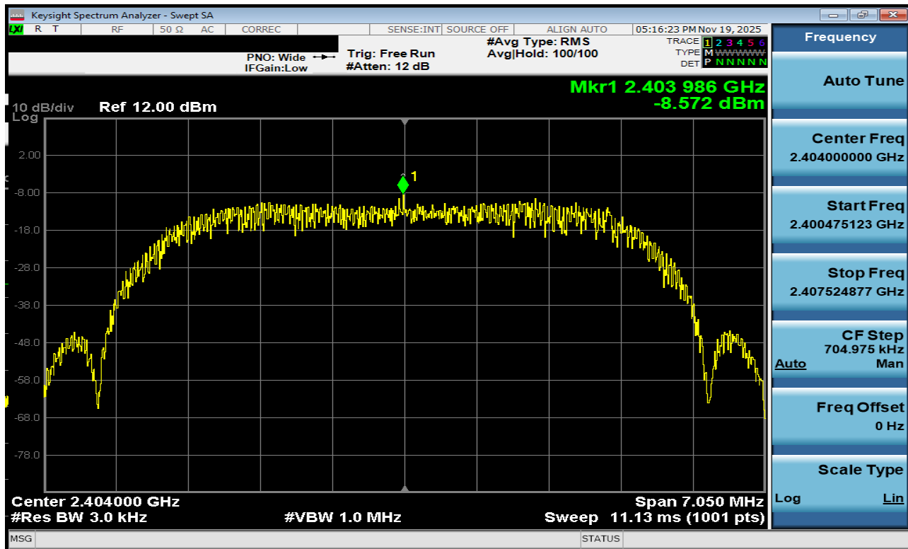
Plot 7-193. Power Spectral Density Plot TxBF Antenna 3a (Bluetooth (HDRPM16), 16Mbps, ePA – Ch. 1)
