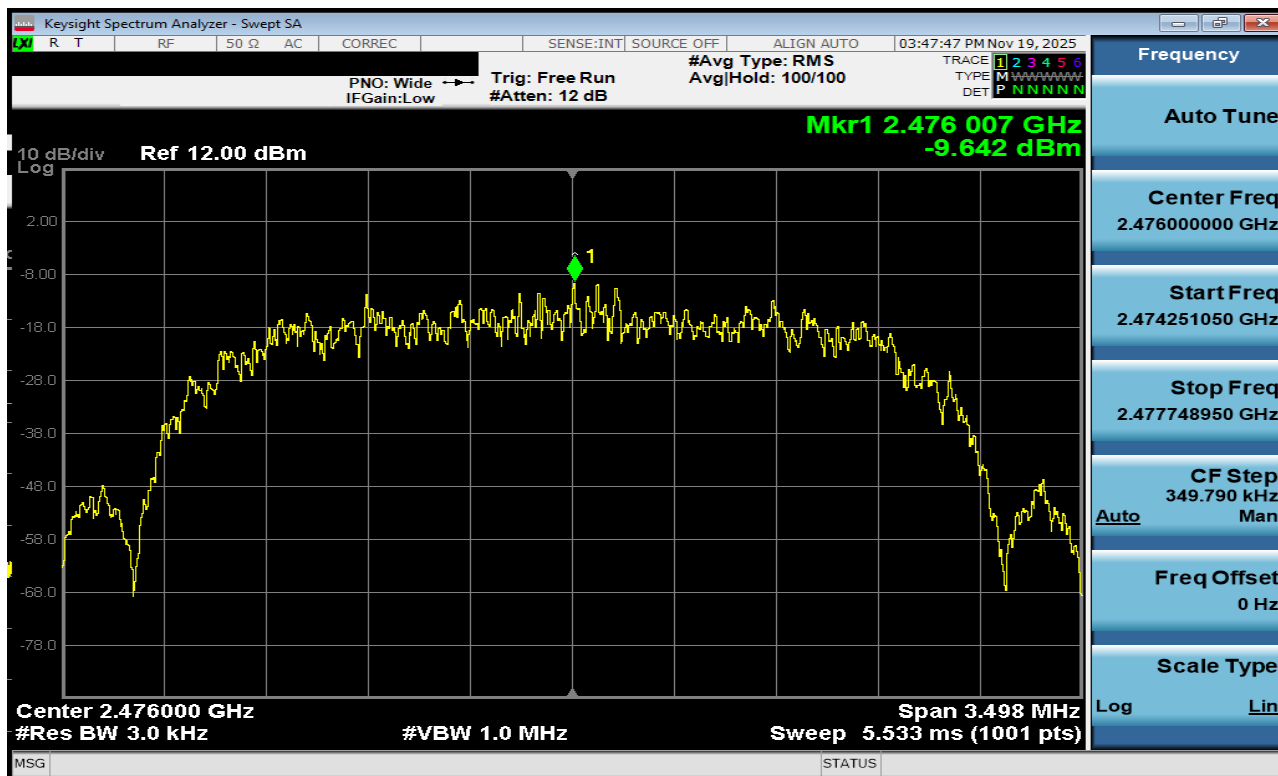
Plot 7-155. Power Spectral Density Plot TxBF Antenna 3a (Bluetooth (HDR4), 4Mbps, iPA – Ch. 73)
