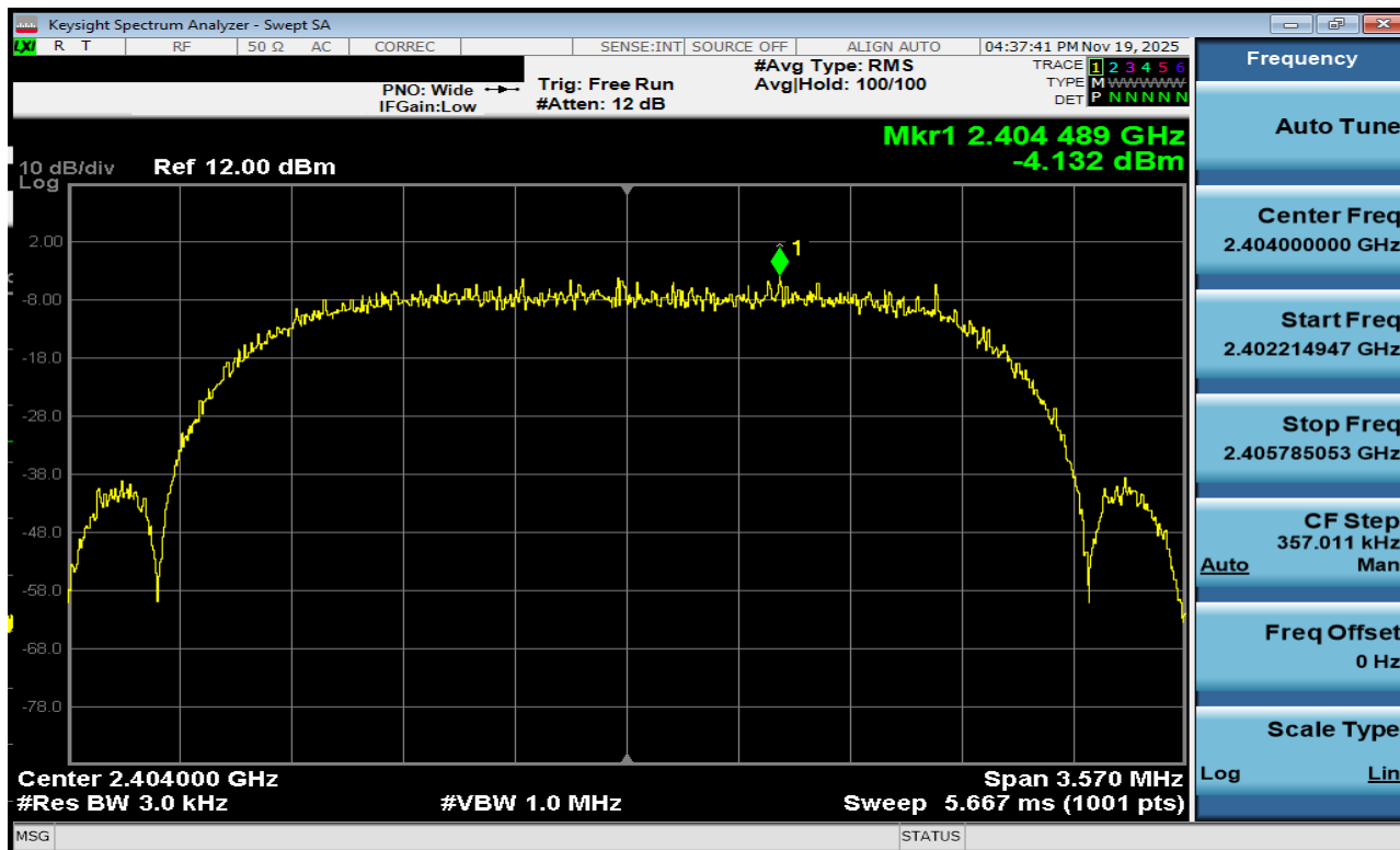
Plot 7-85. Power Spectral Density Plot Antenna 3a (Bluetooth (HDRPS2), 2Mbps, ePA – Ch. 1)
