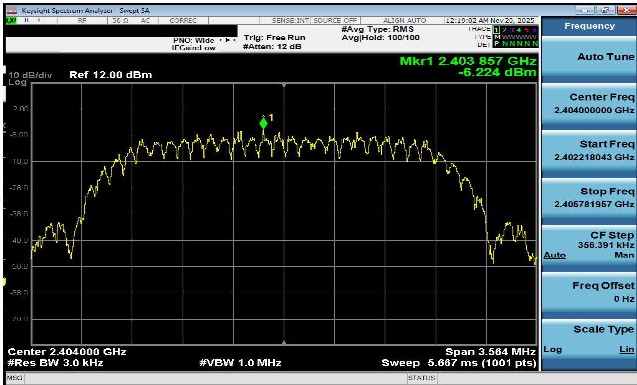
Plot 7-139. Power Spectral Density Plot Antenna 1a (Bluetooth (HDT2), 2Mbps, ePA – Ch. 1)
