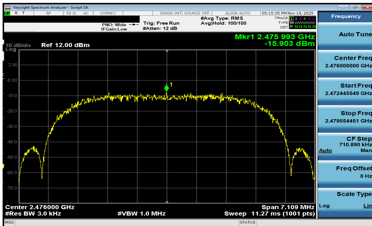
Plot 7-191. Power Spectral Density Plot Tx BF Antenna 3a (Bluetooth (XHDRPM6), 6Mbps, iPA – Ch. 73)
