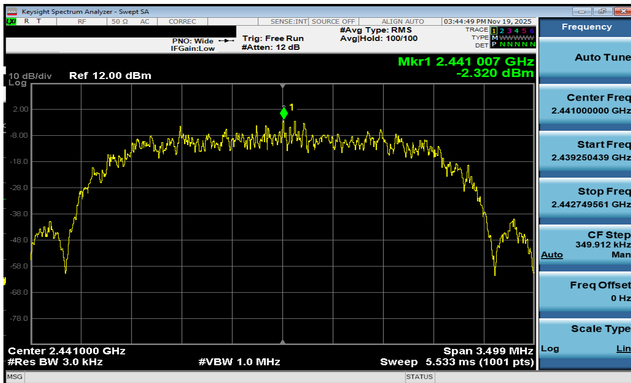
Plot 7-147. Power Spectral Density Plot TxBF Antenna 3a (Bluetooth (HDR4), 4Mbps, ePA – Ch. 38)
