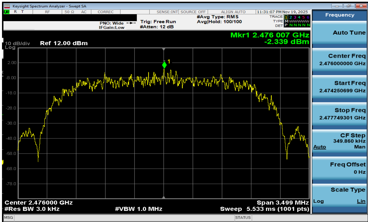
Plot 7-150. Power Spectral Density Plot Tx BF Antenna 1a (Bluetooth (HDR4), 4Mbps, ePA – Ch. 73)
