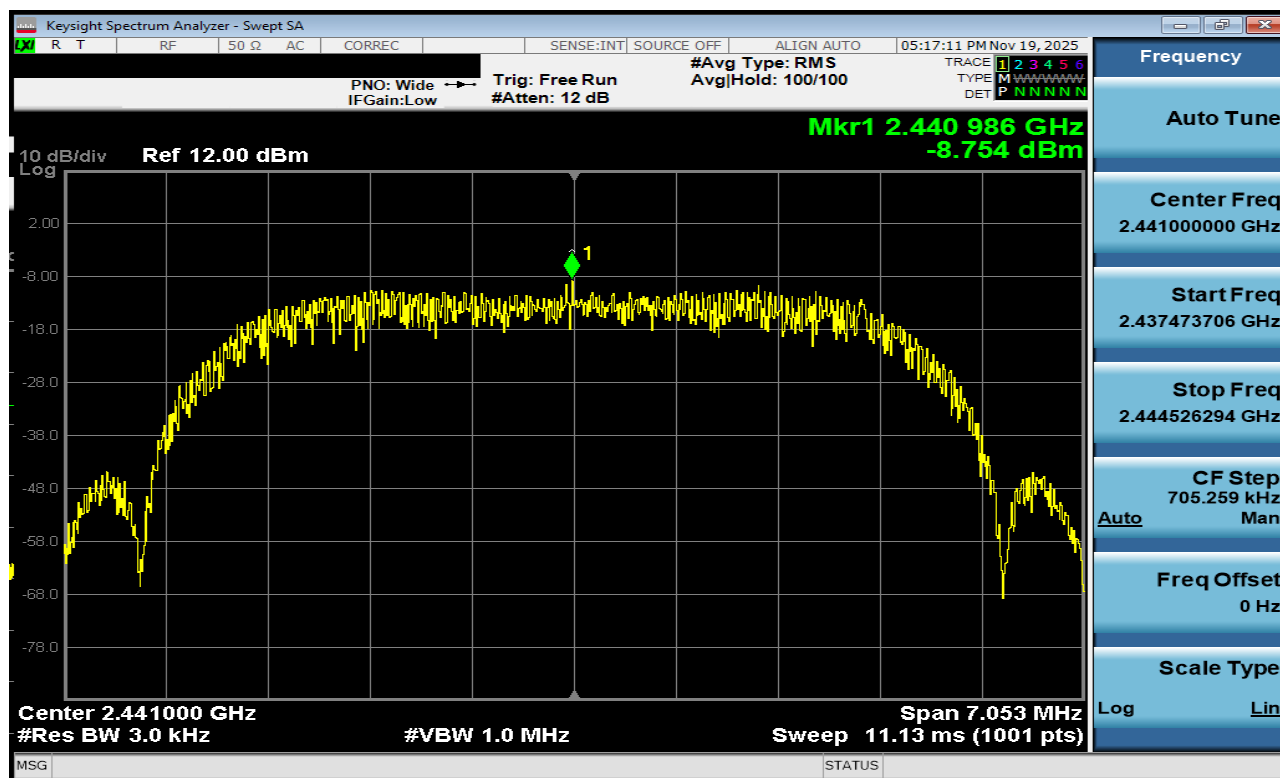
Plot 7-195. Power Spectral Density Plot Tx BF Antenna 3a (Bluetooth (HDRPM16), 16Mbps, ePA – Ch. 38)
