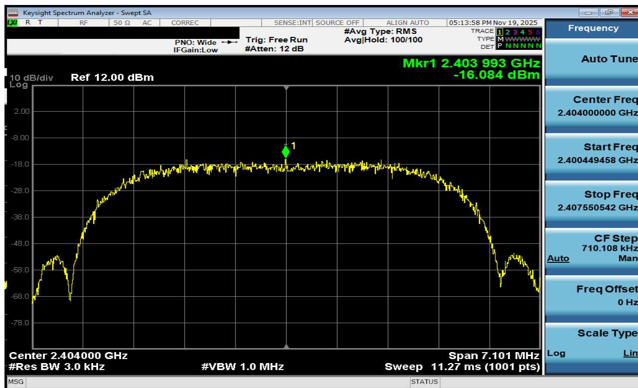
Plot 7-187. Power Spectral Density Plot Tx B Antenna 3a (Bluetooth (XHDRPM6), 6Mbps, iPA – Ch. 1)
