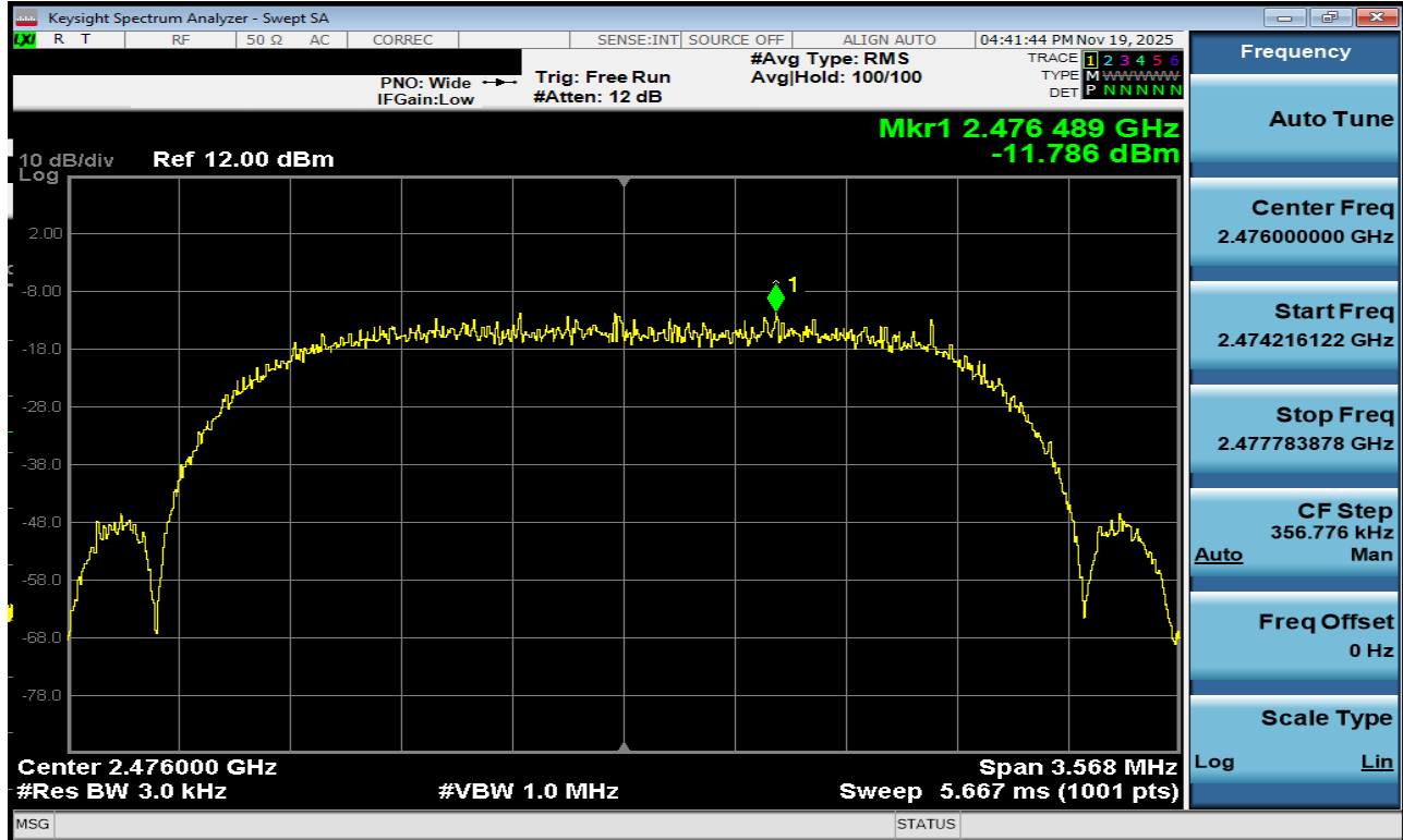
Plot 7-90. Power Spectral Density Plot Antenna 3a (Bluetooth (HDRPS2), 2Mbps, iPA – Ch. 73)
