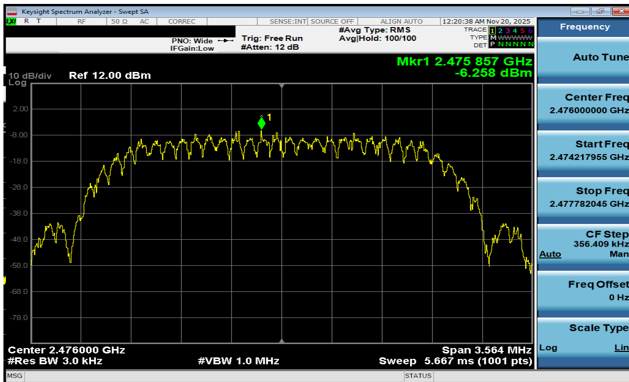
Plot 7-141. Power Spectral Density Plot Antenna 1a (Bluetooth (HDT2), 2Mbps, ePA – Ch. 73)
