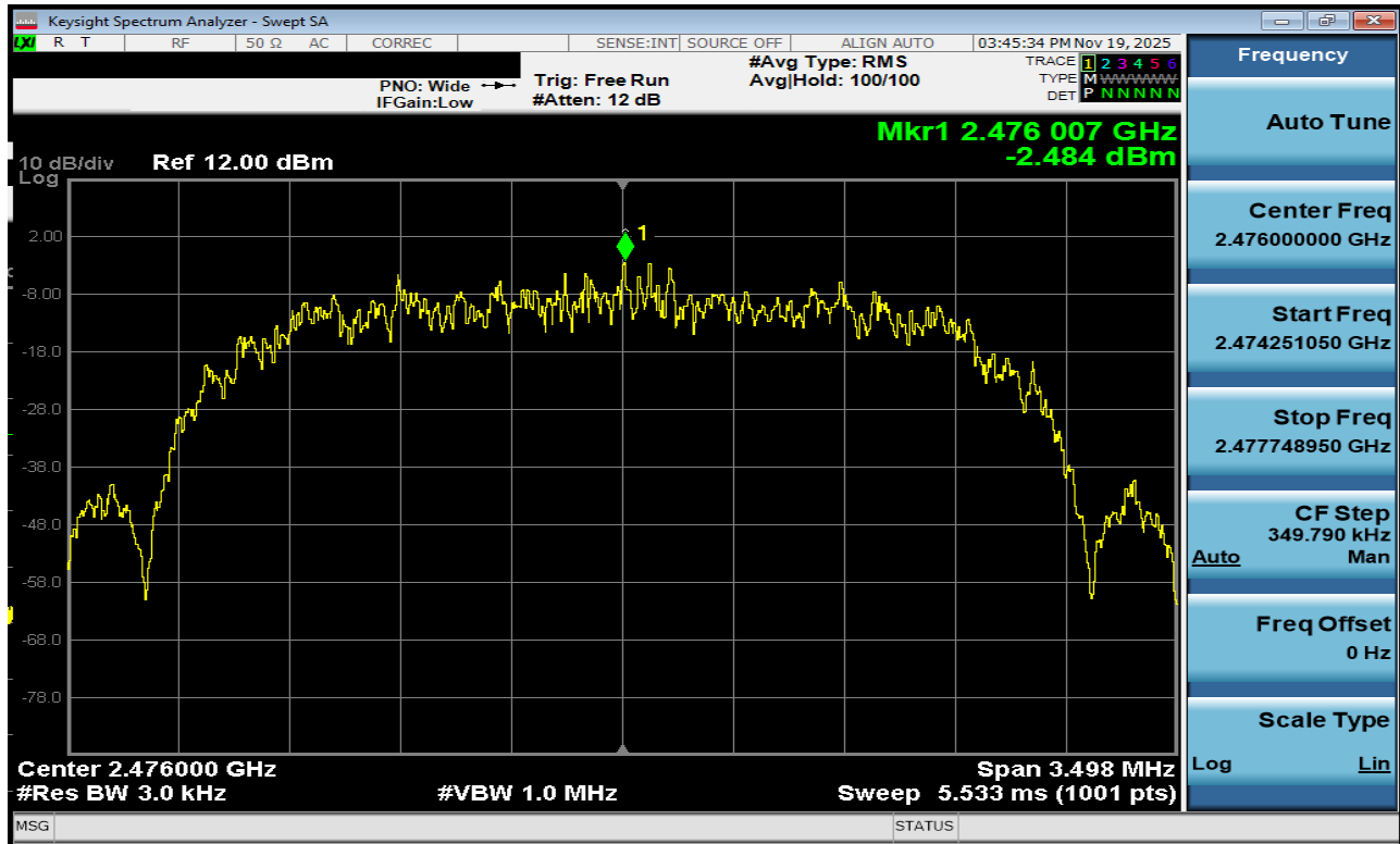
Plot 7-149. Power Spectral Density Plot Tx BF Antenna 3a (Bluetooth (HDR4), 4Mbps, ePA – Ch. 73)
