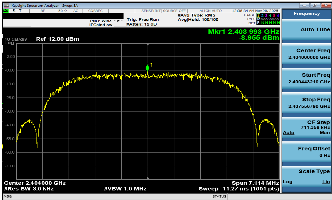
Plot 7-182. Power Spectral Density Plot Tx BF Antenna 1a (Bluetooth (XHDRPM6), 6Mbps, ePA – Ch. 1)
