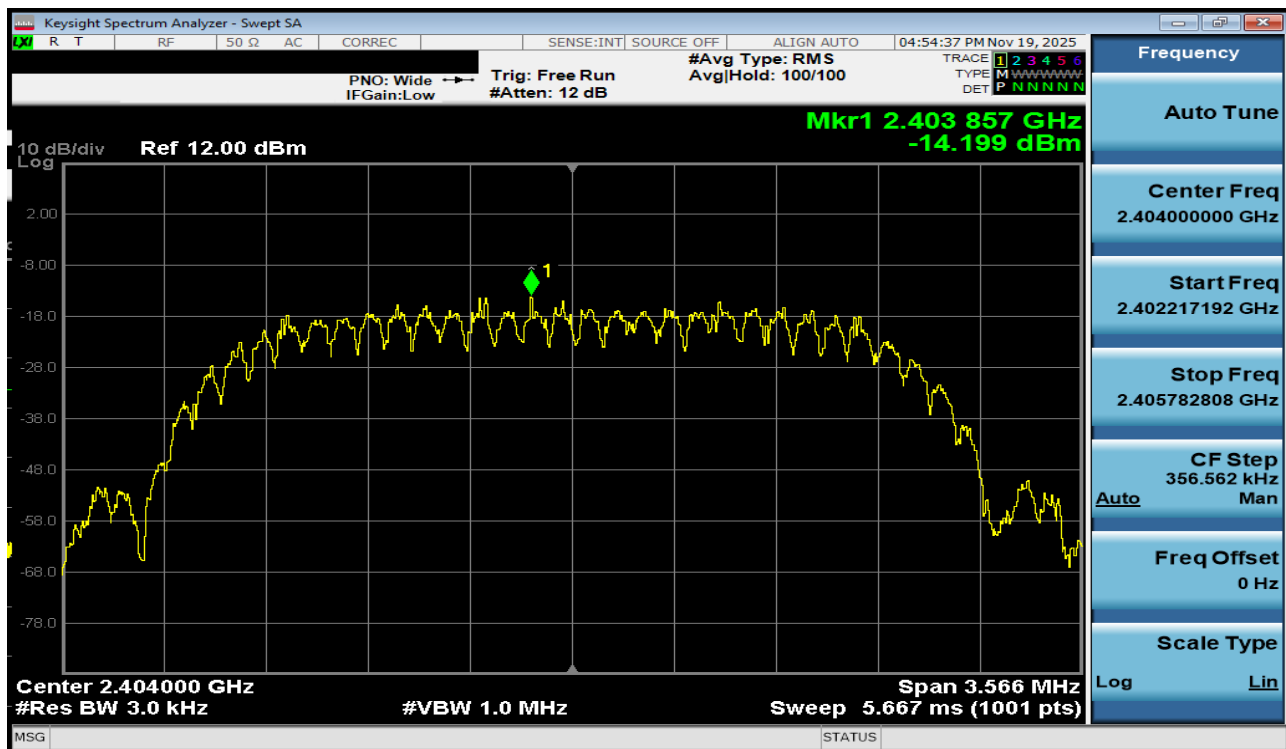
Plot 7-106. Power Spectral Density Plot Antenna 3a (Bluetooth (HDT2), 2Mbps, iPA – Ch. 1)
