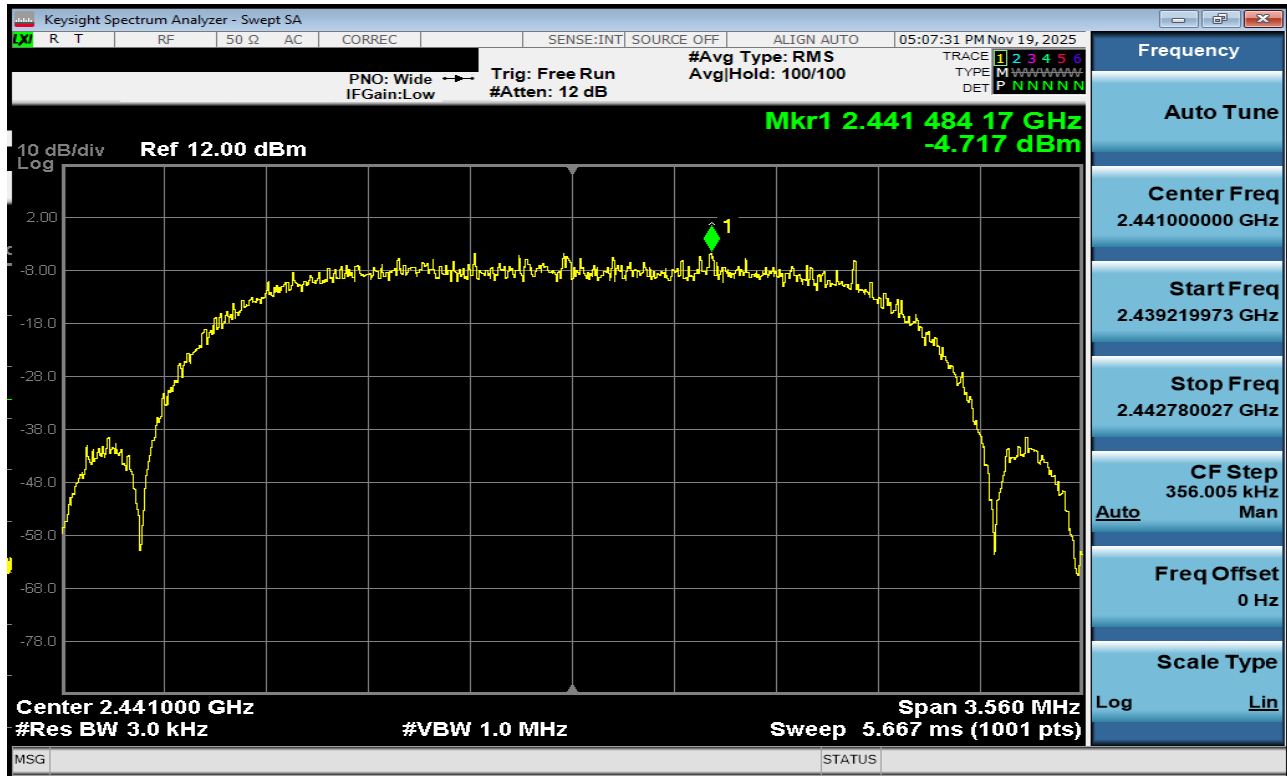
Plot 7-171. Power Spectral Density Plot Tx BF Antenna 3a (Bluetooth (HDRPS2), 2Mbps, ePA – Ch. 38)
