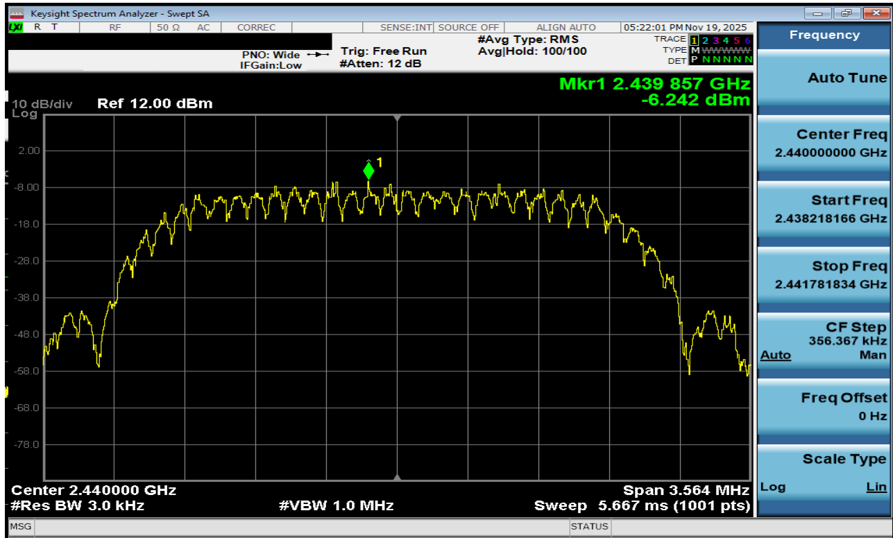
Plot 7-207. Power Spectral Density Plot TxBF Antenna 3a (Bluetooth (HDT2), 2Mbps, ePA – Ch. 37)
