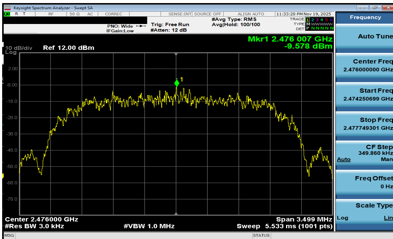
Plot 7-156. Power Spectral Density Plot TxBF Antenna 1a (Bluetooth (HDR4), 4Mbps, iPA – Ch. 73)
