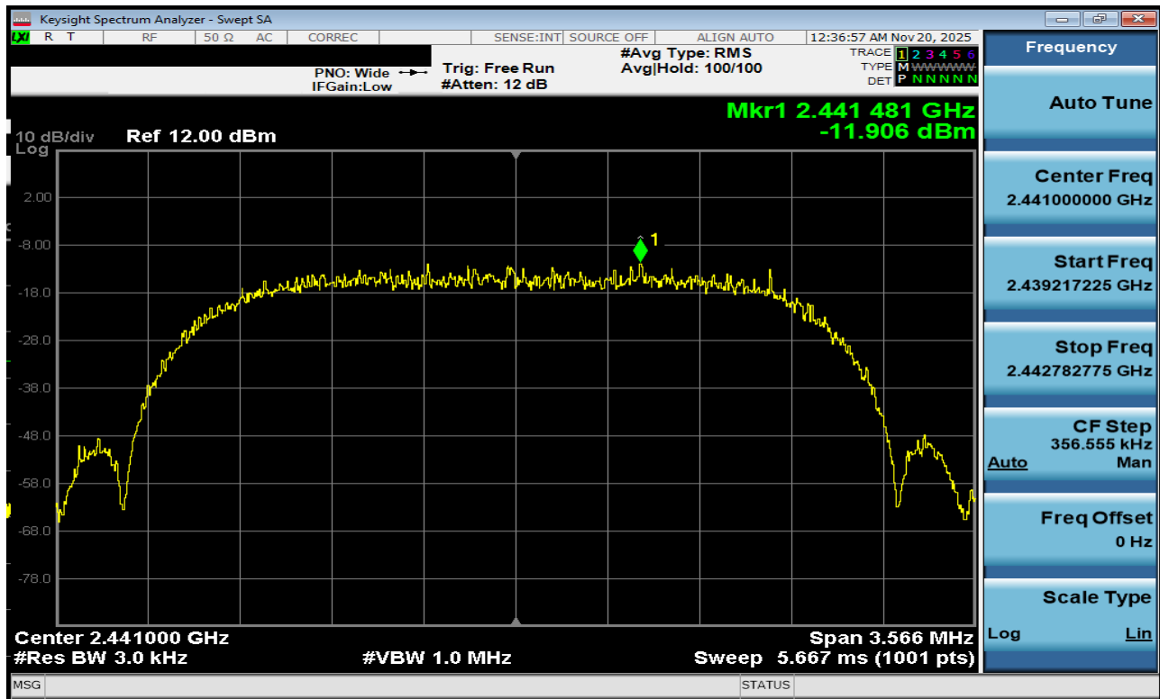
Plot 7-178. Power Spectral Density Plot Tx BF Antenna 1a (Bluetooth (HDRPS2), 2Mbps, iPA – Ch. 38)
