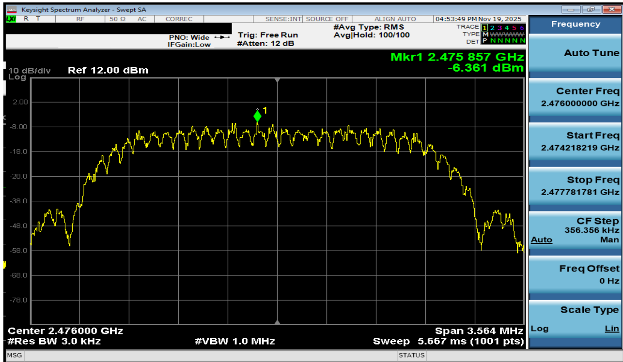
Plot 7-105. Power Spectral Density Plot Antenna 3a (Bluetooth (HDT2), 2Mbps, ePA – Ch. 73)
