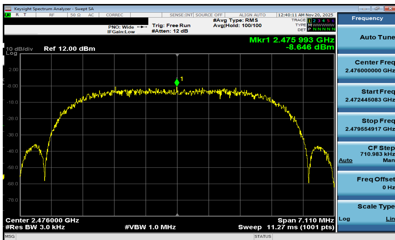
Plot 7-186. Power Spectral Density Plot TxBF Antenna 1a (Bluetooth (XHDRPM6), 6Mbps, ePA – Ch. 73)
