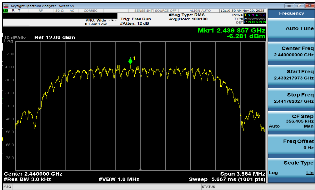
Plot 7-140. Power Spectral Density Plot Antenna 1a (Bluetooth (HDT2), 2Mbps, ePA – Ch. 37)
