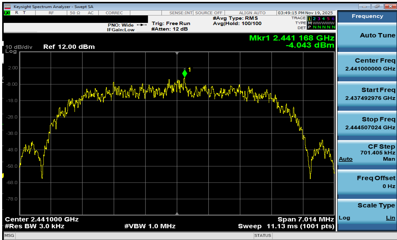
Plot 7-159. Power Spectral Density Plot TxBF Antenna 3a (Bluetooth (HDR8), 8Mbps, ePA – Ch. 38)
