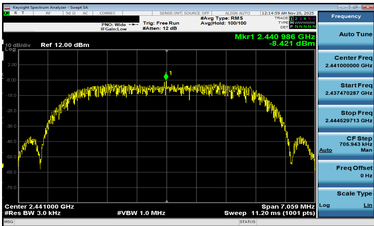
Plot 7-134. Power Spectral Density Plot Antenna 1a (Bluetooth (HDRPM16), 16Mbps, ePA – Ch. 38)
