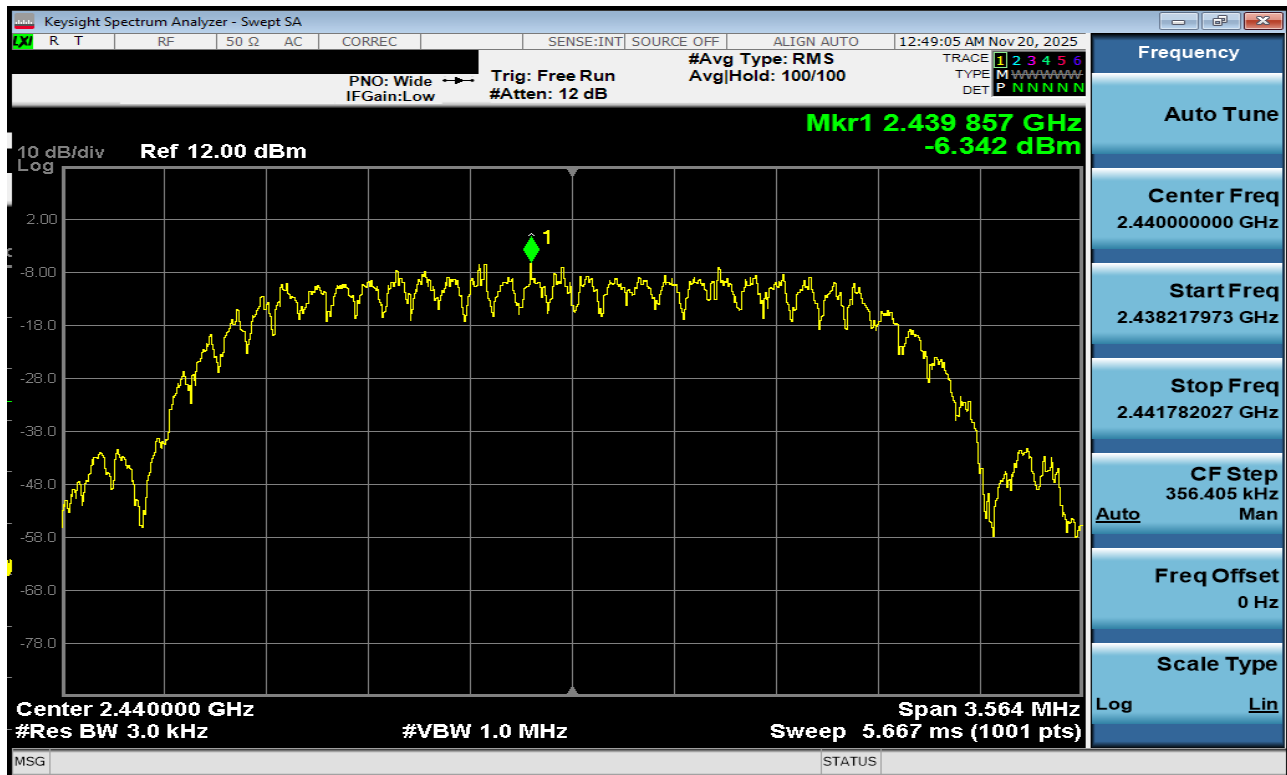
Plot 7-208. Power Spectral Density Plot TxBF Antenna 1a (Bluetooth (HDT2), 2Mbps, ePA – Ch. 37)
