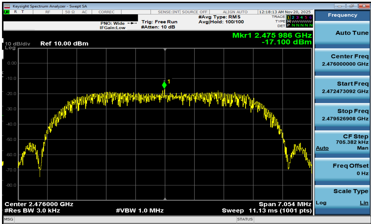
Plot 7-138. Power Spectral Density Plot Antenna 1a (Bluetooth (HDRPM16), 16Mbps, iPA – Ch. 73)
