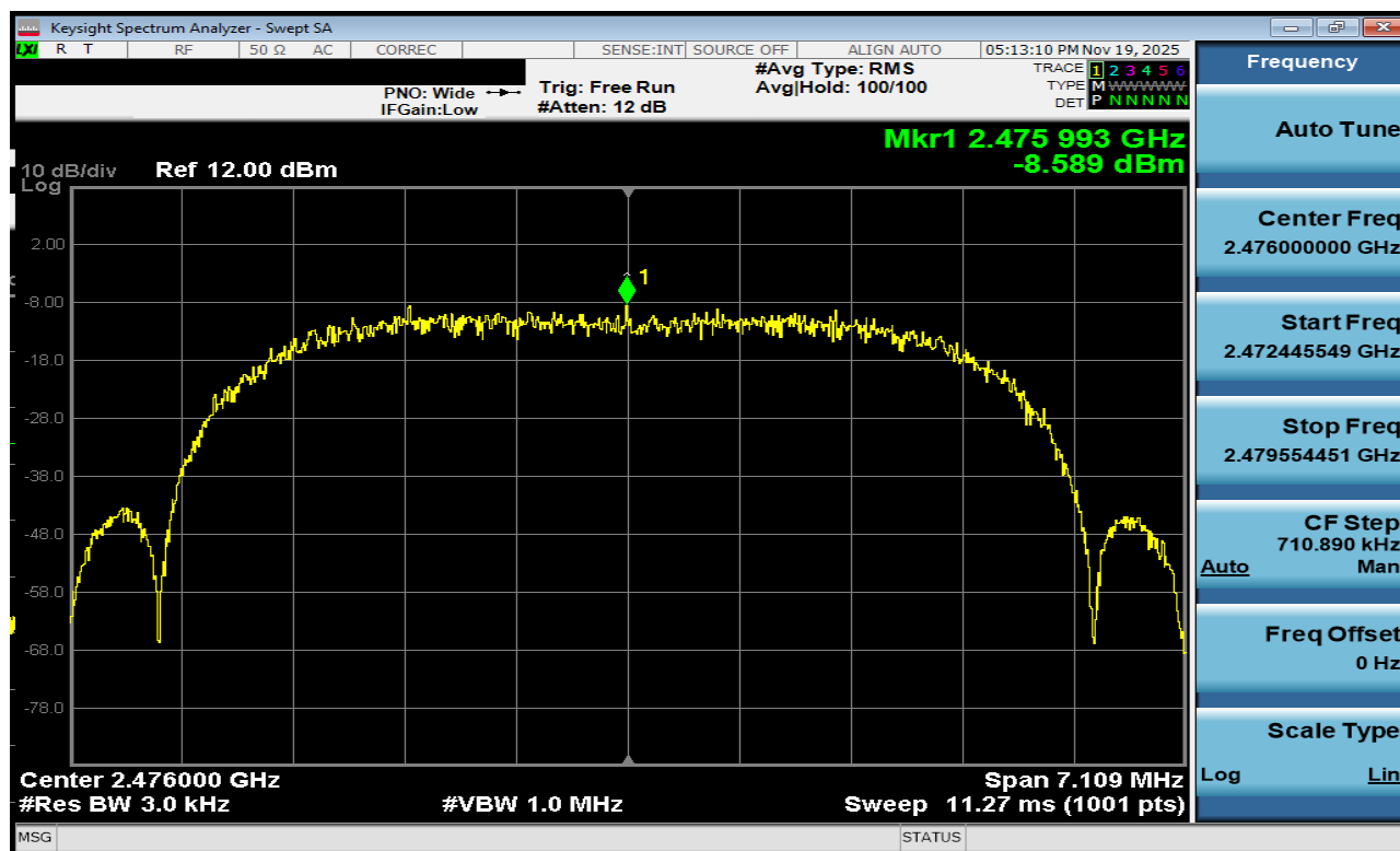
Plot 7-185. Power Spectral Density Plot TxBF Antenna 3a (Bluetooth (XHDRPM6), 6Mbps, ePA – Ch. 73)
