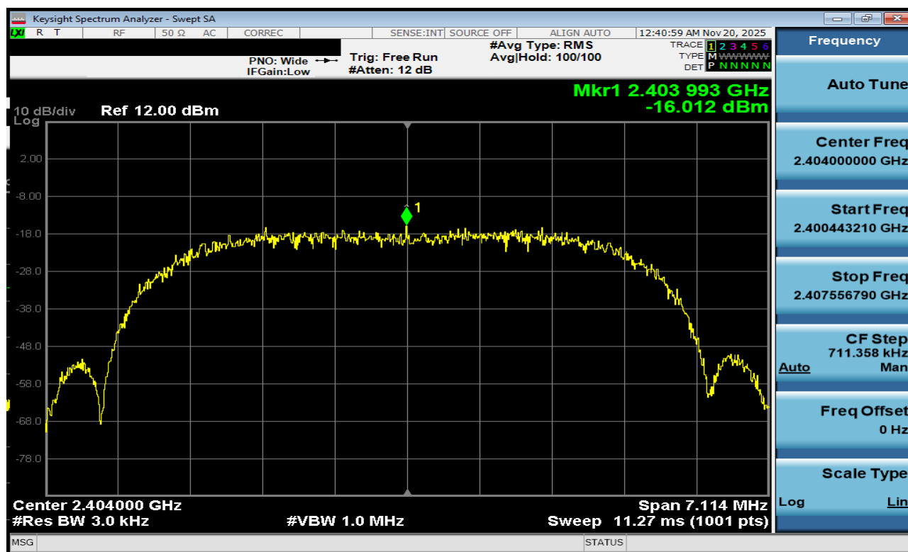
Plot 7-188. Power Spectral Density Plot Tx B Antenna 1a (Bluetooth (XHDRPM6), 6Mbps, iPA – Ch. 1)
