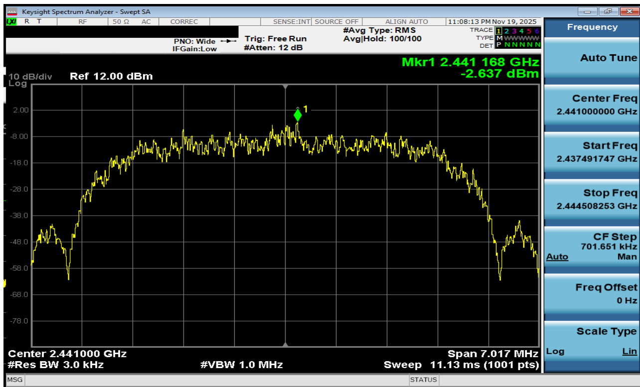
Plot 7-116. Power Spectral Density Plot Antenna 1a (Bluetooth (HDR8), 8Mbps, ePA – Ch. 38)
