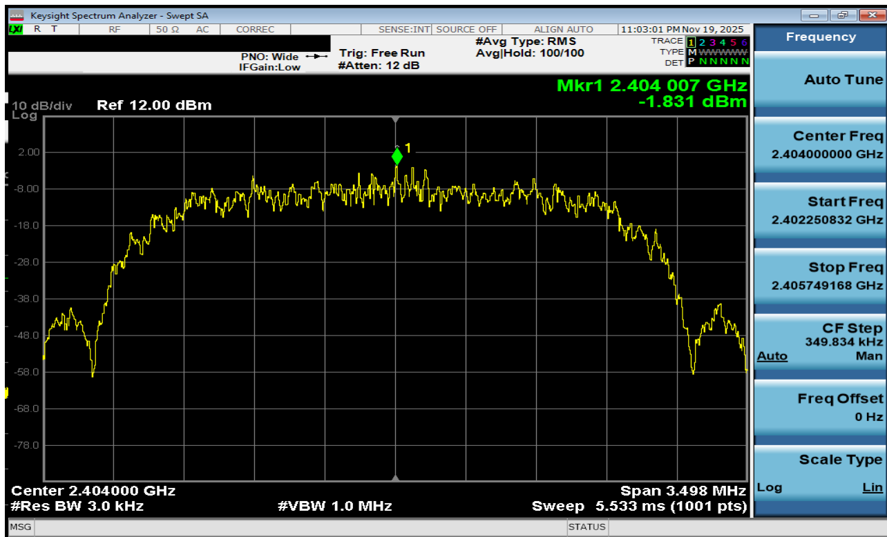
Plot 7-109. Power Spectral Density Plot Antenna 1a (Bluetooth (HDR4), 4Mbps, ePA – Ch. 1)
