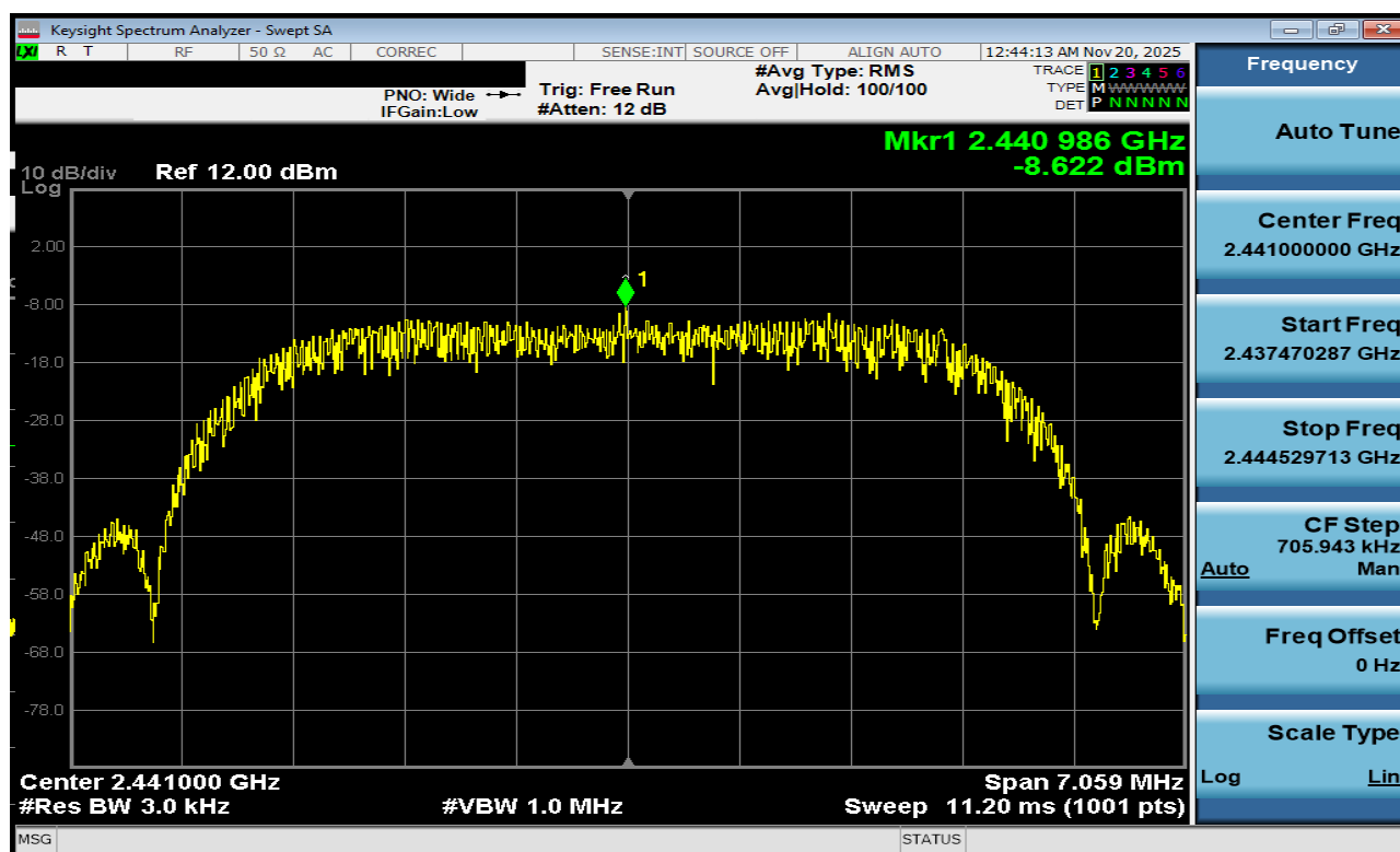
Plot 7-196. Power Spectral Density Plot Tx BF Antenna 1a (Bluetooth (HDRPM16), 16Mbps, ePA – Ch. 38)
