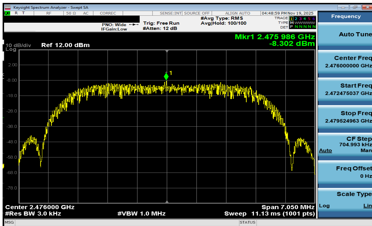
Plot 7-99. Power Spectral Density Plot Antenna 3a (Bluetooth (HDRPM16), 16Mbps, ePA – Ch. 73)
