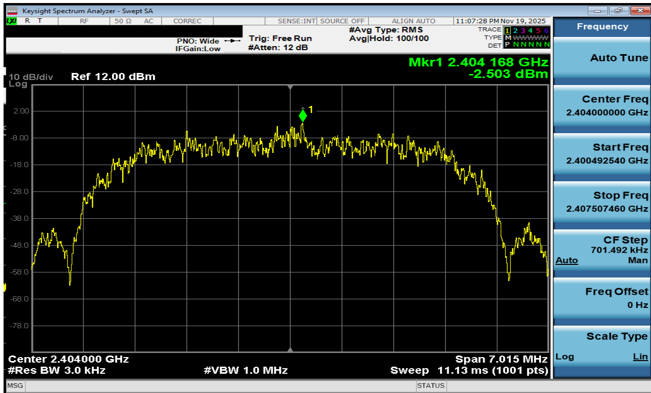
Plot 7-115. Power Spectral Density Plot Antenna 1a (Bluetooth (HDR8), 8Mbps, ePA – Ch. 1)
