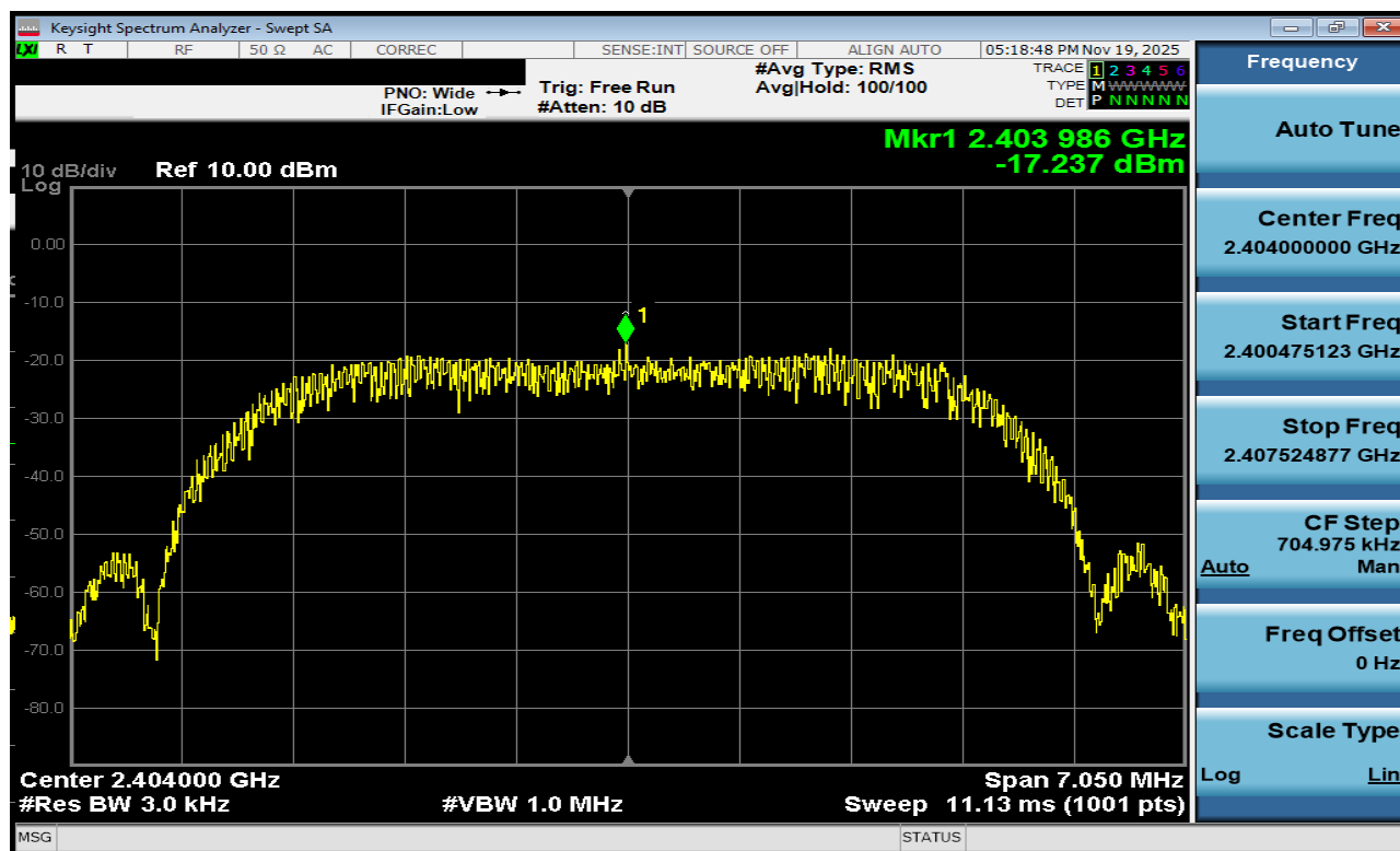
Plot 7-199. Power Spectral Density Plot Tx BF Antenna 3a (Bluetooth (HDRPM16), 16Mbps, iPA – Ch. 1)
