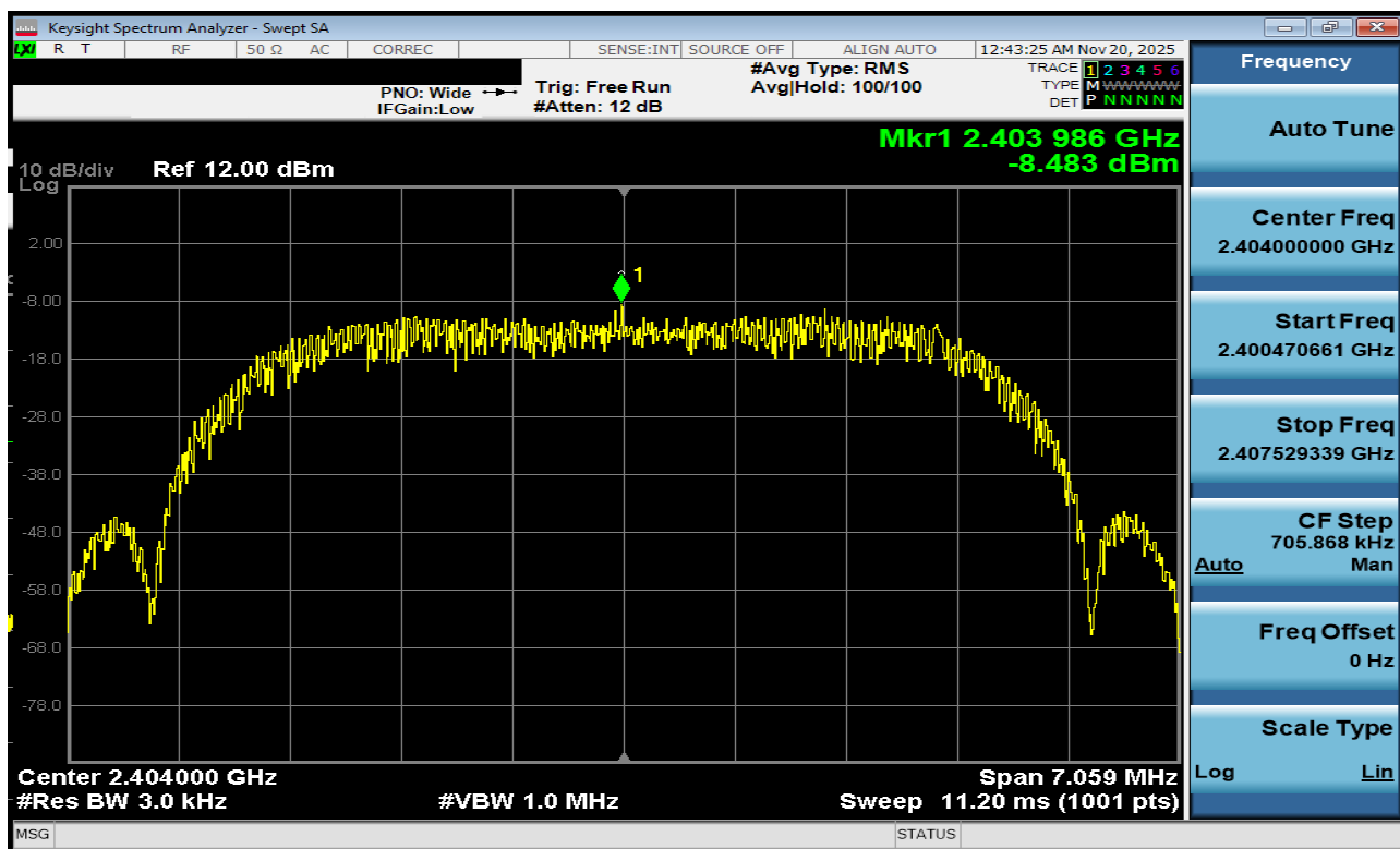
Plot 7-194. Power Spectral Density Plot TxBF Antenna 1a (Bluetooth (HDRPM16), 16Mbps, ePA – Ch. 1)
