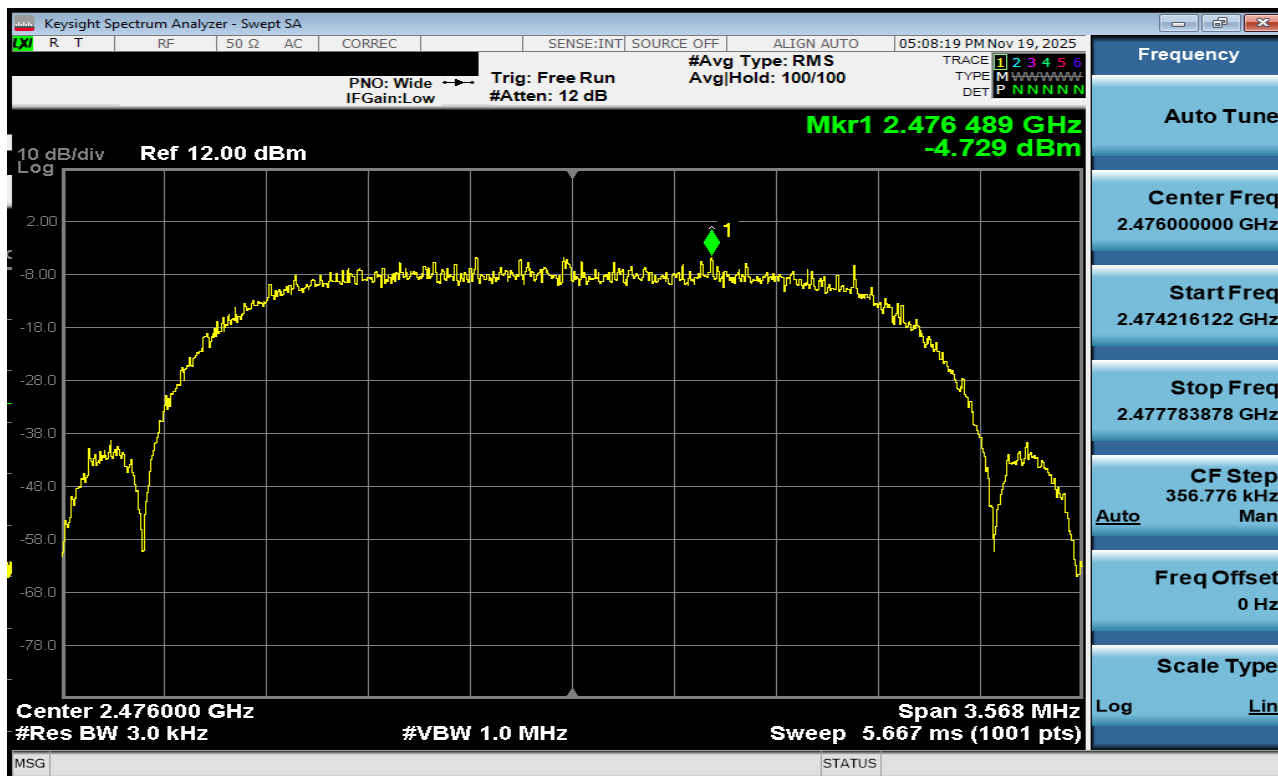
Plot 7-173. Power Spectral Density Plot Tx BF Antenna 3a (Bluetooth (HDRPS2), 2Mbps, ePA – Ch. 73)
