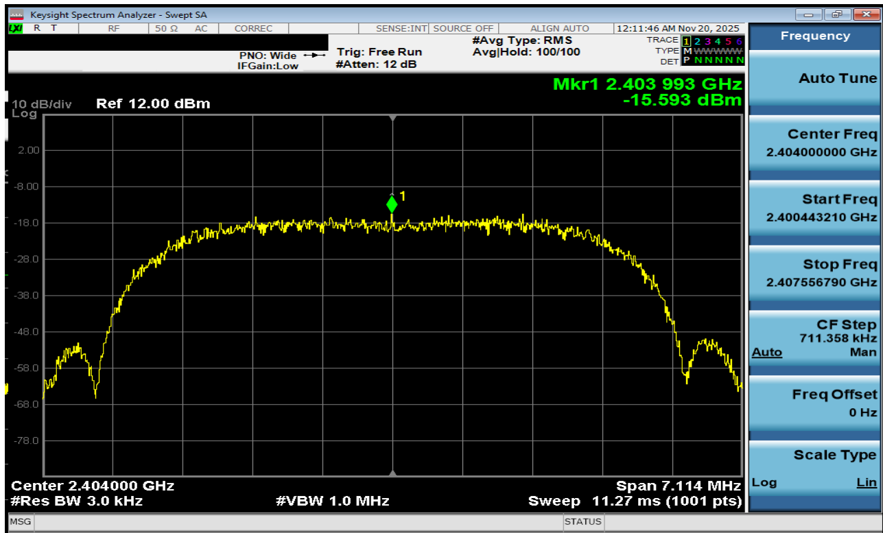
Plot 7-130. Power Spectral Density Plot Antenna 1a (Bluetooth (XHDRPM6), 6Mbps, iPA – Ch. 1)
