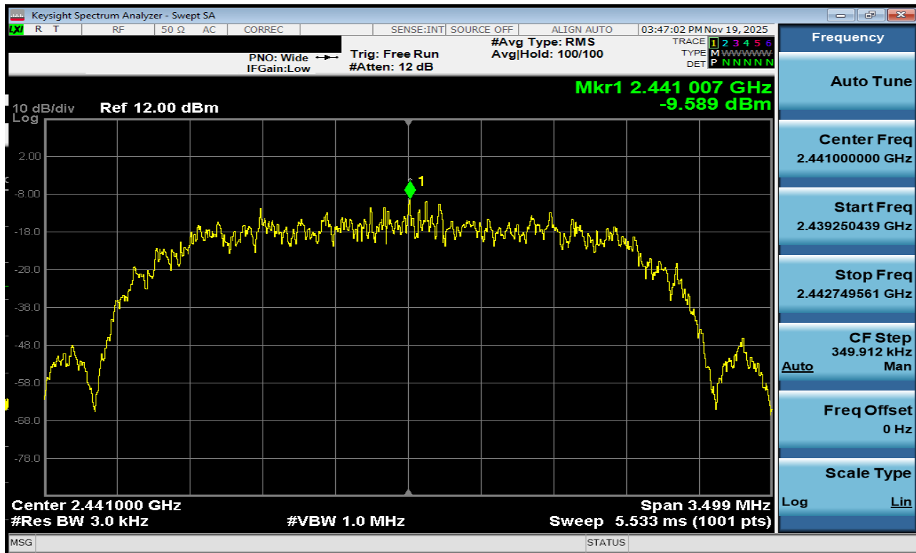
Plot 7-153. Power Spectral Density Plot TxBF Antenna 3a (Bluetooth (HDR4), 4Mbps, iPA – Ch. 38)
