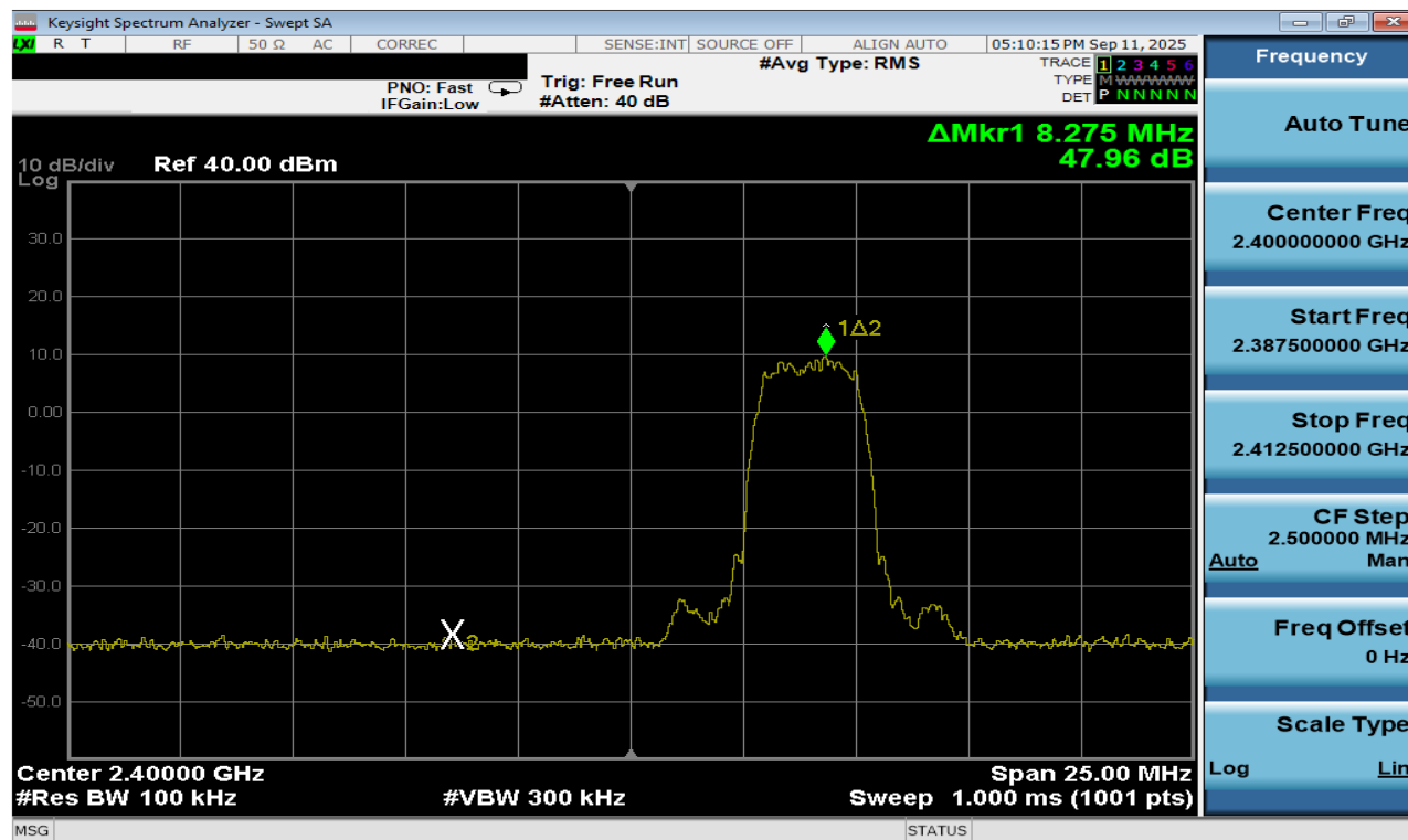
Plot 7-227. Band Edge Plot Antenna 3a (Bluetooth (HDT2), 2Mbps, ePA – Ch. 1)
