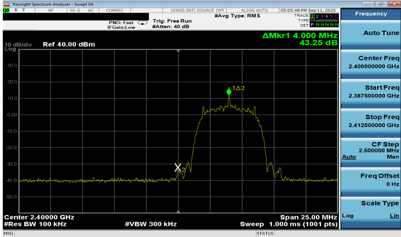
Plot 7-225. Band Edge Plot Antenna 3a (Bluetooth (HDRPM16), 16Mbps, ePA – Ch. 1)
