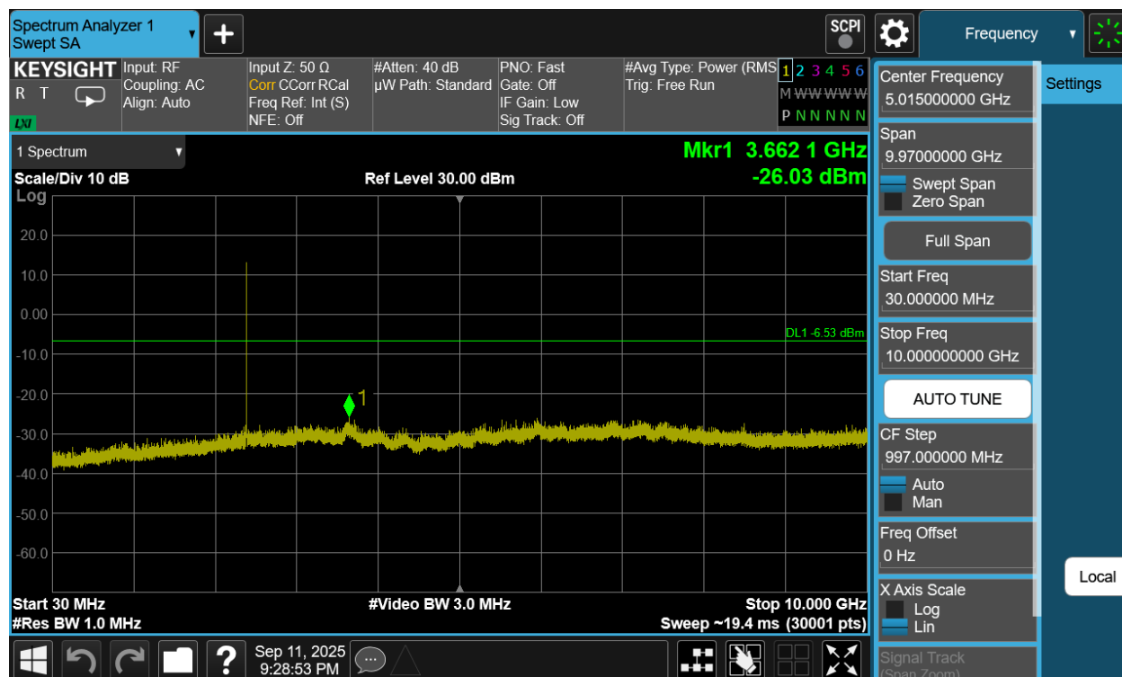
Plot 7-283. Conducted Spurious Plot Antenna 1a (Bluetooth (XHDRPM6), 6Mbps, ePA – Ch. 1)
