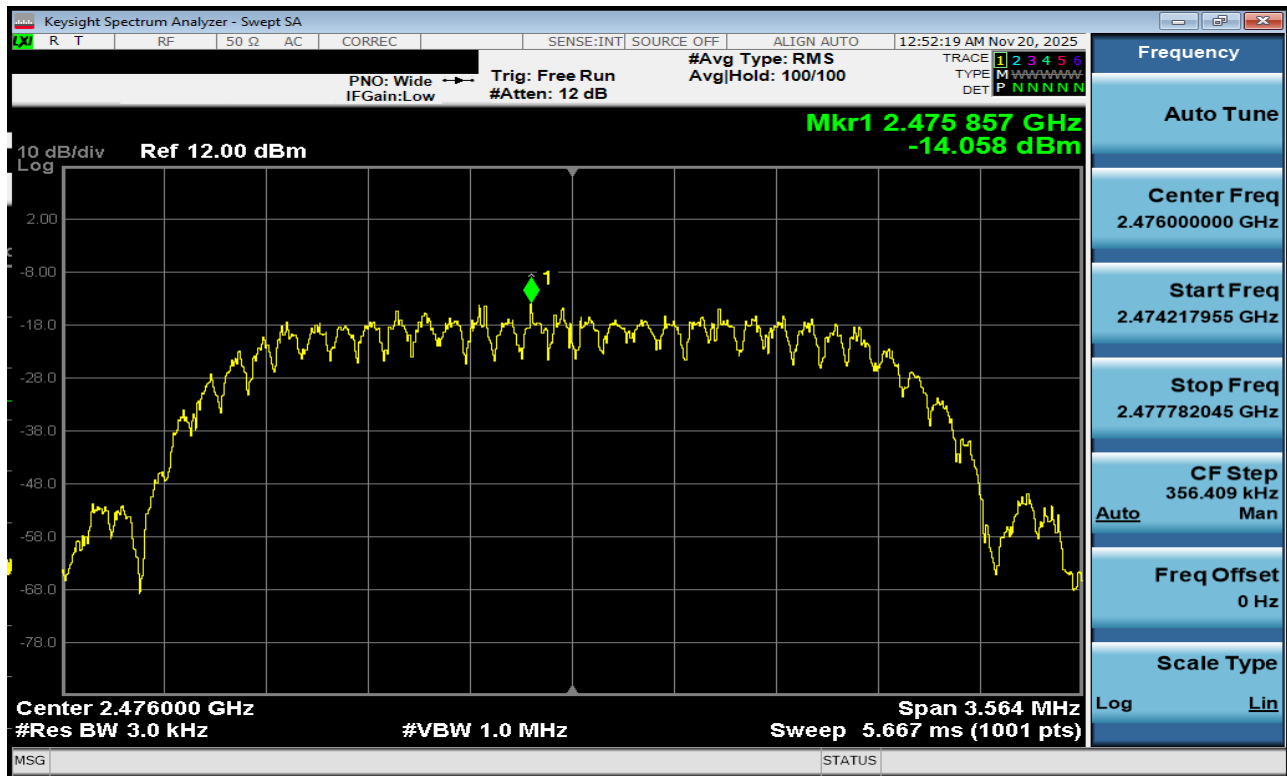
Plot 7-216. Power Spectral Density Plot TxBF Antenna 1a (Bluetooth (HDT2), 2Mbps, iPA – Ch. 73)
