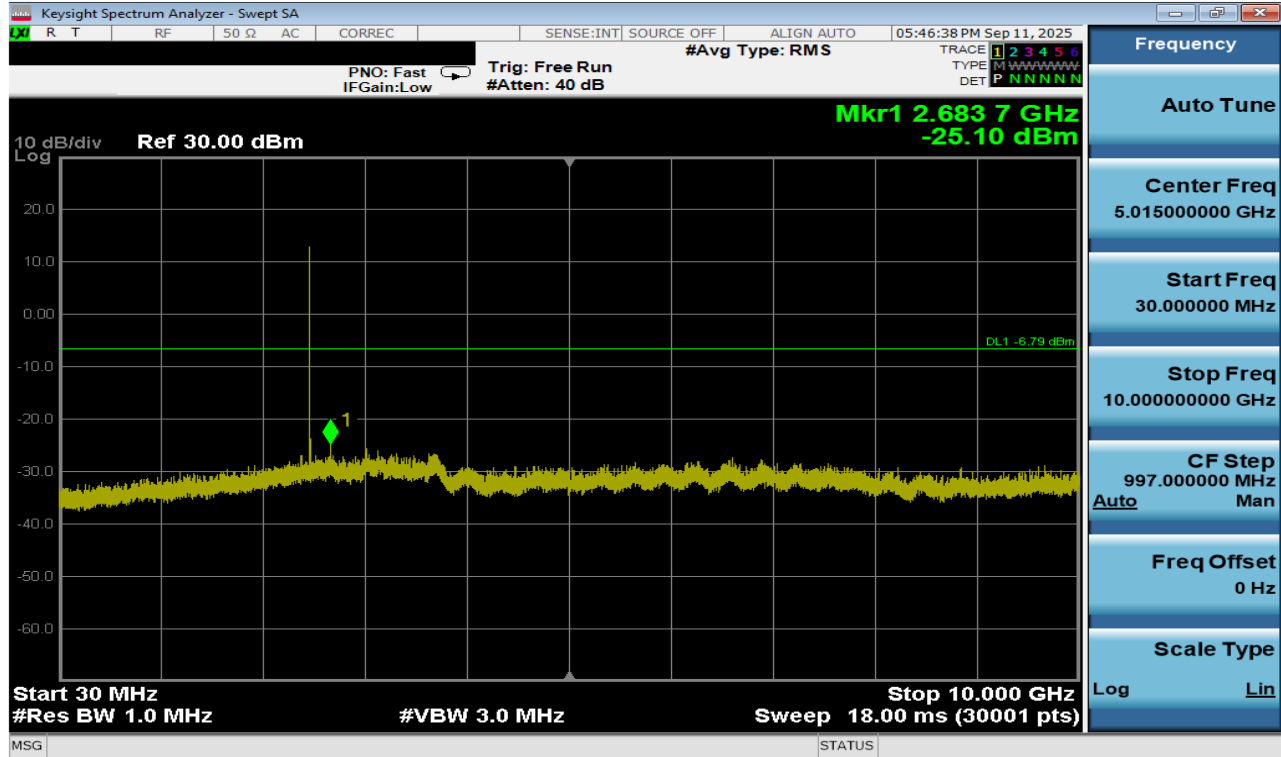
Plot 7-257. Conducted Spurious Plot Antenna 3a (Bluetooth (XHDRPM6), 6Mbps, ePA – Ch. 73)
