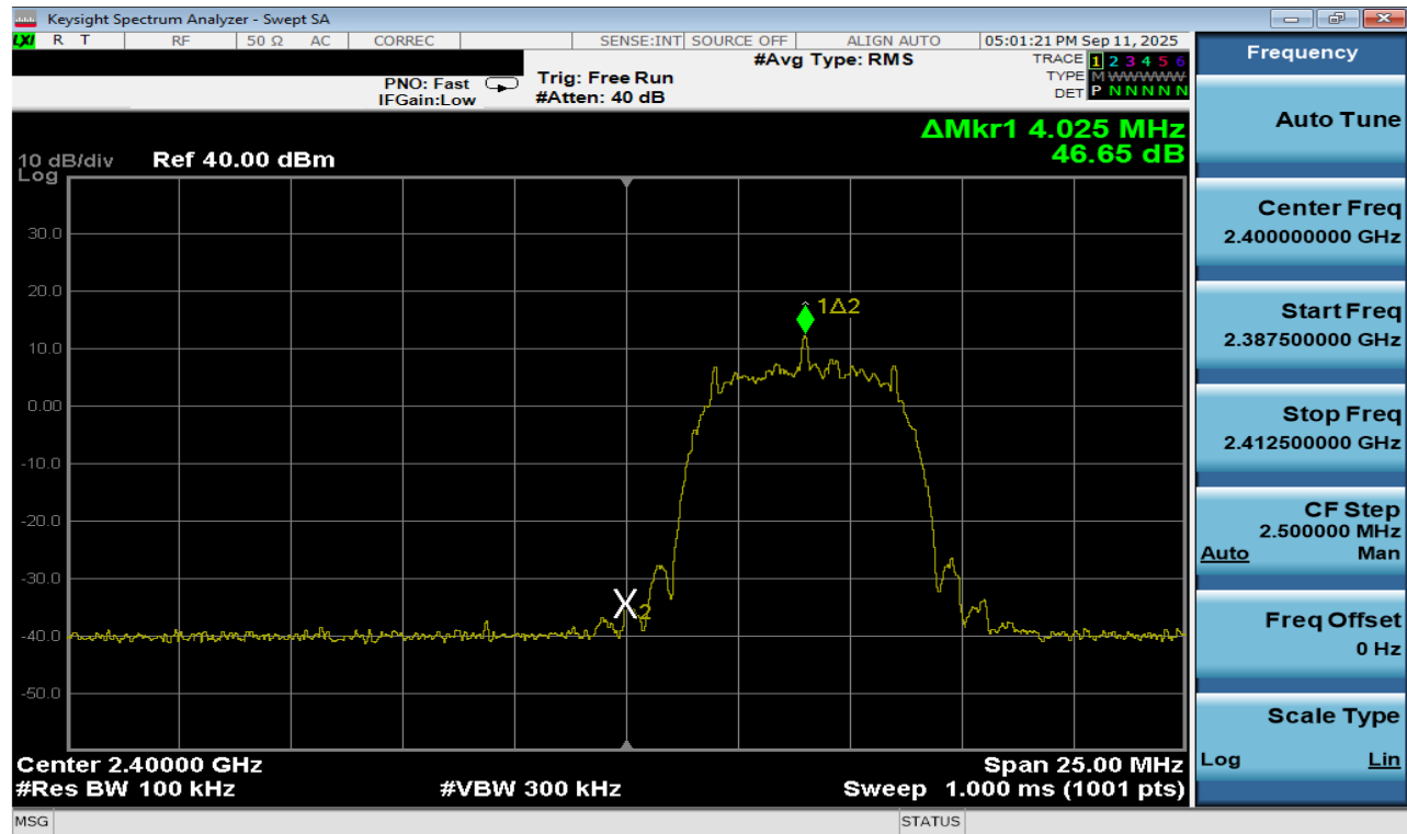
Plot 7-223. Band Edge Plot Antenna 3a (Bluetooth (XHDRPM6), 6Mbps, ePA – Ch. 1)
