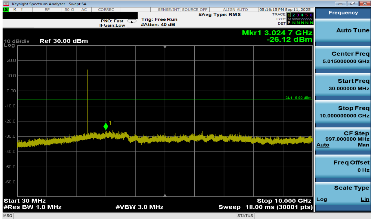
Plot 7-247. Conducted Spurious Plot Antenna 3a (Bluetooth (HDRPS2), 2Mbps, ePA – Ch. 1)
