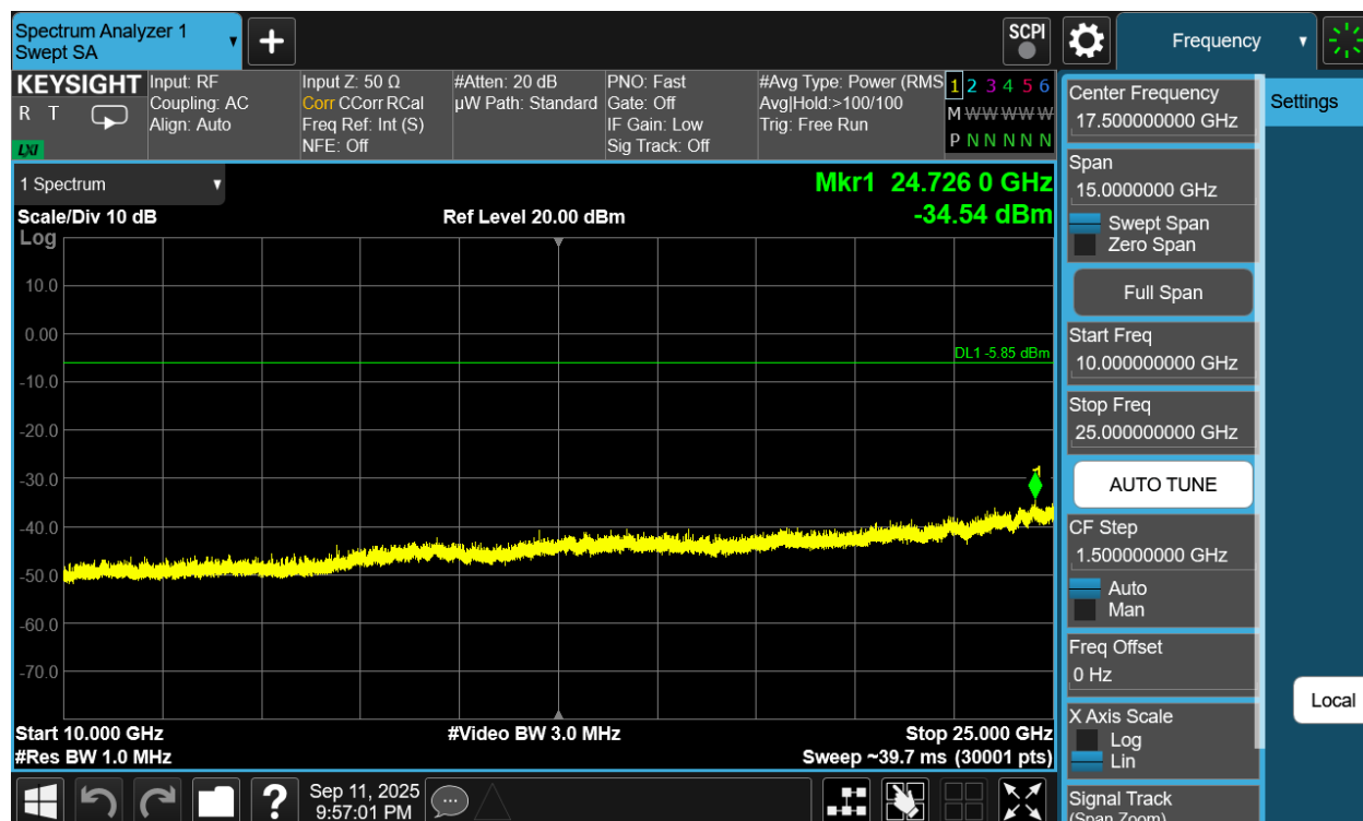
Plot 7-296. Conducted Spurious Plot Antenna 1a (Bluetooth (HDT2), 2Mbps, ePA – Ch. 1)
