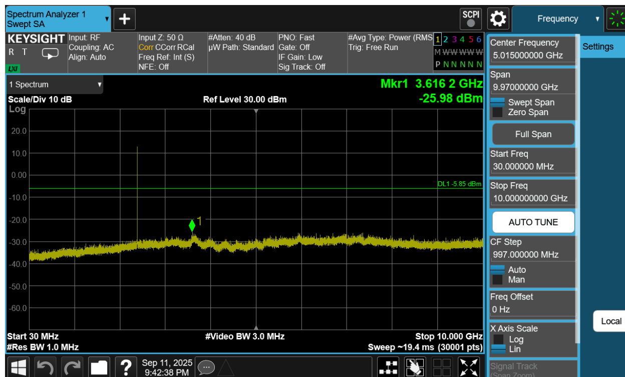
Plot 7-289. Conducted Spurious Plot Antenna 1a (Bluetooth (HDRPM16), 16Mbps, ePA – Ch. 1)
