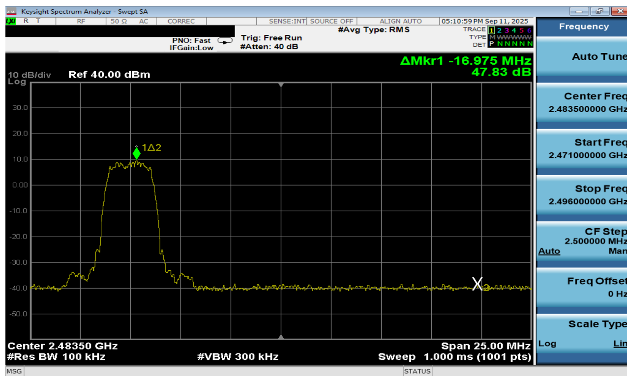
Plot 7-228. Band Edge Plot Antenna 3a (Bluetooth (HDT2), 2Mbps, ePA – Ch. 73)
