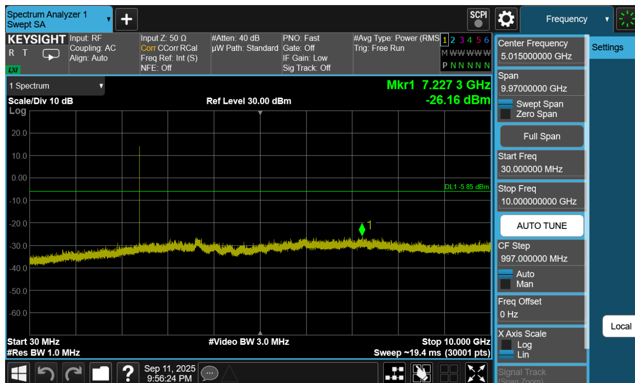
Plot 7-295. Conducted Spurious Plot Antenna 1a (Bluetooth (HDT2), 2Mbps, ePA – Ch. 1)
