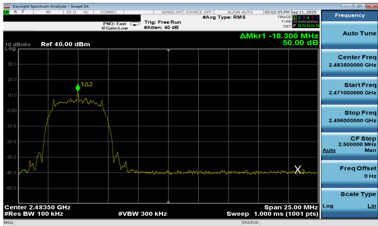
Plot 7-224. Band Edge Plot Antenna 3a (Bluetooth (XHDRPM6), 6Mbps, ePA – Ch. 73)
