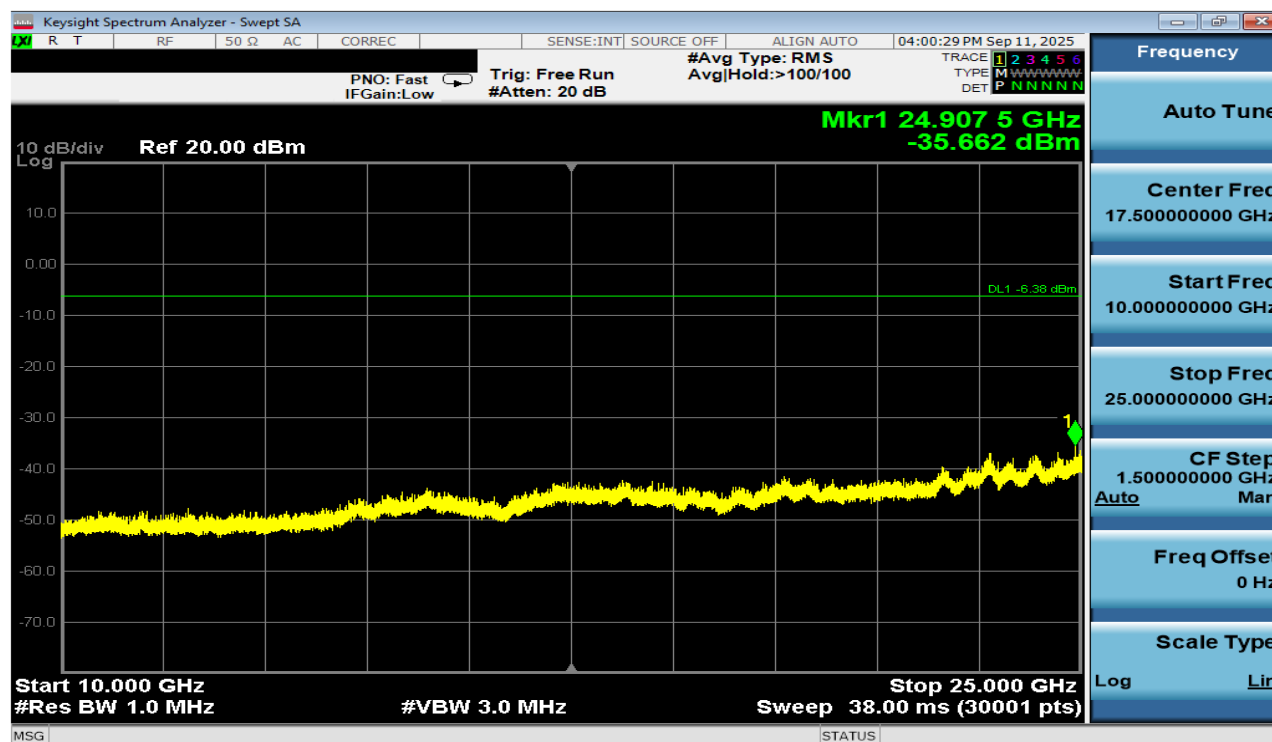
Plot 7-242. Conducted Spurious Plot Antenna 3a (Bluetooth (HDR4), 4 Mbps, ePA – Ch. 1)
