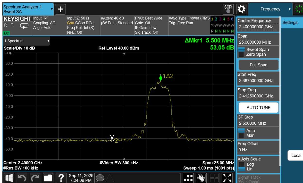
Plot 7-229. Band Edge Plot Antenna 1a (Bluetooth (HDR4), ePA – Ch. 1)
