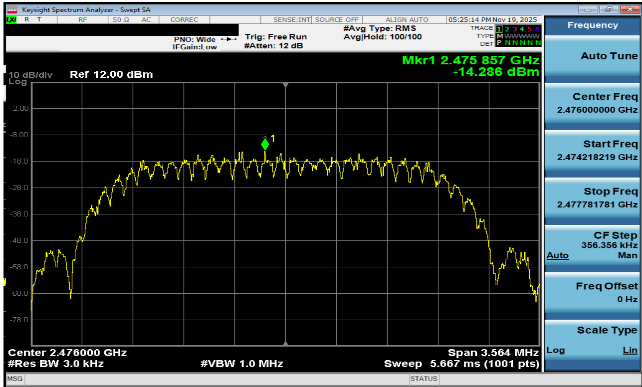
Plot 7-215. Power Spectral Density Plot TxBF Antenna 3a (Bluetooth (HDT2), 2Mbps, iPA – Ch. 73)
