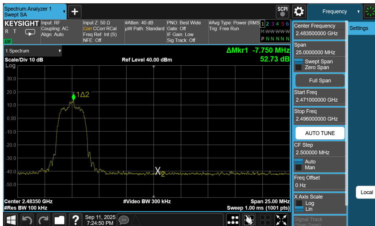
Plot 7-230. Band Edge Plot Antenna 1a (Bluetooth (HDR4), ePA – Ch. 73)
