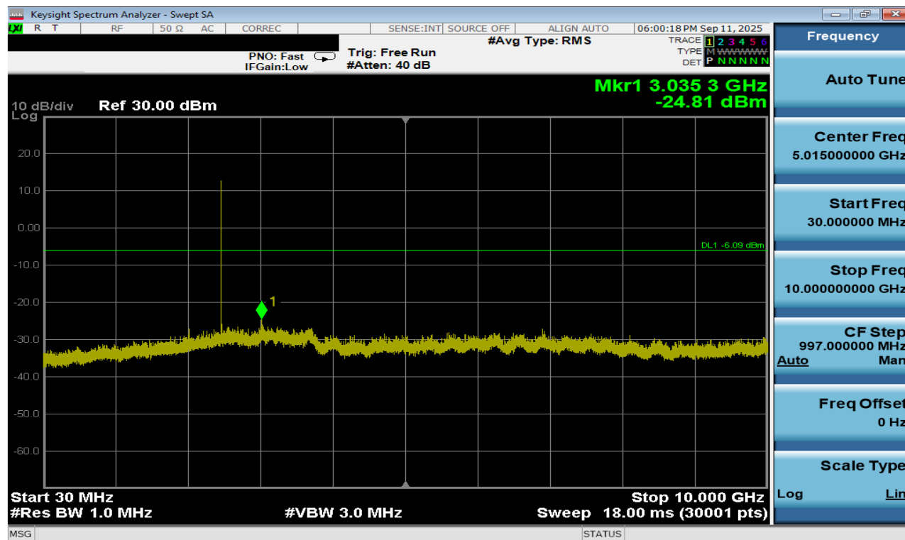
Plot 7-263. Conducted Spurious Plot Antenna 3a (Bluetooth (HDRPM16), 16Mbps, ePA – Ch. 73)
