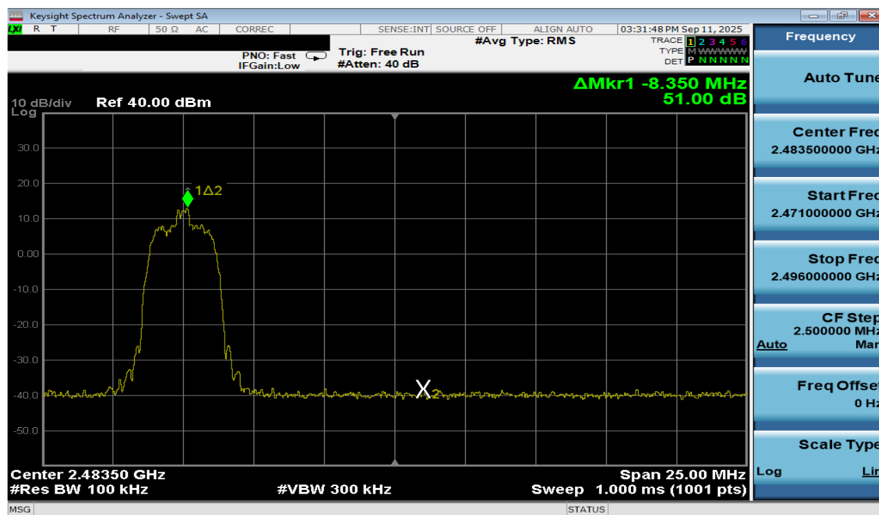
Plot 7-218. Band Edge Plot Antenna 3a (Bluetooth (HDR4), ePA – Ch. 73)
