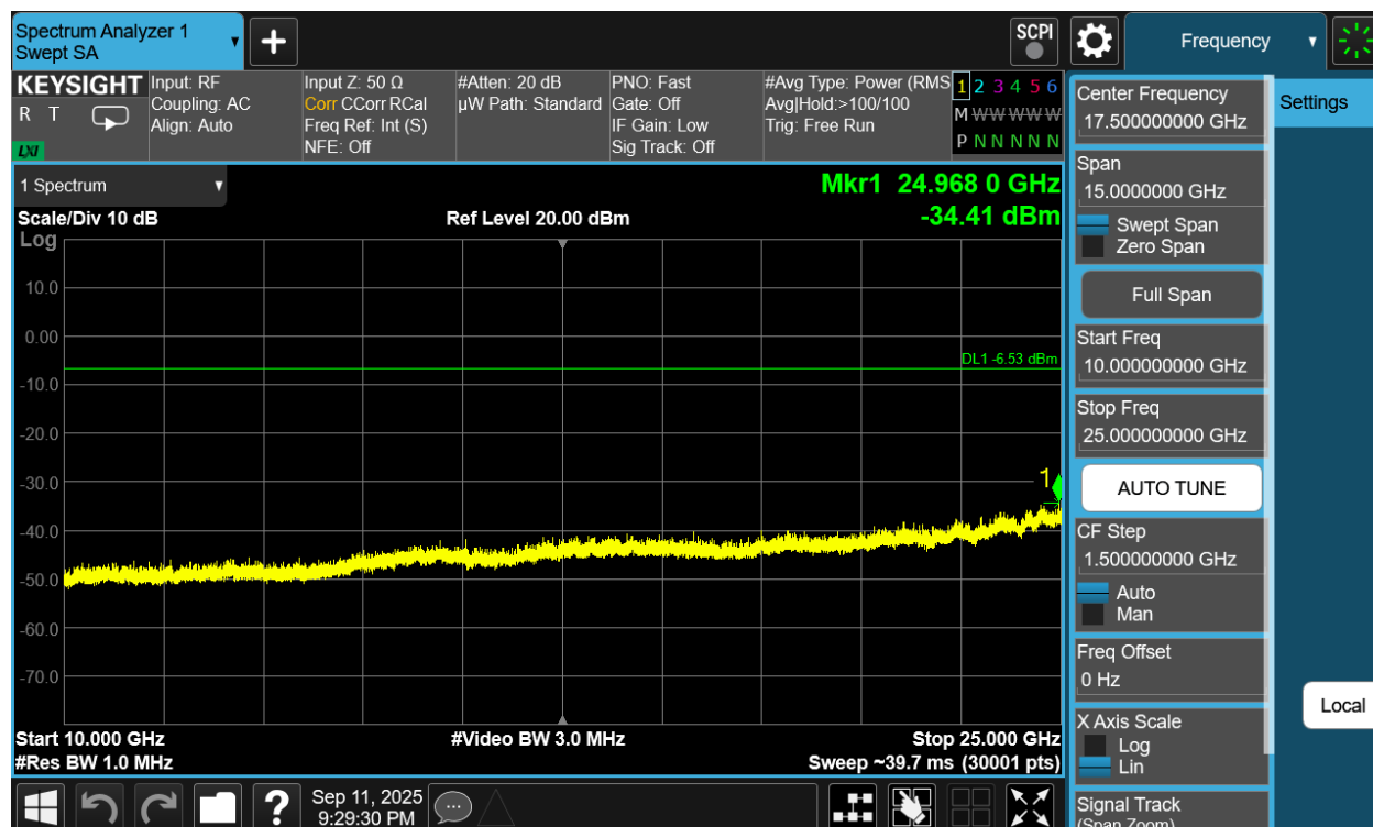
Plot 7-284. Conducted Spurious Plot Antenna 1a (Bluetooth (XHDRPM6), 6Mbps, ePA – Ch. 1)
