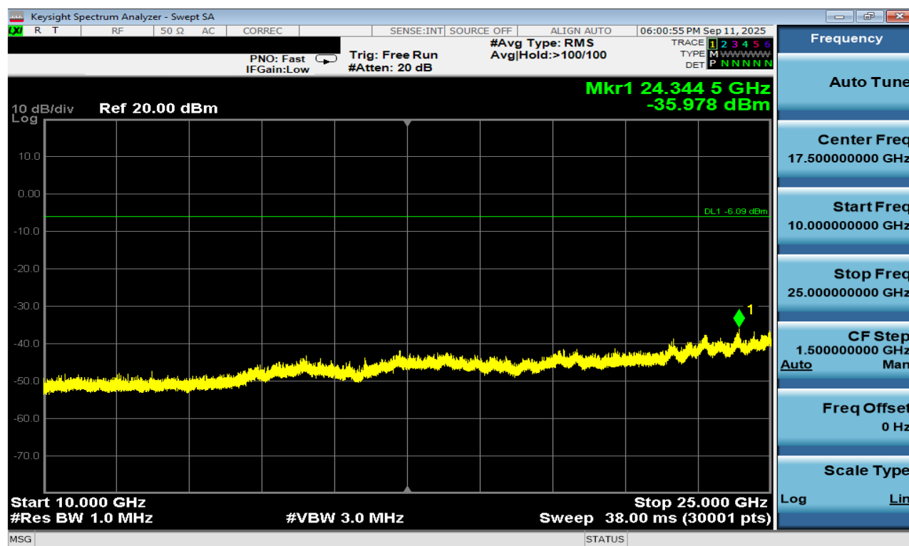
Plot 7-264. Conducted Spurious Plot Antenna 3a (Bluetooth (HDRPM16), 16Mbps, ePA – Ch. 73)
