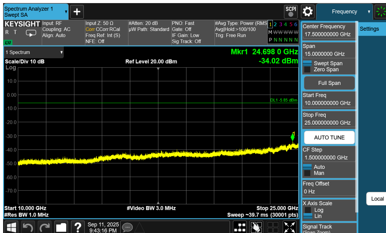
Plot 7-290. Conducted Spurious Plot Antenna 1a (Bluetooth (HDRPM16), 16Mbps, ePA – Ch. 1)
