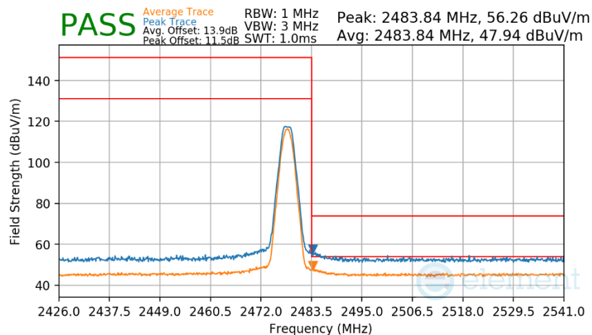
Plot 7-188. Radiated Restricted Upper Band Edge Measurement TxBF (Average & Peak)
