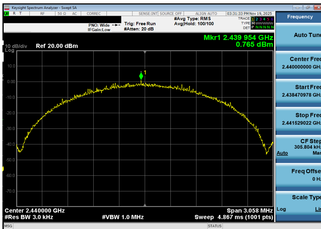
Plot 7-135. Power Spectral Density Plot Antenna 3a (Bluetooth (LE), 2Mbps, ePA – Ch. 19)
