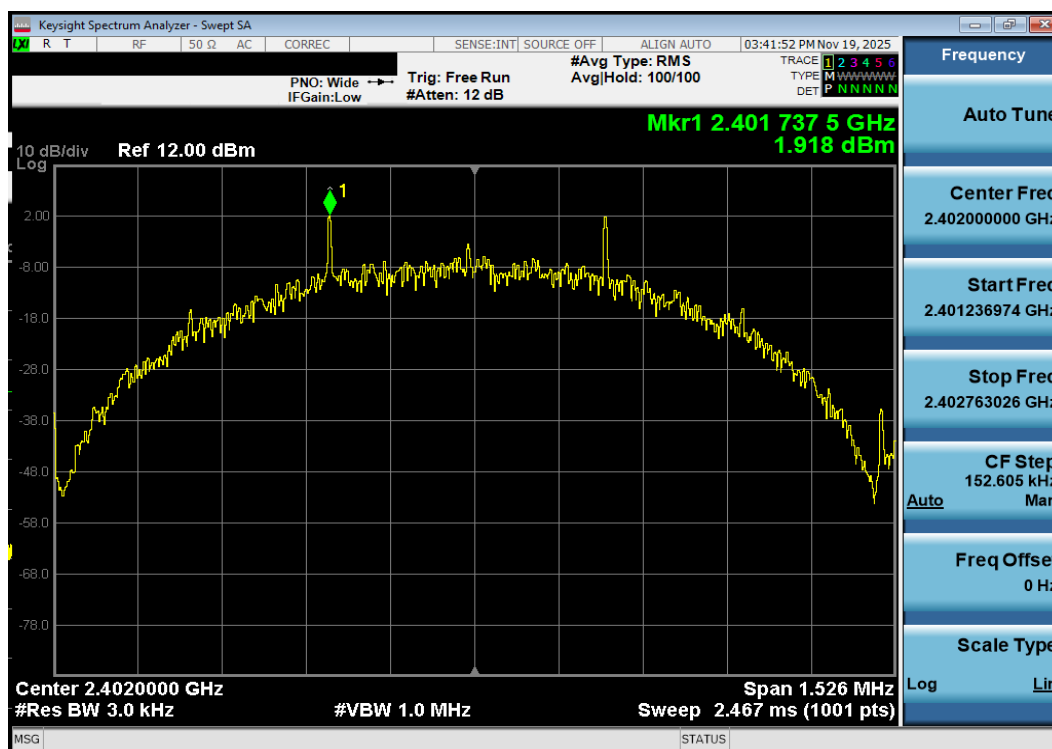
Plot 7-115. Power Spectral Density Plot Antenna 3a (Bluetooth (LE), 500kbps, iPA – Ch. 0)
