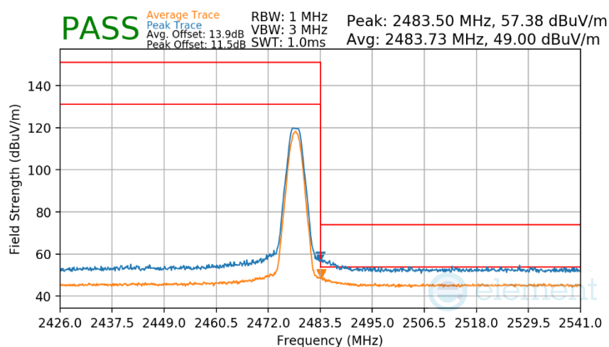
Plot 7-180. Radiated Restricted Upper Band Edge Measurement Antenna 3a (Average & Peak)
