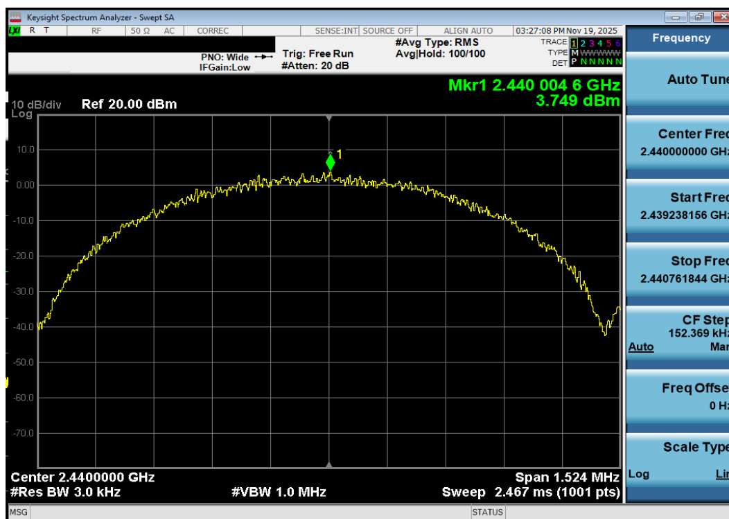
Plot 7-123. Power Spectral Density Plot Antenna 3a (Bluetooth (LE), 1Mbps, ePA – Ch. 19)
