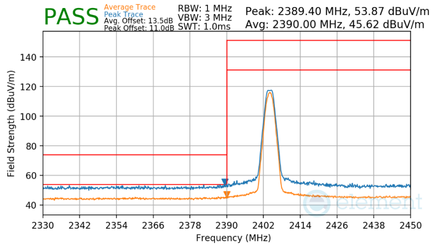
Plot 7-183. Radiated Restricted Lower Band Edge Measurement Antenna 1a (Average & Peak)
