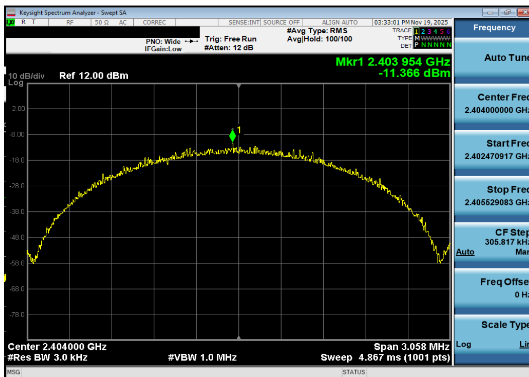
Plot 7-139. Power Spectral Density Plot Antenna 3a (Bluetooth (LE), 2Mbps, iPA – Ch. 1)
