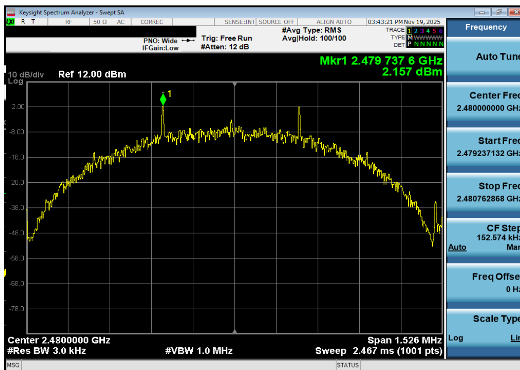
Plot 7-119. Power Spectral Density Plot Antenna 3a (Bluetooth (LE), 500kbps, iPA – Ch. 39)
