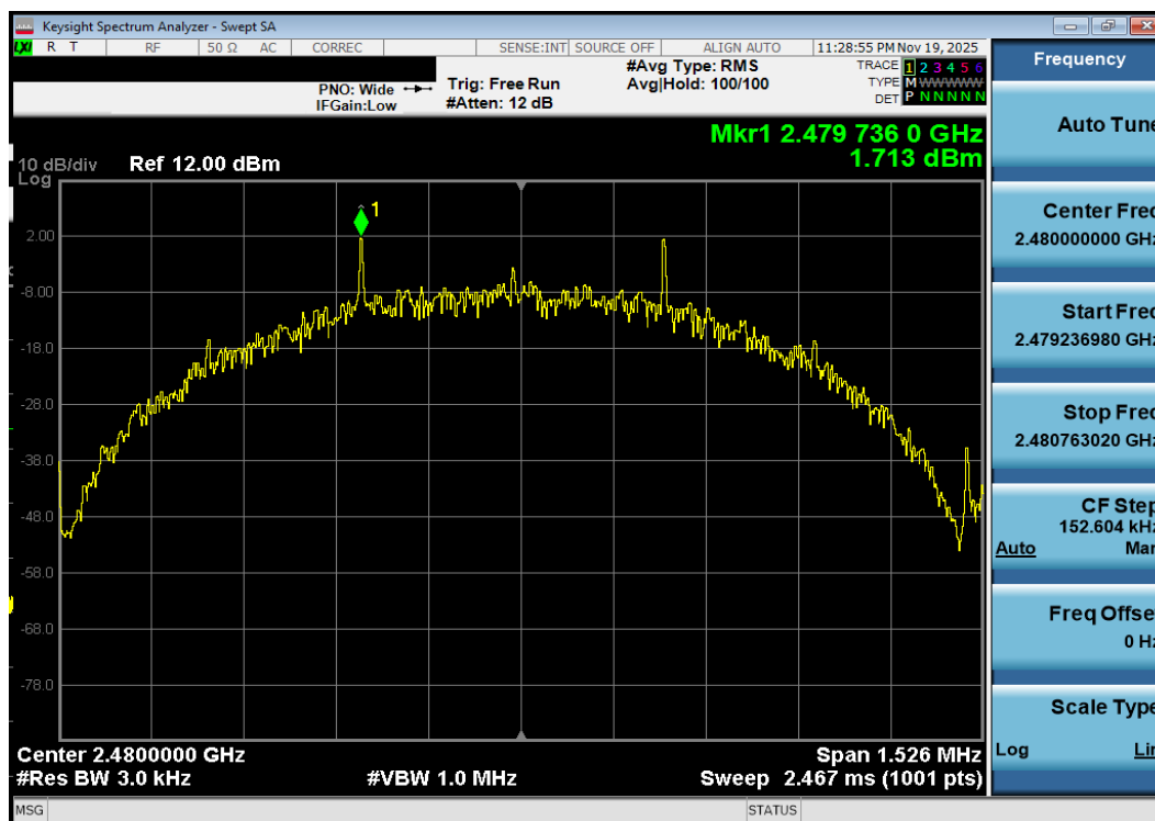
Plot 7-120. Power Spectral Density Plot Antenna 1a (Bluetooth (LE), 500kbps, iPA – Ch. 39)
