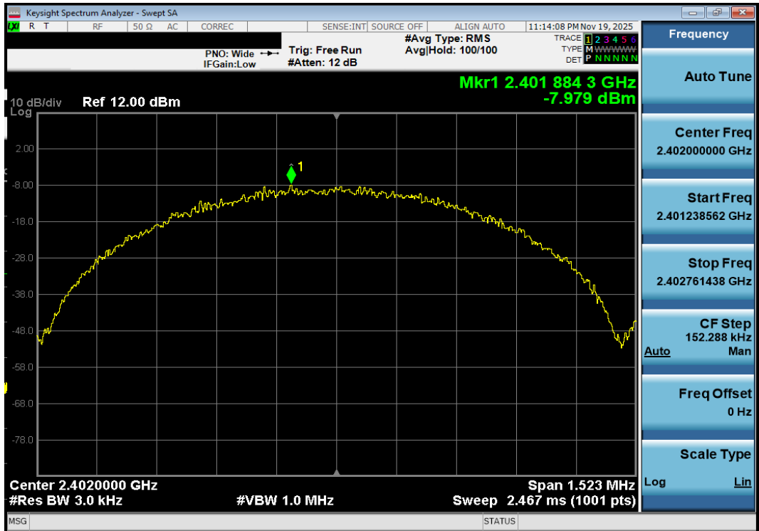
Plot 7-128. Power Spectral Density Plot Antenna 1a (Bluetooth (LE), 1Mbps, iPA – Ch. 0)
