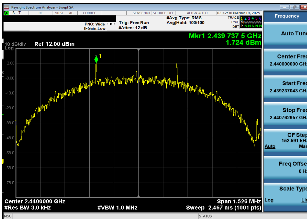
Plot 7-117. Power Spectral Density Plot Antenna 3a (Bluetooth (LE), 500kbps, iPA – Ch. 19)
