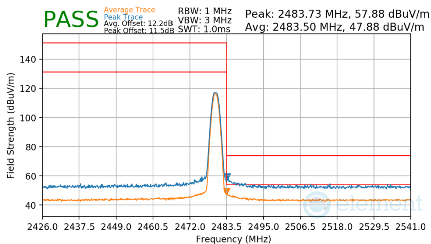
Plot 7-182. Radiated Restricted Upper Band Edge Measurement Antenna 1a (Average & Peak)
