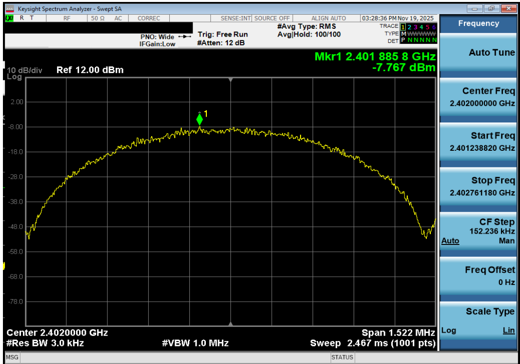
Plot 7-127. Power Spectral Density Plot Antenna 3a (Bluetooth (LE), 1Mbps, iPA – Ch. 0)
