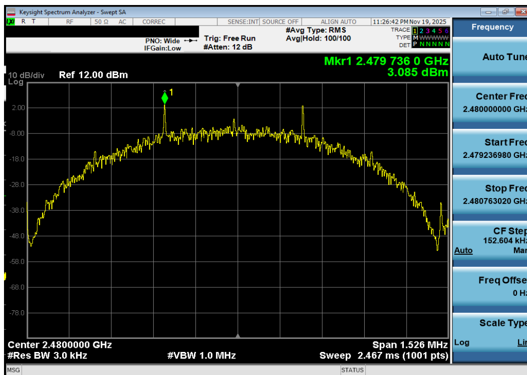
Plot 7-114. Power Spectral Density Plot Antenna 1a (Bluetooth (LE), 500kbps, ePA – Ch. 39)
