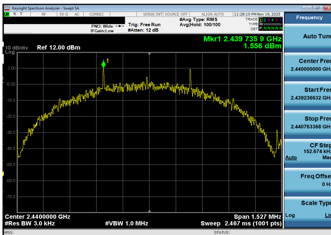
Plot 7-118. Power Spectral Density Plot Antenna 1a (Bluetooth (LE), 500kbps, iPA – Ch. 19)
