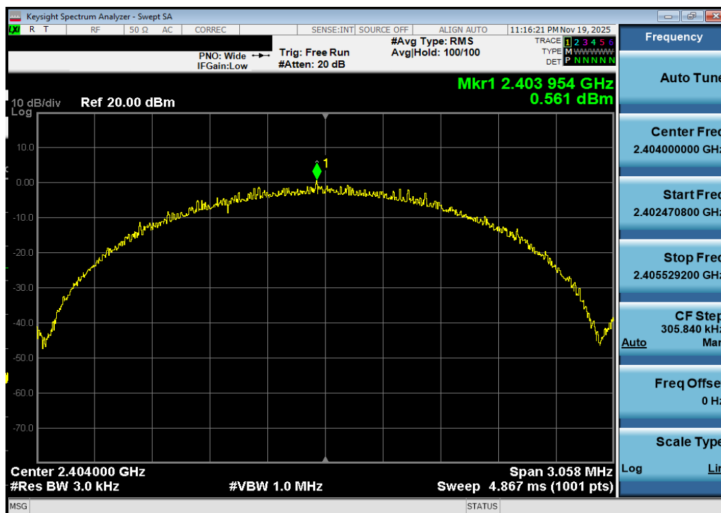
Plot 7-134. Power Spectral Density Plot Antenna 1a (Bluetooth (LE), 2Mbps, ePA – Ch. 1)
