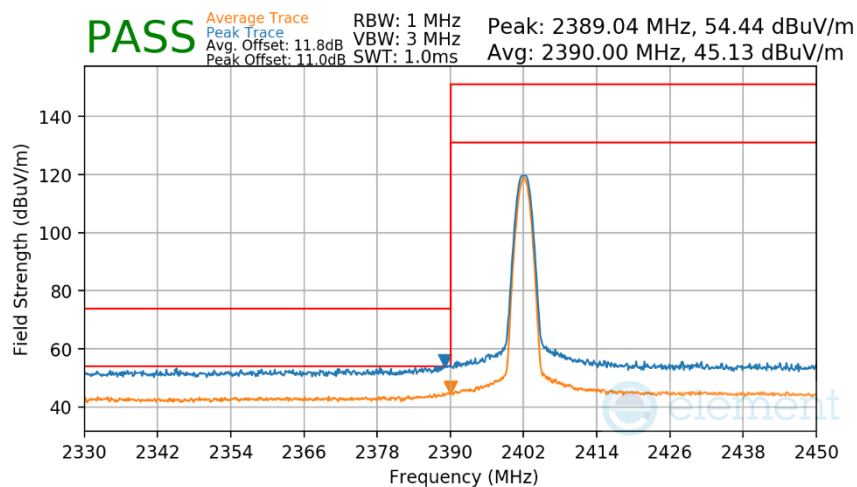
Plot 7-177. Radiated Restricted Lower Band Edge Measurement Antenna 3a (Average & Peak)
