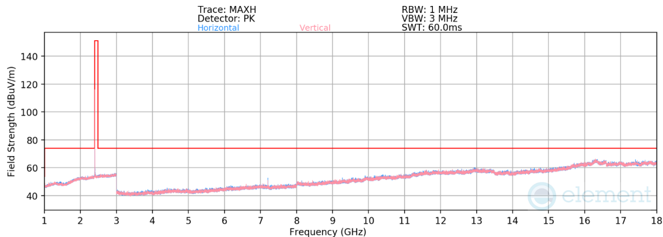
Plot 7-173. Radiated Spurious Emissions 1-18GHz TxBF (1Mbps, ePA – Ch. 0)
