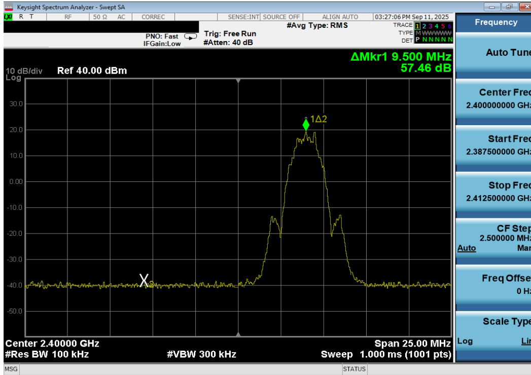
Plot 7-151. Band Edge Plot Antenna 3a (Bluetooth (LE), 2Mbps, ePA – Ch. 1)
