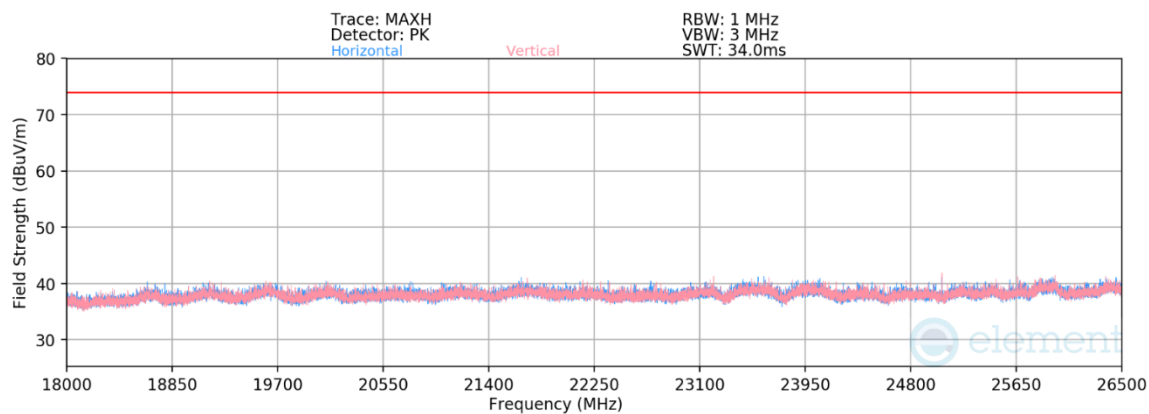
Plot 7-175. Radiated Spurious Emissions Above 18GHz TxBF (1Mbps ePA – Ch. 19)
