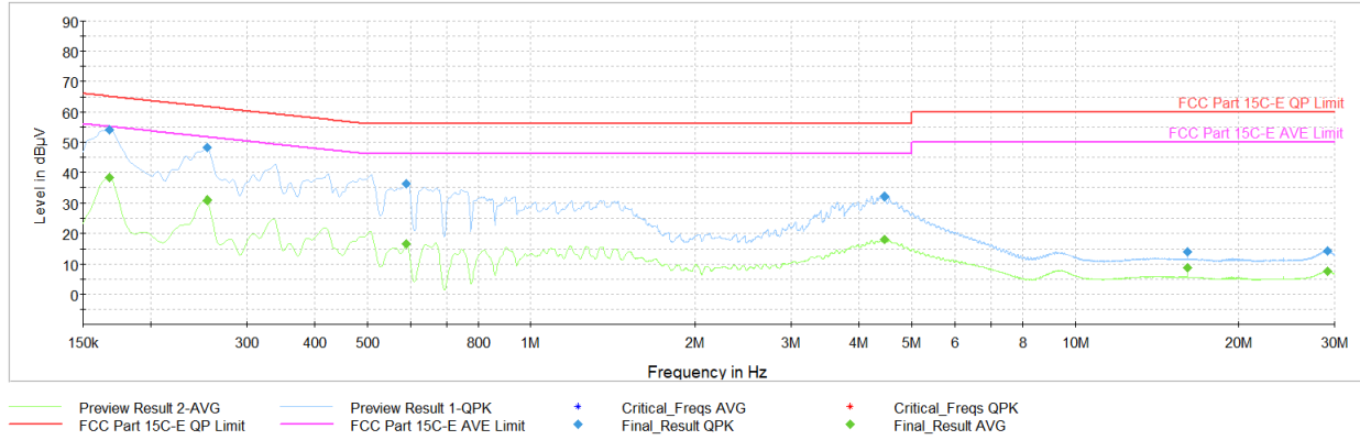
Plot 7-191. AC Line Conducted Plot with Bluetooth LE TxBF (N, 1Mbps ePA – Ch.19, with AC/DC Adapter)
