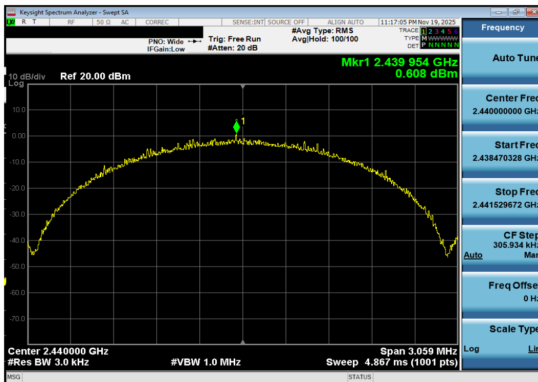
Plot 7-136. Power Spectral Density Plot Antenna 1a (Bluetooth (LE), 2Mbps, ePA – Ch. 19)
