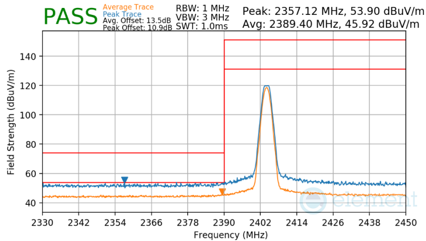
Plot 7-187. Radiated Restricted Lower Band Edge Measurement TxBF (Average & Peak)
