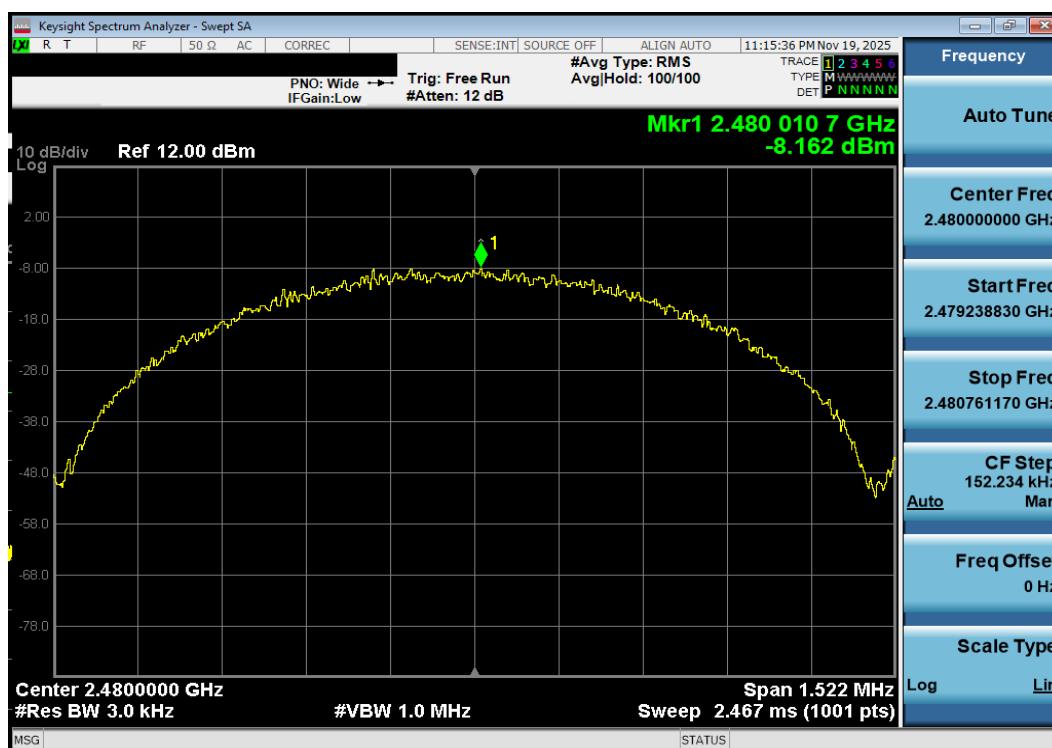
Plot 7-132. Power Spectral Density Plot Antenna 1a (Bluetooth (LE), 1Mbps, iPA – Ch. 39)
