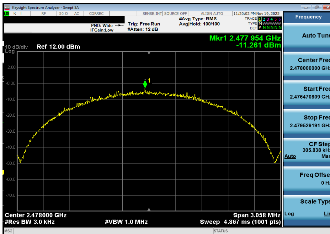
Plot 7-144. Power Spectral Density Plot Antenna 1a (Bluetooth (LE), 2Mbps, iPA – Ch. 38)
