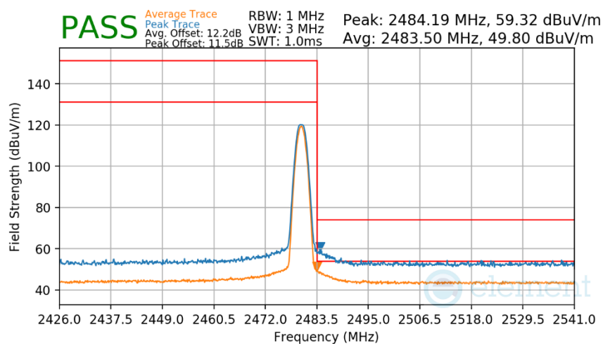
Plot 7-178. Radiated Restricted Upper Band Edge Measurement Antenna 3a (Average & Peak)
