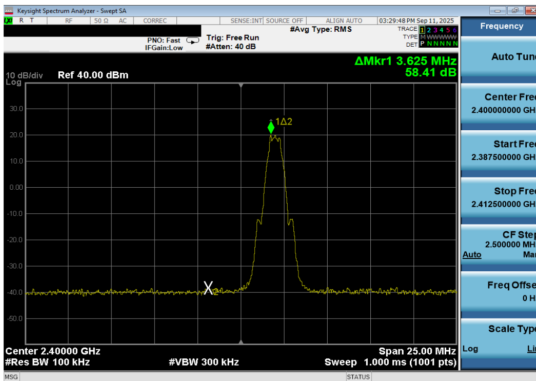
Plot 7-147. Band Edge Plot Antenna 3a (Bluetooth (LE), 500kbps, ePA – Ch.0)
