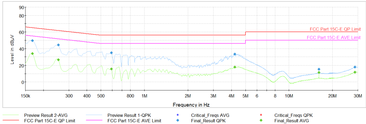
Plot 7-190. AC Line Conducted Plot with Bluetooth LE Tx BF (L1, 1Mbps ePA – Ch.19 with AC/DC Adapter)
