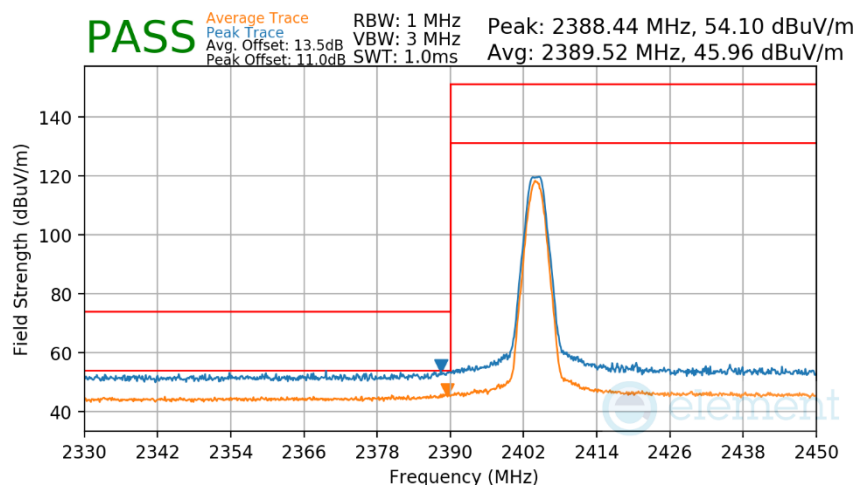
Plot 7-179. Radiated Restricted Lower Band Edge Measurement Antenna 3a (Average & Peak)
