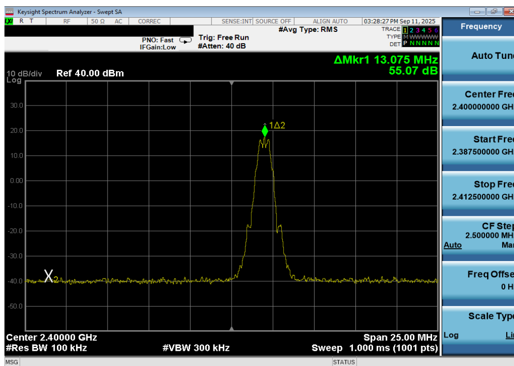
Plot 7-145. Band Edge Plot Antenna 3a (Bluetooth (LE), 125kbps, ePA – Ch.0)
