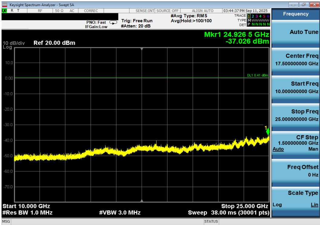
Plot 7-164. Conducted Spurious Plot Antenna 3a (Bluetooth (LE), 1Mbps, ePA – Ch. 19)
