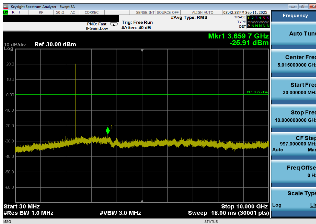
Plot 7-161. Conducted Spurious Plot Antenna 3a (Bluetooth (LE), 1Mbps, ePA – Ch. 0)
