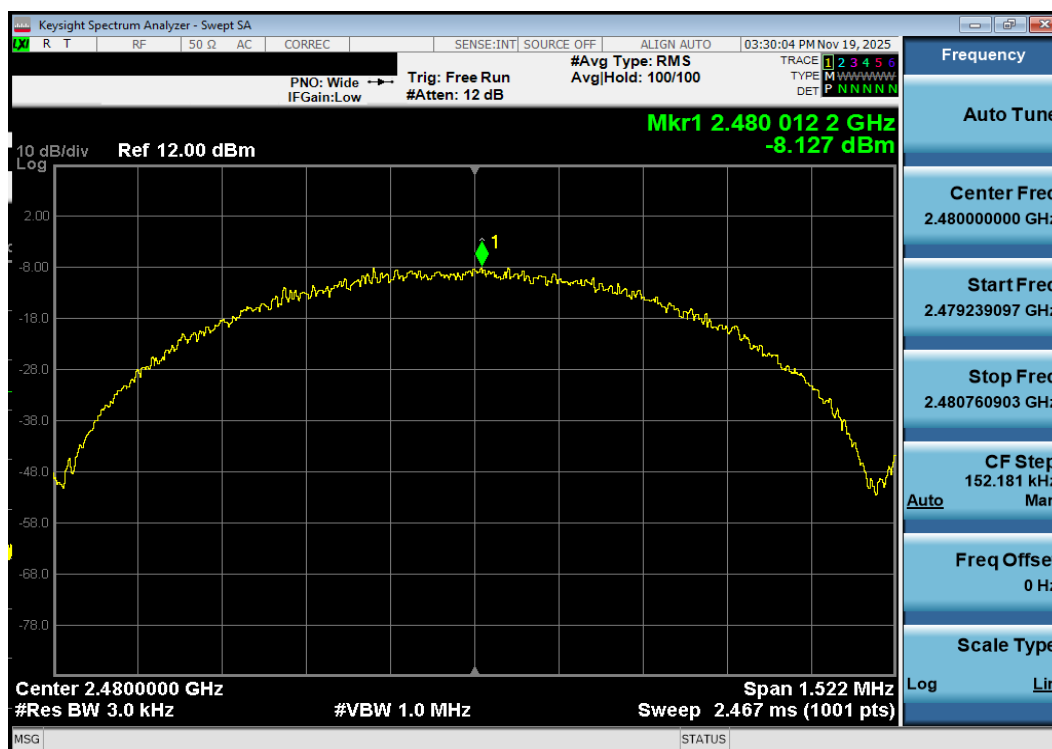
Plot 7-131. Power Spectral Density Plot Antenna 3a (Bluetooth (LE), 1Mbps, iPA – Ch. 39)
