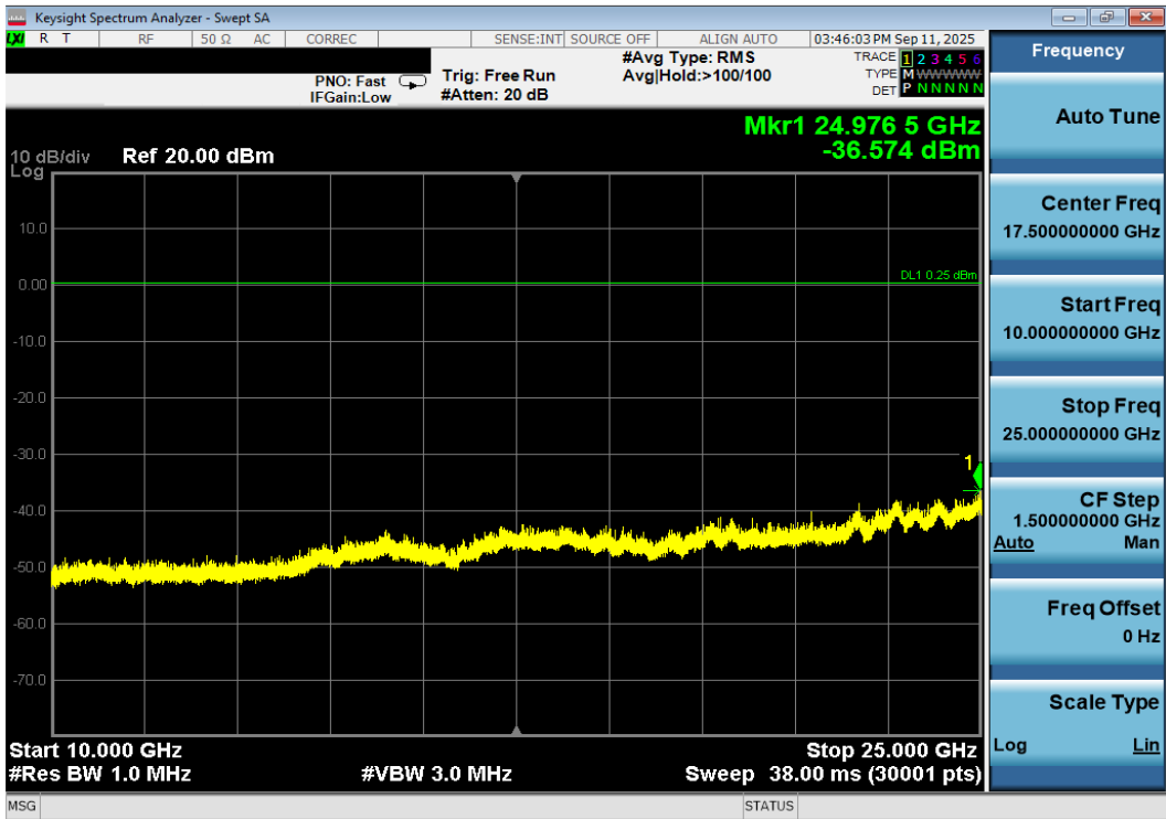
Plot 7-166. Conducted Spurious Plot Antenna 3a (Bluetooth (LE), 1Mbps, ePA – Ch. 39)
