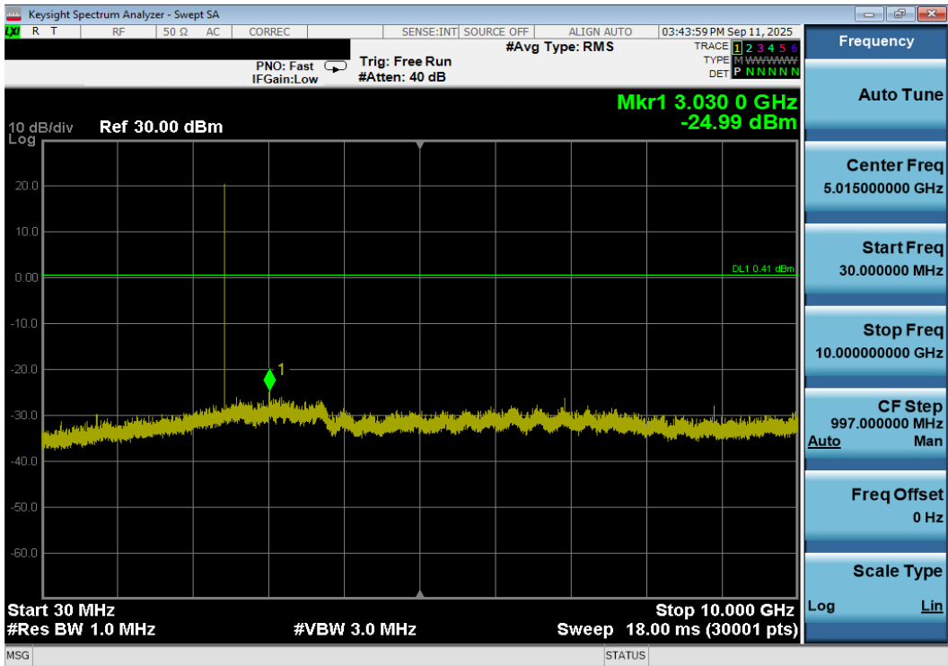
Plot 7-163. Conducted Spurious Plot Antenna 3a (Bluetooth (LE), 1Mbps, ePA – Ch. 19)
