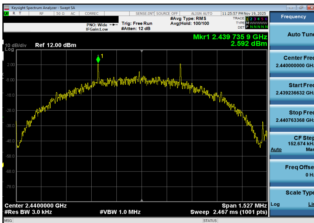
Plot 7-112. Power Spectral Density Plot Antenna 1a (Bluetooth (LE), 500kbps, ePA – Ch. 19)
