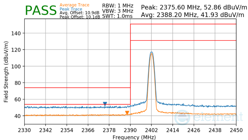
Plot 7-181. Radiated Restricted Lower Band Edge Measurement Antenna 1a (Average & Peak)
