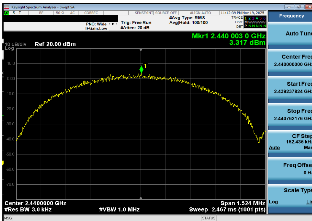
Plot 7-124. Power Spectral Density Plot Antenna 1a (Bluetooth (LE), 1Mbps, ePA – Ch. 19)
