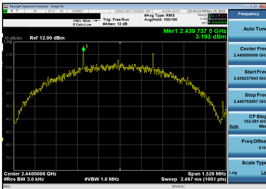
Plot 7-111. Power Spectral Density Plot Antenna 3a (Bluetooth (LE), 500kbps, ePA – Ch. 19)
