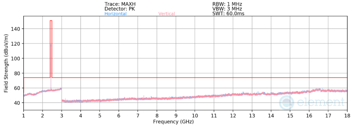
Plot 7-174. Radiated Spurious Emissions 1-18GHz TxBF (1Mbps, ePA – Ch. 19)
