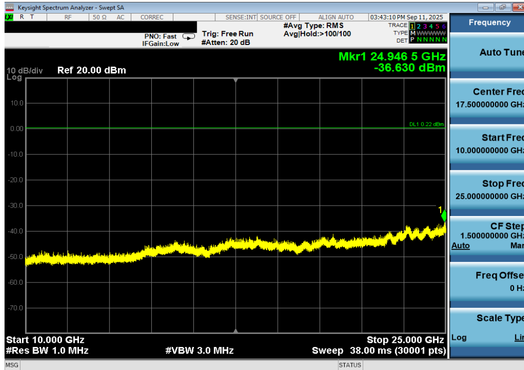
Plot 7-162. Conducted Spurious Plot Antenna 3a (Bluetooth (LE), 1Mbps, ePA – Ch. 0)
