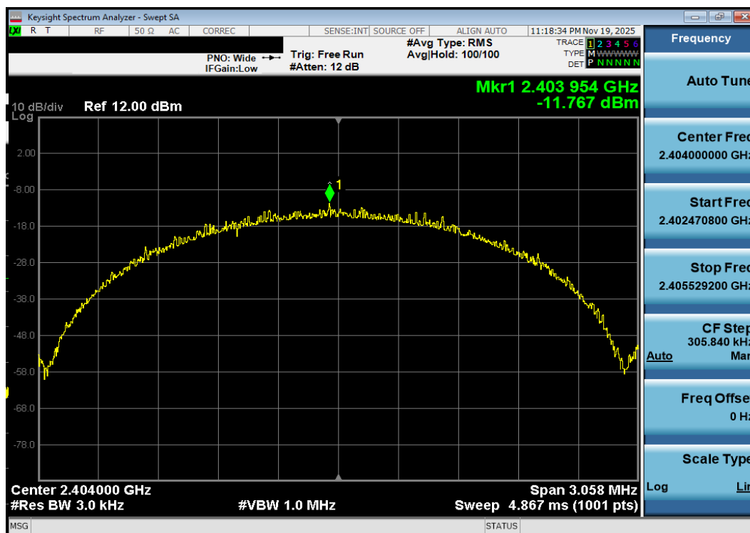
Plot 7-140. Power Spectral Density Plot Antenna 1a (Bluetooth (LE), 2Mbps, iPA – Ch. 1)
