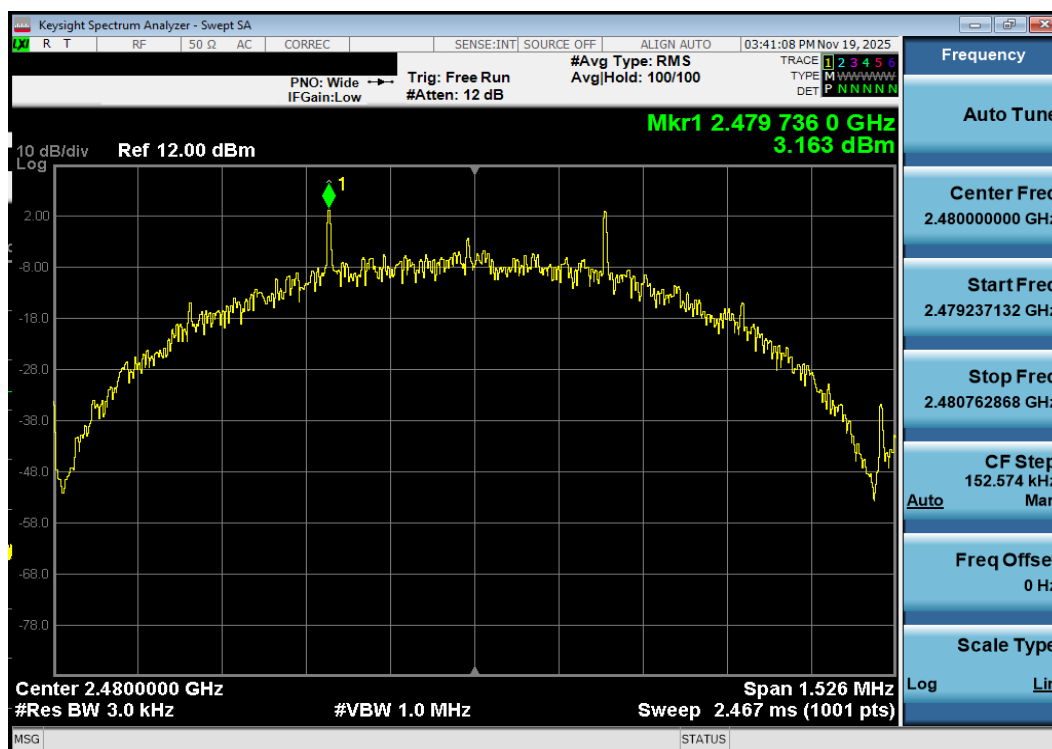
Plot 7-113. Power Spectral Density Plot Antenna 3a (Bluetooth (LE), 500kbps, ePA – Ch. 39)
