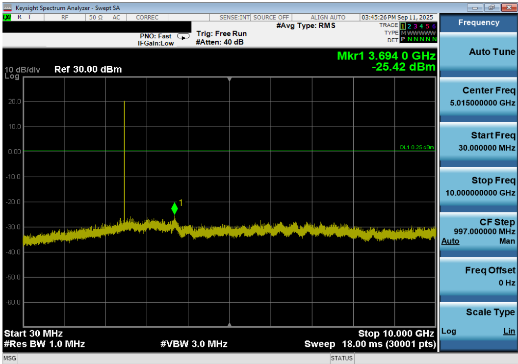
Plot 7-165. Conducted Spurious Plot Antenna 3a (Bluetooth (LE), 1Mbps, ePA – Ch. 39)
