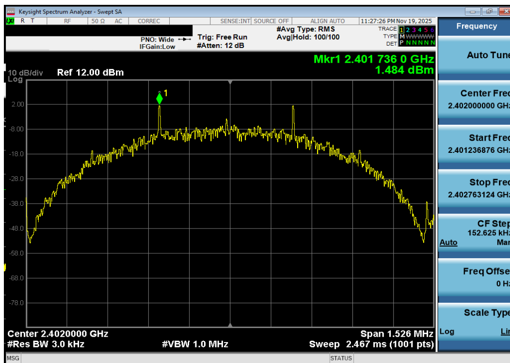
Plot 7-116. Power Spectral Density Plot Antenna 1a (Bluetooth (LE), 500kbps, iPA – Ch. 0)
