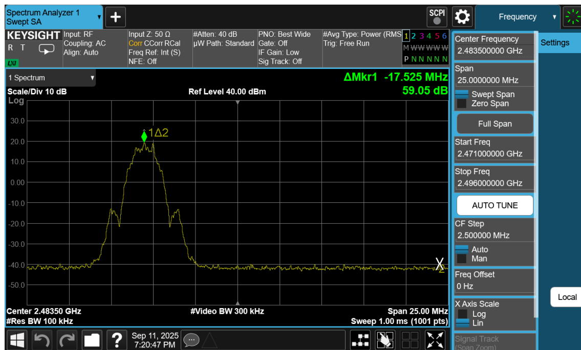
Plot 7-160. Band Edge Plot Antenna 1a (Bluetooth (LE), 2Mbps, ePA – Ch. 38)
