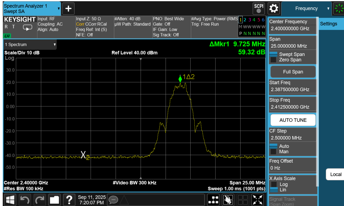
Plot 7-159. Band Edge Plot Antenna 1a (Bluetooth (LE), 2Mbps, ePA – Ch. 1)
