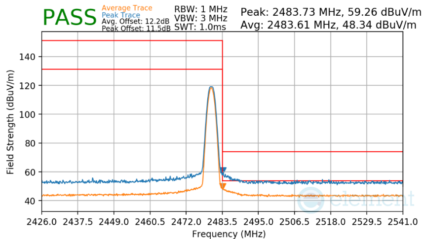
Plot 7-186. Radiated Restricted Upper Band Edge Measurement TxBF (Average & Peak)
