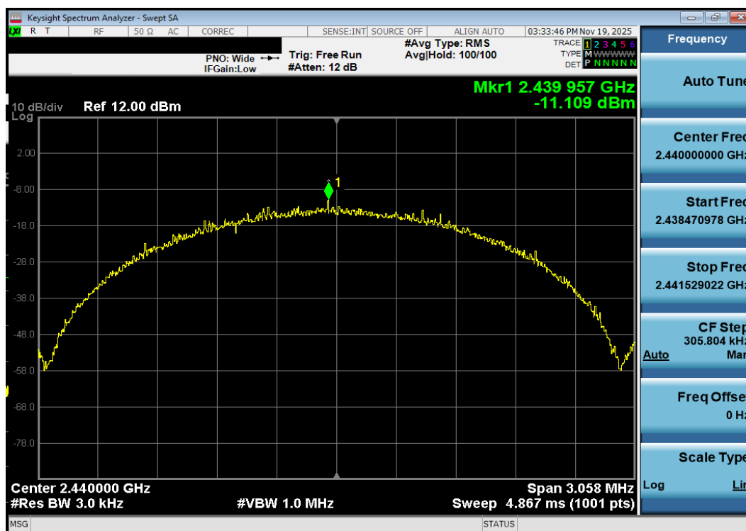
Plot 7-141. Power Spectral Density Plot Antenna 3a (Bluetooth (LE), 2Mbps, iPA – Ch. 19)
