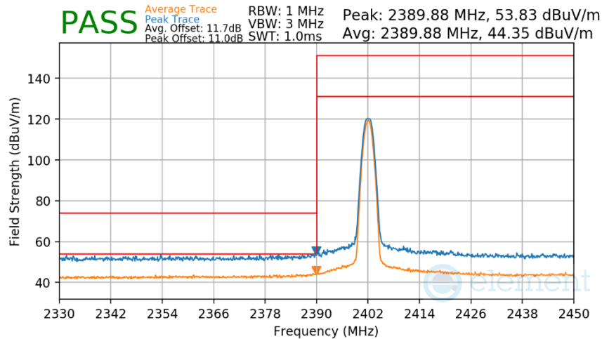
Plot 7-185. Radiated Restricted Lower Band Edge Measurement TxBF (Average & Peak)
