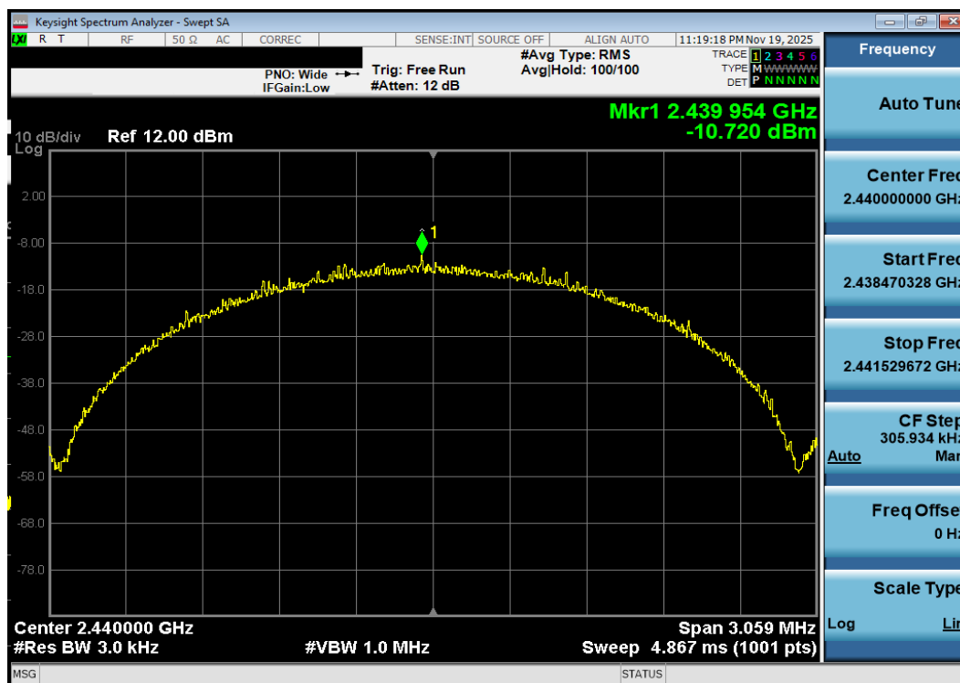
Plot 7-142. Power Spectral Density Plot Antenna 1a (Bluetooth (LE), 2Mbps, iPA – Ch. 19)
