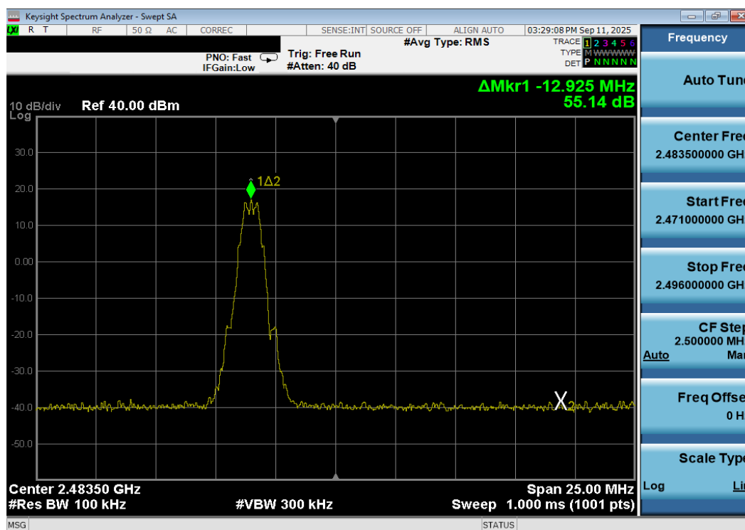
Plot 7-146. Band Edge Plot Antenna 3a (Bluetooth (LE), 125kbps, ePA – Ch. 39)
