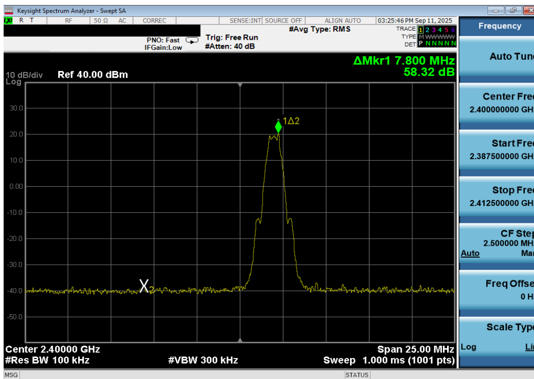
Plot 7-149. Band Edge Plot Antenna 3a (Bluetooth (LE), 1Mbps, ePA – Ch.0)
