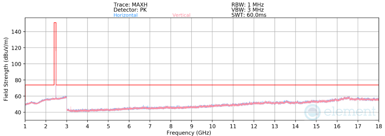
Plot 7-176. Radiated Spurious Emissions 1-18GHz TxBF (1Mbps ePA – Ch. 39)
