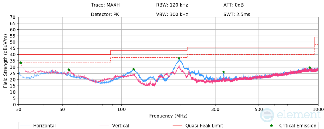
Plot 7-189. Radiated Spurious Emissions Below 1GHz TxBF (1Mbps, ePA – Ch.19, Pol. H & V, with AC/DC Adapter)
