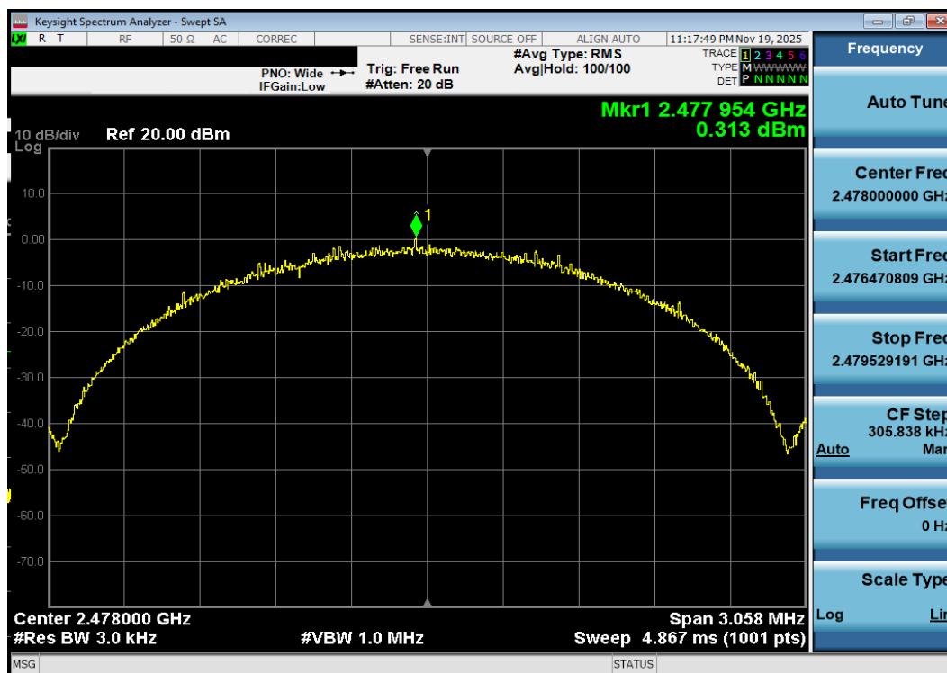
Plot 7-138. Power Spectral Density Plot Antenna 1a (Bluetooth (LE), 2Mbps, ePA – Ch. 38)
