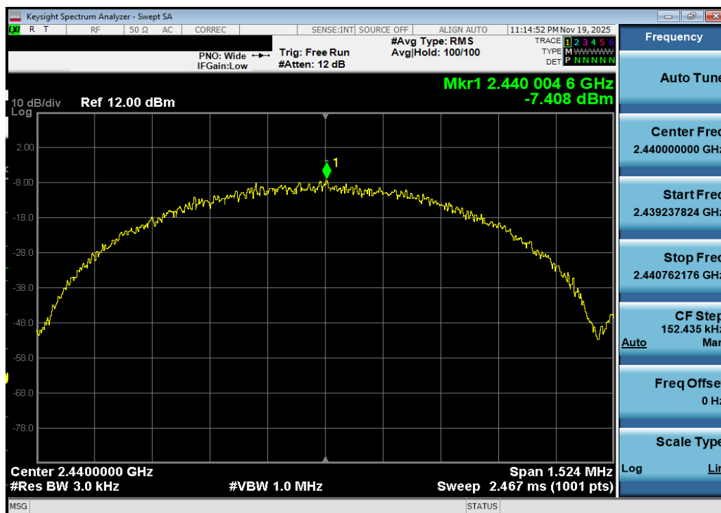
Plot 7-130. Power Spectral Density Plot Antenna 1a (Bluetooth (LE), 1Mbps, iPA – Ch. 19)
