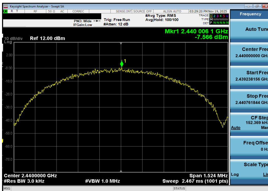
Plot 7-129. Power Spectral Density Plot Antenna 3a (Bluetooth (LE), 1Mbps, iPA – Ch. 19)
