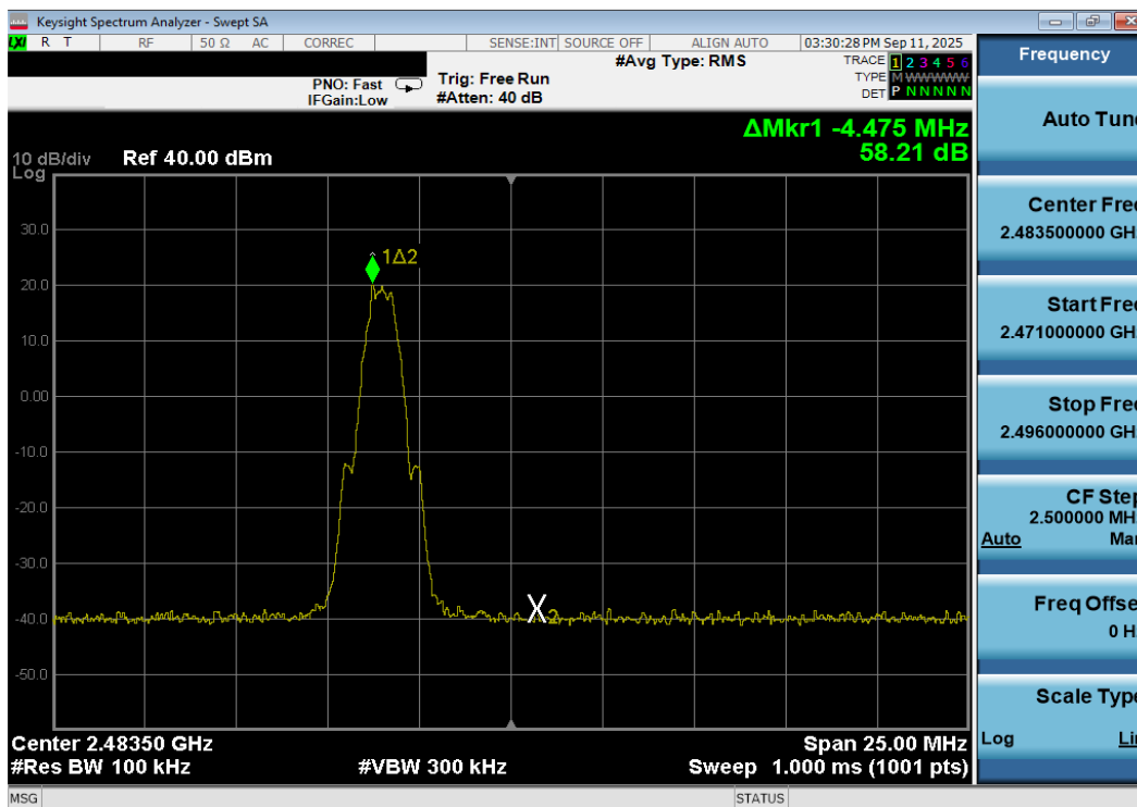
Plot 7-148. Band Edge Plot Antenna 3a (Bluetooth (LE), 500kbps, ePA – Ch. 39)
