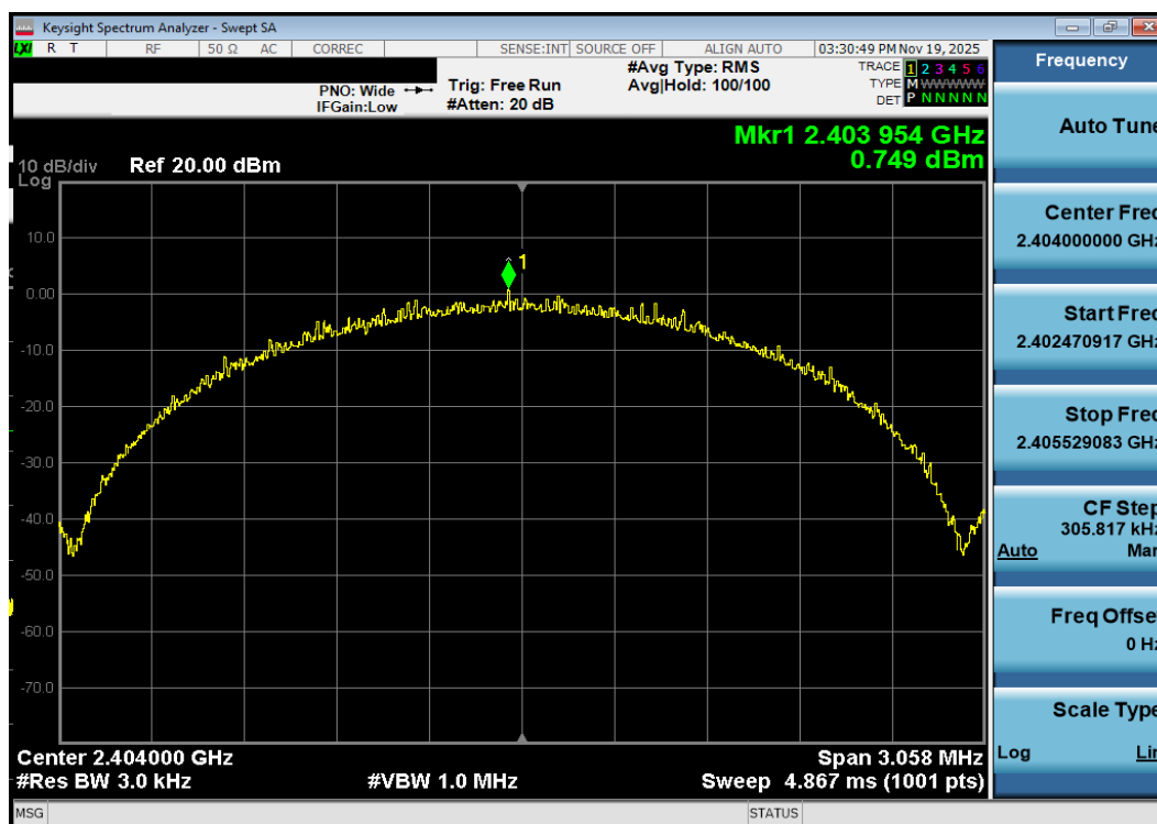
Plot 7-133. Power Spectral Density Plot Antenna 3a (Bluetooth (LE), 2Mbps, ePA – Ch. 1)
