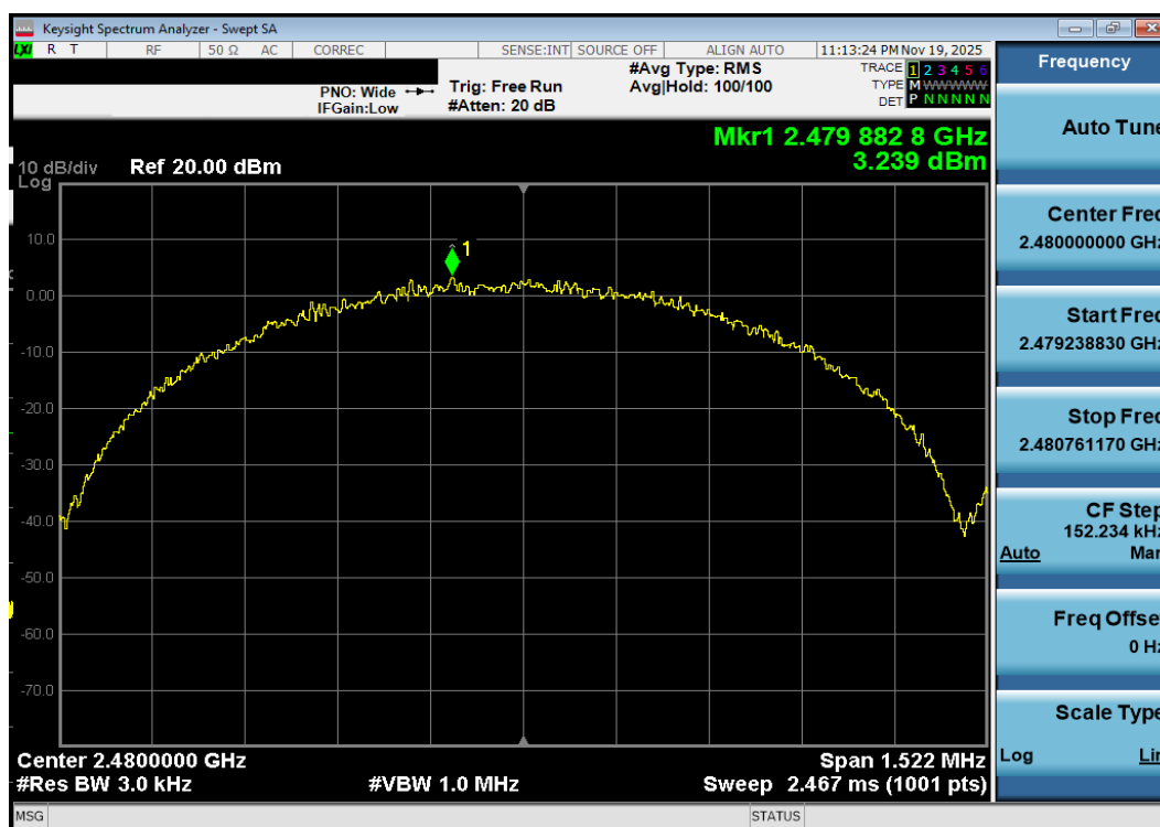
Plot 7-126. Power Spectral Density Plot Antenna 1a (Bluetooth (LE), 1Mbps, ePA – Ch. 39)
