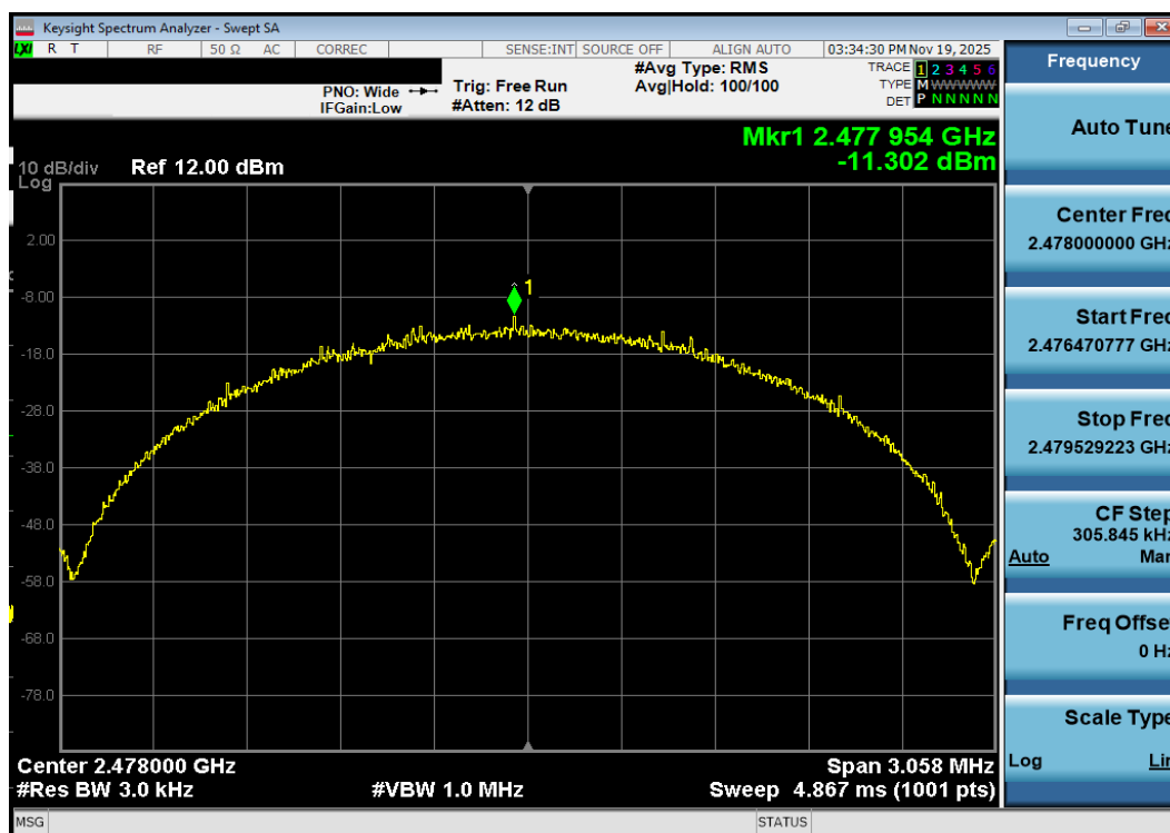
Plot 7-143. Power Spectral Density Plot Antenna 3a (Bluetooth (LE), 2Mbps, iPA – Ch. 38)
