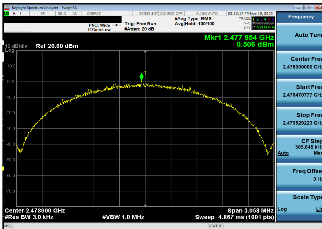
Plot 7-137. Power Spectral Density Plot Antenna 3a (Bluetooth (LE), 2Mbps, ePA – Ch. 38)
