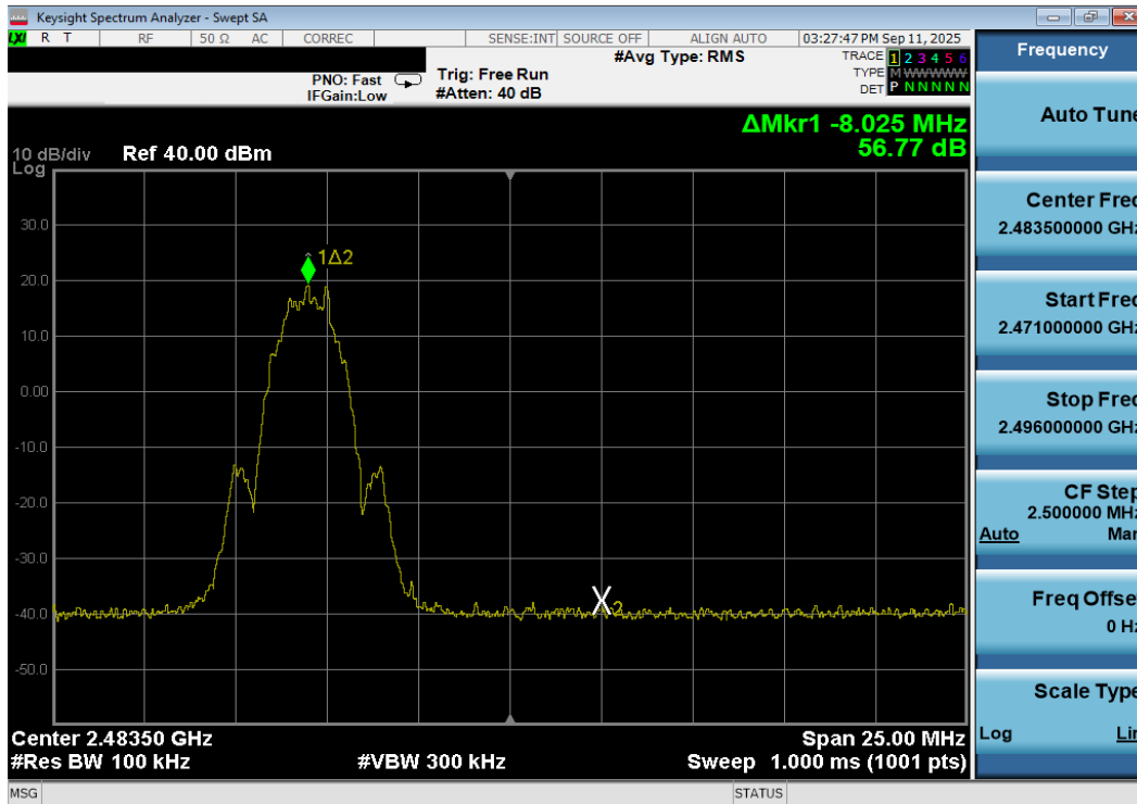
Plot 7-152. Band Edge Plot Antenna 3a (Bluetooth (LE), 2Mbps, ePA – Ch. 38)
