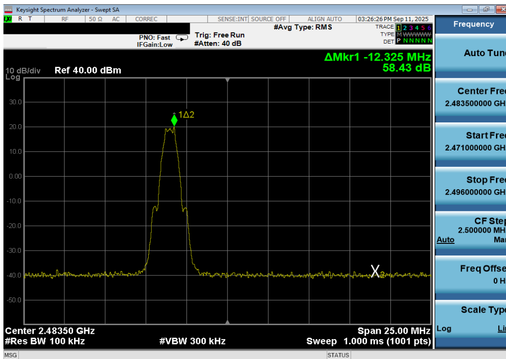
Plot 7-150. Band Edge Plot Antenna 3a (Bluetooth (LE), 1Mbps, ePA – Ch. 39)
