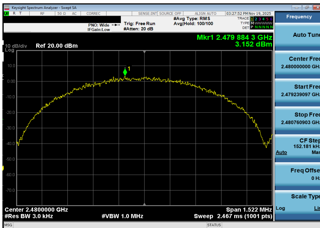
Plot 7-125. Power Spectral Density Plot Antenna 3a (Bluetooth (LE), 1Mbps, ePA – Ch. 39)
