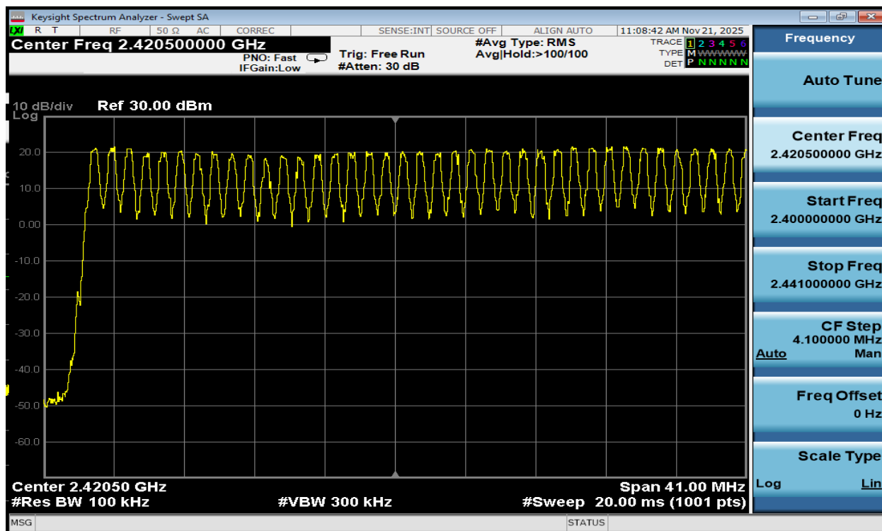
Plot 7-37. Low End Spectrum Channel Hopping Plot Antenna 3a (Bluetooth, GFSK, ePA)
