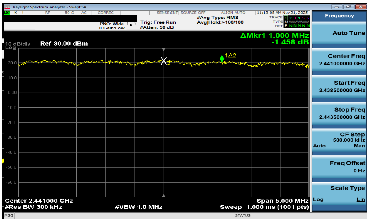
Plot 7-30. Channel Spacing Plot Antenna 3a (Bluetooth, 8DPSK, ePA)
