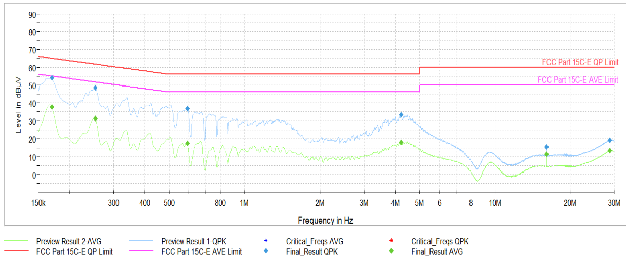
Plot 7-78. AC Line-Conducted Test Plot TxBF (L1, GFSK ePA – Ch.39, with AC/DC Adapter)
