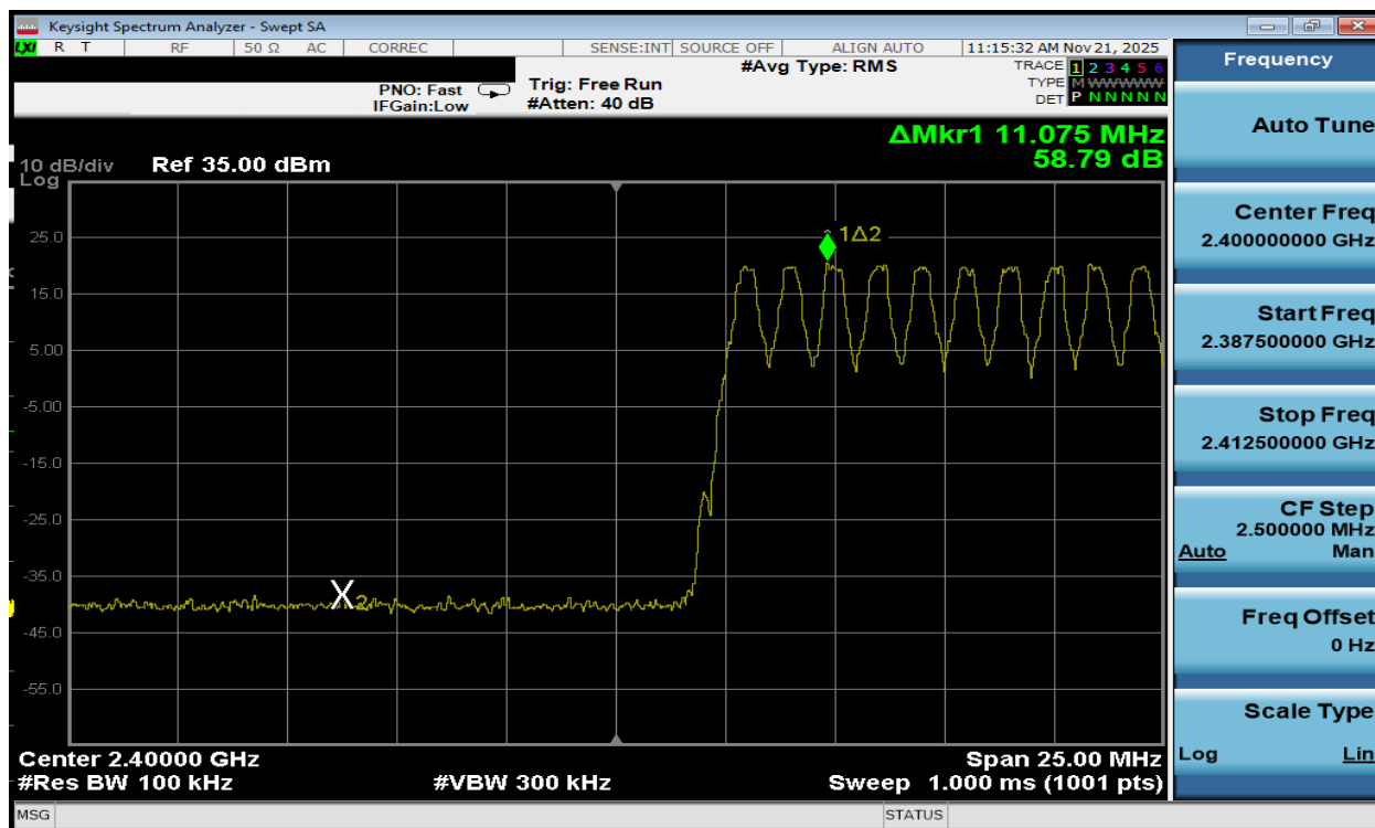
Plot 7-23. Band Edge Plot Antenna 1a (Bluetooth with Hopping Enabled, GFSK, ePA)
