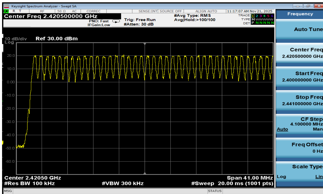
Plot 7-41. Low End Spectrum Channel Hopping Plot Antenna 1a (Bluetooth, GFSK, ePA)
