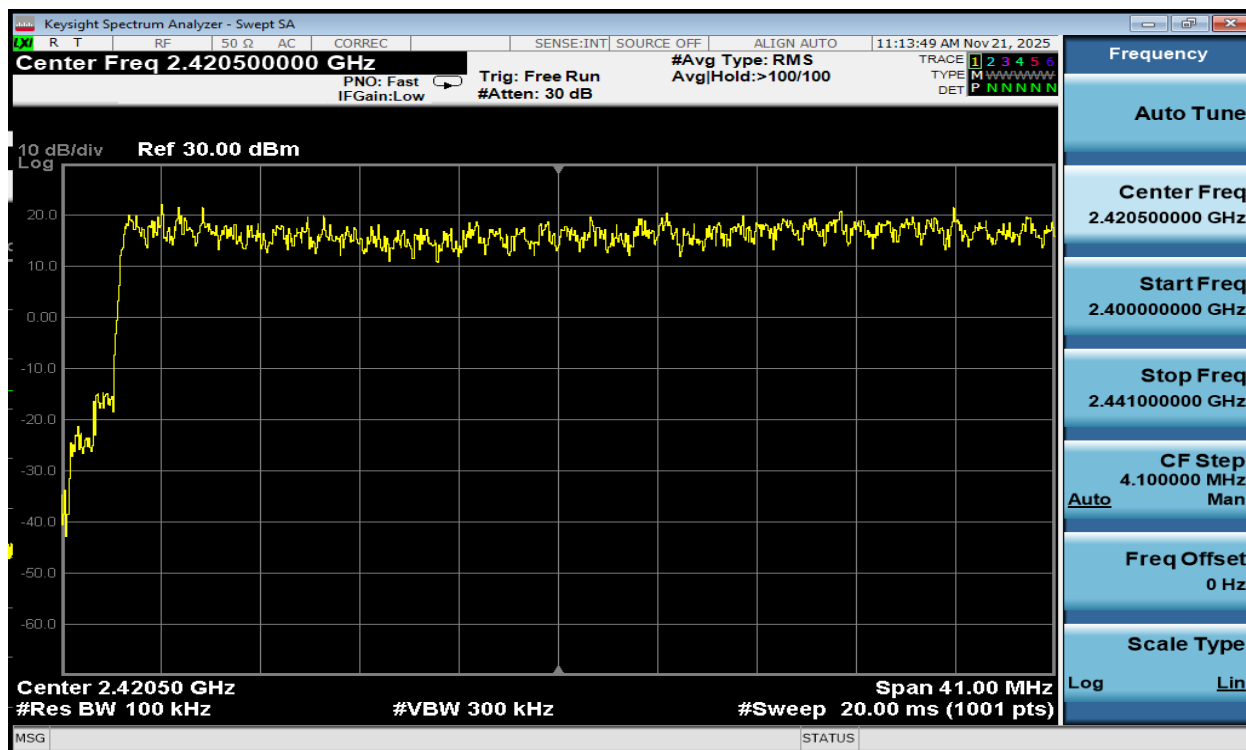
Plot 7-39. Low End Spectrum Channel Hopping Plot Antenna 3a (Bluetooth, 8DPSK, ePA)
