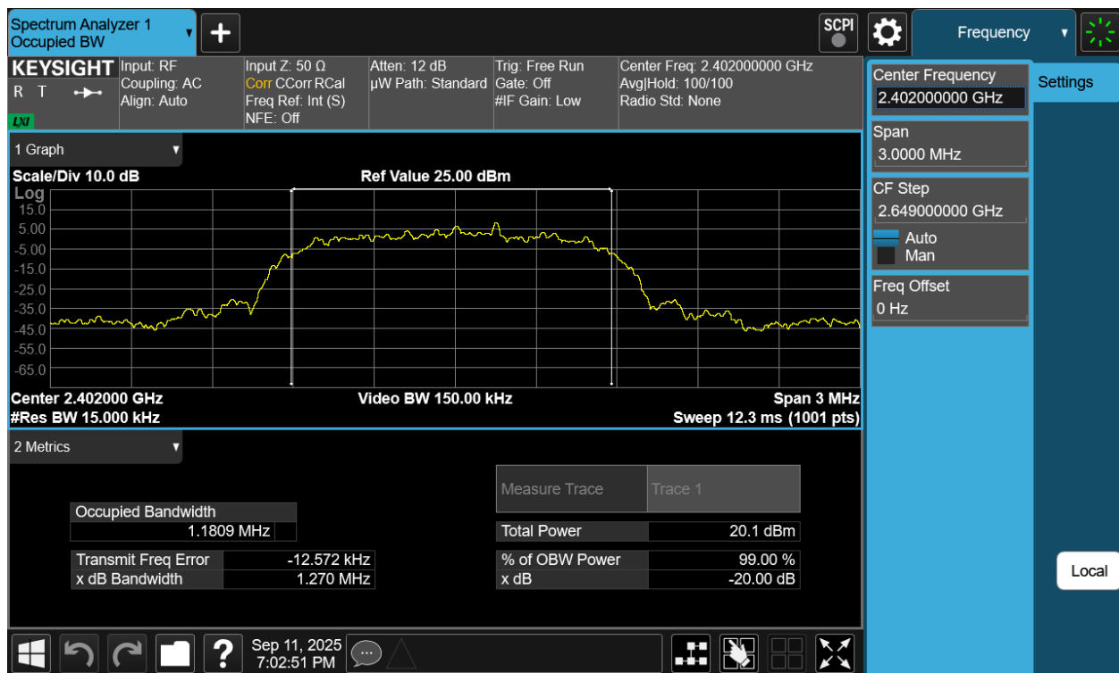
Plot 7-10. 20dB BW and 99% OBW Plot Antenna 1a (Bluetooth, 8DPSK, ePA – Ch. 0)
