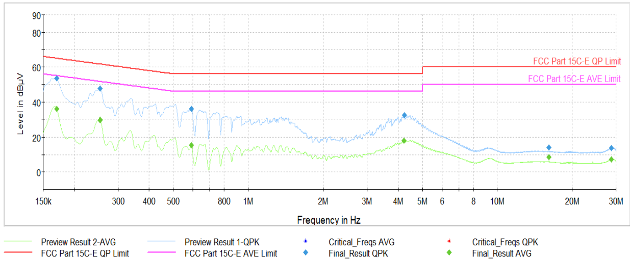
Plot 7-79. AC Line-Conducted Test Plot TxBF (N, GFSK ePA – Ch.39, with AC/DC Adapter)
