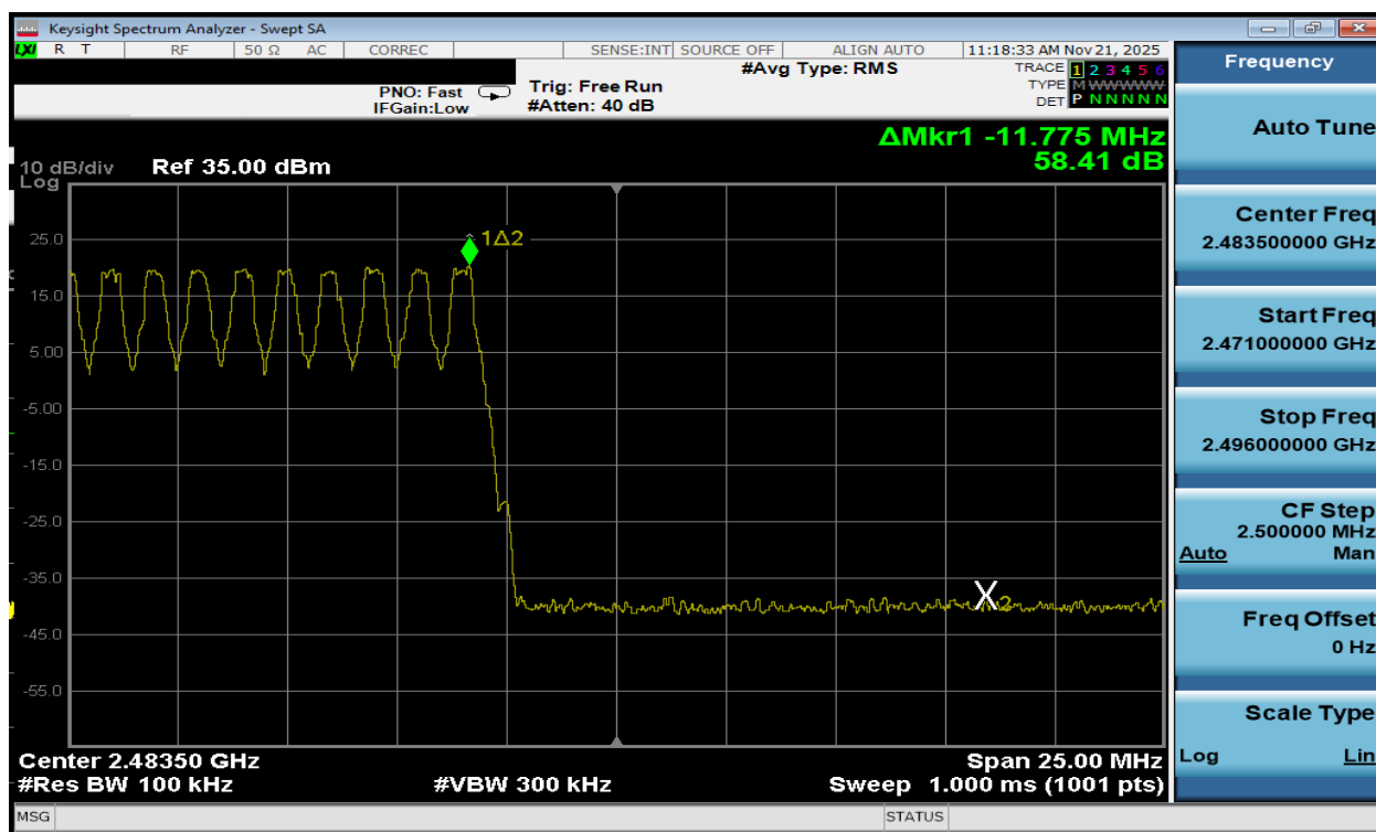
Plot 7-24. Band Edge Plot Antenna 1a (Bluetooth with Hopping Enabled, GFSK, ePA)
