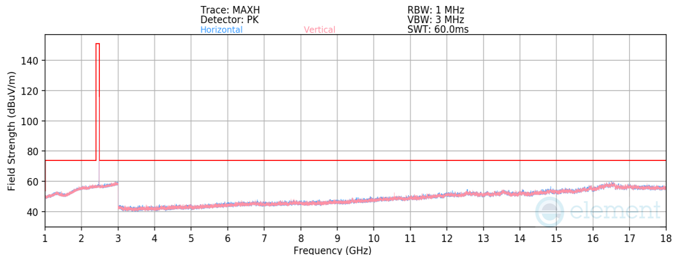
Plot 7-62. Radiated Spurious Emissions above 1GHz TxBF (BT GFSK ePA – Ch. 78)
