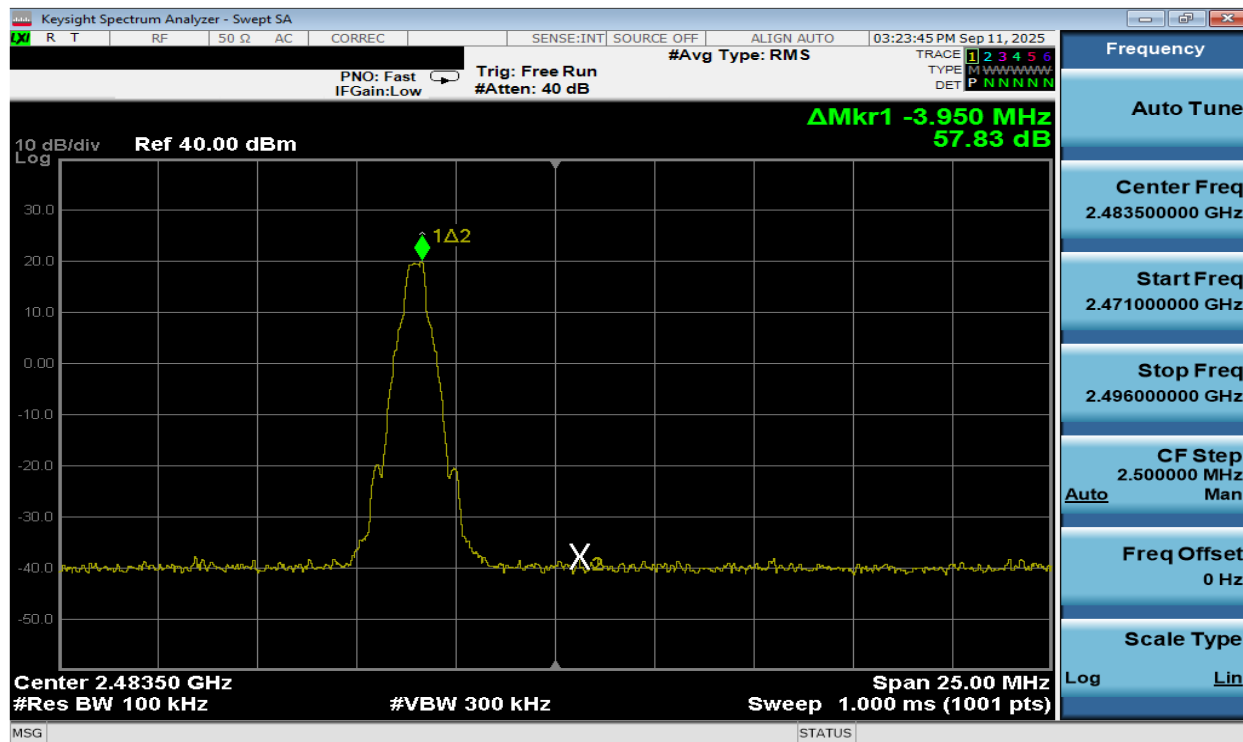
Plot 7-14. Band Edge Plot Antenna 3a (Bluetooth with Hopping Disabled, GFSK, ePA – Ch. 78)
