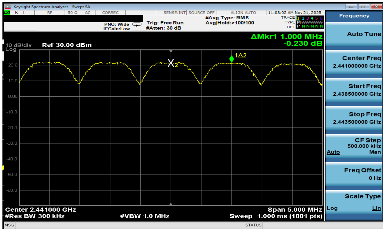
Plot 7-29. Channel Spacing Plot Antenna 3a (Bluetooth, GFSK, ePA)
