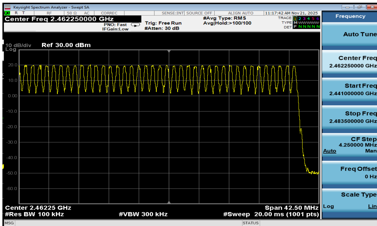
Plot 7-42. High End Spectrum Channel Hopping Plot Antenna 1a (Bluetooth, GFSK, ePA)
