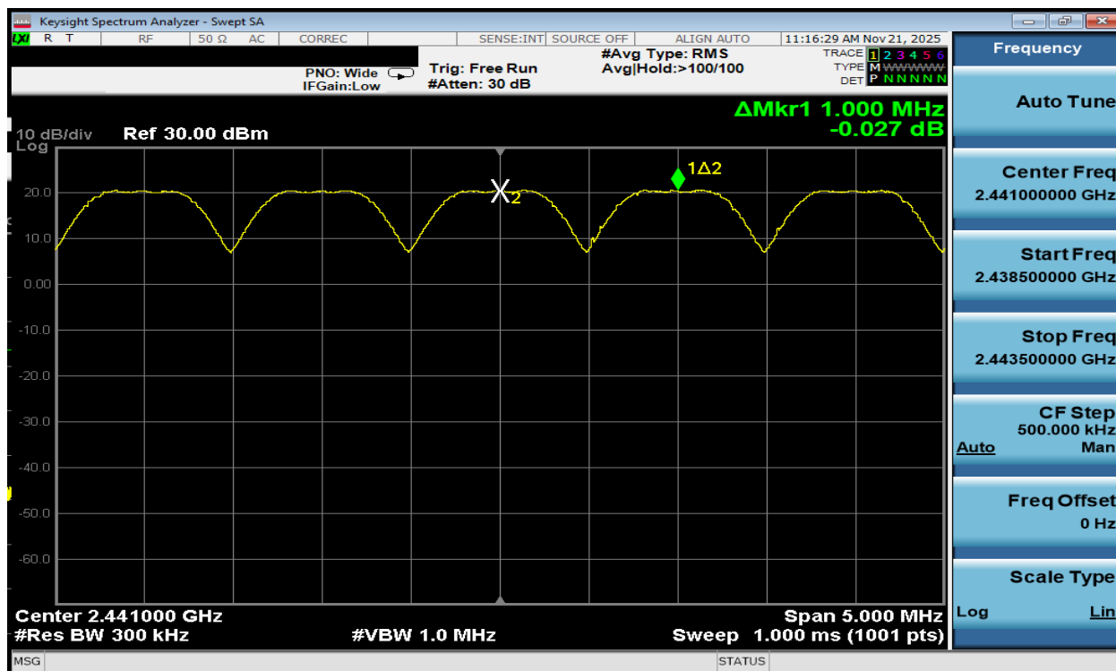
Plot 7-31. Channel Spacing Plot Antenna 1a (Bluetooth, GFSK, ePA)
