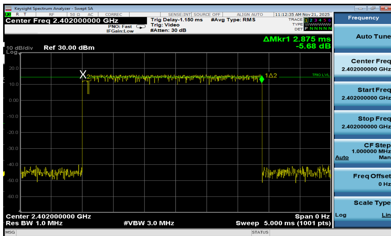
Plot 7-34. Time of Occupancy Plot Antenna 3a (Bluetooth, 8DPSK, ePA)
