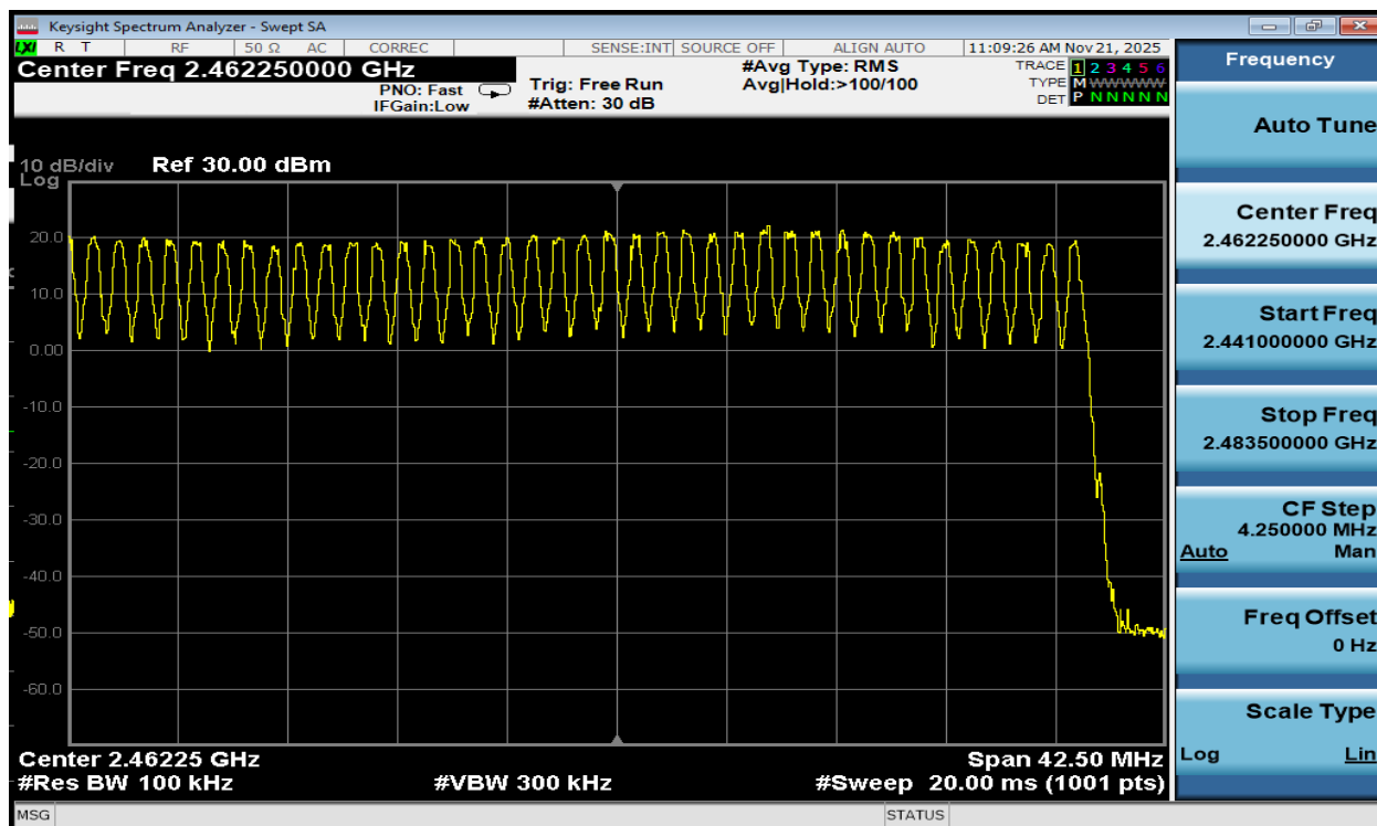
Plot 7-38. High End Spectrum Channel Hopping Plot Antenna 3a (Bluetooth, GFSK, ePA)
