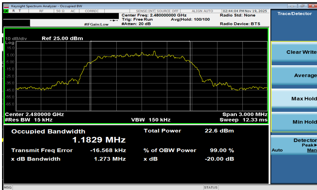
Plot 7-6. 20dB BW and 99% OBW Plot Antenna 3a (Bluetooth, 8DPSK, ePA – Ch. 78)
