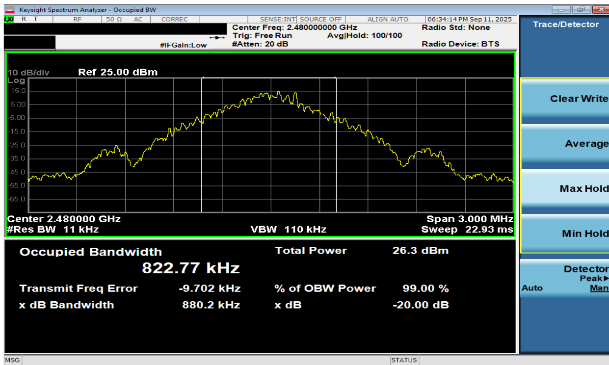
Plot 7-9. 20dB BW and 99% OBW Plot Antenna 1a (Bluetooth, GFSK, ePA – Ch. 78)
