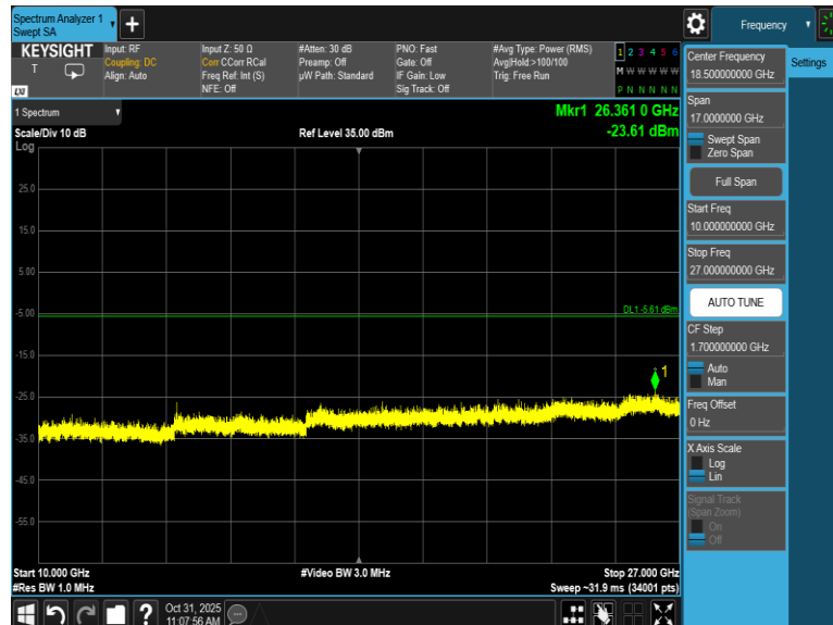
Plot 7-58. Conducted Simultaneous Tx Spurious Plot Antenna 3a (Bluetooth + UNII + LTE Band 41)
