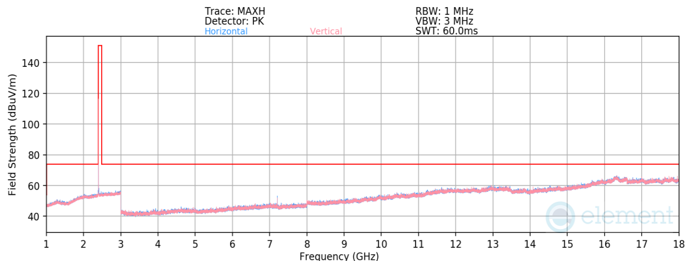
Plot 7-59. Radiated Spurious Emissions above 1GHz TxBF (BT GFSK ePA – Ch. 0)
