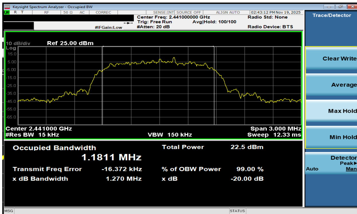
Plot 7-5. 20dB BW and 99% OBW Plot Antenna 3a (Bluetooth, 8DPSK, ePA – Ch. 39)
