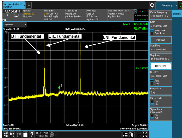
Plot 7-57. Conducted Simultaneous Tx Spurious Plot Antenna 3a (Bluetooth + UNII + LTE Band 41)
