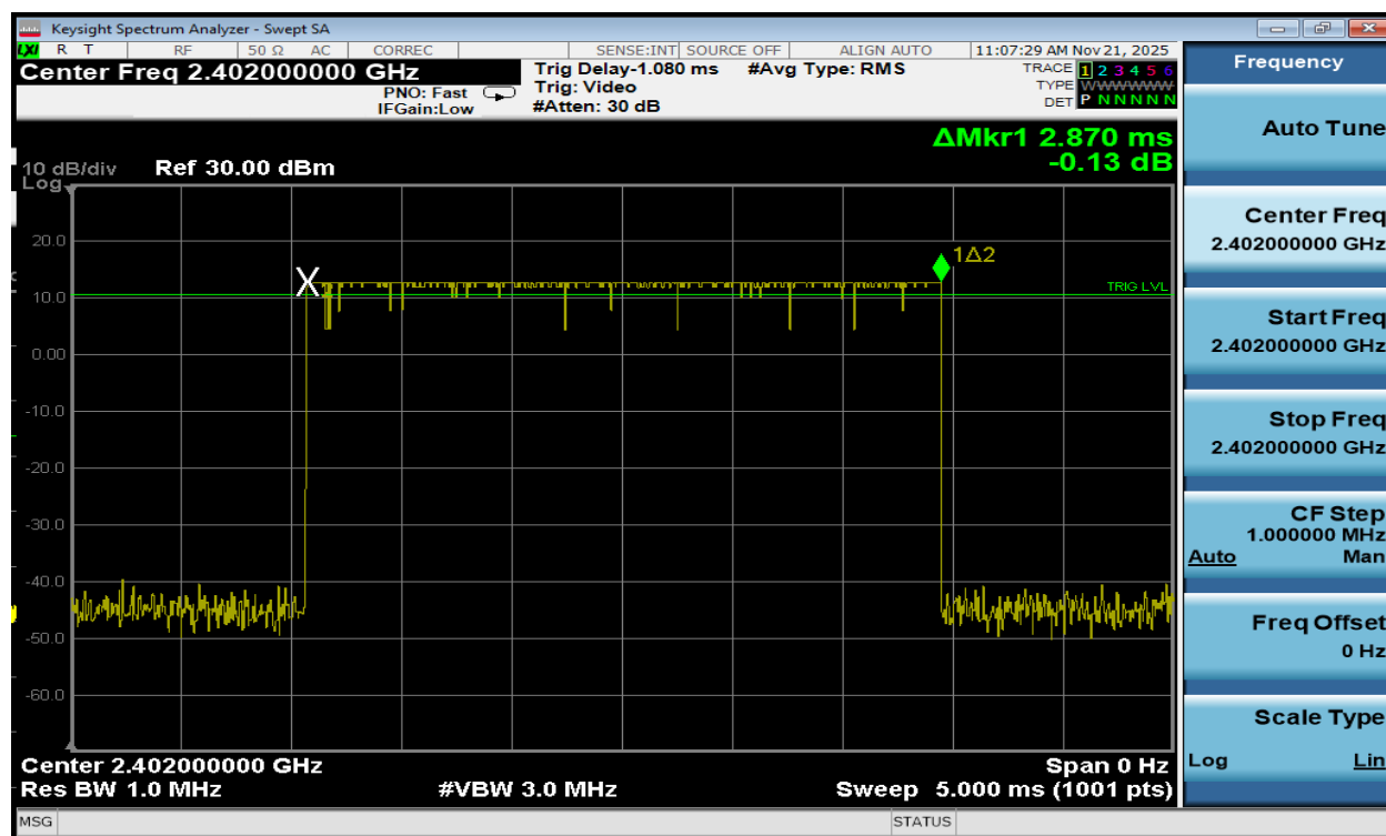
Plot 7-33. Time of Occupancy Plot Antenna 3a (Bluetooth, GFSK, ePA)
