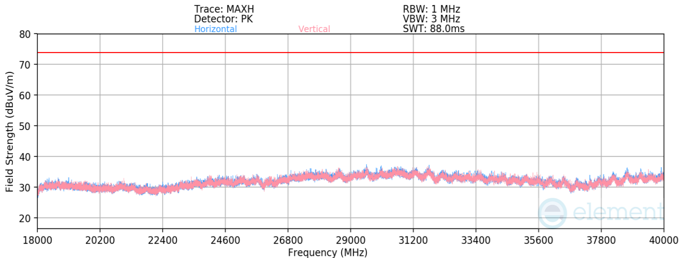
Plot 7-64. Radiated Spurious Emissions above 18GHz – Simultaneous Transmission
