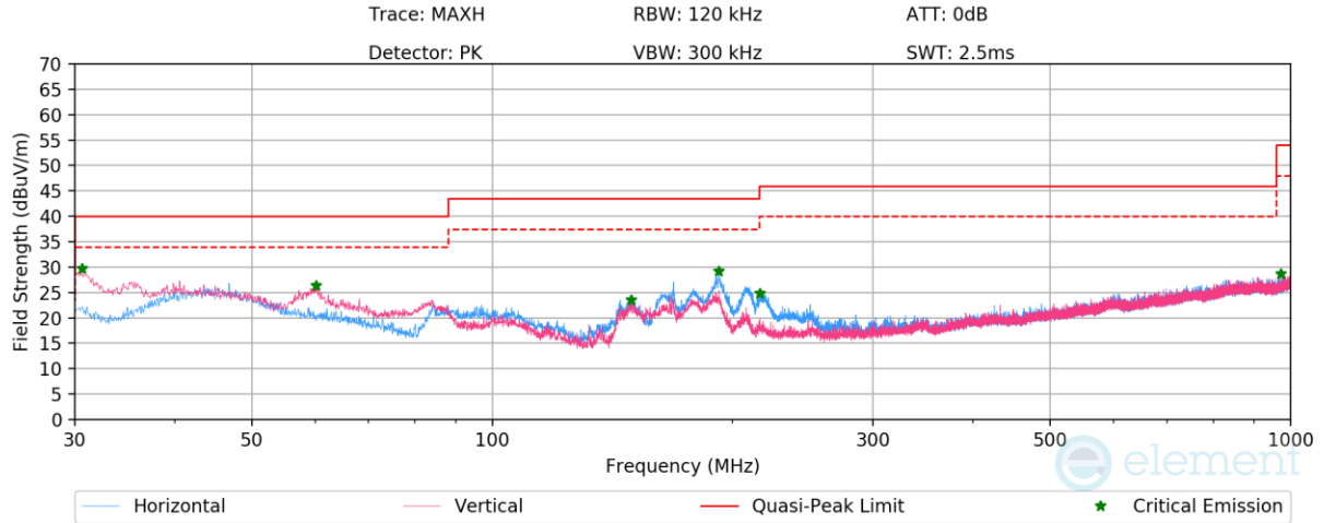
Plot 7-77. Radiated Spurious Emissions Below 1GHz TxBF (GFSK ePA – Ch.39, with AC/DC Adapter)
