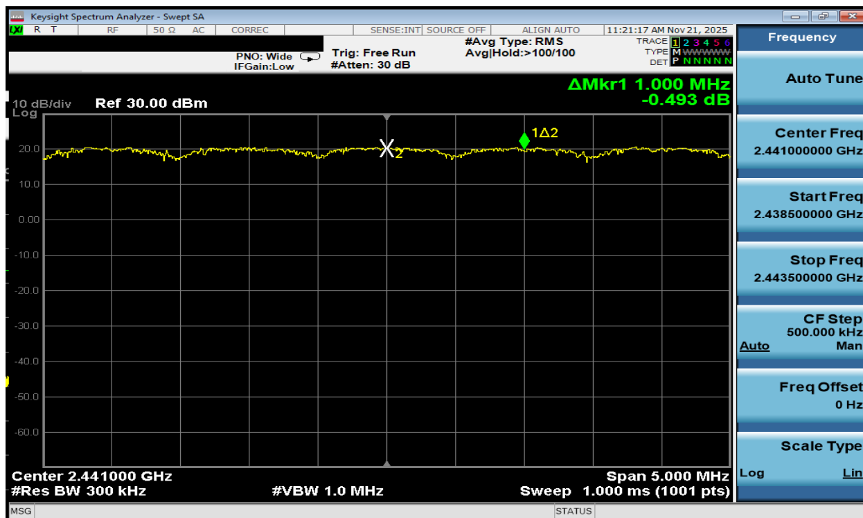
Plot 7-32. Channel Spacing Plot Antenna 1a (Bluetooth, 8DPSK, ePA)
