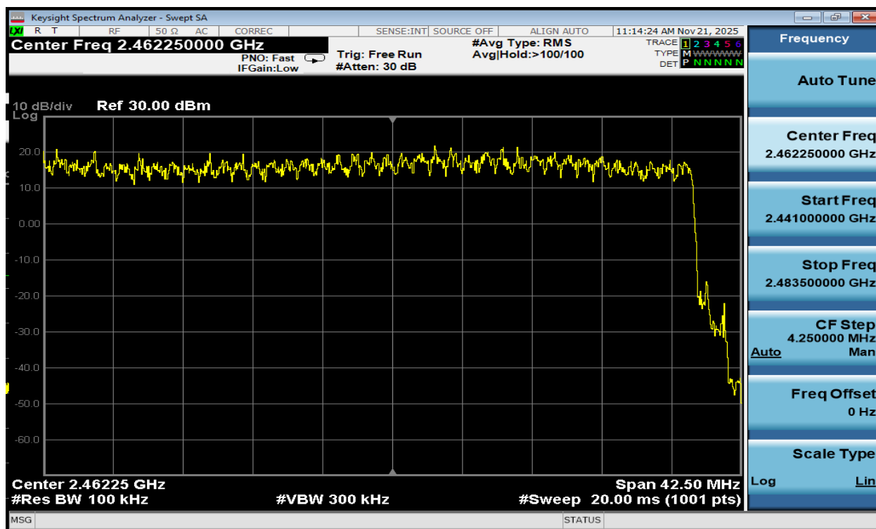
Plot 7-40. High End Spectrum Channel Hopping Plot Antenna 3a (Bluetooth, 8DPSK, ePA)
