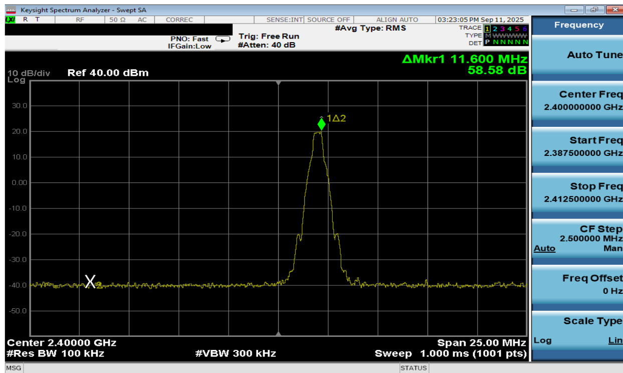
Plot 7-13. Band Edge Plot Antenna 3a (Bluetooth with Hopping Disabled, GFSK, ePA – Ch. 0)
