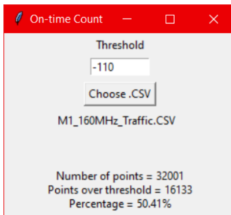
Figure 9-4. 5250MHz - Channel Loading Calculation - Mode 1 (160MHz)
