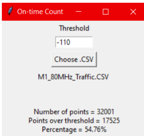
Figure 9-2. 5530MHz - Channel Loading Calculation - Mode 1 (80MHz)
