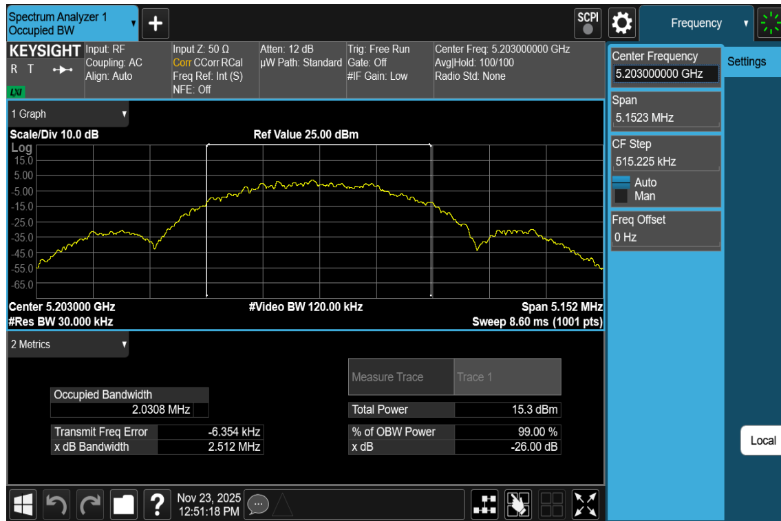
Plot 7-29. 26dB BW & 99% OBW Antenna 3a (NB UNII LE2M, ePA– 5203MHz)
