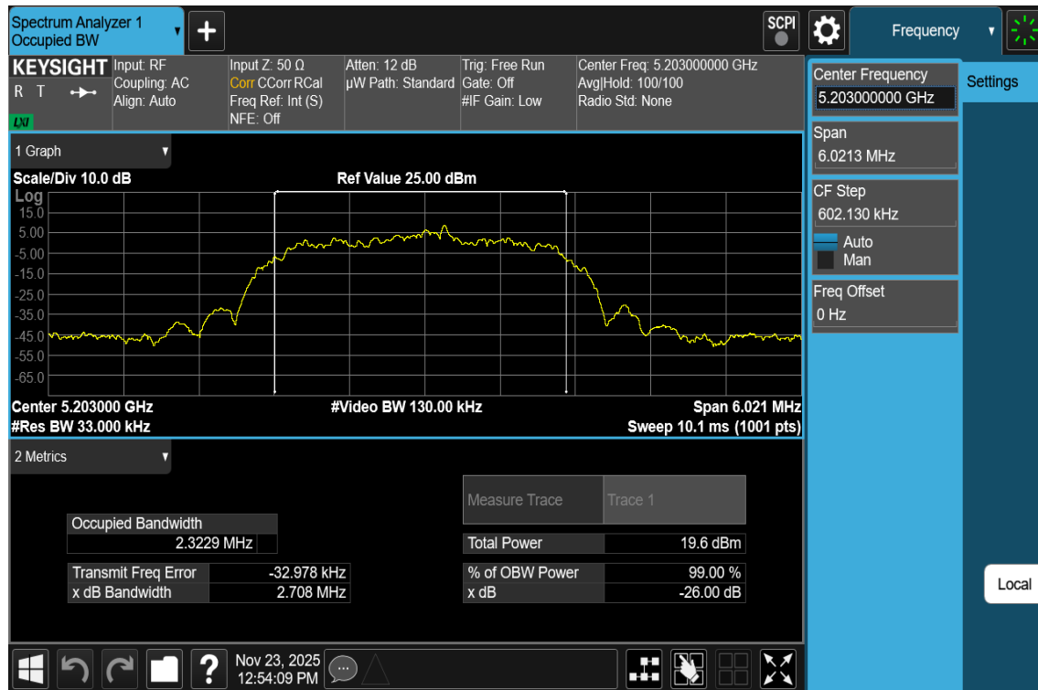
Plot 7-30. 26dB BW & 99% OBW Antenna 3a (NB UNII HDR4, ePA– 5203MHz)
