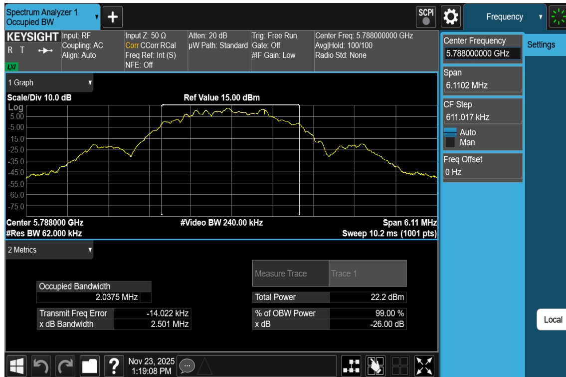
Plot 7-42. 99% OBW Antenna 3a (NB UNII LE2M, ePA- 5788MHz)
