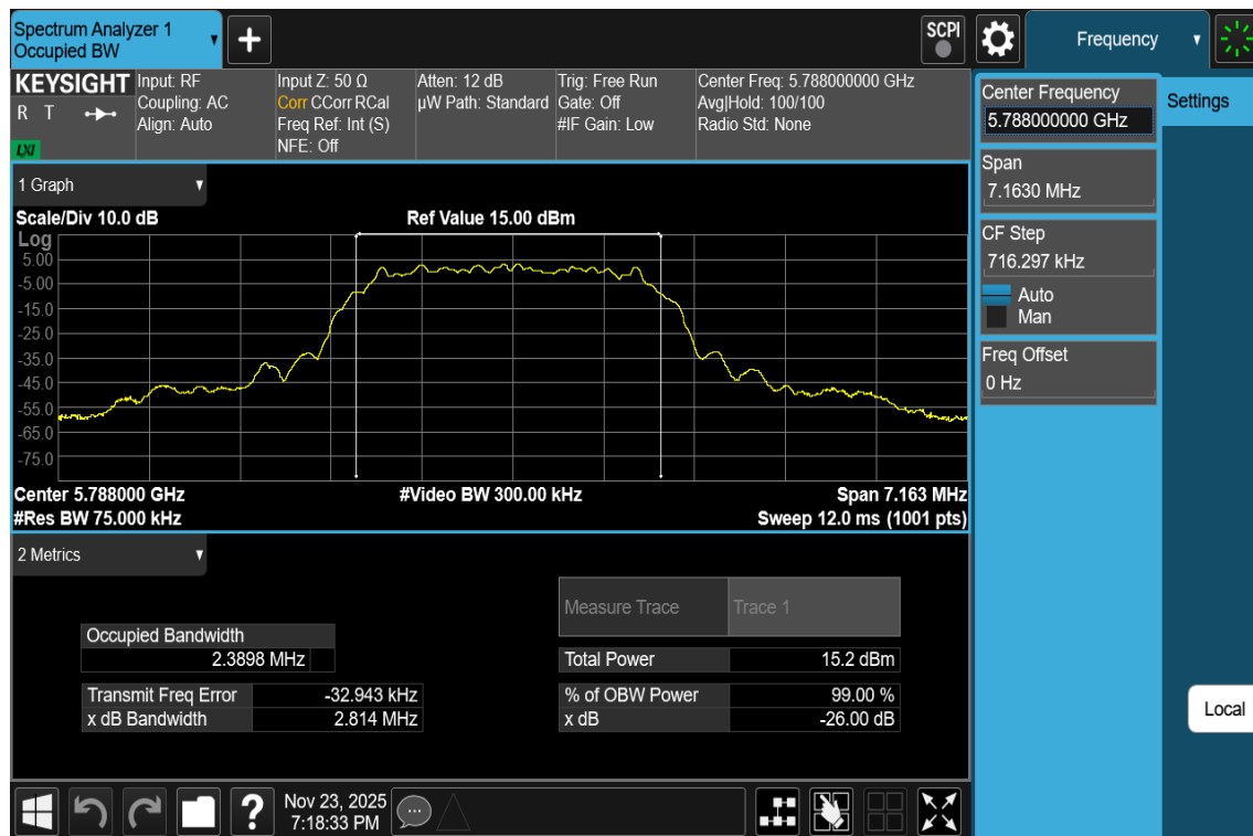
Plot 7-52. 99% OBW Antenna 3a (NB UNII HDT6, ePA– 5788MHz)
