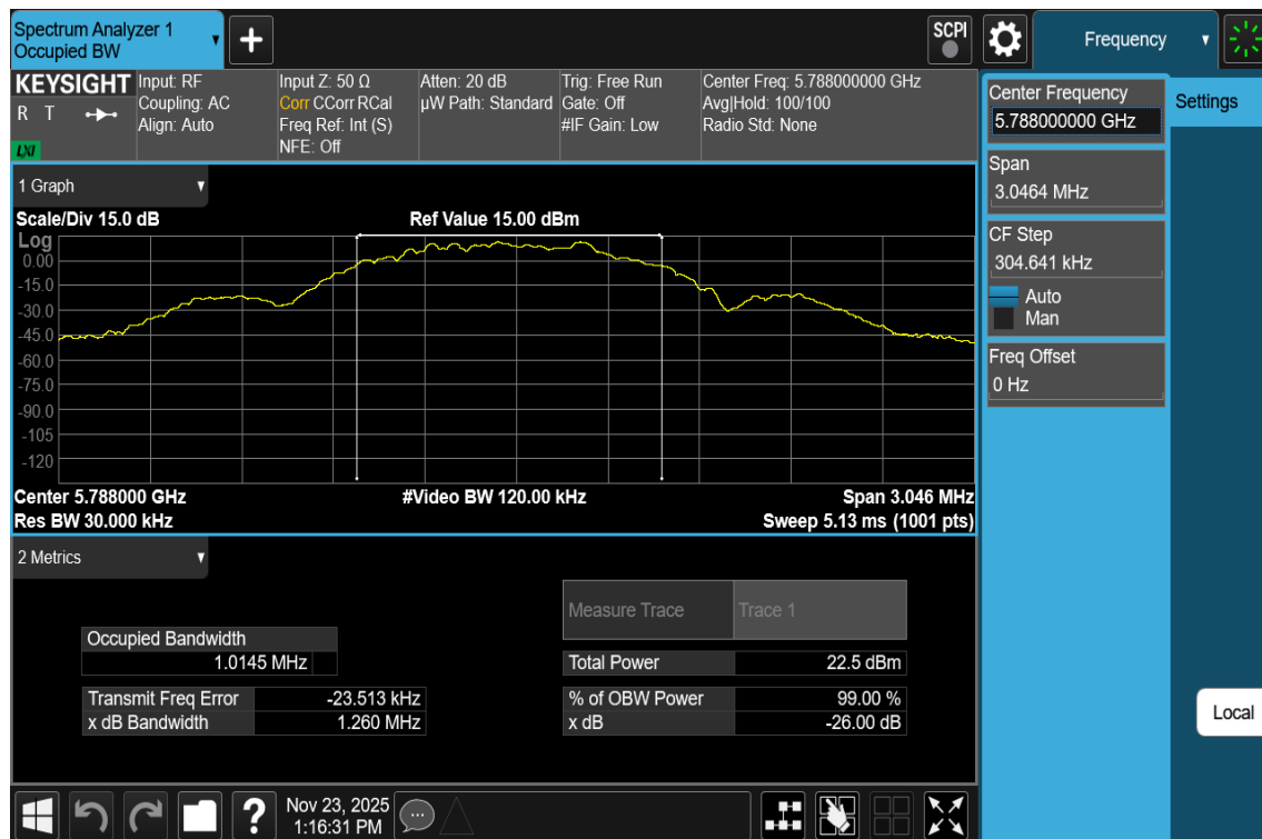
Plot 7-41. 99% OBW Antenna 3a (NB UNII LE1M, ePA – 5788MHz)
