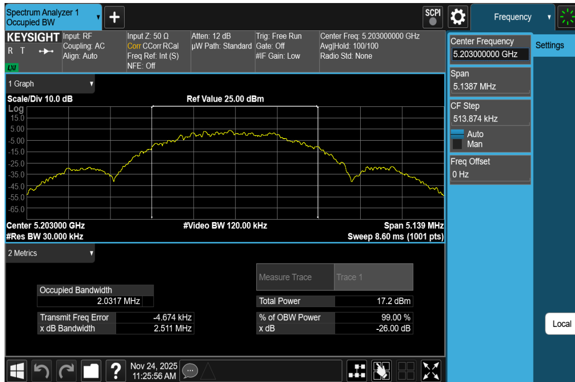
Plot 7-55. 26dB BW & 99% OBW Antenna 1b (NB UNII LE2M, ePA– 5203MHz)
