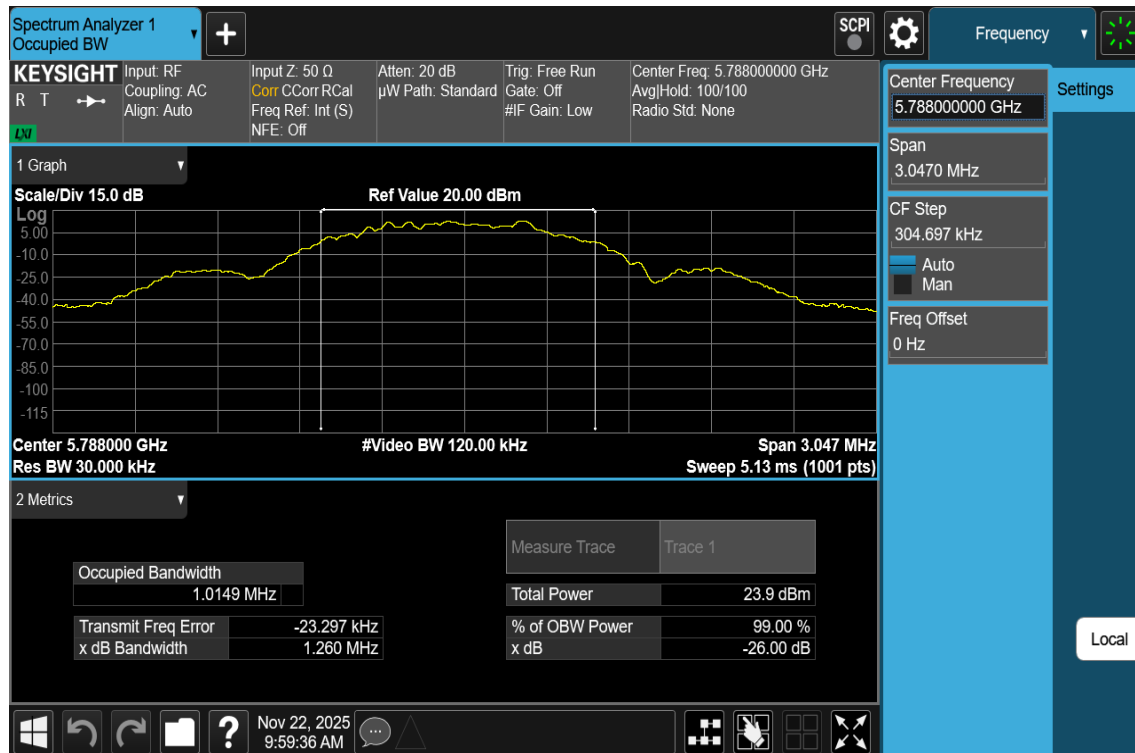
Plot 7-15. 99% OBW Antenna 3c (NB UNII LE1M, ePA – 5788MHz)
