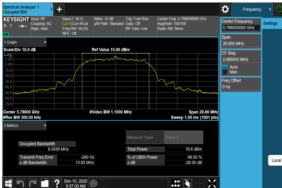
Plot 7-23. 99% OBW Antenna 3c (NB UNII HDRPL32, ePA – 5788MHz)
