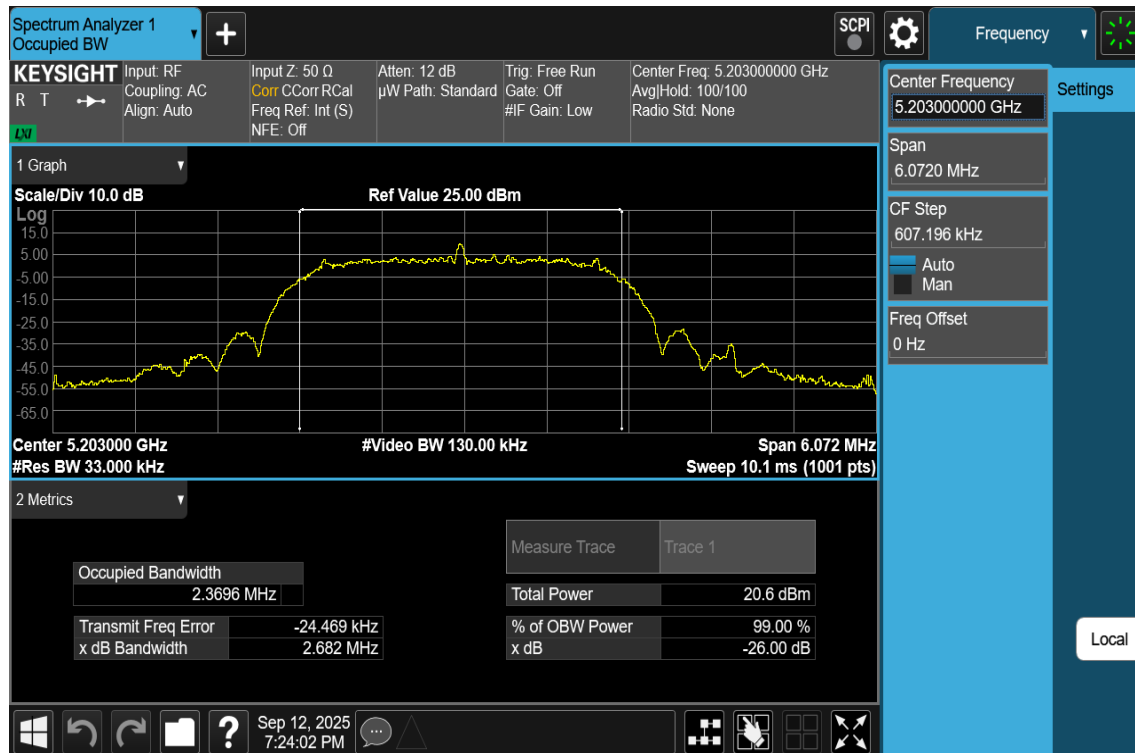
Plot 7-58. 26dB BW & 99% OBW Antenna 1b (NB UNII HDRPS2, ePA– 5203MHz)
