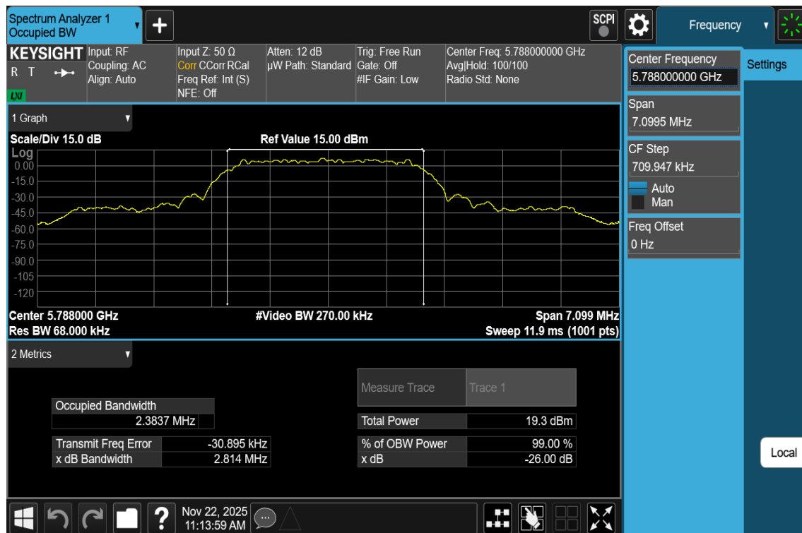
Plot 7-25. 99% OBW Antenna 3c (NB UNII HDT4, ePA- 5788MHz)
