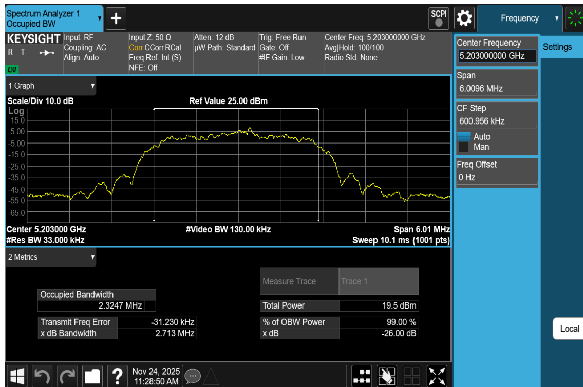
Plot 7-56. 26dB BW & 99% OBW Antenna 1b (NB UNII HDR4, ePA– 5203MHz)
