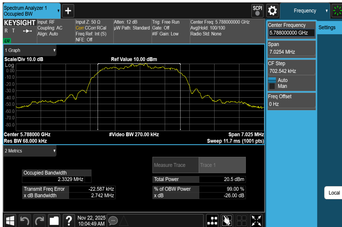
Plot 7-17. 99% OBW Antenna 3c (NB UNII HDR4, ePA – 5788MHz)
