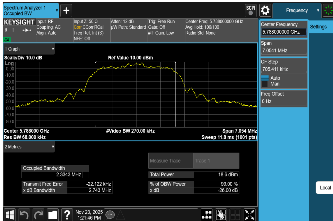
Plot 7-43. 99% OBW Antenna 3a (NB UNII HDR4, ePA - 5788MHz)
