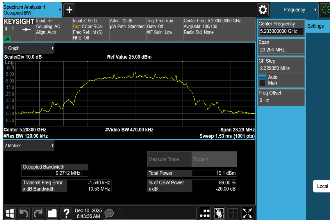
Plot 7-10. 26dB BW & 99% OBW Antenna 3c (NB UNII HDRPL32, ePA- 5203MHz)
