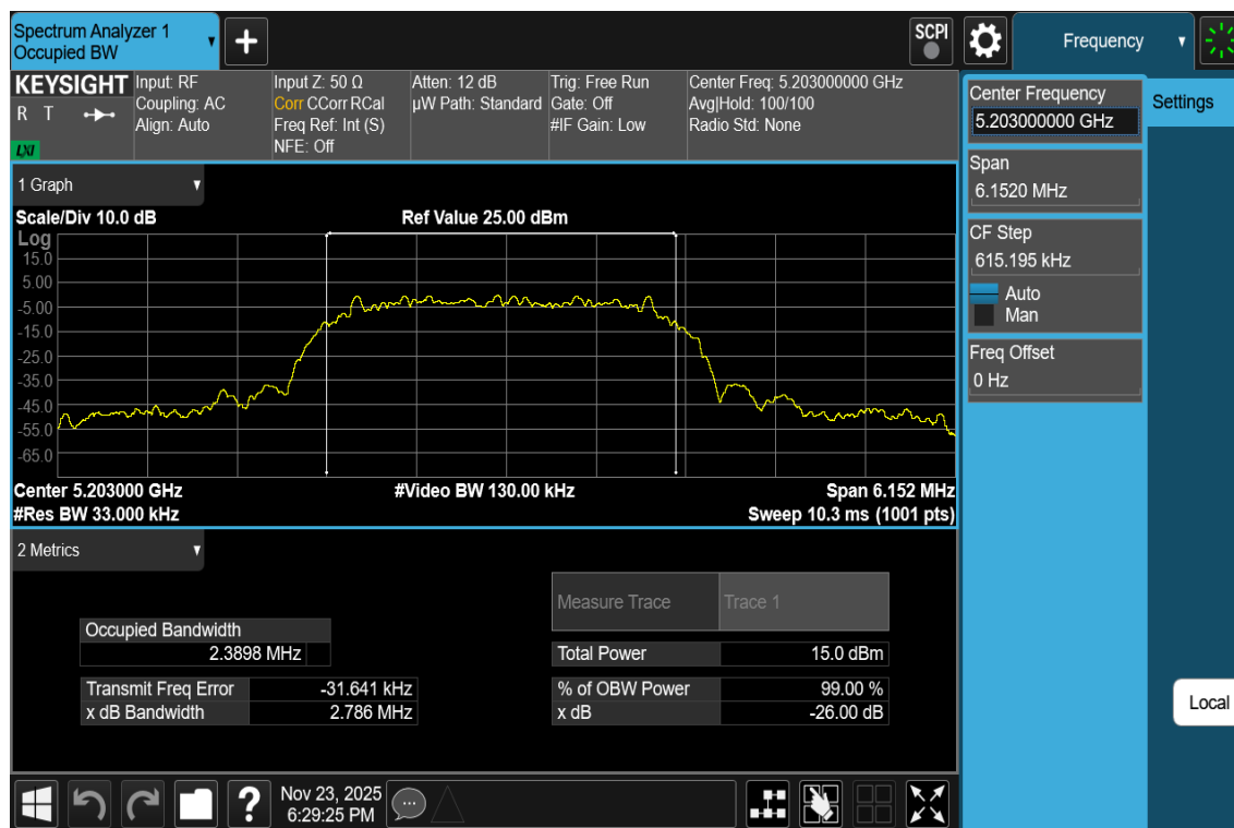
Plot 7-39. 26dB BW & 99% OBW Antenna 3a (NB UNII HDT6, ePA- 5203MHz)
