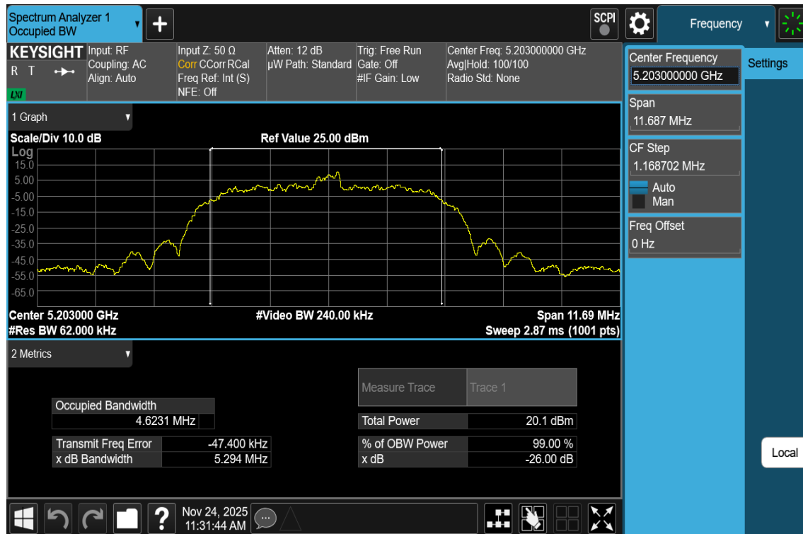
Plot 7-57. 26dB BW & 99% OBW Antenna 1b (NB UNII HDR8, ePA– 5203MHz)
