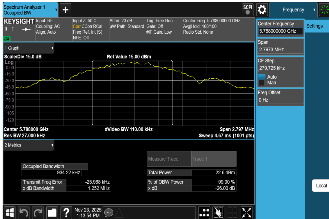
Plot 7-40. 99% OBW Antenna 3a (NB UNII BDR, ePA – 5788MHz)
