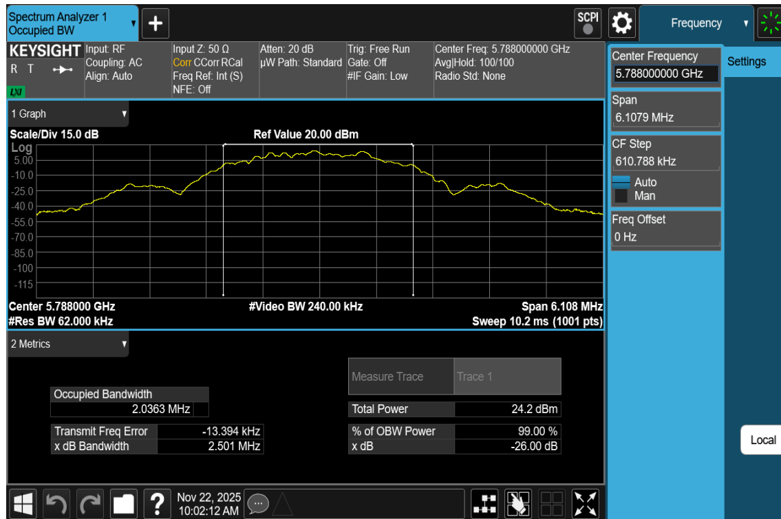
Plot 7-16. 99% OBW Antenna 3c (NB UNII LE2M, ePA– 5788MHz)
