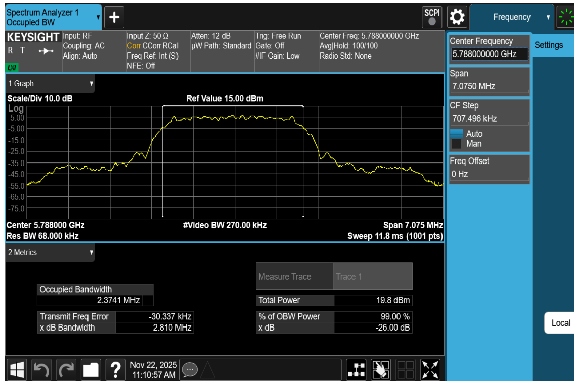
Plot 7-24. 99% OBW Antenna 3c (NB UNII HDT2, ePA- 5788MHz)
