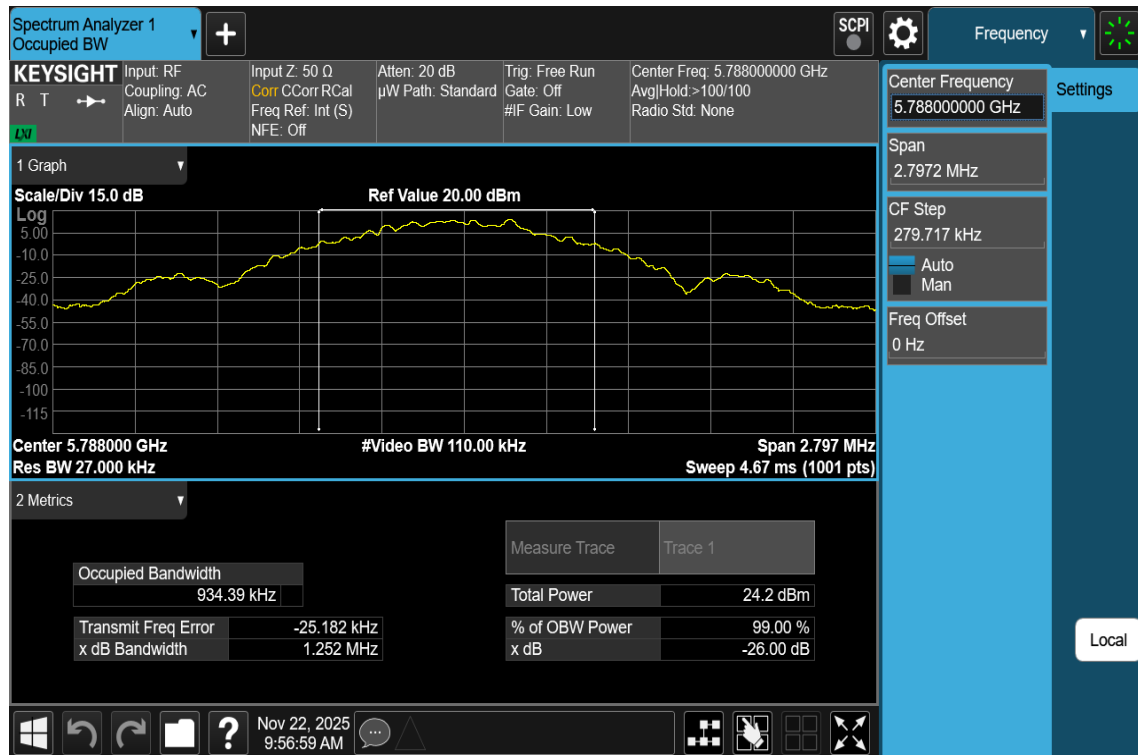
Plot 7-14. 99% OBW Antenna 3c (NB UNII BDR, ePA – 5788MHz)
