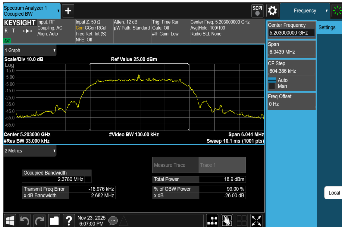
Plot 7-32. 26dB BW & 99% OBW Antenna 3a (NB UNII HDRPS2, ePA– 5203MHz)
