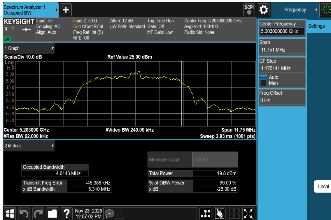
Plot 7-31. 26dB BW & 99% OBW Antenna 3a (NB UNII HDR8, ePA– 5203MHz)
