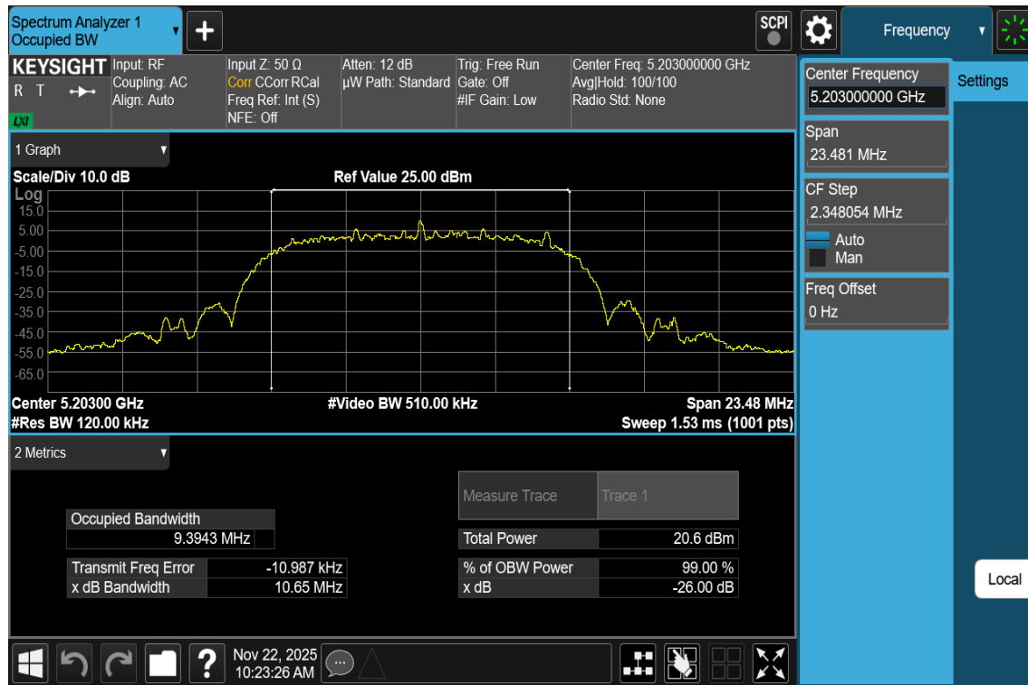
Plot 7-9. 26dB BW & 99% OBW Antenna 3c (NB UNII HDRPL12, ePA- 5203MHz)
