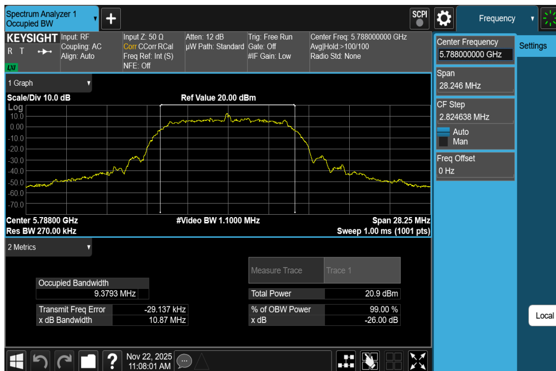
Plot 7-22. 99% OBW Antenna 3c (NB UNII HDRPL12, ePA – 5788MHz)
