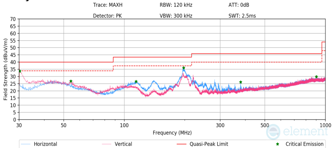
Plot 7-710. Radiated Spurious Emissions Below 1GHz TxBF Primary (NB UNII BDR ePA – 5788MHz), with AC/DC adaptor
