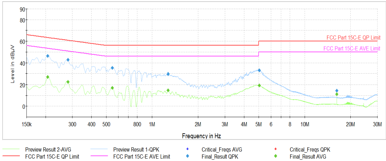
Plot 7-712. AC Line Conducted Plot TxBF Primary (NB UNII BDR ePA – 5788MHz) (L1) with AC/DC adaptor
