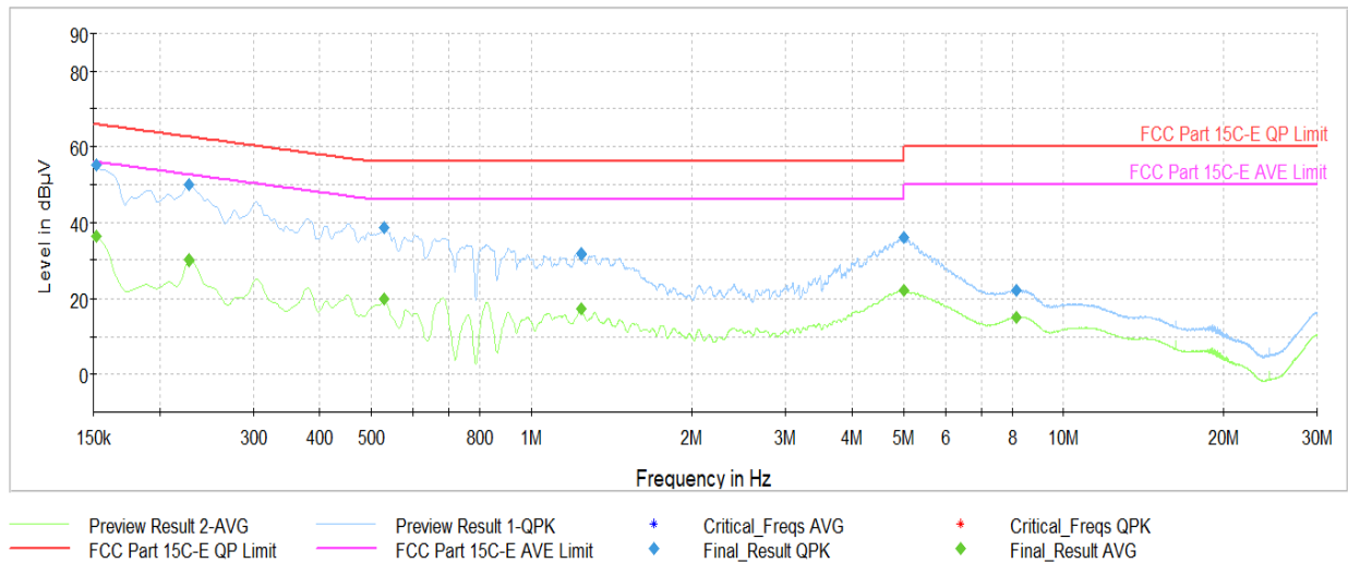
Plot 7-713. AC Line Conducted Plot TxBF Primary (NB UNII BDR ePA – 5788MHz) (N) with AC/DC adaptor
