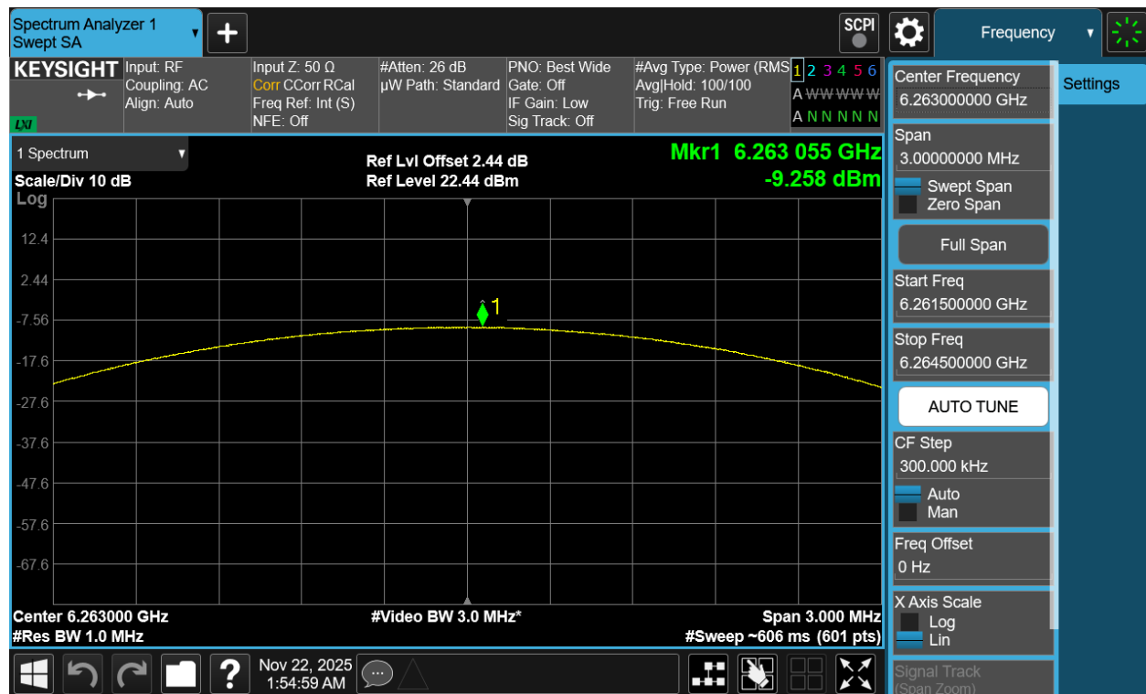
Plot 7-44. PSD Antenna 3c (NB UNII LE2M, ePA - 6263MHz)
