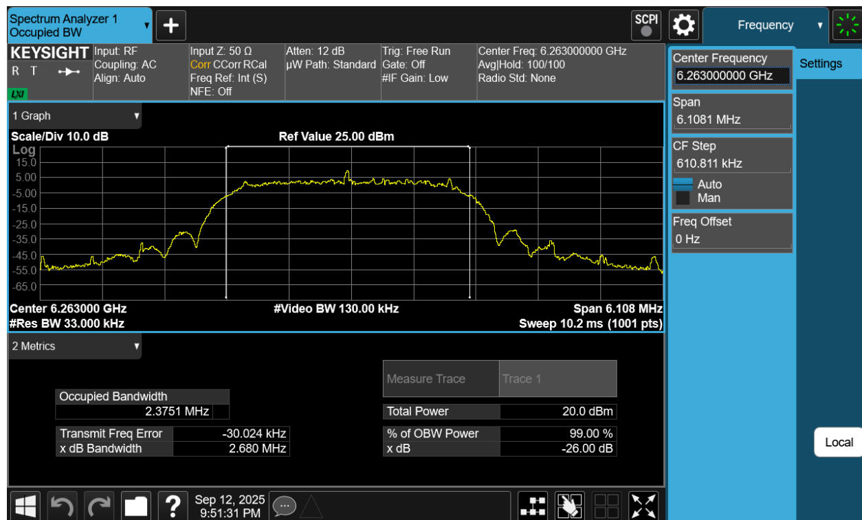
Plot 7-32. 26dB BW & 99% OBW Antenna 1b (NB UNII HDRPS2, ePA- 6263MHz)
