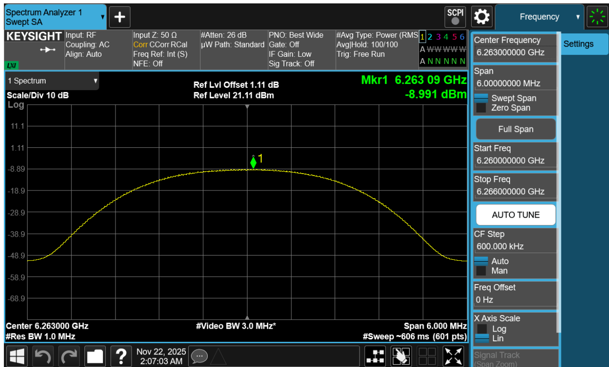
Plot 7-47. PSD Antenna 3c (NB UNII HDR4, iPA – 6263MHz)
