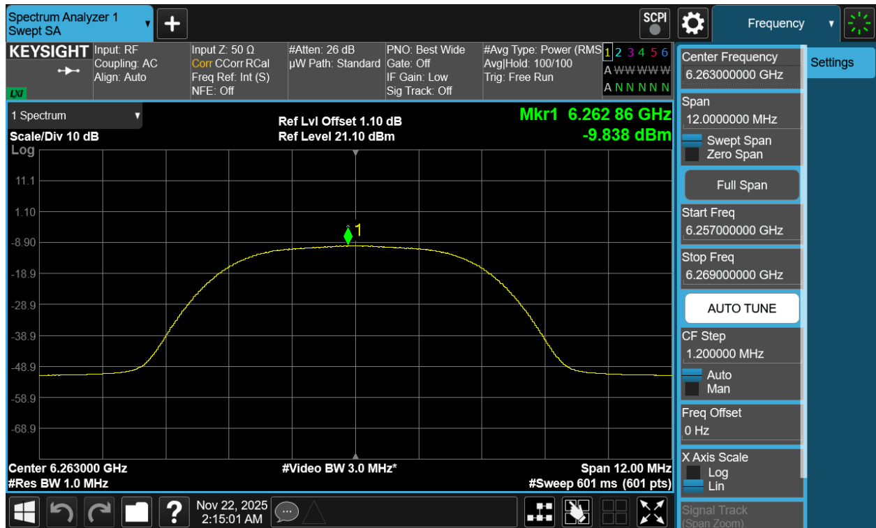
Plot 7-49. PSD Antenna 3c (NB UNII HDR8, iPA – 6263MHz)
