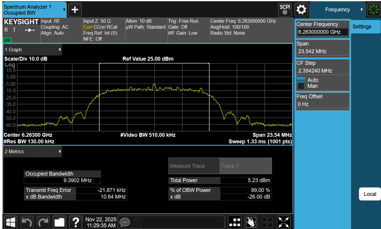
Plot 7-9. 26dB BW & 99% OBW Antenna 3c (NB UNII HDRPL12, ePA- 6263MHz)
