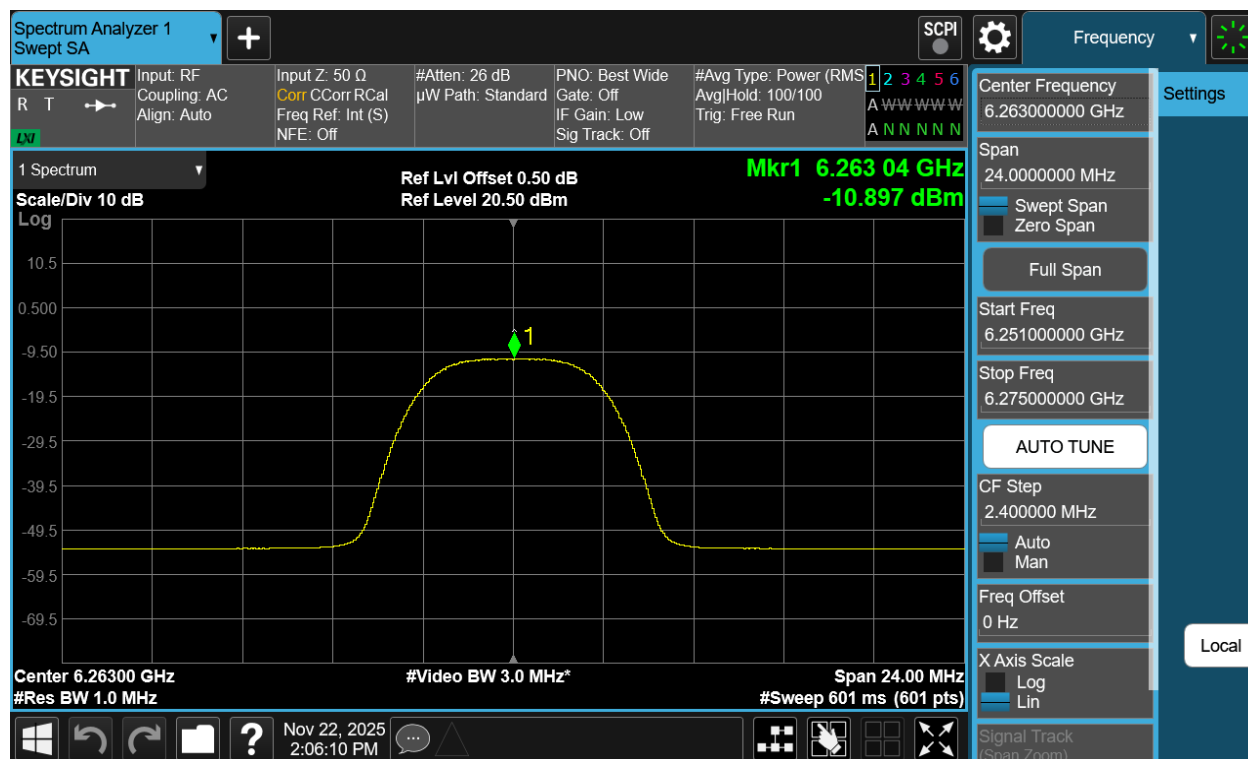
Plot 7-54. PSD Antenna 3c (NB UNII HDRPM16, ePA – 6263MHz)
