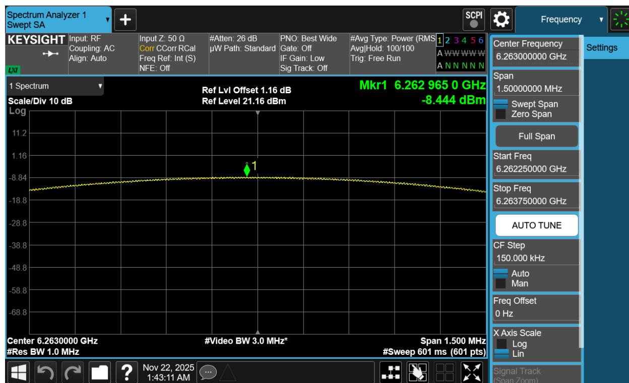
Plot 7-41. PSD Antenna 3c (NB UNII BDR, iPA – 6263MHz)
