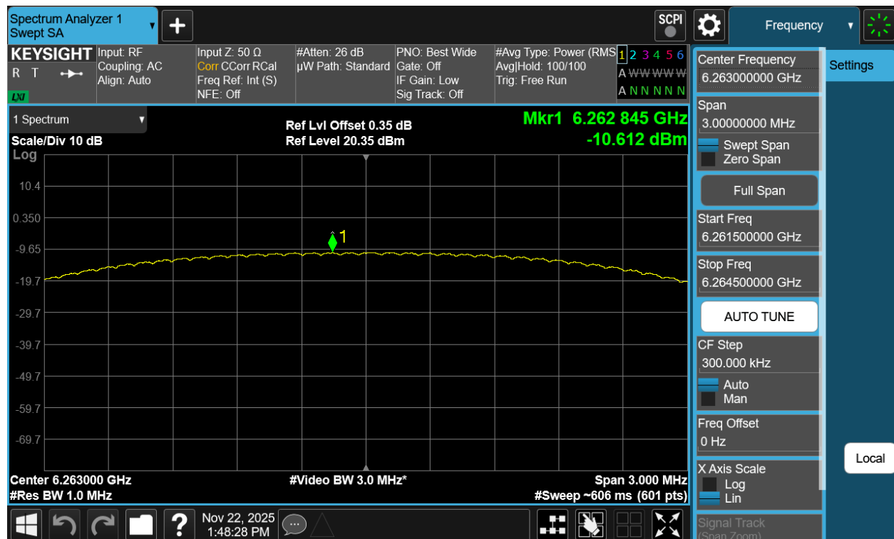
Plot 7-50. PSD Antenna 3c (NB UNII HDRPS2, ePA – 6263MHz)
