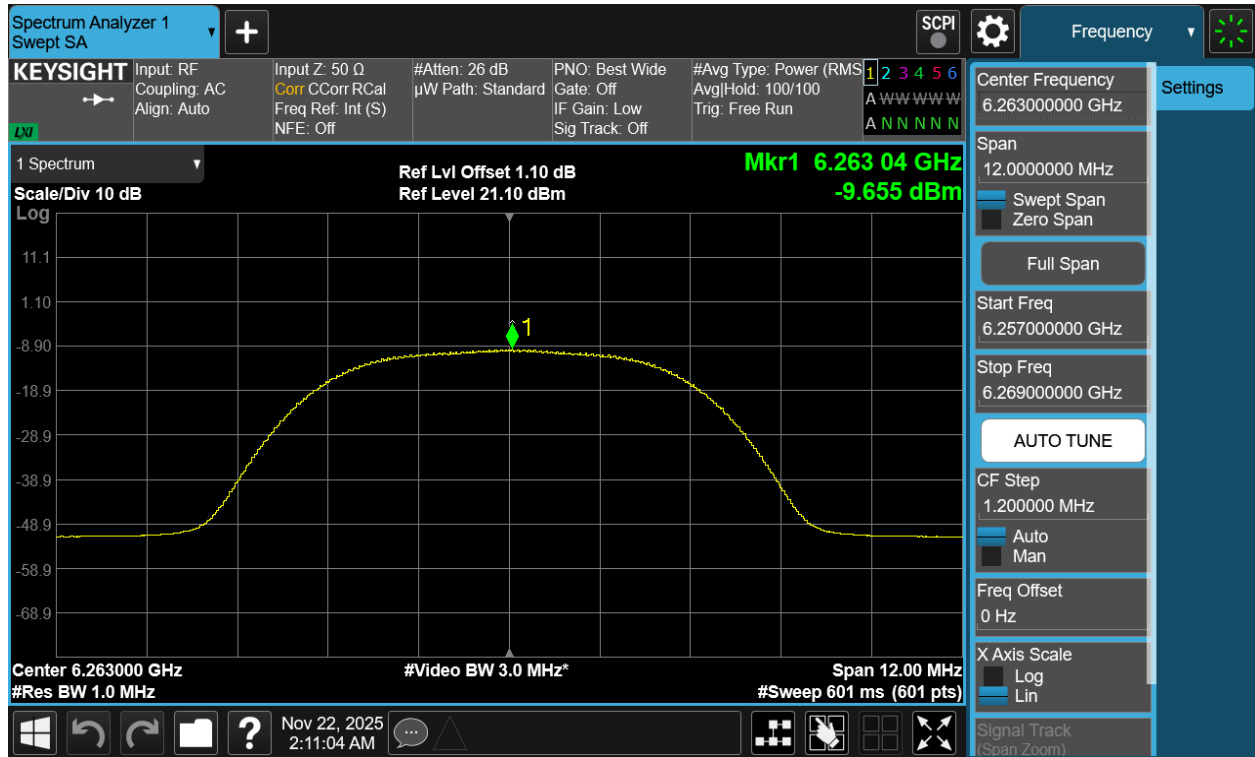
Plot 7-48. PSD Antenna 3c (NB UNII HDR8, ePA – 6263MHz)
