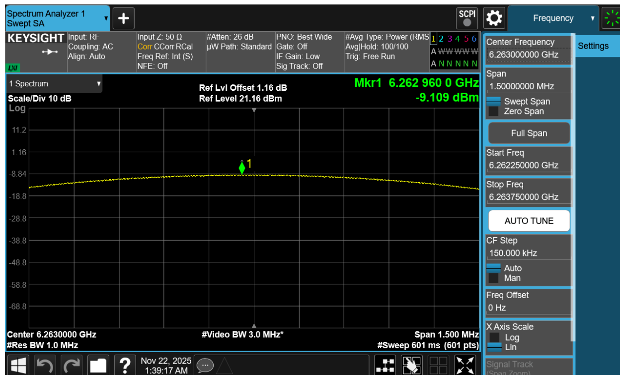
Plot 7-40. PSD Antenna 3c (NB UNII BDR, ePA – 6263MHz)
