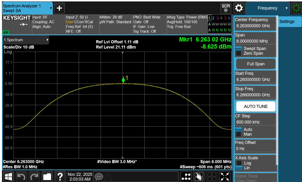
Plot 7-46. PSD Antenna 3c (NB UNII HDR4, ePA – 6263MHz)
