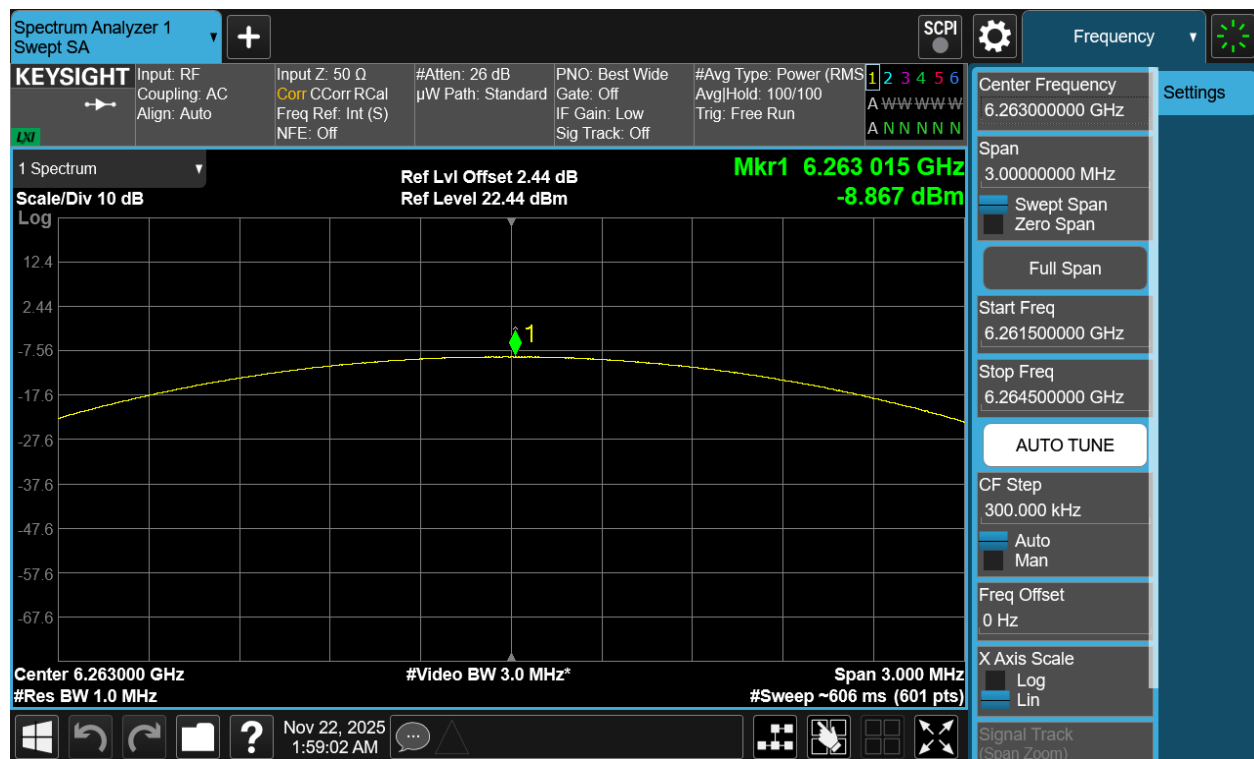
Plot 7-45. PSD Antenna 3c (NB UNII LE2M, iPA - 6263MHz)
