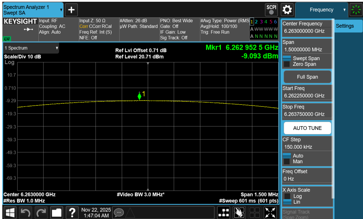
Plot 7-42. PSD Antenna 3c (NB UNII LE1M, ePA – 6263MHz)
