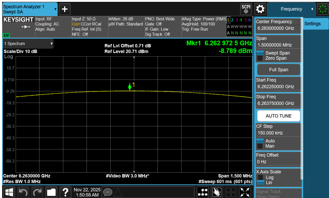
Plot 7-43. PSD Antenna 3c (NB UNII LE1M, iPA – 6263MHz)
