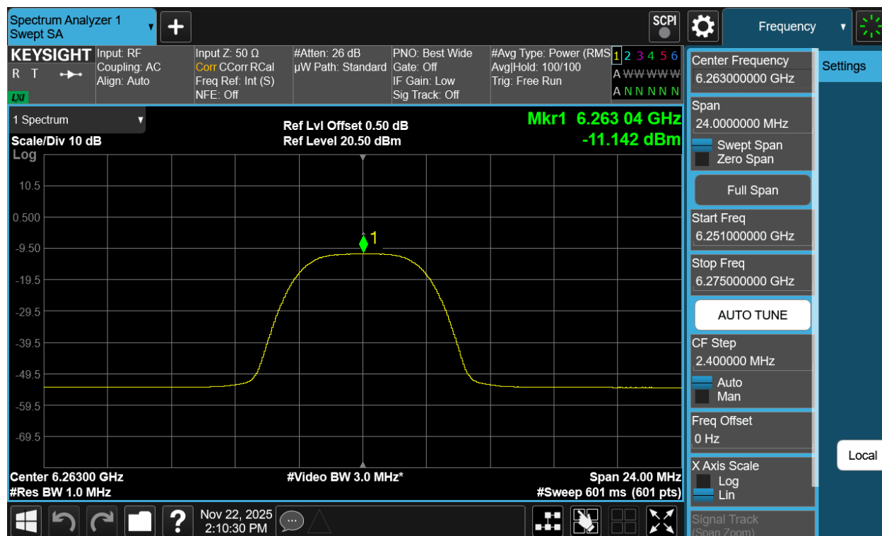
Plot 7-55. PSD Antenna 3c (NB UNII HDRPM16, iPA – 6263MHz)
