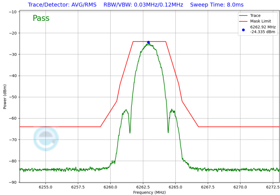
Plot 7-227. In-Band Emission Antenna 3c (NB UNII LE2M, iPA – 6263MHz)
