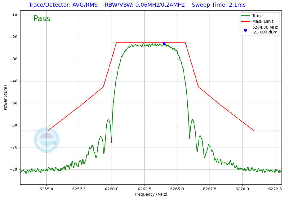
Plot 7-237. In-Band Emission Antenna 3c (NB UNII HDRPM16, iPA – 6263MHz)
