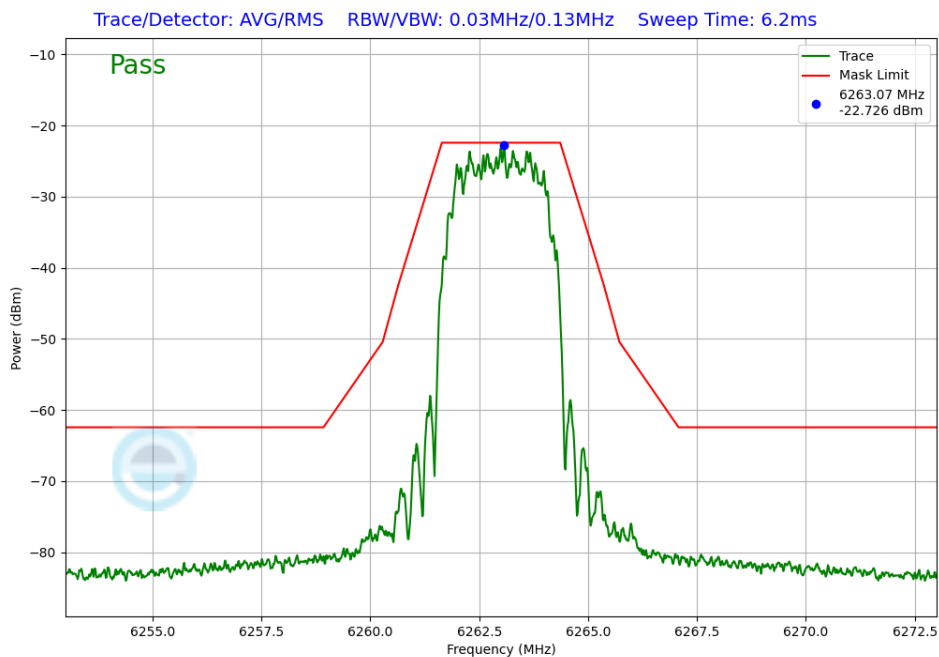
Plot 7-229. In-Band Emission Antenna 3c (NB UNII HDR4, iPA – 6263MHz)
