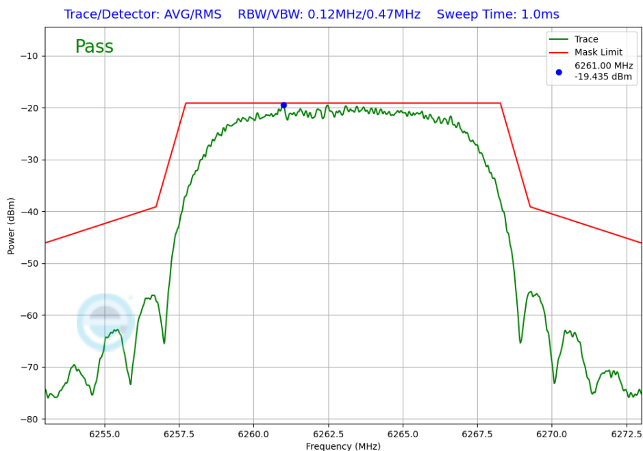
Plot 7-240. In-Band Emission Antenna 3c (NB UNII HDRPL32, ePA – 6263MHz)
