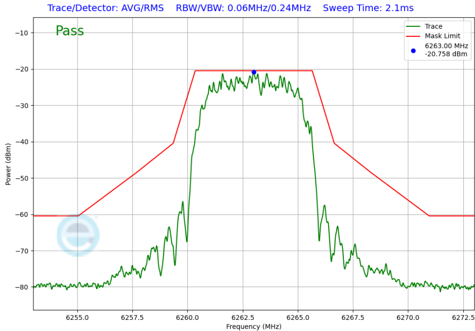
Plot 7-231. In-Band Emission Antenna 3c (NB UNII HDR8, iPA – 6263MHz)
