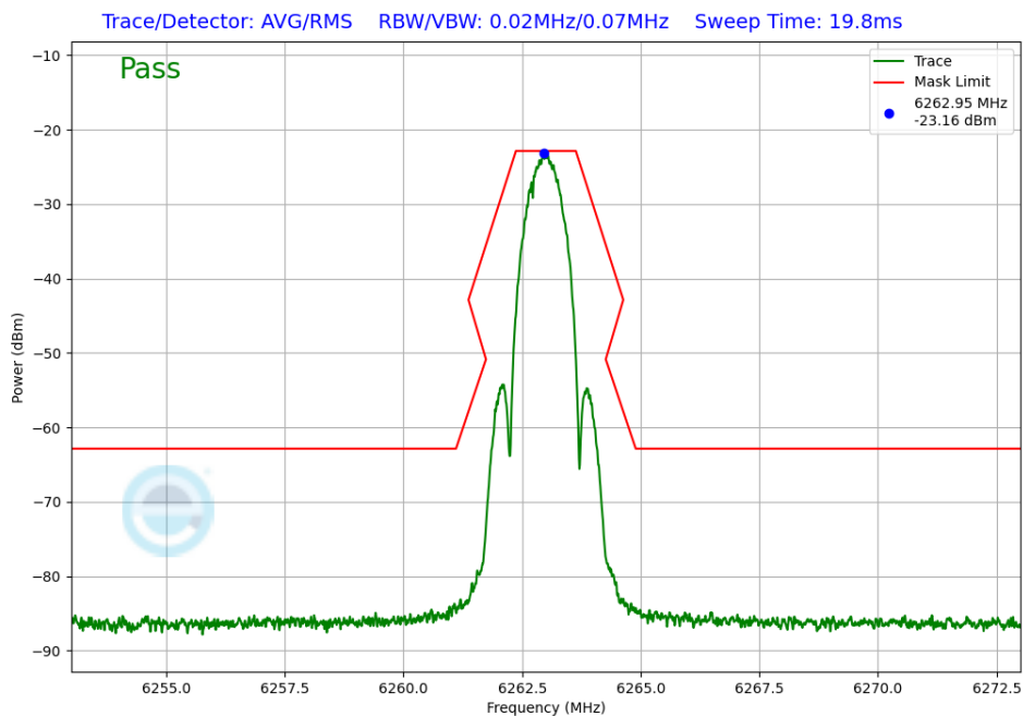
Plot 7-225. In-Band Emission Antenna 3c (NB UNII LE1M, iPA – 6263MHz)
