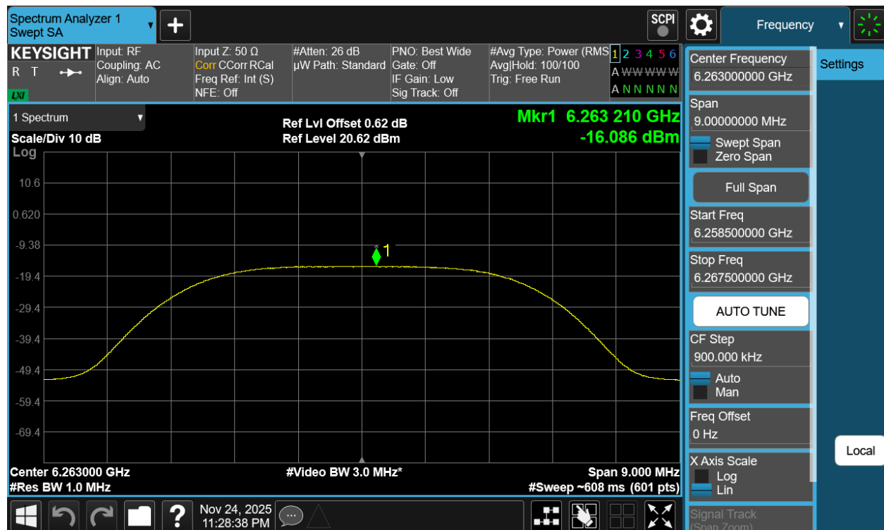
Plot 7-197. PSD TxBF Diversity Antenna 1b (NB UNII XHDRPM6, iPA – 6263MHz)
