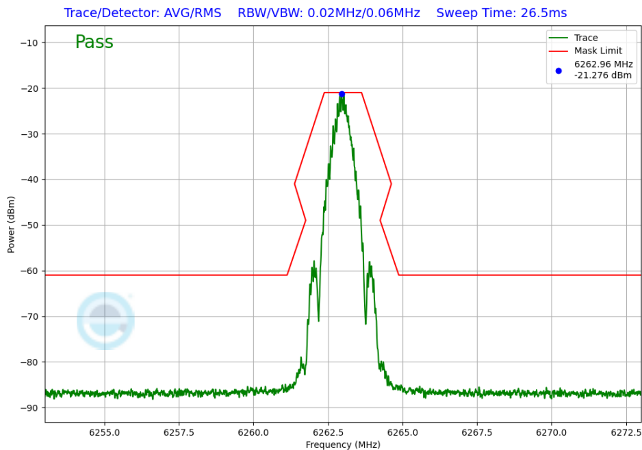
Plot 7-223. In-Band Emission Antenna 3c (NB UNII BDR, iPA – 6263MHz)
