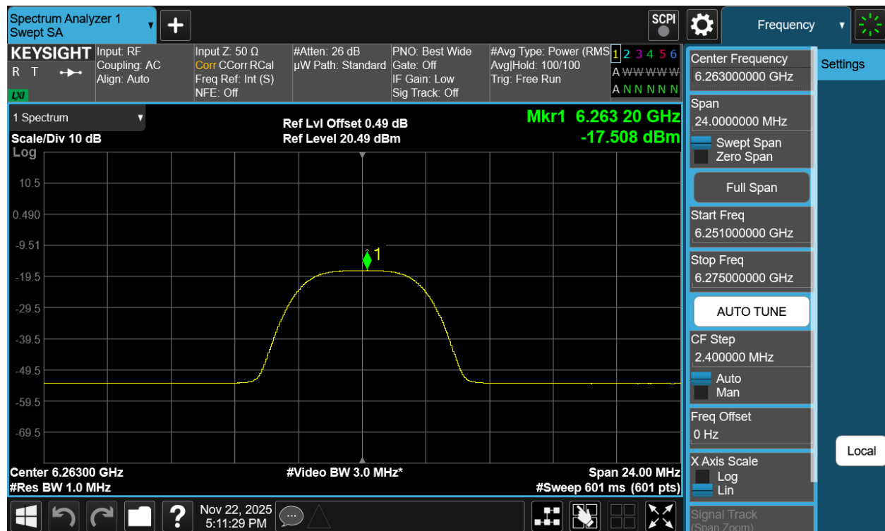
Plot 7-198. PSD TxBF Diversity Antenna 3c (NB UNII HDRPM16, ePA – 6263MHz)
