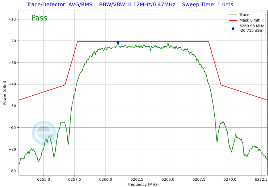
Plot 7-241. In-Band Emission Antenna 3c (NB UNII HDRPL32, iPA – 6263MHz)
