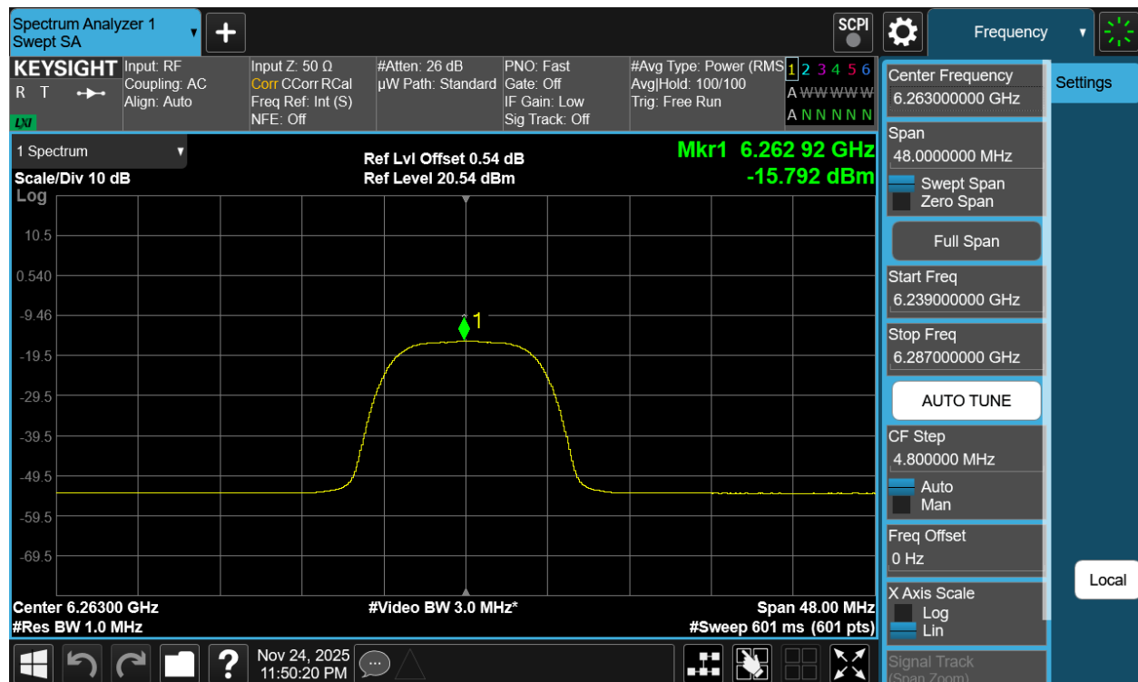
Plot 7-207. PSD TxBF Diversity Antenna 1b (NB UNII HDRPL32, ePA – 6263MHz)
