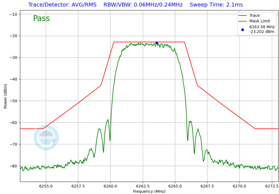
Plot 7-235. In-Band Emission Antenna 3c (NB UNII XHDRPM6, iPA – 6263MHz)
