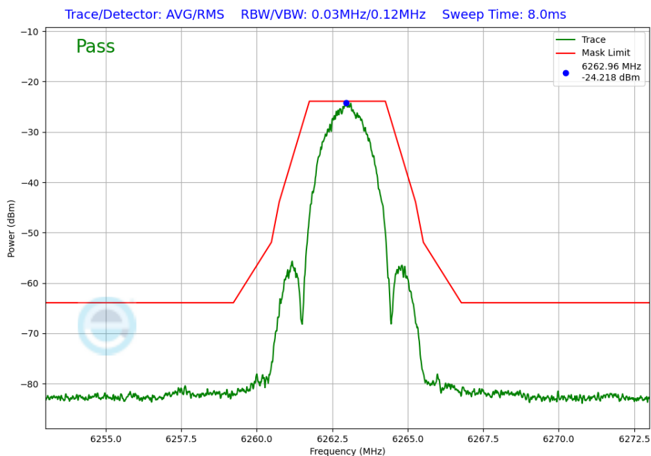
Plot 7-226. In-Band Emission Antenna 3c (NB UNII LE2M, ePA – 6263MHz)
