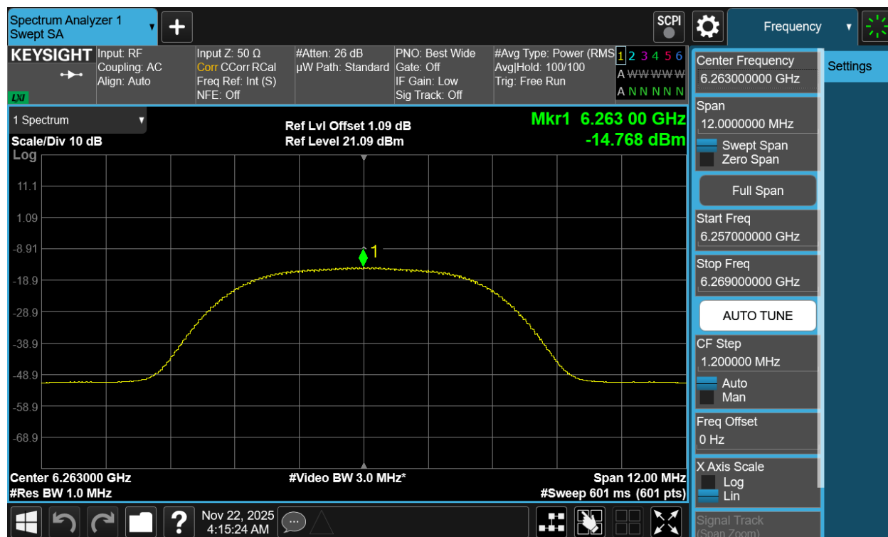
Plot 7-188. PSD TxBF Diversity Antenna 3c (NB UNII HDR8, iPA – 6263MHz)
