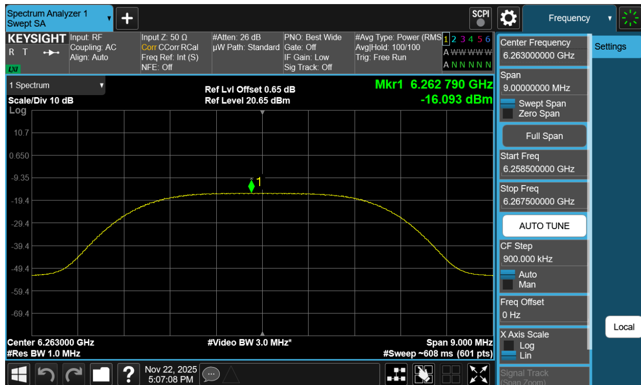
Plot 7-196. PSD TxBF Diversity Antenna 3c (NB UNII XHDRPM6, iPA – 6263MHz)
