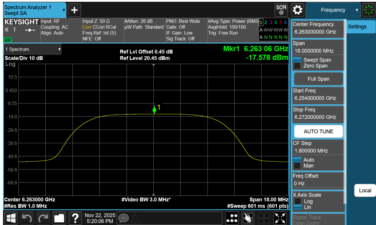
Plot 7-202. PSD TxBF Diversity Antenna 3c (NB UNII HDRPL12, ePA – 6263MHz)
