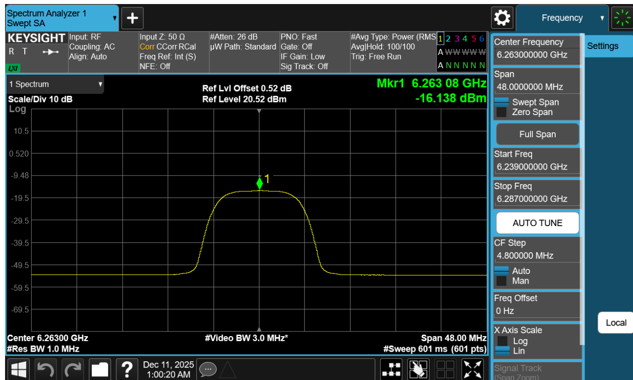
Plot 7-206. PSD TxBF Diversity Antenna 3c (NB UNII HDRPL32, ePA – 6263MHz)
