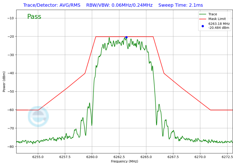
Plot 7-230. In-Band Emission Antenna 3c (NB UNII HDR8, ePA – 6263MHz)
