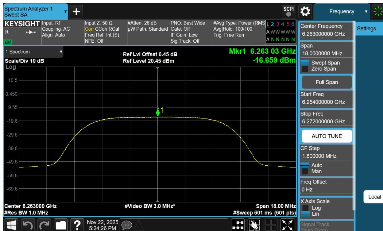
Plot 7-204. PSD TxBF Diversity Antenna 3c (NB UNII HDRPL12, iPA – 6263MHz)
