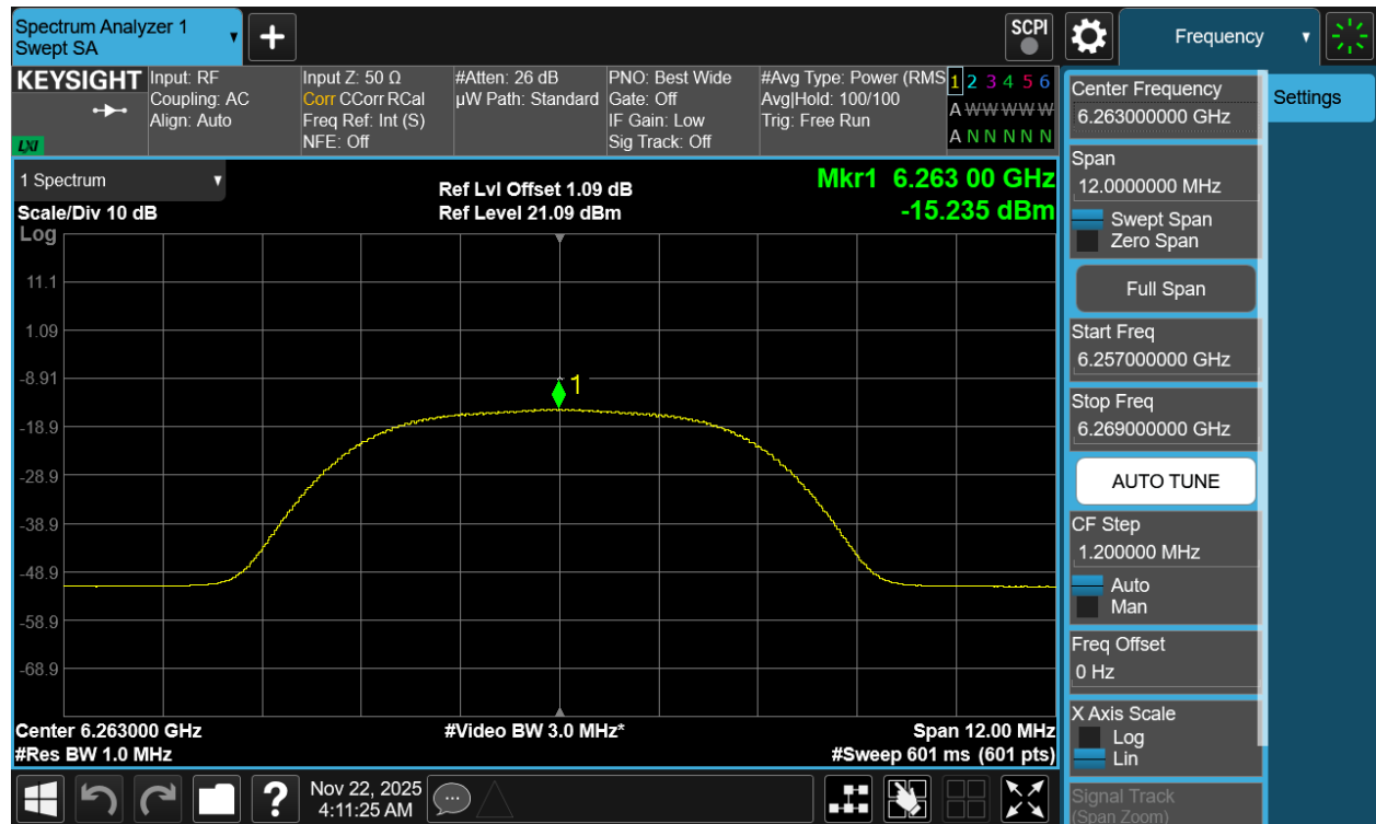
Plot 7-186. PSD TxBF Diversity Antenna 3c (NB UNII HDR8, ePA – 6263MHz)
