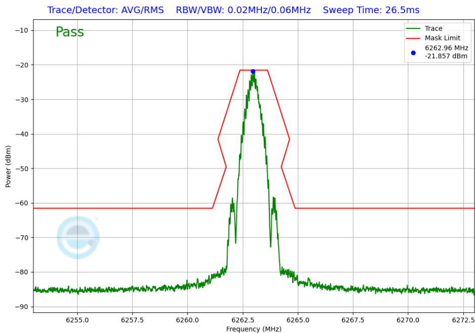
Plot 7-222. In-Band Emission Antenna 3c (NB UNII BDR, ePA – 6263MHz)
