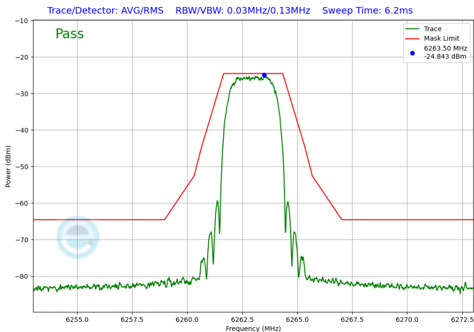
Plot 7-232. In-Band Emission Antenna 3c (NB UNII HDRPS2, ePA – 6263MHz)
