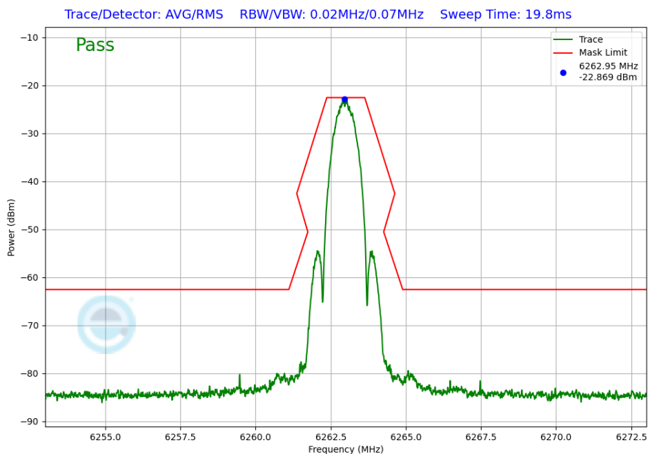
Plot 7-224. In-Band Emission Antenna 3c (NB UNII LE1M, ePA – 6263MHz)
