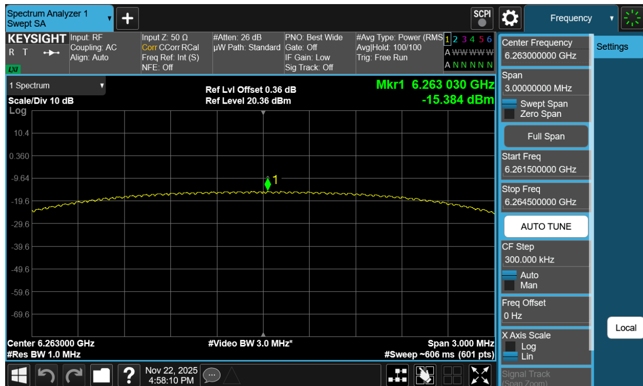
Plot 7-192. PSD TxBF Diversity Antenna 3c (NB UNII HDRPS2, iPA – 6263MHz)
