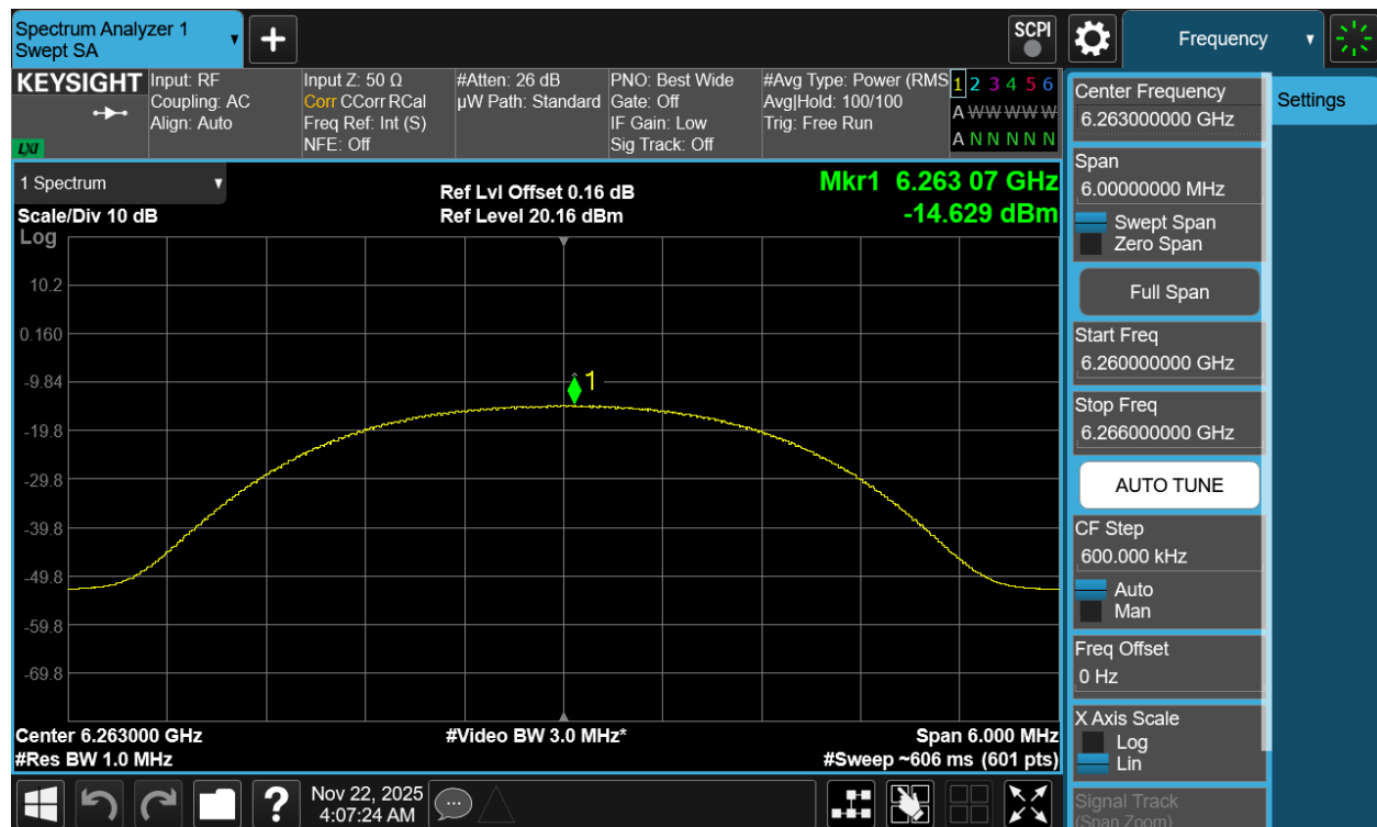
Plot 7-184. PSD Tx BF Diversity Antenna 3c (NB UNII HDR4, iPA – 6263MHz)
