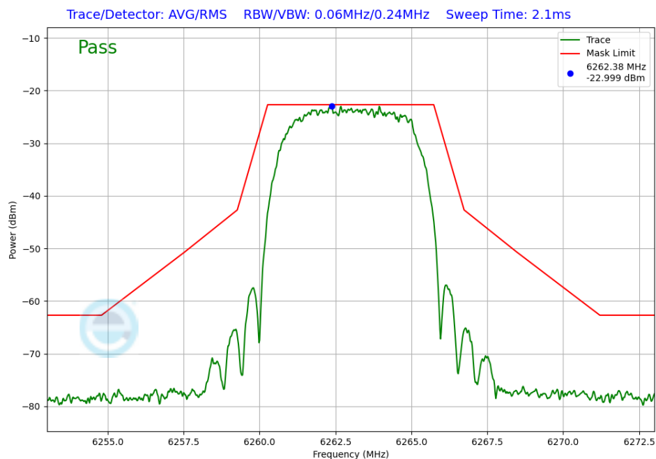
Plot 7-234. In-Band Emission Antenna 3c (NB UNII XHDRPM6, ePA – 6263MHz)
