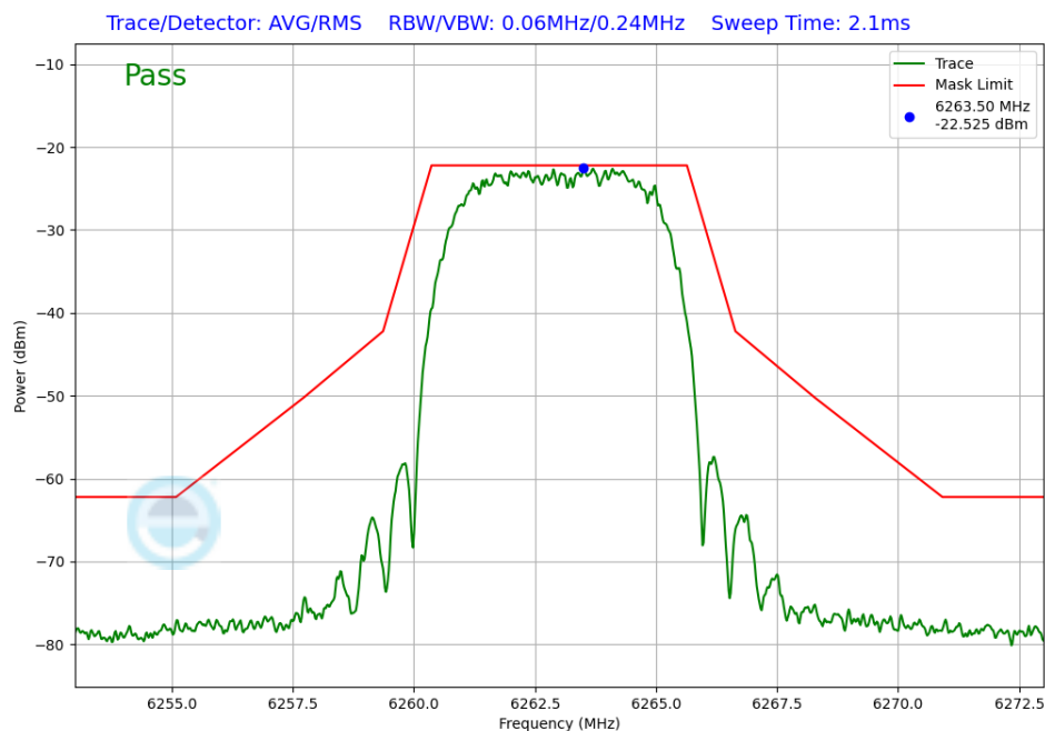
Plot 7-236. In-Band Emission Antenna 3c (NB UNII HDRPM16, ePA – 6263MHz)
