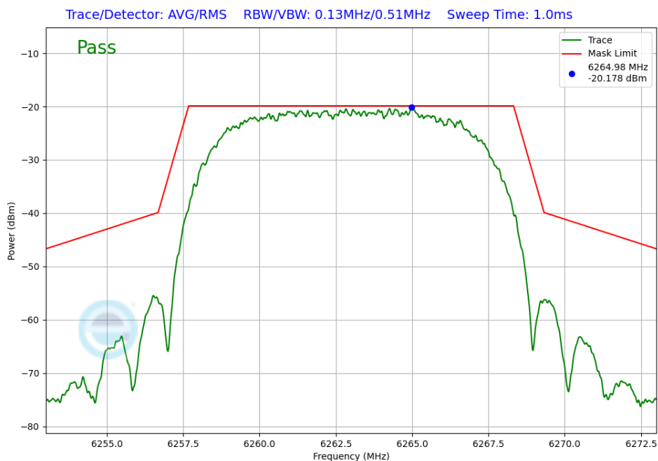
Plot 7-238. In-Band Emission Antenna 3c (NB UNII HDRPL12, ePA – 6263MHz)
