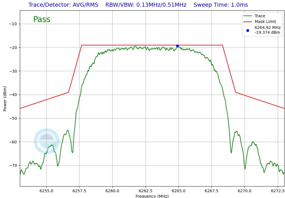
Plot 7-239. In-Band Emission Antenna 3c (NB UNII HDRPL12, iPA – 6263MHz)
