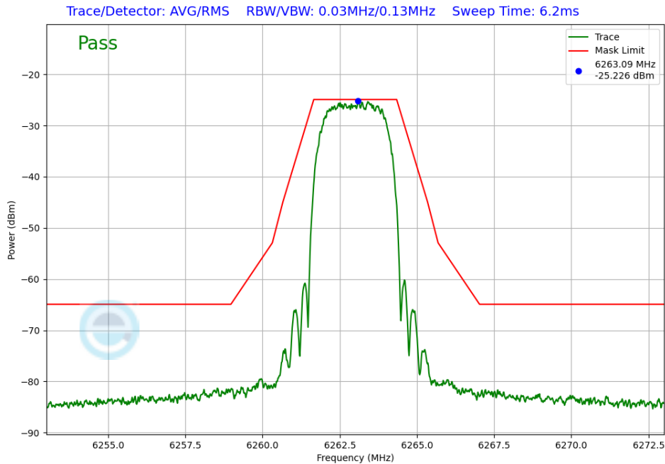
Plot 7-233. In-Band Emission Antenna 3c (NB UNII HDRPS2, iPA – 6263MHz)
