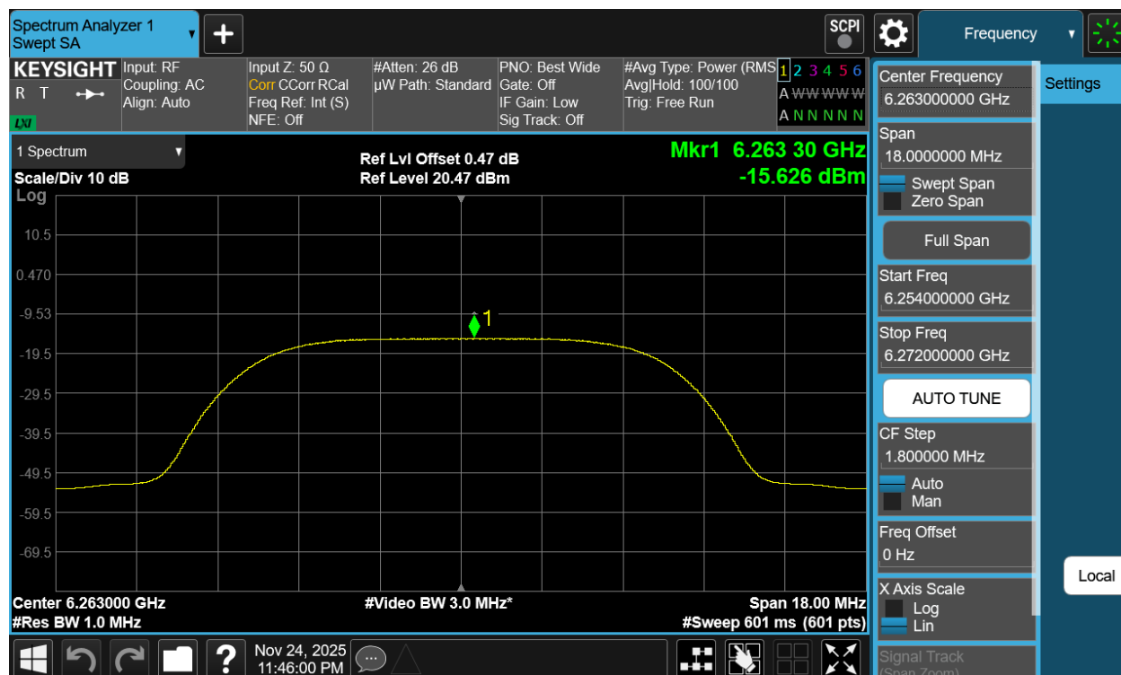
Plot 7-205. PSD TxBF Diversity Antenna 1b (NB UNII HDRPL12, iPA – 6263MHz)
