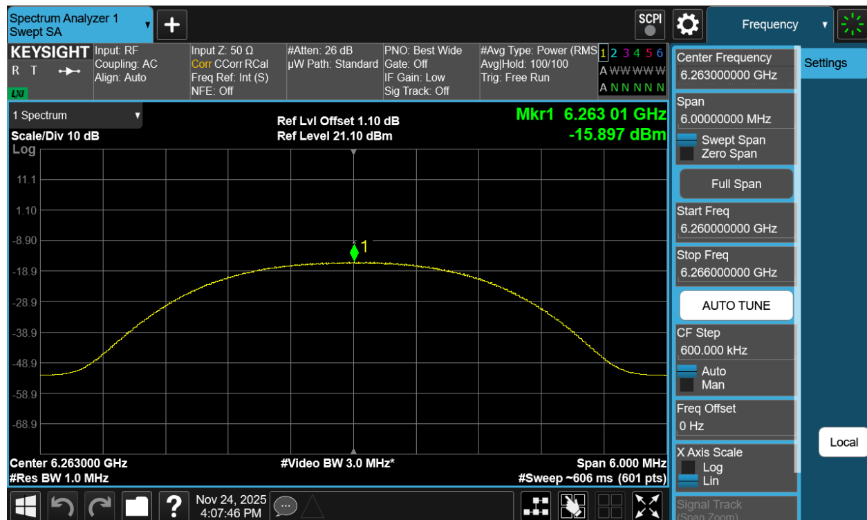
Plot 7-185. PSD Tx BF Diversity Antenna 1b (NB UNII HDR4, iPA – 6263MHz)
