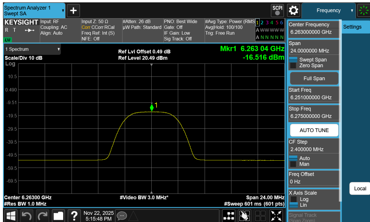
Plot 7-200. PSD TxBF Diversity Antenna 3c (NB UNII HDRPM16, iPA – 6263MHz)
