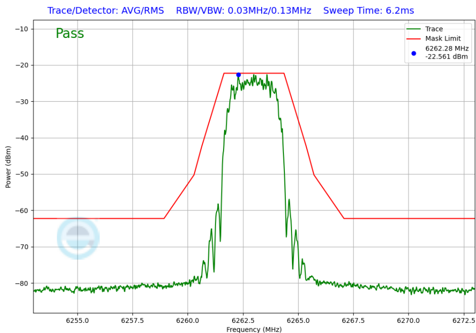
Plot 7-228. In-Band Emission Antenna 3c (NB UNII HDR4, ePA – 6263MHz)
