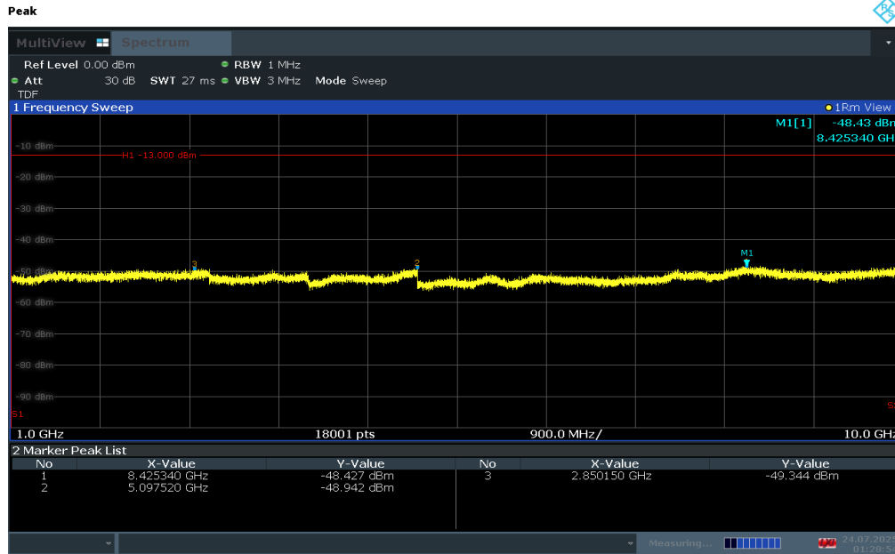
Plot 7-44. Conducted Spurious Plot (LTE Band 26/5 – 10MHz QPSK – RB Size 1, RB Offset 0 – Low Channel)
