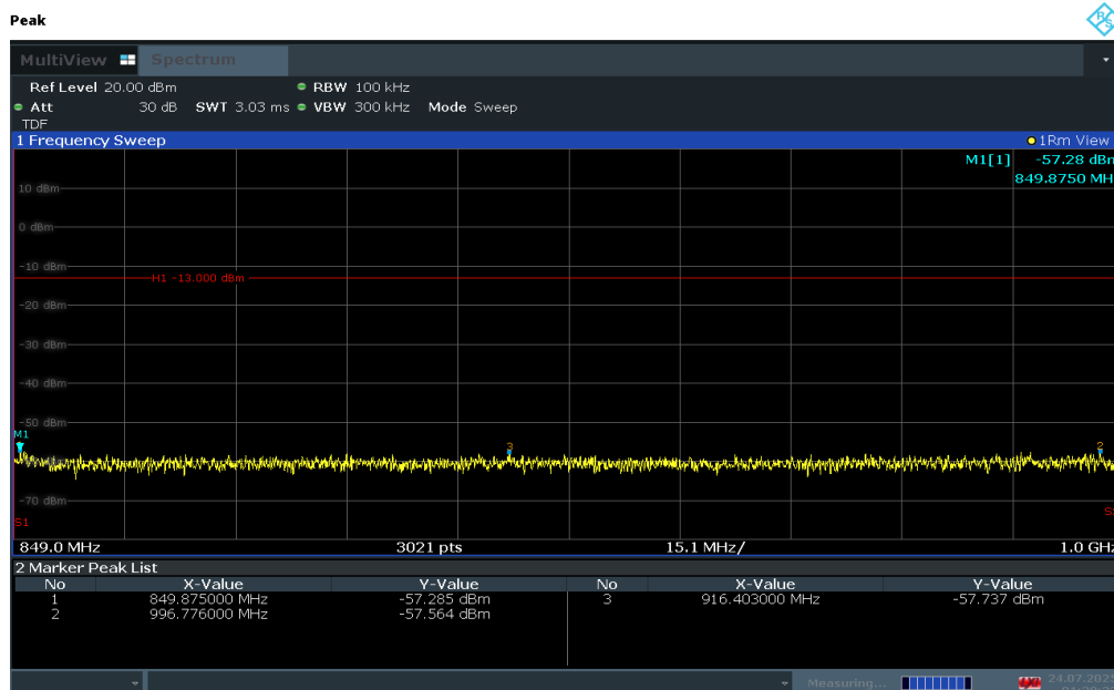
Plot 7-46. Conducted Spurious Plot (LTE Band 26/5 – 10MHz QPSK – RB Size 1, RB Offset 0 – Mid Channel)
