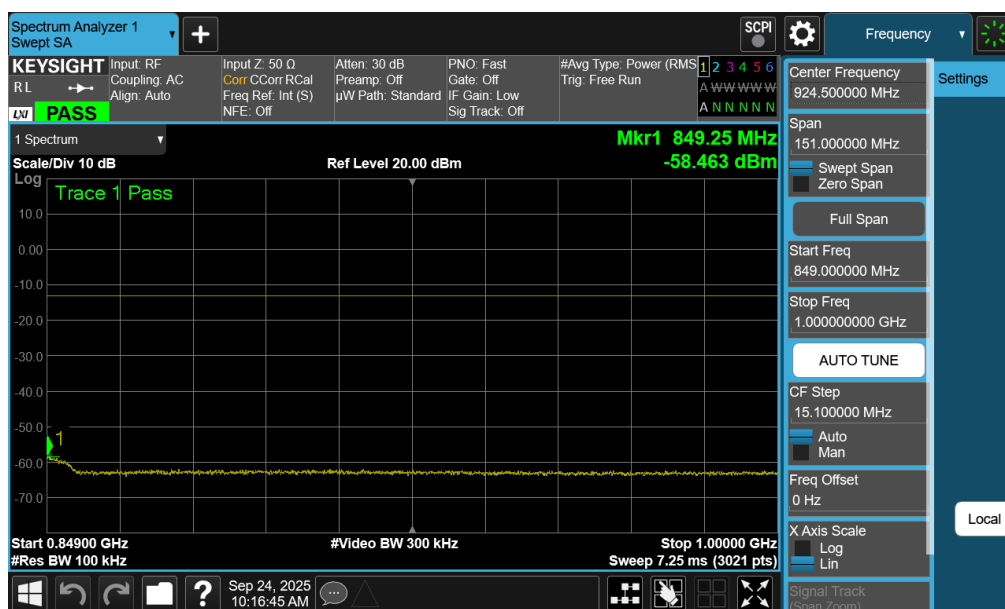
Plot 7-70. Conducted Spurious Plot (WCDMA Ch. 4132)
