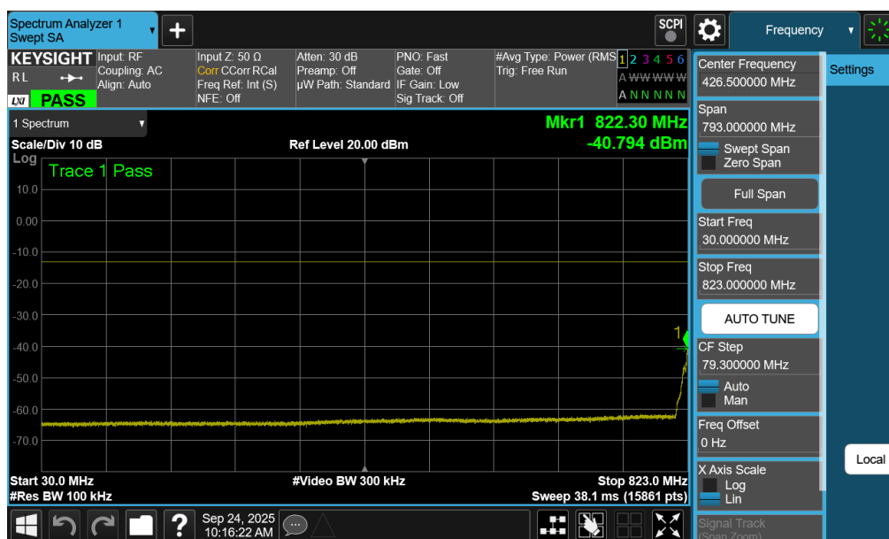
Plot 7-69. Conducted Spurious Plot (WCDMA Ch. 4132)
