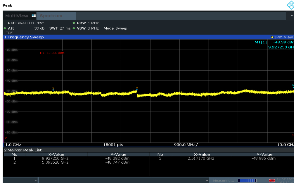
Plot 7-50. Conducted Spurious Plot (LTE Band 26/5 – 10MHz QPSK – RB Size 1, RB Offset 0 – High Channel)
