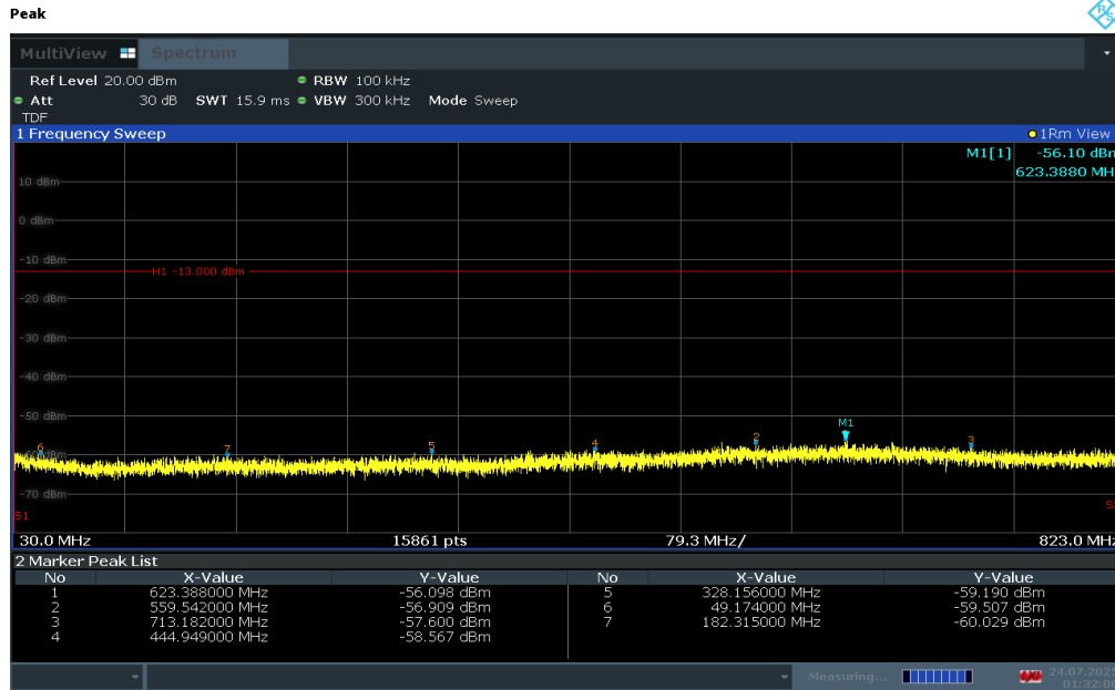
Plot 7-48. Conducted Spurious Plot (LTE Band 26/5 – 10MHz QPSK – RB Size 1, RB Offset 0 – High Channel)
