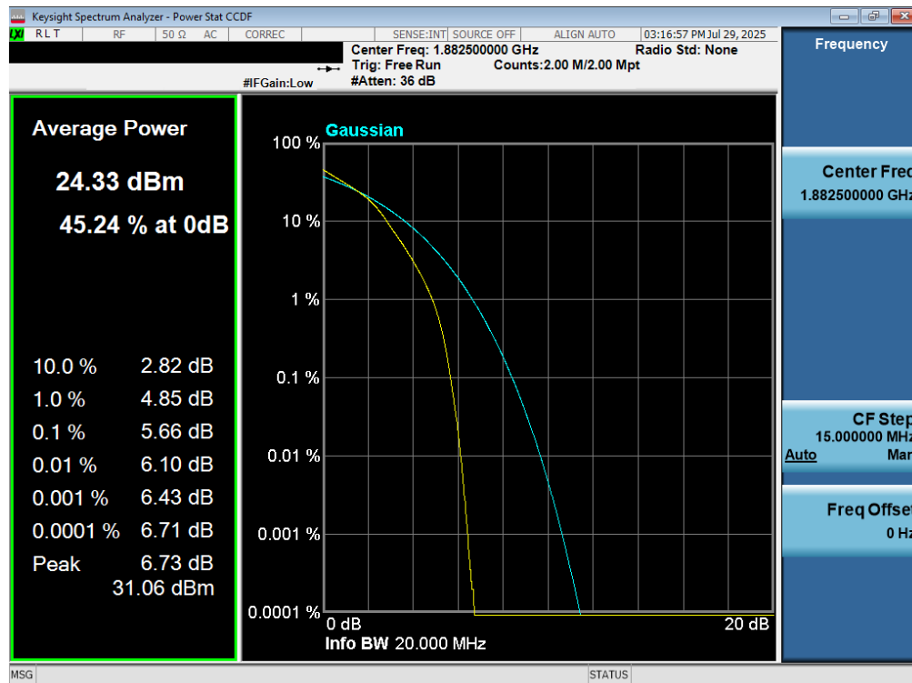
Plot 7-230. PAR Plot (LTE Band 25 - 20MHz 16-QAM - Full RB Configuration)
