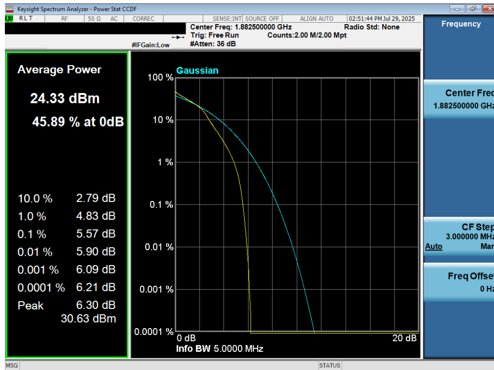
Plot 7-218. PAR Plot (LTE Band 25 - 5MHz 16-QAM - Full RB Configuration)
