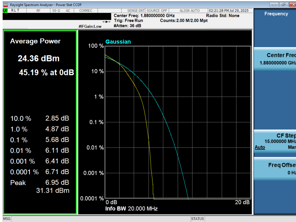
Plot 7-254. PAR Plot (LTE Band 2 - 20MHz 16-QAM - Full RB Configuration)
