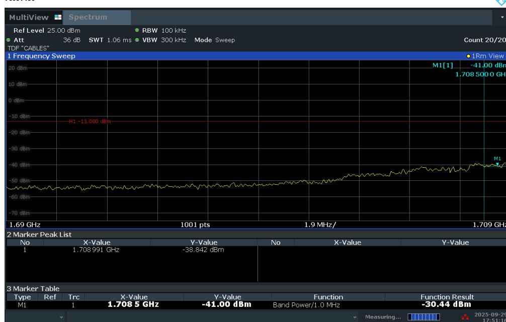
Plot 7-246. Lower Extended Band Edge Plot (LTE Band 66 – 3MHz QPSK – Full RB)
