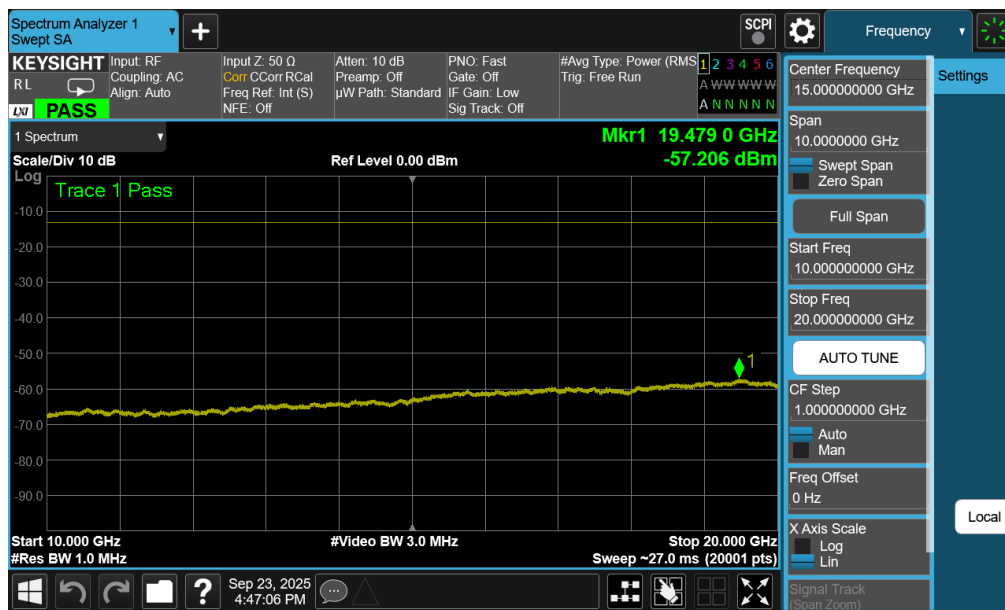
Plot 7-237. Conducted Spurious Plot (WCDMA Ch. 1413- Mid Channel)
