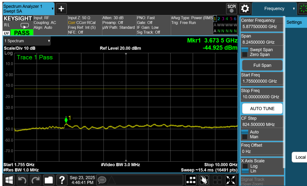
Plot 7-236. Conducted Spurious Plot (WCDMA Ch. 1413- Mid Channel)
