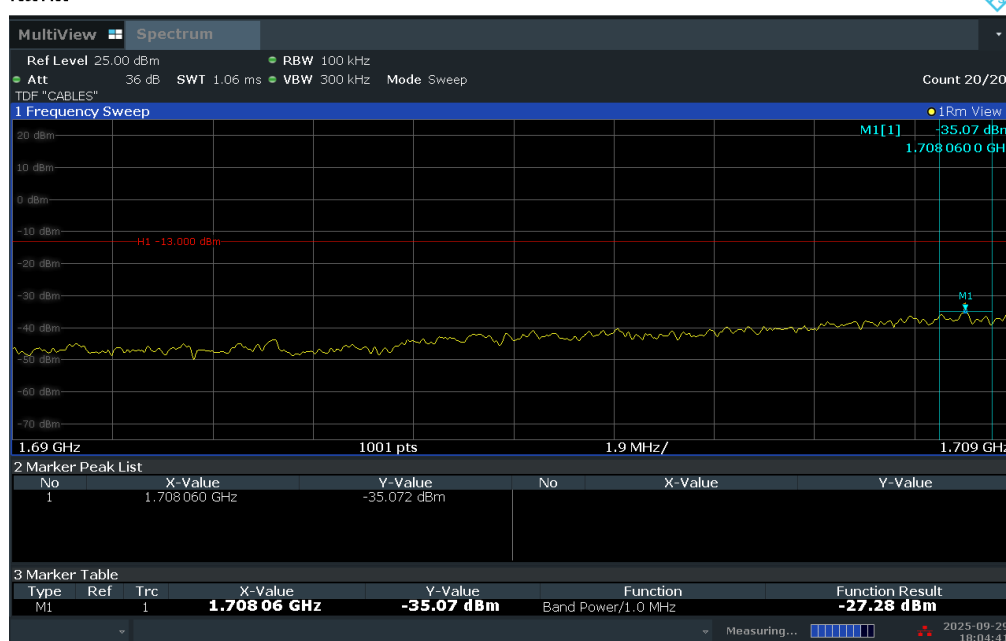
Plot 7-258. Lower Extended Band Edge Plot (LTE Band 66 – 15MHz QPSK – Full RB)
