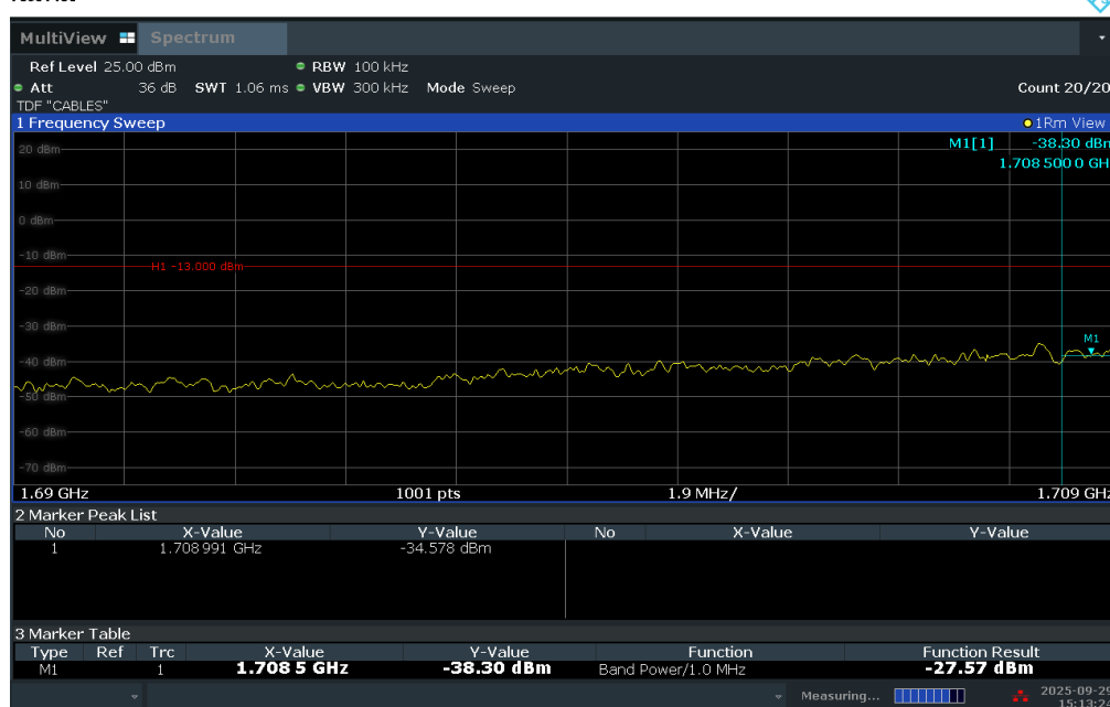
Plot 7-282. Lower Extended Band Edge Plot (LTE Band 4 – 15MHz QPSK – Full RB)
