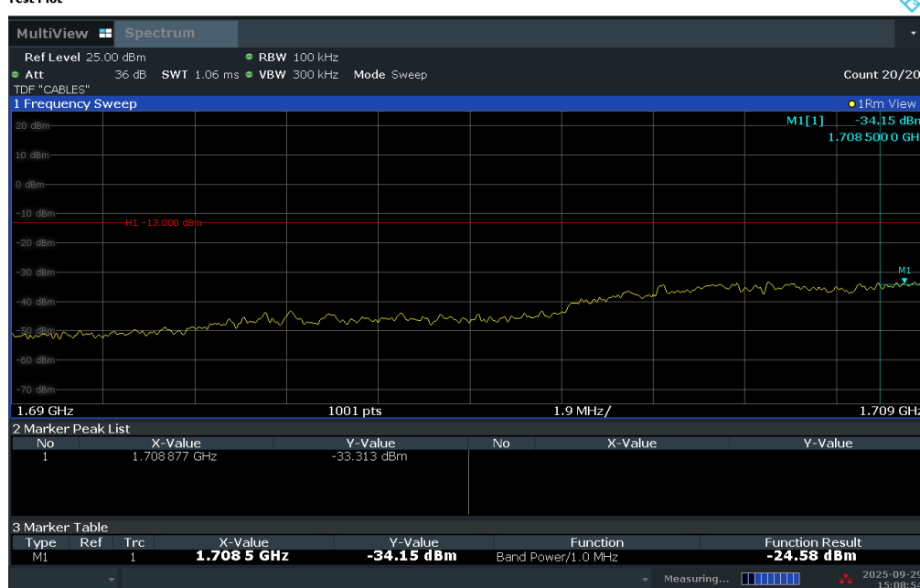
Plot 7-278. Lower Extended Band Edge Plot (LTE Band 4 – 10MHz QPSK – Full RB)
