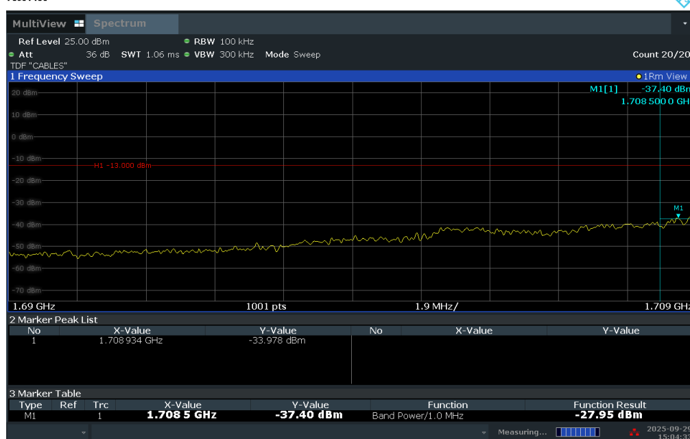
Plot 7-274. Lower Extended Band Edge Plot (LTE Band 4 – 5MHz QPSK – Full RB)
