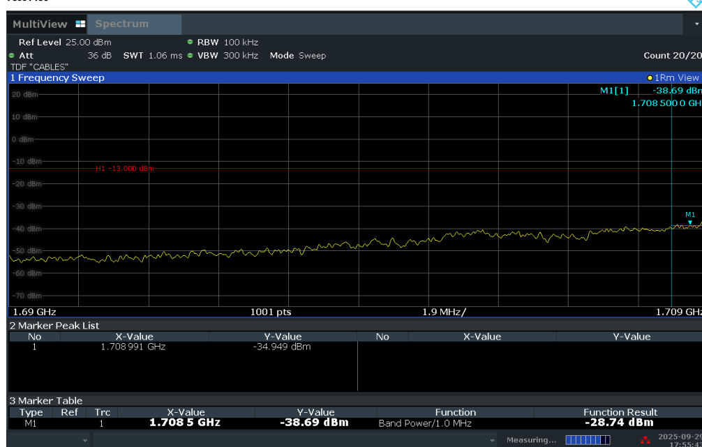
Plot 7-250. Lower Extended Band Edge Plot (LTE Band 66 – 5MHz QPSK – Full RB)
