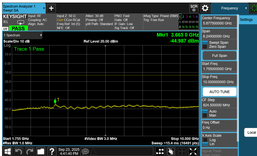
Plot 7-233. Conducted Spurious Plot (WCDMA Ch. 1312- Low Channel)
