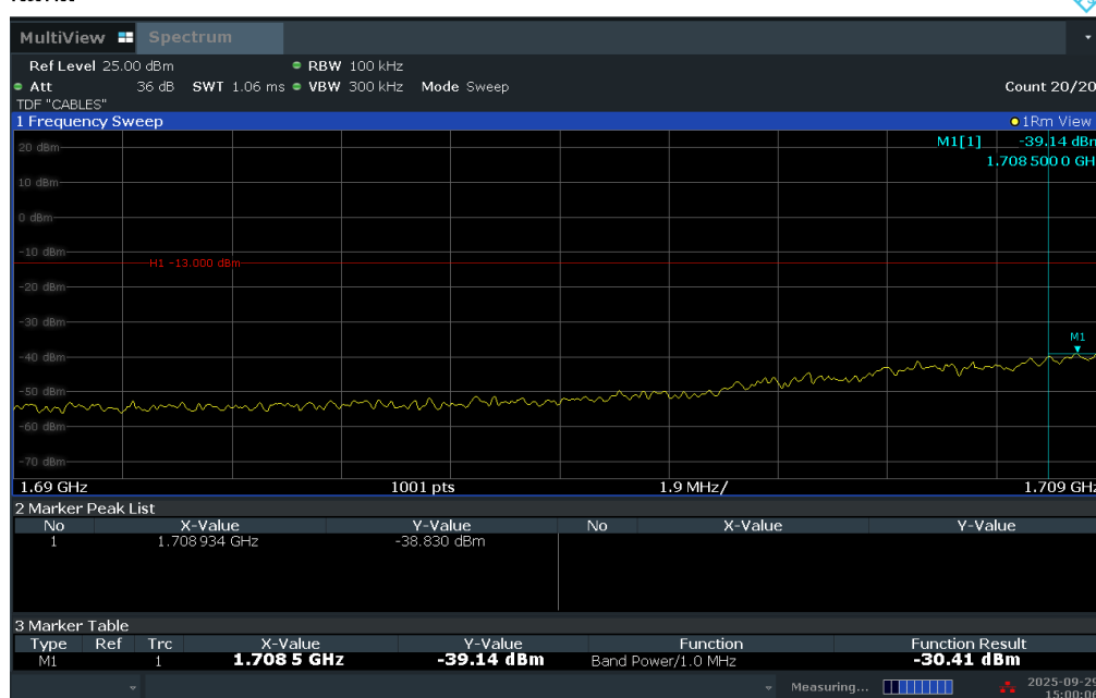
Plot 7-270. Lower Extended Band Edge Plot (LTE Band 4 – 3MHz QPSK – Full RB)
