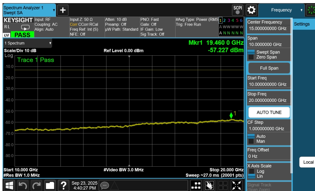
Plot 7-240. Conducted Spurious Plot (WCDMA Ch. 1513- High Channel)
