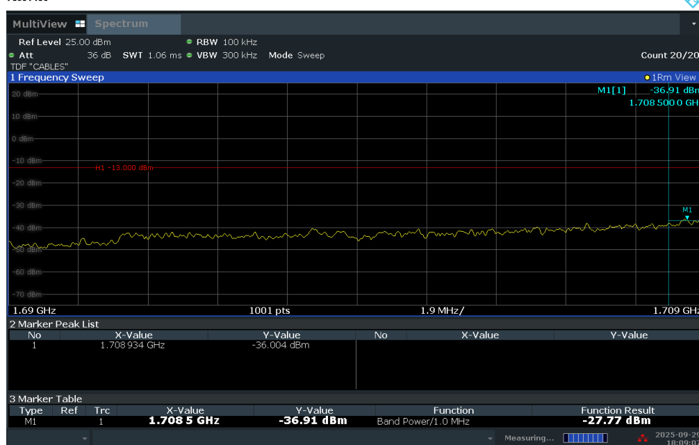
Plot 7-262. Lower Extended Band Edge Plot (LTE Band 66 – 20MHz QPSK – Full RB)
