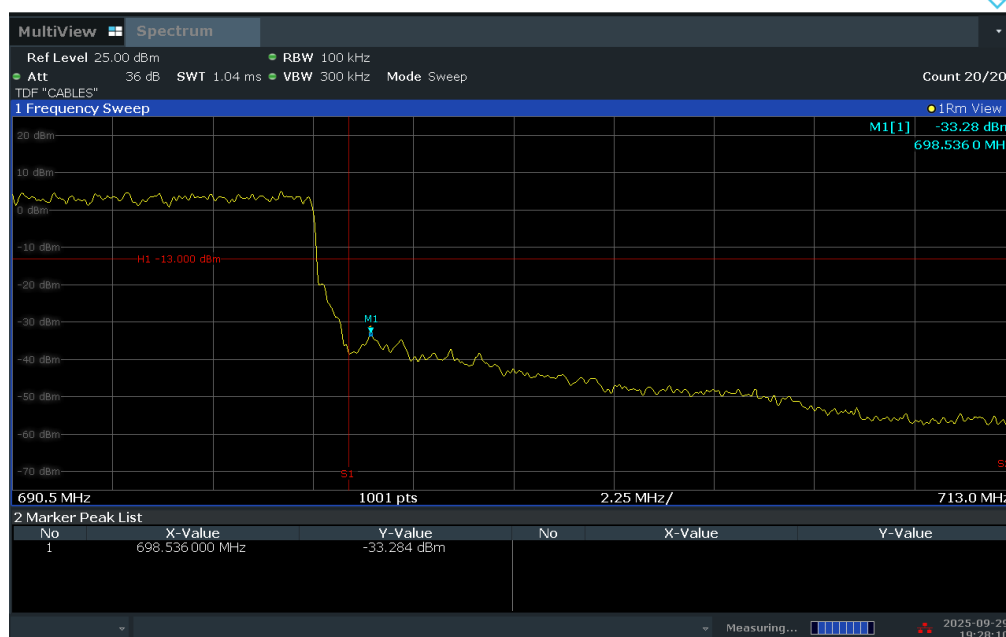
Plot 7-294. Upper Band Edge Plot (LTE Band 71 - 15MHz QPSK – Full RB)
