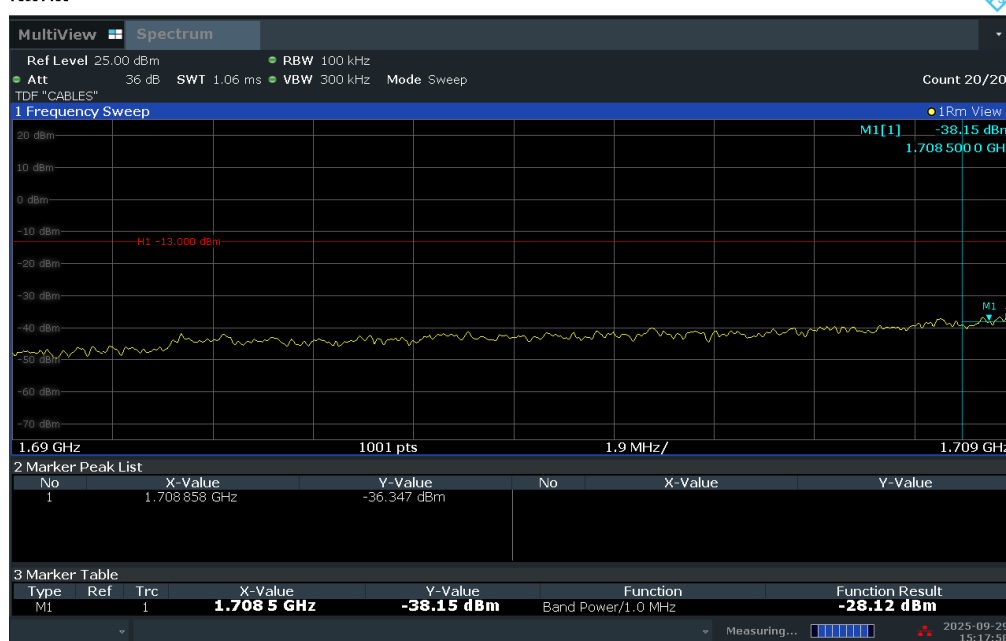
Plot 7-286. Lower Extended Band Edge Plot (LTE Band 4 – 20MHz QPSK – Full RB)
