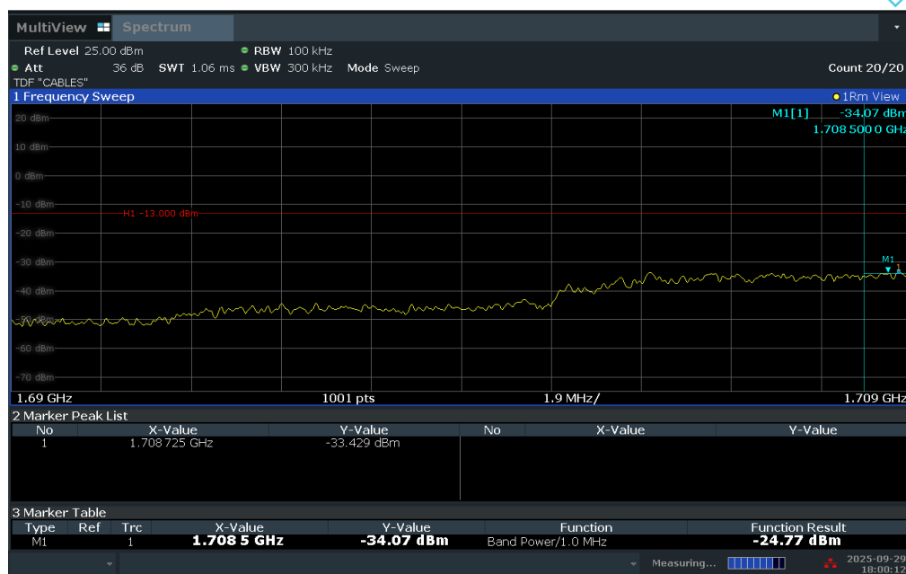
Plot 7-254. Lower Extended Band Edge Plot (LTE Band 66 – 10MHz QPSK – Full RB)
