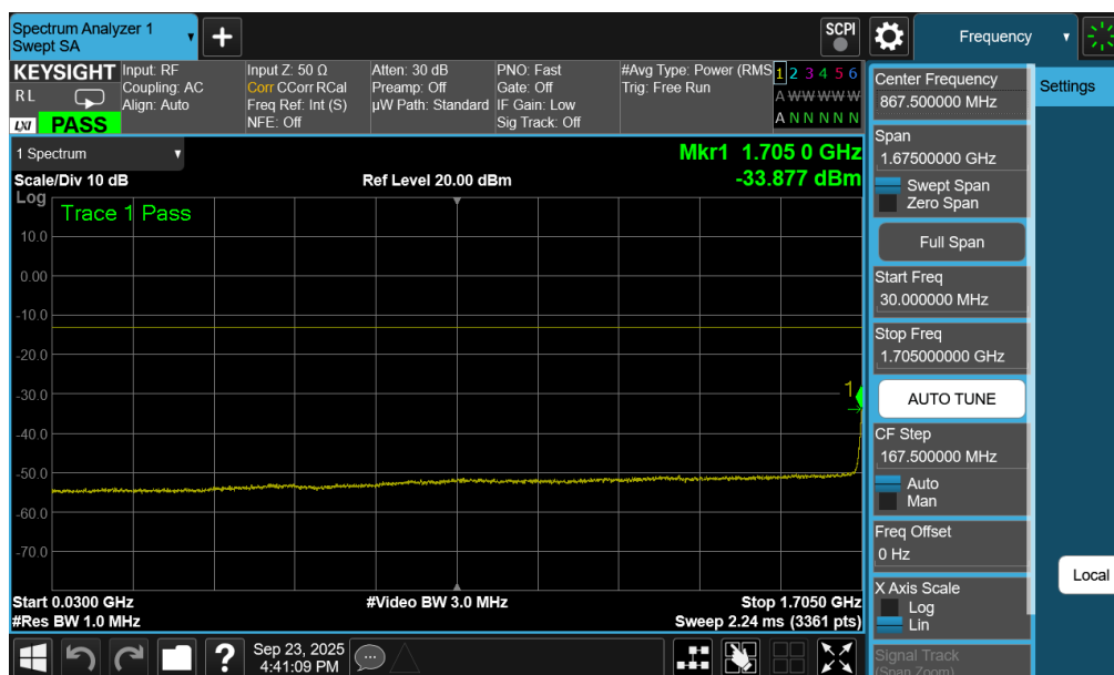
Plot 7-232. Conducted Spurious Plot (WCDMA Ch. 1312- Low Channel)
