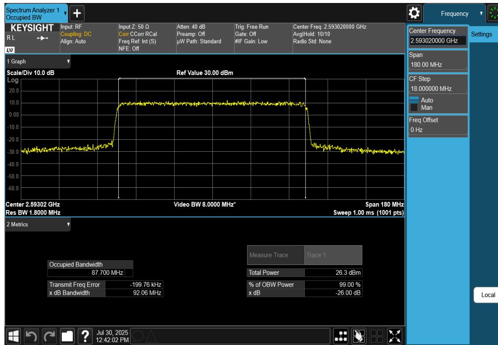
Plot 7-158. Occupied Bandwidth Plot (NR Band n41 - 90MHz CP-OFDM 16-QAM - Full RB)
