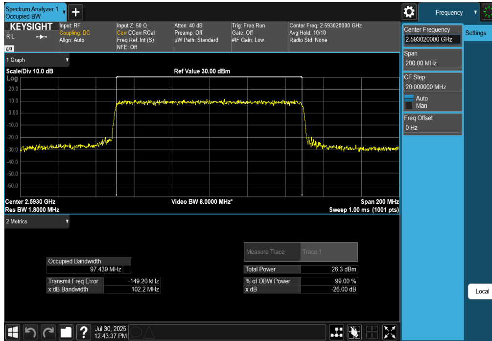
Plot 7-162. Occupied Bandwidth Plot (NR Band n41 - 100MHz CP-OFDM QPSK - Full RB)
