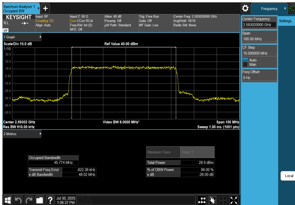
Plot 7-136. Occupied Bandwidth Plot (NR Band n41 - 50MHz DFT-s-OFDM \pi/2 BPSK - Full RB)
