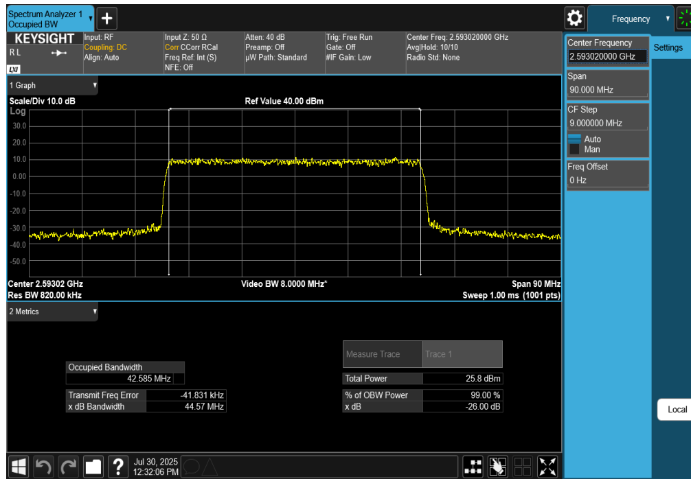
Plot 7-134. Occupied Bandwidth Plot (NR Band n41 - 45MHz CP-OFDM 64-QAM - Full RB)
