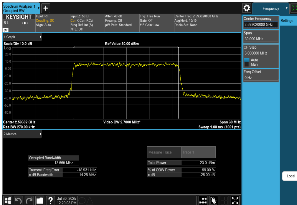
Plot 7-105. Occupied Bandwidth Plot (NR Band n41 - 15MHz CP-OFDM 256-QAM - Full RB)
