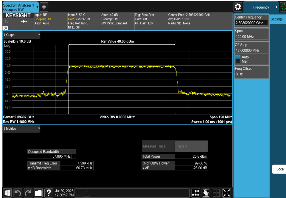
Plot 7-144. Occupied Bandwidth Plot (NR Band n41 - 60MHz CP-OFDM 64-QAM - Full RB)
