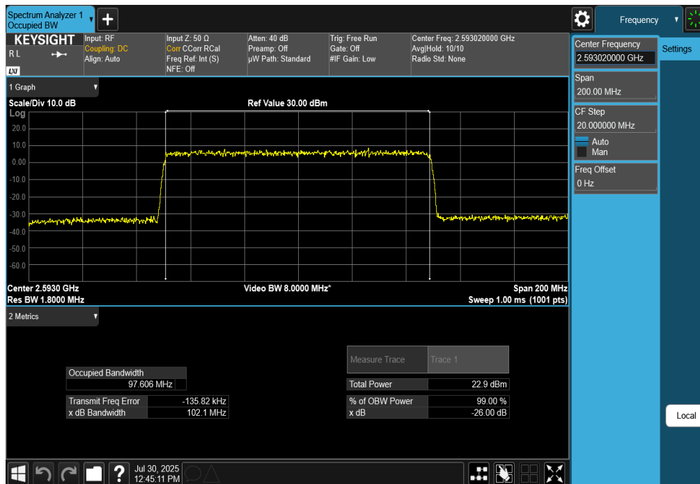
Plot 7-165. Occupied Bandwidth Plot (NR Band n41 - 100MHz CP-OFDM 256-QAM - Full RB)
