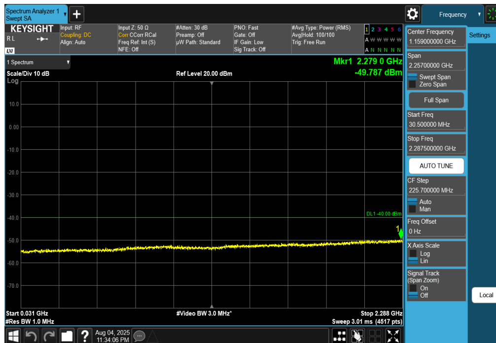
Plot 7-204. Conducted Spurious Plot (NR Band n30 - 10MHz DFT-s-OFDM QPSK – RB Size 1, RB Offset 0 – Mid Channel)
