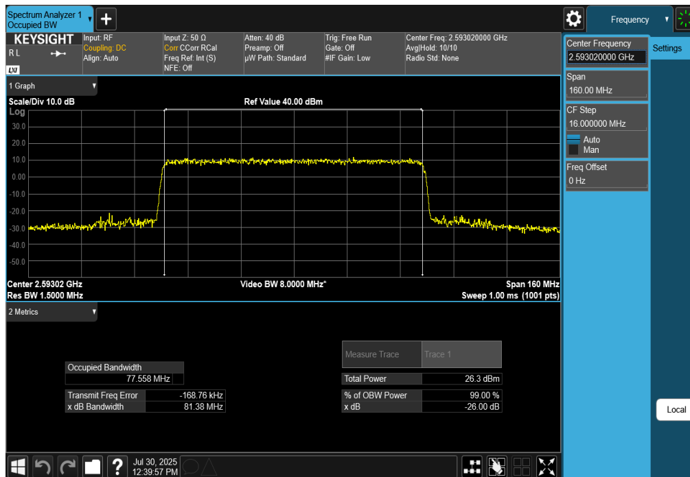
Plot 7-153. Occupied Bandwidth Plot (NR Band n41 - 80MHz CP-OFDM 16-QAM - Full RB)
