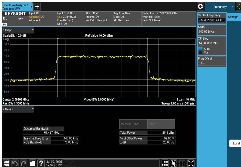
Plot 7-147. Occupied Bandwidth Plot (NR Band n41 - 70MHz CP-OFDM QPSK - Full RB)
