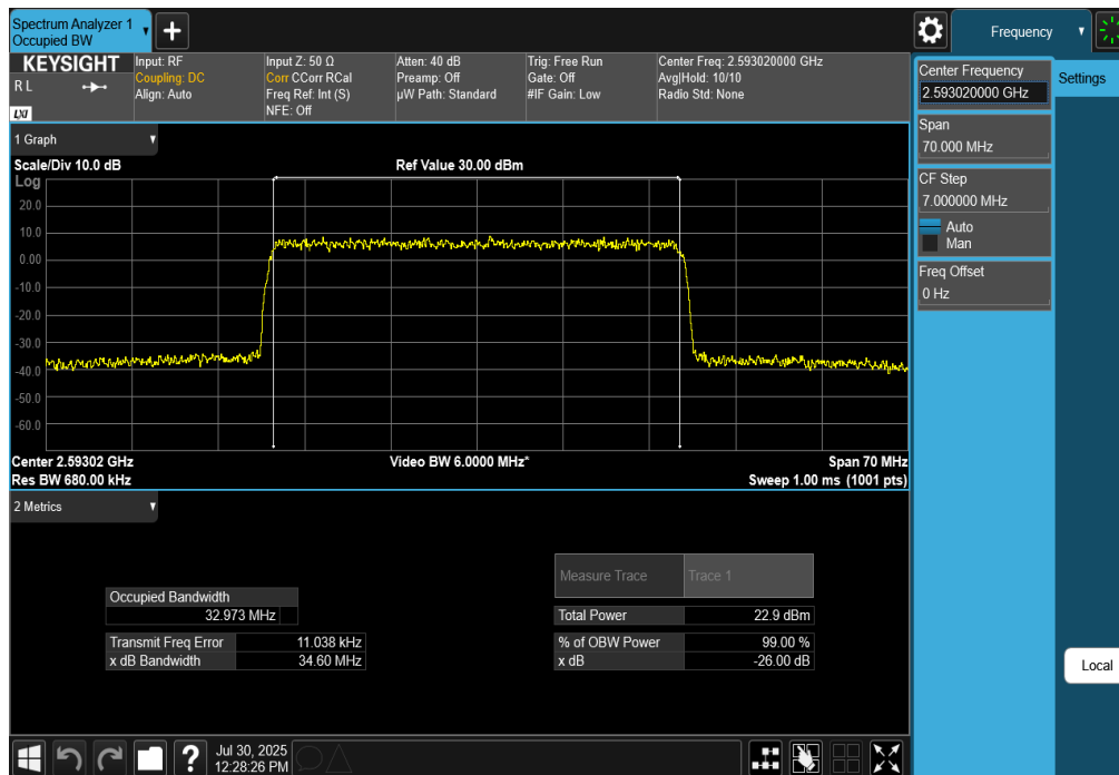
Plot 7-125. Occupied Bandwidth Plot (NR Band n41 - 35MHz CP-OFDM 256-QAM - Full RB)
