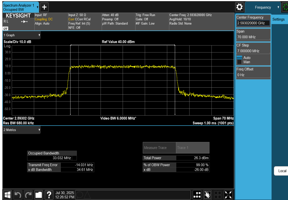
Plot 7-122. Occupied Bandwidth Plot (NR Band n41 - 35MHz CP-OFDM QPSK - Full RB)
