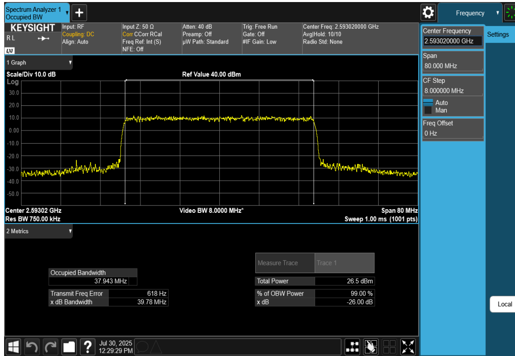
Plot 7-128. Occupied Bandwidth Plot (NR Band n41 - 40MHz CP-OFDM 16-QAM - Full RB)
