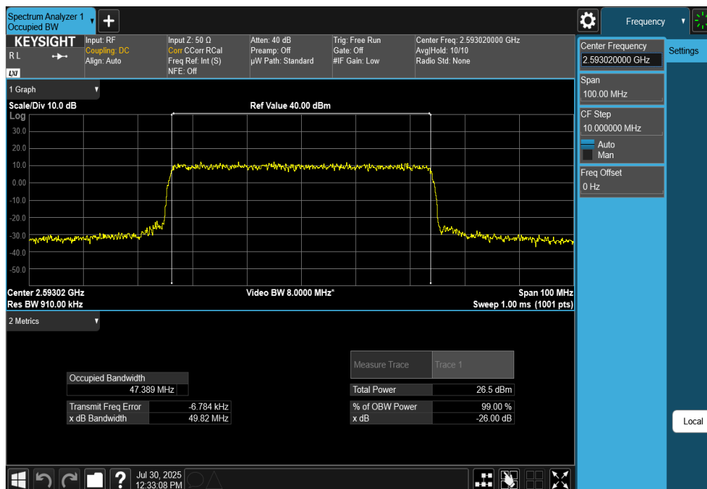
Plot 7-137. Occupied Bandwidth Plot (NR Band n41 - 50MHz CP-OFDM QPSK - Full RB)
