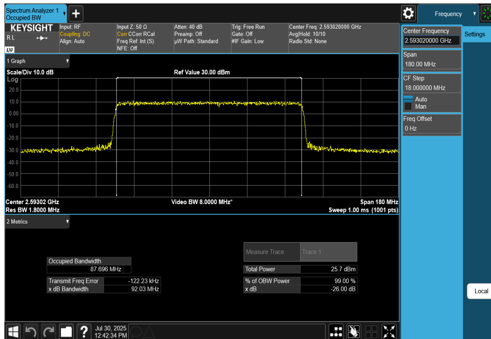
Plot 7-159. Occupied Bandwidth Plot (NR Band n41 - 90MHz CP-OFDM 64-QAM - Full RB)
