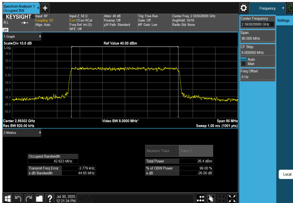
Plot 7-133. Occupied Bandwidth Plot (NR Band n41 - 45MHz CP-OFDM 16-QAM - Full RB)
