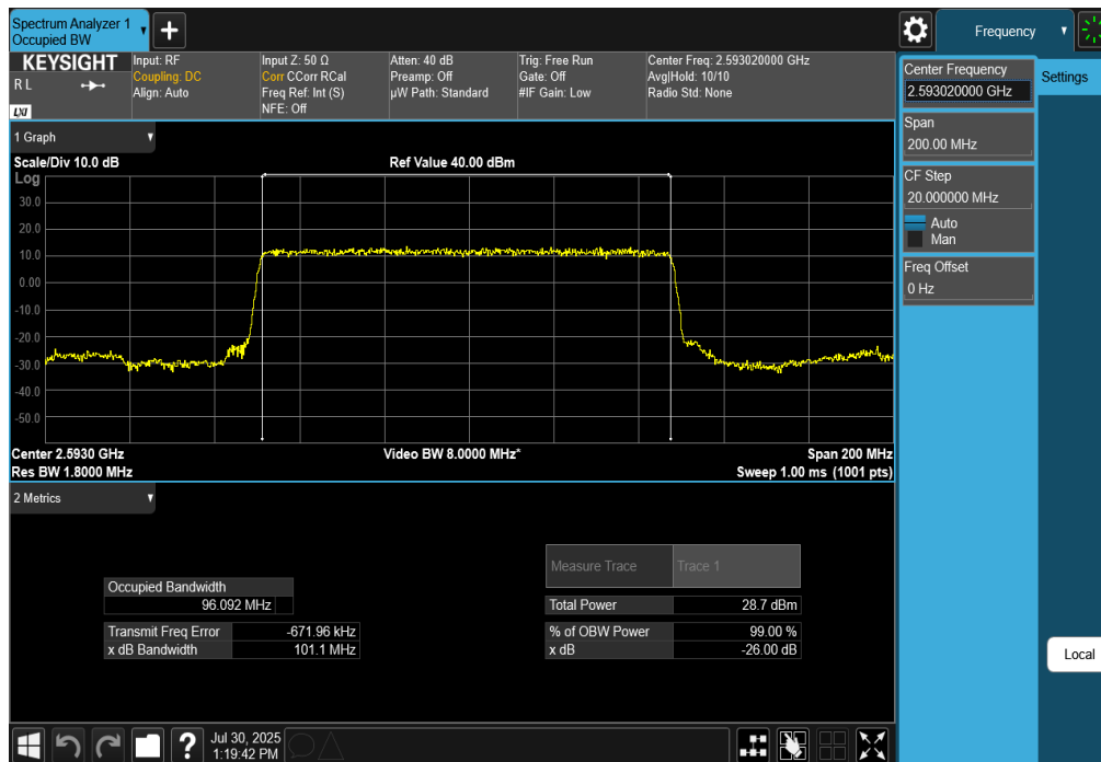
Plot 7-161. Occupied Bandwidth Plot (NR Band n41 - 100MHz DFT-s-OFDM \pi/2 BPSK - Full RB)
