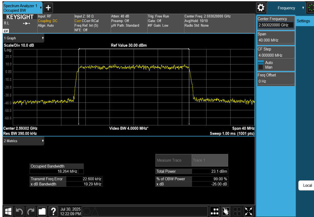
Plot 7-110. Occupied Bandwidth Plot (NR Band n41 - 20MHz CP-OFDM 256-QAM - Full RB)
