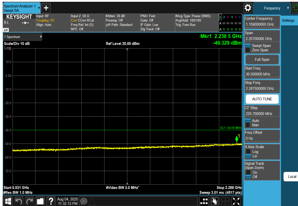
Plot 7-201. Conducted Spurious Plot (NR Band n30 - 5MHz DFT-s-OFDM QPSK – RB Size 1, RB Offset 0 – Low Channel)
