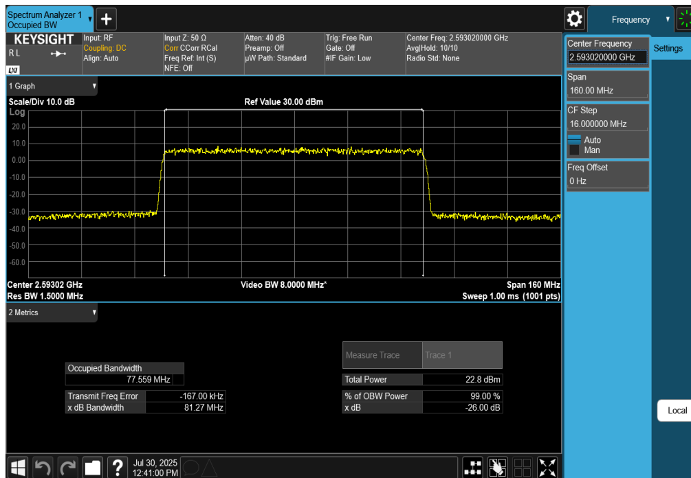
Plot 7-155. Occupied Bandwidth Plot (NR Band n41 - 80MHz CP-OFDM 256-QAM - Full RB)
