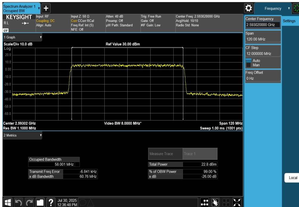
Plot 7-145. Occupied Bandwidth Plot (NR Band n41 - 60MHz CP-OFDM 256-QAM - Full RB)
