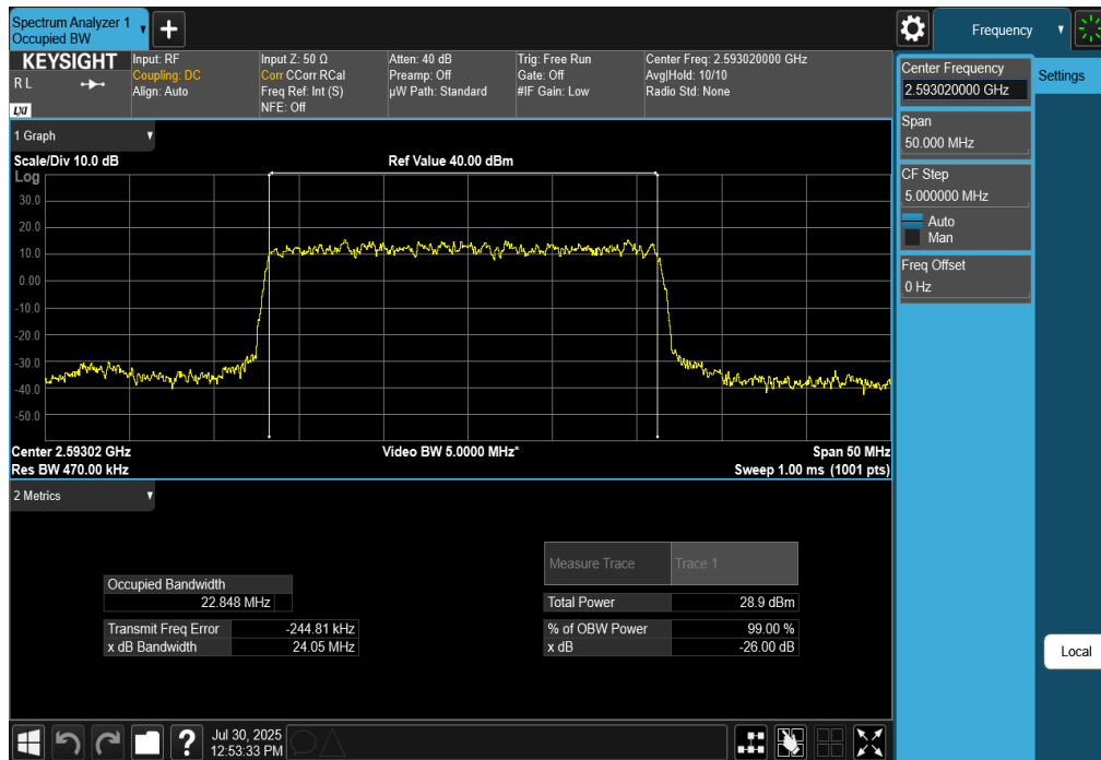
Plot 7-111. Occupied Bandwidth Plot (NR Band n41 - 25MHz DFT-s-OFDM \pi/2 BPSK - Full RB)
