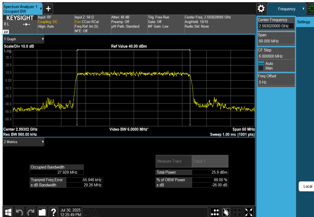
Plot 7-119. Occupied Bandwidth Plot (NR Band n41 - 30MHz CP-OFDM 64-QAM - Full RB)
