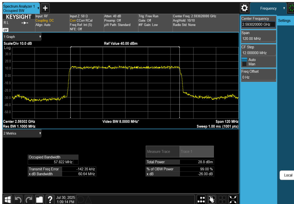
Plot 7-141. Occupied Bandwidth Plot (NR Band n41 - 60MHz DFT-s-OFDM \pi/2 BPSK - Full RB)
