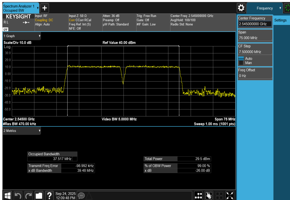
Plot 7-169. Occupied Bandwidth Plot (ULCA LTE Band 7 – (20+20)MHz 256-QAM - Full RB)
