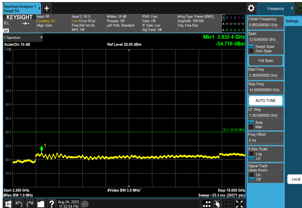
Plot 7-202. Conducted Spurious Plot (NR Band n30 - 5MHz DFT-s-OFDM QPSK – RB Size 1, RB Offset 0 – Low Channel)
