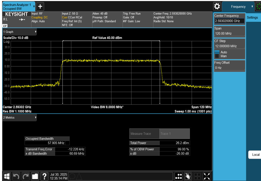
Plot 7-142. Occupied Bandwidth Plot (NR Band n41 - 60MHz CP-OFDM QPSK - Full RB)
