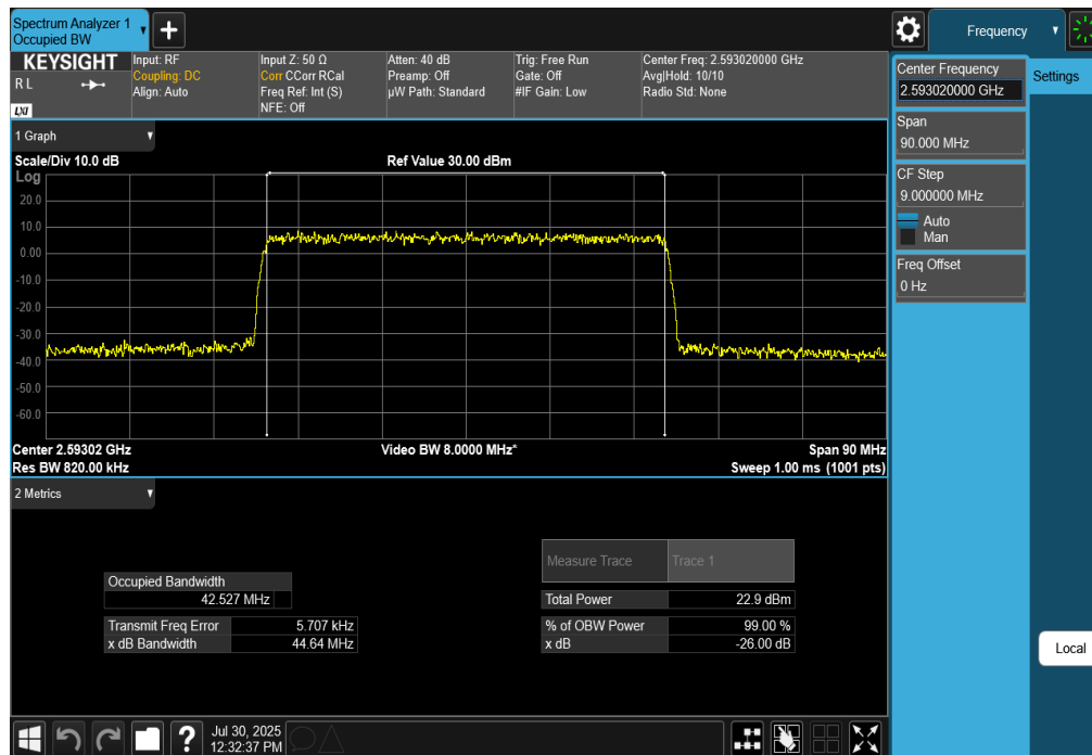
Plot 7-135. Occupied Bandwidth Plot (NR Band n41 - 45MHz CP-OFDM 256-QAM - Full RB)
