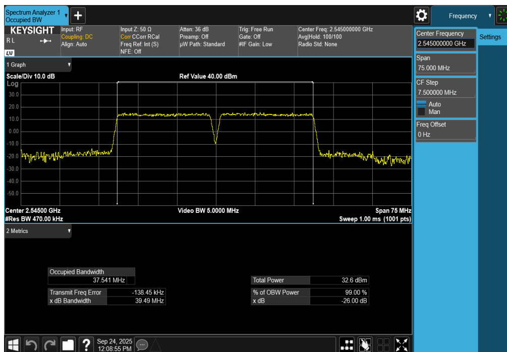
Plot 7-167. Occupied Bandwidth Plot (ULCA LTE Band 7 – (20+20)MHz 16-QAM - Full RB)
