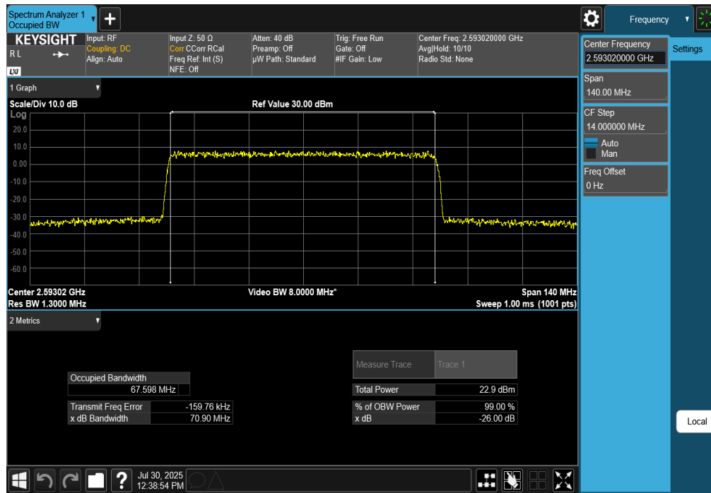
Plot 7-150. Occupied Bandwidth Plot (NR Band n41 - 70MHz CP-OFDM 256-QAM - Full RB)
