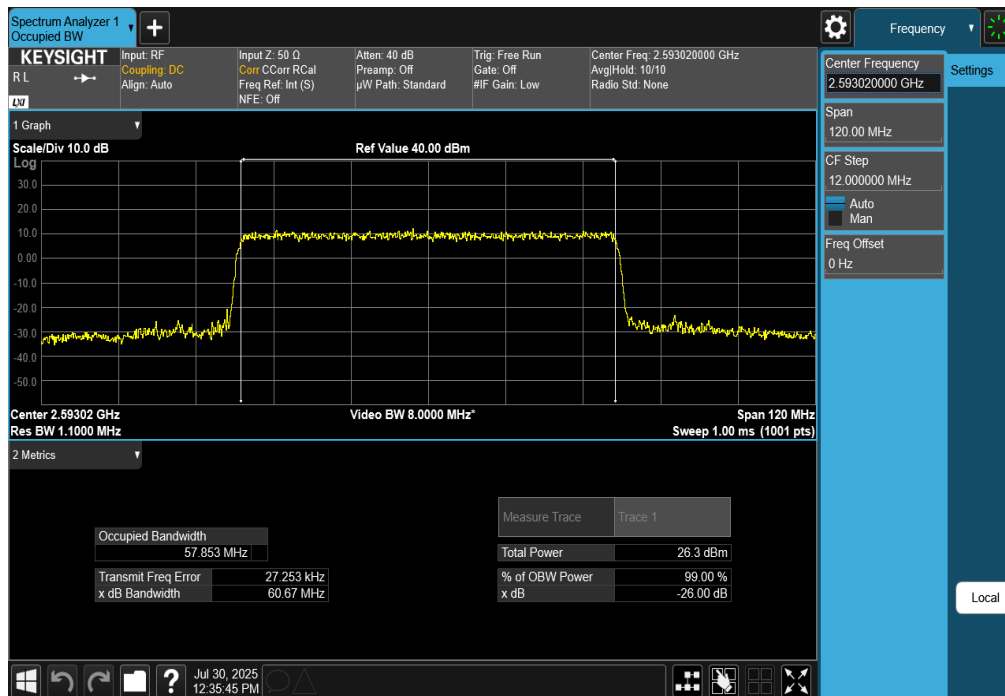
Plot 7-143. Occupied Bandwidth Plot (NR Band n41 - 60MHz CP-OFDM 16-QAM - Full RB)
