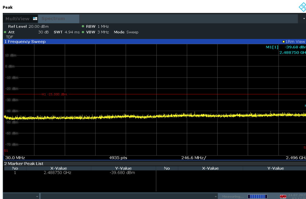
Plot 7-195. Conducted Spurious Plot (LTE Band 41 - 20MHz QPSK – RB Size 1, RB Offset 0 – Mid Channel)
