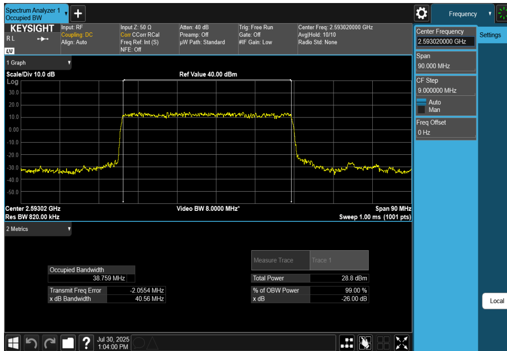
Plot 7-131. Occupied Bandwidth Plot (NR Band n41 - 45MHz DFT-s-OFDM \pi/2 BPSK - Full RB)
