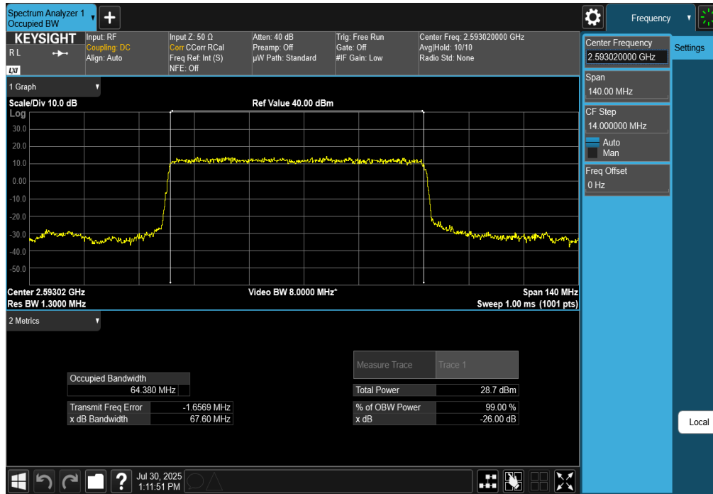
Plot 7-146. Occupied Bandwidth Plot (NR Band n41 - 70MHz DFT-s-OFDM \pi/2 BPSK - Full RB)
