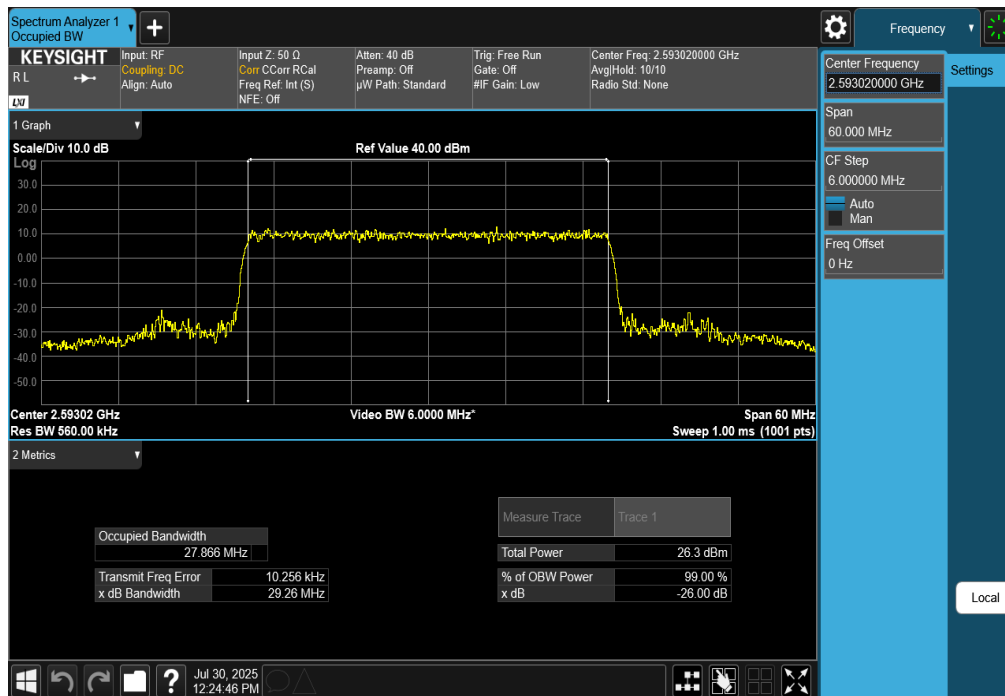
Plot 7-117. Occupied Bandwidth Plot (NR Band n41 - 30MHz CP-OFDM QPSK - Full RB)
