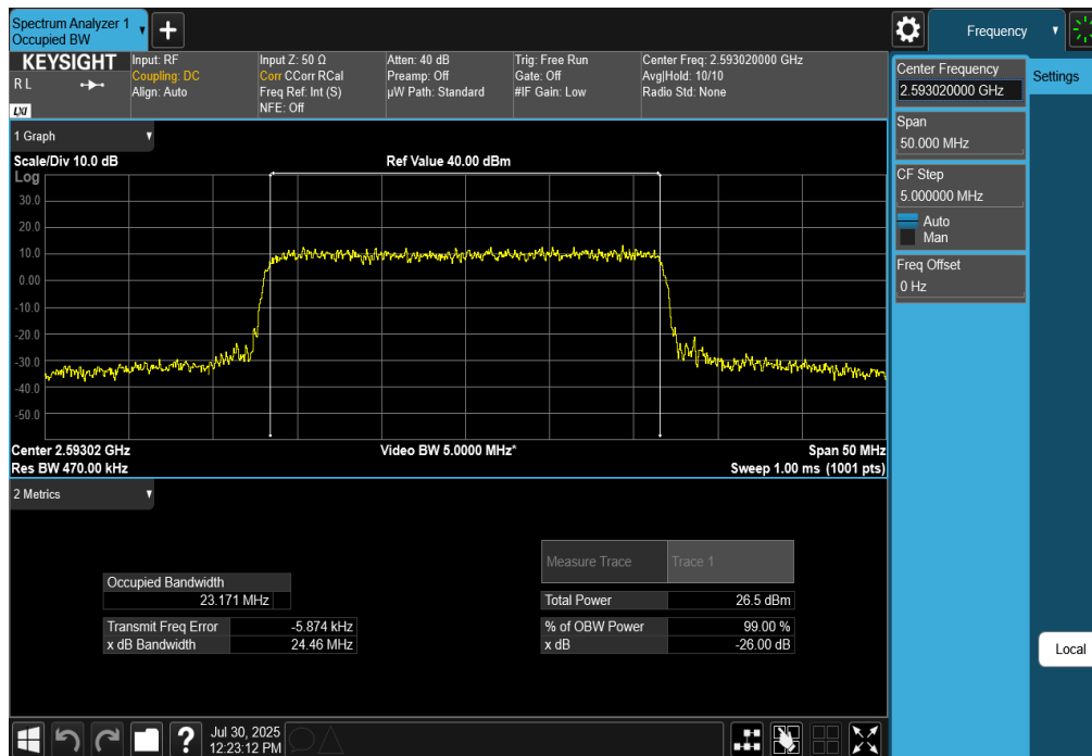
Plot 7-113. Occupied Bandwidth Plot (NR Band n41 - 25MHz CP-OFDM 16-QAM - Full RB)
