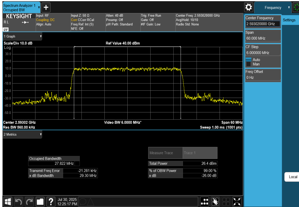
Plot 7-118. Occupied Bandwidth Plot (NR Band n41 - 30MHz CP-OFDM 16-QAM - Full RB)
