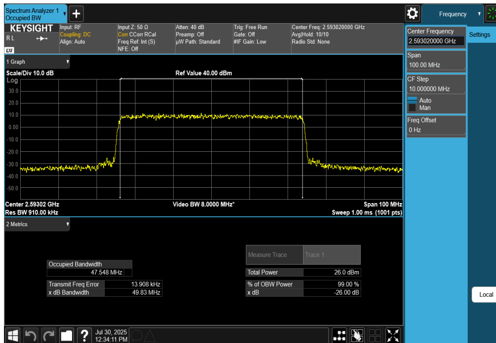
Plot 7-139. Occupied Bandwidth Plot (NR Band n41 - 50MHz CP-OFDM 64-QAM - Full RB)
