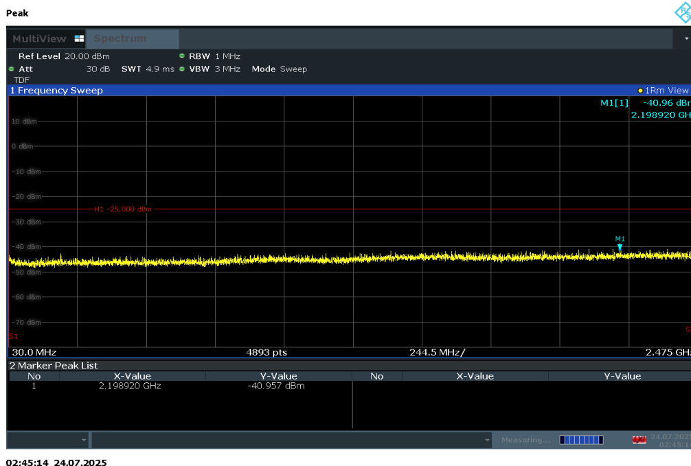
Plot 7-192. Conducted Spurious Plot (LTE Band 41 - 20MHz QPSK – RB Size 1, RB Offset 0 – Low Channel)
