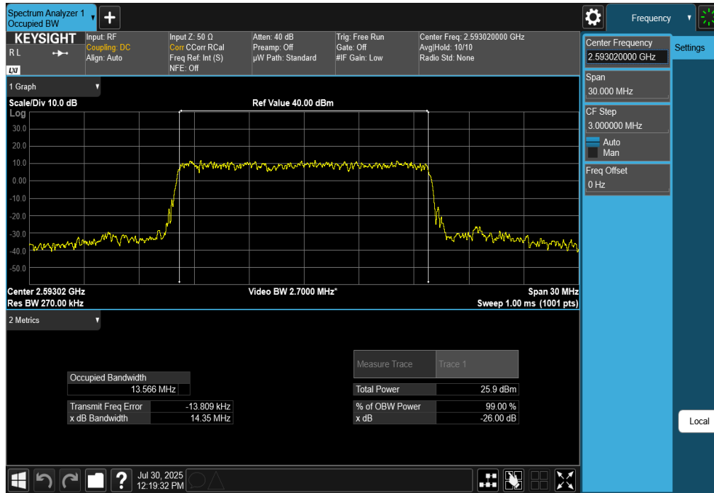
Plot 7-104. Occupied Bandwidth Plot (NR Band n41 - 15MHz CP-OFDM 64-QAM - Full RB)
