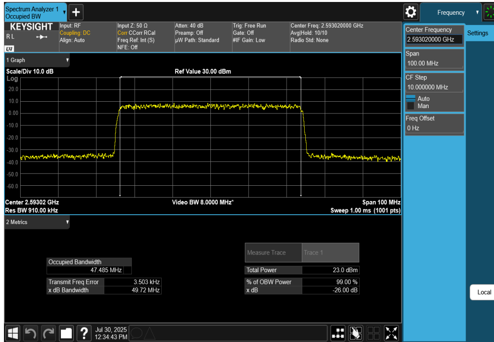
Plot 7-140. Occupied Bandwidth Plot (NR Band n41 - 50MHz CP-OFDM 256-QAM - Full RB)
