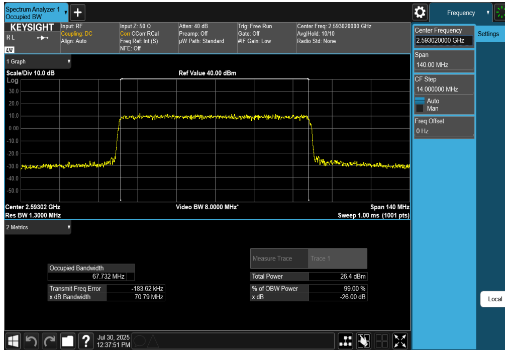
Plot 7-148. Occupied Bandwidth Plot (NR Band n41 - 70MHz CP-OFDM 16-QAM - Full RB)
