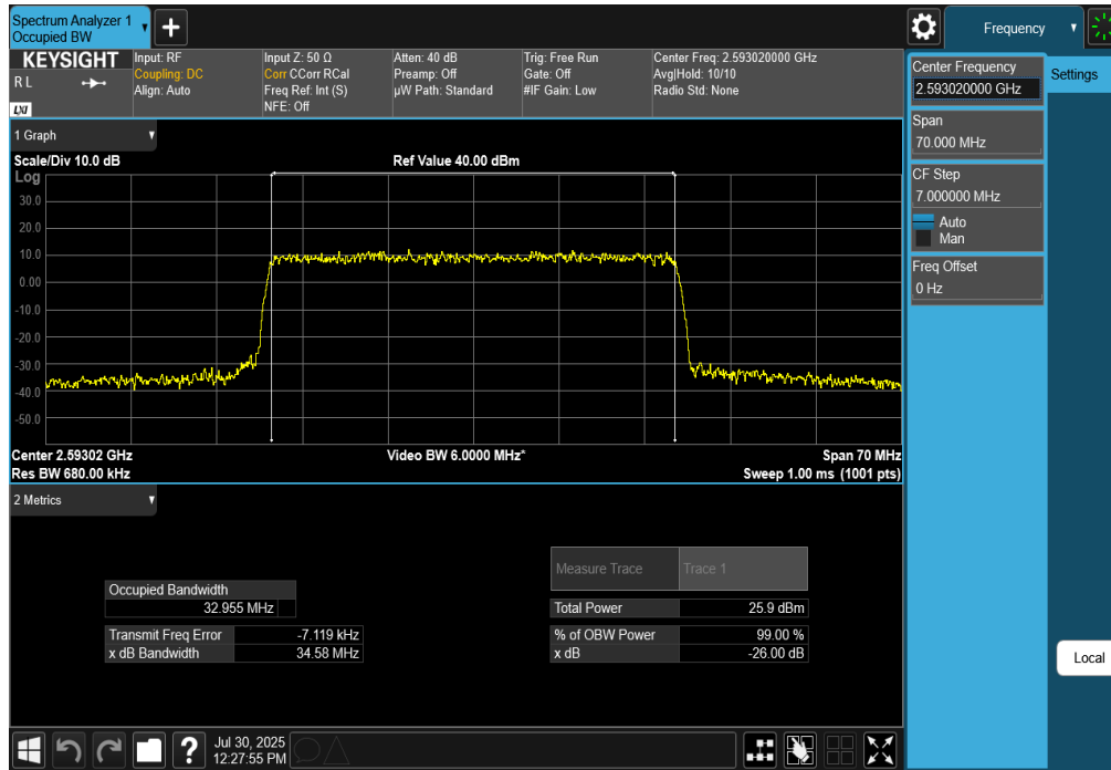
Plot 7-124. Occupied Bandwidth Plot (NR Band n41 - 35MHz CP-OFDM 64-QAM - Full RB)
