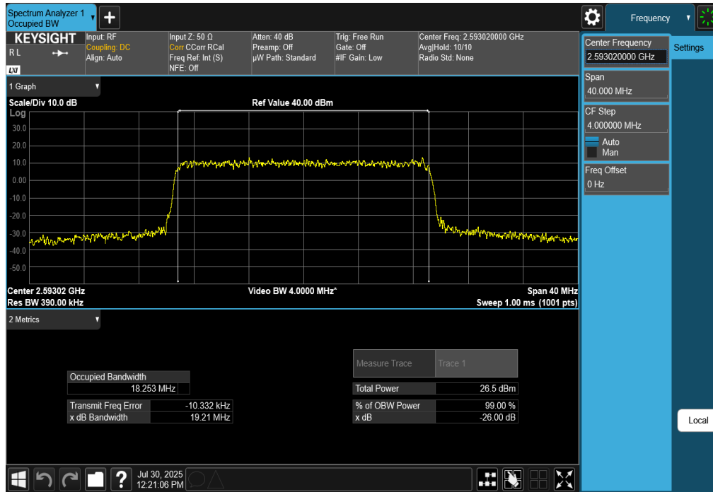
Plot 7-108. Occupied Bandwidth Plot (NR Band n41 - 20MHz CP-OFDM 16-QAM - Full RB)
