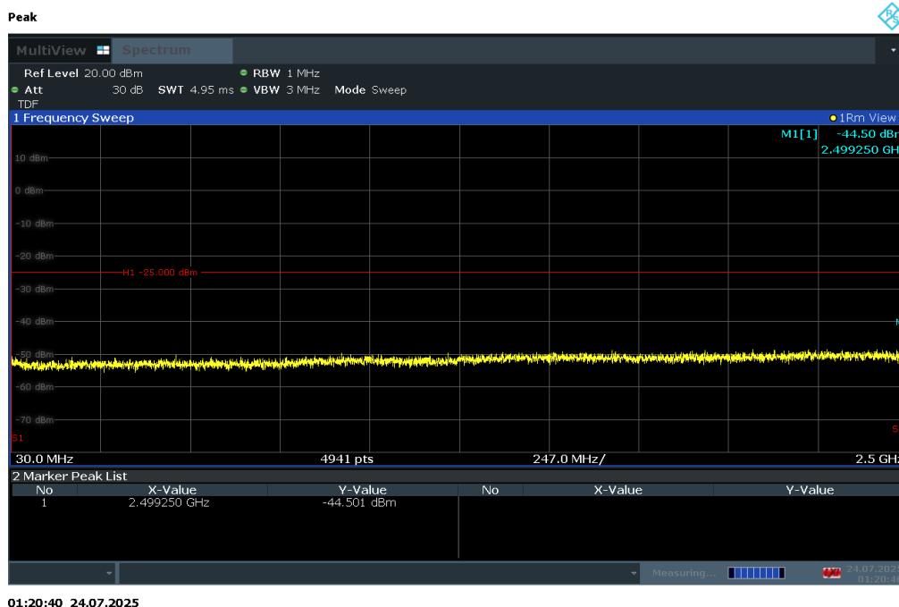
Plot 7-183. Conducted Spurious Plot (LTE Band 7 - 20MHz QPSK – RB Size 1, RB Offset 0 – Low Channel)
