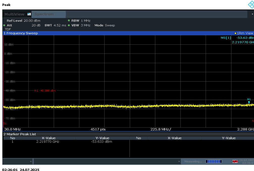
Plot 7-174. Conducted Spurious Plot (LTE Band 30 - 5MHz QPSK – RB Size 1, RB Offset 0 – Low Channel)
