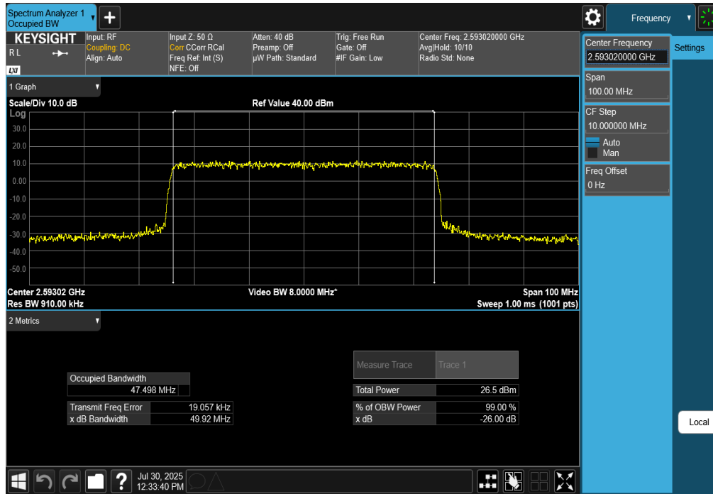
Plot 7-138. Occupied Bandwidth Plot (NR Band n41 - 50MHz CP-OFDM 16-QAM - Full RB)
