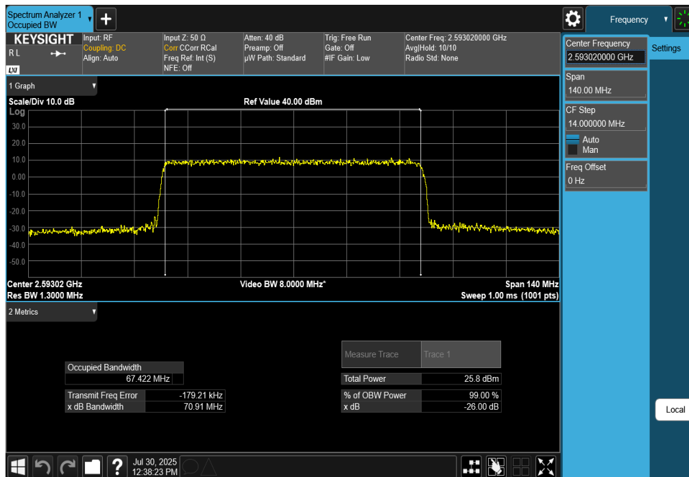
Plot 7-149. Occupied Bandwidth Plot (NR Band n41 - 70MHz CP-OFDM 64-QAM - Full RB)
