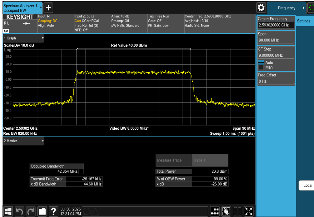
Plot 7-132. Occupied Bandwidth Plot (NR Band n41 - 45MHz CP-OFDM QPSK - Full RB)
