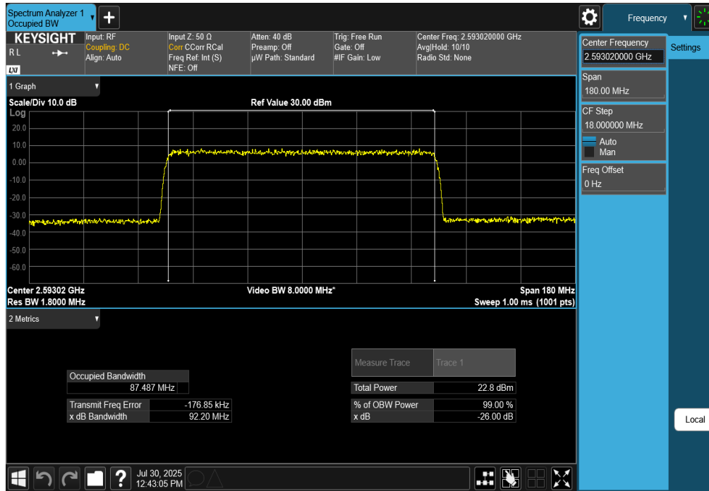
Plot 7-160. Occupied Bandwidth Plot (NR Band n41 - 90MHz CP-OFDM 256-QAM - Full RB)
