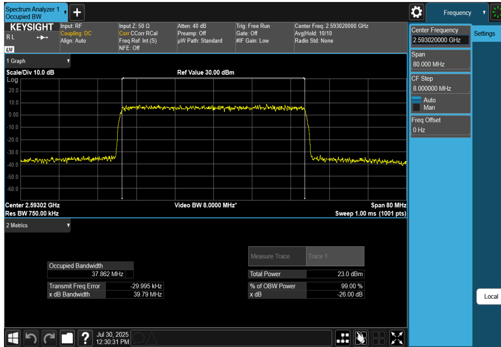
Plot 7-130. Occupied Bandwidth Plot (NR Band n41 - 40MHz CP-OFDM 256-QAM - Full RB)
