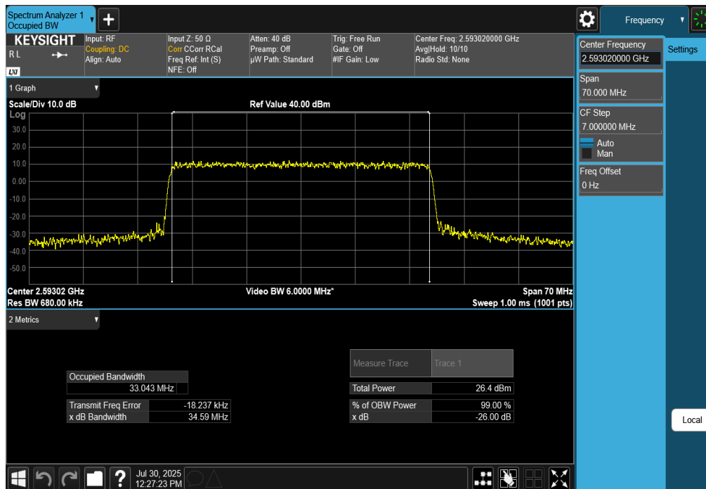
Plot 7-123. Occupied Bandwidth Plot (NR Band n41 - 35MHz CP-OFDM 16-QAM - Full RB)
