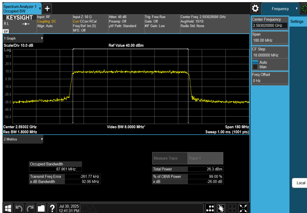
Plot 7-157. Occupied Bandwidth Plot (NR Band n41 - 90MHz CP-OFDM QPSK - Full RB)
