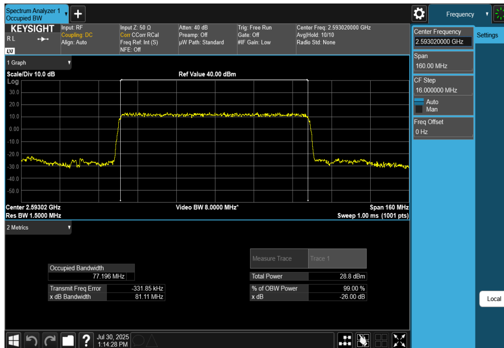
Plot 7-151. Occupied Bandwidth Plot (NR Band n41 - 80MHz DFT-s-OFDM \pi/2 BPSK - Full RB)
