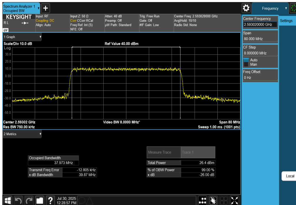
Plot 7-127. Occupied Bandwidth Plot (NR Band n41 - 40MHz CP-OFDM QPSK - Full RB)
