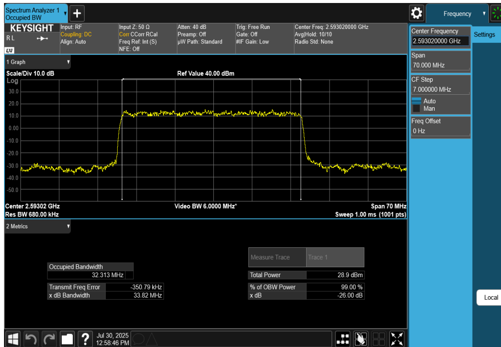
Plot 7-121. Occupied Bandwidth Plot (NR Band n41 - 35MHz DFT-s-OFDM \pi/2 BPSK - Full RB)
