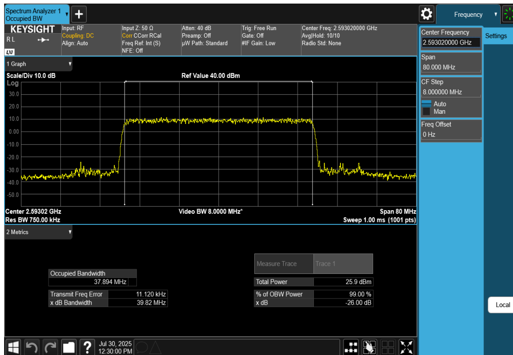
Plot 7-129. Occupied Bandwidth Plot (NR Band n41 - 40MHz CP-OFDM 64-QAM - Full RB)
