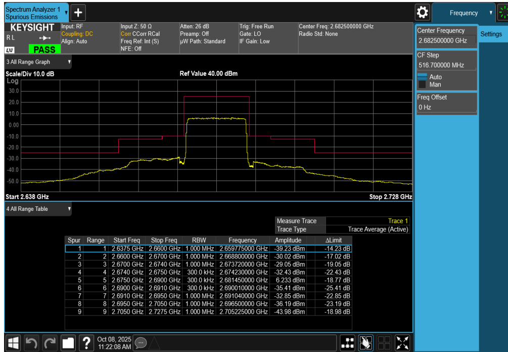
Plot 7-298. Upper ACP Plot (LTE Band 41 - 15MHz QPSK – Full RB)
