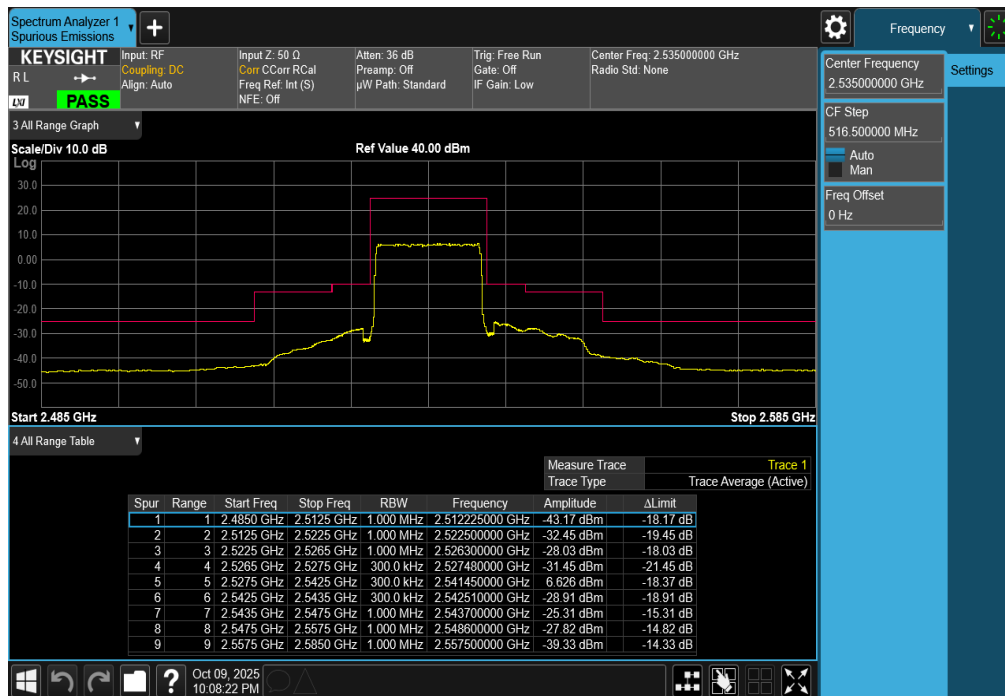
Plot 7-285. Middle ACP Plot (LTE Band 7 - 15MHz QPSK – Full RB)
