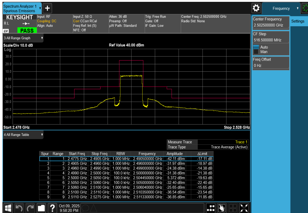
Plot 7-278. Lower ACP Plot (LTE Band 7 - 5MHz QPSK – Full RB)
