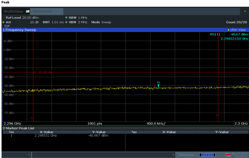
Plot 7-253. Extended Lower Band Edge Plot (LTE Band 30 - 5MHz QPSK – Full RB)
