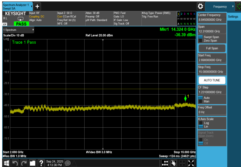
Plot 7-241. Conducted Spurious Plot (ULCA LTE Band 41 – (20+20)MHz QPSK – RB Size 1, RB Offset 0 – Mid Channel)
