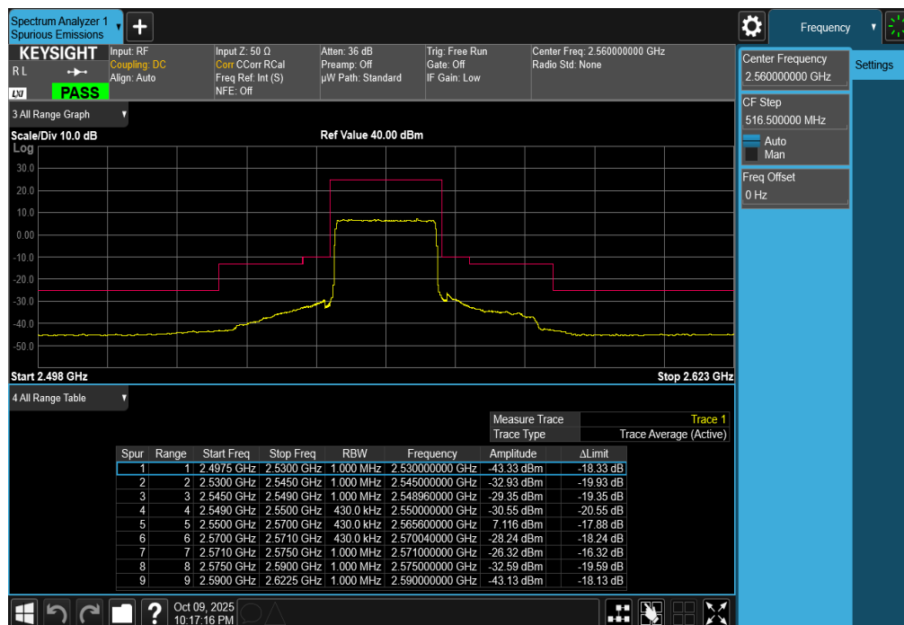
Plot 7-289. Upper ACP Plot (LTE Band 7 - 20MHz QPSK – Full RB)
