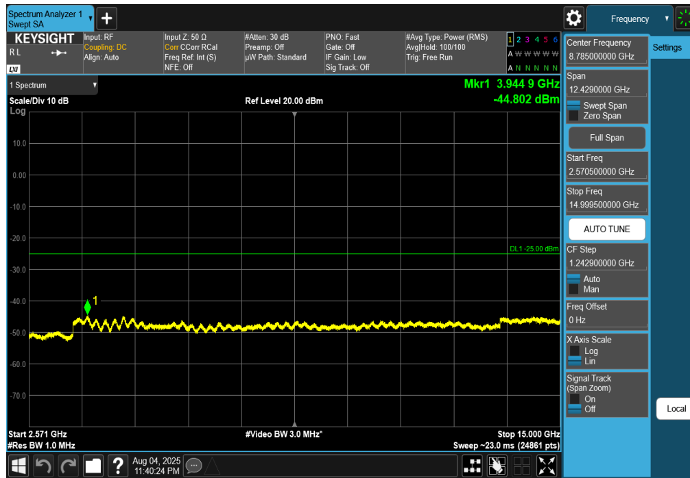
Plot 7-214. Conducted Spurious Plot (NR Band n7 - 50MHz DFT-s-OFDM QPSK – RB Size 1, RB Offset 0 – Mid Channel)
