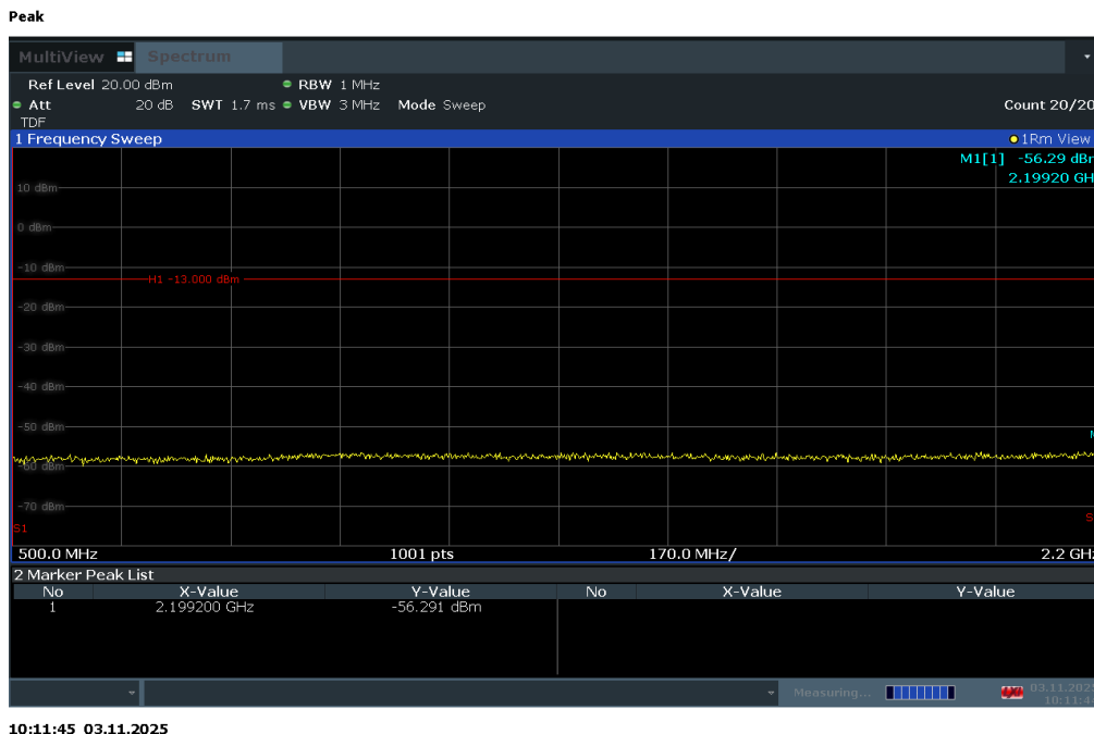
Plot 7-249. Extended Lower Band Edge Plot (LTE Band 30 - 5MHz QPSK – Full RB)
