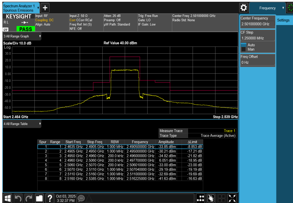
Plot 7-293. Lower ACP Plot (LTE Band 41 - 10MHz QPSK – Full RB)
