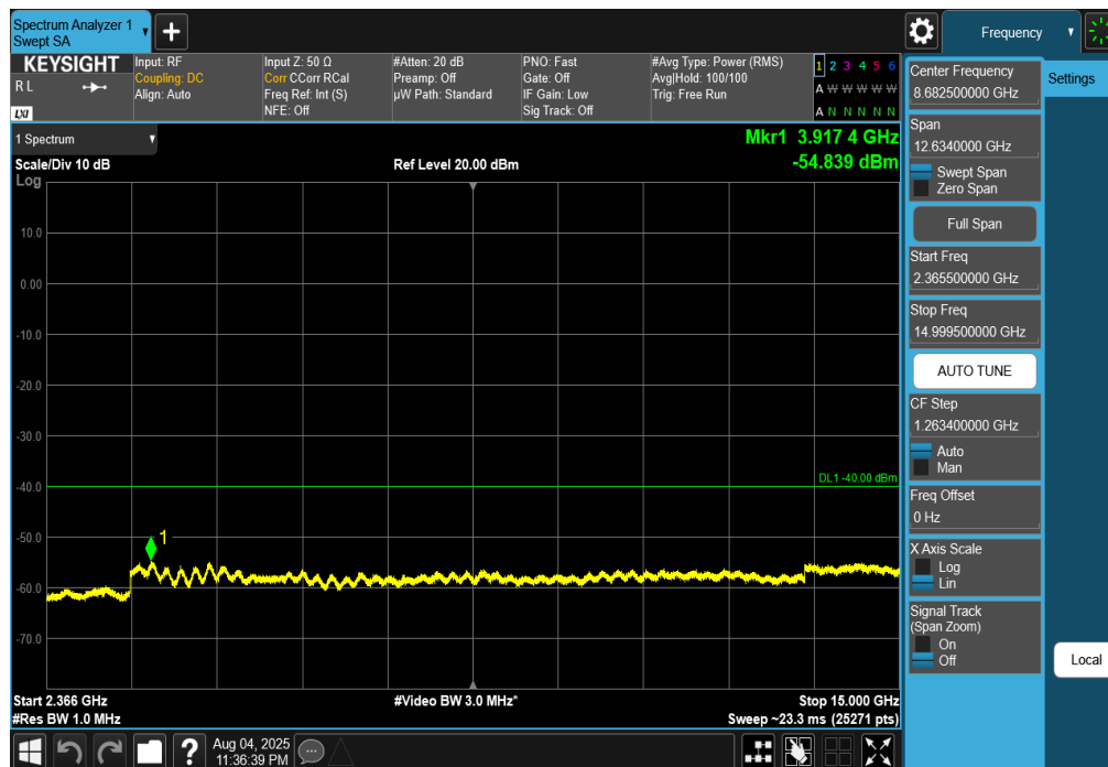
Plot 7-208. Conducted Spurious Plot (NR Band n30 - 5MHz DFT-s-OFDM QPSK – RB Size 1, RB Offset 0 – High Channel)
