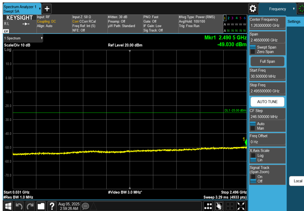
Plot 7-222. Conducted Spurious Plot (NR Band n41 - 100MHz DFT-s-OFDM QPSK – RB Size 1, RB Offset 0 – Mid Channel)
