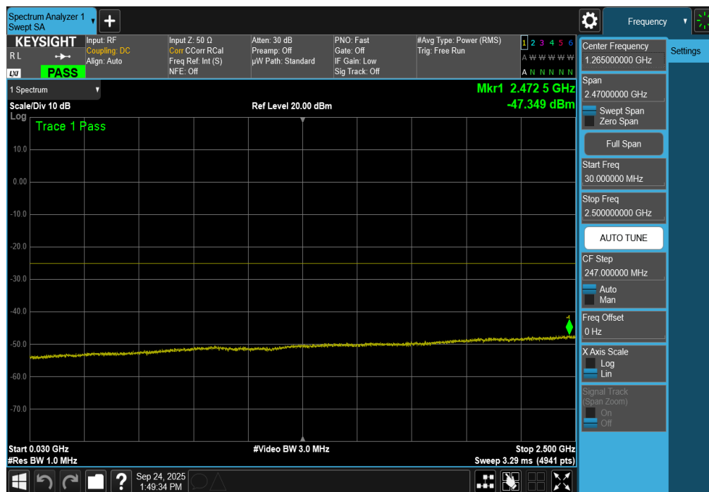
Plot 7-231. Conducted Spurious Plot (ULCA LTE Band 7 – (20+20)MHz QPSK – RB Size 1, RB Offset 0 – Mid Channel)
