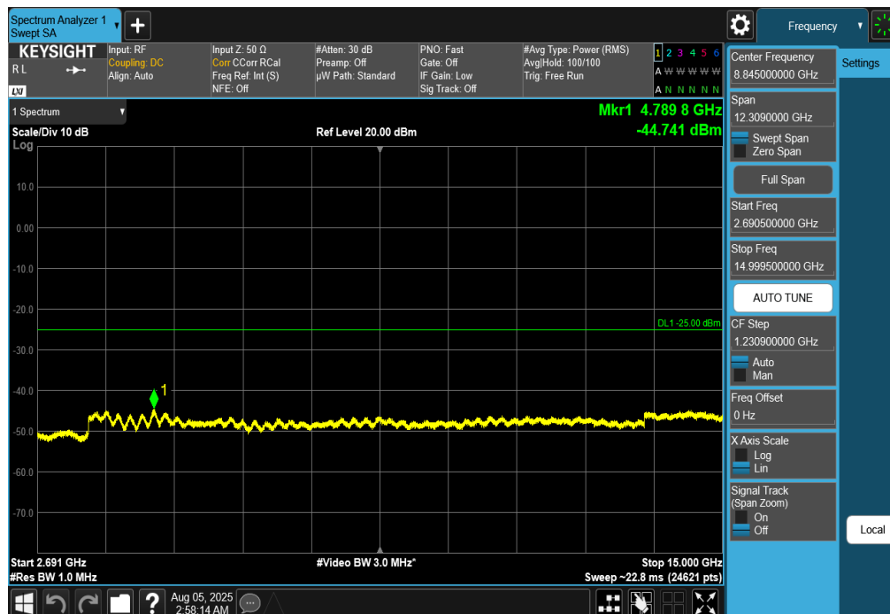
Plot 7-220. Conducted Spurious Plot (NR Band n41 - 100MHz DFT-s-OFDM QPSK – RB Size 1, RB Offset 0 – Low Channel)
