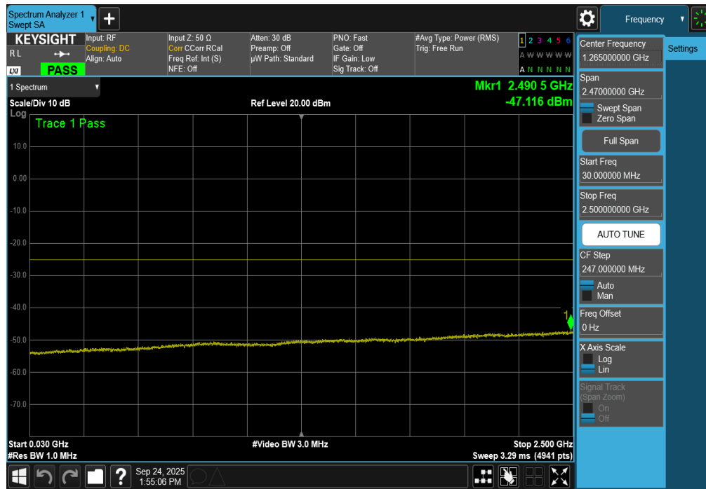
Plot 7-234. Conducted Spurious Plot (ULCA LTE Band 7 – (20+20)MHz QPSK – RB Size 1, RB Offset 0 – High Channel)
