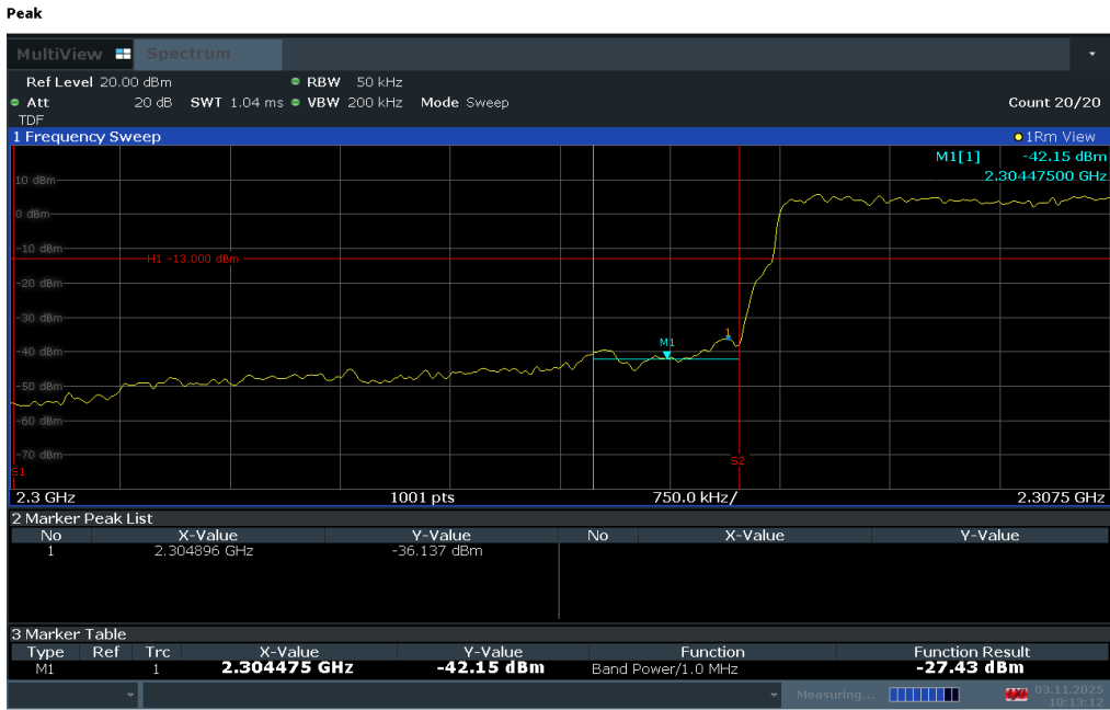
Plot 7-254. Lower Band Edge Plot (LTE Band 30 - 5MHz QPSK – Full RB)
