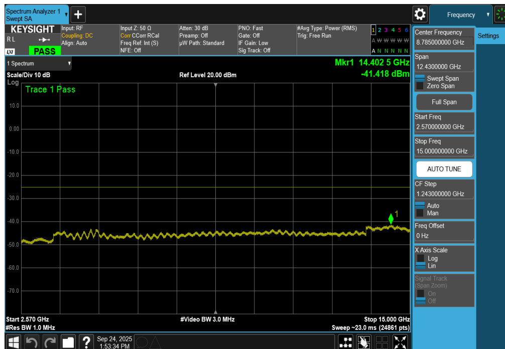
Plot 7-229. Conducted Spurious Plot (ULCA LTE Band 7 – (20+20)MHz QPSK – RB Size 1, RB Offset 0 – Low Channel)
