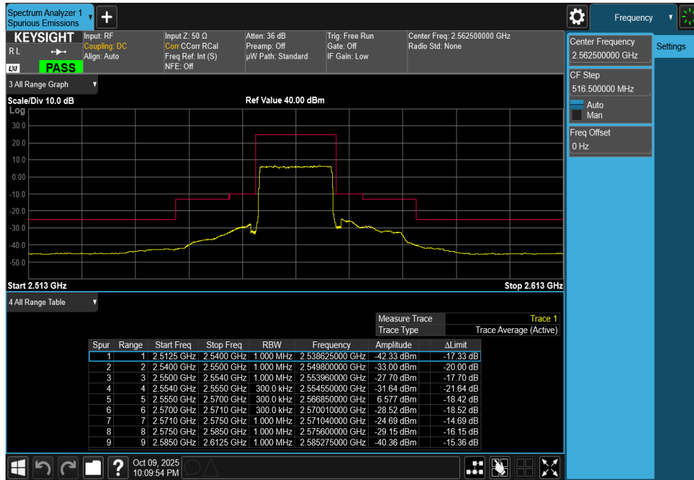
Plot 7-286. Upper ACP Plot (LTE Band 7 - 15MHz QPSK – Full RB)
