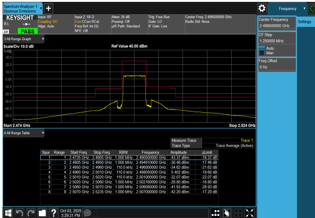
Plot 7-290. Lower ACP Plot (LTE Band 41 - 5MHz QPSK - Full RB)
