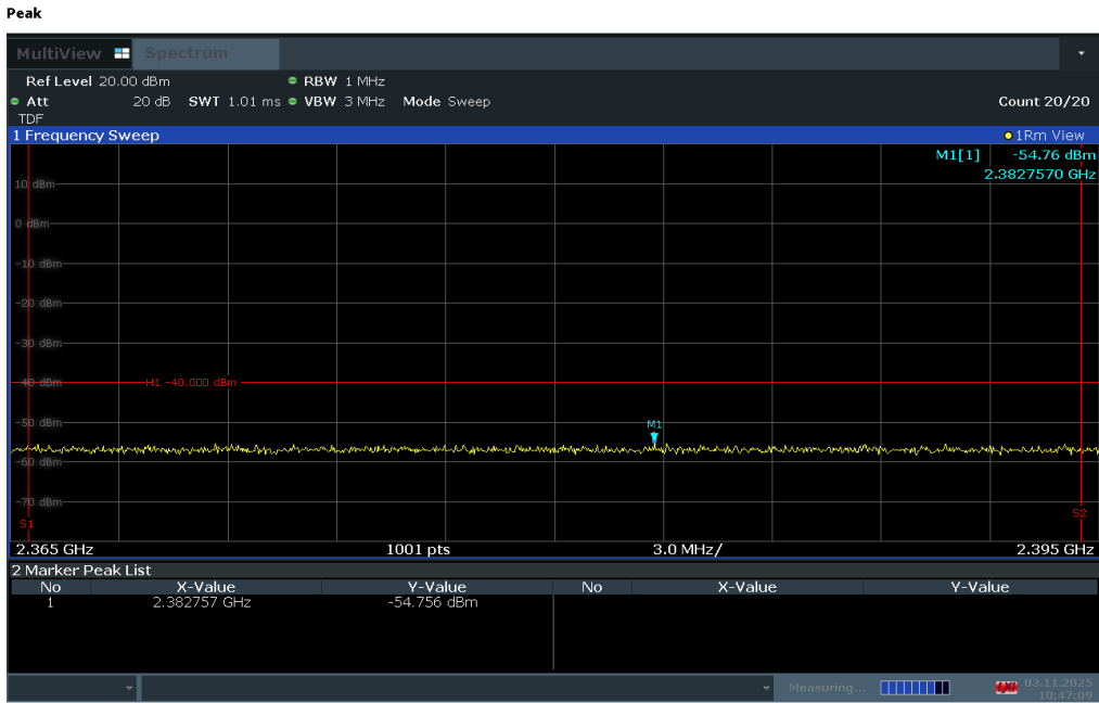
Plot 7-262. Extended Upper Band Edge Plot (LTE Band 30 - 5MHz QPSK – Full RB)
