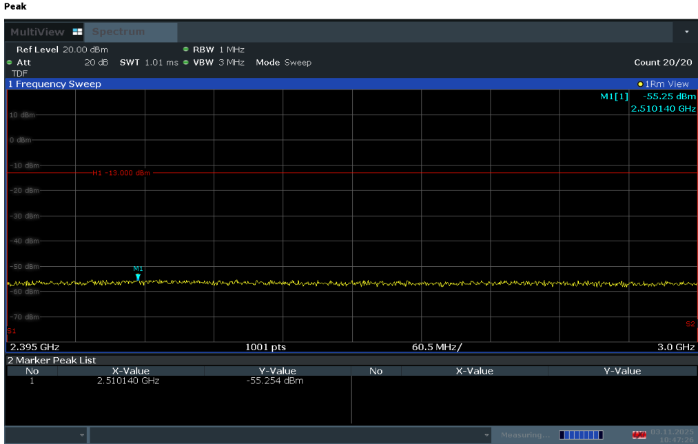
Plot 7-263. Extended Upper Band Edge Plot (LTE Band 30 - 5MHz QPSK – Full RB)
