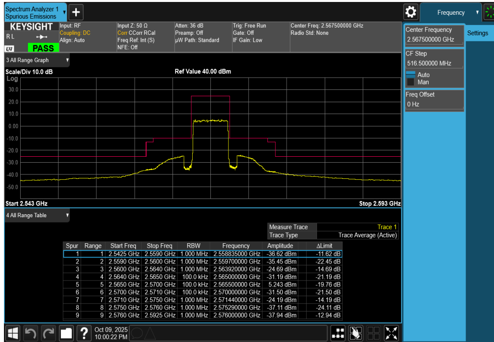
Plot 7-280. Upper ACP Plot (LTE Band 7 - 5MHz QPSK – Full RB)
