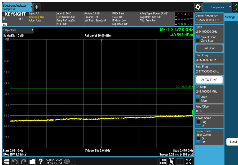
Plot 7-213. Conducted Spurious Plot (NR Band n7 - 50MHz DFT-s-OFDM QPSK – RB Size 1, RB Offset 0 – Mid Channel)
