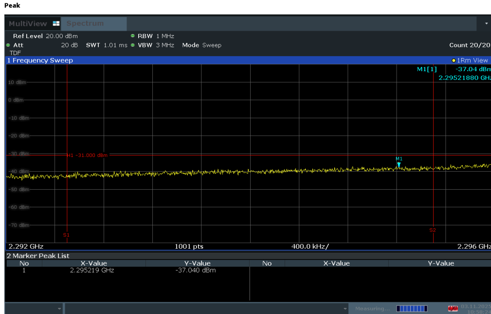
Plot 7-267. Extended Lower Band Edge Plot (LTE Band 30 - 10MHz QPSK – Full RB)
