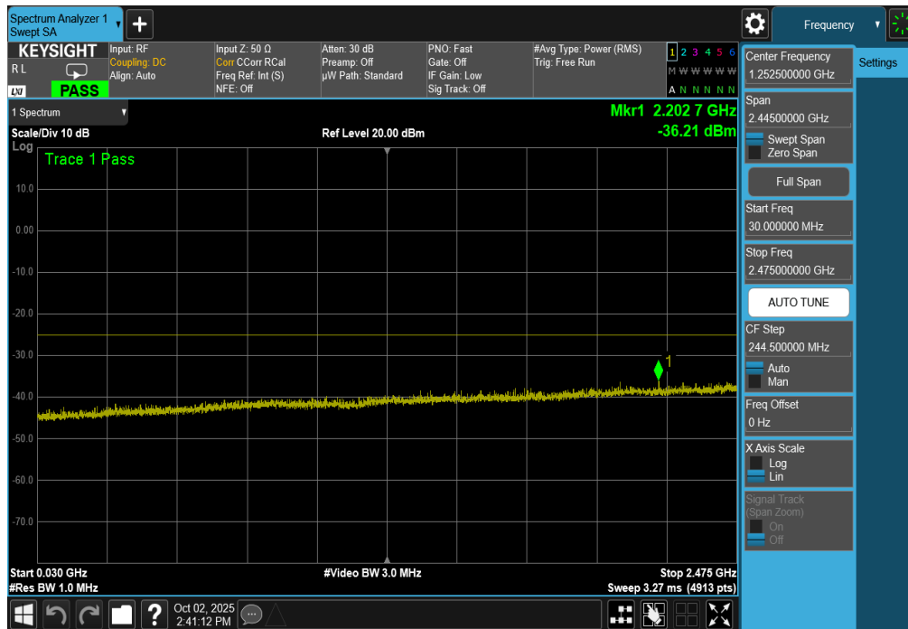
Plot 7-237. Conducted Spurious Plot (ULCA LTE Band 41 – (20+20)MHz QPSK – RB Size 1, RB Offset 0 – Low Channel)
