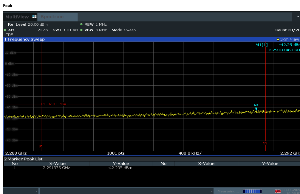
Plot 7-266. Extended Lower Band Edge Plot (LTE Band 30 - 10MHz QPSK – Full RB)
