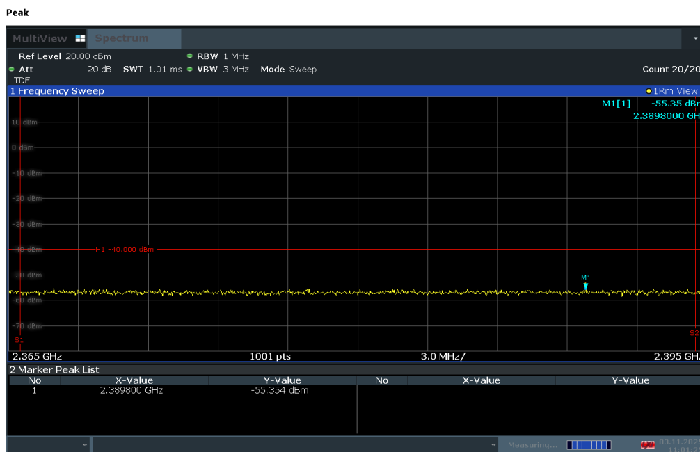
Plot 7-276. Extended Upper Band Edge Plot (LTE Band 30 - 10MHz QPSK – Full RB)
