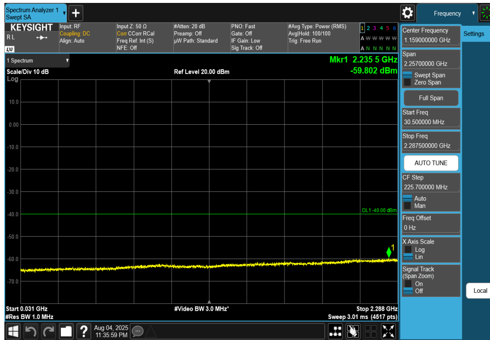
Plot 7-207. Conducted Spurious Plot (NR Band n30 - 5MHz DFT-s-OFDM QPSK – RB Size 1, RB Offset 0 – High Channel)
