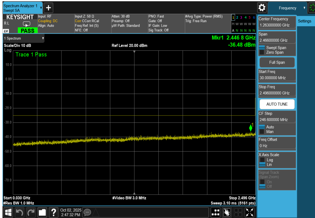
Plot 7-243. Conducted Spurious Plot (ULCA LTE Band 41 – (20+20)MHz QPSK – RB Size 1, RB Offset 0 – High Channel)
