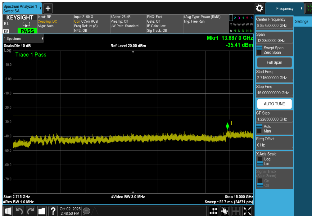
Plot 7-244. Conducted Spurious Plot (ULCA LTE Band 41 – (20+20)MHz QPSK – RB Size 1, RB Offset 0 – High Channel)
