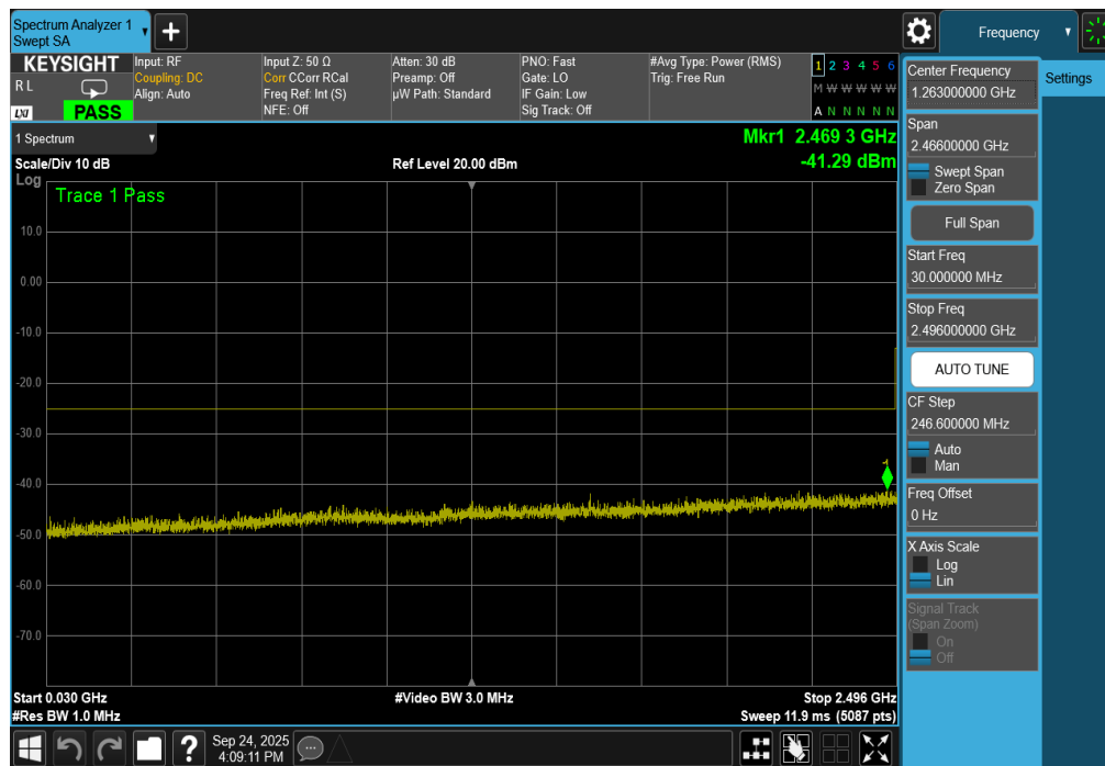
Plot 7-240. Conducted Spurious Plot (ULCA LTE Band 41 – (20+20)MHz QPSK – RB Size 1, RB Offset 0 – Mid Channel)
