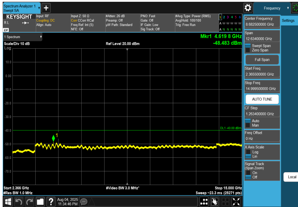
Plot 7-205. Conducted Spurious Plot (NR Band n30 - 10MHz DFT-s-OFDM QPSK – RB Size 1, RB Offset 0 – Mid Channel)
