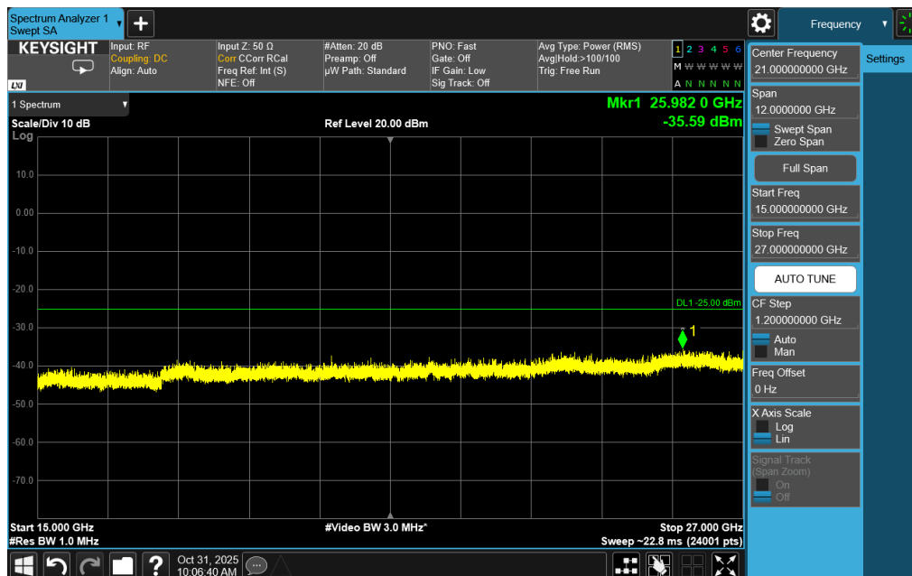
Plot 7-248. Simultaneous TX Spurious Plot (LTE Band 41 PC2 + Bluetooth + UNII)
