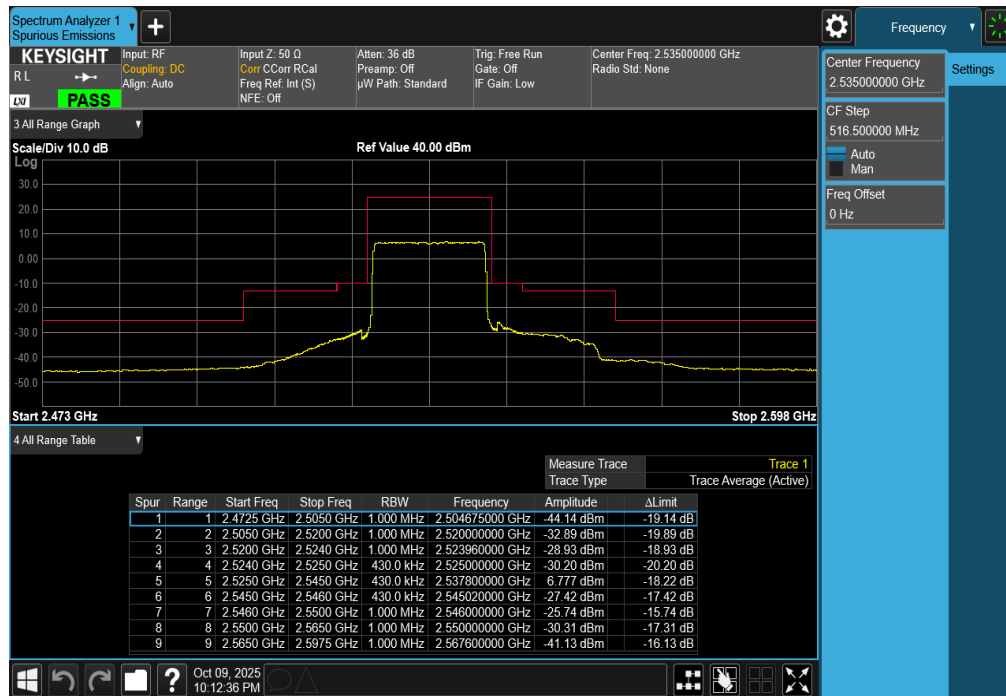
Plot 7-288. Middle ACP Plot (LTE Band 7 - 20MHz QPSK – Full RB)
