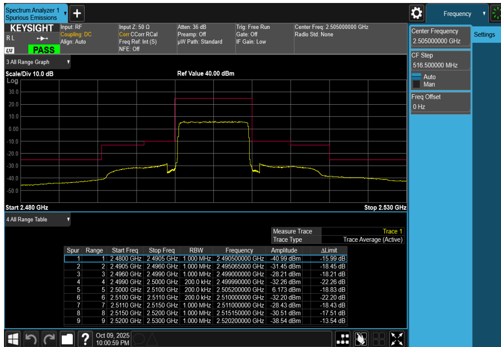
Plot 7-281. Lower ACP Plot (LTE Band 7 - 10MHz QPSK – Full RB)
