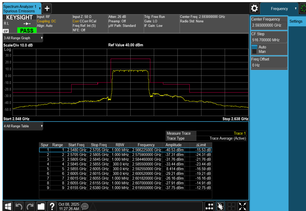
Plot 7-297. Middle ACP Plot (LTE Band 41 - 15MHz QPSK – Full RB)
