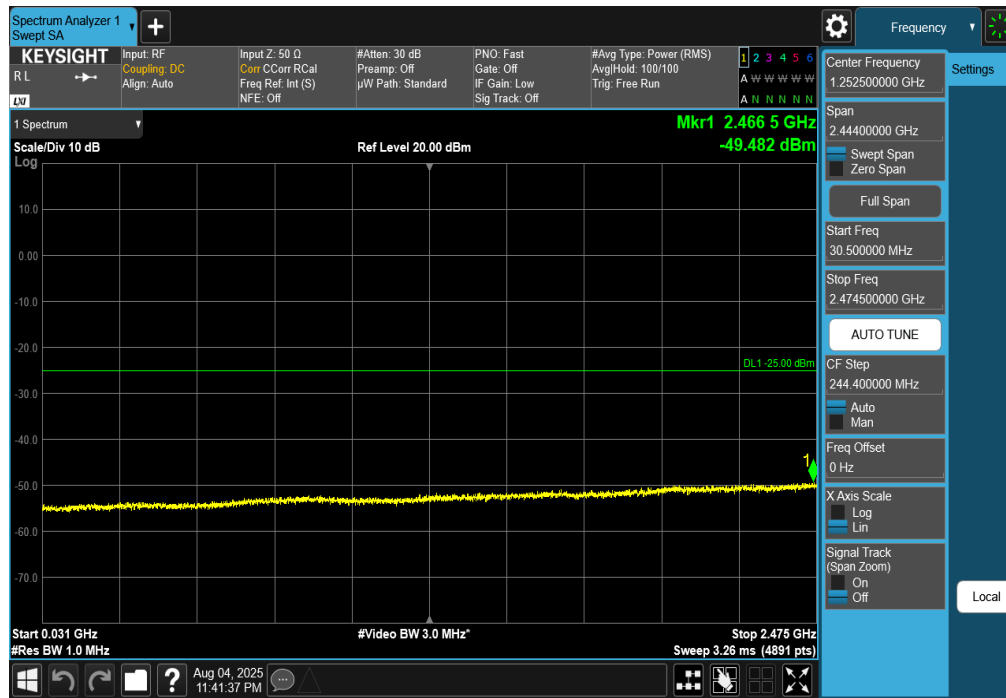
Plot 7-216. Conducted Spurious Plot (NR Band n7 - 50MHz DFT-s-OFDM QPSK – RB Size 1, RB Offset 0 – High Channel)
