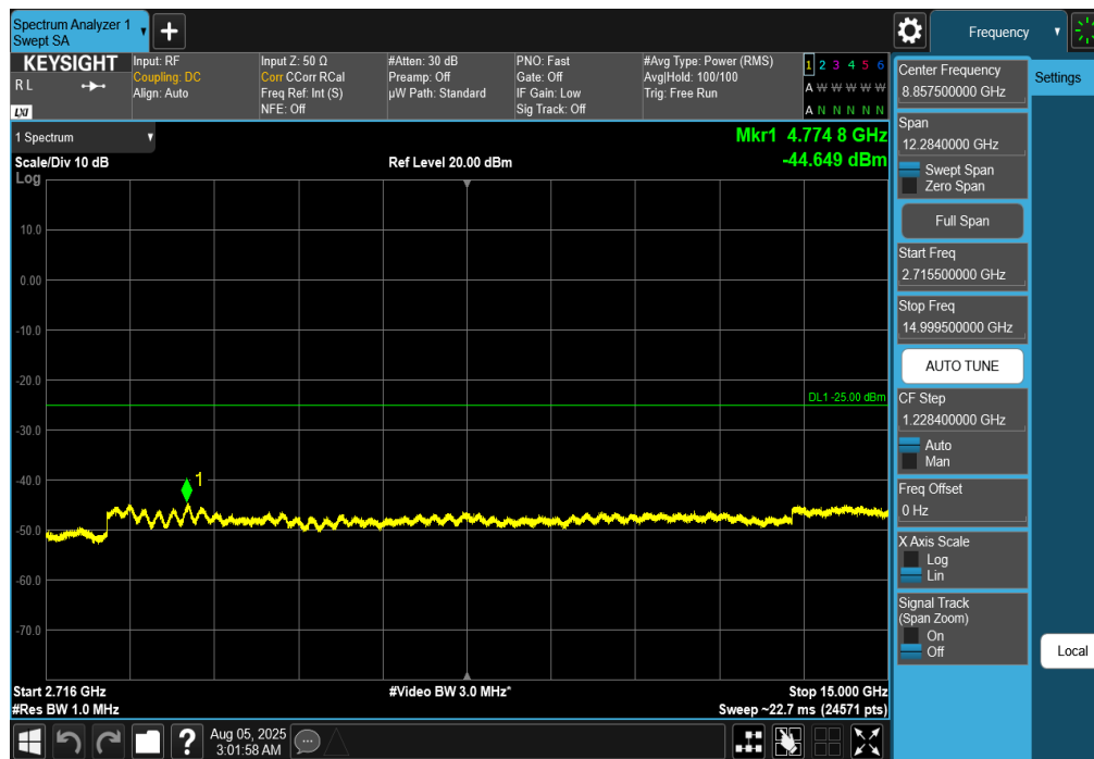
Plot 7-226. Conducted Spurious Plot (NR Band n41 - 100MHz DFT-s-OFDM QPSK – RB Size 1, RB Offset 0 – High Channel)
