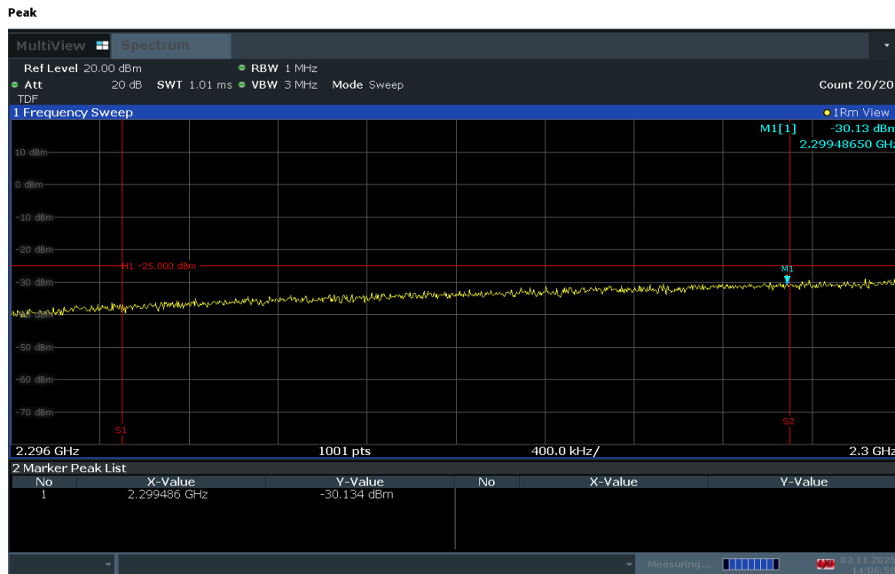
Plot 7-268. Extended Lower Band Edge Plot (LTE Band 30 - 10MHz QPSK – Full RB)
