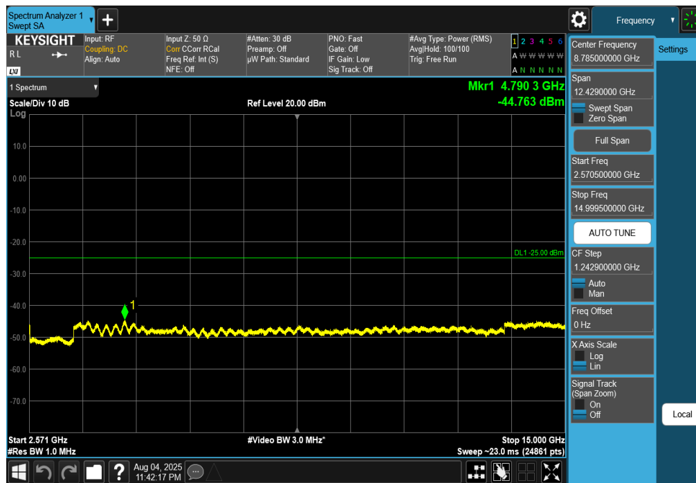
Plot 7-217. Conducted Spurious Plot (NR Band n7 - 50MHz DFT-s-OFDM QPSK – RB Size 1, RB Offset 0 – High Channel)
