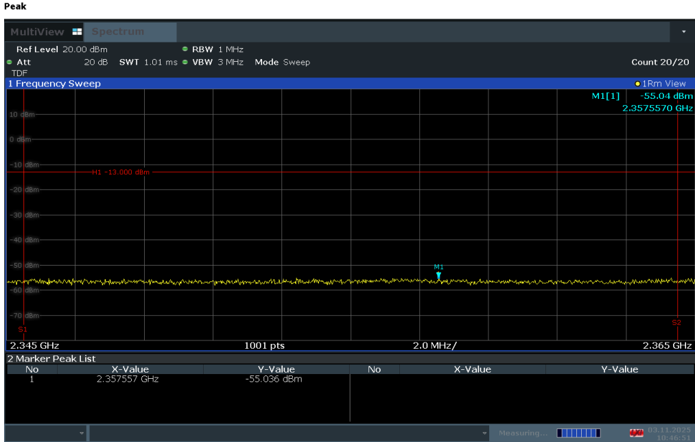
Plot 7-261. Extended Upper Band Edge Plot (LTE Band 30 - 5MHz QPSK – Full RB)
