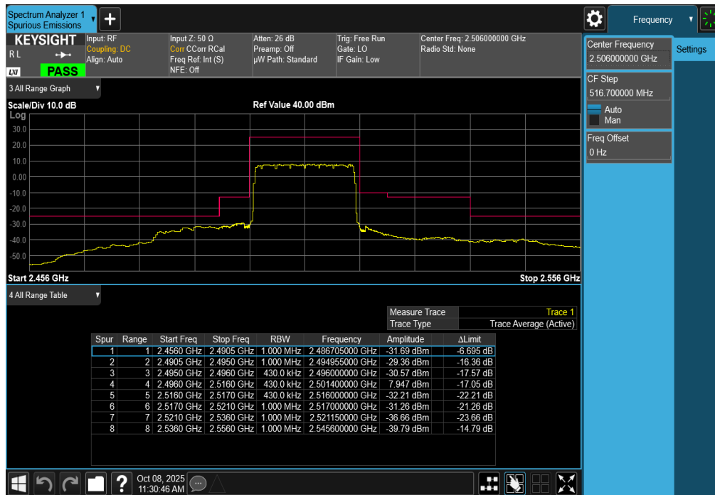
Plot 7-299. Lower ACP Plot (LTE Band 41 - 20MHz QPSK – Full RB)
