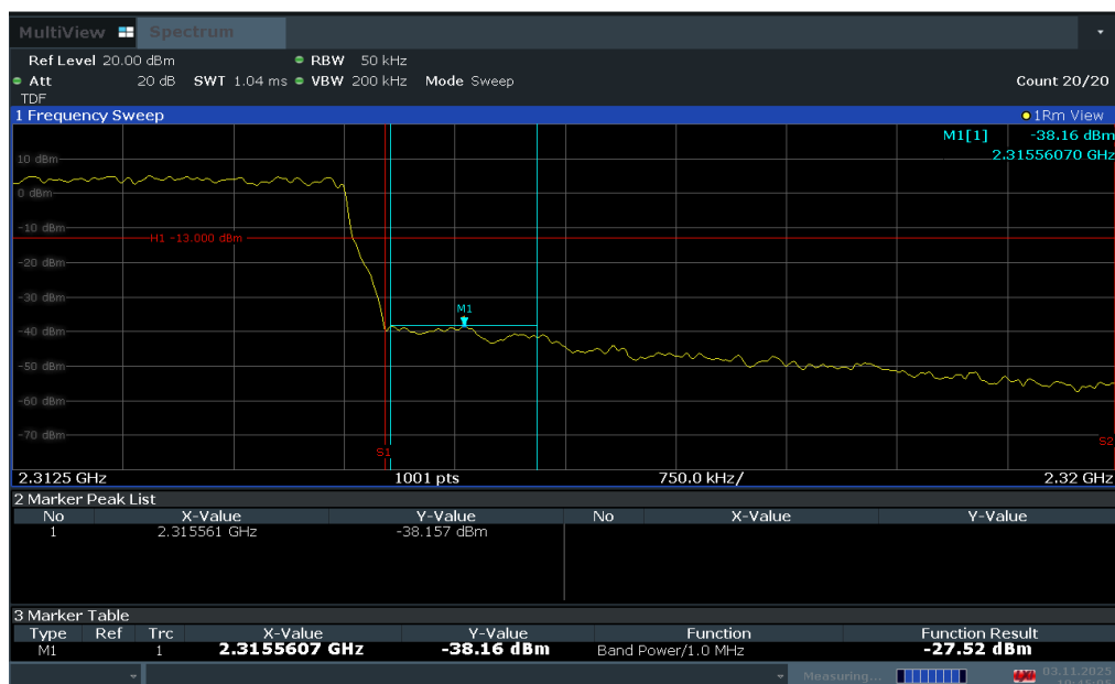
Plot 7-255. Upper Band Edge Plot (LTE Band 30 - 5MHz QPSK – Full RB)
