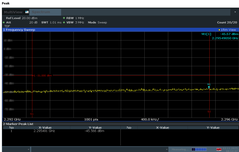
Plot 7-252. Extended Lower Band Edge Plot (LTE Band 30 - 5MHz QPSK – Full RB)
