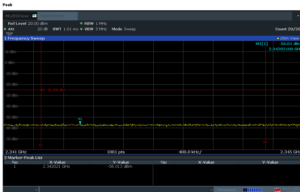
Plot 7-275. Extended Upper Band Edge Plot (LTE Band 30 - 10MHz QPSK – Full RB)
