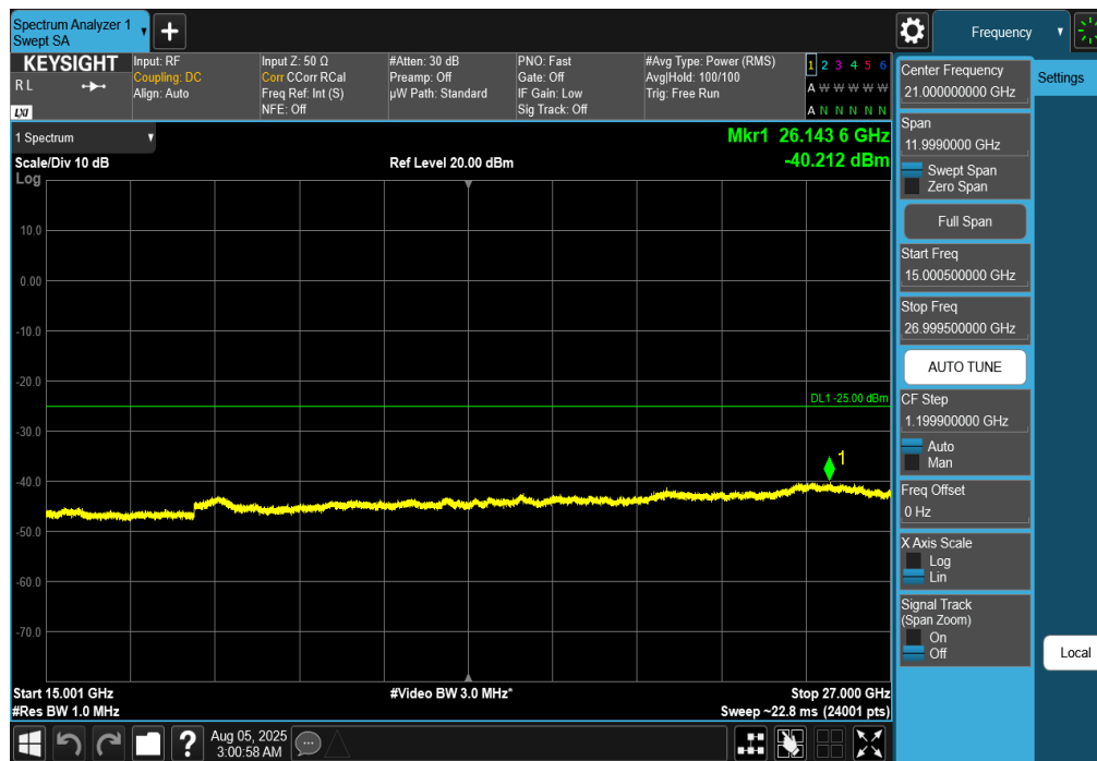
Plot 7-224. Conducted Spurious Plot (NR Band n41 - 100MHz DFT-s-OFDM QPSK – RB Size 1, RB Offset 0 – Mid Channel)
