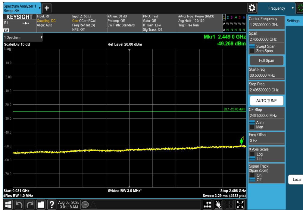
Plot 7-225. Conducted Spurious Plot (NR Band n41 - 100MHz DFT-s-OFDM QPSK – RB Size 1, RB Offset 0 – High Channel)
