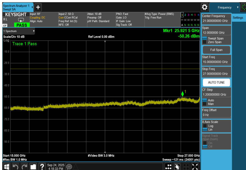
Plot 7-242. Conducted Spurious Plot (ULCA LTE Band 41 – (20+20)MHz QPSK – RB Size 1, RB Offset 0 – Mid Channel)
