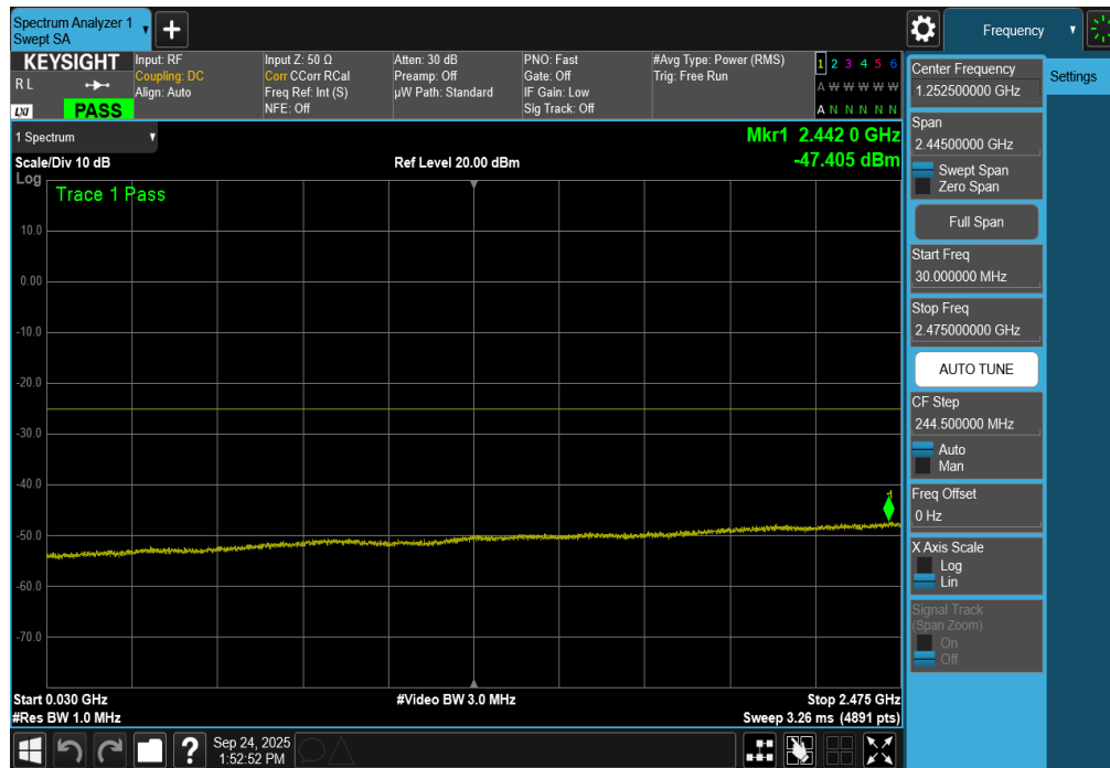
Plot 7-228. Conducted Spurious Plot (ULCA LTE Band 7 – (20+20)MHz QPSK – RB Size 1, RB Offset 0 – Low Channel)
