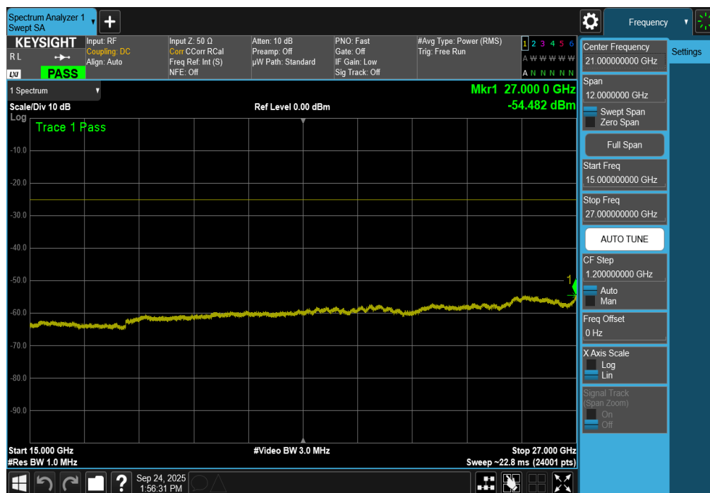
Plot 7-236. Conducted Spurious Plot (ULCA LTE Band 7 – (20+20)MHz QPSK – RB Size 1, RB Offset 0 – High Channel)
