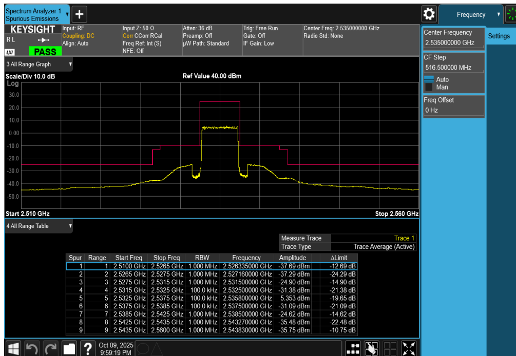
Plot 7-279. Middle ACP Plot (LTE Band 7 - 5MHz QPSK – Full RB)
