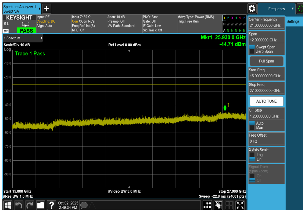
Plot 7-245. Conducted Spurious Plot (ULCA LTE Band 41 – (20+20)MHz QPSK – RB Size 1, RB Offset 0 – High Channel)
