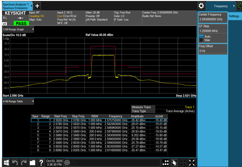
Plot 7-294. Middle ACP Plot (LTE Band 41 - 10MHz QPSK – Full RB)
