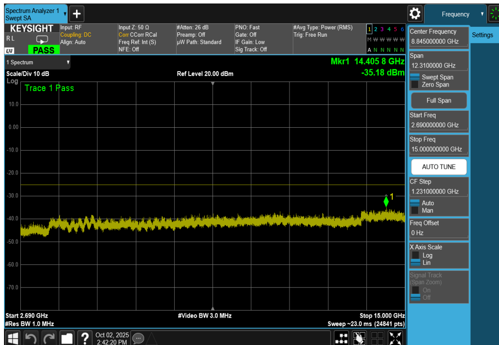
Plot 7-238. Conducted Spurious Plot (ULCA LTE Band 41 – (20+20)MHz QPSK – RB Size 1, RB Offset 0 – Low Channel)
