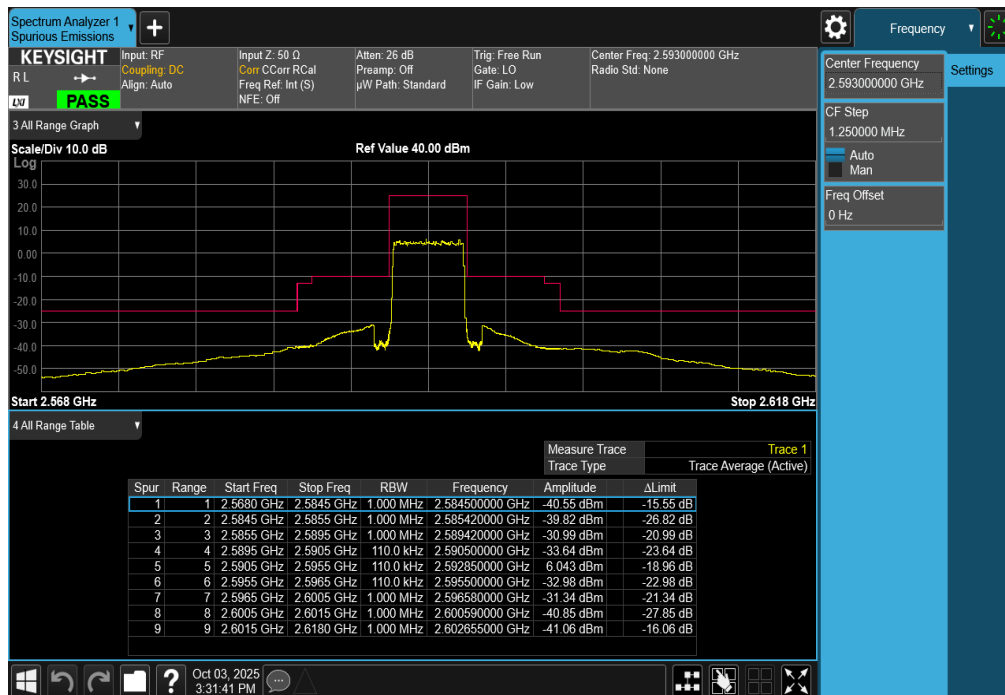
Plot 7-291. Middle ACP Plot (LTE Band 41 - 5MHz QPSK - Full RB)
