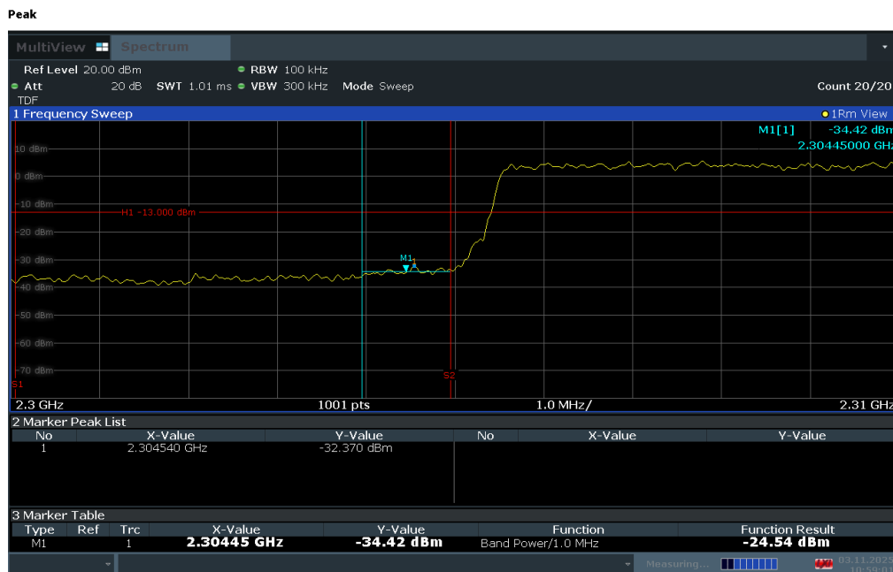
Plot 7-269. Lower Band Edge Plot (LTE Band 30 - 10MHz QPSK – Full RB)
