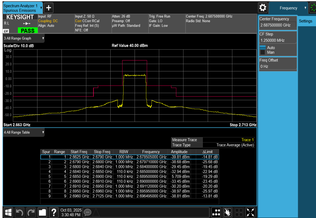
Plot 7-292. Upper ACP Plot (LTE Band 41 - 5MHz QPSK – Full RB)
