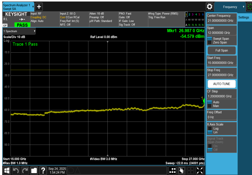
Plot 7-230. Conducted Spurious Plot (ULCA LTE Band 7 – (20+20)MHz QPSK – RB Size 1, RB Offset 0 – Low Channel)
