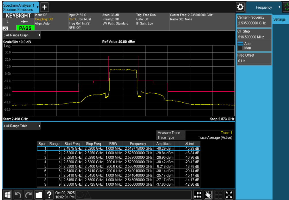
Plot 7-282. Middle ACP Plot (LTE Band 7 - 10MHz QPSK – Full RB)
