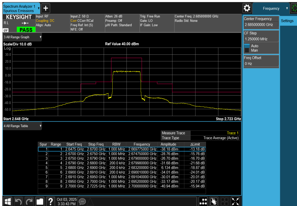
Plot 7-295. Upper ACP Plot (LTE Band 41 - 10MHz QPSK – Full RB)
