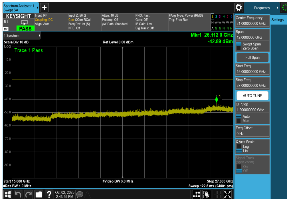
Plot 7-239. Conducted Spurious Plot (ULCA LTE Band 41 – (20+20)MHz QPSK – RB Size 1, RB Offset 0 – Low Channel)
