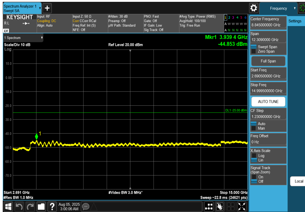
Plot 7-223. Conducted Spurious Plot (NR Band n41 - 100MHz DFT-s-OFDM QPSK – RB Size 1, RB Offset 0 – Mid Channel)
