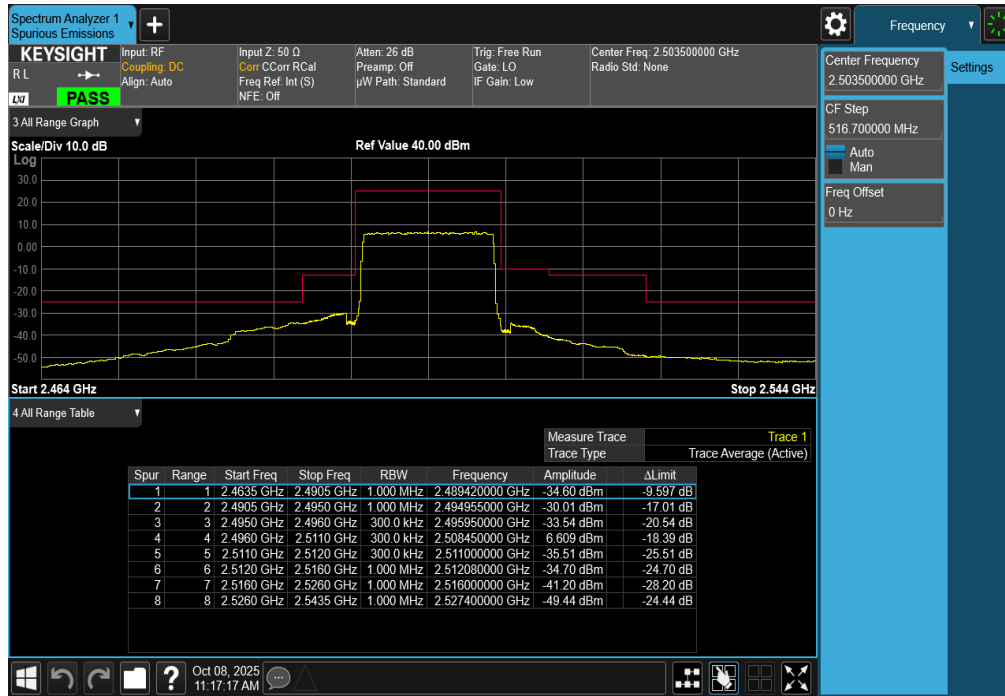
Plot 7-296. Lower ACP Plot (LTE Band 41 - 15MHz QPSK – Full RB)
