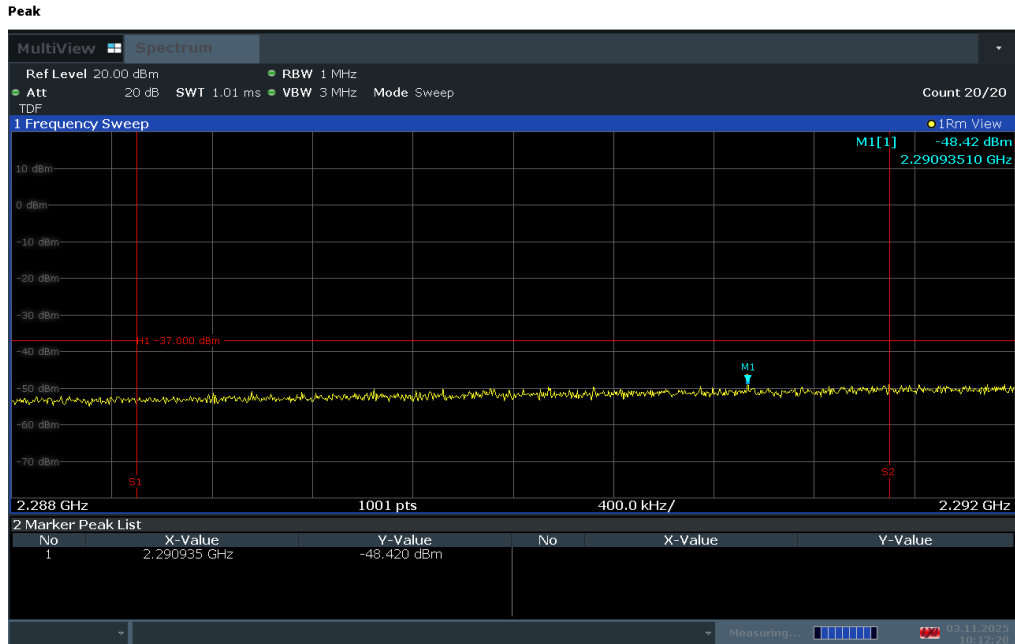
Plot 7-251. Extended Lower Band Edge Plot (LTE Band 30 - 5MHz QPSK – Full RB)
