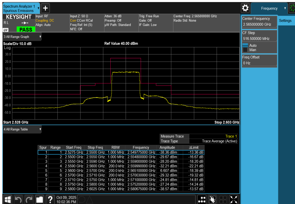
Plot 7-283. Upper ACP Plot (LTE Band 7 - 10MHz QPSK – Full RB)
