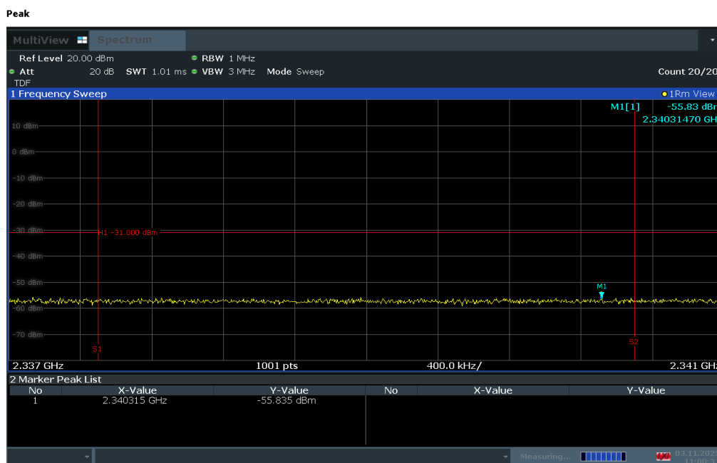
Plot 7-274. Extended Upper Band Edge Plot (LTE Band 30 - 10MHz QPSK – Full RB)
