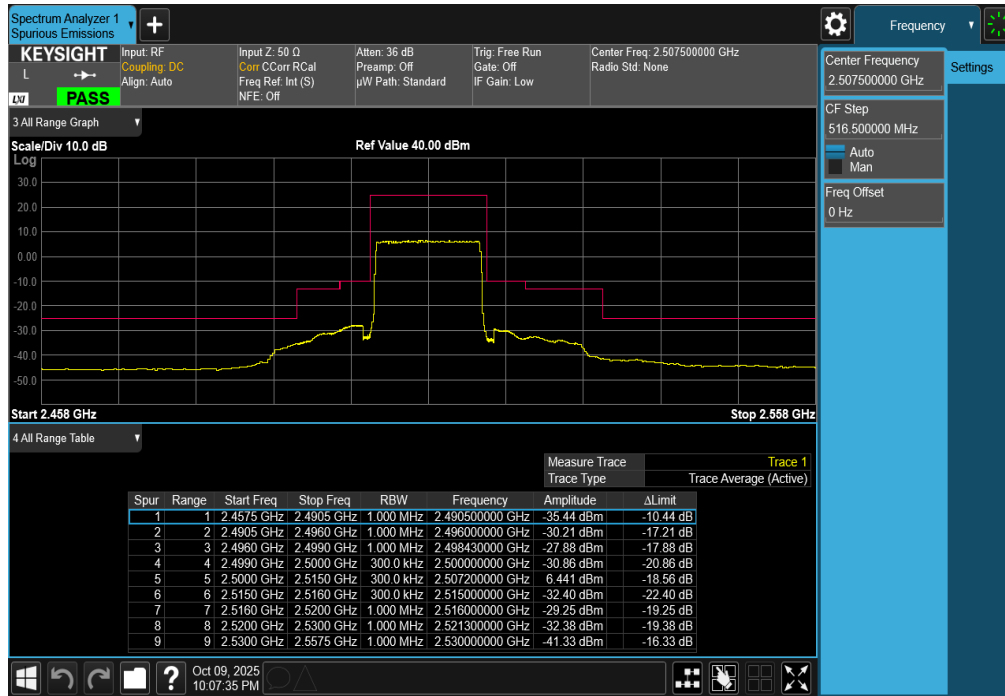
Plot 7-284. Lower ACP Plot (LTE Band 7 - 15MHz QPSK – Full RB)
