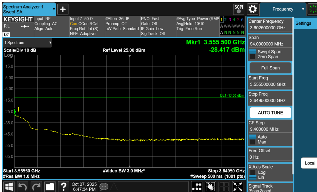
Plot 7-150. Extended Upper Band Edge Plot (NR Band n77 DoD-Band - 15MHz DFT-s-OFDM QPSK – Full RB)
