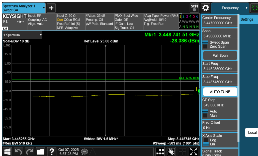
Plot 7-152. Extended Lower Band Edge Plot (NR Band n77 DoD-Band - 20MHz DFT-s-OFDM QPSK – Full RB)
