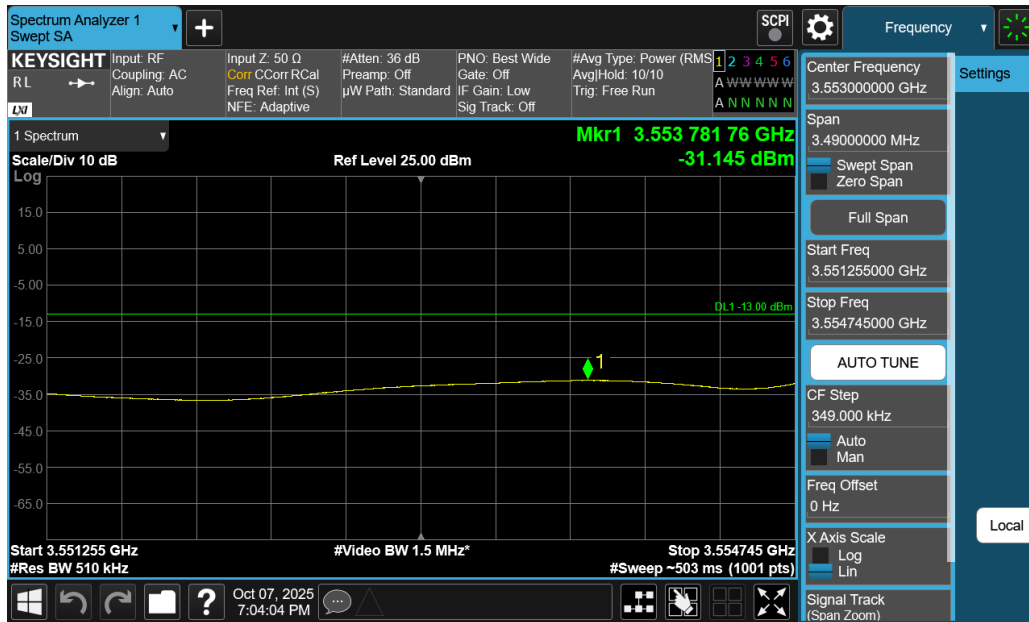
Plot 7-167. Extended Upper Band Edge Plot (NR Band n77 DoD-Band - 30MHz DFT-s-OFDM QPSK – Full RB)
