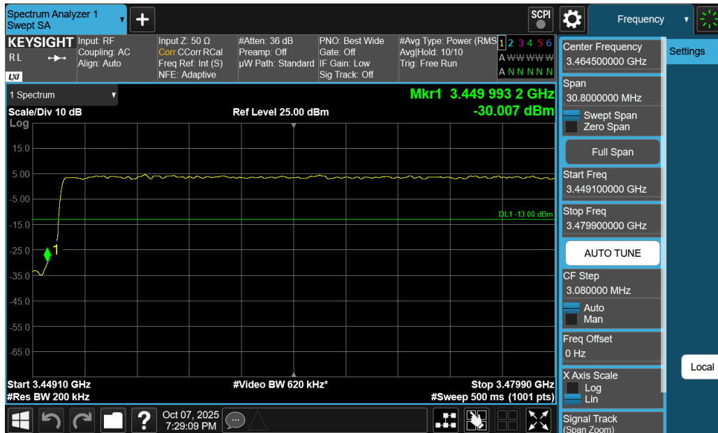
Plot 7-183. Lower Band Edge Plot (NR Band n77 DoD-Band - 60MHz DFT-s-OFDM QPSK – Full RB)
