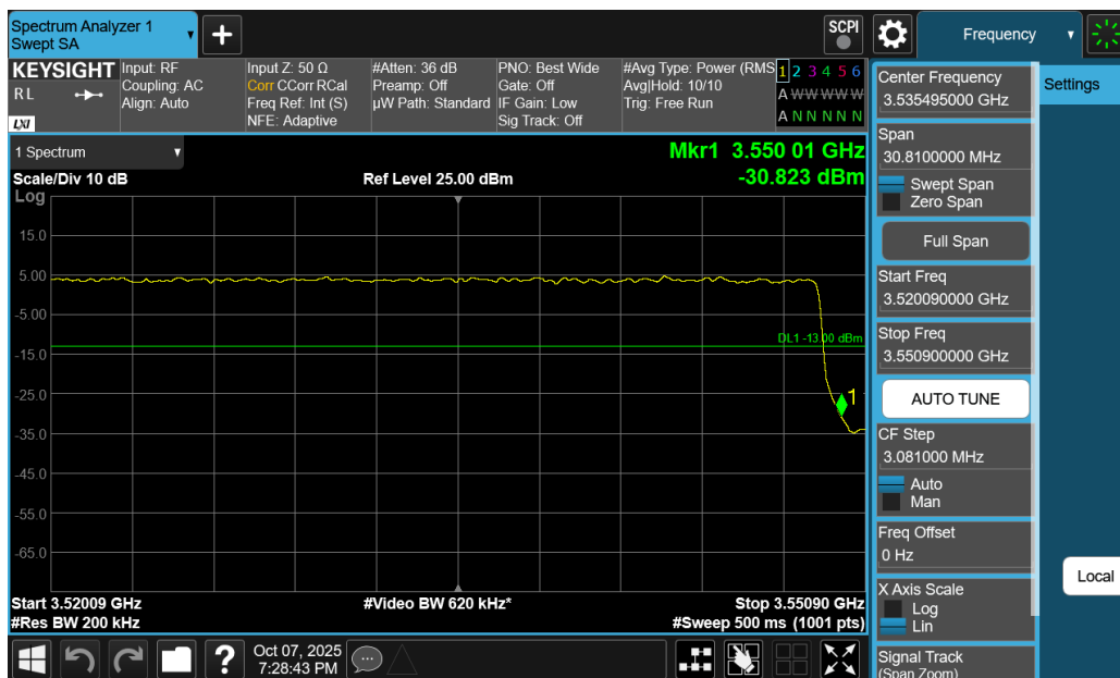
Plot 7-184. Upper Band Edge Plot (NR Band n77 DoD-Band - 60MHz DFT-s-OFDM QPSK – Full RB)
