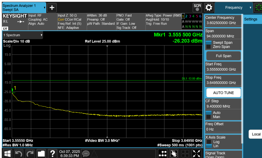
Plot 7-144. Extended Upper Band Edge Plot (NR Band n77 DoD-Band - 10MHz DFT-s-OFDM QPSK – Full RB)
