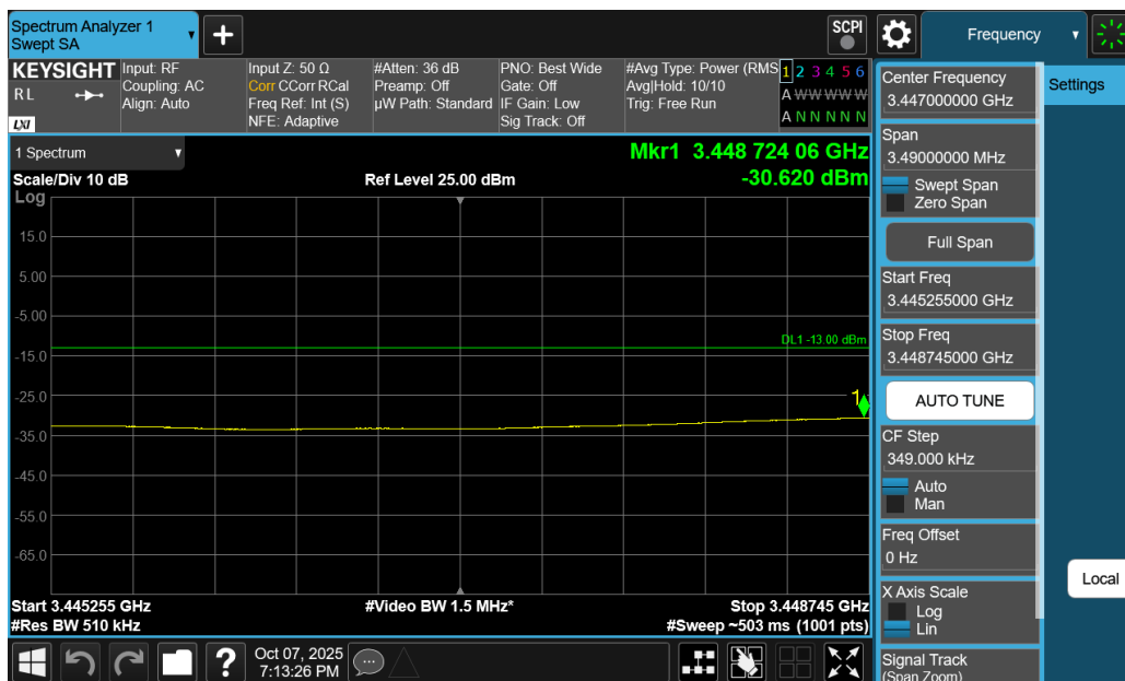
Plot 7-170. Extended Lower Band Edge Plot (NR Band n77 DoD-Band - 40MHz DFT-s-OFDM QPSK – Full RB)
