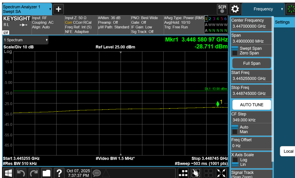
Plot 7-188. Extended Lower Band Edge Plot (NR Band n77 DoD-Band - 70MHz DFT-s-OFDM QPSK – Full RB)
