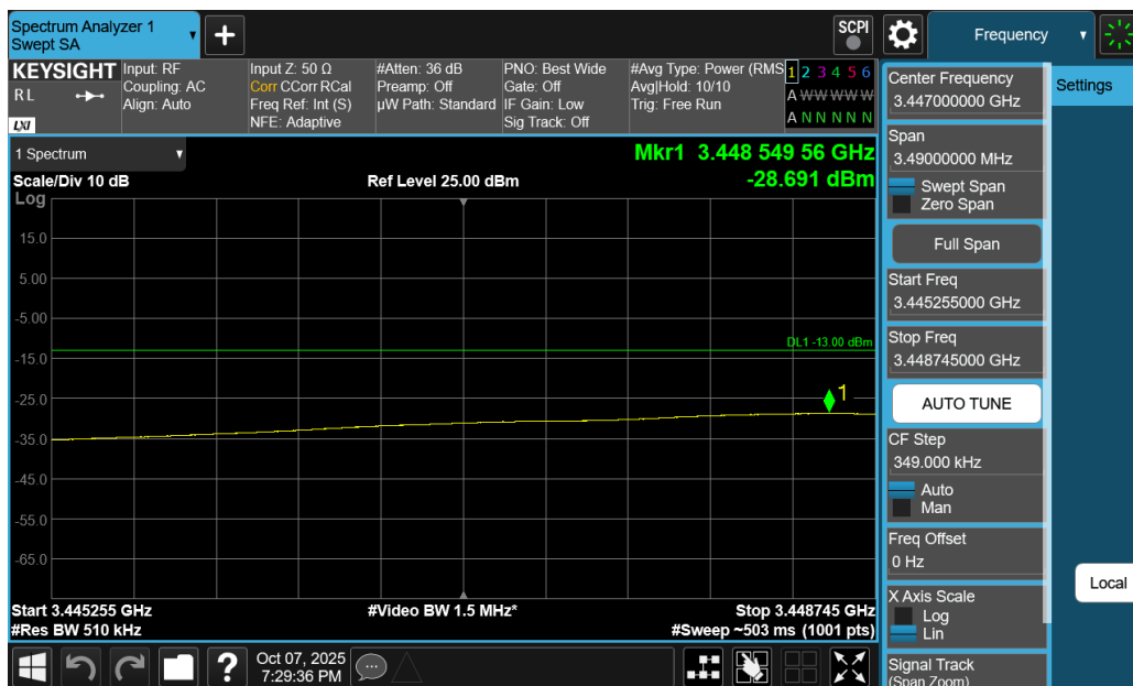
Plot 7-182. Extended Lower Band Edge Plot (NR Band n77 DoD-Band - 60MHz DFT-s-OFDM QPSK – Full RB)
