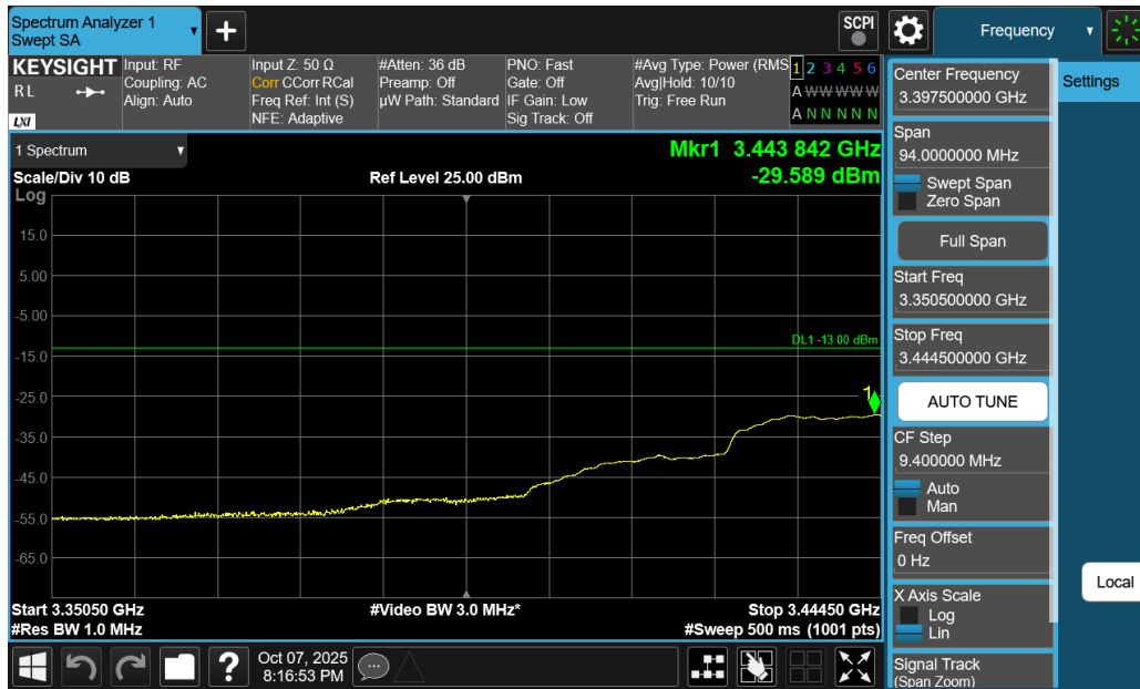
Plot 7-157. Extended Lower Band Edge Plot (NR Band n77 DoD-Band - 25MHz DFT-s-OFDM QPSK – Full RB)
