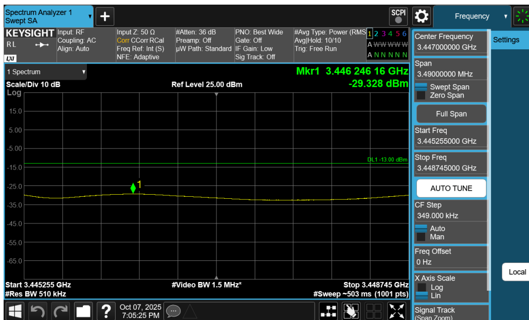
Plot 7-164. Extended Lower Band Edge Plot (NR Band n77 DoD-Band - 30MHz DFT-s-OFDM QPSK – Full RB)
