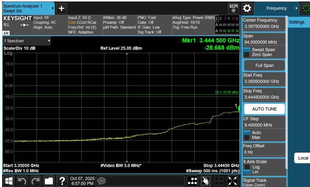
Plot 7-151. Extended Lower Band Edge Plot (NR Band n77 DoD-Band - 20MHz DFT-s-OFDM QPSK – Full RB)
