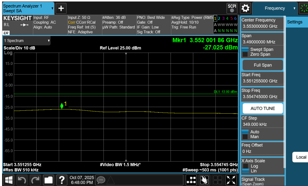
Plot 7-149. Extended Upper Band Edge Plot (NR Band n77 DoD-Band - 15MHz DFT-s-OFDM QPSK – Full RB)
