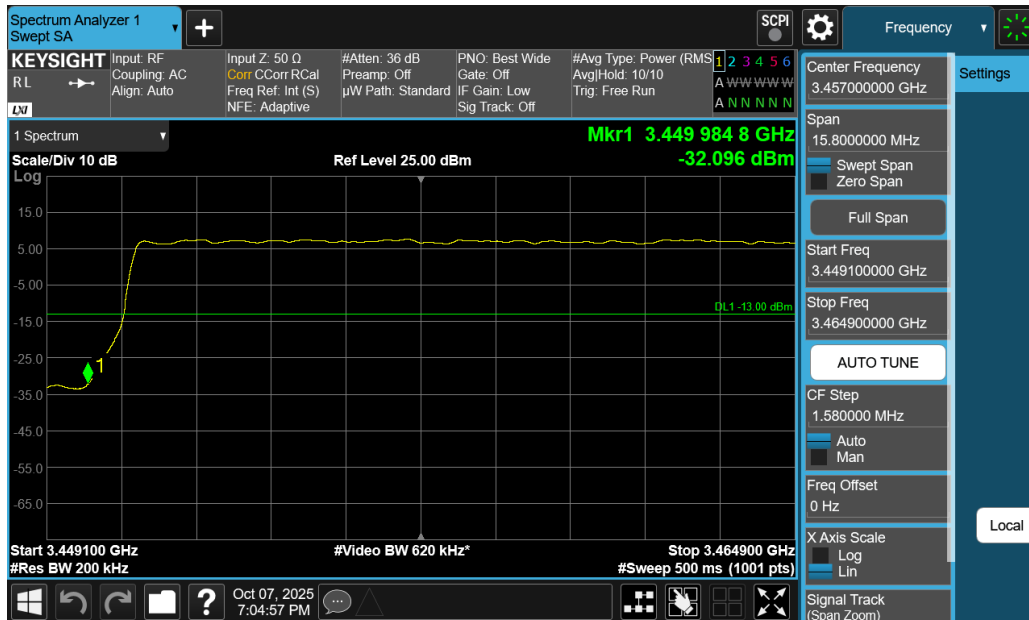
Plot 7-165. Lower Band Edge Plot (NR Band n77 DoD-Band - 30MHz DFT-s-OFDM QPSK – Full RB)
