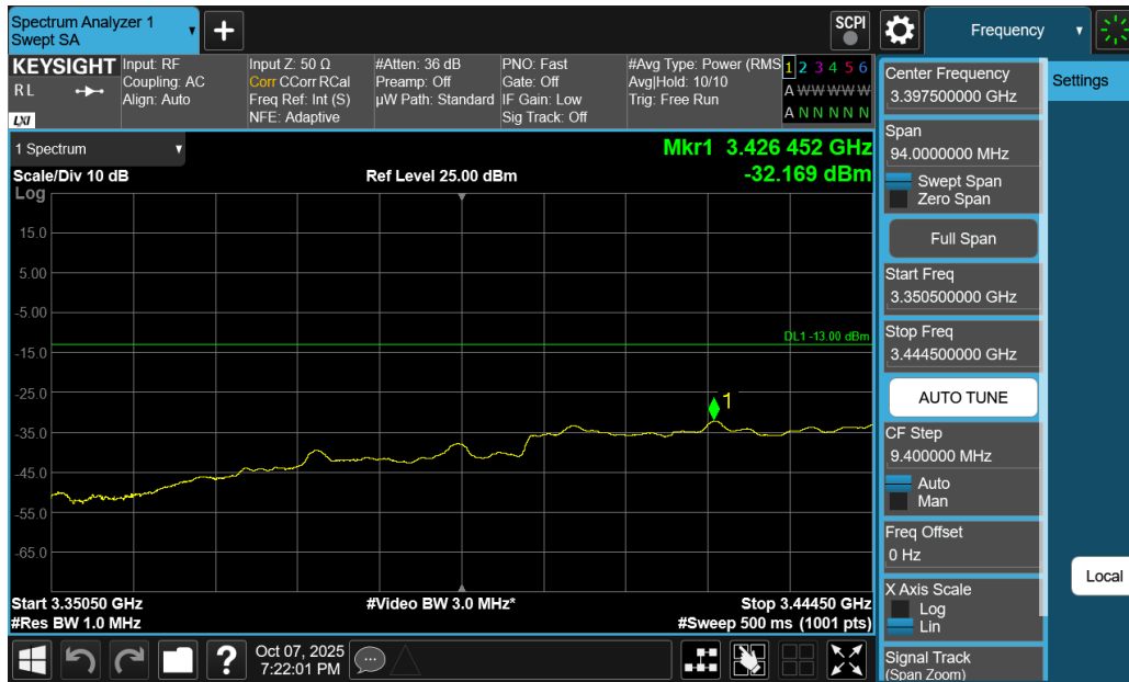
Plot 7-175. Extended Lower Band Edge Plot (NR Band n77 DoD-Band - 50MHz DFT-s-OFDM QPSK – Full RB)
