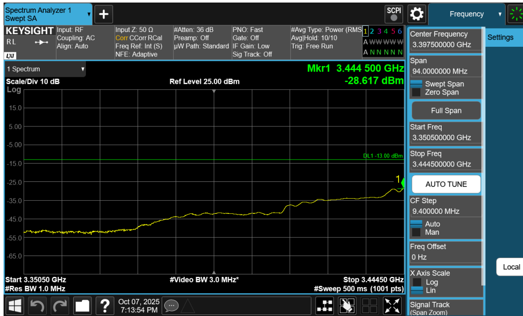
Plot 7-169. Extended Lower Band Edge Plot (NR Band n77 DoD-Band - 40MHz DFT-s-OFDM QPSK – Full RB)
