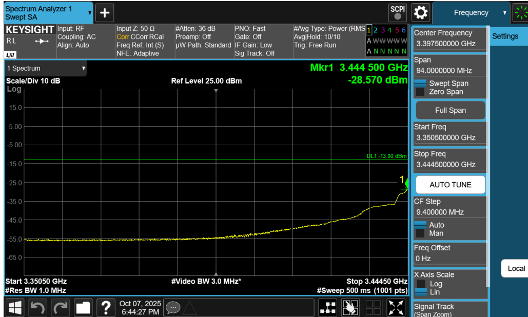
Plot 7-139. Extended Lower Band Edge Plot (NR Band n77 DoD-Band - 10MHz DFT-s-OFDM QPSK – Full RB)
