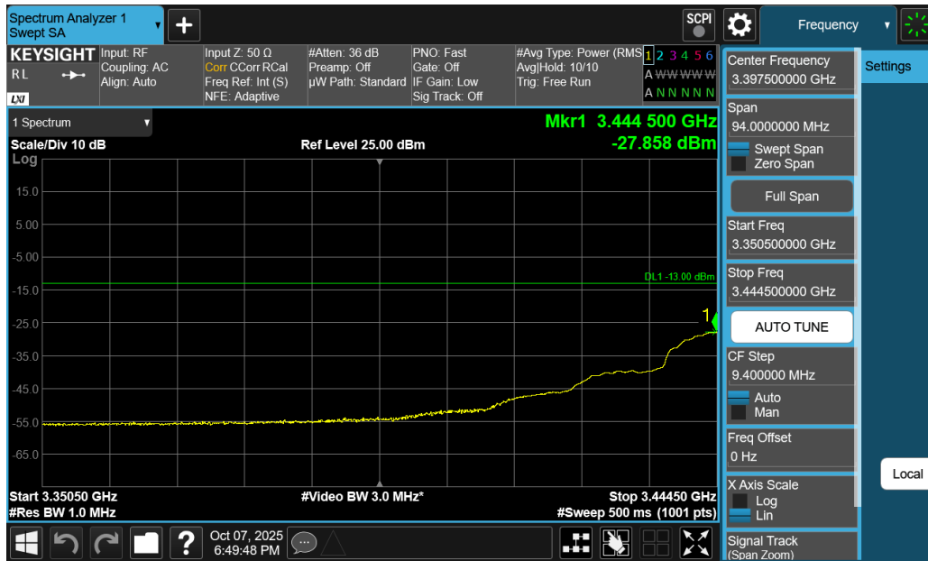
Plot 7-145. Extended Lower Band Edge Plot (NR Band n77 DoD-Band - 15MHz DFT-s-OFDM QPSK – Full RB)
