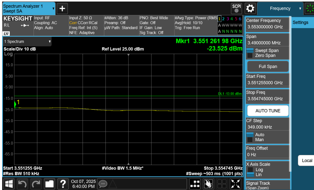
Plot 7-143. Extended Upper Band Edge Plot (NR Band n77 DoD-Band - 10MHz DFT-s-OFDM QPSK – Full RB)
