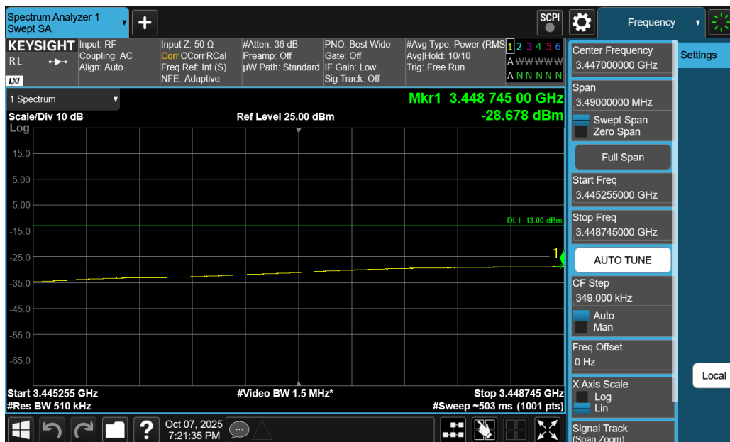
Plot 7-176. Extended Lower Band Edge Plot (NR Band n77 DoD-Band - 50MHz DFT-s-OFDM QPSK – Full RB)
