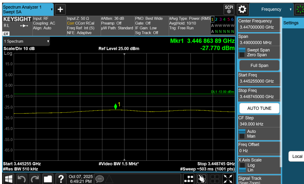
Plot 7-146. Extended Lower Band Edge Plot (NR Band n77 DoD-Band - 15MHz DFT-s-OFDM QPSK – Full RB)
