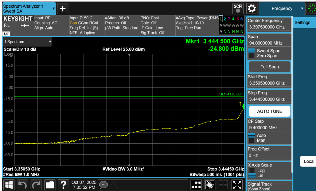
Plot 7-163. Extended Lower Band Edge Plot (NR Band n77 DoD-Band - 30MHz DFT-s-OFDM QPSK – Full RB)
