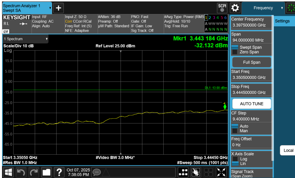
Plot 7-187. Extended Lower Band Edge Plot (NR Band n77 DoD-Band - 70MHz DFT-s-OFDM QPSK – Full RB)
