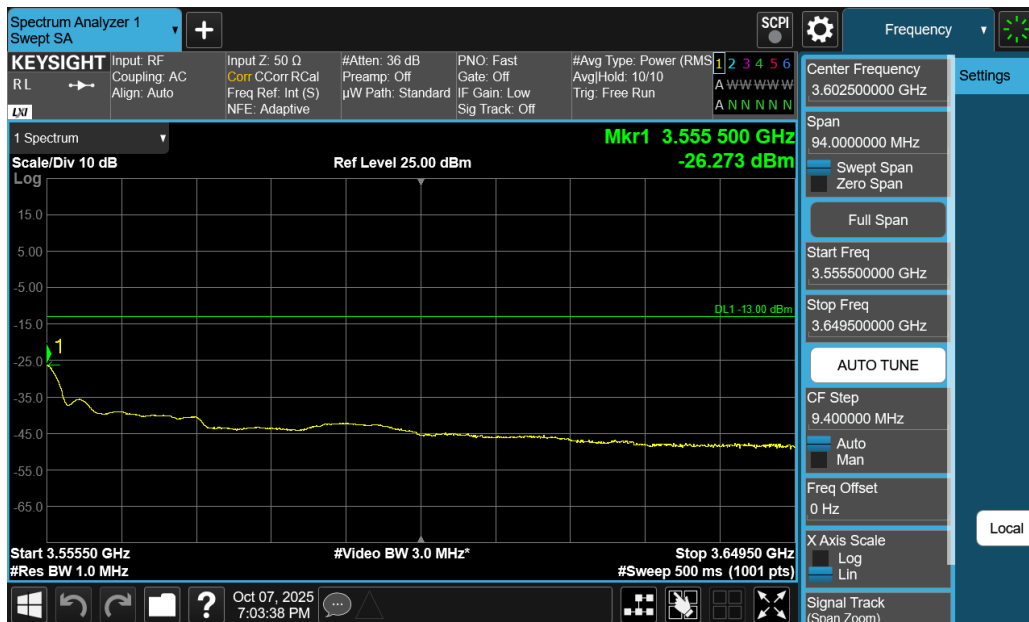
Plot 7-168. Extended Upper Band Edge Plot (NR Band n77 DoD-Band - 30MHz DFT-s-OFDM QPSK – Full RB)
