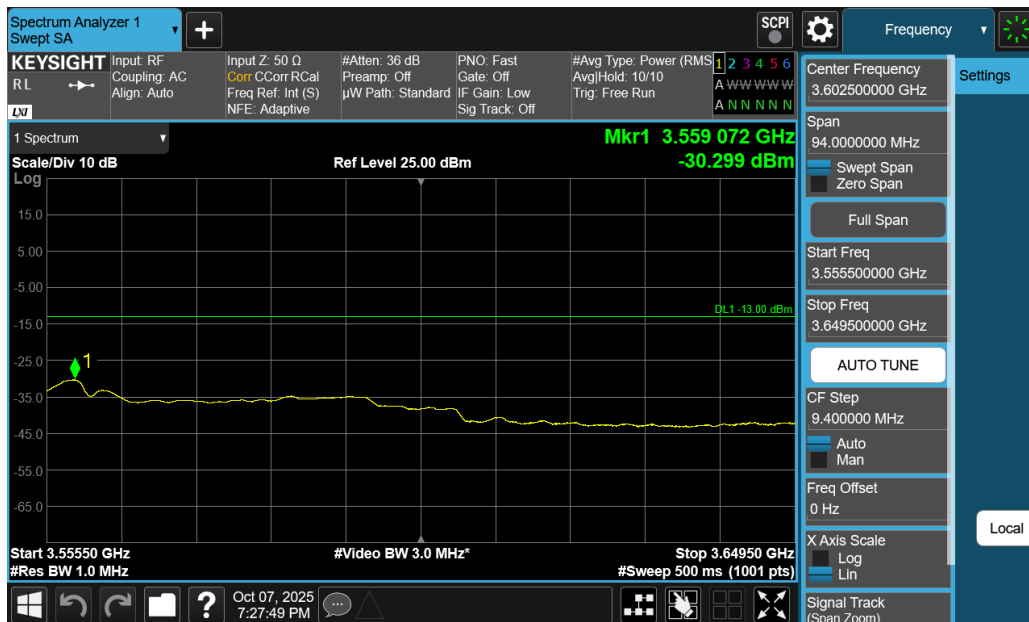
Plot 7-186. Extended Upper Band Edge Plot (NR Band n77 DoD-Band - 60MHz DFT-s-OFDM QPSK – Full RB)
