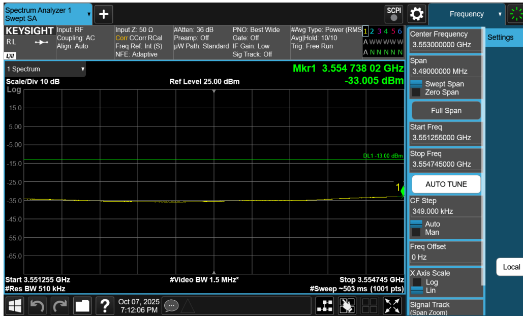
Plot 7-173. Extended Upper Band Edge Plot (NR Band n77 DoD-Band - 40MHz DFT-s-OFDM QPSK – Full RB)
