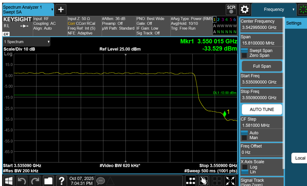
Plot 7-166. Upper Band Edge Plot (NR Band n77 DoD-Band - 30MHz DFT-s-OFDM QPSK – Full RB)
