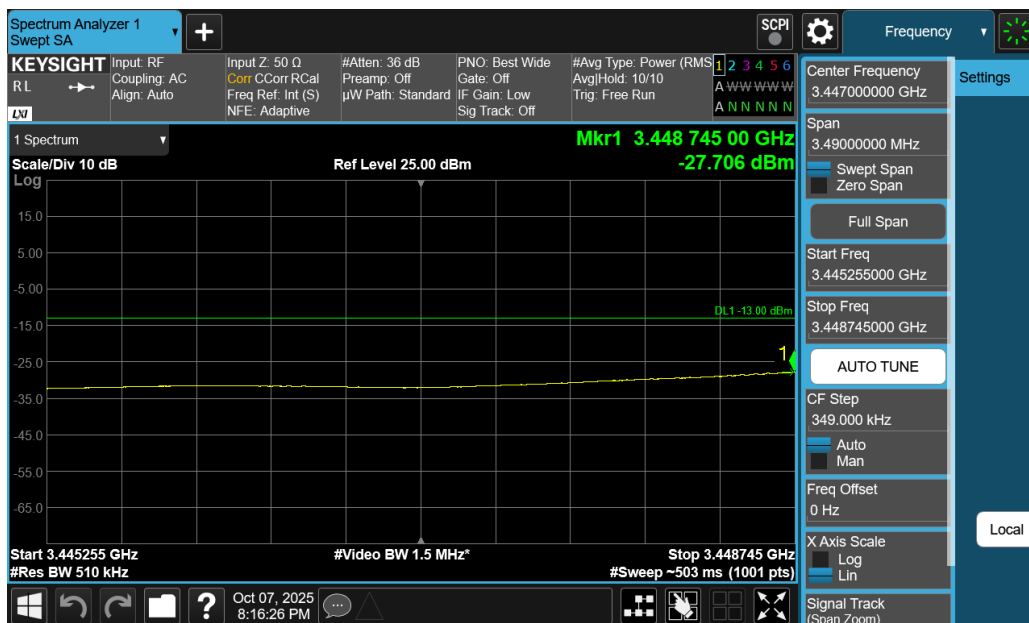
Plot 7-158. Extended Lower Band Edge Plot (NR Band n77 DoD-Band - 25MHz DFT-s-OFDM QPSK – Full RB)
